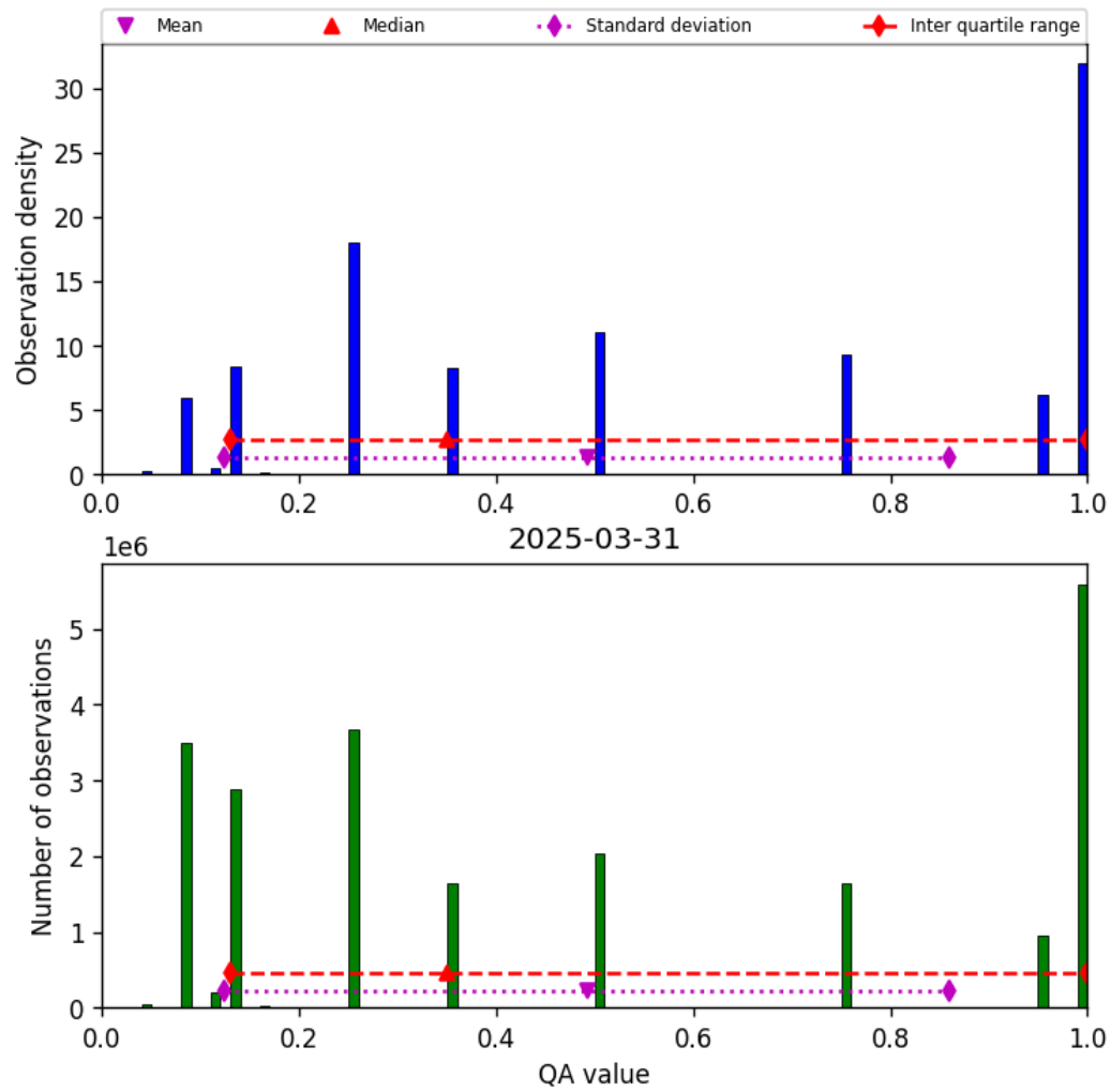
Figure 32: Histogram of “QA value” for 2025-03-31 to 2025-03-31
