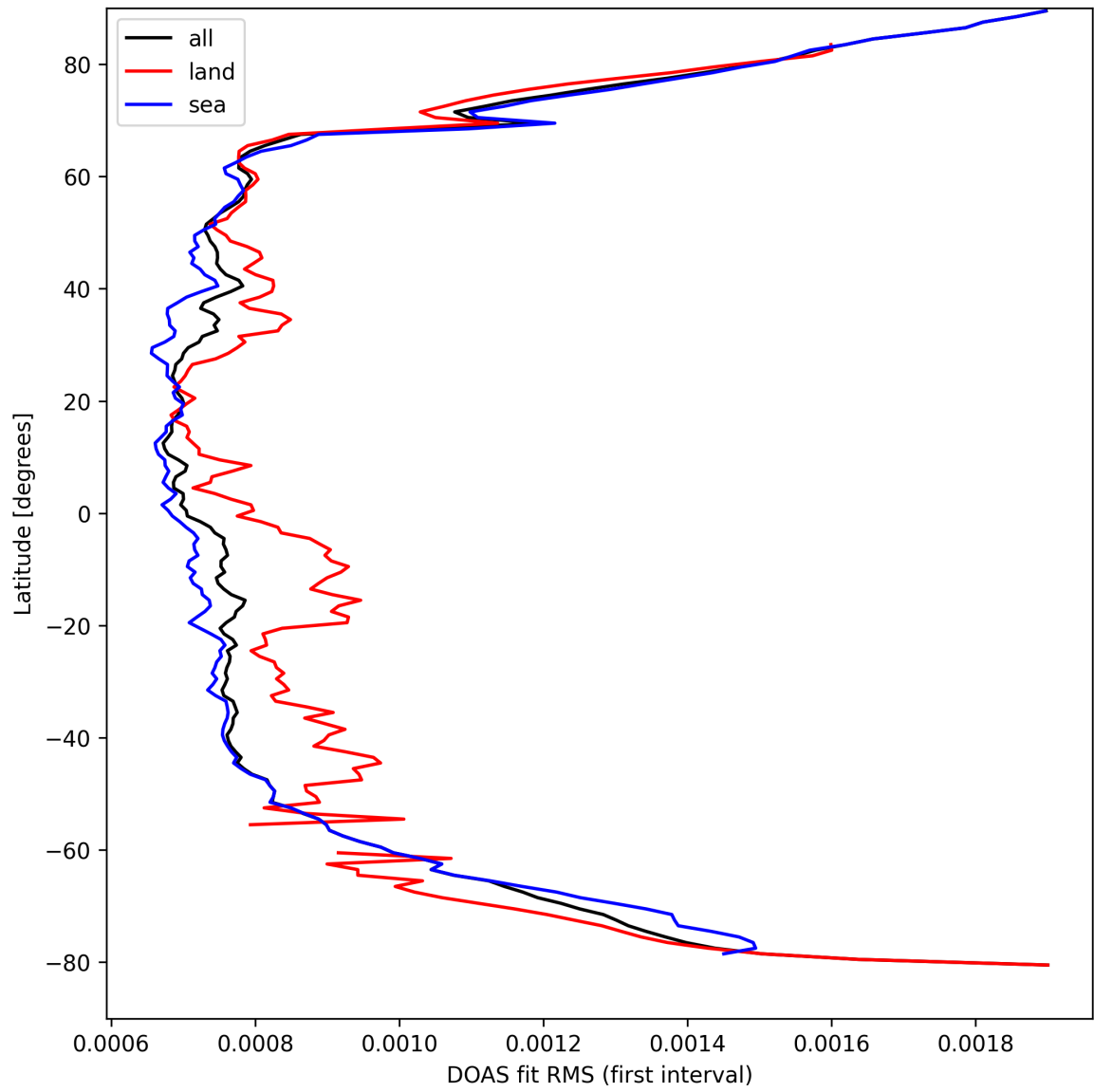
Figure 30: Zonal average of “DOAS fit RMS (first interval)” for 2025-03-31 to 2025-03-31.
