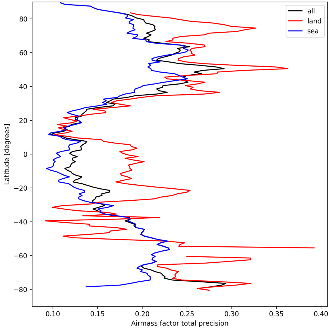
Figure 25: Zonal average of “Airmass factor total precision” for 2025-03-31 to 2025-03-31.
