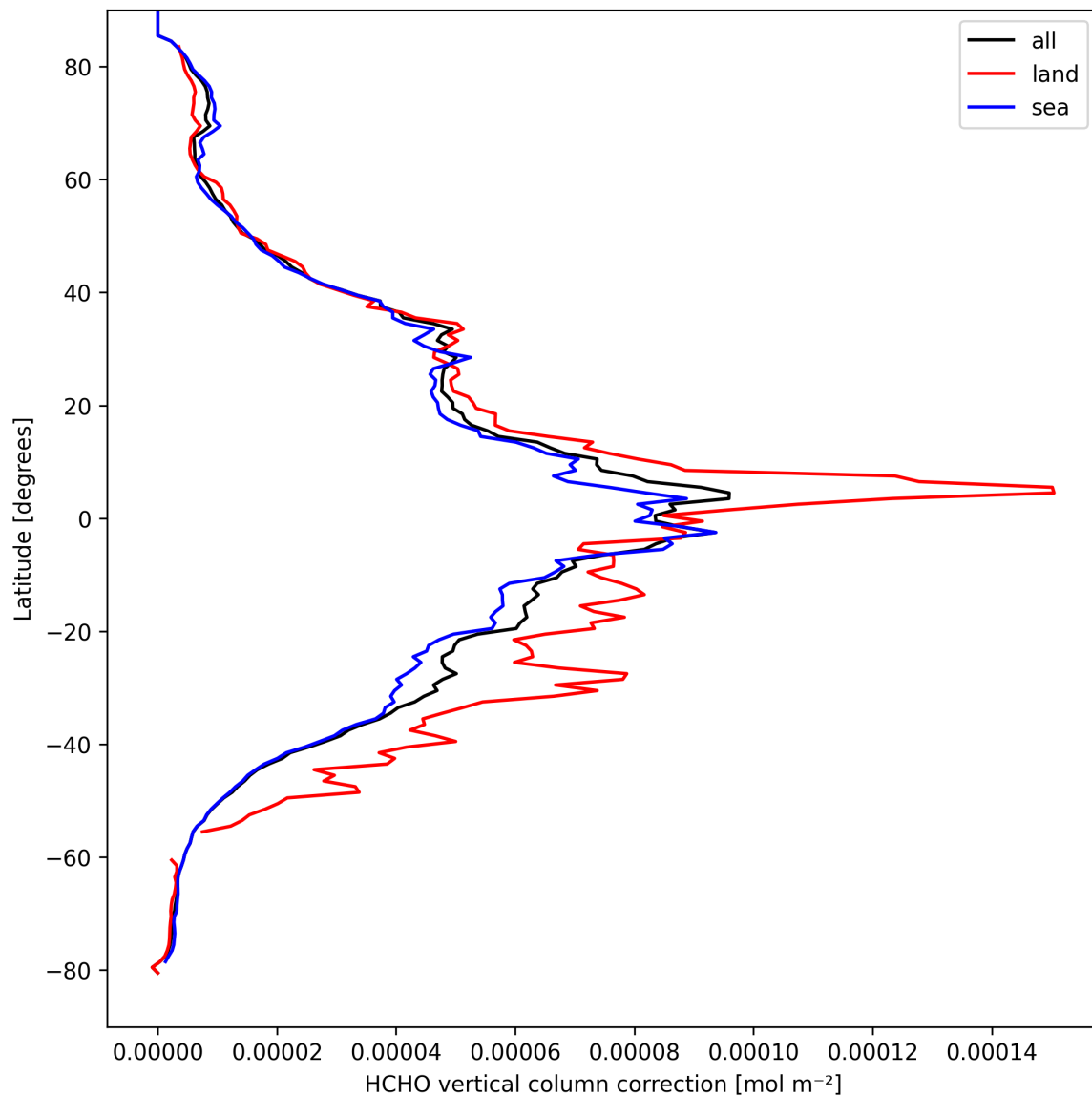
Figure 21: Zonal average of “HCHO vertical column correction” for 2025-03-31 to 2025-03-31.
