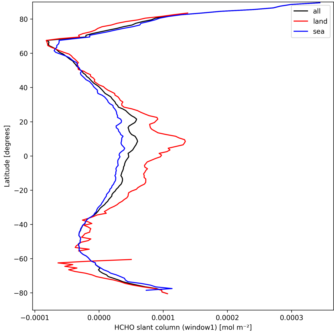
Figure 22: Zonal average of “HCHO slant column (window1)” for 2025-03-31 to 2025-03-31.
