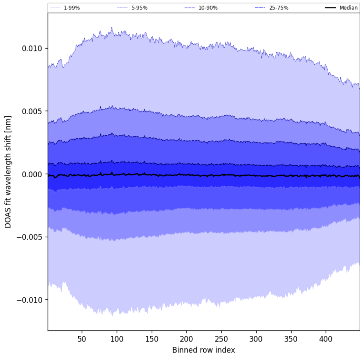
Figure 56: Along track statistics of “DOAS fit wavelength shift” for 2025-03-31 to 2025-03-31
