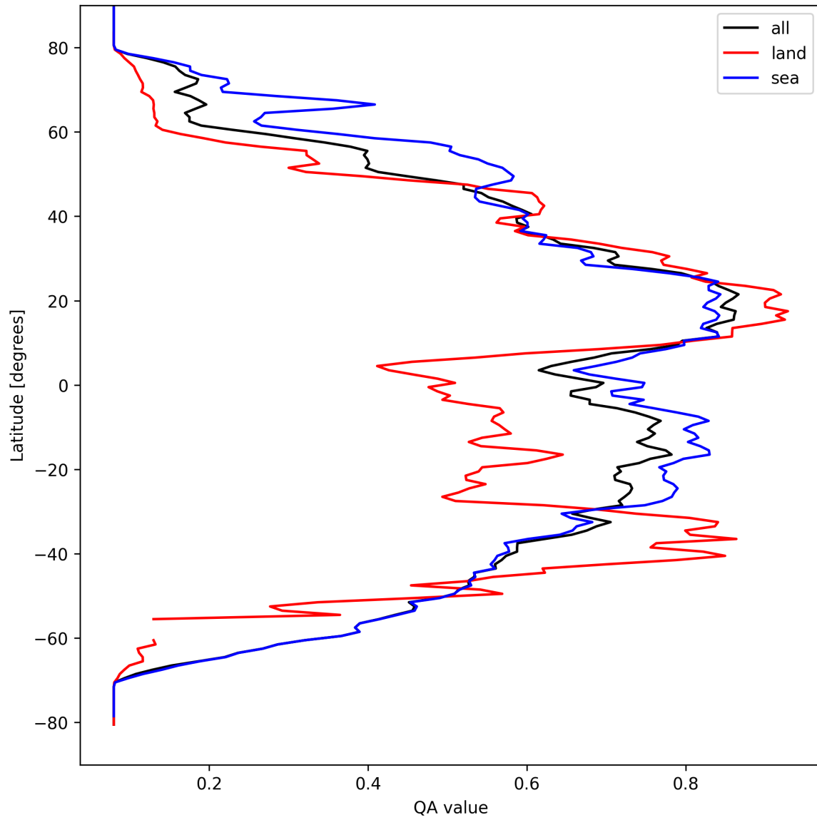
Figure 18: Zonal average of “QA value” for 2025-03-31 to 2025-03-31.
