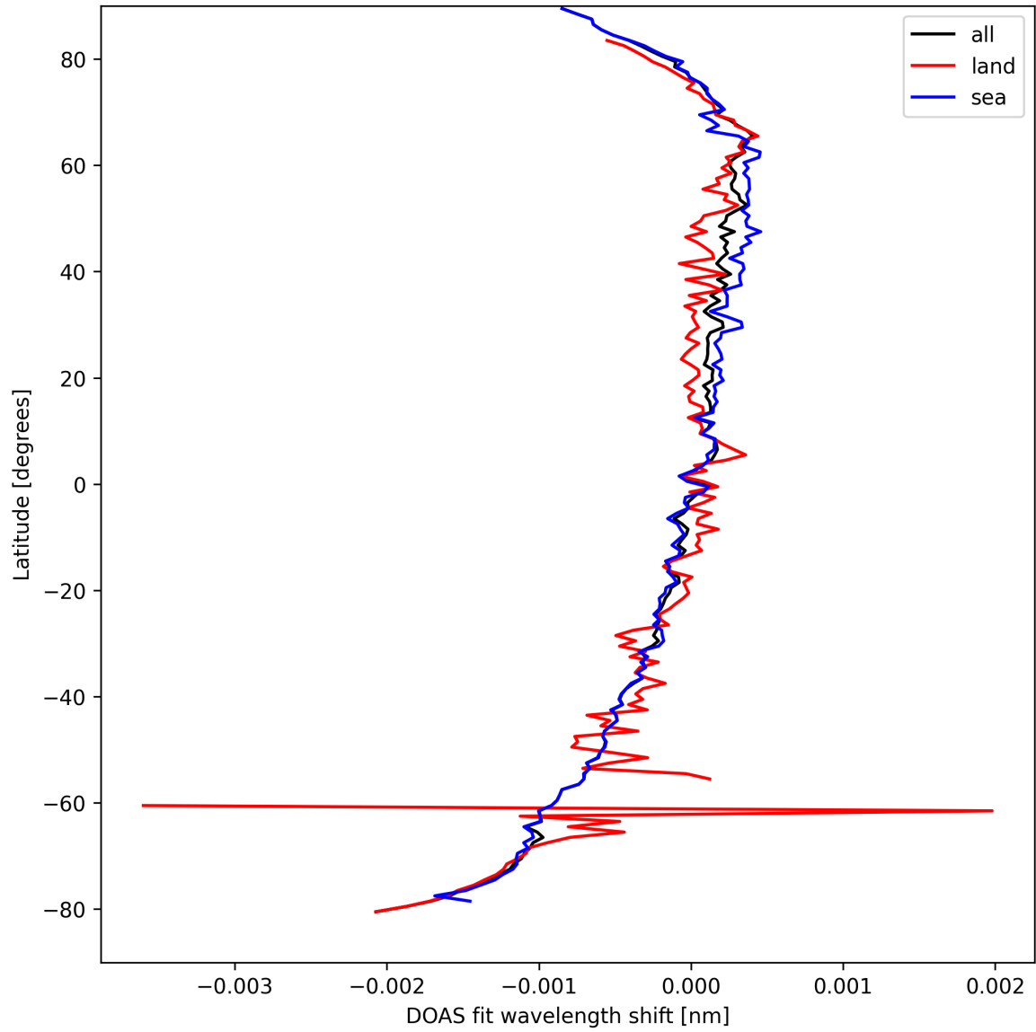
Figure 28: Zonal average of "DOAS fit wavelength shift" for 2025-03-31 to 2025-03-31.
