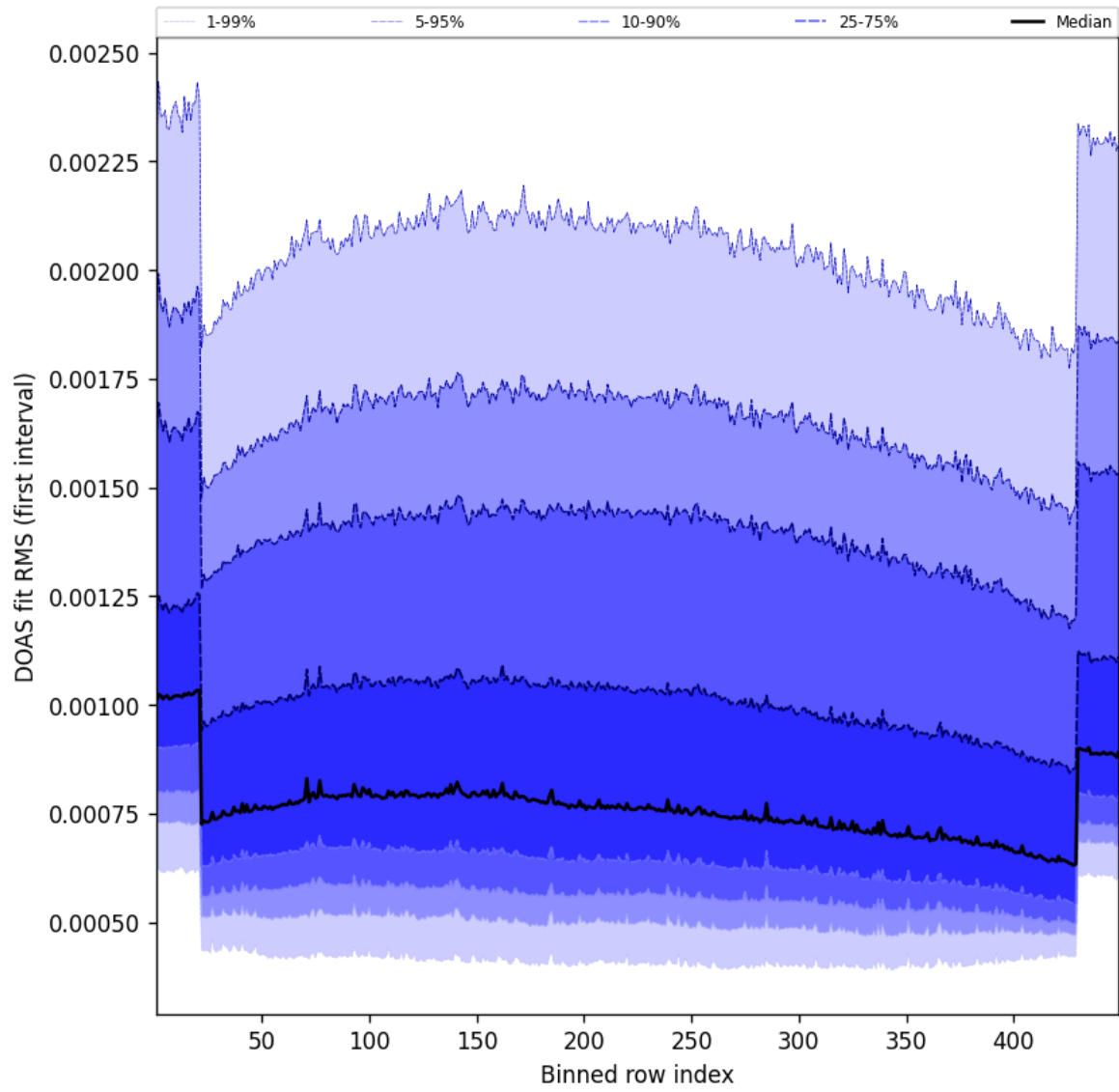
Figure 58: Along track statistics of “DOAS fit RMS (first interval)” for 2025-03-31 to 2025-03-31
