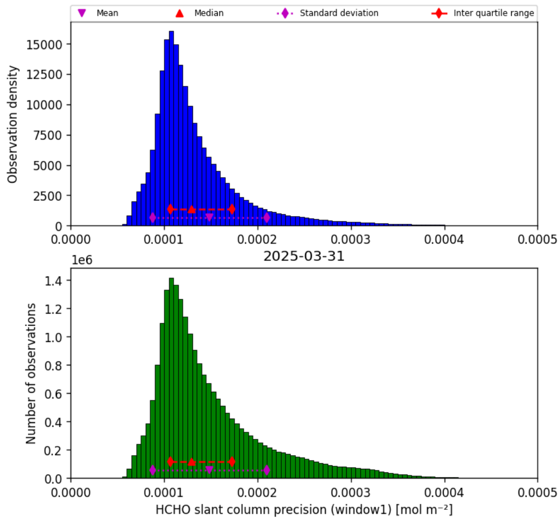
Figure 37: Histogram of “HCHO slant column precision (window1)” for 2025-03-31 to 2025-03-31
