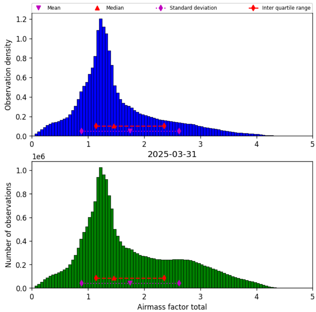
Figure 38: Histogram of “Airmass factor total” for 2025-03-31 to 2025-03-31
