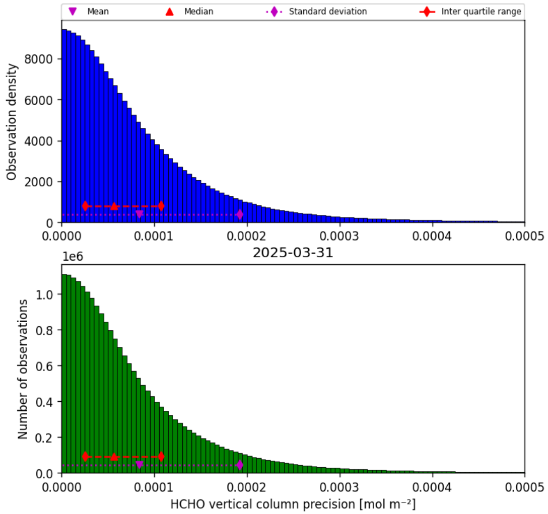
Figure 34: Histogram of “HCHO vertical column precision” for 2025-03-31 to 2025-03-31
