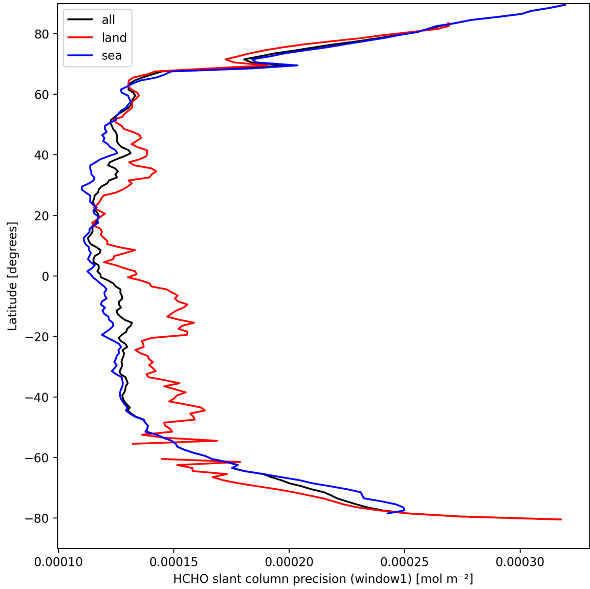
Figure 23: Zonal average of “HCHO slant column precision (window1)” for 2025-03-31 to 2025-03-31.
