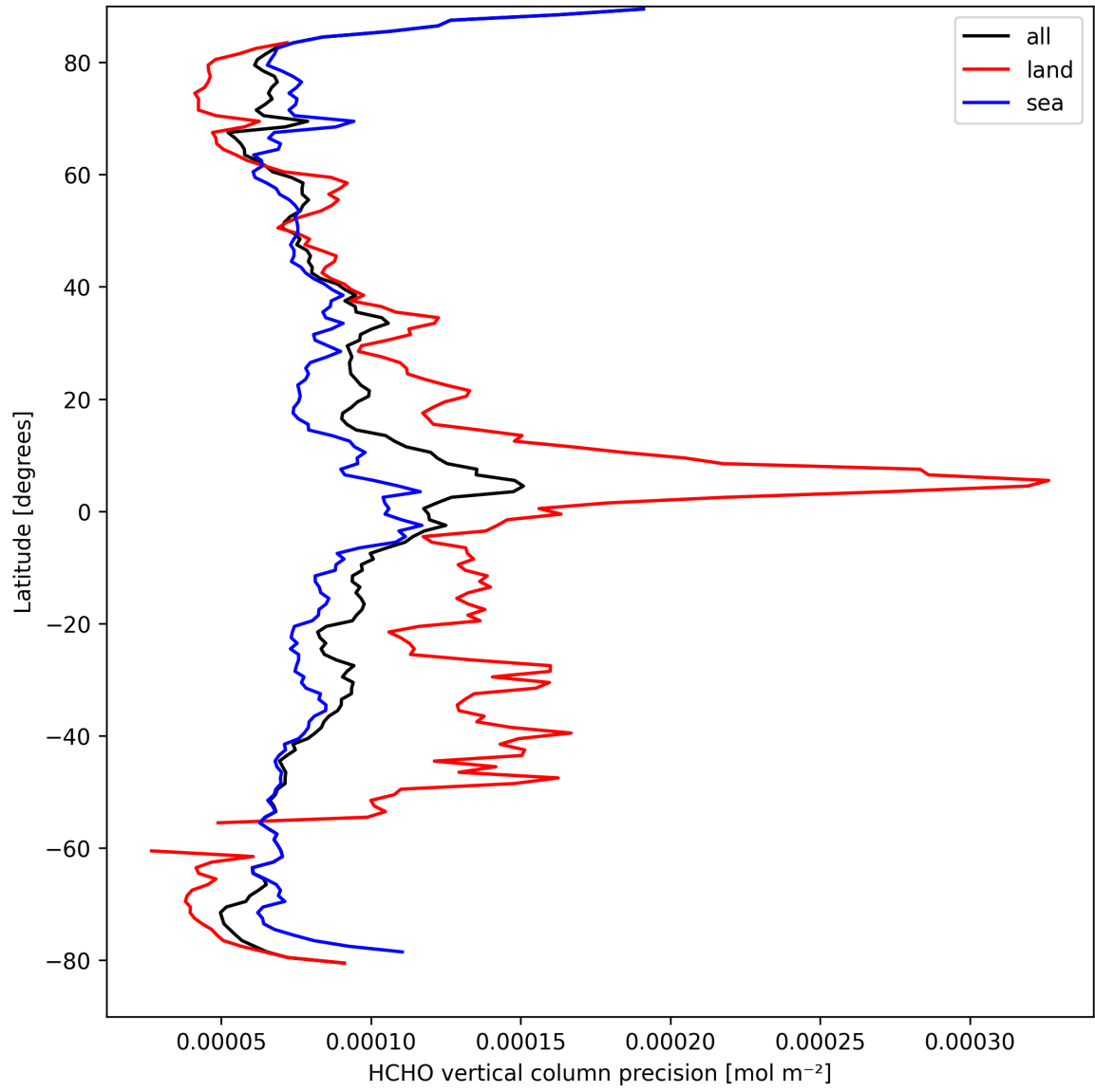
Figure 20: Zonal average of "HCHO vertical column precision" for 2025-03-31 to 2025-03-31.
