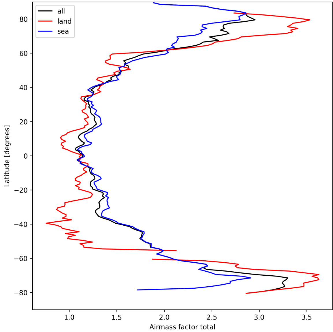
Figure 24: Zonal average of “Airmass factor total” for 2025-03-31 to 2025-03-31.
