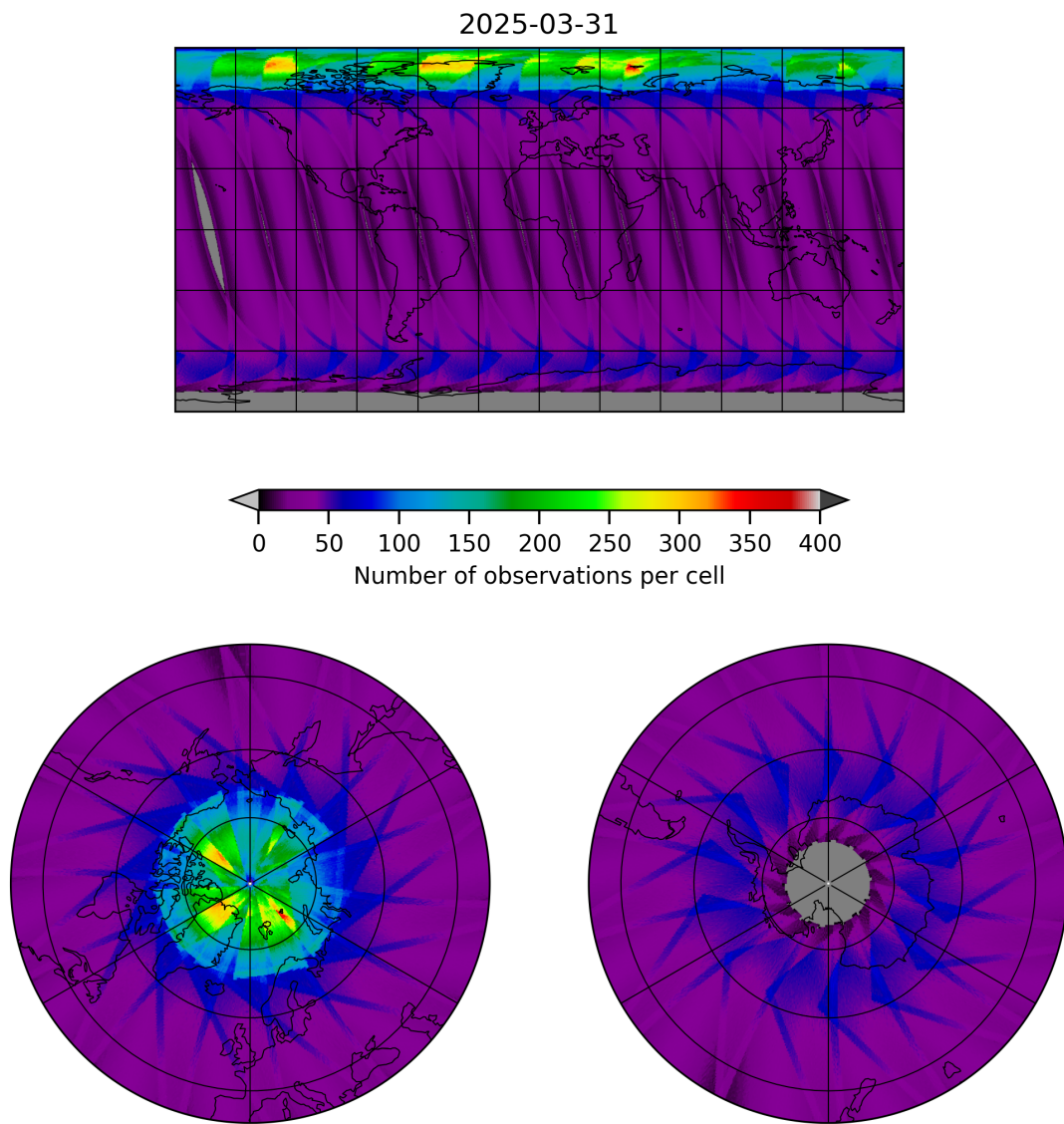
Figure 17: Map of the number of observations for 2025-03-31 to 2025-03-31
