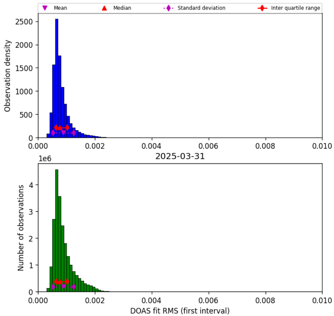
Figure 44: Histogram of “DOAS fit RMS (first interval)” for 2025-03-31 to 2025-03-31
