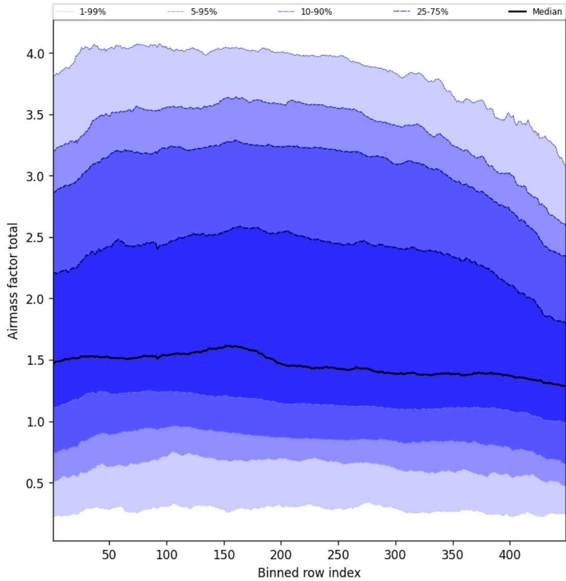
Figure 52: Along track statistics of “Airmass factor total” for 2025-03-31 to 2025-03-31
