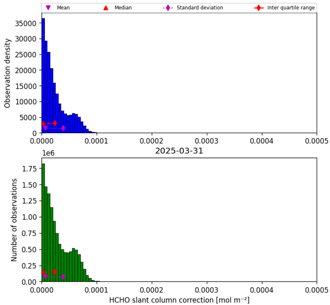
Figure 45: Histogram of “HCHO slant column correction” for 2025-03-31 to 2025-03-31
