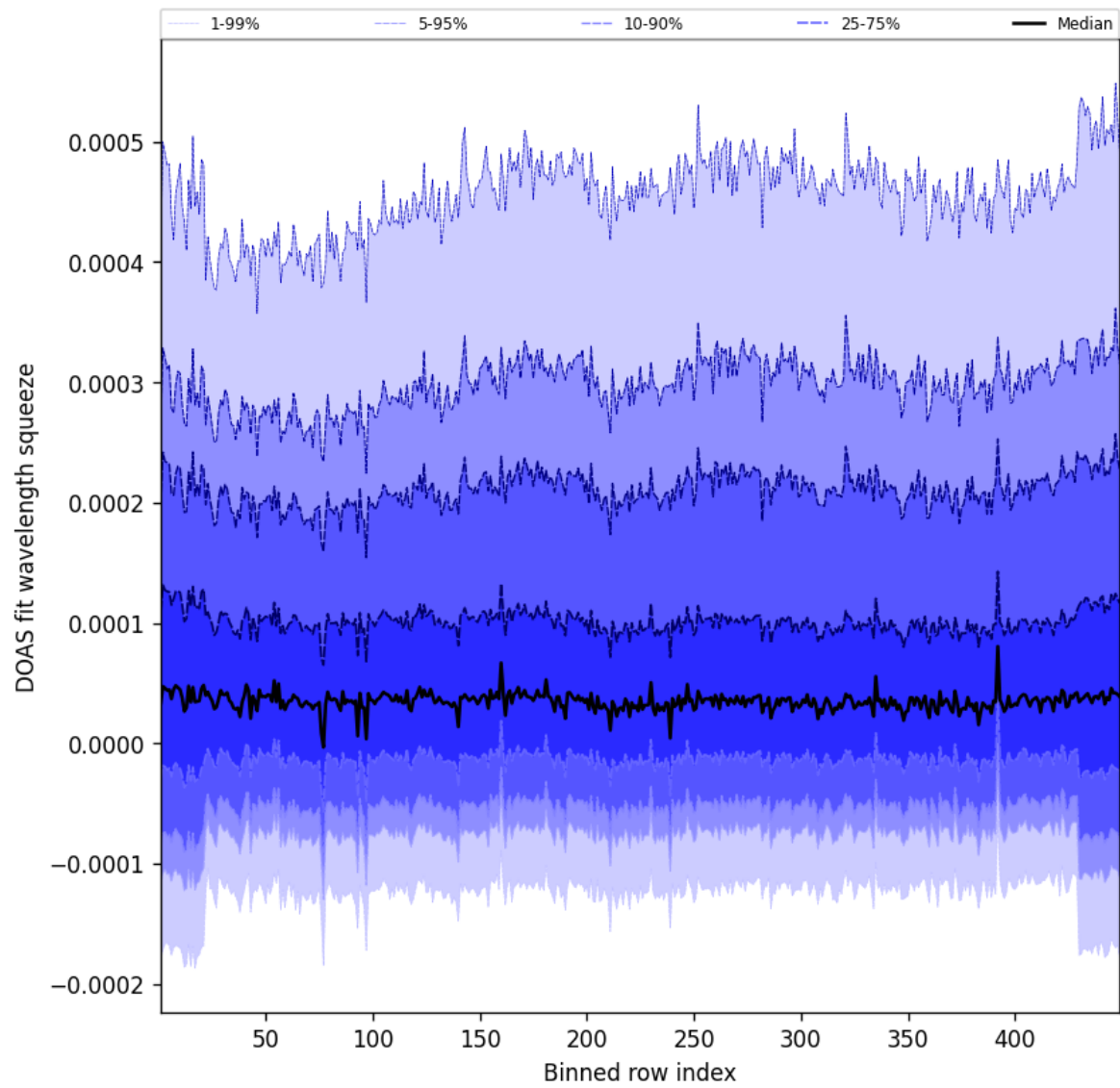
Figure 57: Along track statistics of “DOAS fit wavelength squeeze” for 2025-03-31 to 2025-03-31
