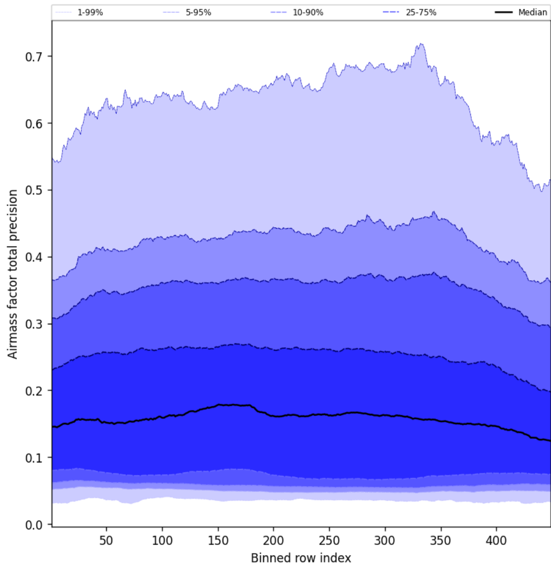
Figure 53: Along track statistics of “Airmass factor total precision” for 2025-03-31 to 2025-03-31
