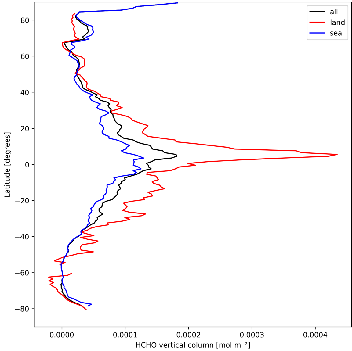
Figure 19: Zonal average of “HCHO vertical column” for 2025-03-31 to 2025-03-31.
