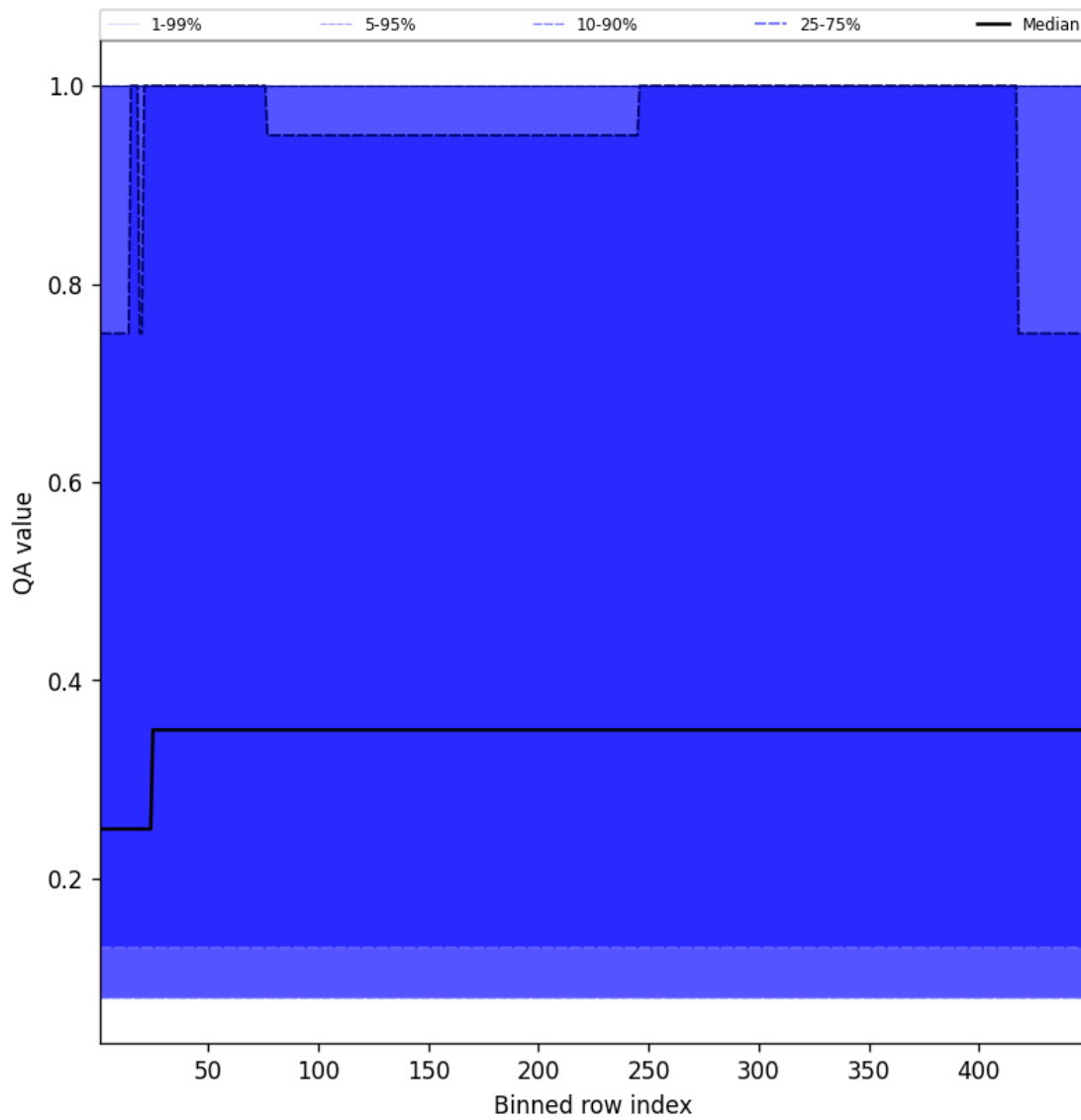
Figure 46: Along track statistics of “QA value” for 2025-03-31 to 2025-03-31
