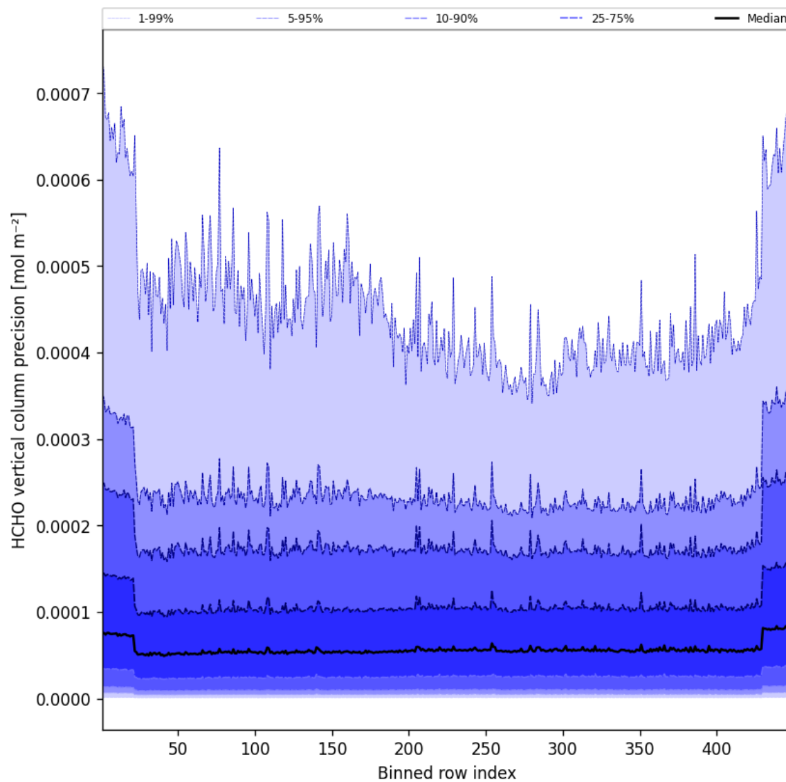
Figure 48: Along track statistics of “HCHO vertical column precision” for 2025-03-31 to 2025-03-31
