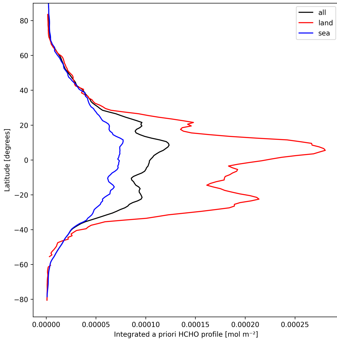
Figure 27: Zonal average of “Integrated a priori HCHO profile” for 2025-03-31 to 2025-03-31.
