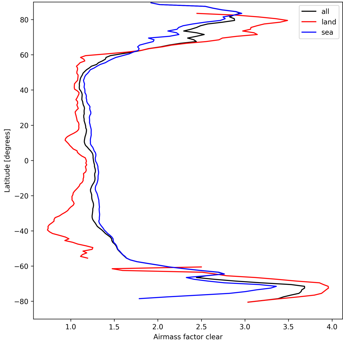
Figure 26: Zonal average of “Airmass factor clear” for 2025-03-31 to 2025-03-31.
