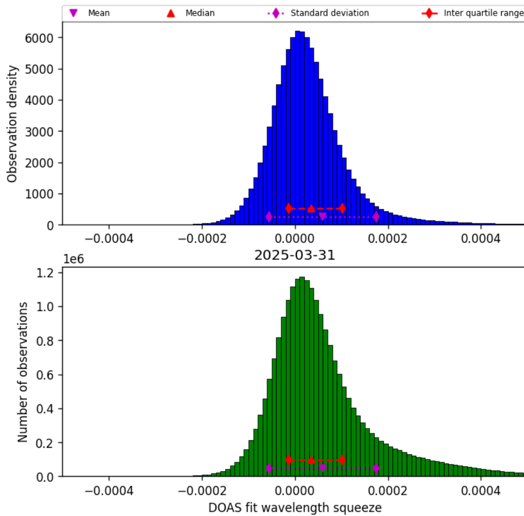
Figure 43: Histogram of “DOAS fit wavelength squeeze” for 2025-03-31 to 2025-03-31
