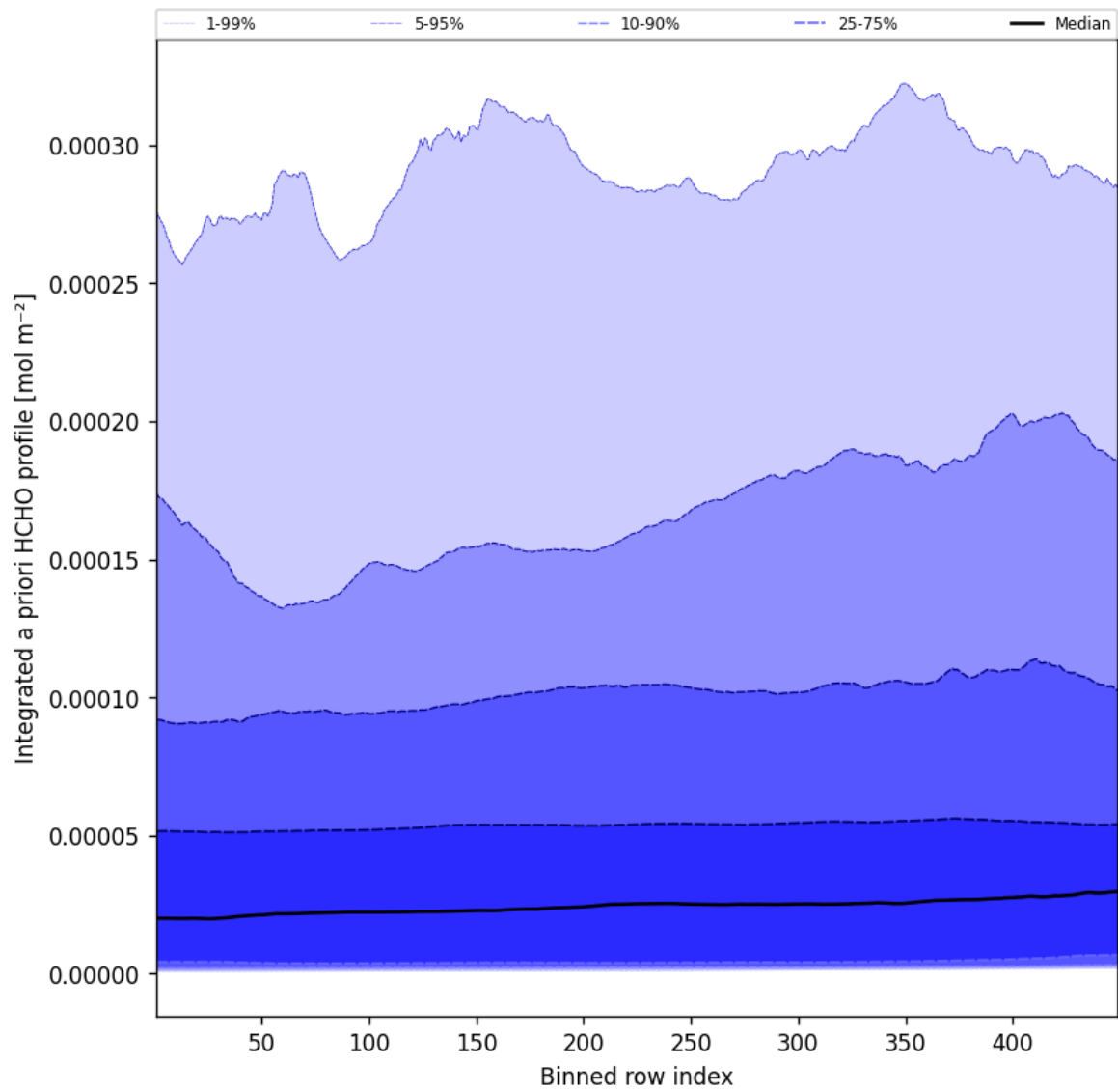
Figure 55: Along track statistics of "Integrated a priori HCHO profile" for 2025-03-31 to 2025-03-31
