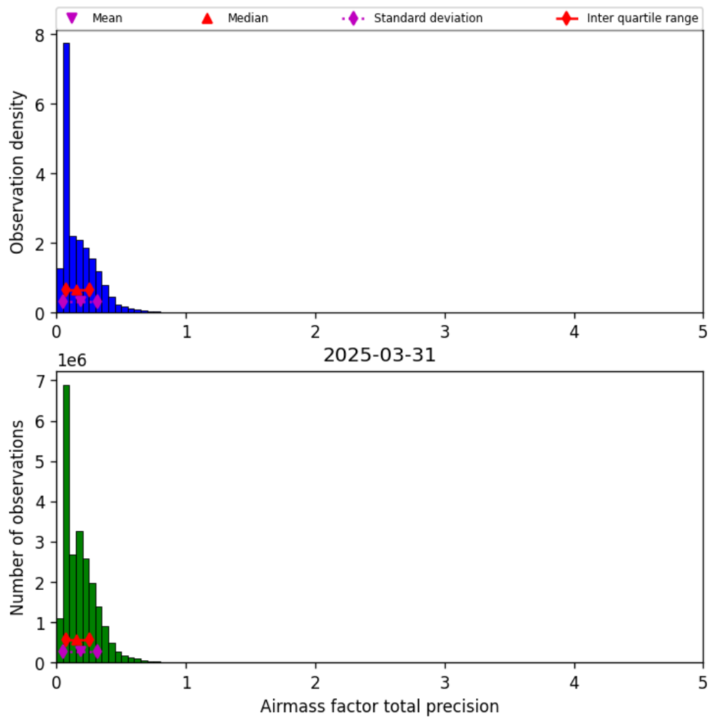
Figure 39: Histogram of “Airmass factor total precision” for 2025-03-31 to 2025-03-31
