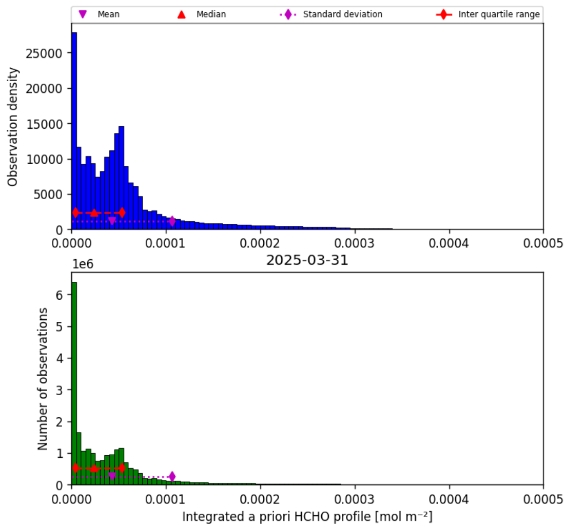
Figure 41: Histogram of “Integrated a priori HCHO profile” for 2025-03-31 to 2025-03-31
