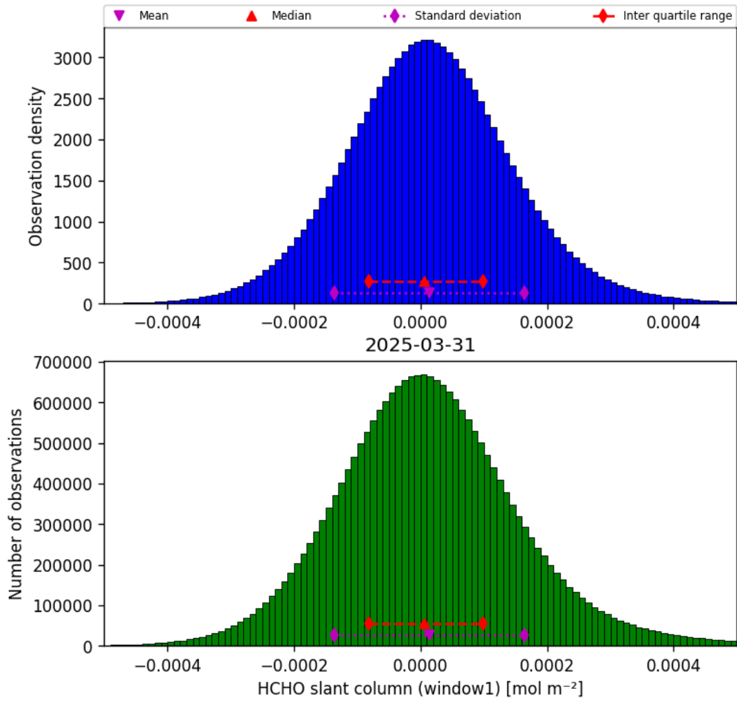
Figure 36: Histogram of “HCHO slant column (window1)” for 2025-03-31 to 2025-03-31
