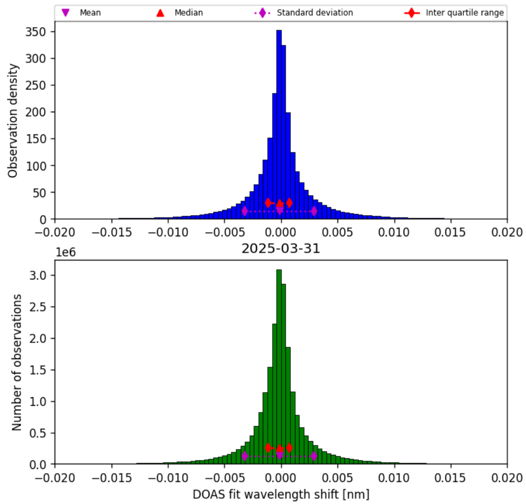
Figure 42: Histogram of “DOAS fit wavelength shift” for 2025-03-31 to 2025-03-31
