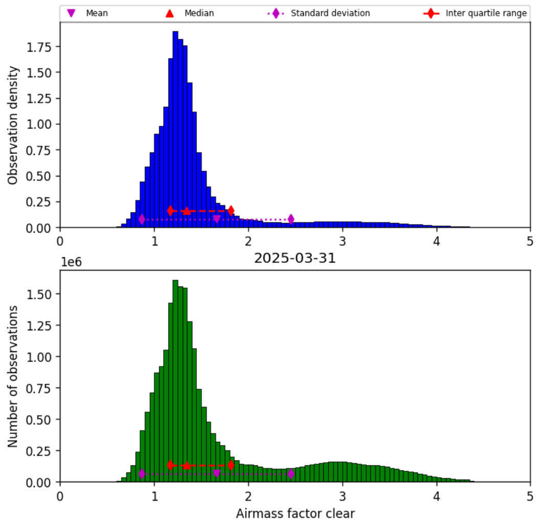
Figure 40: Histogram of “Airmass factor clear” for 2025-03-31 to 2025-03-31
