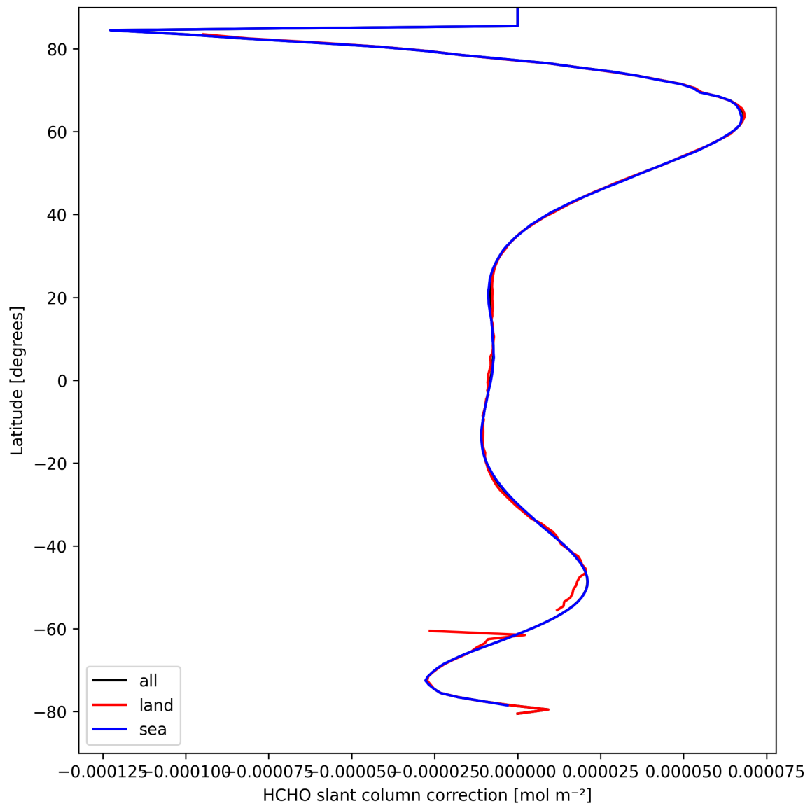
Figure 31: Zonal average of “HCHO slant column correction” for 2025-03-31 to 2025-03-31.
