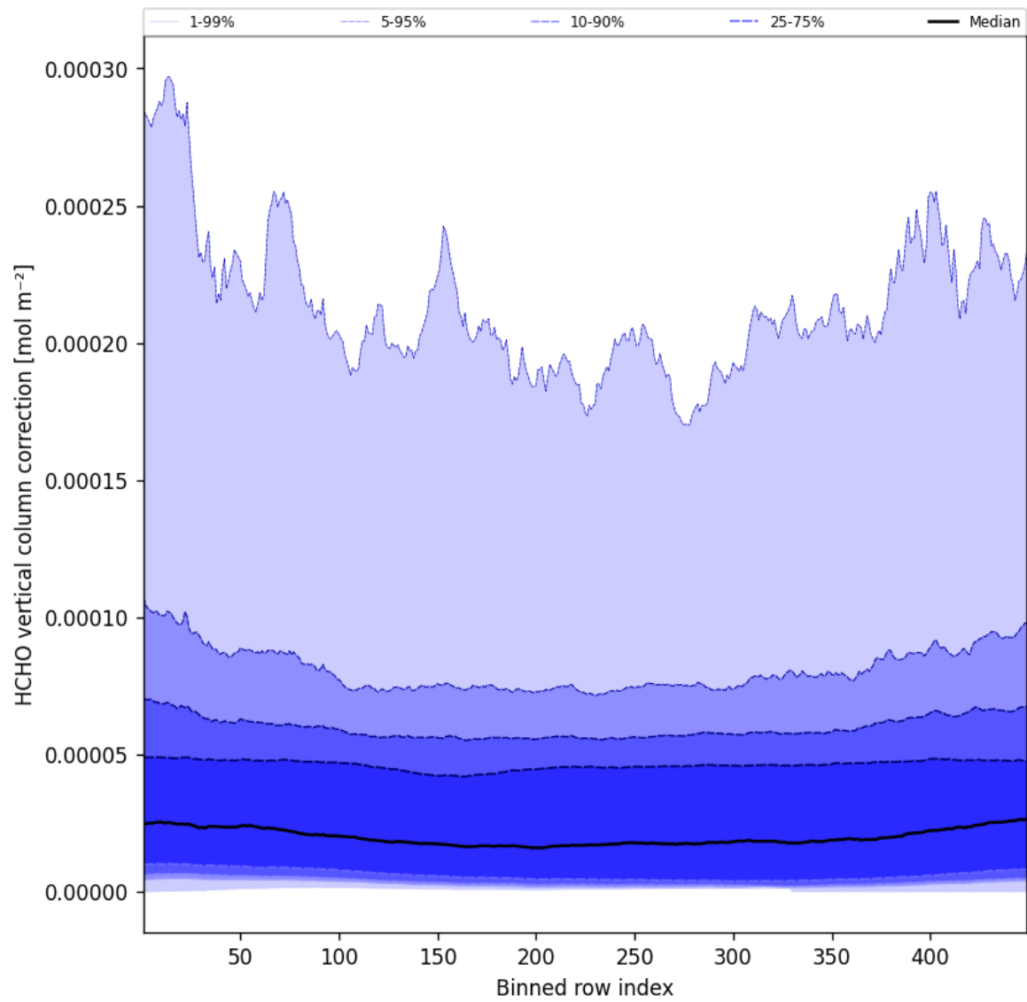
Figure 49: Along track statistics of “HCHO vertical column correction” for 2025-03-31 to 2025-03-31
