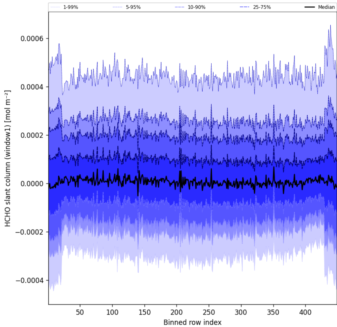
Figure 50: Along track statistics of “HCHO slant column (window1)” for 2025-03-31 to 2025-03-31
