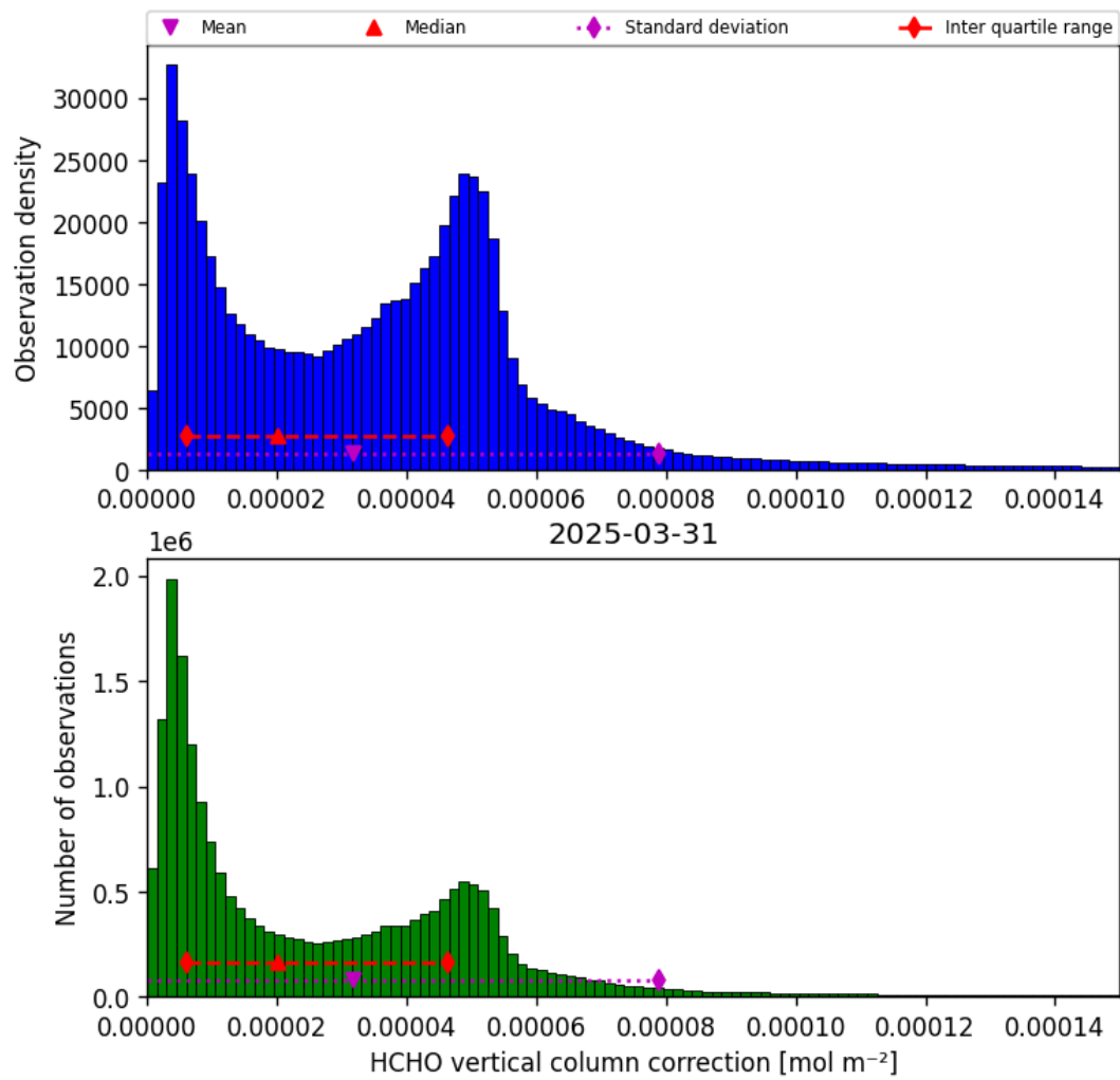
Figure 35: Histogram of “HCHO vertical column correction” for 2025-03-31 to 2025-03-31
