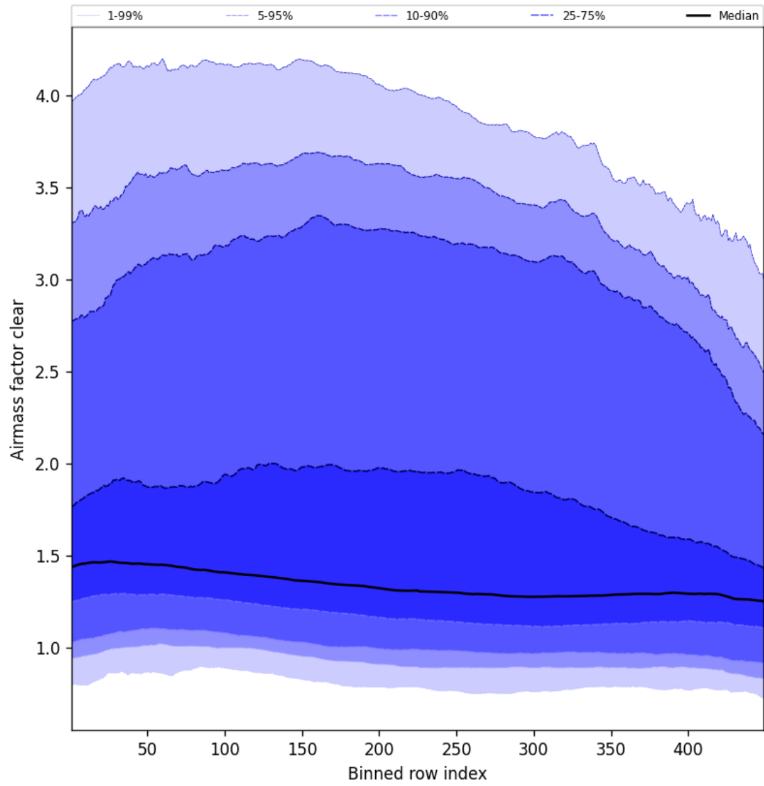
Figure 54: Along track statistics of “Airmass factor clear” for 2025-03-31 to 2025-03-31
