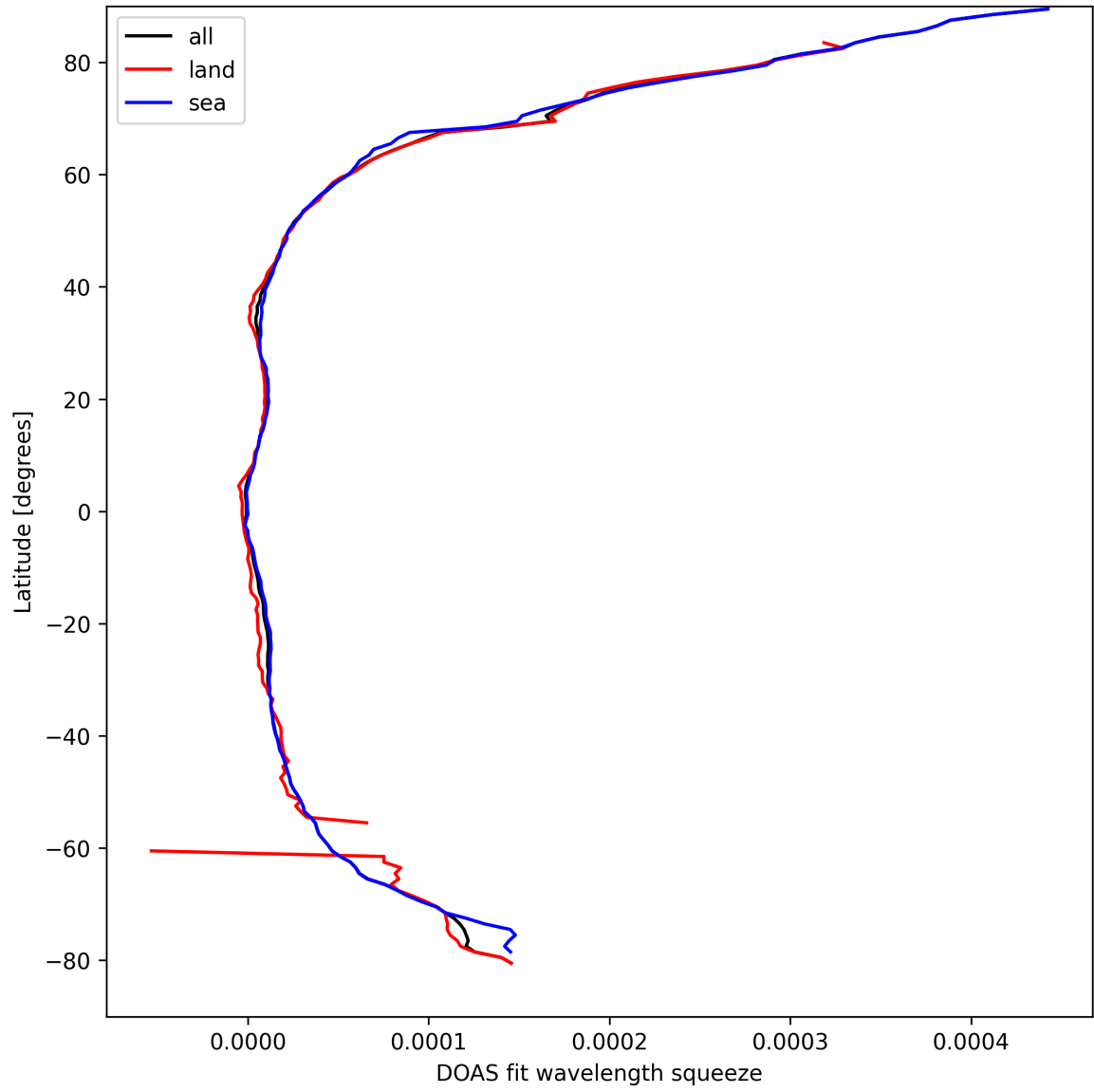
Figure 29: Zonal average of “DOAS fit wavelength squeeze” for 2025-03-31 to 2025-03-31.
