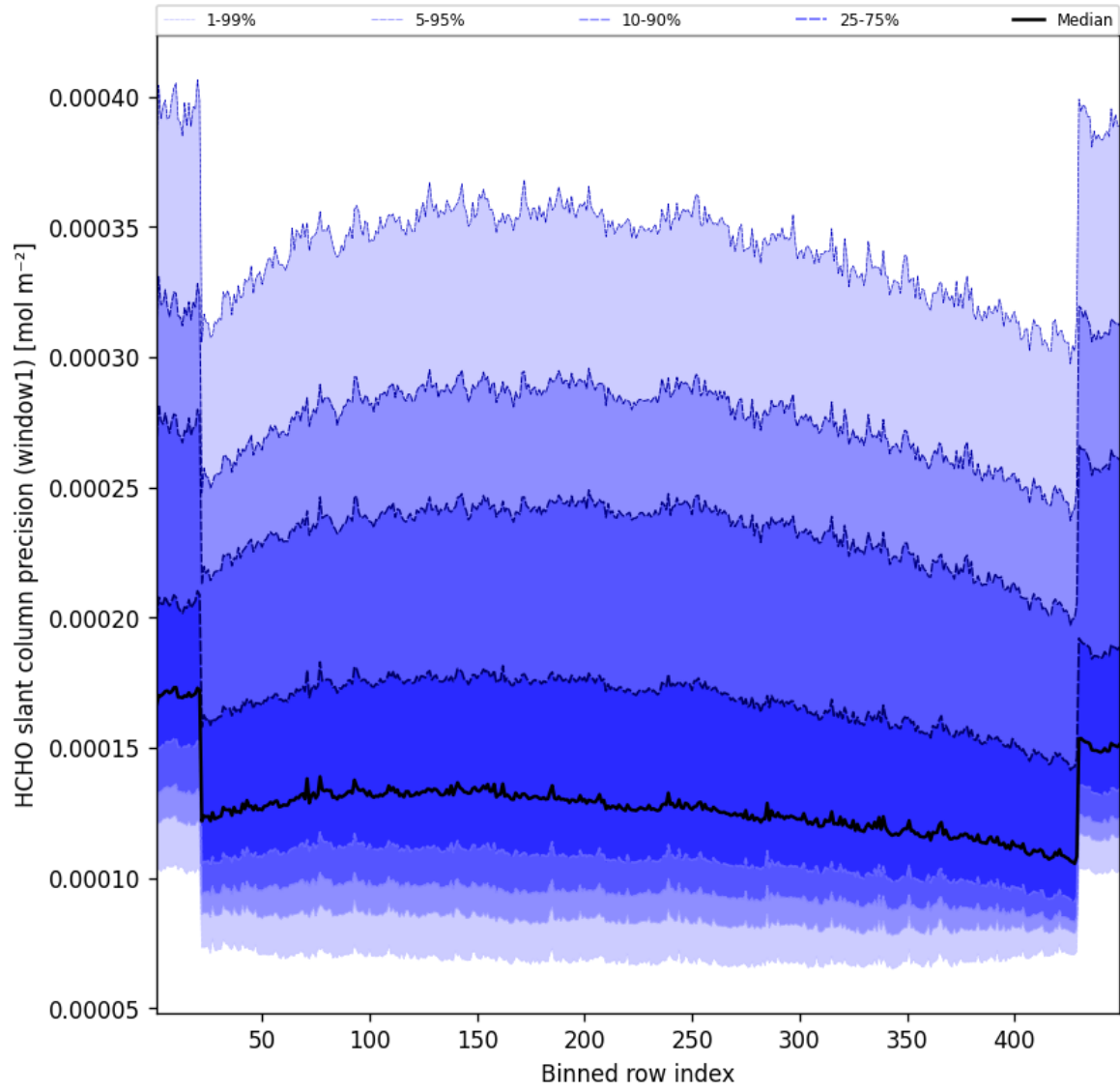
Figure 51: Along track statistics of “HCHO slant column precision (window1)” for 2025-03-31 to 2025-03-31
