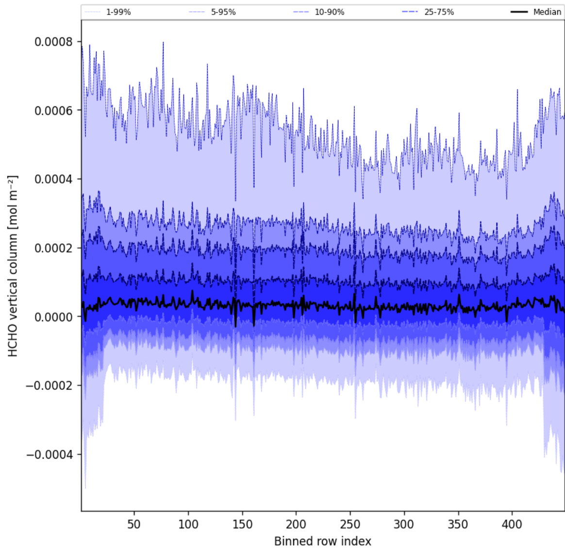
Figure 47: Along track statistics of “HCHO vertical column” for 2025-03-31 to 2025-03-31
