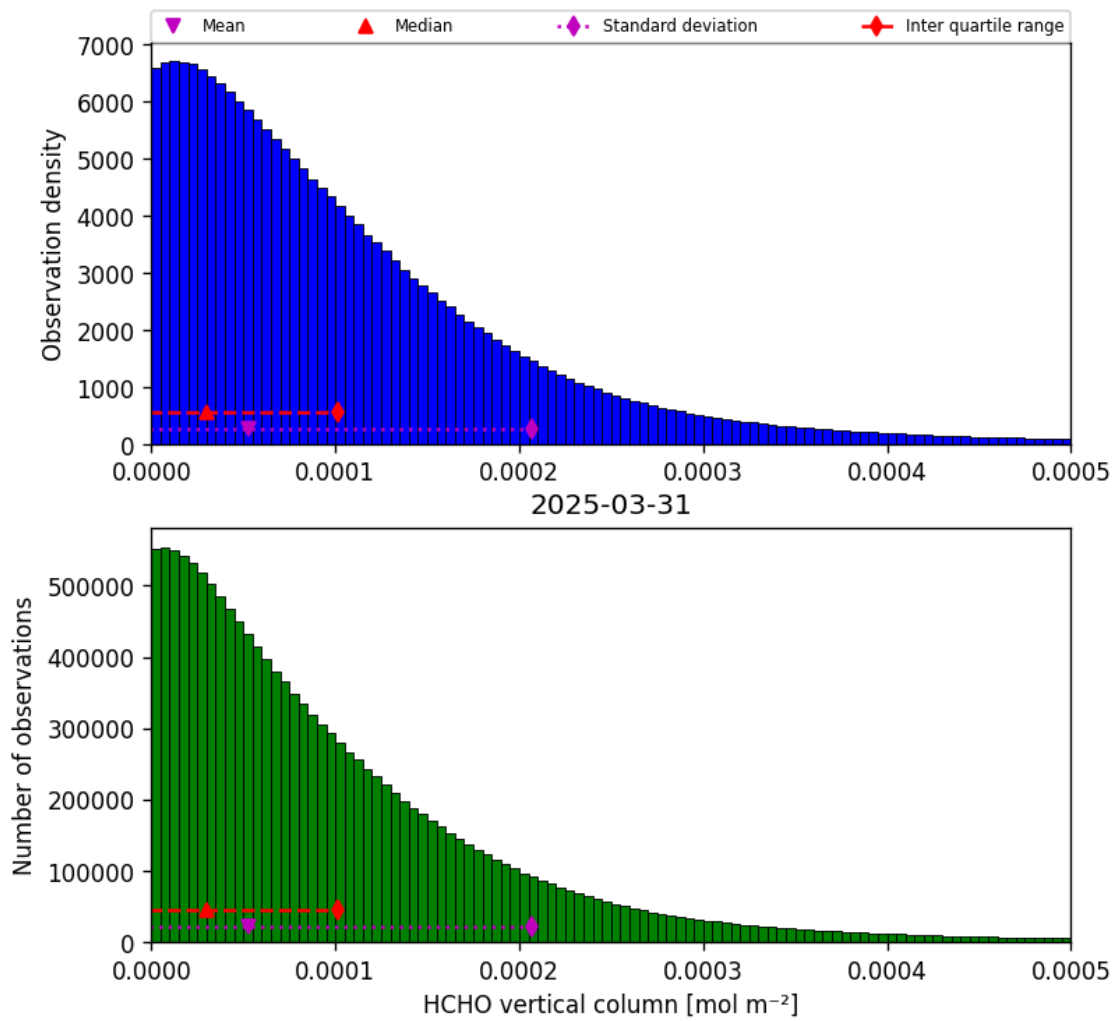
Figure 33: Histogram of “HCHO vertical column” for 2025-03-31 to 2025-03-31
