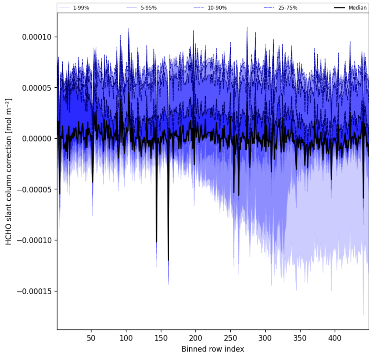
Figure 59: Along track statistics of “HCHO slant column correction” for 2025-03-31 to 2025-03-31
