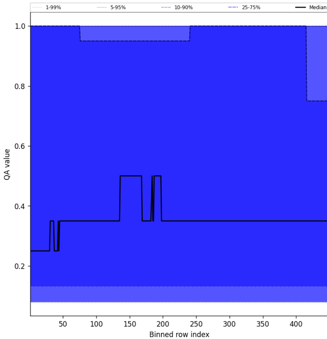
Figure 46: Along track statistics of “QA value” for 2025-04-01 to 2025-04-02
