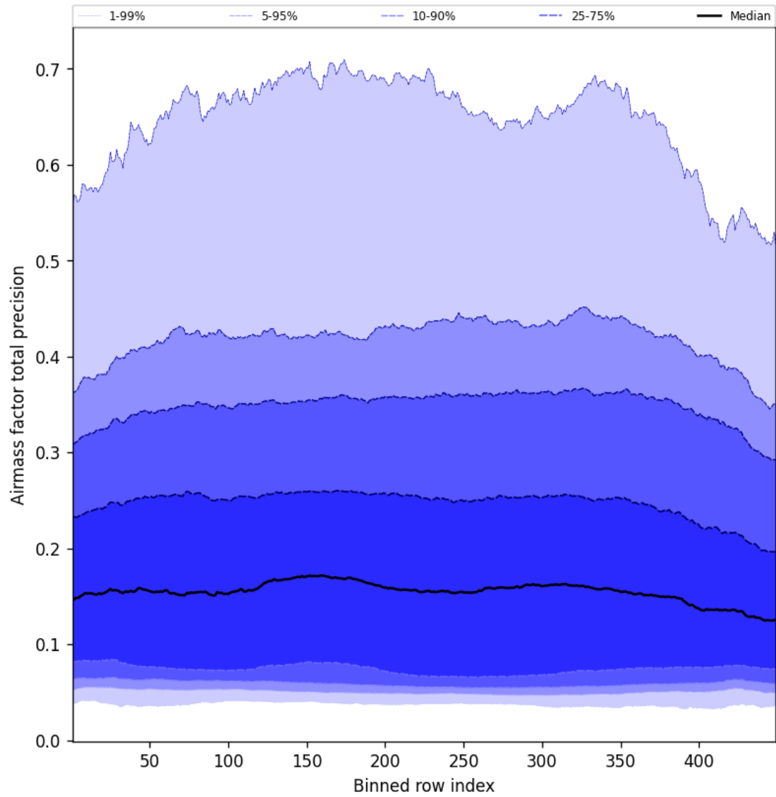
Figure 53: Along track statistics of “Airmass factor total precision” for 2025-04-01 to 2025-04-02
