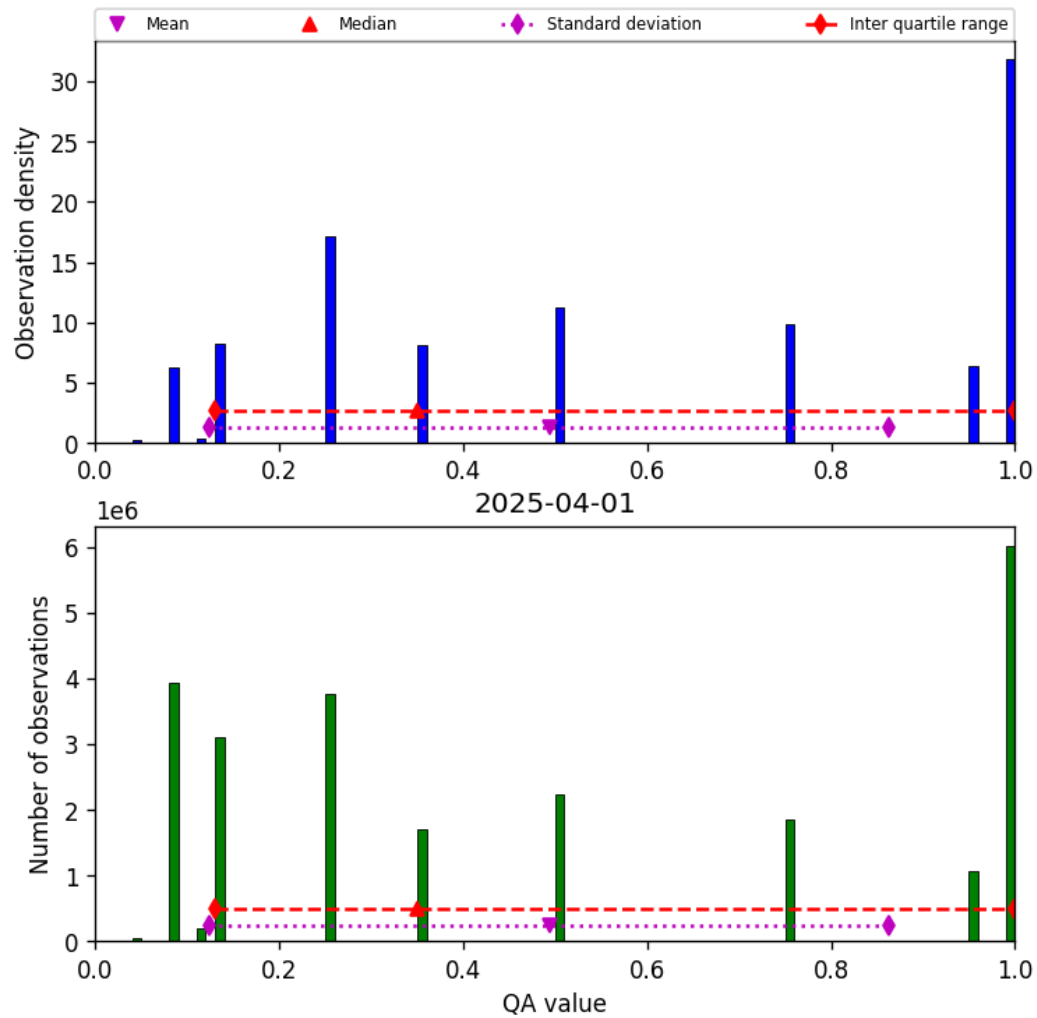
Figure 32: Histogram of “QA value” for 2025-04-01 to 2025-04-02
