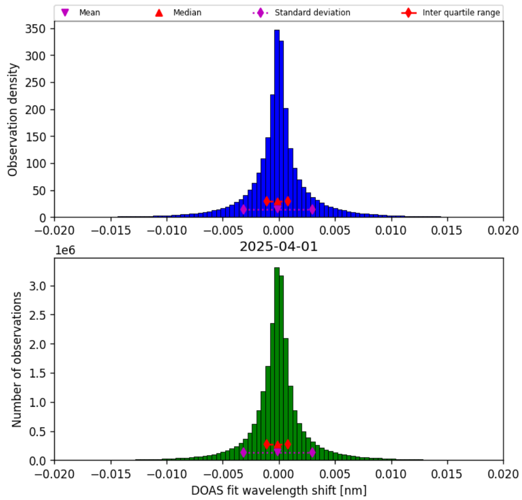
Figure 42: Histogram of “DOAS fit wavelength shift” for 2025-04-01 to 2025-04-02
