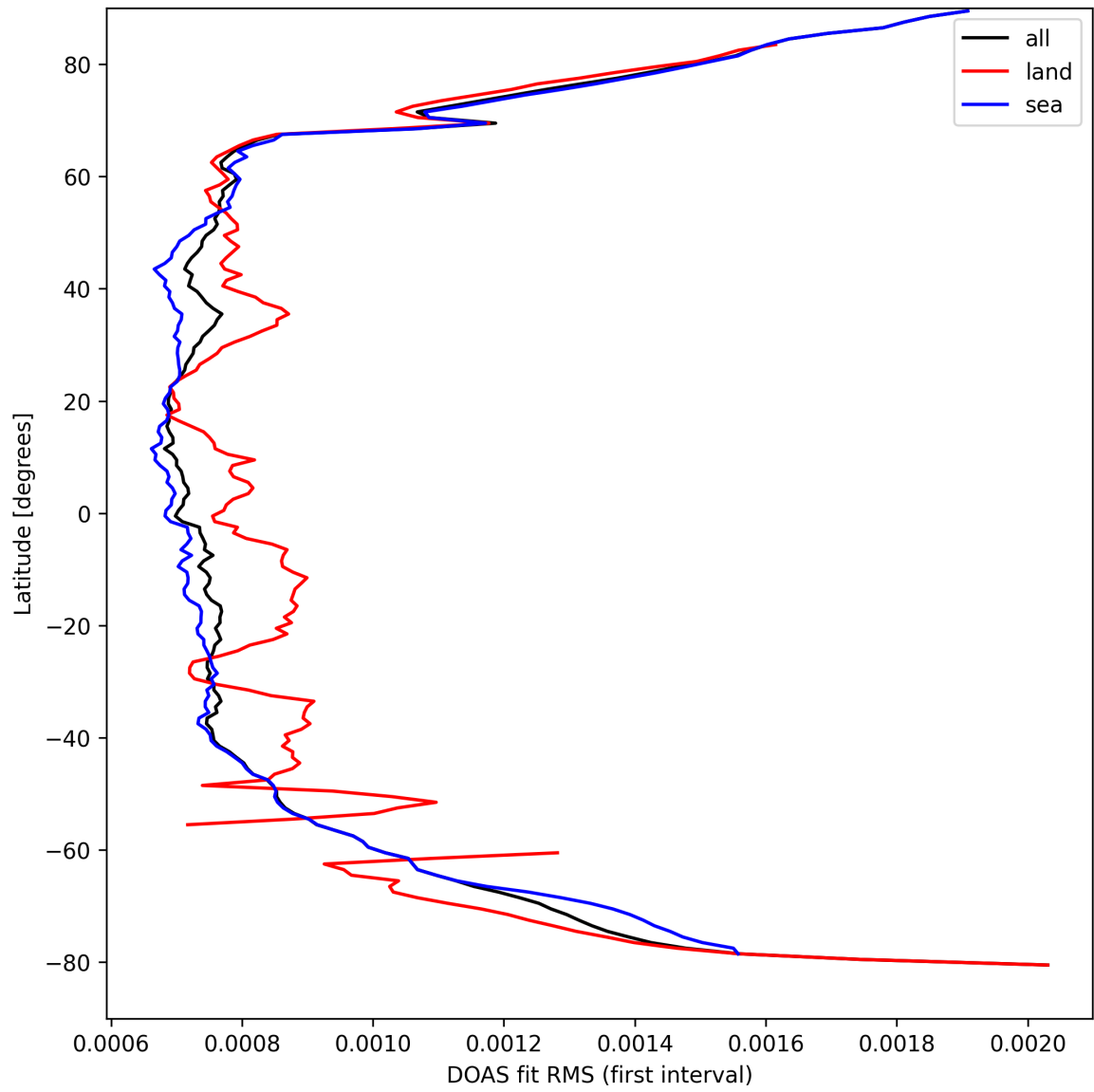
Figure 30: Zonal average of "DOAS fit RMS (first interval)" for 2025-04-01 to 2025-04-02.
