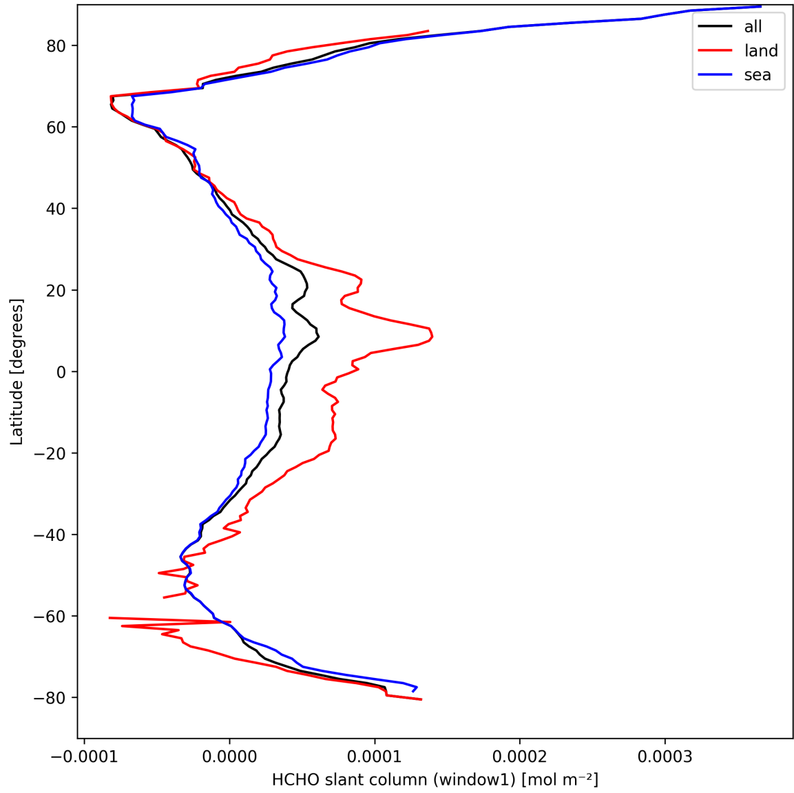
Figure 22: Zonal average of “HCHO slant column (window1)” for 2025-04-01 to 2025-04-02.
