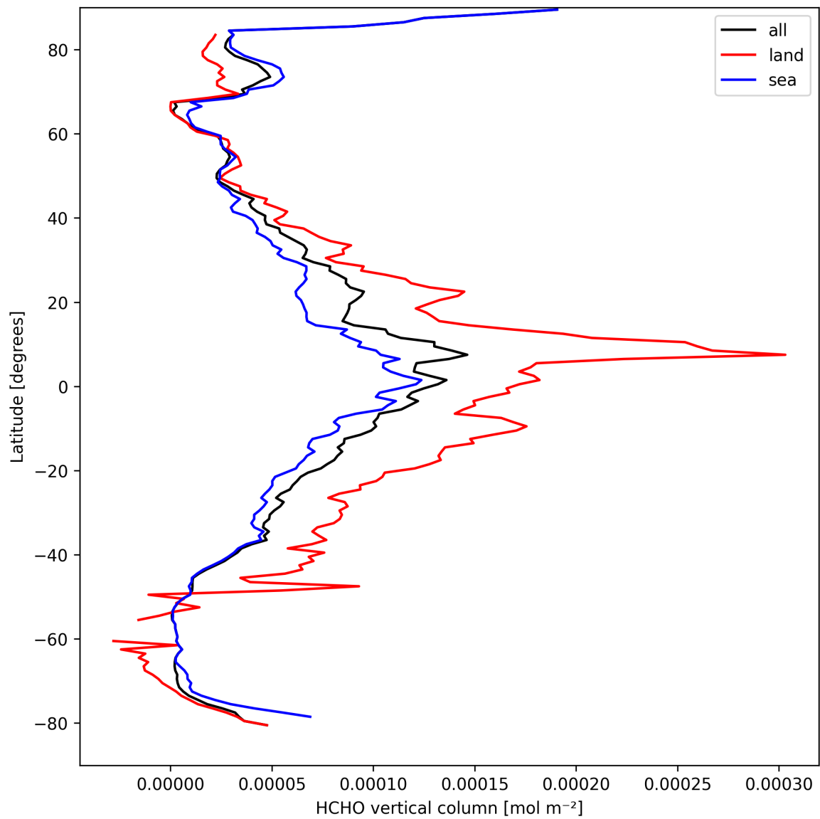
Figure 19: Zonal average of “HCHO vertical column” for 2025-04-01 to 2025-04-02.
