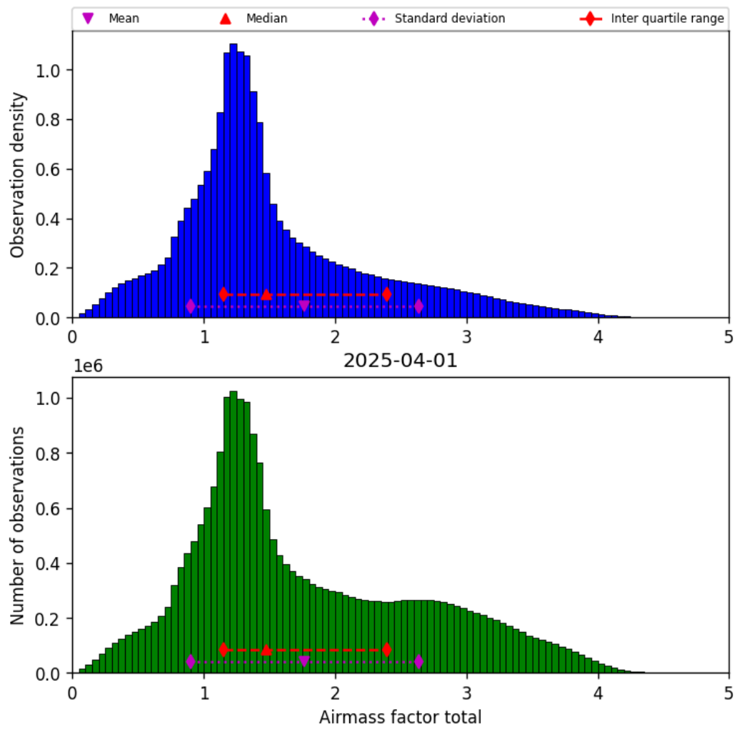
Figure 38: Histogram of “Airmass factor total” for 2025-04-01 to 2025-04-02
