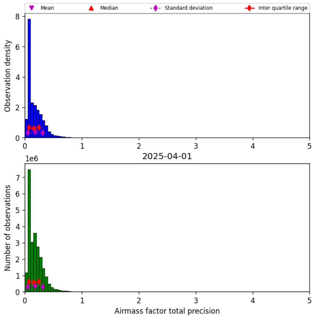
Figure 39: Histogram of “Airmass factor total precision” for 2025-04-01 to 2025-04-02
