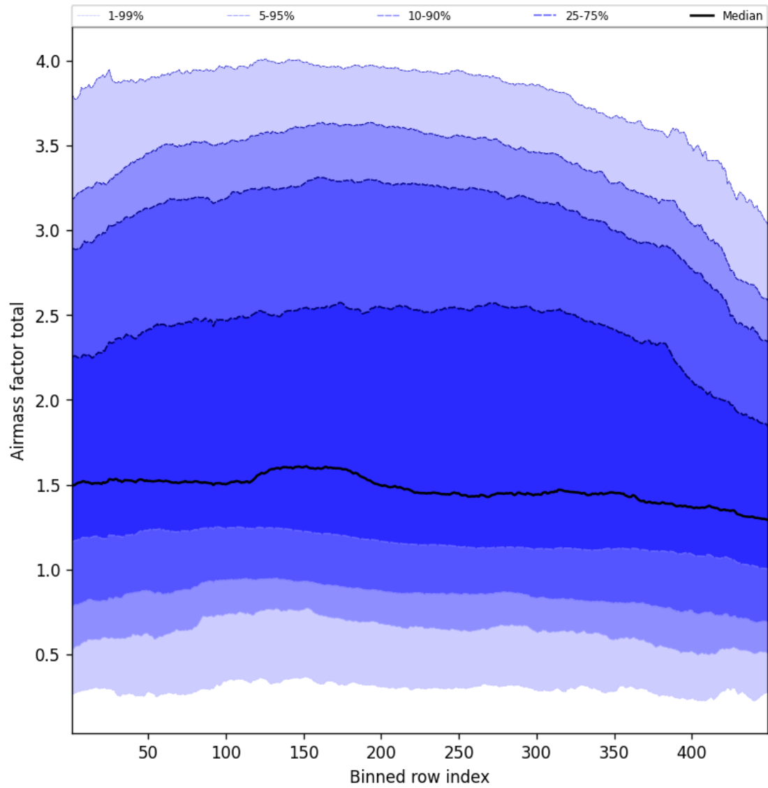
Figure 52: Along track statistics of “Airmass factor total” for 2025-04-01 to 2025-04-02
