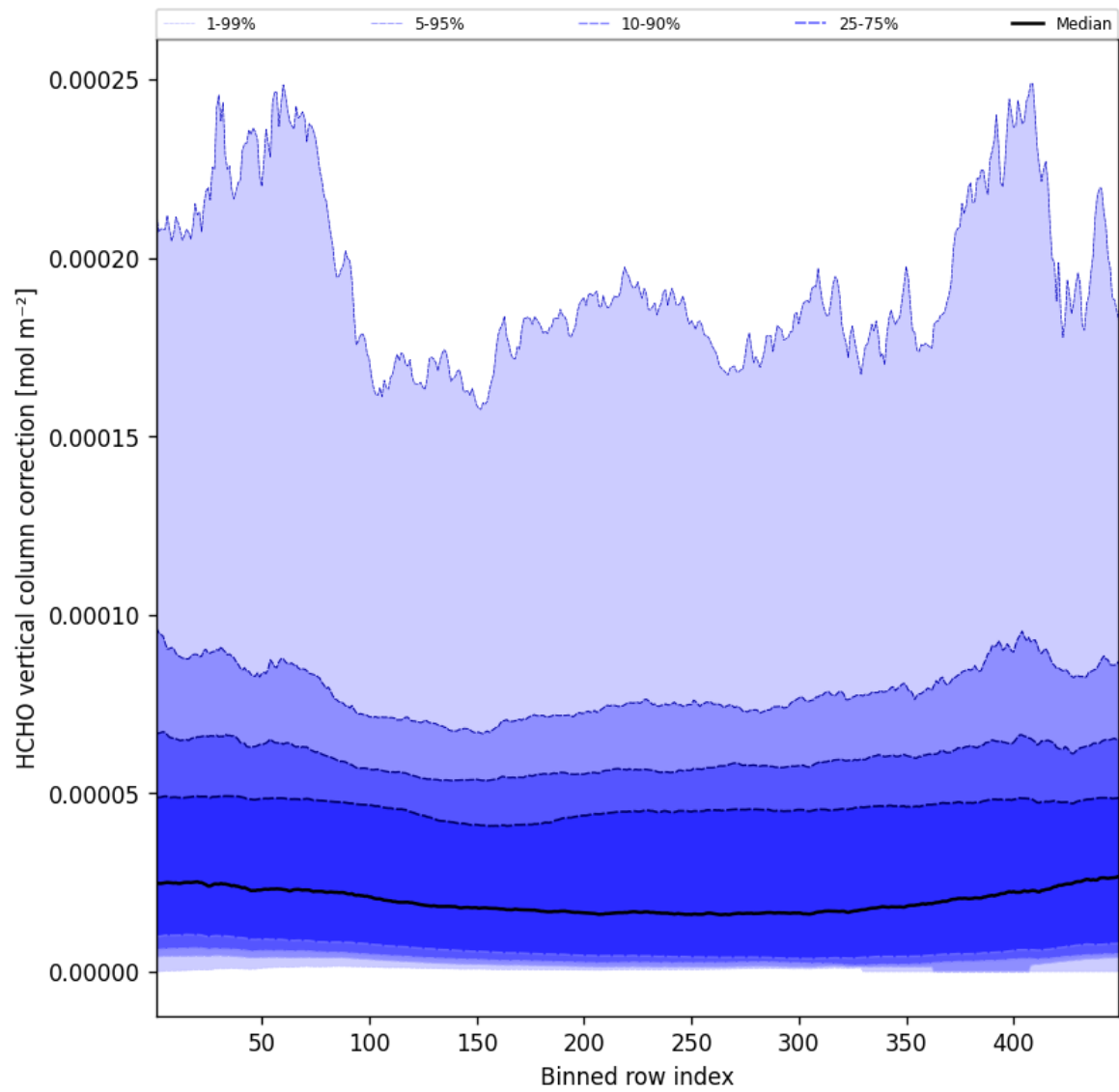
Figure 49: Along track statistics of “HCHO vertical column correction” for 2025-04-01 to 2025-04-02
