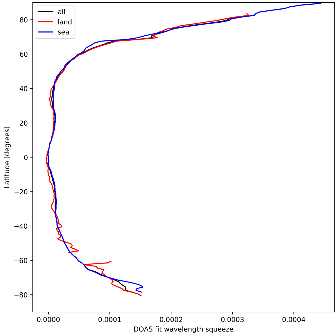
Figure 29: Zonal average of “DOAS fit wavelength squeeze” for 2025-04-01 to 2025-04-02.
