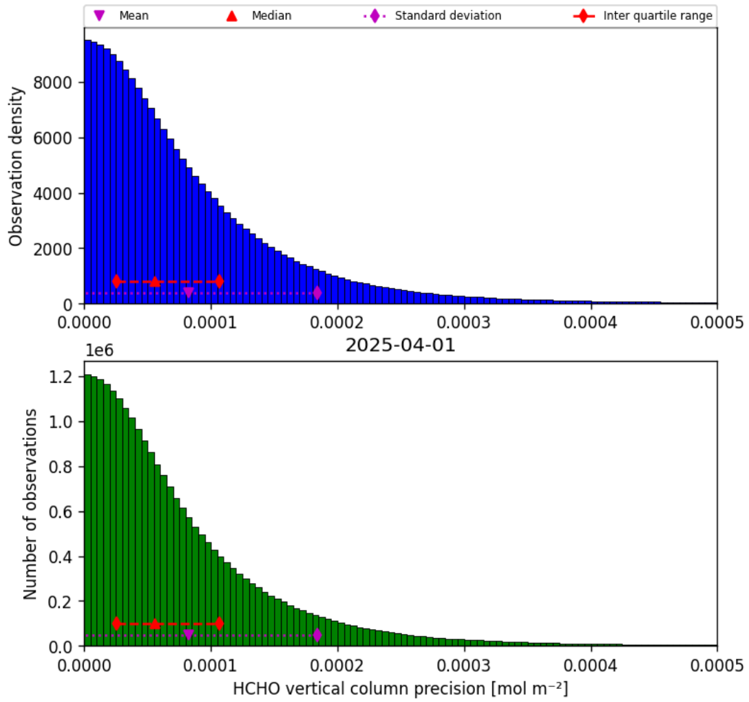
Figure 34: Histogram of “HCHO vertical column precision” for 2025-04-01 to 2025-04-02
