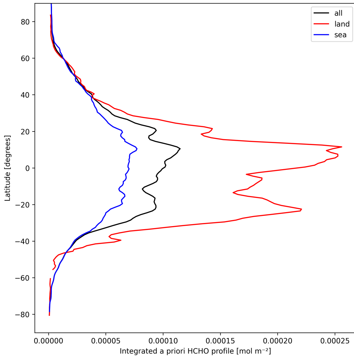
Figure 27: Zonal average of “Integrated a priori HCHO profile” for 2025-04-01 to 2025-04-02.
