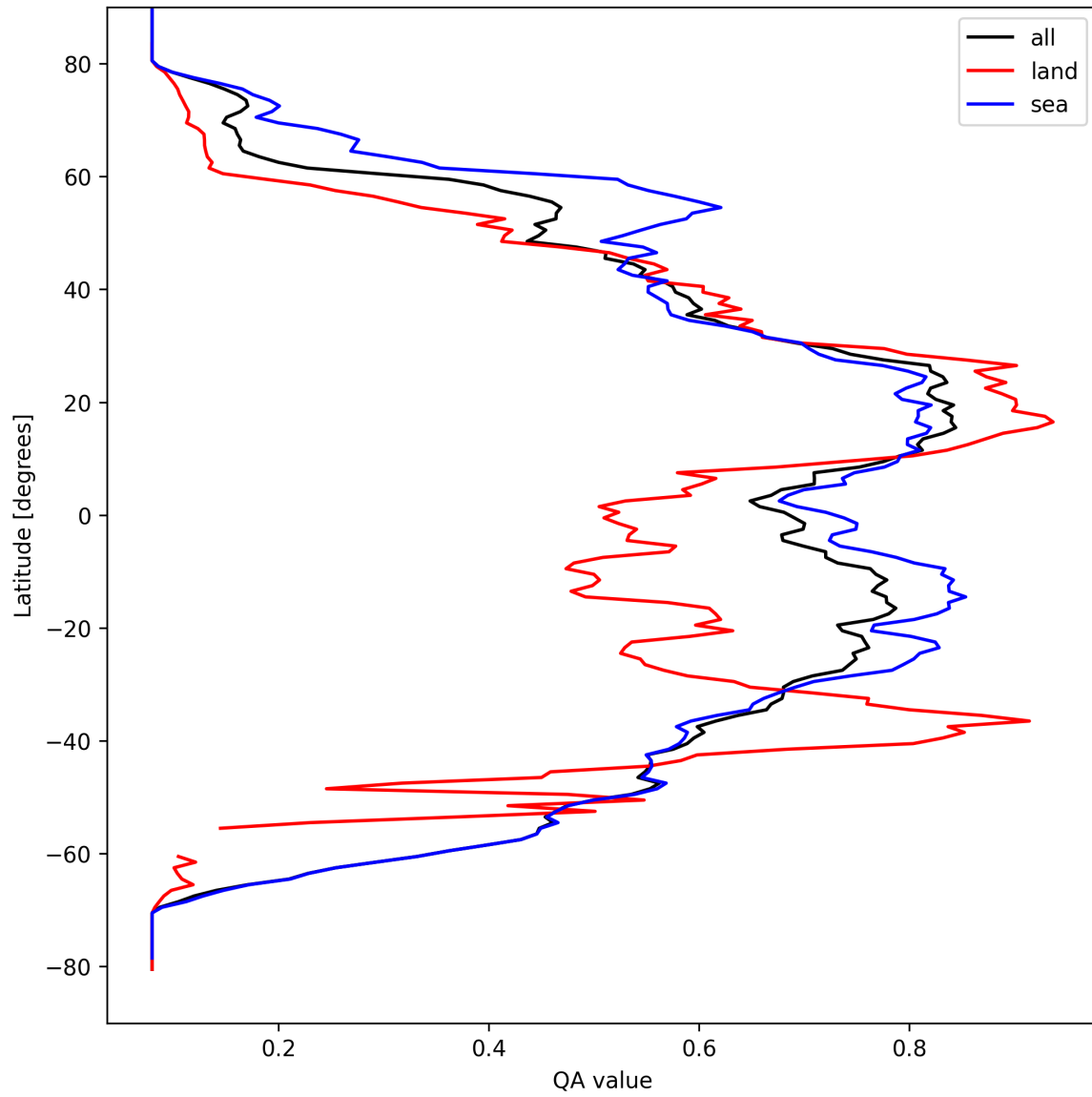
Figure 18: Zonal average of “QA value” for 2025-04-01 to 2025-04-02.
