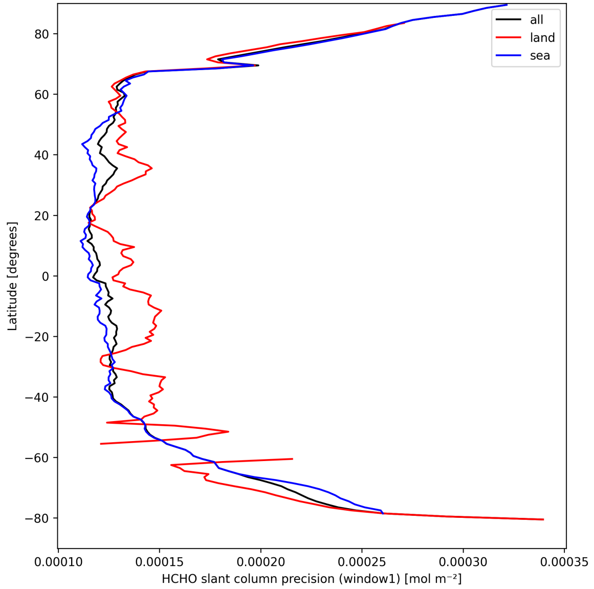
Figure 23: Zonal average of “HCHO slant column precision (window1)” for 2025-04-01 to 2025-04-02.
