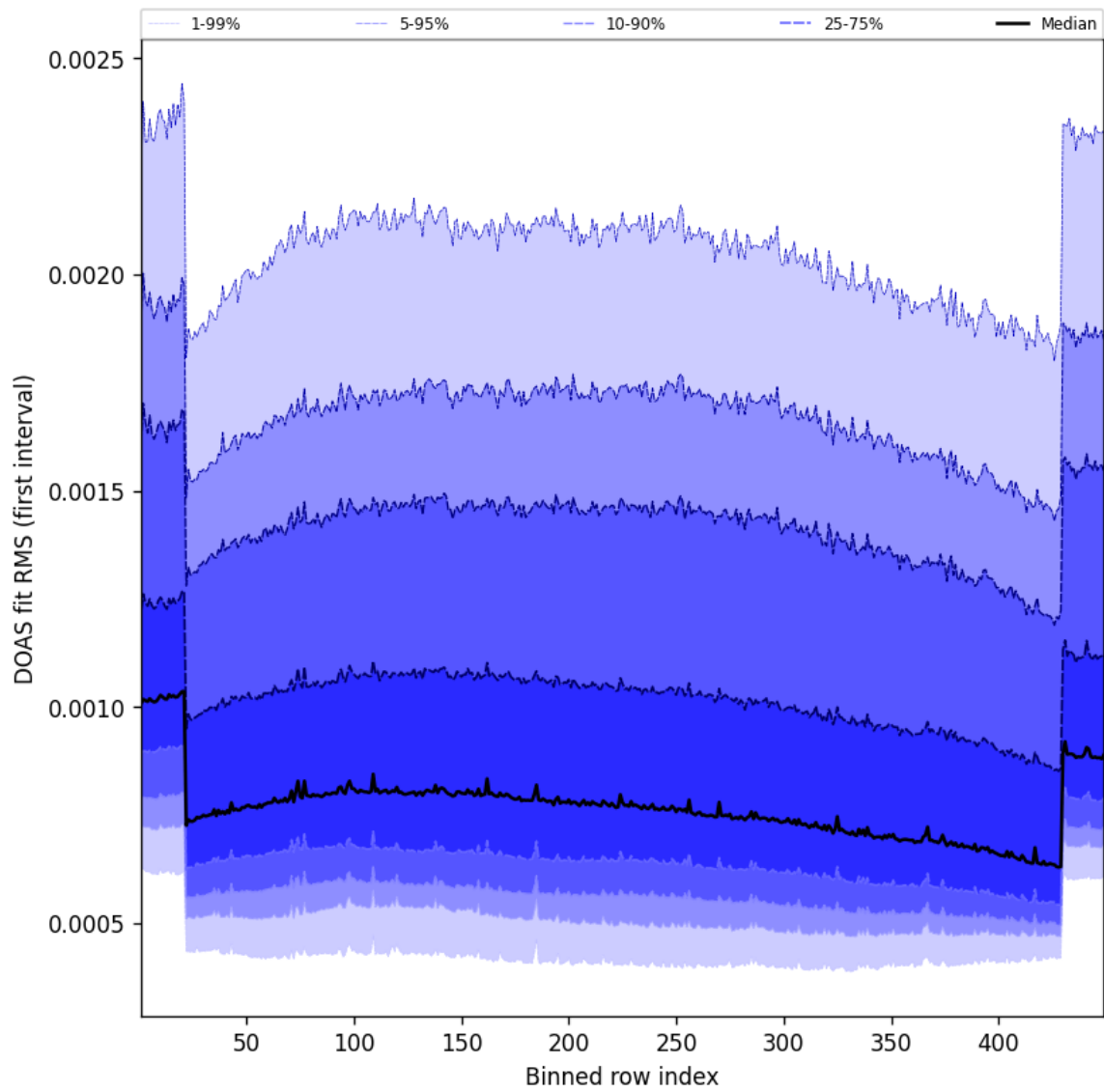
Figure 58: Along track statistics of “DOAS fit RMS (first interval)” for 2025-04-01 to 2025-04-02
