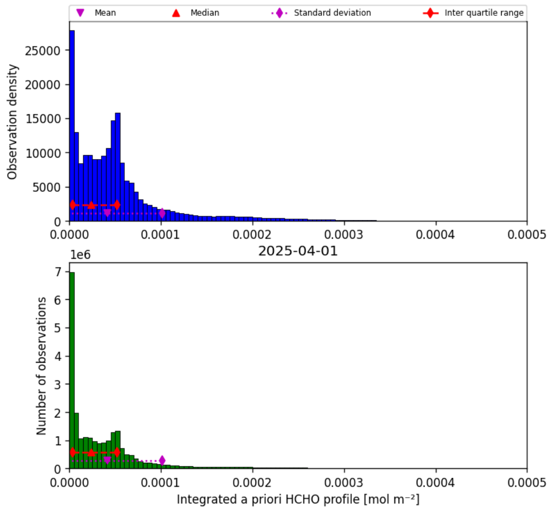
Figure 41: Histogram of “Integrated a priori HCHO profile” for 2025-04-01 to 2025-04-02
