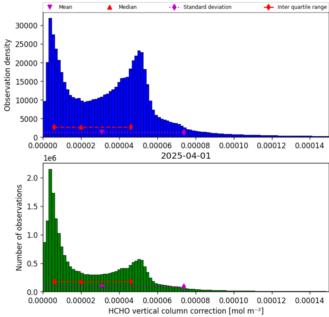
Figure 35: Histogram of “HCHO vertical column correction” for 2025-04-01 to 2025-04-02
