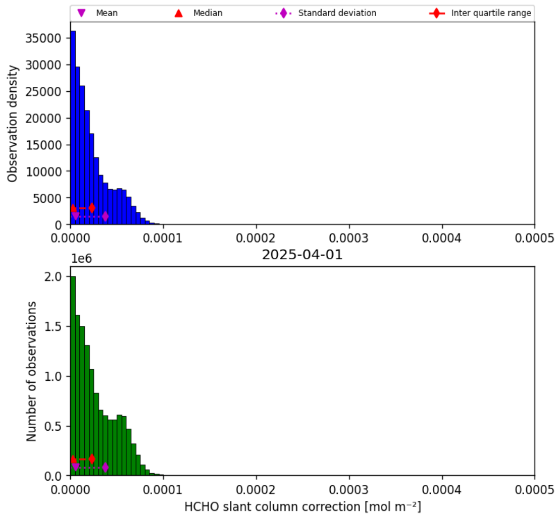
Figure 45: Histogram of “HCHO slant column correction” for 2025-04-01 to 2025-04-02
