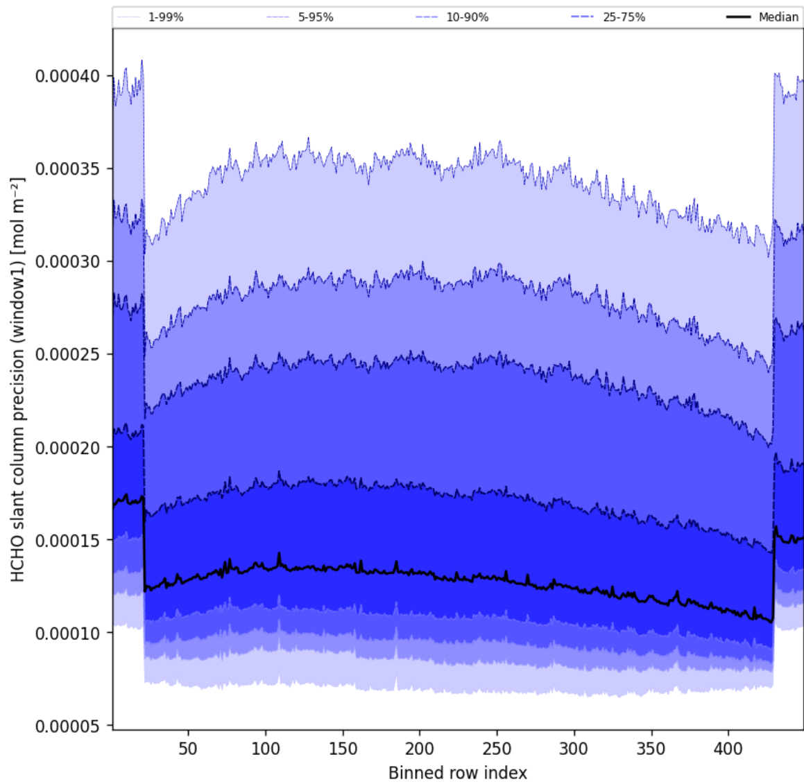
Figure 51: Along track statistics of “HCHO slant column precision (window1)” for 2025-04-01 to 2025-04-02
