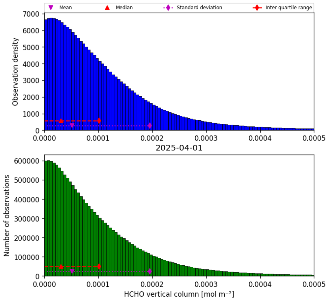
Figure 33: Histogram of “HCHO vertical column” for 2025-04-01 to 2025-04-02
