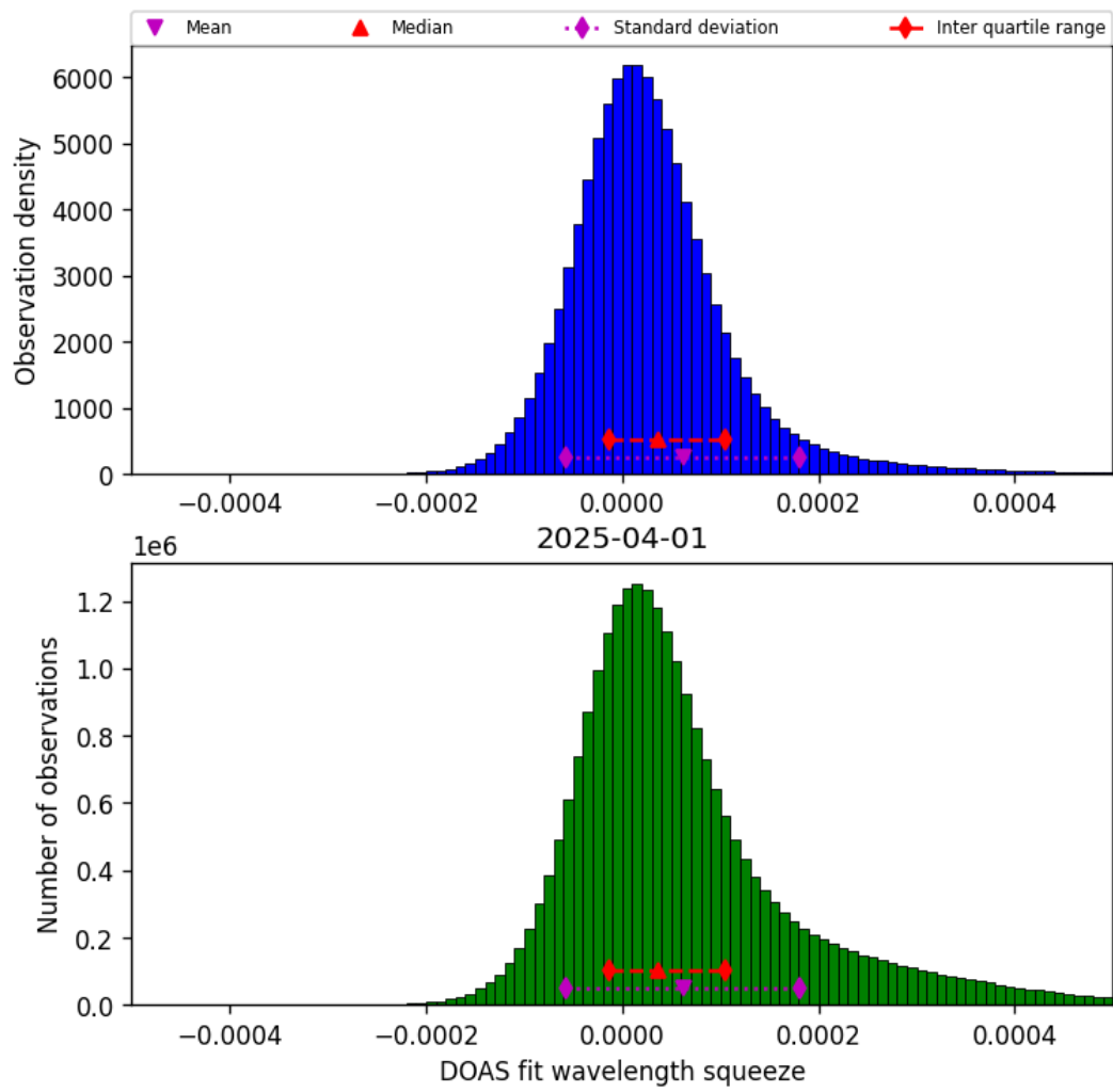
Figure 43: Histogram of “DOAS fit wavelength squeeze” for 2025-04-01 to 2025-04-02
