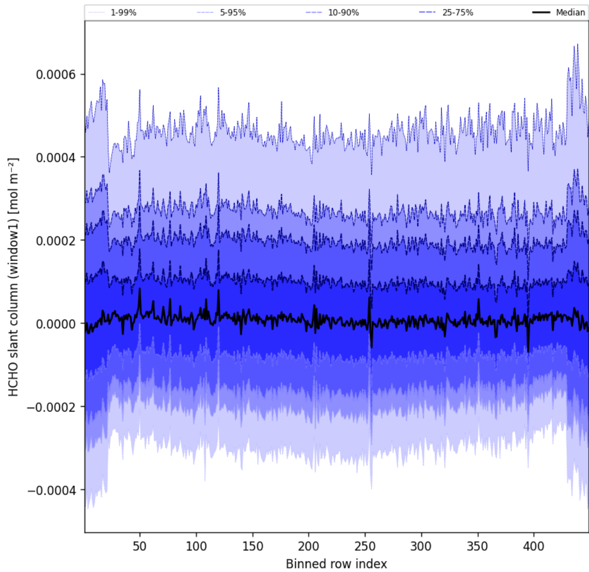
Figure 50: Along track statistics of “HCHO slant column (window1)” for 2025-04-01 to 2025-04-02
