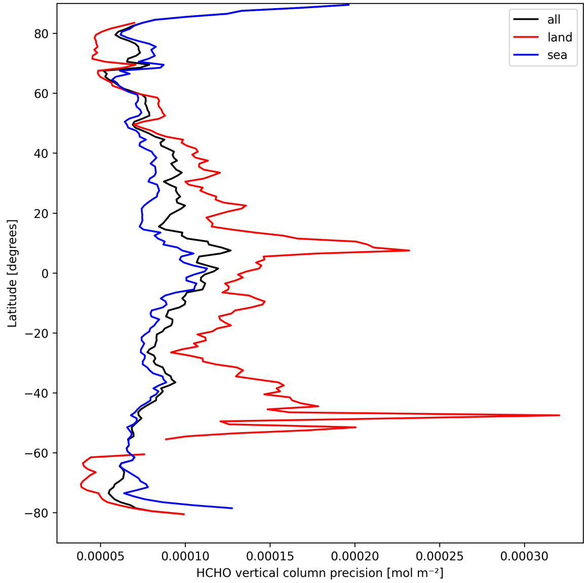
Figure 20: Zonal average of “HCHO vertical column precision” for 2025-04-01 to 2025-04-02.
