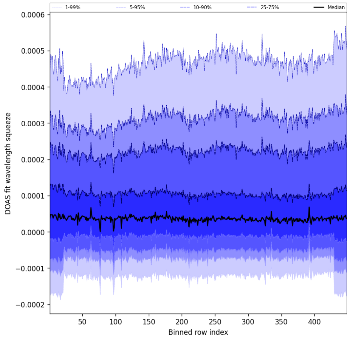
Figure 57: Along track statistics of “DOAS fit wavelength squeeze” for 2025-04-01 to 2025-04-02
