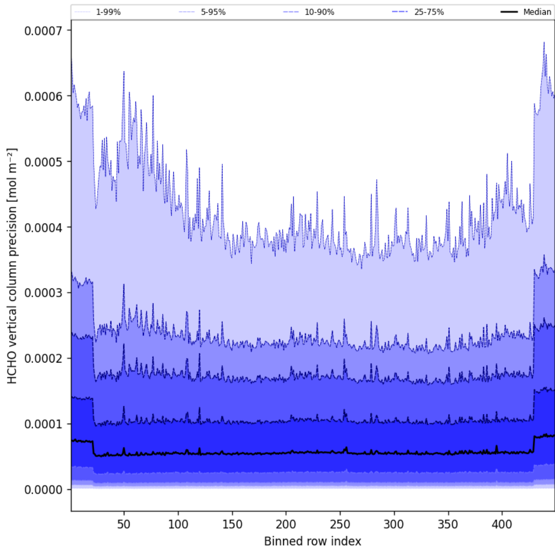
Figure 48: Along track statistics of “HCHO vertical column precision” for 2025-04-01 to 2025-04-02
