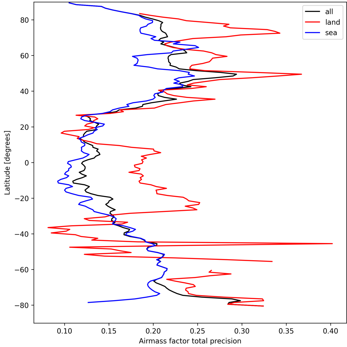
Figure 25: Zonal average of “Airmass factor total precision” for 2025-04-01 to 2025-04-02.
