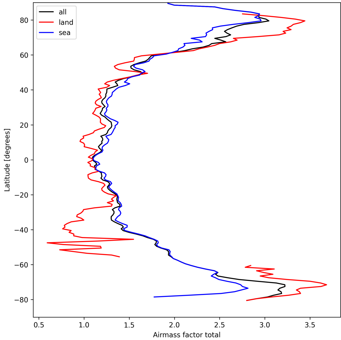
Figure 24: Zonal average of “Airmass factor total” for 2025-04-01 to 2025-04-02.
