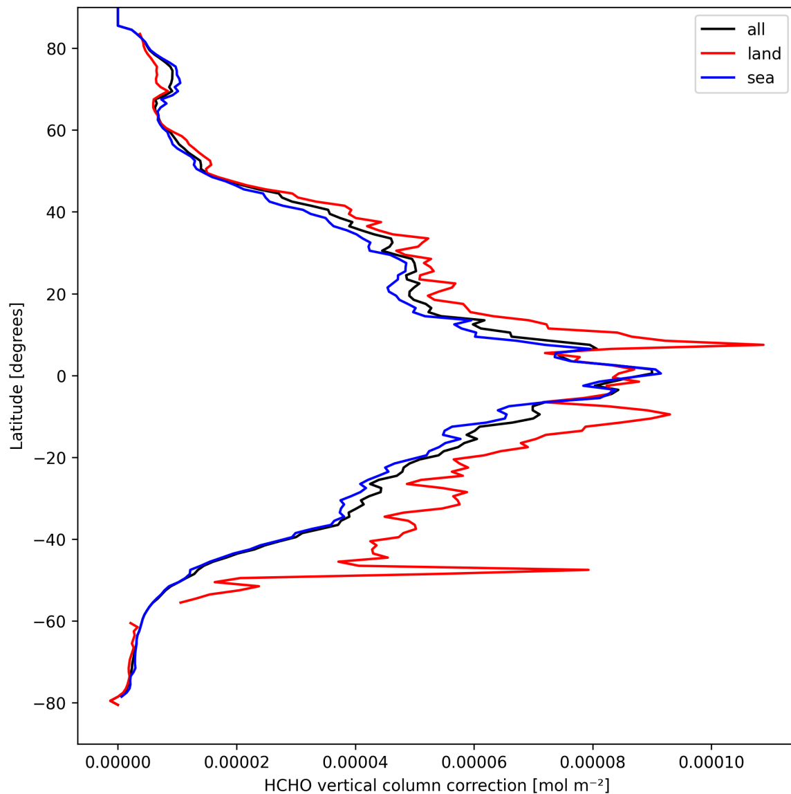
Figure 21: Zonal average of “HCHO vertical column correction” for 2025-04-01 to 2025-04-02.
