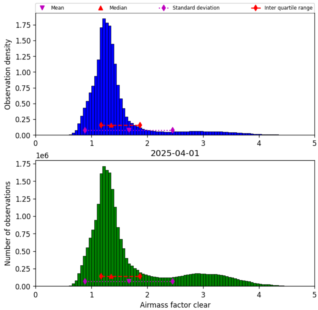
Figure 40: Histogram of “Airmass factor clear” for 2025-04-01 to 2025-04-02
