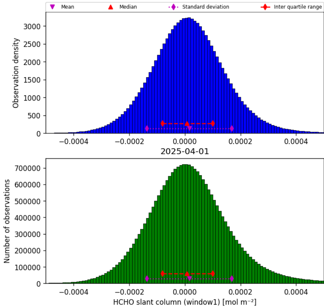
Figure 36: Histogram of “HCHO slant column (window1)” for 2025-04-01 to 2025-04-02
