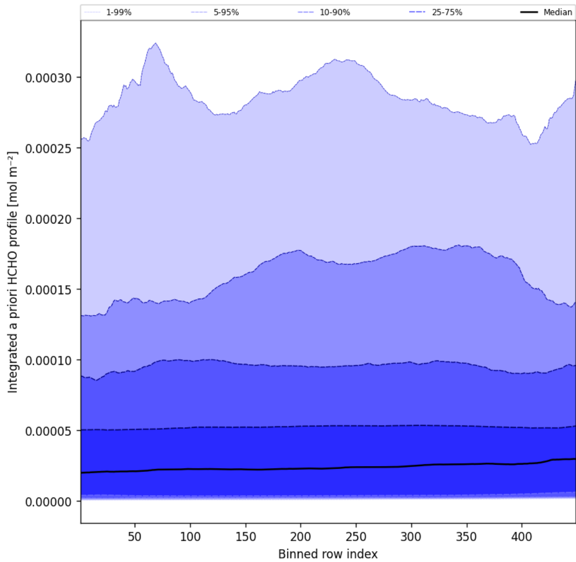
Figure 55: Along track statistics of "Integrated a priori HCHO profile" for 2025-04-01 to 2025-04-02
