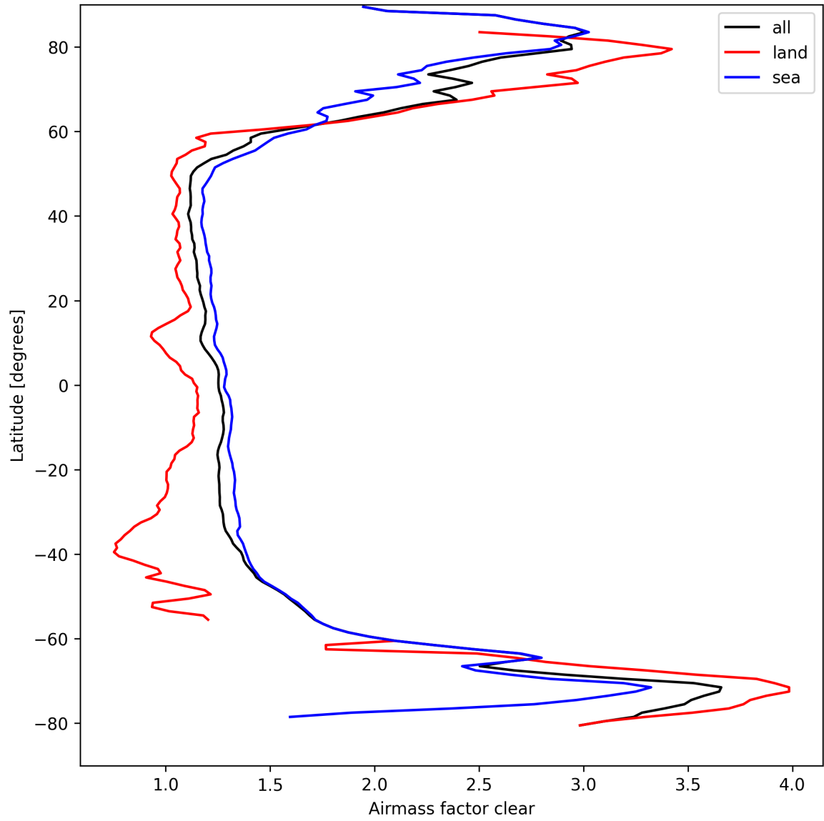
Figure 26: Zonal average of “Airmass factor clear” for 2025-04-01 to 2025-04-02.
