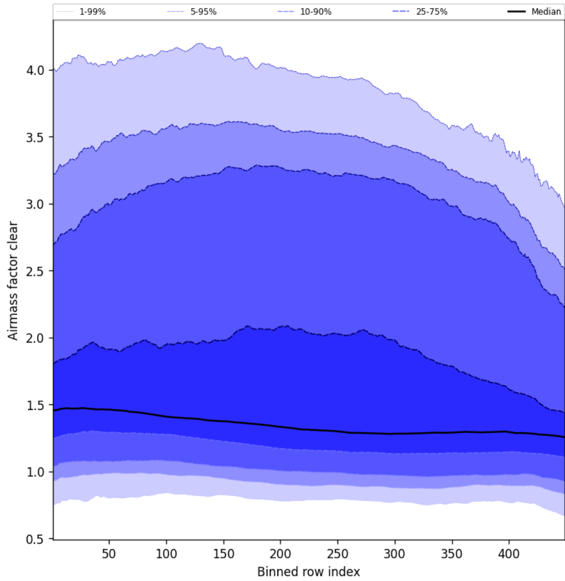
Figure 54: Along track statistics of “Airmass factor clear” for 2025-04-01 to 2025-04-02
