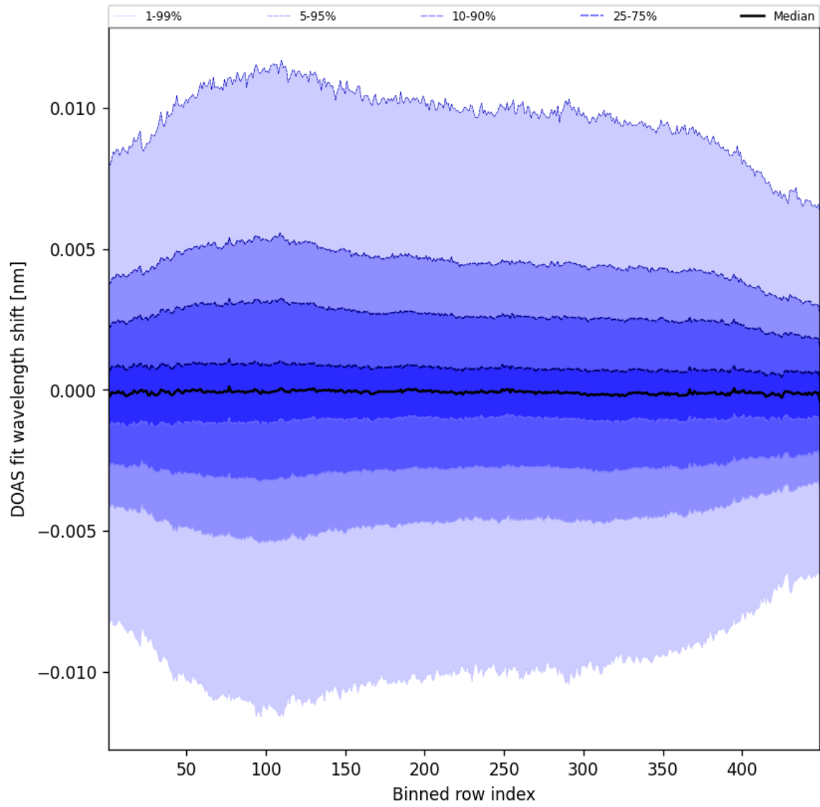
Figure 56: Along track statistics of “DOAS fit wavelength shift” for 2025-04-01 to 2025-04-02
