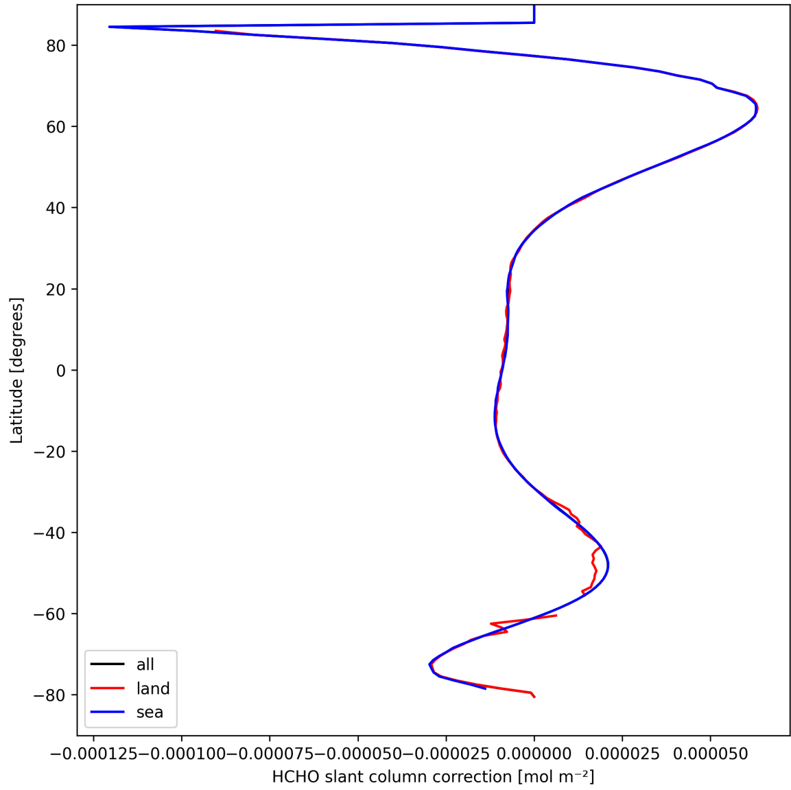
Figure 31: Zonal average of “HCHO slant column correction” for 2025-04-01 to 2025-04-02.
