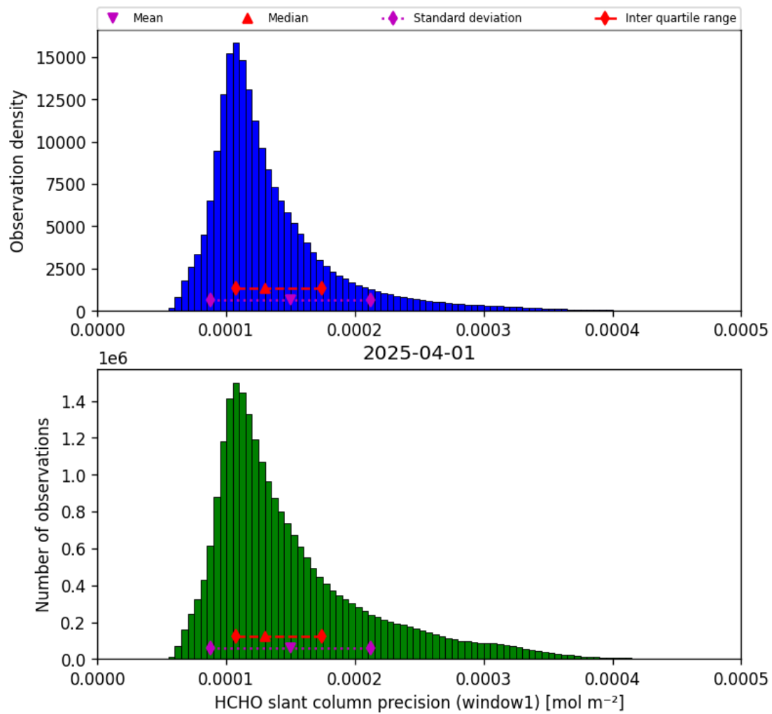
Figure 37: Histogram of “HCHO slant column precision (window1)” for 2025-04-01 to 2025-04-02
