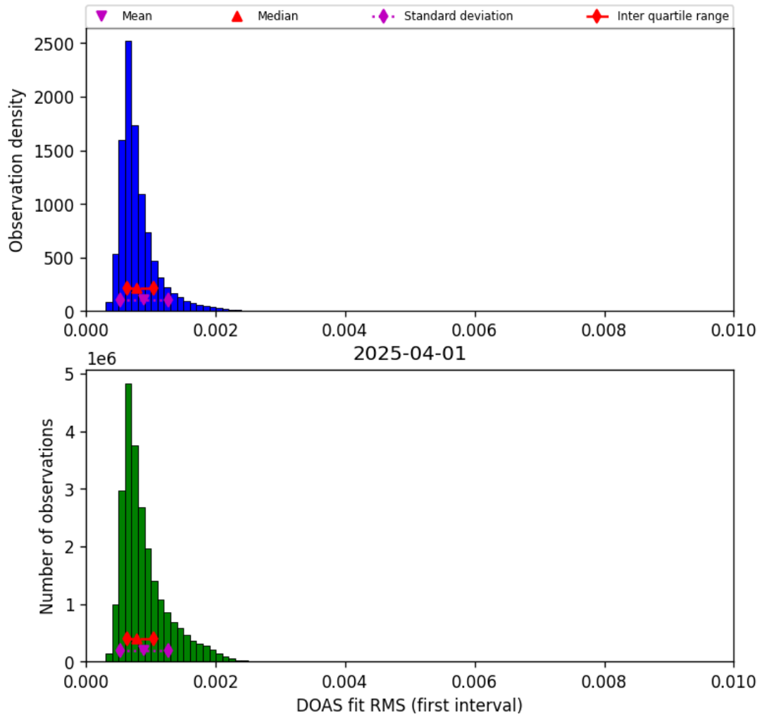
Figure 44: Histogram of “DOAS fit RMS (first interval)” for 2025-04-01 to 2025-04-02
