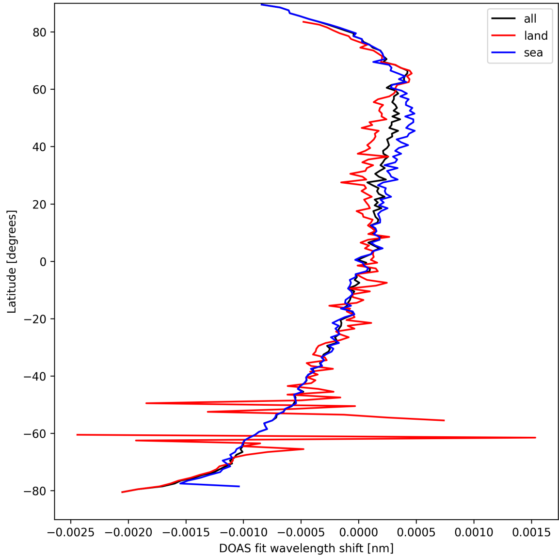
Figure 28: Zonal average of "DOAS fit wavelength shift" for 2025-04-01 to 2025-04-02.
