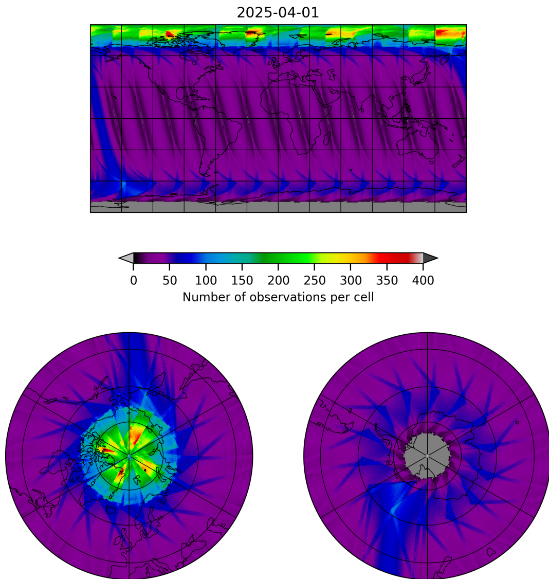
Figure 17: Map of the number of observations for 2025-04-01 to 2025-04-02
