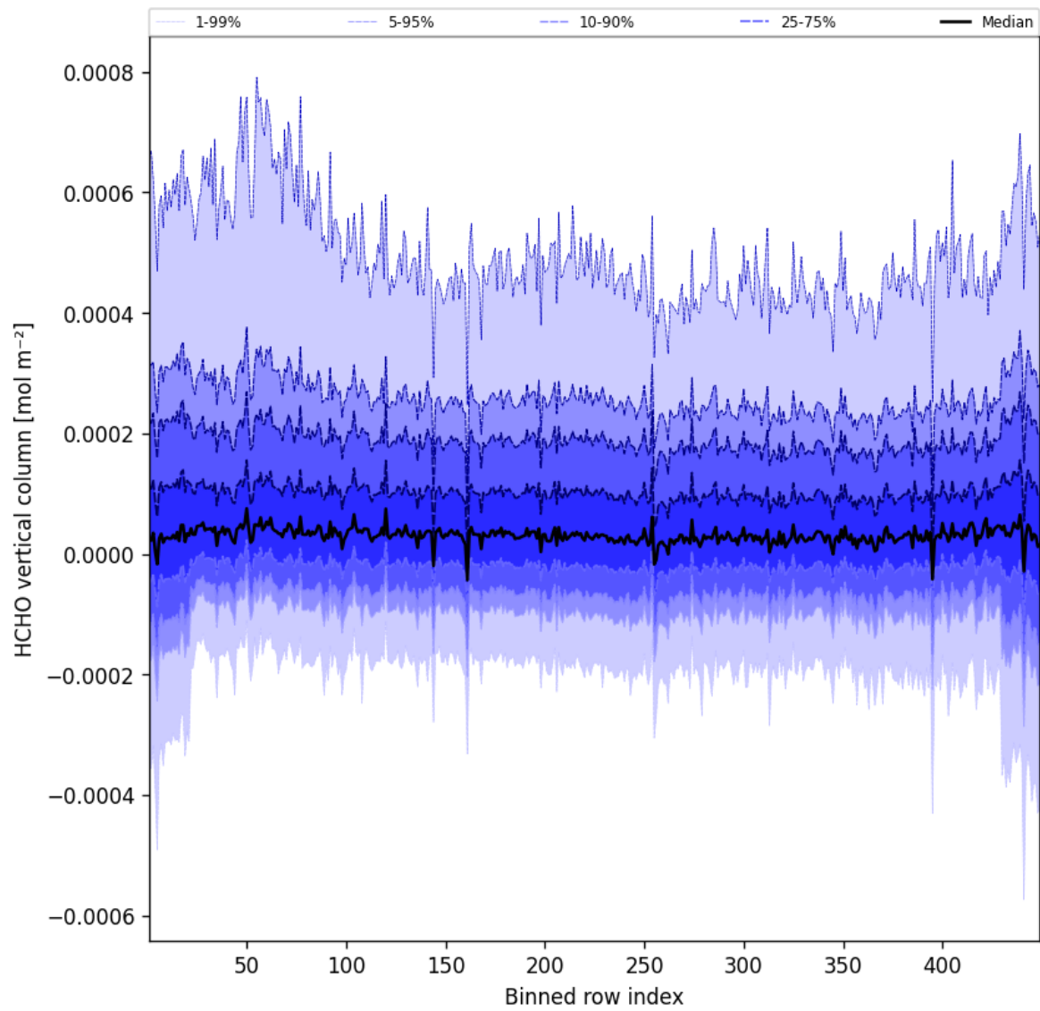
Figure 47: Along track statistics of “HCHO vertical column” for 2025-04-01 to 2025-04-02
