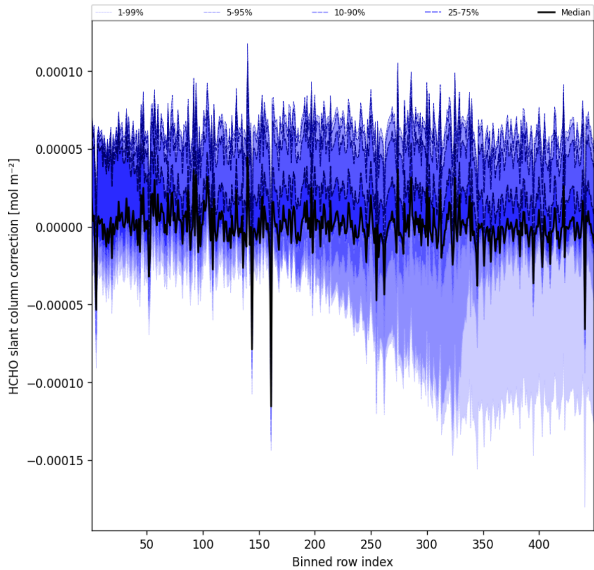
Figure 59: Along track statistics of “HCHO slant column correction” for 2025-04-01 to 2025-04-02
