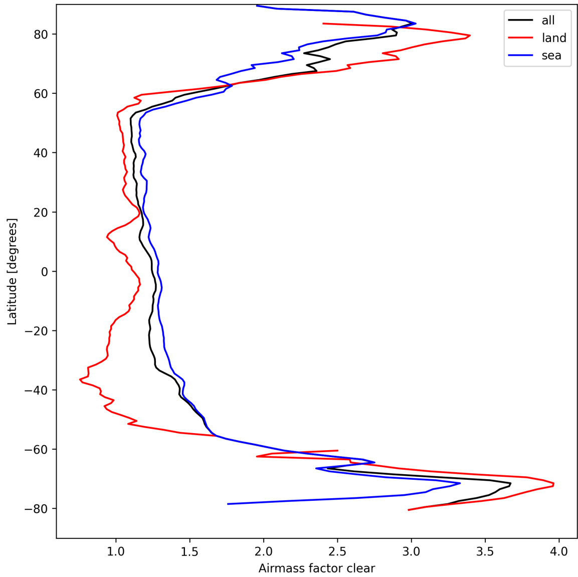
Figure 26: Zonal average of “Airmass factor clear” for 2025-04-02 to 2025-04-03.
