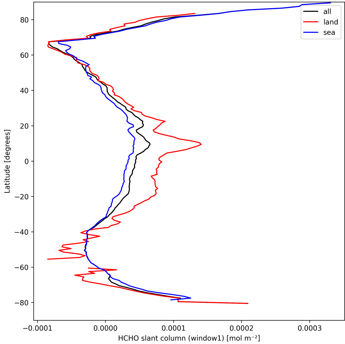
Figure 22: Zonal average of “HCHO slant column (window1)” for 2025-04-02 to 2025-04-03.
