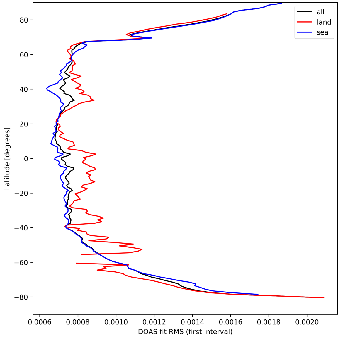
Figure 30: Zonal average of “DOAS fit RMS (first interval)” for 2025-04-02 to 2025-04-03.
