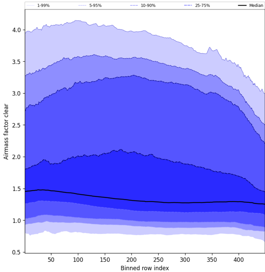
Figure 54: Along track statistics of “Airmass factor clear” for 2025-04-02 to 2025-04-03
