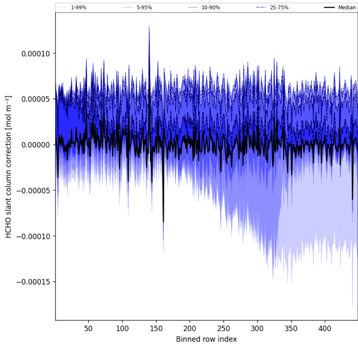
Figure 59: Along track statistics of “HCHO slant column correction” for 2025-04-02 to 2025-04-03
