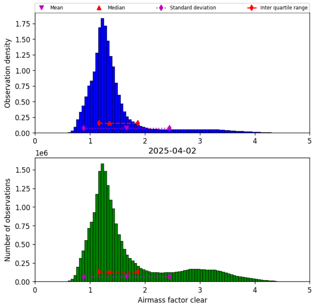
Figure 40: Histogram of “Airmass factor clear” for 2025-04-02 to 2025-04-03
