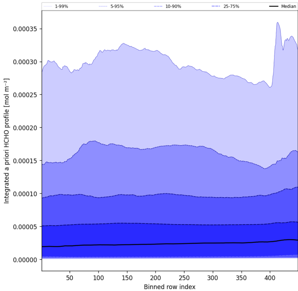
Figure 55: Along track statistics of “Integrated a priori HCHO profile” for 2025-04-02 to 2025-04-03
