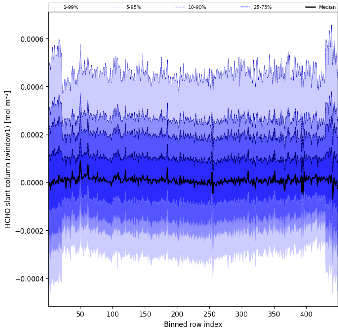
Figure 50: Along track statistics of "HCHO slant column (window1)" for 2025-04-02 to 2025-04-03
