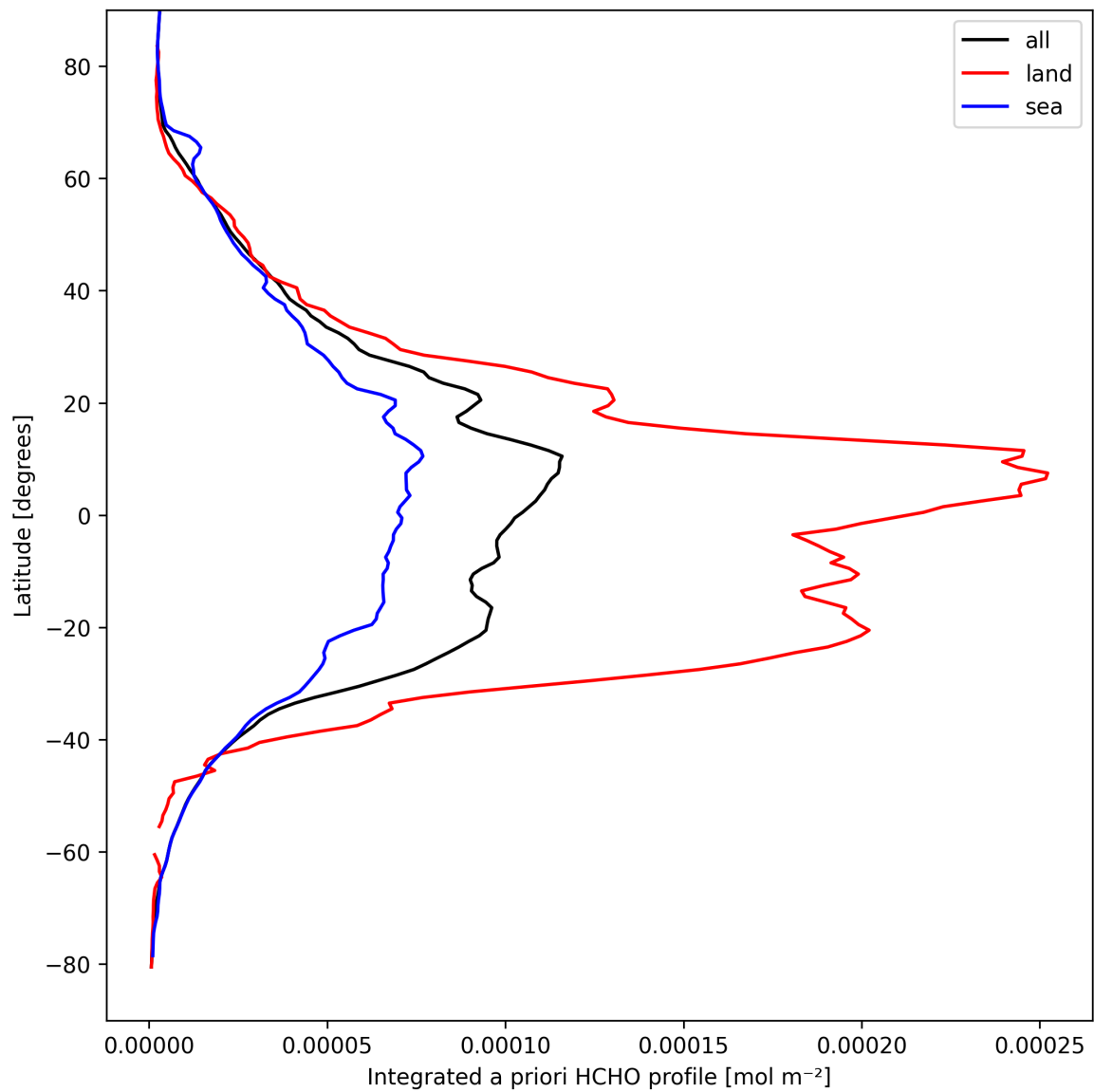
Figure 27: Zonal average of “Integrated a priori HCHO profile” for 2025-04-02 to 2025-04-03.
