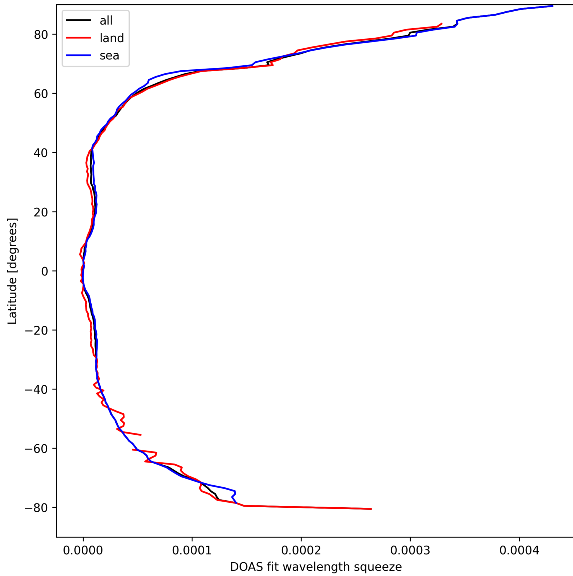
Figure 29: Zonal average of “DOAS fit wavelength squeeze” for 2025-04-02 to 2025-04-03.
