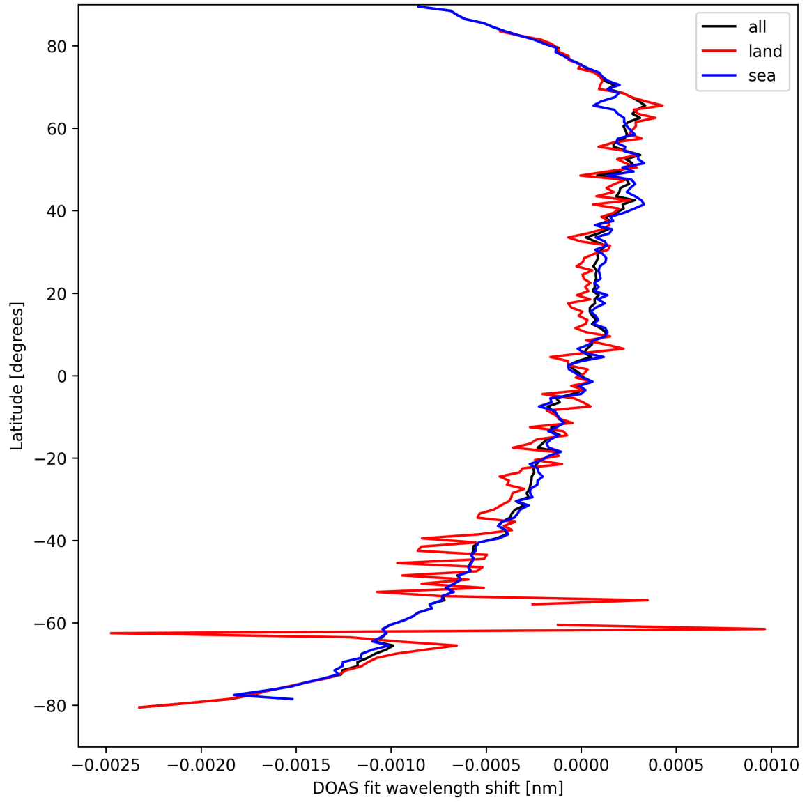
Figure 28: Zonal average of "DOAS fit wavelength shift" for 2025-04-02 to 2025-04-03.
