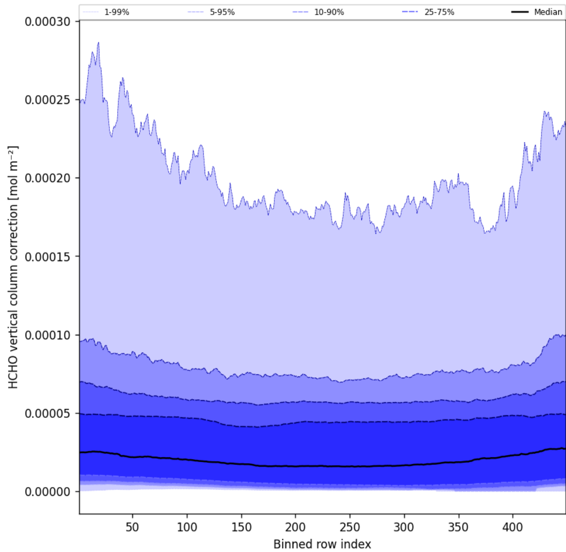
Figure 49: Along track statistics of “HCHO vertical column correction” for 2025-04-02 to 2025-04-03
