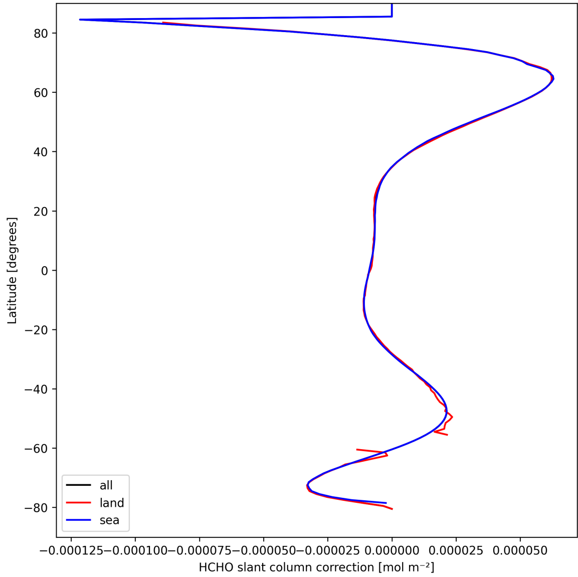
Figure 31: Zonal average of "HCHO slant column correction" for 2025-04-02 to 2025-04-03.
