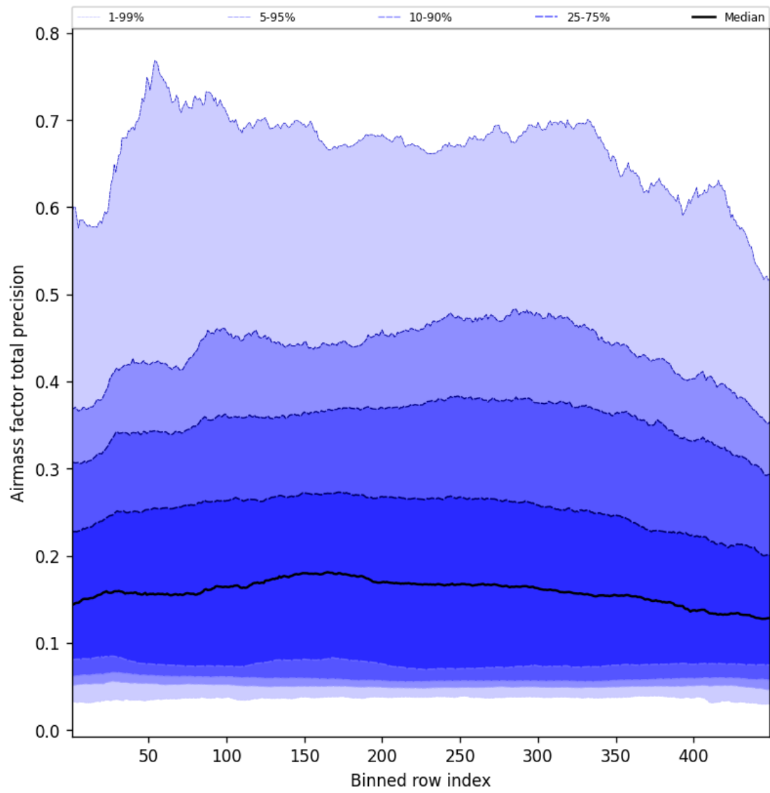
Figure 53: Along track statistics of “Airmass factor total precision” for 2025-04-02 to 2025-04-03
