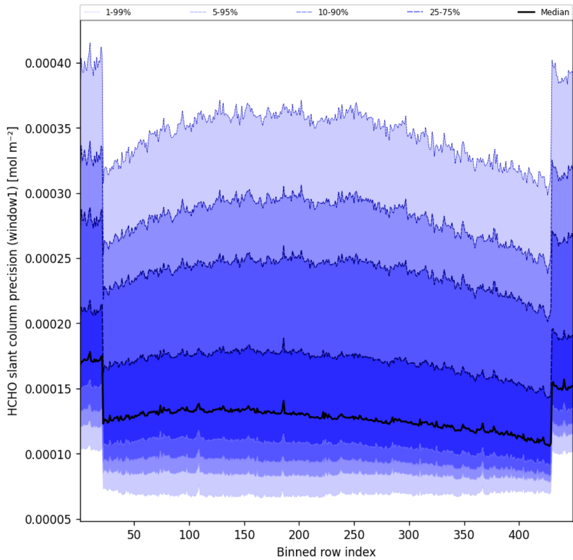
Figure 51: Along track statistics of “HCHO slant column precision (window1)” for 2025-04-02 to 2025-04-03
