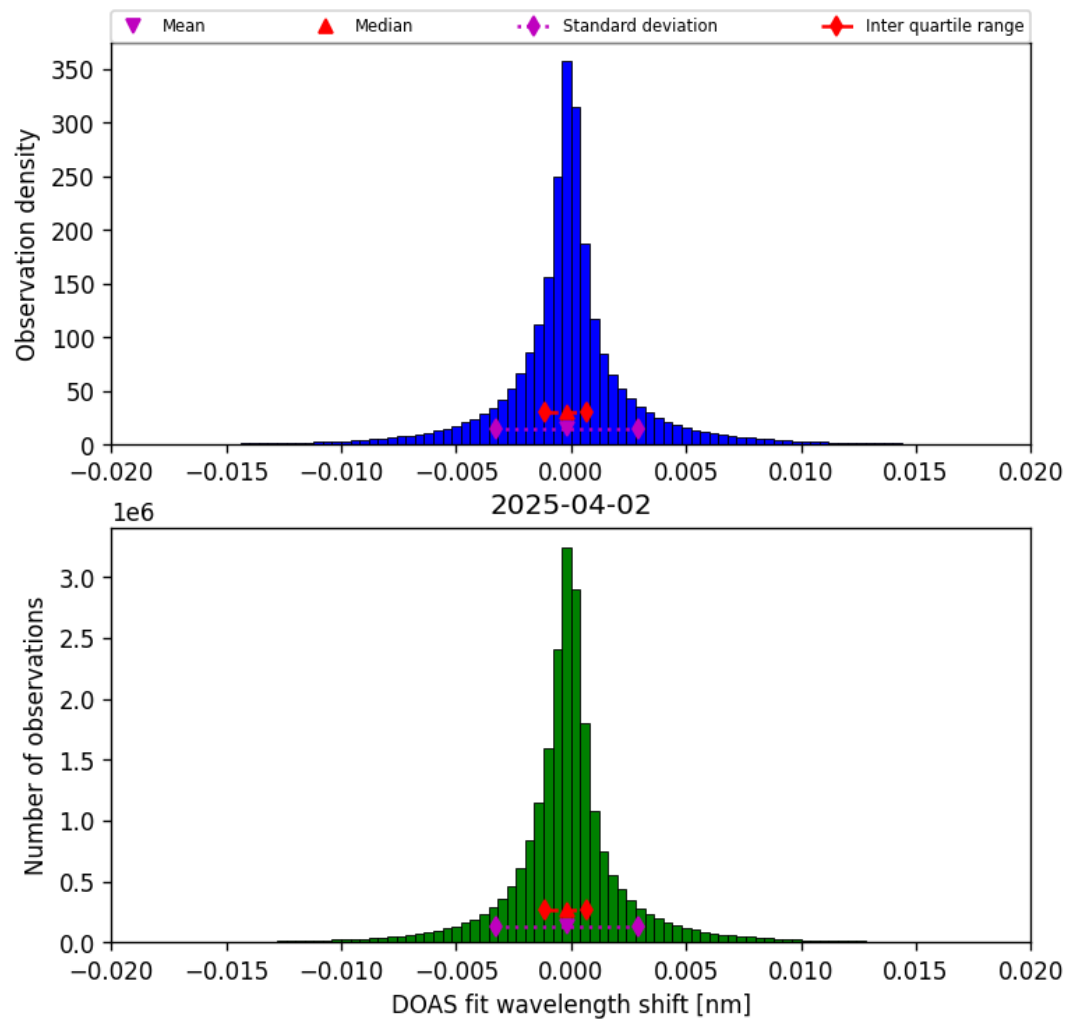
Figure 42: Histogram of “DOAS fit wavelength shift” for 2025-04-02 to 2025-04-03
