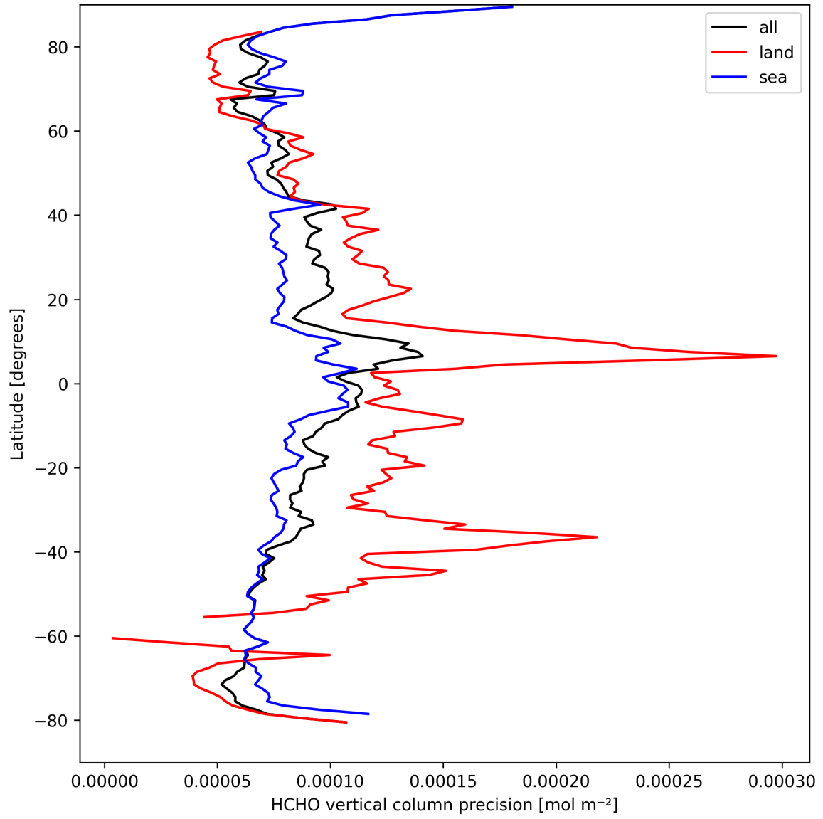
Figure 20: Zonal average of "HCHO vertical column precision" for 2025-04-02 to 2025-04-03.
