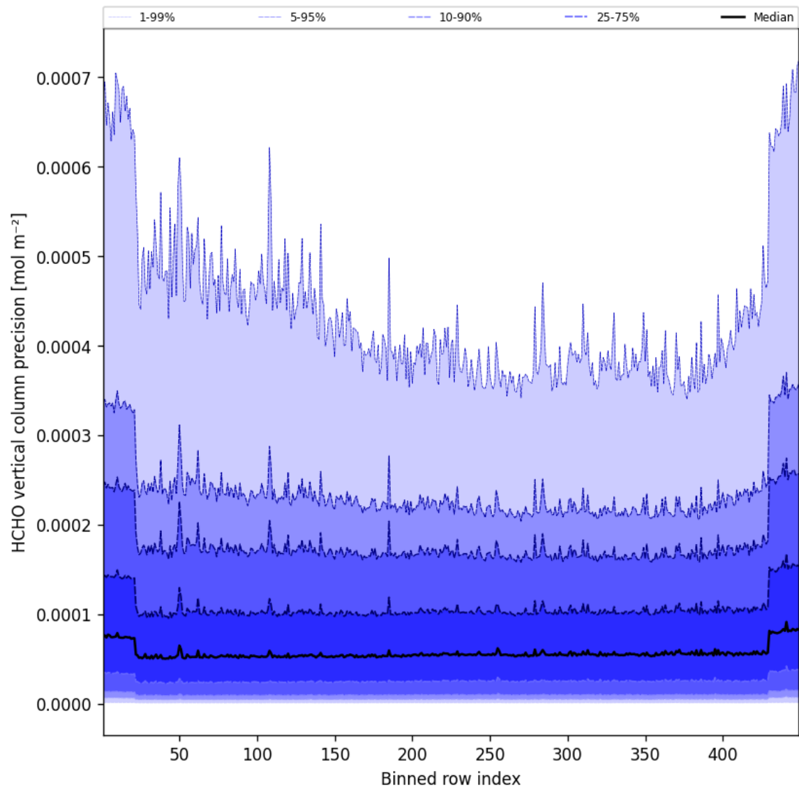
Figure 48: Along track statistics of “HCHO vertical column precision” for 2025-04-02 to 2025-04-03
