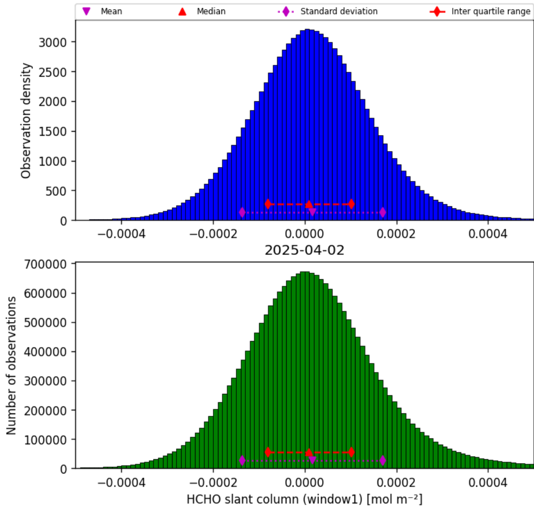
Figure 36: Histogram of “HCHO slant column (window1)” for 2025-04-02 to 2025-04-03
