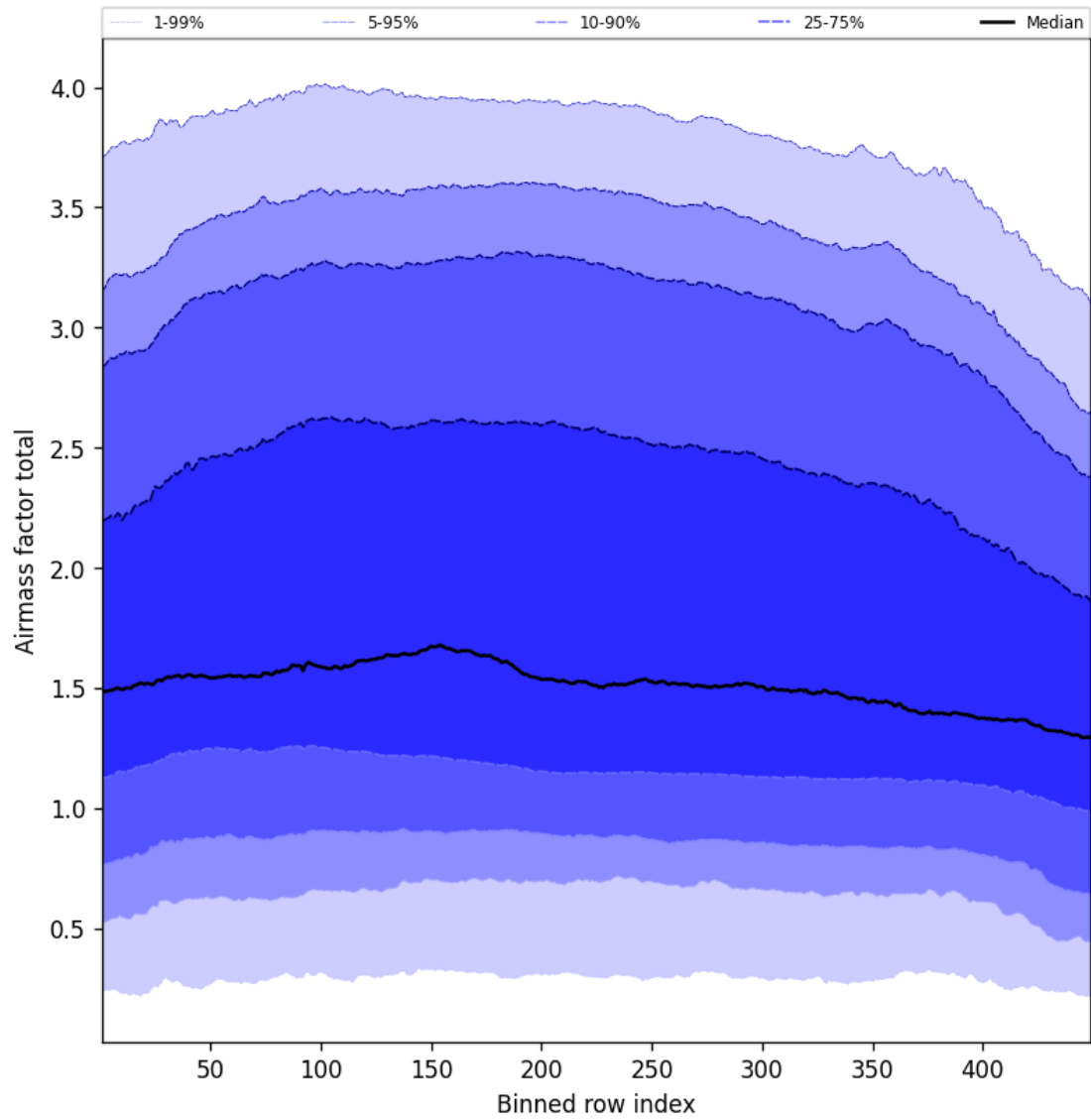
Figure 52: Along track statistics of “Airmass factor total” for 2025-04-02 to 2025-04-03
