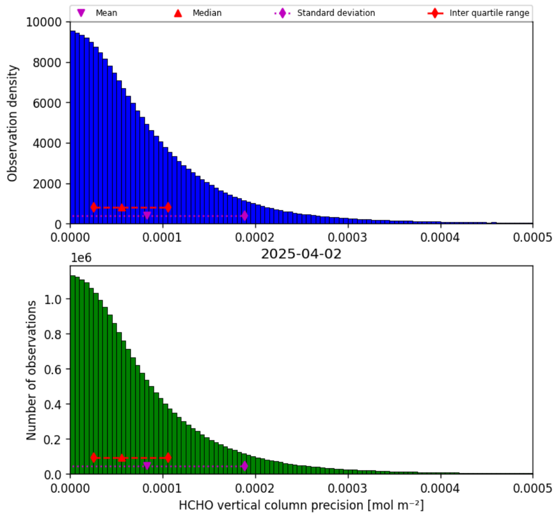
Figure 34: Histogram of “HCHO vertical column precision” for 2025-04-02 to 2025-04-03
