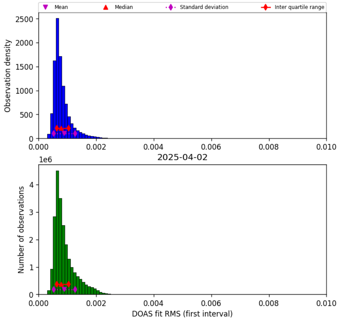
Figure 44: Histogram of “DOAS fit RMS (first interval)” for 2025-04-02 to 2025-04-03
