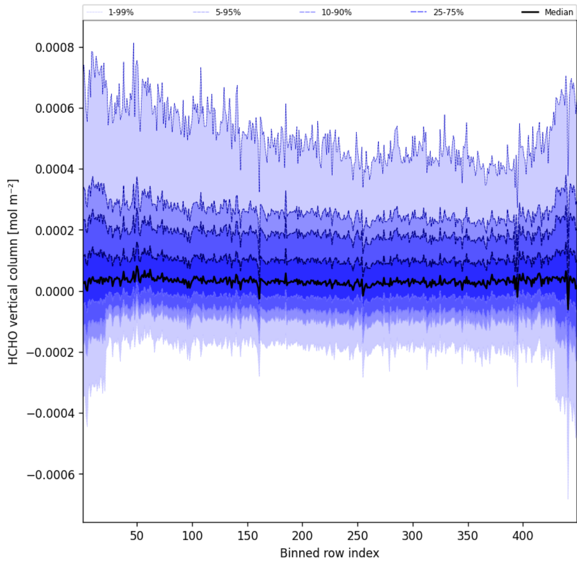
Figure 47: Along track statistics of “HCHO vertical column” for 2025-04-02 to 2025-04-03
