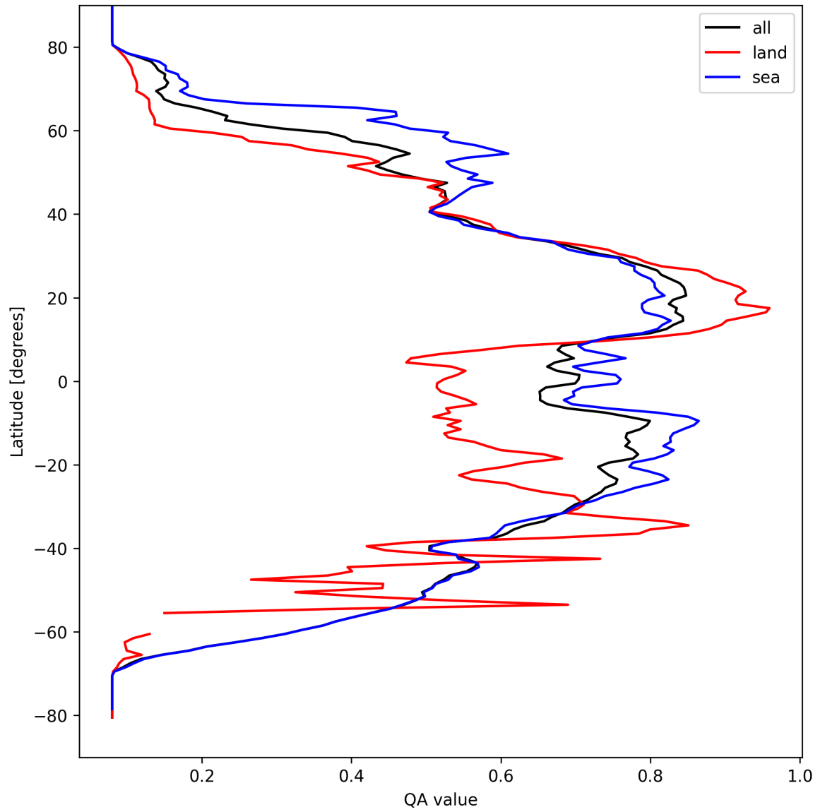
Figure 18: Zonal average of “QA value” for 2025-04-02 to 2025-04-03.
