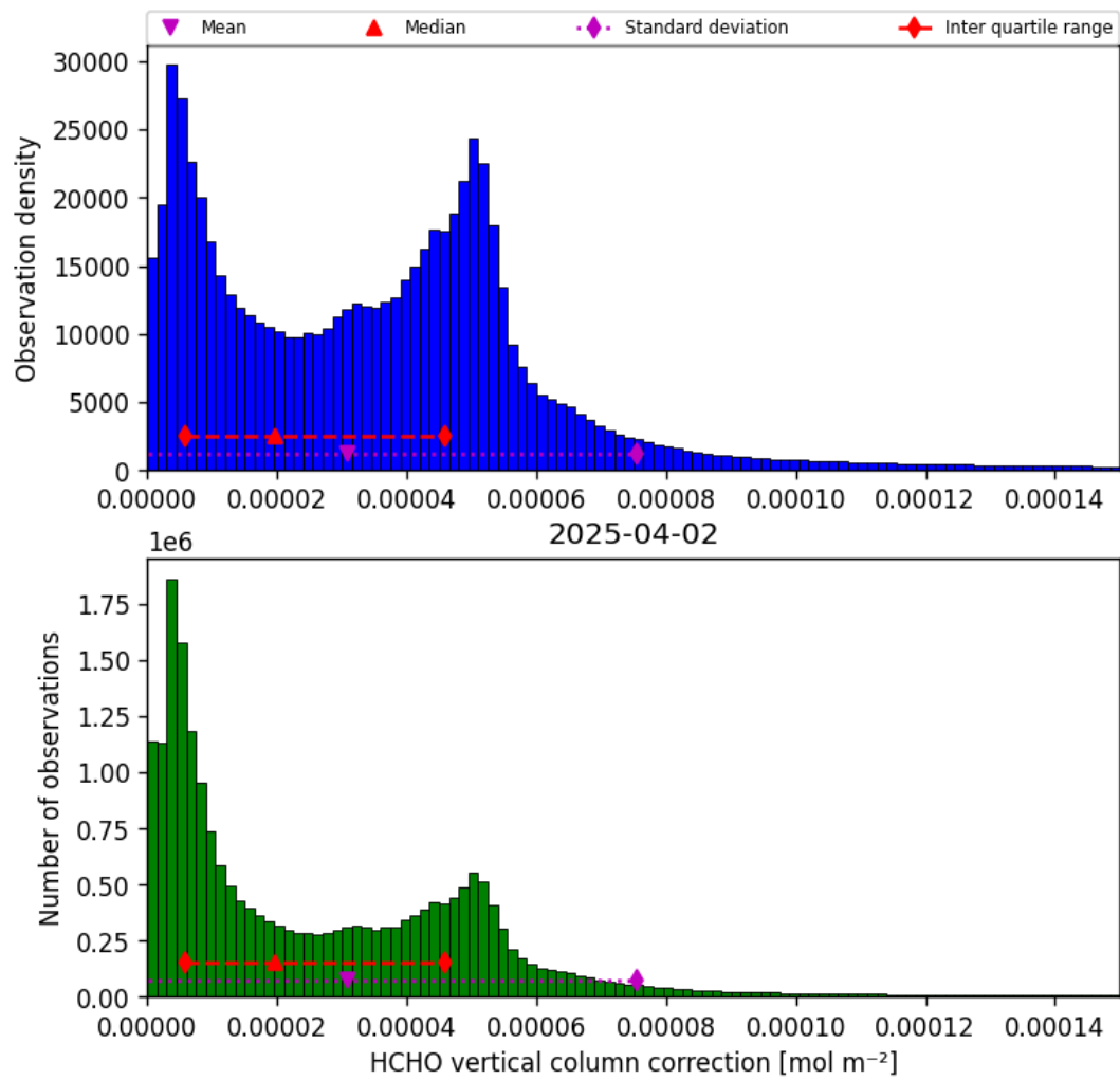
Figure 35: Histogram of “HCHO vertical column correction” for 2025-04-02 to 2025-04-03
