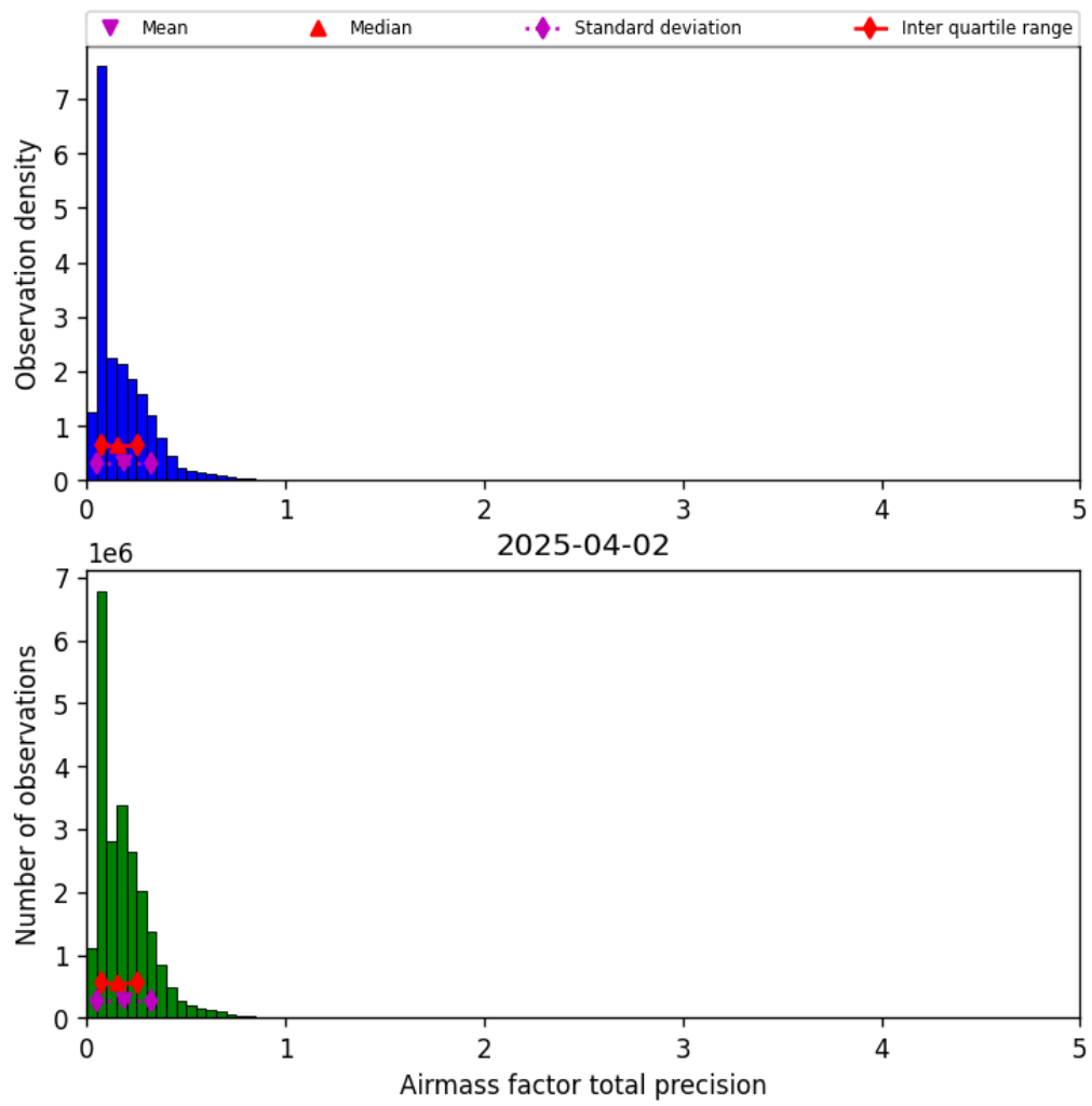
Figure 39: Histogram of “Airmass factor total precision” for 2025-04-02 to 2025-04-03
