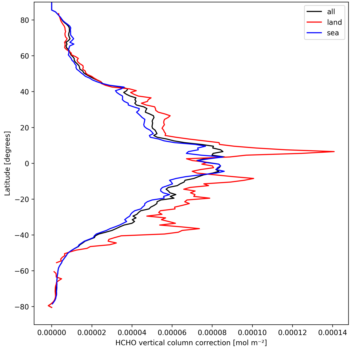
Figure 21: Zonal average of “HCHO vertical column correction” for 2025-04-02 to 2025-04-03.
