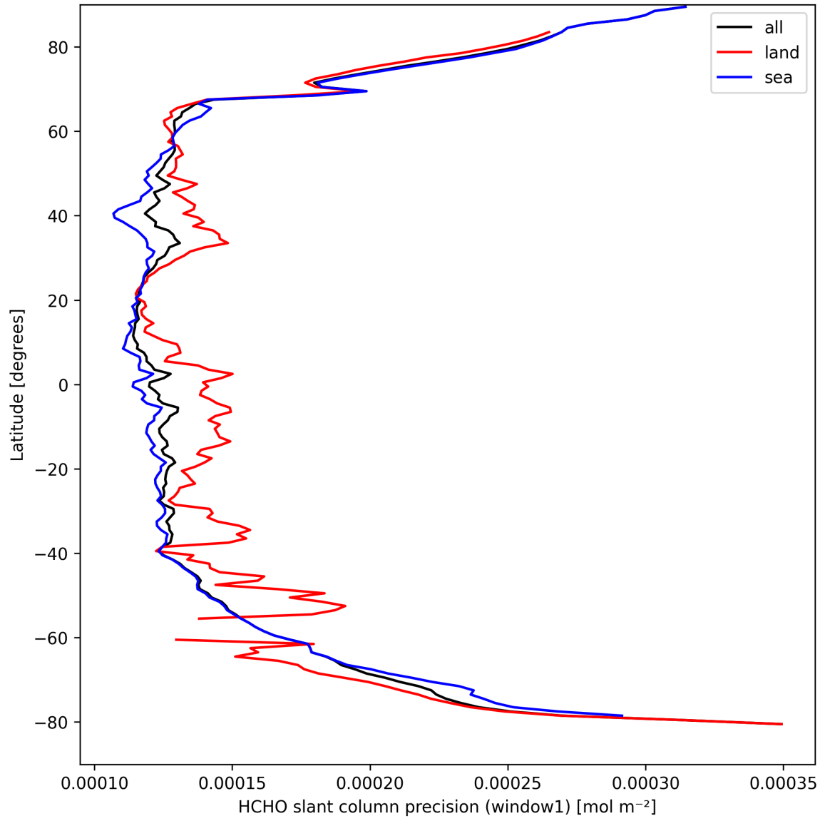
Figure 23: Zonal average of “HCHO slant column precision (window1)” for 2025-04-02 to 2025-04-03.
