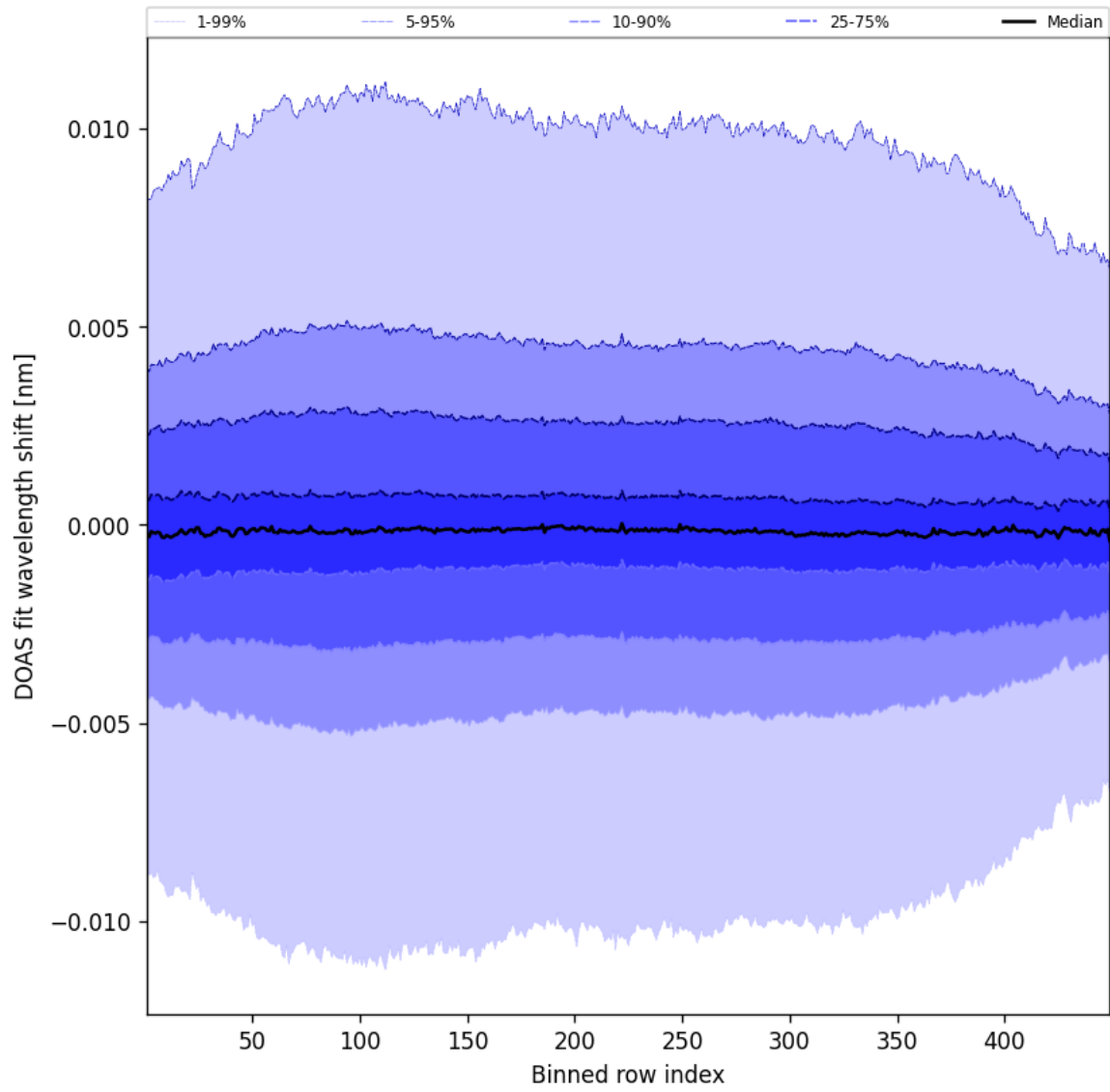
Figure 56: Along track statistics of “DOAS fit wavelength shift” for 2025-04-02 to 2025-04-03
