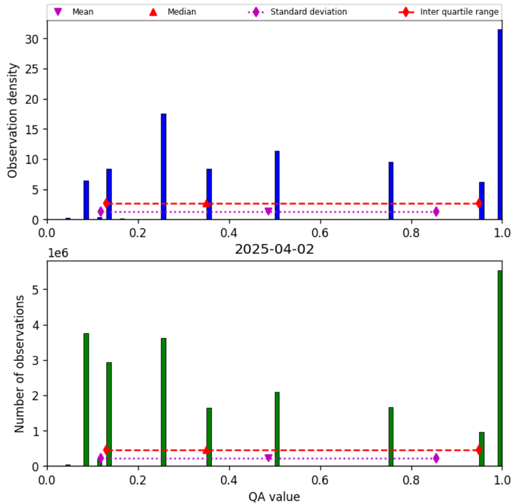
Figure 32: Histogram of “QA value” for 2025-04-02 to 2025-04-03
