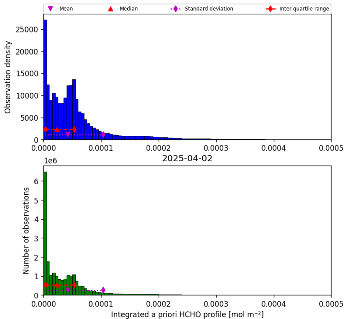
Figure 41: Histogram of “Integrated a priori HCHO profile” for 2025-04-02 to 2025-04-03
