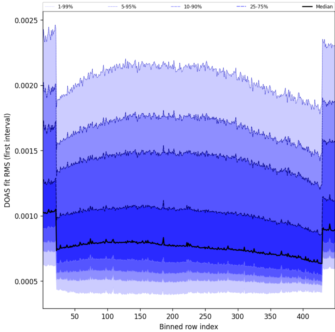
Figure 58: Along track statistics of “DOAS fit RMS (first interval)” for 2025-04-02 to 2025-04-03
