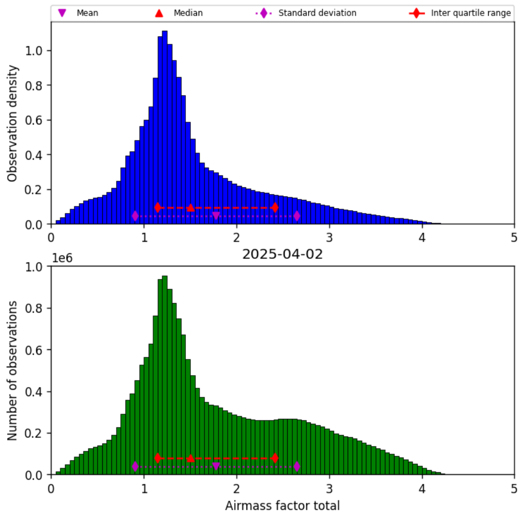
Figure 38: Histogram of “Airmass factor total” for 2025-04-02 to 2025-04-03
