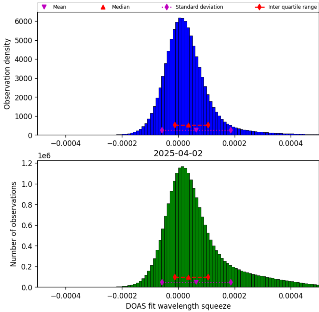
Figure 43: Histogram of “DOAS fit wavelength squeeze” for 2025-04-02 to 2025-04-03
