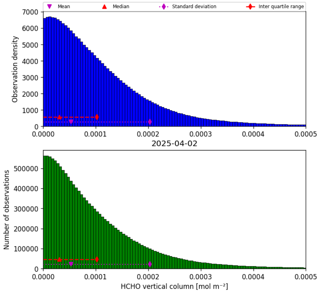
Figure 33: Histogram of “HCHO vertical column” for 2025-04-02 to 2025-04-03
