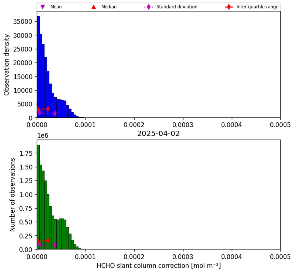
Figure 45: Histogram of “HCHO slant column correction” for 2025-04-02 to 2025-04-03
