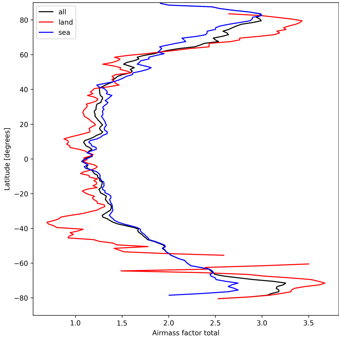
Figure 24: Zonal average of “Airmass factor total” for 2025-04-02 to 2025-04-03.
