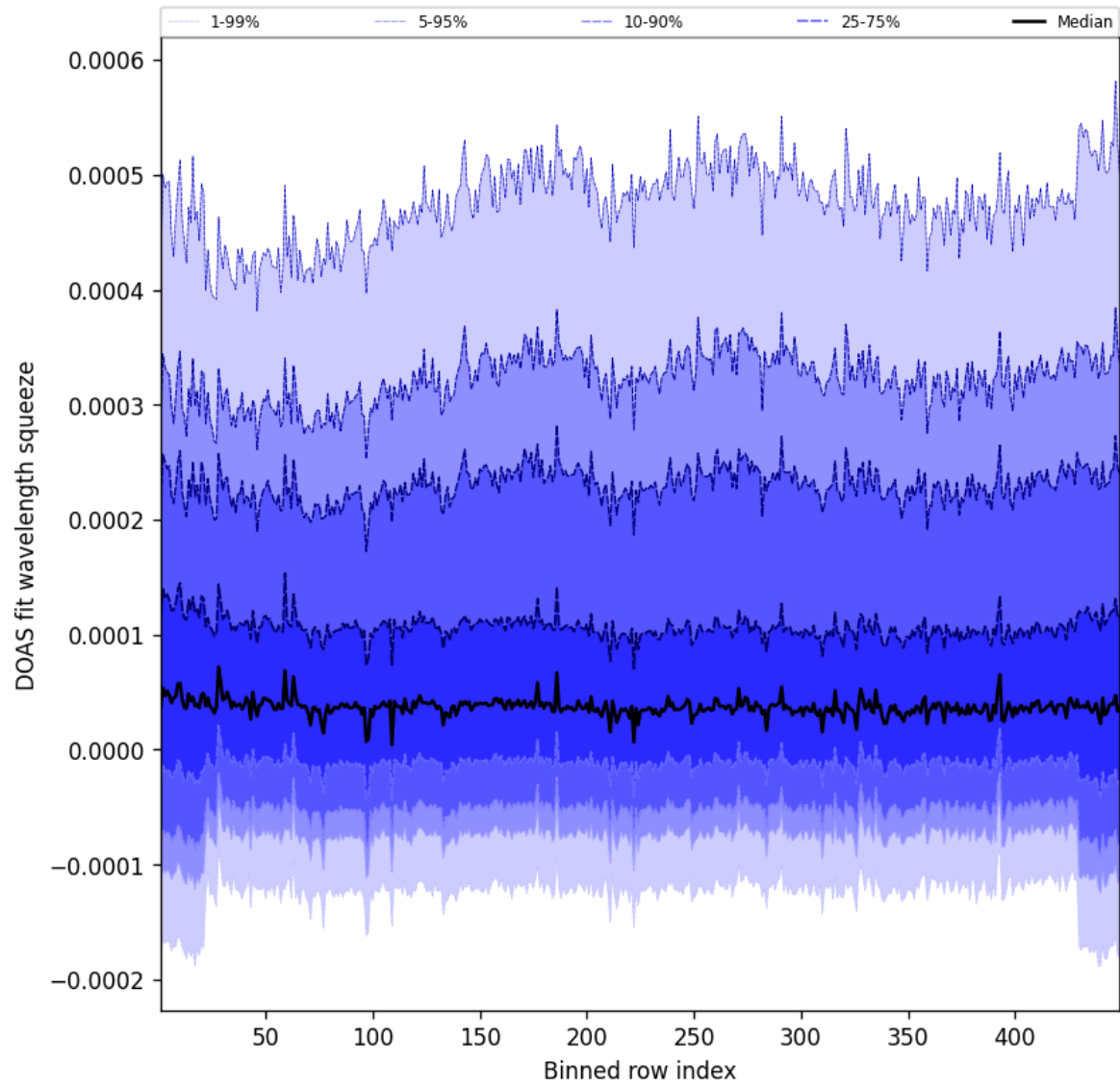
Figure 57: Along track statistics of “DOAS fit wavelength squeeze” for 2025-04-02 to 2025-04-03
