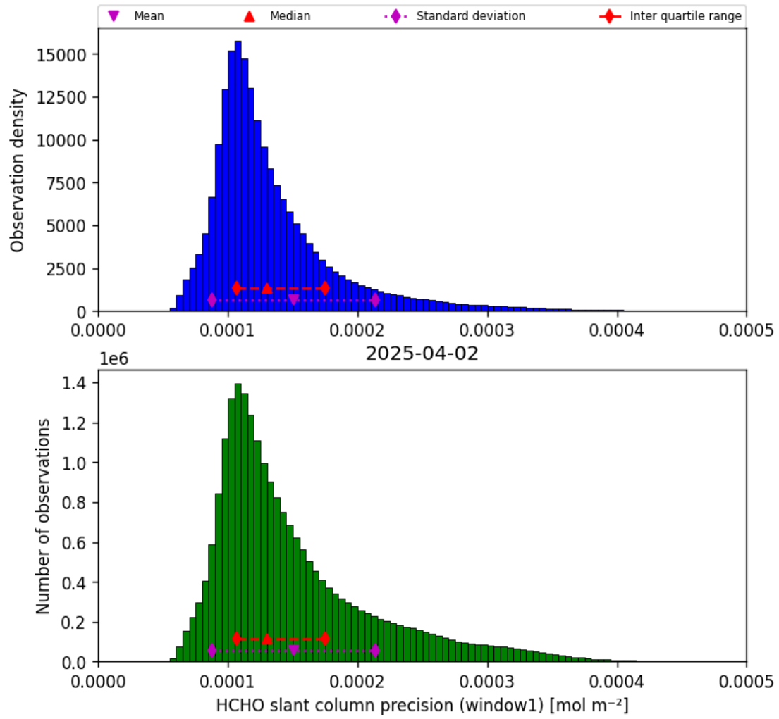
Figure 37: Histogram of “HCHO slant column precision (window1)” for 2025-04-02 to 2025-04-03
