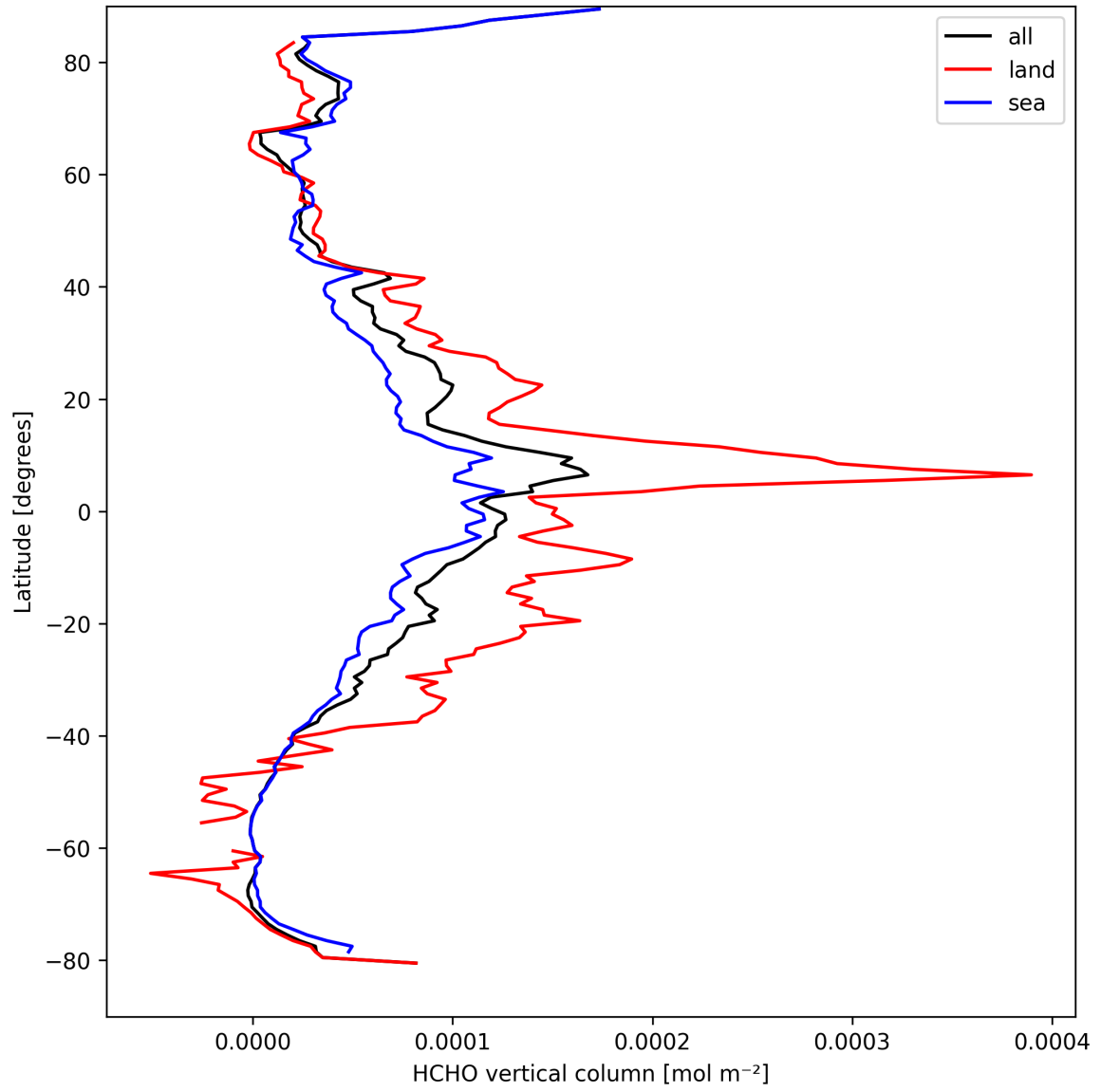
Figure 19: Zonal average of “HCHO vertical column” for 2025-04-02 to 2025-04-03.
