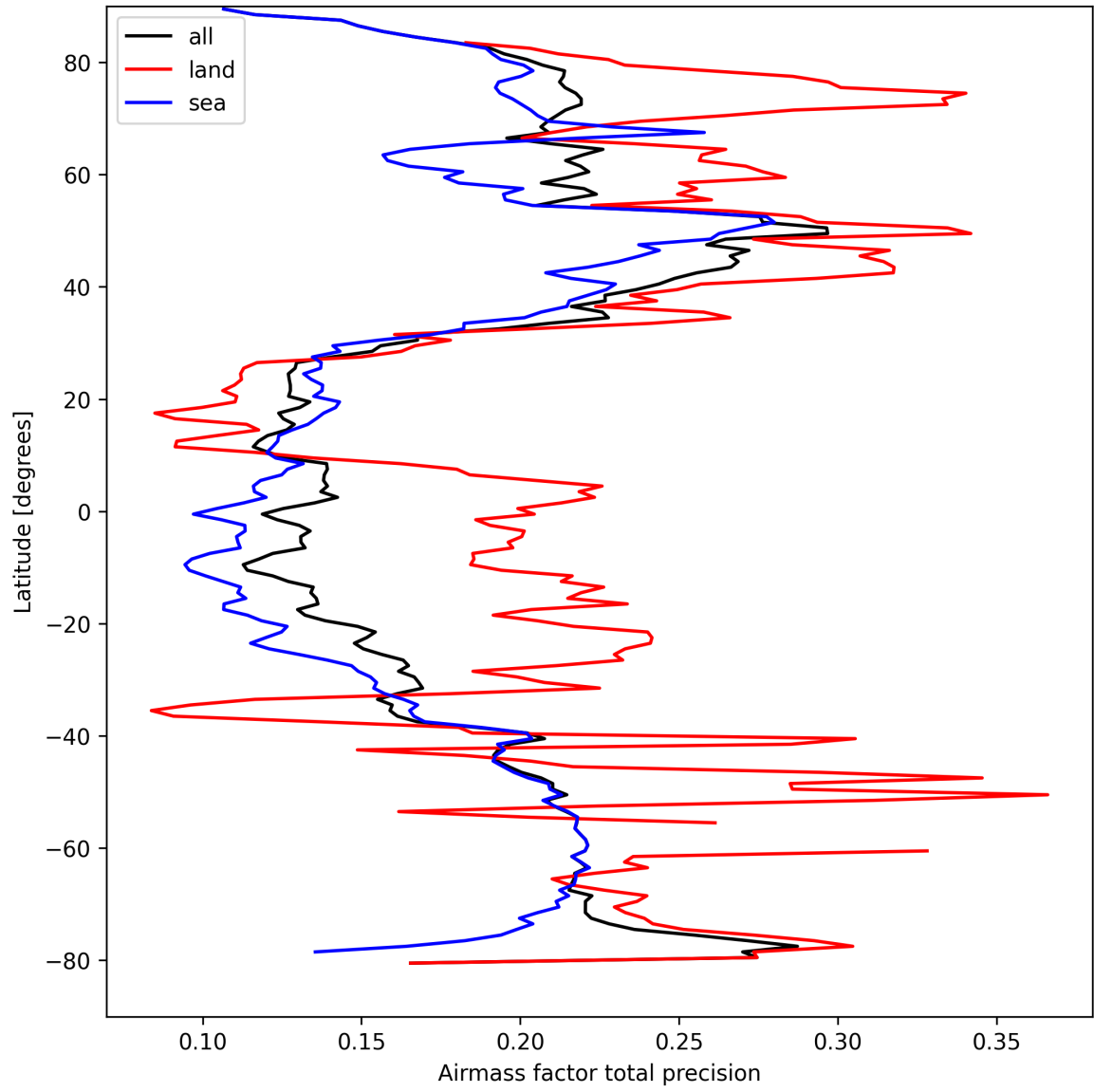
Figure 25: Zonal average of “Airmass factor total precision” for 2025-04-02 to 2025-04-03.
