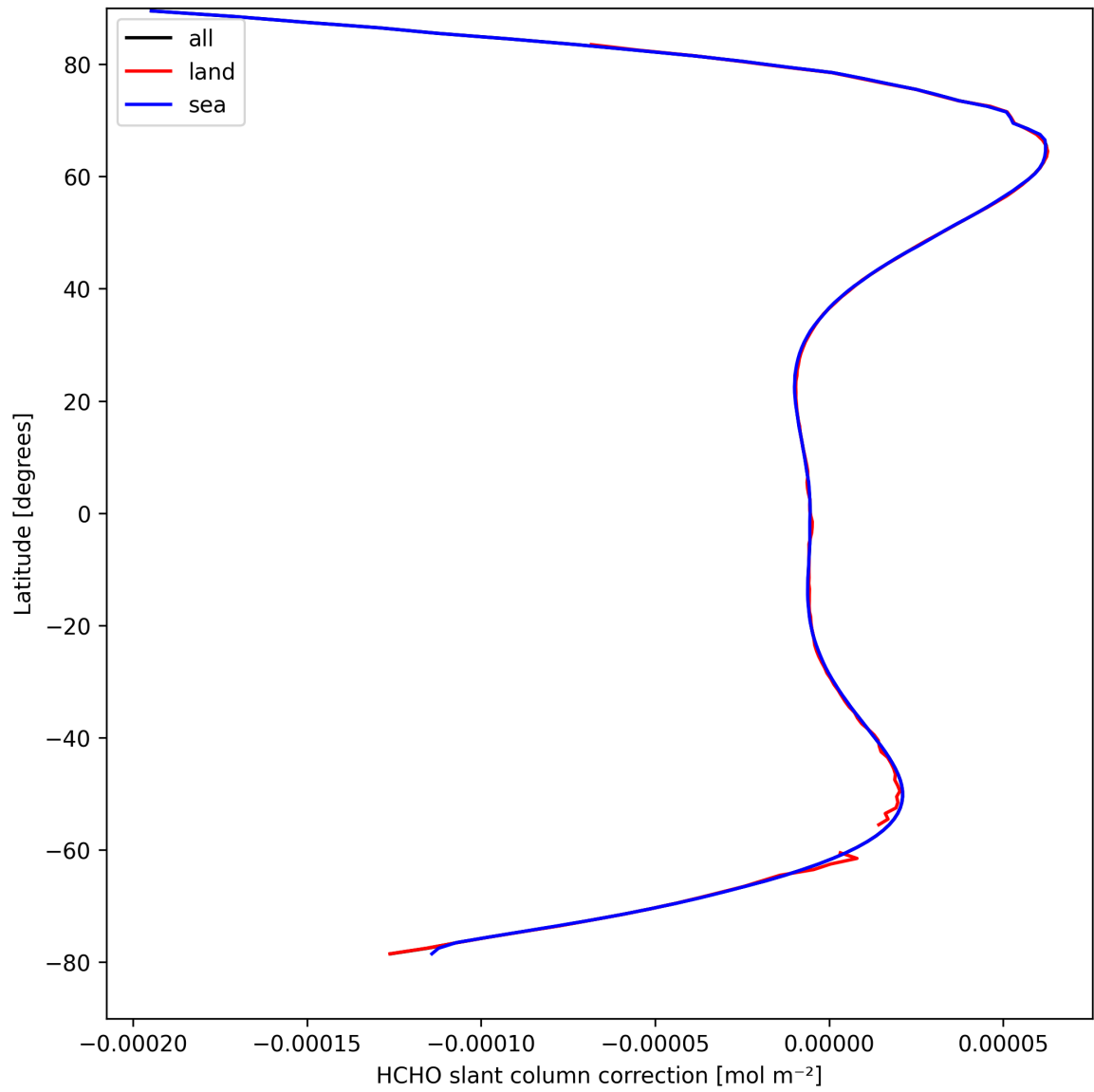
Figure 31: Zonal average of “HCHO slant column correction” for 2025-04-05 to 2025-04-06.
