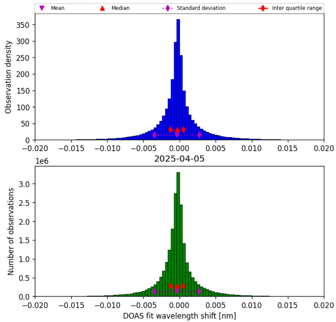
Figure 42: Histogram of “DOAS fit wavelength shift” for 2025-04-05 to 2025-04-06
