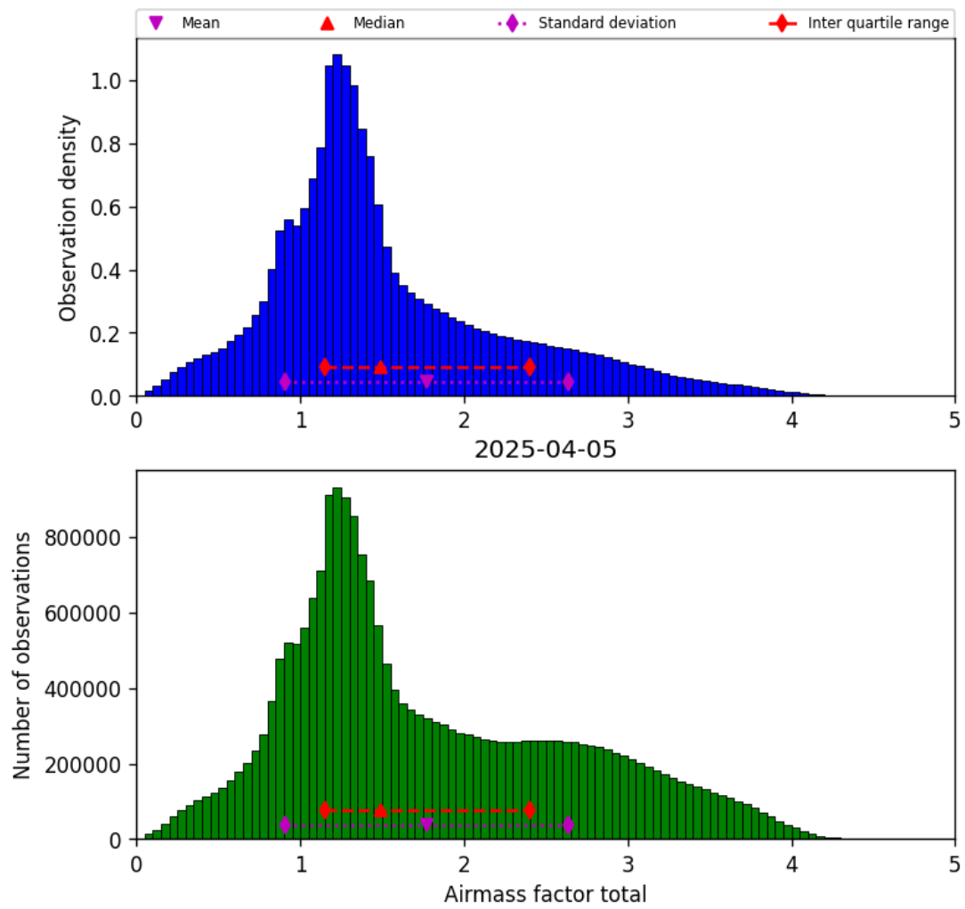
Figure 38: Histogram of “Airmass factor total” for 2025-04-05 to 2025-04-06
