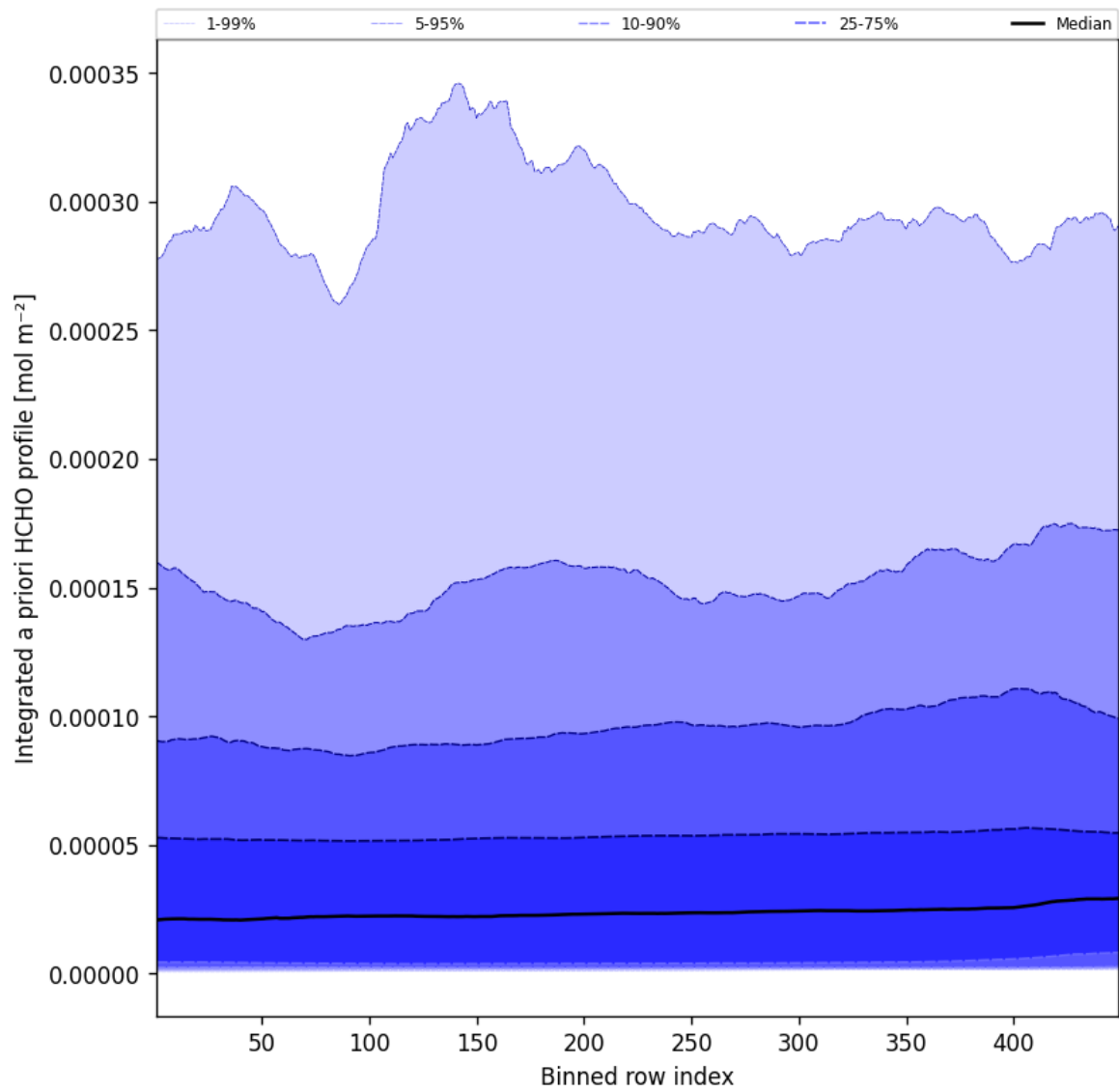
Figure 55: Along track statistics of "Integrated a priori HCHO profile" for 2025-04-05 to 2025-04-06
