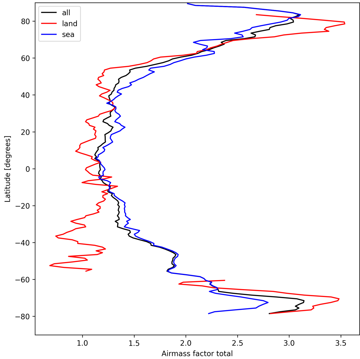
Figure 24: Zonal average of “Airmass factor total” for 2025-04-05 to 2025-04-06.
