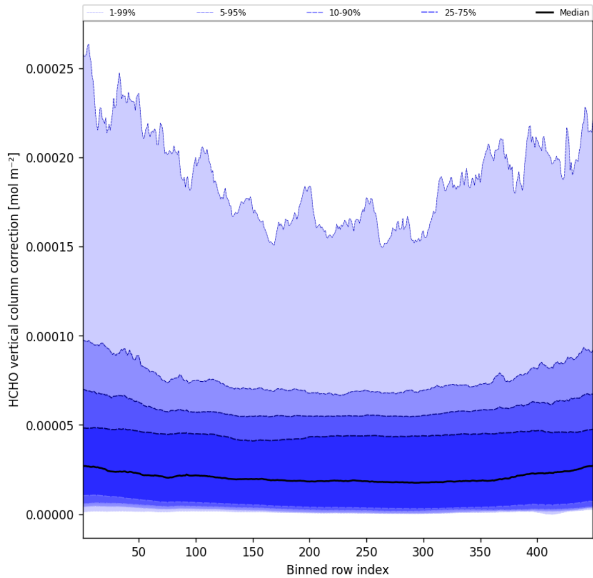
Figure 49: Along track statistics of “HCHO vertical column correction” for 2025-04-05 to 2025-04-06
