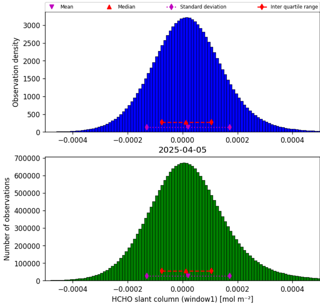
Figure 36: Histogram of “HCHO slant column (window1)” for 2025-04-05 to 2025-04-06
