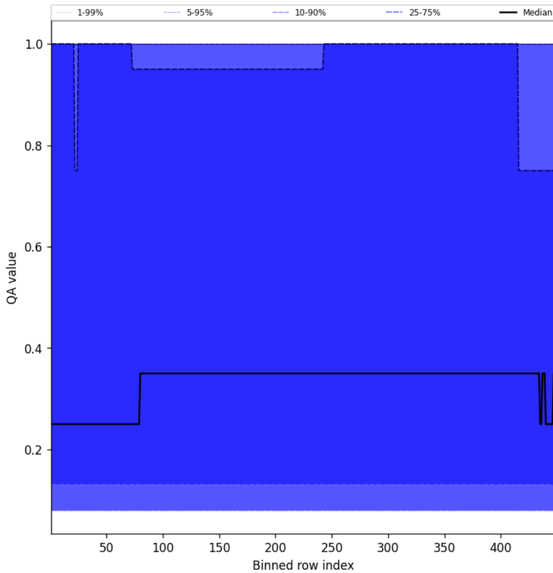
Figure 46: Along track statistics of “QA value” for 2025-04-05 to 2025-04-06
