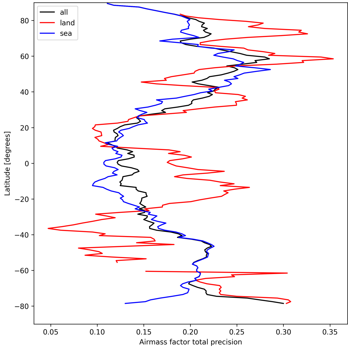
Figure 25: Zonal average of “Airmass factor total precision” for 2025-04-05 to 2025-04-06.
