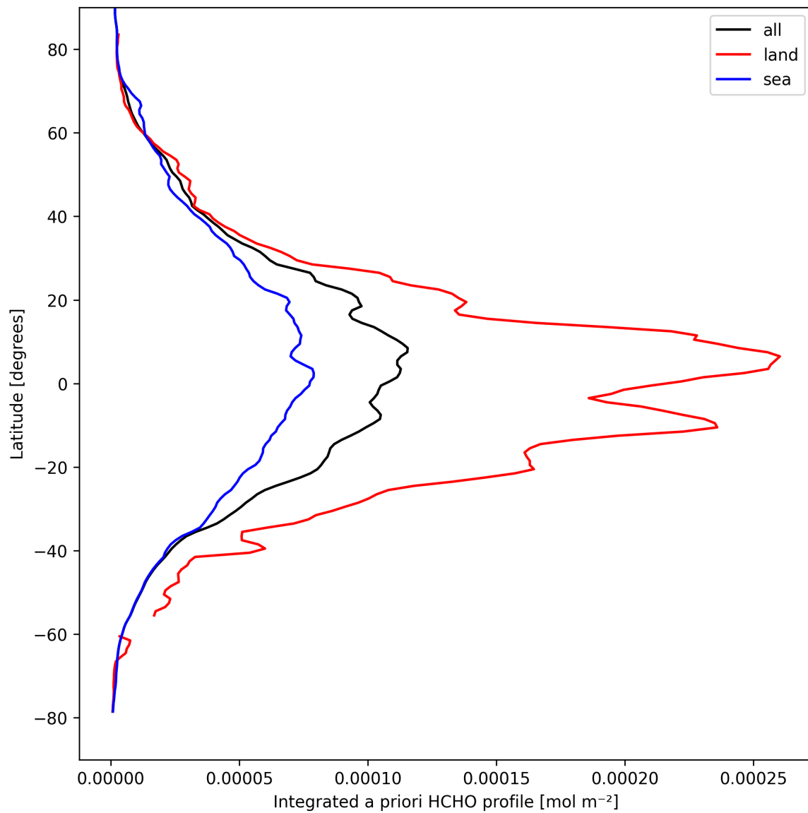
Figure 27: Zonal average of “Integrated a priori HCHO profile” for 2025-04-05 to 2025-04-06.
