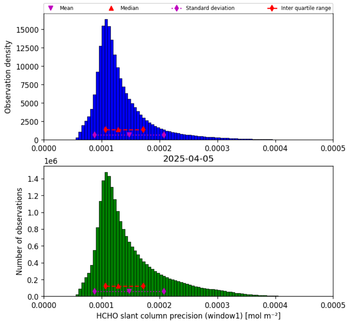
Figure 37: Histogram of “HCHO slant column precision (window1)” for 2025-04-05 to 2025-04-06
