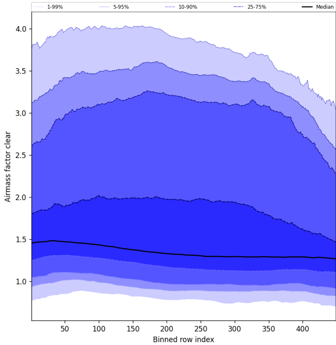
Figure 54: Along track statistics of “Airmass factor clear” for 2025-04-05 to 2025-04-06
