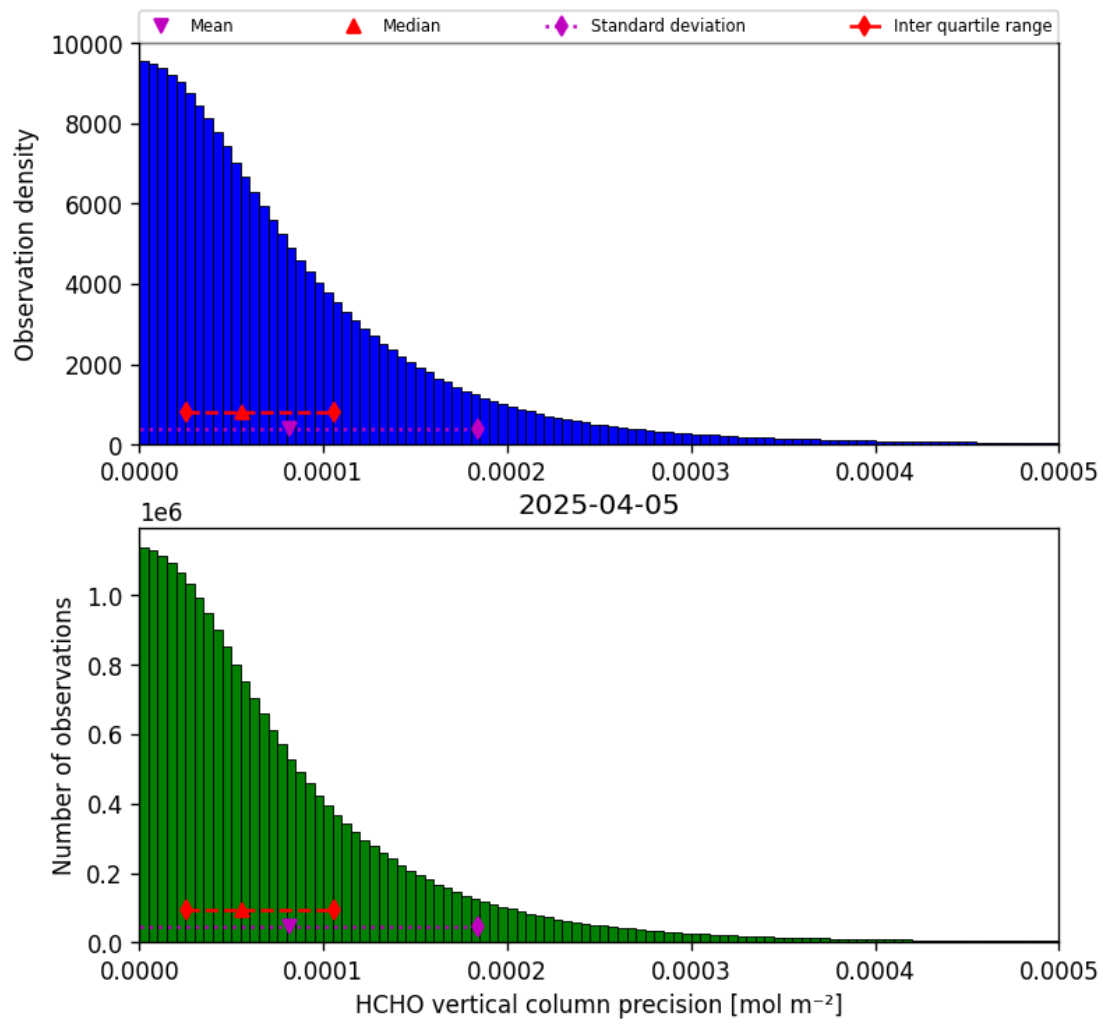
Figure 34: Histogram of “HCHO vertical column precision” for 2025-04-05 to 2025-04-06
