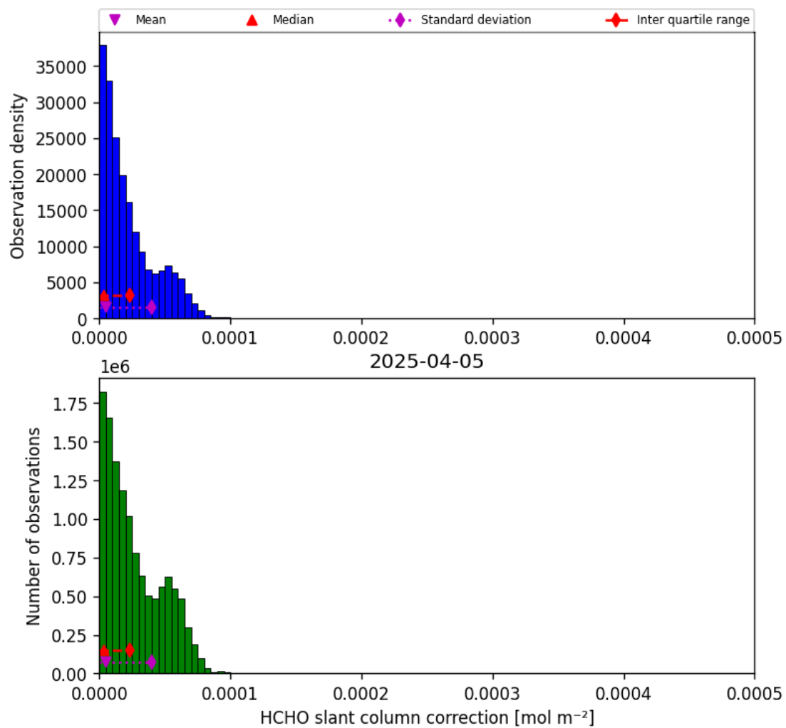
Figure 45: Histogram of “HCHO slant column correction” for 2025-04-05 to 2025-04-06
