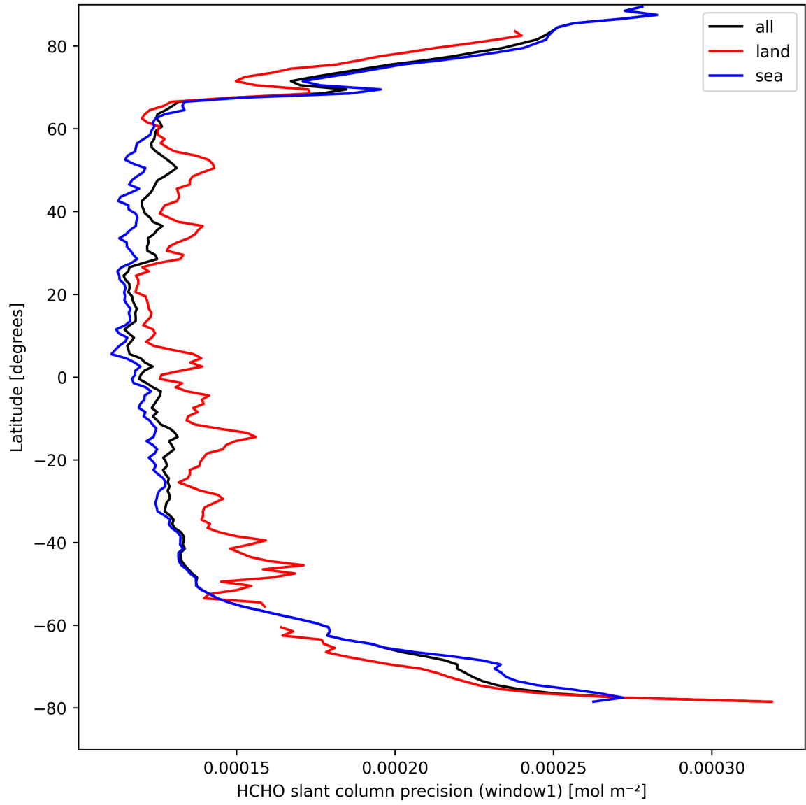
Figure 23: Zonal average of “HCHO slant column precision (window1)” for 2025-04-05 to 2025-04-06.
