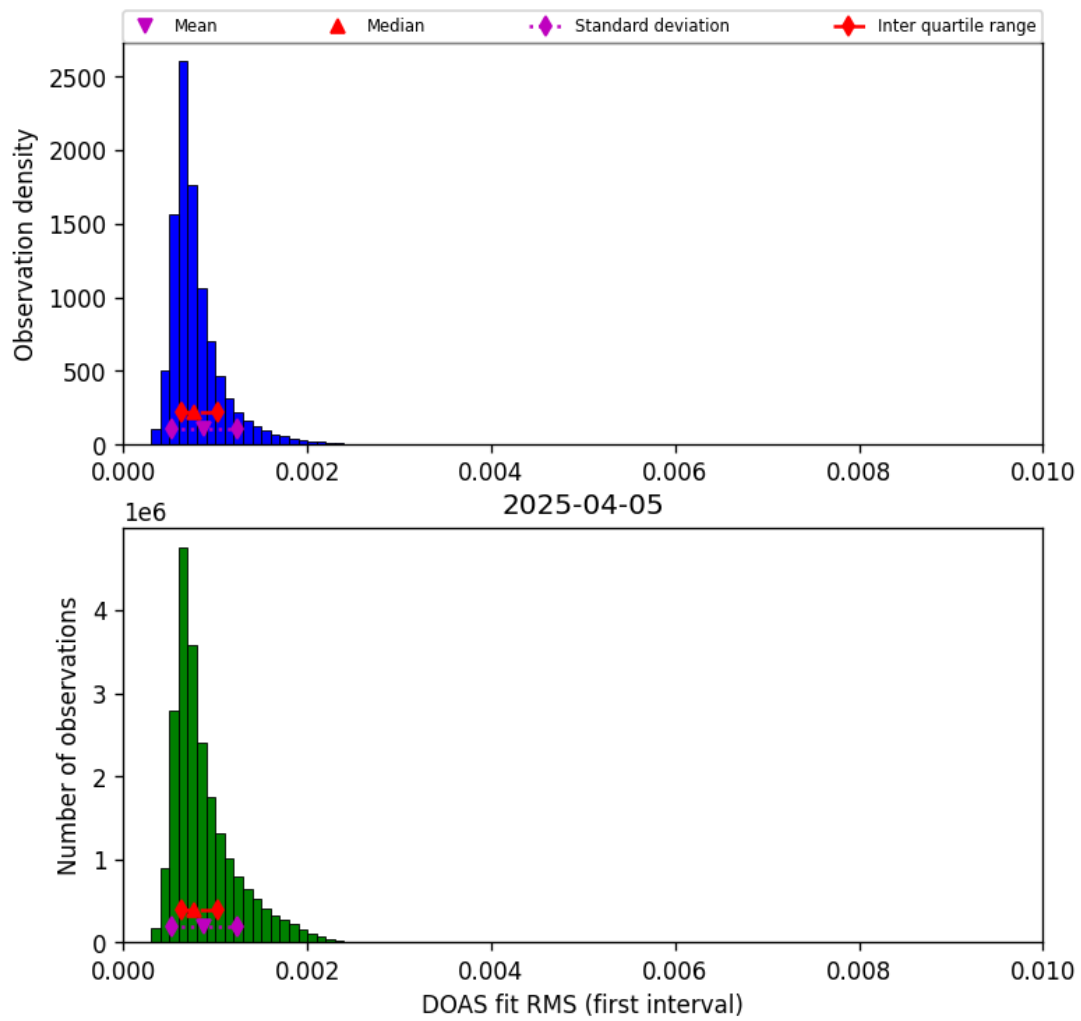
Figure 44: Histogram of “DOAS fit RMS (first interval)” for 2025-04-05 to 2025-04-06
