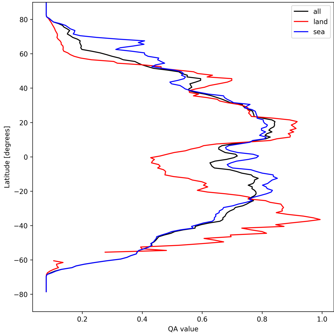
Figure 18: Zonal average of “QA value” for 2025-04-05 to 2025-04-06.
