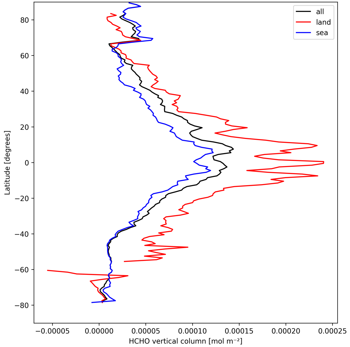
Figure 19: Zonal average of “HCHO vertical column” for 2025-04-05 to 2025-04-06.
