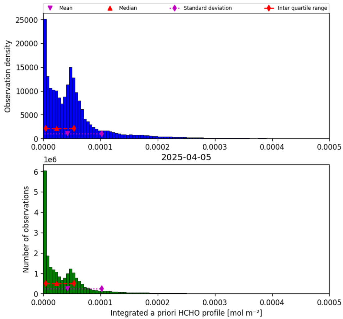
Figure 41: Histogram of “Integrated a priori HCHO profile” for 2025-04-05 to 2025-04-06
