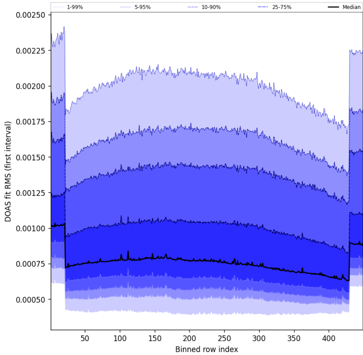
Figure 58: Along track statistics of “DOAS fit RMS (first interval)” for 2025-04-05 to 2025-04-06
