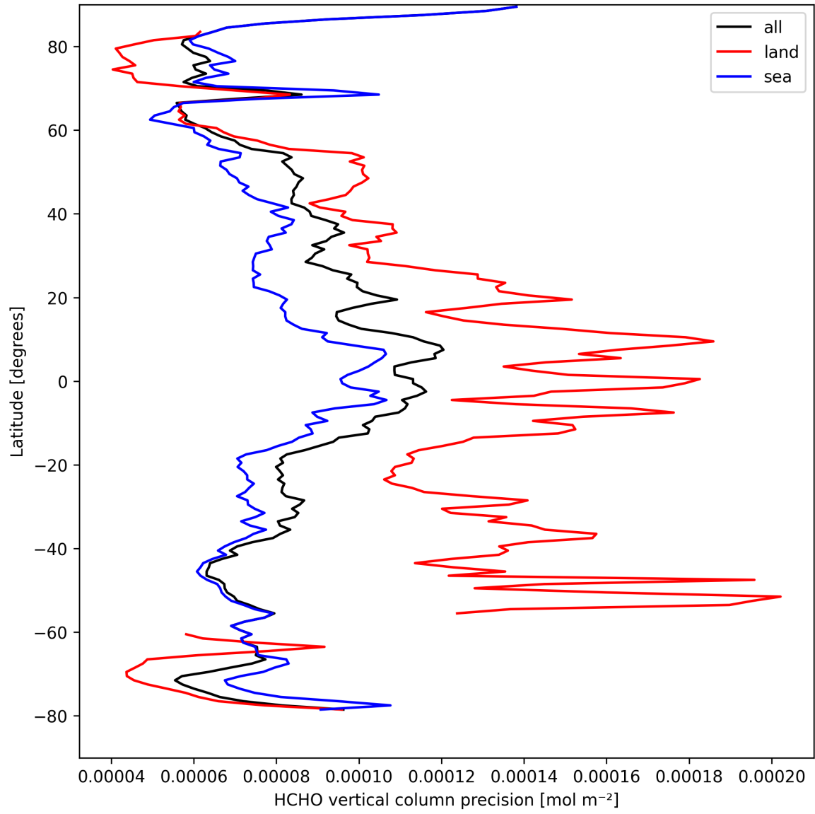
Figure 20: Zonal average of “HCHO vertical column precision” for 2025-04-05 to 2025-04-06.
