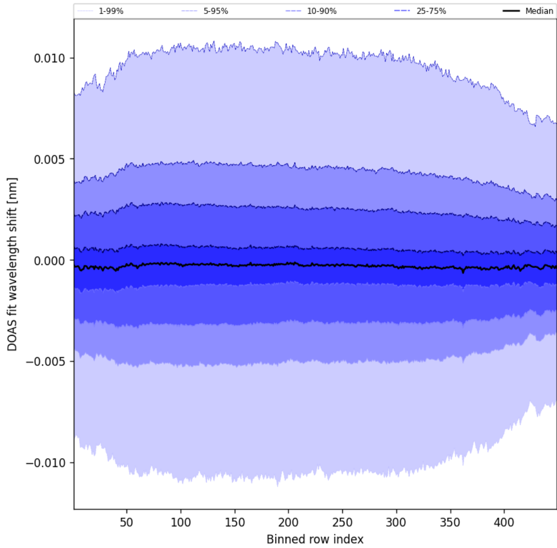
Figure 56: Along track statistics of “DOAS fit wavelength shift” for 2025-04-05 to 2025-04-06
