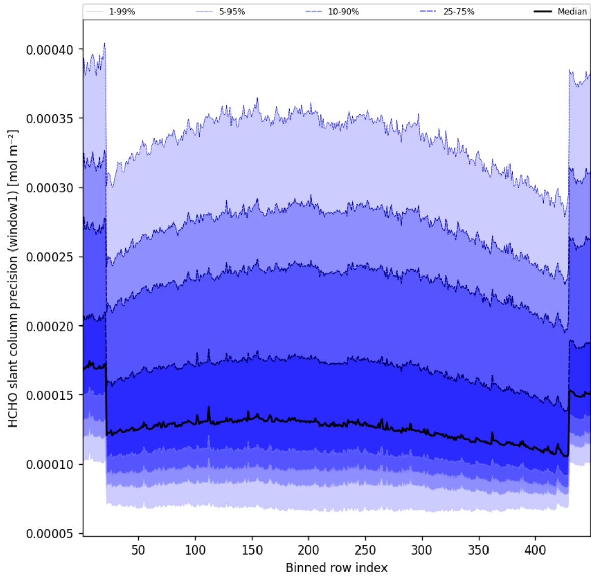
Figure 51: Along track statistics of “HCHO slant column precision (window1)” for 2025-04-05 to 2025-04-06
