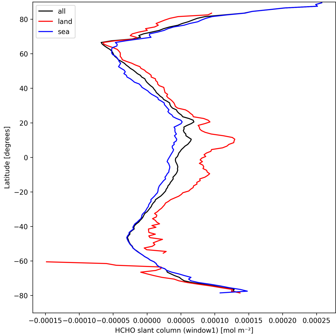
Figure 22: Zonal average of “HCHO slant column (window1)” for 2025-04-05 to 2025-04-06.
