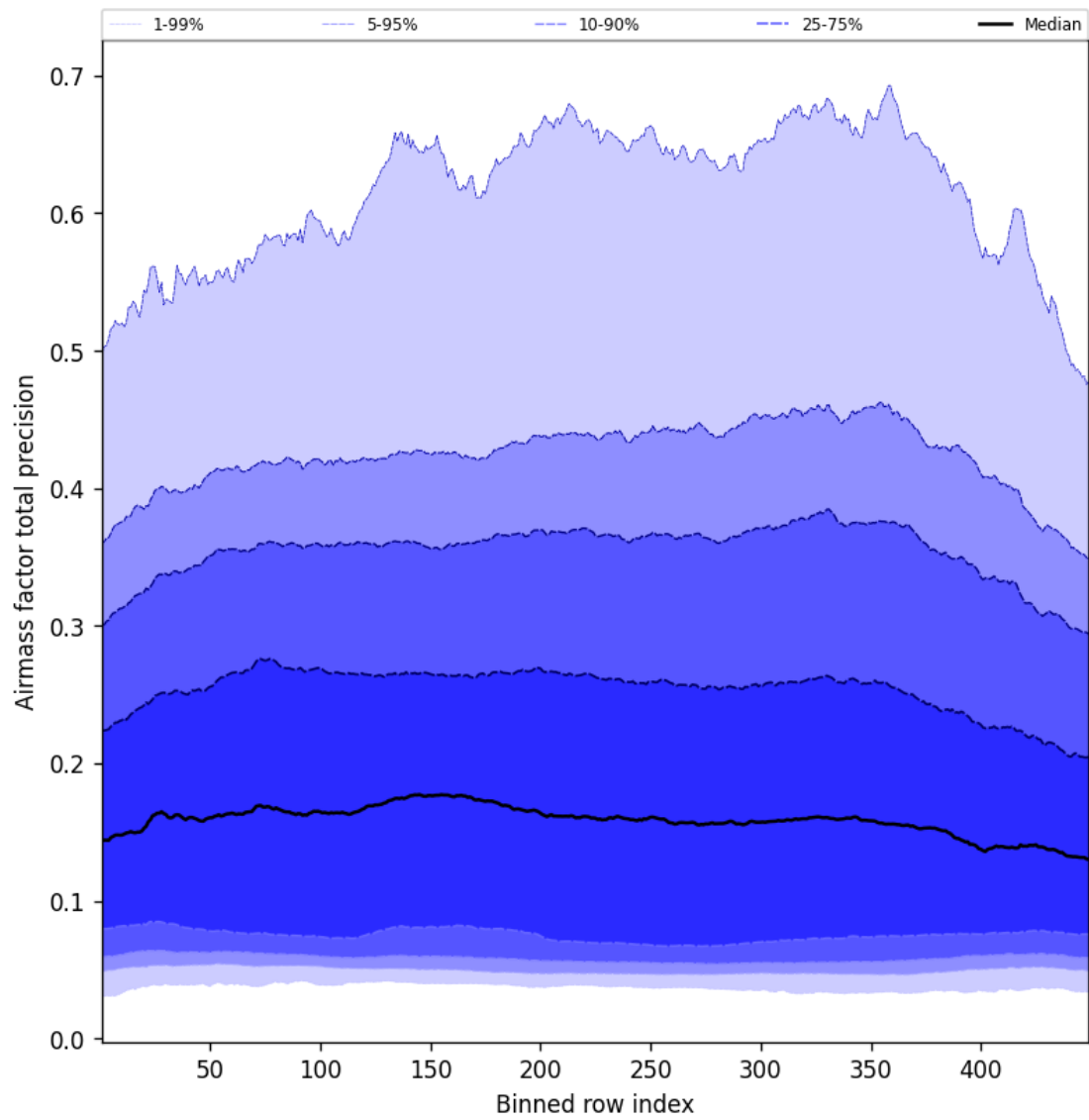
Figure 53: Along track statistics of “Airmass factor total precision” for 2025-04-05 to 2025-04-06
