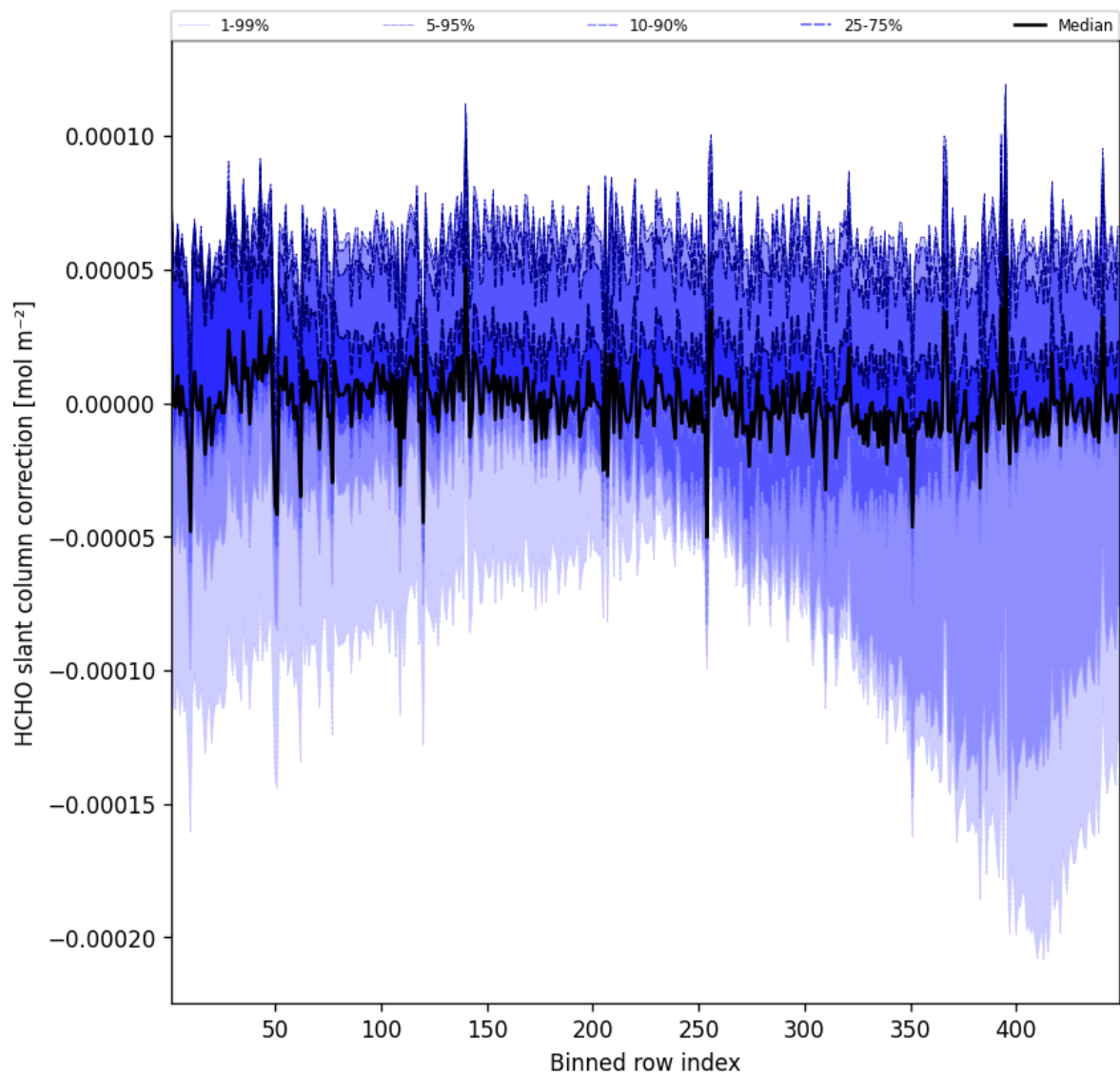
Figure 59: Along track statistics of “HCHO slant column correction” for 2025-04-05 to 2025-04-06
