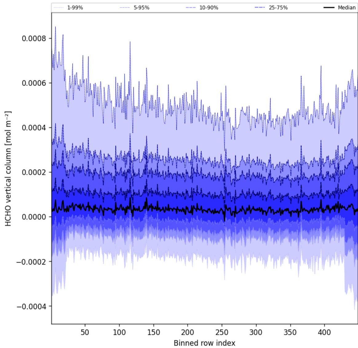
Figure 47: Along track statistics of “HCHO vertical column” for 2025-04-05 to 2025-04-06
