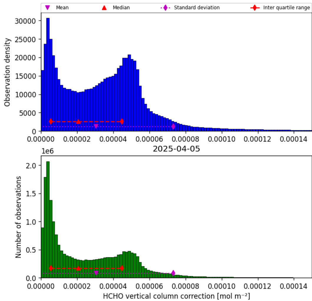
Figure 35: Histogram of “HCHO vertical column correction” for 2025-04-05 to 2025-04-06
