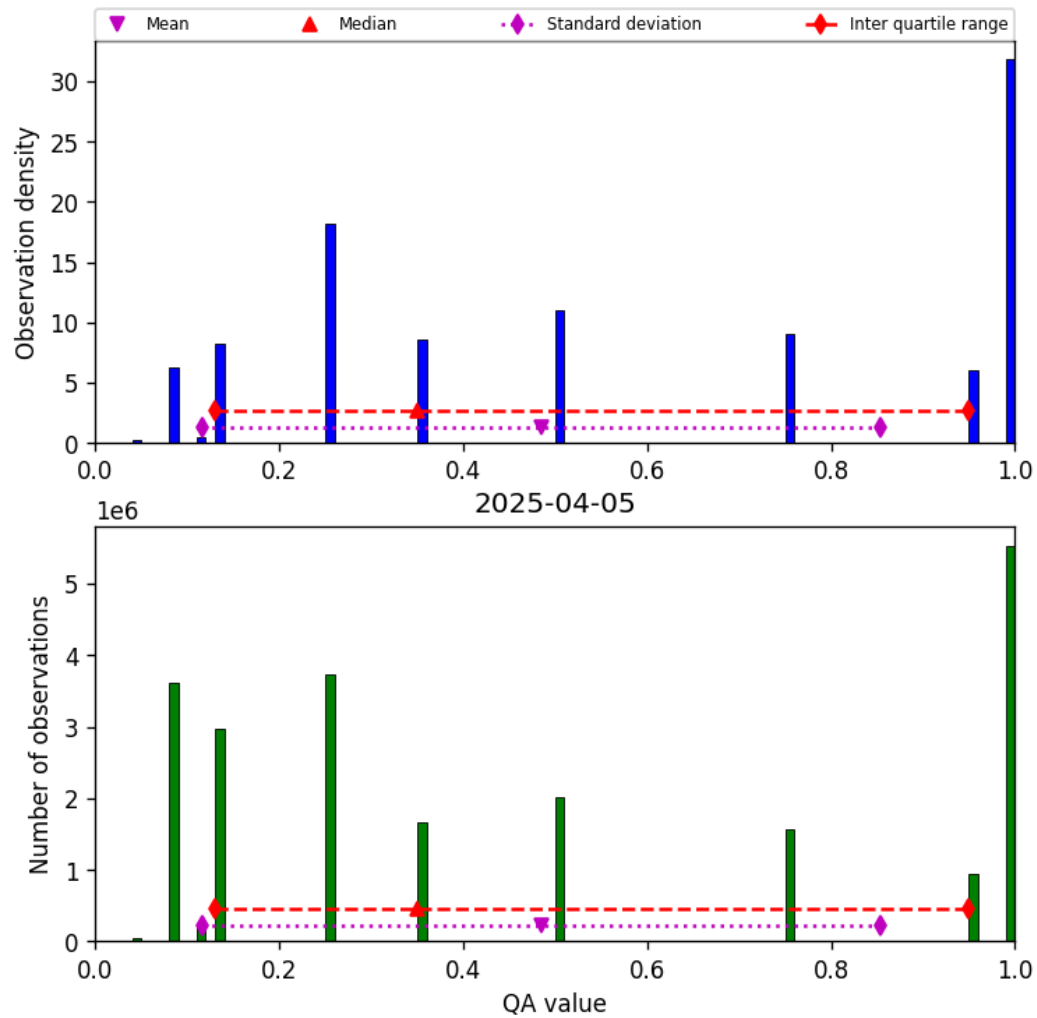
Figure 32: Histogram of “QA value” for 2025-04-05 to 2025-04-06
