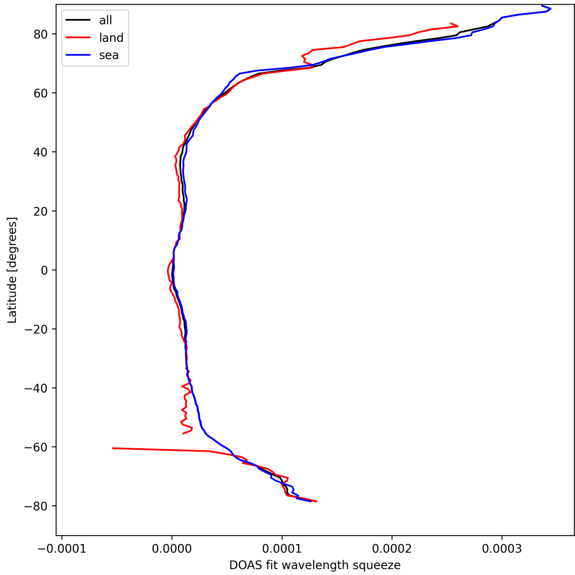
Figure 29: Zonal average of “DOAS fit wavelength squeeze” for 2025-04-05 to 2025-04-06.
