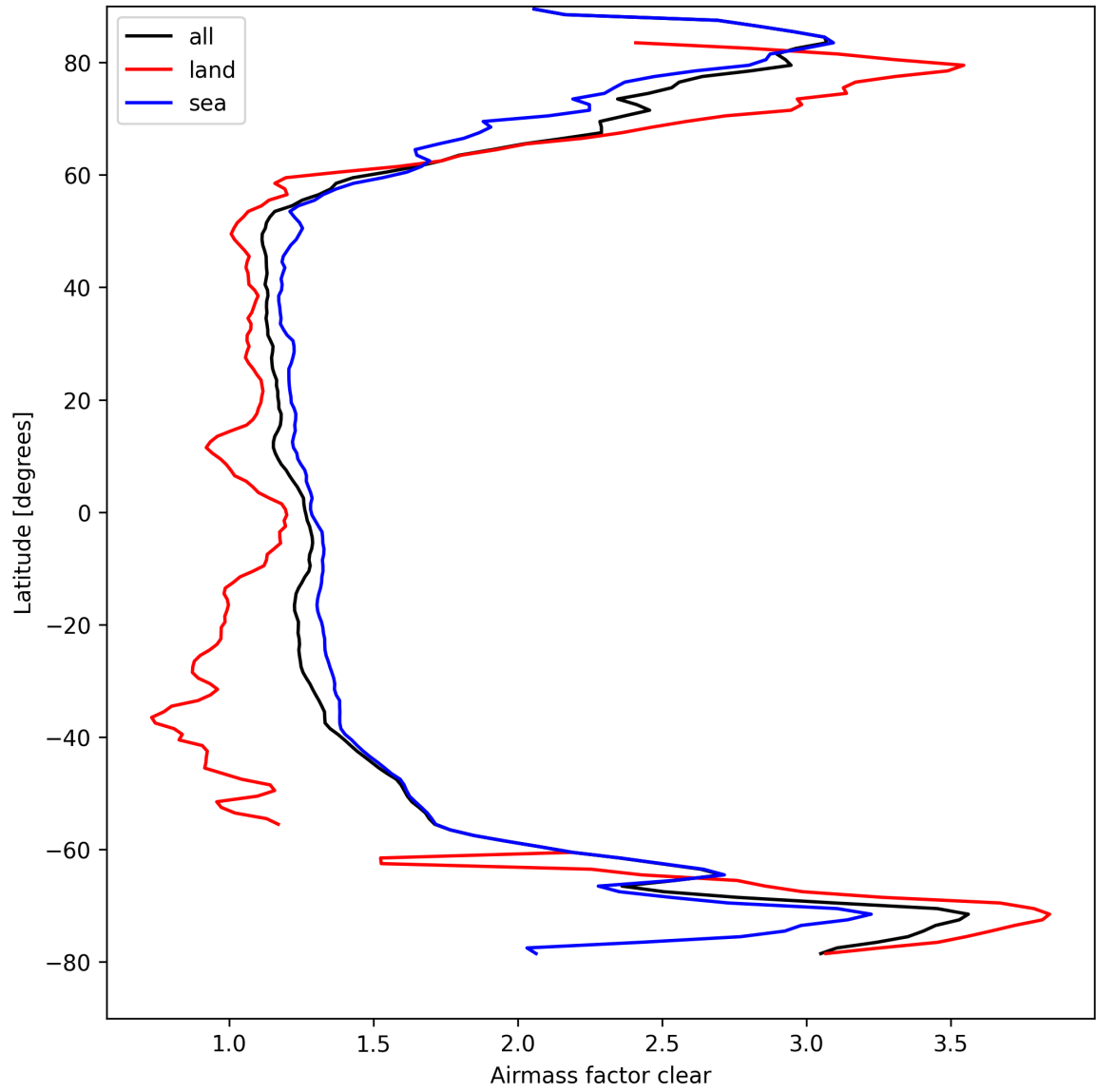
Figure 26: Zonal average of “Airmass factor clear” for 2025-04-05 to 2025-04-06.
