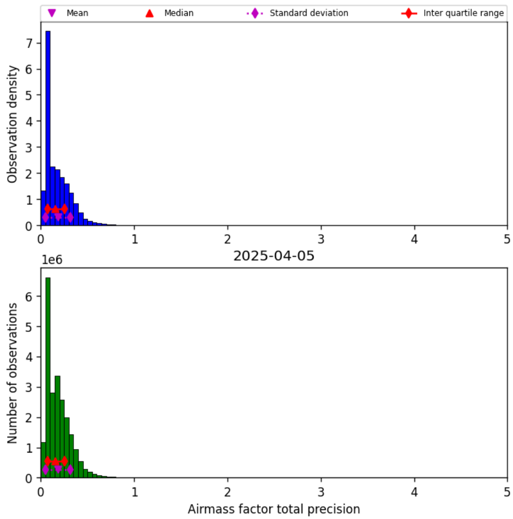
Figure 39: Histogram of “Airmass factor total precision” for 2025-04-05 to 2025-04-06
