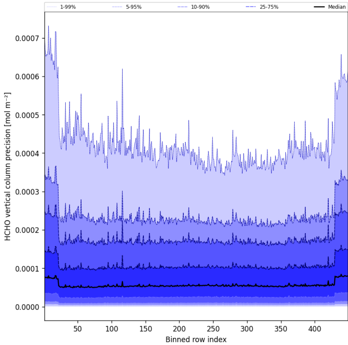
Figure 48: Along track statistics of “HCHO vertical column precision” for 2025-04-05 to 2025-04-06
