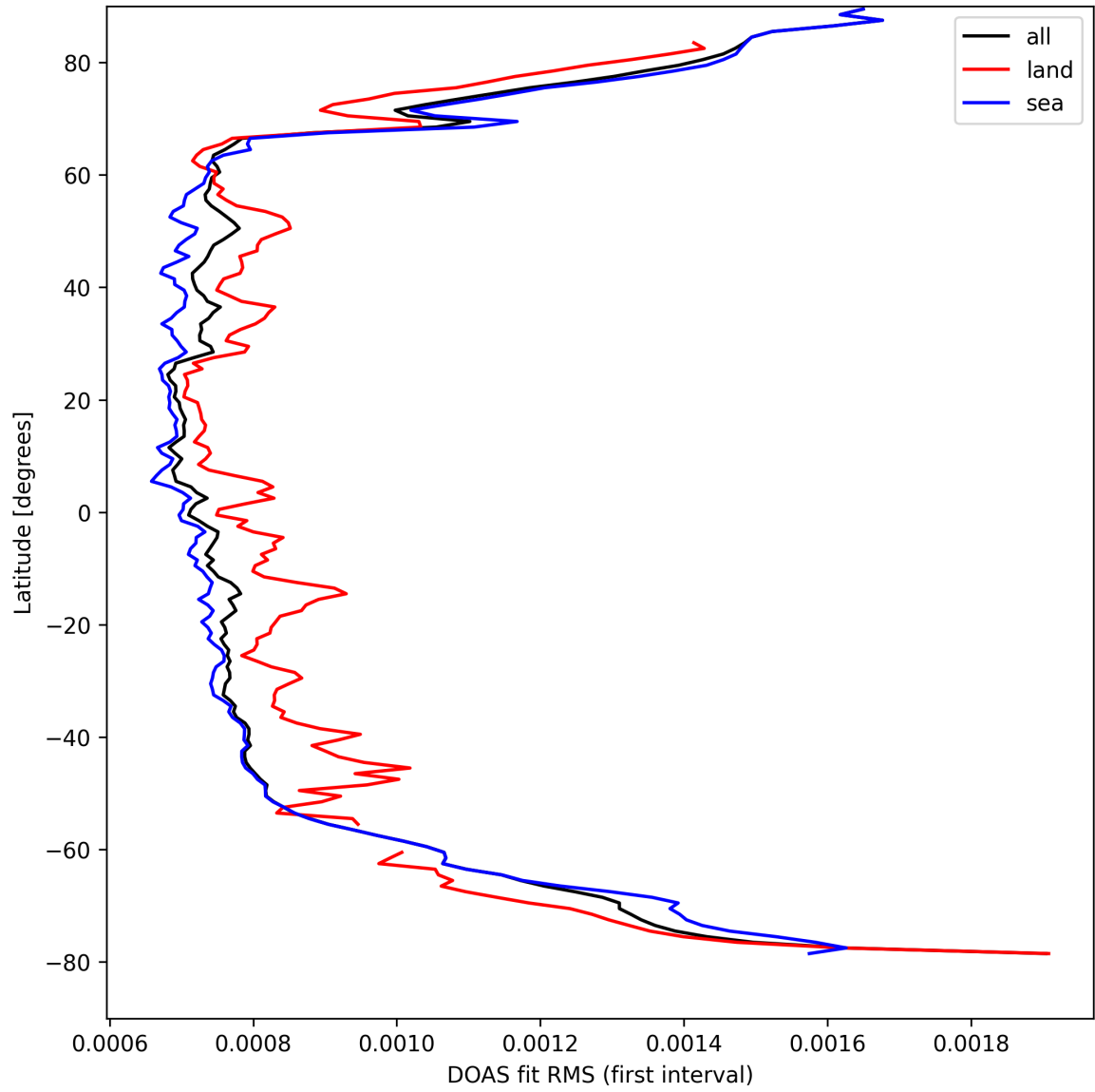
Figure 30: Zonal average of "DOAS fit RMS (first interval)" for 2025-04-05 to 2025-04-06.
