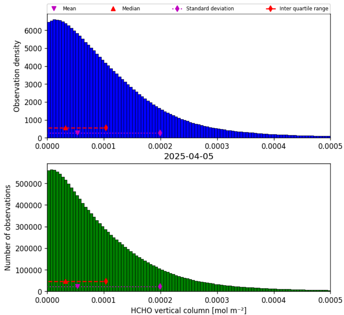
Figure 33: Histogram of “HCHO vertical column” for 2025-04-05 to 2025-04-06
