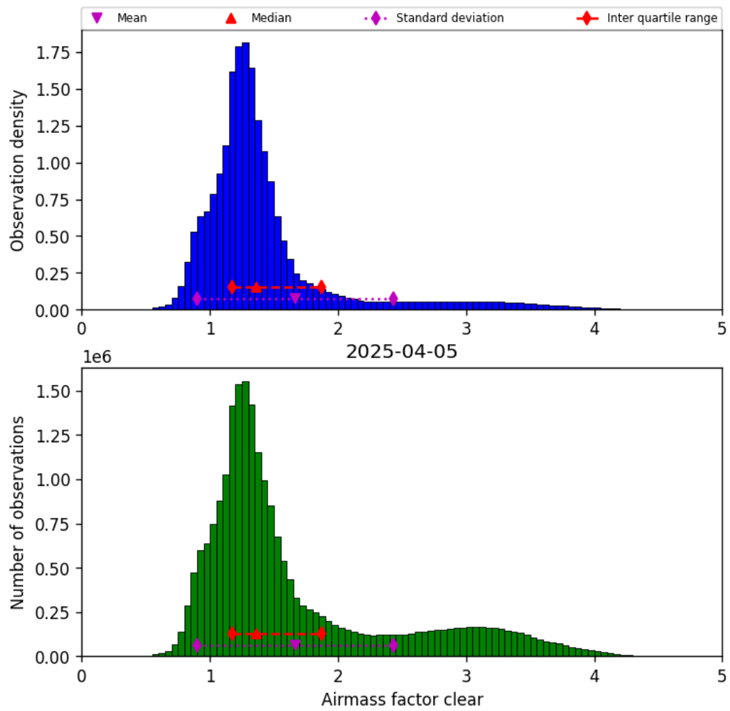
Figure 40: Histogram of “Airmass factor clear” for 2025-04-05 to 2025-04-06
