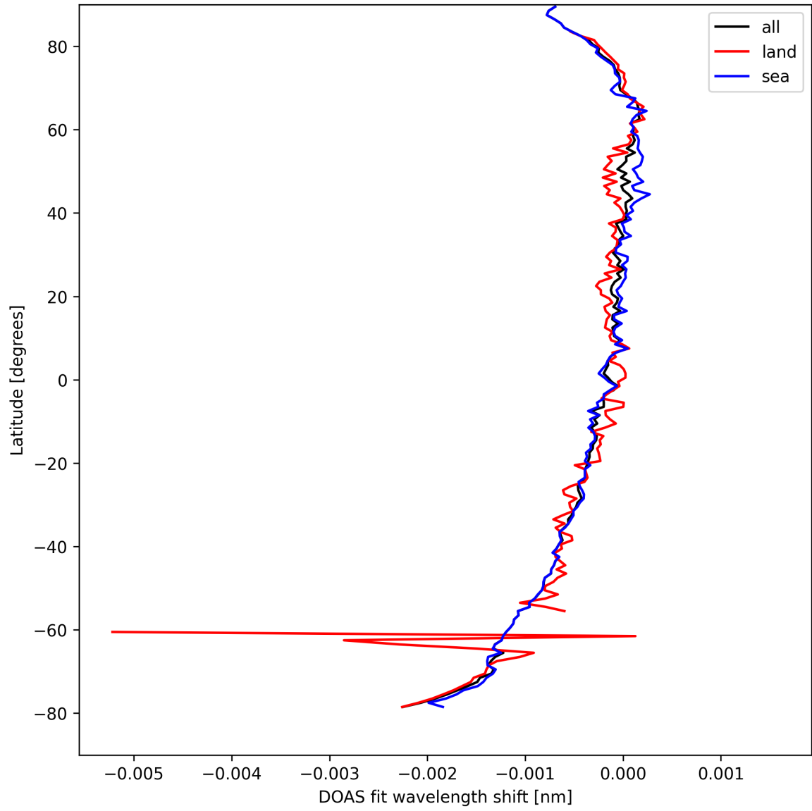
Figure 28: Zonal average of “DOAS fit wavelength shift” for 2025-04-05 to 2025-04-06.
