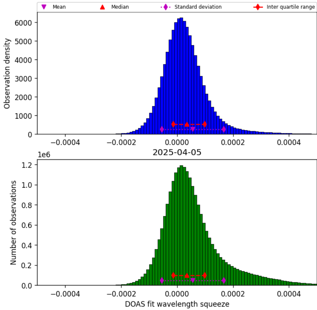
Figure 43: Histogram of “DOAS fit wavelength squeeze” for 2025-04-05 to 2025-04-06
