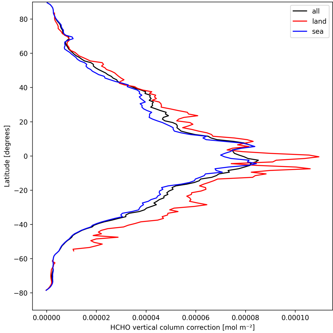
Figure 21: Zonal average of “HCHO vertical column correction” for 2025-04-05 to 2025-04-06.
