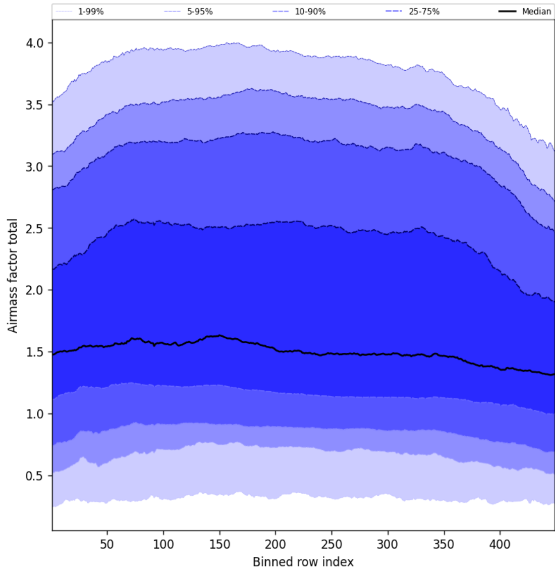
Figure 52: Along track statistics of “Airmass factor total” for 2025-04-05 to 2025-04-06
