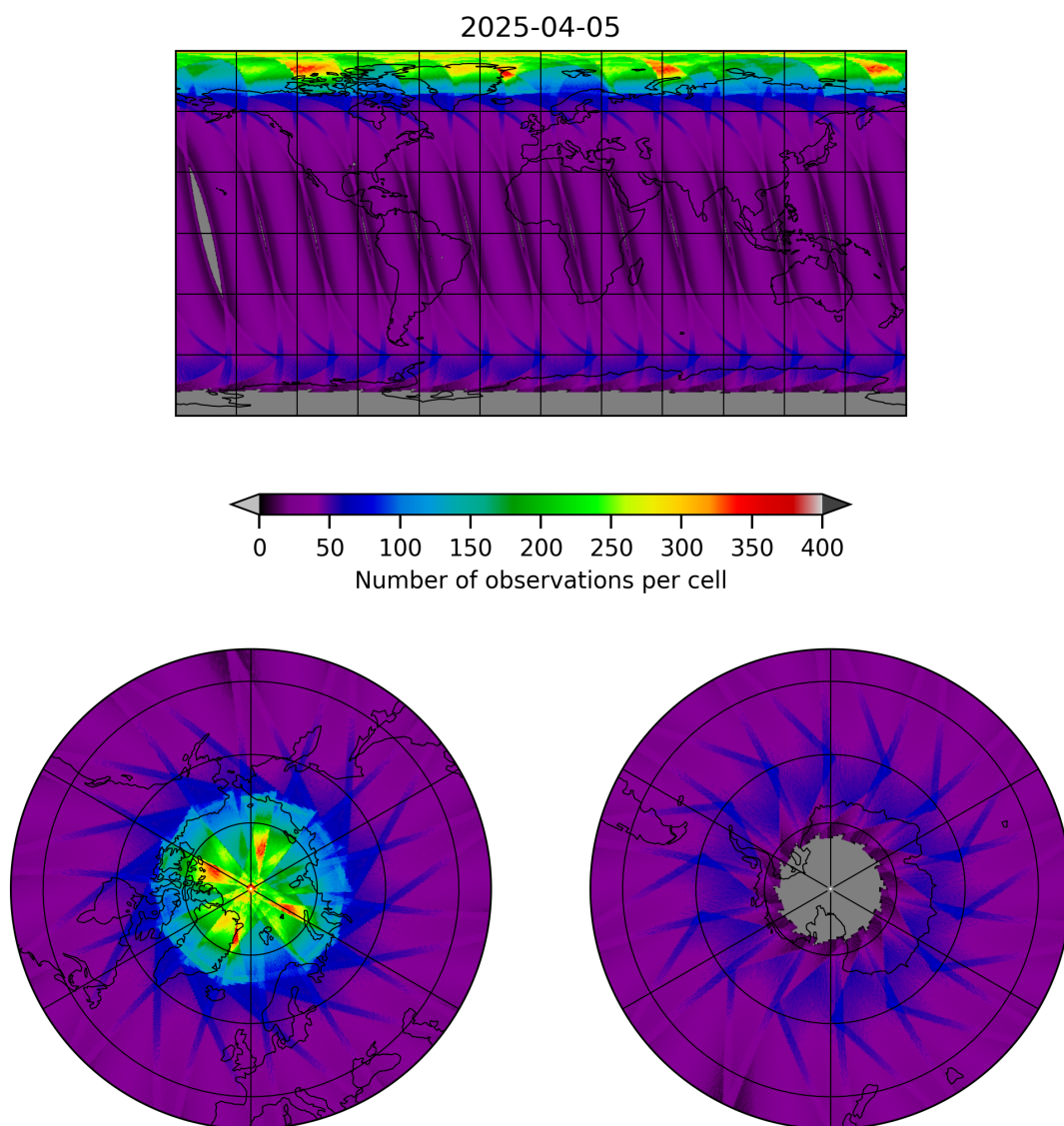
Figure 17: Map of the number of observations for 2025-04-05 to 2025-04-06
