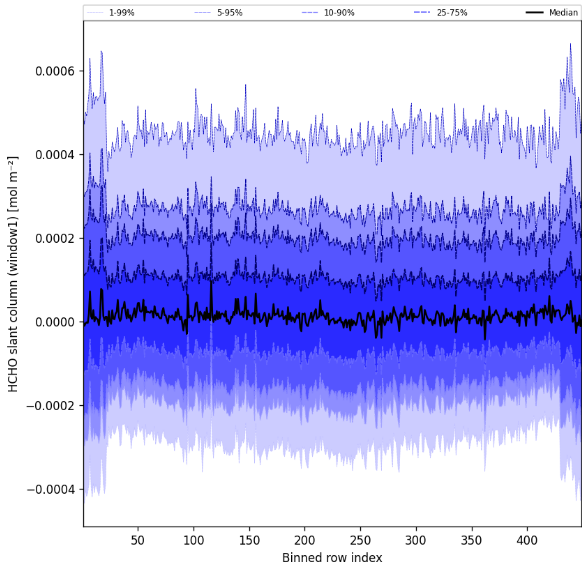
Figure 50: Along track statistics of “HCHO slant column (window1)” for 2025-04-05 to 2025-04-06
