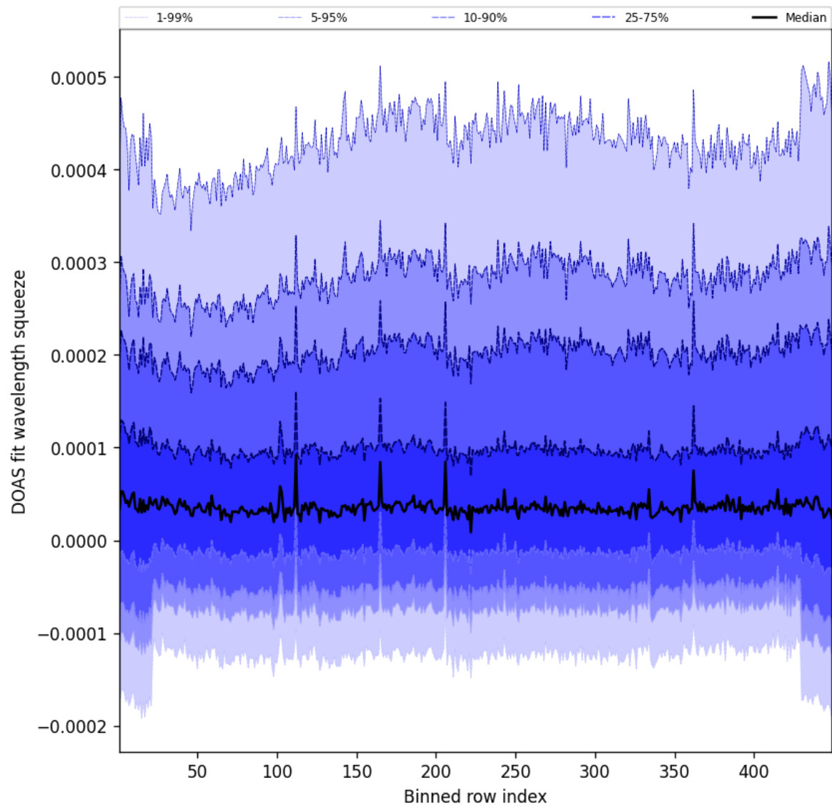
Figure 57: Along track statistics of “DOAS fit wavelength squeeze” for 2025-04-05 to 2025-04-06
