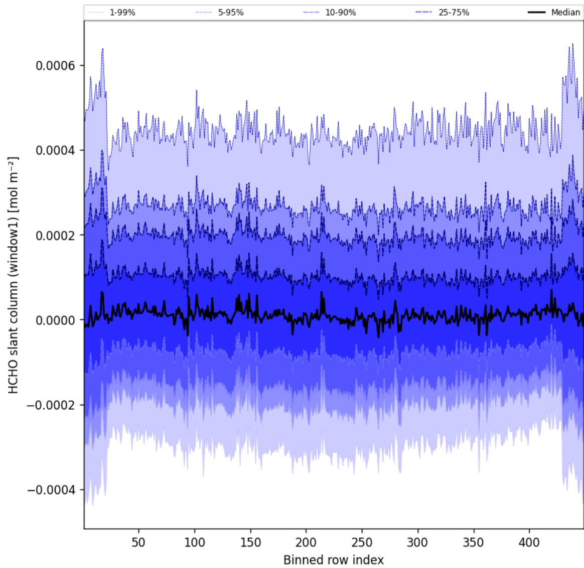
Figure 50: Along track statistics of “HCHO slant column (window1)” for 2025-04-06 to 2025-04-06
