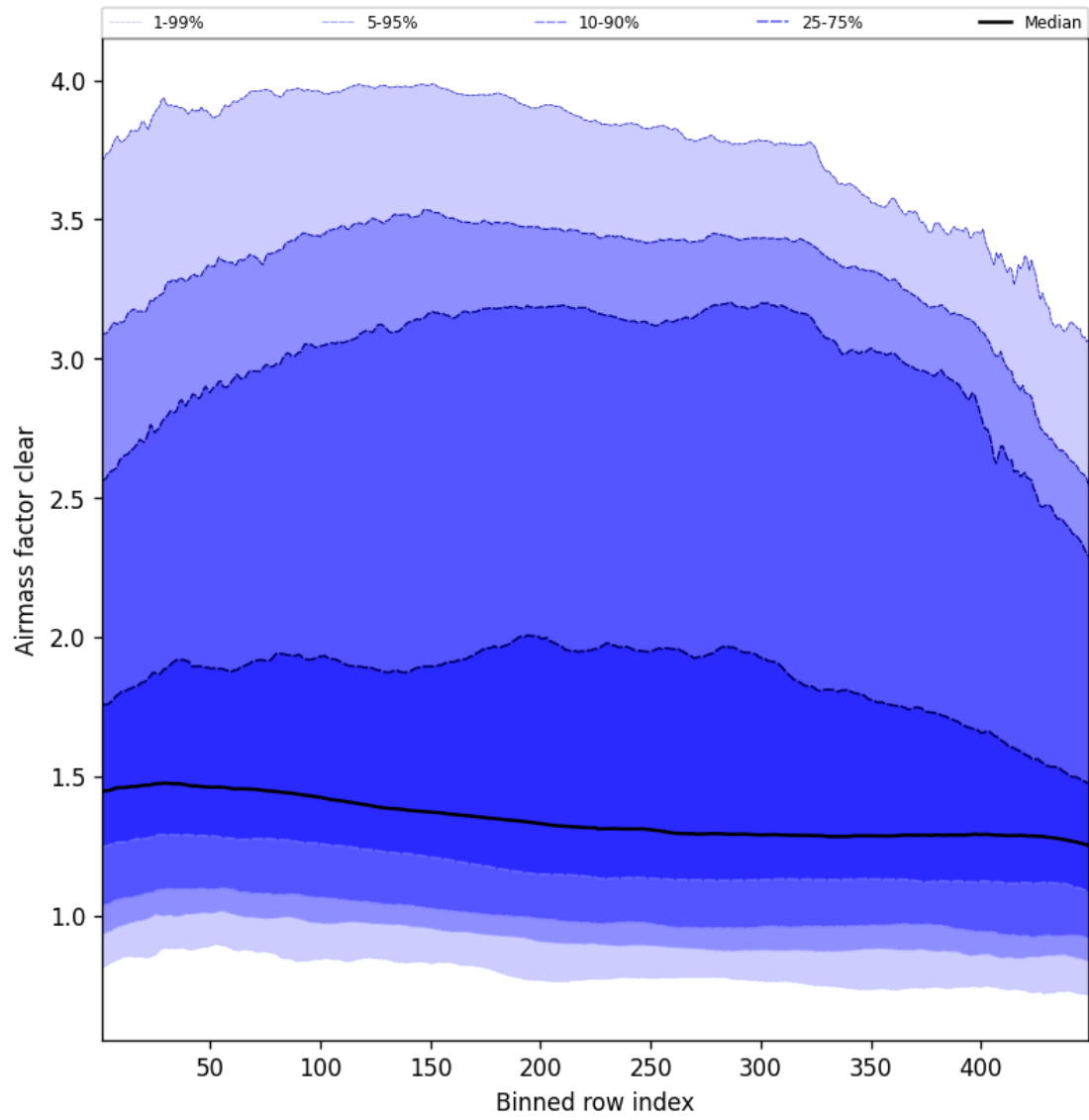
Figure 54: Along track statistics of “Airmass factor clear” for 2025-04-06 to 2025-04-06
