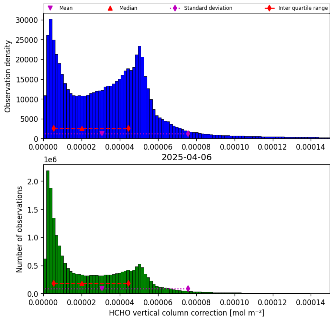
Figure 35: Histogram of “HCHO vertical column correction” for 2025-04-06 to 2025-04-06
