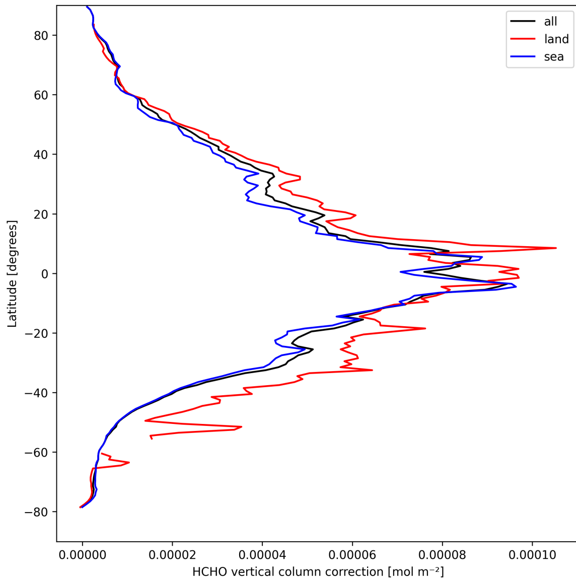
Figure 21: Zonal average of “HCHO vertical column correction” for 2025-04-06 to 2025-04-06.
