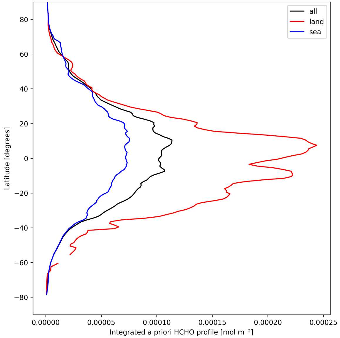
Figure 27: Zonal average of “Integrated a priori HCHO profile” for 2025-04-06 to 2025-04-06.
