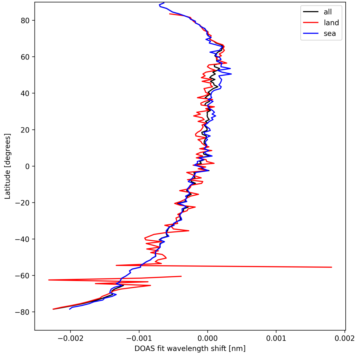
Figure 28: Zonal average of “DOAS fit wavelength shift” for 2025-04-06 to 2025-04-06.
