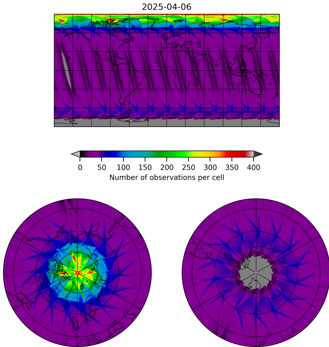
Figure 17: Map of the number of observations for 2025-04-06 to 2025-04-06
