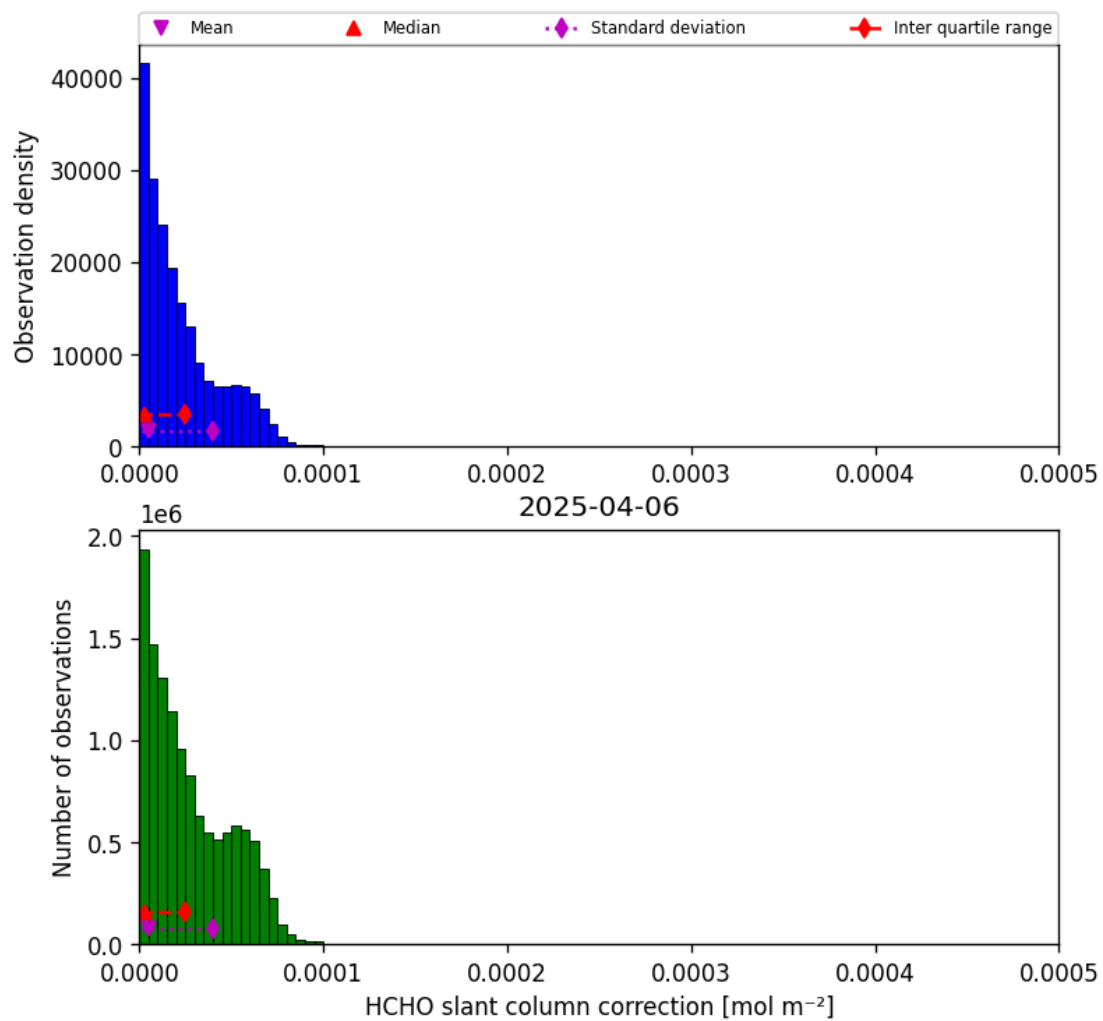
Figure 45: Histogram of “HCHO slant column correction” for 2025-04-06 to 2025-04-06
