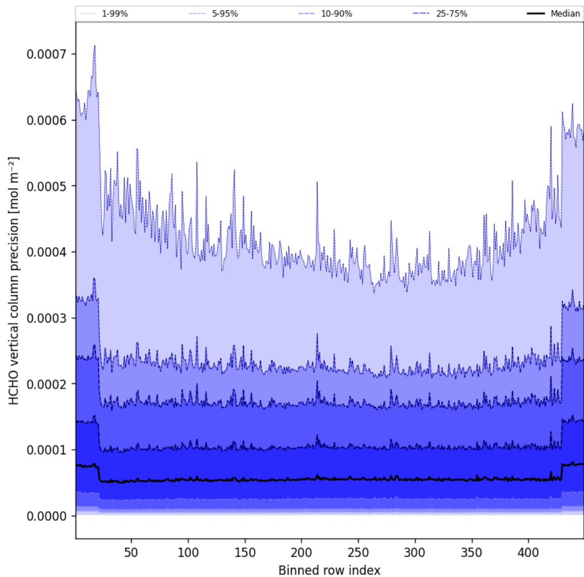
Figure 48: Along track statistics of "HCHO vertical column precision" for 2025-04-06 to 2025-04-06
