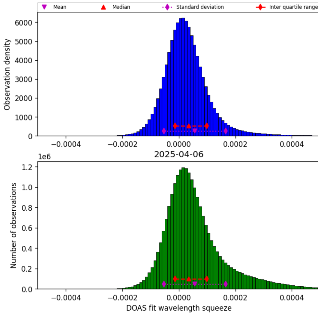
Figure 43: Histogram of “DOAS fit wavelength squeeze” for 2025-04-06 to 2025-04-06
