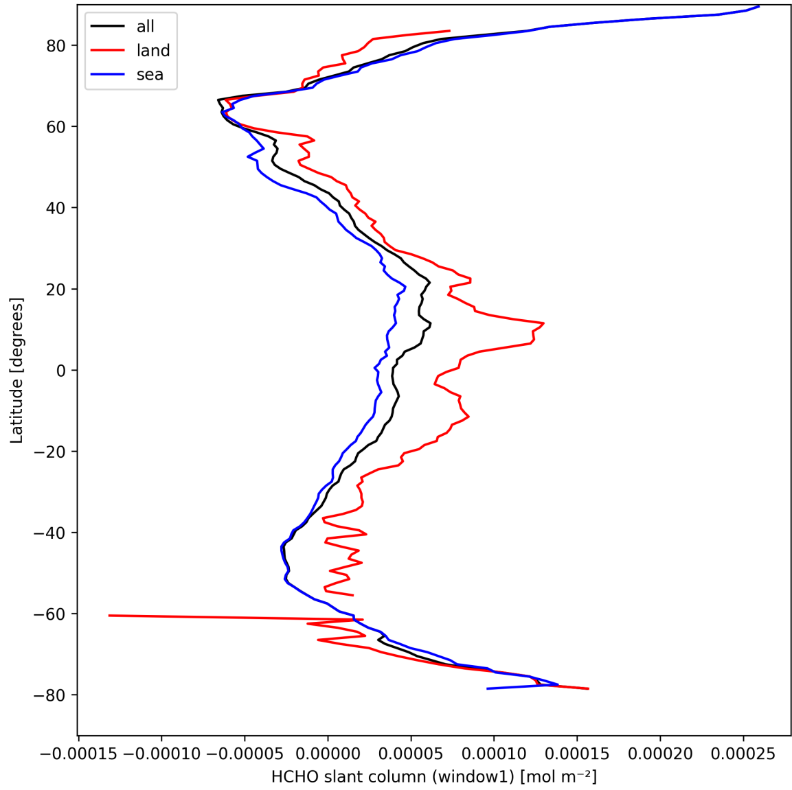
Figure 22: Zonal average of “HCHO slant column (window1)” for 2025-04-06 to 2025-04-06.
