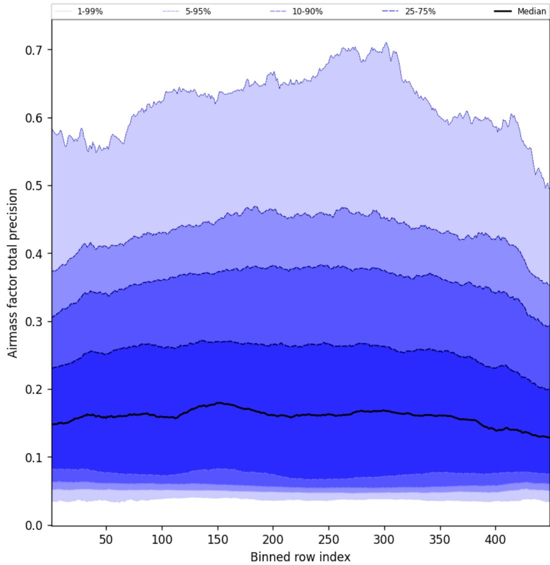
Figure 53: Along track statistics of “Airmass factor total precision” for 2025-04-06 to 2025-04-06
