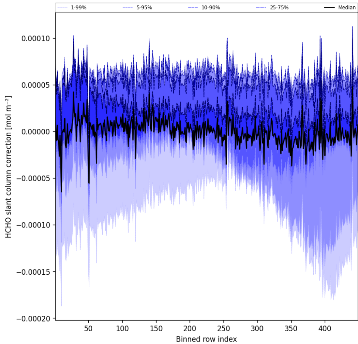
Figure 59: Along track statistics of “HCHO slant column correction” for 2025-04-06 to 2025-04-06
