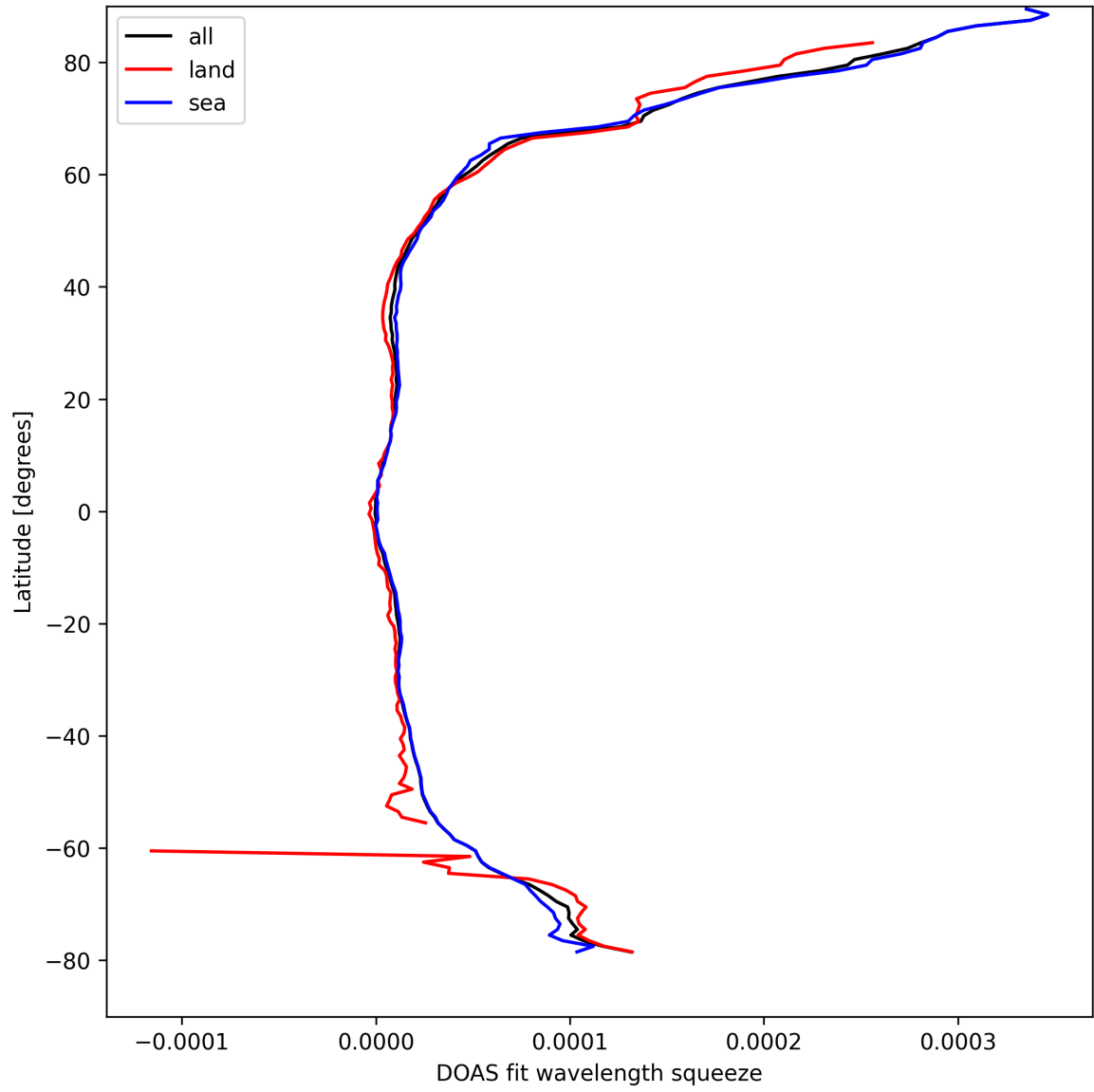
Figure 29: Zonal average of “DOAS fit wavelength squeeze” for 2025-04-06 to 2025-04-06.
