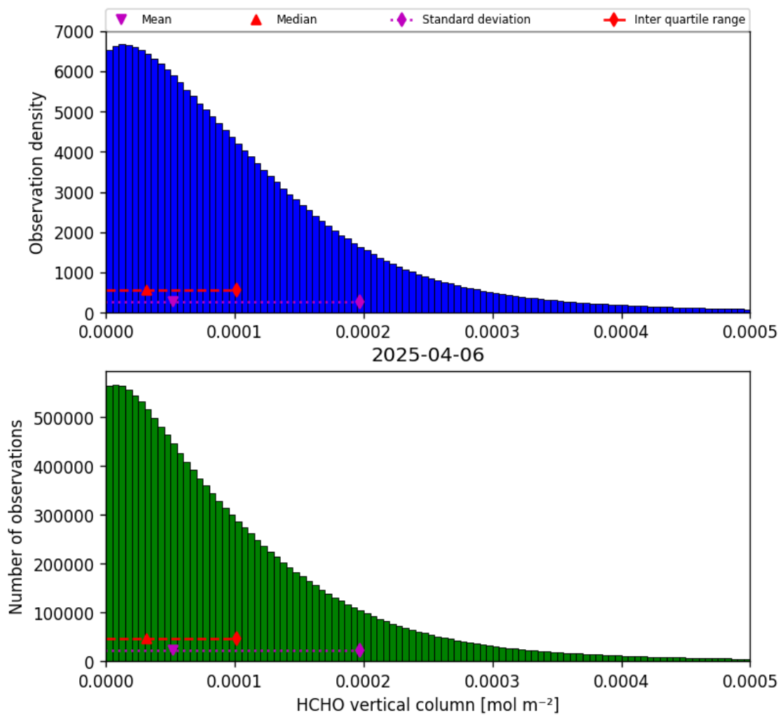
Figure 33: Histogram of “HCHO vertical column” for 2025-04-06 to 2025-04-06
