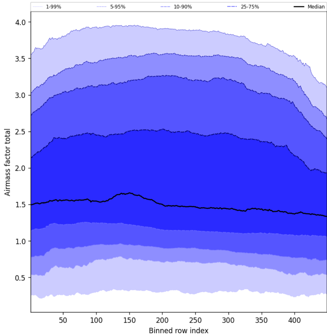
Figure 52: Along track statistics of “Airmass factor total” for 2025-04-06 to 2025-04-06
