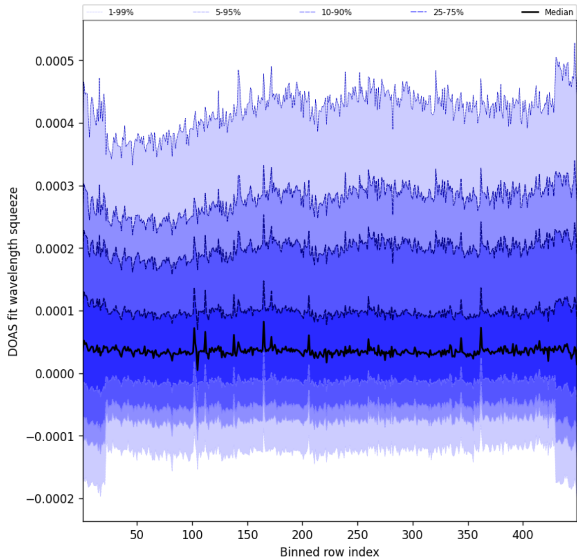
Figure 57: Along track statistics of “DOAS fit wavelength squeeze” for 2025-04-06 to 2025-04-06
