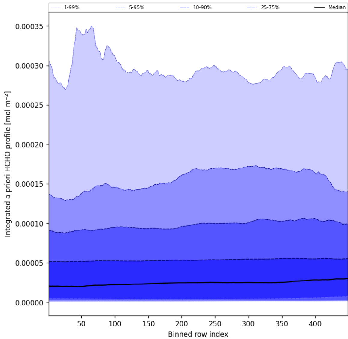
Figure 55: Along track statistics of “Integrated a priori HCHO profile” for 2025-04-06 to 2025-04-06
