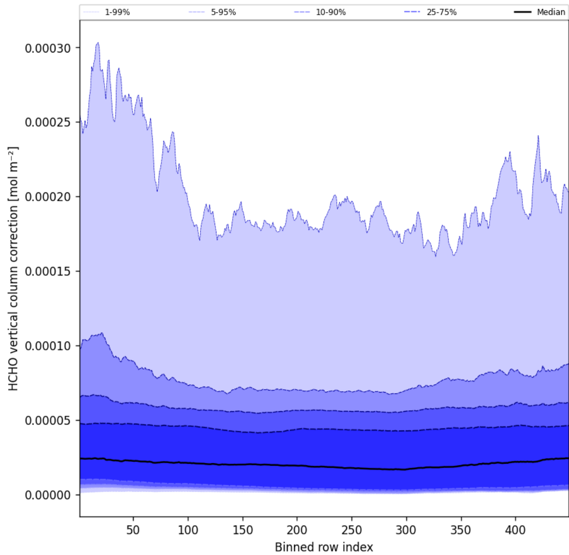
Figure 49: Along track statistics of “HCHO vertical column correction” for 2025-04-06 to 2025-04-06
