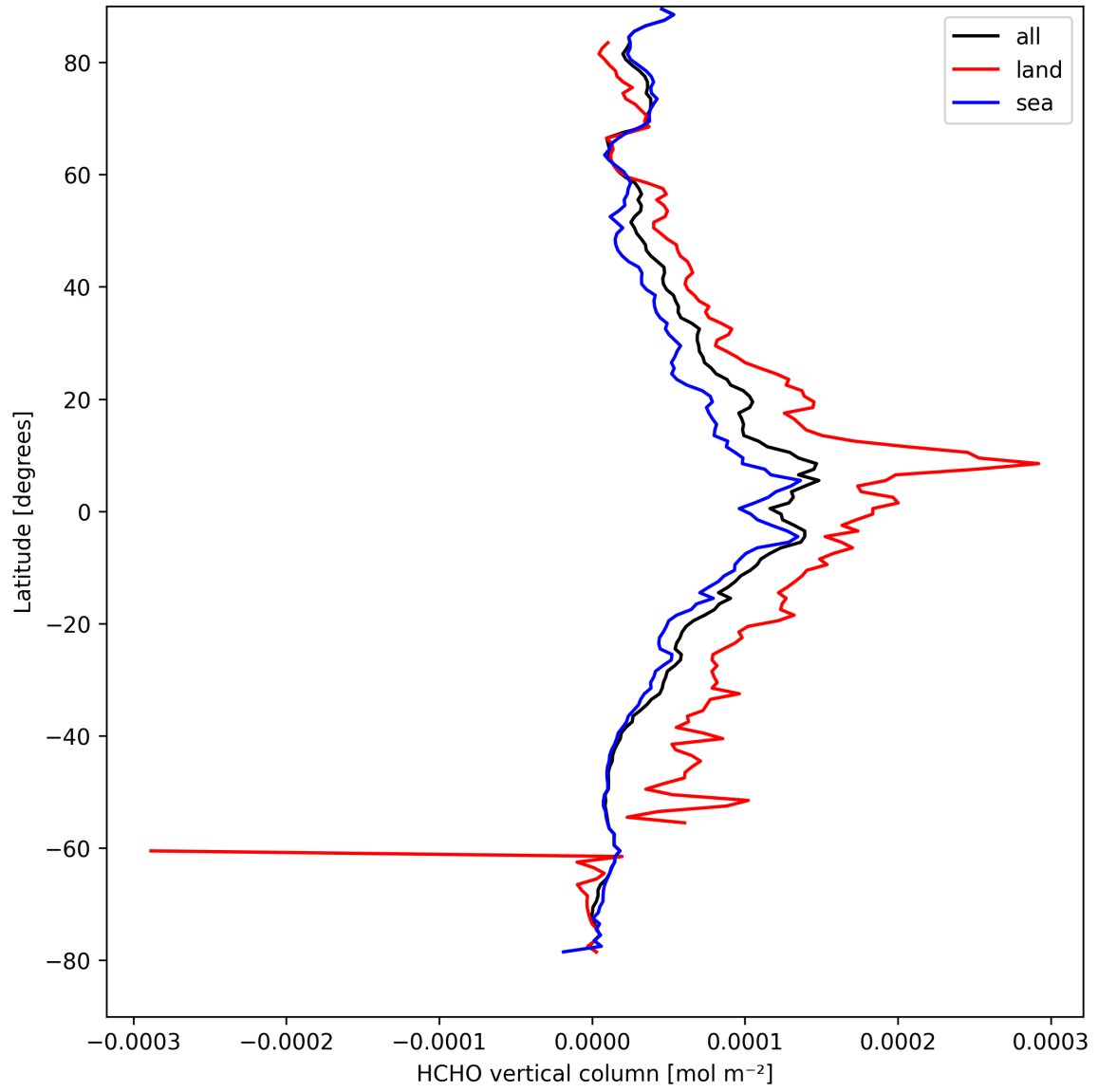
Figure 19: Zonal average of “HCHO vertical column” for 2025-04-06 to 2025-04-06.
