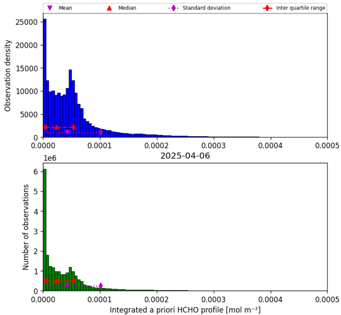
Figure 41: Histogram of “Integrated a priori HCHO profile” for 2025-04-06 to 2025-04-06
