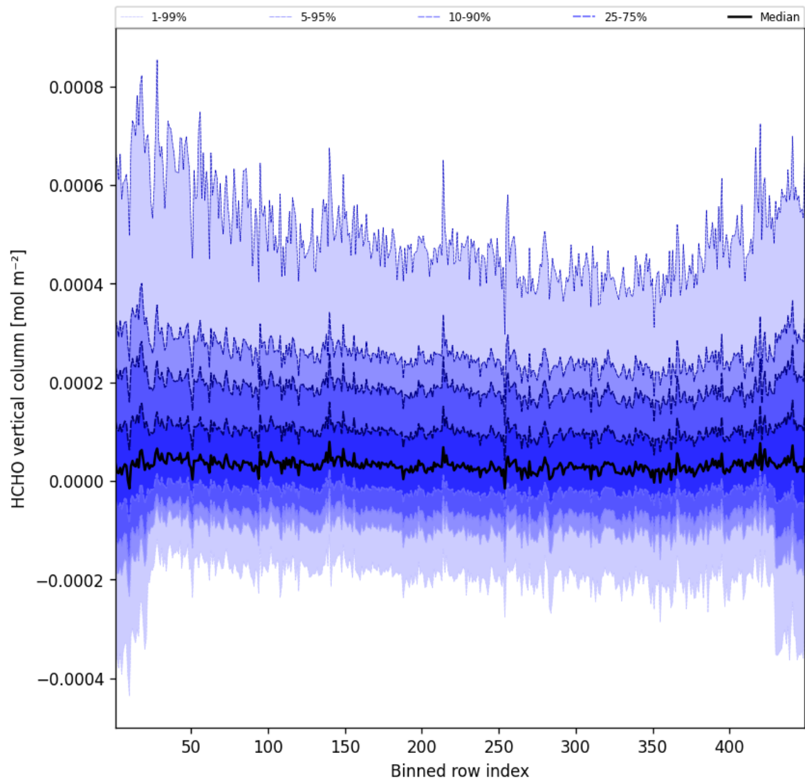
Figure 47: Along track statistics of “HCHO vertical column” for 2025-04-06 to 2025-04-06
