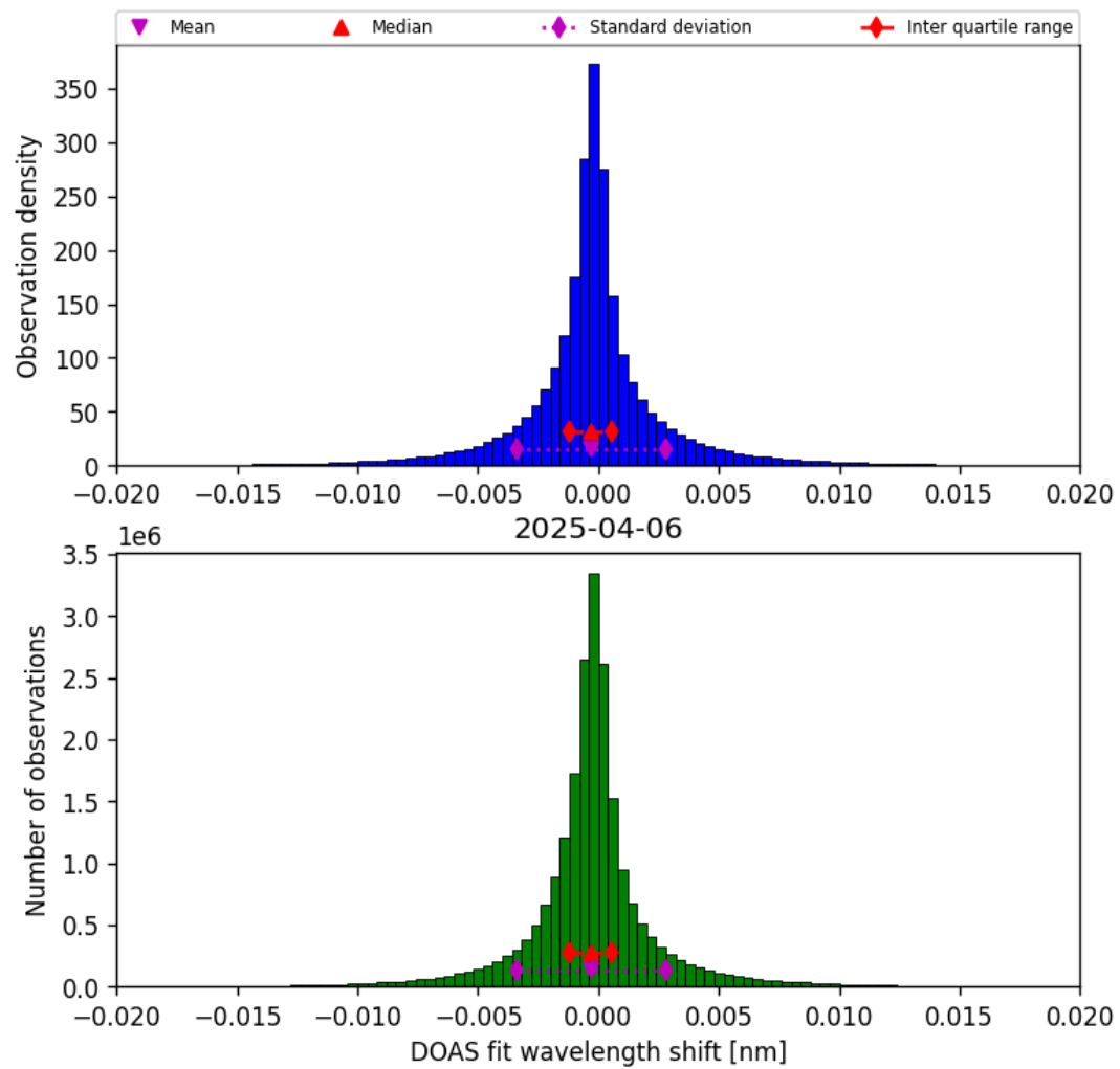
Figure 42: Histogram of “DOAS fit wavelength shift” for 2025-04-06 to 2025-04-06
