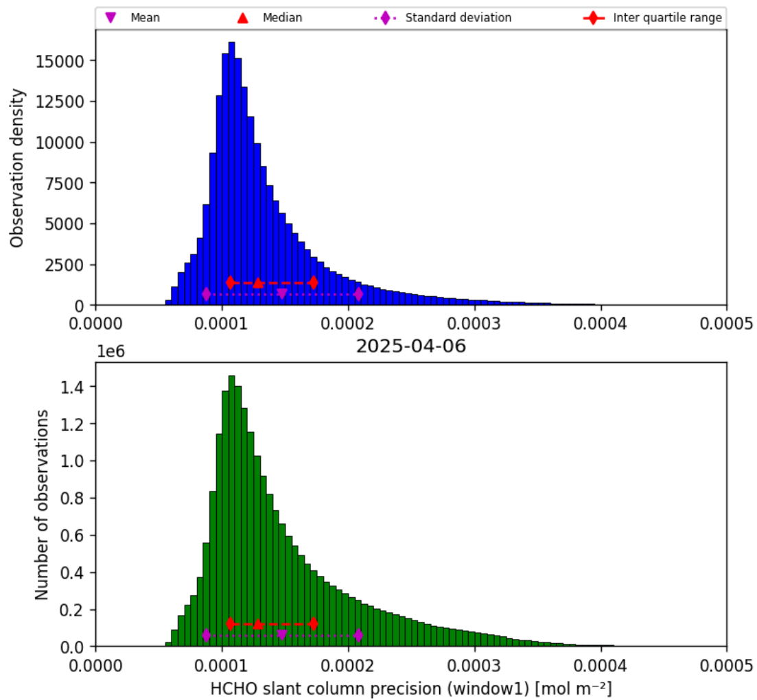
Figure 37: Histogram of “HCHO slant column precision (window1)” for 2025-04-06 to 2025-04-06
