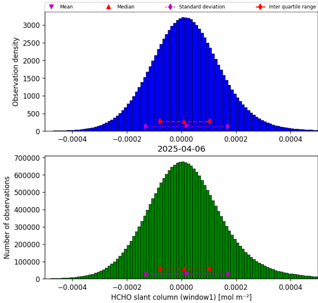
Figure 36: Histogram of “HCHO slant column (window1)” for 2025-04-06 to 2025-04-06
