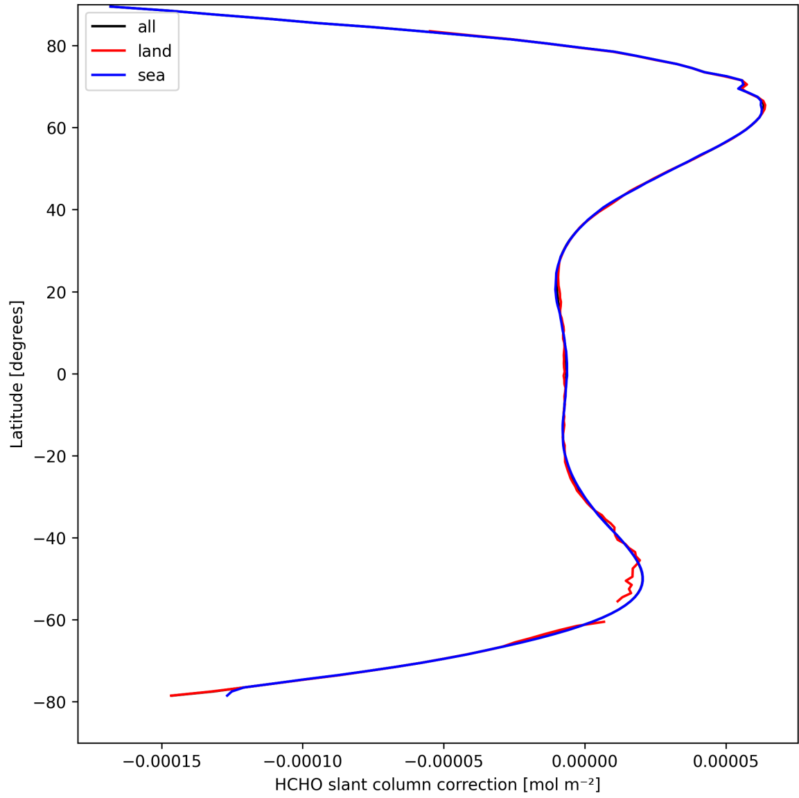
Figure 31: Zonal average of “HCHO slant column correction” for 2025-04-06 to 2025-04-06.
