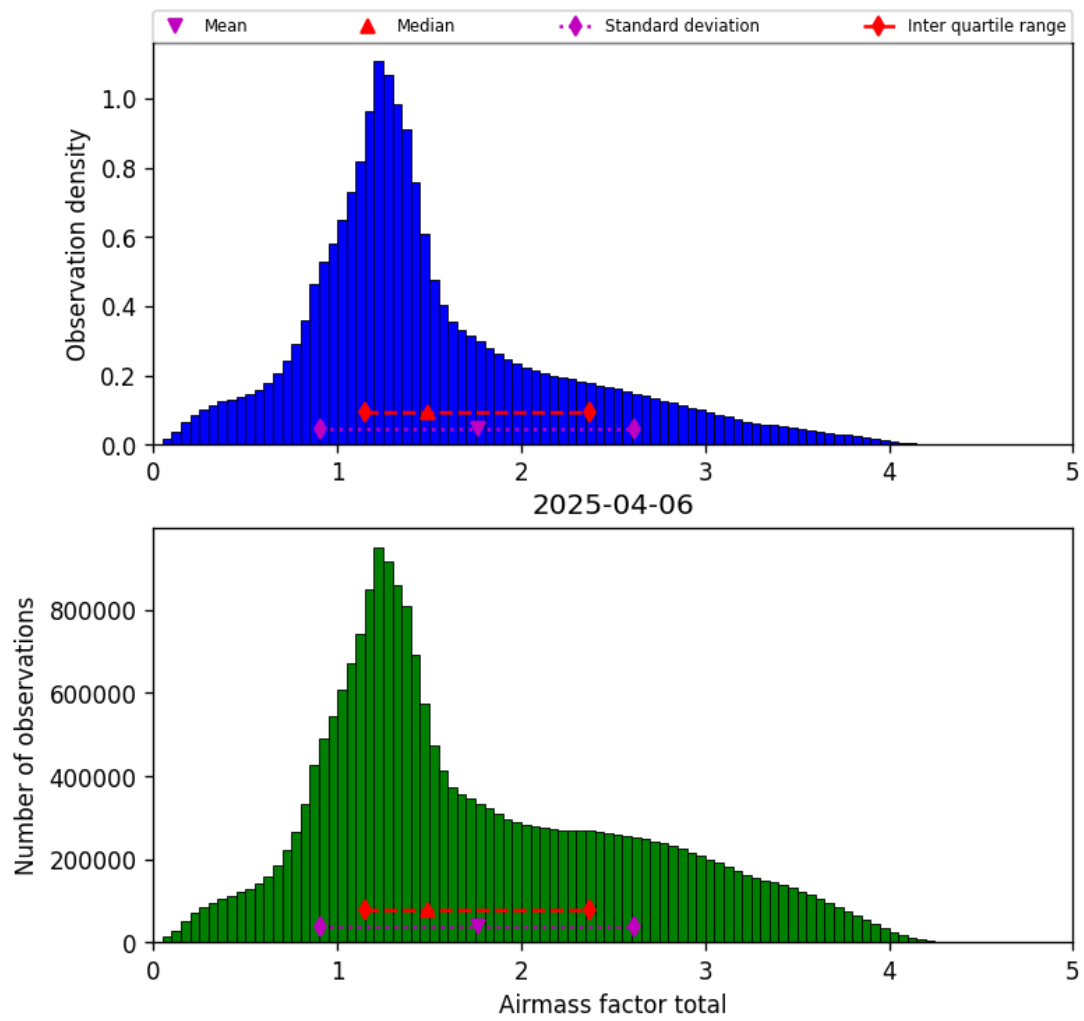
Figure 38: Histogram of “Airmass factor total” for 2025-04-06 to 2025-04-06
