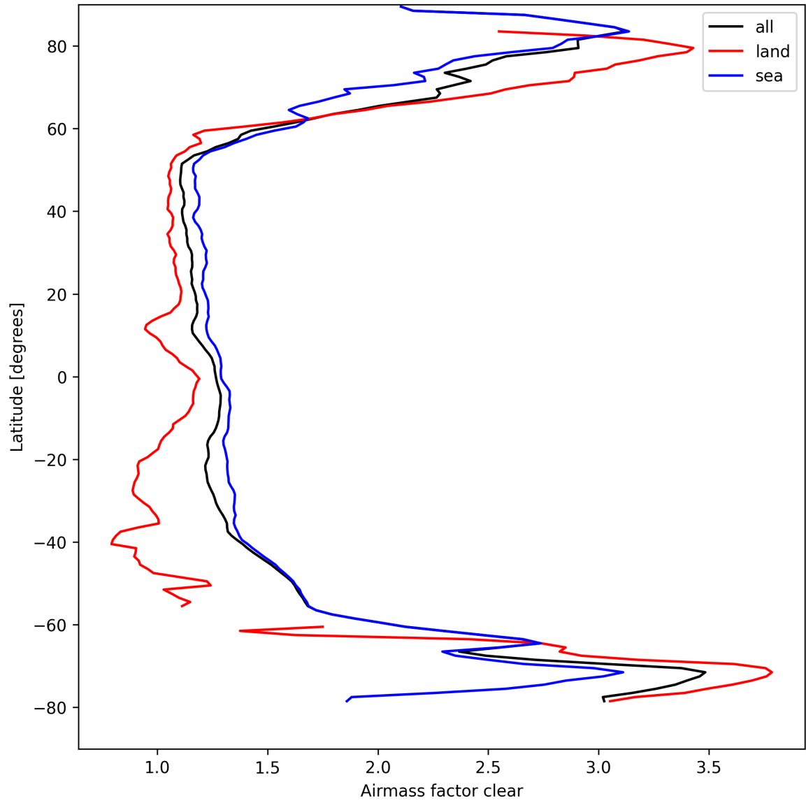
Figure 26: Zonal average of “Airmass factor clear” for 2025-04-06 to 2025-04-06.
