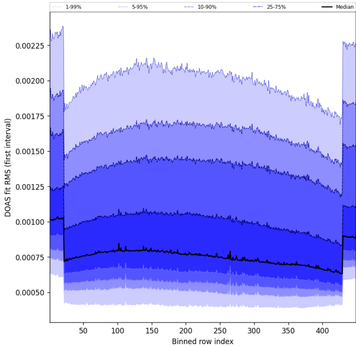
Figure 58: Along track statistics of “DOAS fit RMS (first interval)” for 2025-04-06 to 2025-04-06
