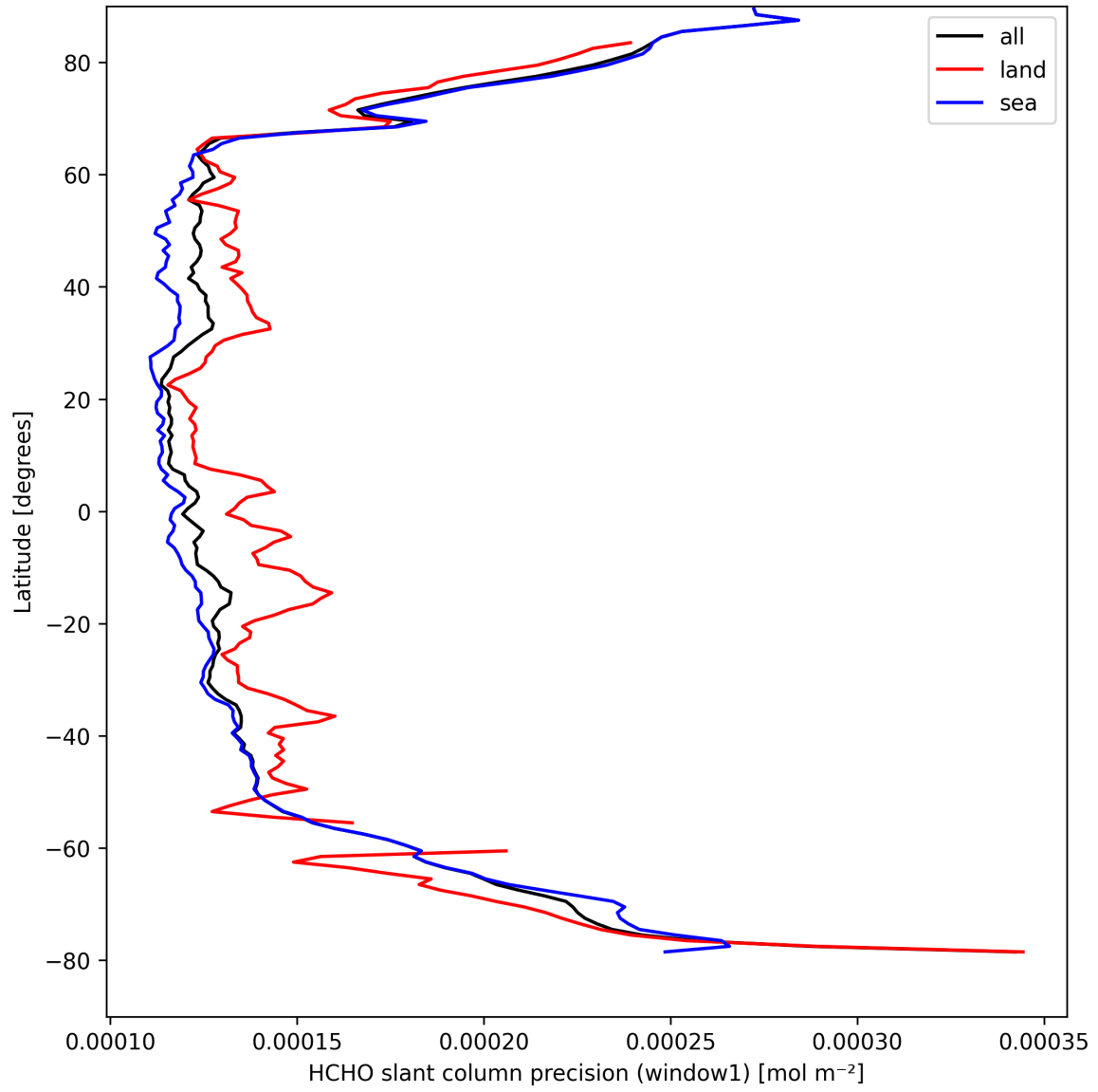
Figure 23: Zonal average of "HCHO slant column precision (window1)" for 2025-04-06 to 2025-04-06.
