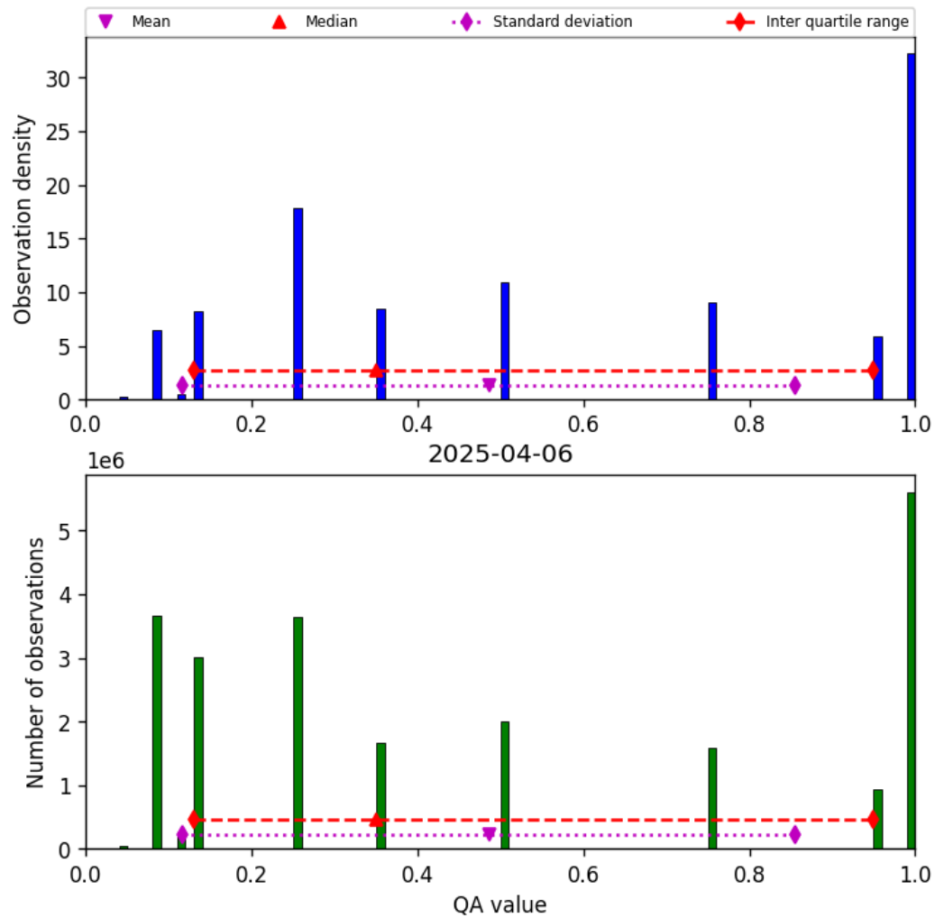
Figure 32: Histogram of “QA value” for 2025-04-06 to 2025-04-06
