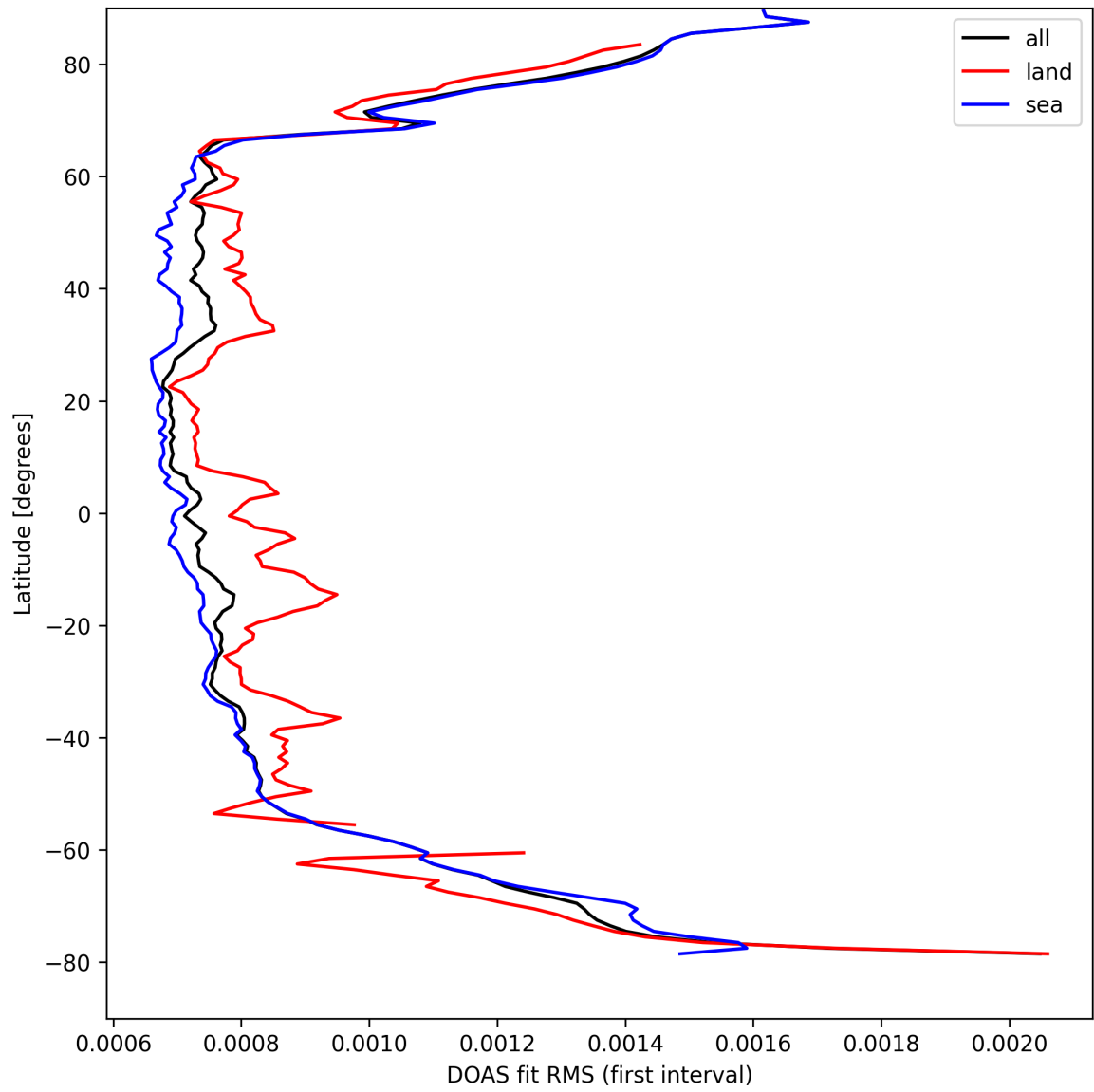
Figure 30: Zonal average of “DOAS fit RMS (first interval)” for 2025-04-06 to 2025-04-06.
