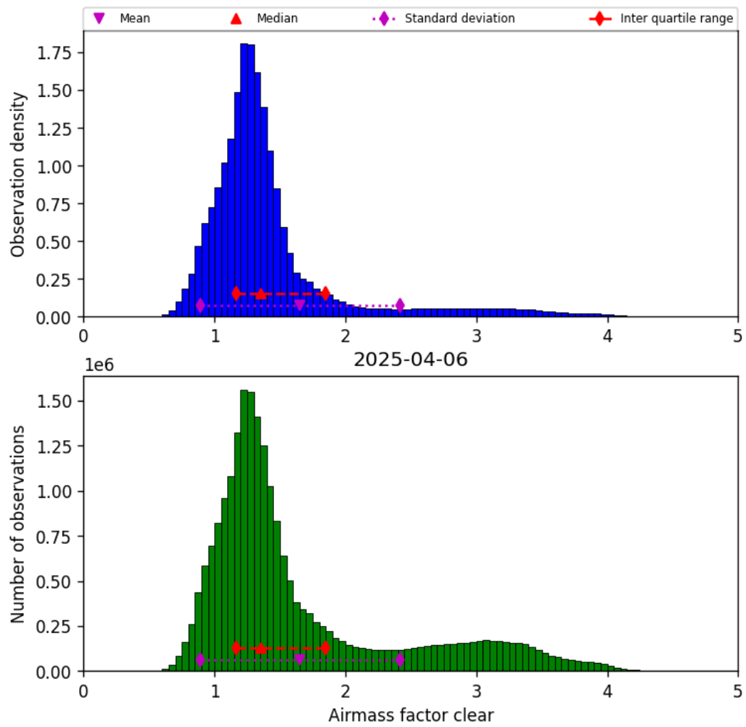
Figure 40: Histogram of “Airmass factor clear” for 2025-04-06 to 2025-04-06
