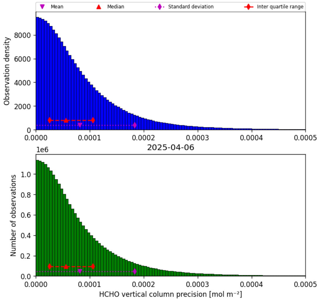
Figure 34: Histogram of “HCHO vertical column precision” for 2025-04-06 to 2025-04-06
