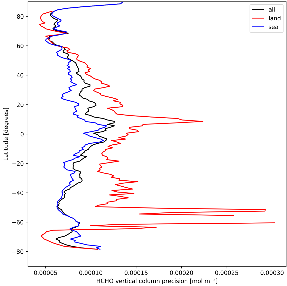
Figure 20: Zonal average of “HCHO vertical column precision” for 2025-04-06 to 2025-04-06.
