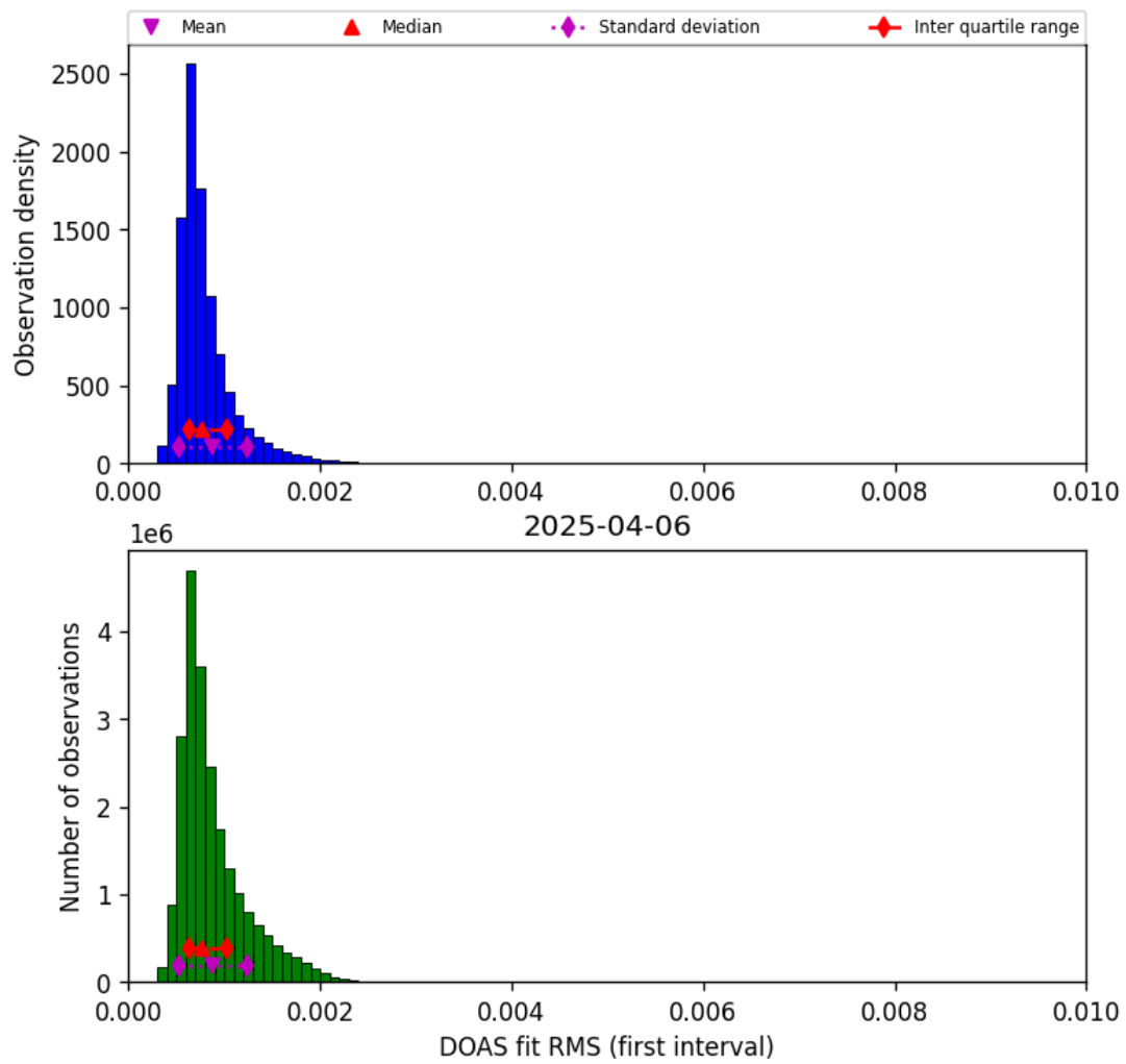
Figure 44: Histogram of “DOAS fit RMS (first interval)” for 2025-04-06 to 2025-04-06
