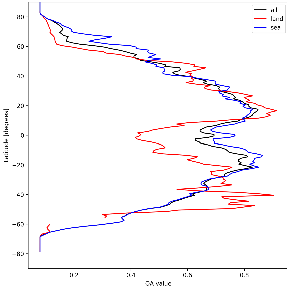
Figure 18: Zonal average of “QA value” for 2025-04-06 to 2025-04-06.
