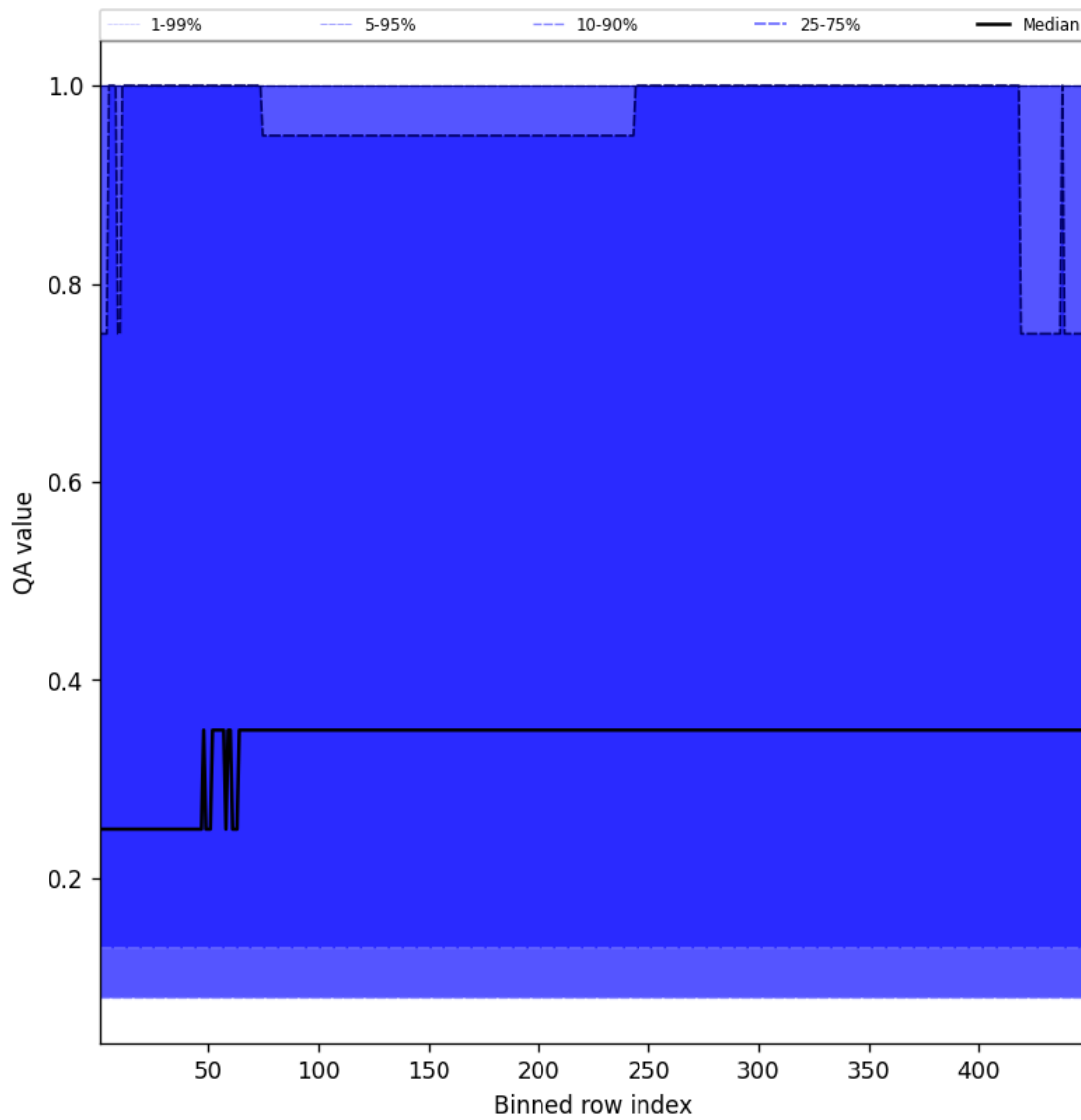
Figure 46: Along track statistics of “QA value” for 2025-04-06 to 2025-04-06
