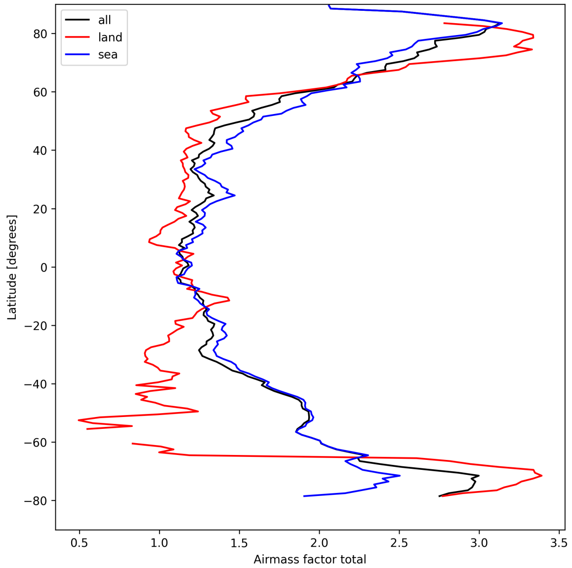
Figure 24: Zonal average of “Airmass factor total” for 2025-04-06 to 2025-04-06.
