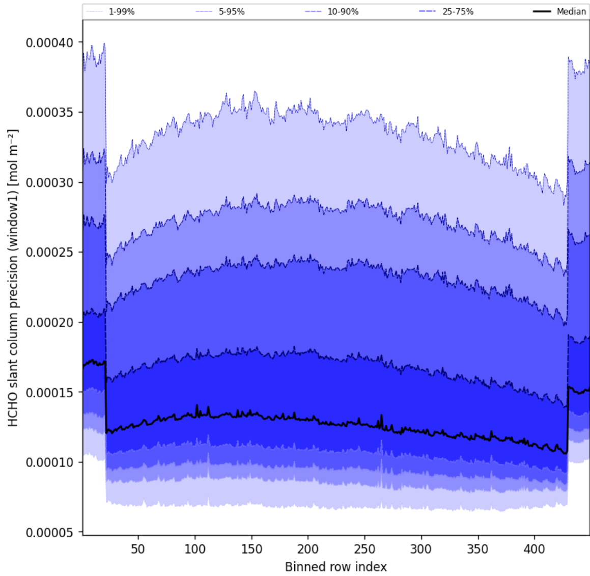
Figure 51: Along track statistics of “HCHO slant column precision (window1)” for 2025-04-06 to 2025-04-06
