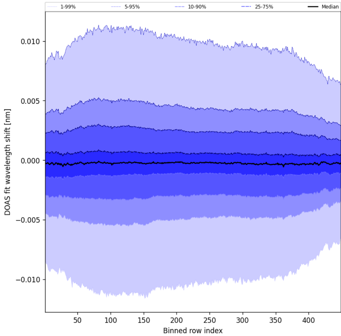
Figure 56: Along track statistics of “DOAS fit wavelength shift” for 2025-04-06 to 2025-04-06
