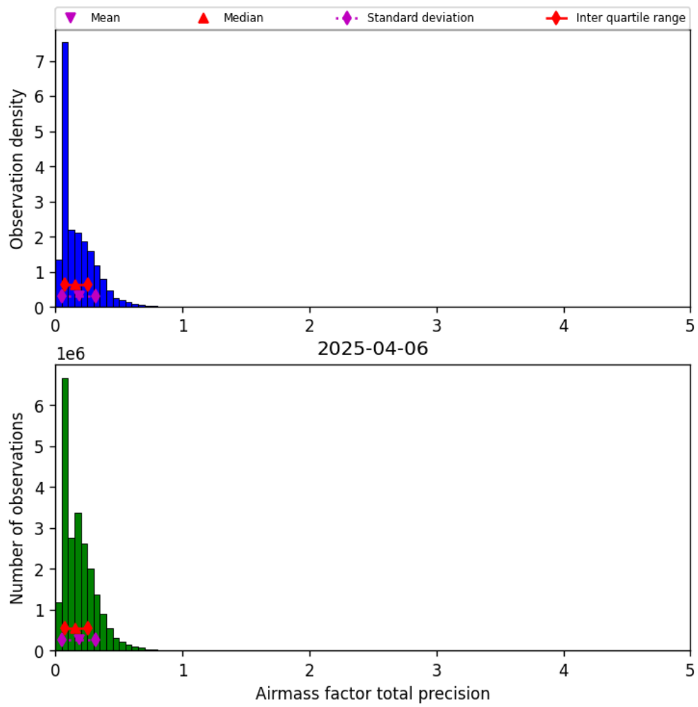
Figure 39: Histogram of “Airmass factor total precision” for 2025-04-06 to 2025-04-06
