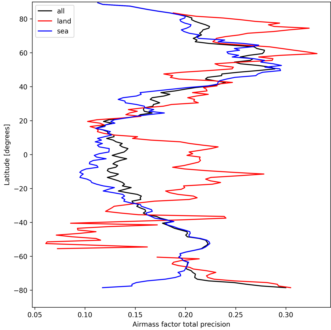
Figure 25: Zonal average of “Airmass factor total precision” for 2025-04-06 to 2025-04-06.
