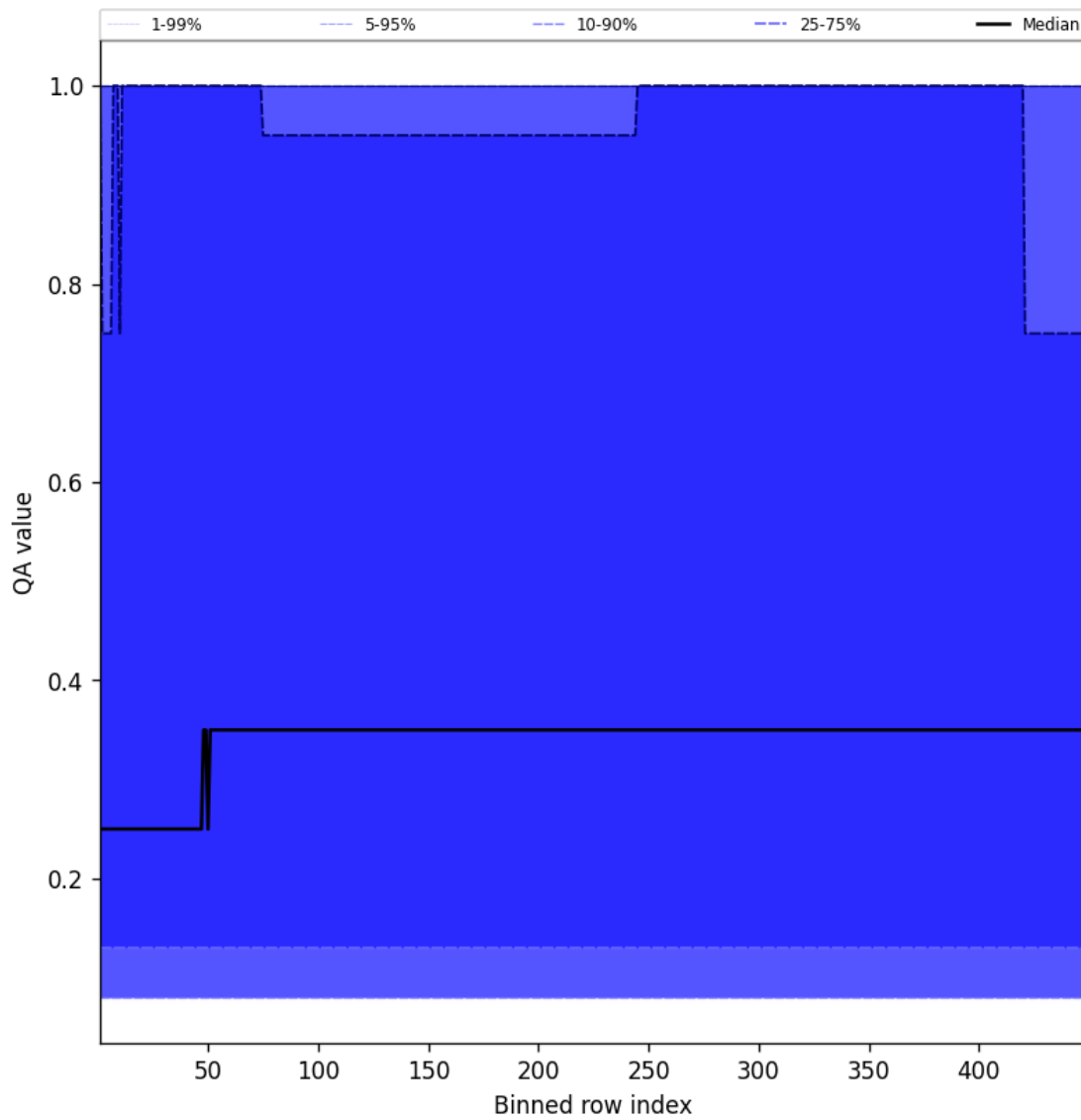
Figure 46: Along track statistics of “QA value” for 2025-04-07 to 2025-04-08
