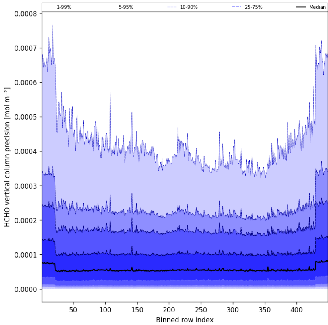
Figure 48: Along track statistics of “HCHO vertical column precision” for 2025-04-07 to 2025-04-08
