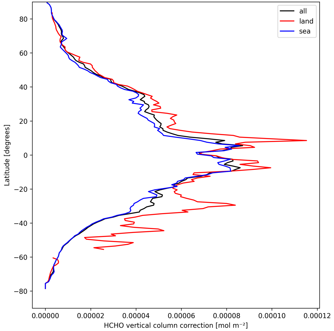
Figure 21: Zonal average of “HCHO vertical column correction” for 2025-04-07 to 2025-04-08.
