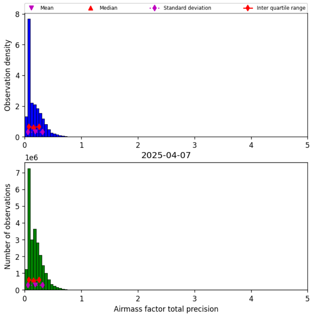
Figure 39: Histogram of “Airmass factor total precision” for 2025-04-07 to 2025-04-08
