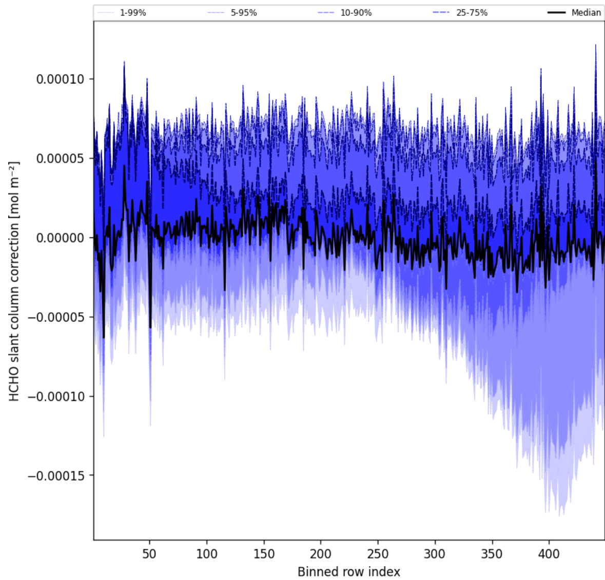
Figure 59: Along track statistics of “HCHO slant column correction” for 2025-04-07 to 2025-04-08
