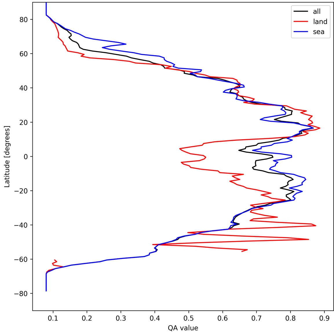
Figure 18: Zonal average of “QA value” for 2025-04-07 to 2025-04-08.
