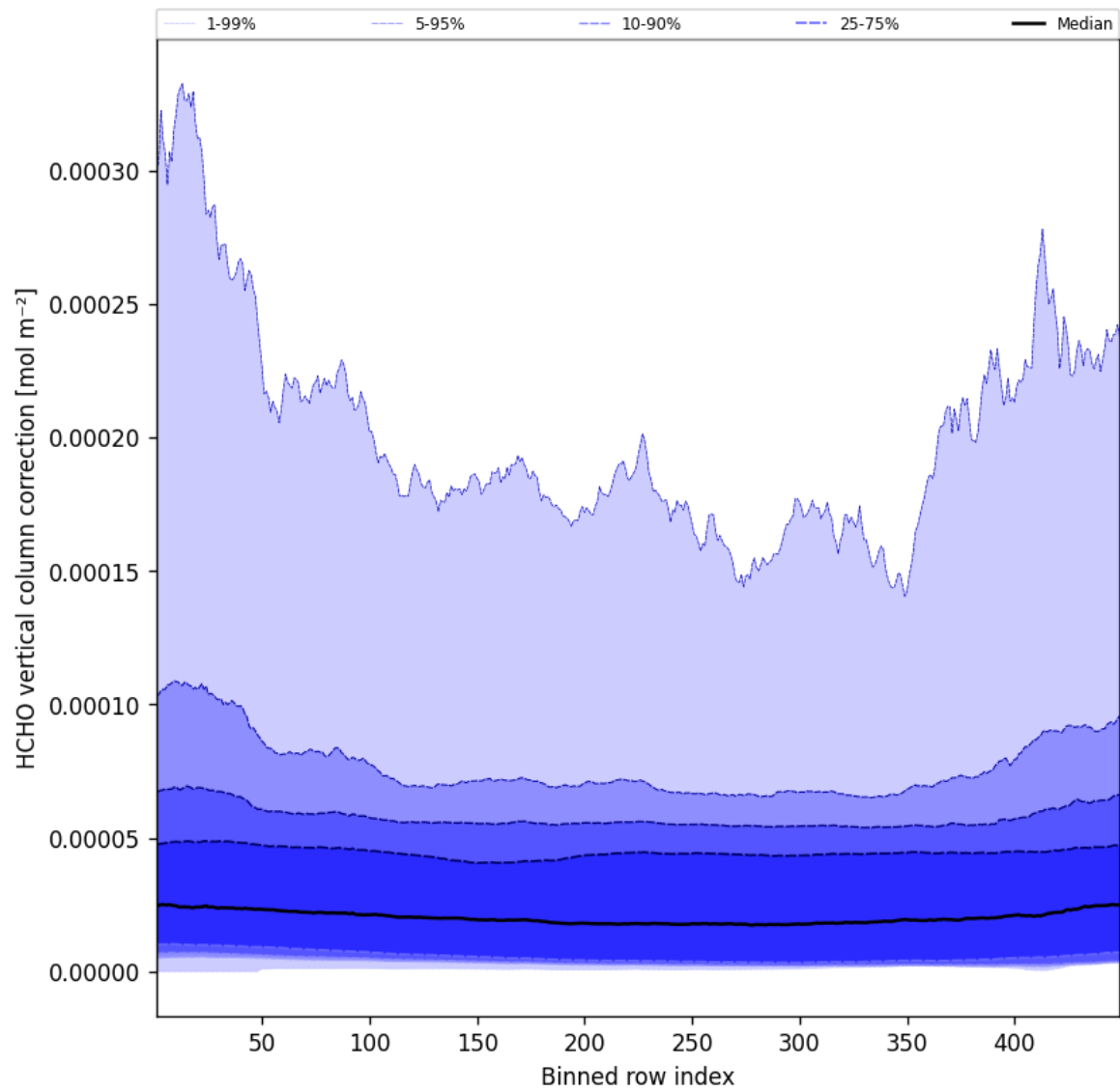
Figure 49: Along track statistics of “HCHO vertical column correction” for 2025-04-07 to 2025-04-08
