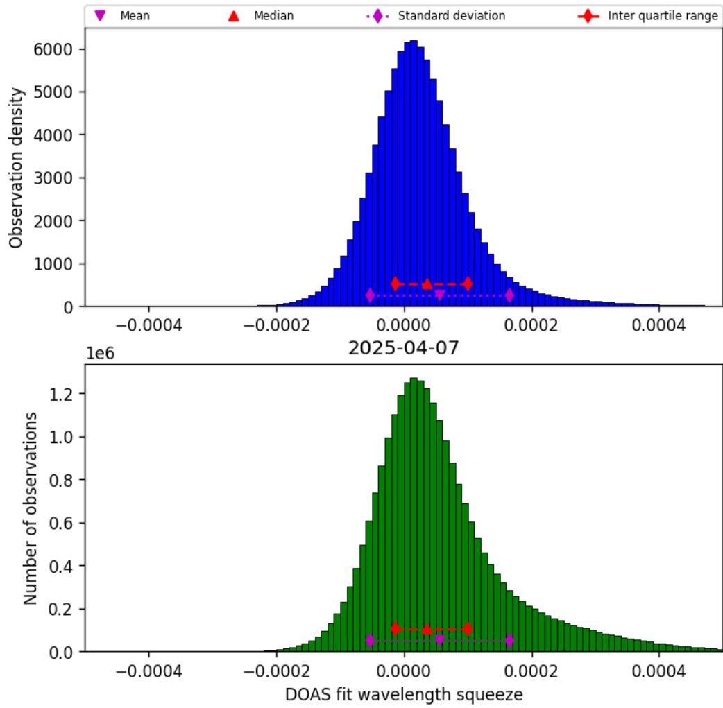
Figure 43: Histogram of “DOAS fit wavelength squeeze” for 2025-04-07 to 2025-04-08
