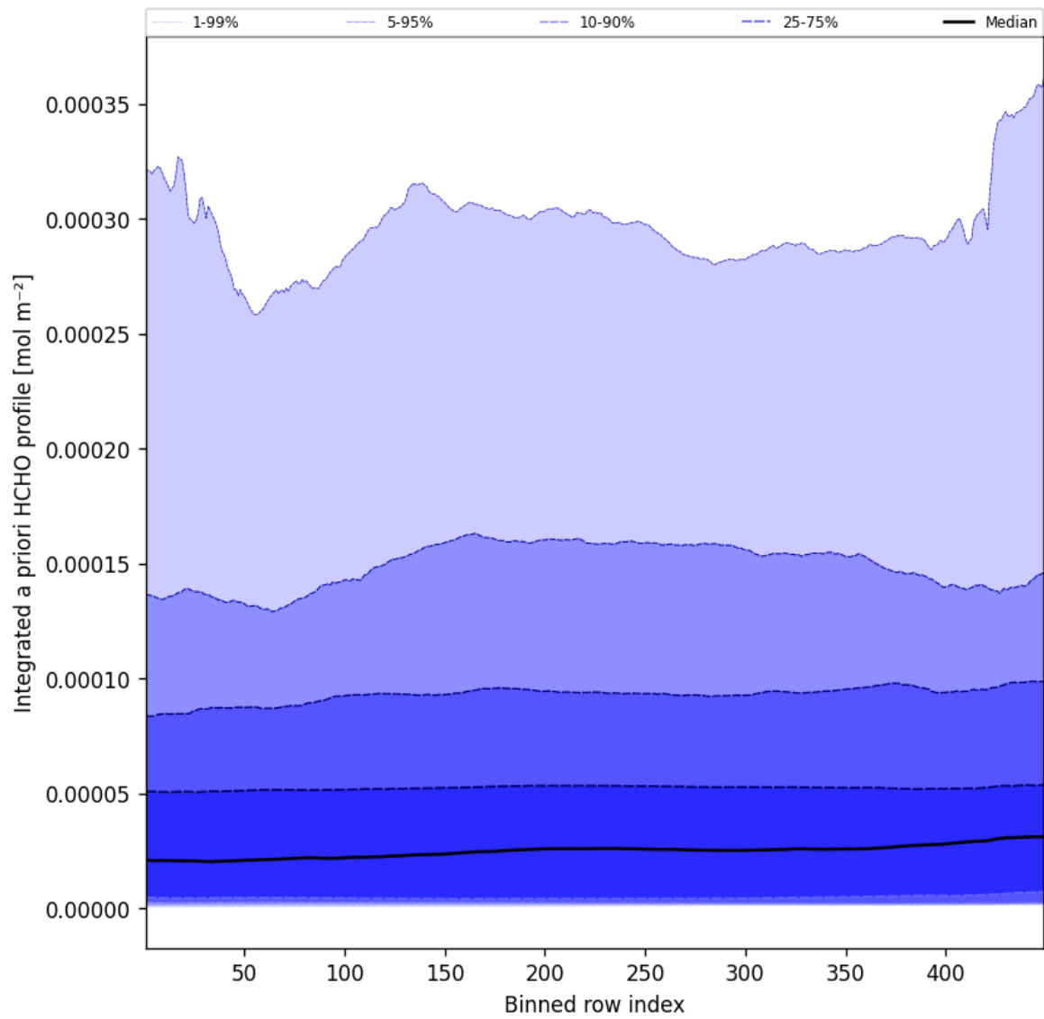
Figure 55: Along track statistics of “Integrated a priori HCHO profile” for 2025-04-07 to 2025-04-08
