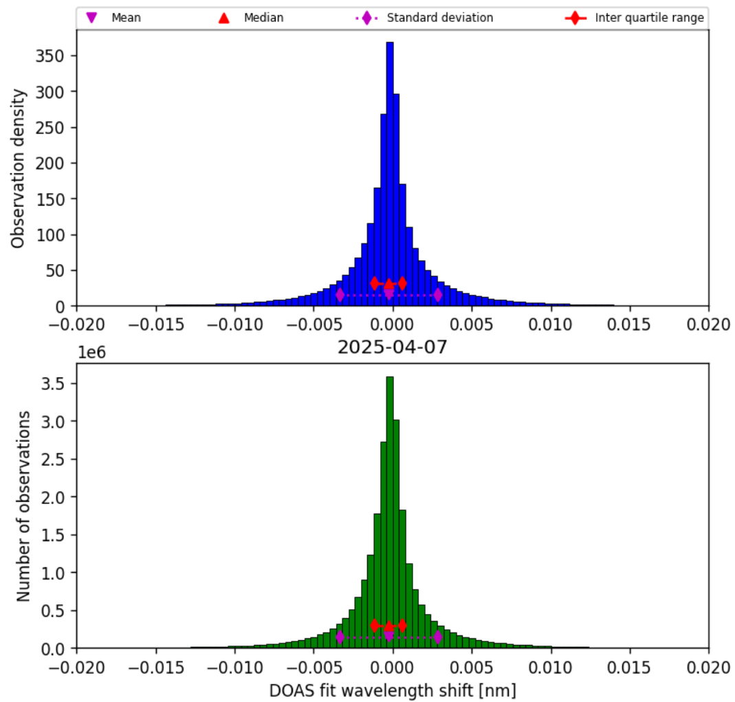
Figure 42: Histogram of “DOAS fit wavelength shift” for 2025-04-07 to 2025-04-08
