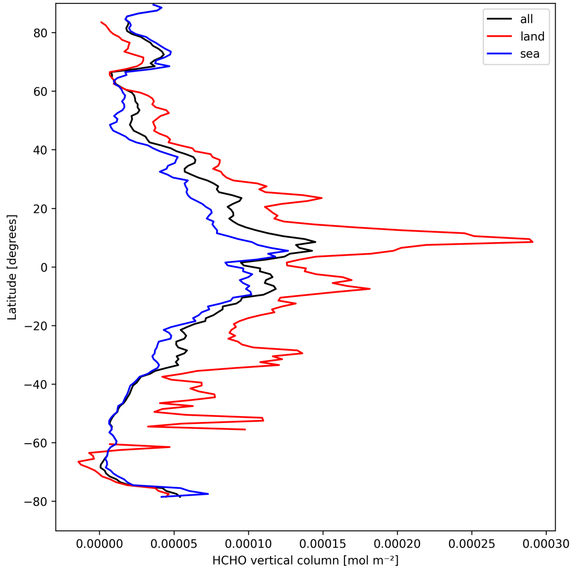
Figure 19: Zonal average of “HCHO vertical column” for 2025-04-07 to 2025-04-08.
