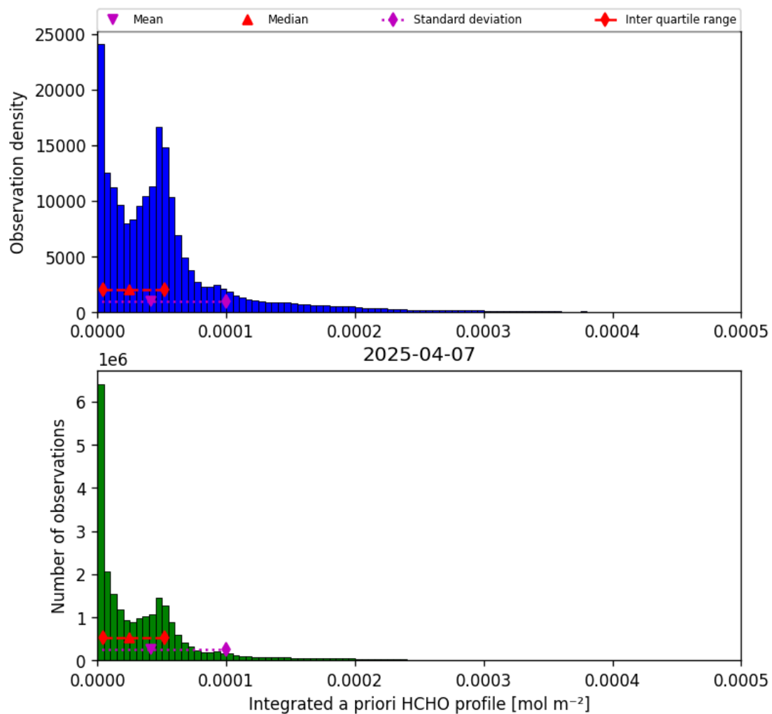
Figure 41: Histogram of “Integrated a priori HCHO profile” for 2025-04-07 to 2025-04-08
