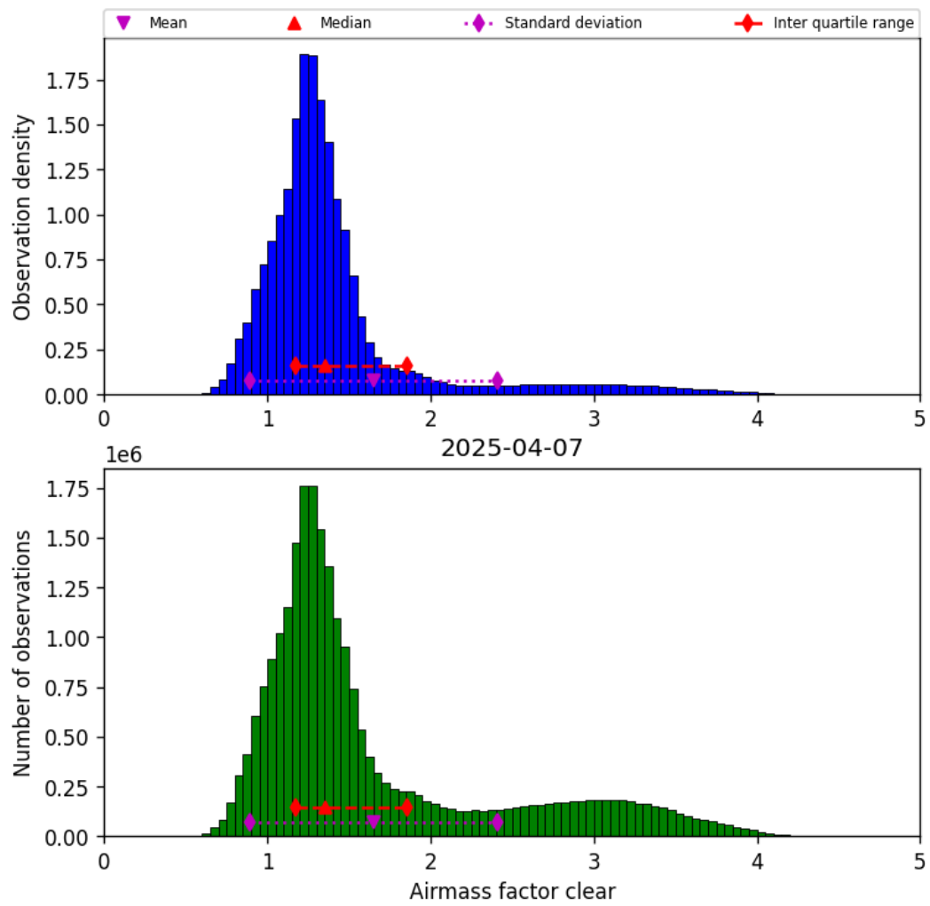
Figure 40: Histogram of “Airmass factor clear” for 2025-04-07 to 2025-04-08
