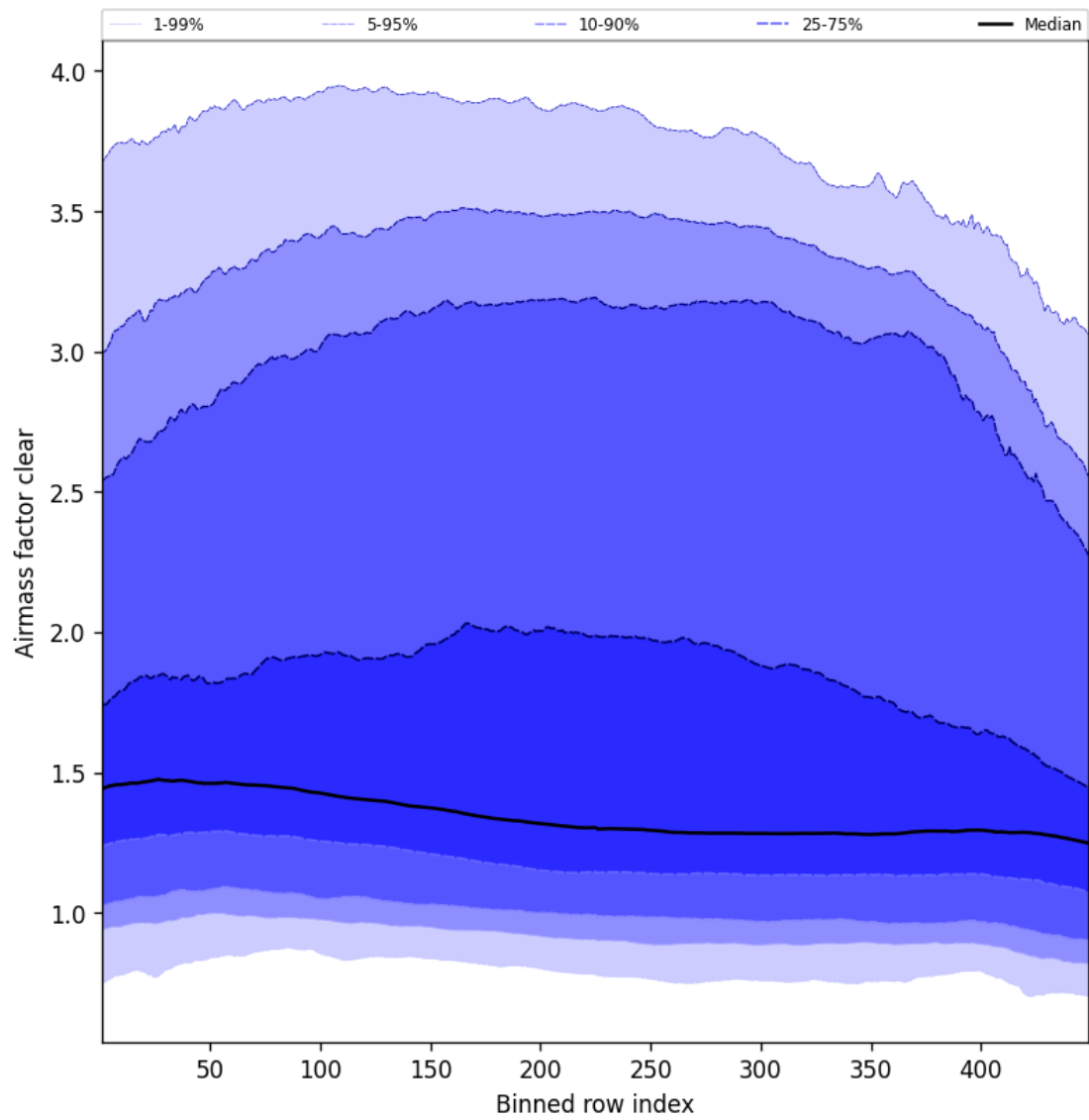
Figure 54: Along track statistics of “Airmass factor clear” for 2025-04-07 to 2025-04-08
