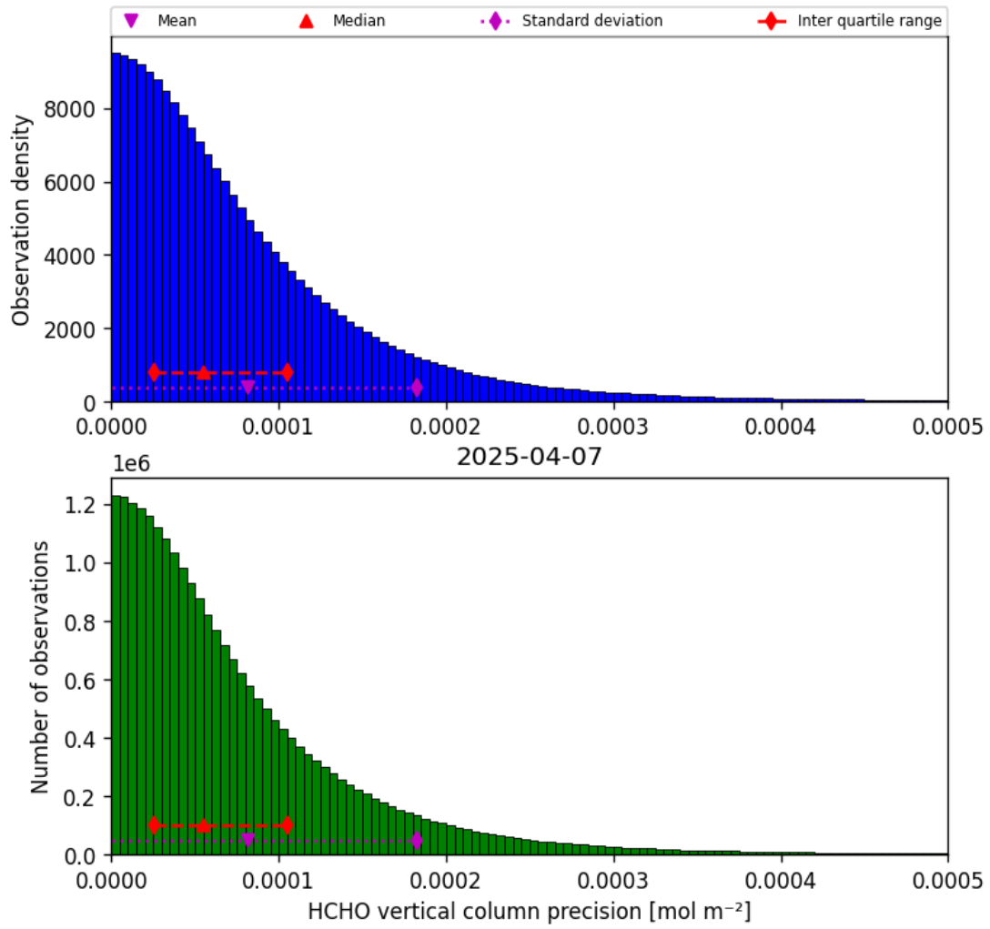
Figure 34: Histogram of “HCHO vertical column precision” for 2025-04-07 to 2025-04-08
