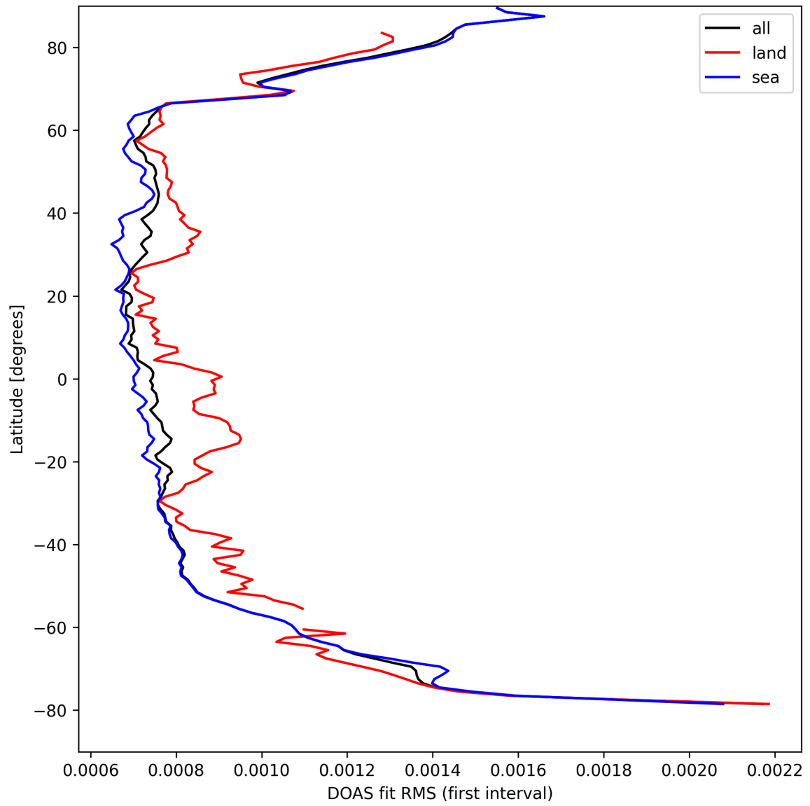
Figure 30: Zonal average of “DOAS fit RMS (first interval)” for 2025-04-07 to 2025-04-08.
