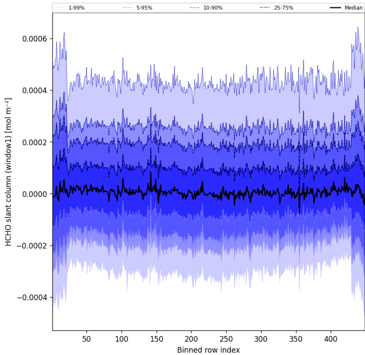
Figure 50: Along track statistics of “HCHO slant column (window1)” for 2025-04-07 to 2025-04-08
