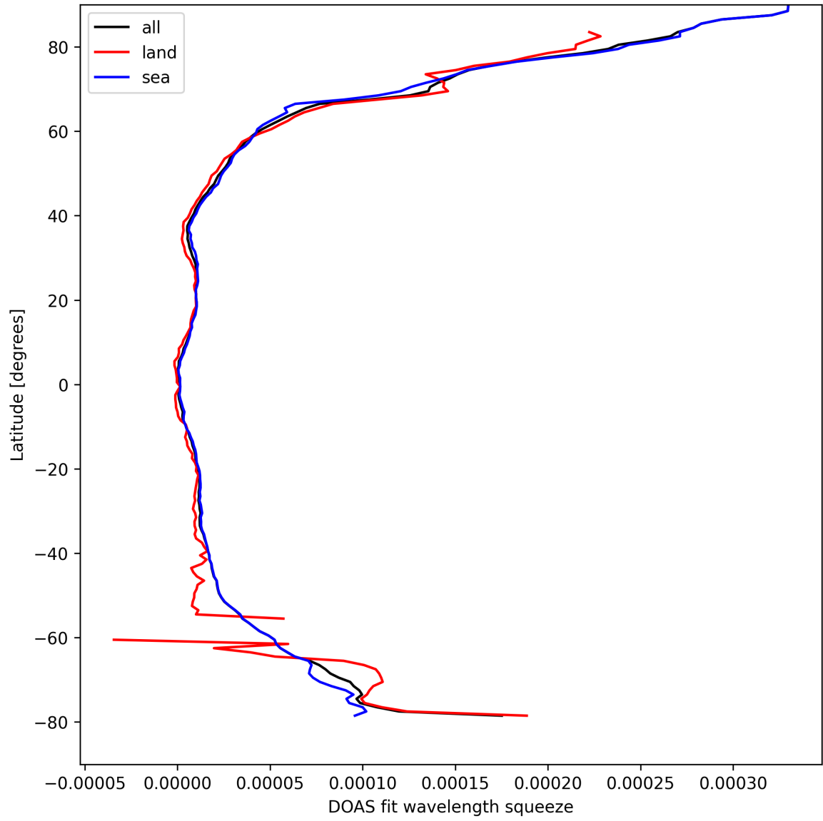
Figure 29: Zonal average of “DOAS fit wavelength squeeze” for 2025-04-07 to 2025-04-08.
