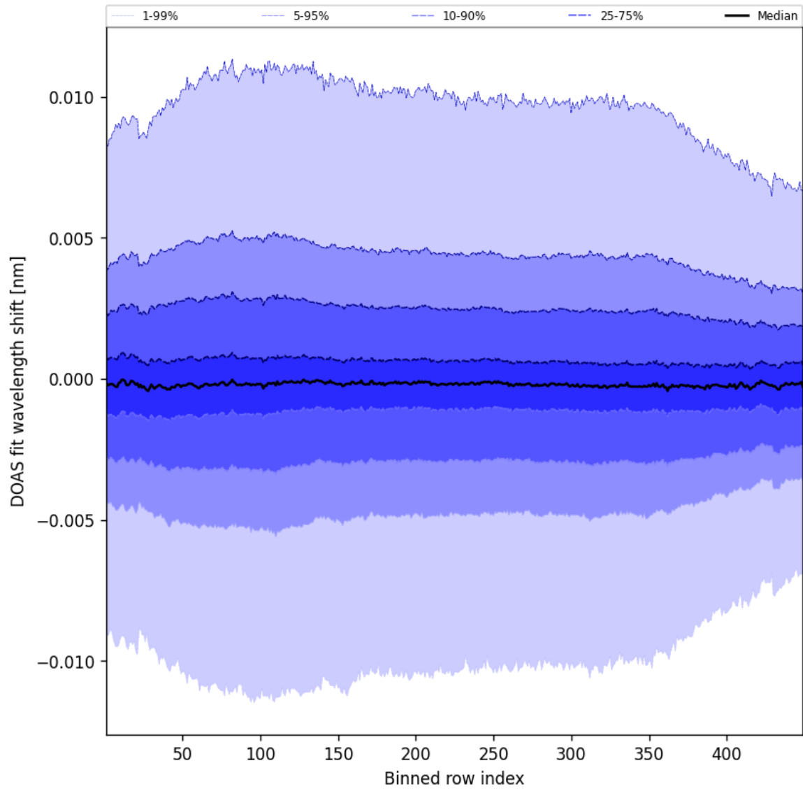
Figure 56: Along track statistics of “DOAS fit wavelength shift” for 2025-04-07 to 2025-04-08
