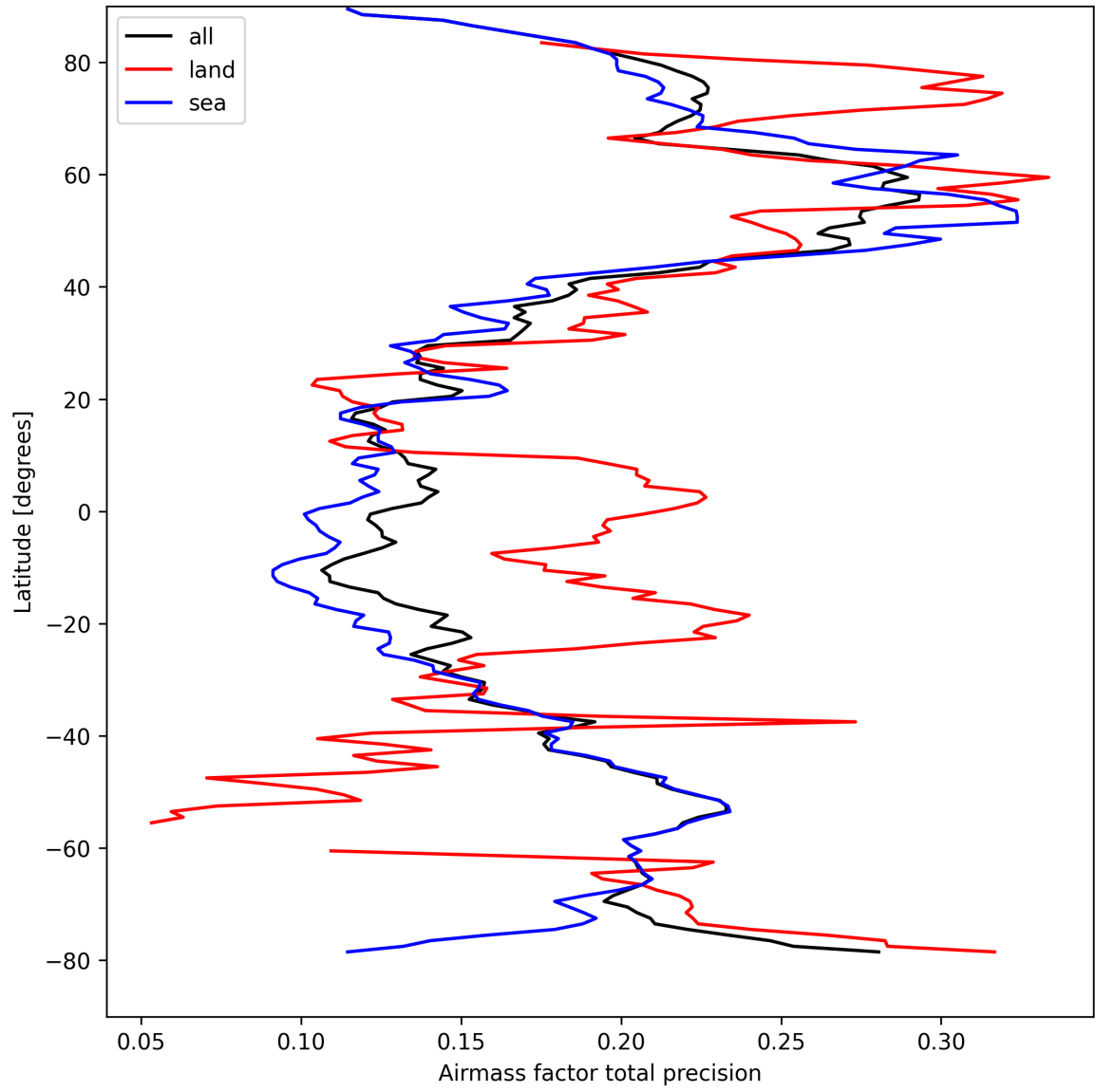
Figure 25: Zonal average of “Airmass factor total precision” for 2025-04-07 to 2025-04-08.
