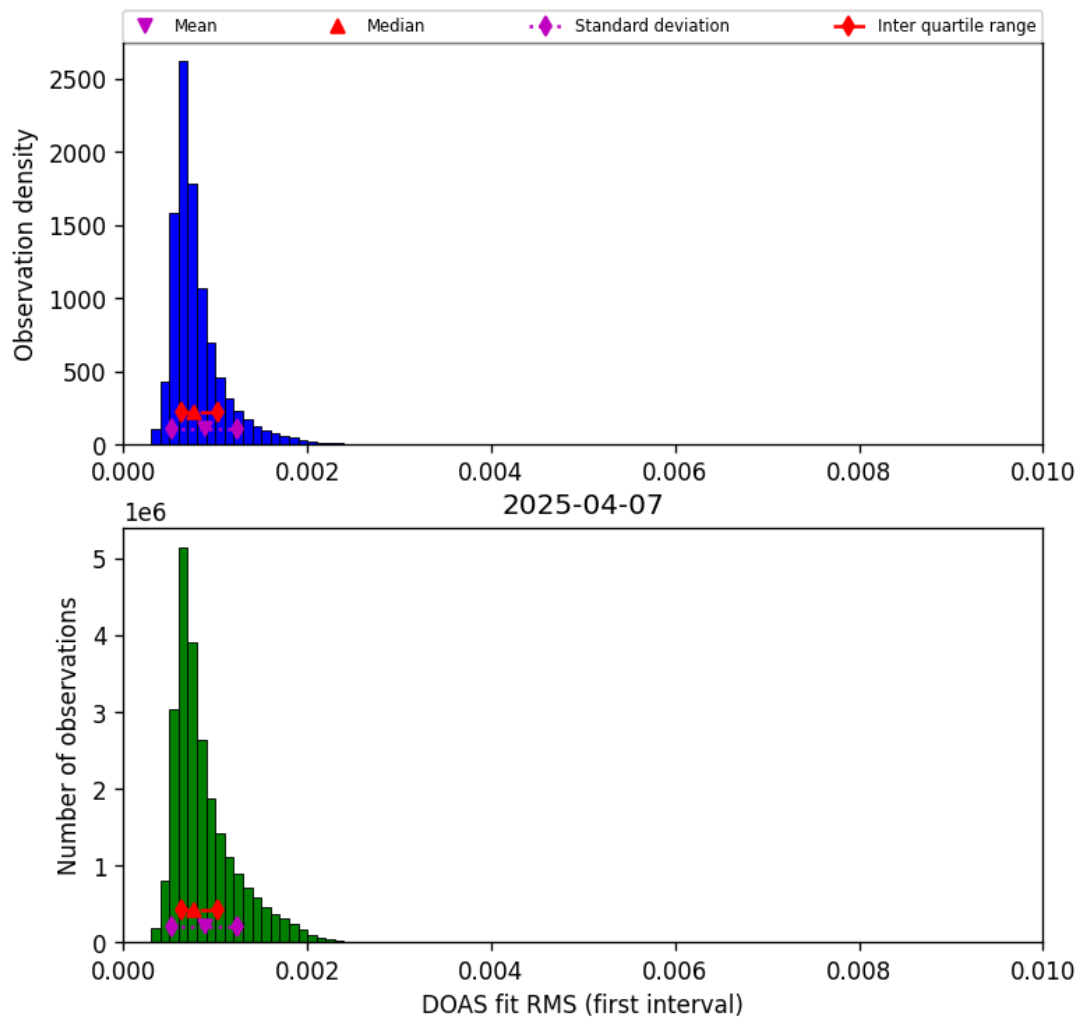
Figure 44: Histogram of “DOAS fit RMS (first interval)” for 2025-04-07 to 2025-04-08
