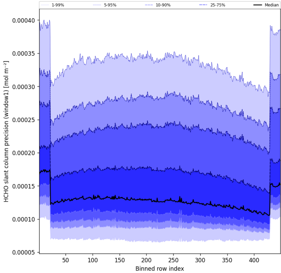
Figure 51: Along track statistics of “HCHO slant column precision (window1)” for 2025-04-07 to 2025-04-08
