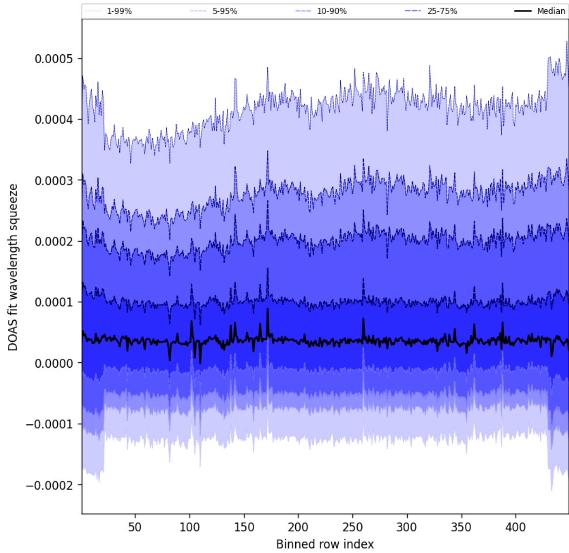
Figure 57: Along track statistics of “DOAS fit wavelength squeeze” for 2025-04-07 to 2025-04-08
