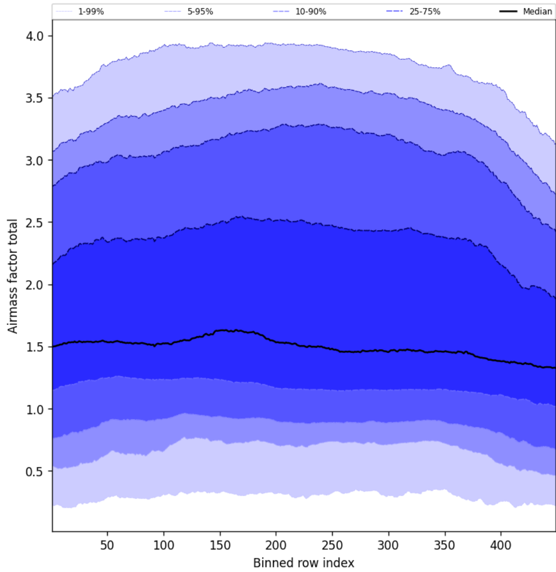
Figure 52: Along track statistics of “Airmass factor total” for 2025-04-07 to 2025-04-08
