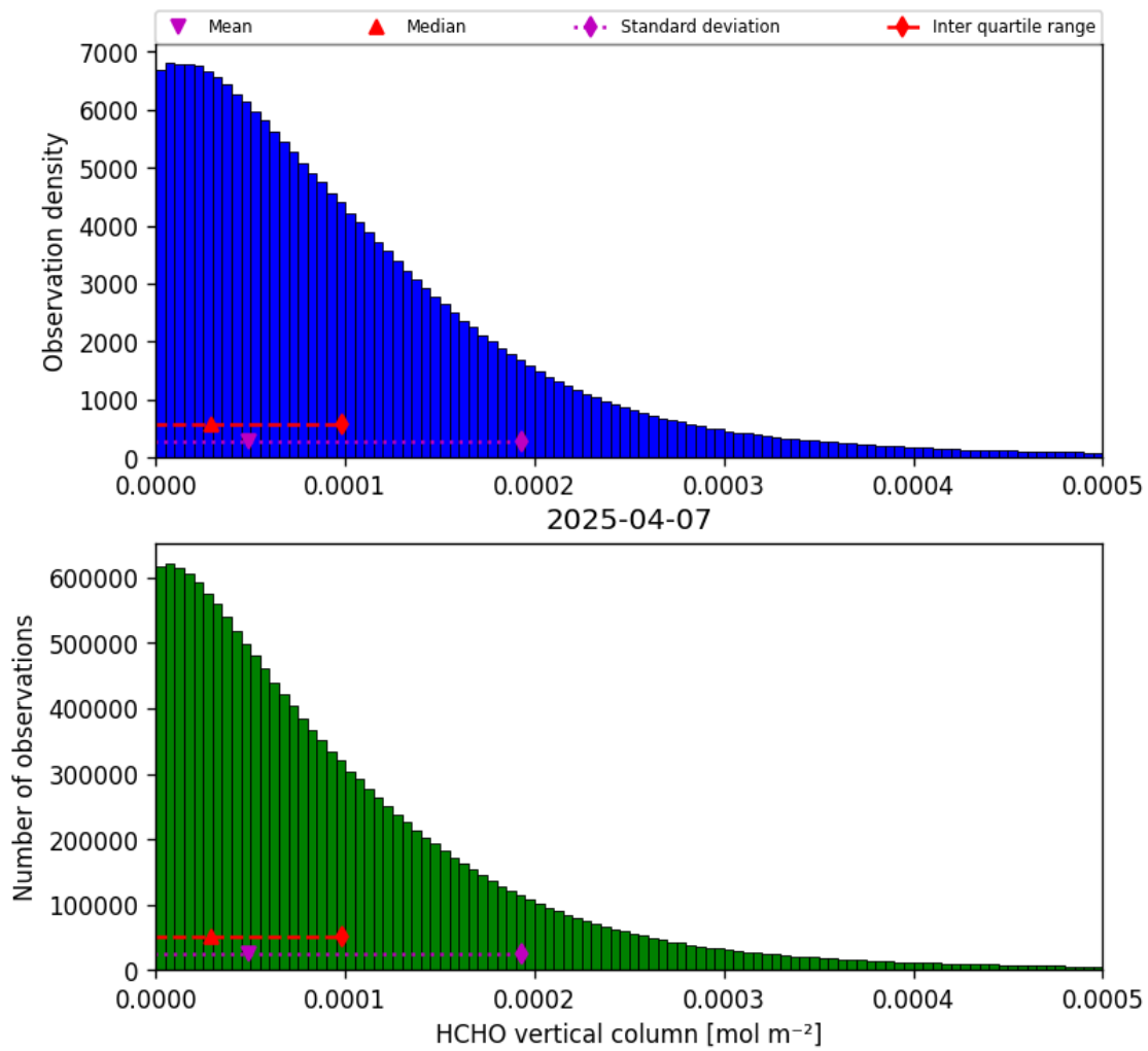
Figure 33: Histogram of “HCHO vertical column” for 2025-04-07 to 2025-04-08
