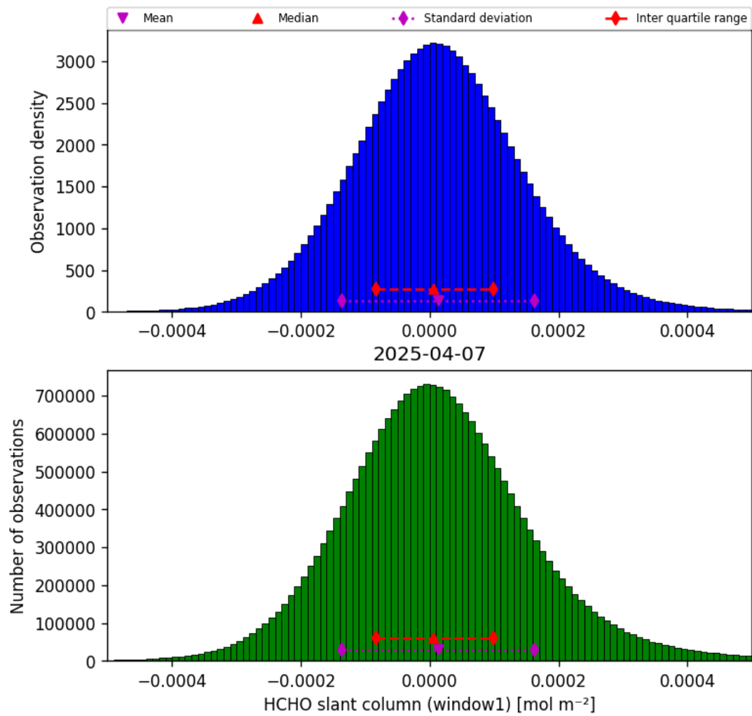
Figure 36: Histogram of “HCHO slant column (window1)” for 2025-04-07 to 2025-04-08
