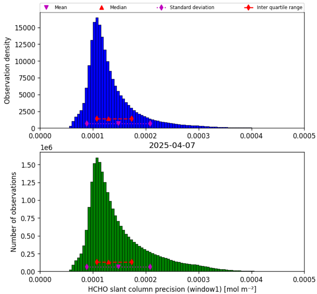
Figure 37: Histogram of “HCHO slant column precision (window1)” for 2025-04-07 to 2025-04-08
