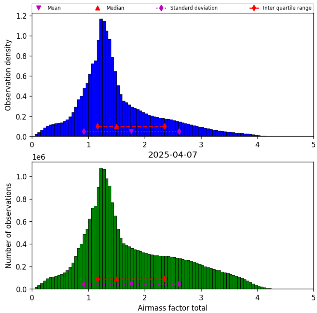
Figure 38: Histogram of “Airmass factor total” for 2025-04-07 to 2025-04-08
