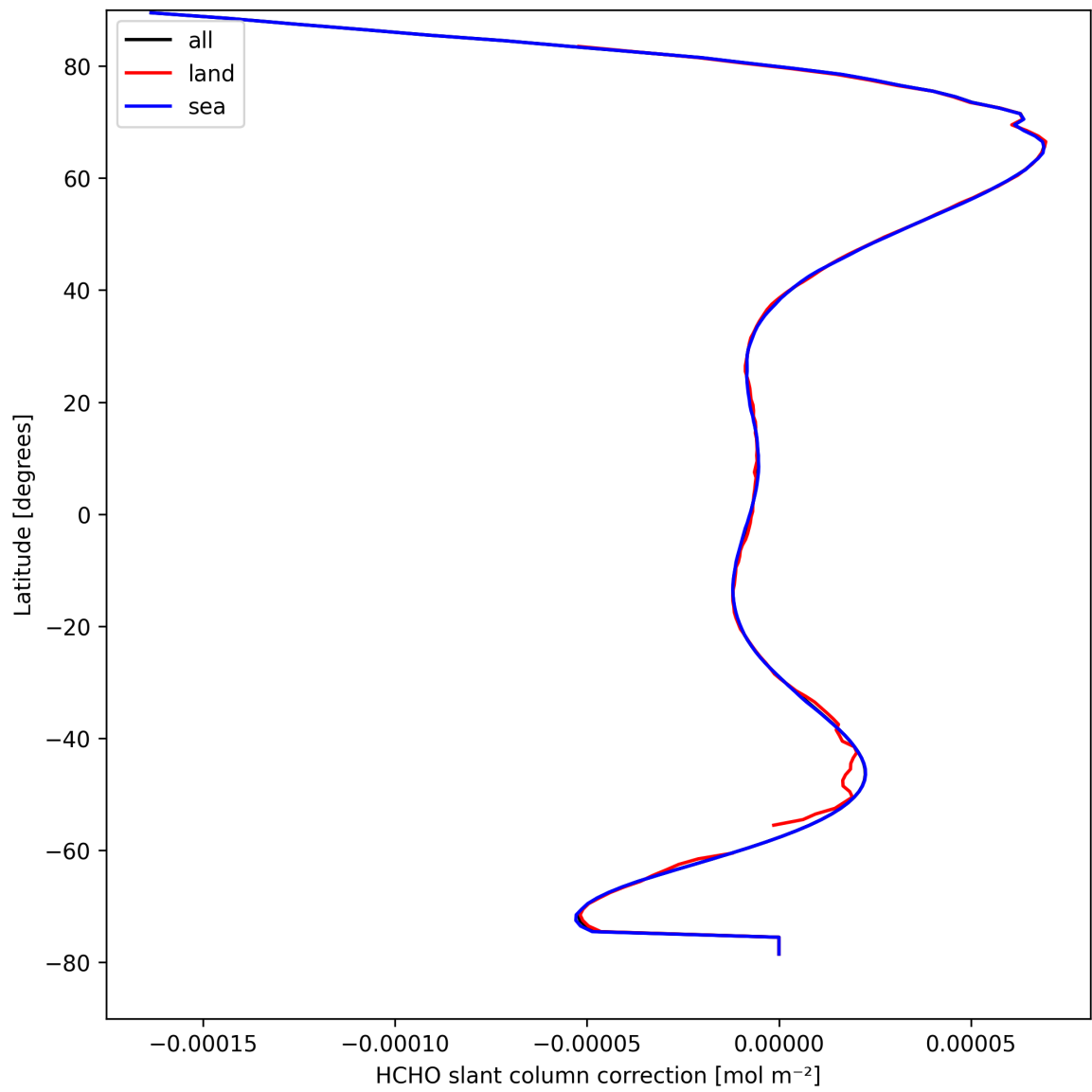
Figure 31: Zonal average of "HCHO slant column correction" for 2025-04-07 to 2025-04-08.
