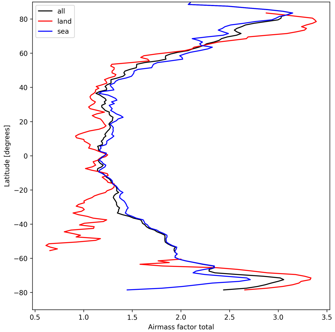
Figure 24: Zonal average of “Airmass factor total” for 2025-04-07 to 2025-04-08.
