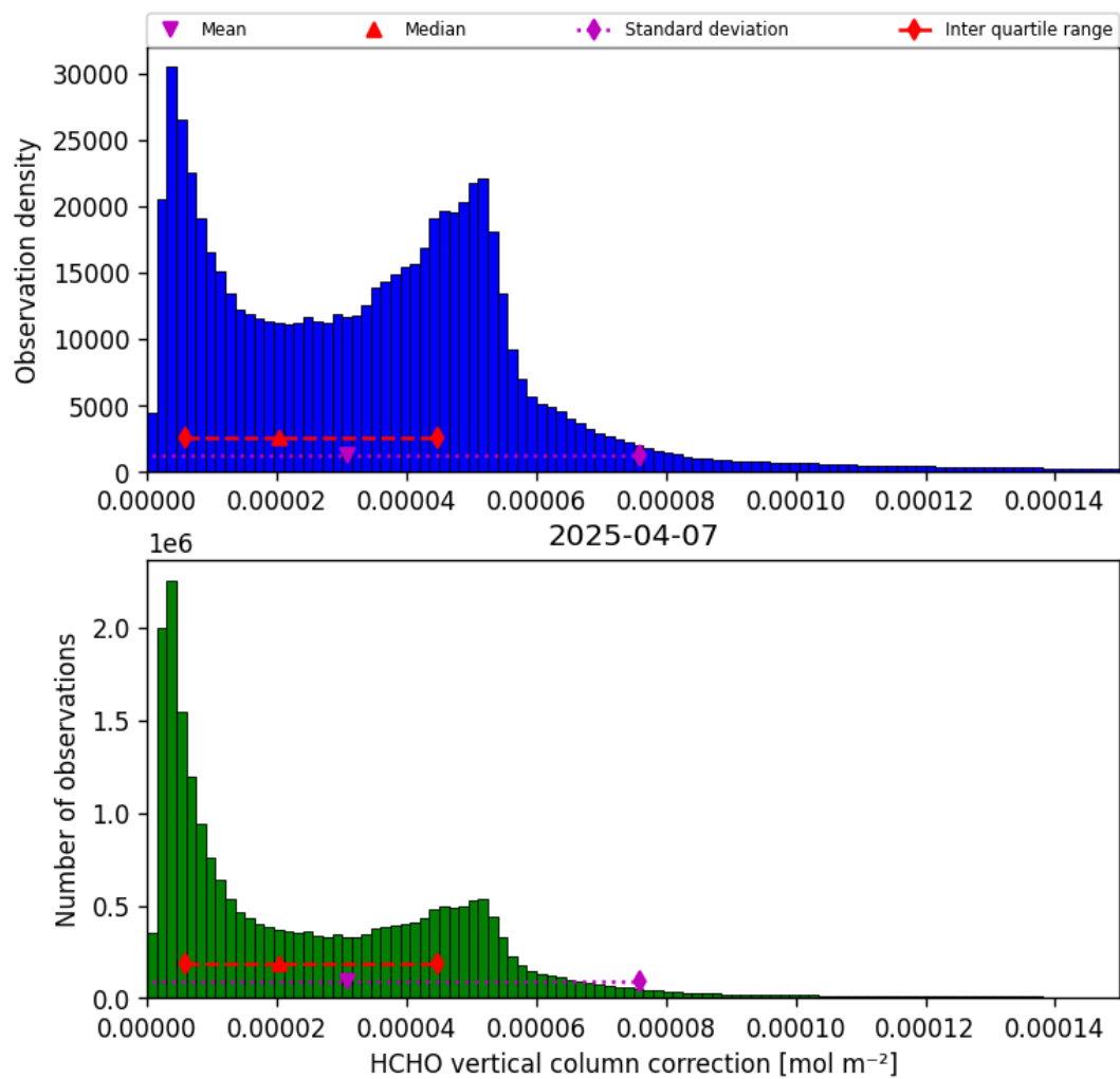
Figure 35: Histogram of “HCHO vertical column correction” for 2025-04-07 to 2025-04-08
