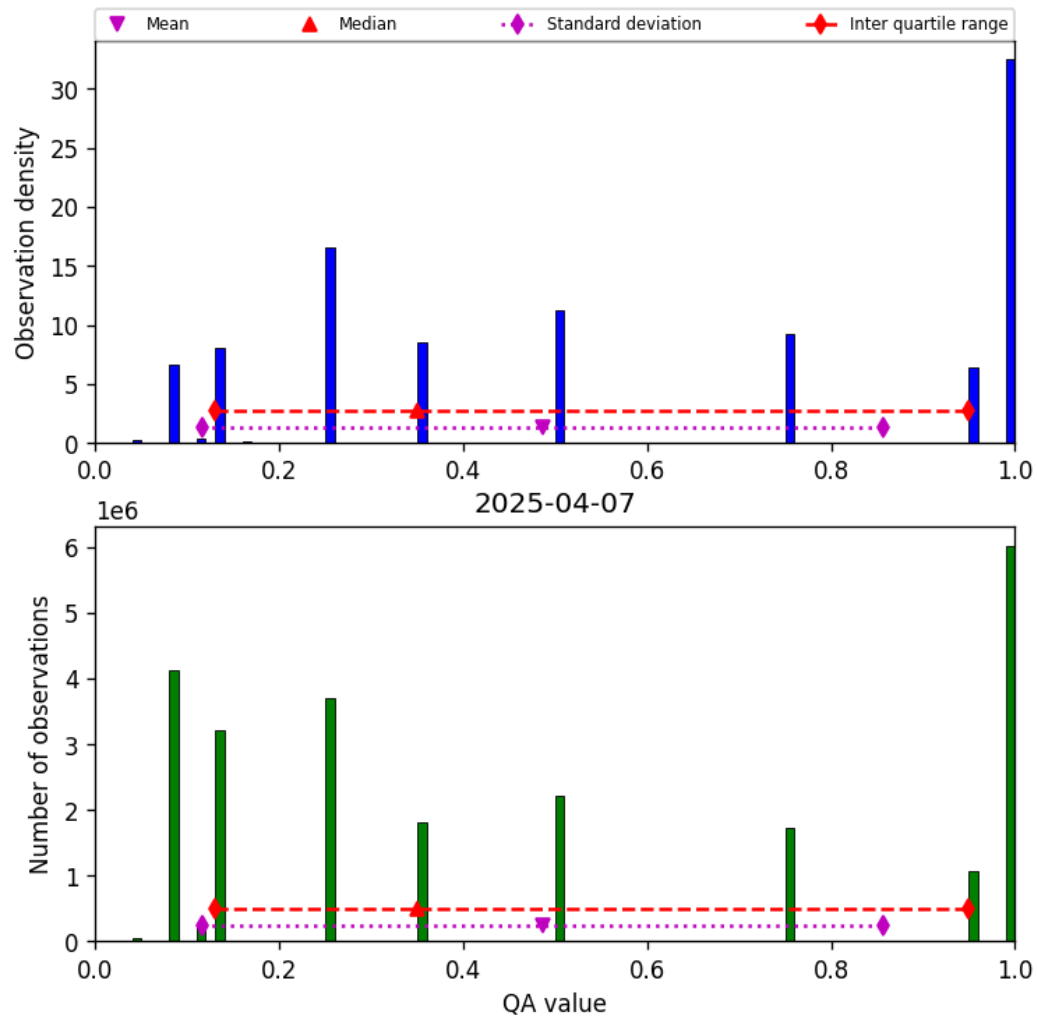
Figure 32: Histogram of “QA value” for 2025-04-07 to 2025-04-08
