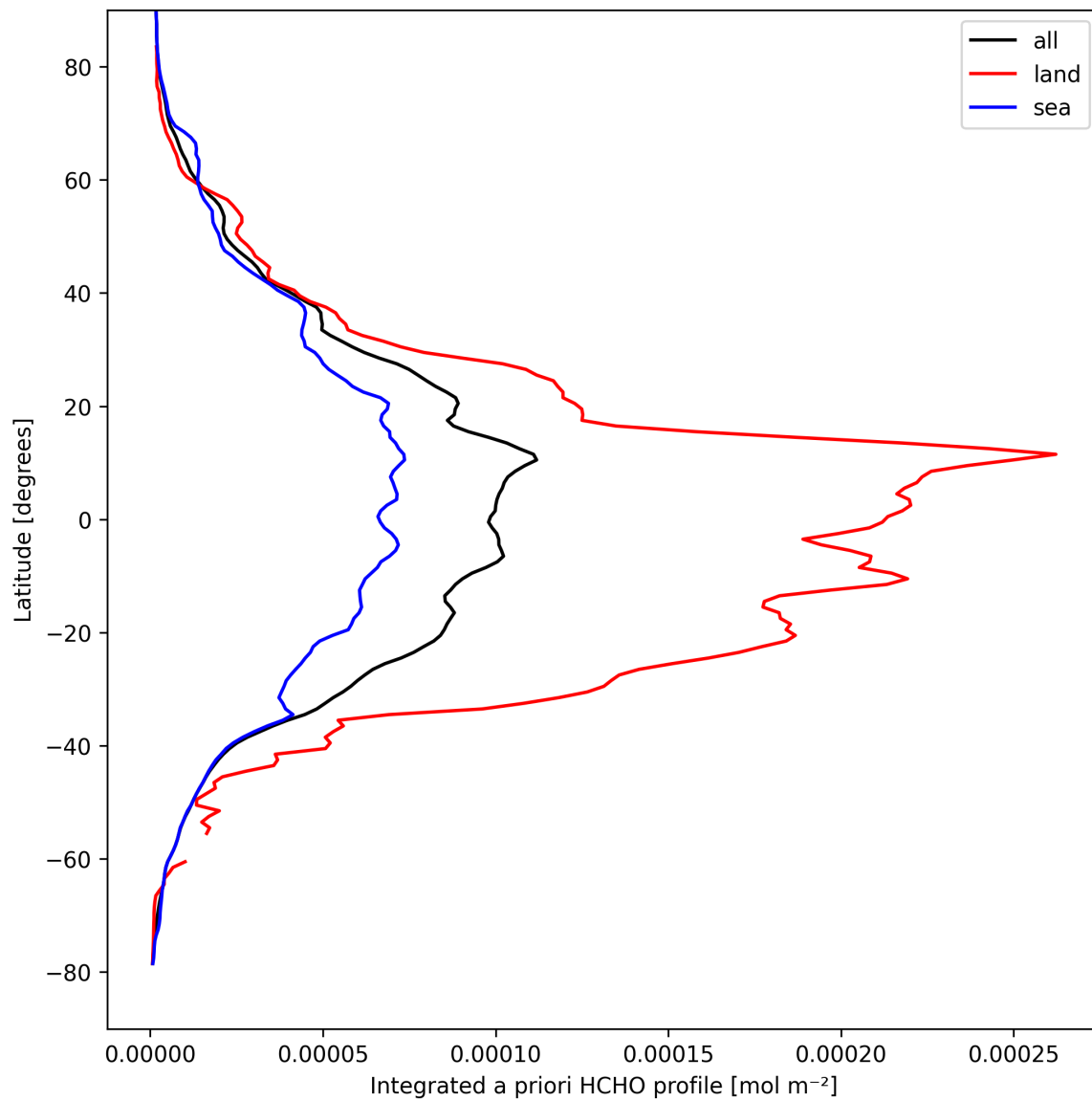
Figure 27: Zonal average of “Integrated a priori HCHO profile” for 2025-04-07 to 2025-04-08.
