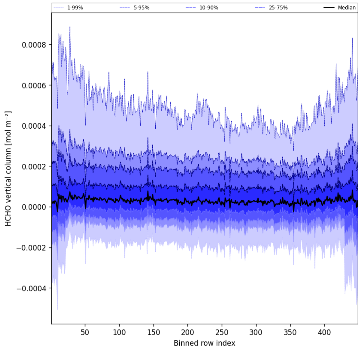
Figure 47: Along track statistics of “HCHO vertical column” for 2025-04-07 to 2025-04-08
