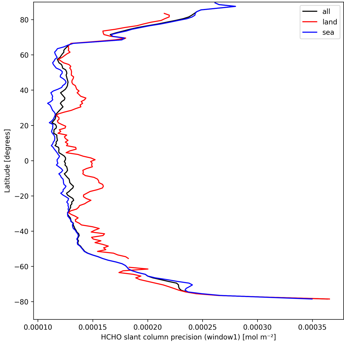
Figure 23: Zonal average of “HCHO slant column precision (window1)” for 2025-04-07 to 2025-04-08.
