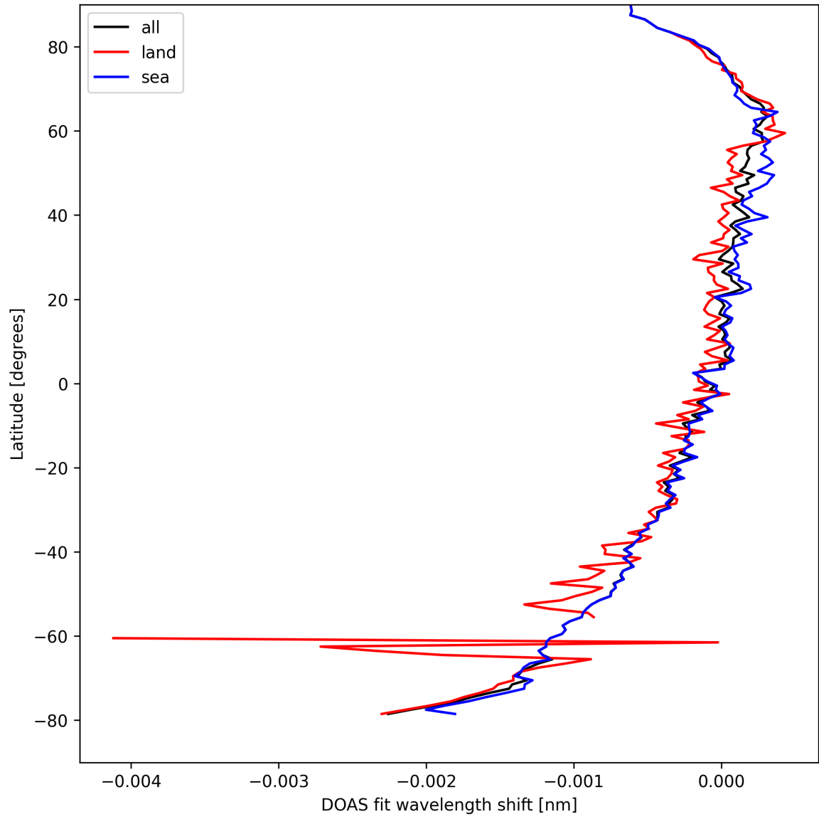
Figure 28: Zonal average of “DOAS fit wavelength shift” for 2025-04-07 to 2025-04-08.
