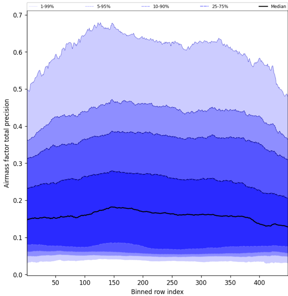
Figure 53: Along track statistics of “Airmass factor total precision” for 2025-04-07 to 2025-04-08
