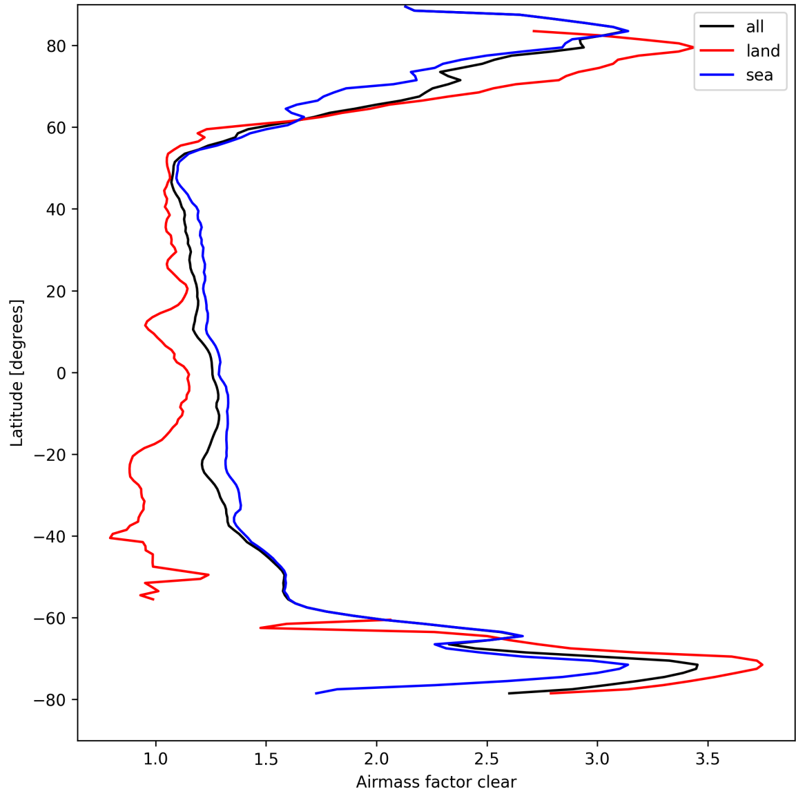
Figure 26: Zonal average of “Airmass factor clear” for 2025-04-07 to 2025-04-08.
