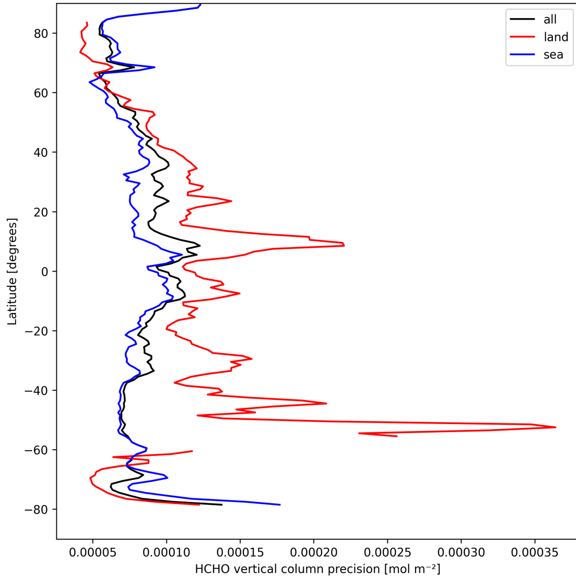
Figure 20: Zonal average of “HCHO vertical column precision” for 2025-04-07 to 2025-04-08.
