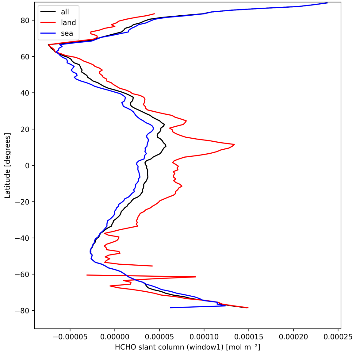
Figure 22: Zonal average of “HCHO slant column (window1)” for 2025-04-07 to 2025-04-08.
