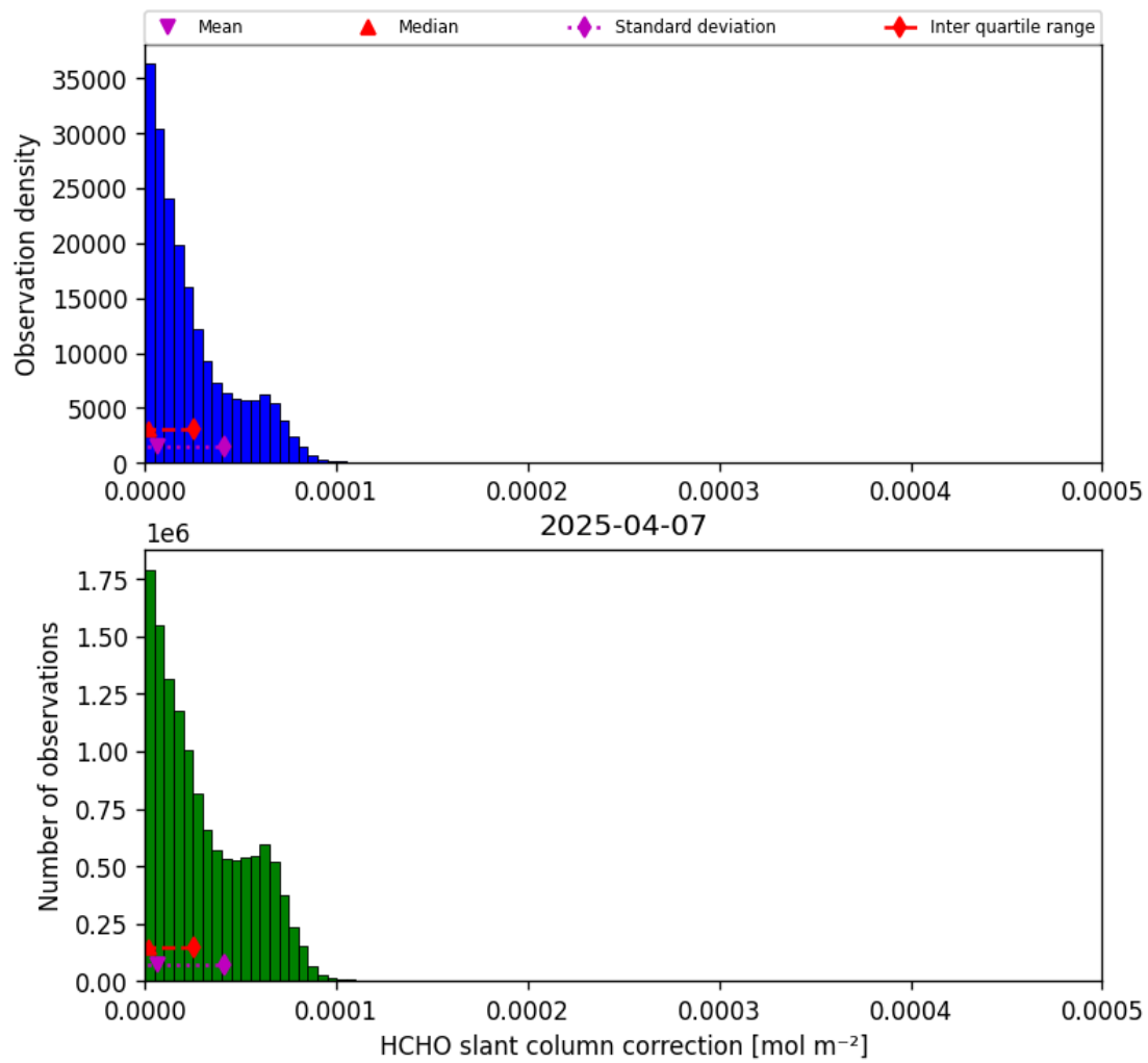
Figure 45: Histogram of “HCHO slant column correction” for 2025-04-07 to 2025-04-08
