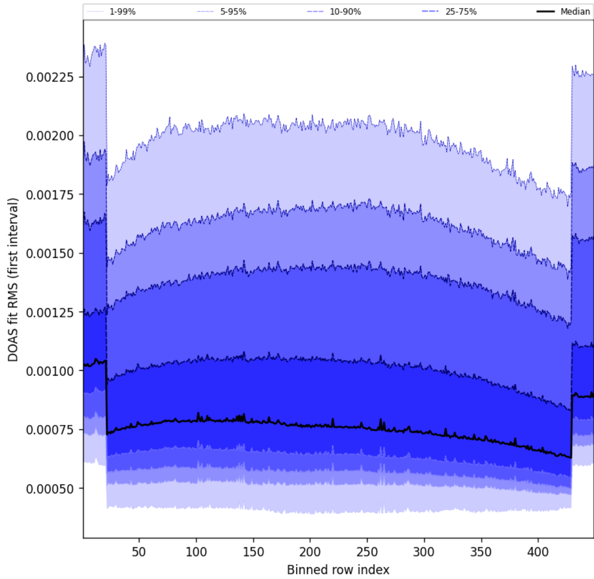
Figure 58: Along track statistics of “DOAS fit RMS (first interval)” for 2025-04-07 to 2025-04-08
