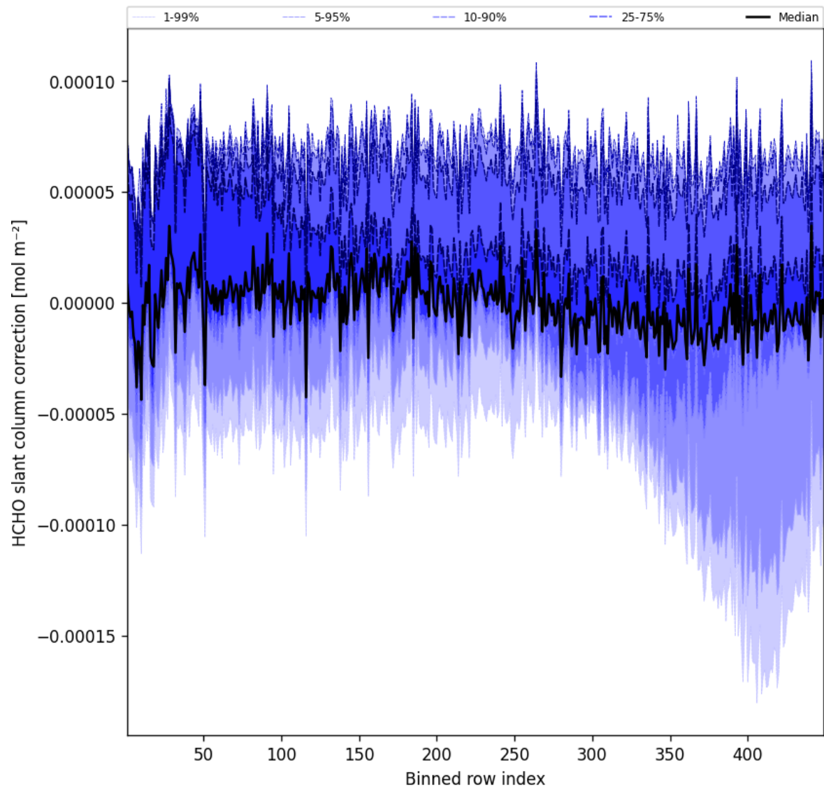
Figure 59: Along track statistics of “HCHO slant column correction” for 2025-04-08 to 2025-04-09
