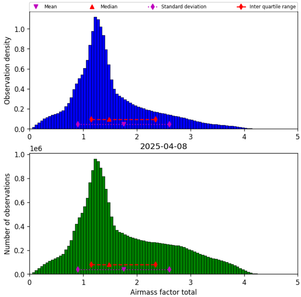
Figure 38: Histogram of “Airmass factor total” for 2025-04-08 to 2025-04-09
