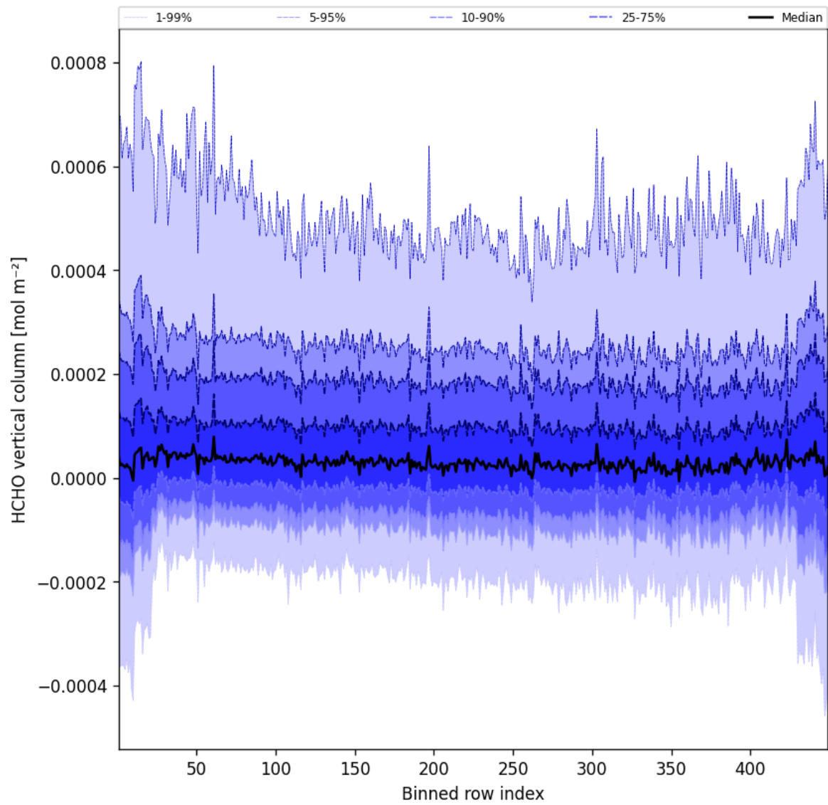
Figure 47: Along track statistics of “HCHO vertical column” for 2025-04-08 to 2025-04-09
