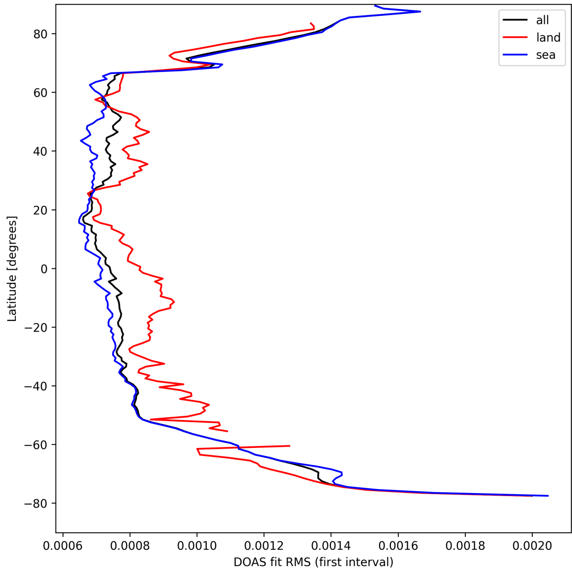
Figure 30: Zonal average of “DOAS fit RMS (first interval)” for 2025-04-08 to 2025-04-09.
