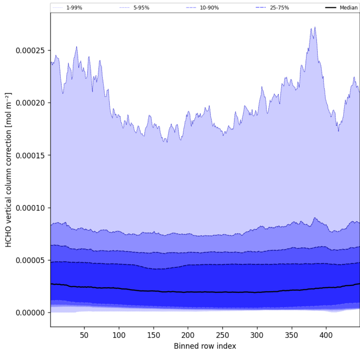
Figure 49: Along track statistics of “HCHO vertical column correction” for 2025-04-08 to 2025-04-09
