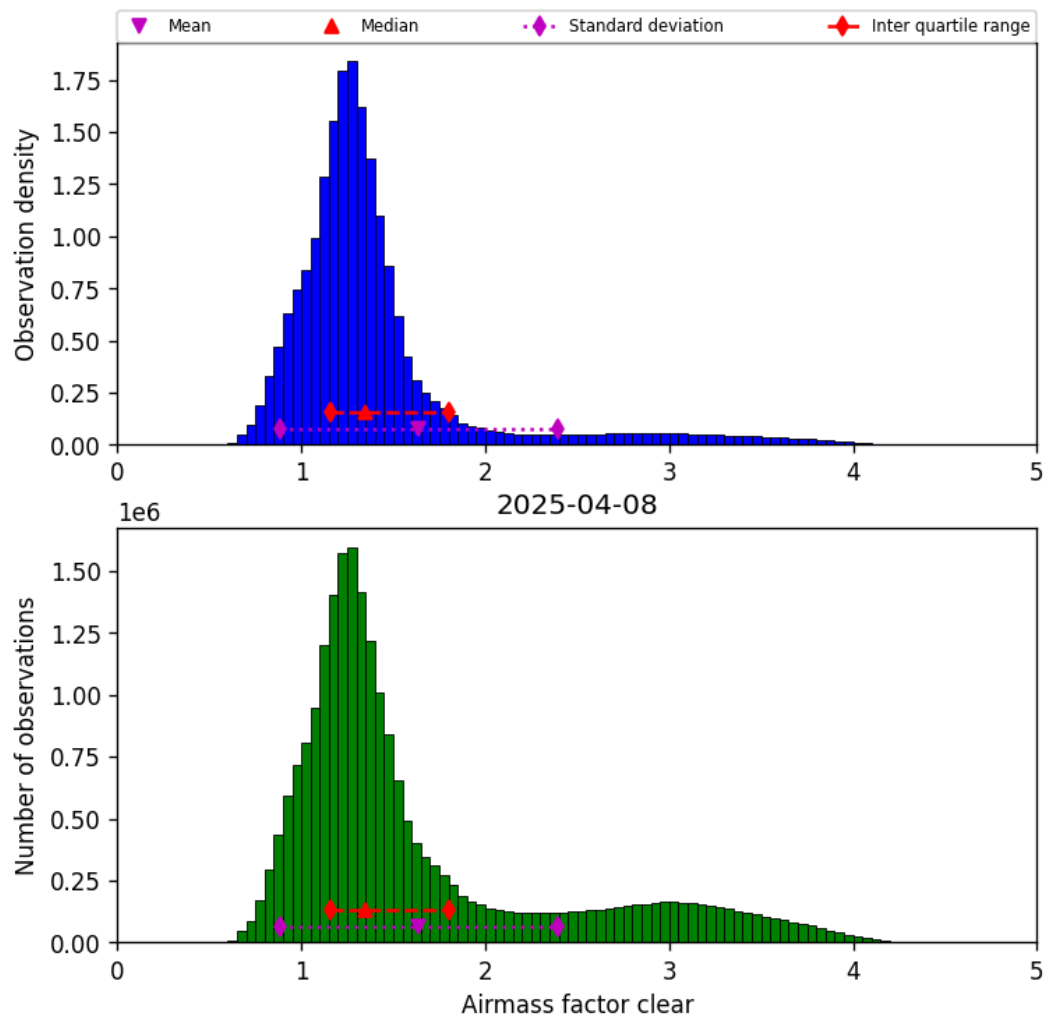
Figure 40: Histogram of “Airmass factor clear” for 2025-04-08 to 2025-04-09
