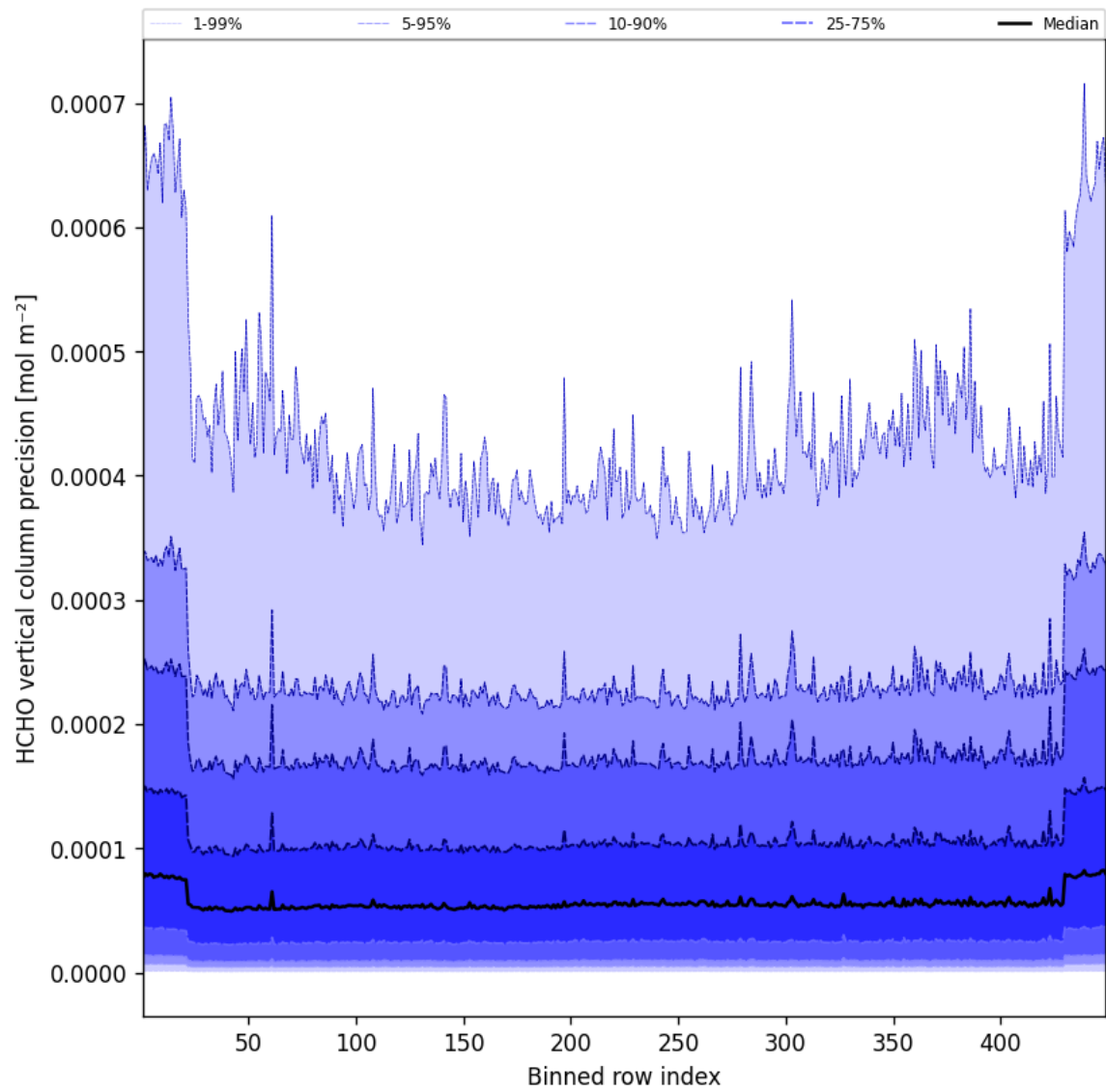
Figure 48: Along track statistics of "HCHO vertical column precision" for 2025-04-08 to 2025-04-09
