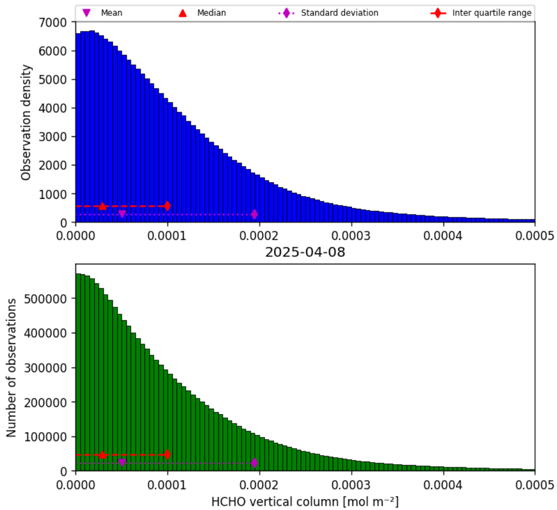
Figure 33: Histogram of “HCHO vertical column” for 2025-04-08 to 2025-04-09
