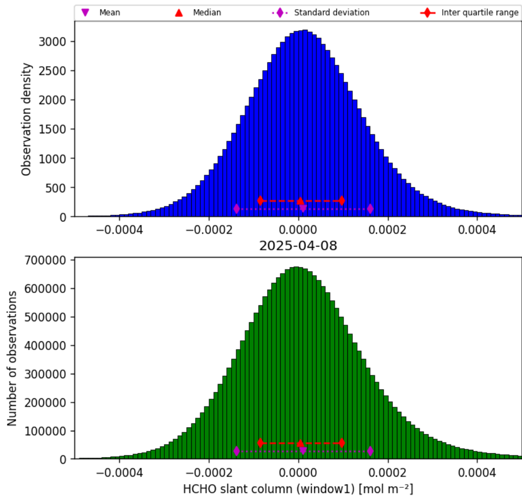
Figure 36: Histogram of “HCHO slant column (window1)” for 2025-04-08 to 2025-04-09
