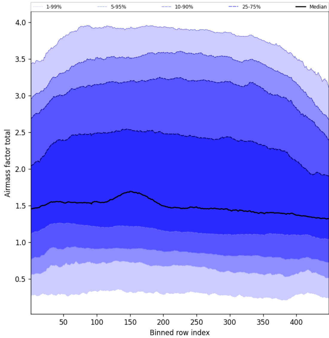
Figure 52: Along track statistics of “Airmass factor total” for 2025-04-08 to 2025-04-09
