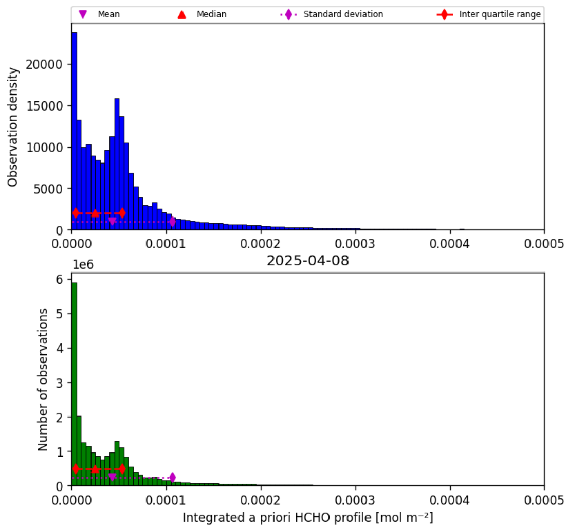
Figure 41: Histogram of “Integrated a priori HCHO profile” for 2025-04-08 to 2025-04-09
