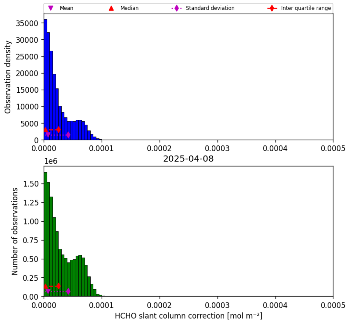
Figure 45: Histogram of “HCHO slant column correction” for 2025-04-08 to 2025-04-09
