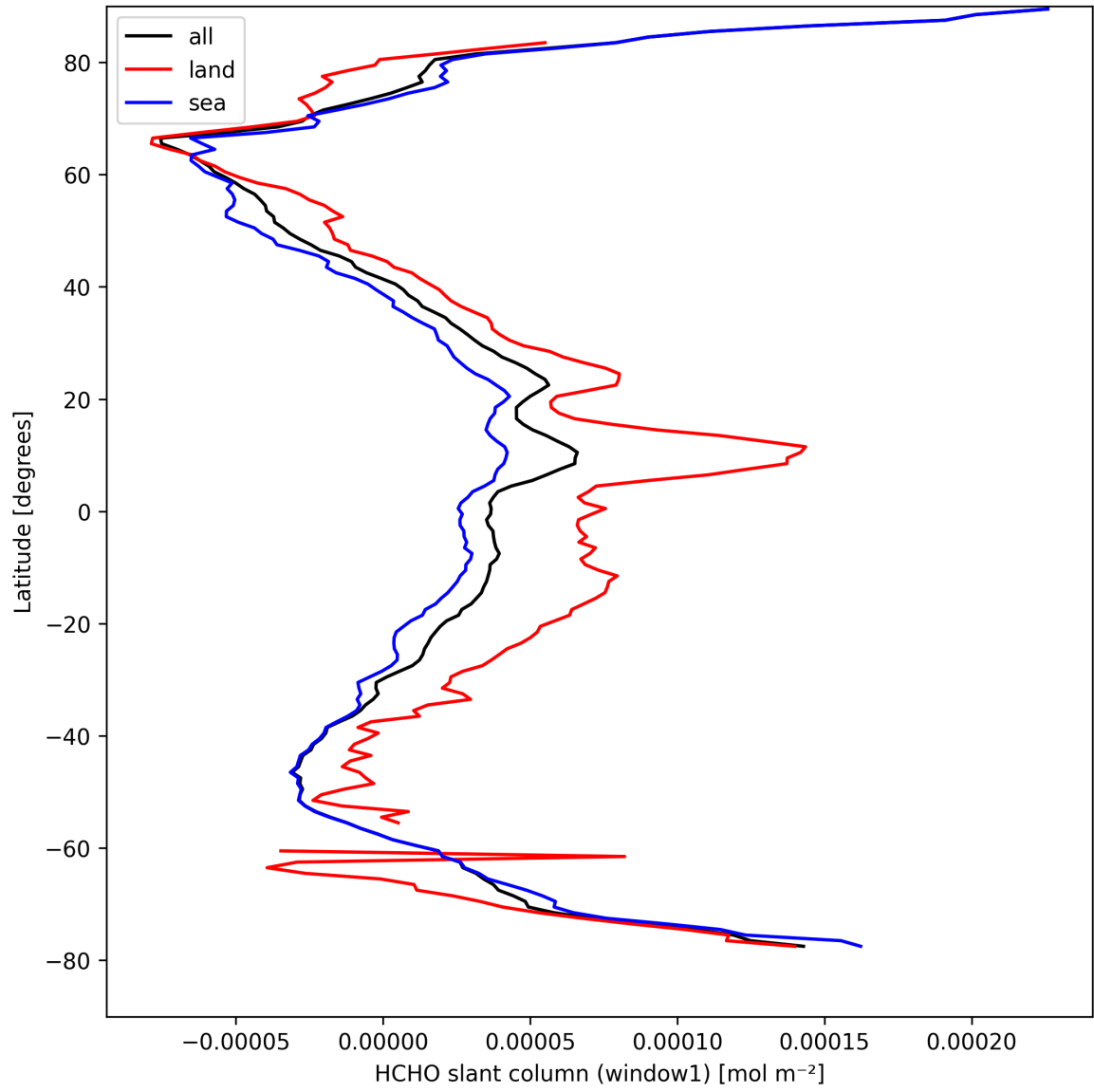
Figure 22: Zonal average of “HCHO slant column (window1)” for 2025-04-08 to 2025-04-09.
