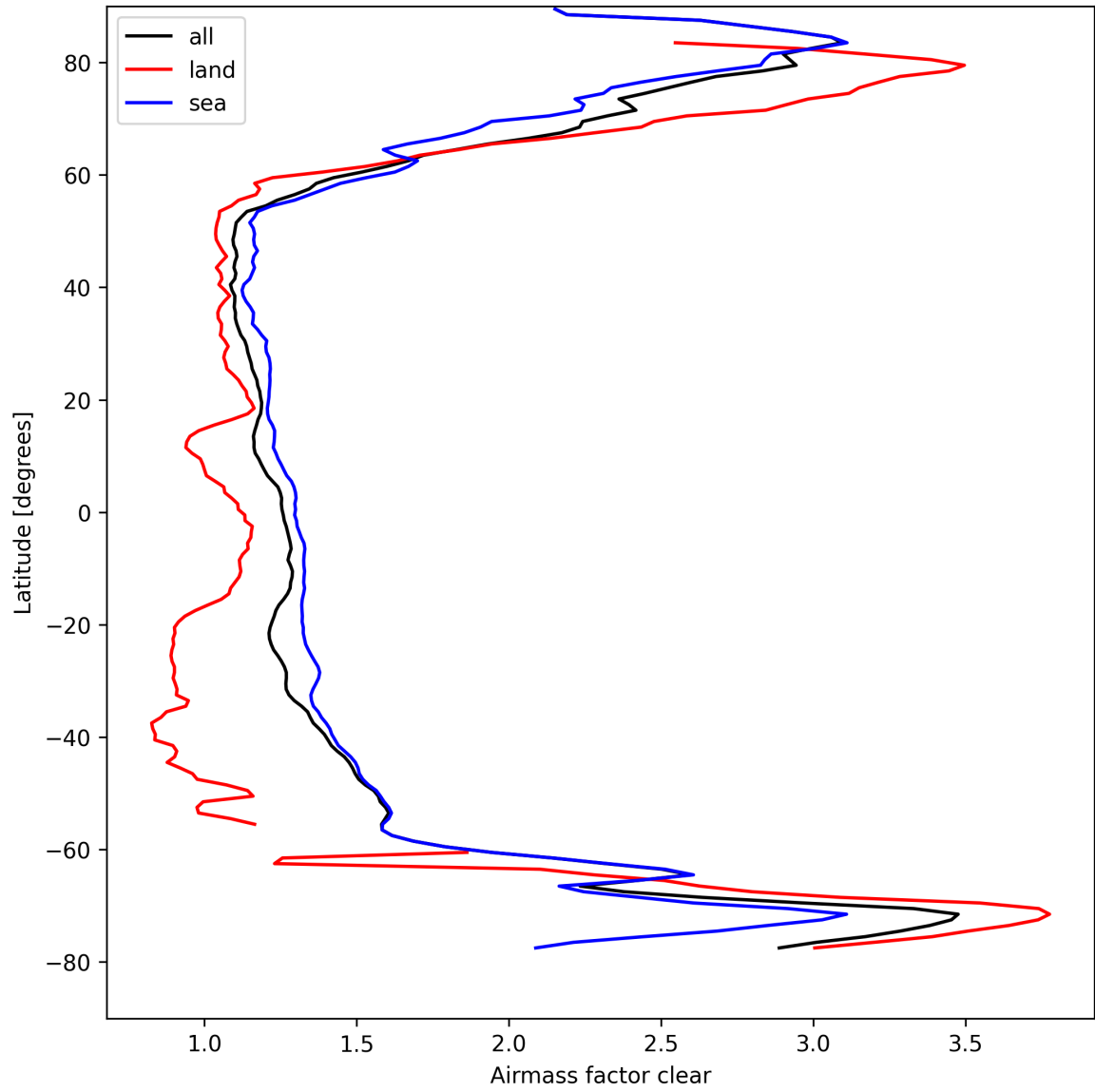
Figure 26: Zonal average of “Airmass factor clear” for 2025-04-08 to 2025-04-09.
