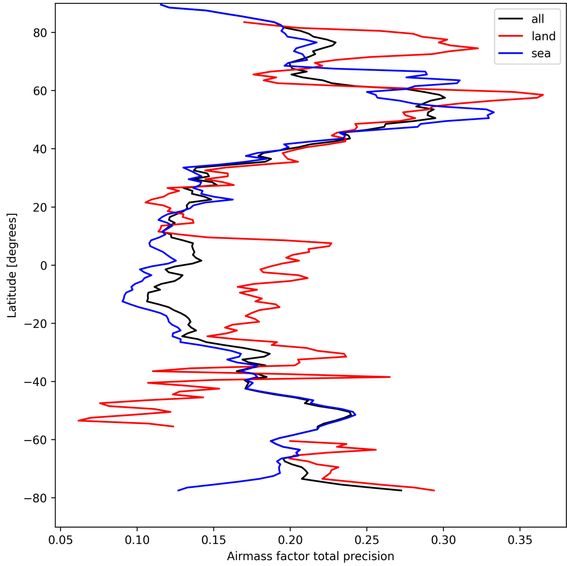
Figure 25: Zonal average of “Airmass factor total precision” for 2025-04-08 to 2025-04-09.
