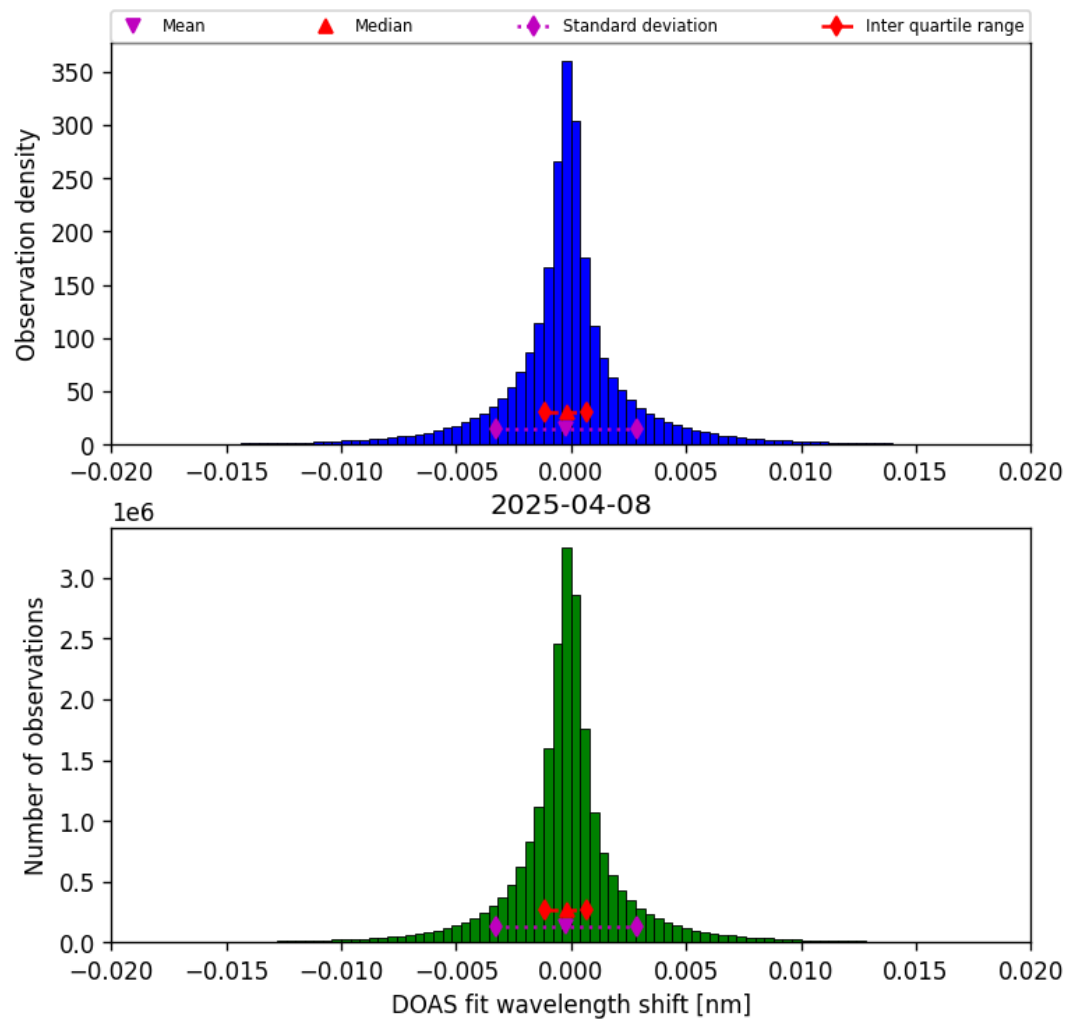
Figure 42: Histogram of “DOAS fit wavelength shift” for 2025-04-08 to 2025-04-09
