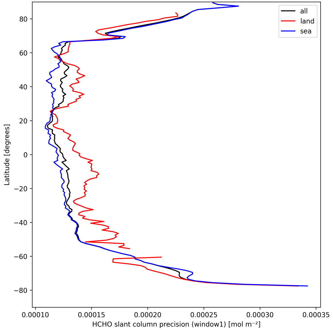
Figure 23: Zonal average of “HCHO slant column precision (window1)” for 2025-04-08 to 2025-04-09.
