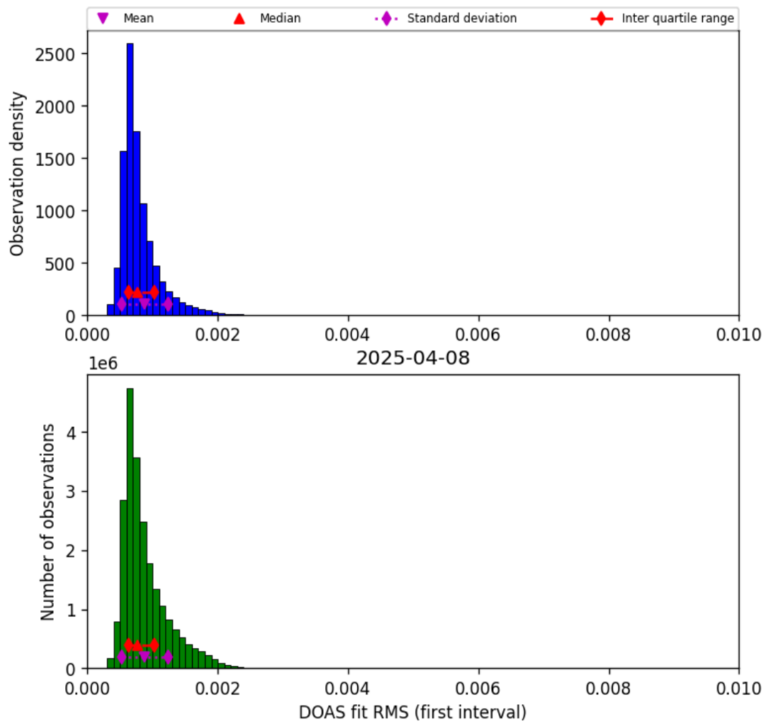
Figure 44: Histogram of “DOAS fit RMS (first interval)” for 2025-04-08 to 2025-04-09
