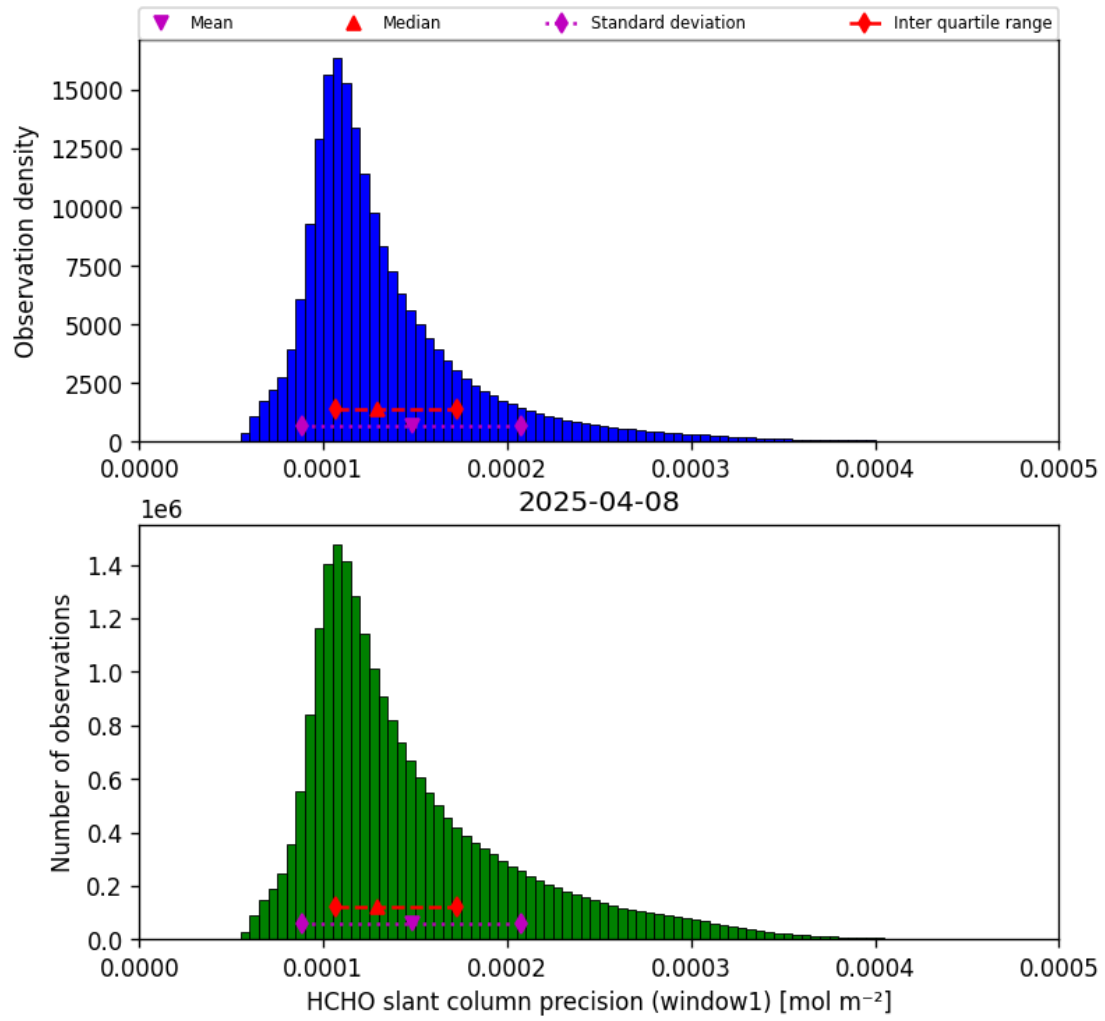
Figure 37: Histogram of “HCHO slant column precision (window1)” for 2025-04-08 to 2025-04-09
