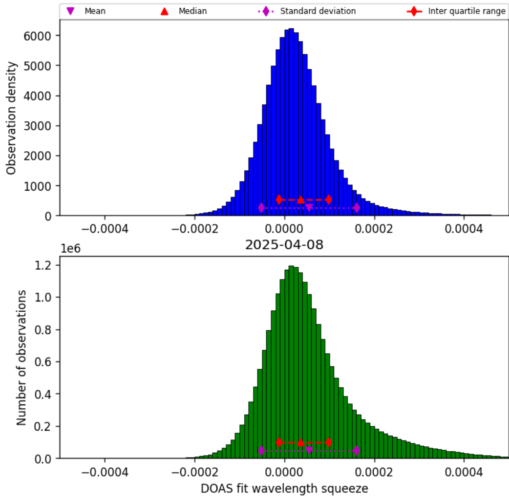
Figure 43: Histogram of “DOAS fit wavelength squeeze” for 2025-04-08 to 2025-04-09
