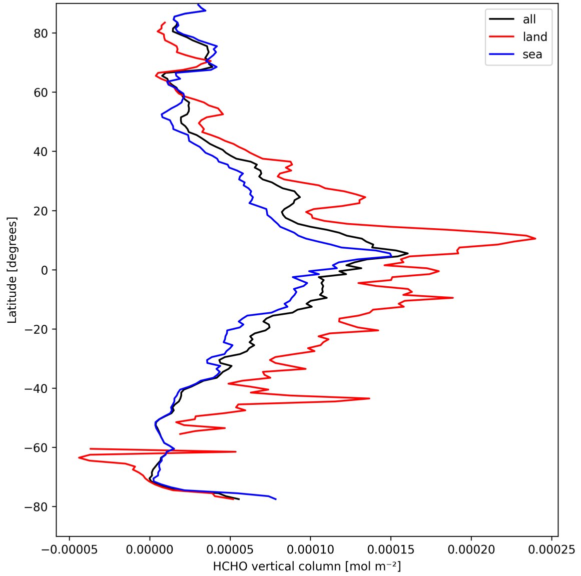
Figure 19: Zonal average of “HCHO vertical column” for 2025-04-08 to 2025-04-09.
