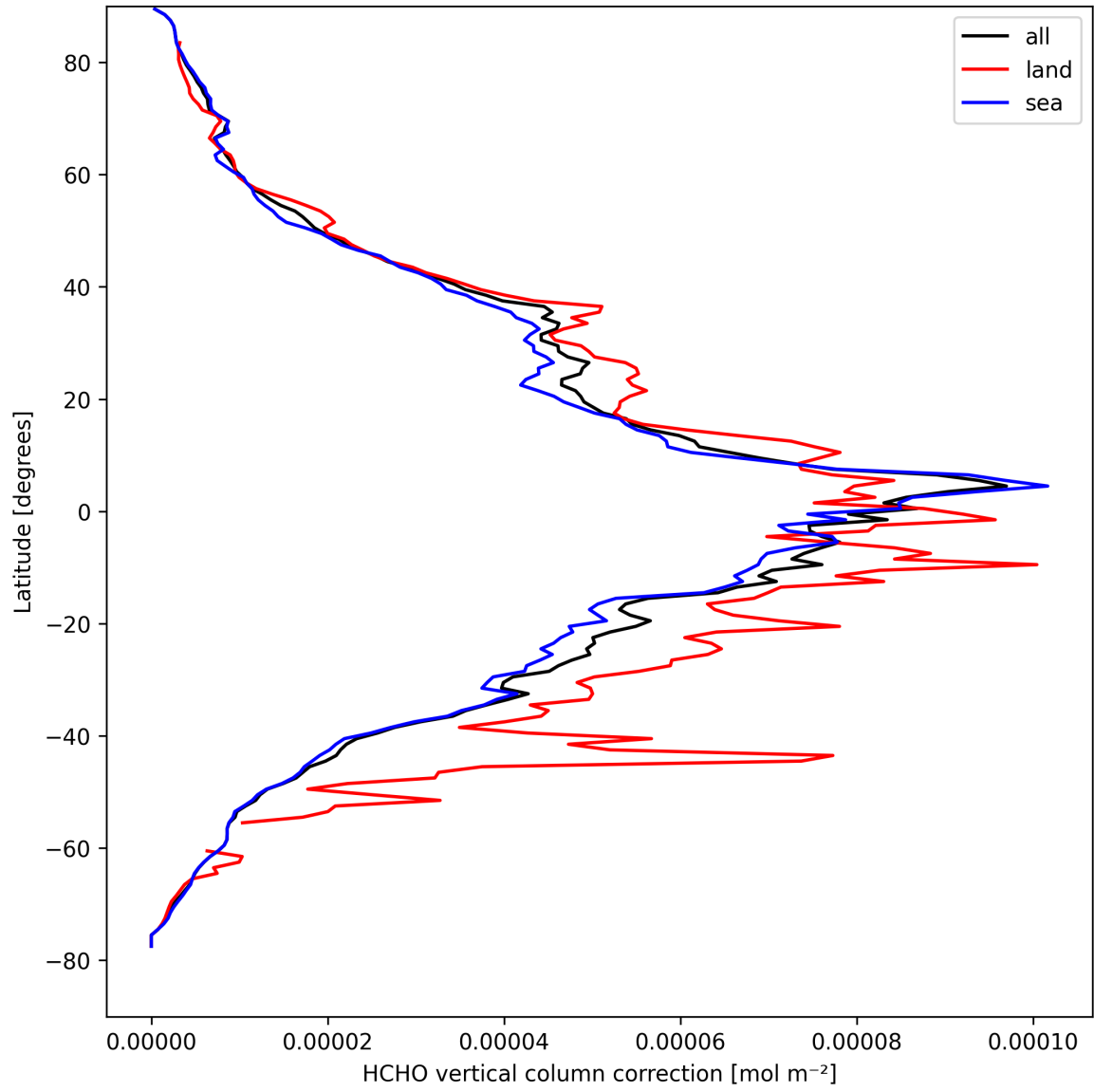
Figure 21: Zonal average of “HCHO vertical column correction” for 2025-04-08 to 2025-04-09.
