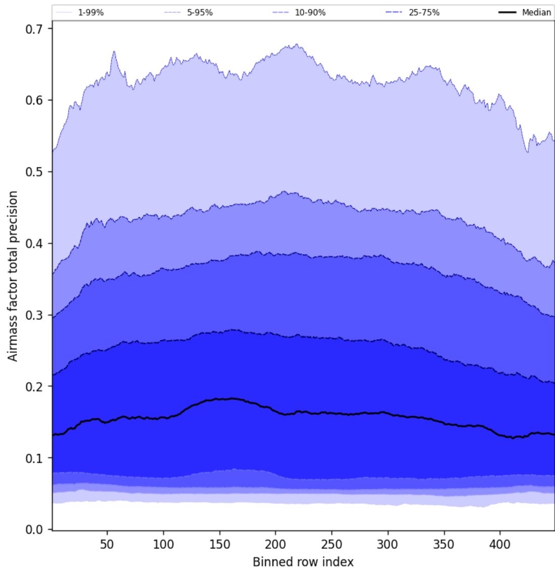
Figure 53: Along track statistics of “Airmass factor total precision” for 2025-04-08 to 2025-04-09
