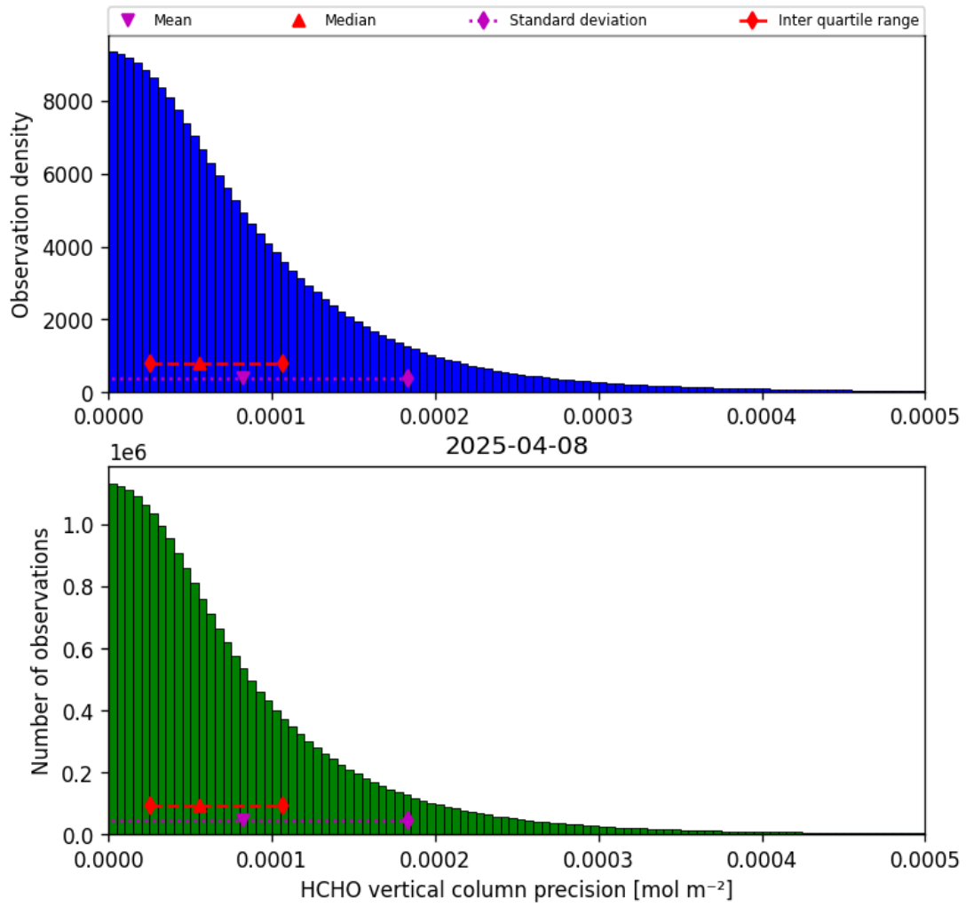
Figure 34: Histogram of “HCHO vertical column precision” for 2025-04-08 to 2025-04-09
