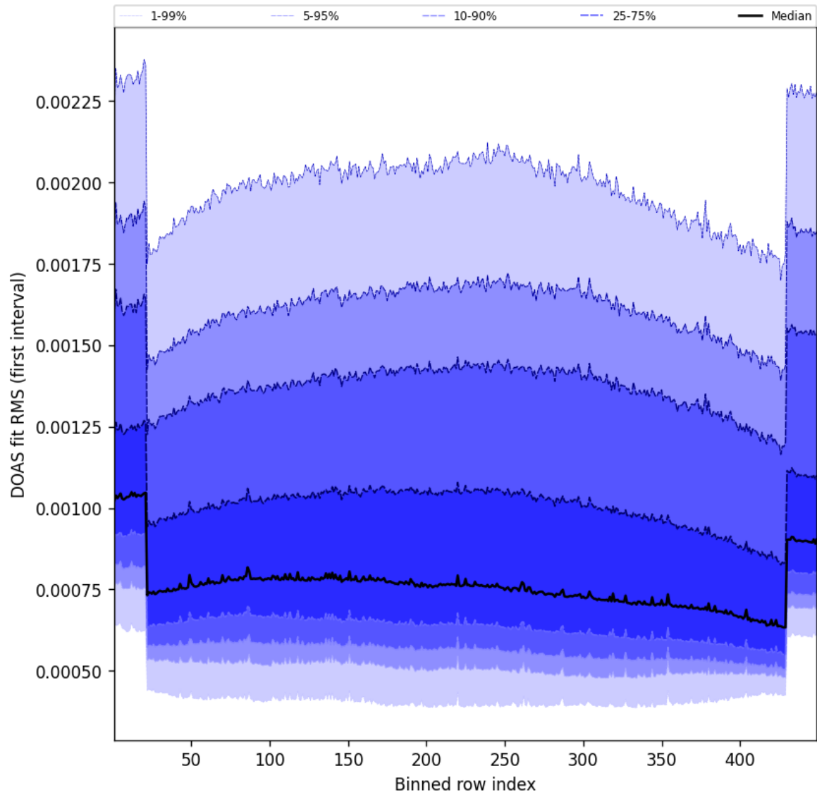
Figure 58: Along track statistics of “DOAS fit RMS (first interval)” for 2025-04-08 to 2025-04-09
