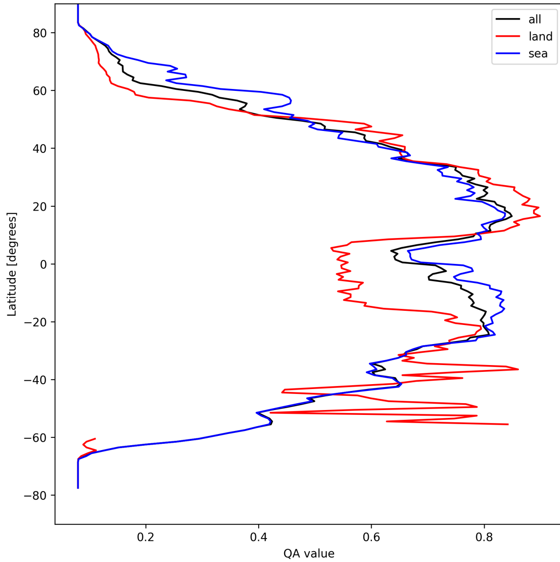
Figure 18: Zonal average of “QA value” for 2025-04-08 to 2025-04-09.
