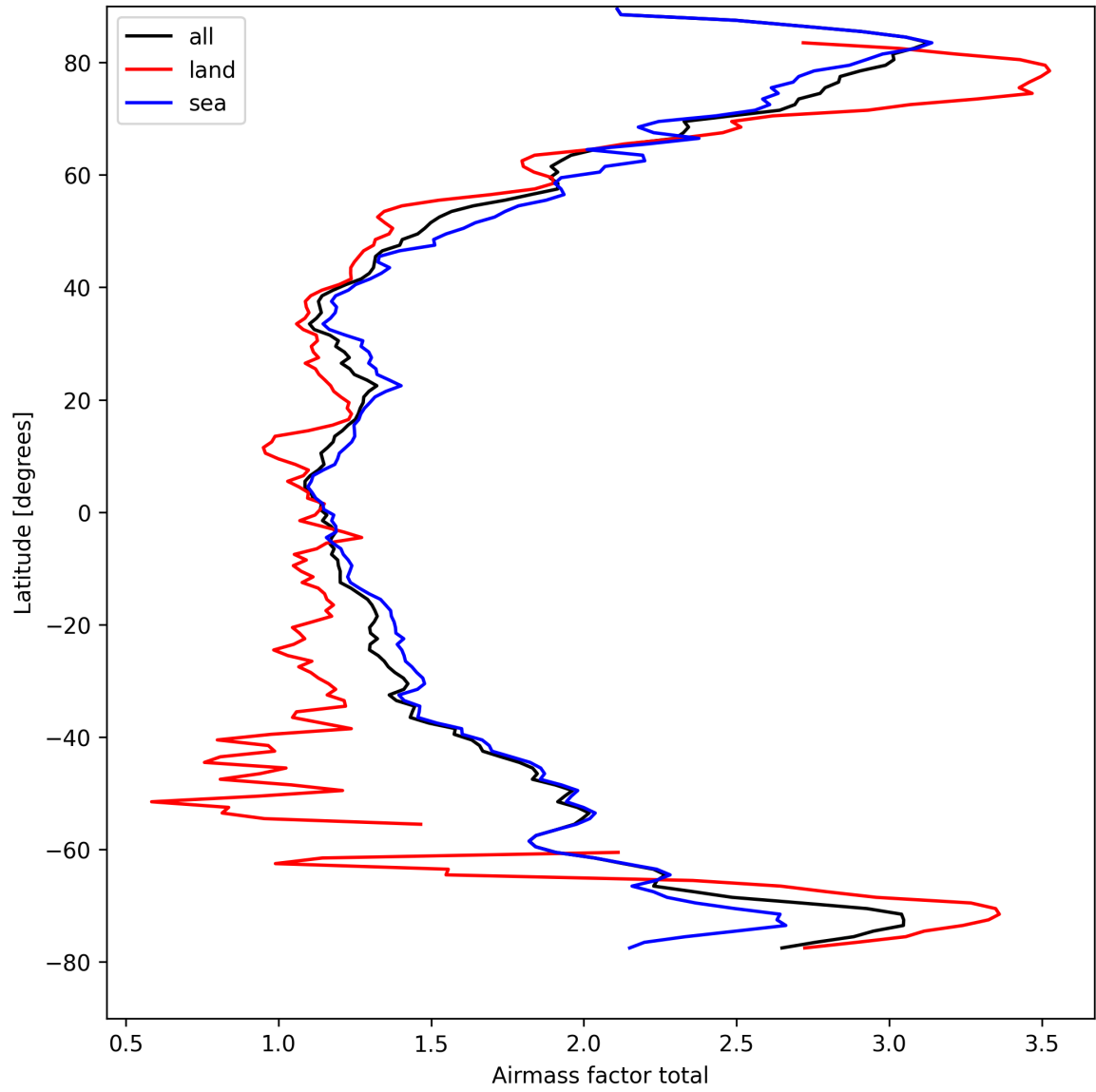
Figure 24: Zonal average of “Airmass factor total” for 2025-04-08 to 2025-04-09.
