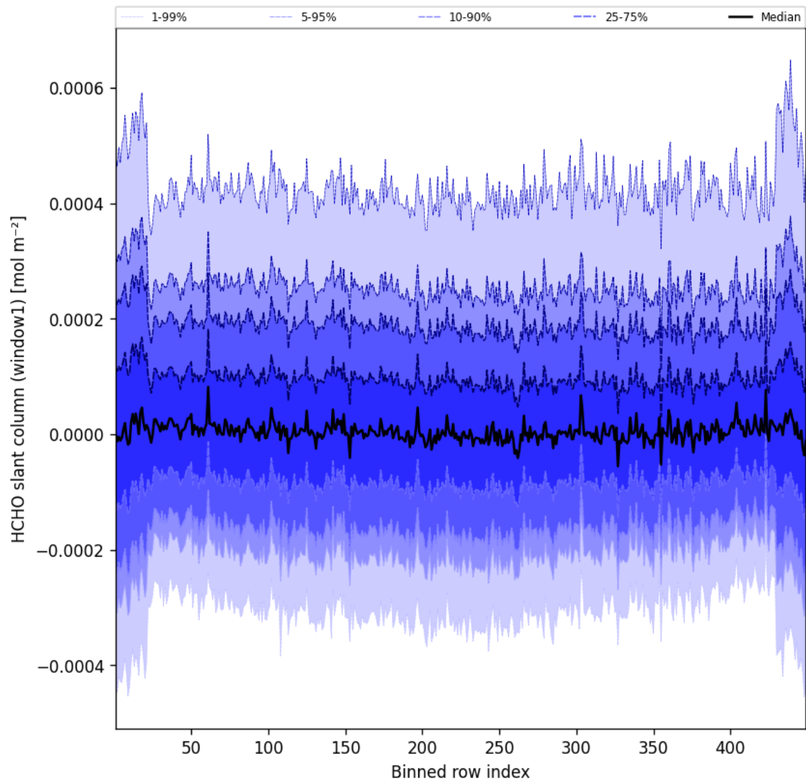
Figure 50: Along track statistics of “HCHO slant column (window1)” for 2025-04-08 to 2025-04-09
