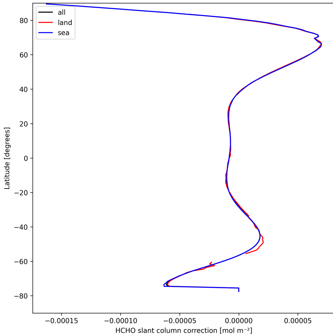
Figure 31: Zonal average of “HCHO slant column correction” for 2025-04-08 to 2025-04-09.
