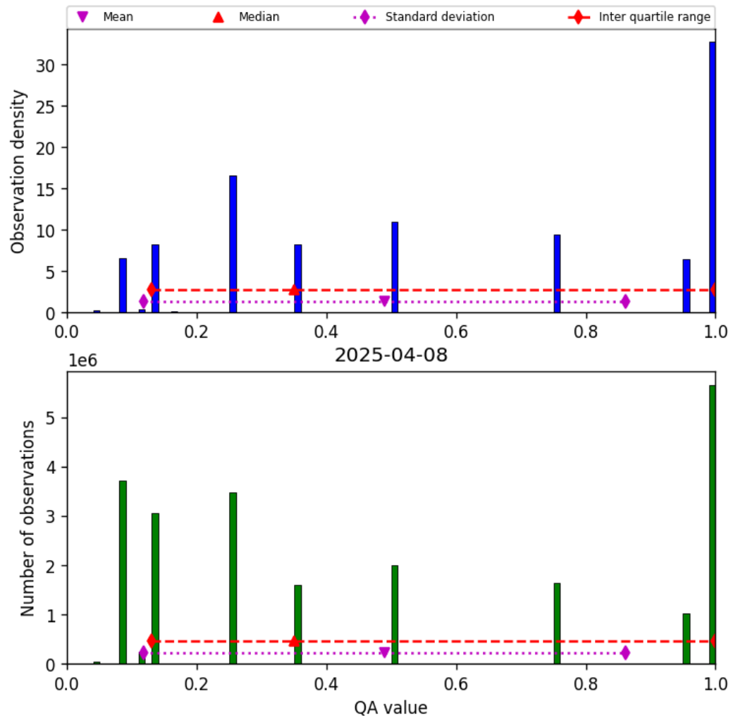
Figure 32: Histogram of “QA value” for 2025-04-08 to 2025-04-09
