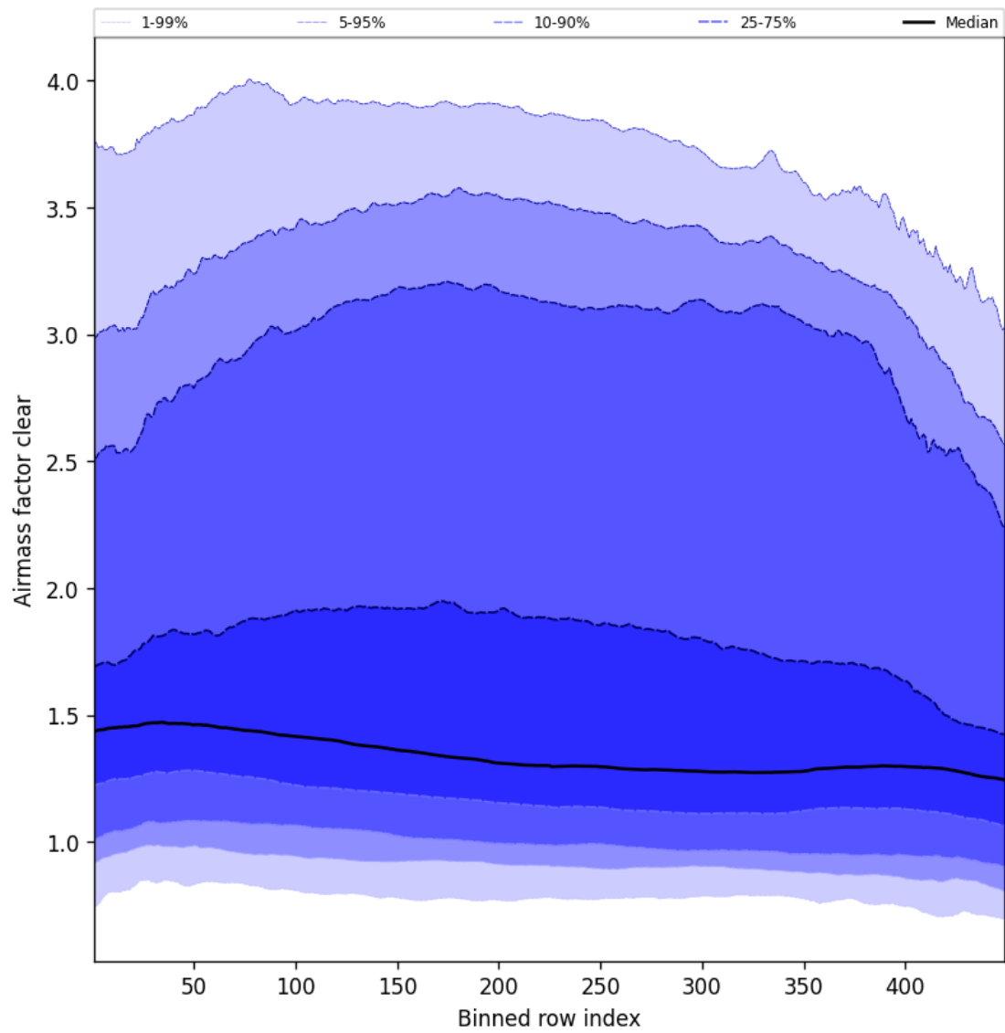
Figure 54: Along track statistics of “Airmass factor clear” for 2025-04-08 to 2025-04-09
