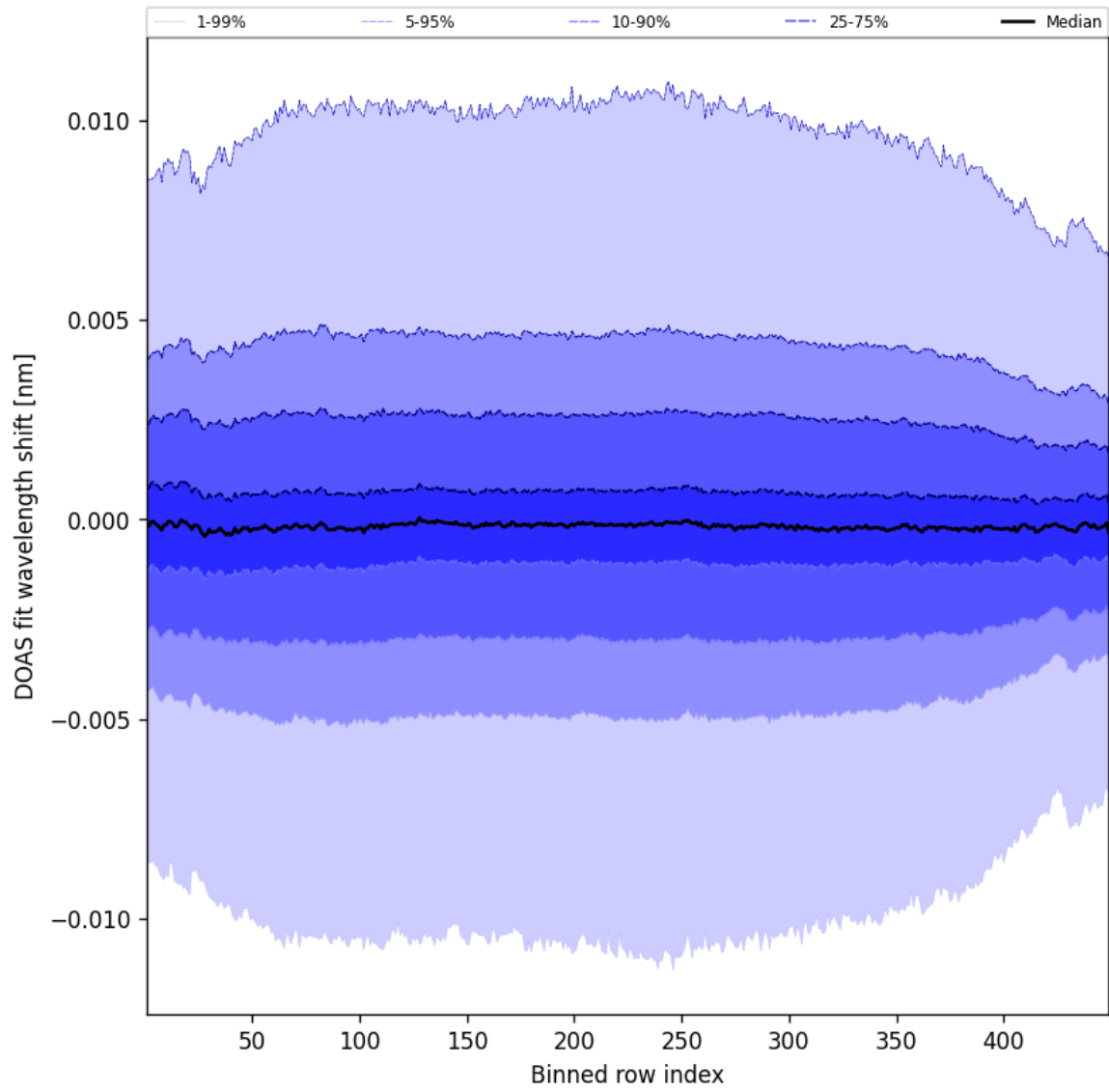
Figure 56: Along track statistics of “DOAS fit wavelength shift” for 2025-04-08 to 2025-04-09
