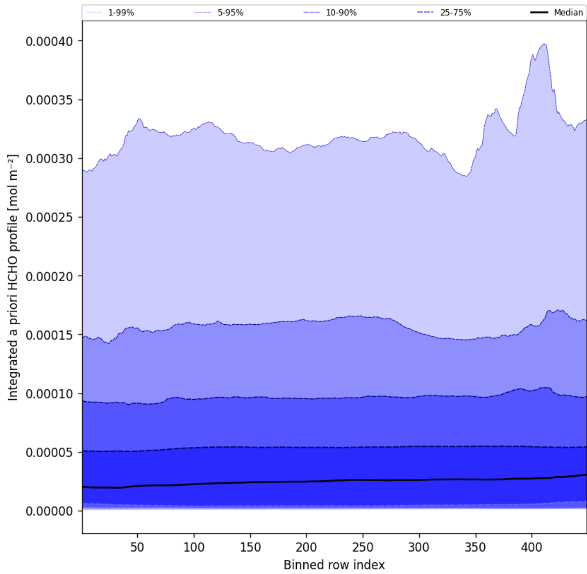
Figure 55: Along track statistics of "Integrated a priori HCHO profile" for 2025-04-08 to 2025-04-09
