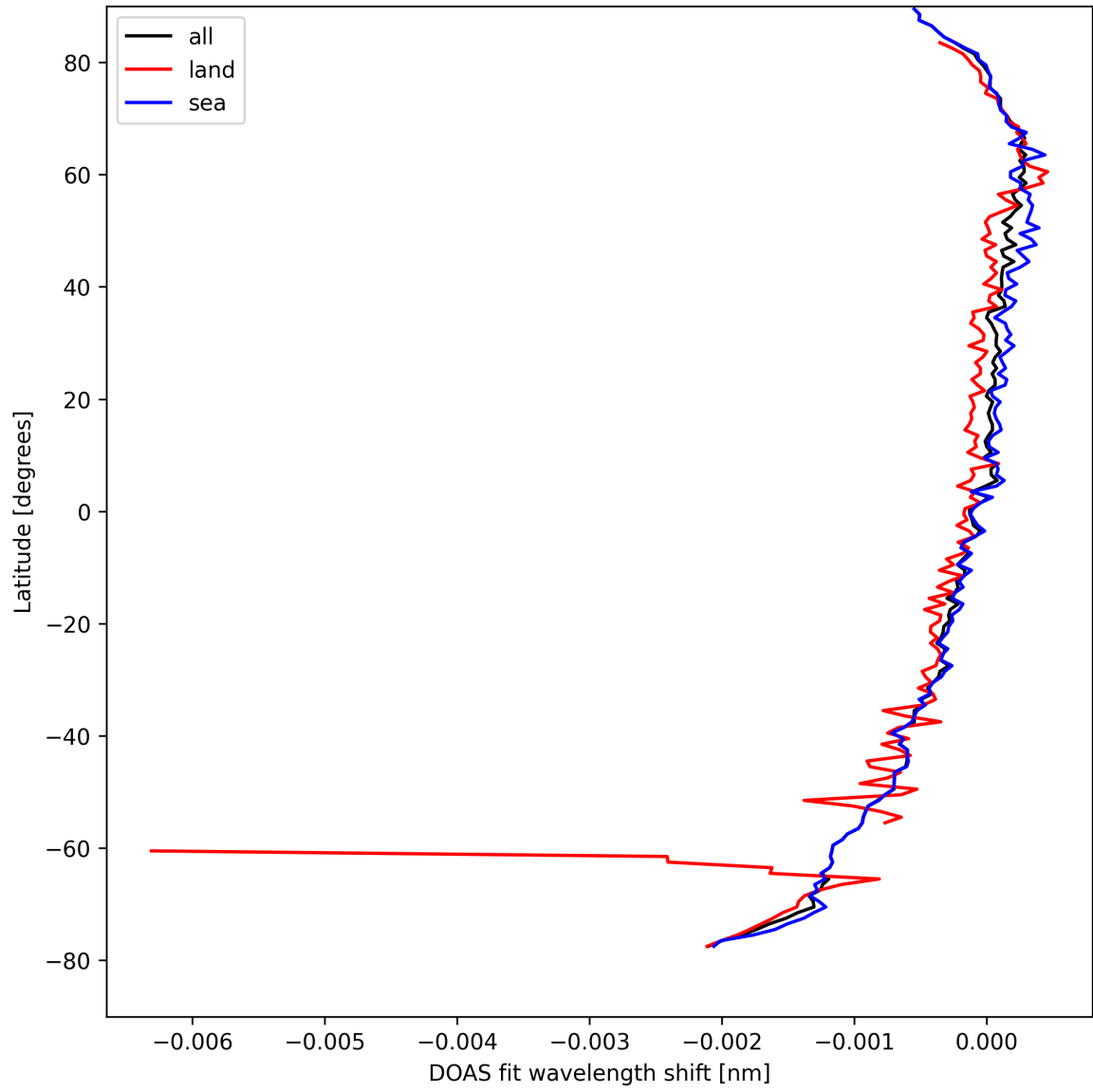
Figure 28: Zonal average of “DOAS fit wavelength shift” for 2025-04-08 to 2025-04-09.
