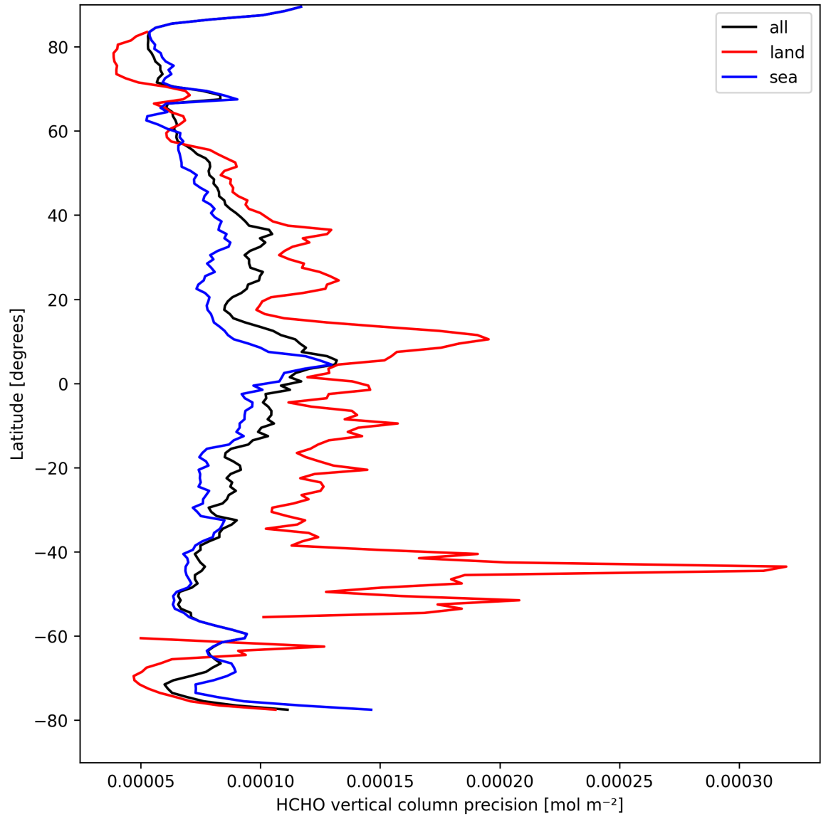
Figure 20: Zonal average of “HCHO vertical column precision” for 2025-04-08 to 2025-04-09.
