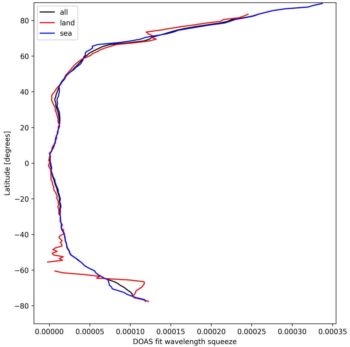
Figure 29: Zonal average of “DOAS fit wavelength squeeze” for 2025-04-08 to 2025-04-09.
