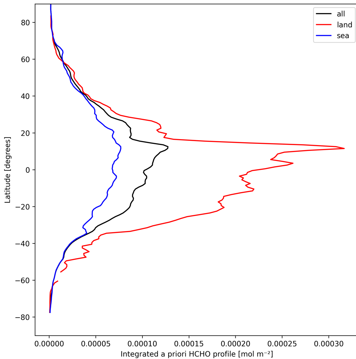
Figure 27: Zonal average of “Integrated a priori HCHO profile” for 2025-04-08 to 2025-04-09.
