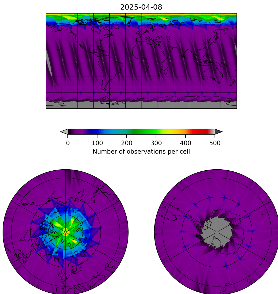
Figure 17: Map of the number of observations for 2025-04-08 to 2025-04-09
