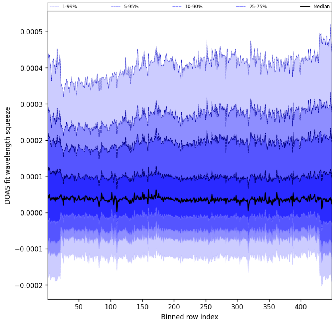
Figure 57: Along track statistics of “DOAS fit wavelength squeeze” for 2025-04-08 to 2025-04-09
