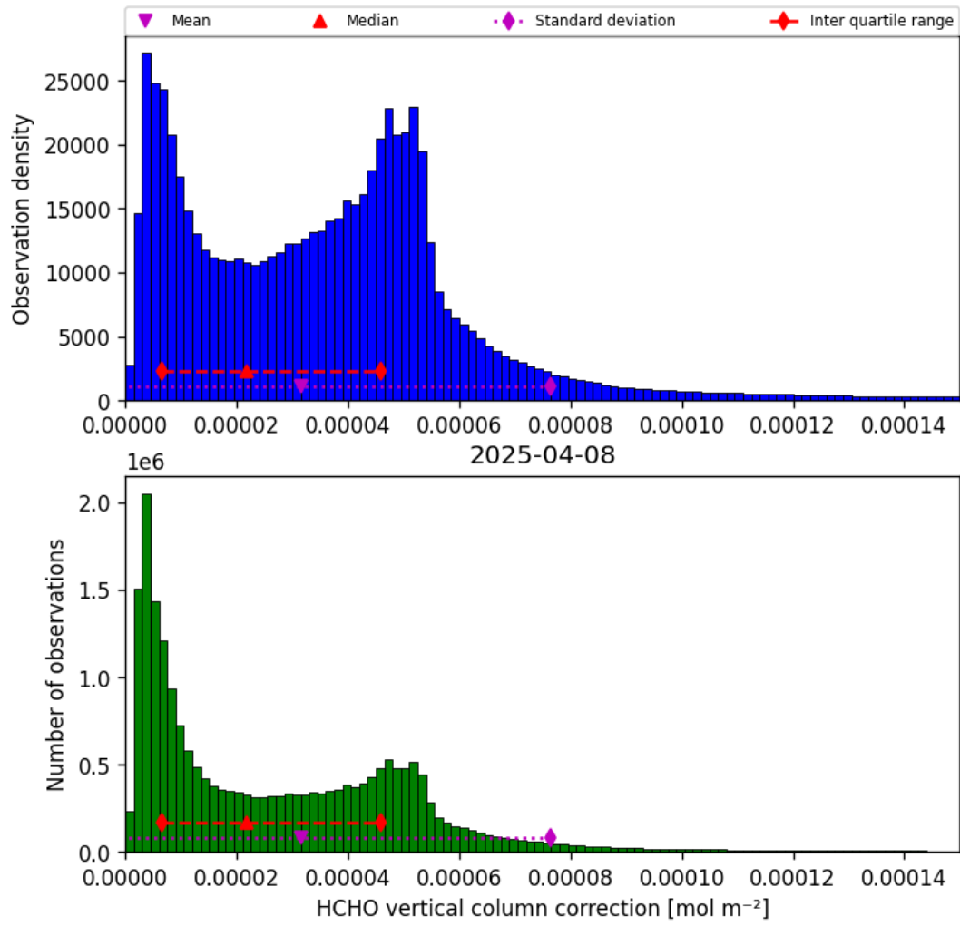
Figure 35: Histogram of “HCHO vertical column correction” for 2025-04-08 to 2025-04-09
