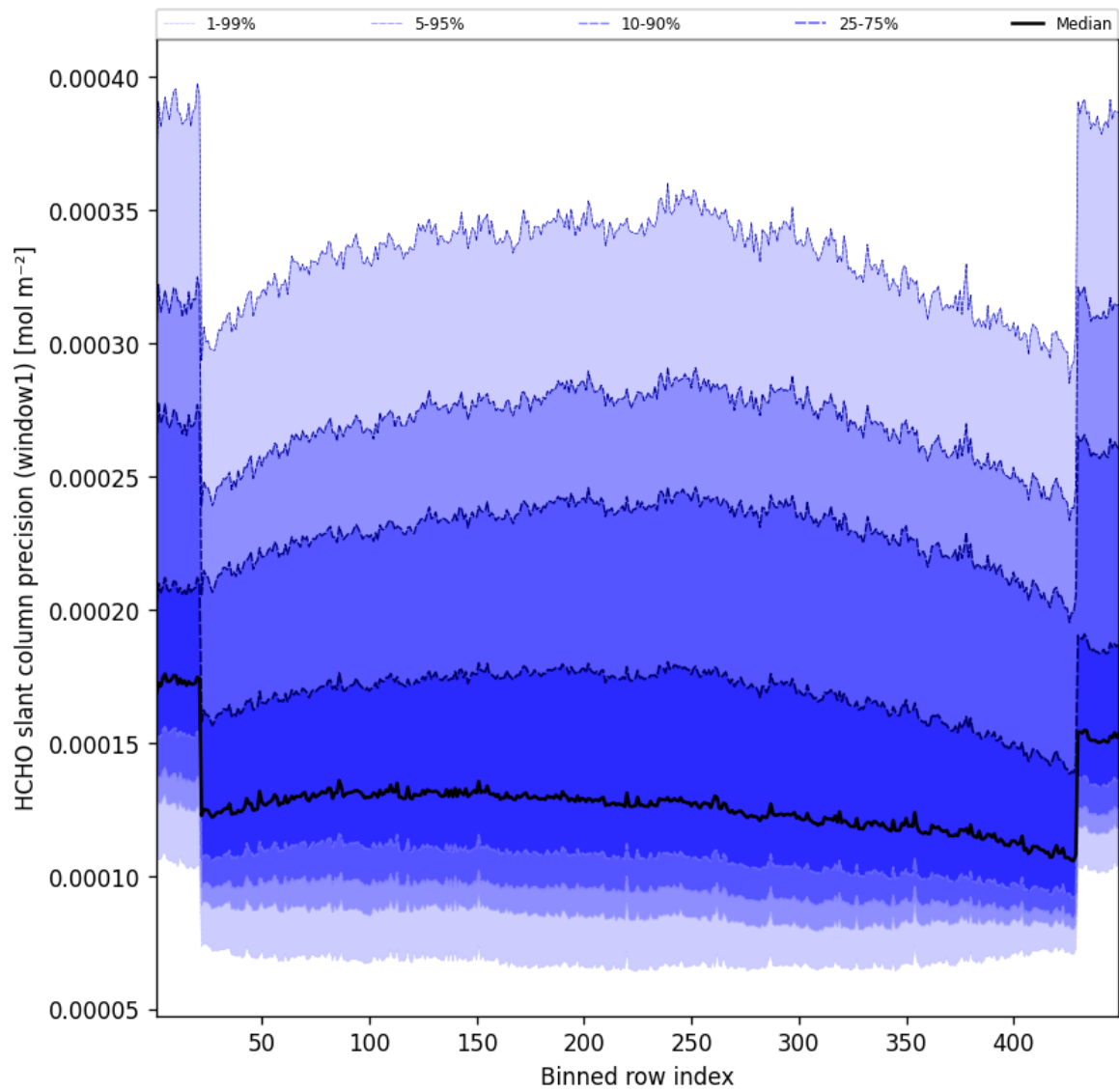
Figure 51: Along track statistics of “HCHO slant column precision (window1)” for 2025-04-08 to 2025-04-09
