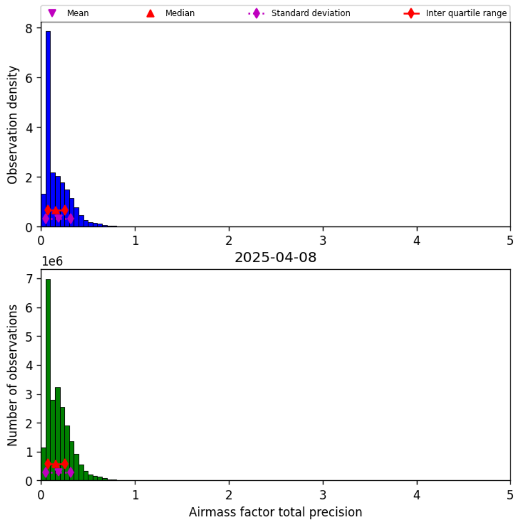
Figure 39: Histogram of “Airmass factor total precision” for 2025-04-08 to 2025-04-09
