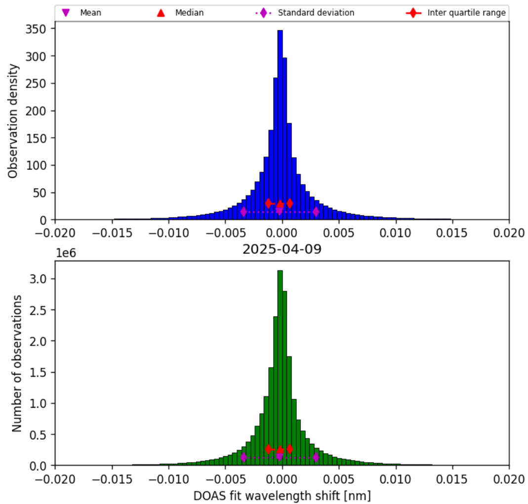
Figure 42: Histogram of “DOAS fit wavelength shift” for 2025-04-09 to 2025-04-10
