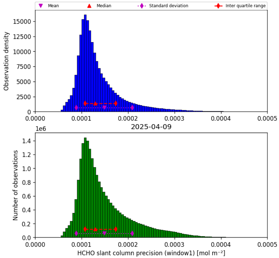
Figure 37: Histogram of “HCHO slant column precision (window1)” for 2025-04-09 to 2025-04-10
