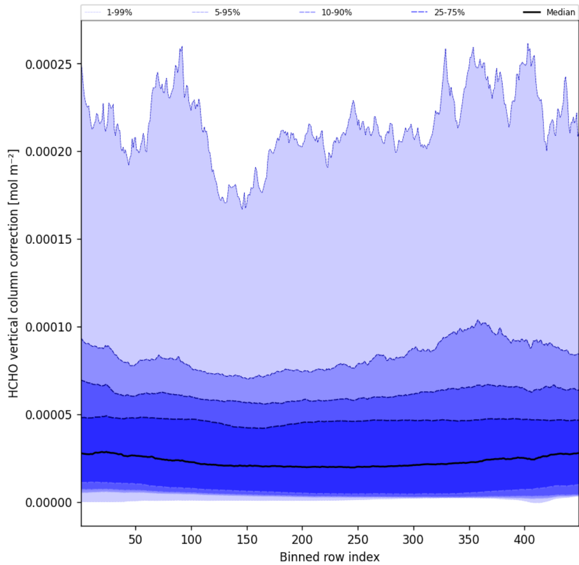
Figure 49: Along track statistics of “HCHO vertical column correction” for 2025-04-09 to 2025-04-10
