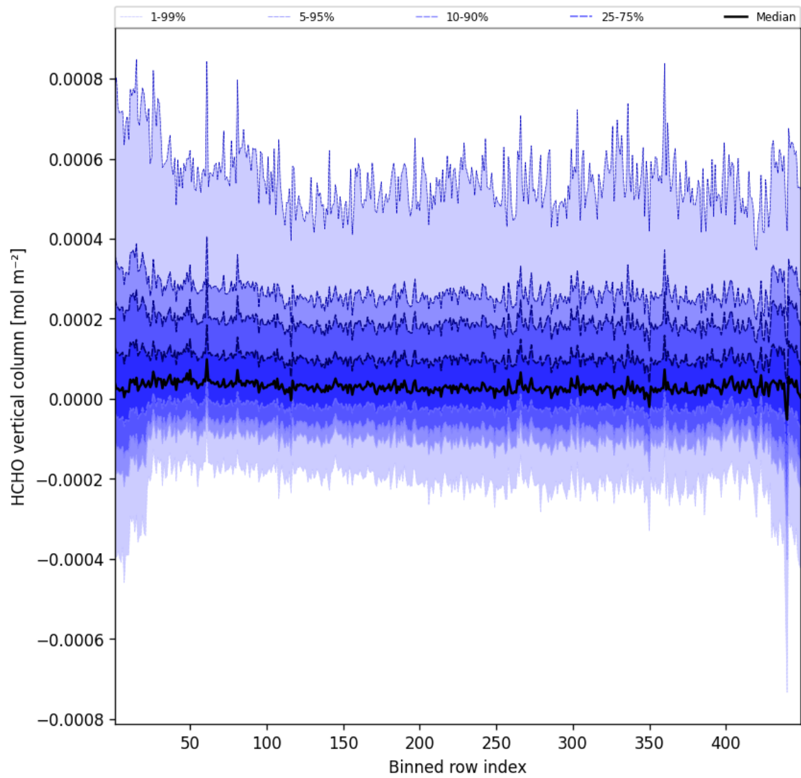
Figure 47: Along track statistics of “HCHO vertical column” for 2025-04-09 to 2025-04-10
