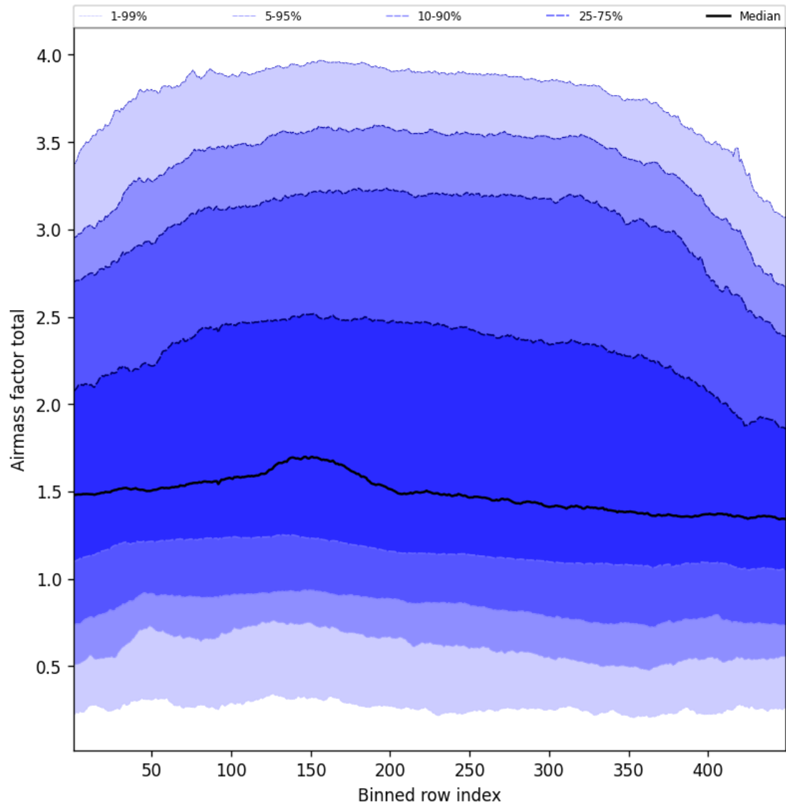
Figure 52: Along track statistics of “Airmass factor total” for 2025-04-09 to 2025-04-10
