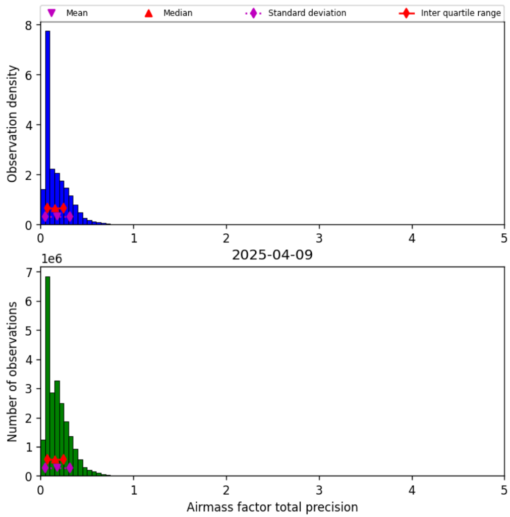
Figure 39: Histogram of “Airmass factor total precision” for 2025-04-09 to 2025-04-10
