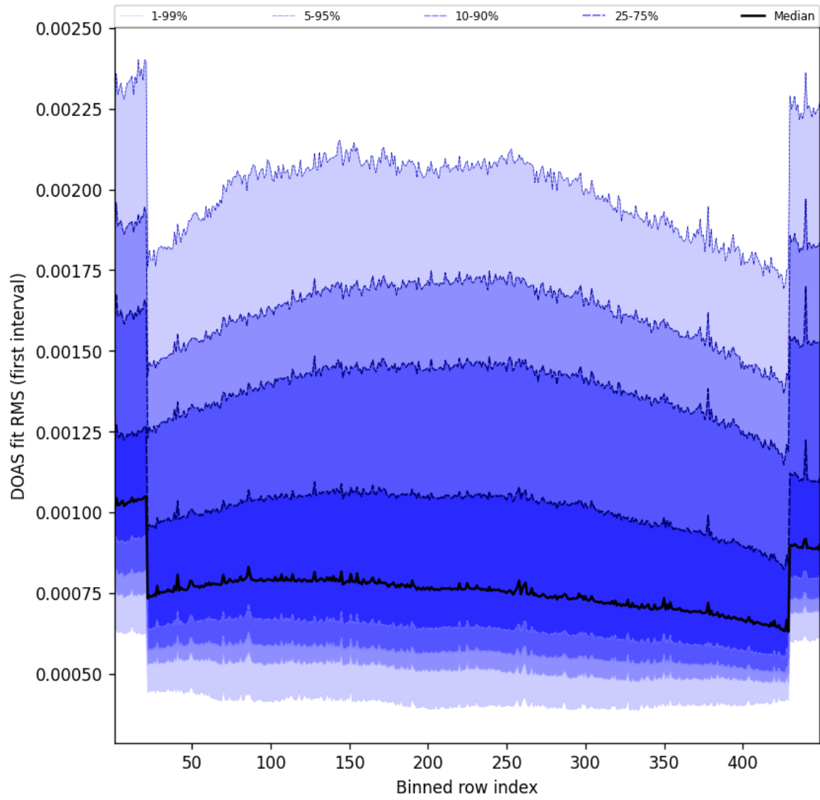
Figure 58: Along track statistics of “DOAS fit RMS (first interval)” for 2025-04-09 to 2025-04-10
