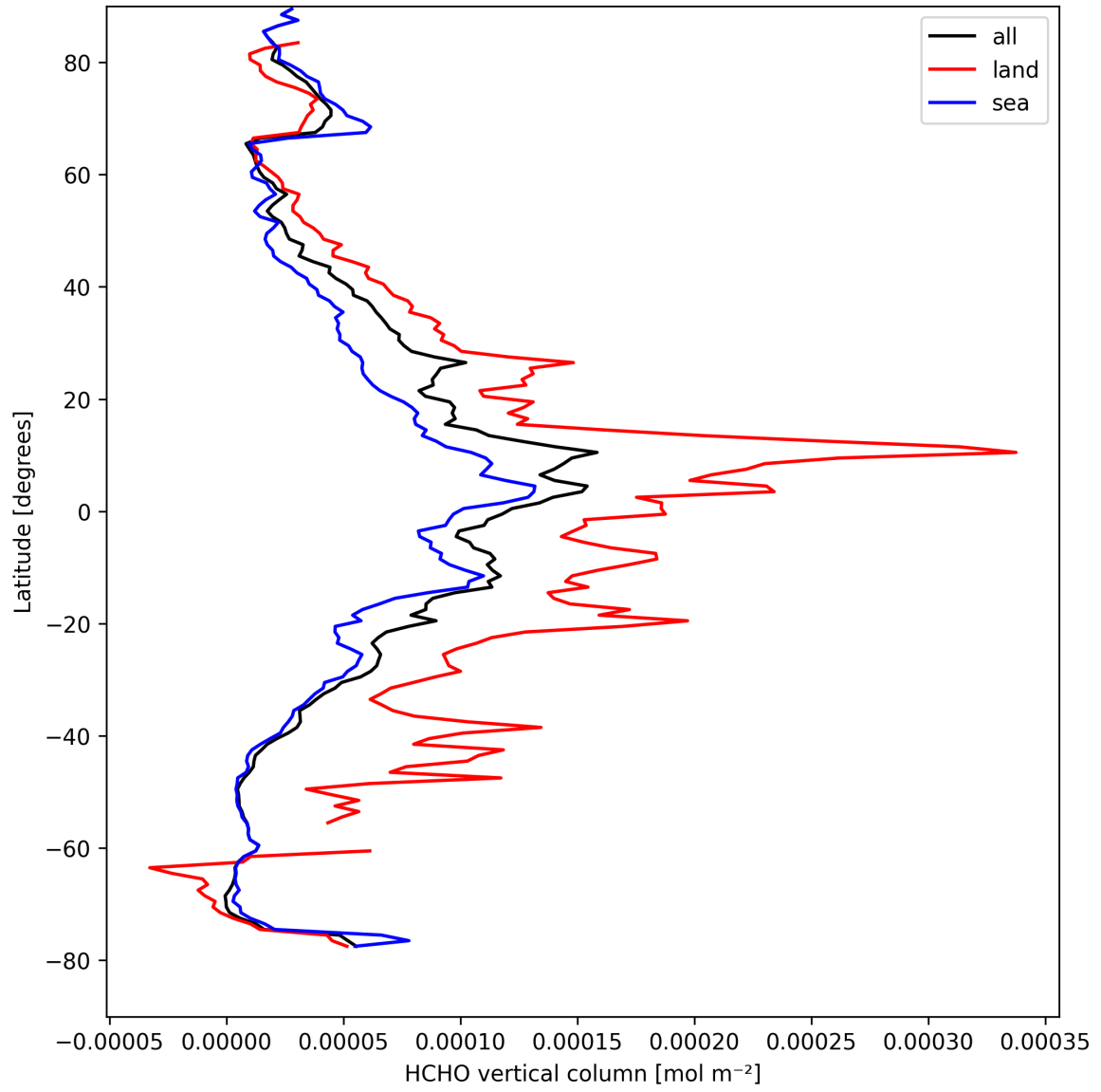
Figure 19: Zonal average of “HCHO vertical column” for 2025-04-09 to 2025-04-10.
