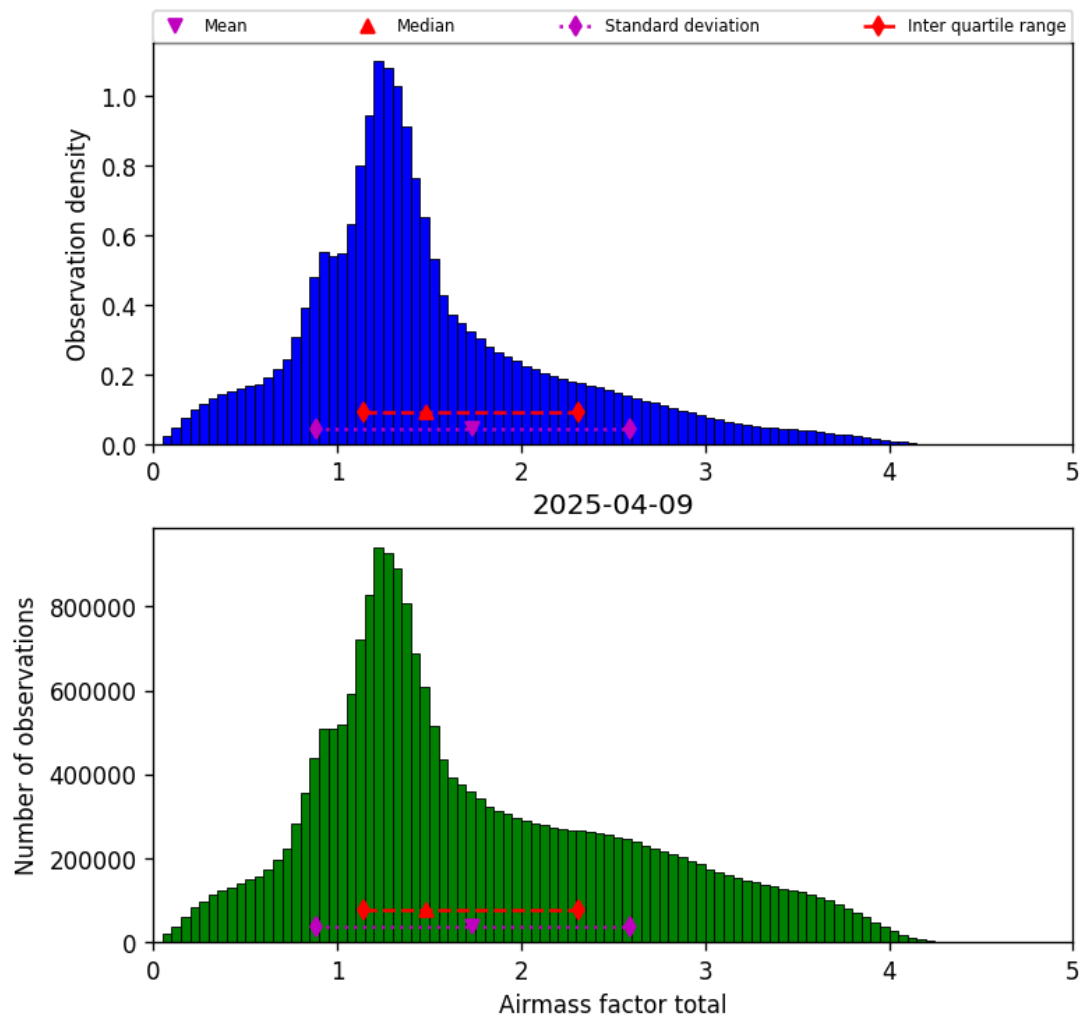
Figure 38: Histogram of “Airmass factor total” for 2025-04-09 to 2025-04-10
