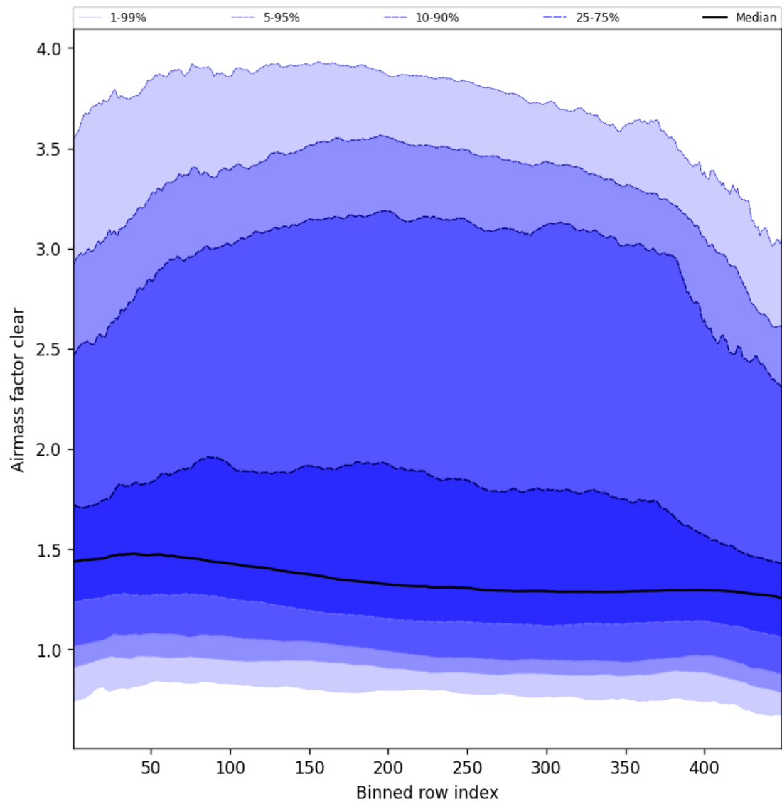
Figure 54: Along track statistics of “Airmass factor clear” for 2025-04-09 to 2025-04-10
