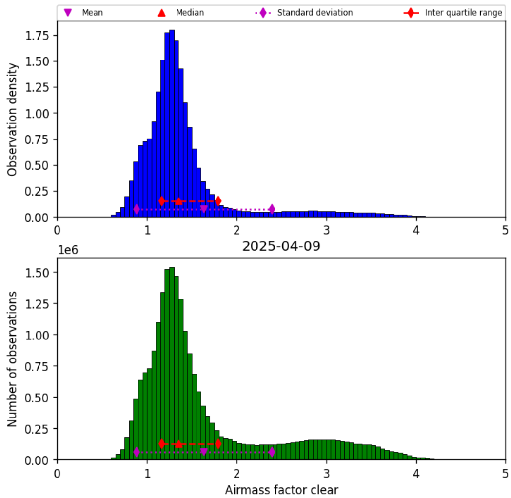
Figure 40: Histogram of “Airmass factor clear” for 2025-04-09 to 2025-04-10
