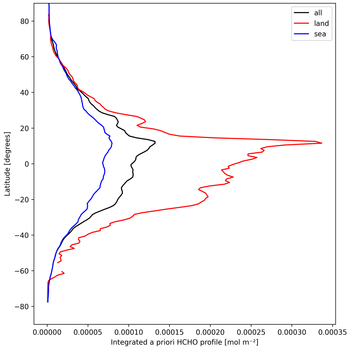
Figure 27: Zonal average of “Integrated a priori HCHO profile” for 2025-04-09 to 2025-04-10.
