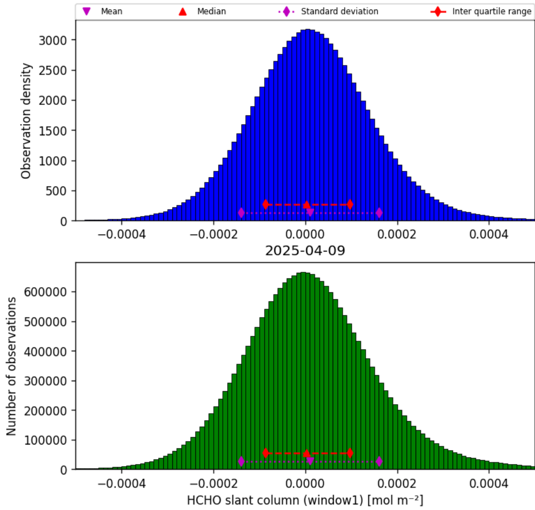
Figure 36: Histogram of “HCHO slant column (window1)” for 2025-04-09 to 2025-04-10
