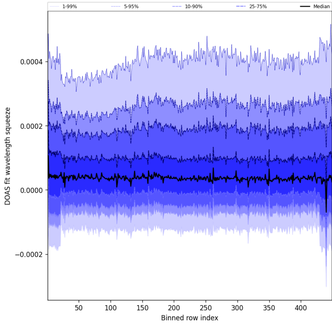
Figure 57: Along track statistics of “DOAS fit wavelength squeeze” for 2025-04-09 to 2025-04-10
