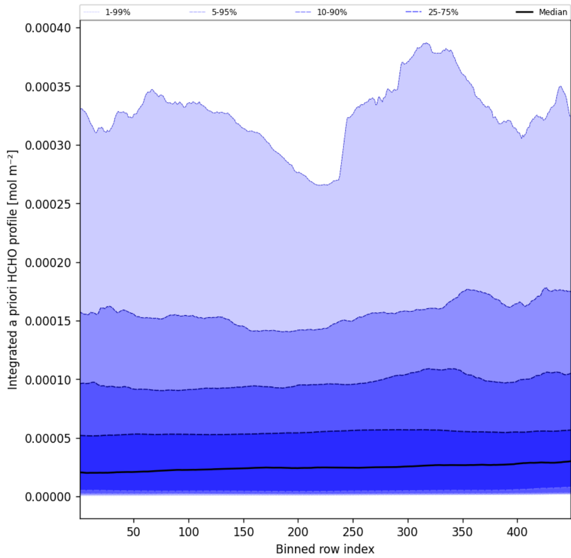
Figure 55: Along track statistics of “Integrated a priori HCHO profile” for 2025-04-09 to 2025-04-10
