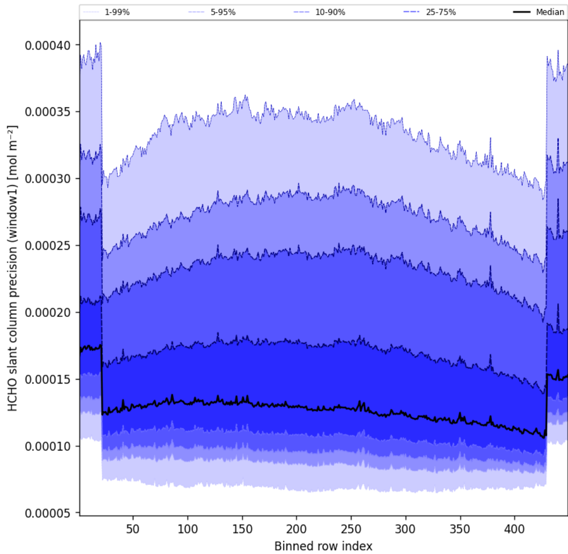
Figure 51: Along track statistics of “HCHO slant column precision (window1)” for 2025-04-09 to 2025-04-10
