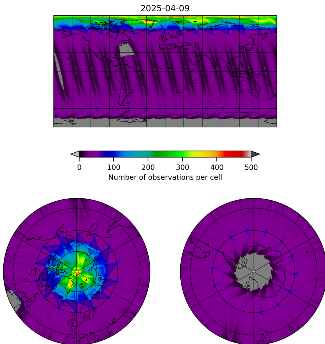
Figure 17: Map of the number of observations for 2025-04-09 to 2025-04-10
