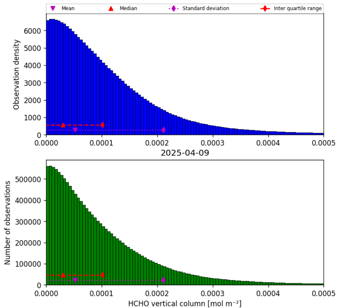
Figure 33: Histogram of “HCHO vertical column” for 2025-04-09 to 2025-04-10
