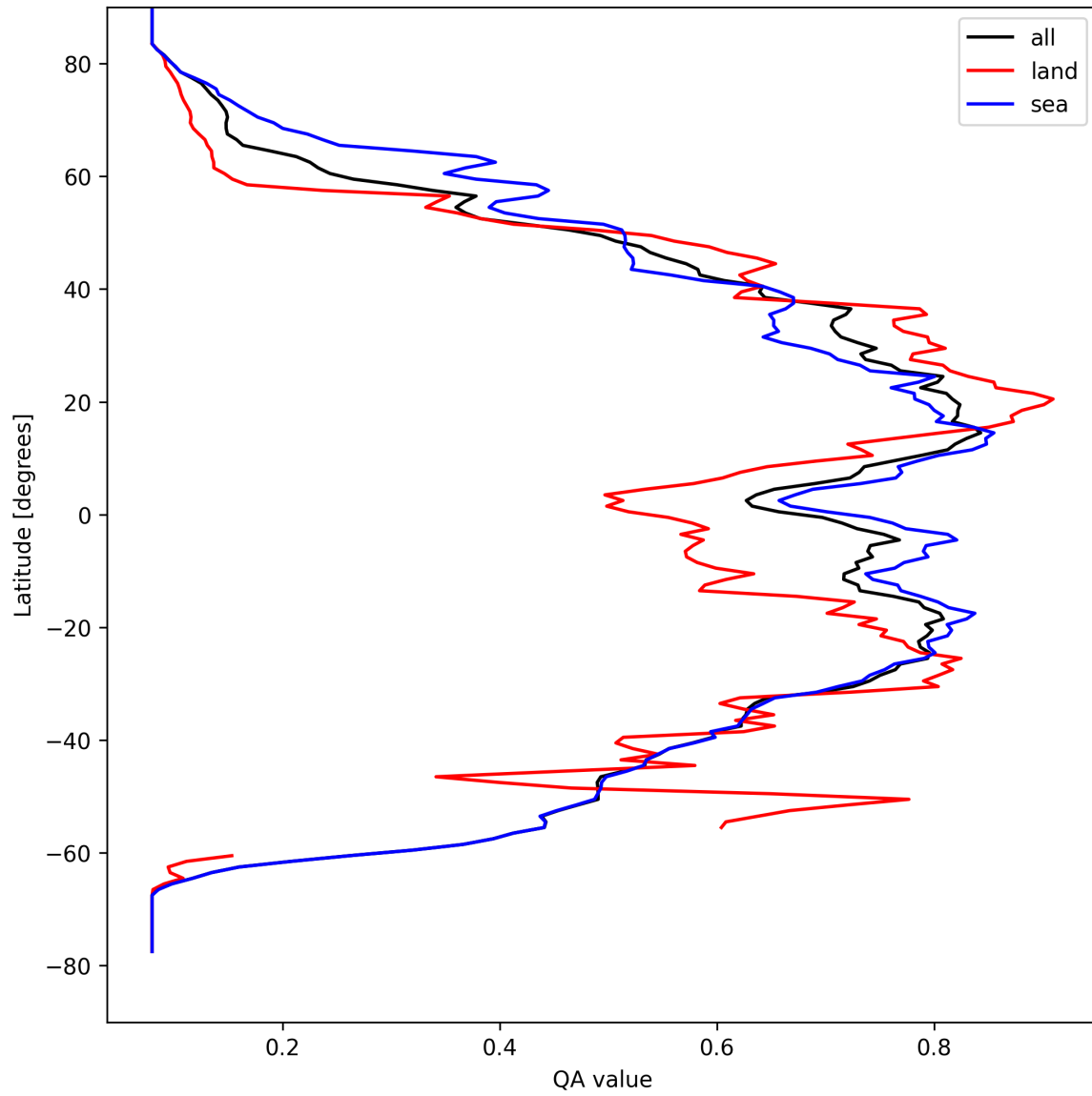
Figure 18: Zonal average of “QA value” for 2025-04-09 to 2025-04-10.
