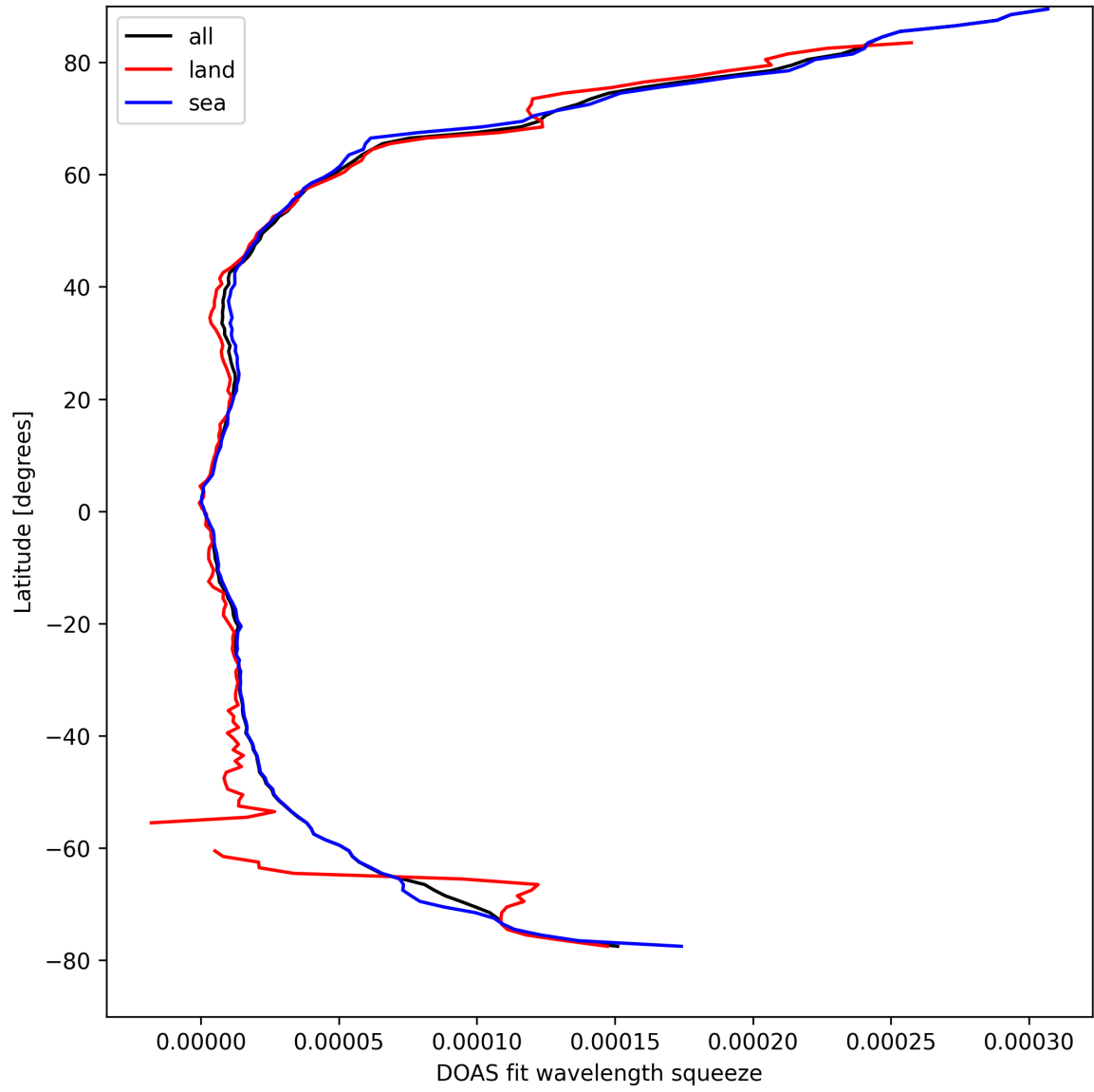
Figure 29: Zonal average of “DOAS fit wavelength squeeze” for 2025-04-09 to 2025-04-10.
