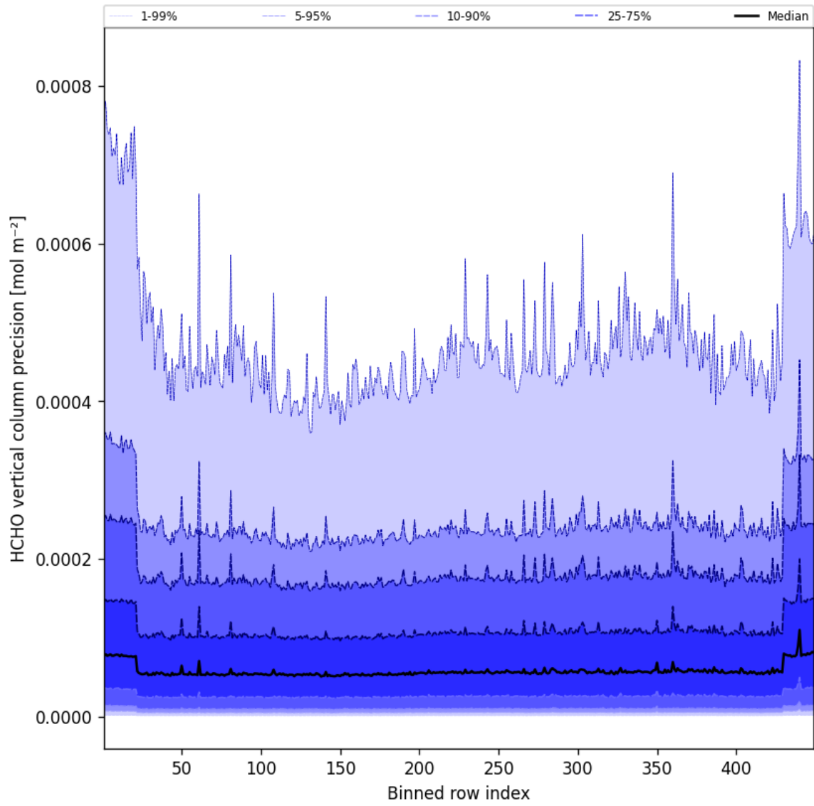
Figure 48: Along track statistics of “HCHO vertical column precision” for 2025-04-09 to 2025-04-10
