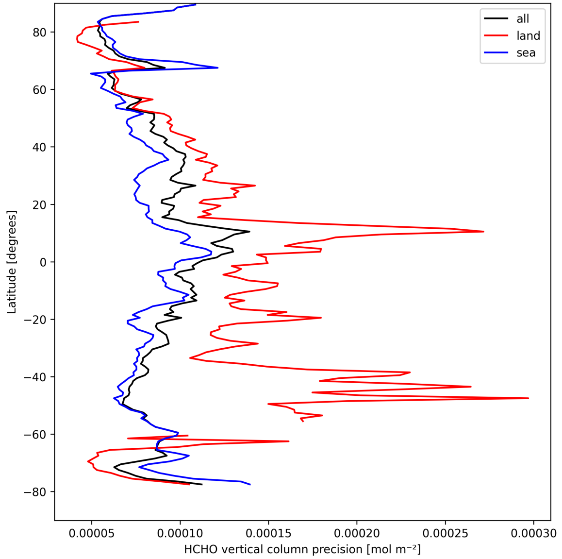
Figure 20: Zonal average of “HCHO vertical column precision” for 2025-04-09 to 2025-04-10.
