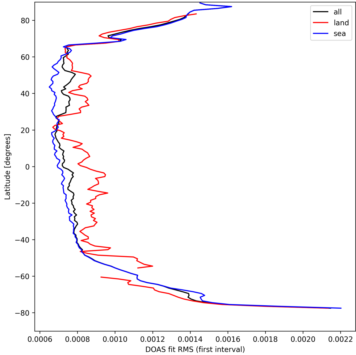
Figure 30: Zonal average of “DOAS fit RMS (first interval)” for 2025-04-09 to 2025-04-10.
