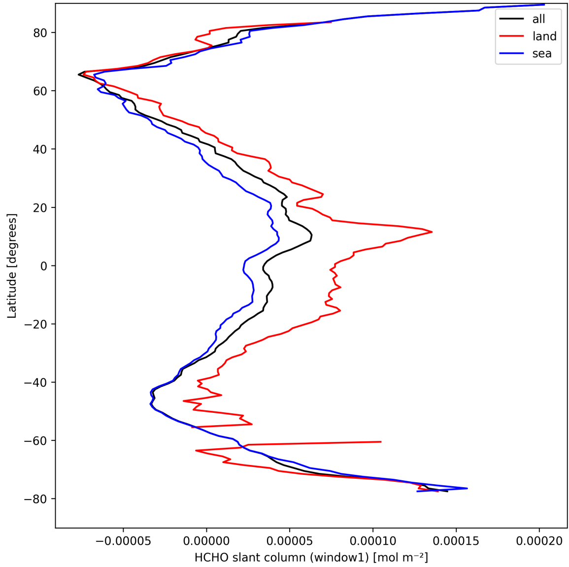
Figure 22: Zonal average of “HCHO slant column (window1)” for 2025-04-09 to 2025-04-10.
