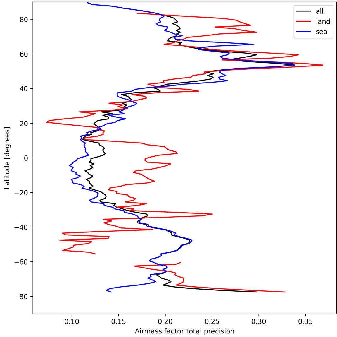
Figure 25: Zonal average of “Airmass factor total precision” for 2025-04-09 to 2025-04-10.
