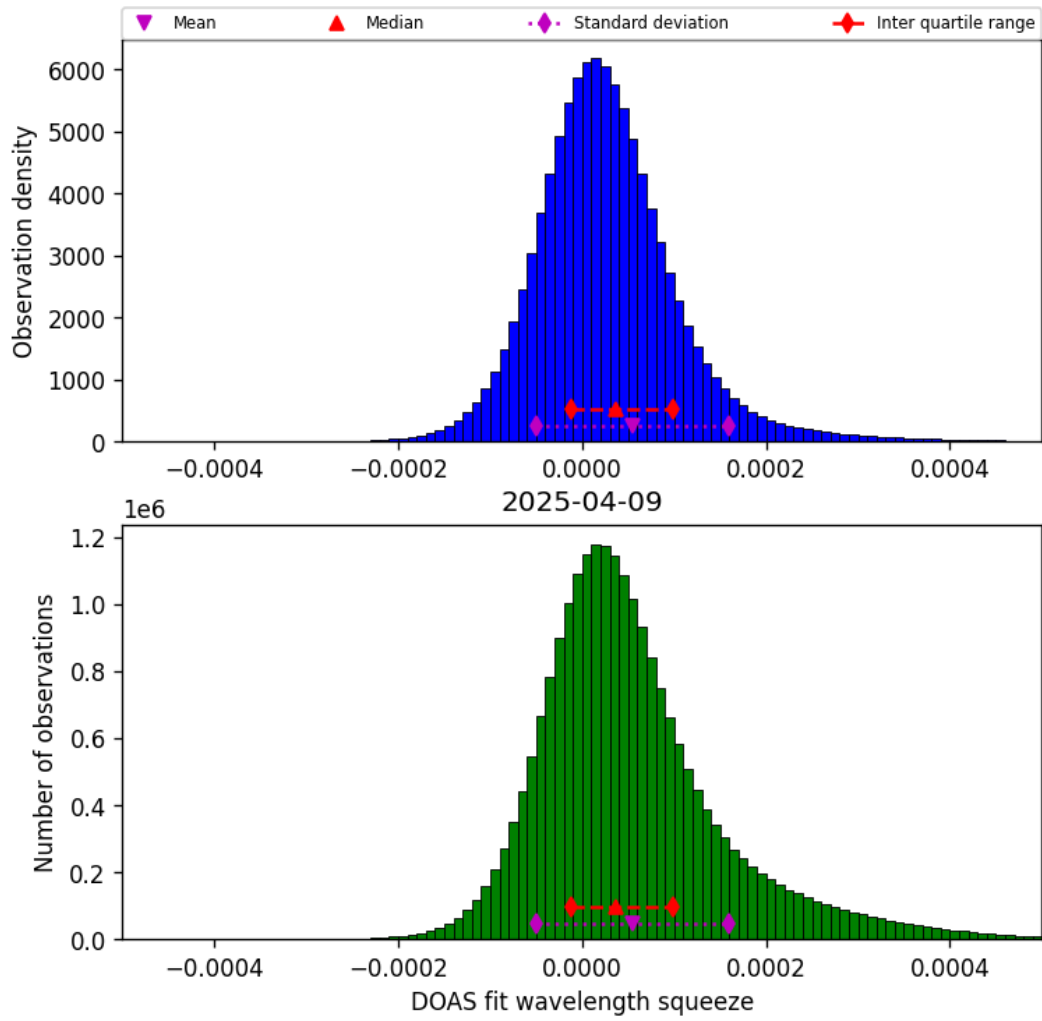
Figure 43: Histogram of “DOAS fit wavelength squeeze” for 2025-04-09 to 2025-04-10
