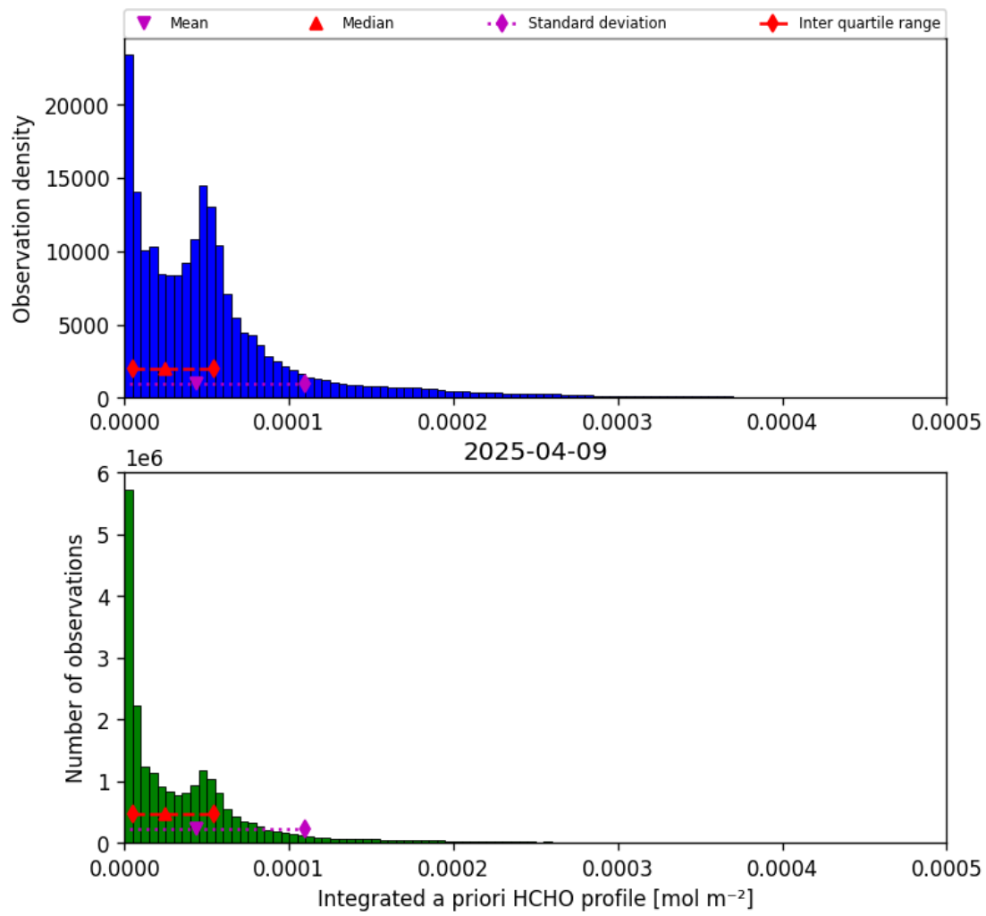
Figure 41: Histogram of “Integrated a priori HCHO profile” for 2025-04-09 to 2025-04-10
