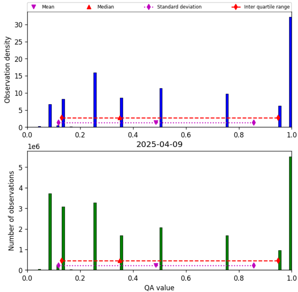
Figure 32: Histogram of “QA value” for 2025-04-09 to 2025-04-10
