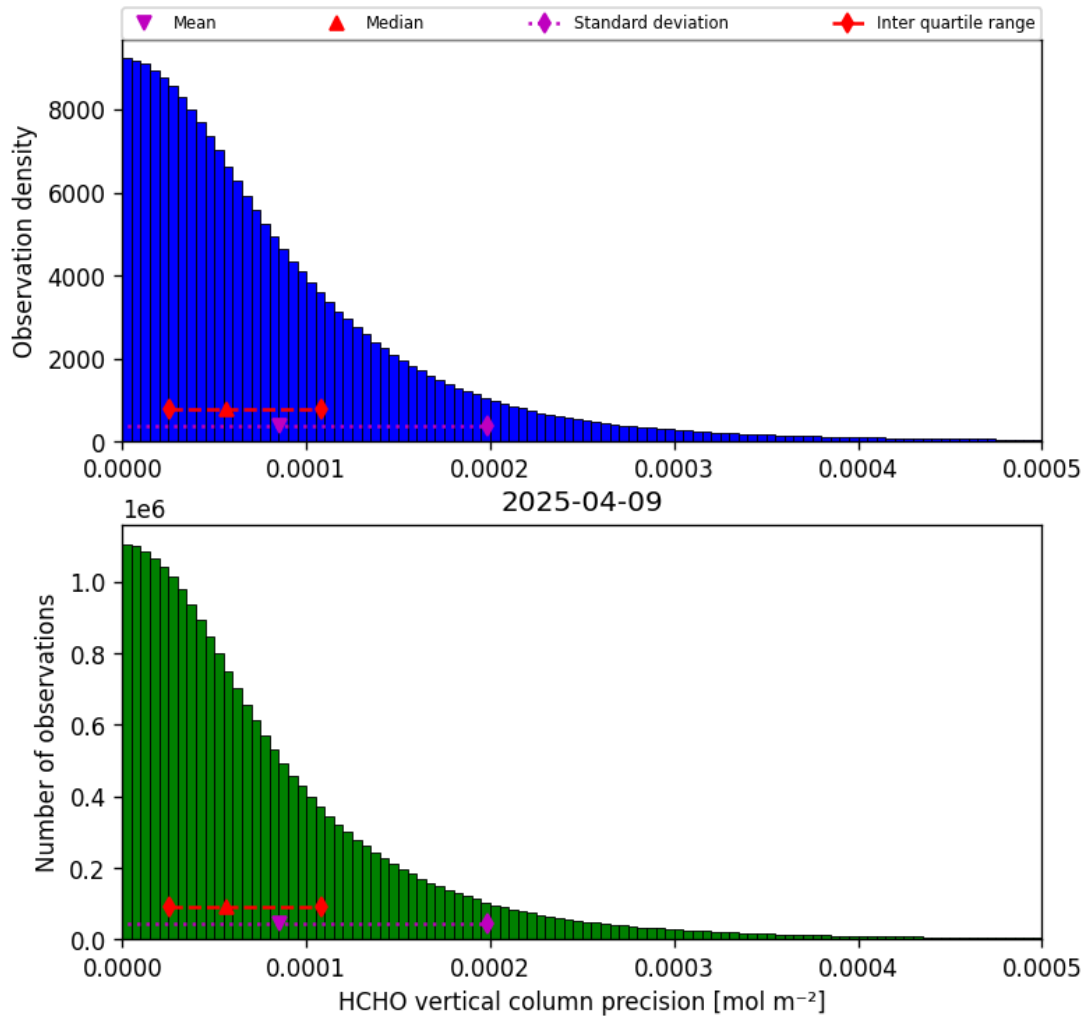
Figure 34: Histogram of “HCHO vertical column precision” for 2025-04-09 to 2025-04-10
