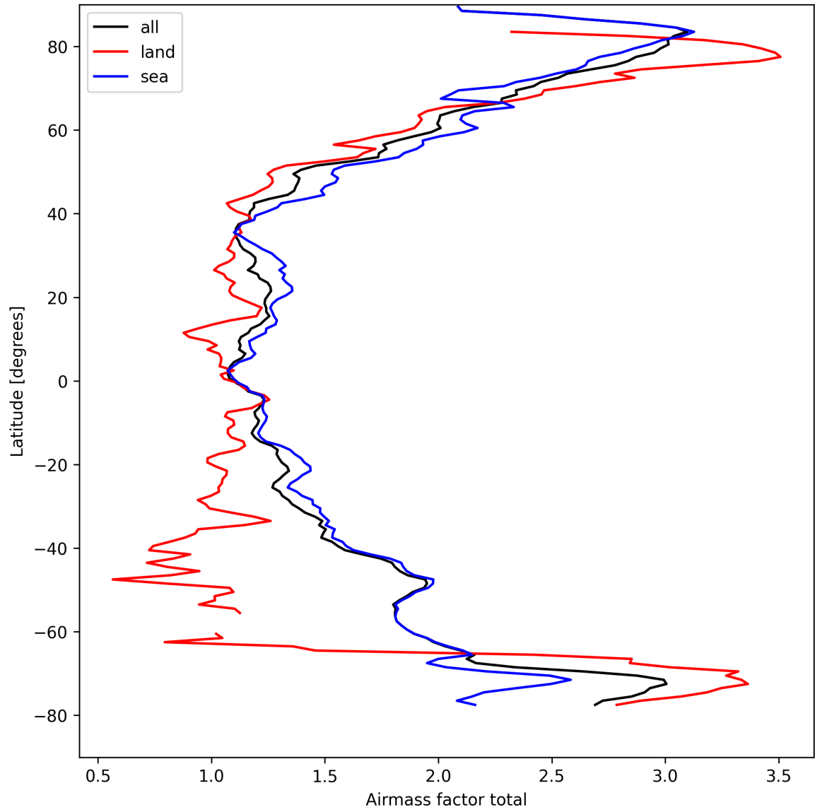
Figure 24: Zonal average of “Airmass factor total” for 2025-04-09 to 2025-04-10.
