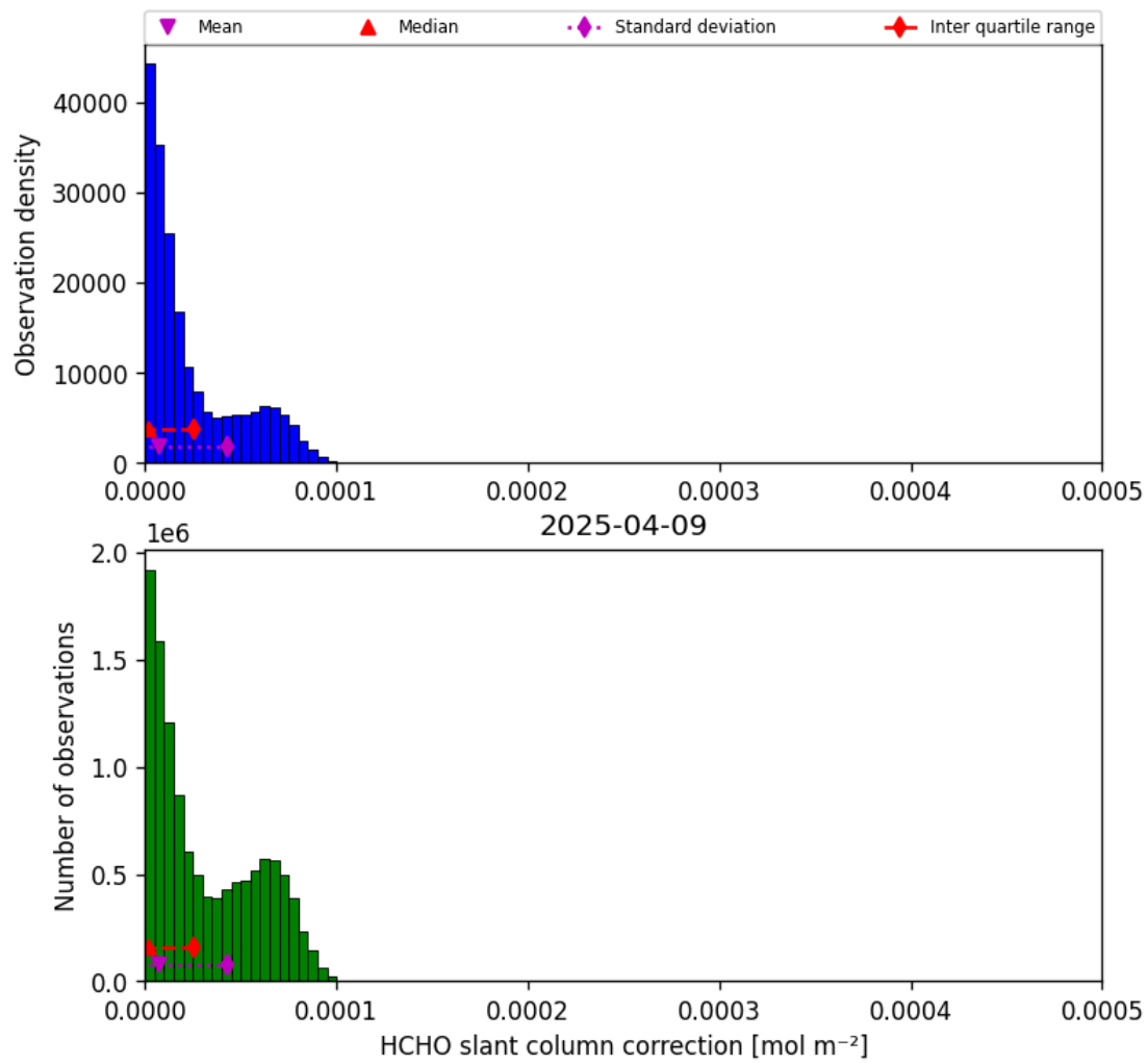
Figure 45: Histogram of “HCHO slant column correction” for 2025-04-09 to 2025-04-10
