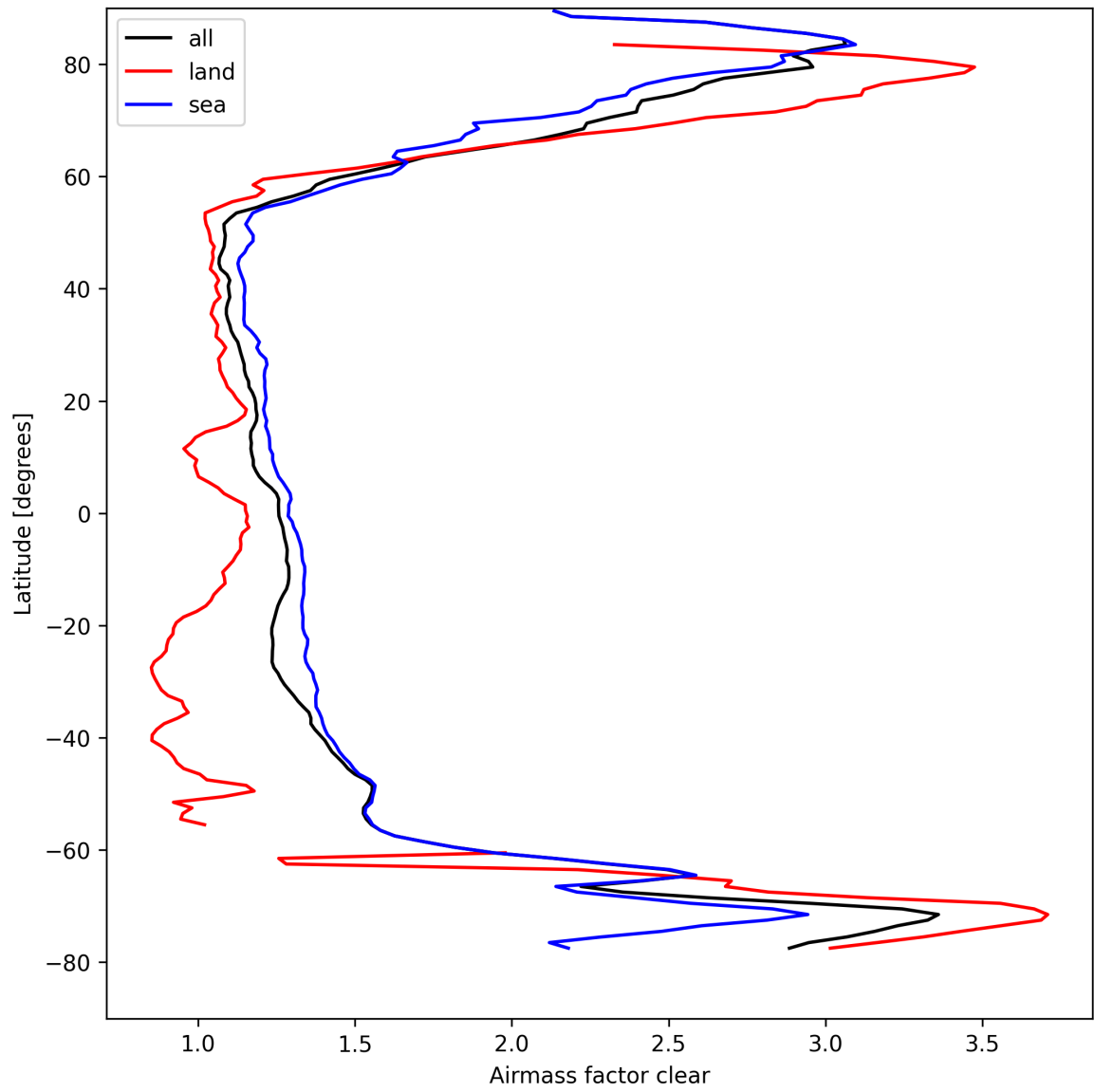
Figure 26: Zonal average of “Airmass factor clear” for 2025-04-09 to 2025-04-10.
