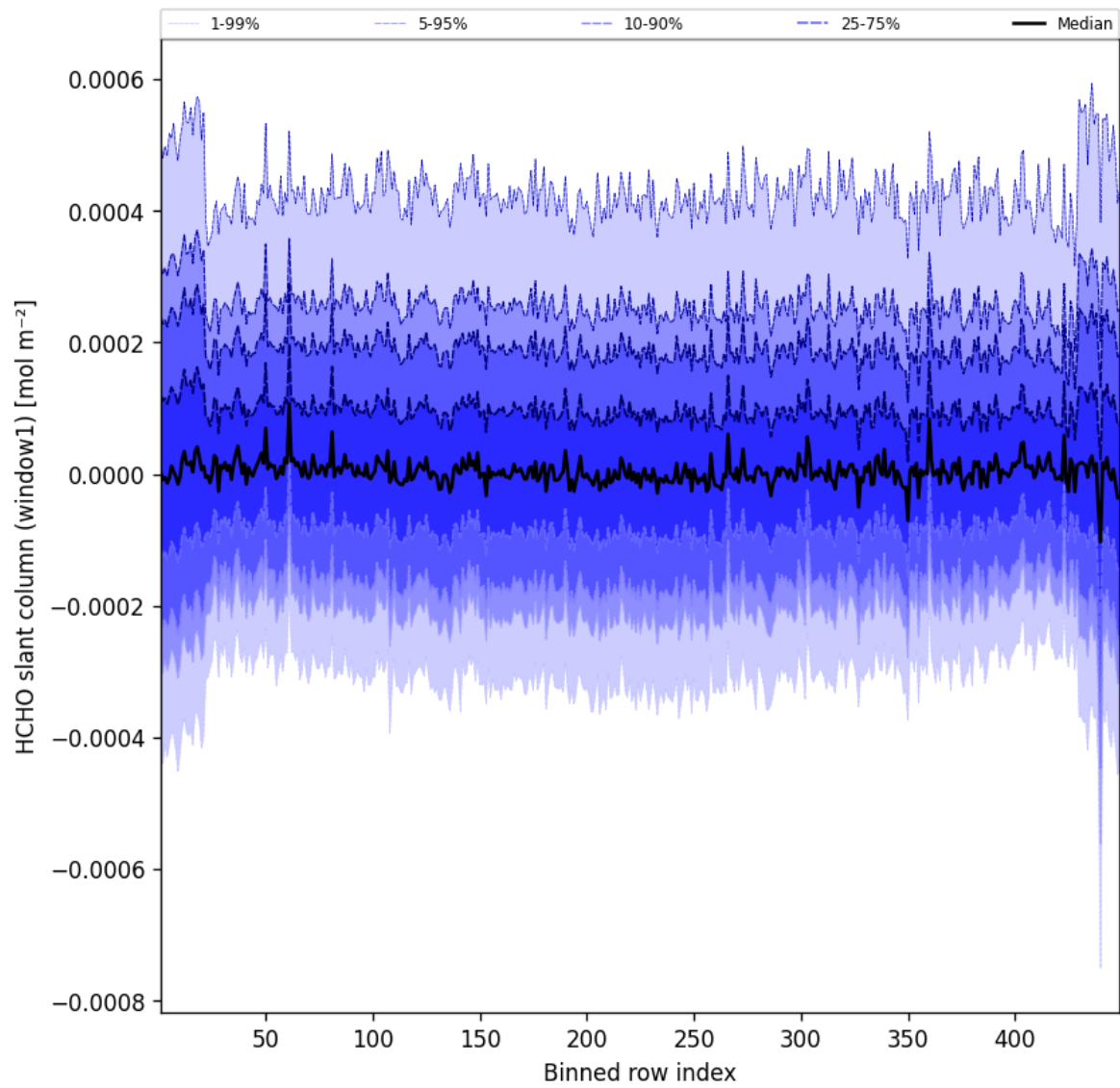
Figure 50: Along track statistics of “HCHO slant column (window1)” for 2025-04-09 to 2025-04-10
