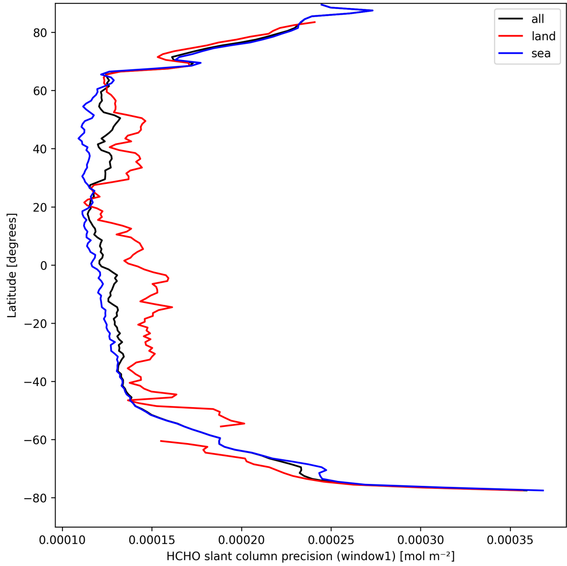
Figure 23: Zonal average of “HCHO slant column precision (window1)” for 2025-04-09 to 2025-04-10.
