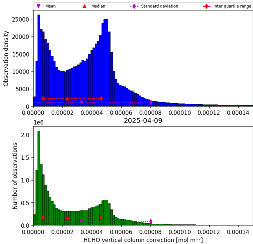
Figure 35: Histogram of “HCHO vertical column correction” for 2025-04-09 to 2025-04-10
