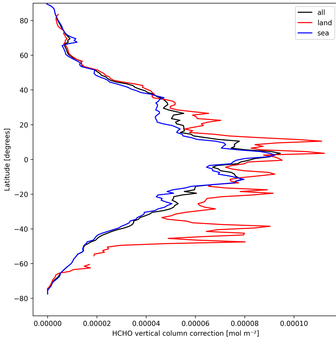
Figure 21: Zonal average of “HCHO vertical column correction” for 2025-04-09 to 2025-04-10.
