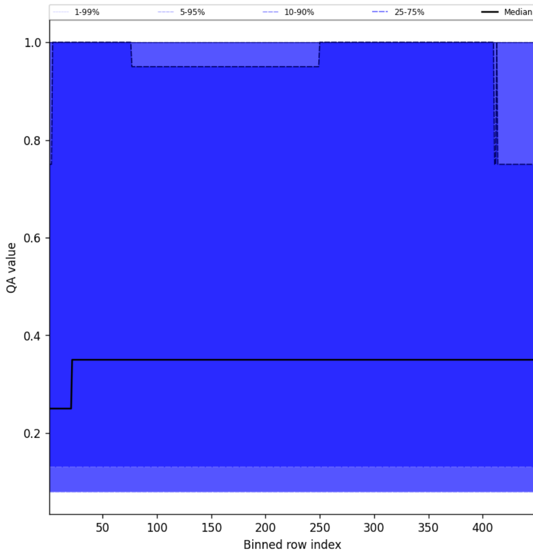
Figure 46: Along track statistics of “QA value” for 2025-04-09 to 2025-04-10
