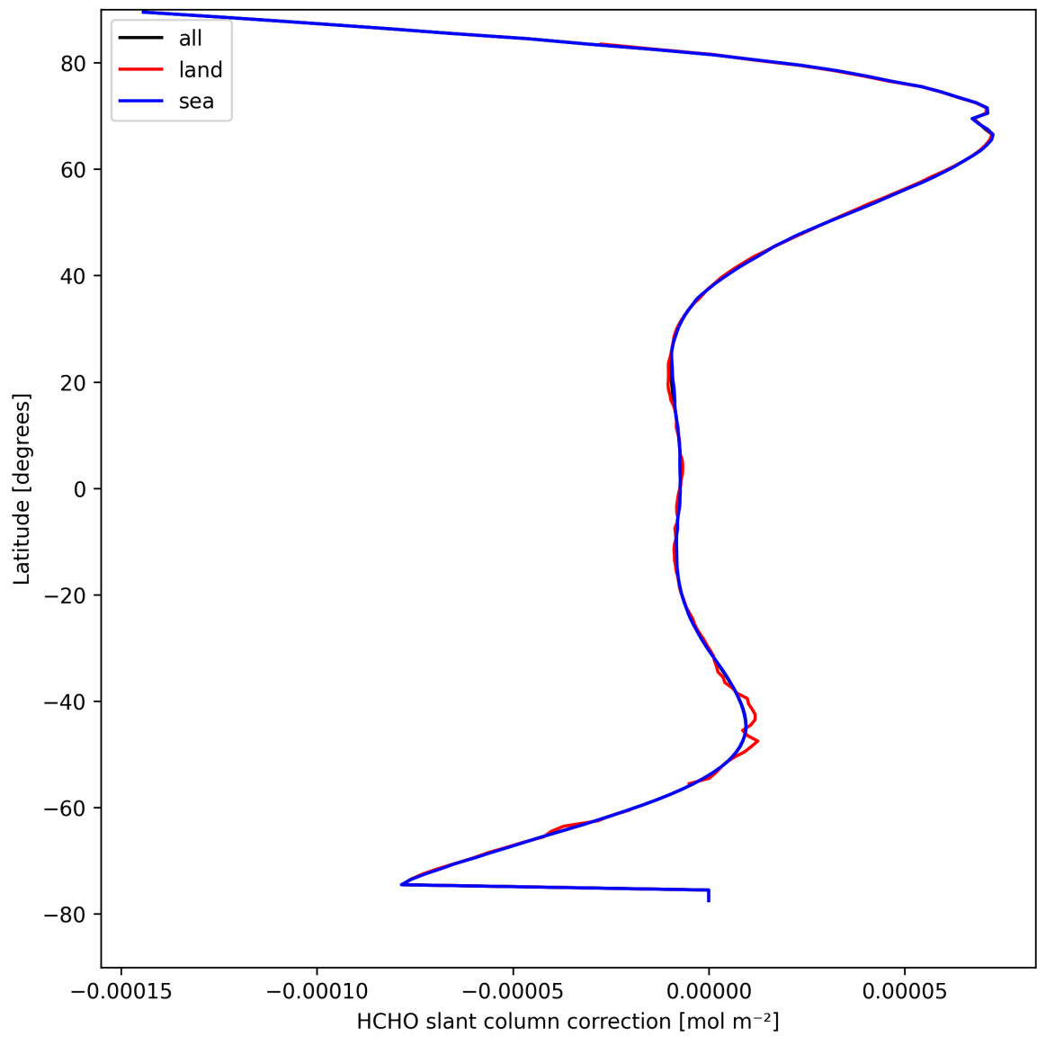
Figure 31: Zonal average of “HCHO slant column correction” for 2025-04-09 to 2025-04-10.
