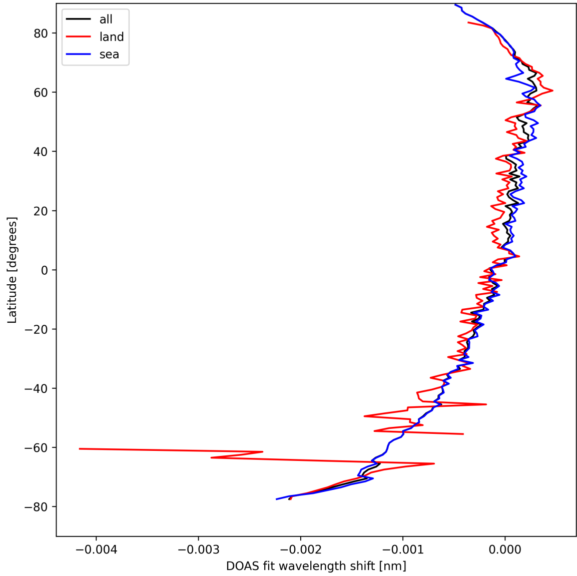
Figure 28: Zonal average of “DOAS fit wavelength shift” for 2025-04-09 to 2025-04-10.
