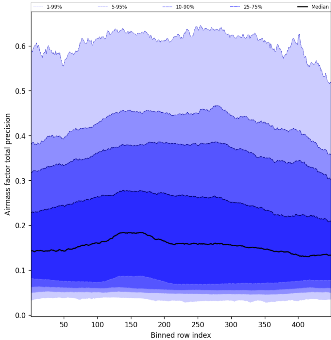
Figure 53: Along track statistics of “Airmass factor total precision” for 2025-04-09 to 2025-04-10
