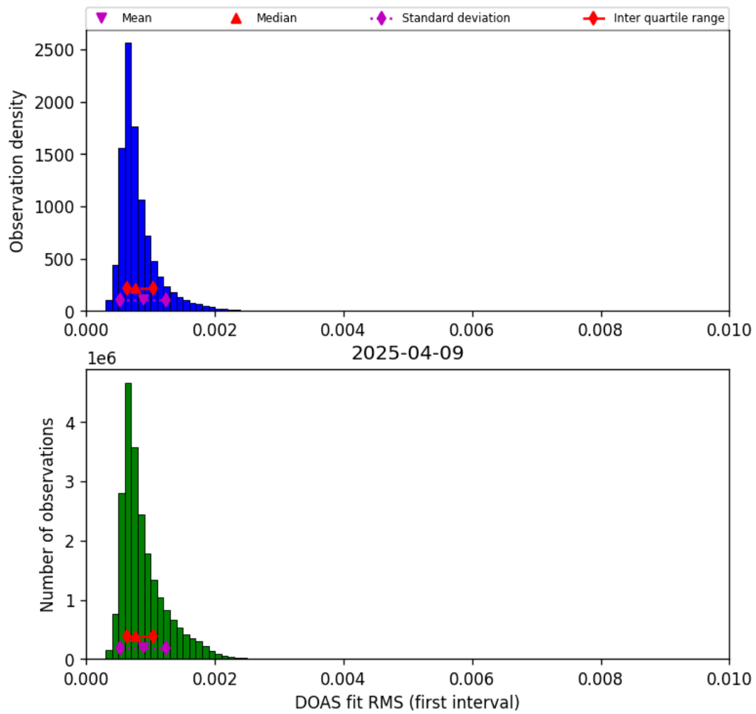
Figure 44: Histogram of “DOAS fit RMS (first interval)” for 2025-04-09 to 2025-04-10
