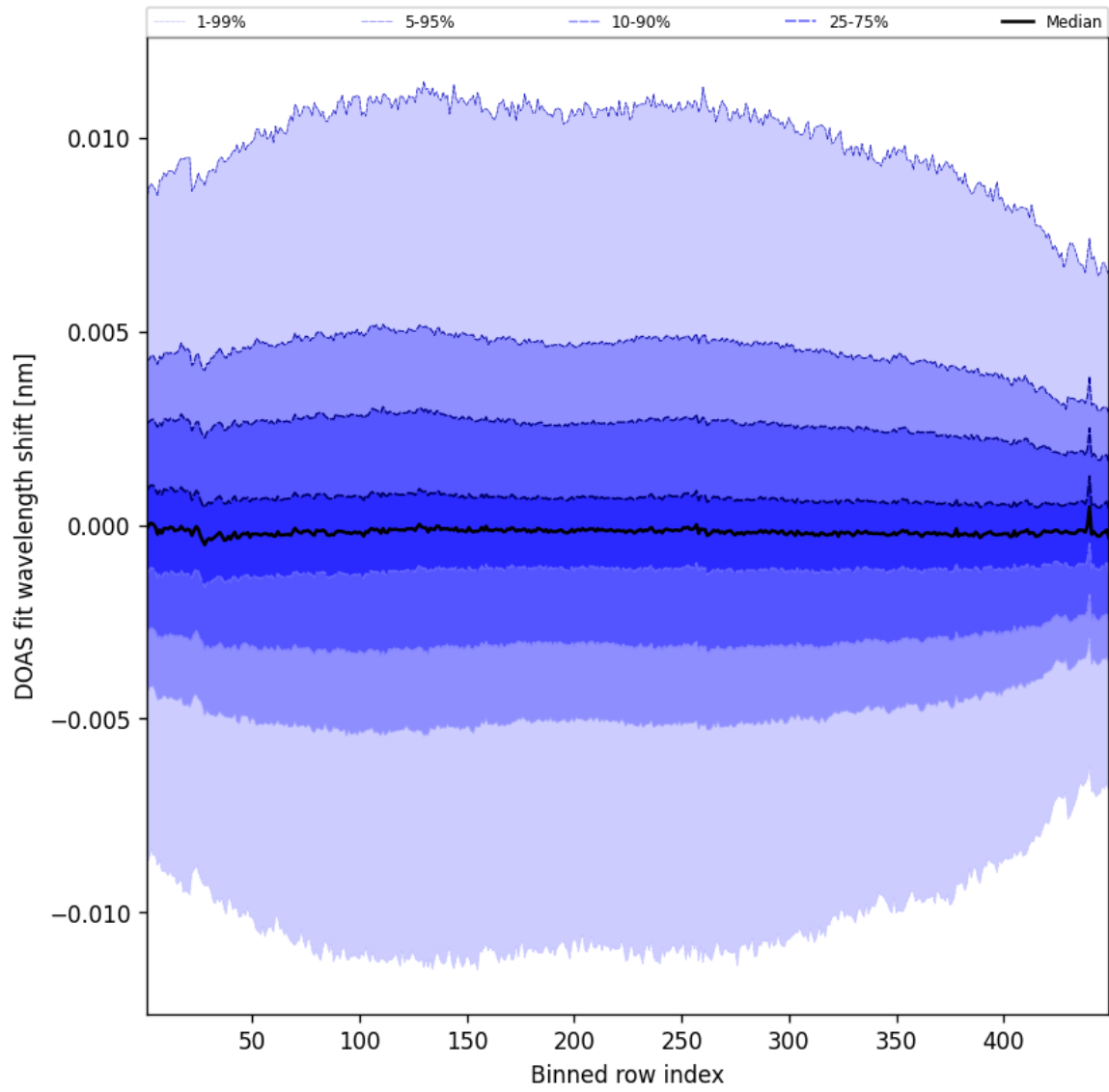
Figure 56: Along track statistics of “DOAS fit wavelength shift” for 2025-04-09 to 2025-04-10
