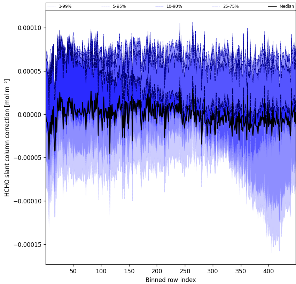
Figure 59: Along track statistics of “HCHO slant column correction” for 2025-04-09 to 2025-04-10
