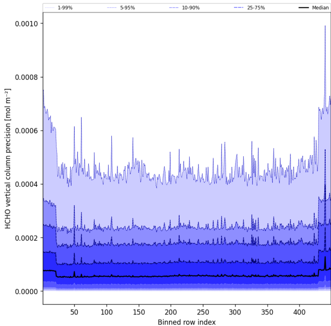
Figure 48: Along track statistics of “HCHO vertical column precision” for 2025-04-10 to 2025-04-11
