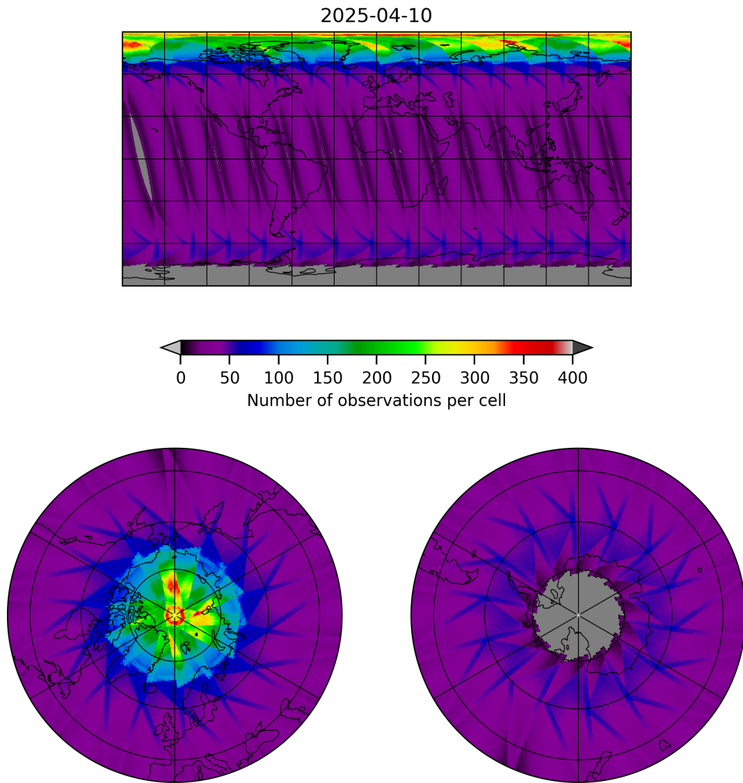
Figure 17: Map of the number of observations for 2025-04-10 to 2025-04-11
