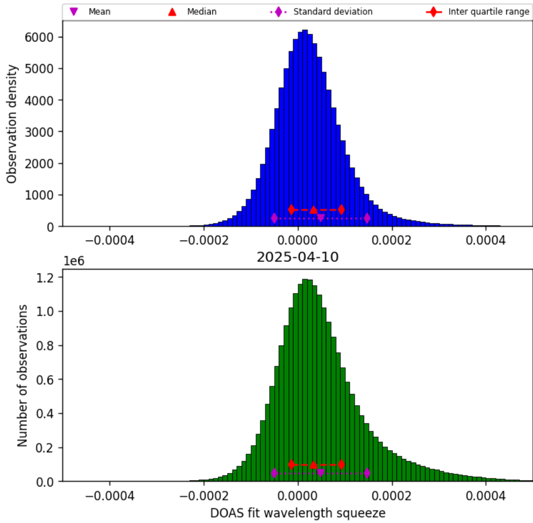
Figure 43: Histogram of “DOAS fit wavelength squeeze” for 2025-04-10 to 2025-04-11
