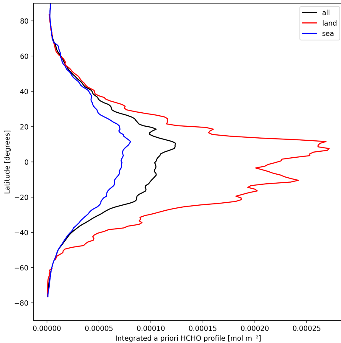
Figure 27: Zonal average of “Integrated a priori HCHO profile” for 2025-04-10 to 2025-04-11.
