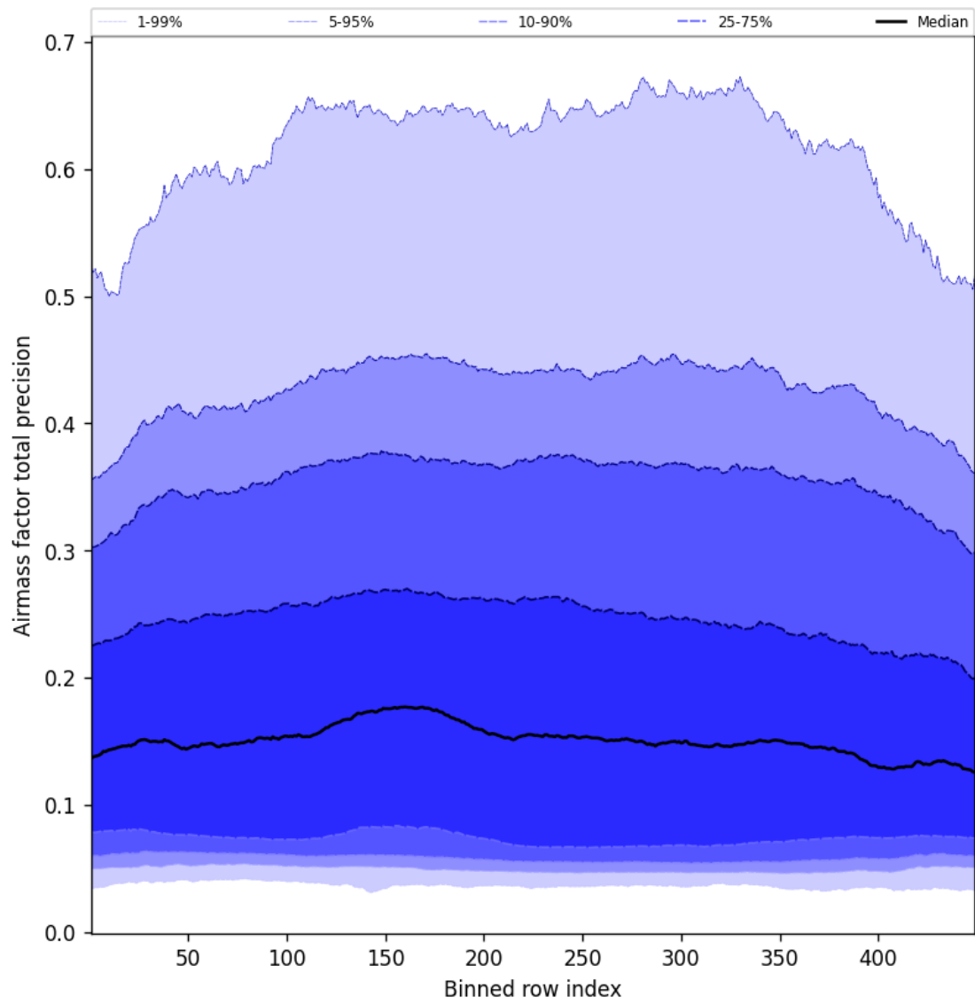
Figure 53: Along track statistics of “Airmass factor total precision” for 2025-04-10 to 2025-04-11
