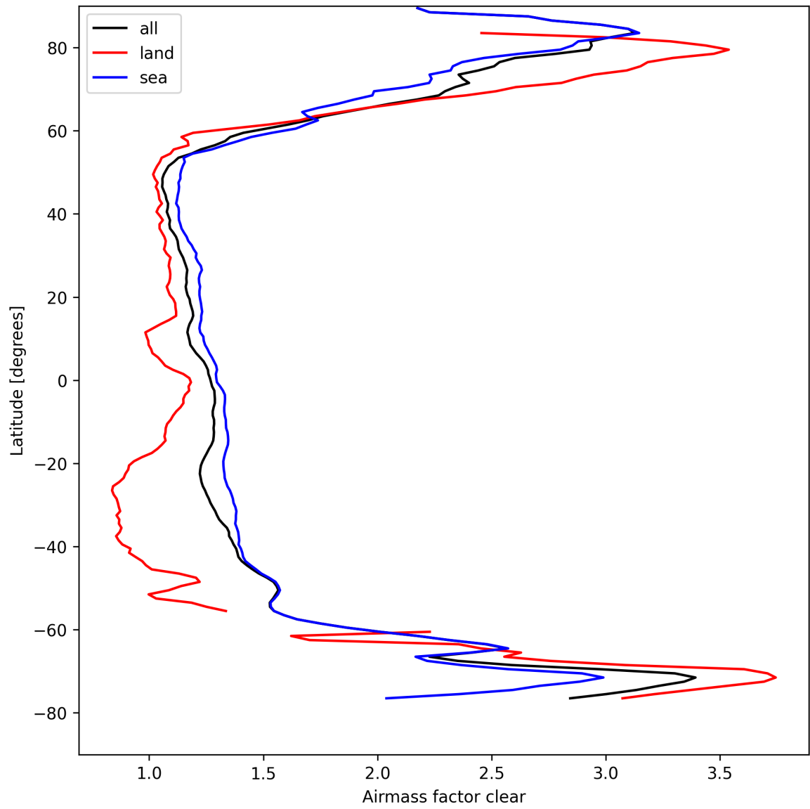
Figure 26: Zonal average of “Airmass factor clear” for 2025-04-10 to 2025-04-11.
