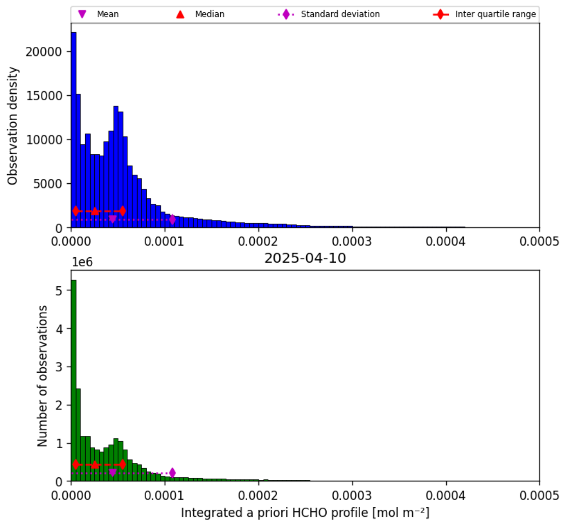
Figure 41: Histogram of “Integrated a priori HCHO profile” for 2025-04-10 to 2025-04-11
