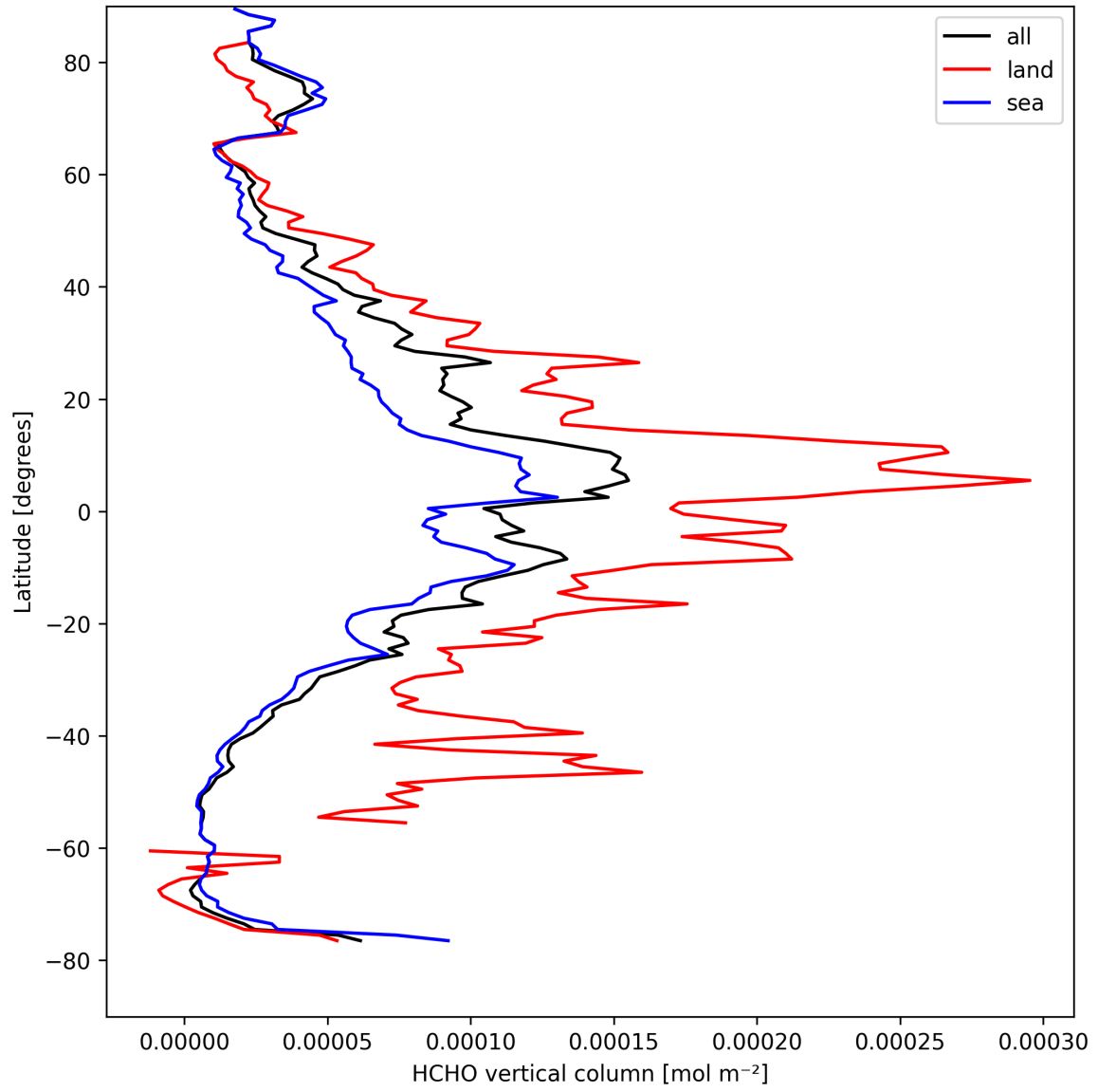
Figure 19: Zonal average of “HCHO vertical column” for 2025-04-10 to 2025-04-11.
