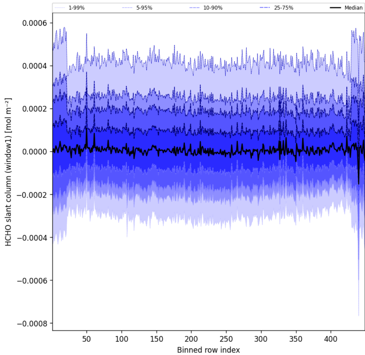
Figure 50: Along track statistics of “HCHO slant column (window1)” for 2025-04-10 to 2025-04-11
