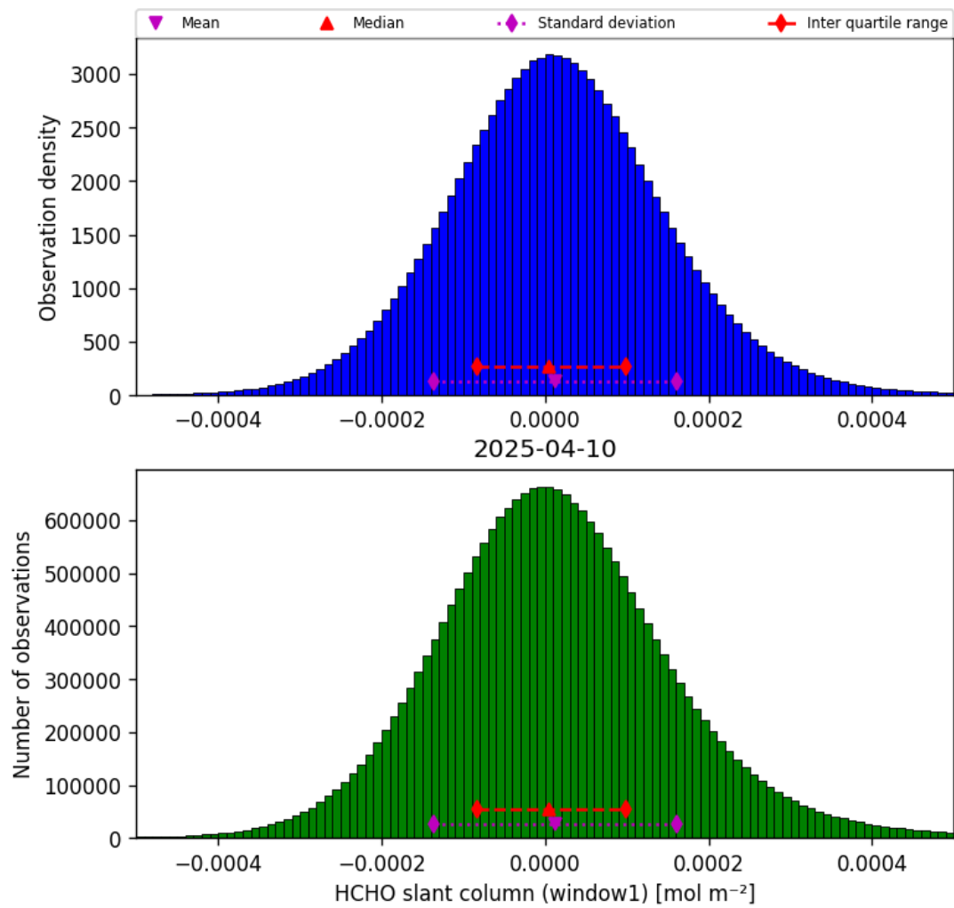
Figure 36: Histogram of “HCHO slant column (window1)” for 2025-04-10 to 2025-04-11
