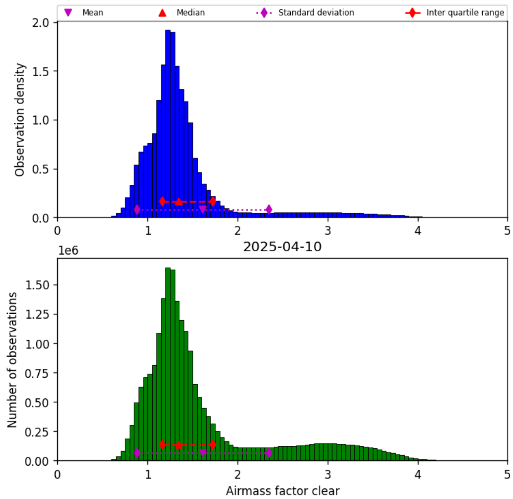
Figure 40: Histogram of “Airmass factor clear” for 2025-04-10 to 2025-04-11
