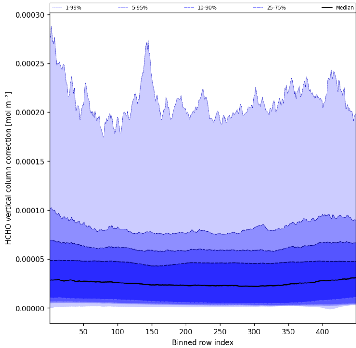
Figure 49: Along track statistics of “HCHO vertical column correction” for 2025-04-10 to 2025-04-11
