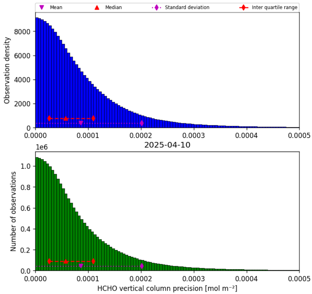
Figure 34: Histogram of “HCHO vertical column precision” for 2025-04-10 to 2025-04-11
