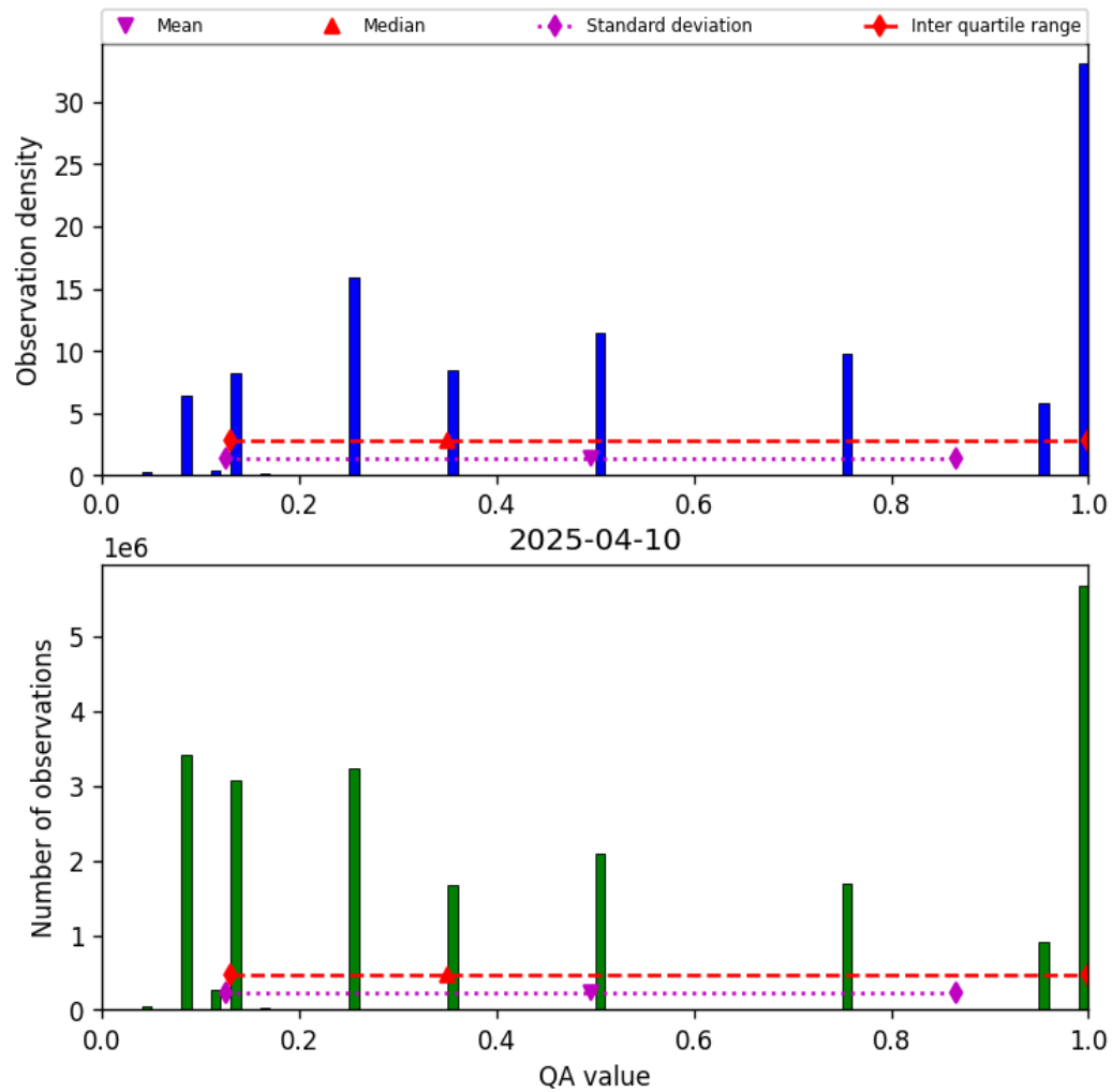
Figure 32: Histogram of “QA value” for 2025-04-10 to 2025-04-11
