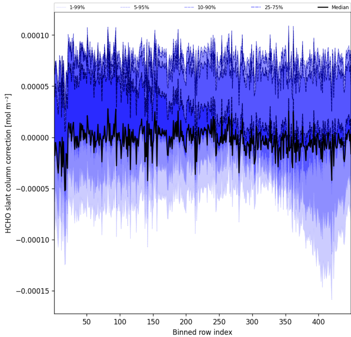
Figure 59: Along track statistics of “HCHO slant column correction” for 2025-04-10 to 2025-04-11
