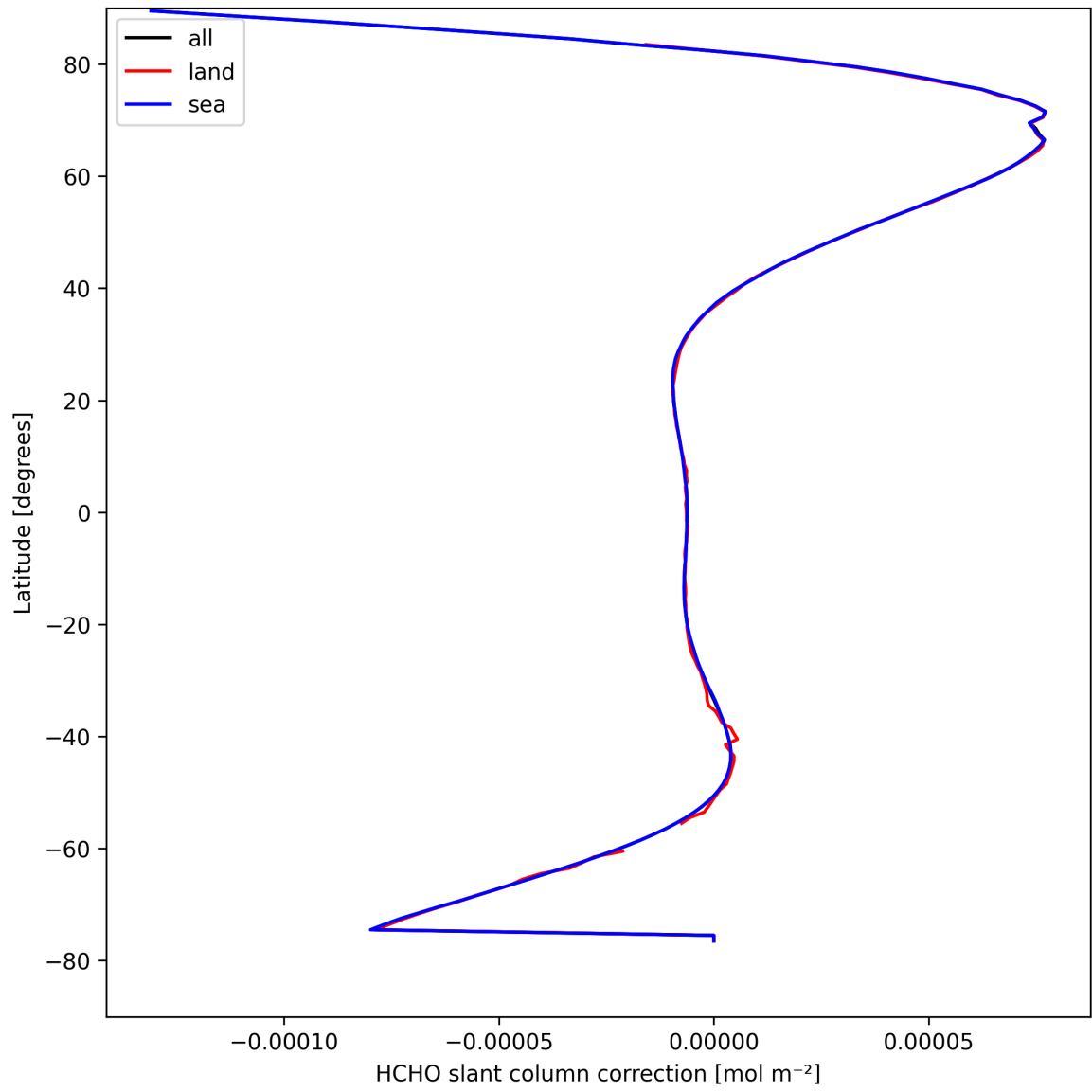
Figure 31: Zonal average of “HCHO slant column correction” for 2025-04-10 to 2025-04-11.
