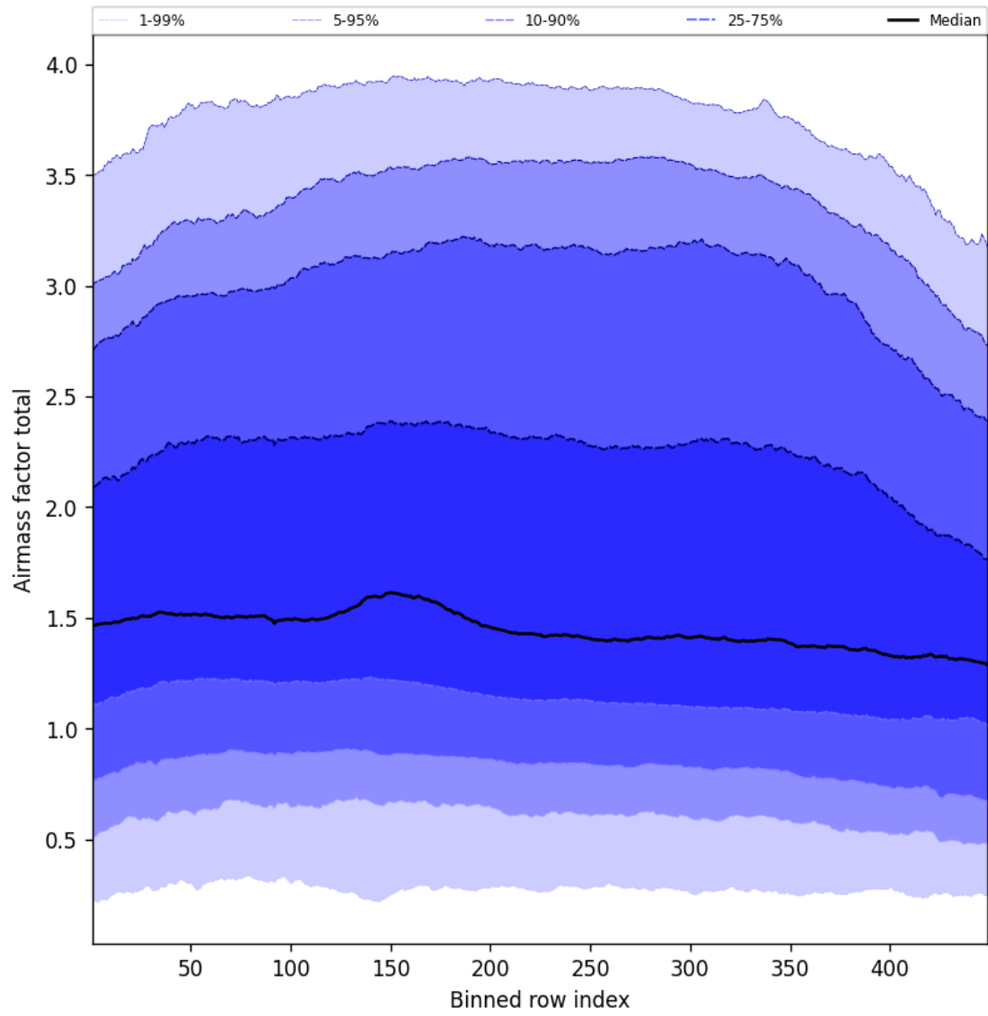
Figure 52: Along track statistics of “Airmass factor total” for 2025-04-10 to 2025-04-11
