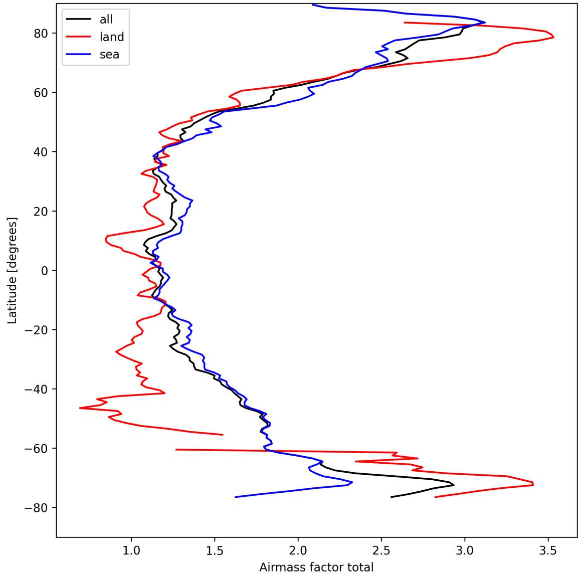
Figure 24: Zonal average of “Airmass factor total” for 2025-04-10 to 2025-04-11.
