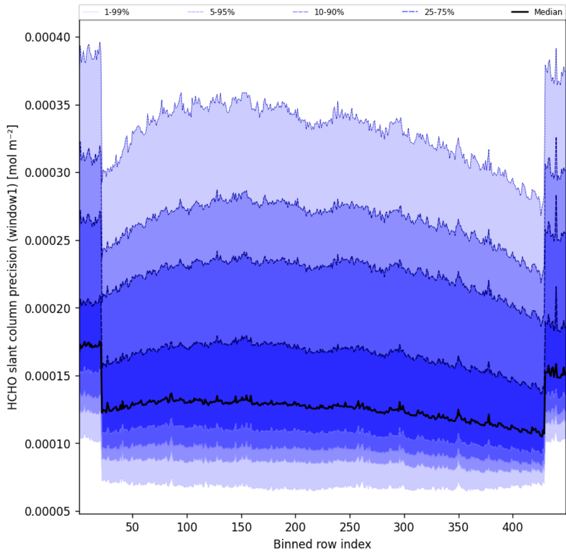
Figure 51: Along track statistics of “HCHO slant column precision (window1)” for 2025-04-10 to 2025-04-11
