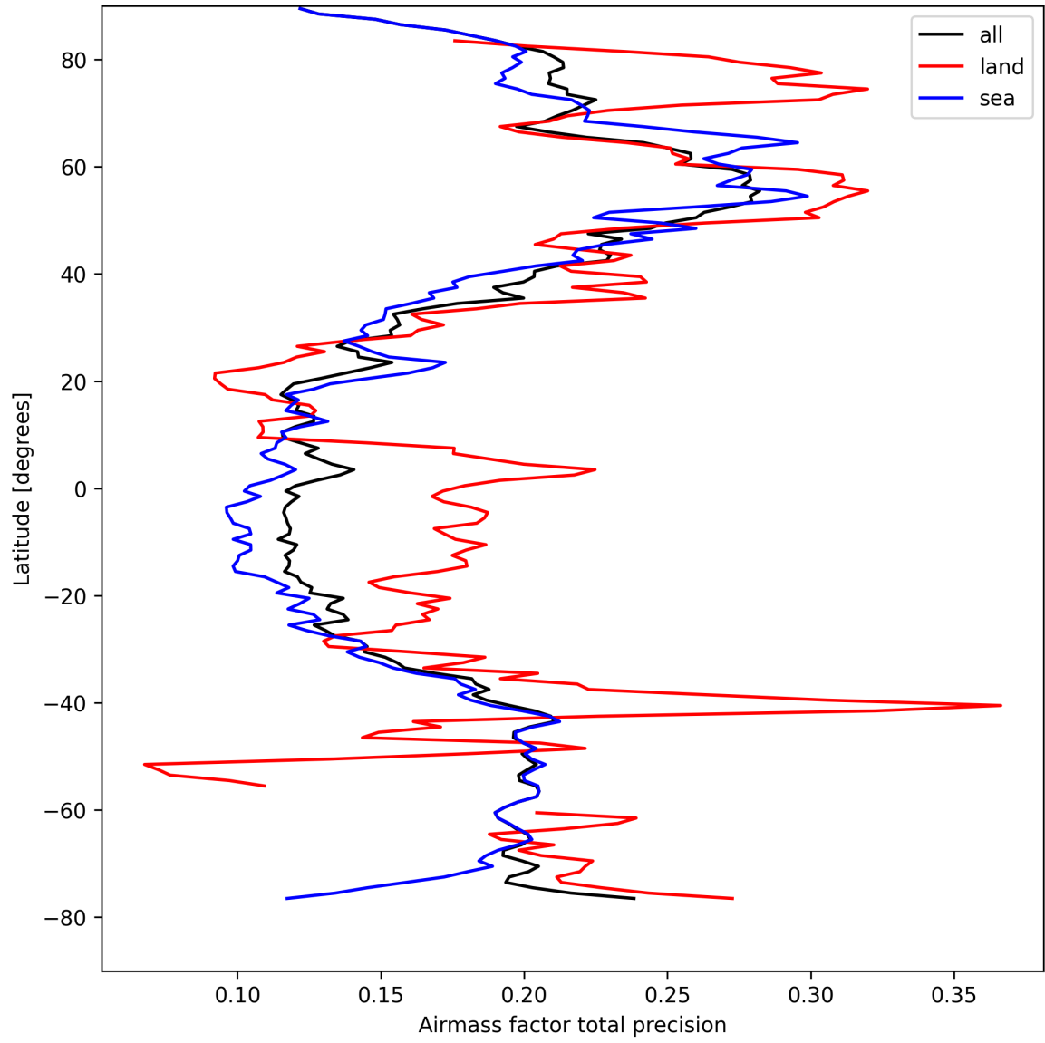
Figure 25: Zonal average of “Airmass factor total precision” for 2025-04-10 to 2025-04-11.
