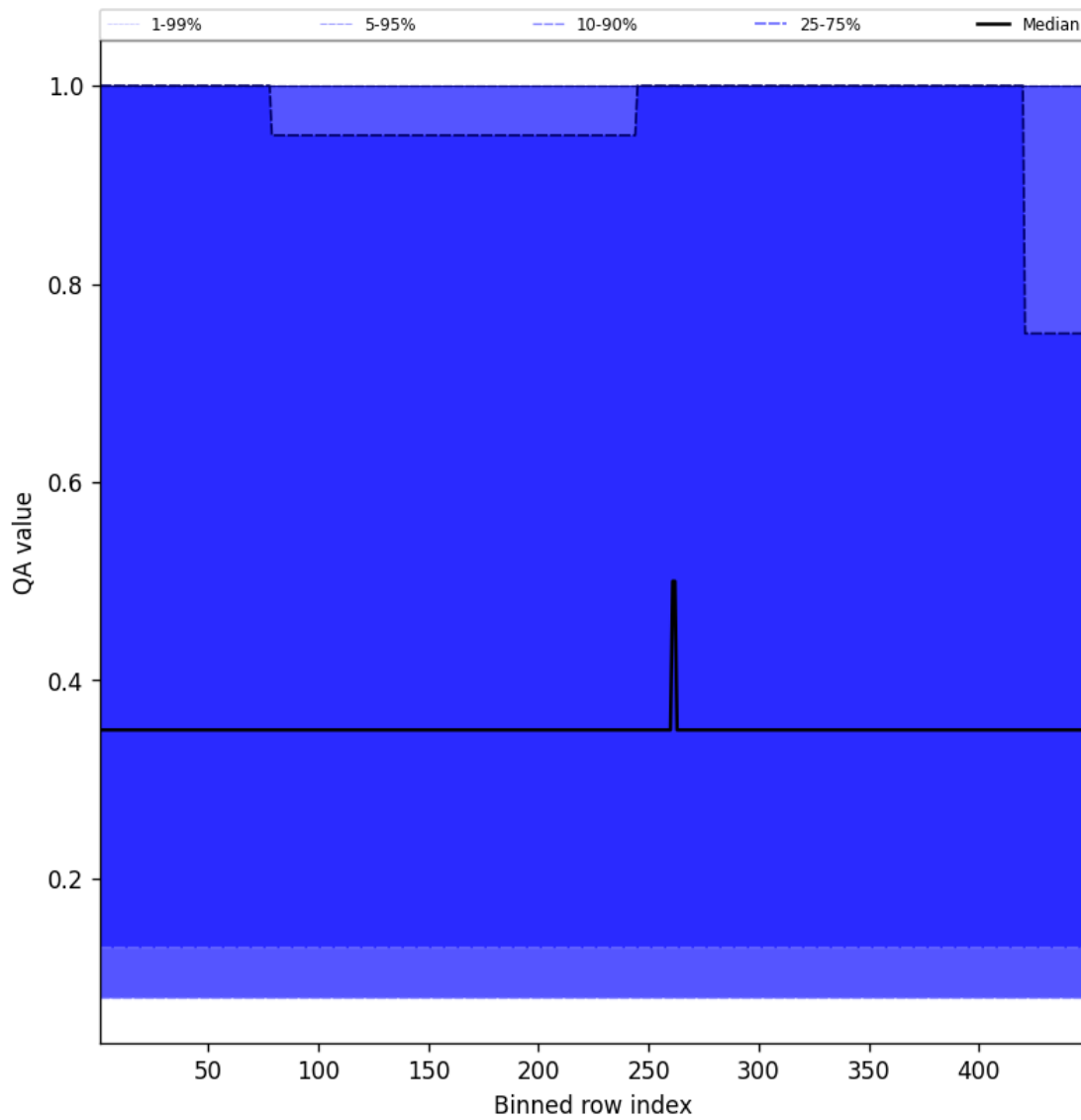
Figure 46: Along track statistics of “QA value” for 2025-04-10 to 2025-04-11
