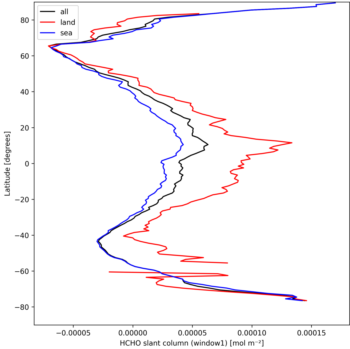
Figure 22: Zonal average of “HCHO slant column (window1)” for 2025-04-10 to 2025-04-11.
