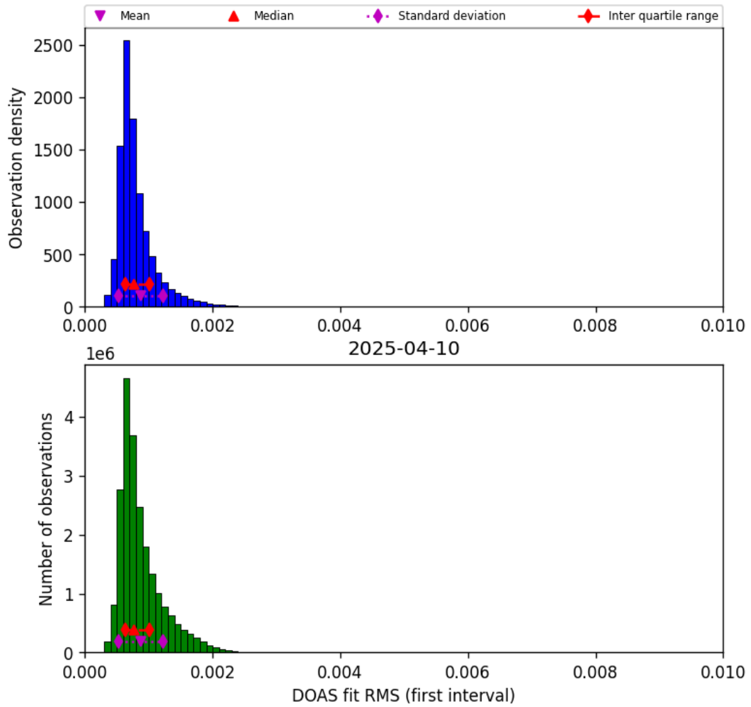
Figure 44: Histogram of “DOAS fit RMS (first interval)” for 2025-04-10 to 2025-04-11
