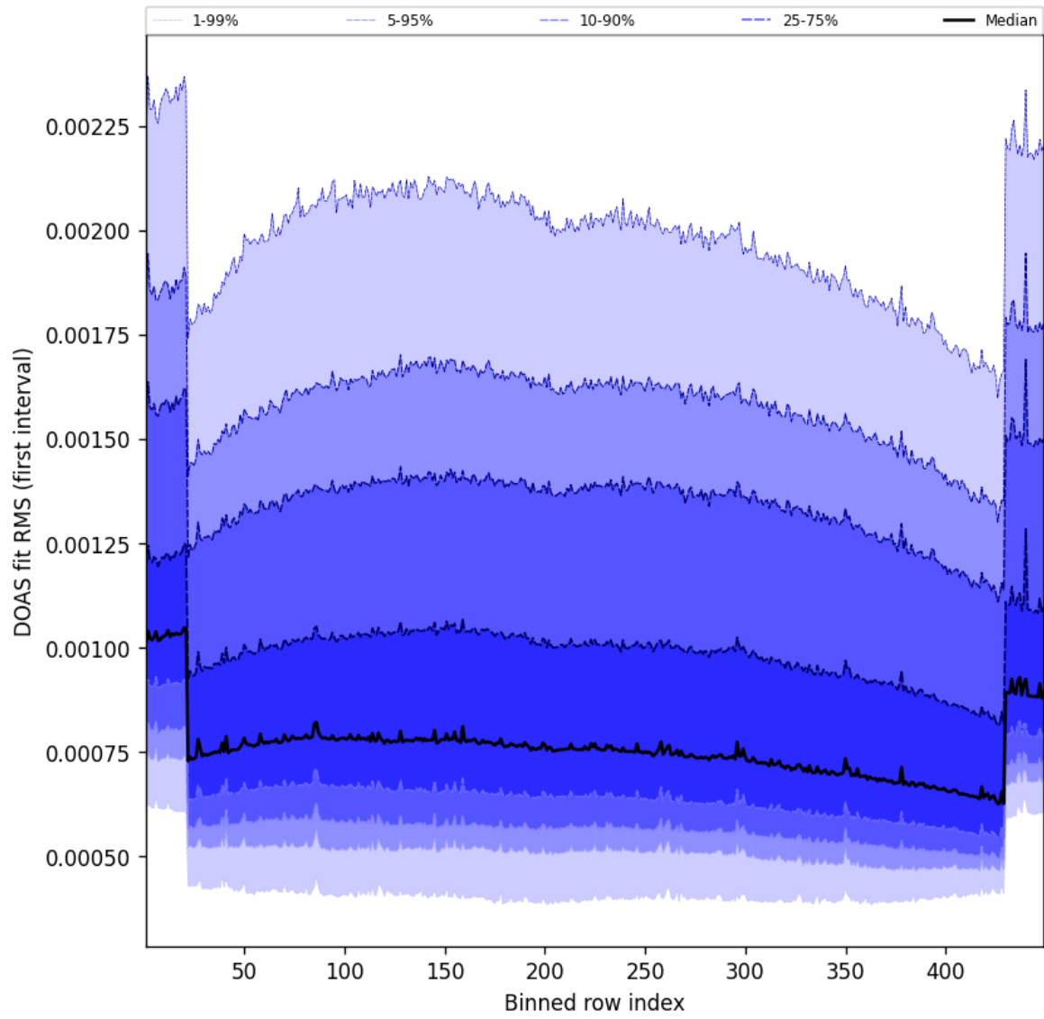
Figure 58: Along track statistics of “DOAS fit RMS (first interval)” for 2025-04-10 to 2025-04-11
