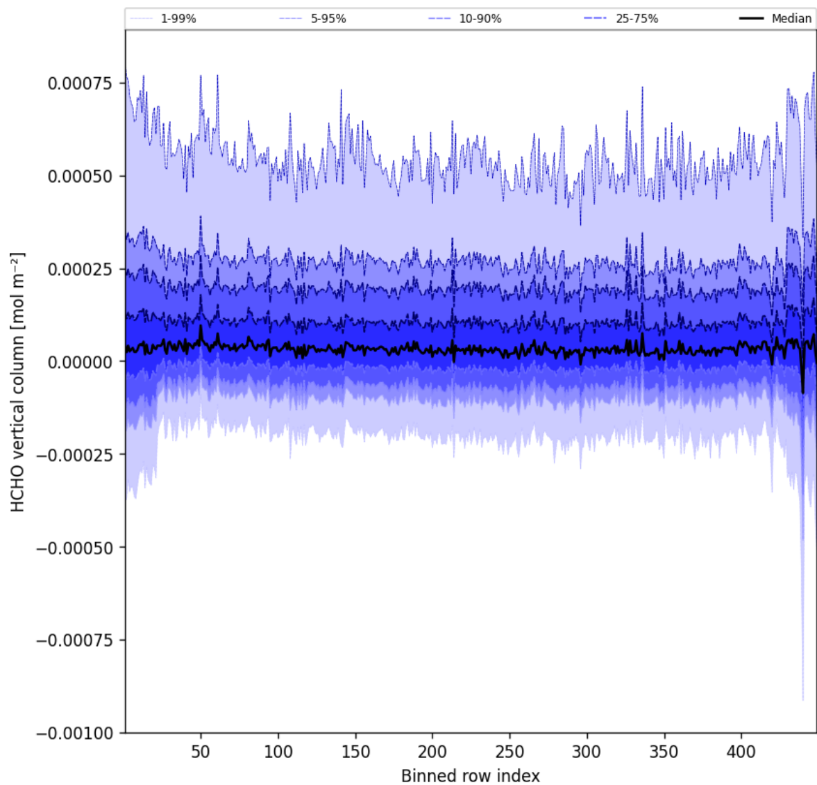
Figure 47: Along track statistics of “HCHO vertical column” for 2025-04-10 to 2025-04-11
