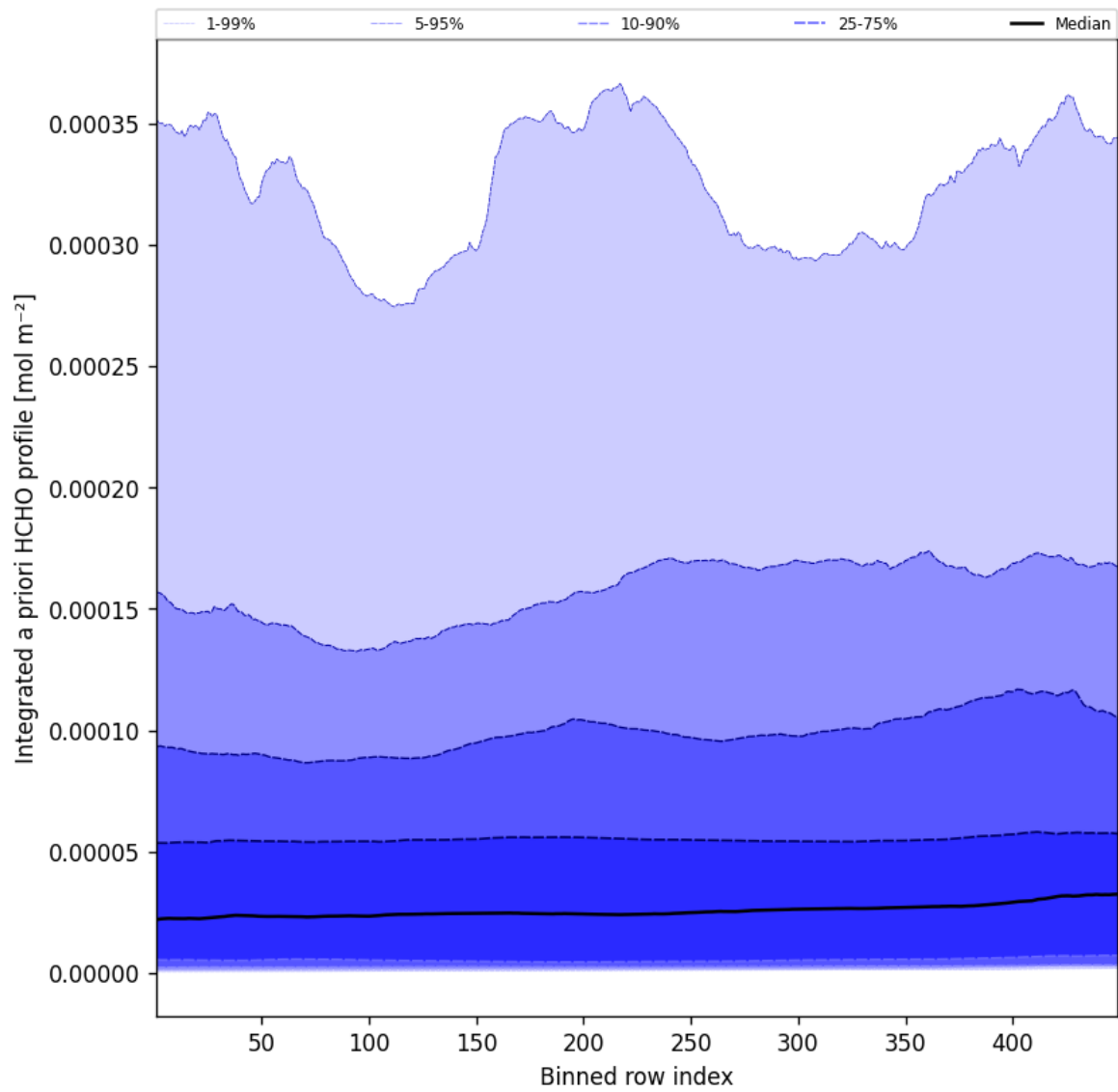
Figure 55: Along track statistics of "Integrated a priori HCHO profile" for 2025-04-10 to 2025-04-11
