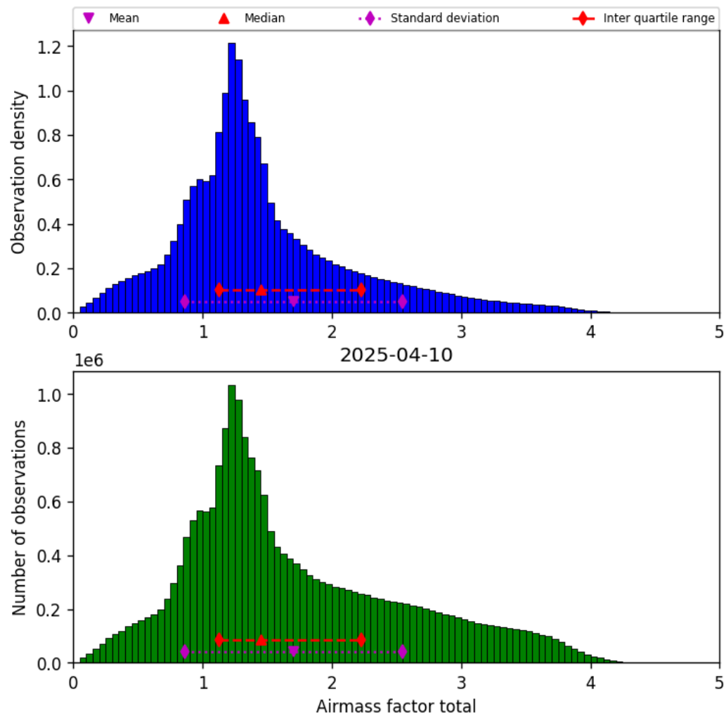
Figure 38: Histogram of “Airmass factor total” for 2025-04-10 to 2025-04-11
