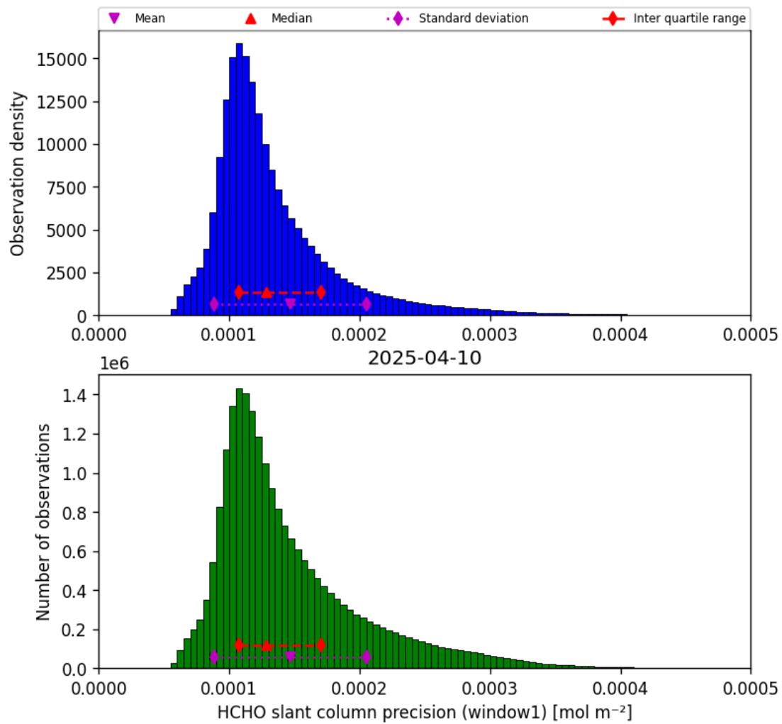
Figure 37: Histogram of “HCHO slant column precision (window1)” for 2025-04-10 to 2025-04-11
