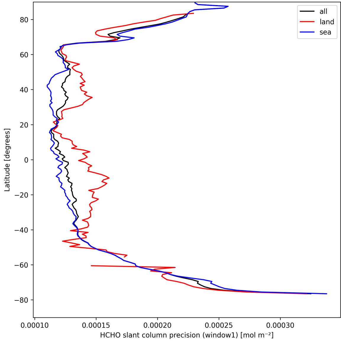
Figure 23: Zonal average of “HCHO slant column precision (window1)” for 2025-04-10 to 2025-04-11.
