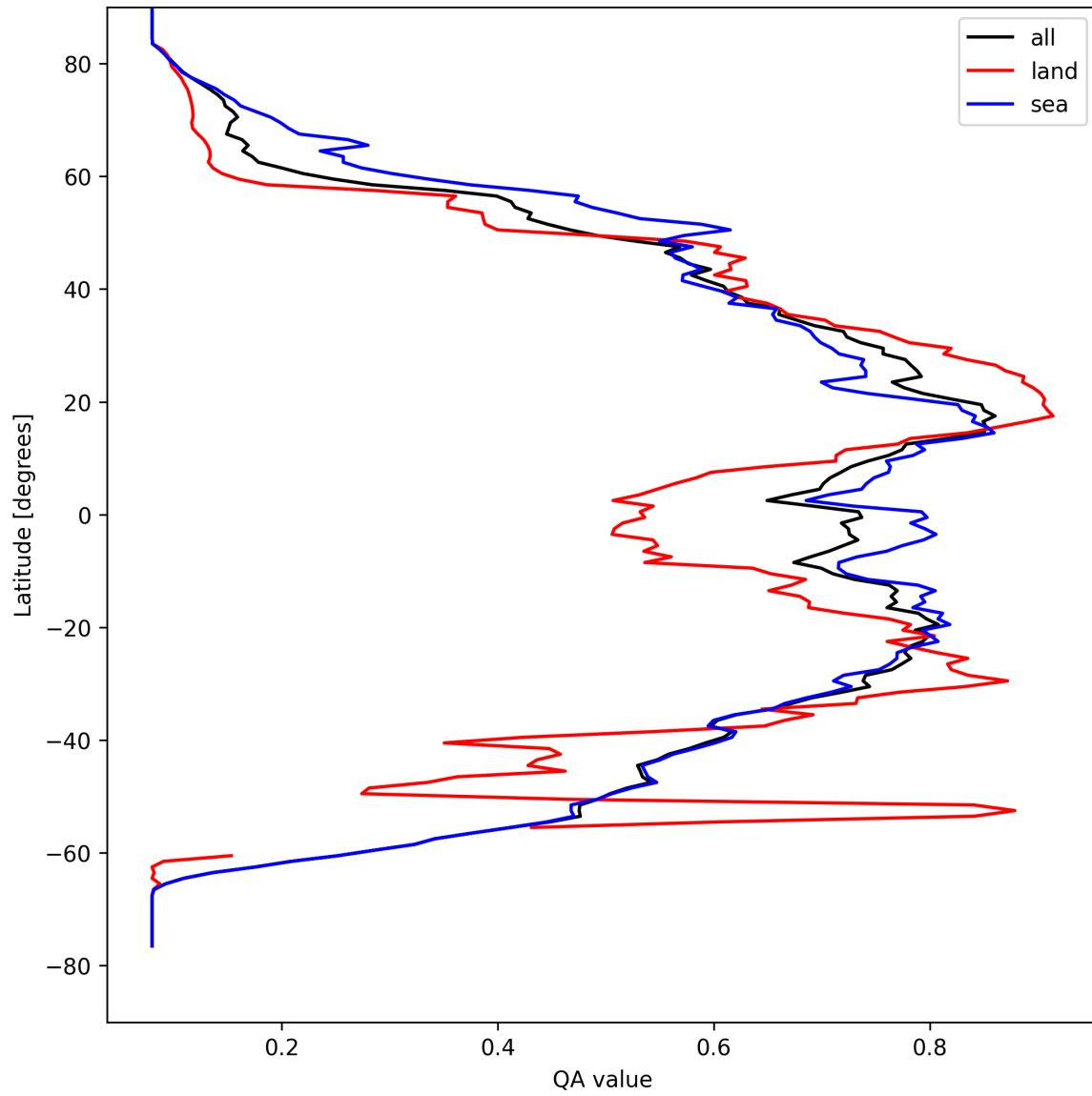
Figure 18: Zonal average of “QA value” for 2025-04-10 to 2025-04-11.
