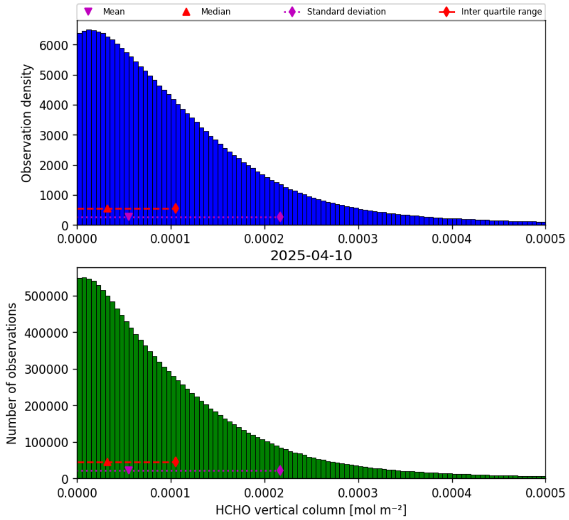
Figure 33: Histogram of “HCHO vertical column” for 2025-04-10 to 2025-04-11
