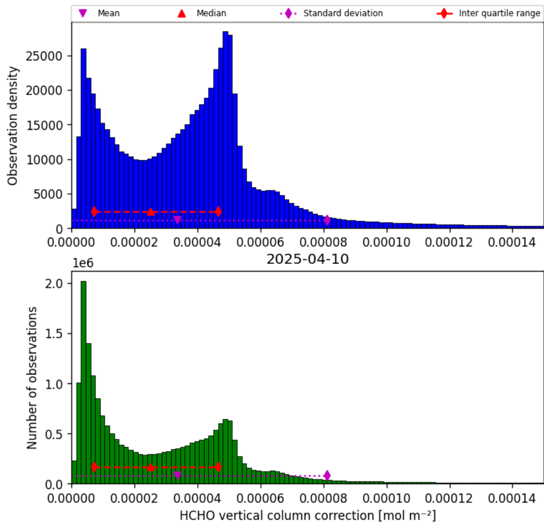
Figure 35: Histogram of “HCHO vertical column correction” for 2025-04-10 to 2025-04-11
