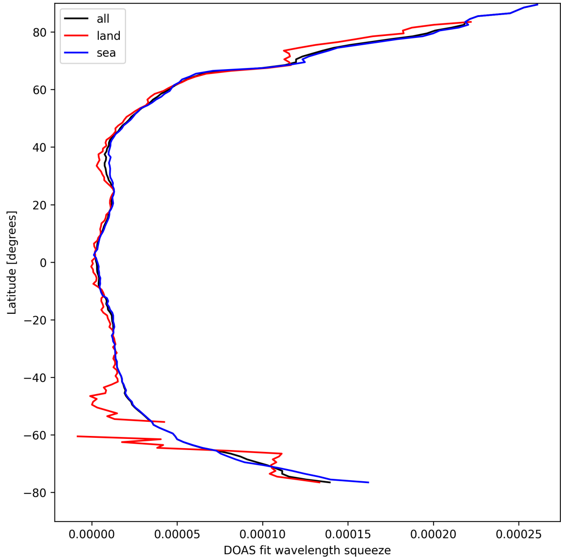
Figure 29: Zonal average of “DOAS fit wavelength squeeze” for 2025-04-10 to 2025-04-11.
