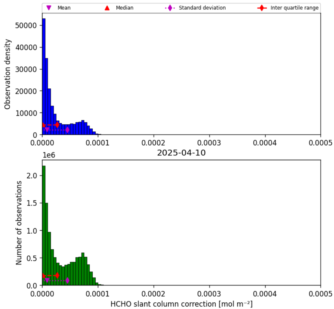
Figure 45: Histogram of “HCHO slant column correction” for 2025-04-10 to 2025-04-11
