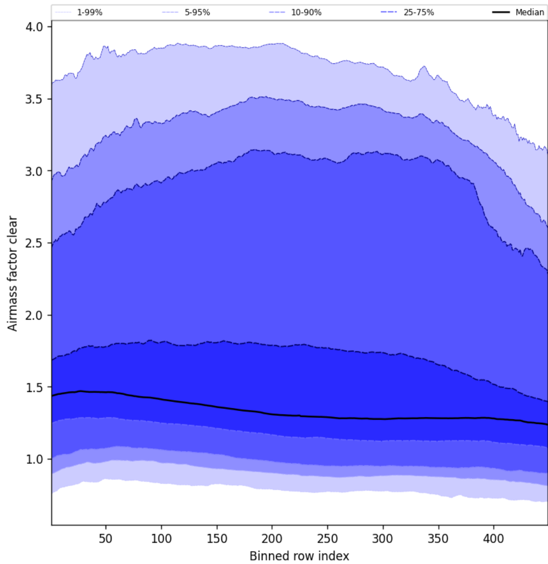
Figure 54: Along track statistics of “Airmass factor clear” for 2025-04-10 to 2025-04-11
