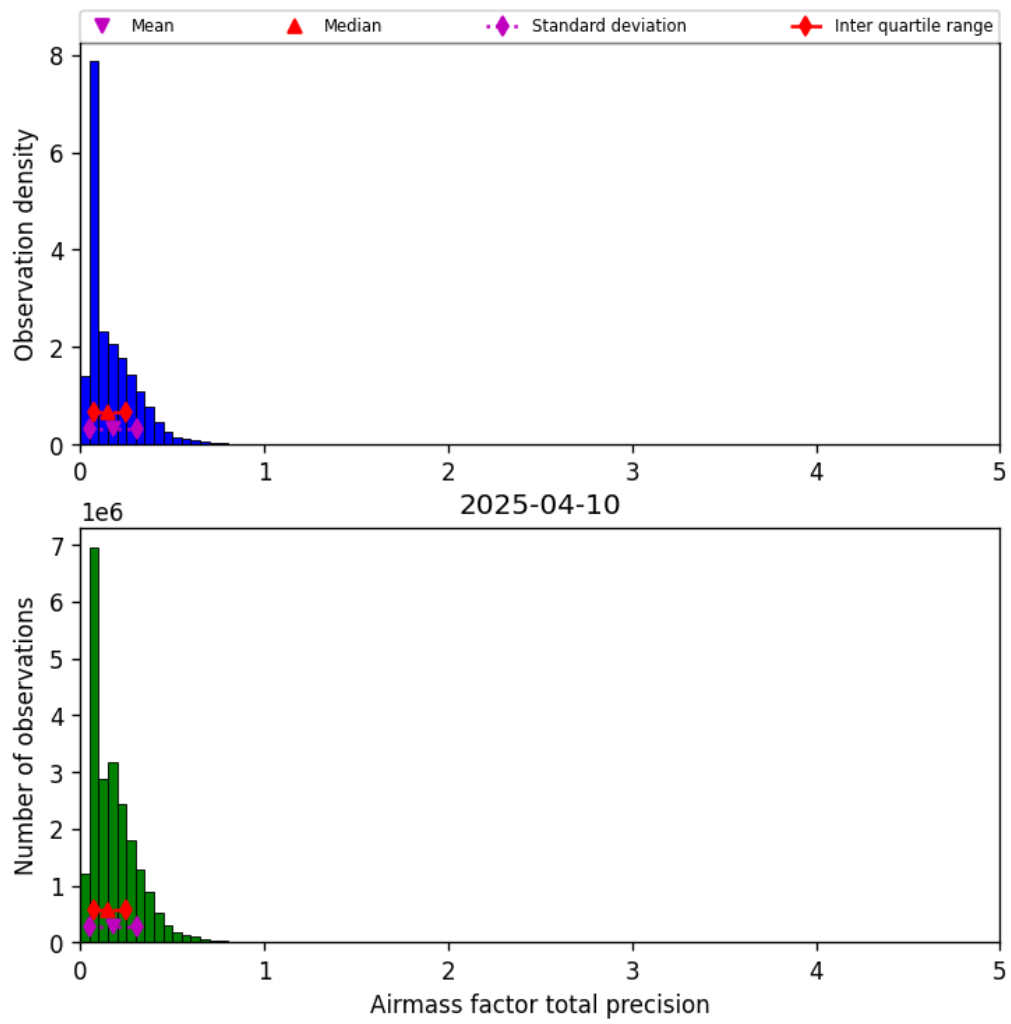
Figure 39: Histogram of “Airmass factor total precision” for 2025-04-10 to 2025-04-11
