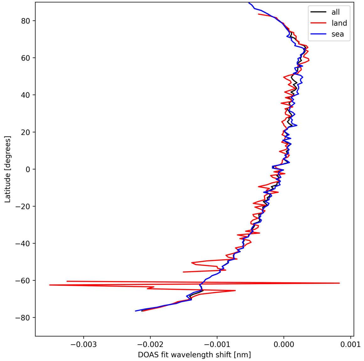
Figure 28: Zonal average of “DOAS fit wavelength shift” for 2025-04-10 to 2025-04-11.
