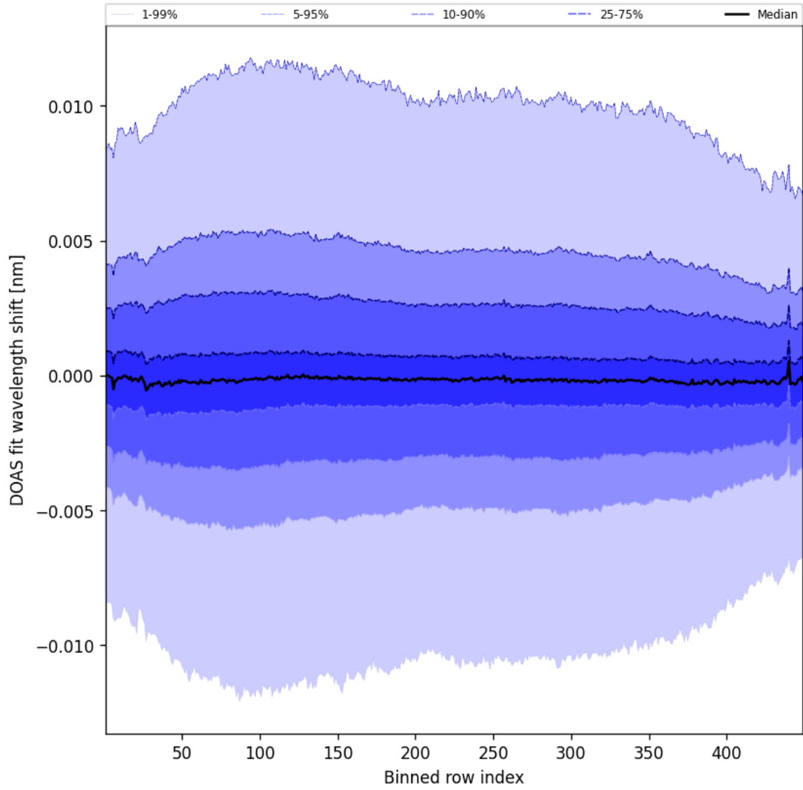
Figure 56: Along track statistics of “DOAS fit wavelength shift” for 2025-04-10 to 2025-04-11
