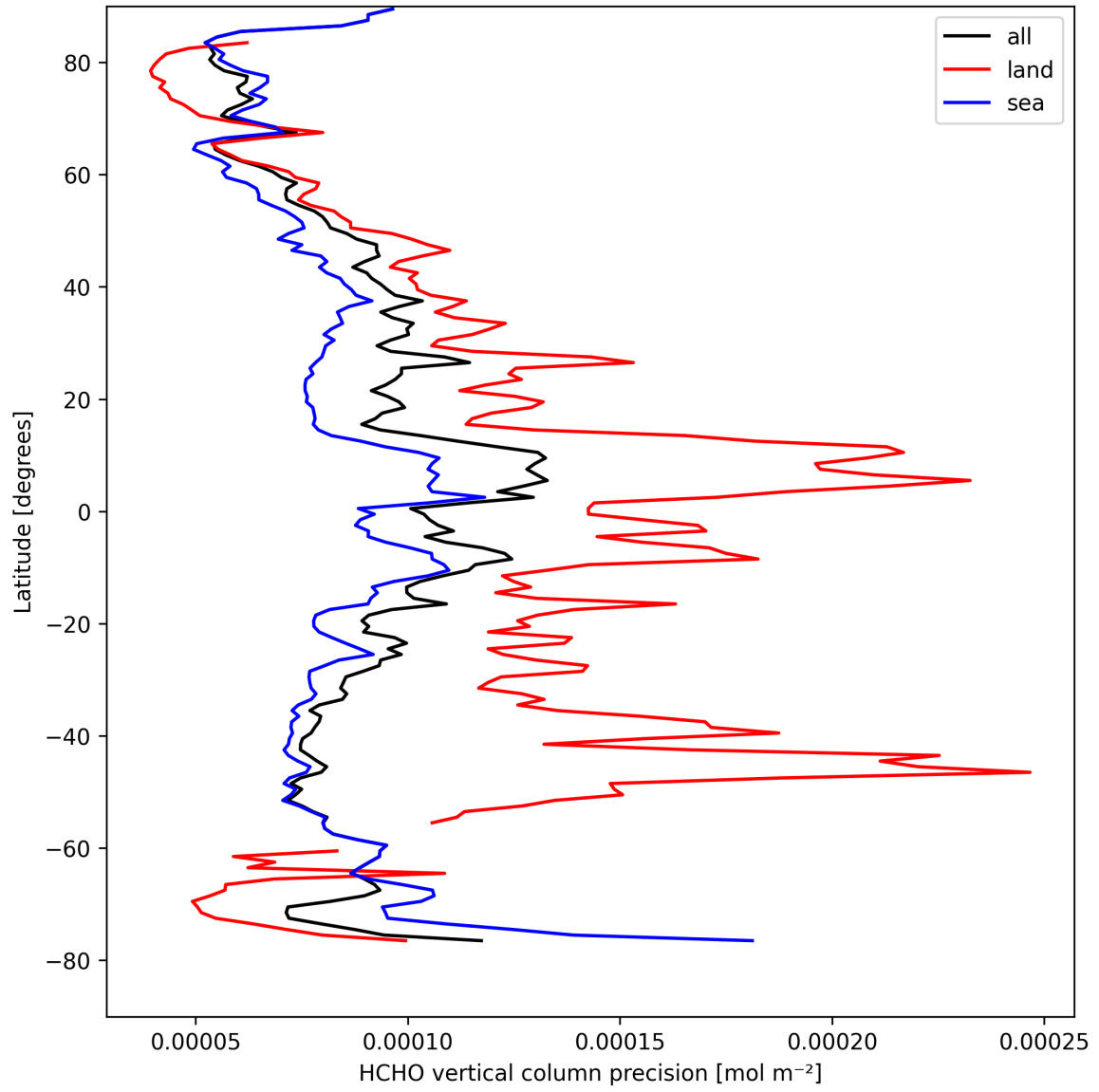
Figure 20: Zonal average of “HCHO vertical column precision” for 2025-04-10 to 2025-04-11.
