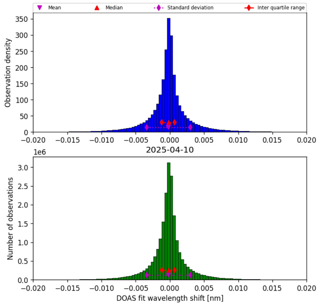
Figure 42: Histogram of “DOAS fit wavelength shift” for 2025-04-10 to 2025-04-11
