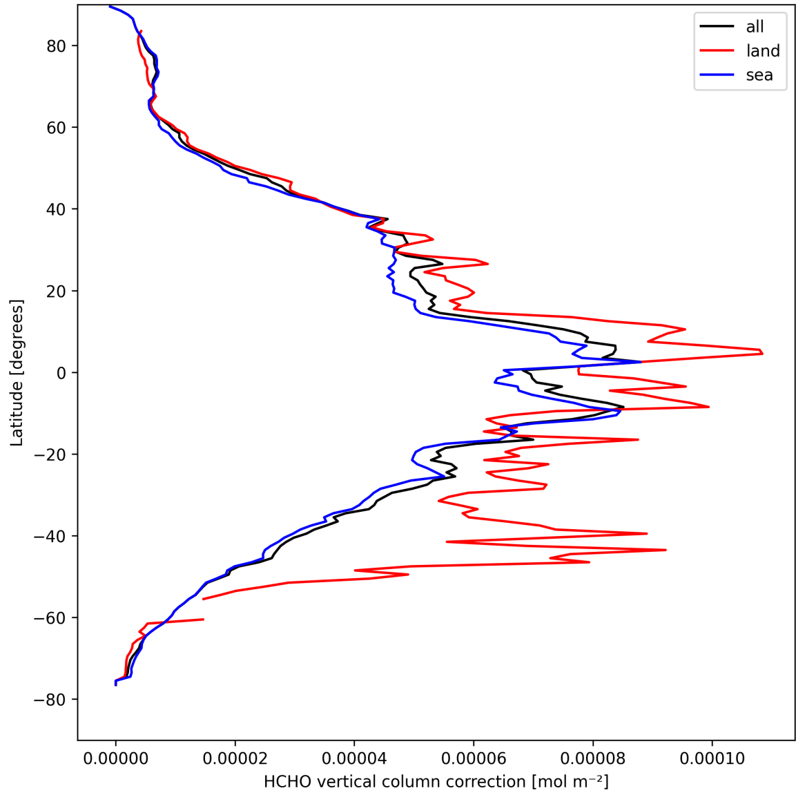
Figure 21: Zonal average of “HCHO vertical column correction” for 2025-04-10 to 2025-04-11.
