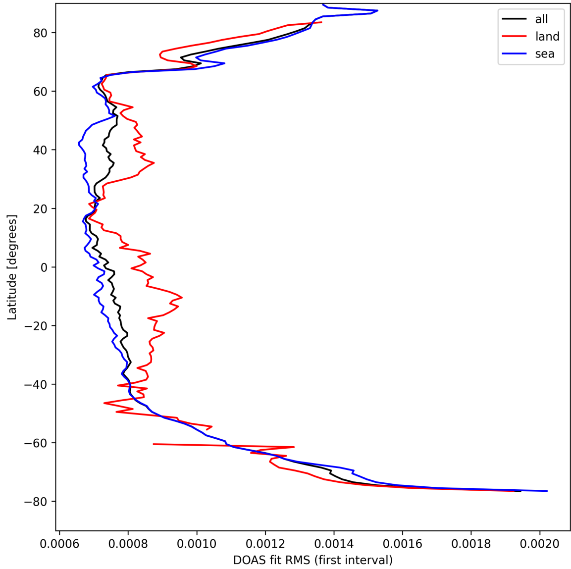
Figure 30: Zonal average of “DOAS fit RMS (first interval)” for 2025-04-10 to 2025-04-11.
