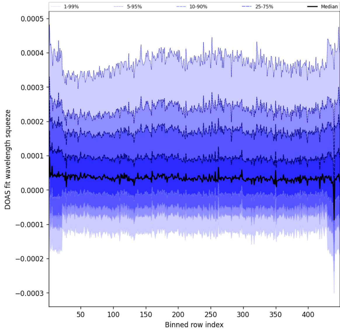
Figure 57: Along track statistics of “DOAS fit wavelength squeeze” for 2025-04-10 to 2025-04-11
