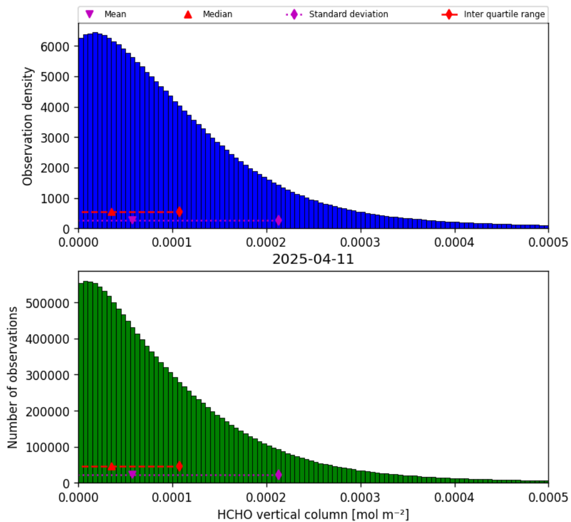
Figure 33: Histogram of “HCHO vertical column” for 2025-04-11 to 2025-04-11
