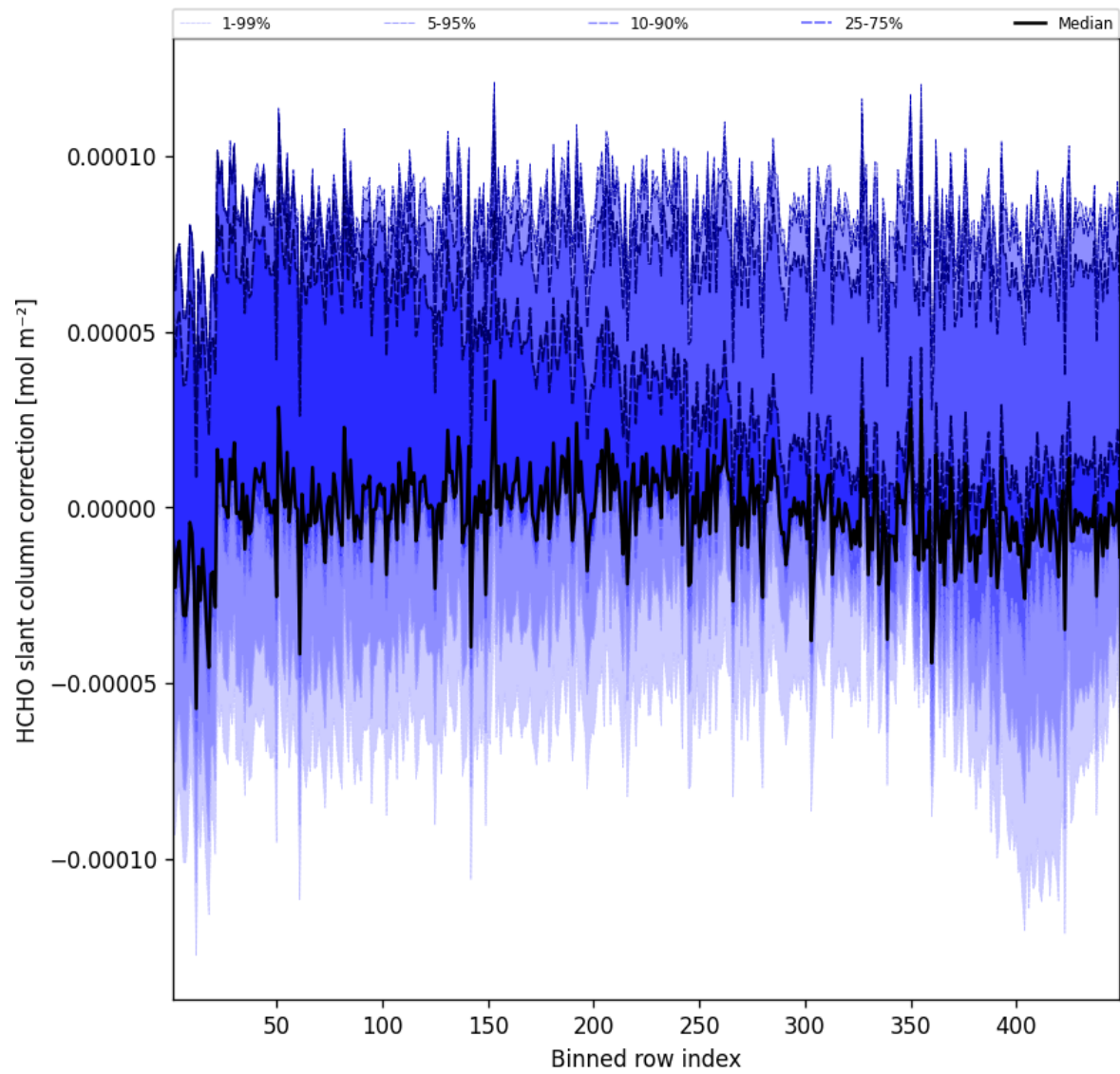
Figure 59: Along track statistics of “HCHO slant column correction” for 2025-04-11 to 2025-04-11
