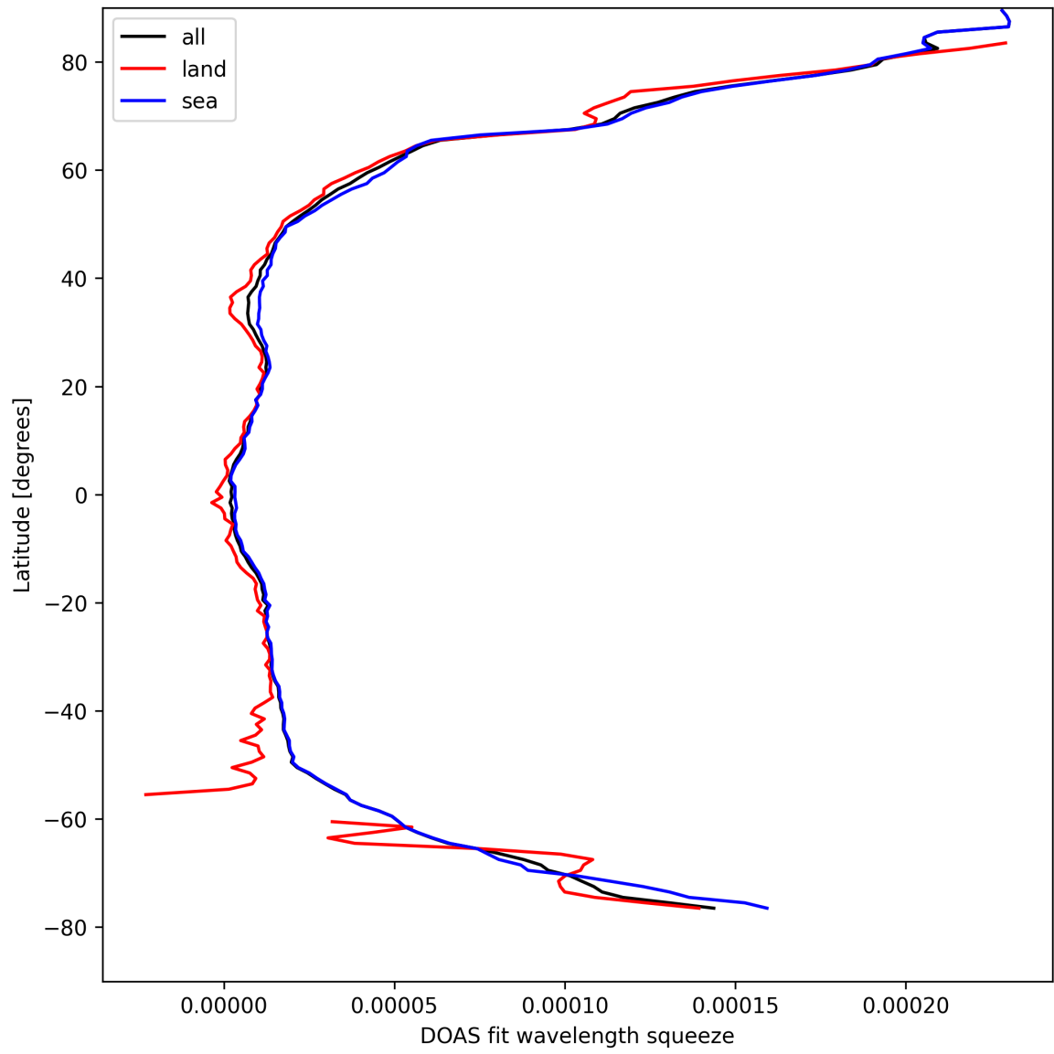
Figure 29: Zonal average of “DOAS fit wavelength squeeze” for 2025-04-11 to 2025-04-11.
