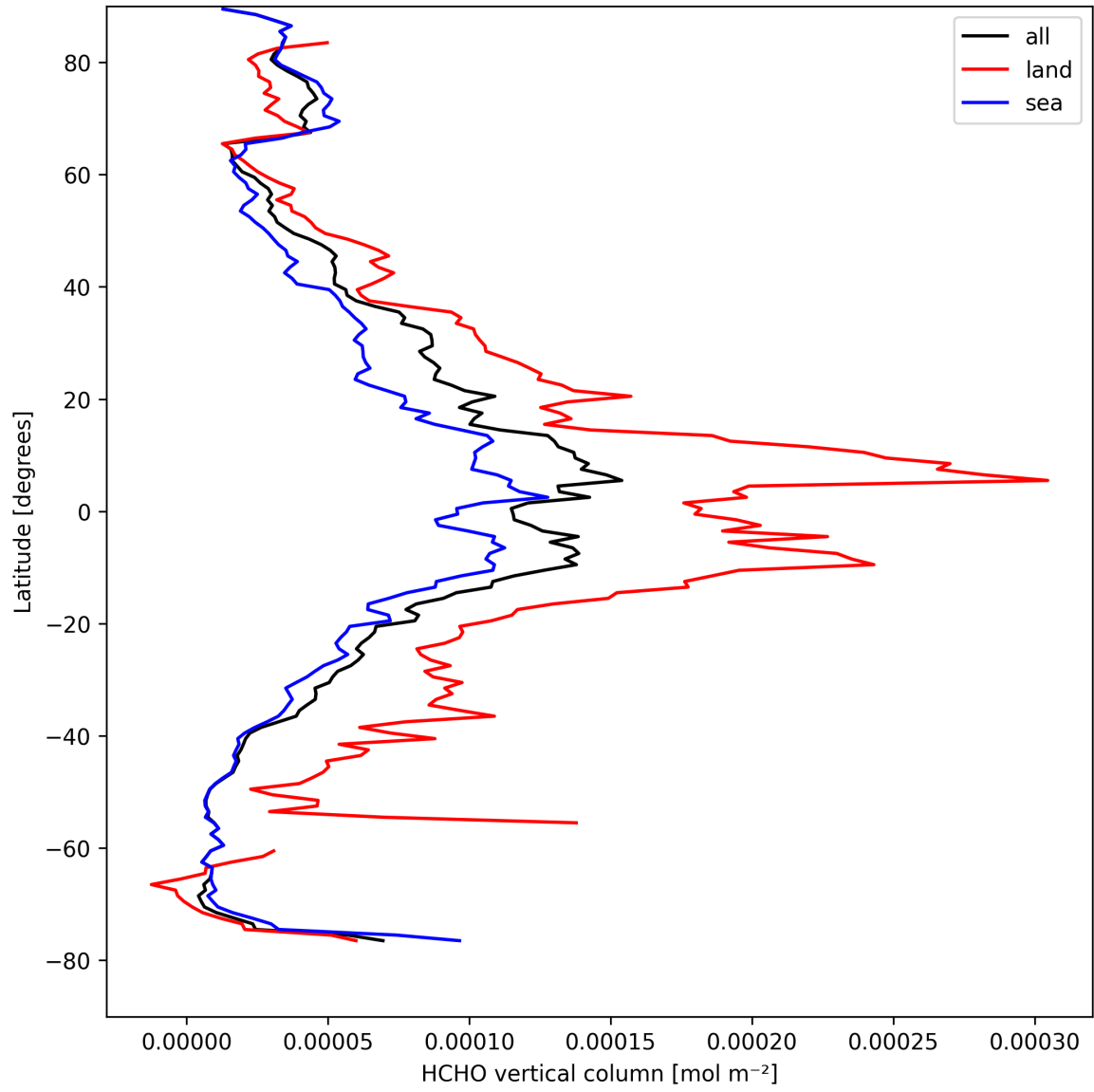
Figure 19: Zonal average of “HCHO vertical column” for 2025-04-11 to 2025-04-11.
