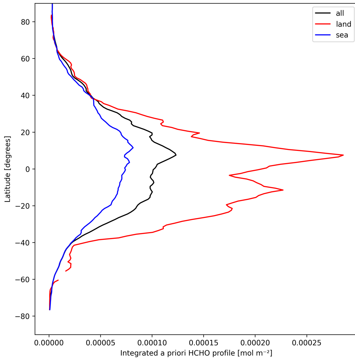
Figure 27: Zonal average of “Integrated a priori HCHO profile” for 2025-04-11 to 2025-04-11.
