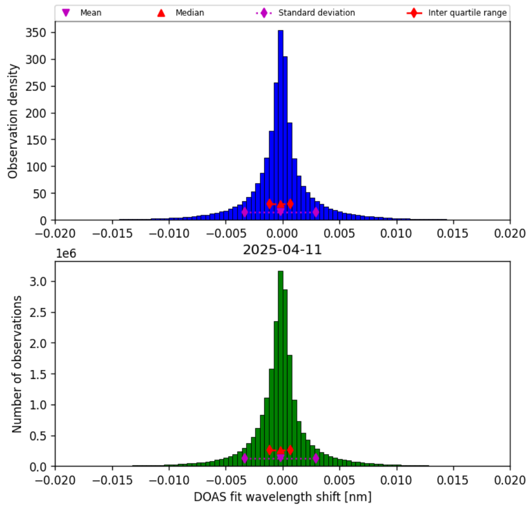
Figure 42: Histogram of “DOAS fit wavelength shift” for 2025-04-11 to 2025-04-11
