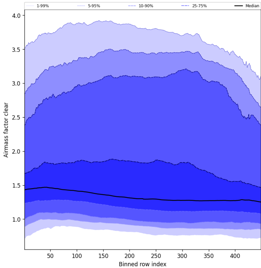
Figure 54: Along track statistics of “Airmass factor clear” for 2025-04-11 to 2025-04-11
