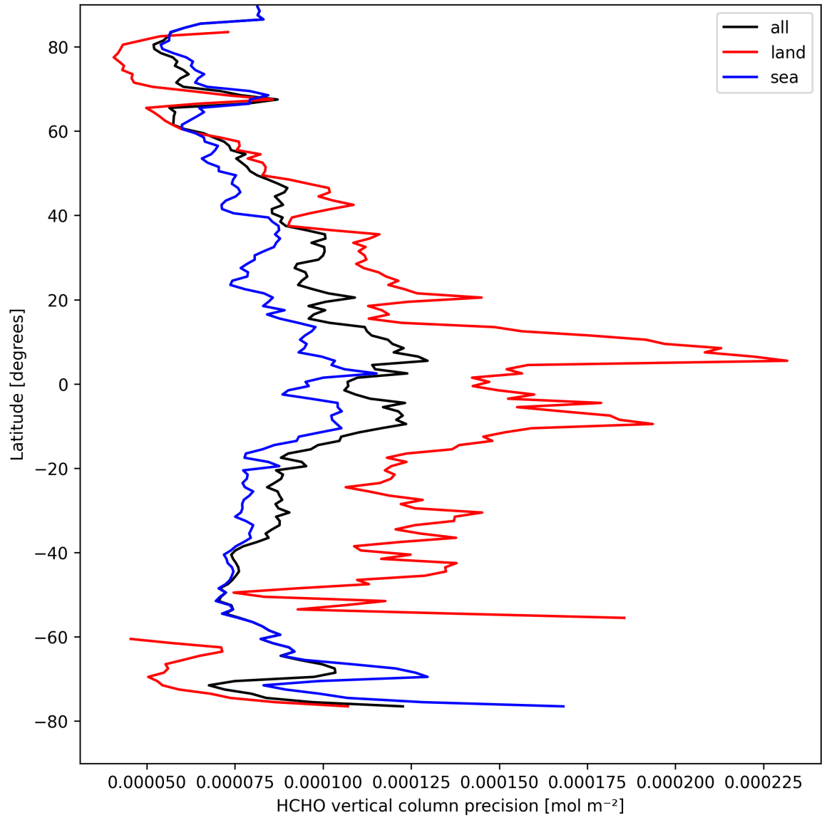
Figure 20: Zonal average of “HCHO vertical column precision” for 2025-04-11 to 2025-04-11.
