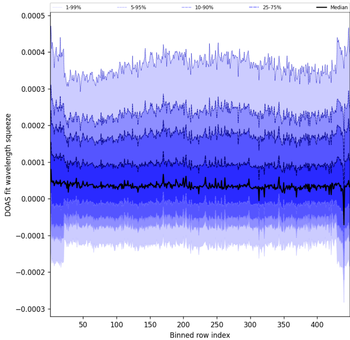
Figure 57: Along track statistics of “DOAS fit wavelength squeeze” for 2025-04-11 to 2025-04-11
