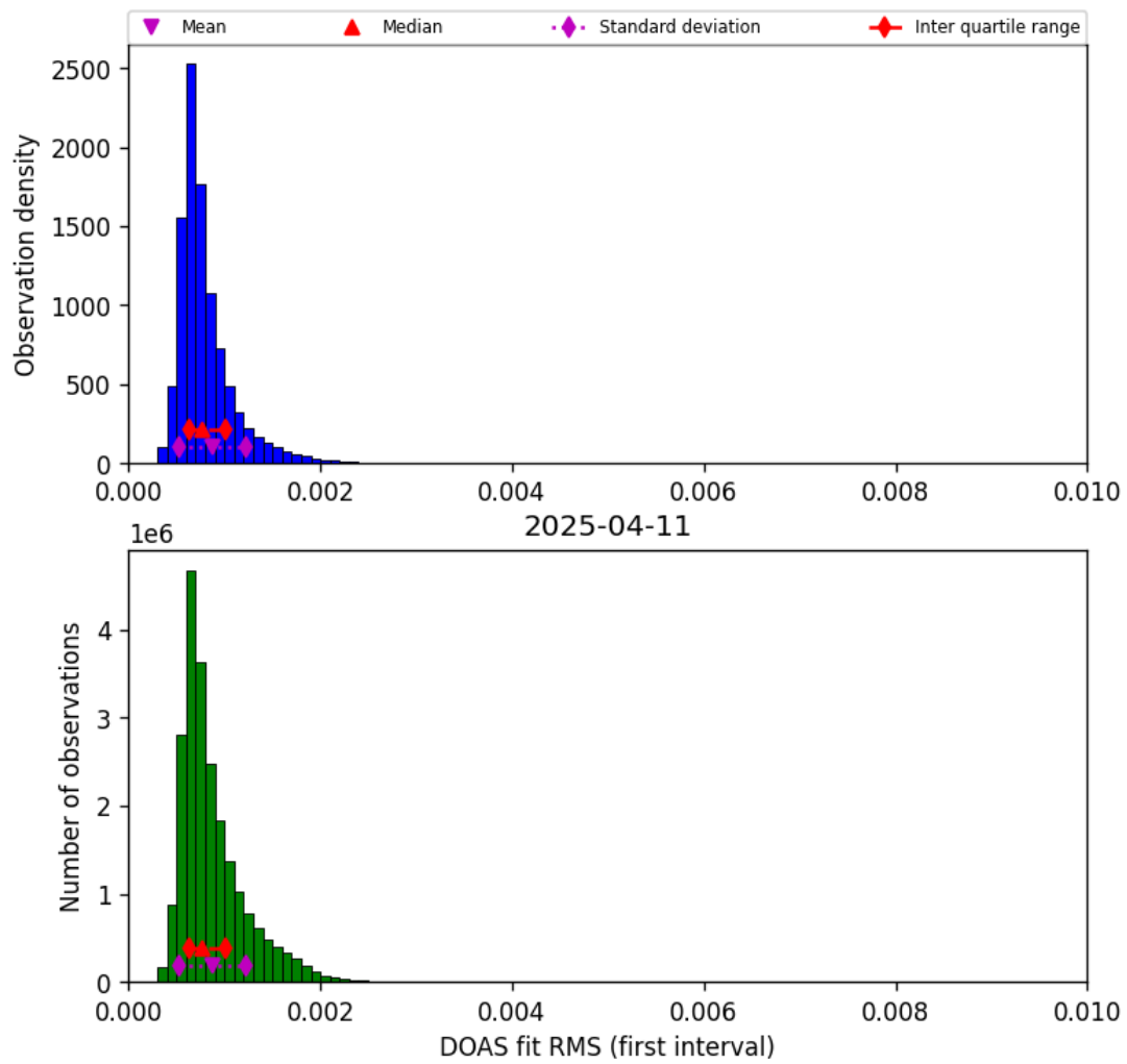
Figure 44: Histogram of “DOAS fit RMS (first interval)” for 2025-04-11 to 2025-04-11
