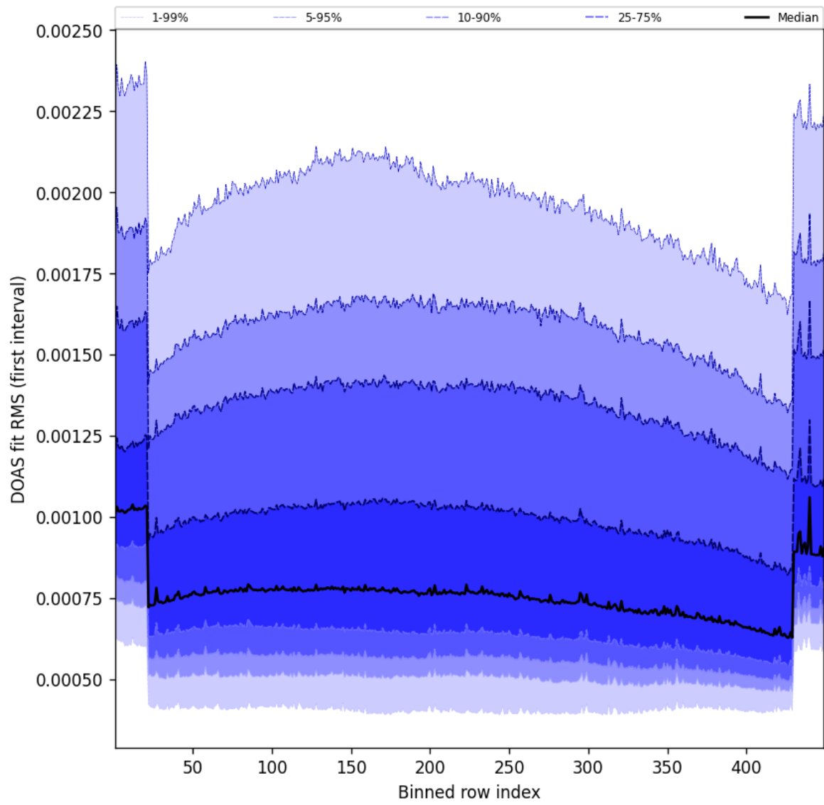
Figure 58: Along track statistics of “DOAS fit RMS (first interval)” for 2025-04-11 to 2025-04-11
