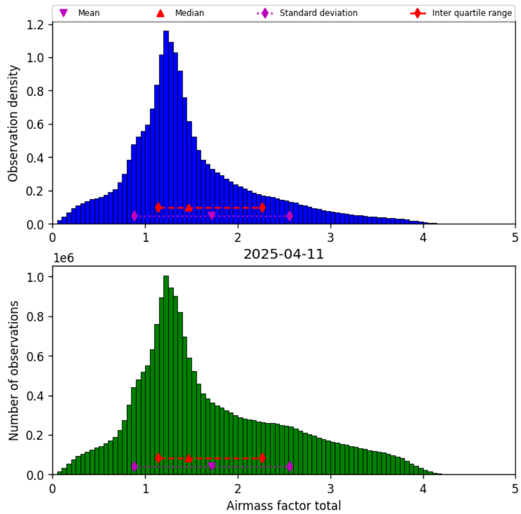
Figure 38: Histogram of “Airmass factor total” for 2025-04-11 to 2025-04-11
