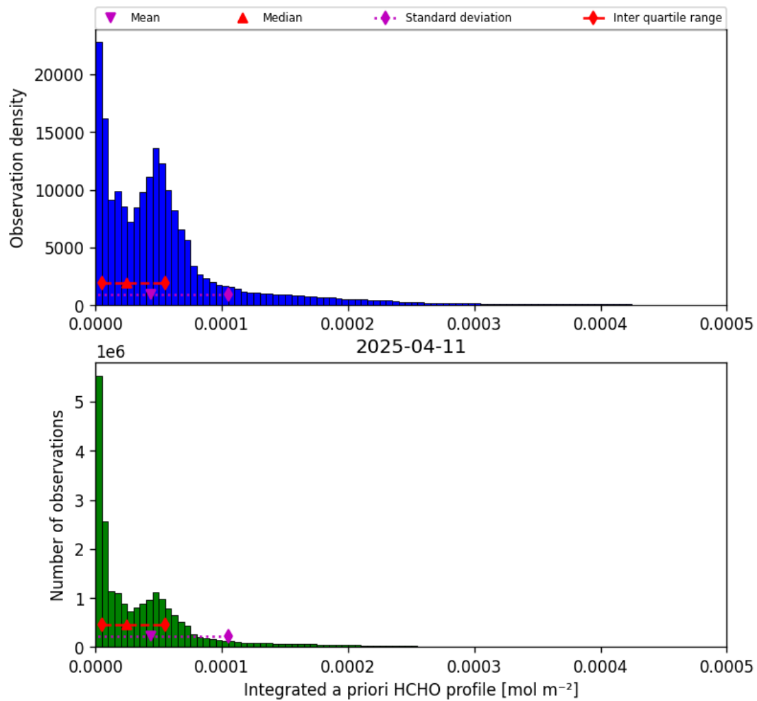
Figure 41: Histogram of “Integrated a priori HCHO profile” for 2025-04-11 to 2025-04-11
