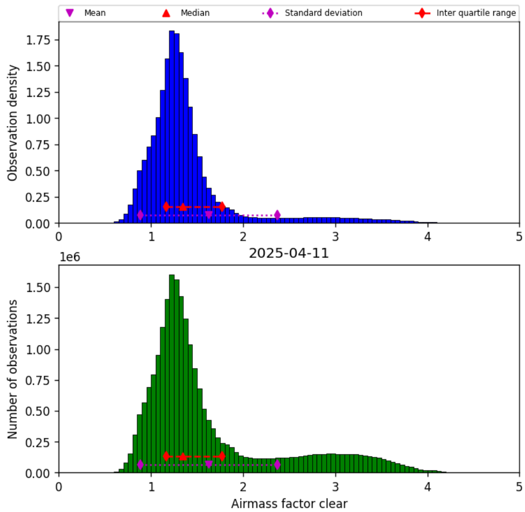
Figure 40: Histogram of “Airmass factor clear” for 2025-04-11 to 2025-04-11
