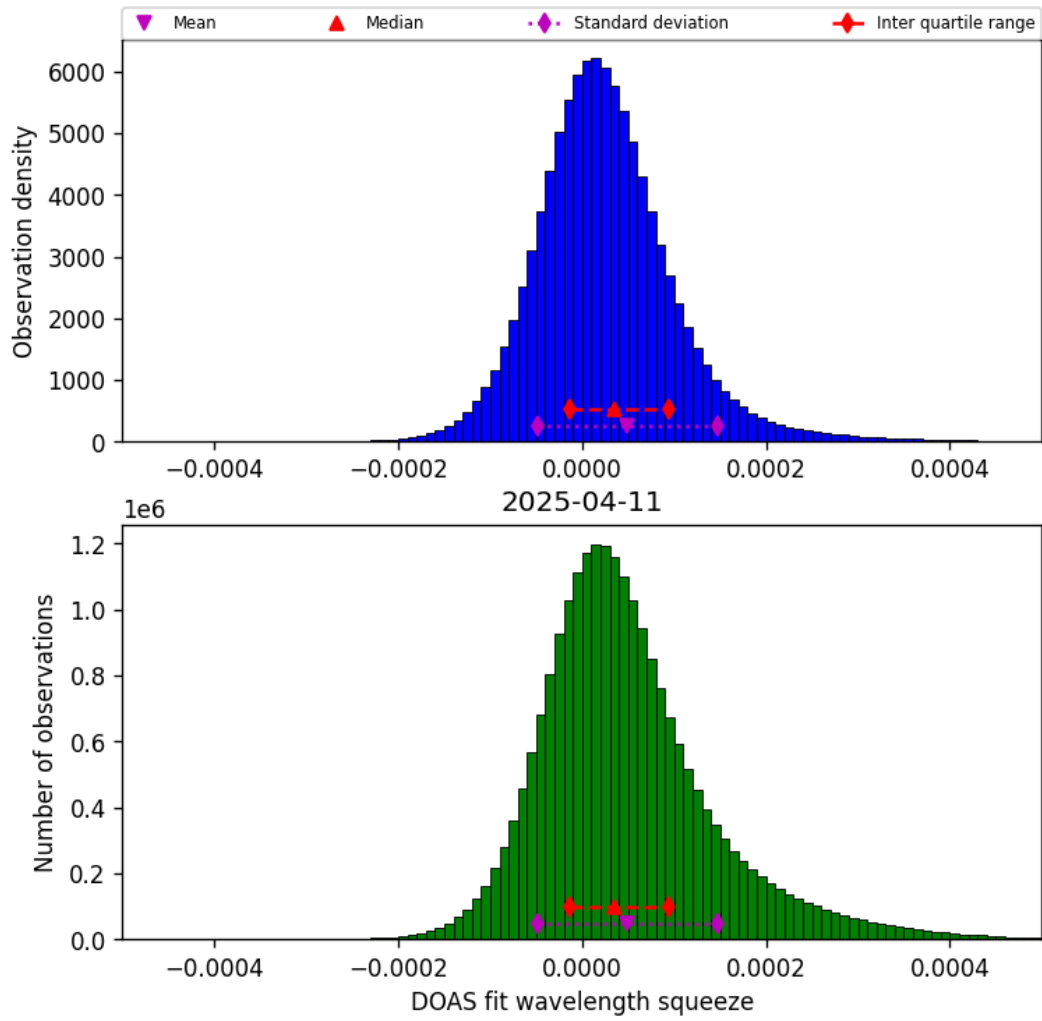
Figure 43: Histogram of “DOAS fit wavelength squeeze” for 2025-04-11 to 2025-04-11
