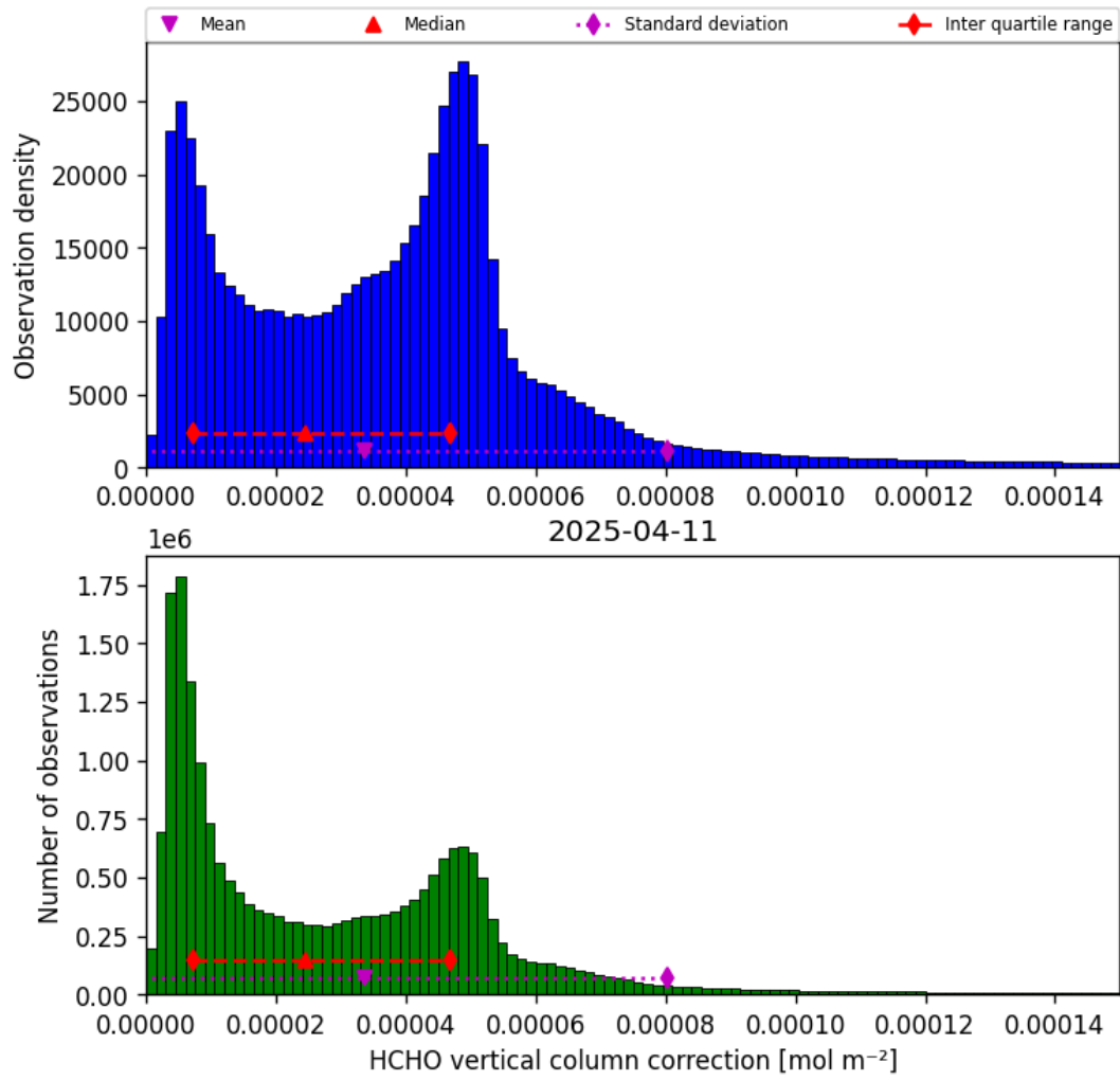
Figure 35: Histogram of “HCHO vertical column correction” for 2025-04-11 to 2025-04-11
