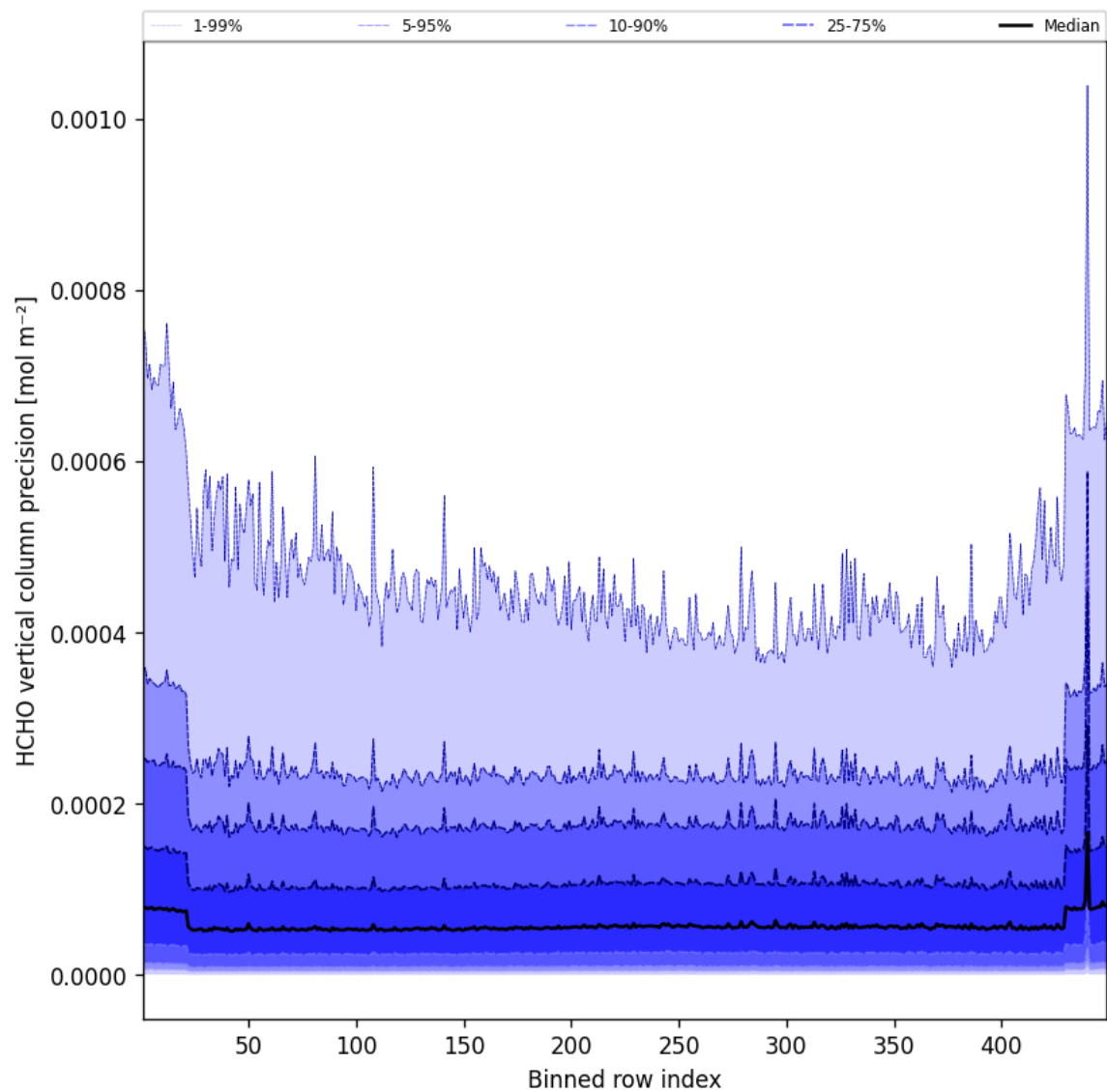
Figure 48: Along track statistics of “HCHO vertical column precision” for 2025-04-11 to 2025-04-11
