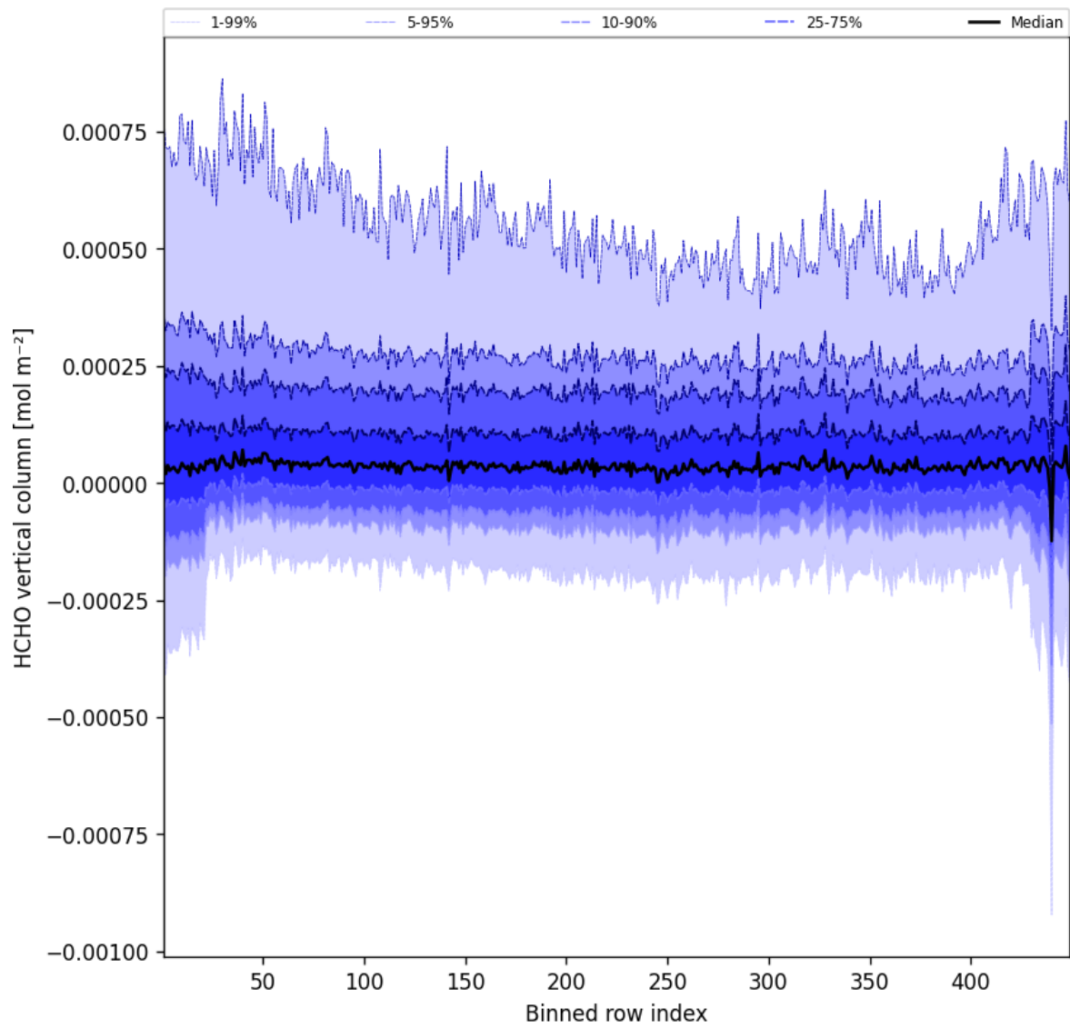
Figure 47: Along track statistics of “HCHO vertical column” for 2025-04-11 to 2025-04-11
