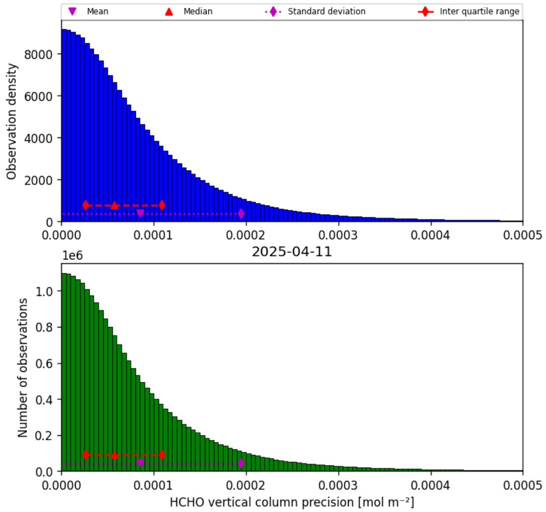
Figure 34: Histogram of “HCHO vertical column precision” for 2025-04-11 to 2025-04-11
