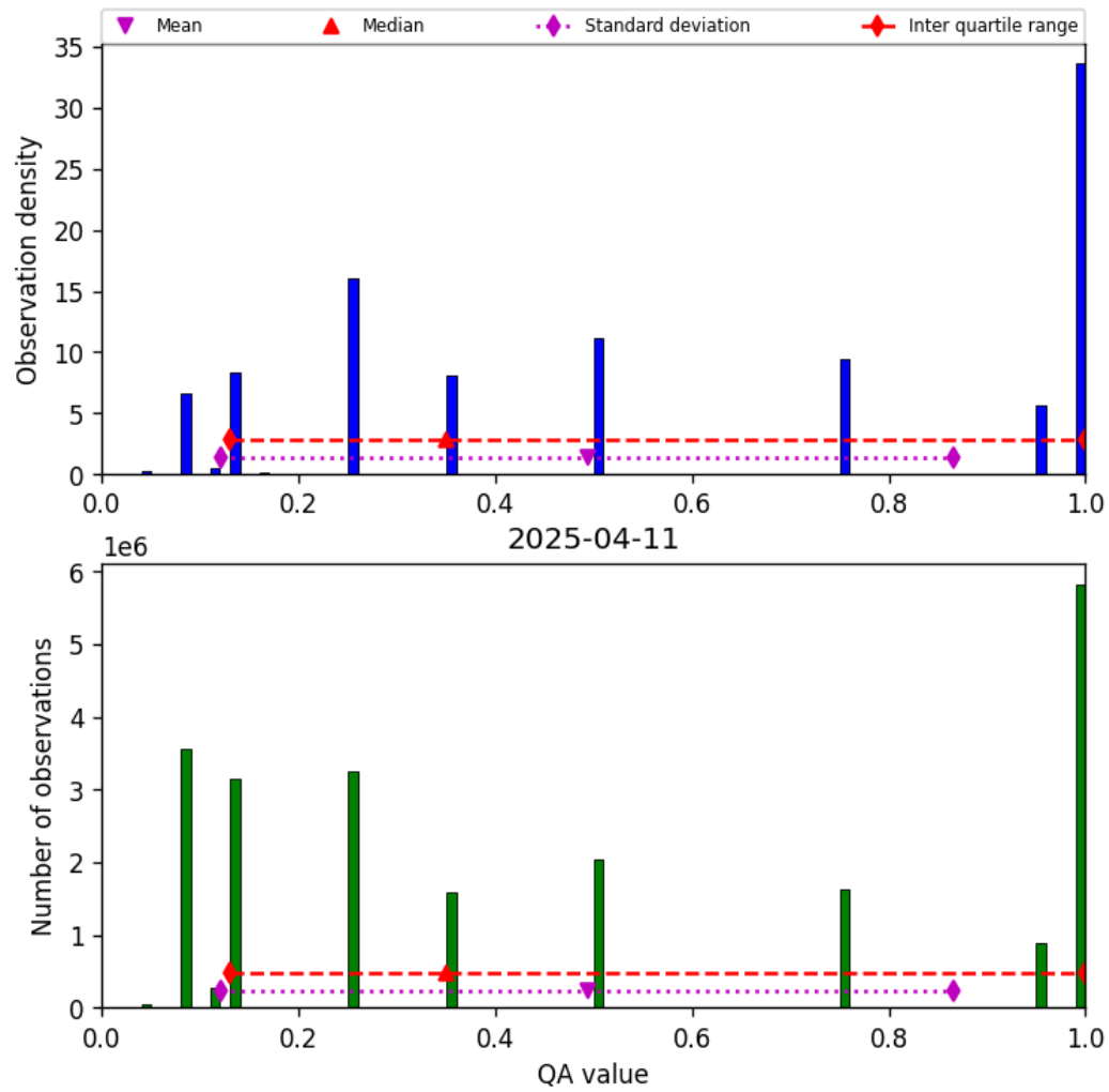
Figure 32: Histogram of “QA value” for 2025-04-11 to 2025-04-11
