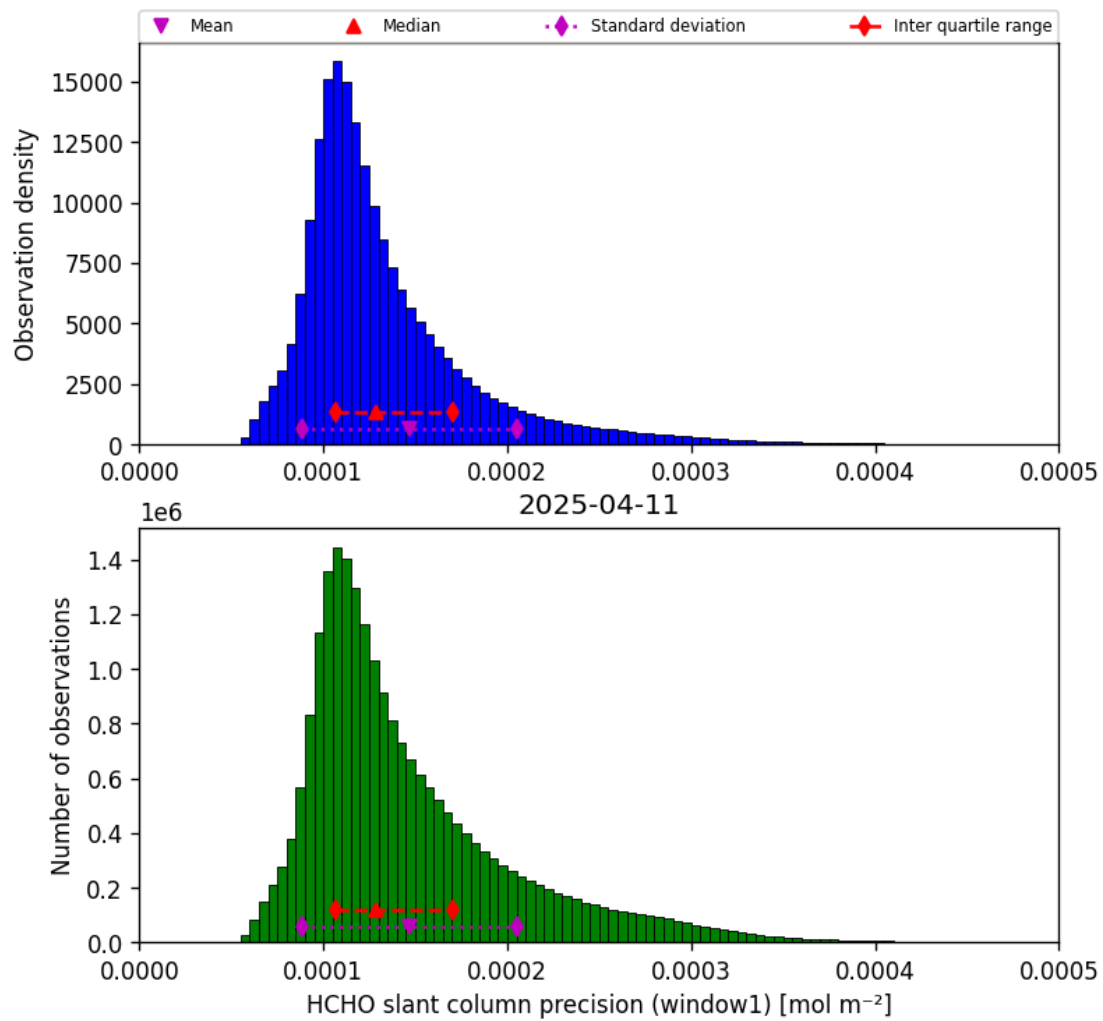
Figure 37: Histogram of “HCHO slant column precision (window1)” for 2025-04-11 to 2025-04-11
