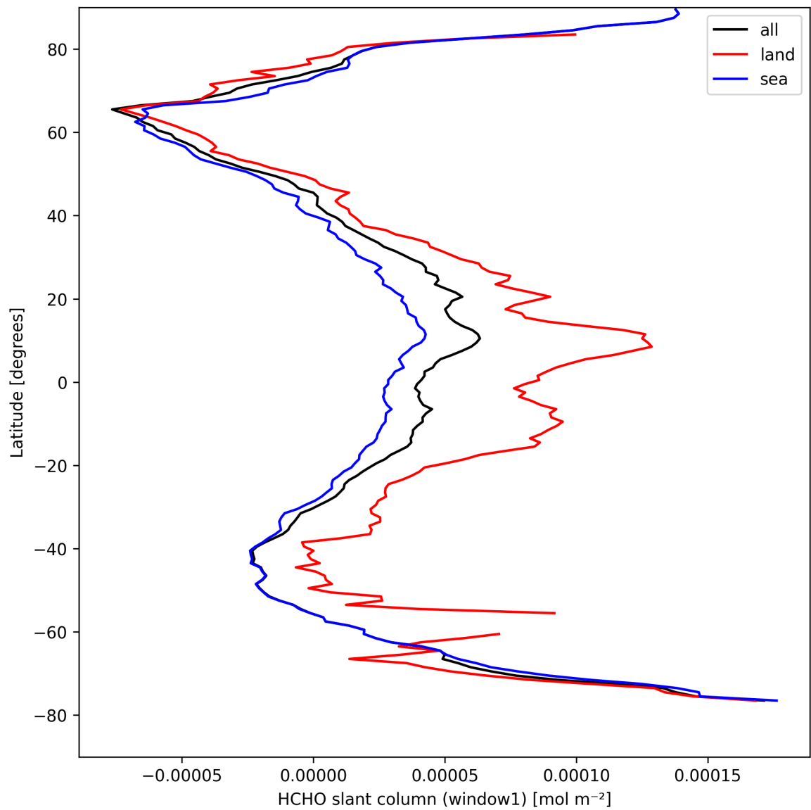
Figure 22: Zonal average of “HCHO slant column (window1)” for 2025-04-11 to 2025-04-11.
