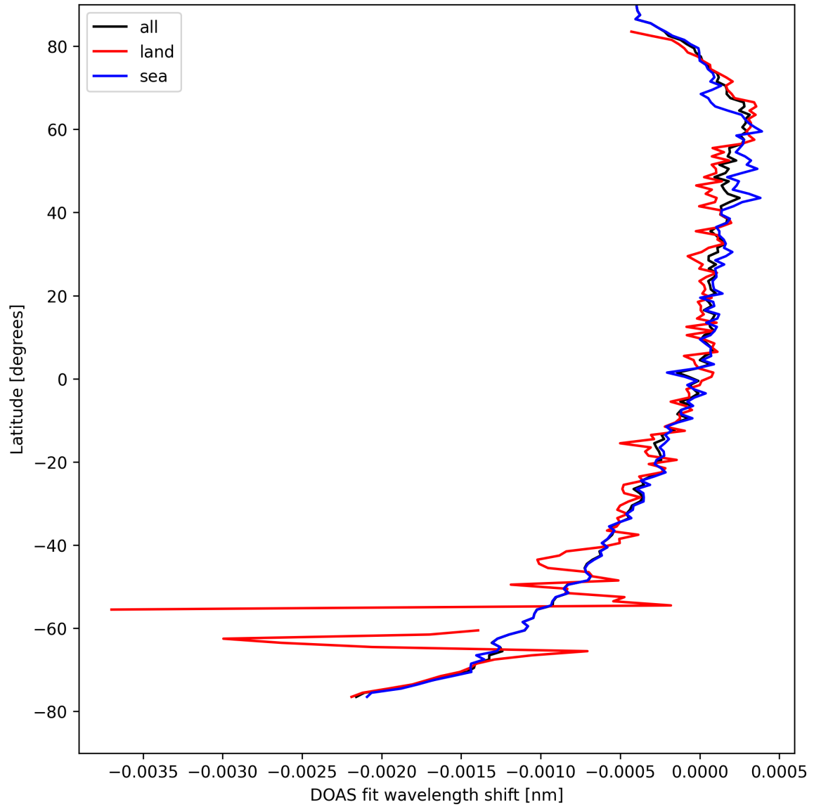
Figure 28: Zonal average of “DOAS fit wavelength shift” for 2025-04-11 to 2025-04-11.
