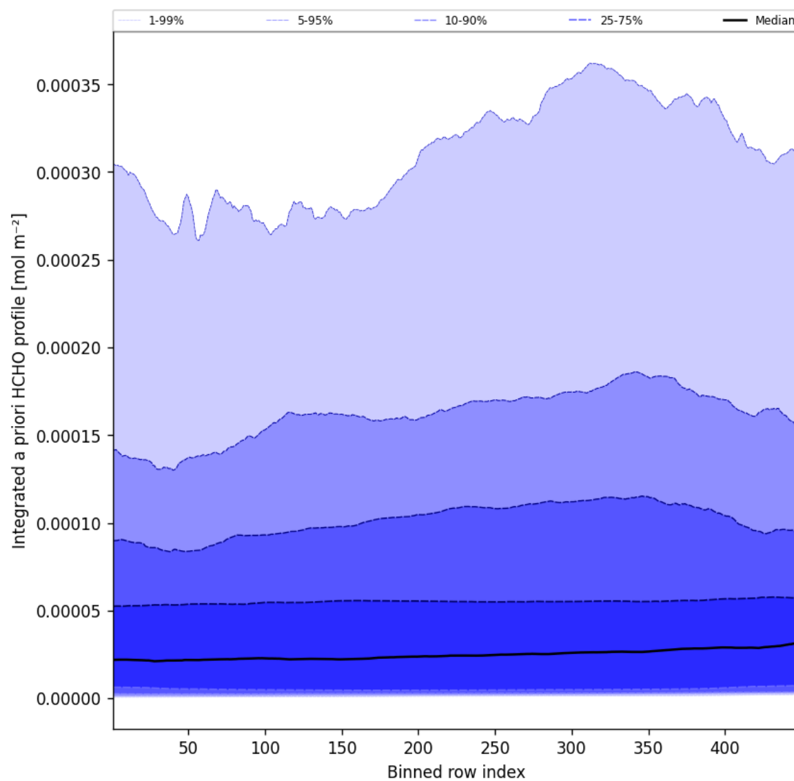
Figure 55: Along track statistics of “Integrated a priori HCHO profile” for 2025-04-11 to 2025-04-11
