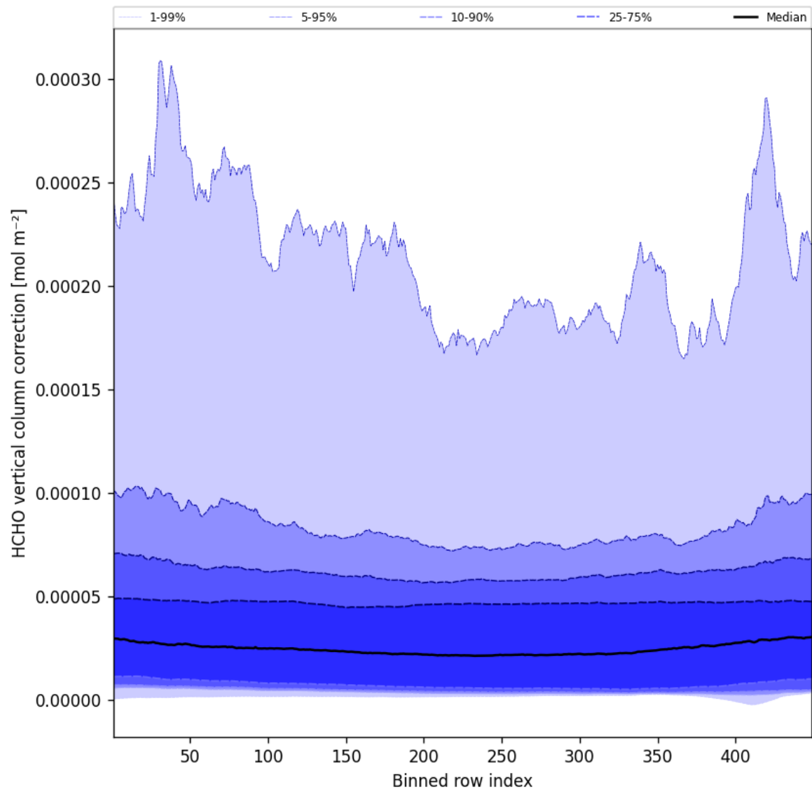
Figure 49: Along track statistics of “HCHO vertical column correction” for 2025-04-11 to 2025-04-11
