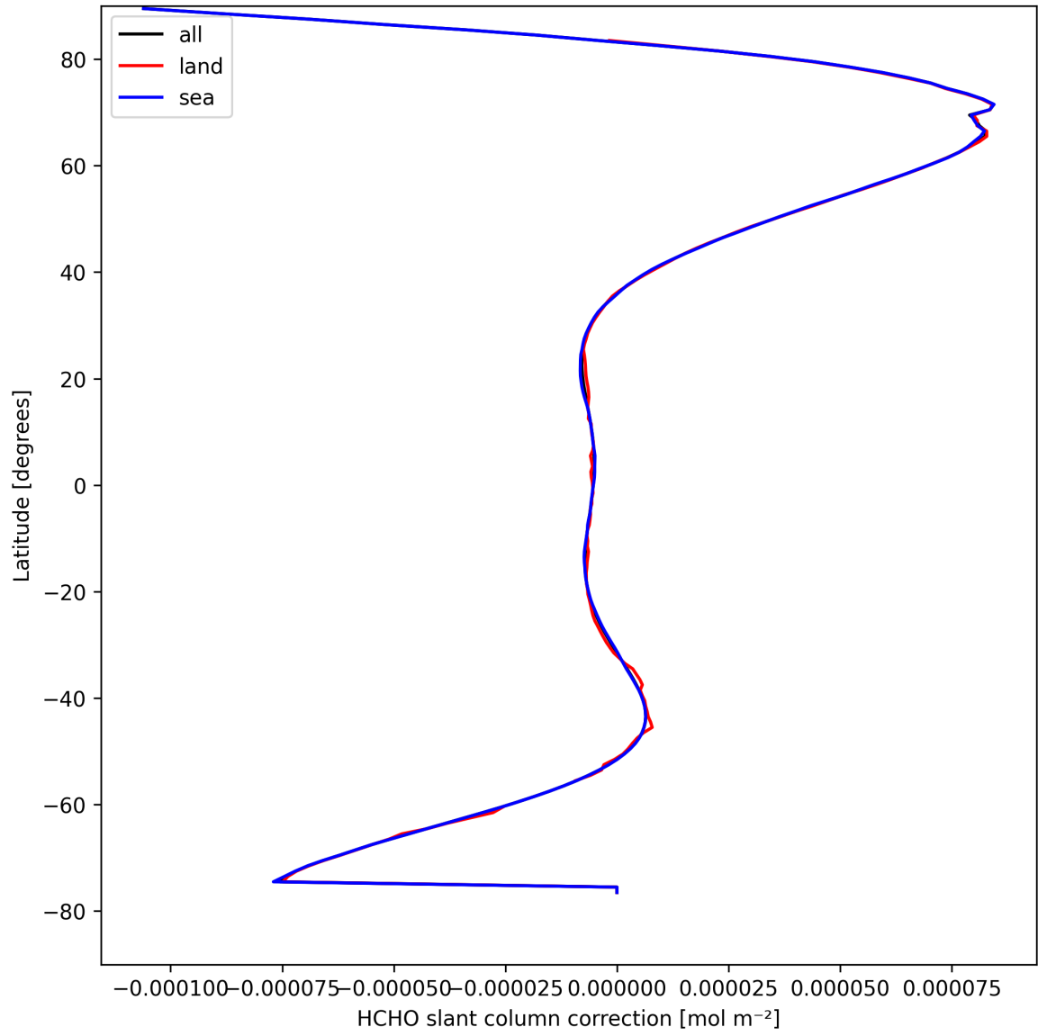
Figure 31: Zonal average of “HCHO slant column correction” for 2025-04-11 to 2025-04-11.
