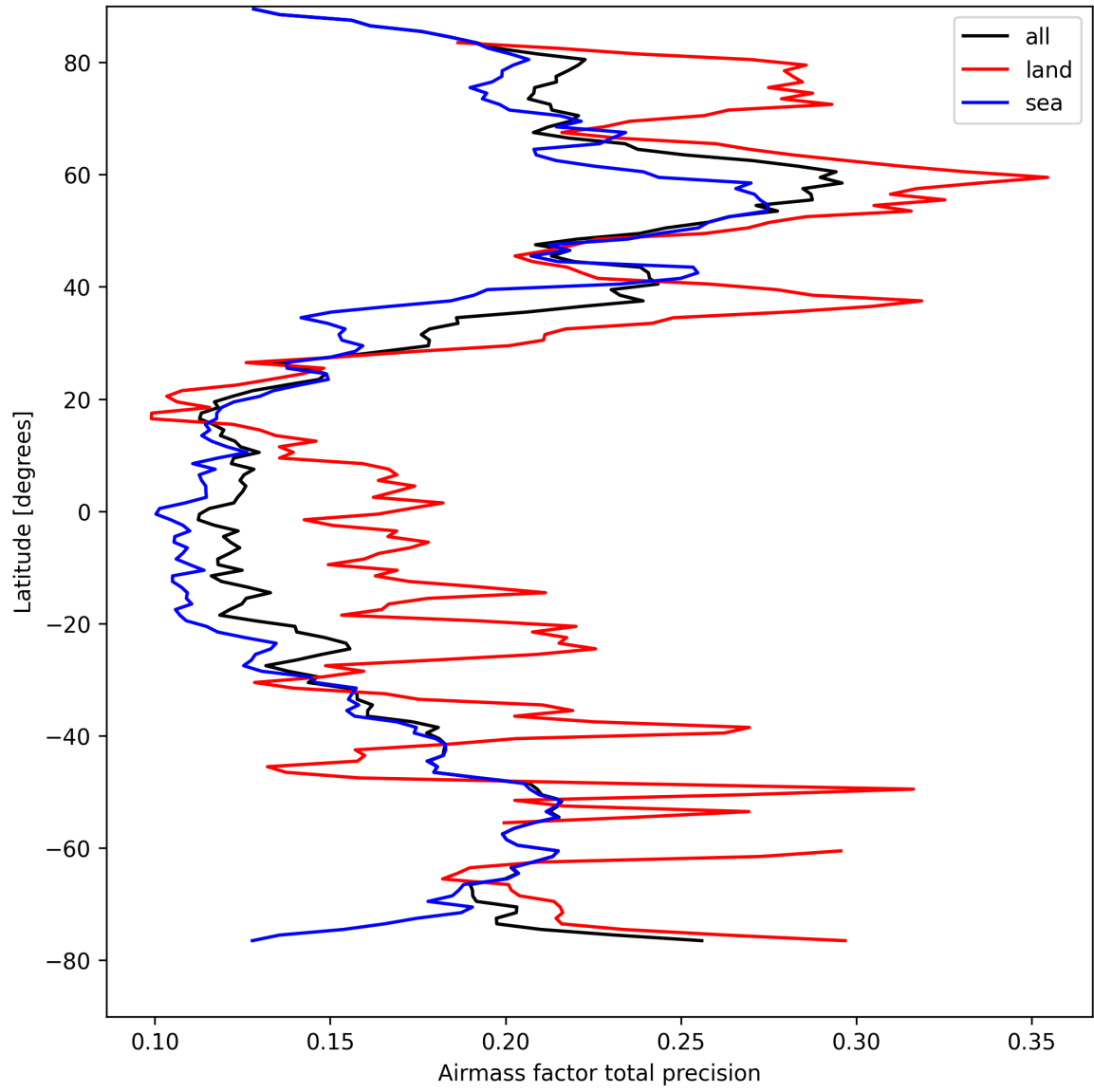
Figure 25: Zonal average of “Airmass factor total precision” for 2025-04-11 to 2025-04-11.
