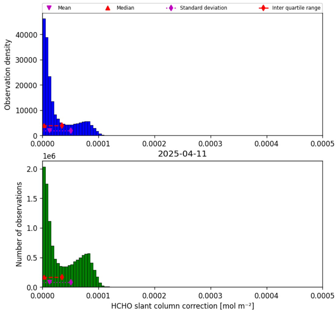
Figure 45: Histogram of “HCHO slant column correction” for 2025-04-11 to 2025-04-11
