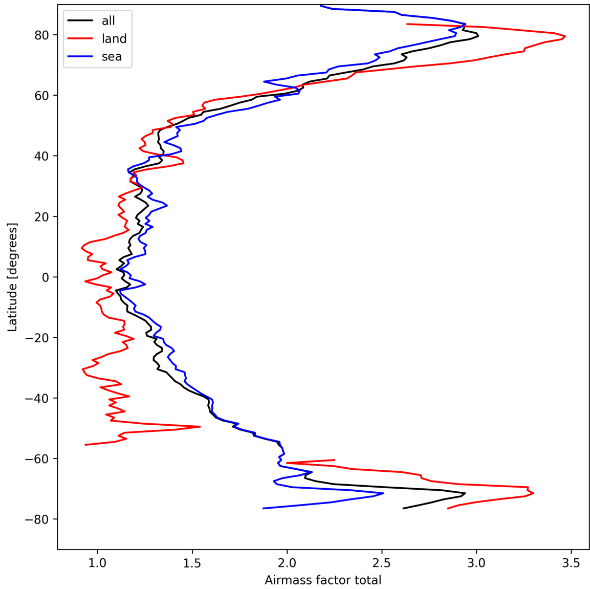
Figure 24: Zonal average of “Airmass factor total” for 2025-04-11 to 2025-04-11.
