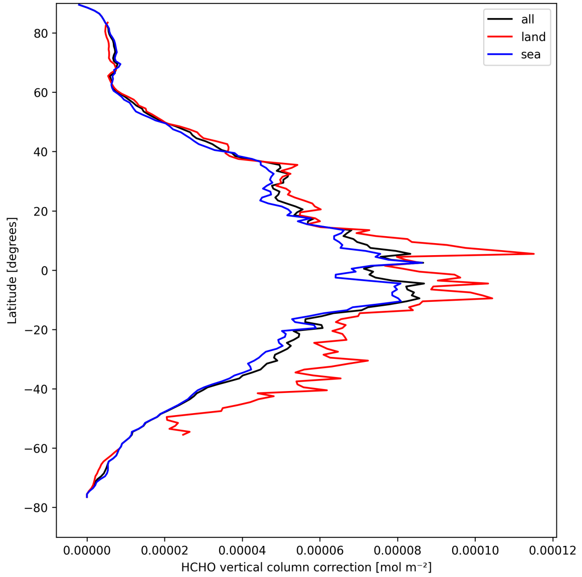
Figure 21: Zonal average of “HCHO vertical column correction” for 2025-04-11 to 2025-04-11.
