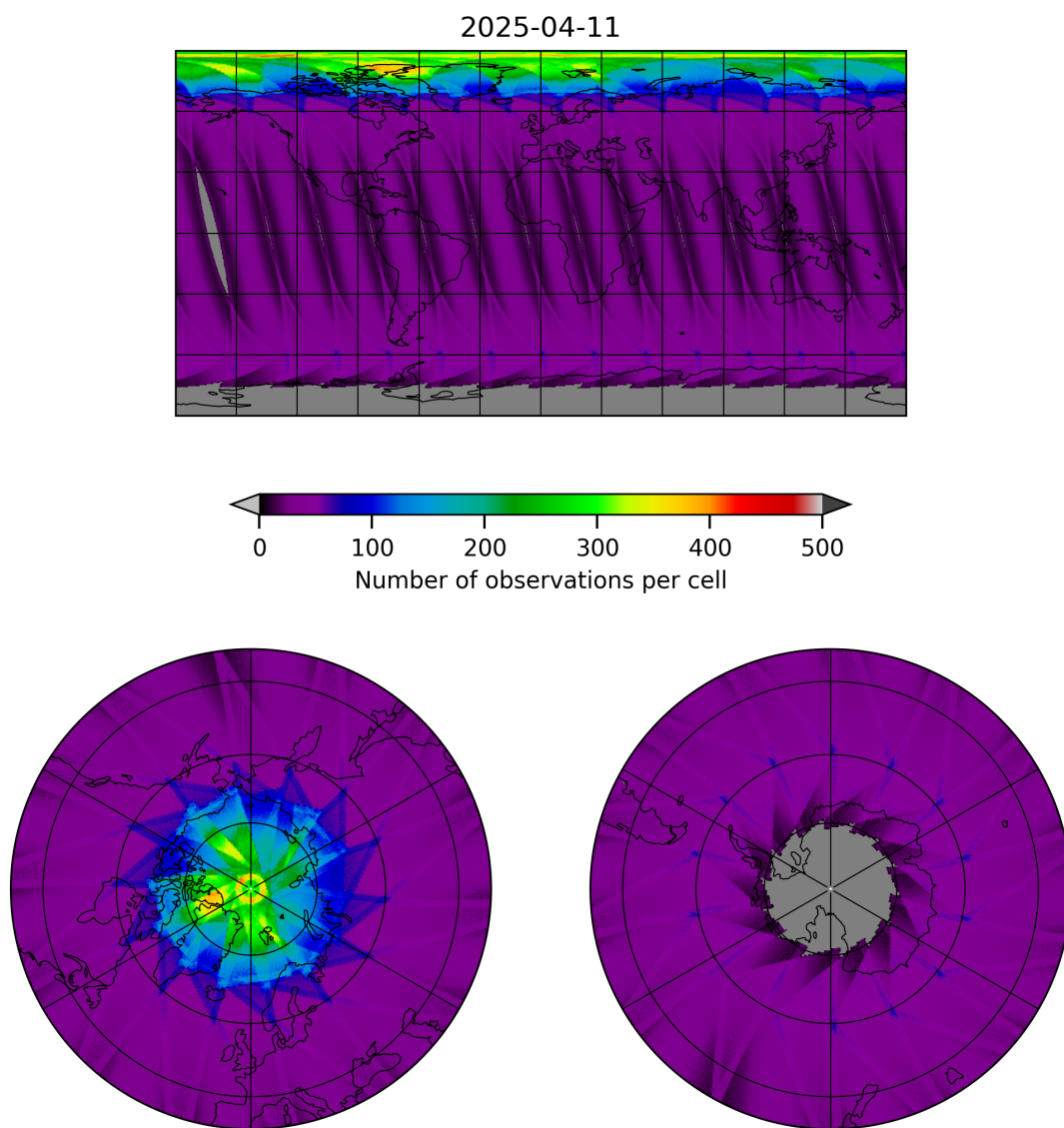
Figure 17: Map of the number of observations for 2025-04-11 to 2025-04-11
