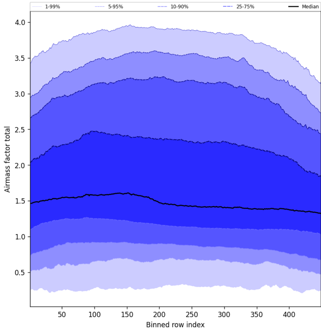
Figure 52: Along track statistics of “Airmass factor total” for 2025-04-11 to 2025-04-11
