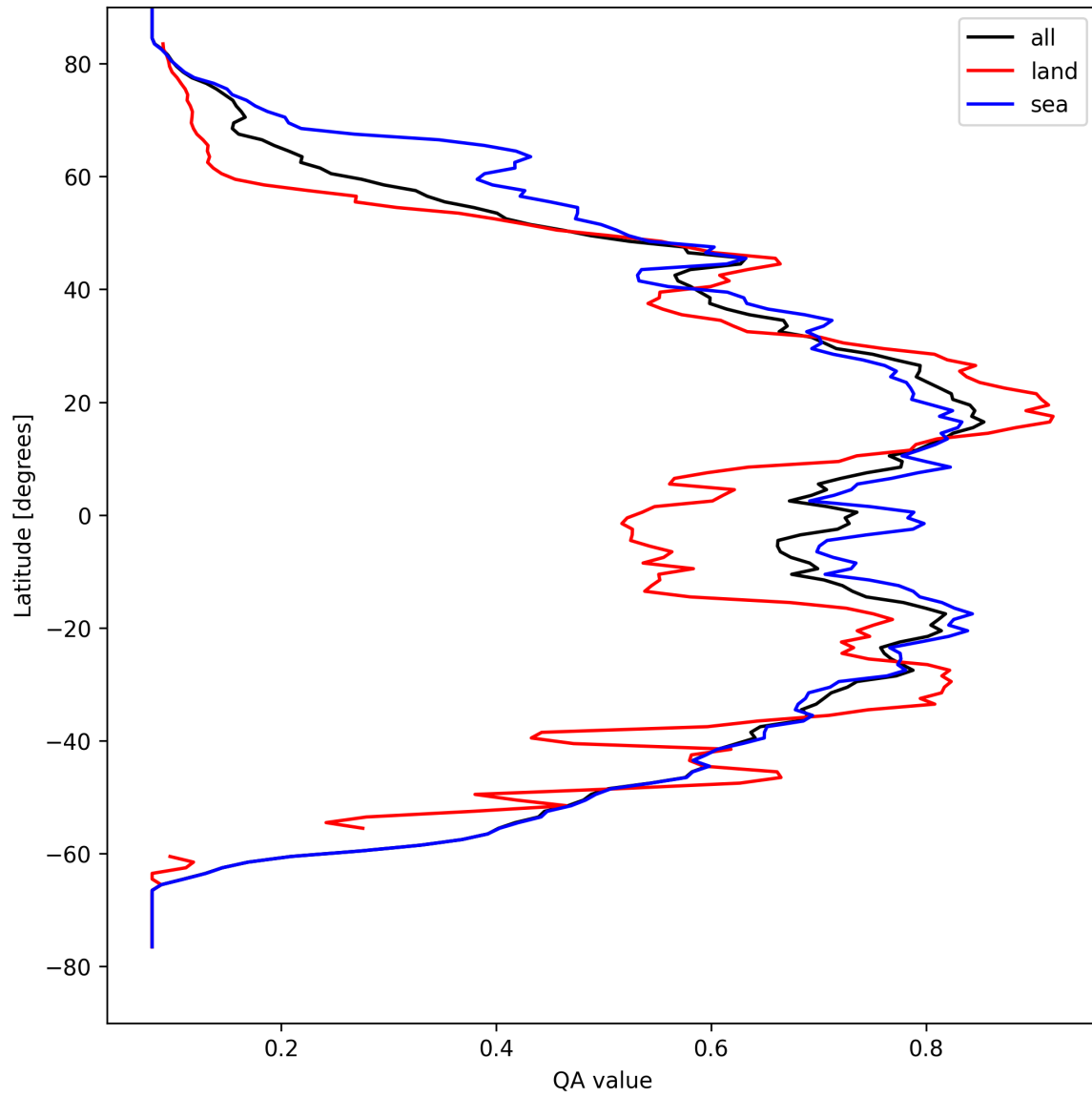
Figure 18: Zonal average of “QA value” for 2025-04-11 to 2025-04-11.
