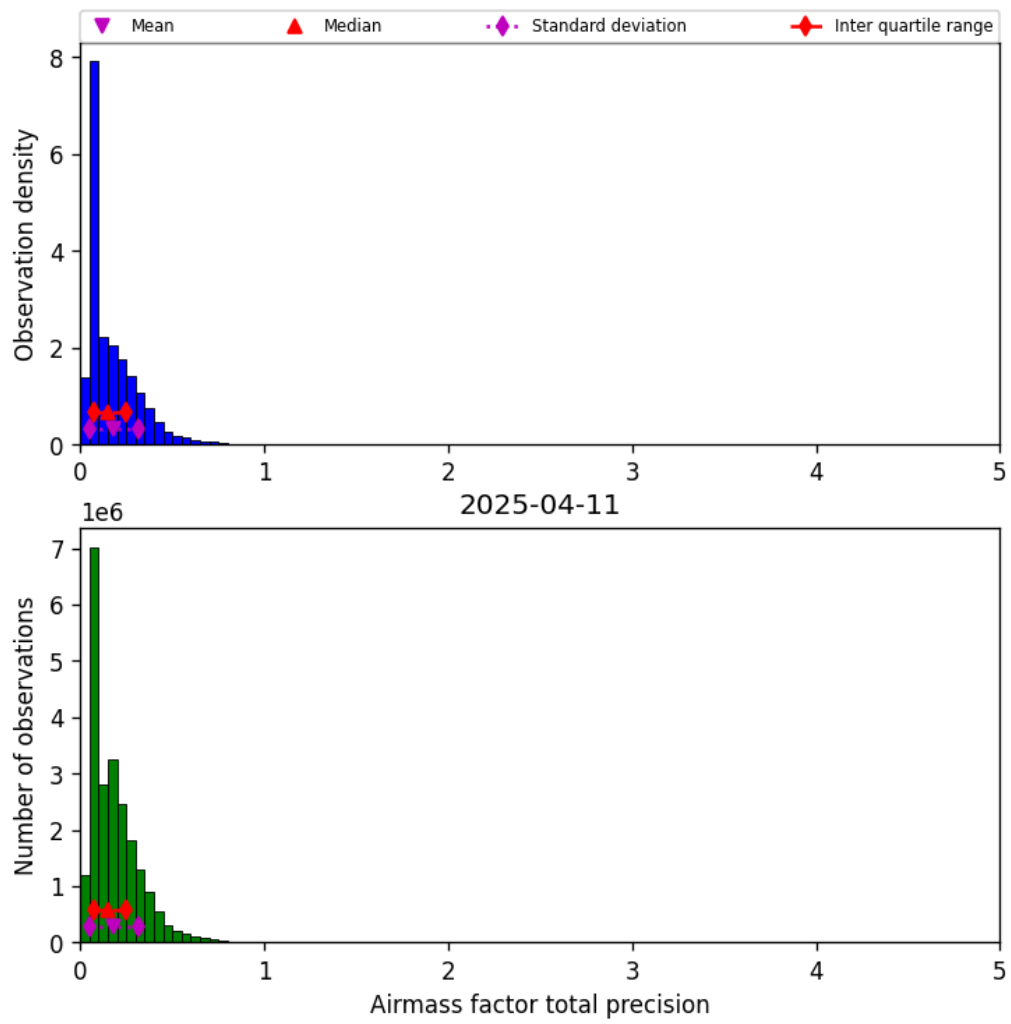
Figure 39: Histogram of “Airmass factor total precision” for 2025-04-11 to 2025-04-11
