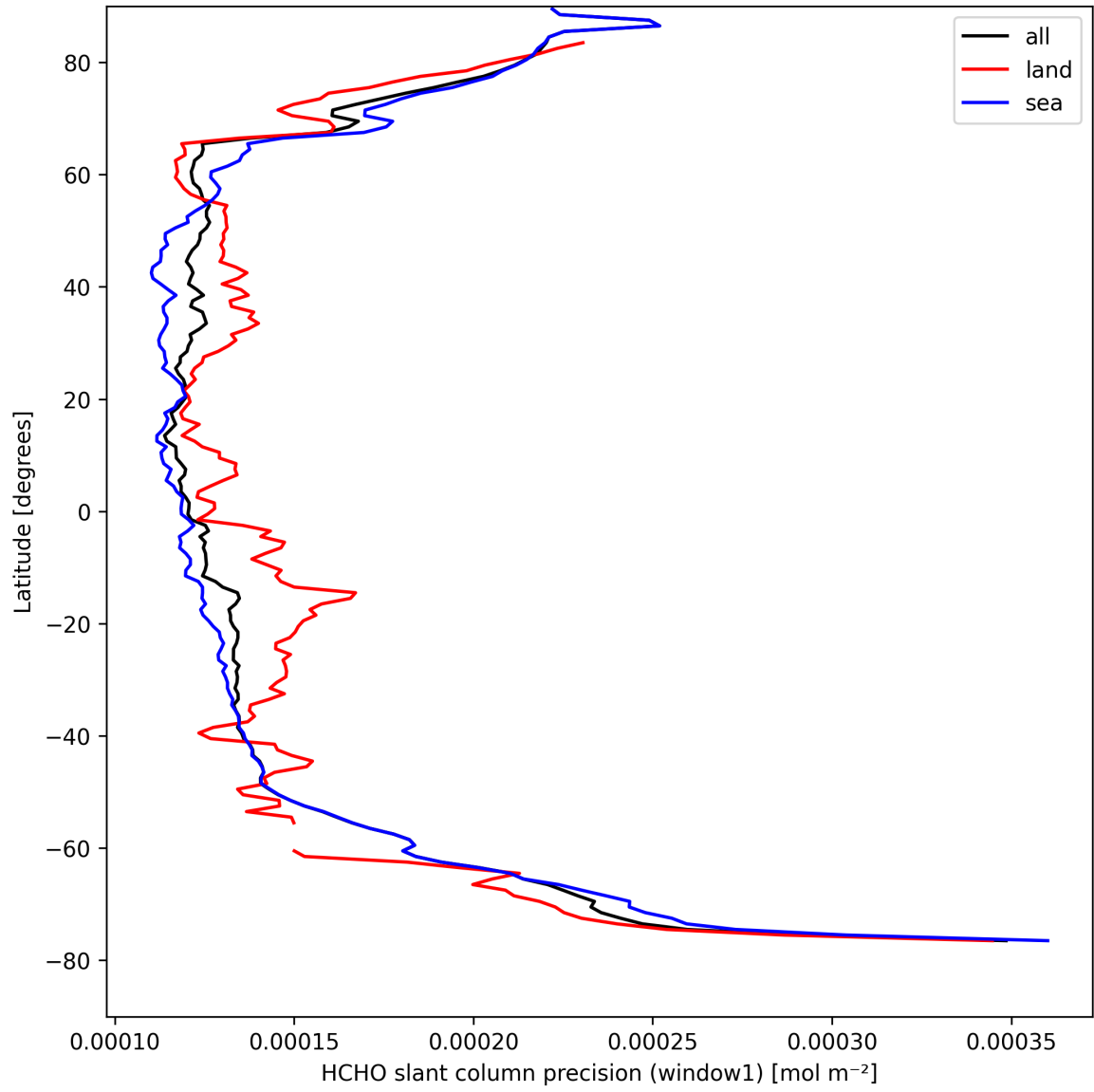
Figure 23: Zonal average of "HCHO slant column precision (window1)" for 2025-04-11 to 2025-04-11.
