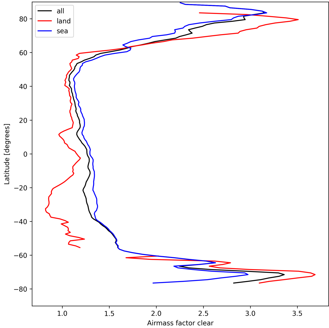
Figure 26: Zonal average of “Airmass factor clear” for 2025-04-11 to 2025-04-11.
