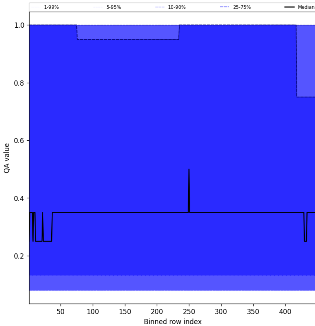
Figure 46: Along track statistics of “QA value” for 2025-04-11 to 2025-04-11
