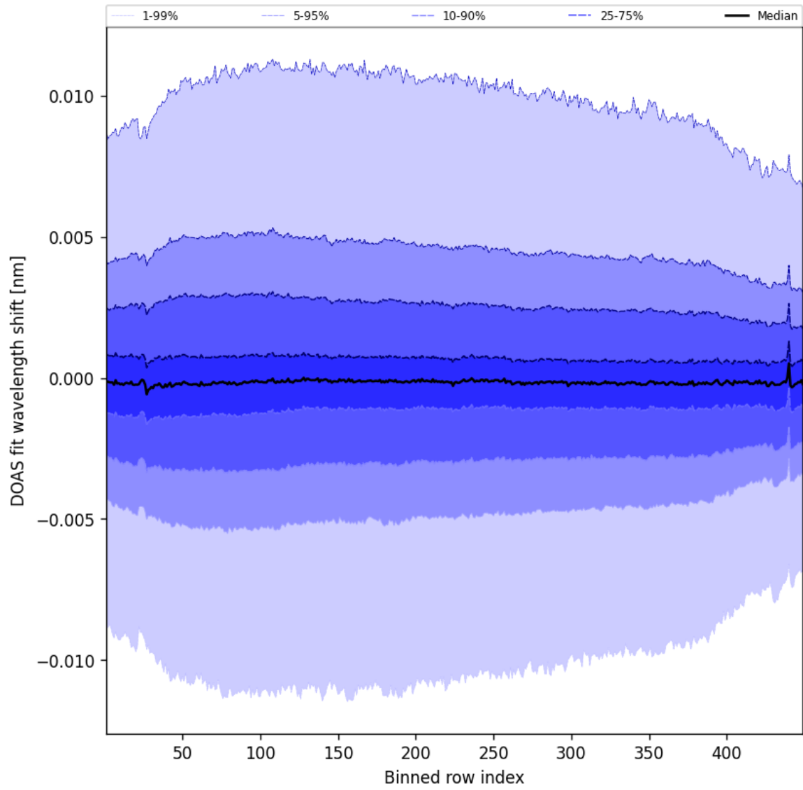
Figure 56: Along track statistics of “DOAS fit wavelength shift” for 2025-04-11 to 2025-04-11
