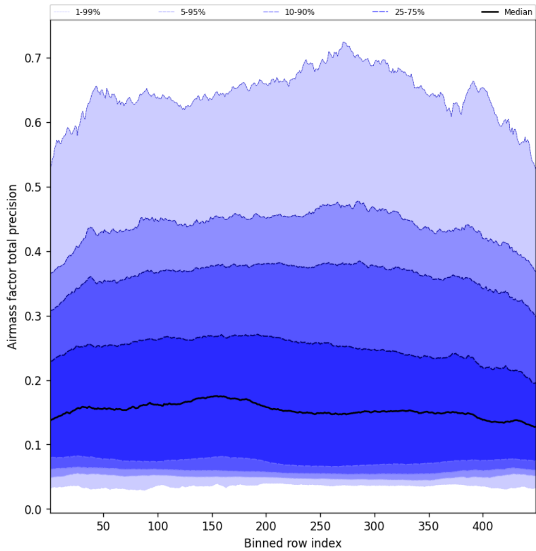
Figure 53: Along track statistics of “Airmass factor total precision” for 2025-04-11 to 2025-04-11
