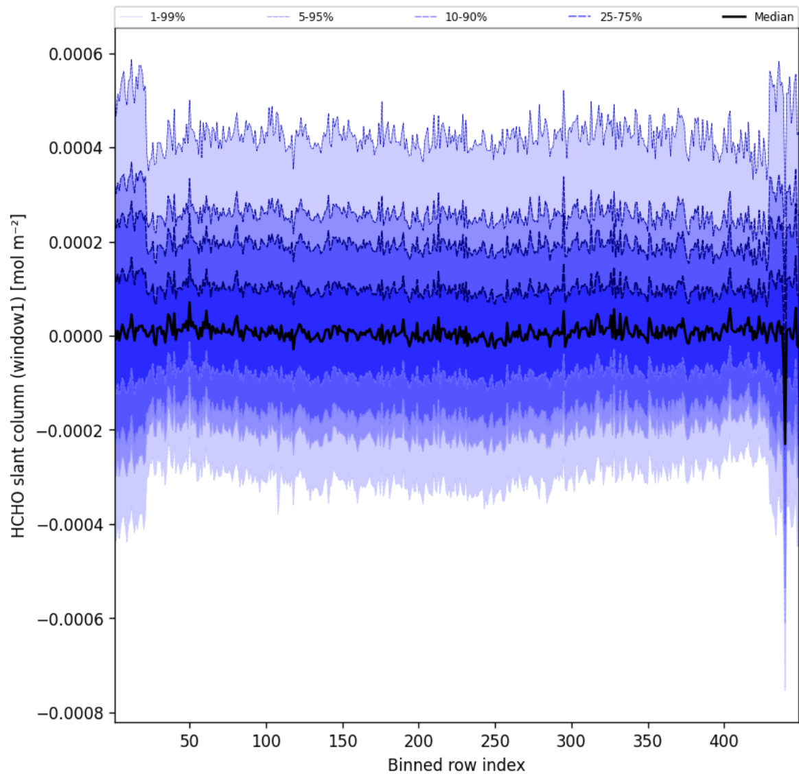
Figure 50: Along track statistics of “HCHO slant column (window1)” for 2025-04-11 to 2025-04-11
