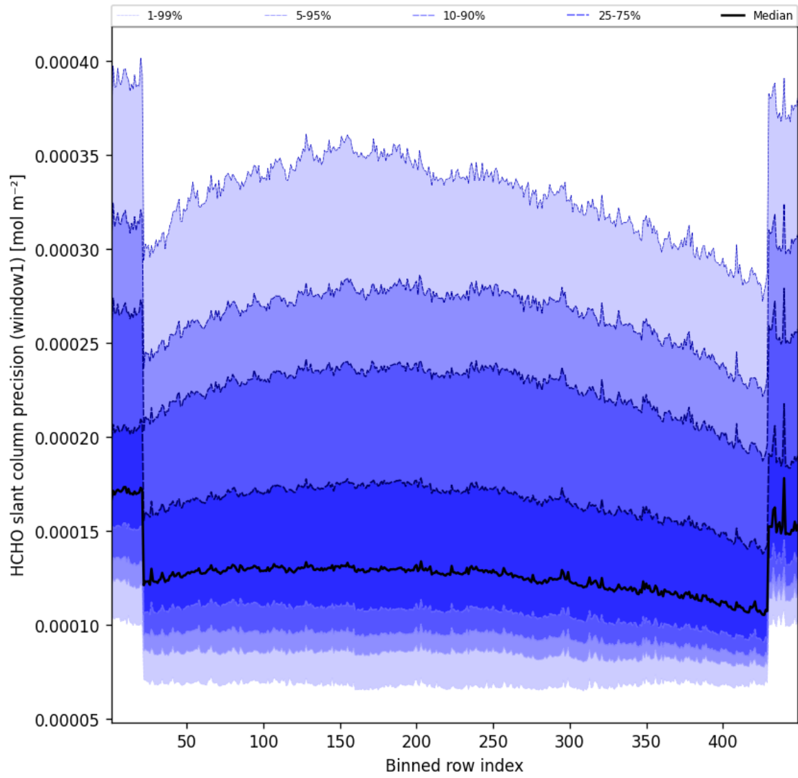
Figure 51: Along track statistics of “HCHO slant column precision (window1)” for 2025-04-11 to 2025-04-11
