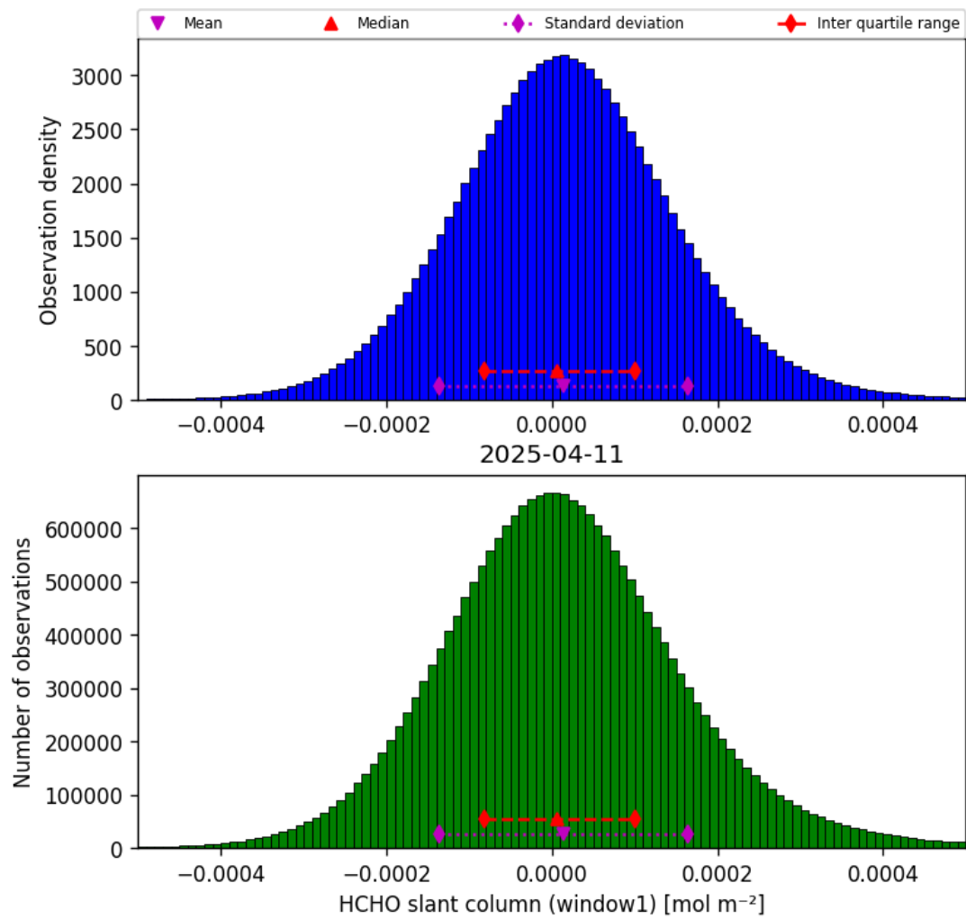
Figure 36: Histogram of “HCHO slant column (window1)” for 2025-04-11 to 2025-04-11
