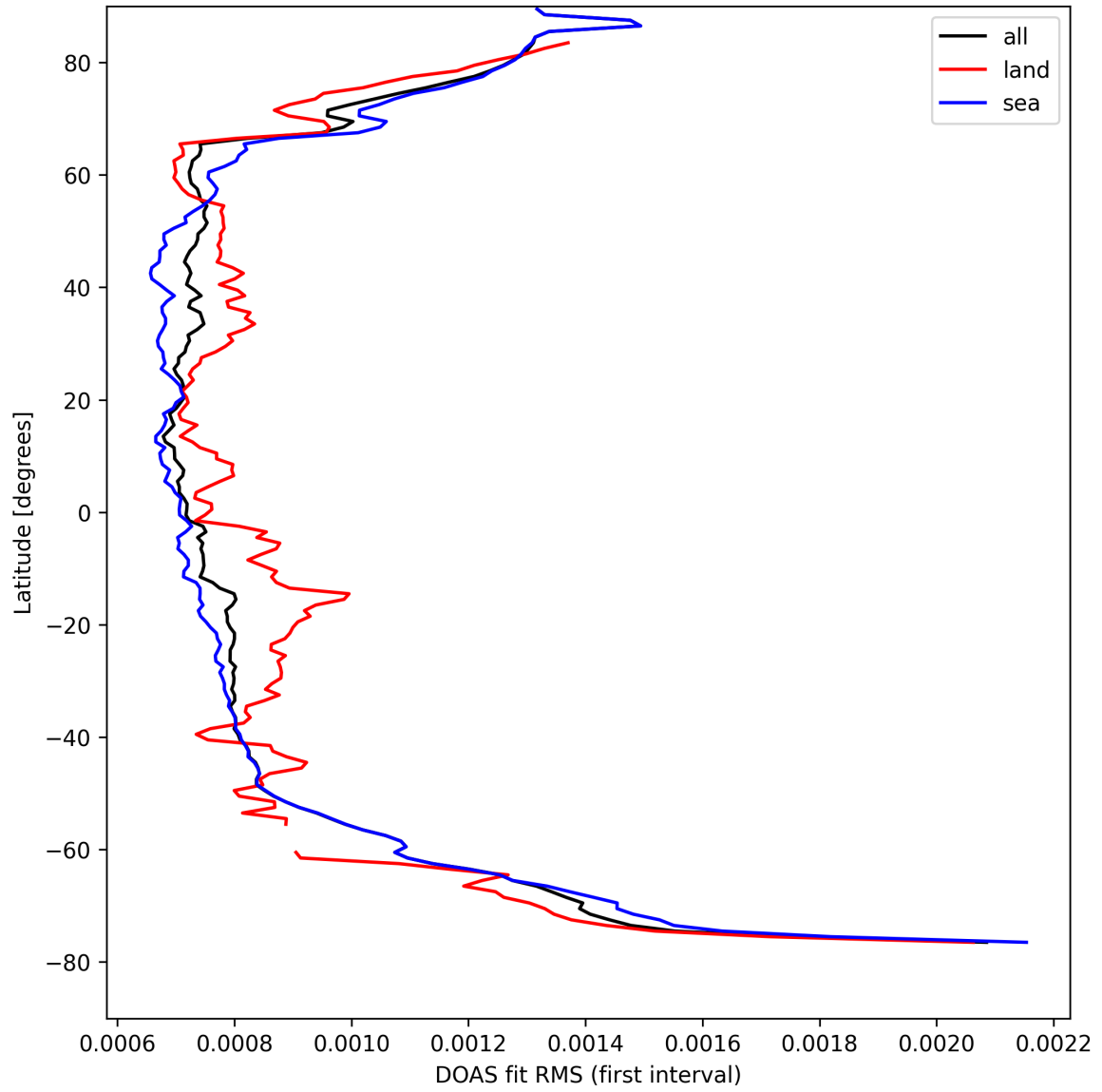
Figure 30: Zonal average of "DOAS fit RMS (first interval)" for 2025-04-11 to 2025-04-11.
