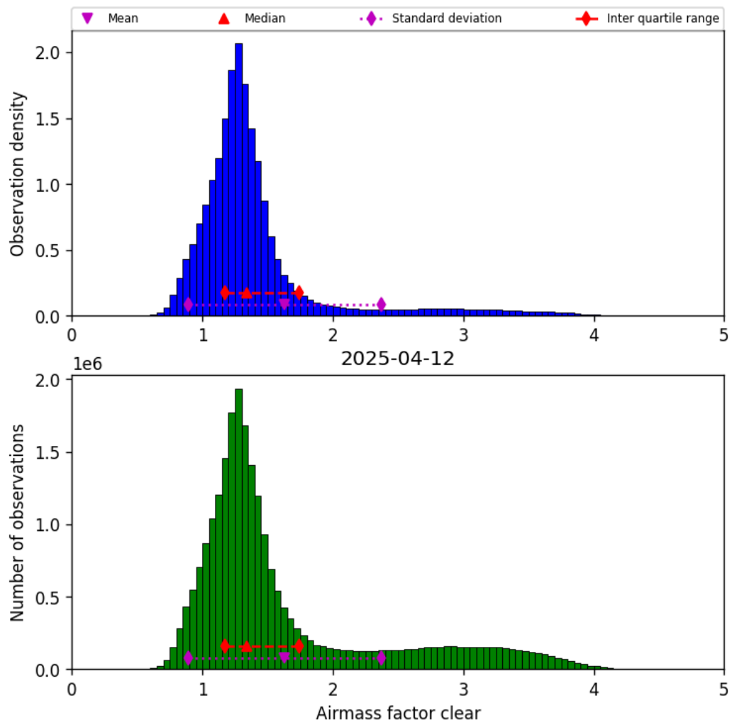
Figure 40: Histogram of “Airmass factor clear” for 2025-04-12 to 2025-04-13
