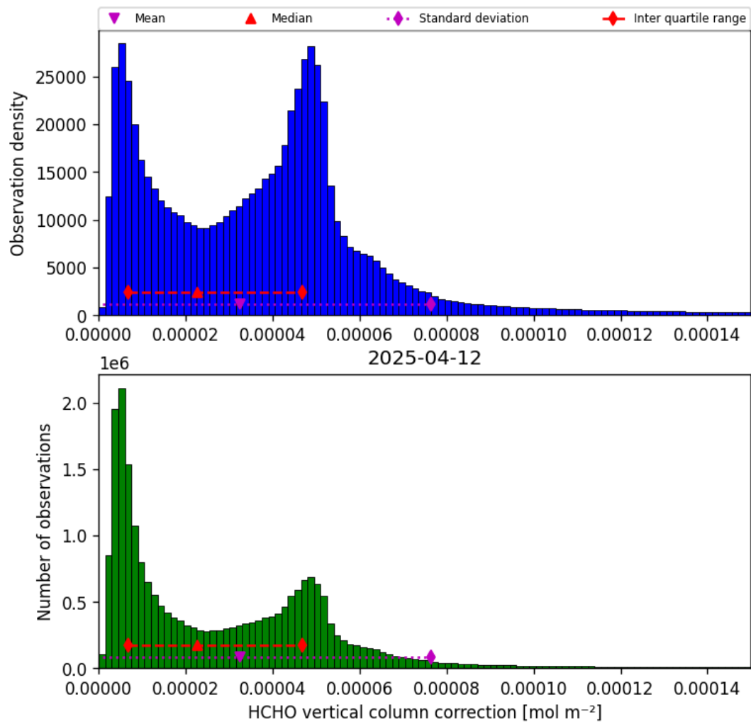
Figure 35: Histogram of “HCHO vertical column correction” for 2025-04-12 to 2025-04-13
