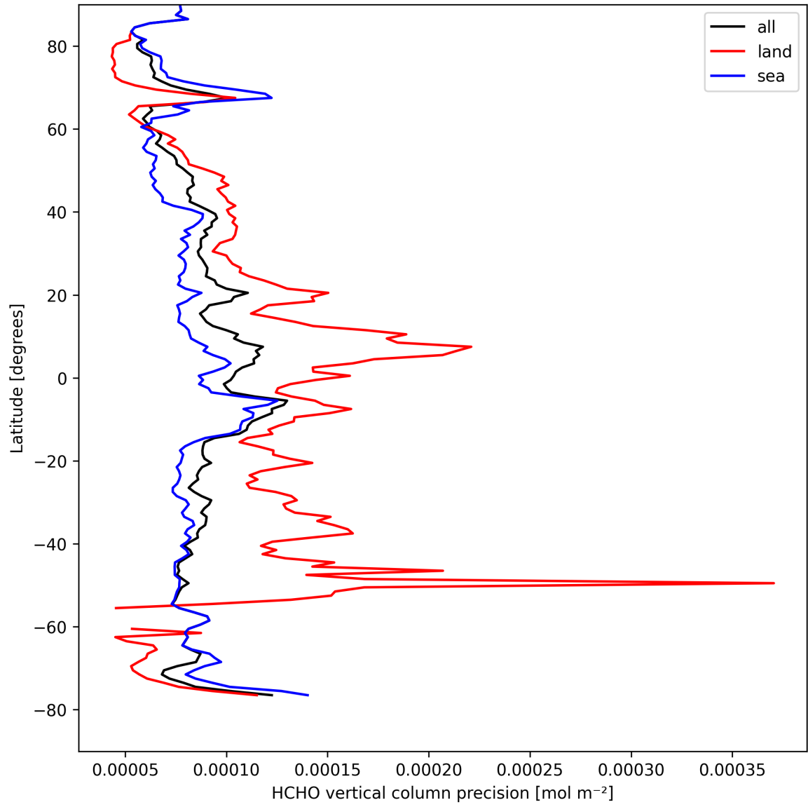
Figure 20: Zonal average of “HCHO vertical column precision” for 2025-04-12 to 2025-04-13.
