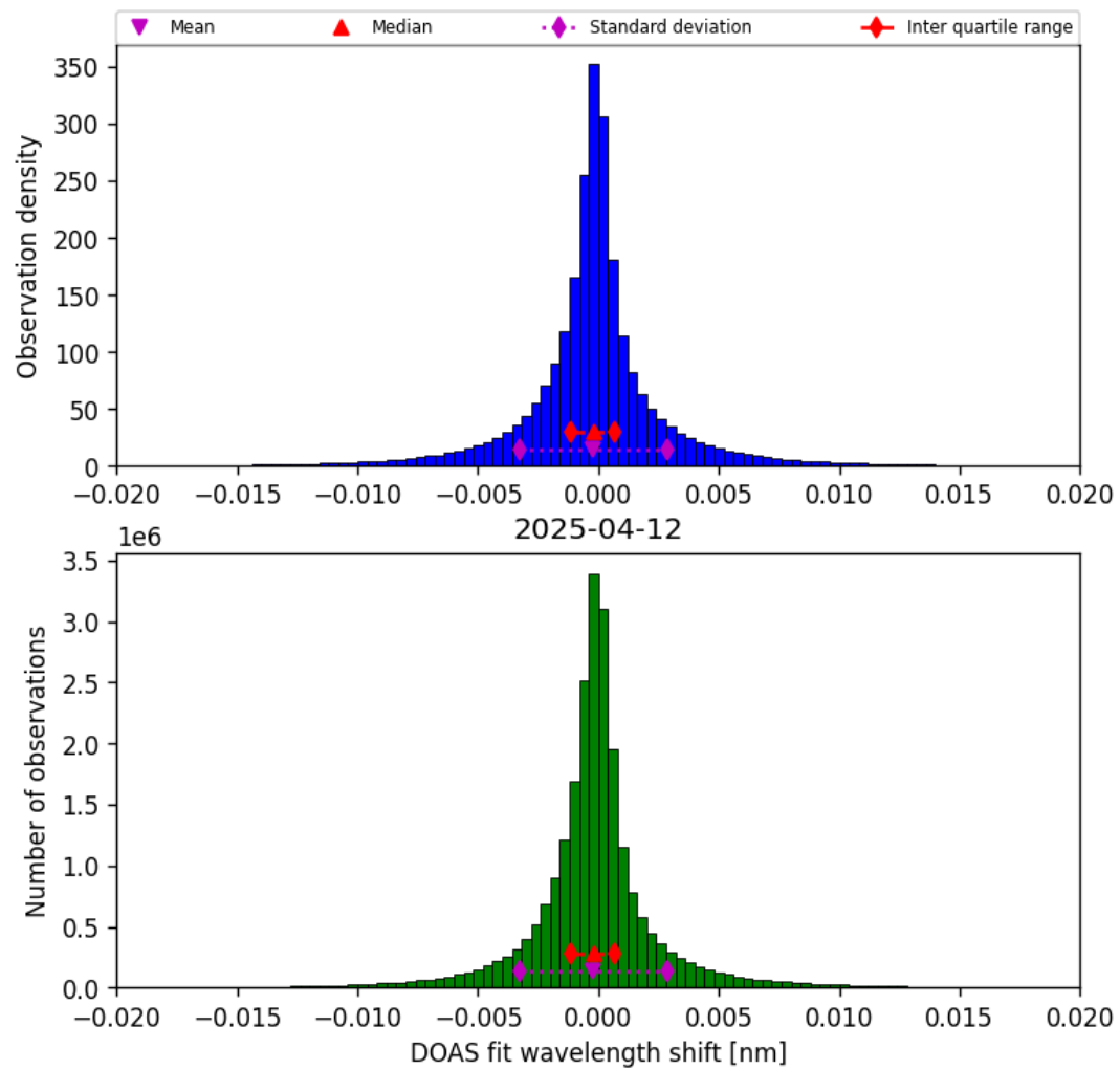
Figure 42: Histogram of “DOAS fit wavelength shift” for 2025-04-12 to 2025-04-13
