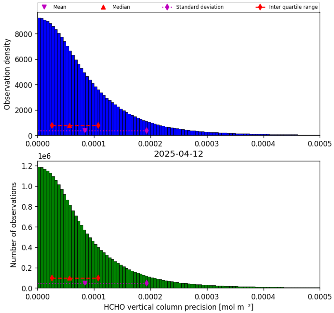
Figure 34: Histogram of “HCHO vertical column precision” for 2025-04-12 to 2025-04-13
