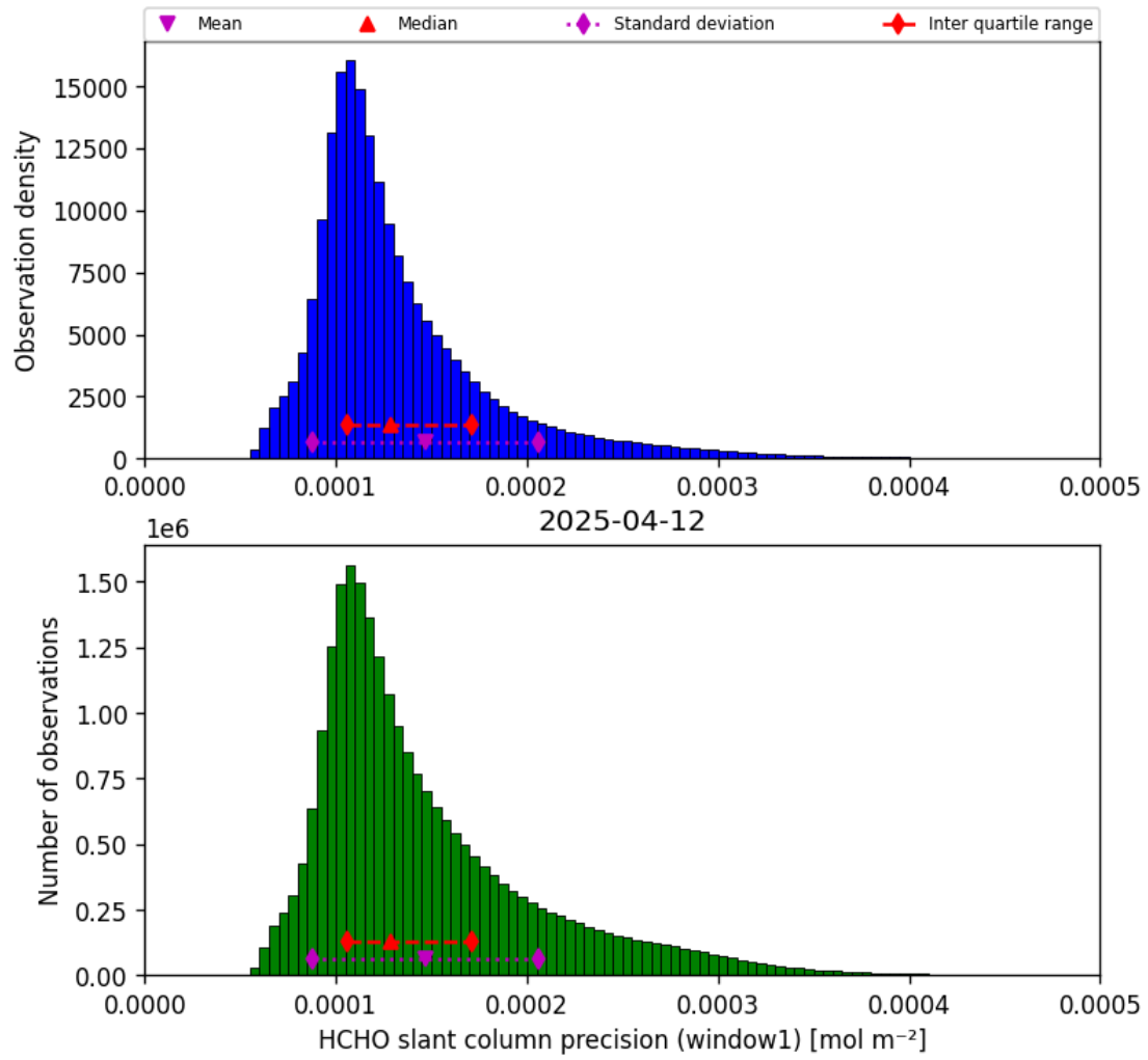
Figure 37: Histogram of “HCHO slant column precision (window1)” for 2025-04-12 to 2025-04-13
