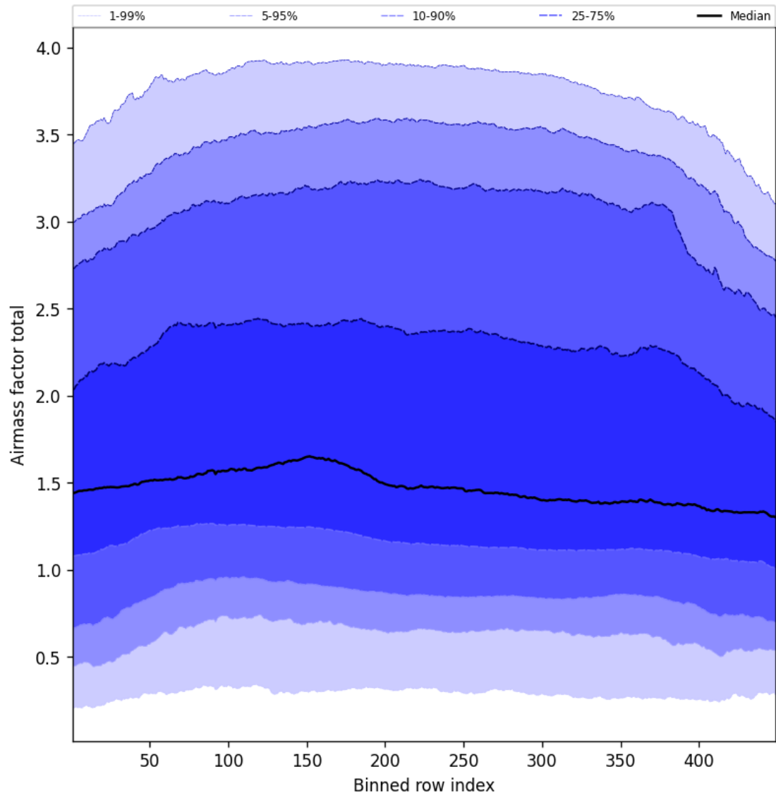
Figure 52: Along track statistics of “Airmass factor total” for 2025-04-12 to 2025-04-13
