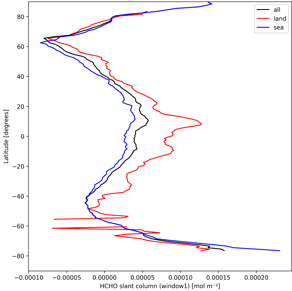
Figure 22: Zonal average of “HCHO slant column (window1)” for 2025-04-12 to 2025-04-13.
