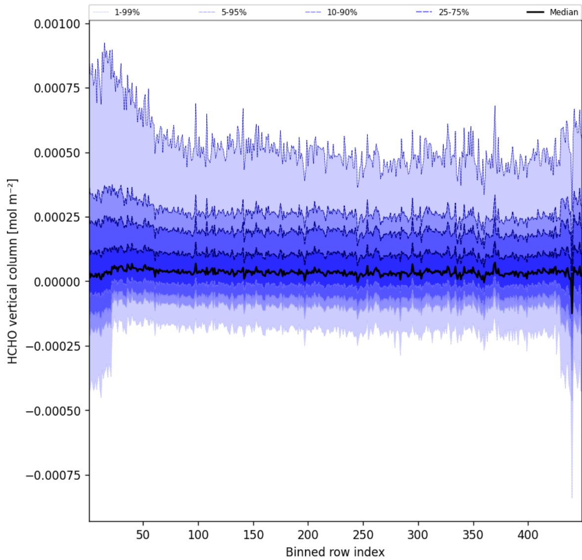
Figure 47: Along track statistics of “HCHO vertical column” for 2025-04-12 to 2025-04-13
