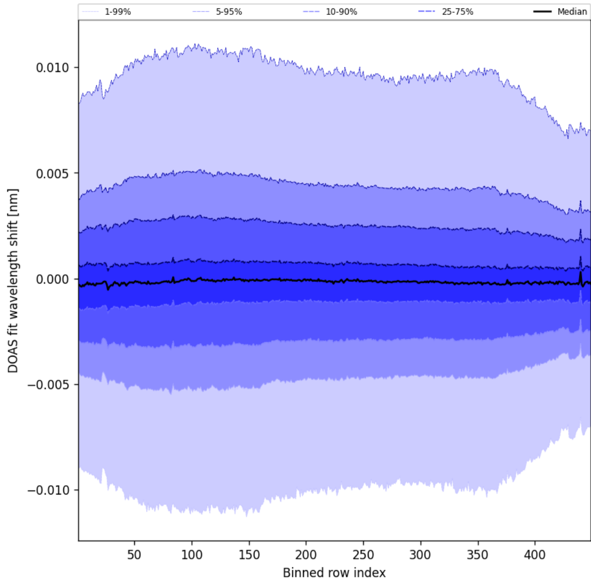
Figure 56: Along track statistics of “DOAS fit wavelength shift” for 2025-04-12 to 2025-04-13
