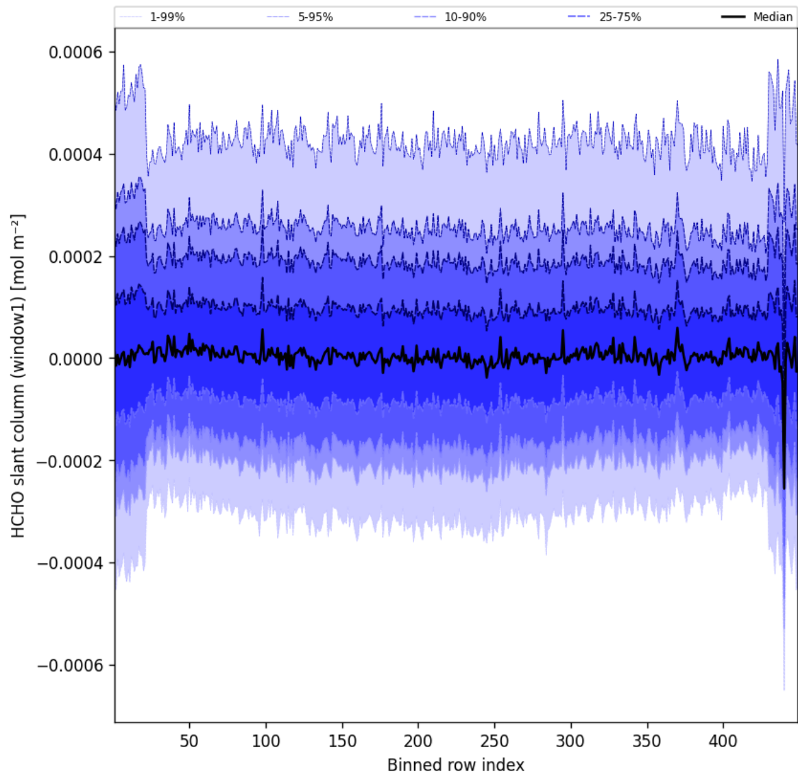
Figure 50: Along track statistics of “HCHO slant column (window1)” for 2025-04-12 to 2025-04-13
