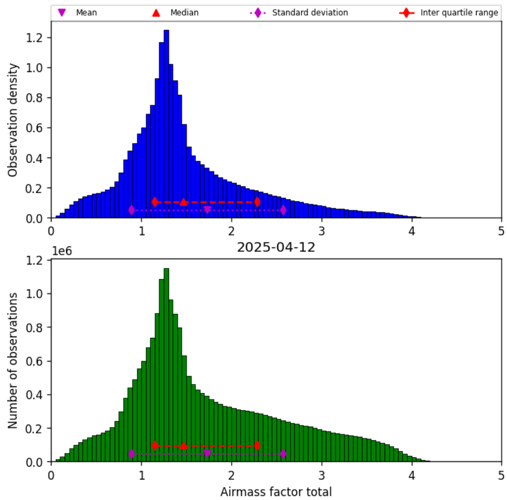
Figure 38: Histogram of “Airmass factor total” for 2025-04-12 to 2025-04-13
