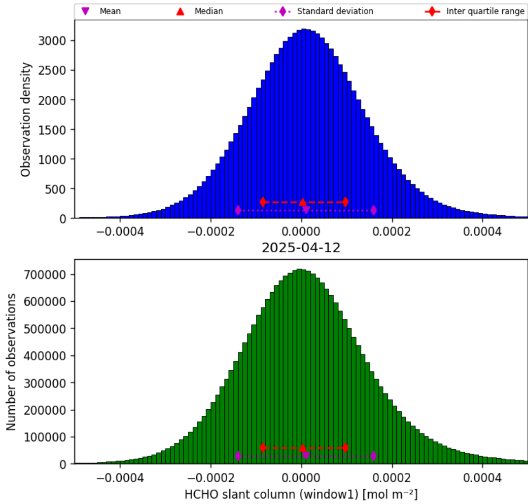
Figure 36: Histogram of “HCHO slant column (window1)” for 2025-04-12 to 2025-04-13
