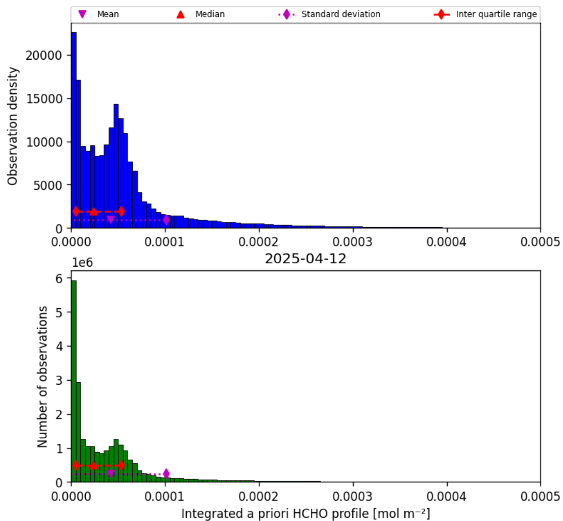
Figure 41: Histogram of “Integrated a priori HCHO profile” for 2025-04-12 to 2025-04-13
