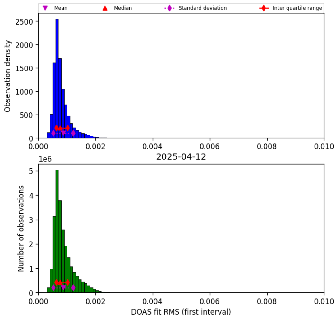
Figure 44: Histogram of “DOAS fit RMS (first interval)” for 2025-04-12 to 2025-04-13
