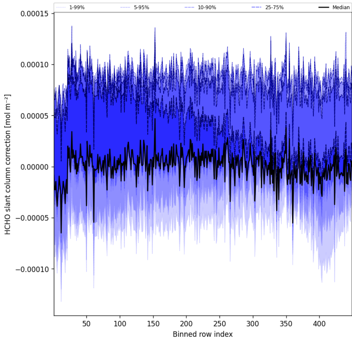
Figure 59: Along track statistics of “HCHO slant column correction” for 2025-04-12 to 2025-04-13
