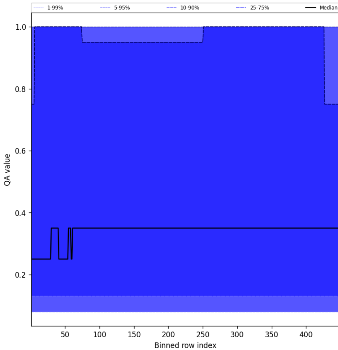
Figure 46: Along track statistics of “QA value” for 2025-04-12 to 2025-04-13
