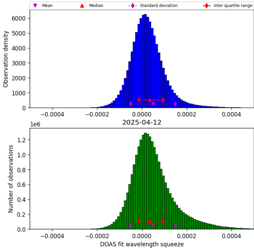
Figure 43: Histogram of “DOAS fit wavelength squeeze” for 2025-04-12 to 2025-04-13
