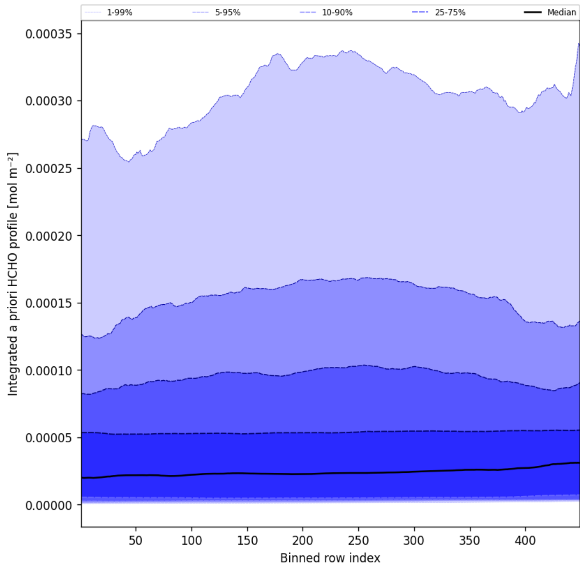
Figure 55: Along track statistics of “Integrated a priori HCHO profile” for 2025-04-12 to 2025-04-13
