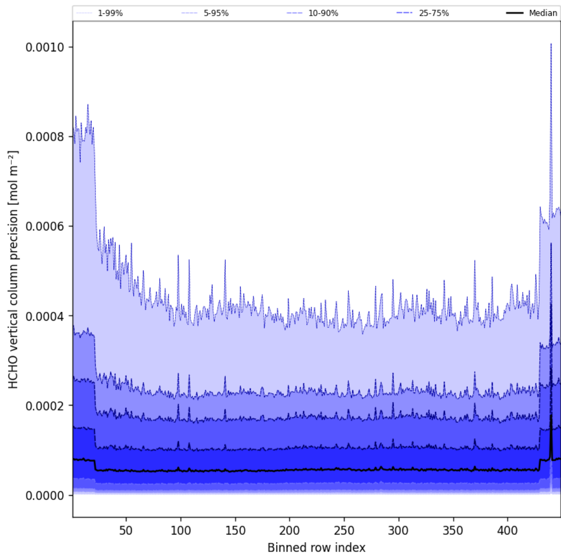
Figure 48: Along track statistics of “HCHO vertical column precision” for 2025-04-12 to 2025-04-13
