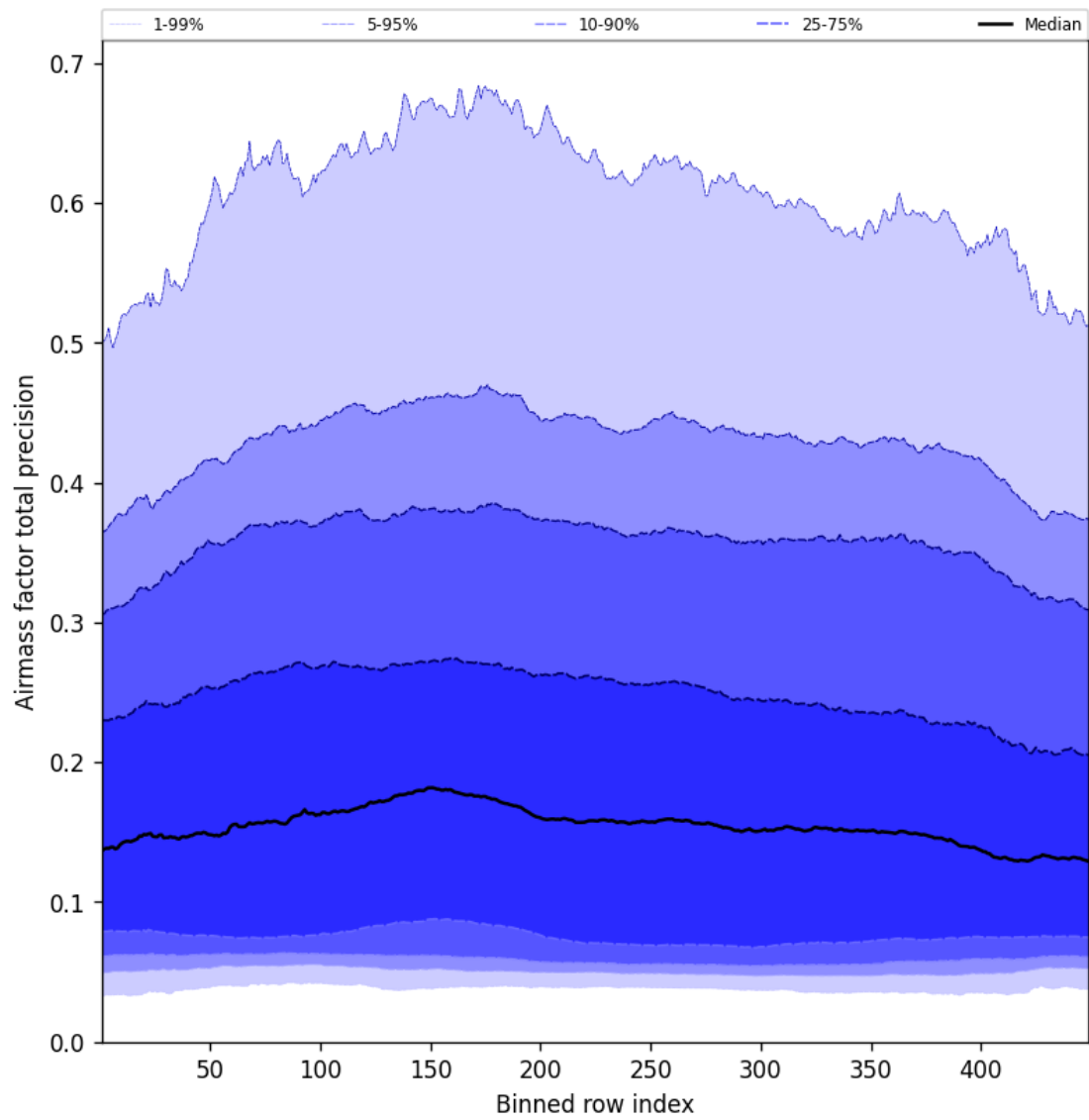
Figure 53: Along track statistics of “Airmass factor total precision” for 2025-04-12 to 2025-04-13
