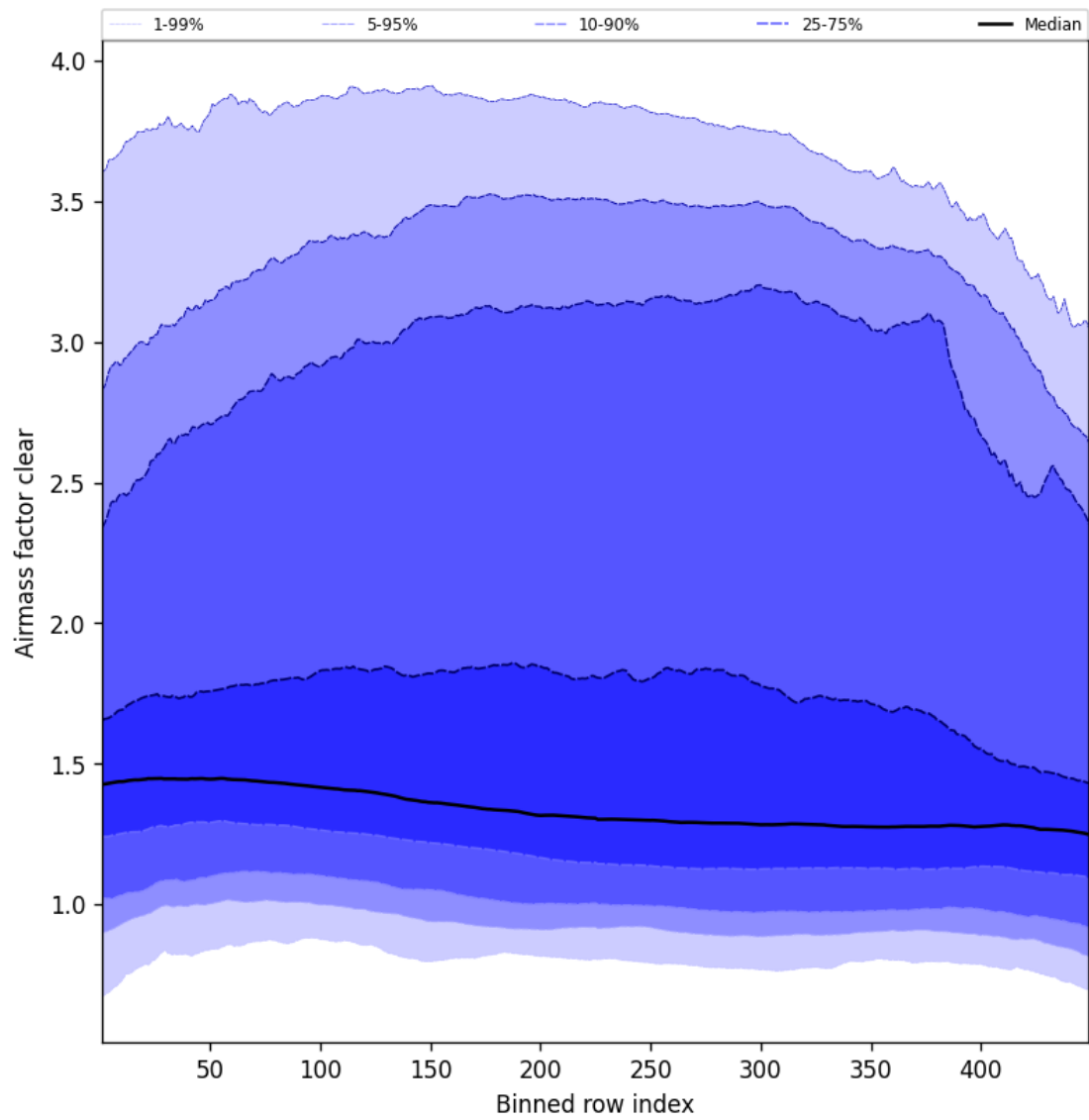
Figure 54: Along track statistics of “Air mass factor clear” for 2025-04-12 to 2025-04-13
