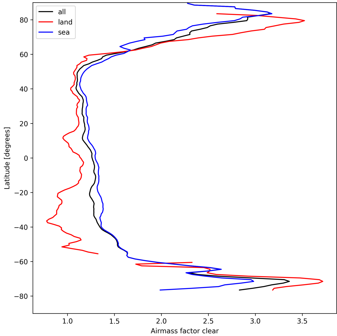
Figure 26: Zonal average of “Airmass factor clear” for 2025-04-12 to 2025-04-13.
