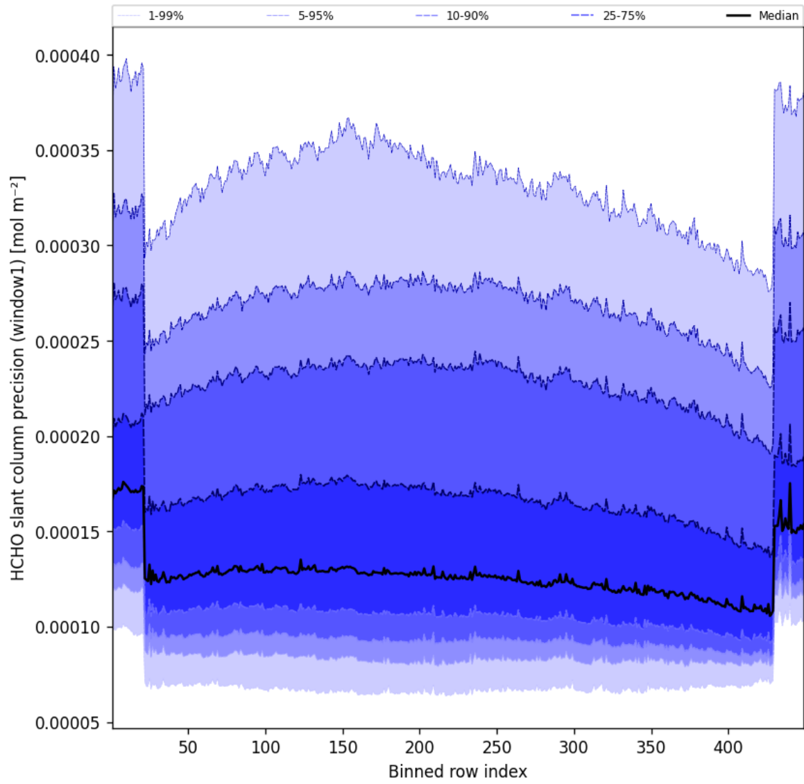
Figure 51: Along track statistics of “HCHO slant column precision (window1)” for 2025-04-12 to 2025-04-13
