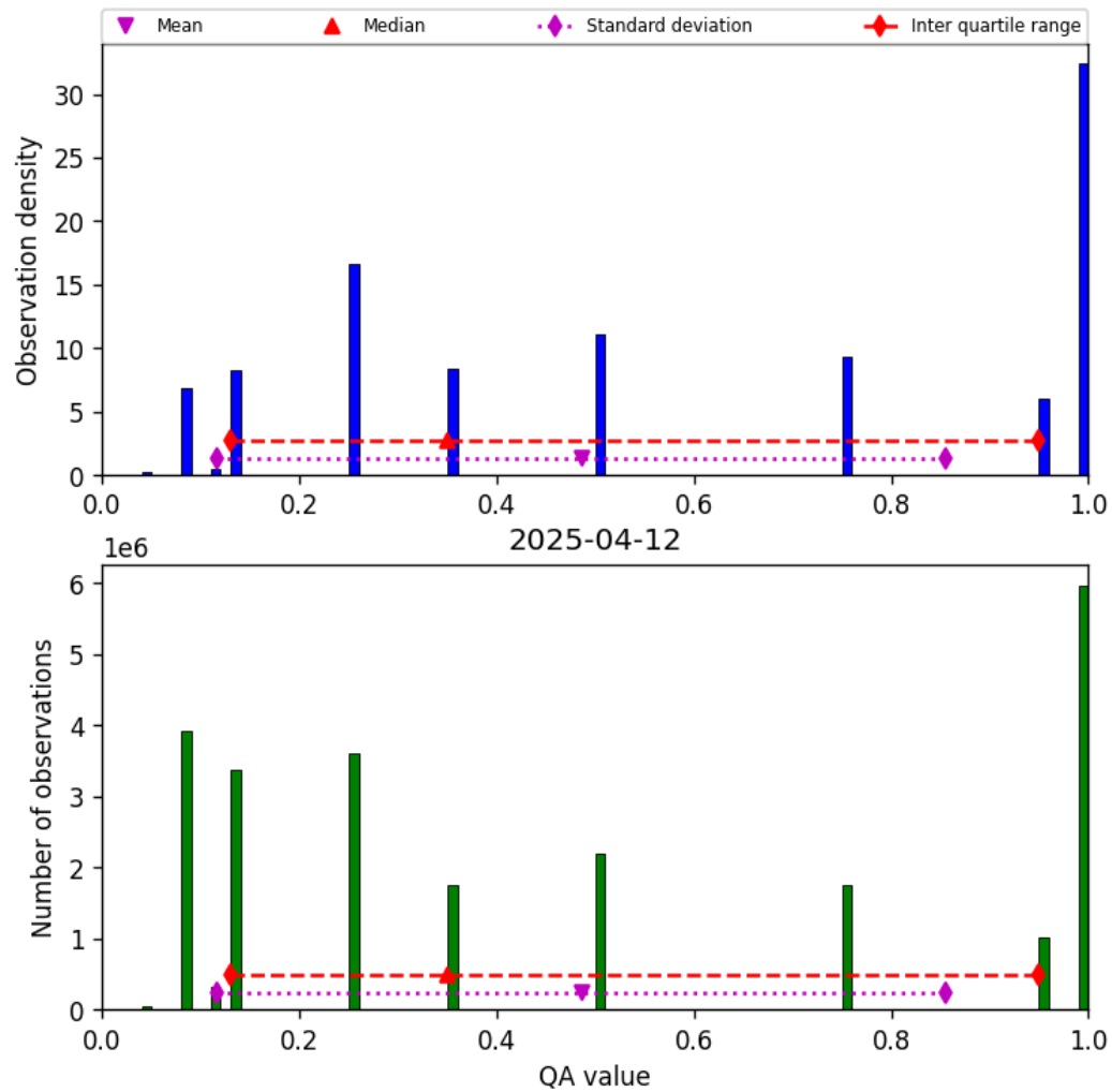
Figure 32: Histogram of “QA value” for 2025-04-12 to 2025-04-13
