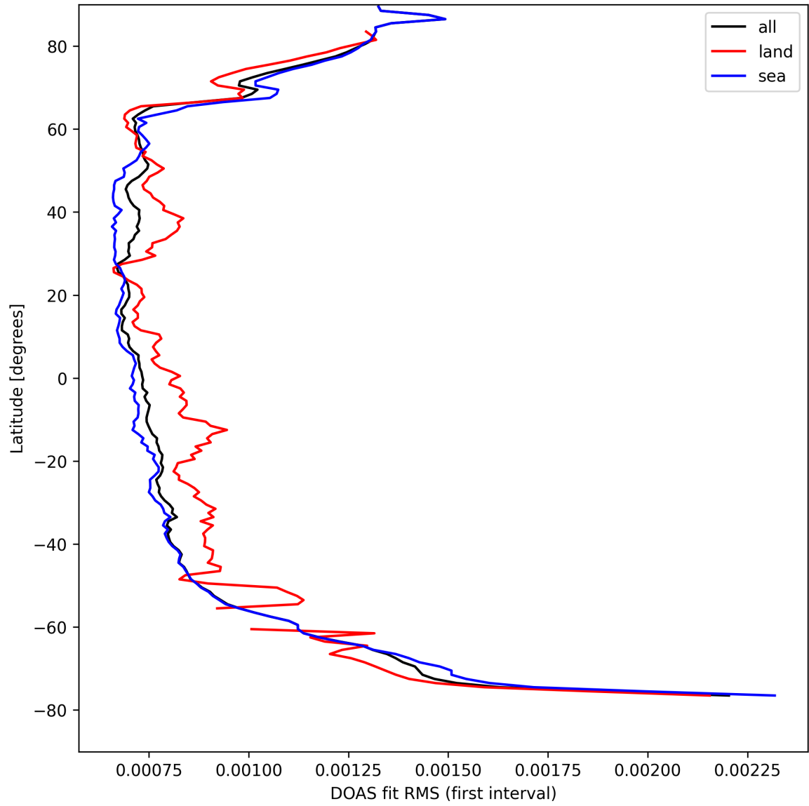
Figure 30: Zonal average of "DOAS fit RMS (first interval)" for 2025-04-12 to 2025-04-13.
