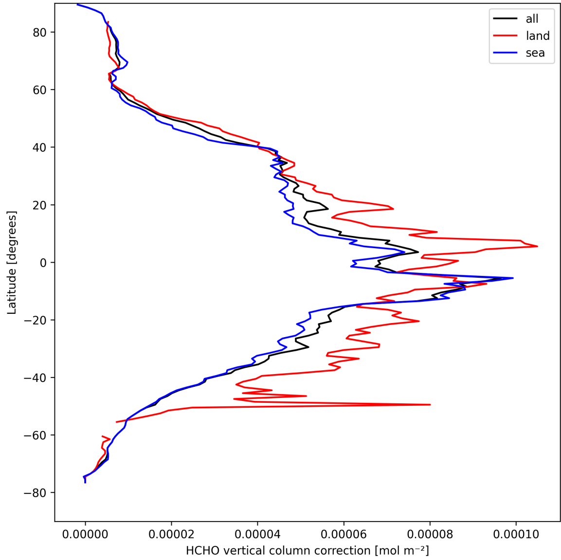
Figure 21: Zonal average of “HCHO vertical column correction” for 2025-04-12 to 2025-04-13.
