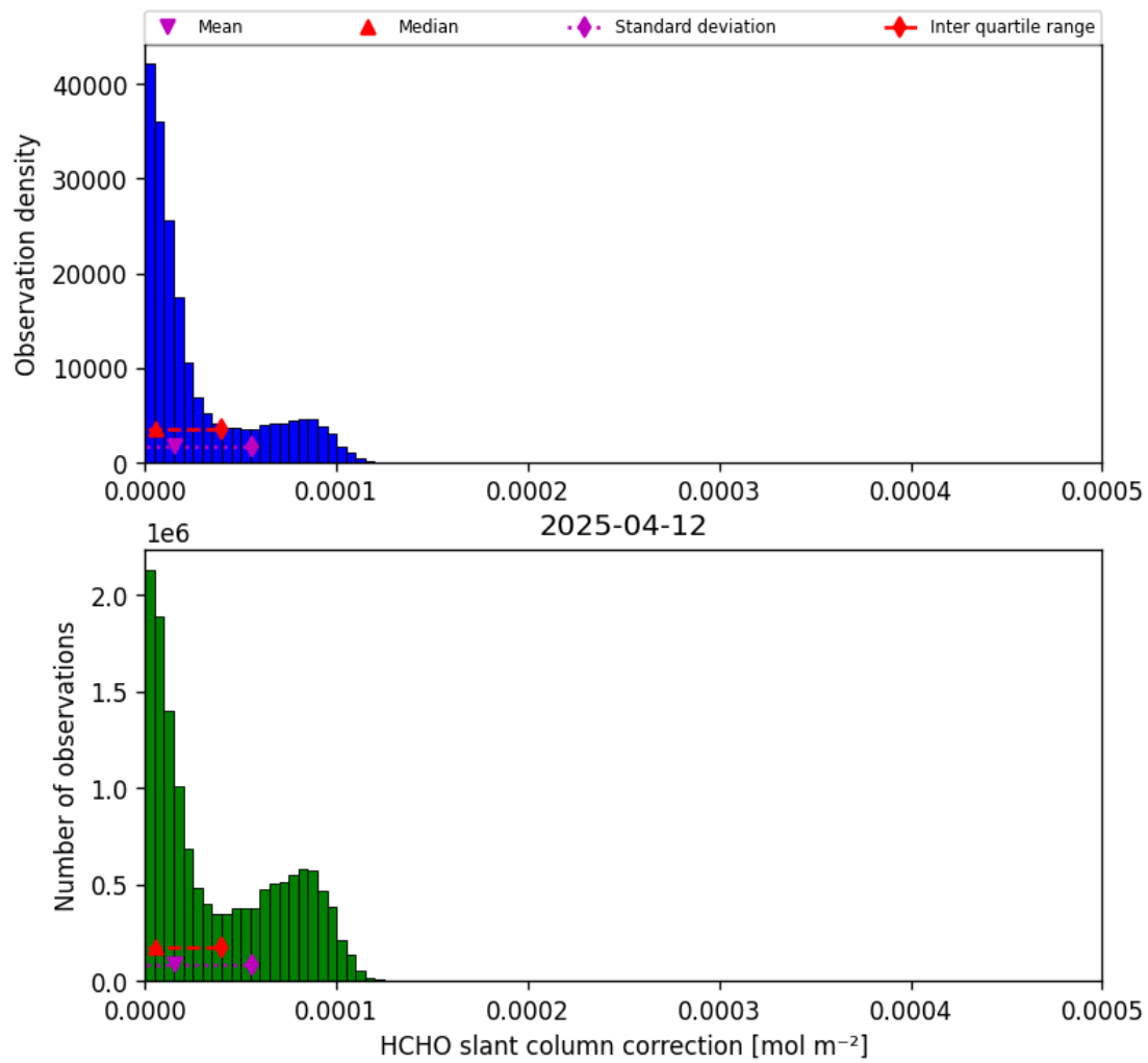
Figure 45: Histogram of “HCHO slant column correction” for 2025-04-12 to 2025-04-13
