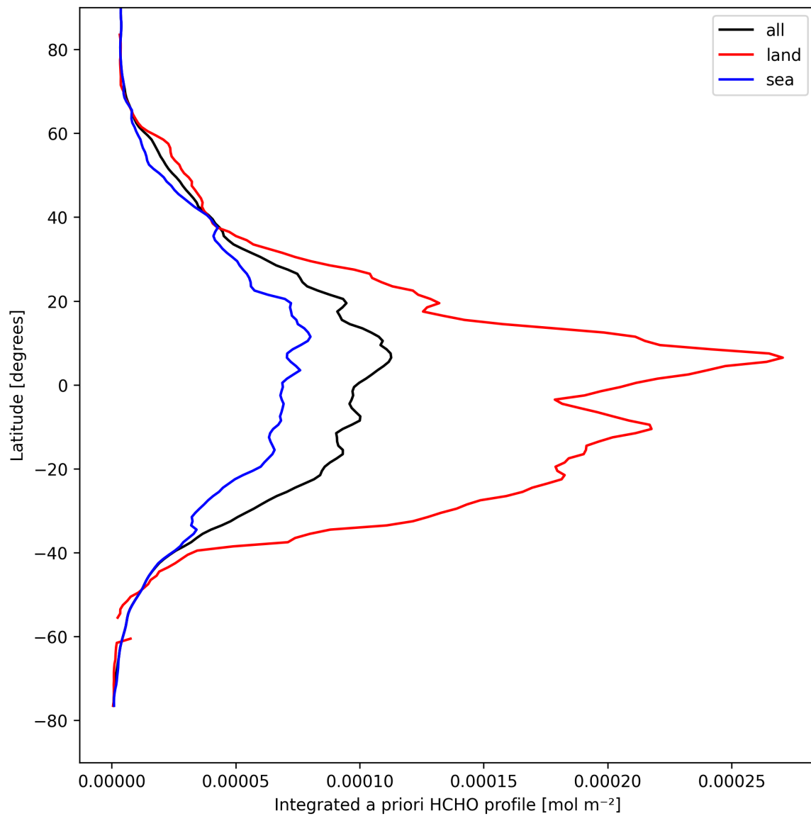
Figure 27: Zonal average of “Integrated a priori HCHO profile” for 2025-04-12 to 2025-04-13.
