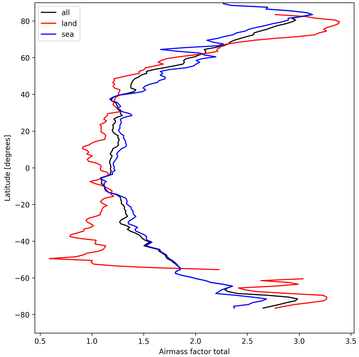
Figure 24: Zonal average of “Airmass factor total” for 2025-04-12 to 2025-04-13.
