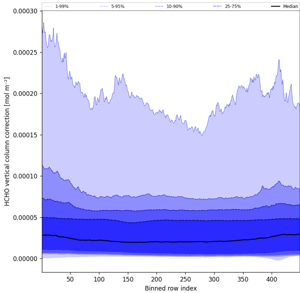
Figure 49: Along track statistics of “HCHO vertical column correction” for 2025-04-12 to 2025-04-13
