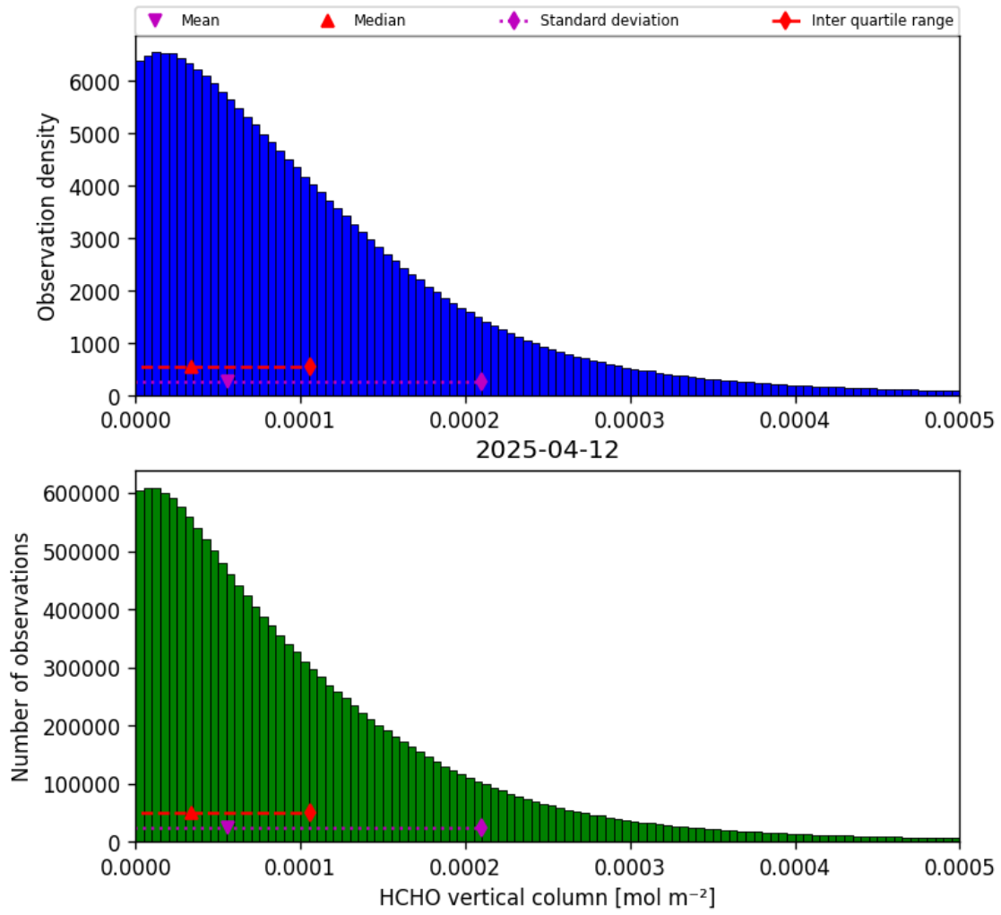
Figure 33: Histogram of “HCHO vertical column” for 2025-04-12 to 2025-04-13
