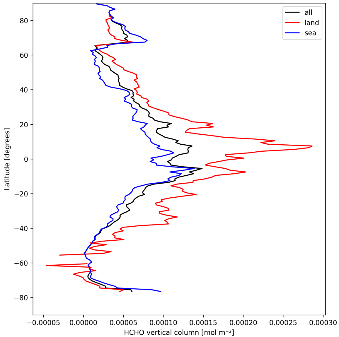
Figure 19: Zonal average of “HCHO vertical column” for 2025-04-12 to 2025-04-13.
