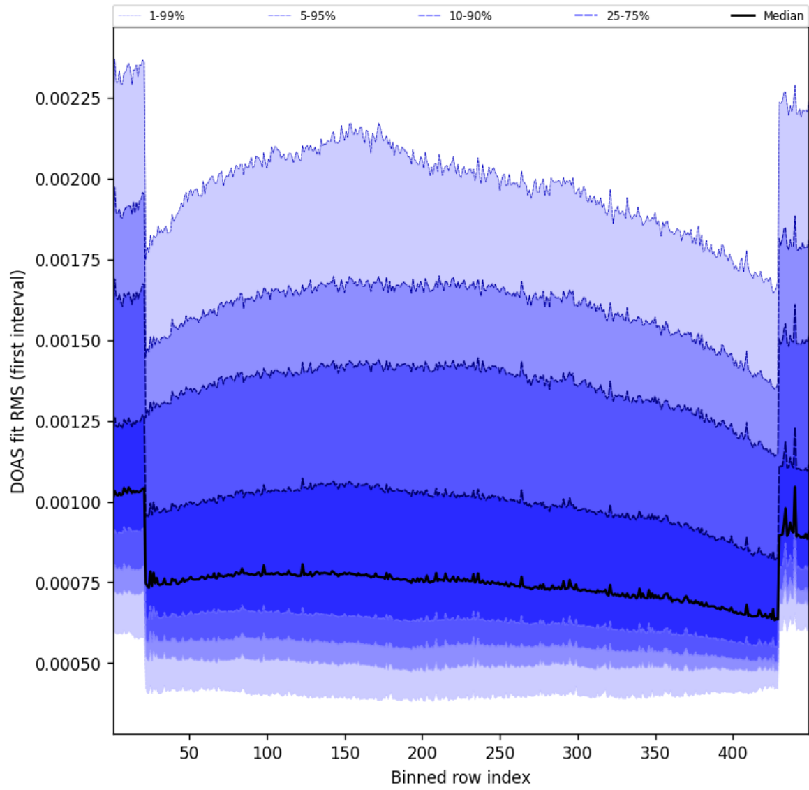
Figure 58: Along track statistics of “DOAS fit RMS (first interval)” for 2025-04-12 to 2025-04-13
