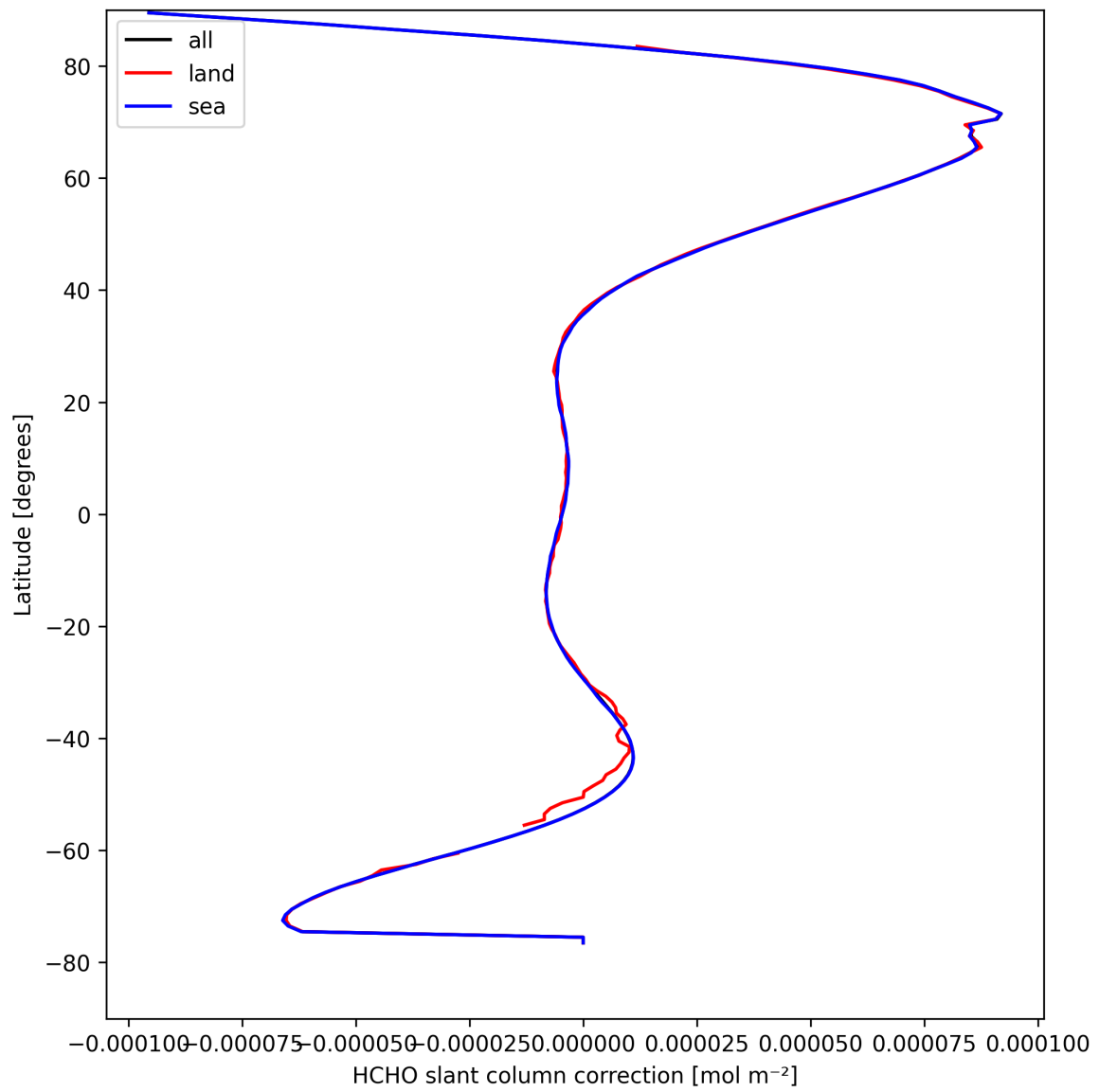
Figure 31: Zonal average of "HCHO slant column correction" for 2025-04-12 to 2025-04-13.
