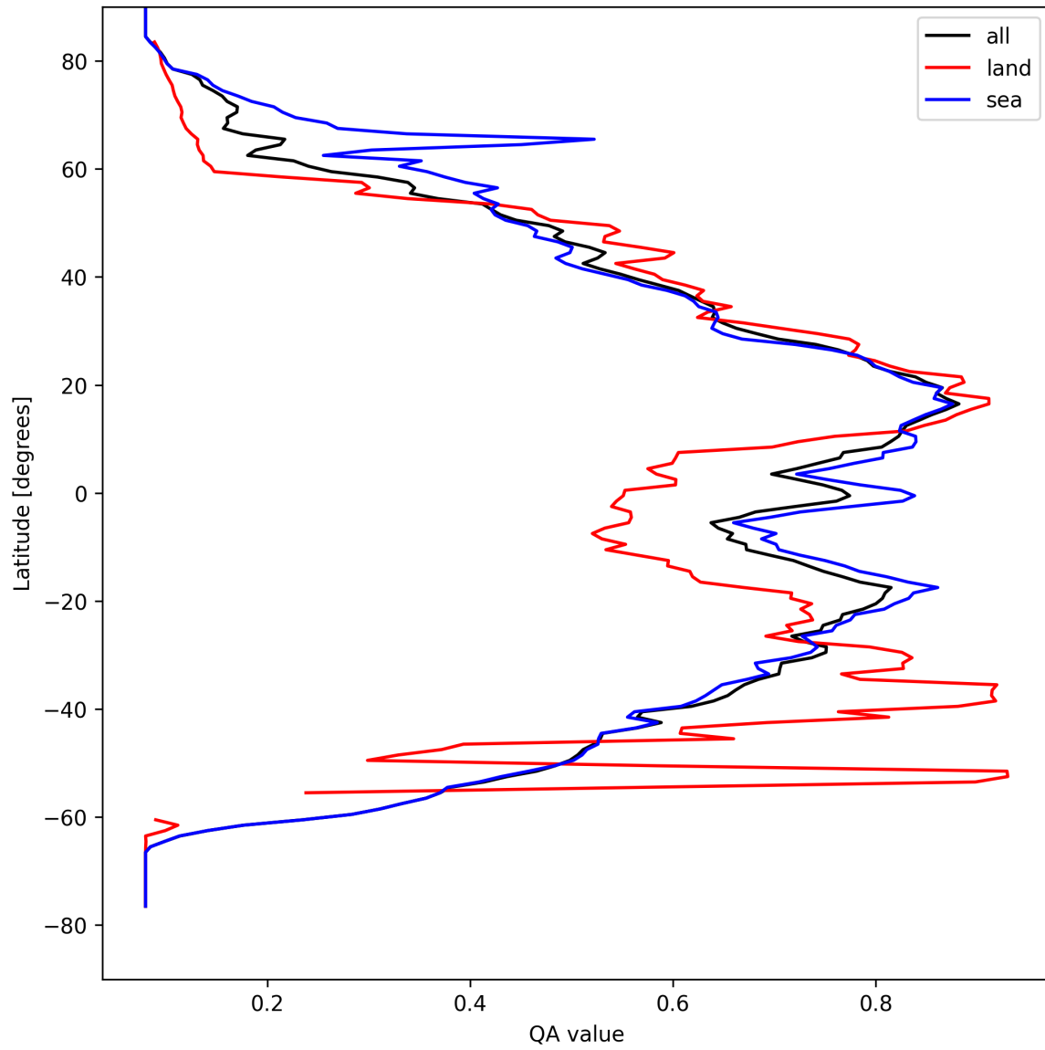
Figure 18: Zonal average of “QA value” for 2025-04-12 to 2025-04-13.
