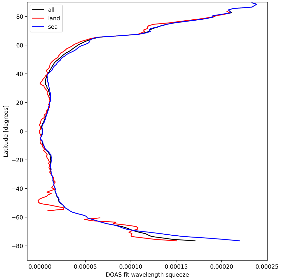
Figure 29: Zonal average of “DOAS fit wavelength squeeze” for 2025-04-12 to 2025-04-13.
