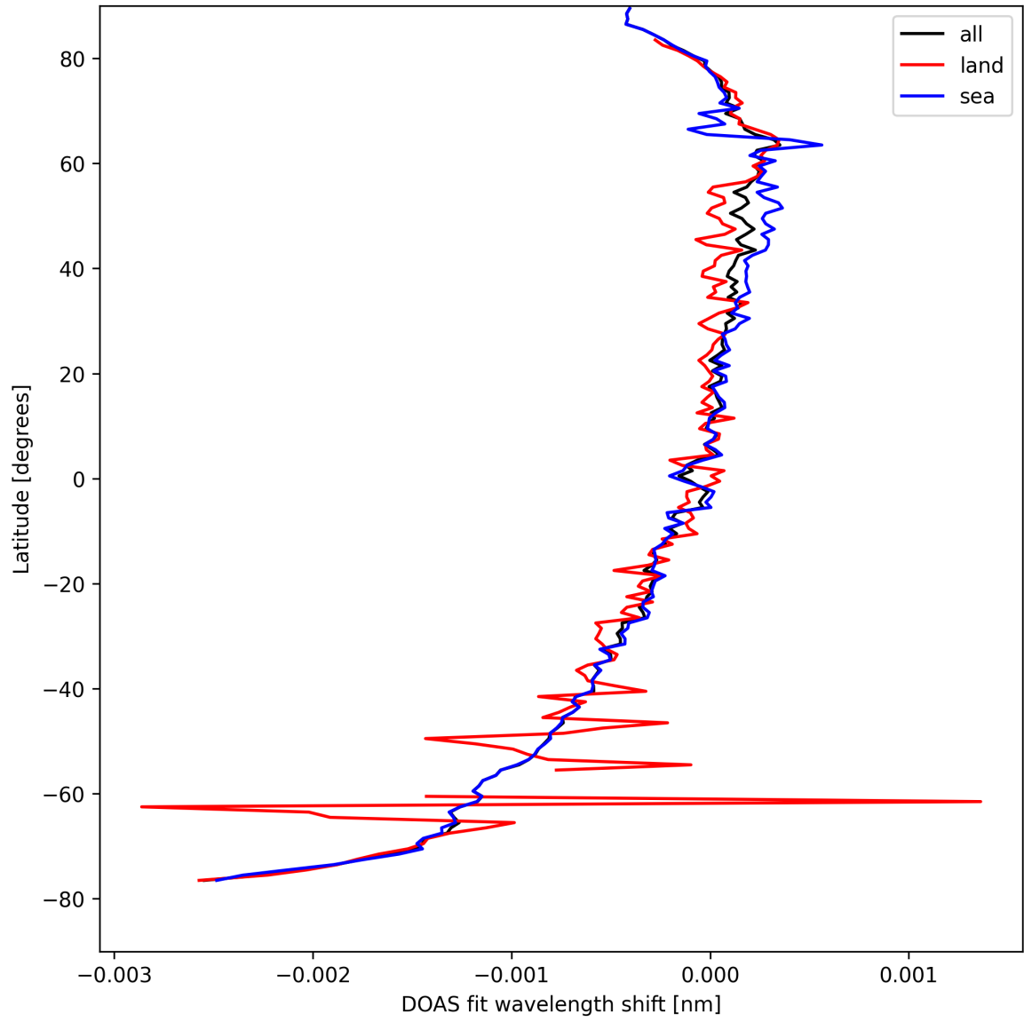
Figure 28: Zonal average of "DOAS fit wavelength shift" for 2025-04-12 to 2025-04-13.
