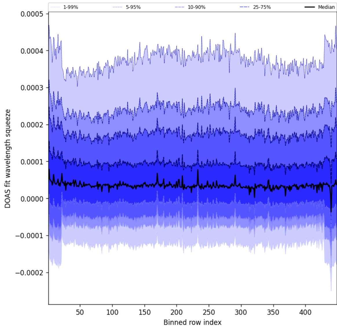
Figure 57: Along track statistics of “DOAS fit wavelength squeeze” for 2025-04-12 to 2025-04-13
