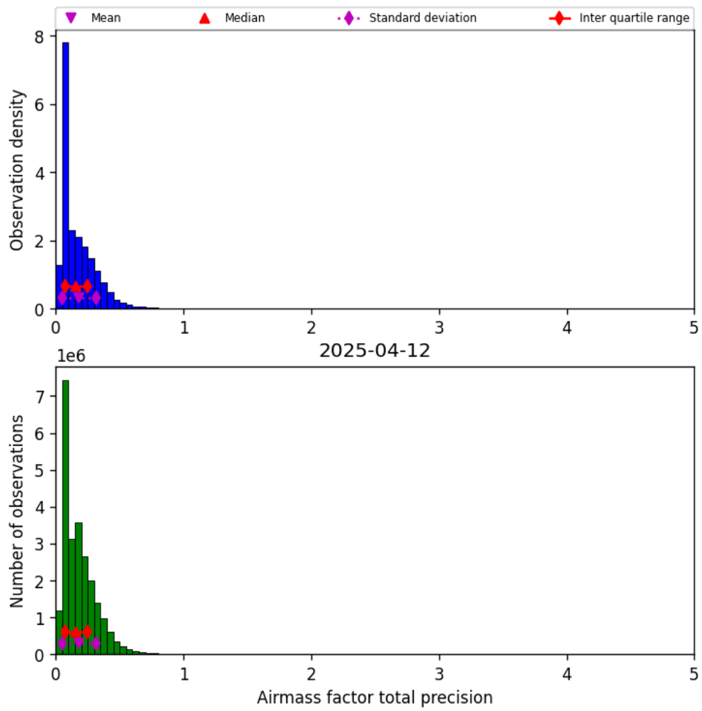
Figure 39: Histogram of “Airmass factor total precision” for 2025-04-12 to 2025-04-13
