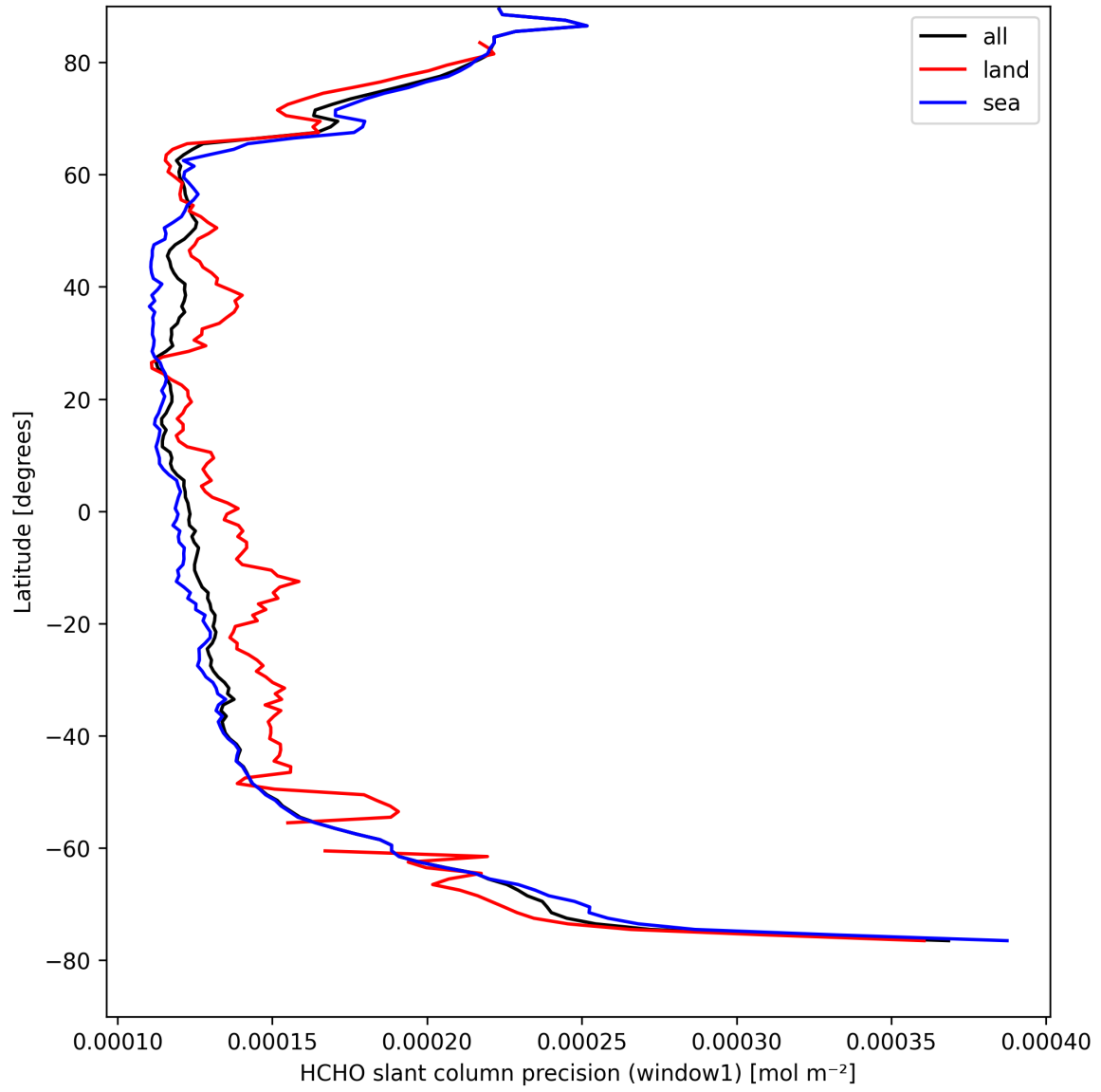
Figure 23: Zonal average of “HCHO slant column precision (window1)” for 2025-04-12 to 2025-04-13.
