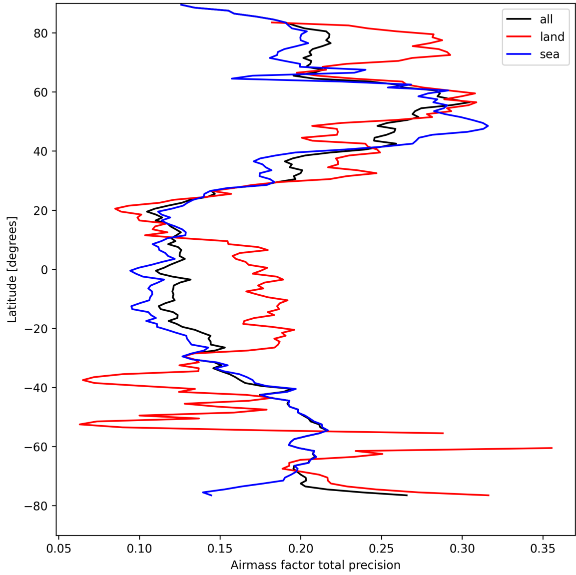
Figure 25: Zonal average of “Airmass factor total precision” for 2025-04-12 to 2025-04-13.
