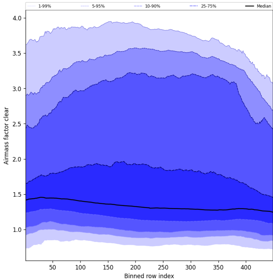
Figure 54: Along track statistics of “Airmass factor clear” for 2025-04-13 to 2025-04-14
