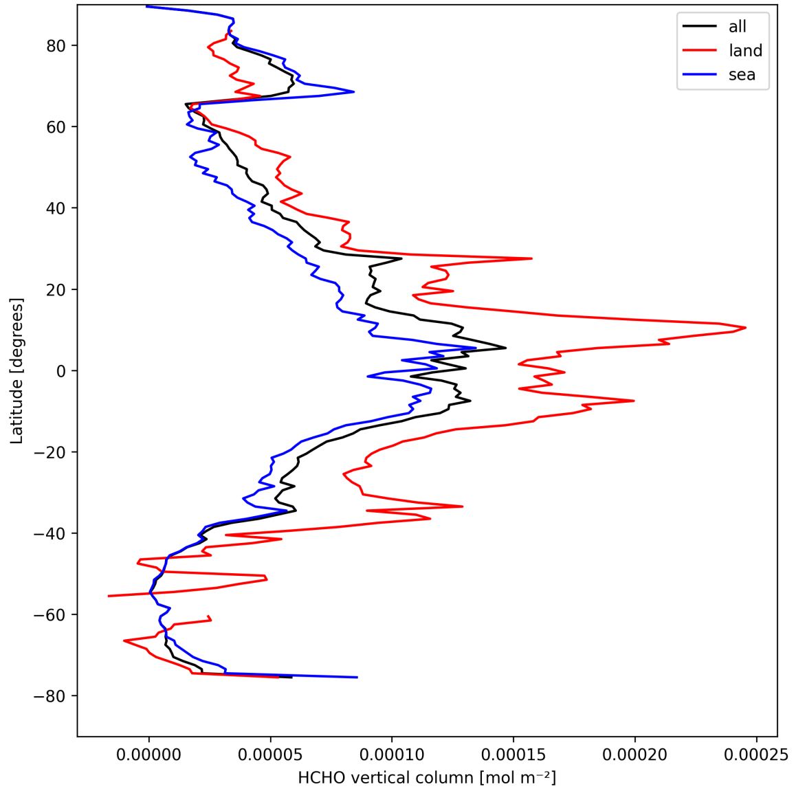
Figure 19: Zonal average of “HCHO vertical column” for 2025-04-13 to 2025-04-14.
