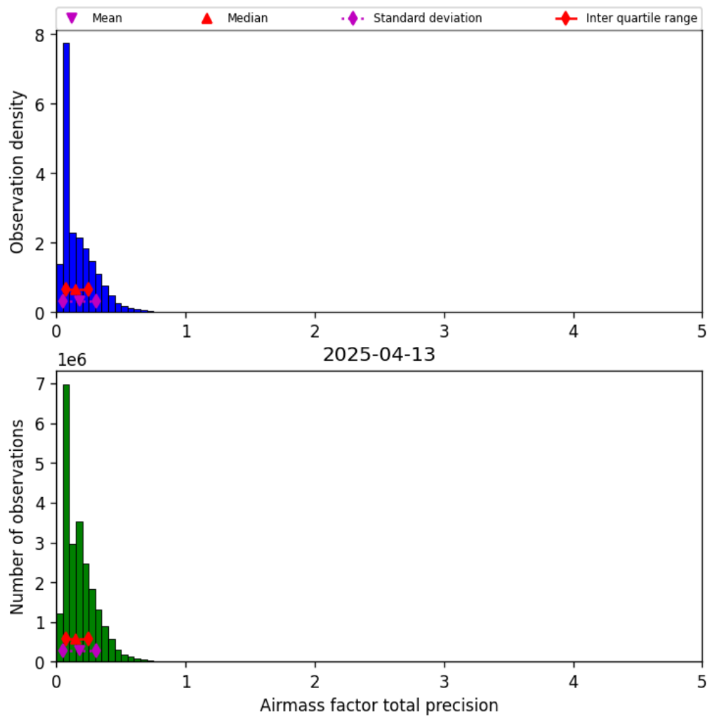
Figure 39: Histogram of “Airmass factor total precision” for 2025-04-13 to 2025-04-14
