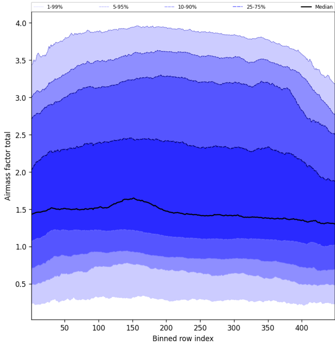
Figure 52: Along track statistics of “Airmass factor total” for 2025-04-13 to 2025-04-14
