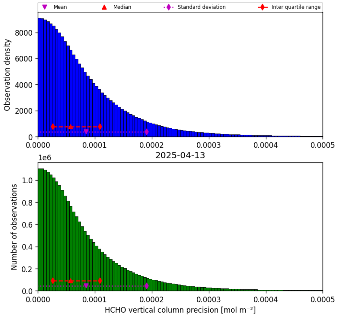
Figure 34: Histogram of “HCHO vertical column precision” for 2025-04-13 to 2025-04-14
