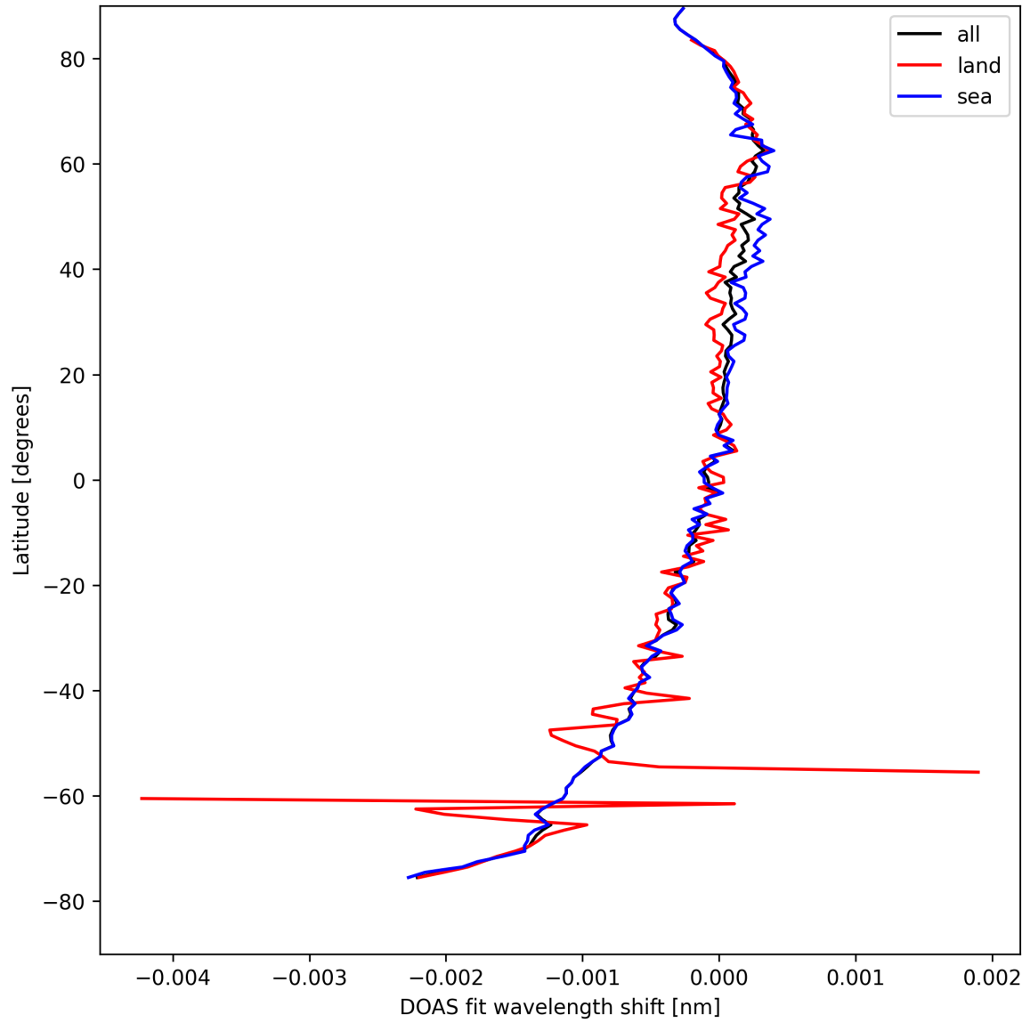
Figure 28: Zonal average of “DOAS fit wavelength shift” for 2025-04-13 to 2025-04-14.
