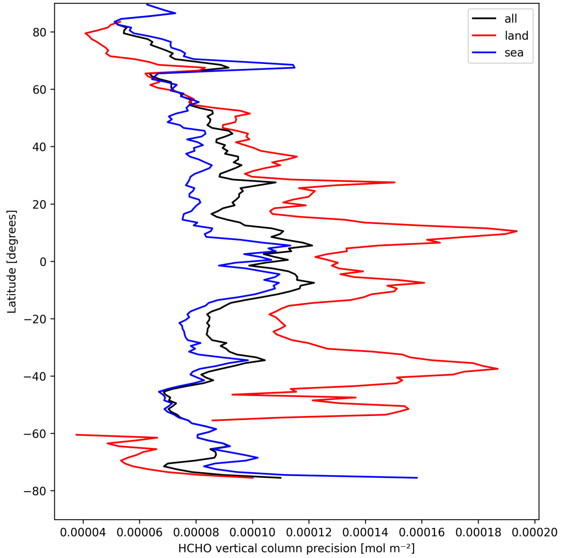
Figure 20: Zonal average of “HCHO vertical column precision” for 2025-04-13 to 2025-04-14.
