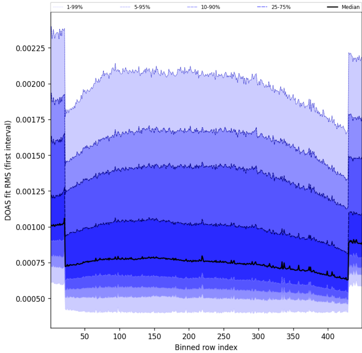
Figure 58: Along track statistics of “DOAS fit RMS (first interval)” for 2025-04-14 to 2025-04-15
