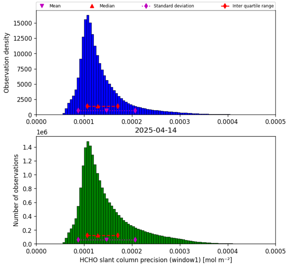
Figure 37: Histogram of “HCHO slant column precision (window1)” for 2025-04-14 to 2025-04-15
