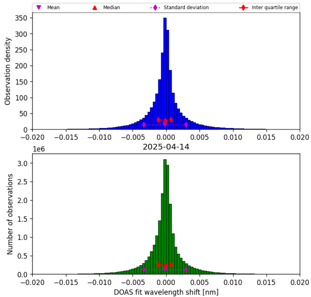
Figure 42: Histogram of “DOAS fit wavelength shift” for 2025-04-14 to 2025-04-15
