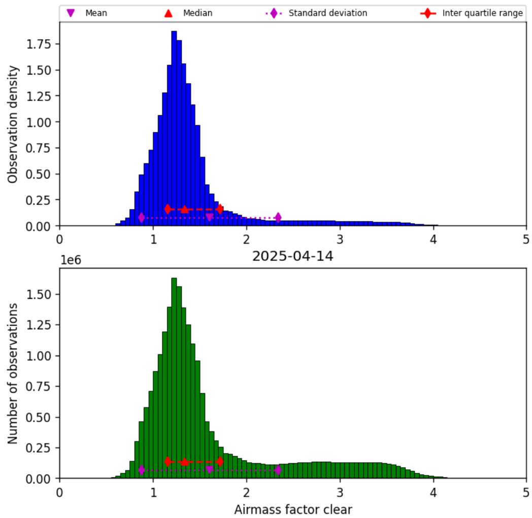
Figure 40: Histogram of “Airmass factor clear” for 2025-04-14 to 2025-04-15
