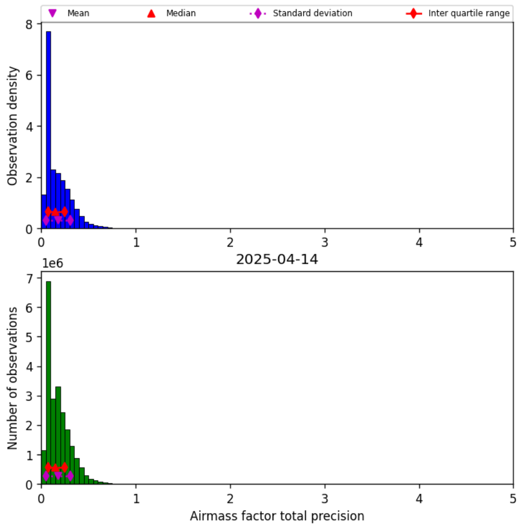
Figure 39: Histogram of “Airmass factor total precision” for 2025-04-14 to 2025-04-15
