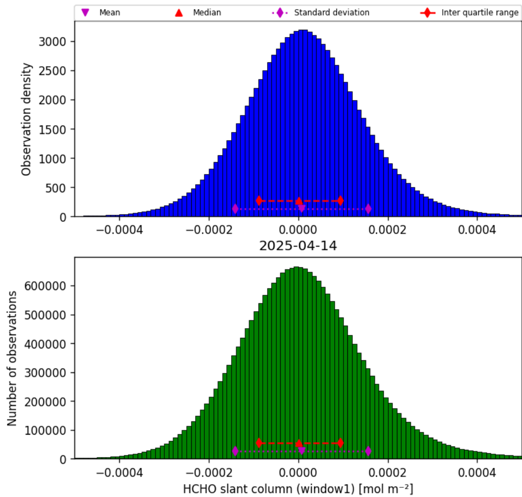
Figure 36: Histogram of “HCHO slant column (window1)” for 2025-04-14 to 2025-04-15
