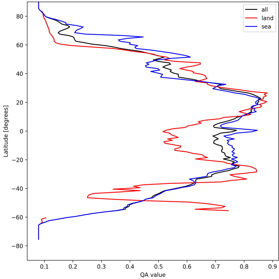
Figure 18: Zonal average of “QA value” for 2025-04-14 to 2025-04-15.
