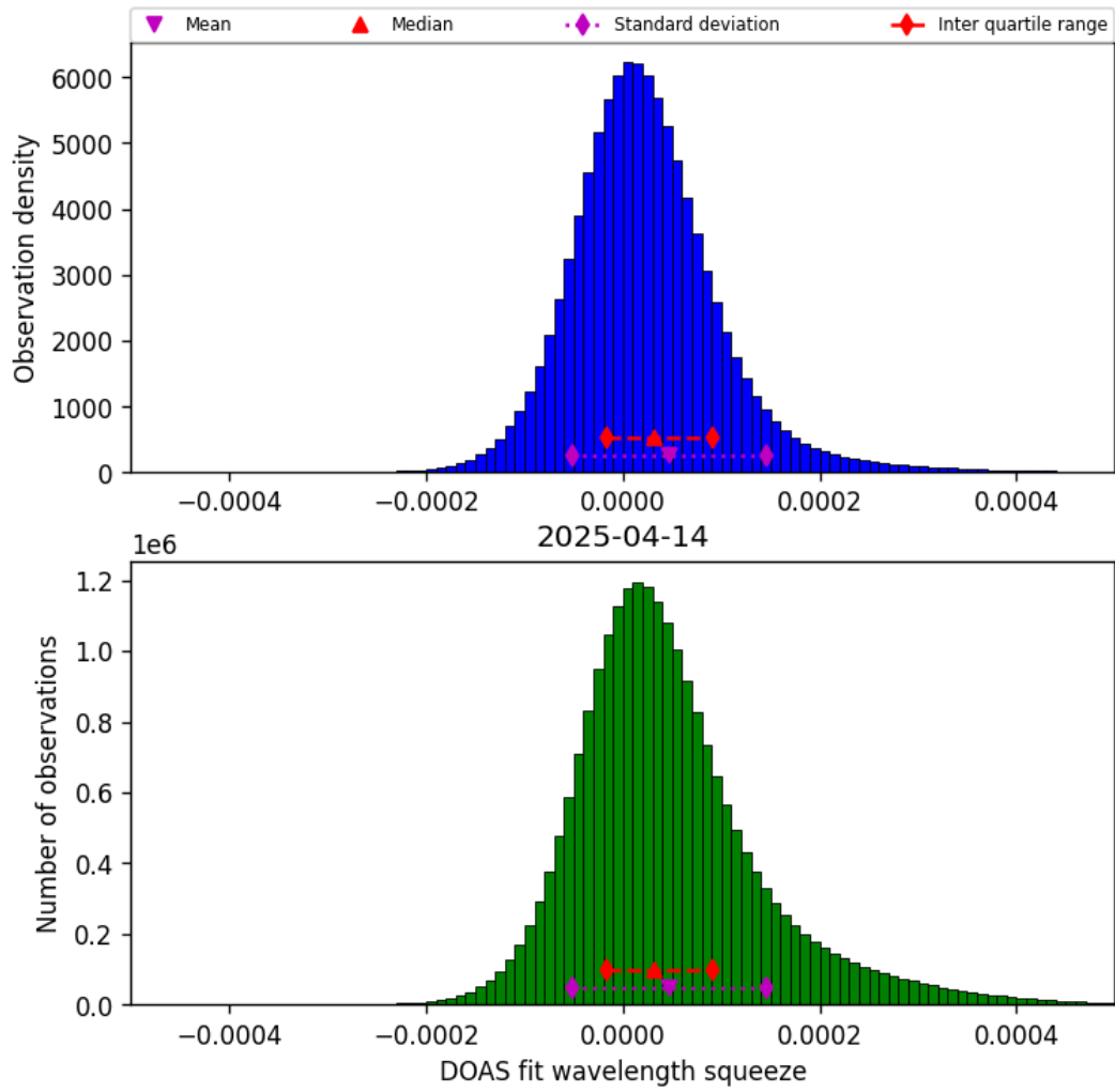
Figure 43: Histogram of “DOAS fit wavelength squeeze” for 2025-04-14 to 2025-04-15
