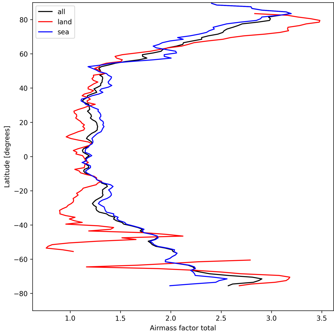
Figure 24: Zonal average of “Airmass factor total” for 2025-04-14 to 2025-04-15.
