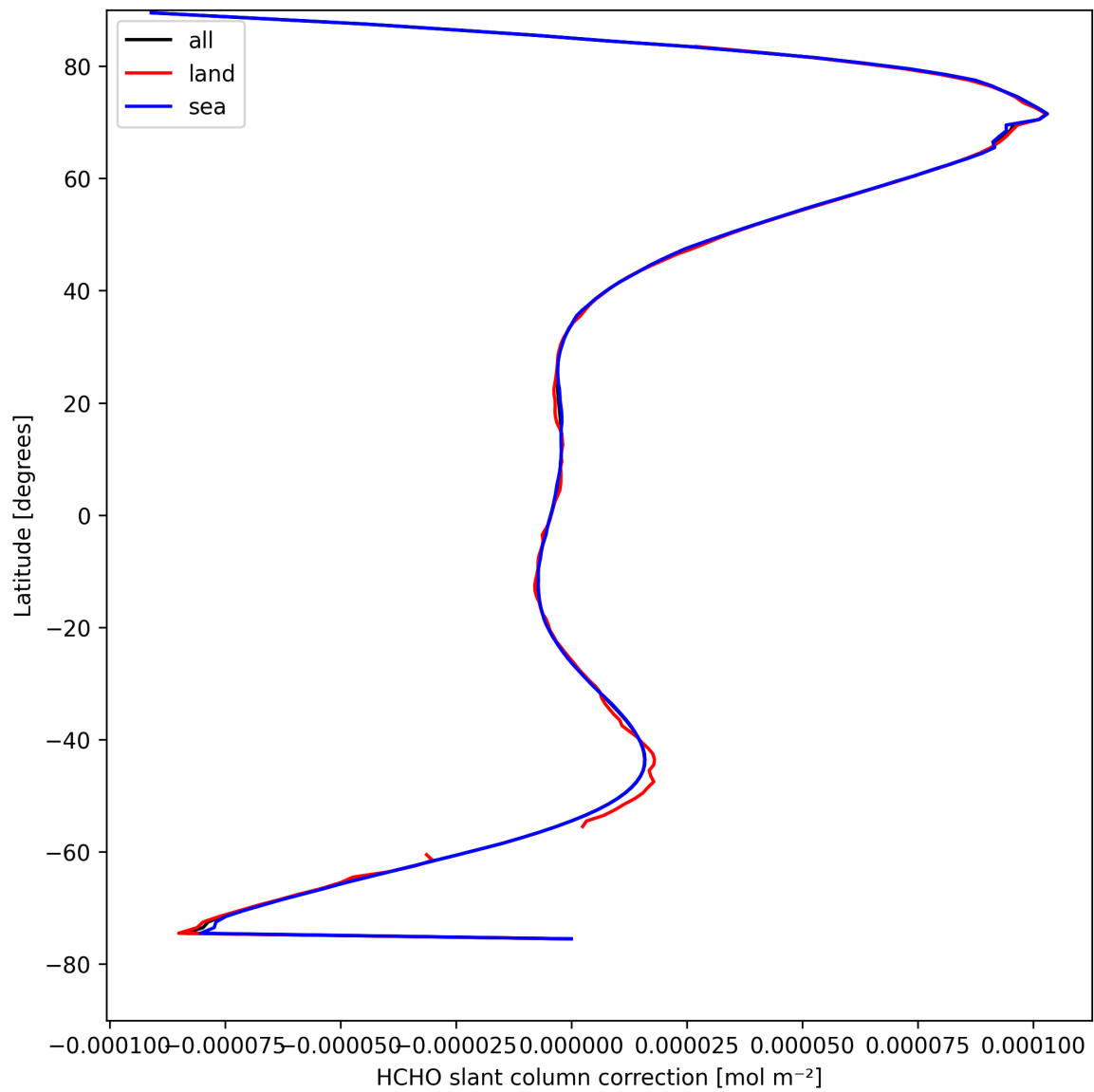
Figure 31: Zonal average of “HCHO slant column correction” for 2025-04-14 to 2025-04-15.
