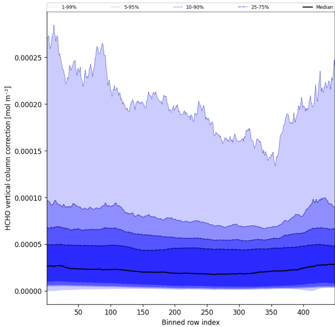
Figure 49: Along track statistics of “HCHO vertical column correction” for 2025-04-14 to 2025-04-15
