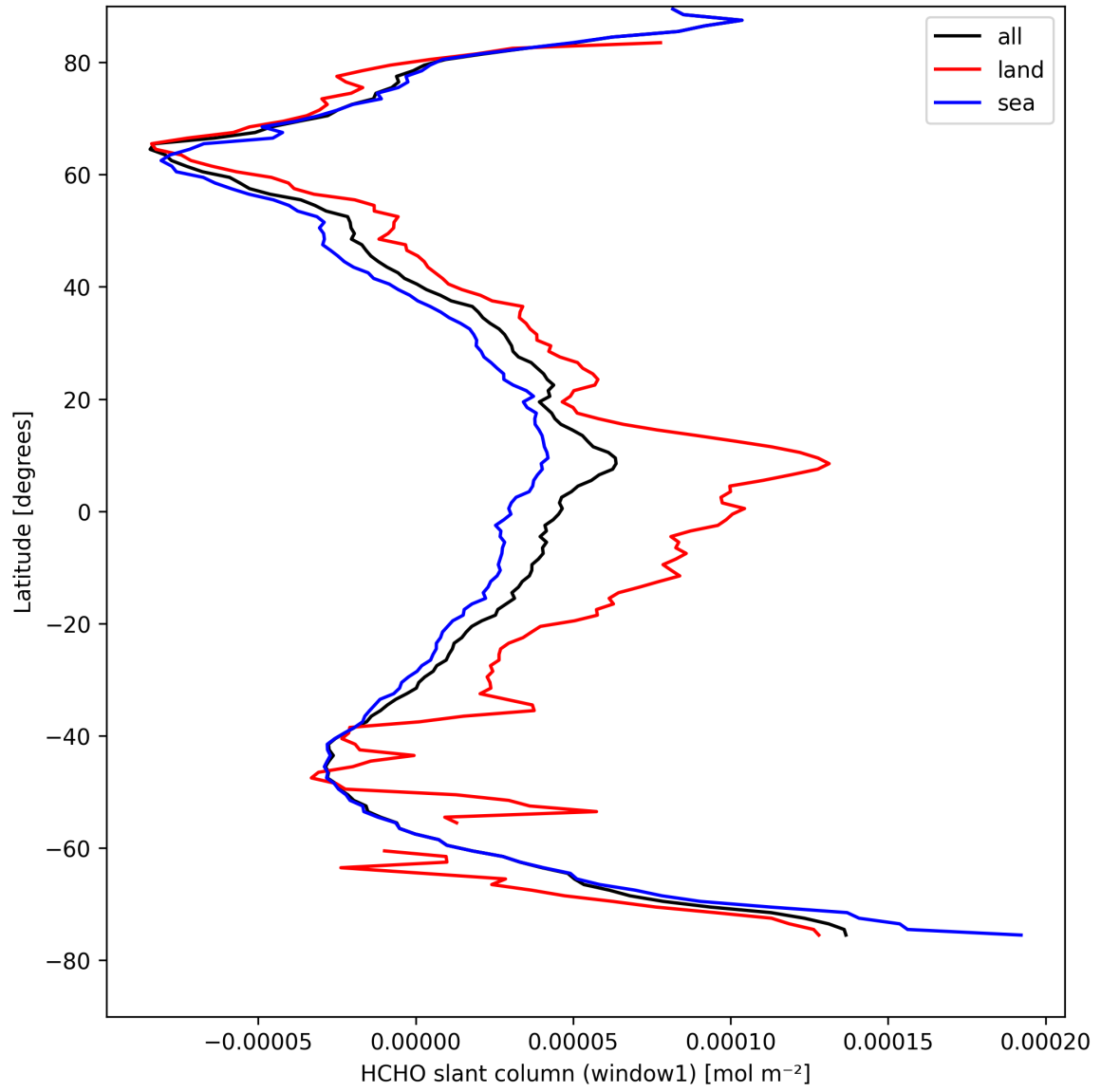
Figure 22: Zonal average of “HCHO slant column (window1)” for 2025-04-14 to 2025-04-15.
