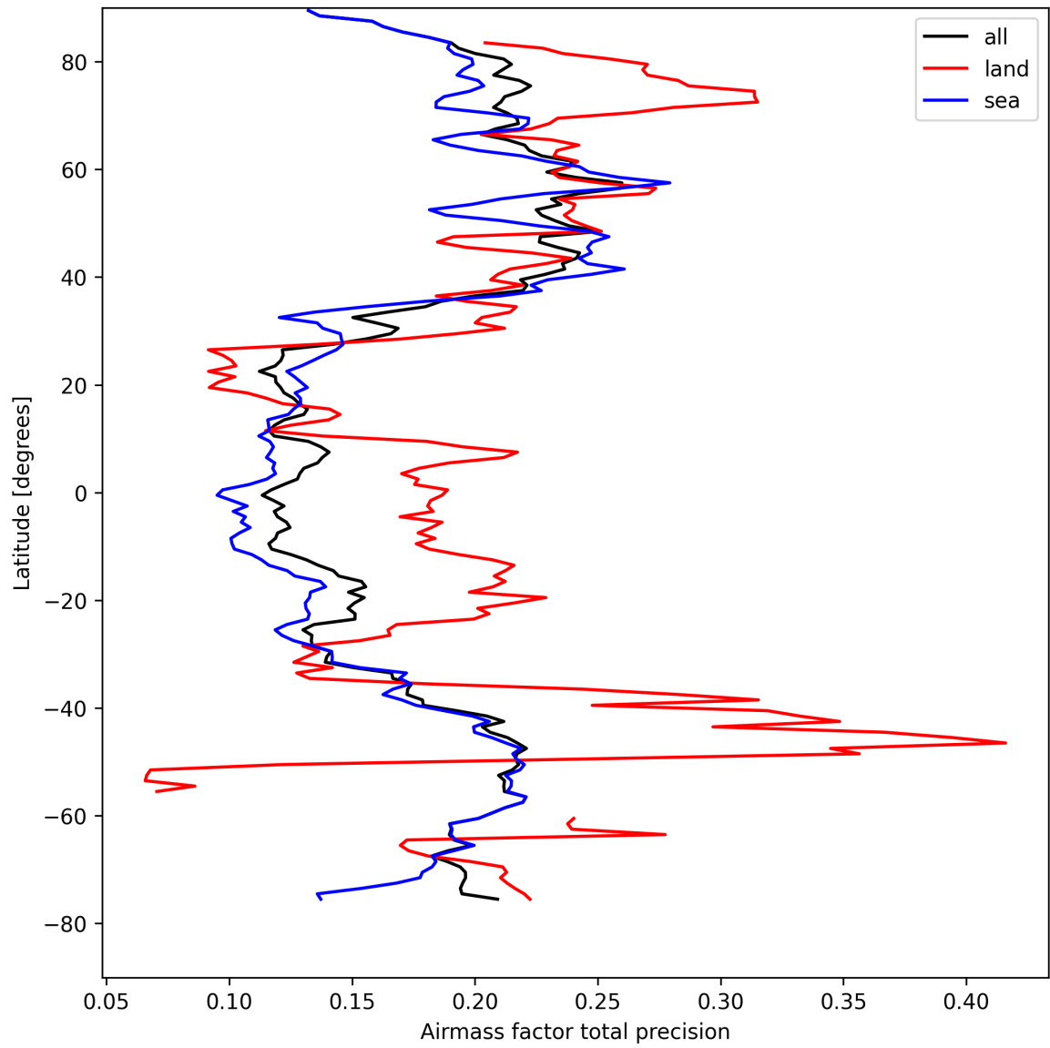
Figure 25: Zonal average of “Airmass factor total precision” for 2025-04-14 to 2025-04-15.
