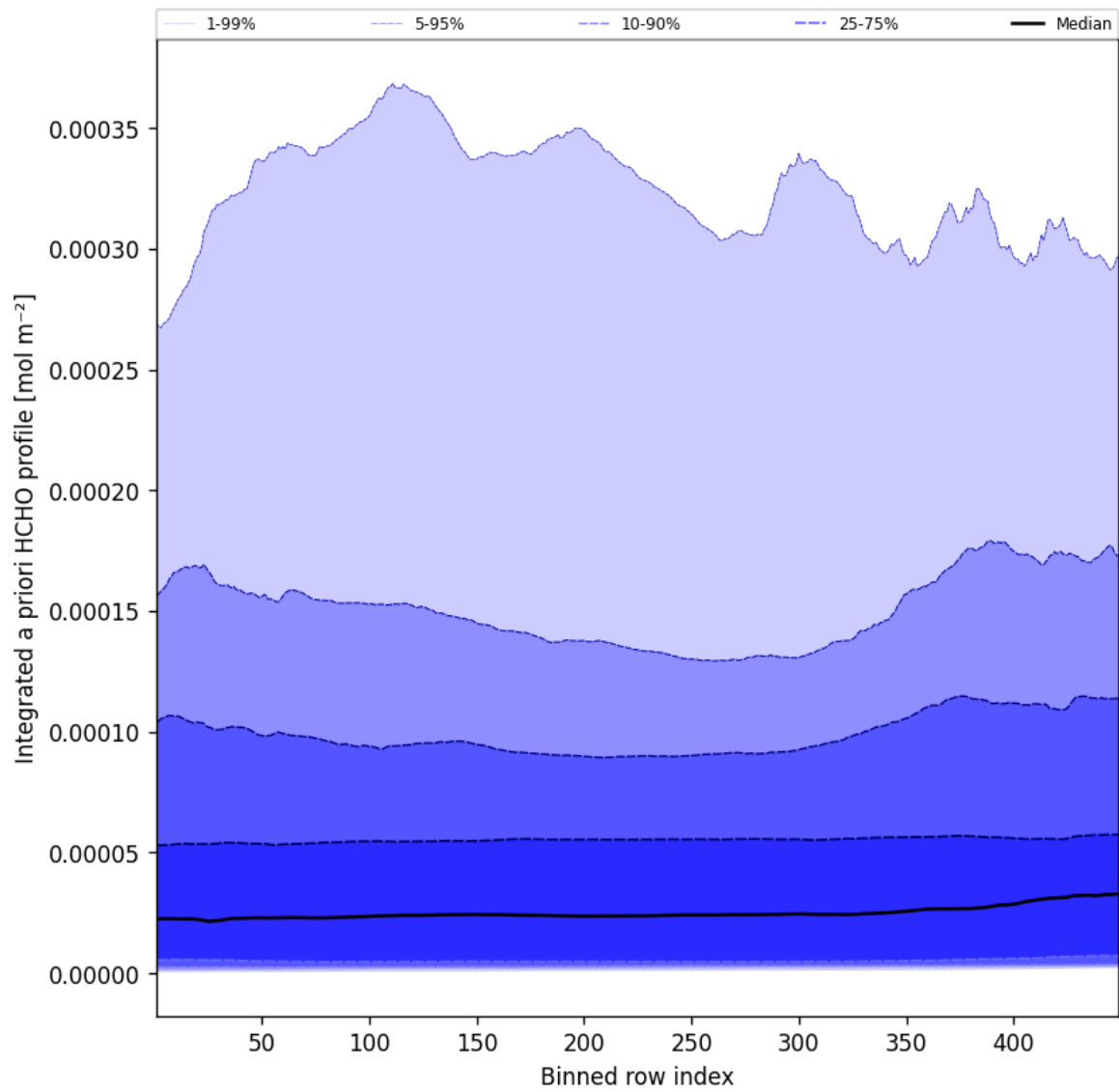
Figure 55: Along track statistics of "Integrated a priori HCHO profile" for 2025-04-14 to 2025-04-15
