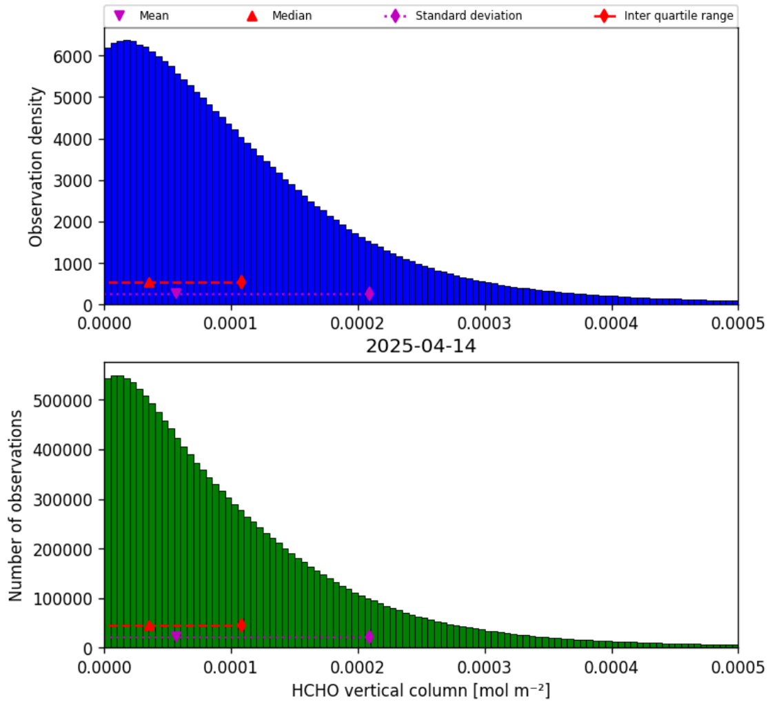
Figure 33: Histogram of “HCHO vertical column” for 2025-04-14 to 2025-04-15
