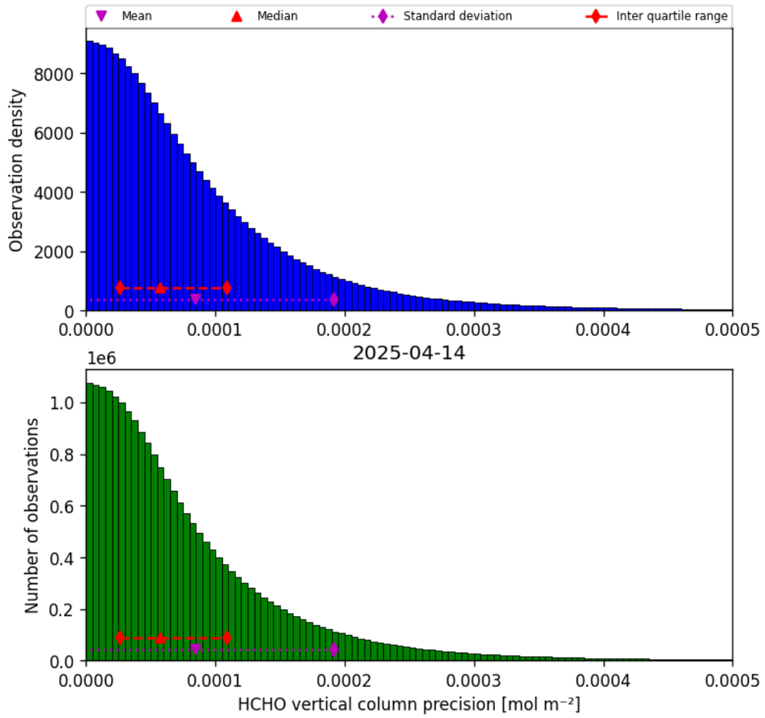
Figure 34: Histogram of “HCHO vertical column precision” for 2025-04-14 to 2025-04-15
