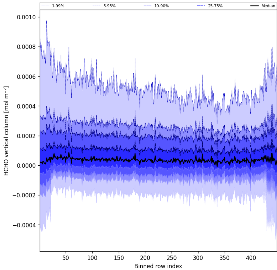
Figure 47: Along track statistics of “HCHO vertical column” for 2025-04-14 to 2025-04-15
