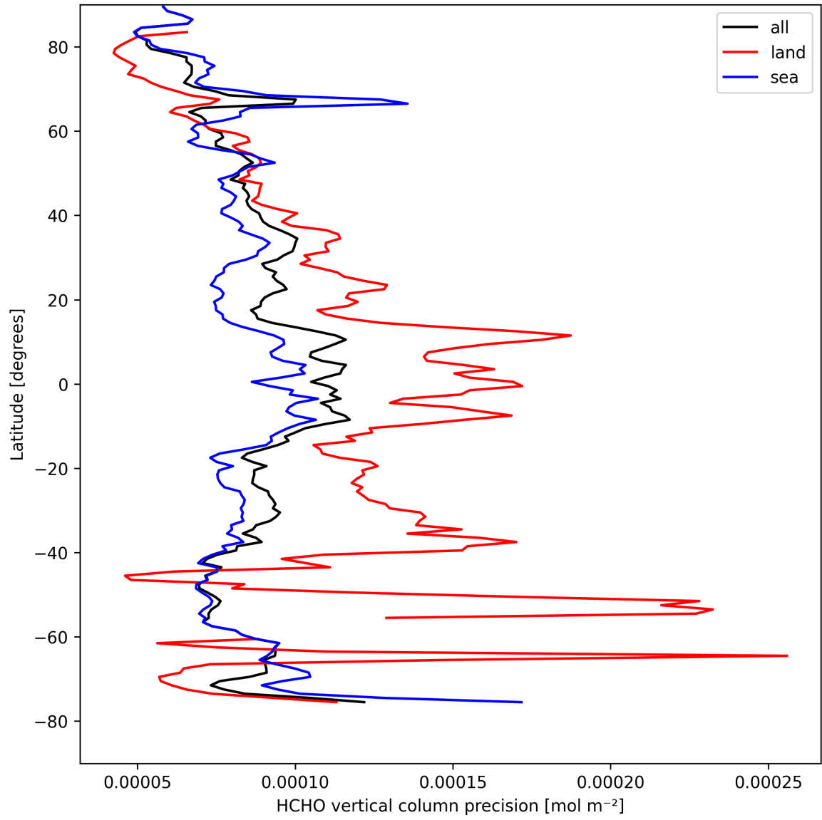
Figure 20: Zonal average of “HCHO vertical column precision” for 2025-04-14 to 2025-04-15.
