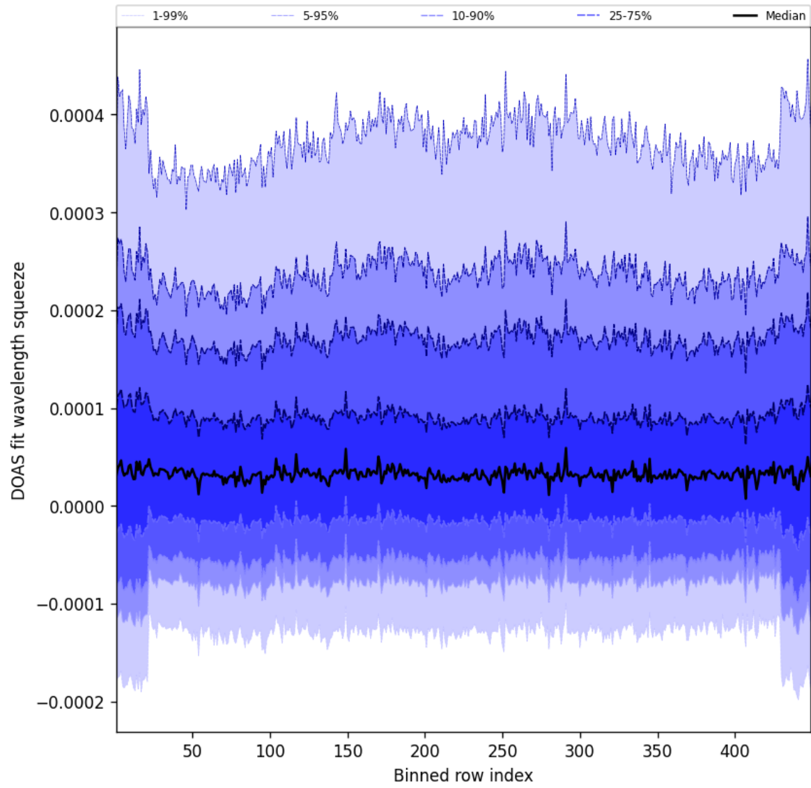
Figure 57: Along track statistics of “DOAS fit wavelength squeeze” for 2025-04-14 to 2025-04-15
