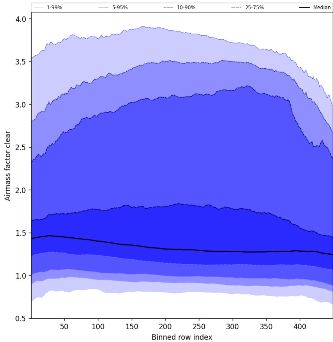
Figure 54: Along track statistics of “Airmass factor clear” for 2025-04-14 to 2025-04-15
