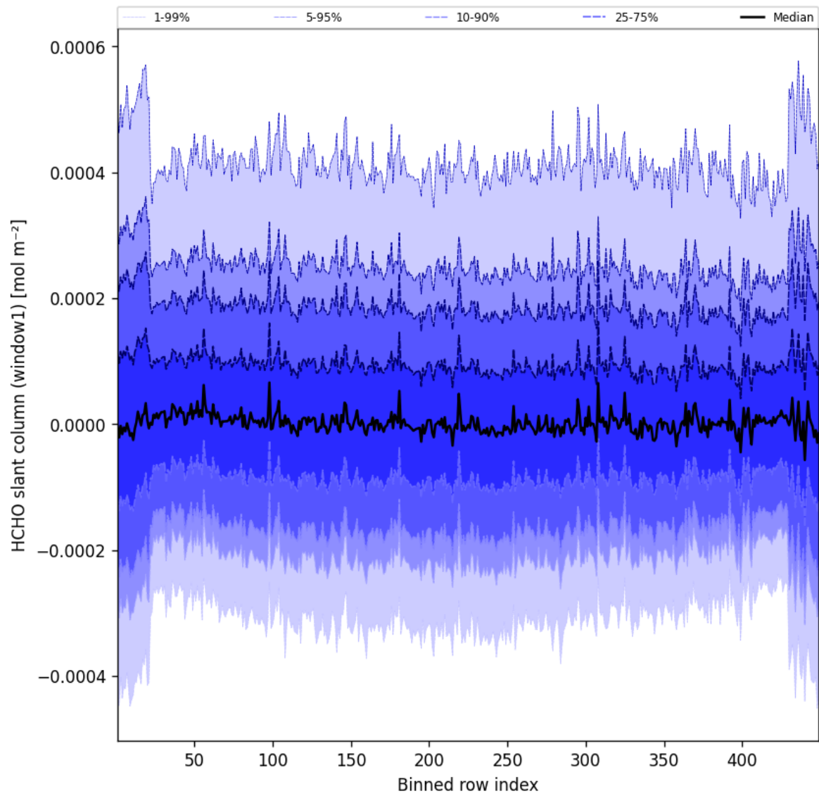
Figure 50: Along track statistics of “HCHO slant column (window1)” for 2025-04-14 to 2025-04-15
