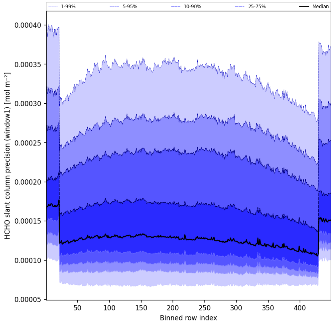
Figure 51: Along track statistics of “HCHO slant column precision (window1)” for 2025-04-14 to 2025-04-15
