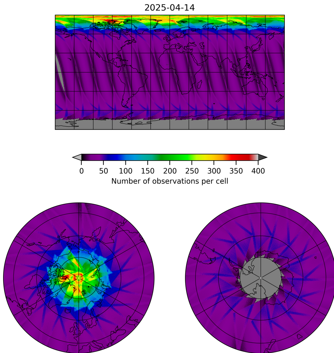
Figure 17: Map of the number of observations for 2025-04-14 to 2025-04-15
