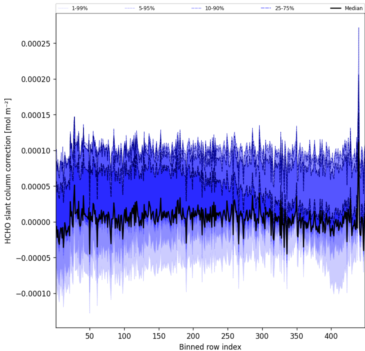
Figure 59: Along track statistics of “HCHO slant column correction” for 2025-04-14 to 2025-04-15
