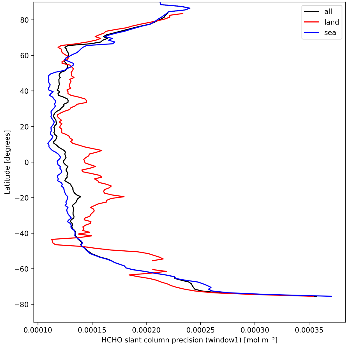
Figure 23: Zonal average of “HCHO slant column precision (window1)” for 2025-04-14 to 2025-04-15.
