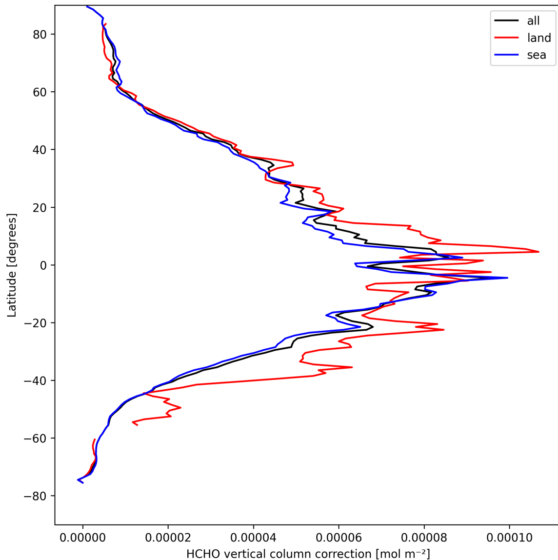
Figure 21: Zonal average of “HCHO vertical column correction” for 2025-04-15 to 2025-04-16.
