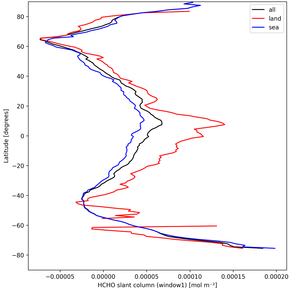
Figure 22: Zonal average of “HCHO slant column (window1)” for 2025-04-15 to 2025-04-16.
