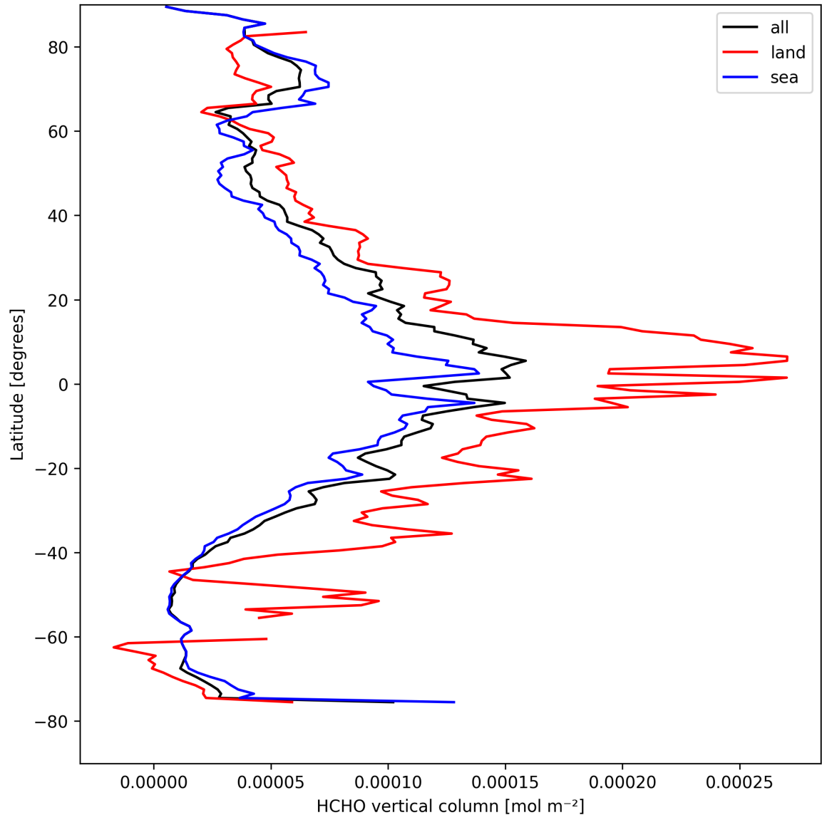
Figure 19: Zonal average of “HCHO vertical column” for 2025-04-15 to 2025-04-16.
