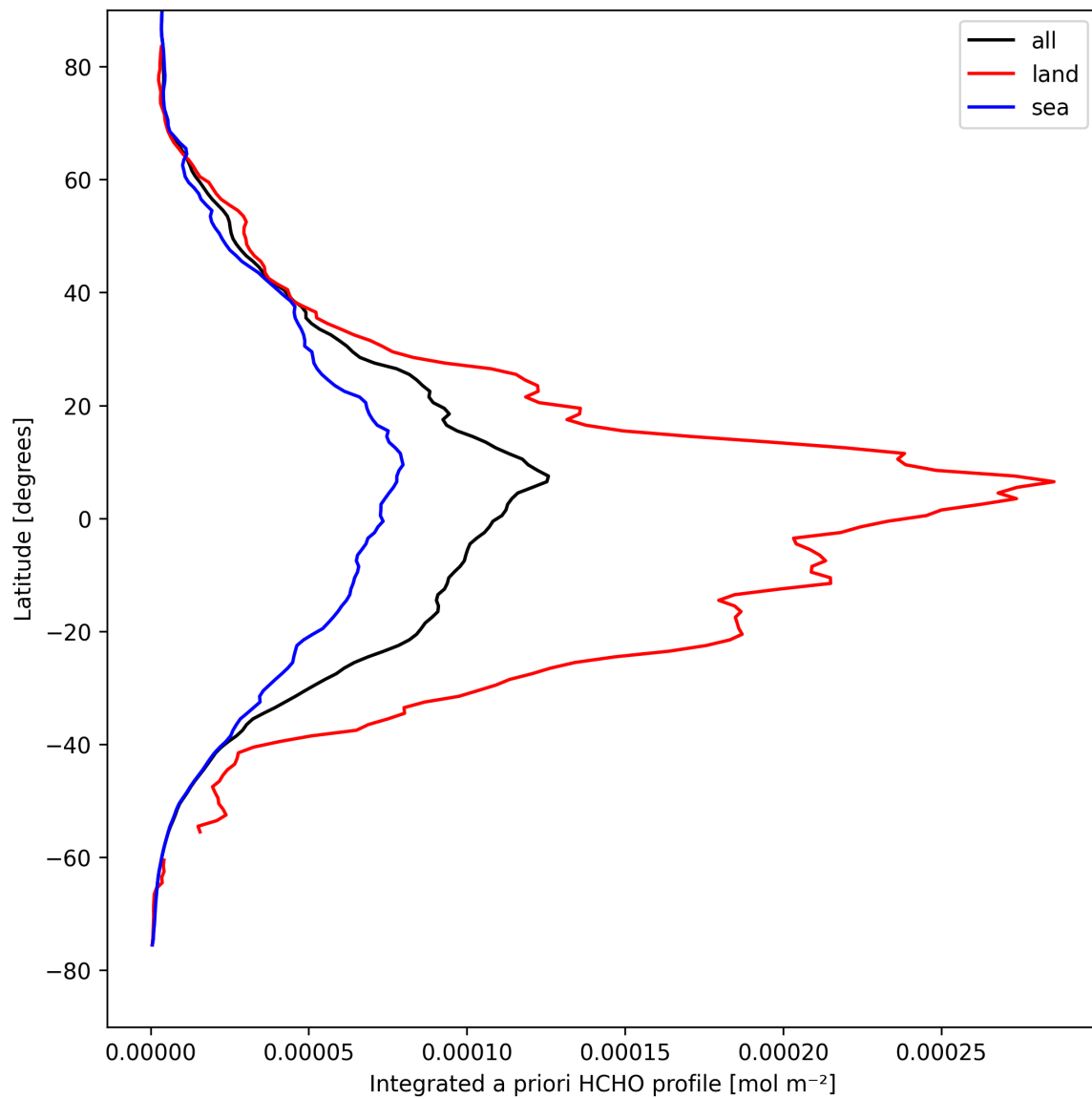
Figure 27: Zonal average of “Integrated a priori HCHO profile” for 2025-04-15 to 2025-04-16.
