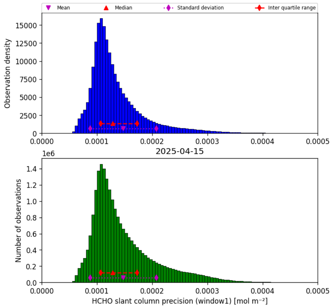
Figure 37: Histogram of “HCHO slant column precision (window1)” for 2025-04-15 to 2025-04-16
