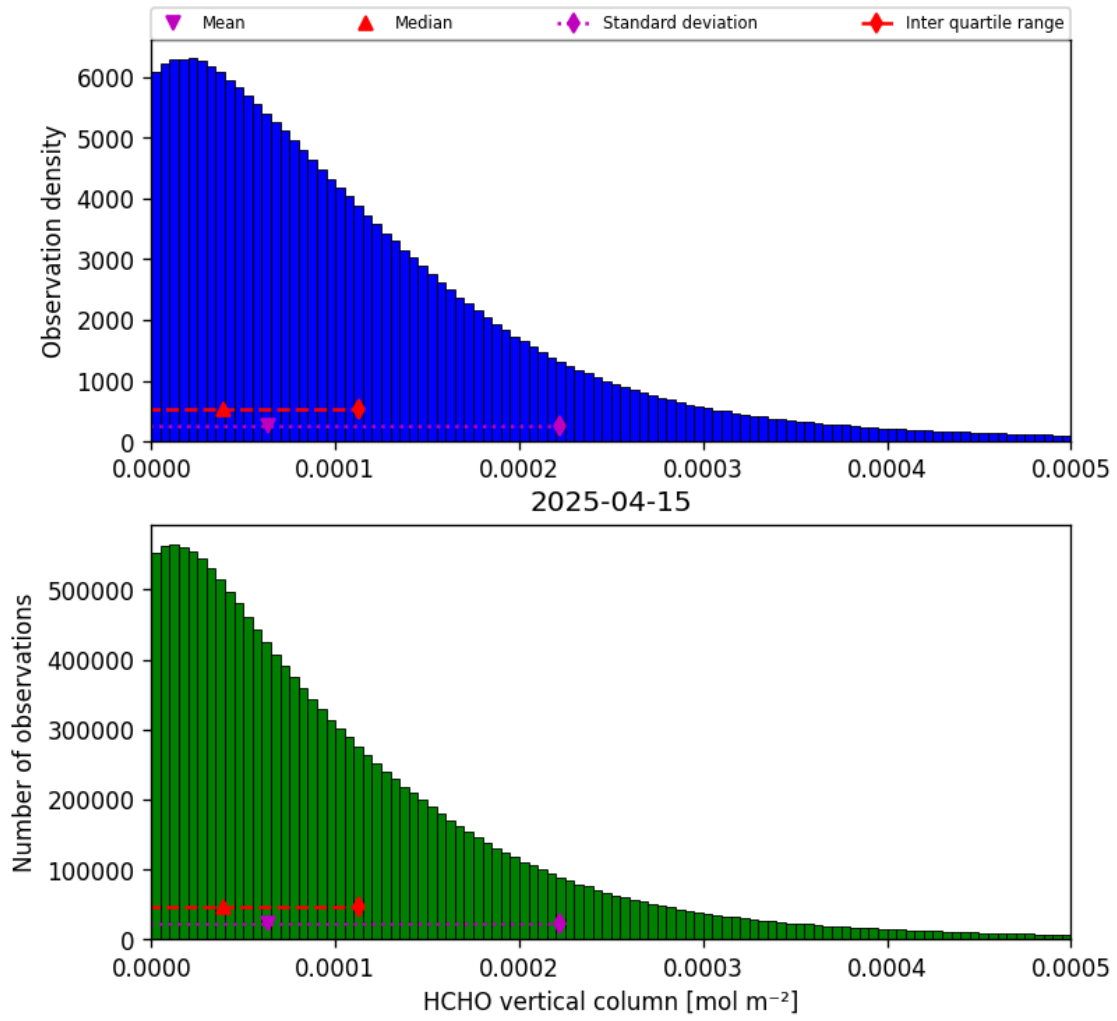
Figure 33: Histogram of “HCHO vertical column” for 2025-04-15 to 2025-04-16
