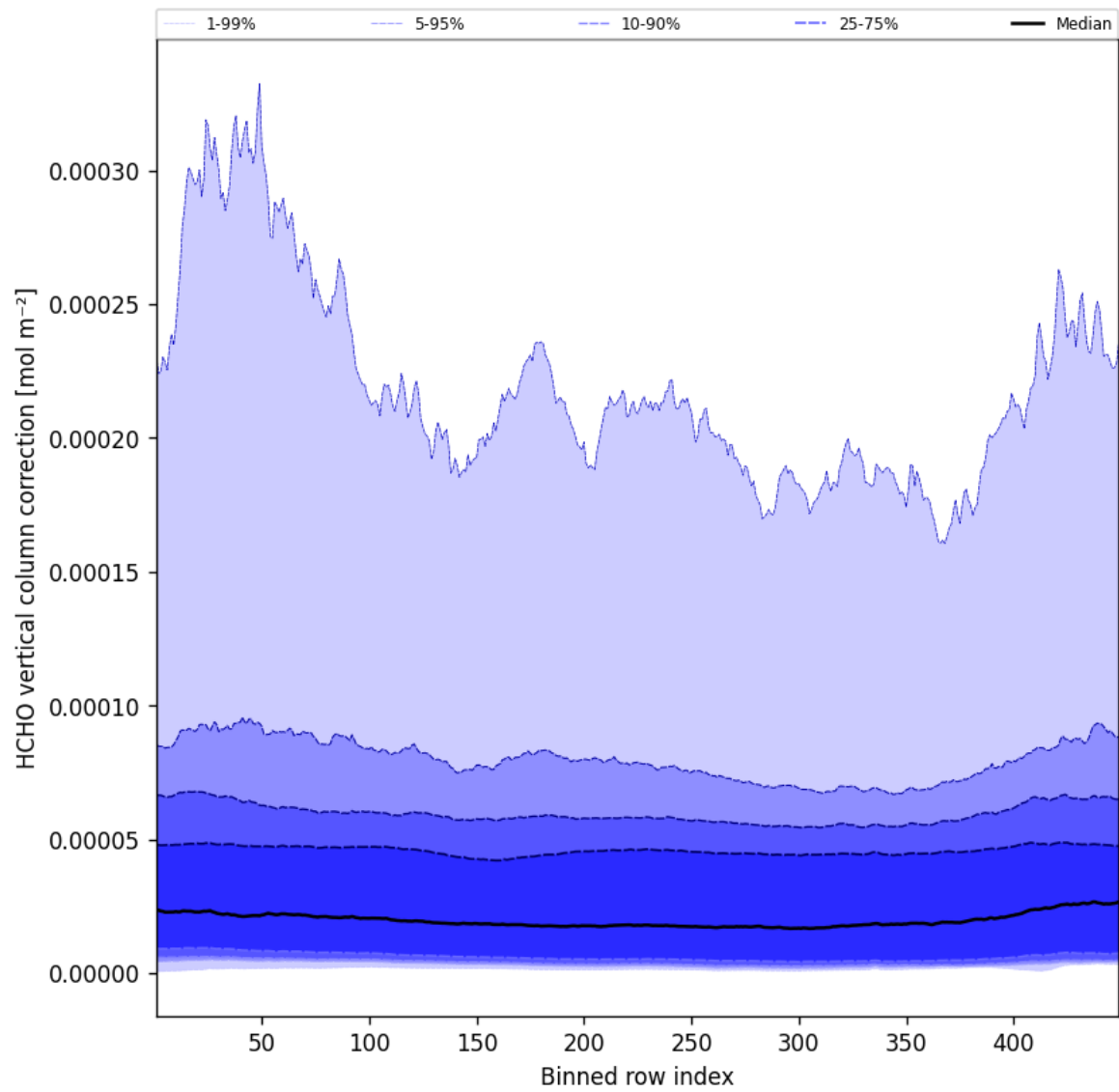
Figure 49: Along track statistics of “HCHO vertical column correction” for 2025-04-15 to 2025-04-16
