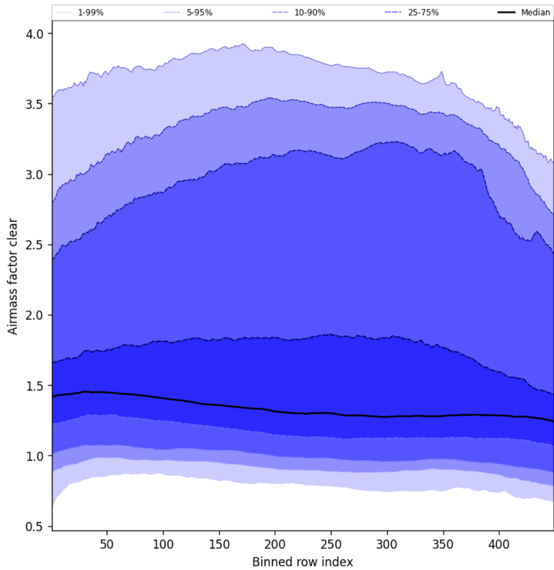
Figure 54: Along track statistics of “Airmass factor clear” for 2025-04-15 to 2025-04-16
