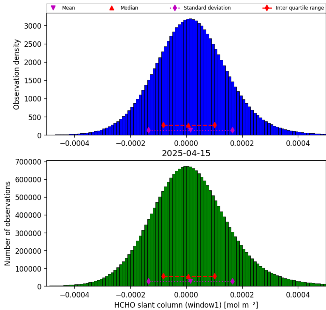
Figure 36: Histogram of “HCHO slant column (window1)” for 2025-04-15 to 2025-04-16
