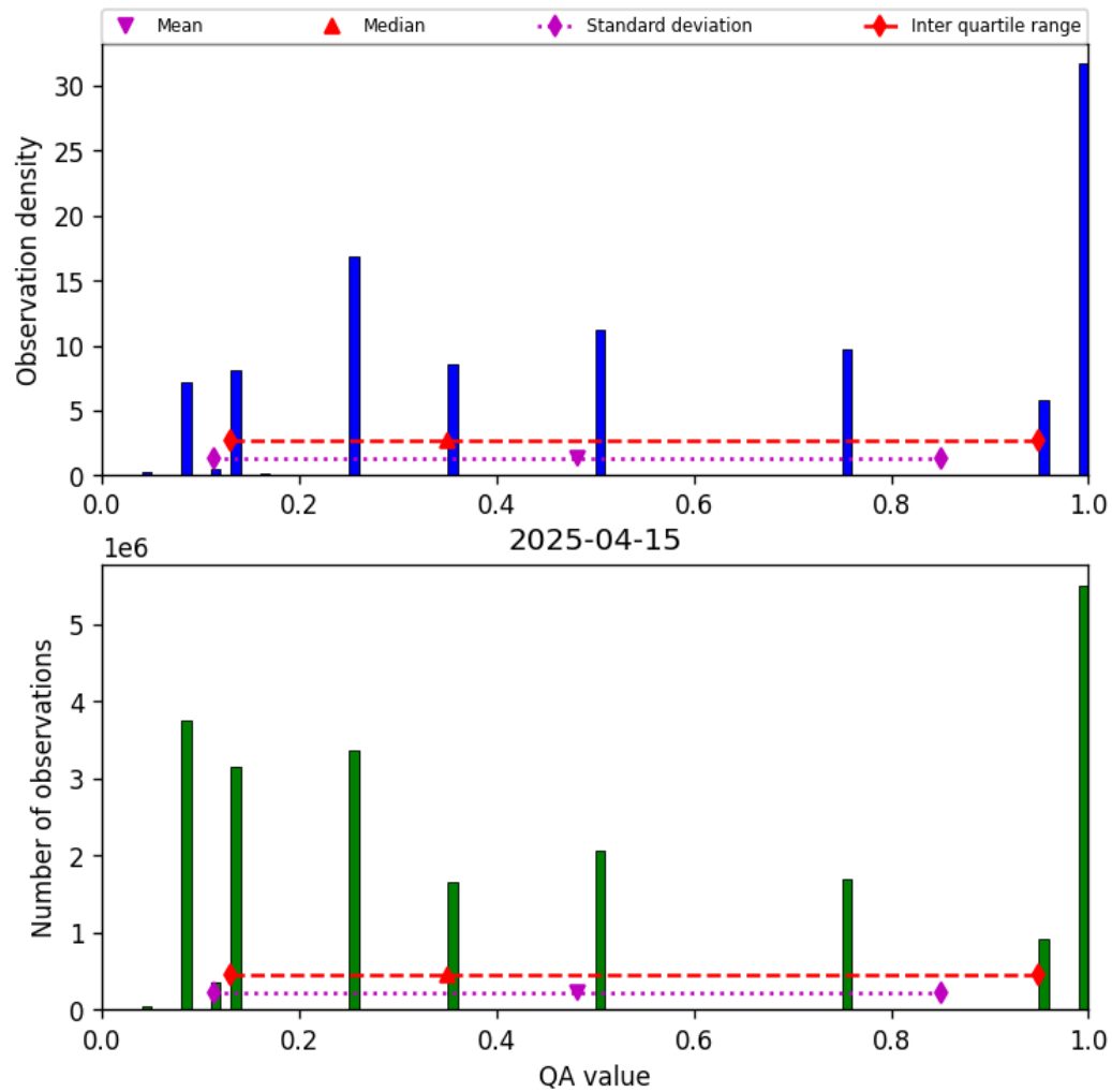
Figure 32: Histogram of “QA value” for 2025-04-15 to 2025-04-16
