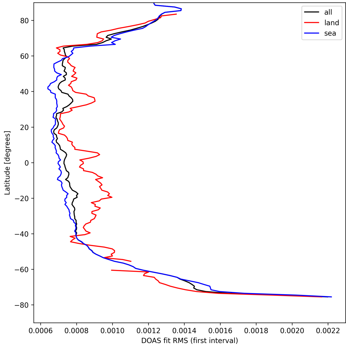
Figure 30: Zonal average of "DOAS fit RMS (first interval)" for 2025-04-15 to 2025-04-16.
