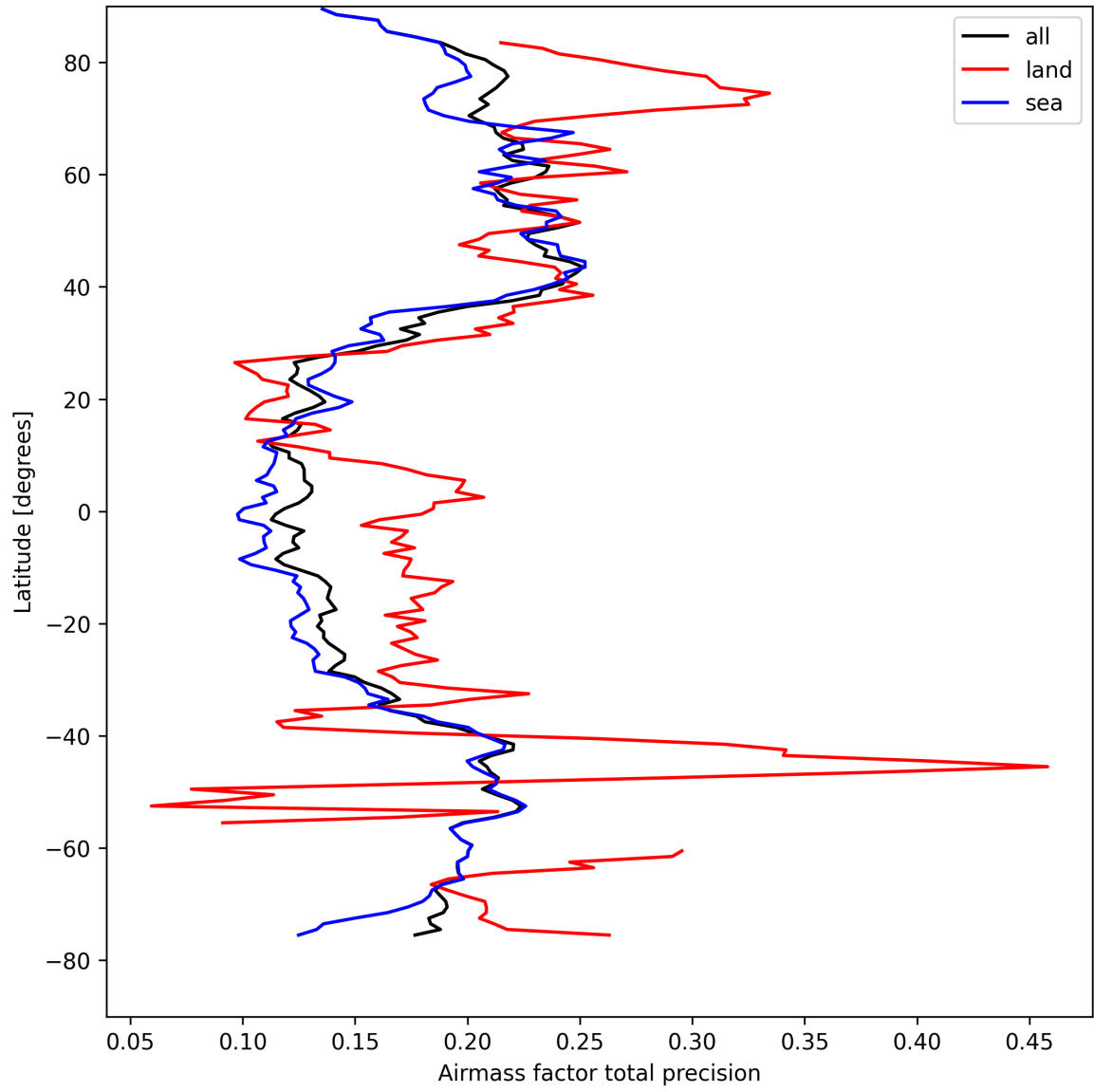
Figure 25: Zonal average of “Airmass factor total precision” for 2025-04-15 to 2025-04-16.
