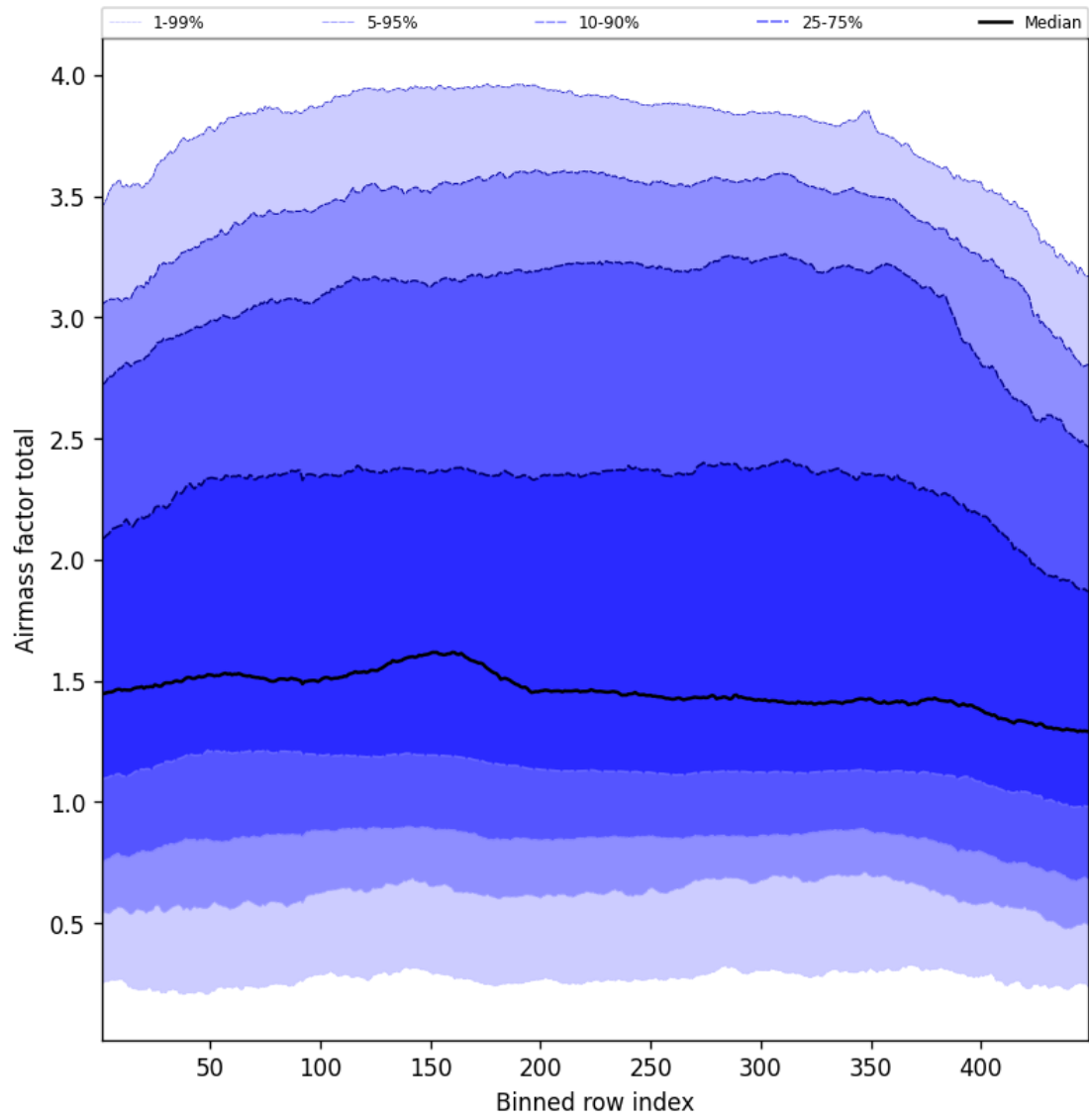
Figure 52: Along track statistics of “Airmass factor total” for 2025-04-15 to 2025-04-16
