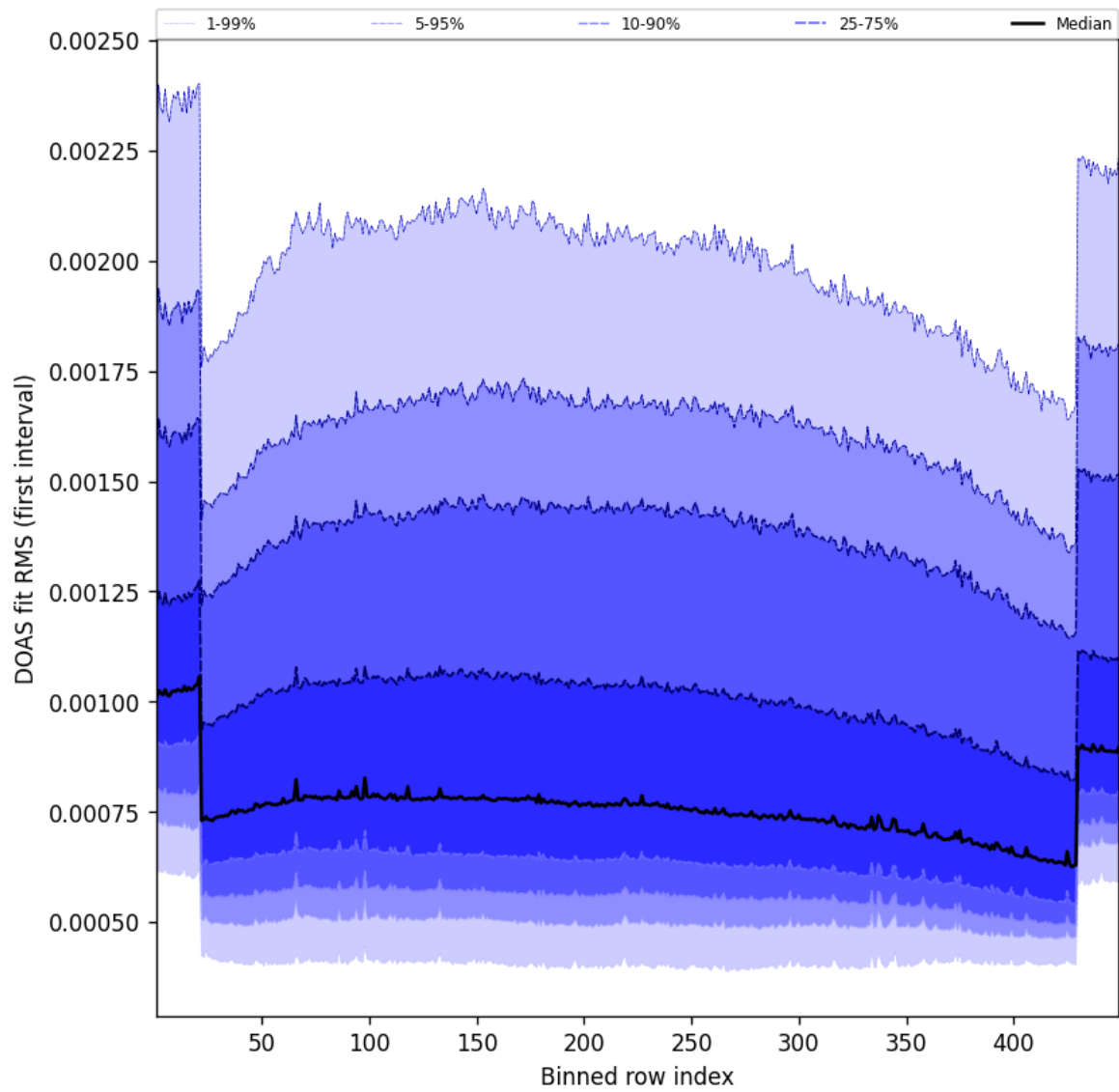
Figure 58: Along track statistics of “DOAS fit RMS (first interval)” for 2025-04-15 to 2025-04-16
