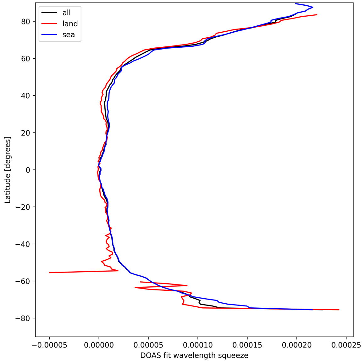
Figure 29: Zonal average of “DOAS fit wavelength squeeze” for 2025-04-15 to 2025-04-16.
