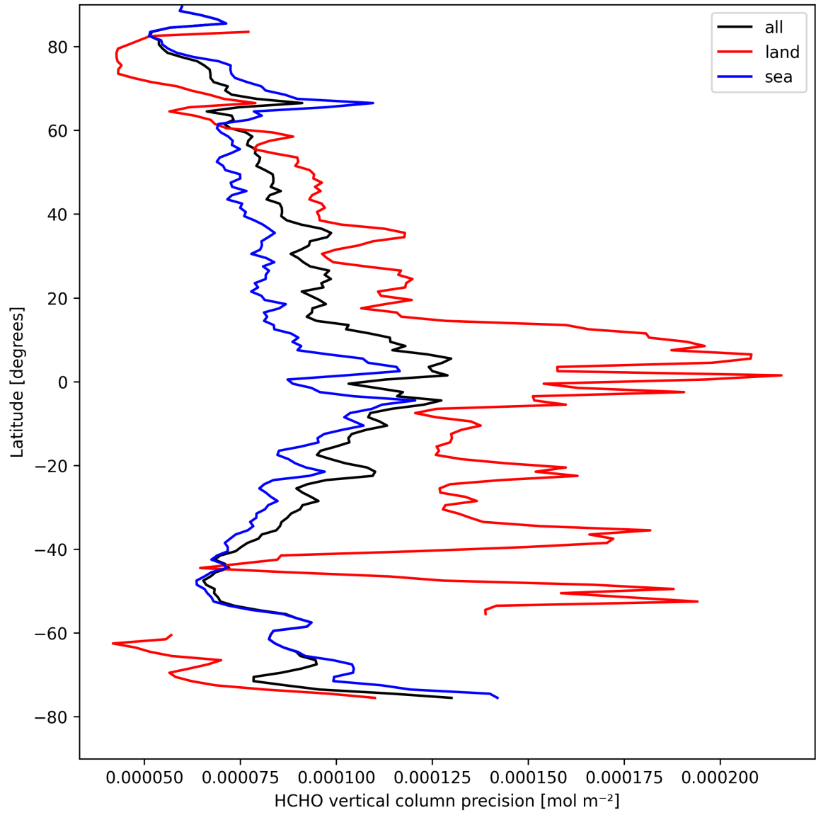
Figure 20: Zonal average of “HCHO vertical column precision” for 2025-04-15 to 2025-04-16.
