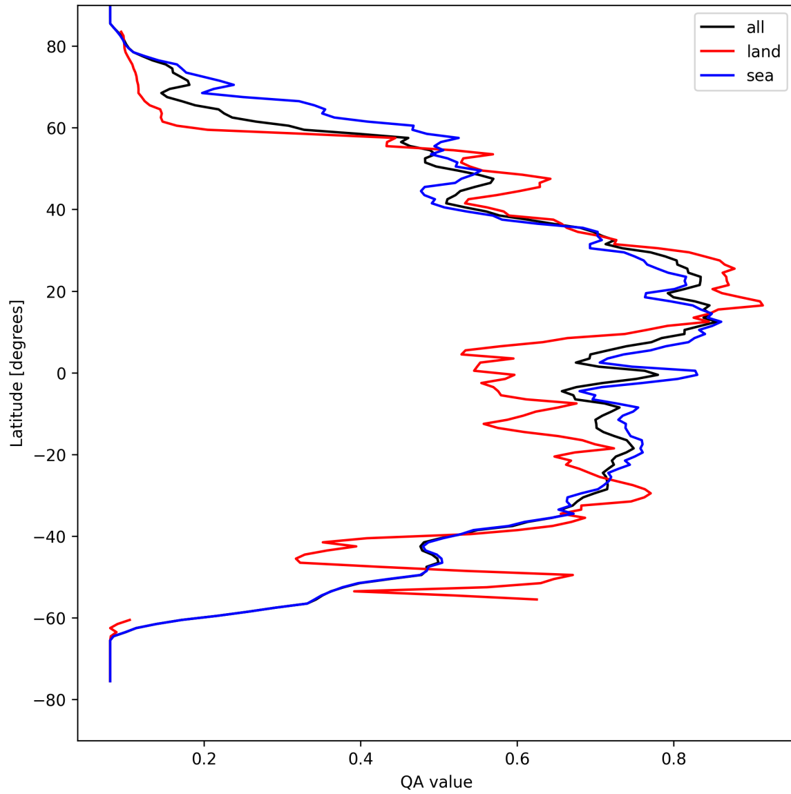
Figure 18: Zonal average of “QA value” for 2025-04-15 to 2025-04-16.
