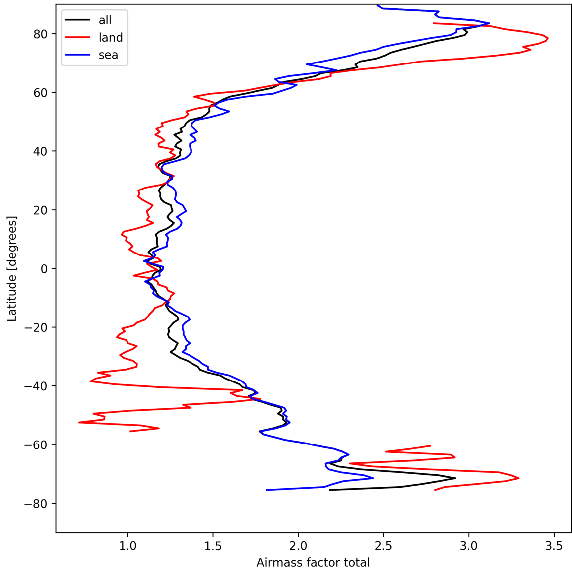
Figure 24: Zonal average of “Airmass factor total” for 2025-04-15 to 2025-04-16.
