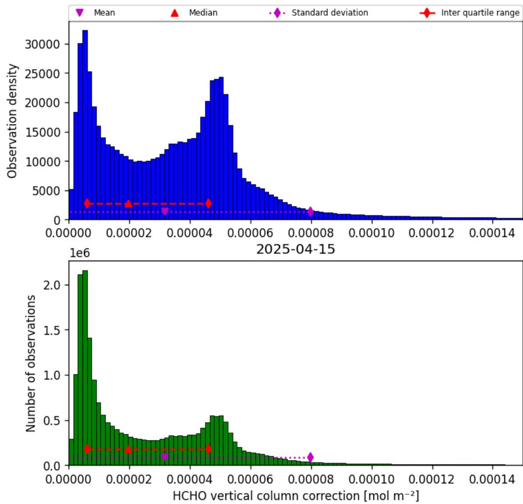
Figure 35: Histogram of “HCHO vertical column correction” for 2025-04-15 to 2025-04-16
