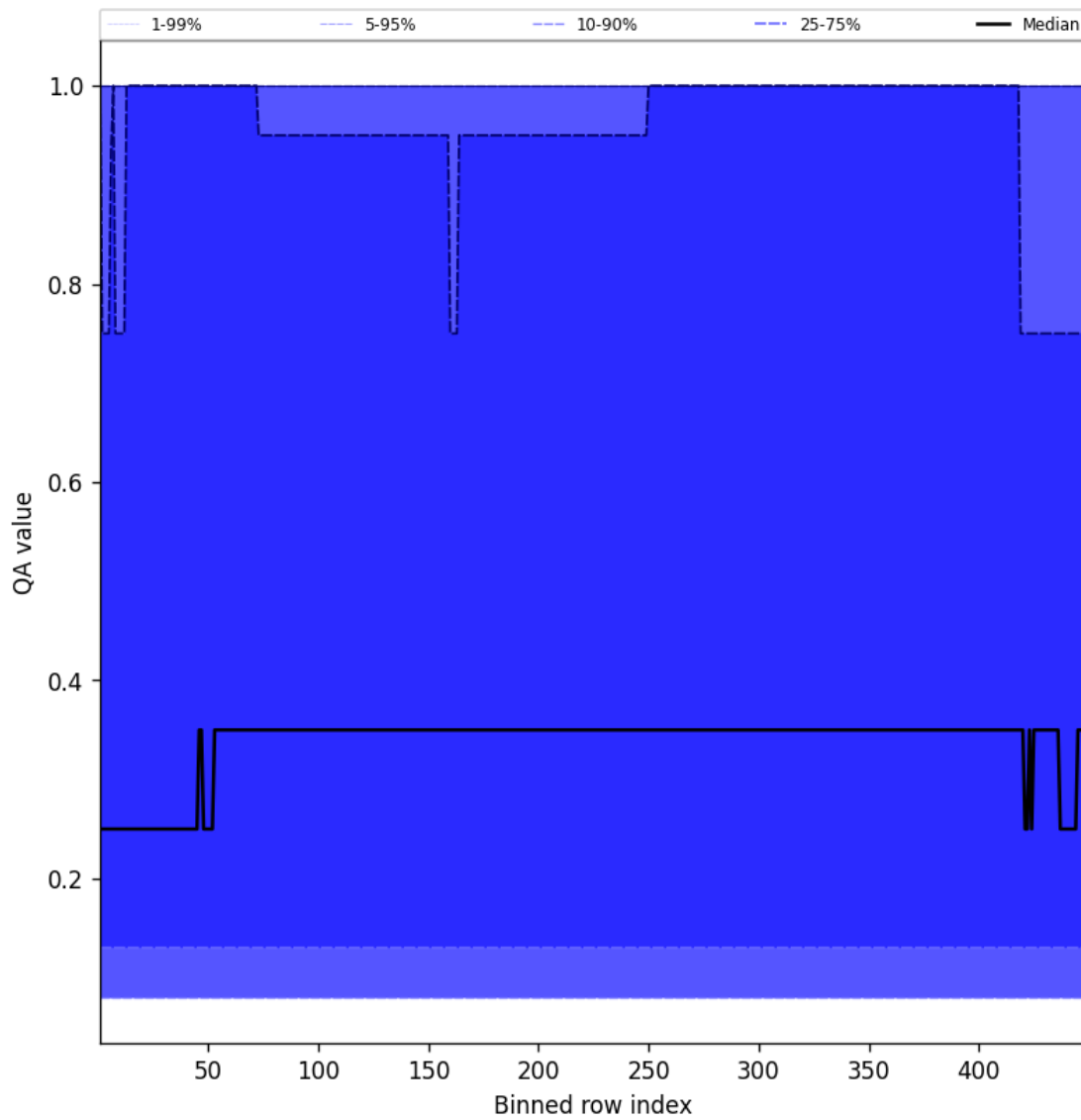
Figure 46: Along track statistics of “QA value” for 2025-04-15 to 2025-04-16
