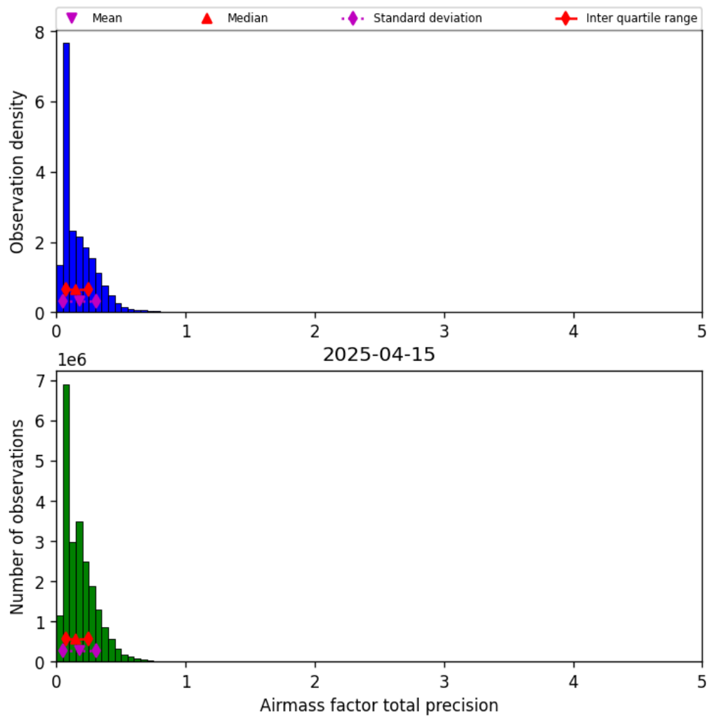
Figure 39: Histogram of “Airmass factor total precision” for 2025-04-15 to 2025-04-16
