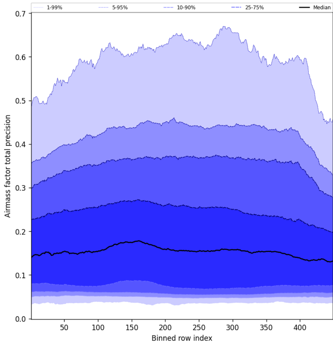
Figure 53: Along track statistics of “Airmass factor total precision” for 2025-04-15 to 2025-04-16
