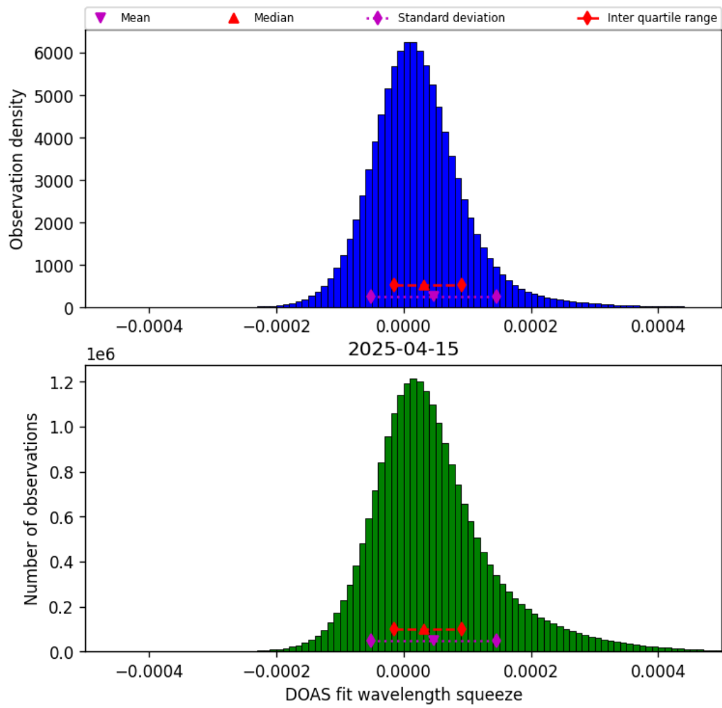
Figure 43: Histogram of “DOAS fit wavelength squeeze” for 2025-04-15 to 2025-04-16
