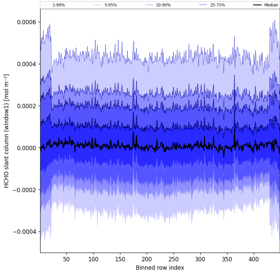
Figure 50: Along track statistics of “HCHO slant column (window1)” for 2025-04-15 to 2025-04-16
