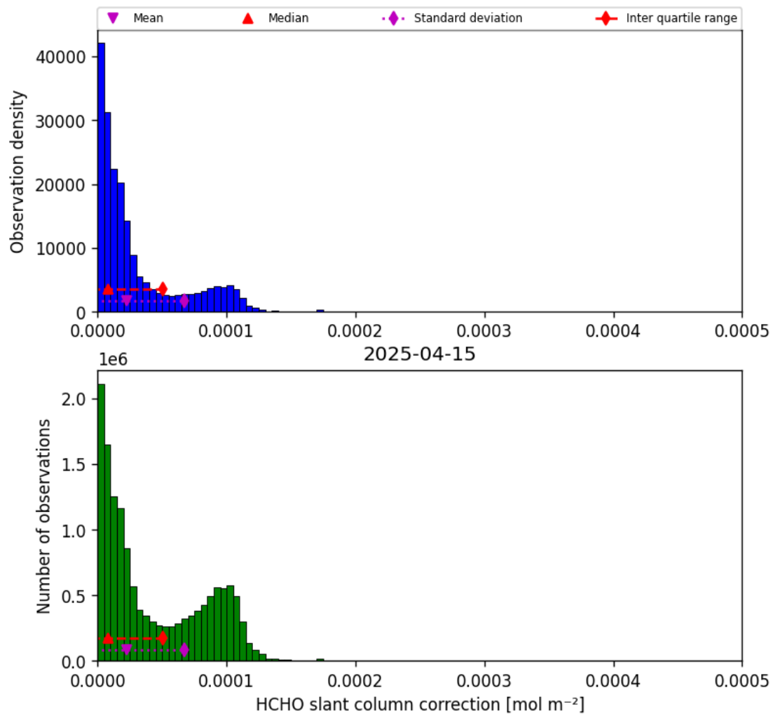
Figure 45: Histogram of “HCHO slant column correction” for 2025-04-15 to 2025-04-16
