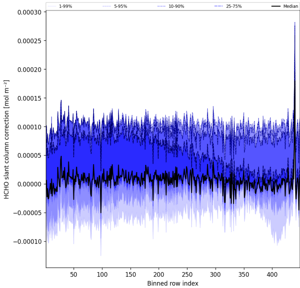
Figure 59: Along track statistics of “HCHO slant column correction” for 2025-04-15 to 2025-04-16
