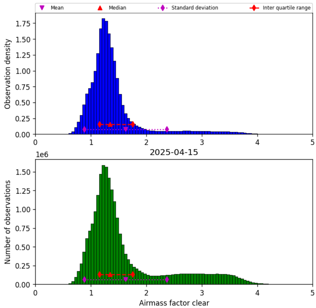
Figure 40: Histogram of “Airmass factor clear” for 2025-04-15 to 2025-04-16
