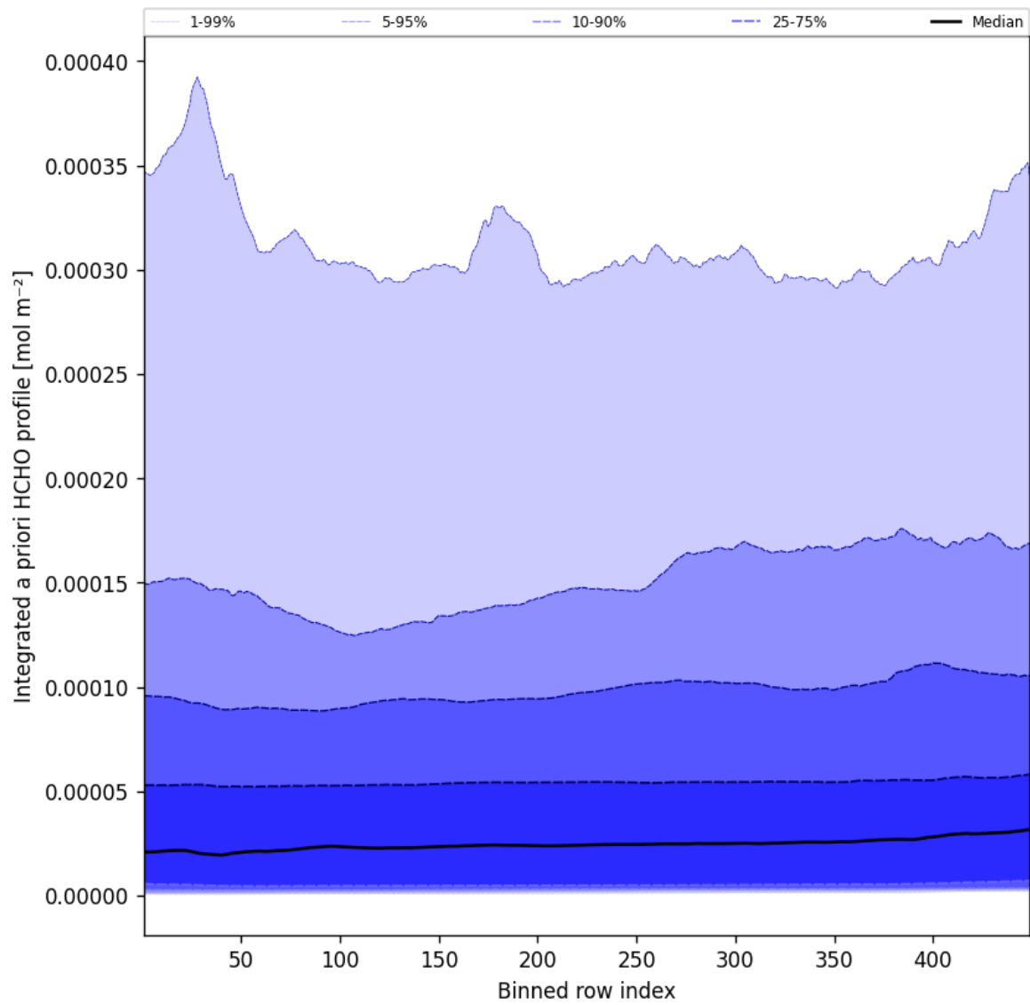
Figure 55: Along track statistics of “Integrated a priori HCHO profile” for 2025-04-15 to 2025-04-16
