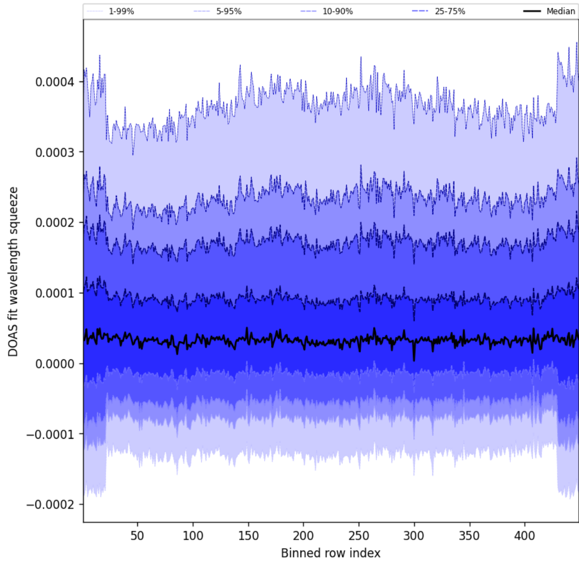
Figure 57: Along track statistics of “DOAS fit wavelength squeeze” for 2025-04-15 to 2025-04-16
