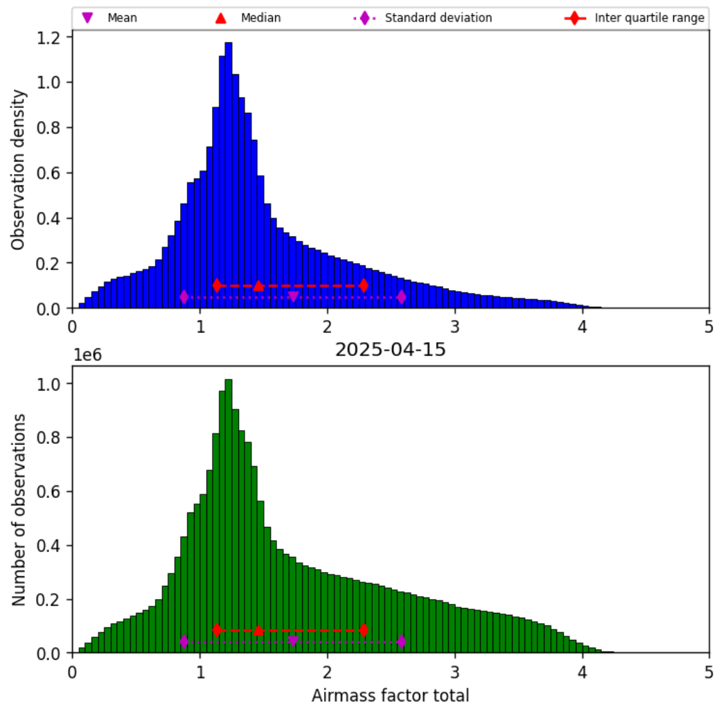
Figure 38: Histogram of “Airmass factor total” for 2025-04-15 to 2025-04-16
