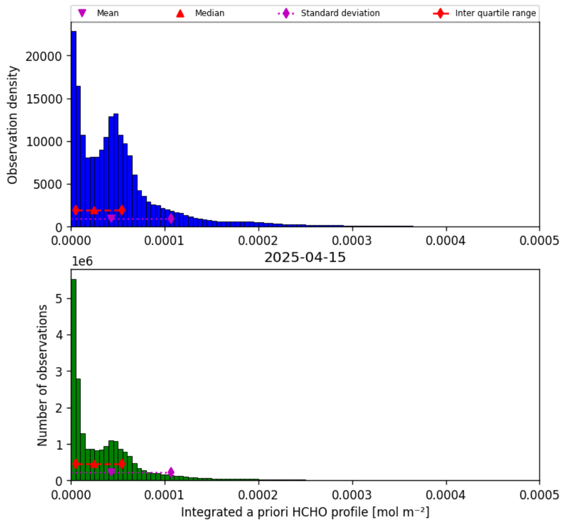
Figure 41: Histogram of “Integrated a priori HCHO profile” for 2025-04-15 to 2025-04-16
