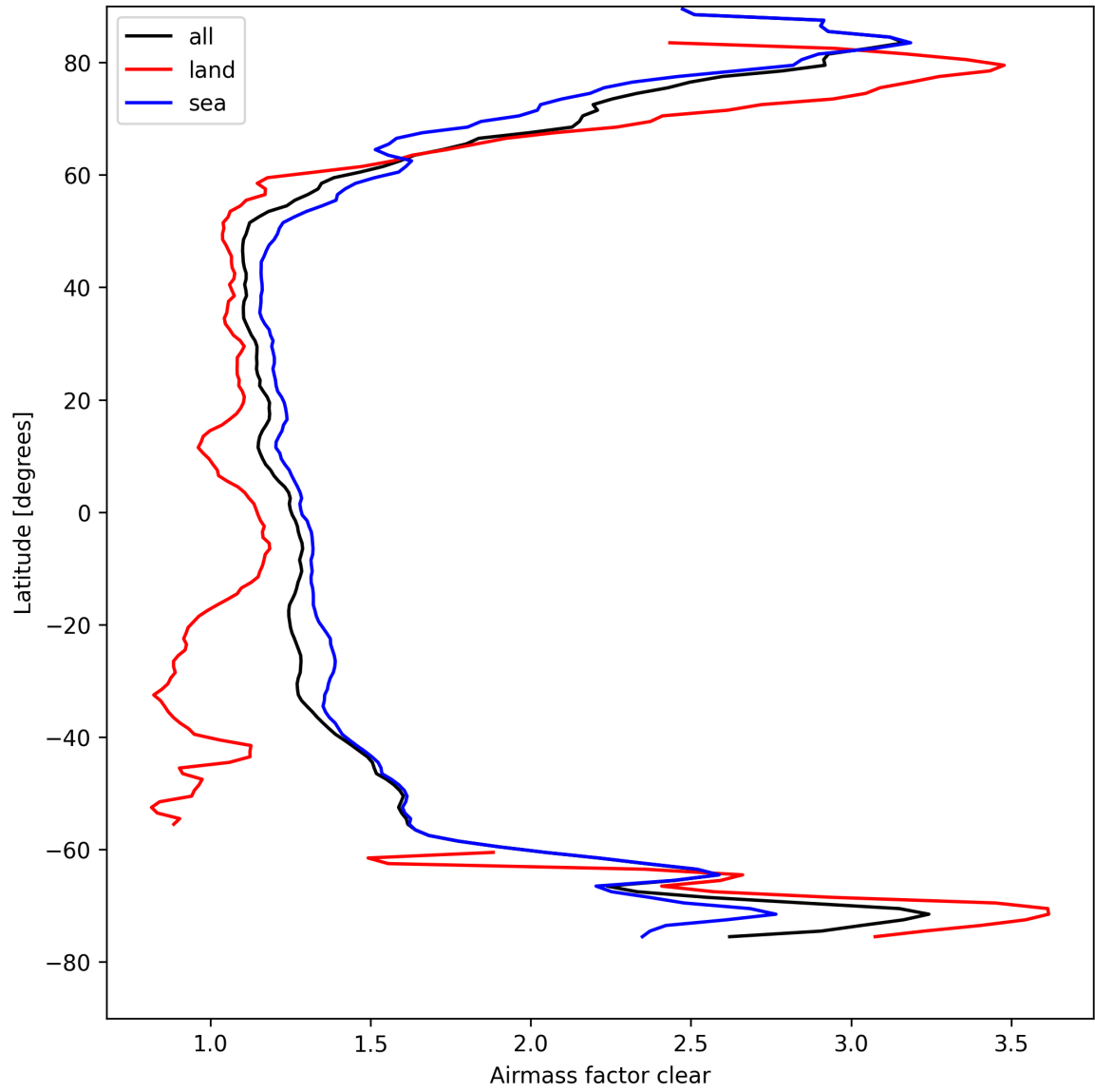
Figure 26: Zonal average of “Airmass factor clear” for 2025-04-15 to 2025-04-16.
