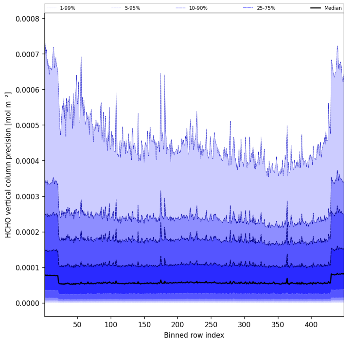
Figure 48: Along track statistics of “HCHO vertical column precision” for 2025-04-15 to 2025-04-16
