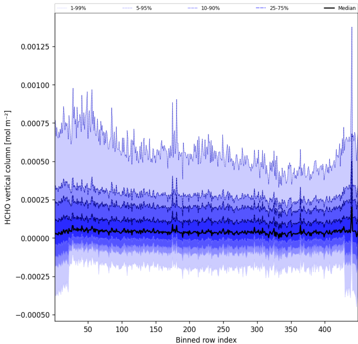
Figure 47: Along track statistics of “HCHO vertical column” for 2025-04-15 to 2025-04-16
