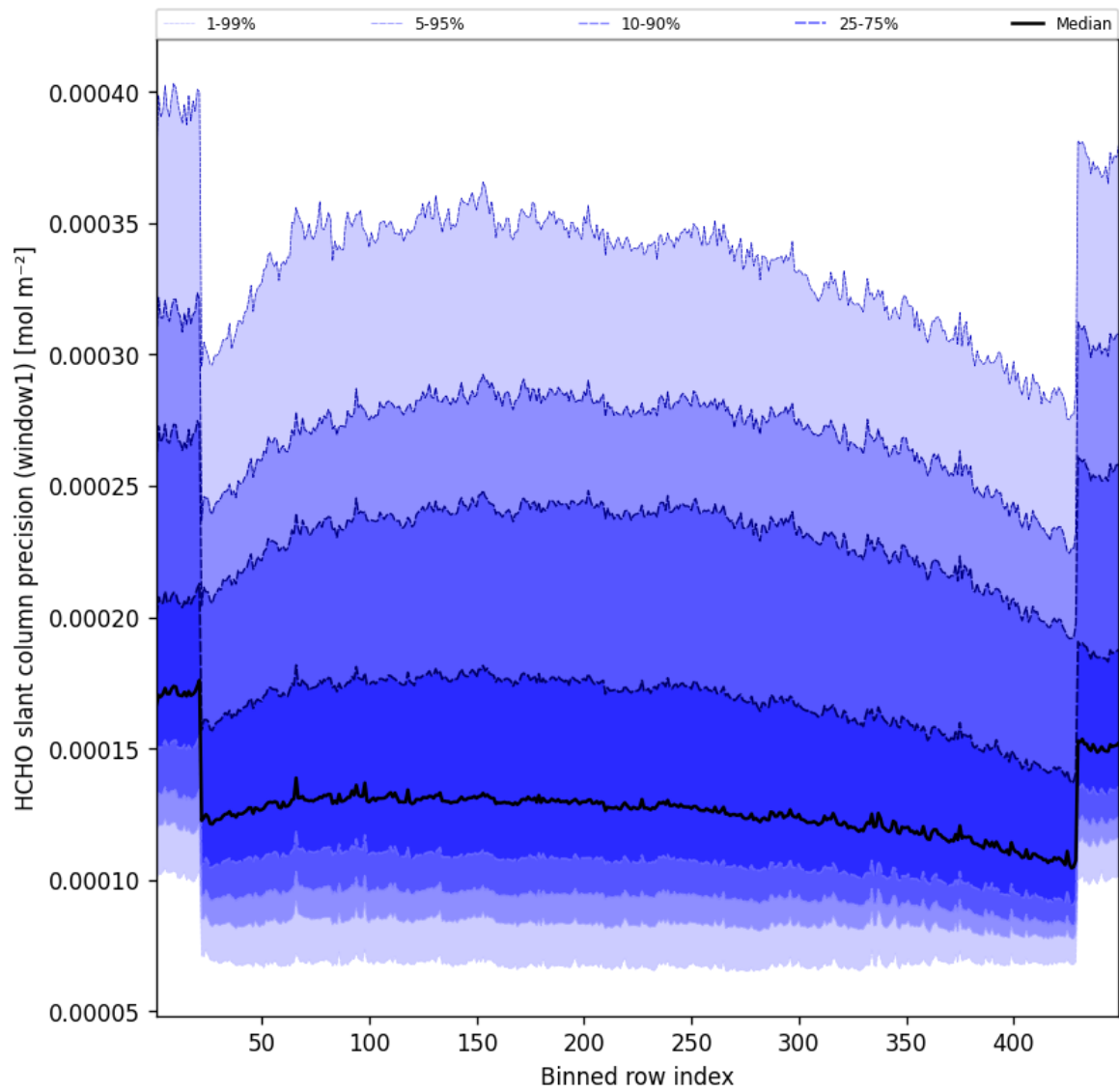
Figure 51: Along track statistics of “HCHO slant column precision (window1)” for 2025-04-15 to 2025-04-16
