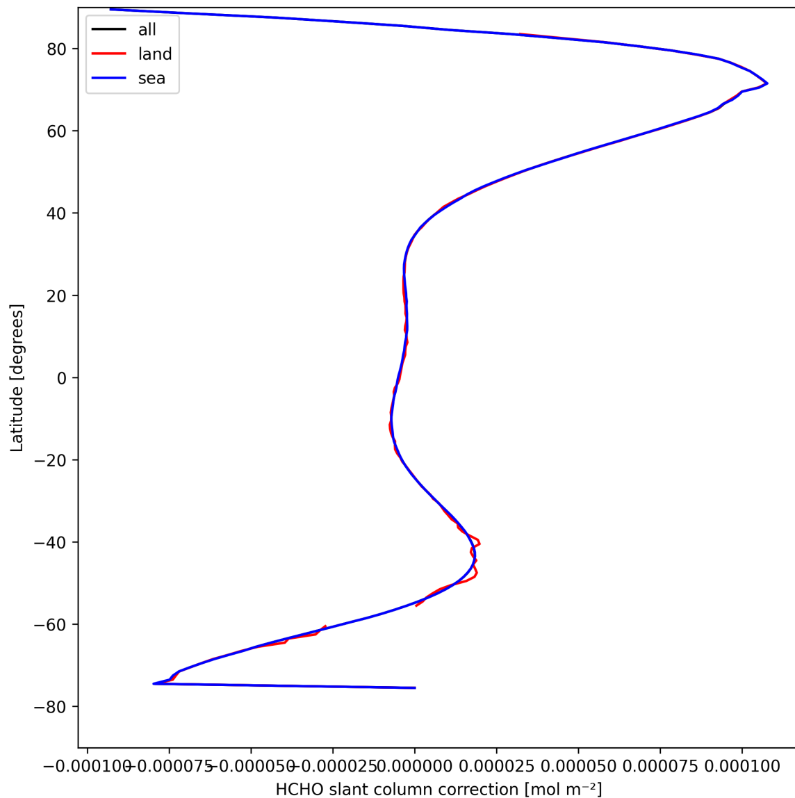
Figure 31: Zonal average of “HCHO slant column correction” for 2025-04-15 to 2025-04-16.
