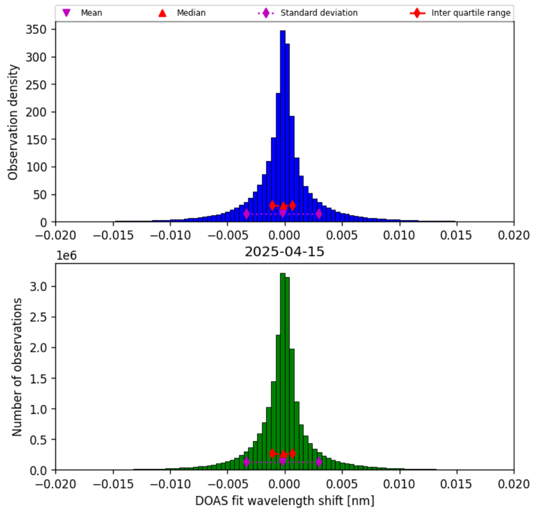
Figure 42: Histogram of “DOAS fit wavelength shift” for 2025-04-15 to 2025-04-16
