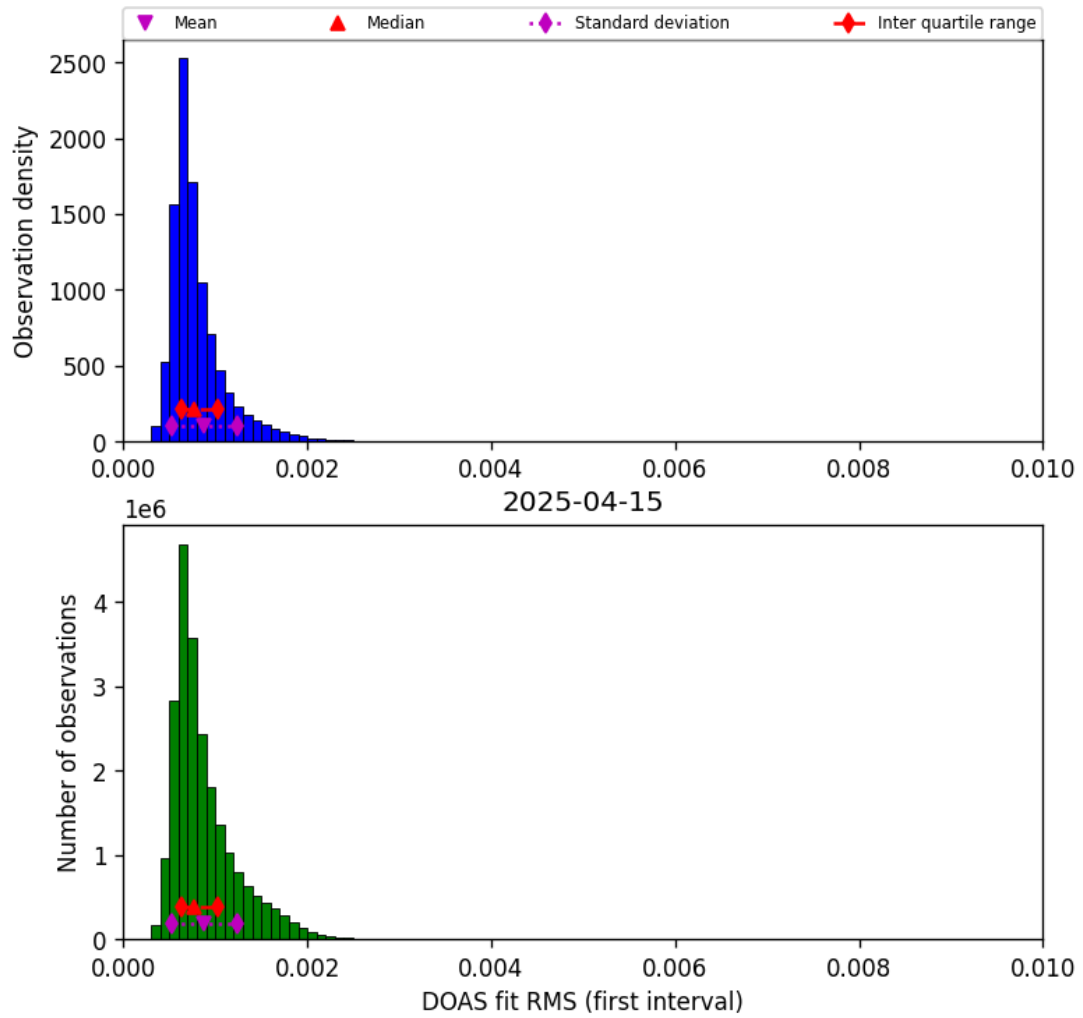
Figure 44: Histogram of “DOAS fit RMS (first interval)” for 2025-04-15 to 2025-04-16
