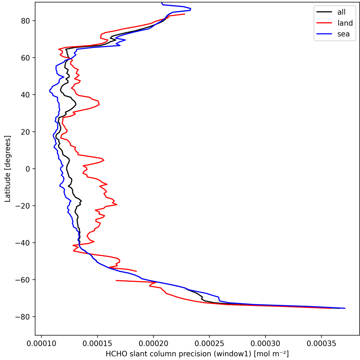
Figure 23: Zonal average of “HCHO slant column precision (window1)” for 2025-04-15 to 2025-04-16.
