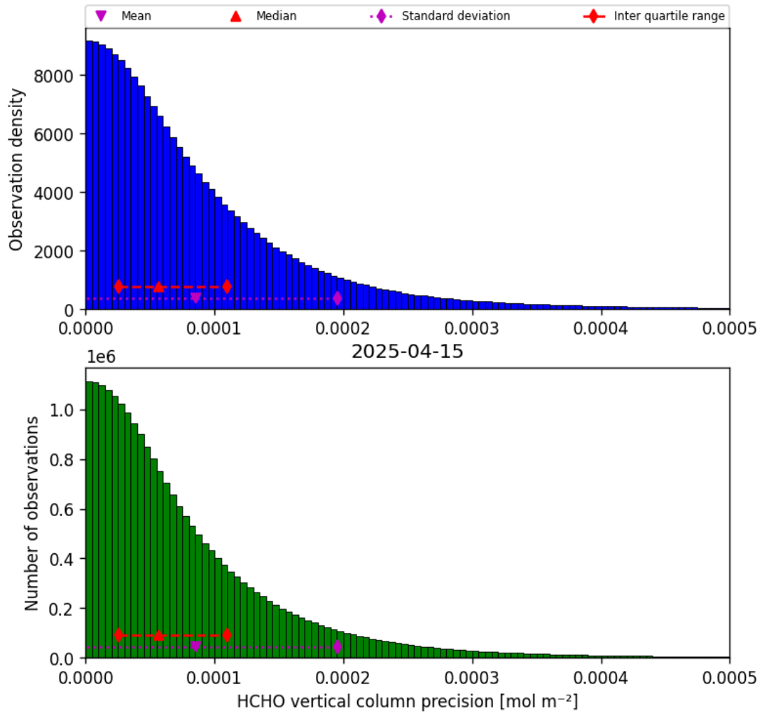
Figure 34: Histogram of “HCHO vertical column precision” for 2025-04-15 to 2025-04-16
