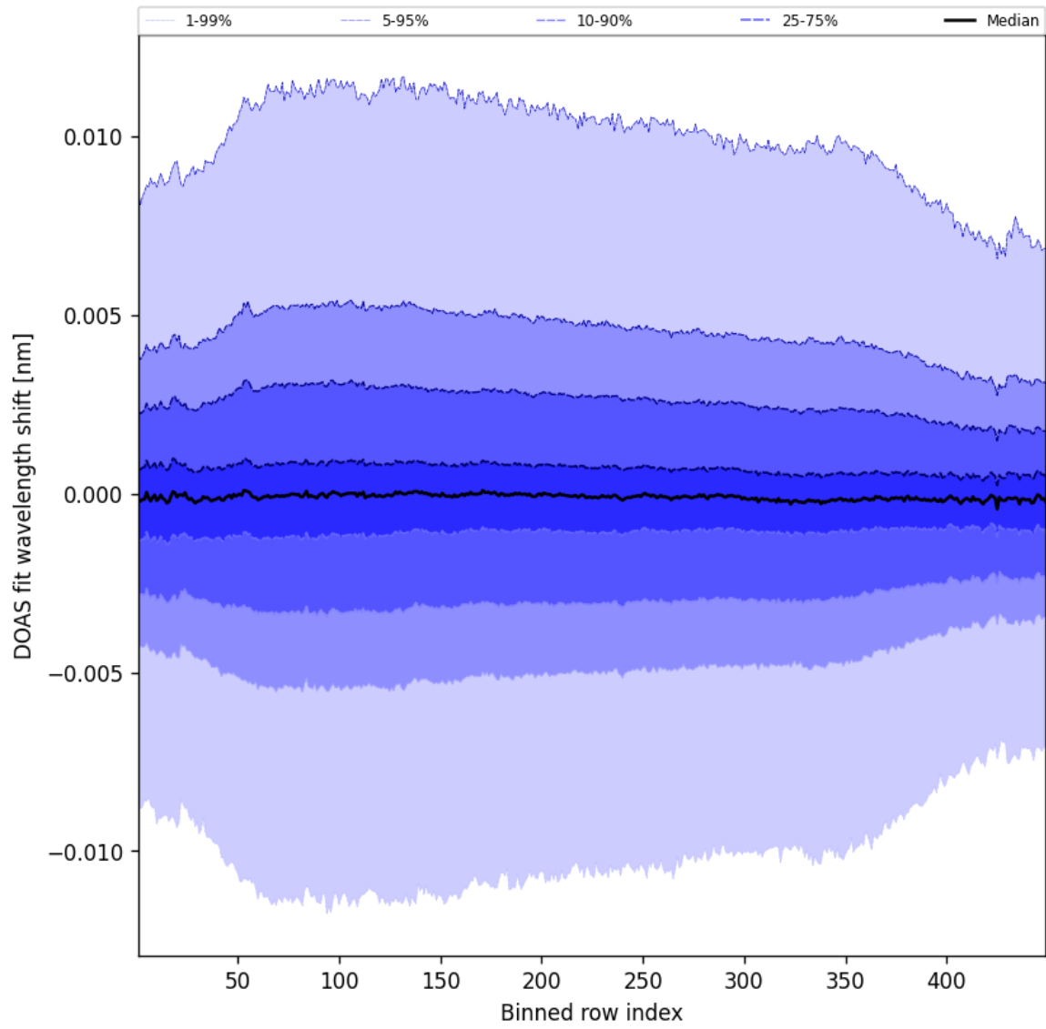
Figure 56: Along track statistics of “DOAS fit wavelength shift” for 2025-04-15 to 2025-04-16
