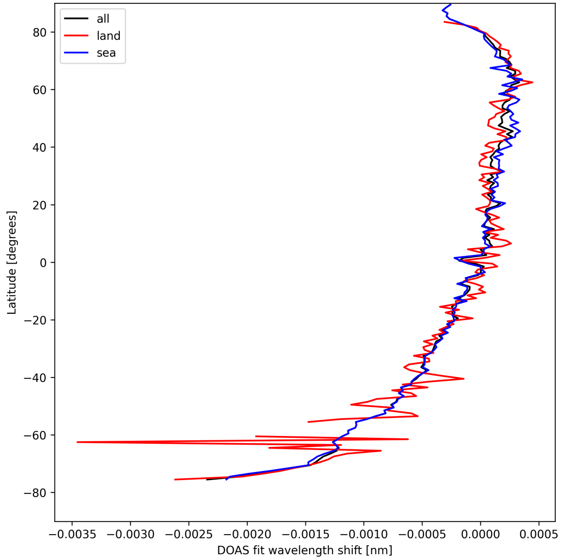
Figure 28: Zonal average of “DOAS fit wavelength shift” for 2025-04-15 to 2025-04-16.
