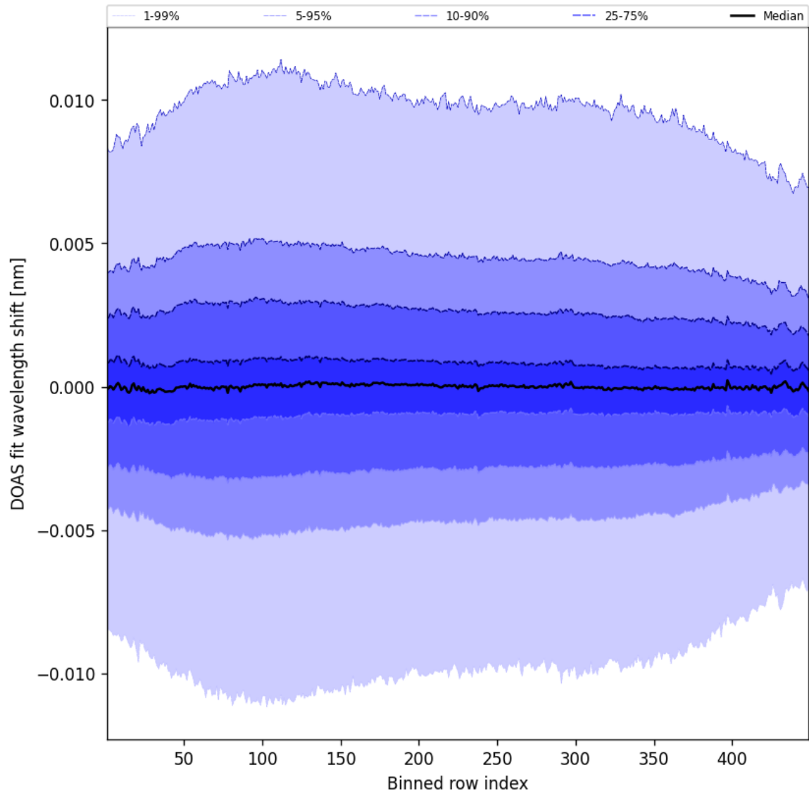
Figure 56: Along track statistics of “DOAS fit wavelength shift” for 2025-04-17 to 2025-04-18
