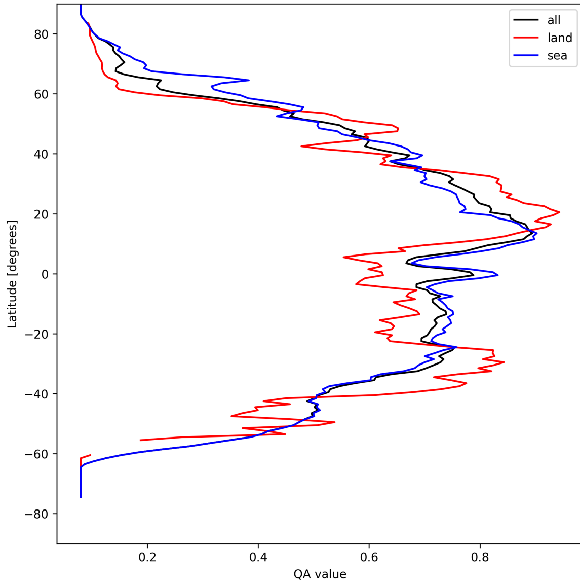
Figure 18: Zonal average of “QA value” for 2025-04-17 to 2025-04-18.
