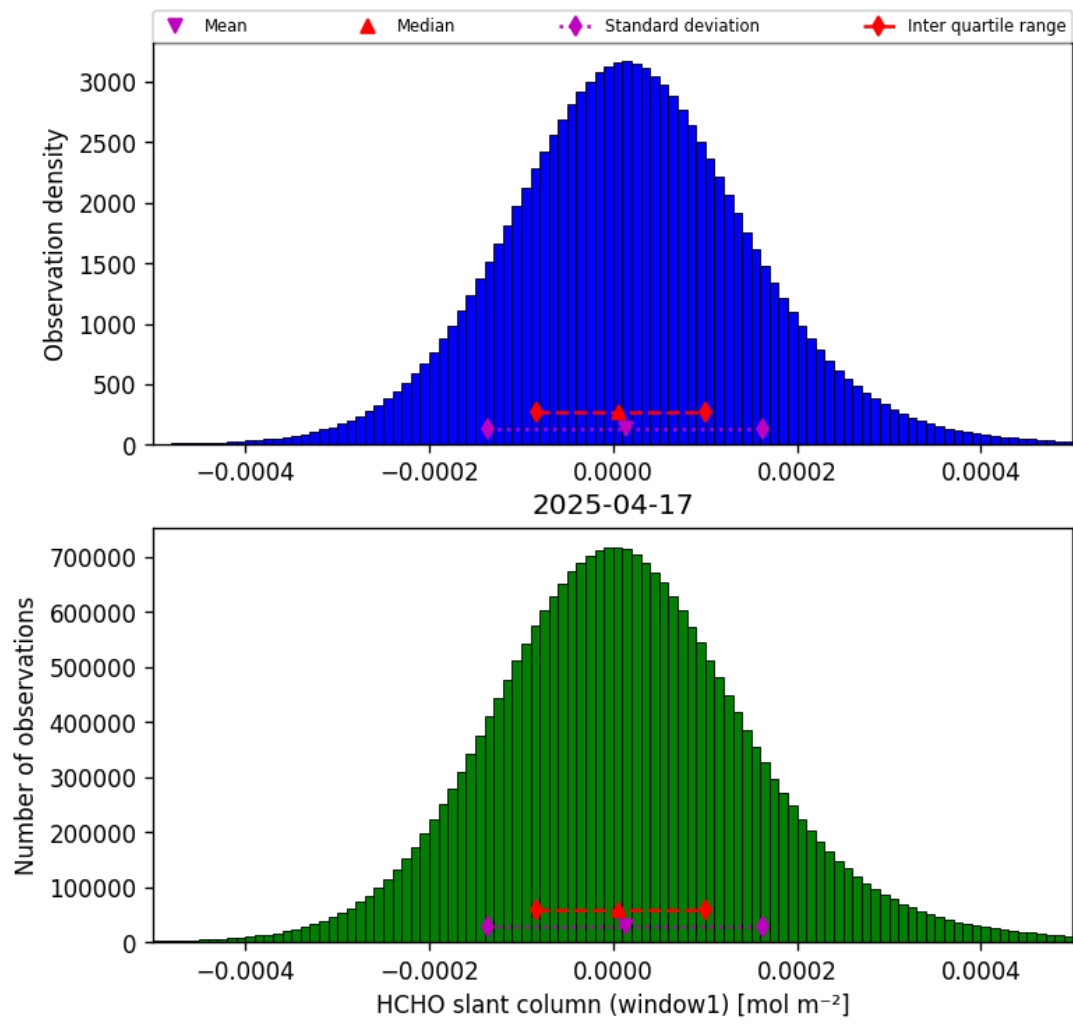
Figure 36: Histogram of “HCHO slant column (window1)” for 2025-04-17 to 2025-04-18
