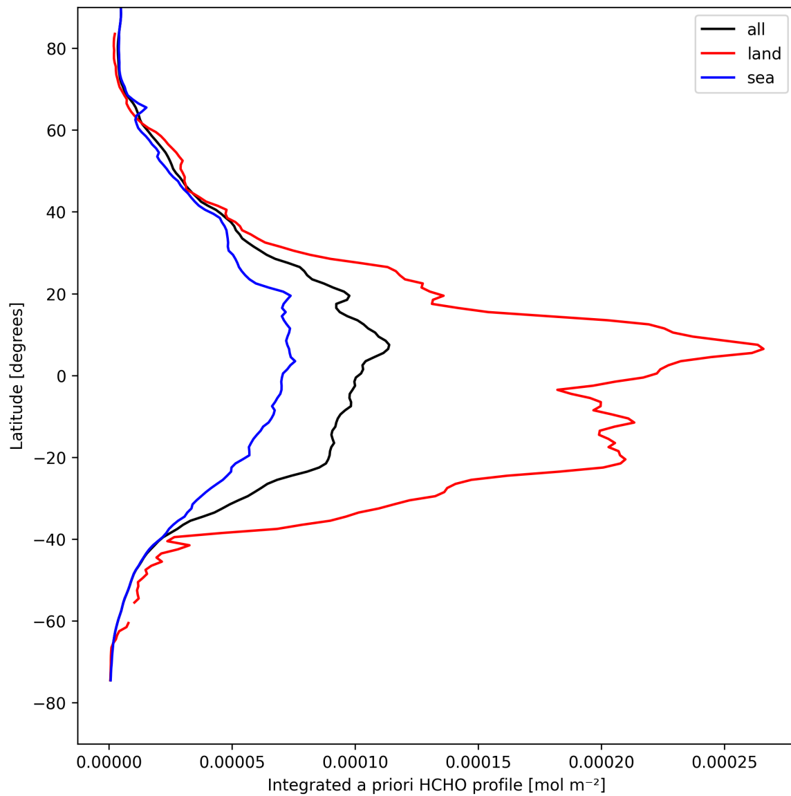
Figure 27: Zonal average of “Integrated a priori HCHO profile” for 2025-04-17 to 2025-04-18.
