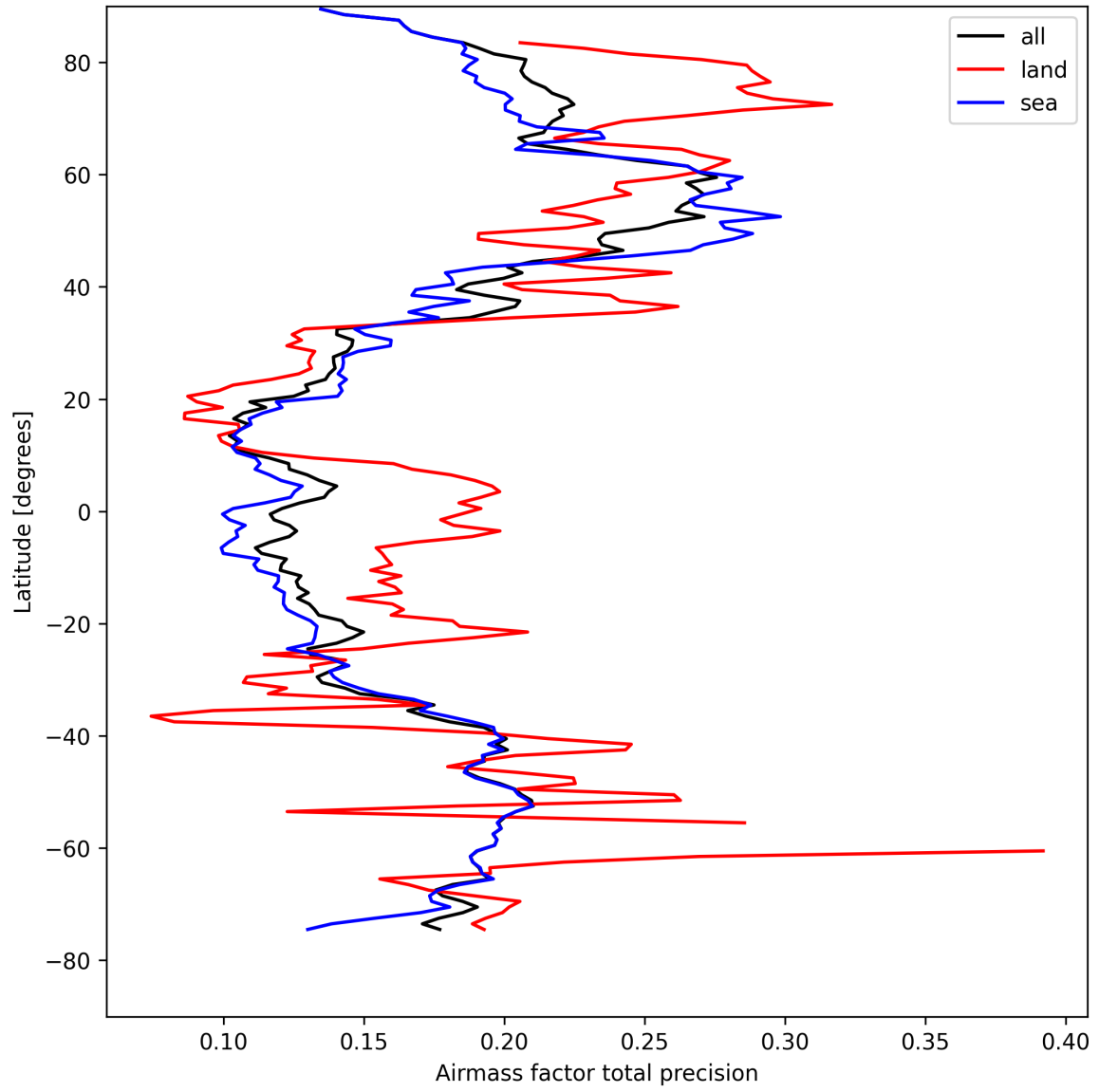
Figure 25: Zonal average of “Airmass factor total precision” for 2025-04-17 to 2025-04-18.
