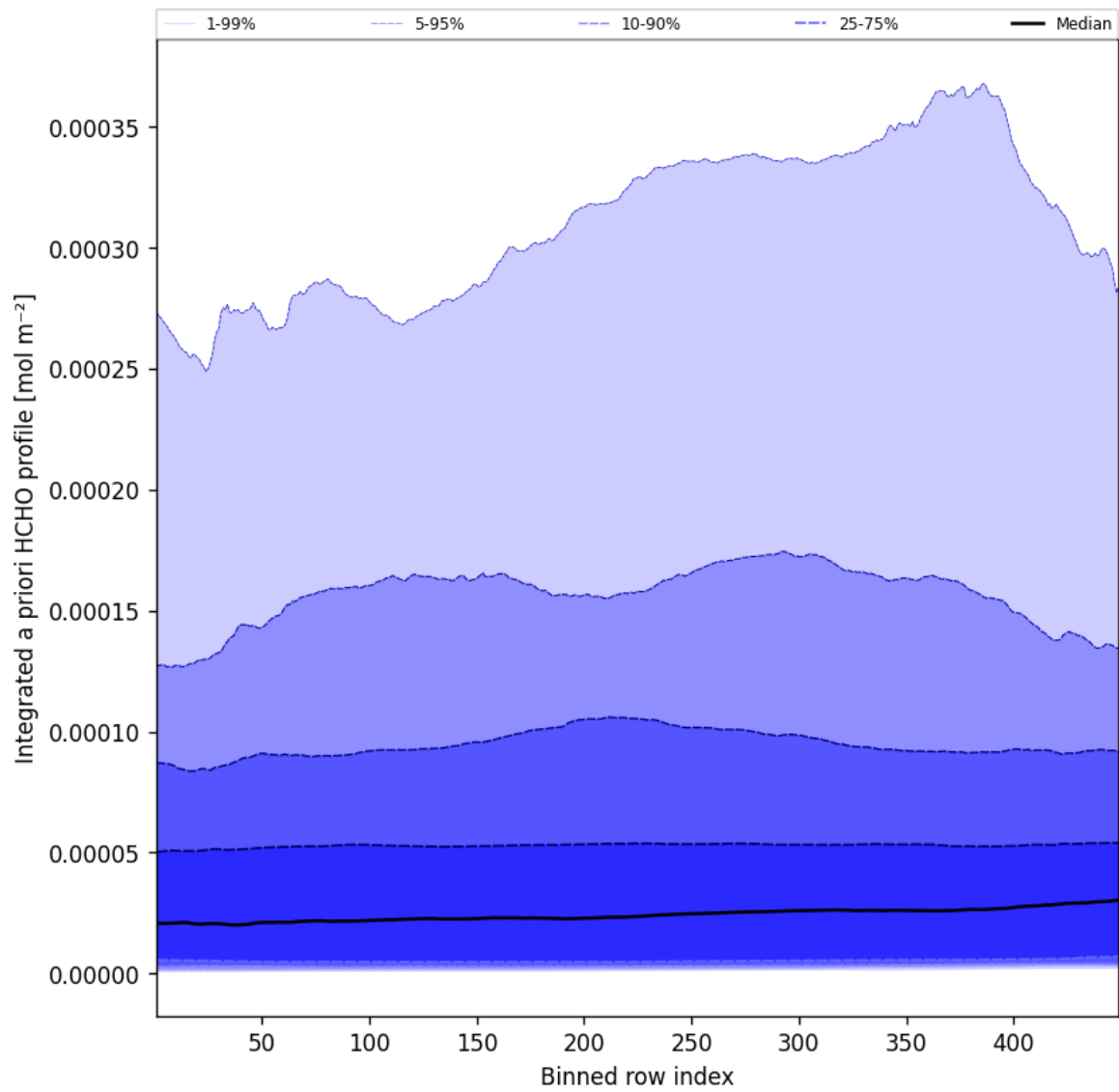
Figure 55: Along track statistics of “Integrated a priori HCHO profile” for 2025-04-17 to 2025-04-18
