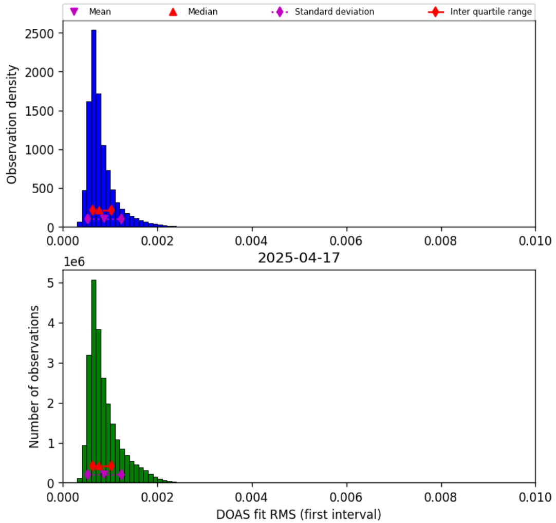
Figure 44: Histogram of “DOAS fit RMS (first interval)” for 2025-04-17 to 2025-04-18
