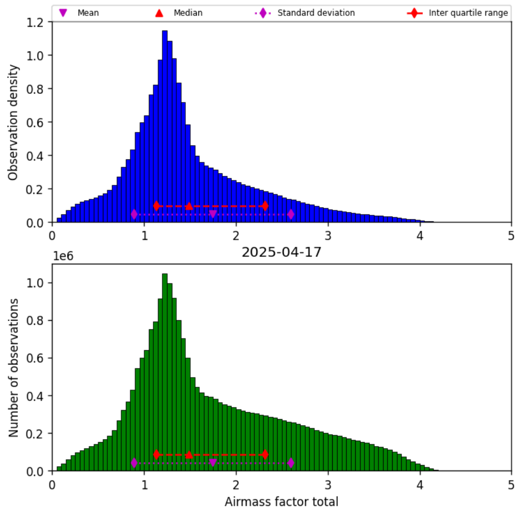
Figure 38: Histogram of “Airmass factor total” for 2025-04-17 to 2025-04-18
