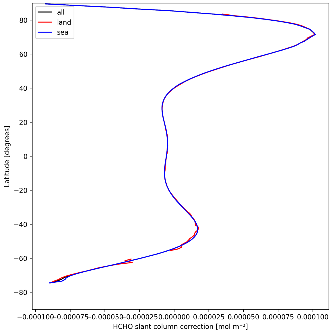
Figure 31: Zonal average of “HCHO slant column correction” for 2025-04-17 to 2025-04-18.
