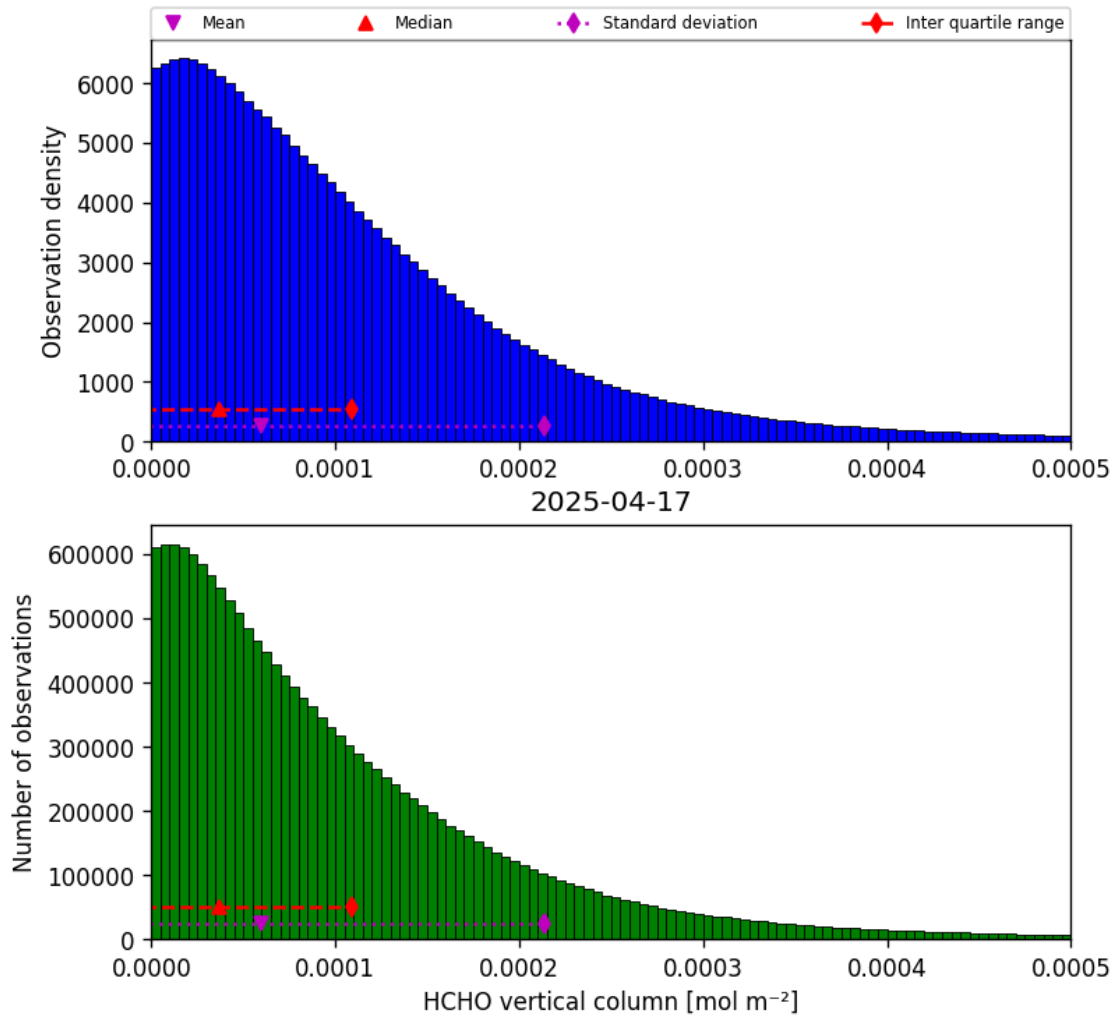
Figure 33: Histogram of “HCHO vertical column” for 2025-04-17 to 2025-04-18
