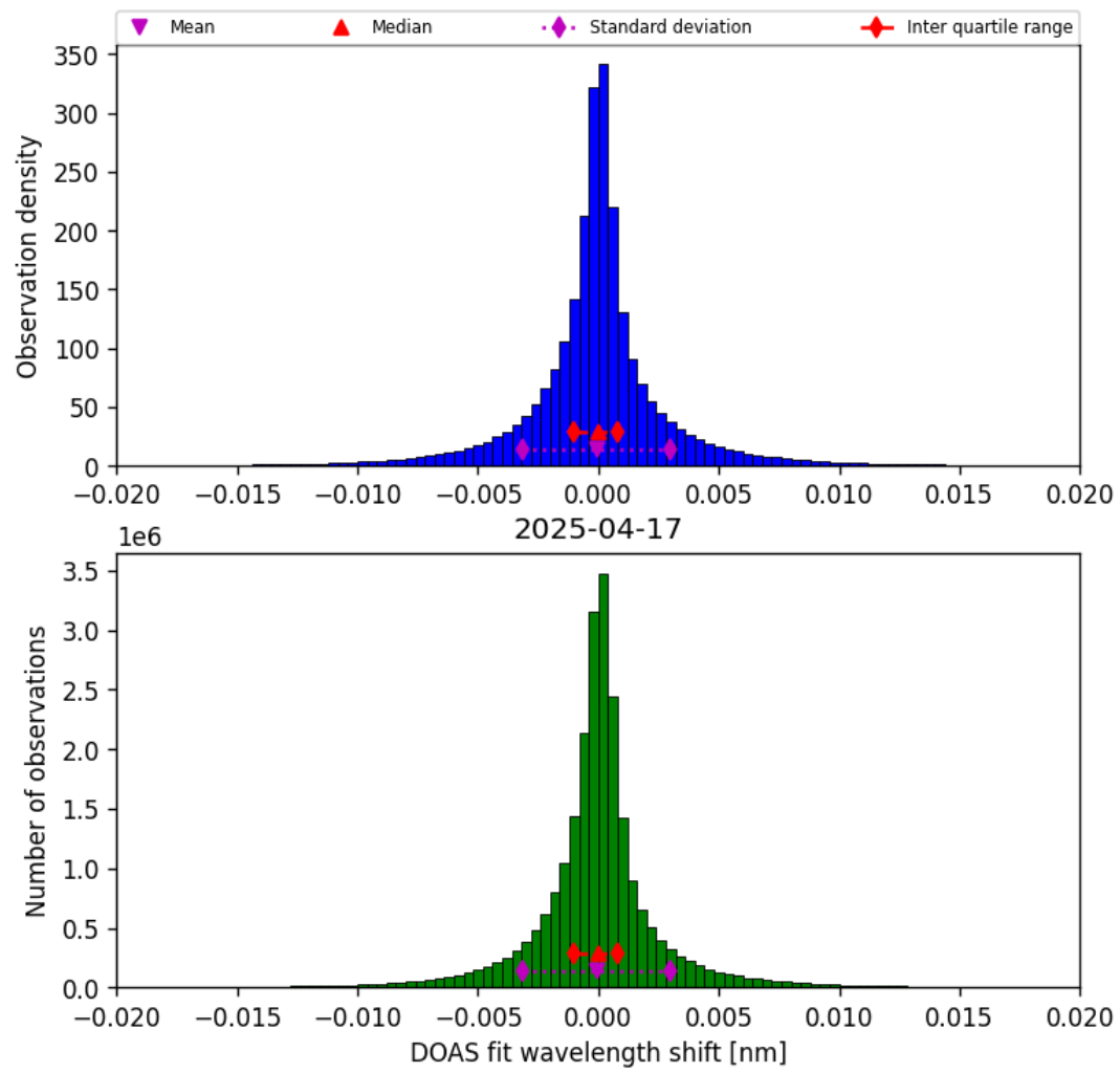
Figure 42: Histogram of “DOAS fit wavelength shift” for 2025-04-17 to 2025-04-18
