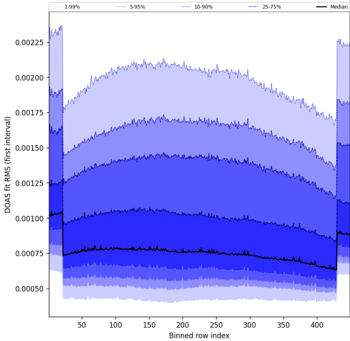
Figure 58: Along track statistics of “DOAS fit RMS (first interval)” for 2025-04-17 to 2025-04-18
