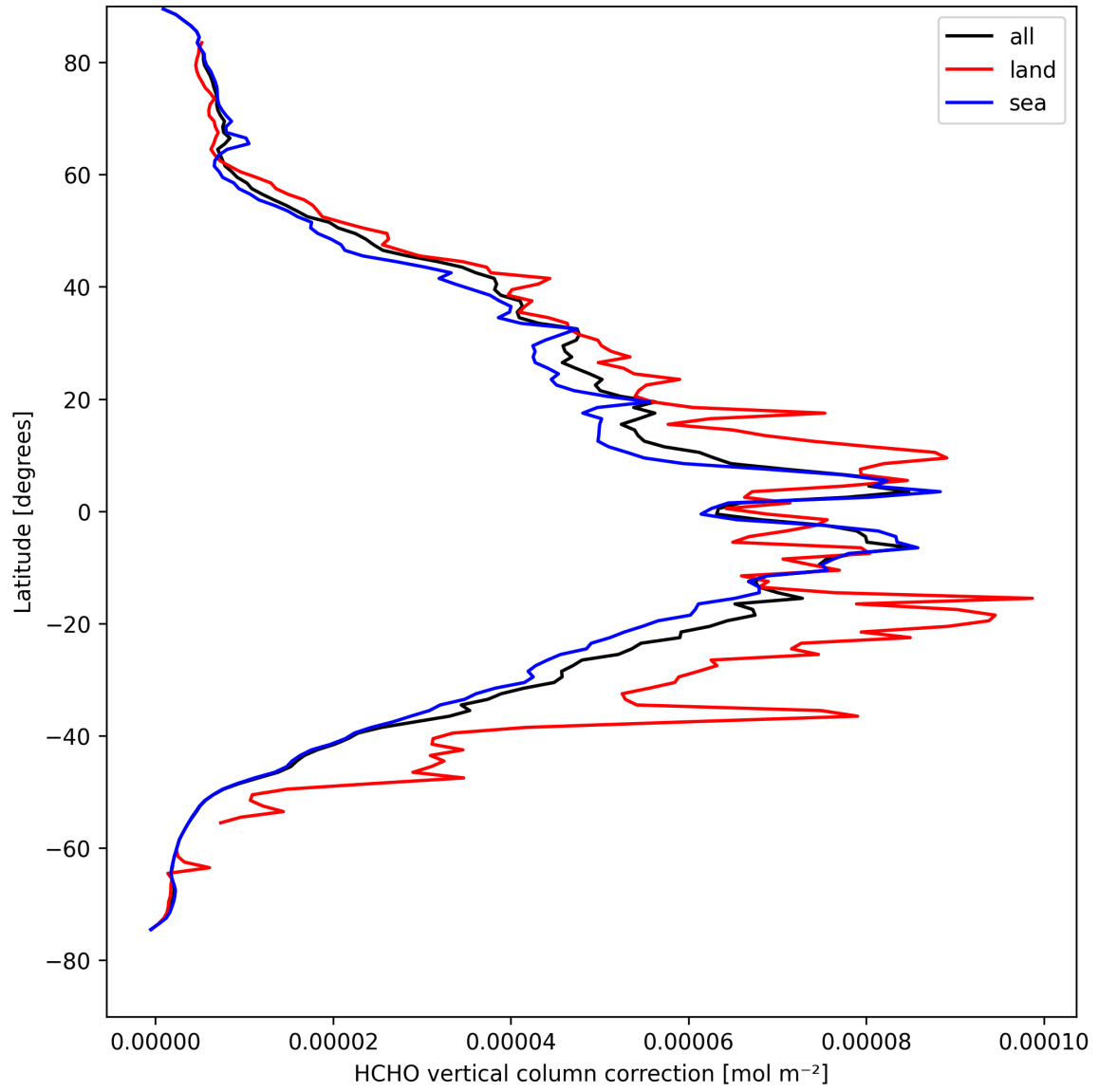
Figure 21: Zonal average of “HCHO vertical column correction” for 2025-04-17 to 2025-04-18.
