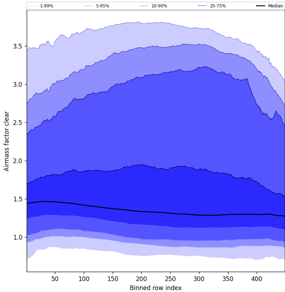
Figure 54: Along track statistics of “Airmass factor clear” for 2025-04-17 to 2025-04-18
