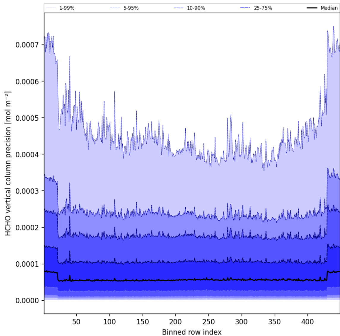
Figure 48: Along track statistics of “HCHO vertical column precision” for 2025-04-17 to 2025-04-18
