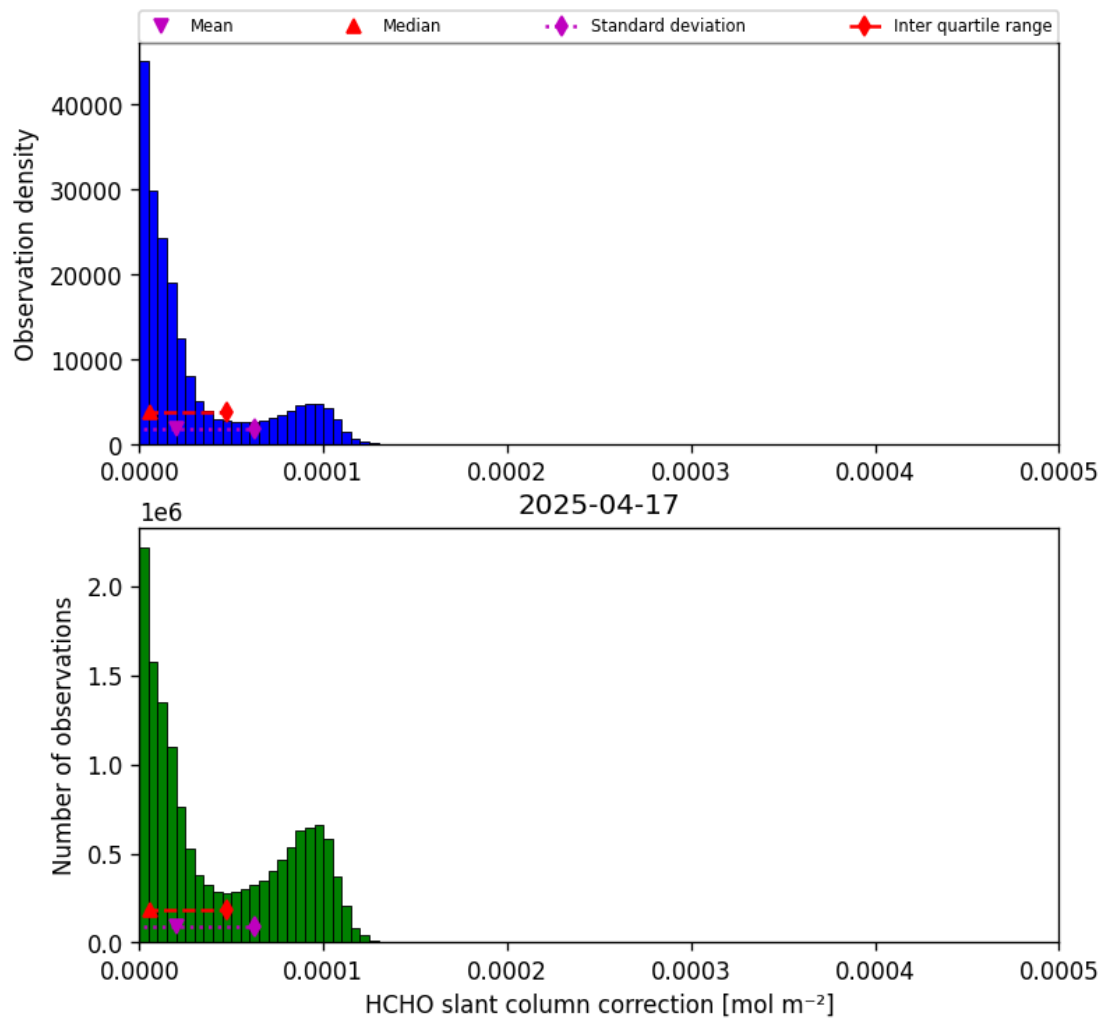
Figure 45: Histogram of “HCHO slant column correction” for 2025-04-17 to 2025-04-18
