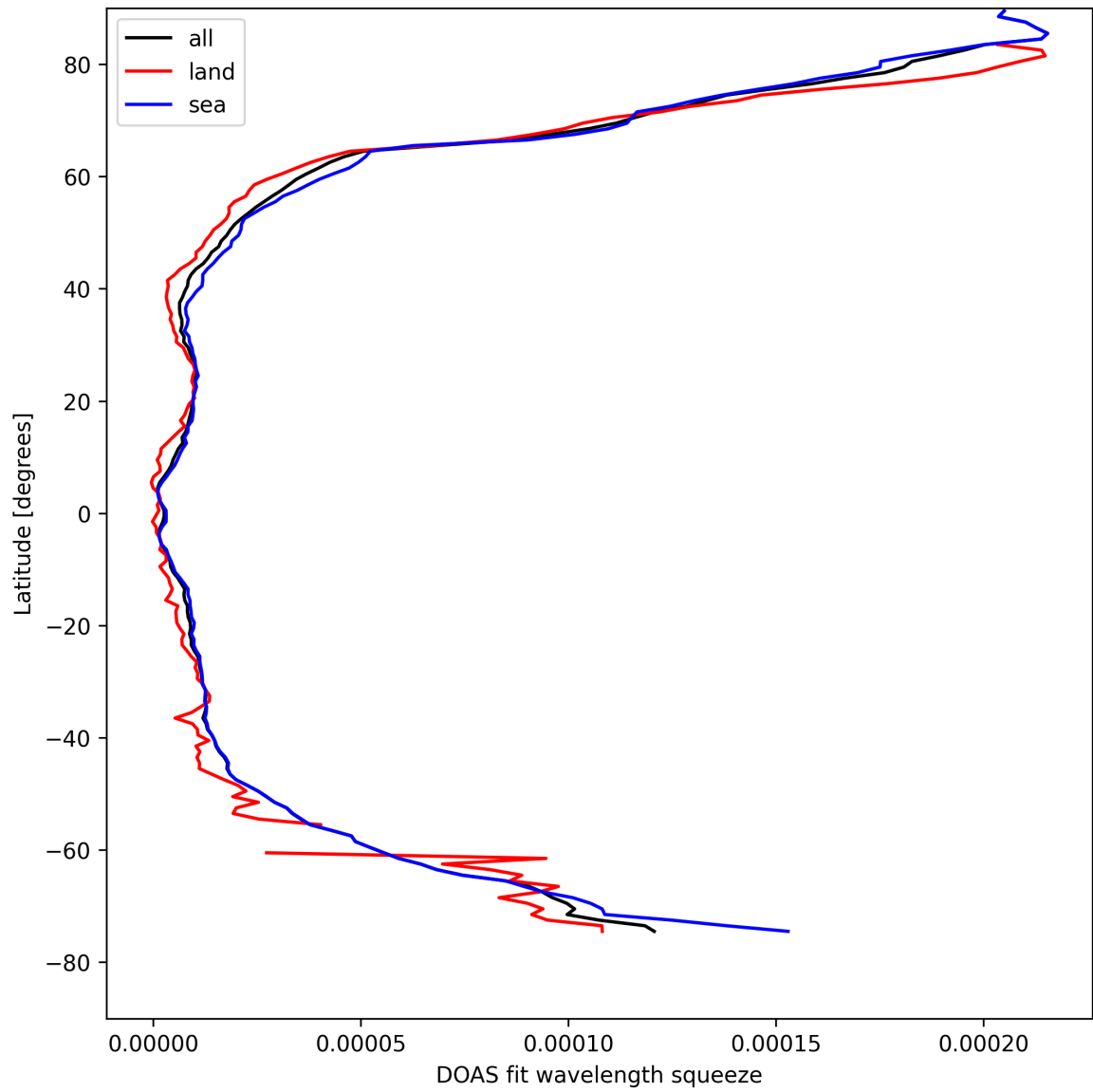
Figure 29: Zonal average of “DOAS fit wavelength squeeze” for 2025-04-17 to 2025-04-18.
