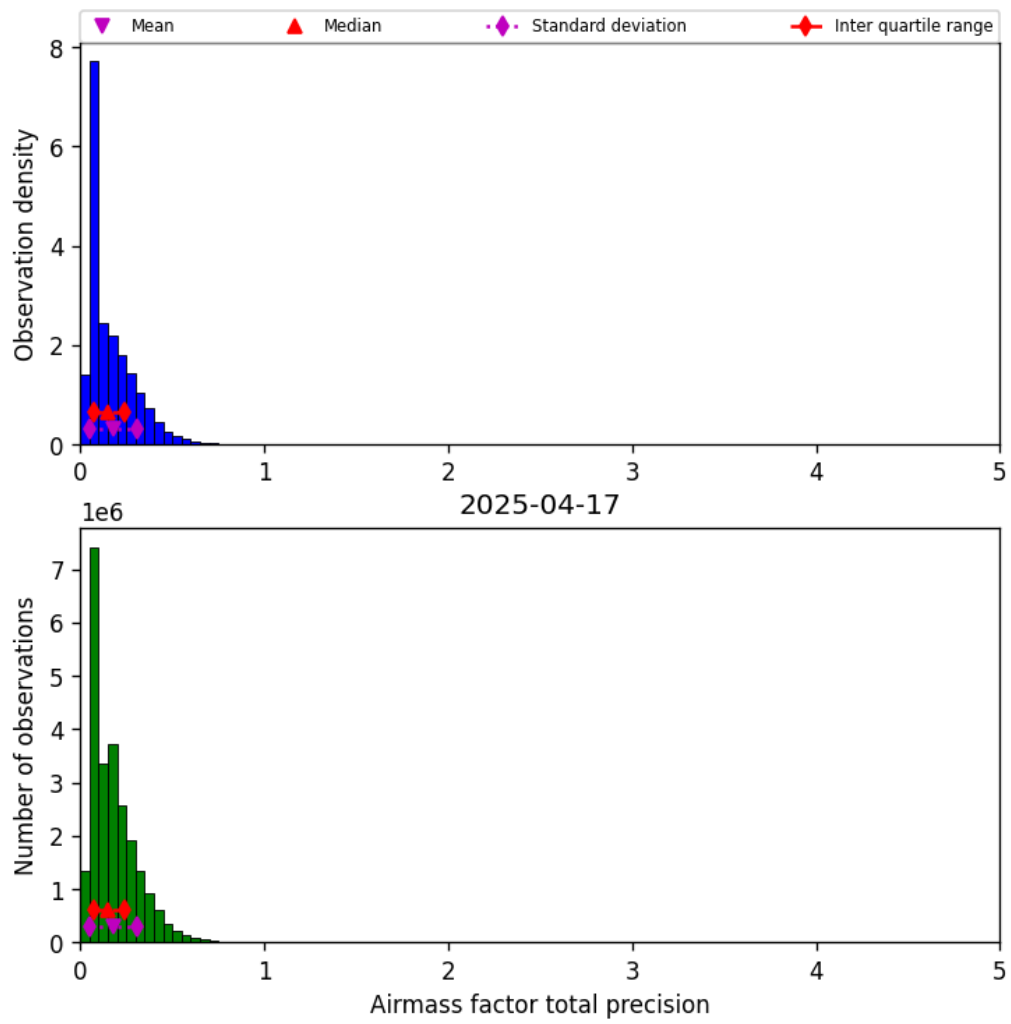
Figure 39: Histogram of “Airmass factor total precision” for 2025-04-17 to 2025-04-18
