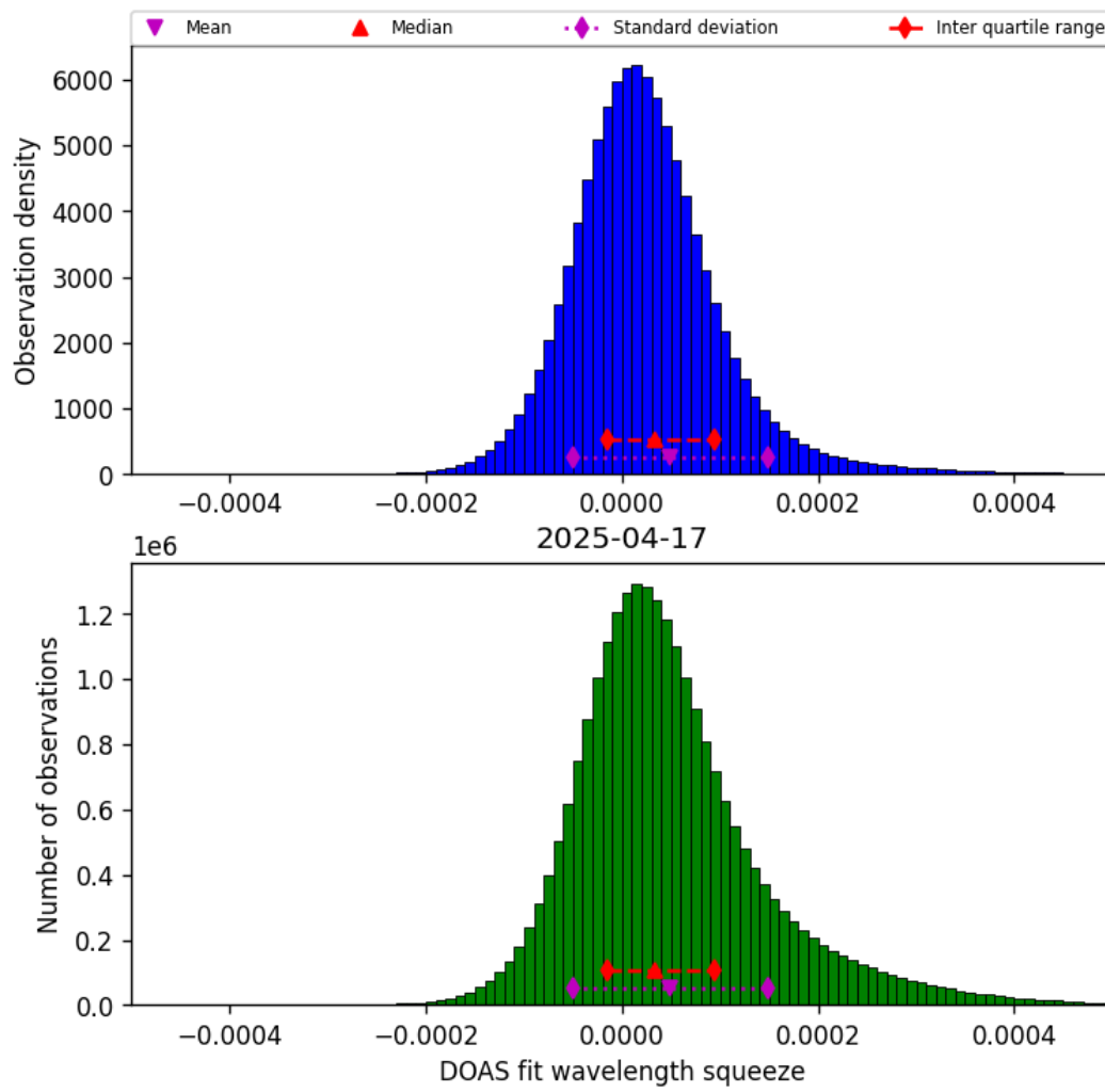
Figure 43: Histogram of “DOAS fit wavelength squeeze” for 2025-04-17 to 2025-04-18
