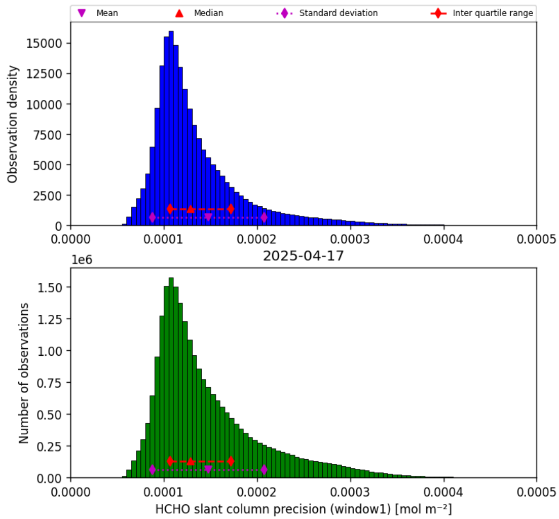
Figure 37: Histogram of “HCHO slant column precision (window1)” for 2025-04-17 to 2025-04-18
