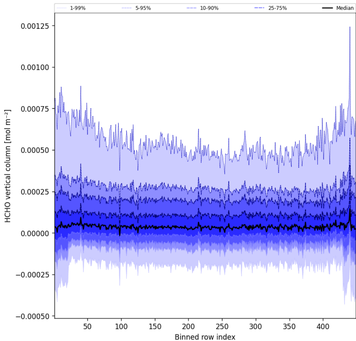
Figure 47: Along track statistics of “HCHO vertical column” for 2025-04-17 to 2025-04-18
