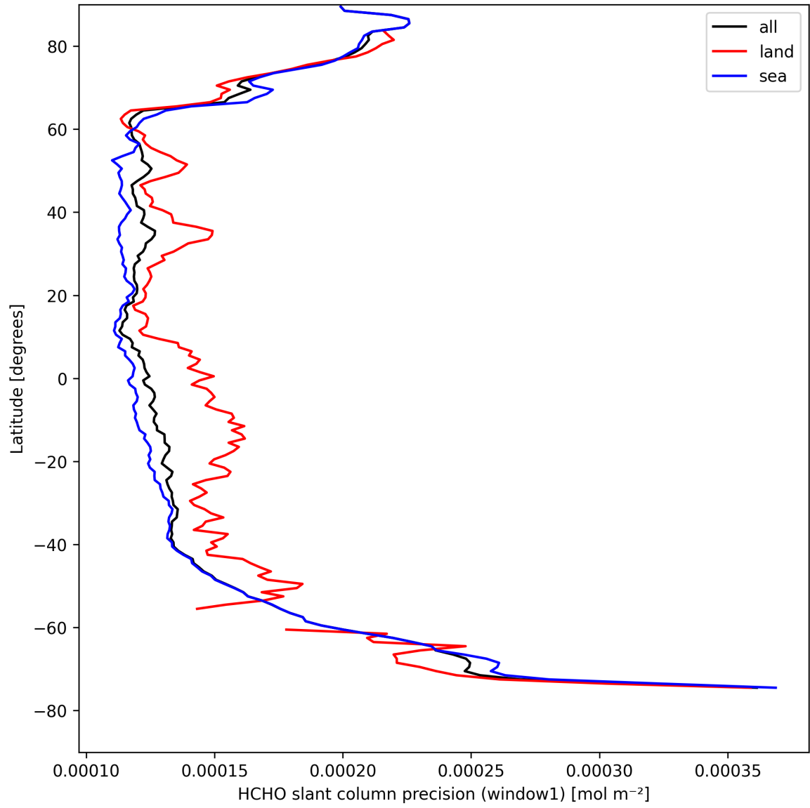
Figure 23: Zonal average of “HCHO slant column precision (window1)” for 2025-04-17 to 2025-04-18.
