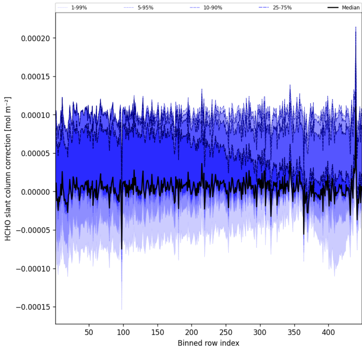
Figure 59: Along track statistics of “HCHO slant column correction” for 2025-04-17 to 2025-04-18
