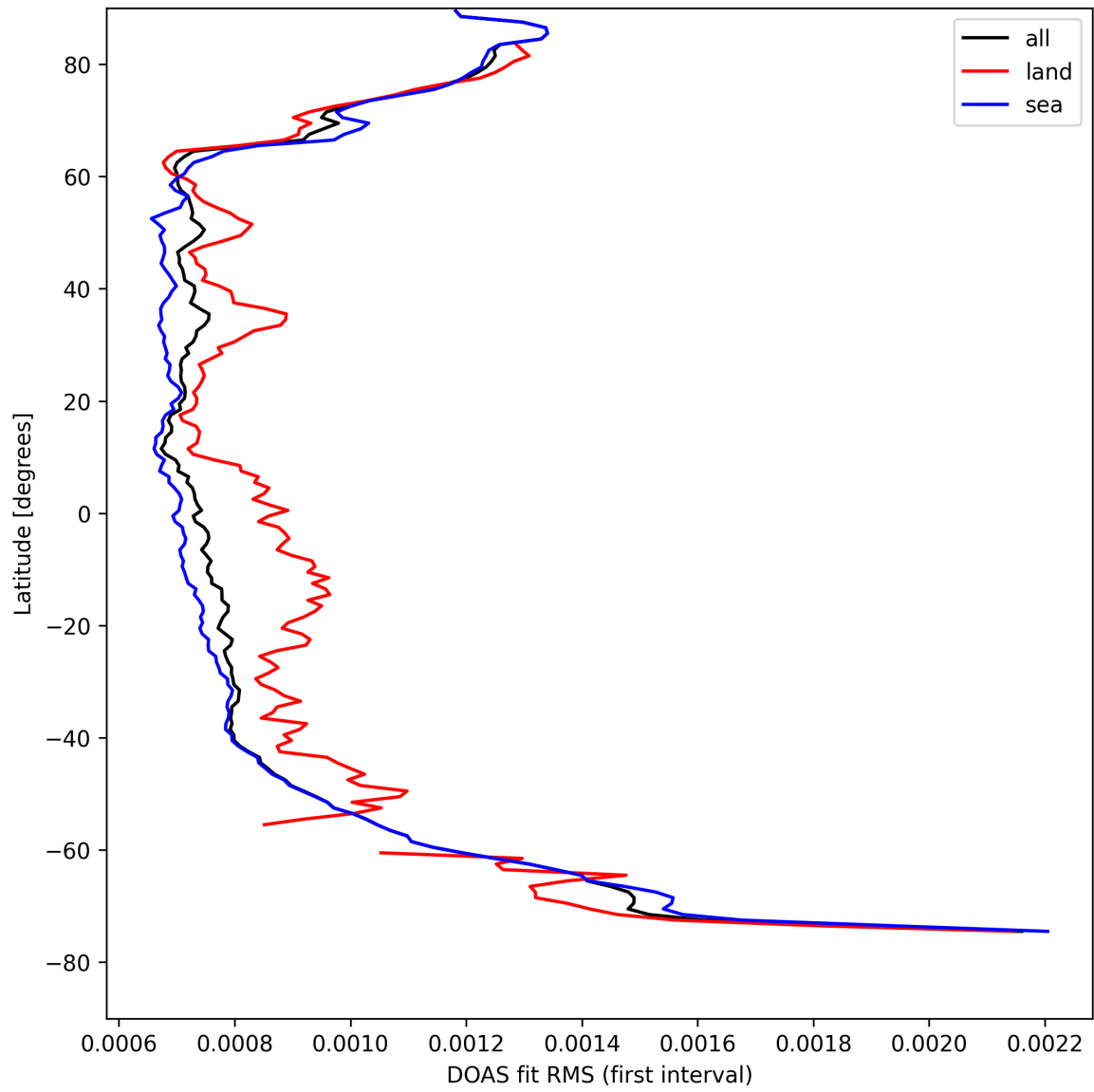
Figure 30: Zonal average of “DOAS fit RMS (first interval)” for 2025-04-17 to 2025-04-18.
