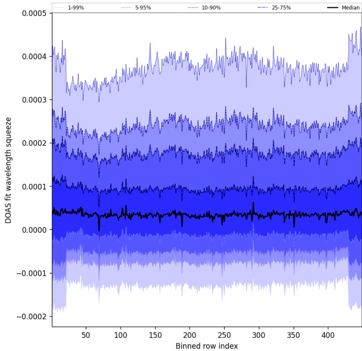
Figure 57: Along track statistics of “DOAS fit wavelength squeeze” for 2025-04-17 to 2025-04-18
