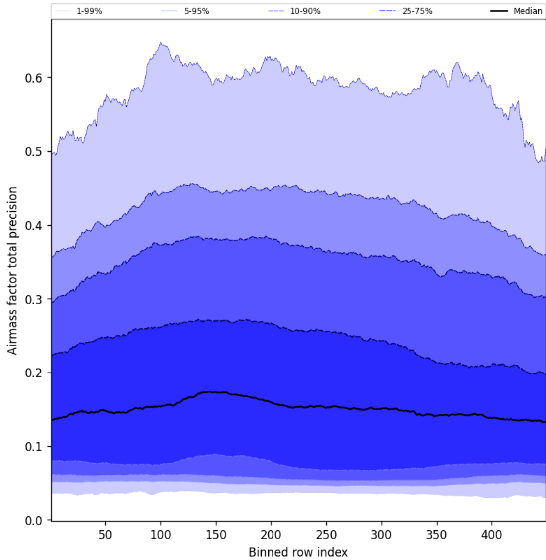
Figure 53: Along track statistics of “Airmass factor total precision” for 2025-04-17 to 2025-04-18
