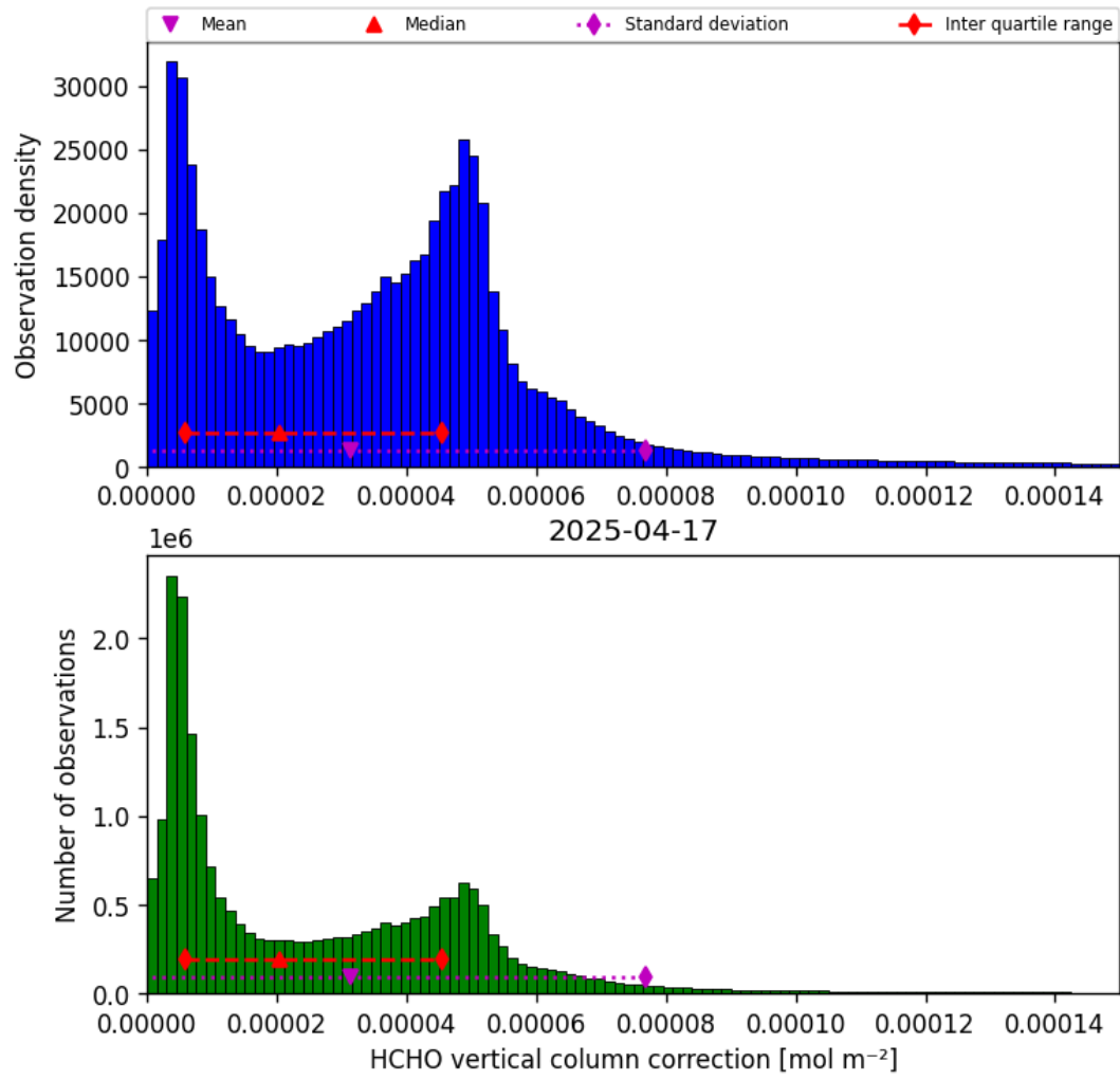
Figure 35: Histogram of “HCHO vertical column correction” for 2025-04-17 to 2025-04-18
