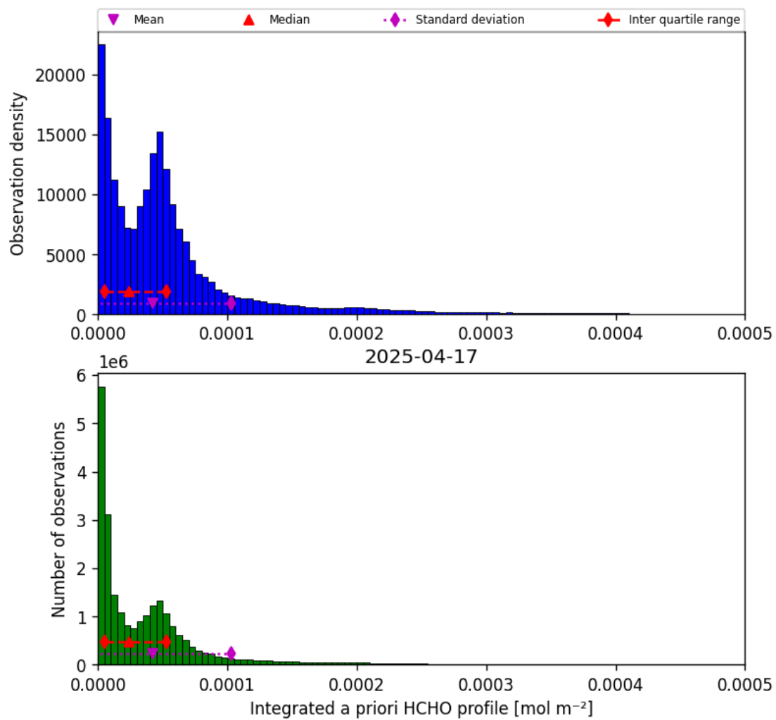
Figure 41: Histogram of “Integrated a priori HCHO profile” for 2025-04-17 to 2025-04-18
