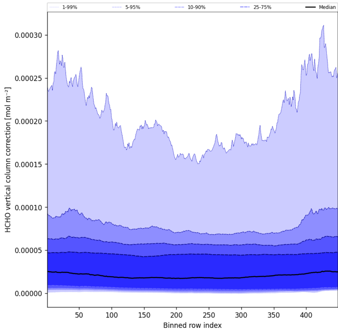
Figure 49: Along track statistics of “HCHO vertical column correction” for 2025-04-17 to 2025-04-18
