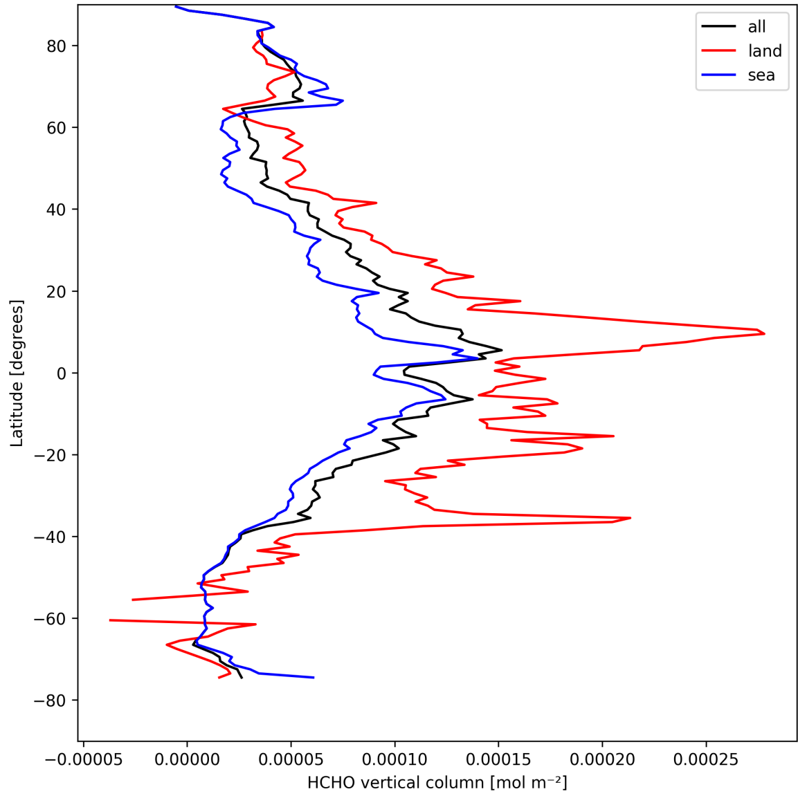
Figure 19: Zonal average of “HCHO vertical column” for 2025-04-17 to 2025-04-18.
