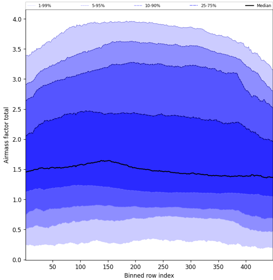
Figure 52: Along track statistics of “Airmass factor total” for 2025-04-17 to 2025-04-18
