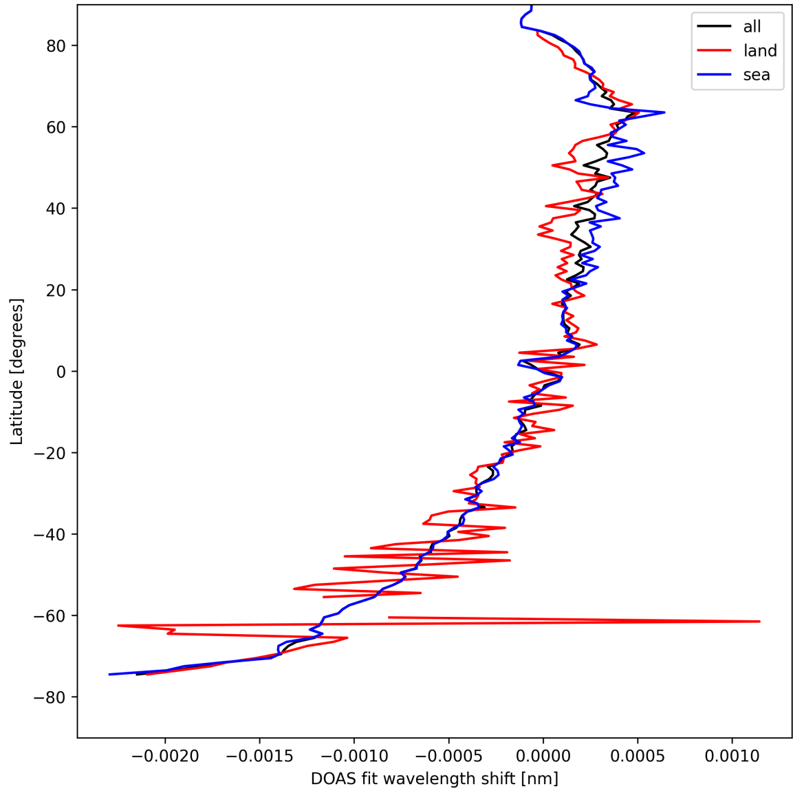
Figure 28: Zonal average of “DOAS fit wavelength shift” for 2025-04-17 to 2025-04-18.
