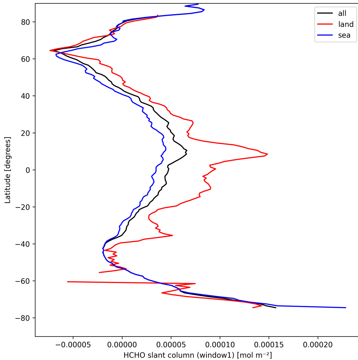
Figure 22: Zonal average of “HCHO slant column (window1)” for 2025-04-17 to 2025-04-18.
