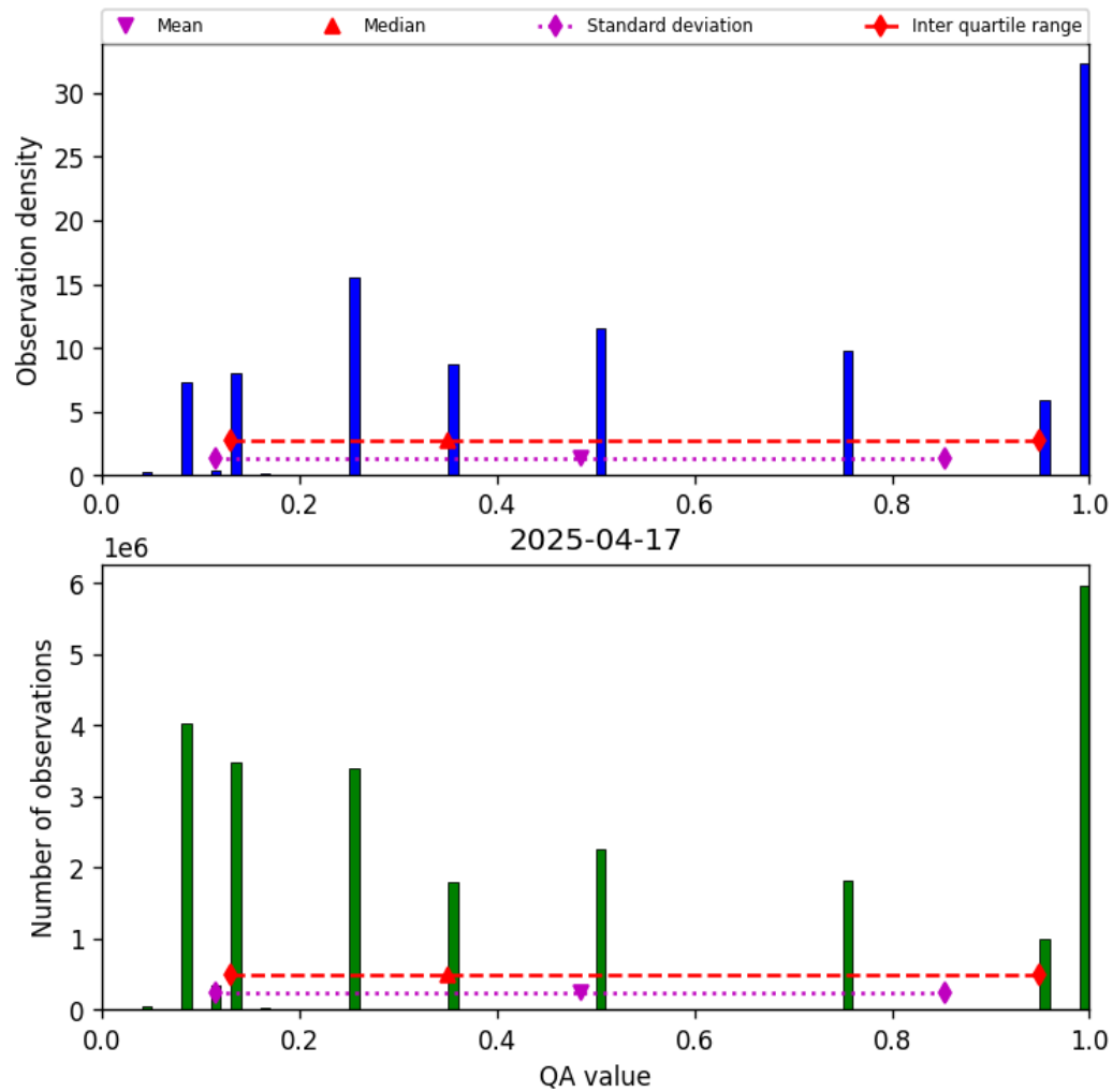
Figure 32: Histogram of “QA value” for 2025-04-17 to 2025-04-18
