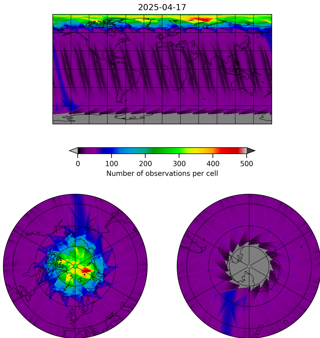
Figure 17: Map of the number of observations for 2025-04-17 to 2025-04-18
