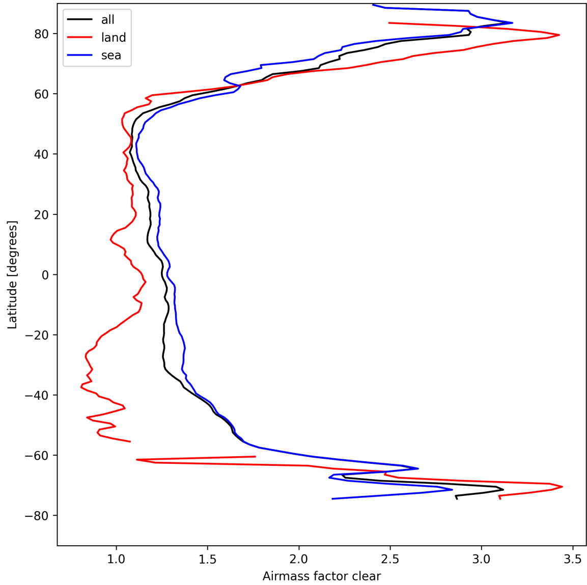
Figure 26: Zonal average of “Airmass factor clear” for 2025-04-17 to 2025-04-18.
