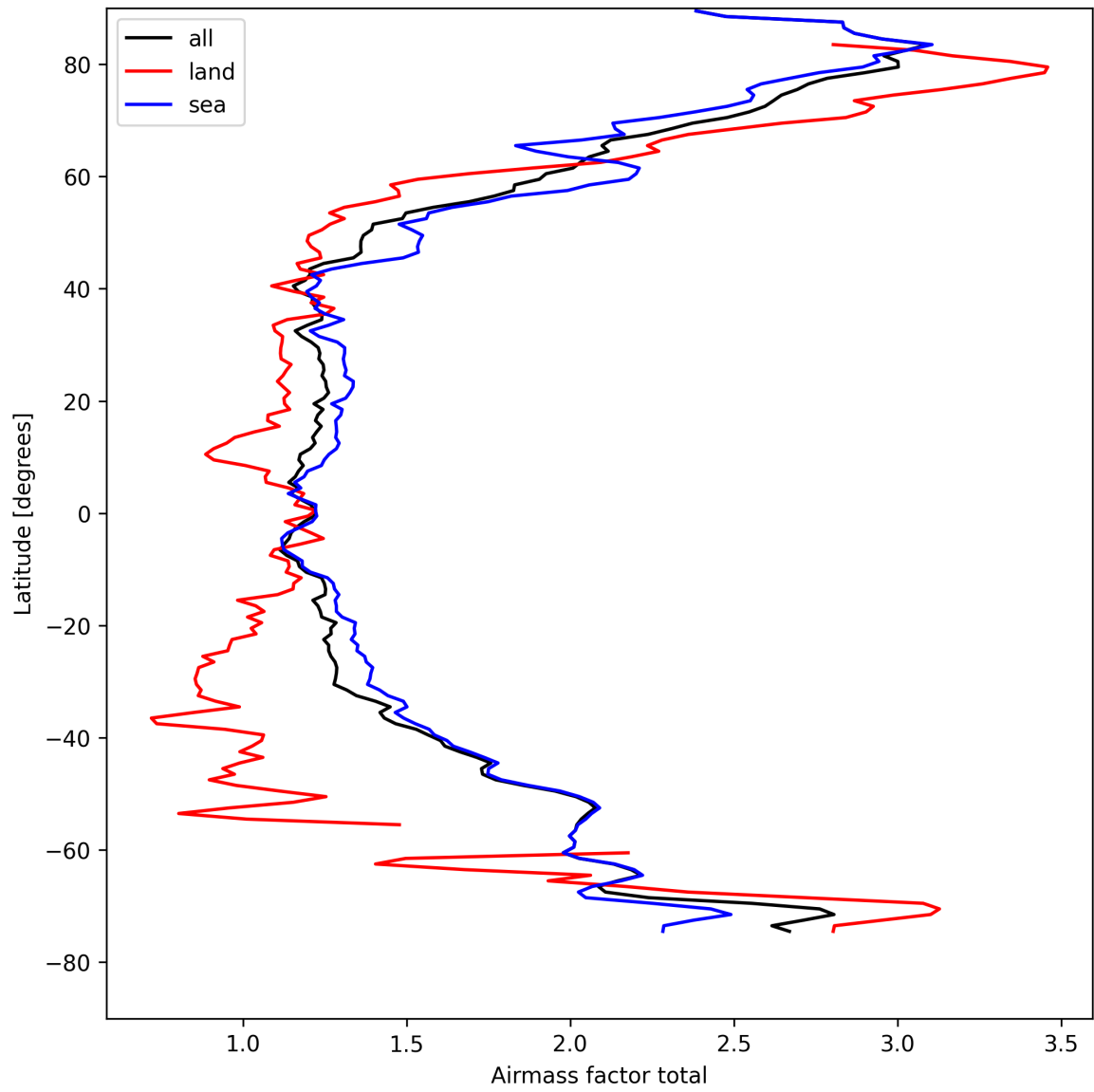
Figure 24: Zonal average of “Airmass factor total” for 2025-04-17 to 2025-04-18.
