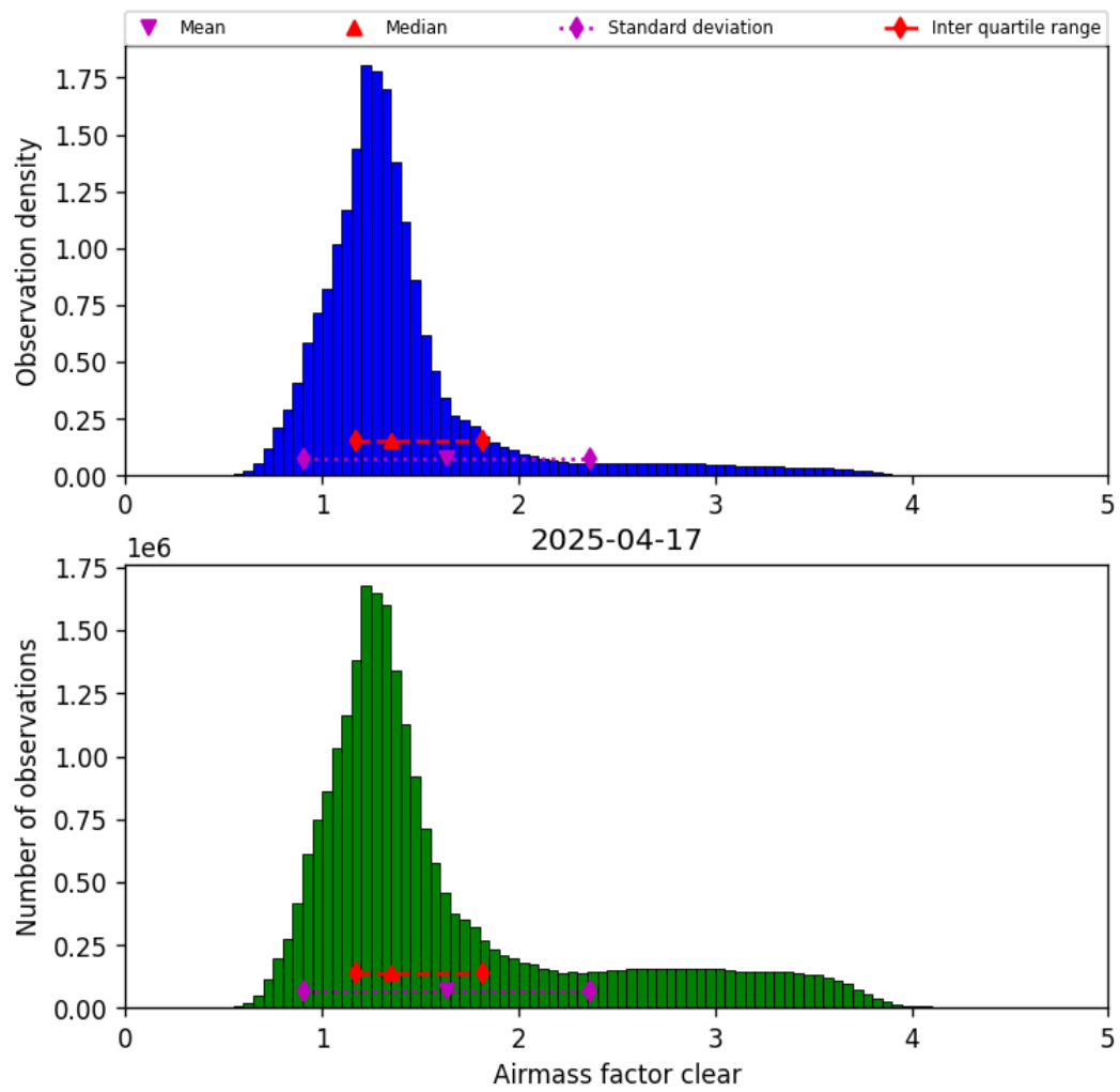
Figure 40: Histogram of “Airmass factor clear” for 2025-04-17 to 2025-04-18
