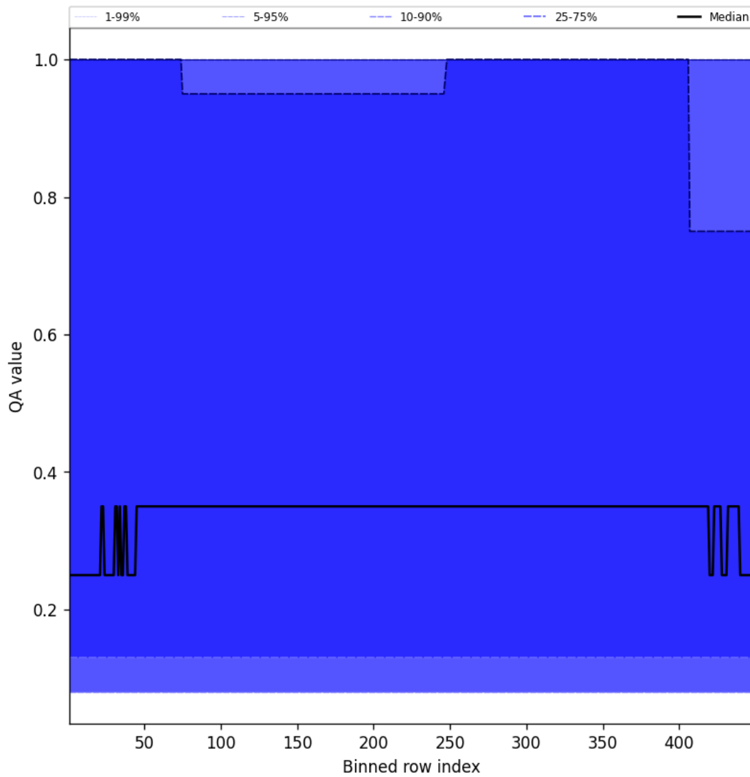
Figure 46: Along track statistics of “QA value” for 2025-04-17 to 2025-04-18
