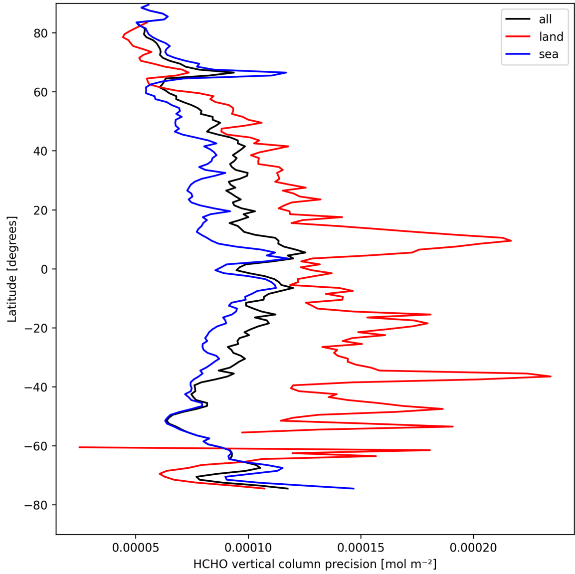
Figure 20: Zonal average of “HCHO vertical column precision” for 2025-04-17 to 2025-04-18.
