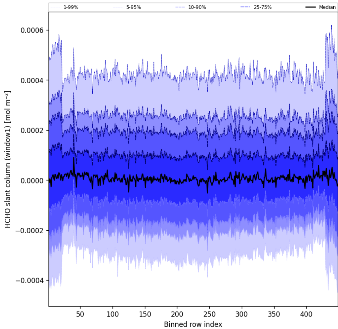
Figure 50: Along track statistics of “HCHO slant column (window1)” for 2025-04-17 to 2025-04-18
