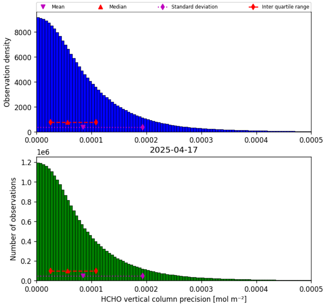
Figure 34: Histogram of “HCHO vertical column precision” for 2025-04-17 to 2025-04-18
