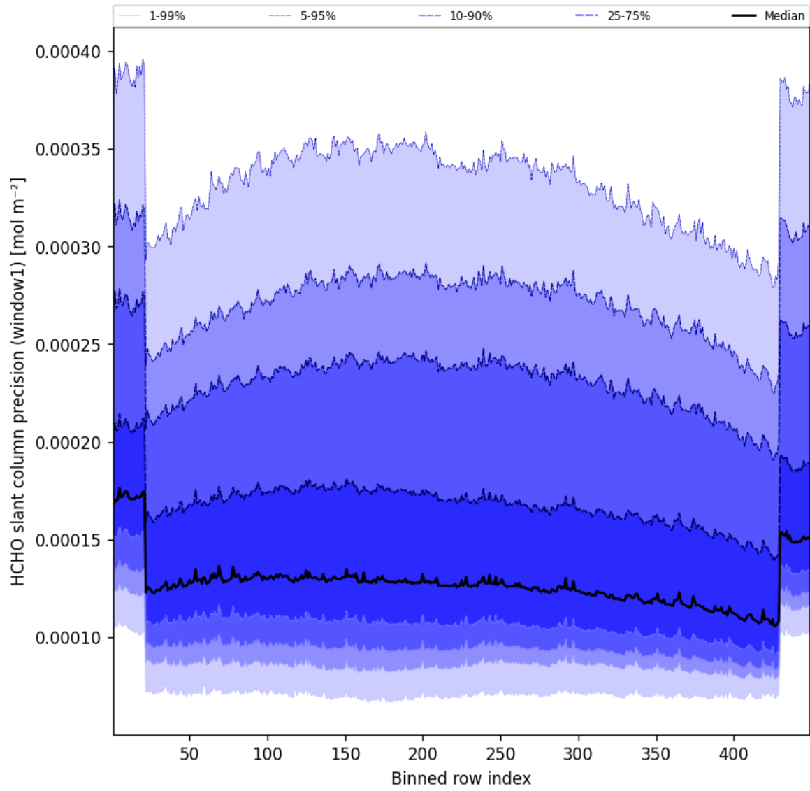
Figure 51: Along track statistics of “HCHO slant column precision (window1)” for 2025-04-17 to 2025-04-18
