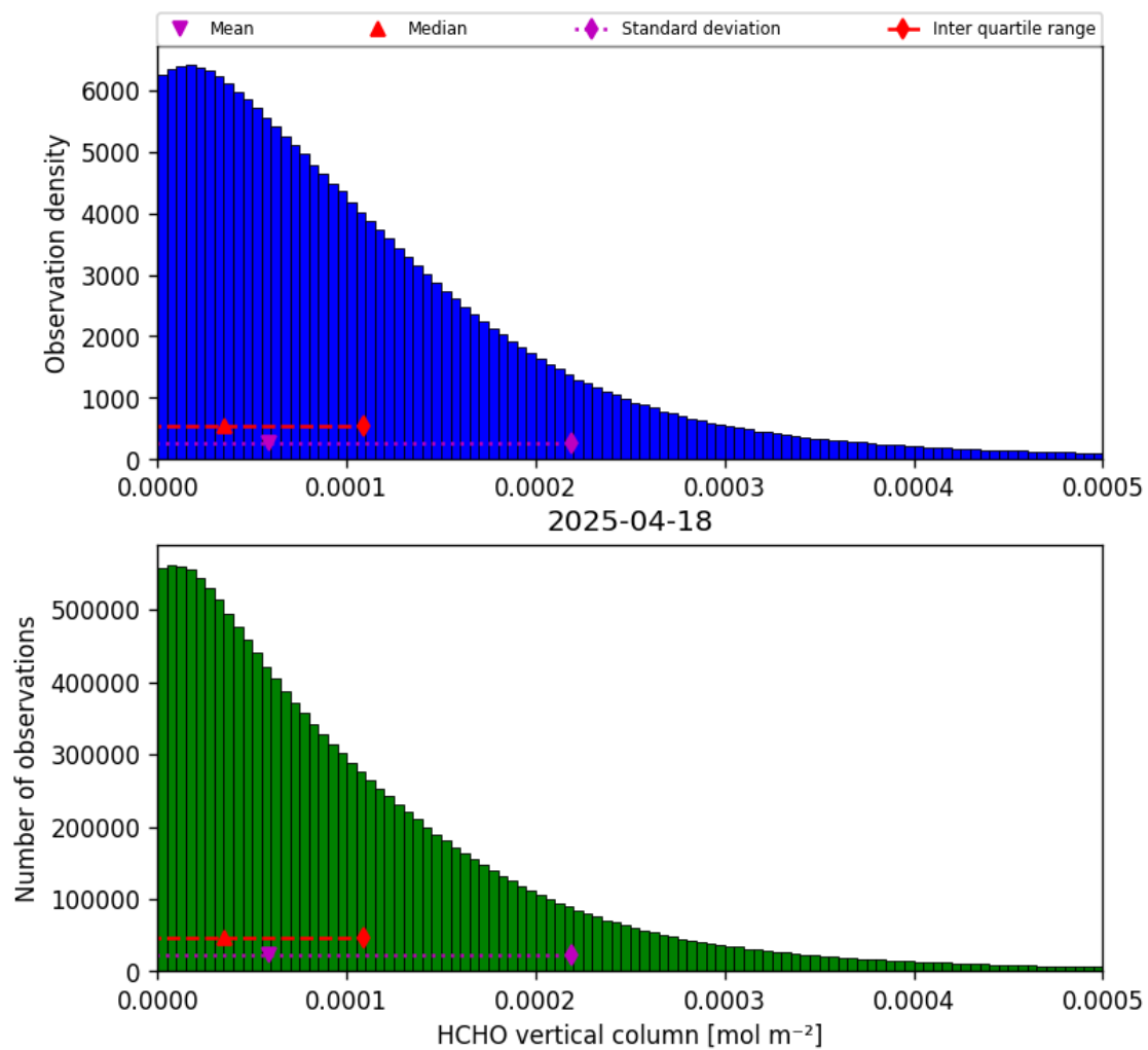
Figure 33: Histogram of “HCHO vertical column” for 2025-04-18 to 2025-04-19
