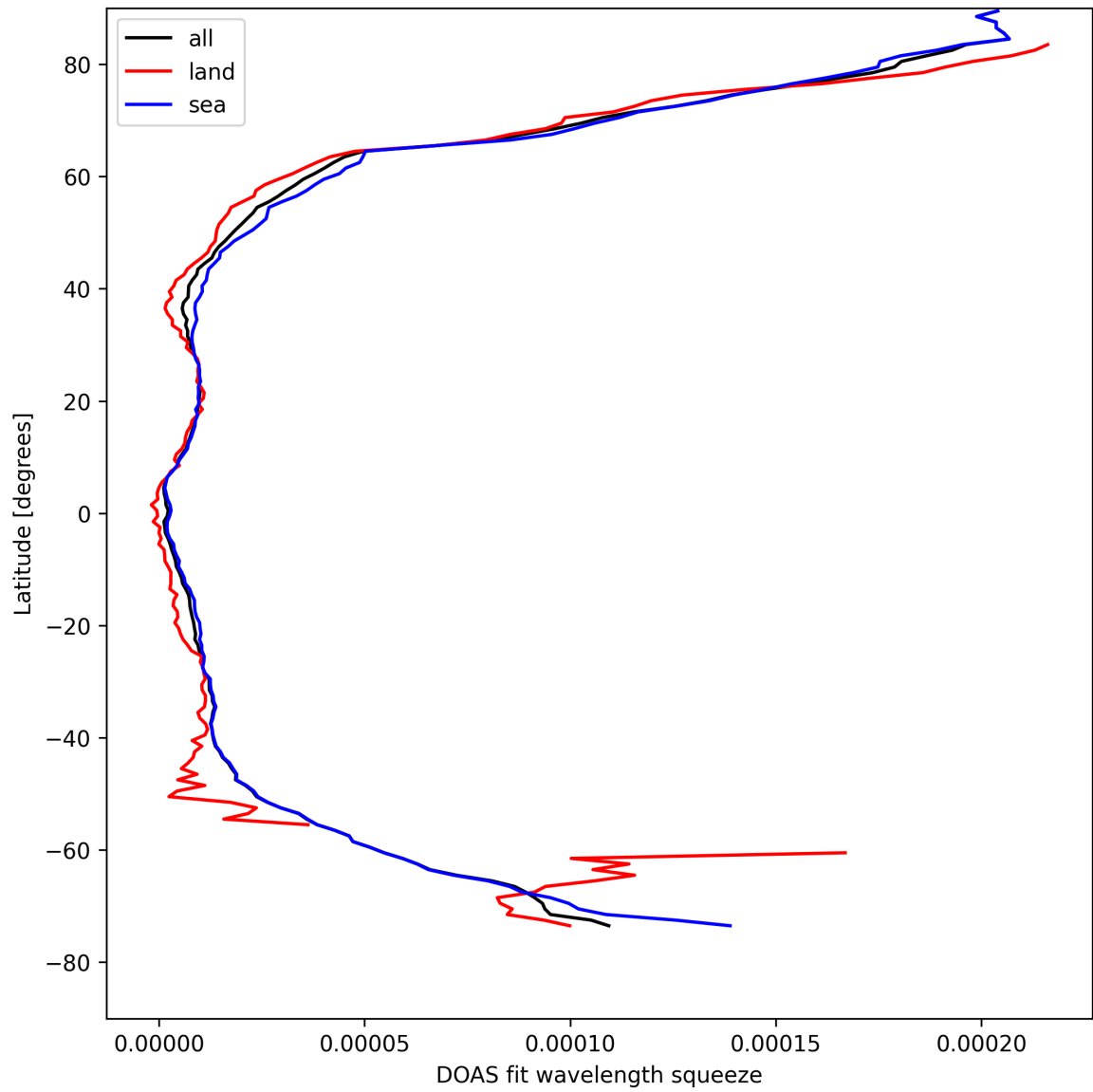
Figure 29: Zonal average of “DOAS fit wavelength squeeze” for 2025-04-18 to 2025-04-19.
