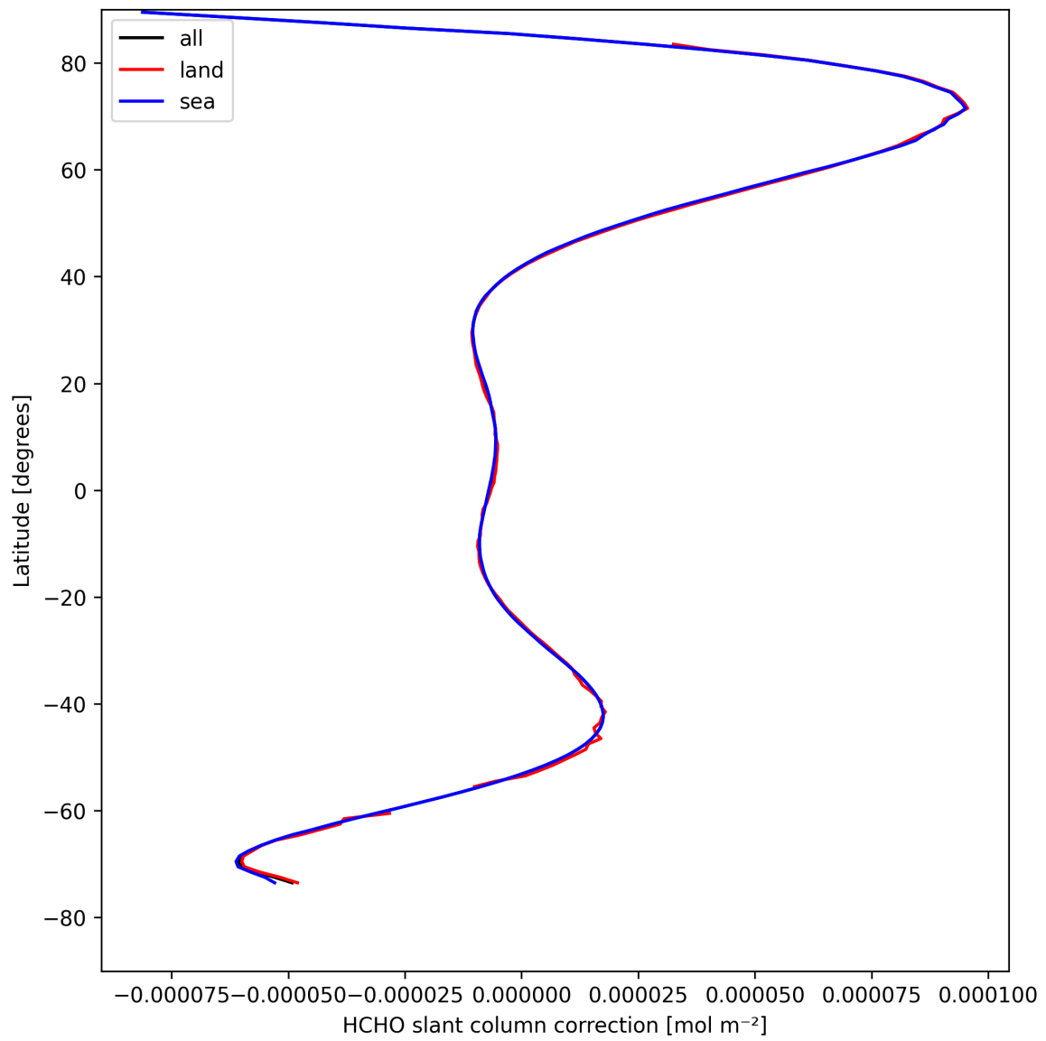
Figure 31: Zonal average of “HCHO slant column correction” for 2025-04-18 to 2025-04-19.
