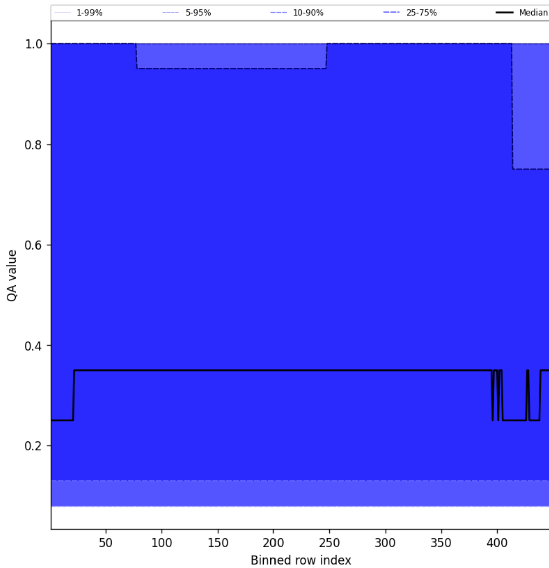
Figure 46: Along track statistics of “QA value” for 2025-04-18 to 2025-04-19
