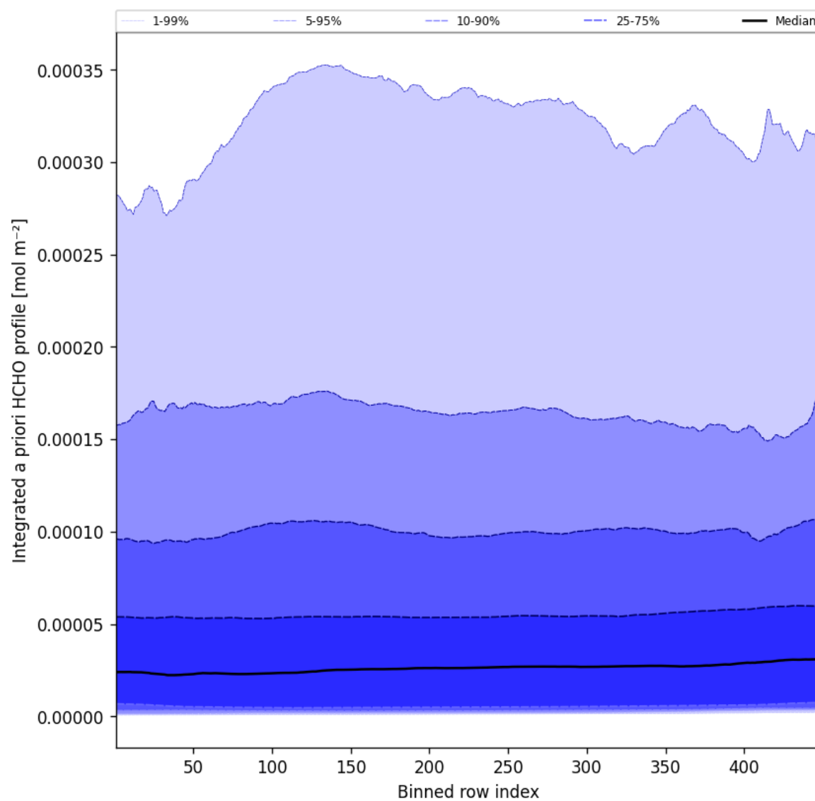
Figure 55: Along track statistics of “Integrated a priori HCHO profile” for 2025-04-18 to 2025-04-19
