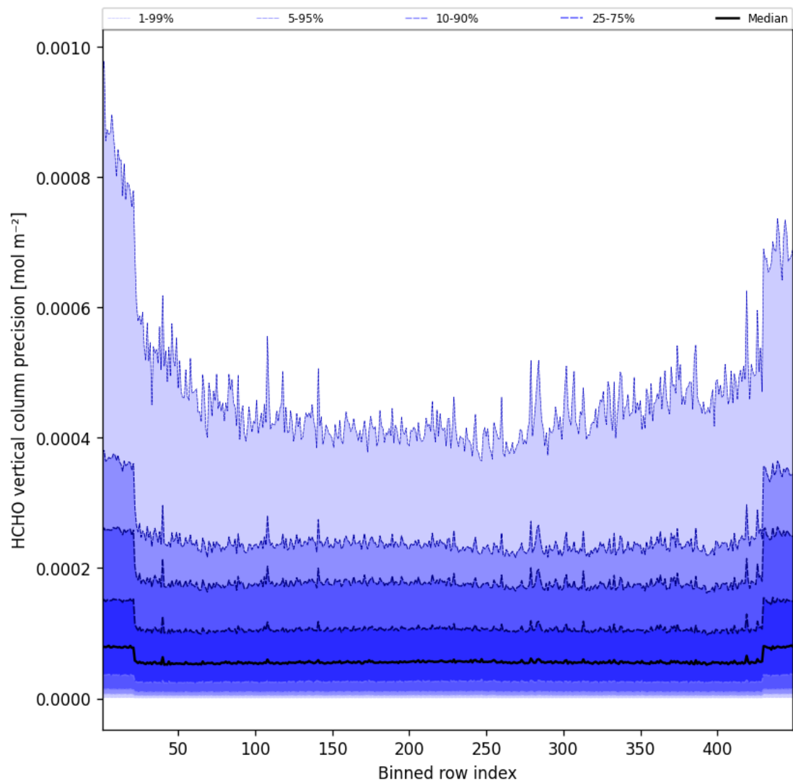
Figure 48: Along track statistics of “HCHO vertical column precision” for 2025-04-18 to 2025-04-19
