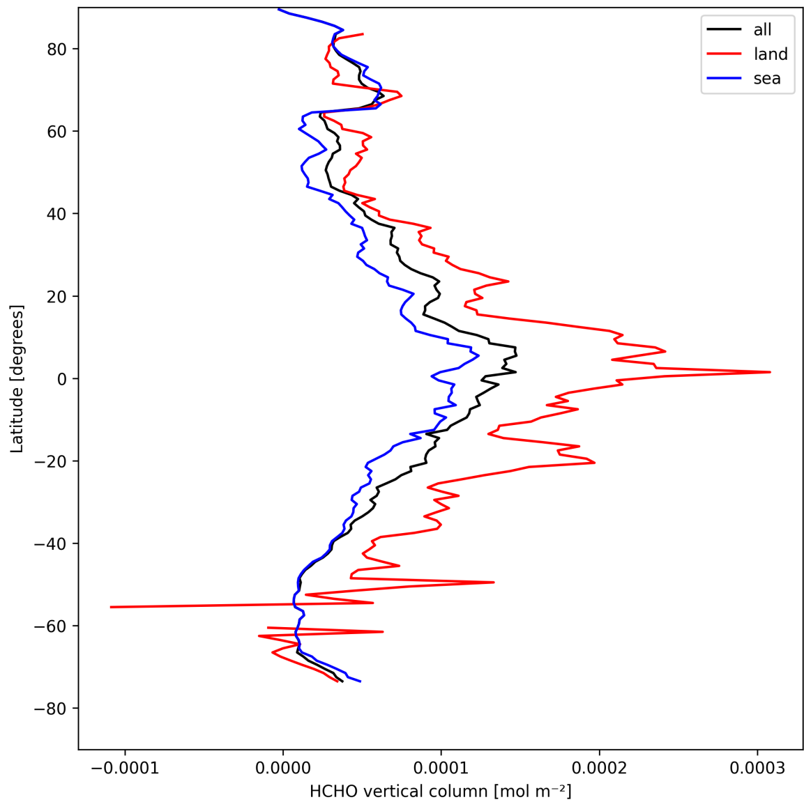
Figure 19: Zonal average of “HCHO vertical column” for 2025-04-18 to 2025-04-19.
