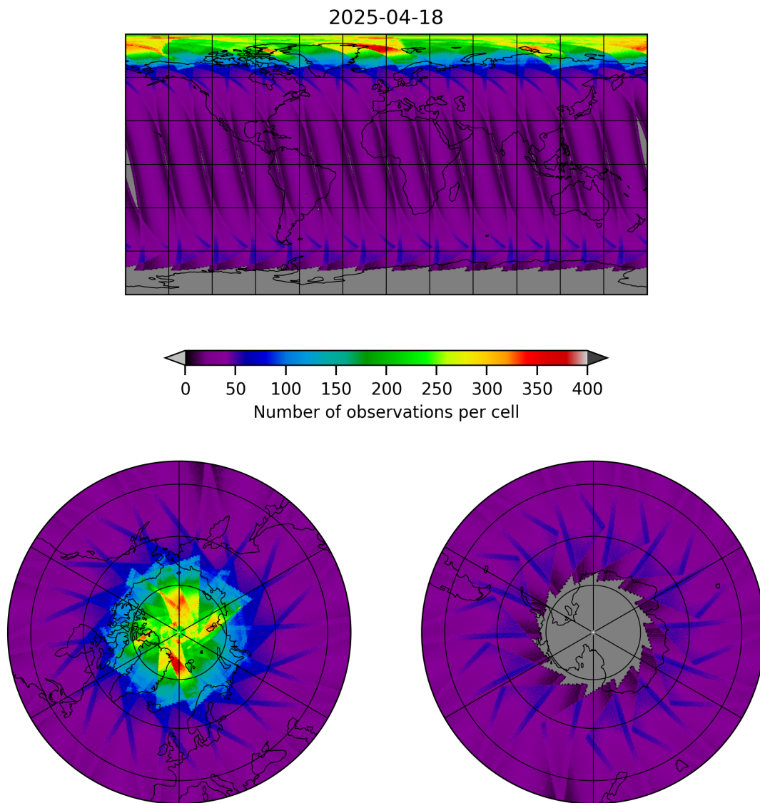
Figure 17: Map of the number of observations for 2025-04-18 to 2025-04-19
