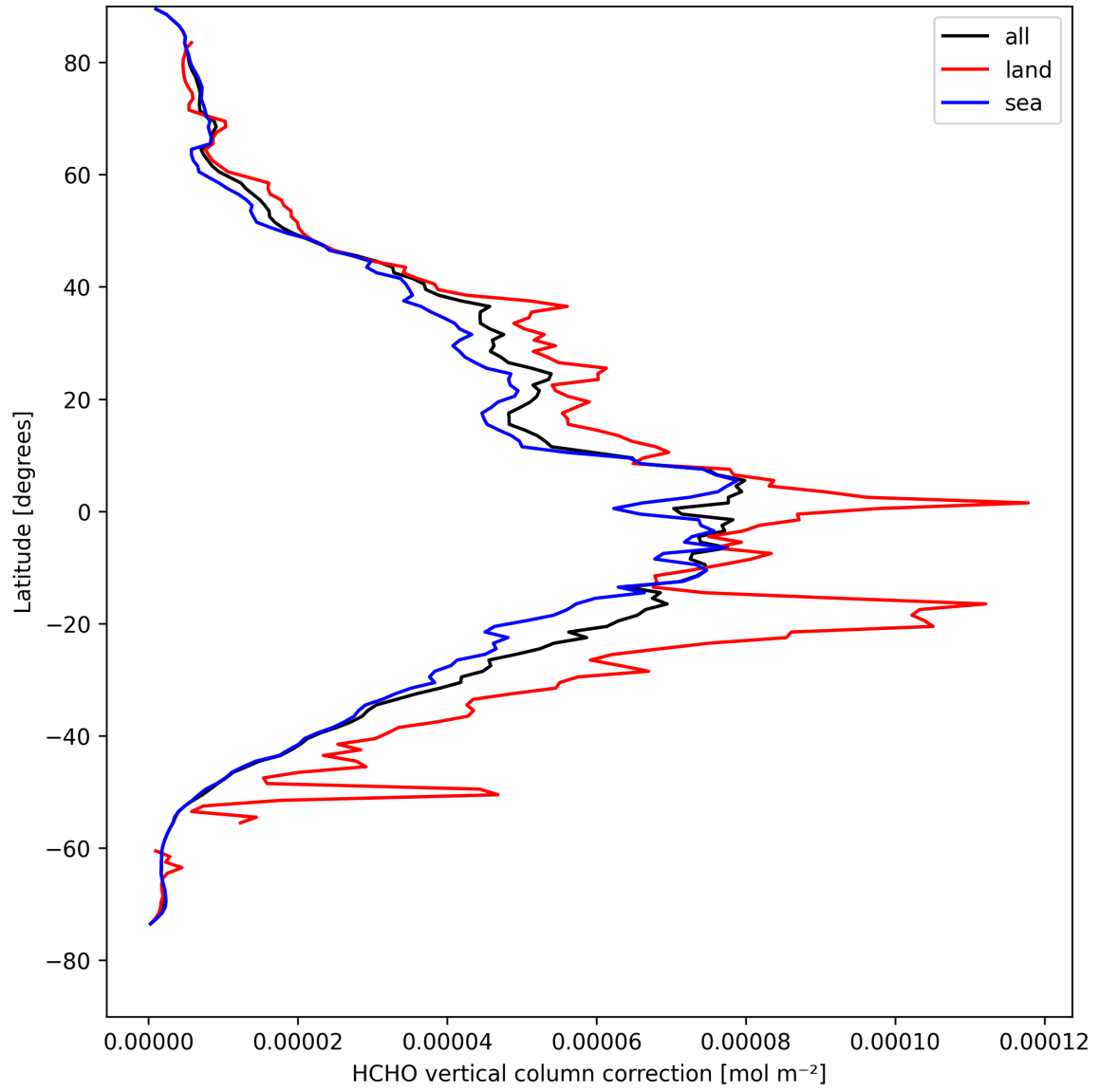
Figure 21: Zonal average of “HCHO vertical column correction” for 2025-04-18 to 2025-04-19.
