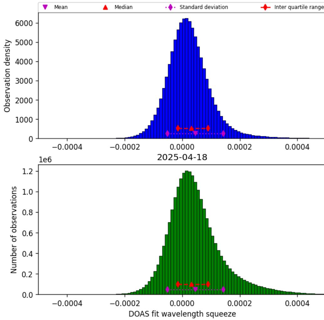
Figure 43: Histogram of “DOAS fit wavelength squeeze” for 2025-04-18 to 2025-04-19
