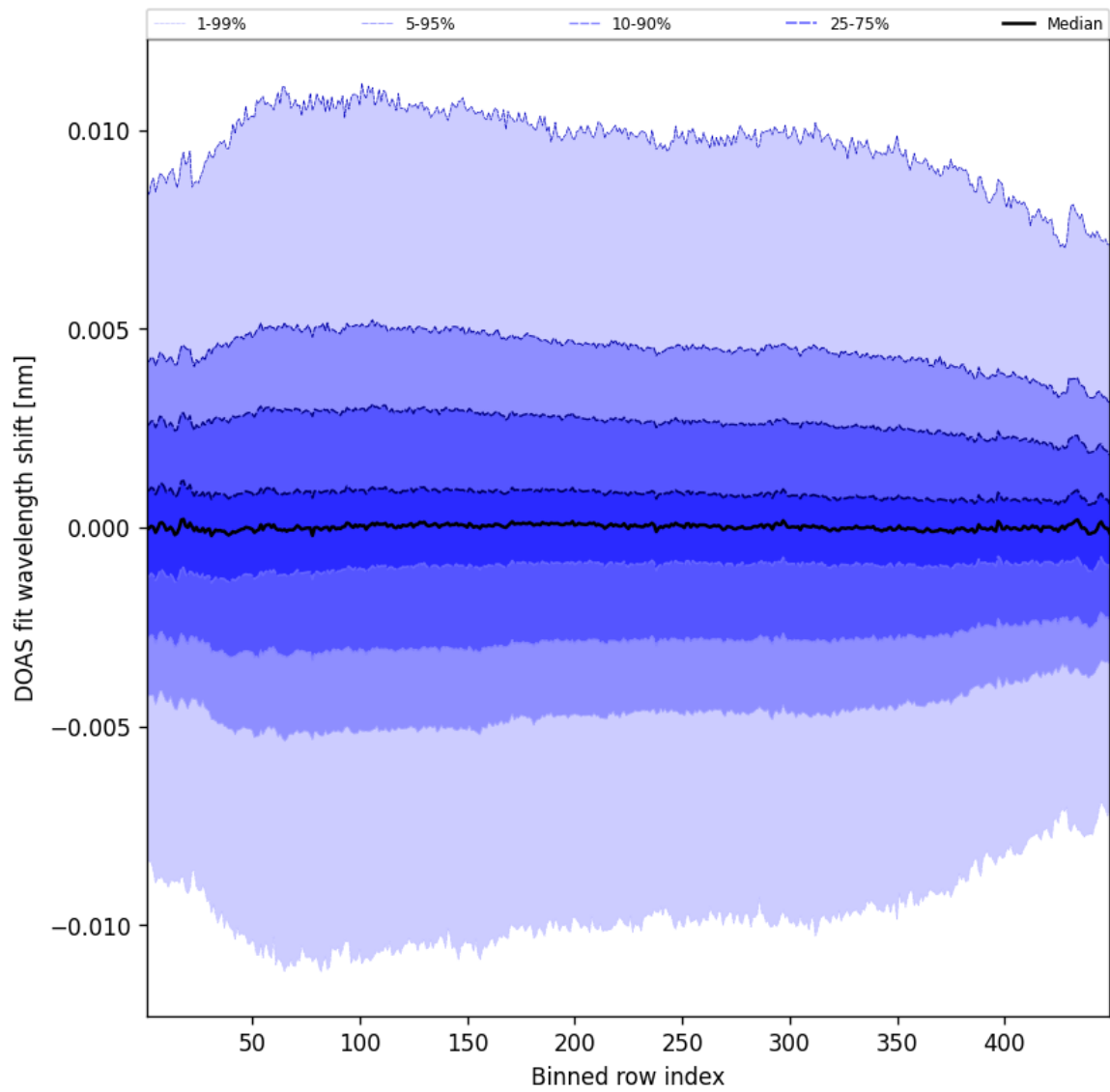
Figure 56: Along track statistics of “DOAS fit wavelength shift” for 2025-04-18 to 2025-04-19
