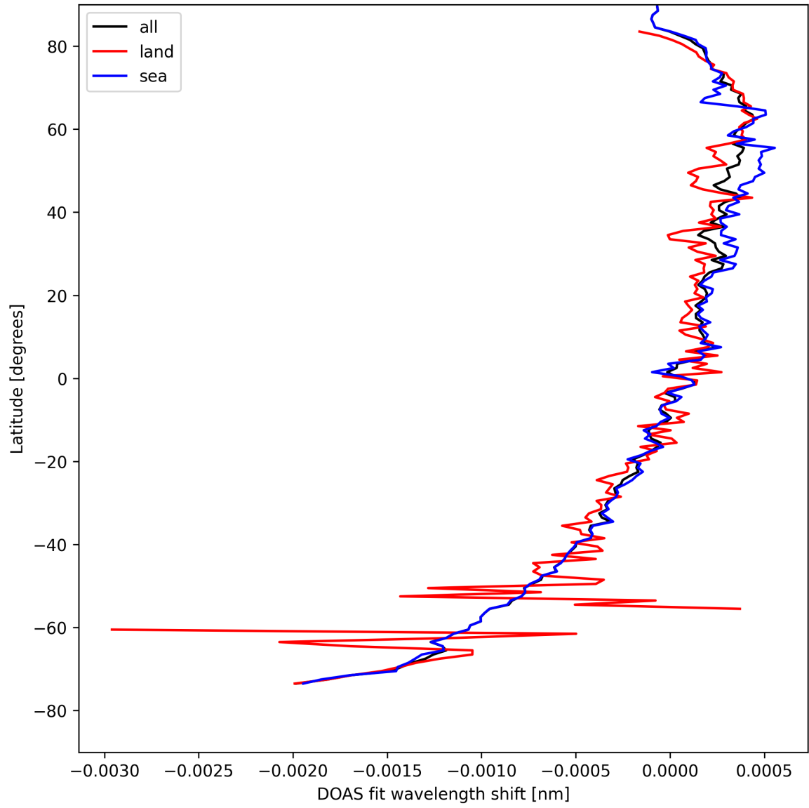
Figure 28: Zonal average of "DOAS fit wavelength shift" for 2025-04-18 to 2025-04-19.
