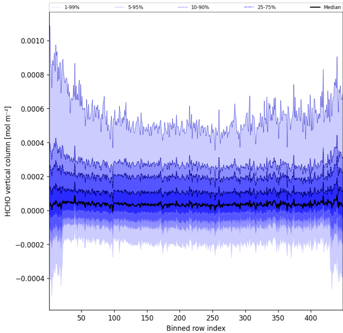
Figure 47: Along track statistics of “HCHO vertical column” for 2025-04-18 to 2025-04-19
