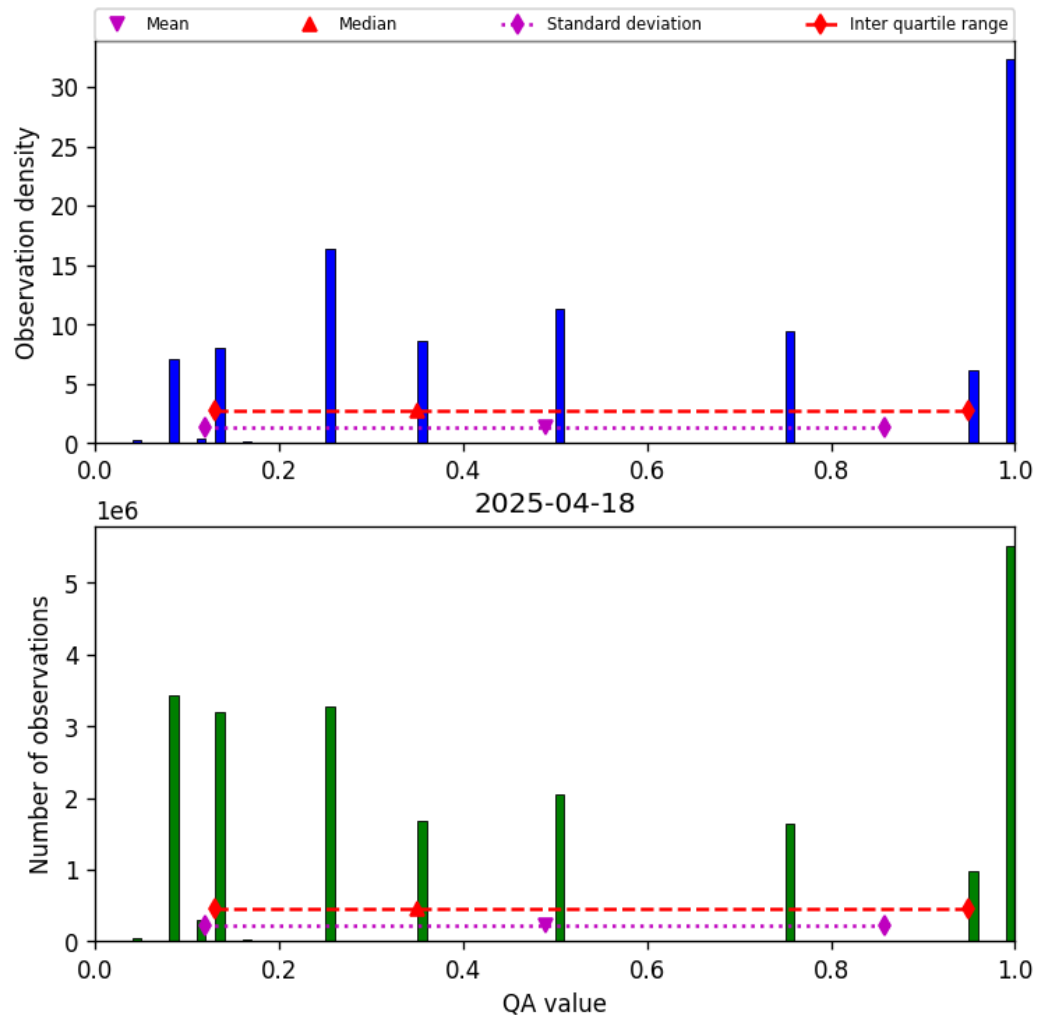
Figure 32: Histogram of “QA value” for 2025-04-18 to 2025-04-19
