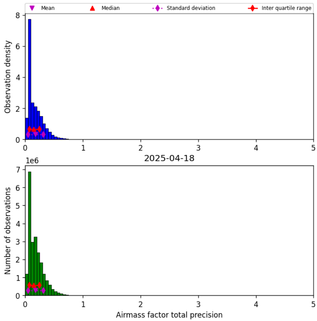
Figure 39: Histogram of “Airmass factor total precision” for 2025-04-18 to 2025-04-19
