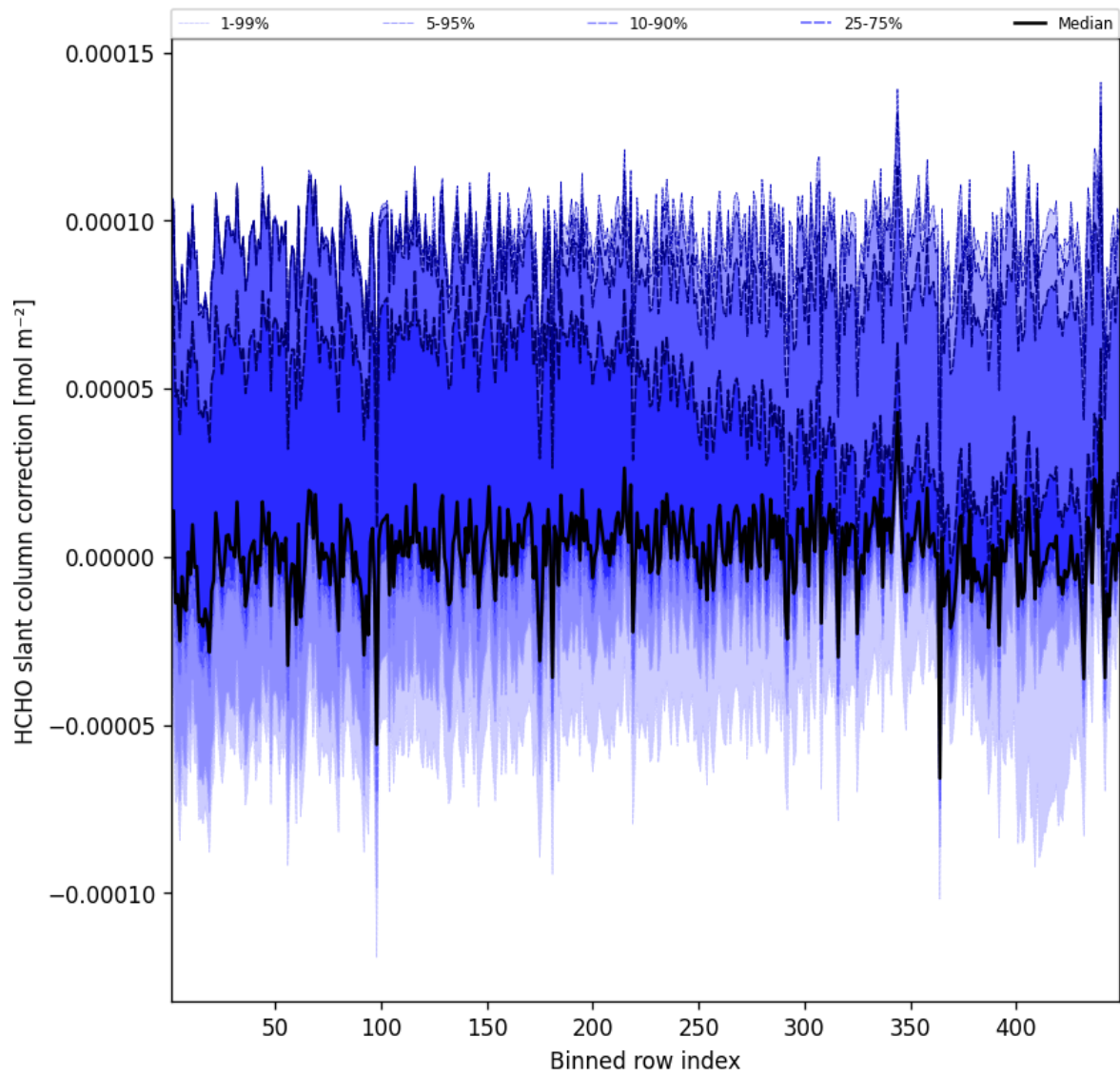
Figure 59: Along track statistics of “HCHO slant column correction” for 2025-04-18 to 2025-04-19
