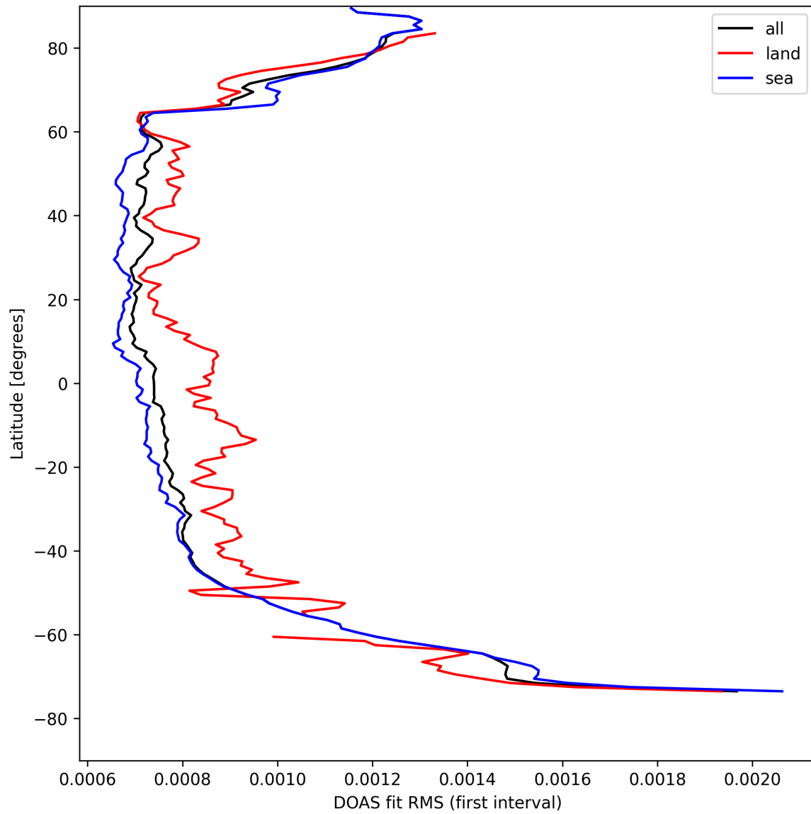
Figure 30: Zonal average of “DOAS fit RMS (first interval)” for 2025-04-18 to 2025-04-19.
