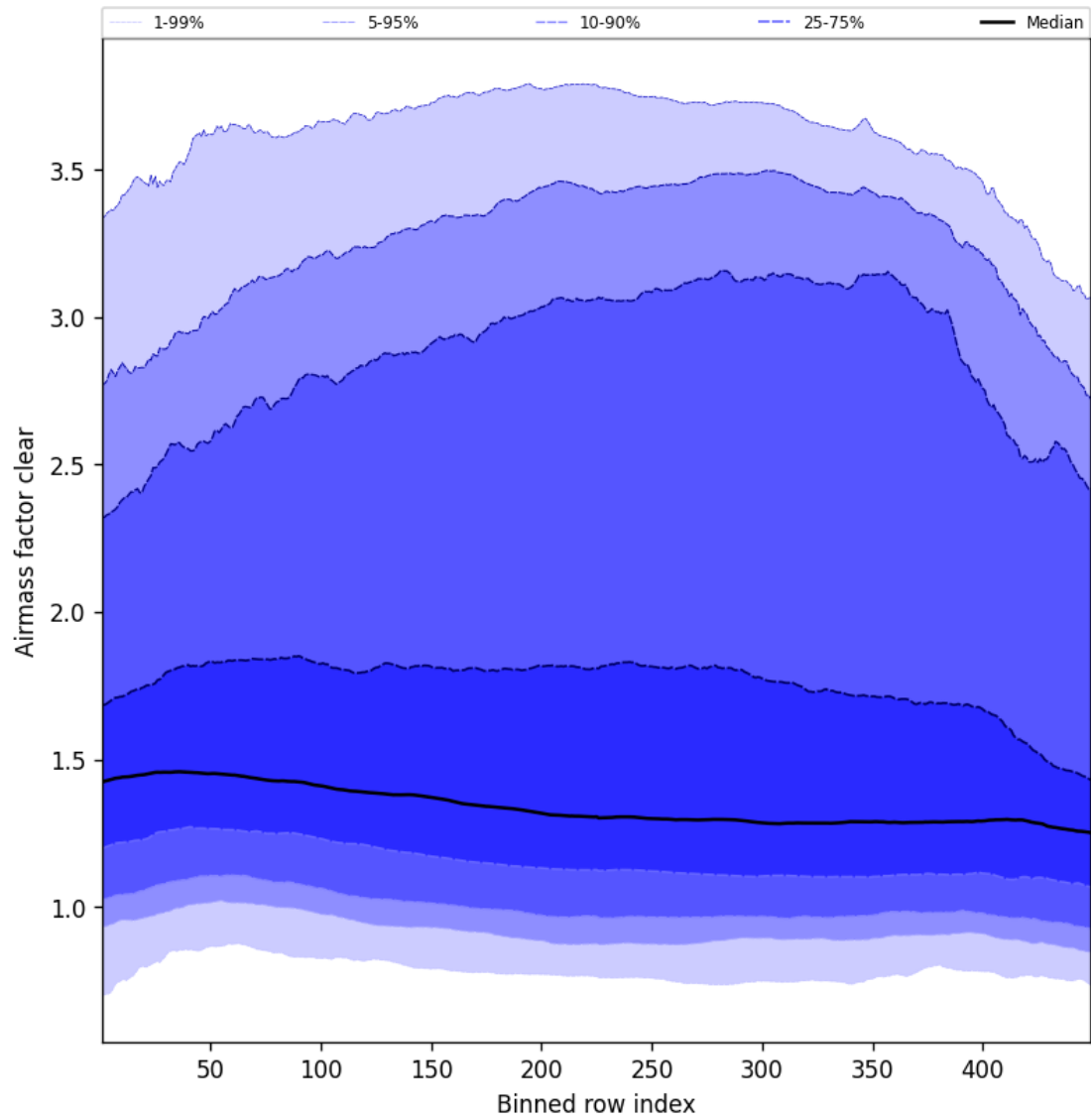
Figure 54: Along track statistics of “Airmass factor clear” for 2025-04-18 to 2025-04-19
