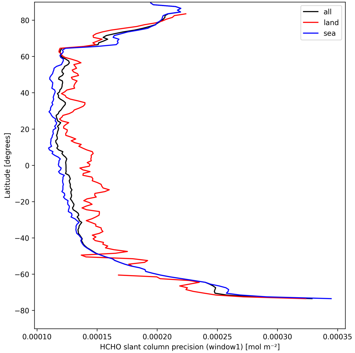
Figure 23: Zonal average of “HCHO slant column precision (window1)” for 2025-04-18 to 2025-04-19.
