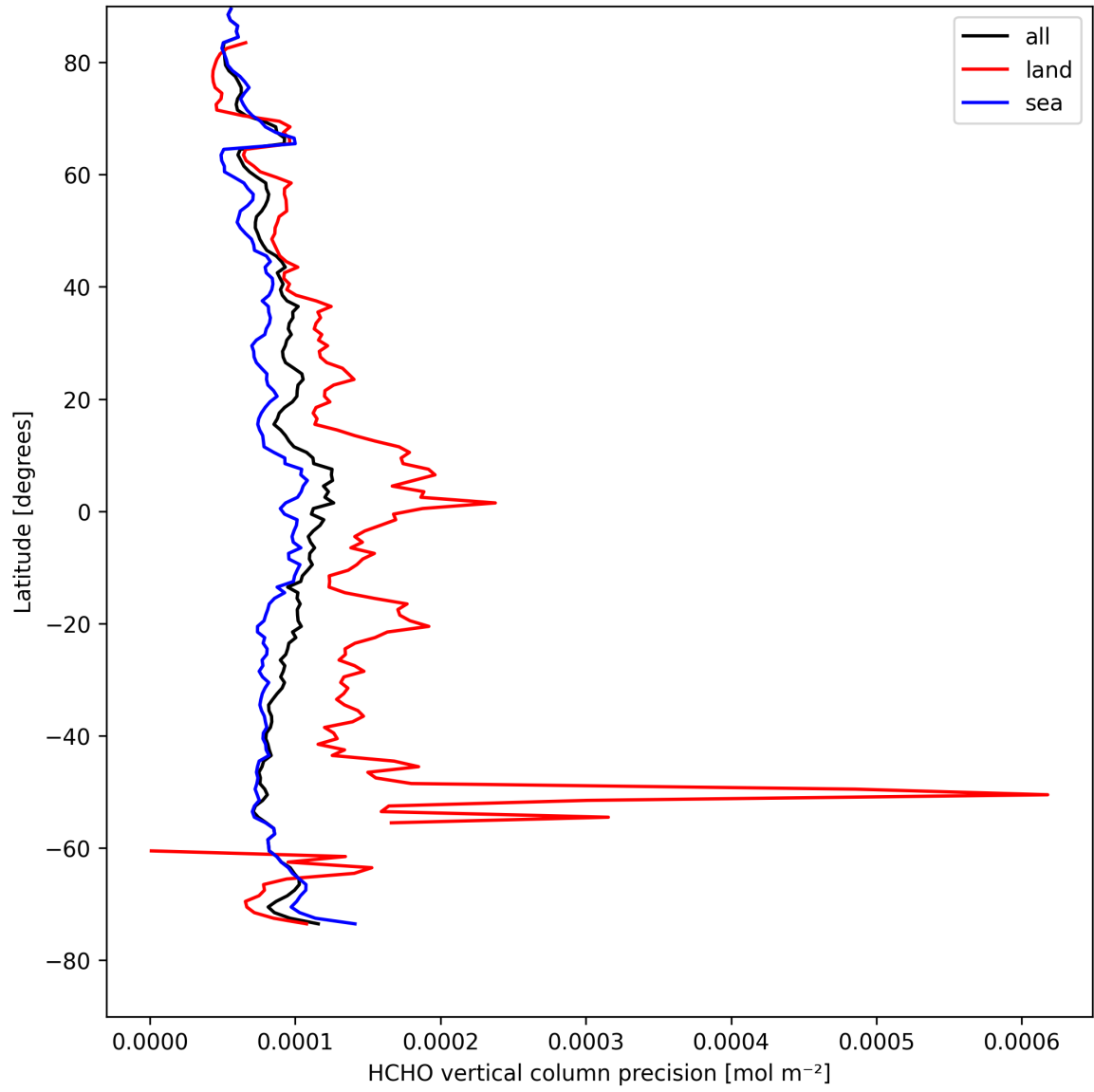
Figure 20: Zonal average of “HCHO vertical column precision” for 2025-04-18 to 2025-04-19.
