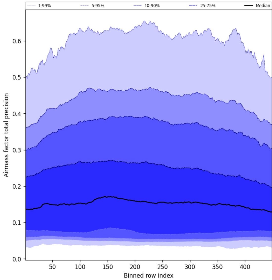
Figure 53: Along track statistics of “Airmass factor total precision” for 2025-04-18 to 2025-04-19
