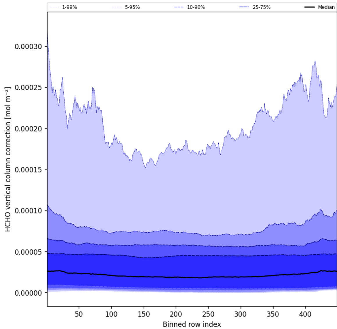
Figure 49: Along track statistics of “HCHO vertical column correction” for 2025-04-18 to 2025-04-19
