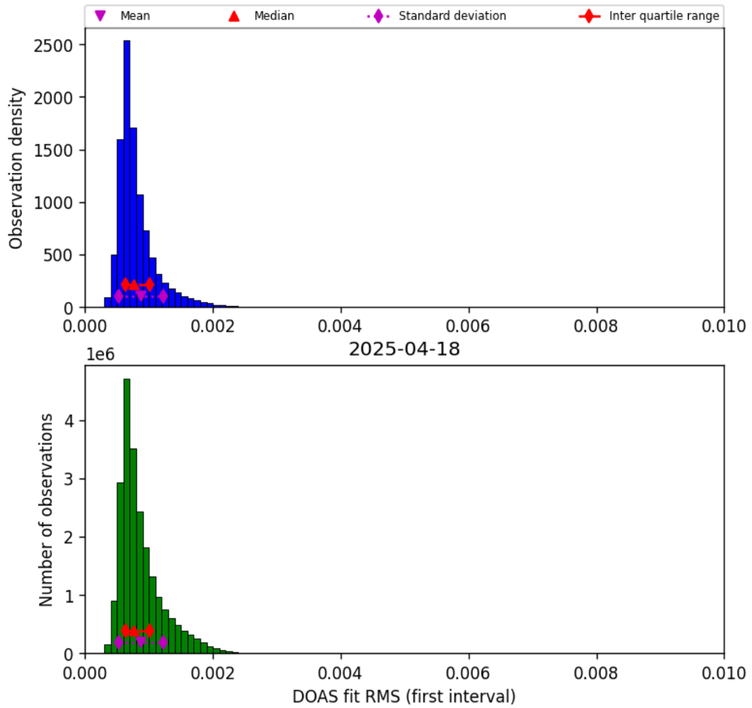
Figure 44: Histogram of “DOAS fit RMS (first interval)” for 2025-04-18 to 2025-04-19
