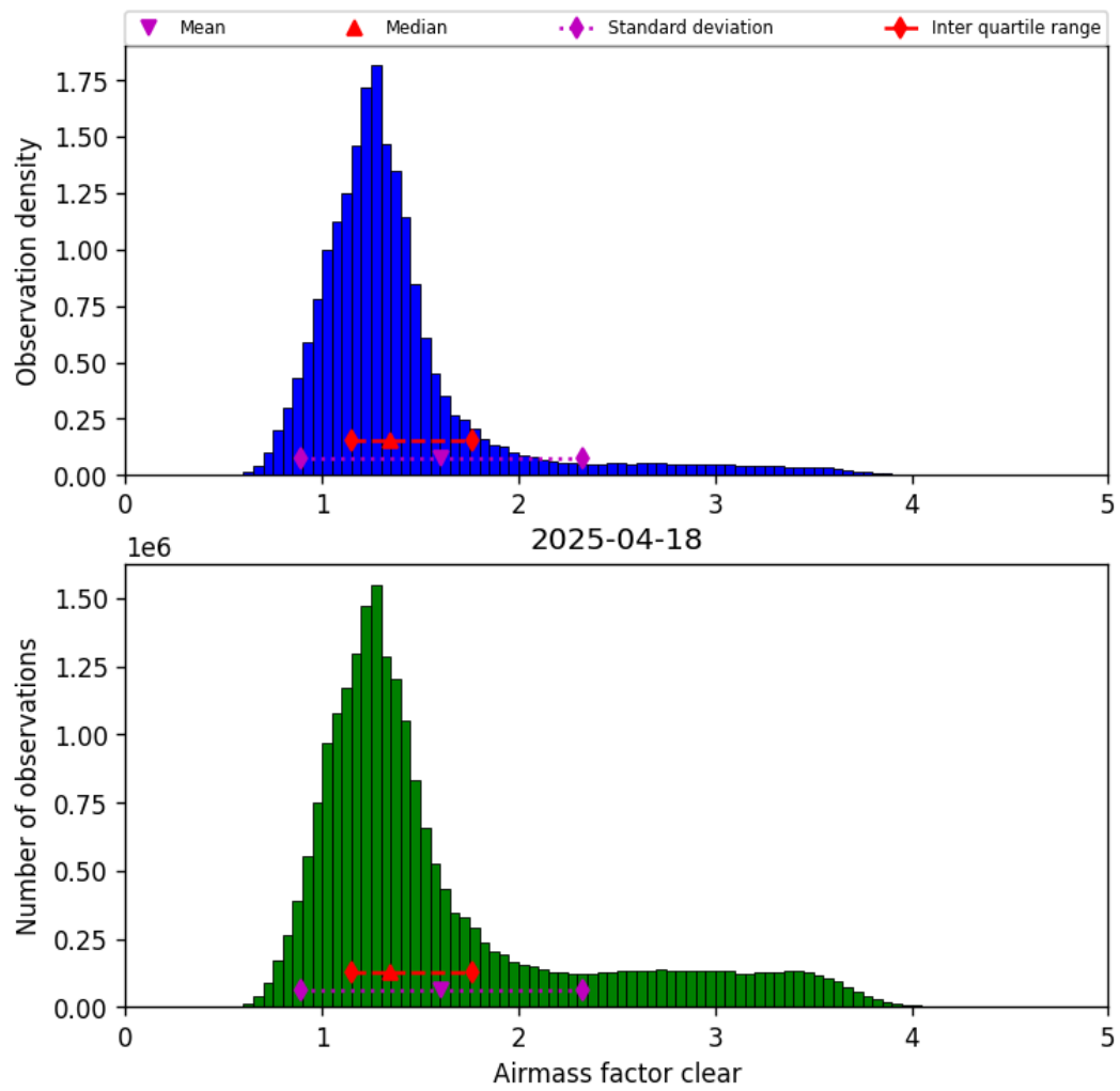
Figure 40: Histogram of “Airmass factor clear” for 2025-04-18 to 2025-04-19
