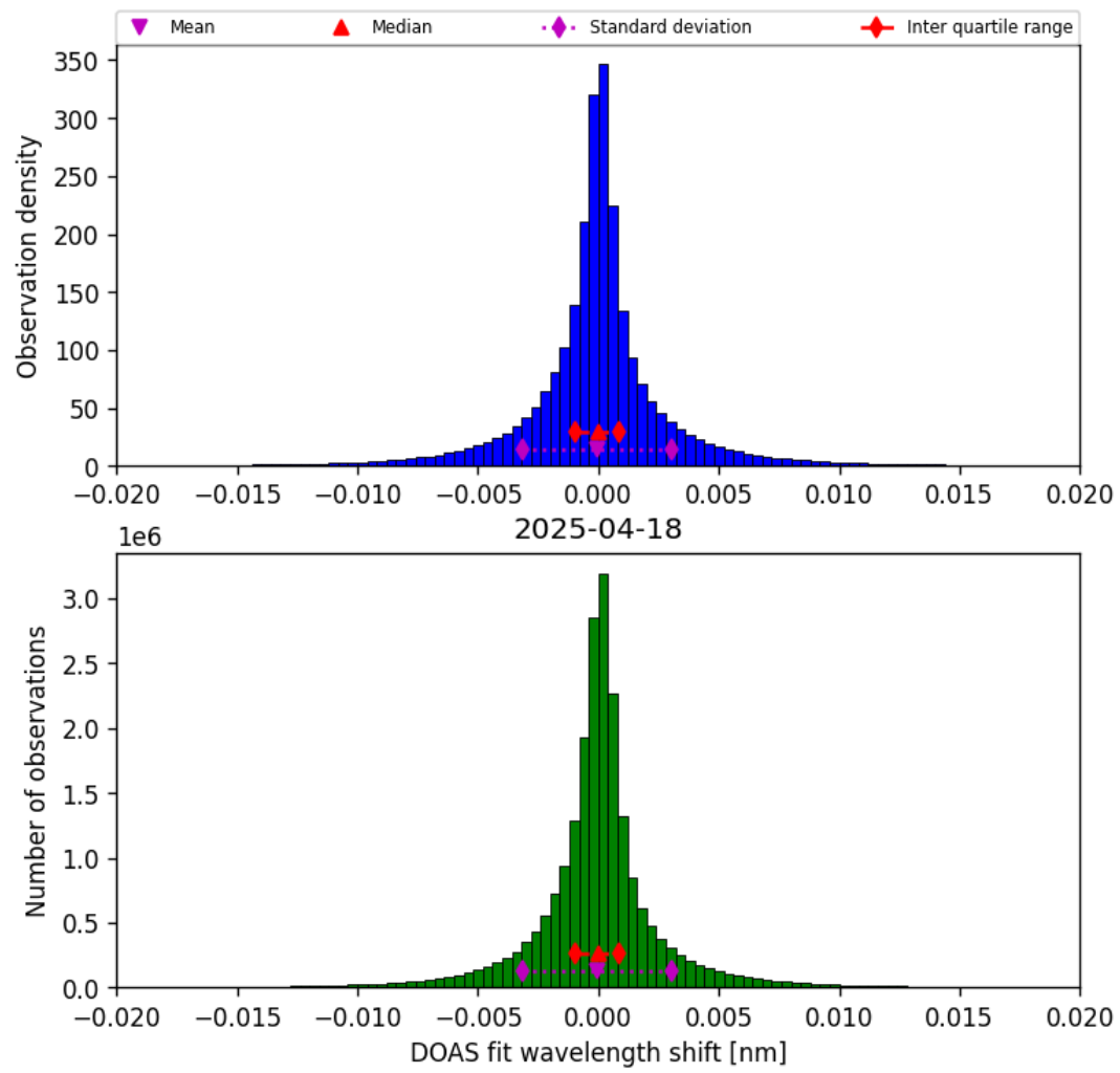
Figure 42: Histogram of “DOAS fit wavelength shift” for 2025-04-18 to 2025-04-19
