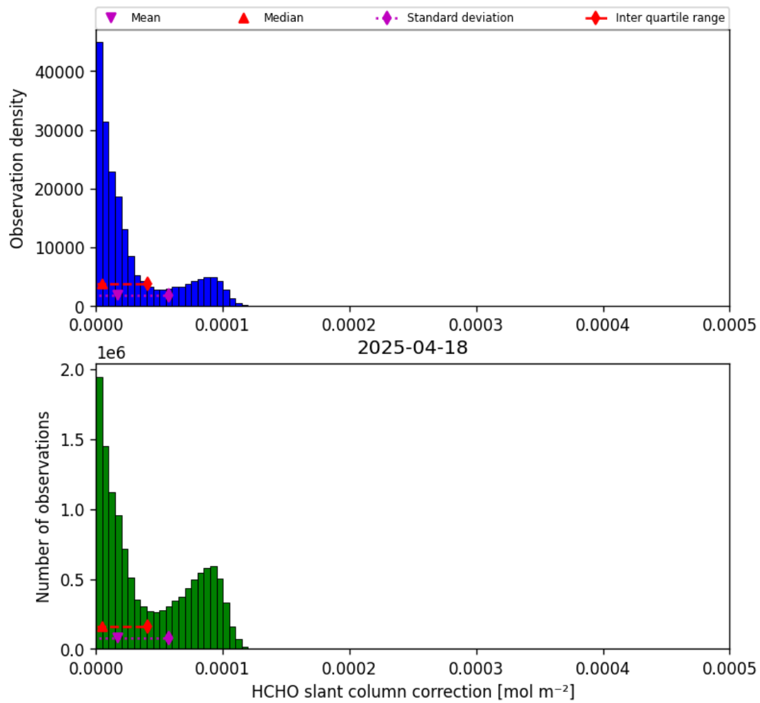
Figure 45: Histogram of “HCHO slant column correction” for 2025-04-18 to 2025-04-19
