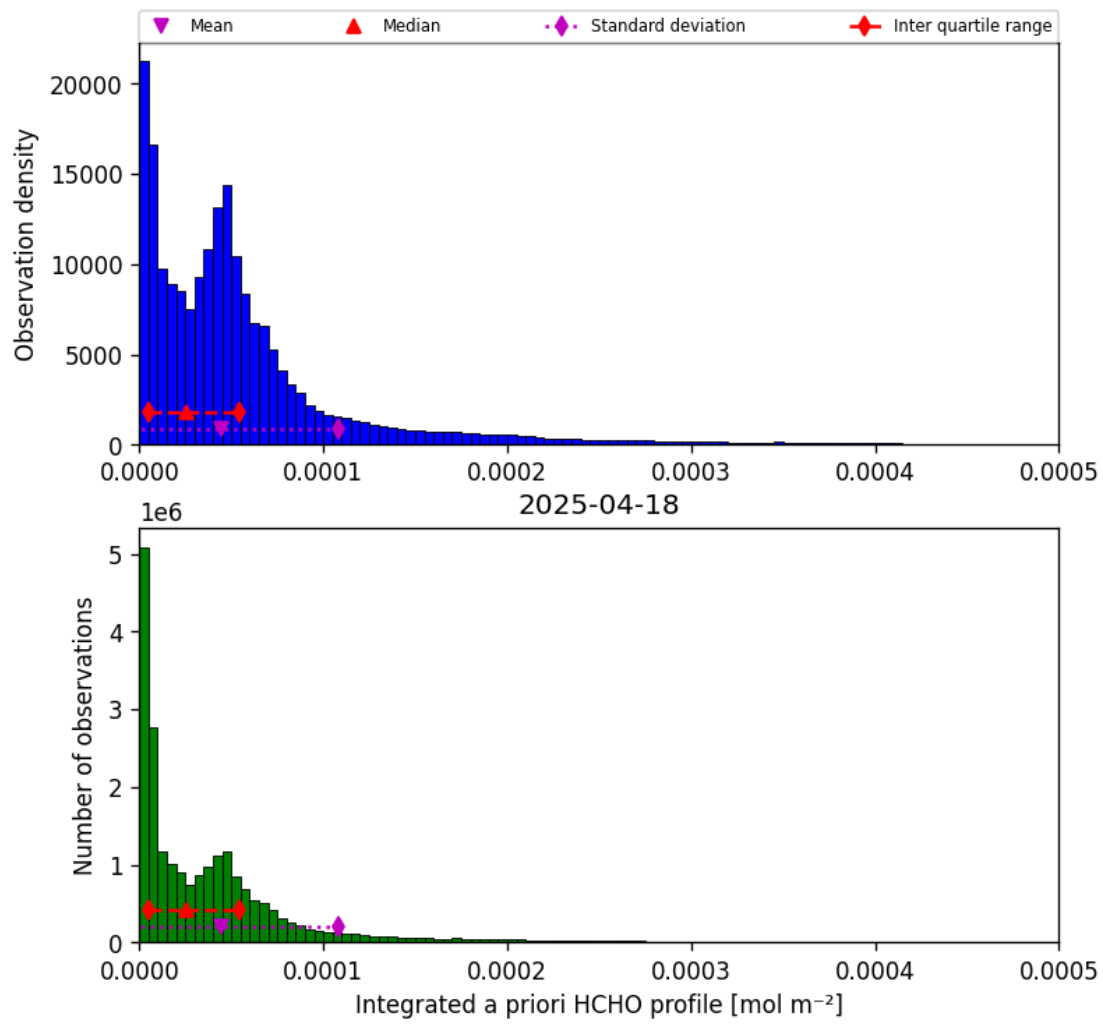
Figure 41: Histogram of “Integrated a priori HCHO profile” for 2025-04-18 to 2025-04-19
