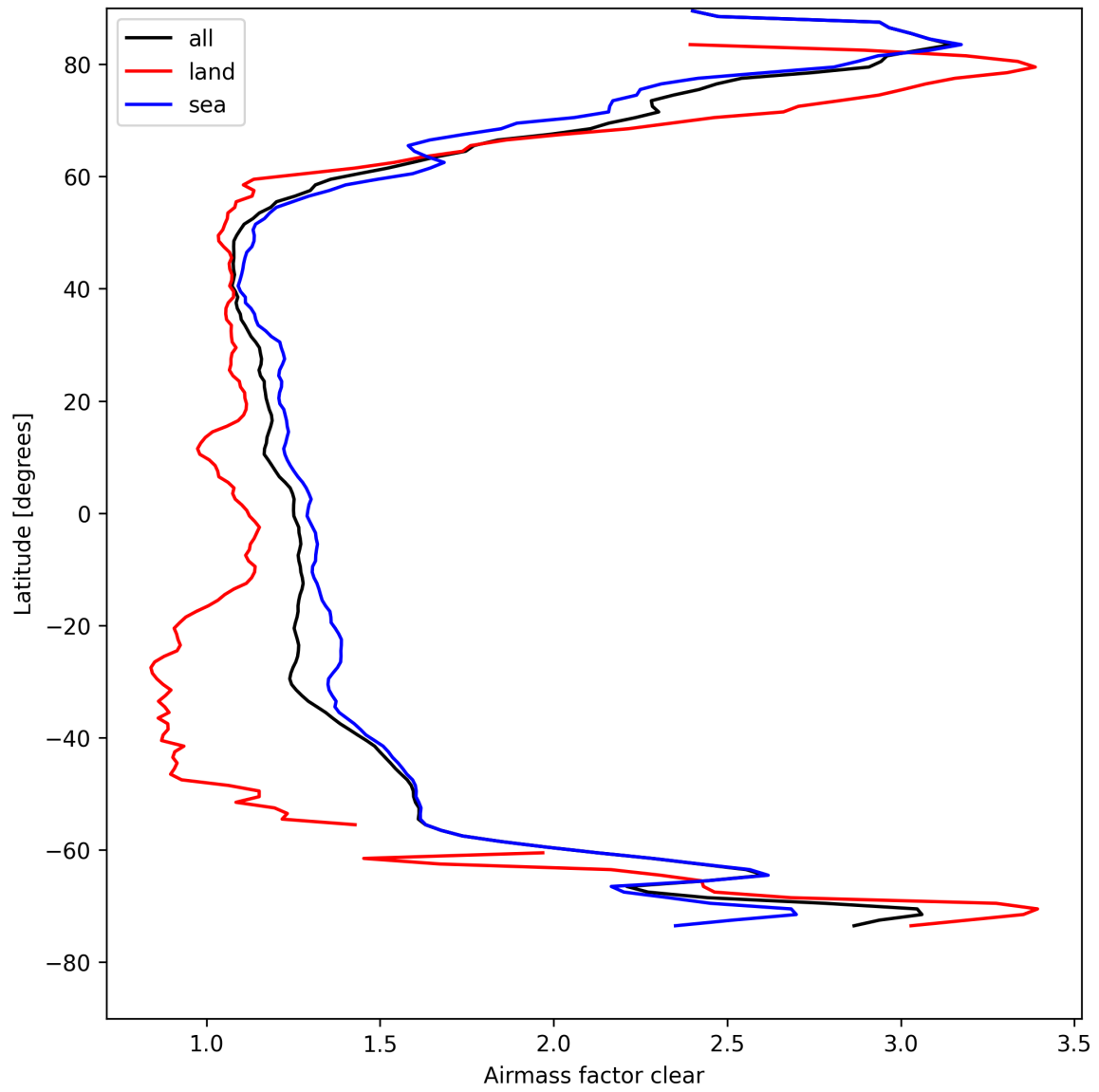
Figure 26: Zonal average of “Airmass factor clear” for 2025-04-18 to 2025-04-19.
