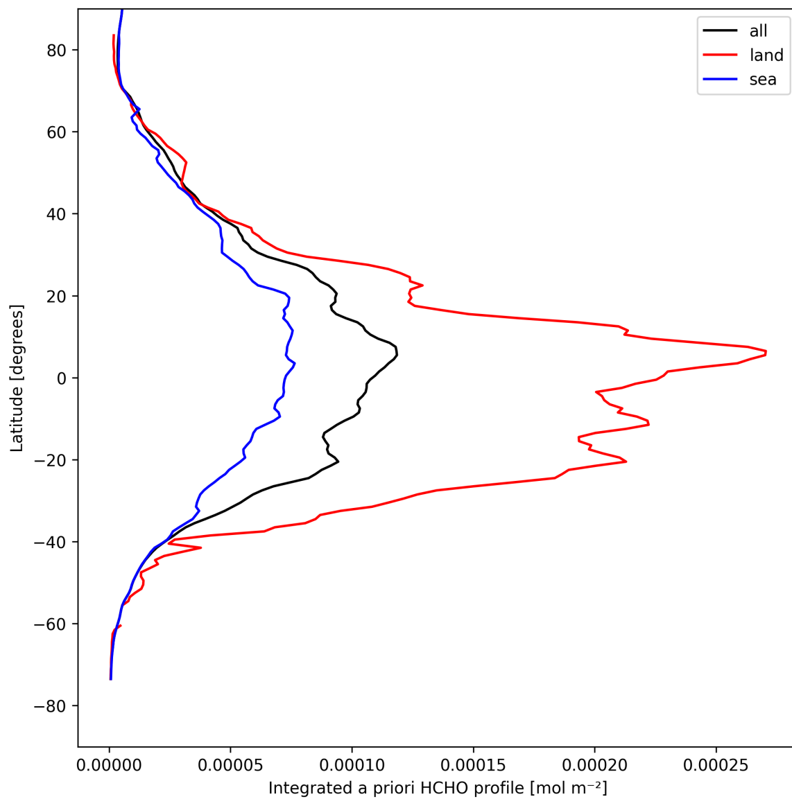
Figure 27: Zonal average of “Integrated a priori HCHO profile” for 2025-04-18 to 2025-04-19.
