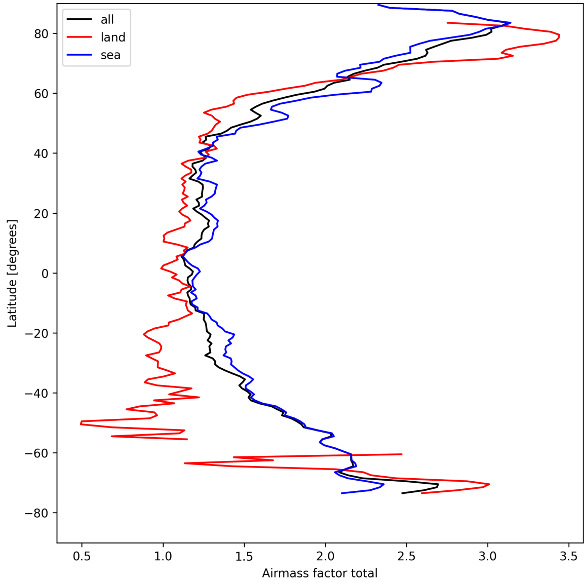
Figure 24: Zonal average of “Airmass factor total” for 2025-04-18 to 2025-04-19.
