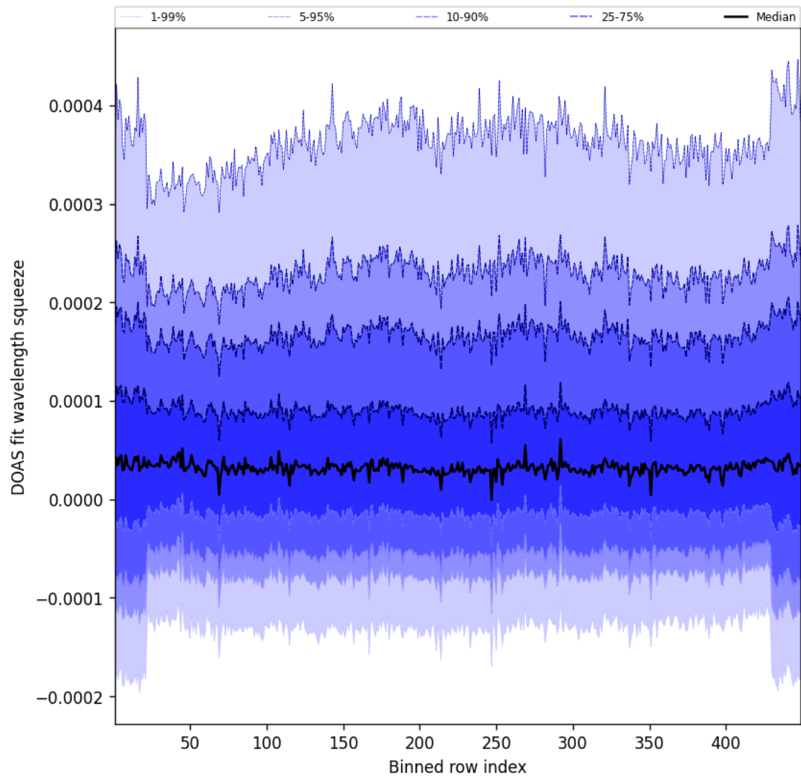
Figure 57: Along track statistics of “DOAS fit wavelength squeeze” for 2025-04-18 to 2025-04-19
