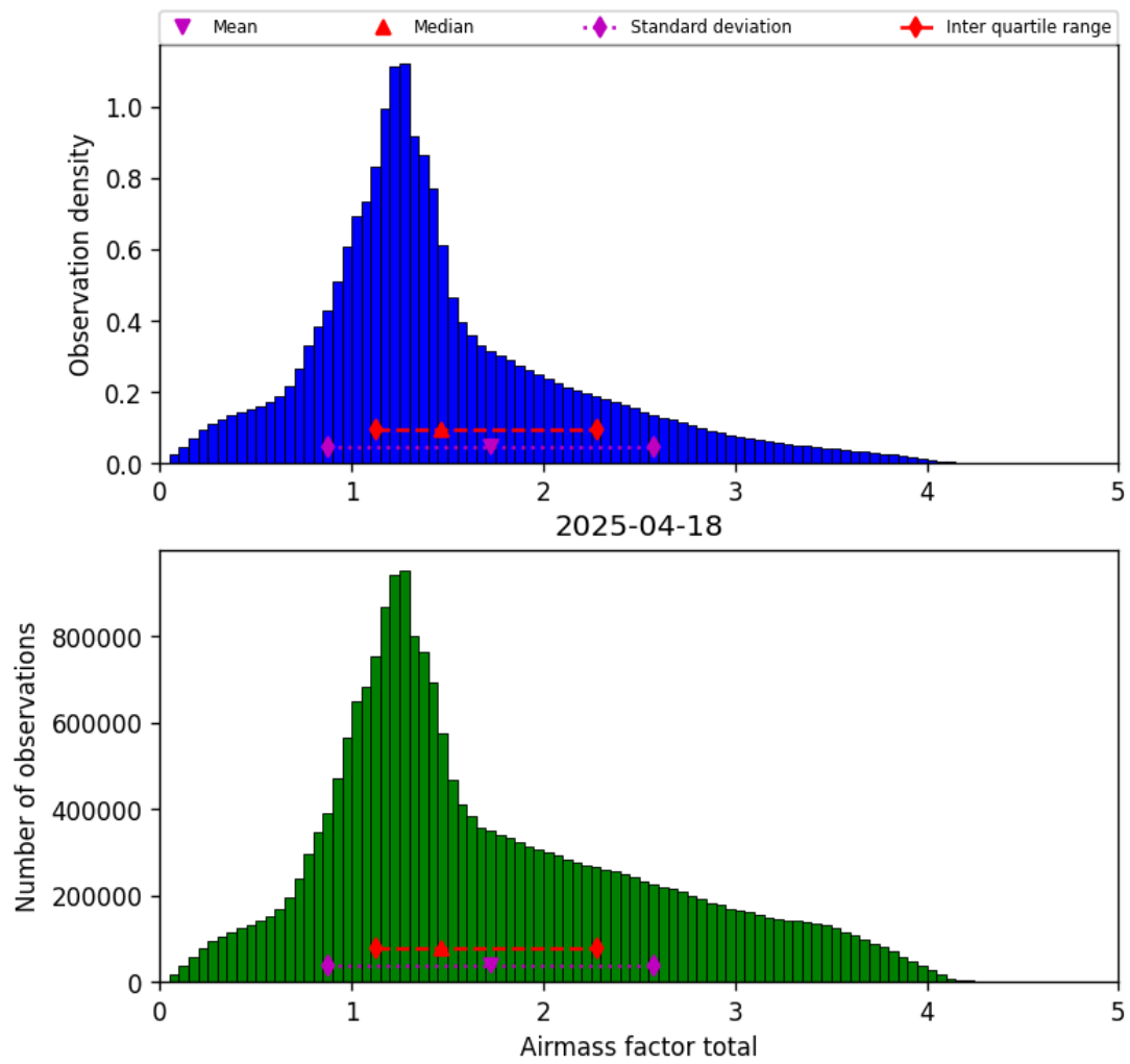
Figure 38: Histogram of “Airmass factor total” for 2025-04-18 to 2025-04-19
