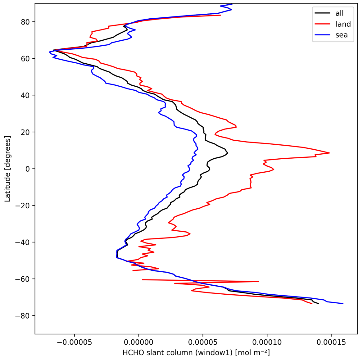
Figure 22: Zonal average of “HCHO slant column (window1)” for 2025-04-18 to 2025-04-19.
