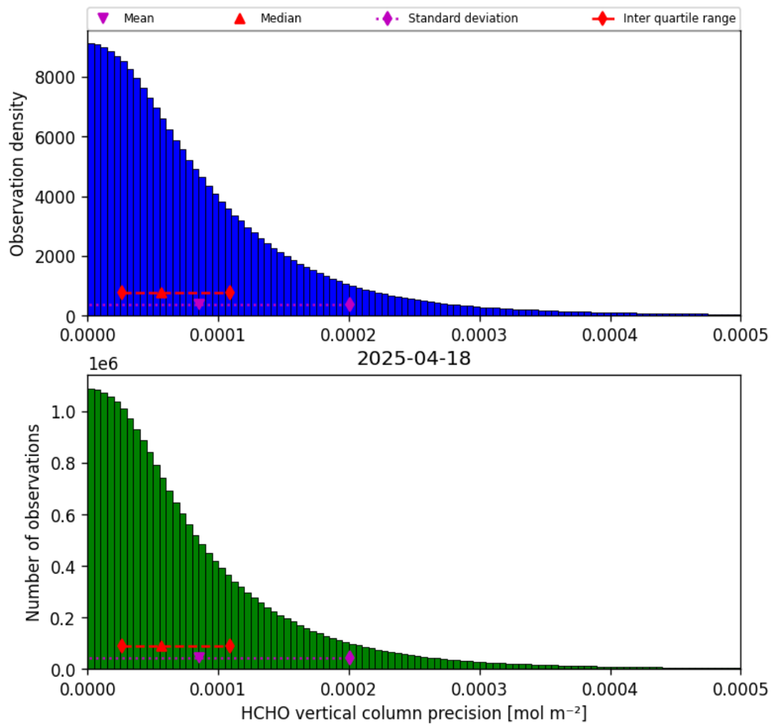
Figure 34: Histogram of “HCHO vertical column precision” for 2025-04-18 to 2025-04-19
