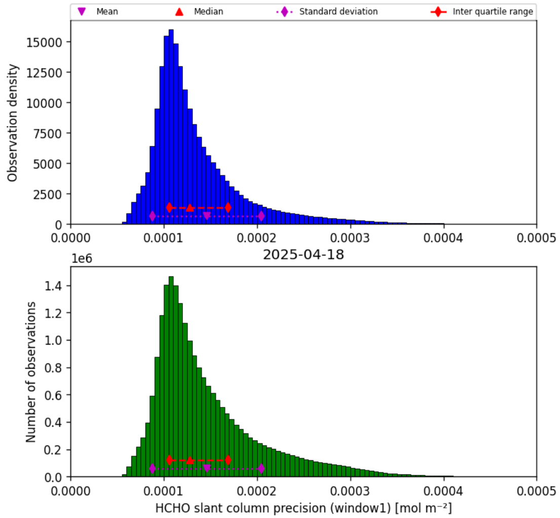
Figure 37: Histogram of “HCHO slant column precision (window1)” for 2025-04-18 to 2025-04-19
