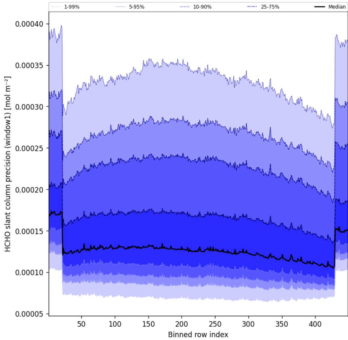
Figure 51: Along track statistics of “HCHO slant column precision (window1)” for 2025-04-18 to 2025-04-19
