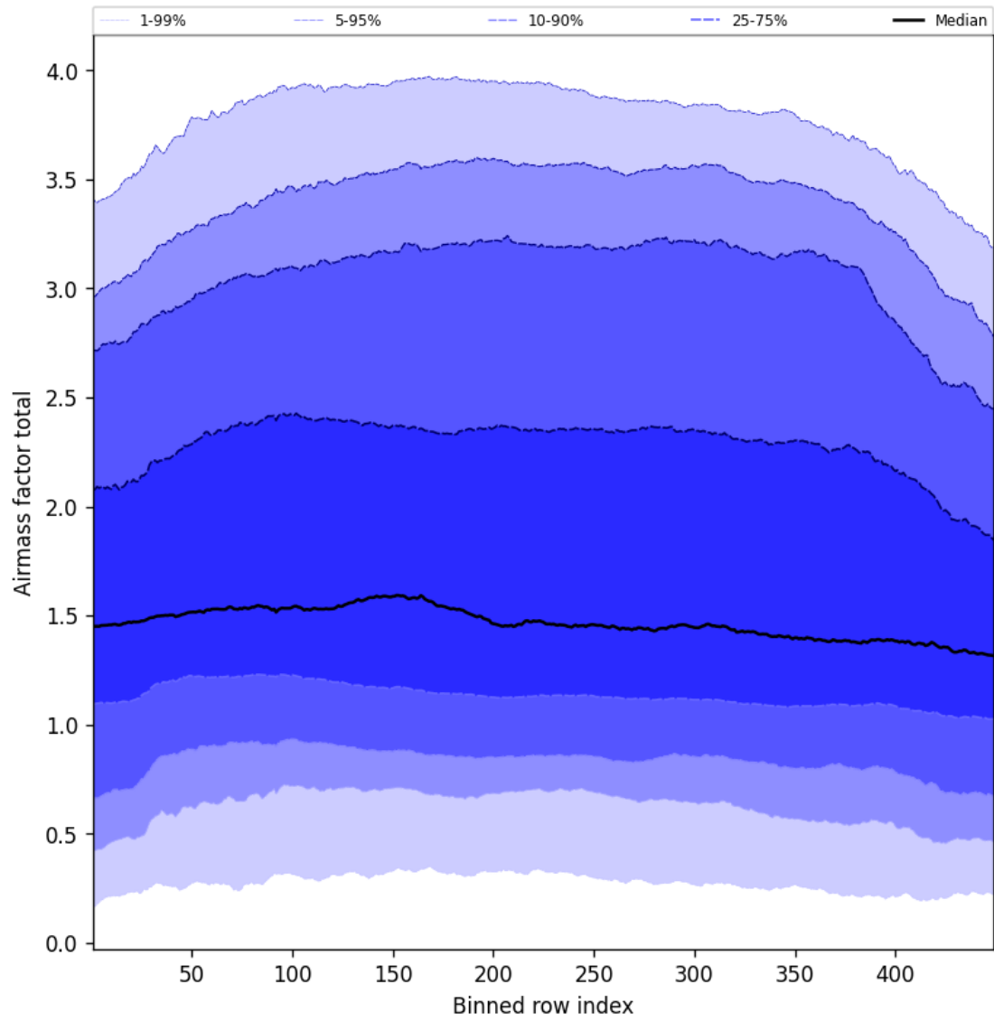
Figure 52: Along track statistics of “Airmass factor total” for 2025-04-18 to 2025-04-19
