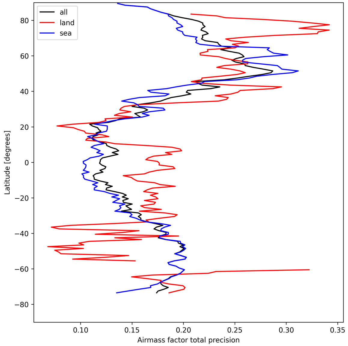
Figure 25: Zonal average of “Airmass factor total precision” for 2025-04-18 to 2025-04-19.
