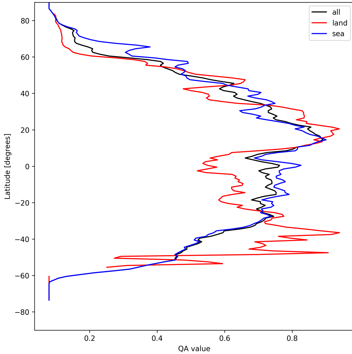
Figure 18: Zonal average of “QA value” for 2025-04-18 to 2025-04-19.
