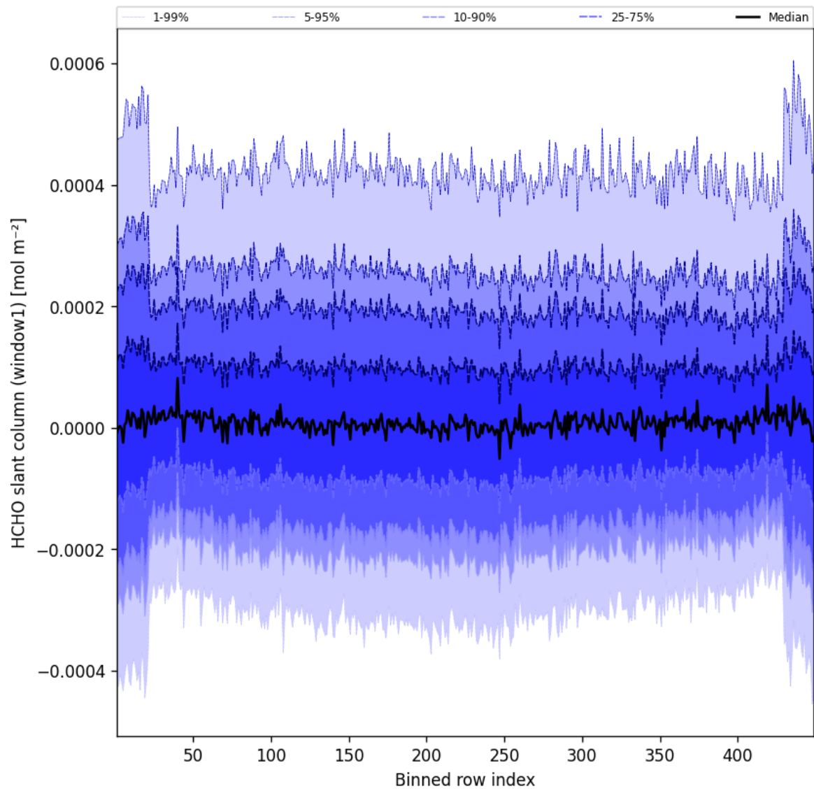
Figure 50: Along track statistics of “HCHO slant column (window1)” for 2025-04-18 to 2025-04-19
