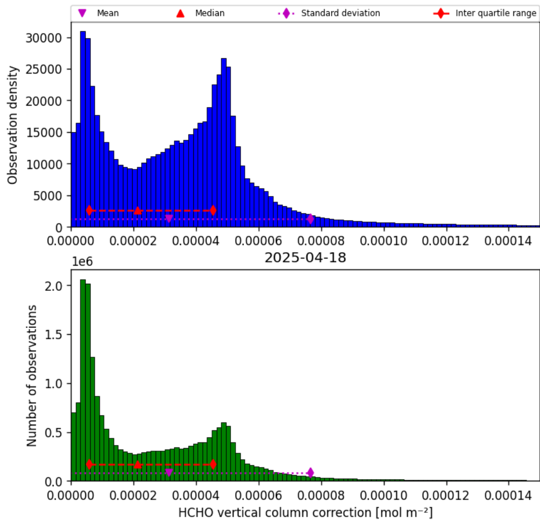
Figure 35: Histogram of “HCHO vertical column correction” for 2025-04-18 to 2025-04-19
