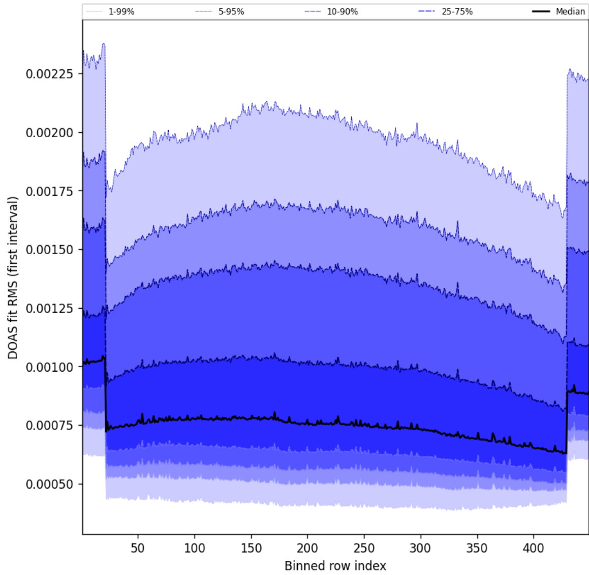
Figure 58: Along track statistics of “DOAS fit RMS (first interval)” for 2025-04-18 to 2025-04-19
