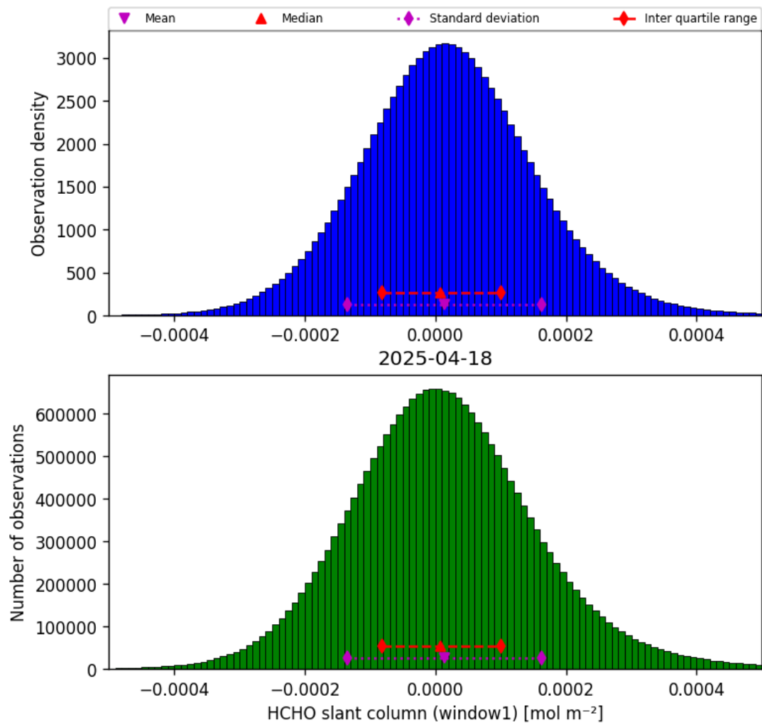
Figure 36: Histogram of “HCHO slant column (window1)” for 2025-04-18 to 2025-04-19
