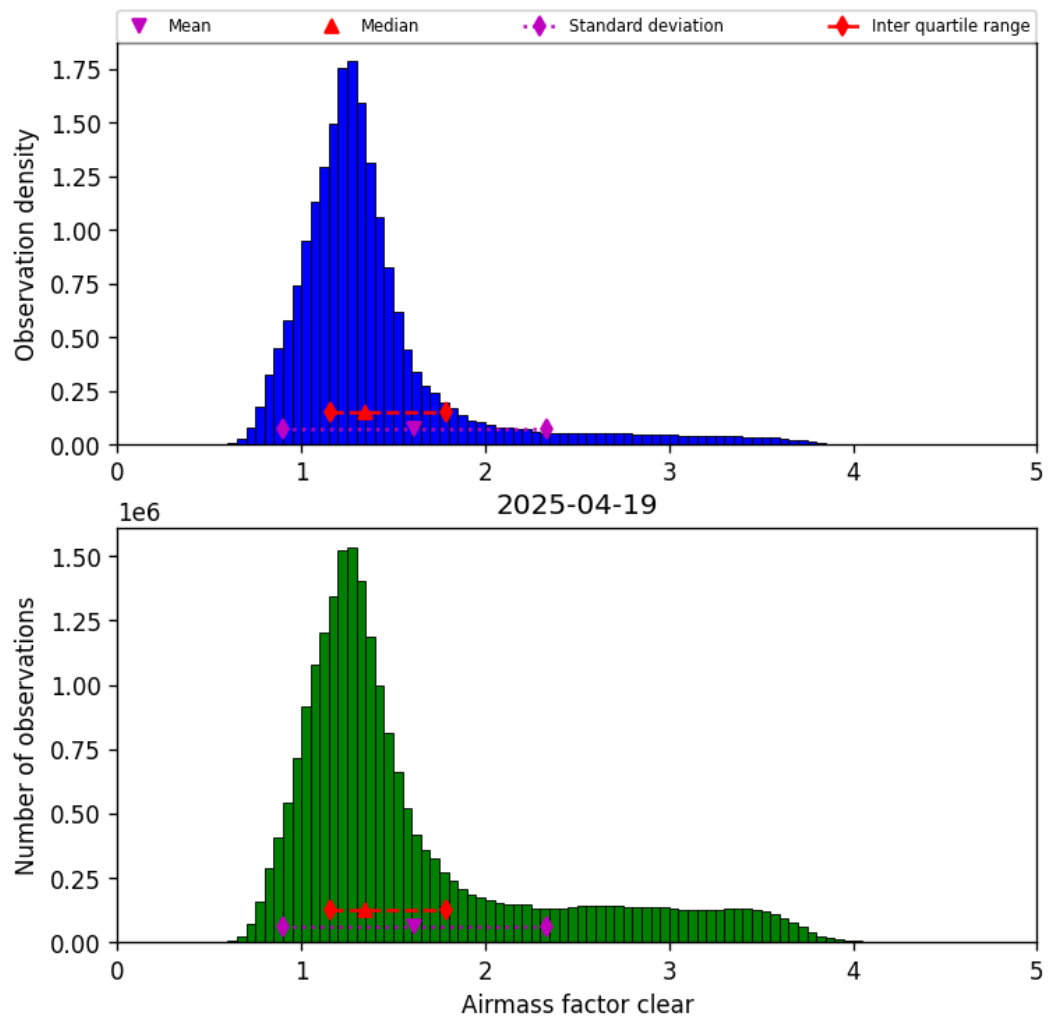
Figure 40: Histogram of “Airmass factor clear” for 2025-04-19 to 2025-04-20
