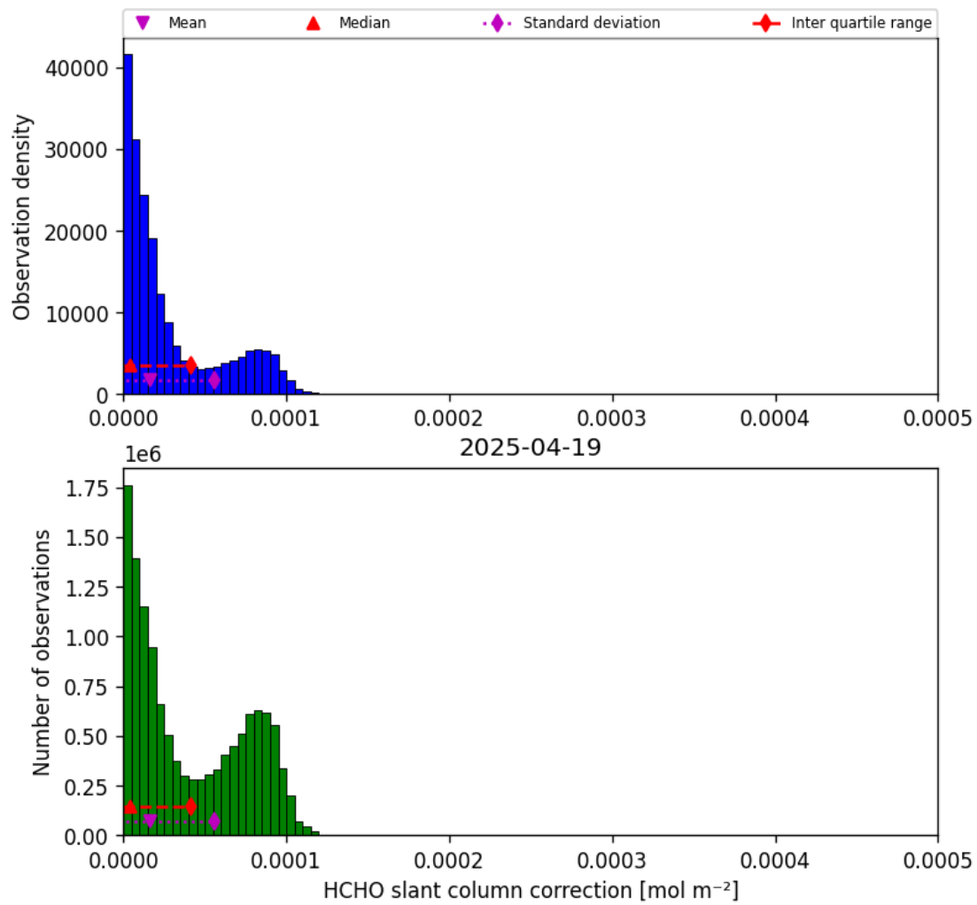
Figure 45: Histogram of “HCHO slant column correction” for 2025-04-19 to 2025-04-20
