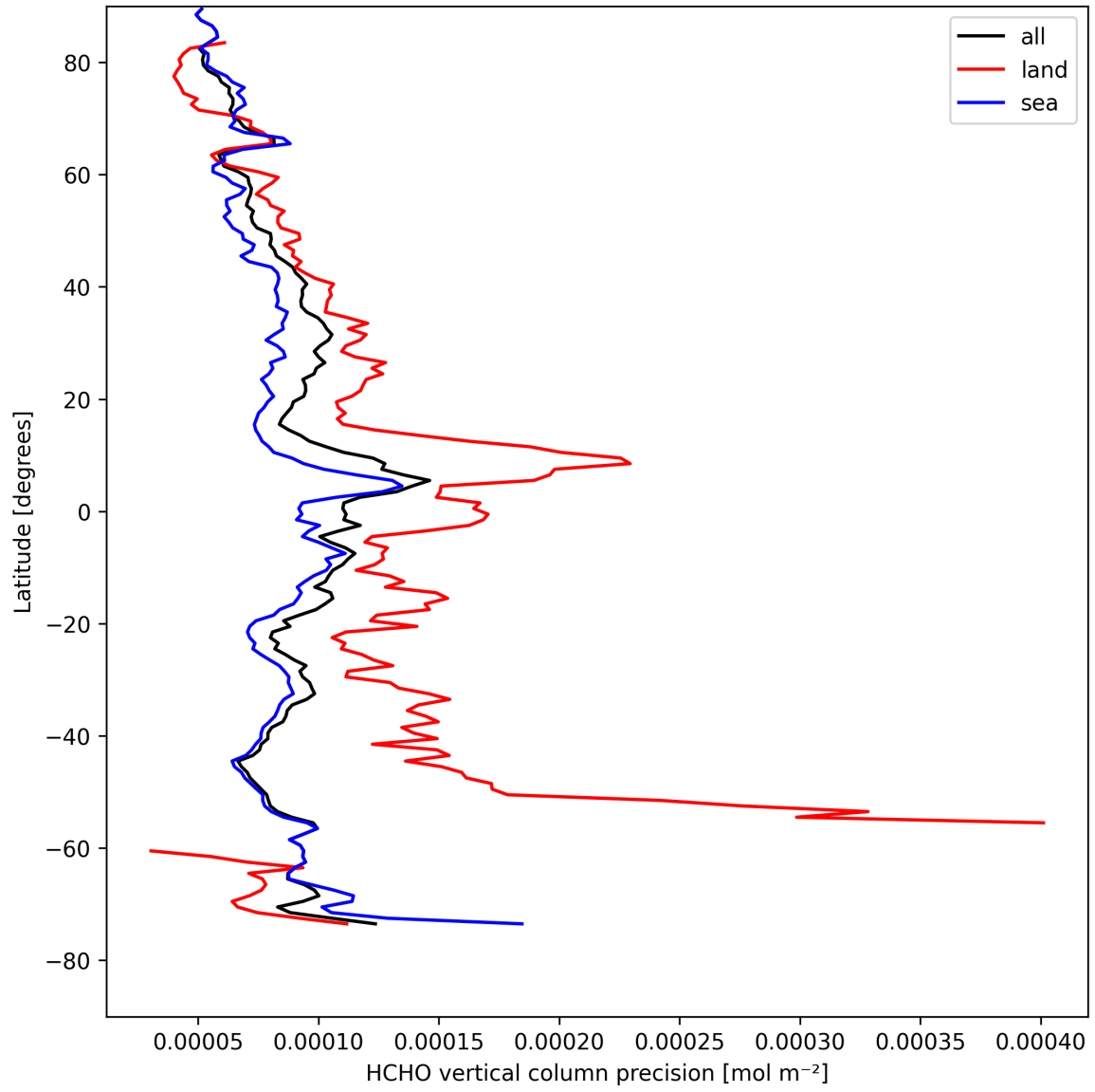
Figure 20: Zonal average of “HCHO vertical column precision” for 2025-04-19 to 2025-04-20.
