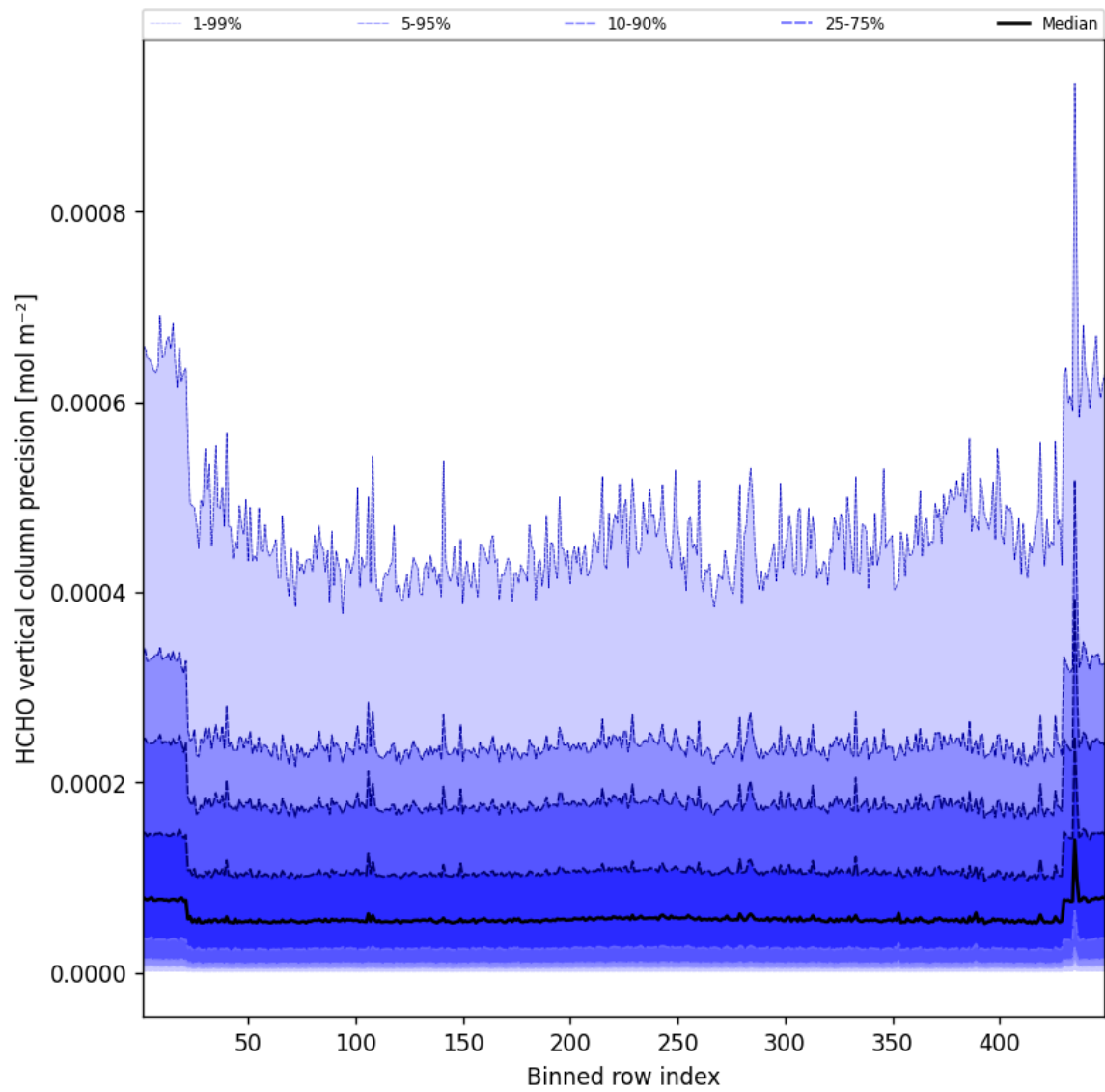
Figure 48: Along track statistics of “HCHO vertical column precision” for 2025-04-19 to 2025-04-20
