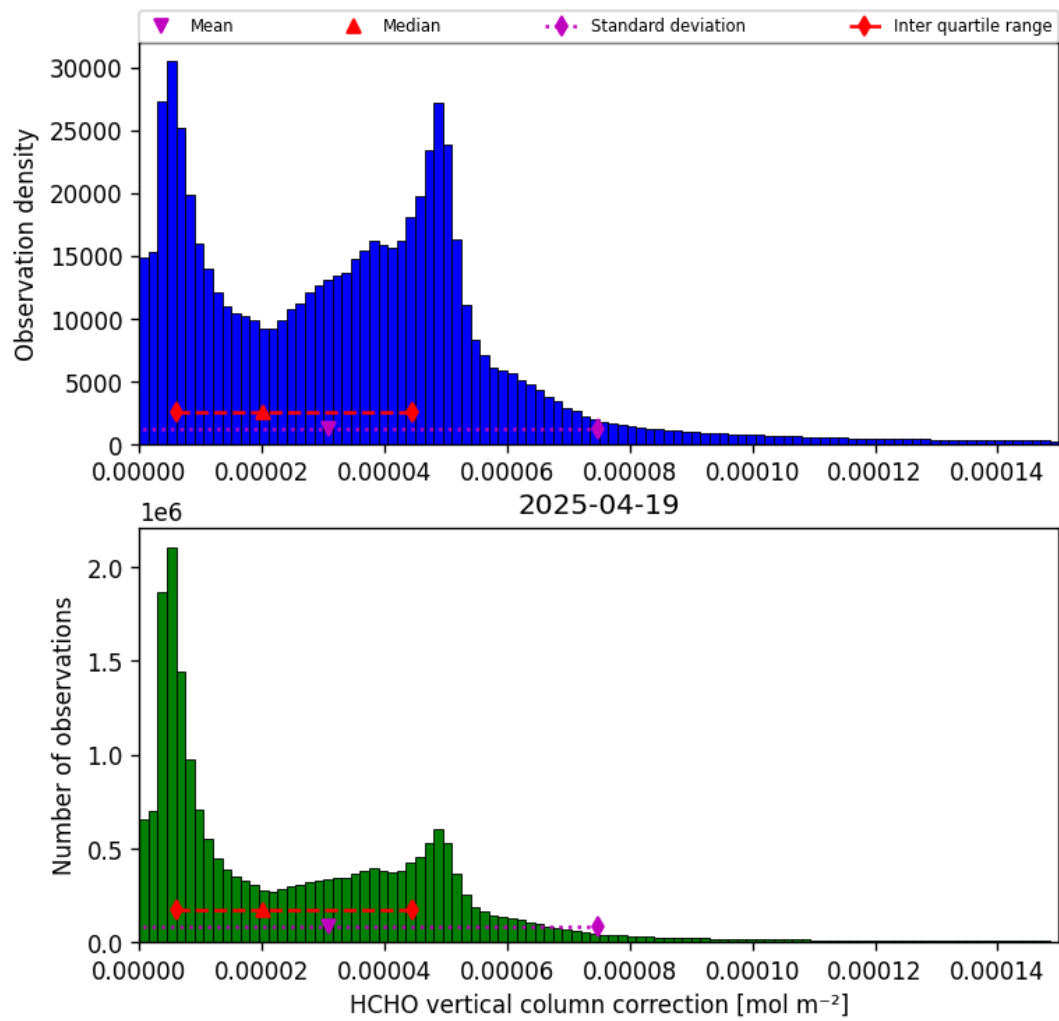
Figure 35: Histogram of “HCHO vertical column correction” for 2025-04-19 to 2025-04-20
