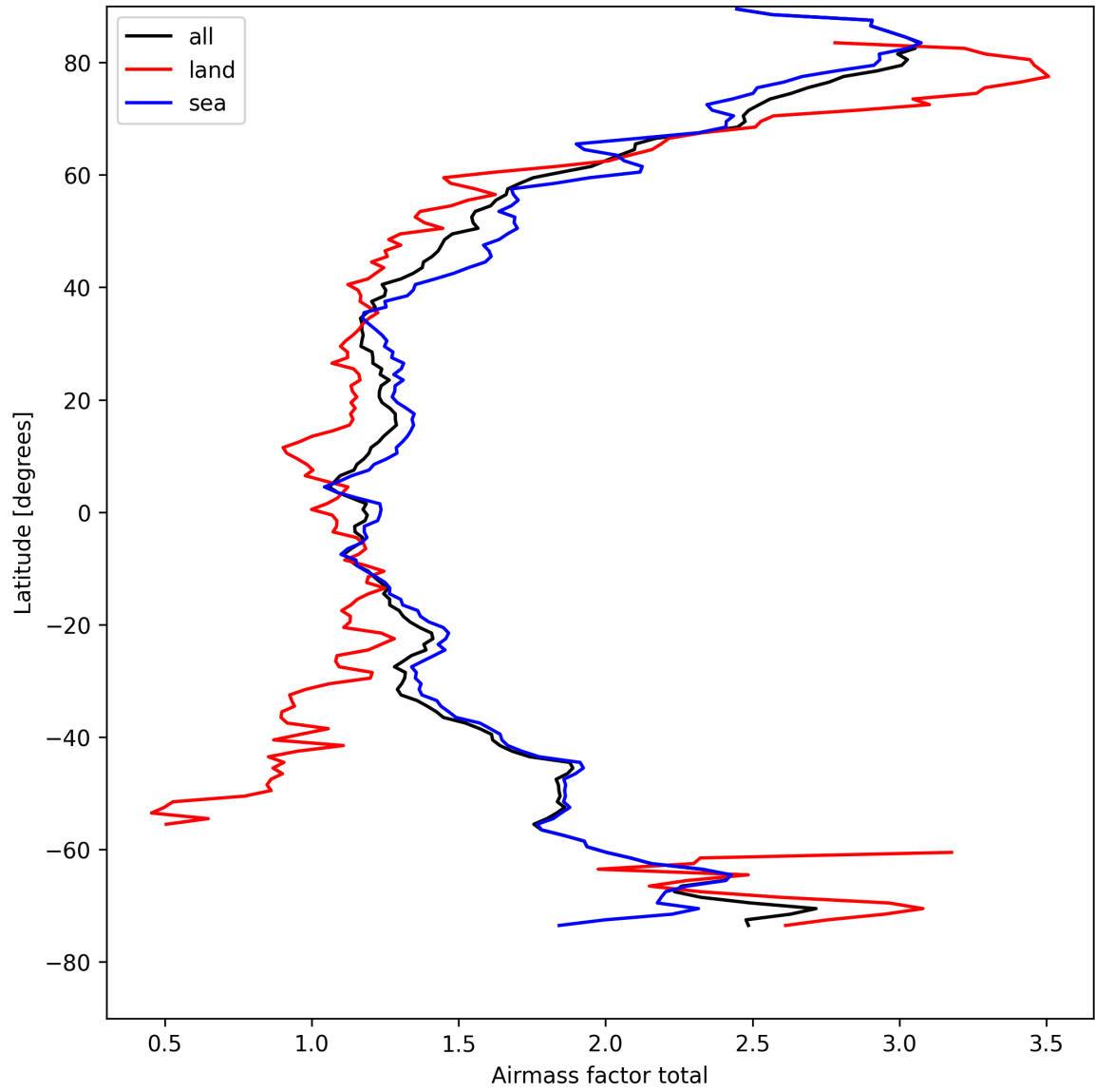
Figure 24: Zonal average of “Airmass factor total” for 2025-04-19 to 2025-04-20.
