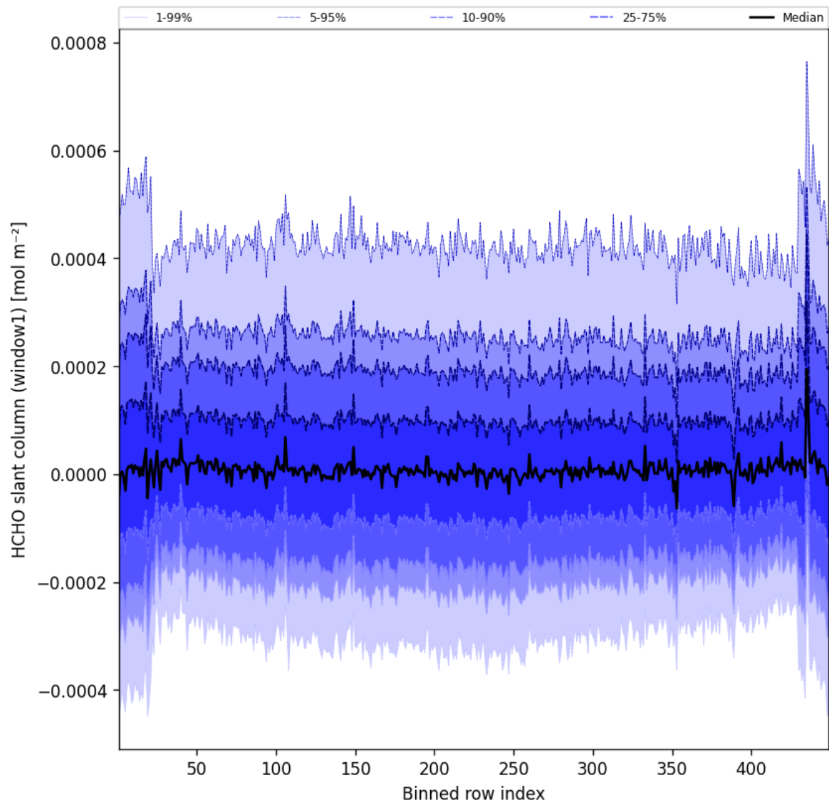
Figure 50: Along track statistics of “HCHO slant column (window1)” for 2025-04-19 to 2025-04-20
