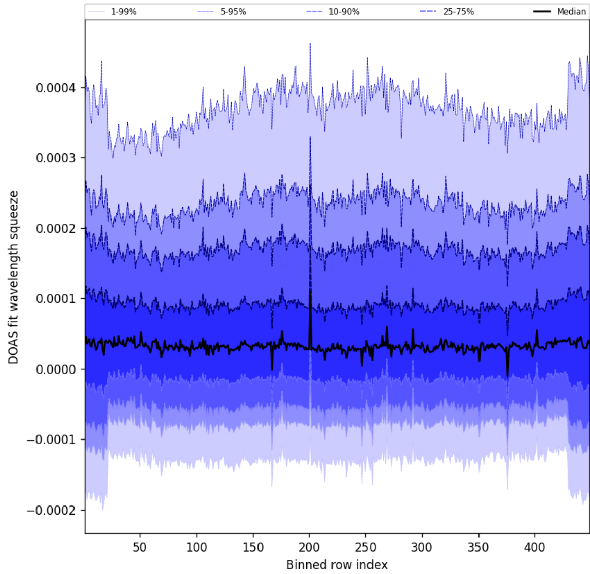
Figure 57: Along track statistics of “DOAS fit wavelength squeeze” for 2025-04-19 to 2025-04-20
