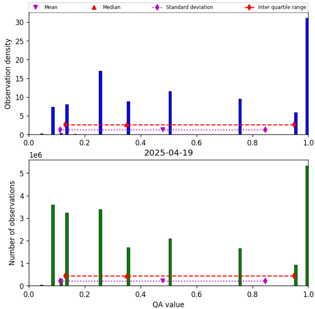
Figure 32: Histogram of “QA value” for 2025-04-19 to 2025-04-20
