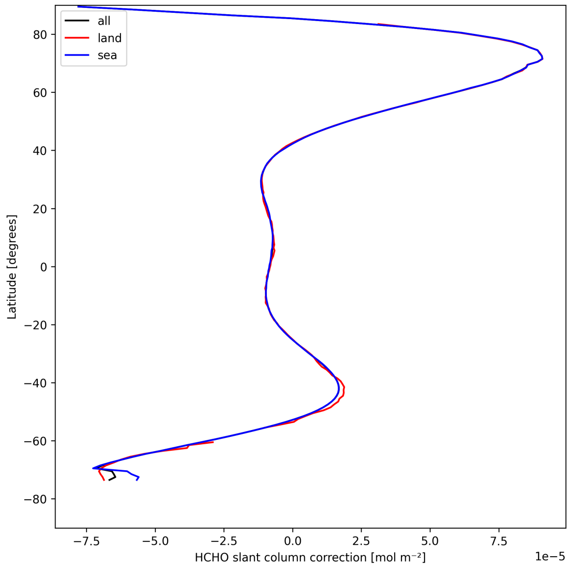
Figure 31: Zonal average of “HCHO slant column correction” for 2025-04-19 to 2025-04-20.
