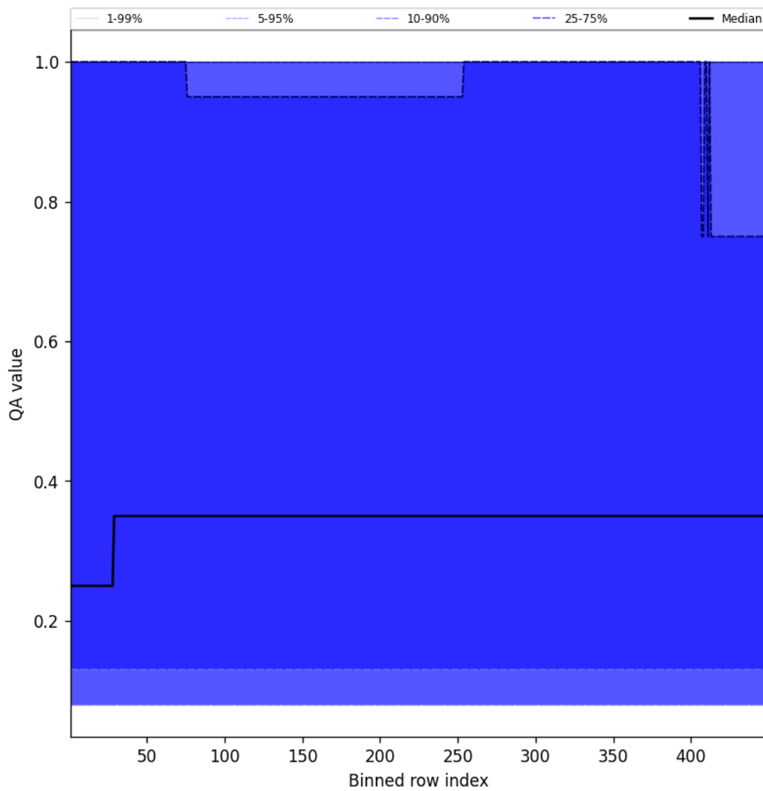
Figure 46: Along track statistics of “QA value” for 2025-04-19 to 2025-04-20
