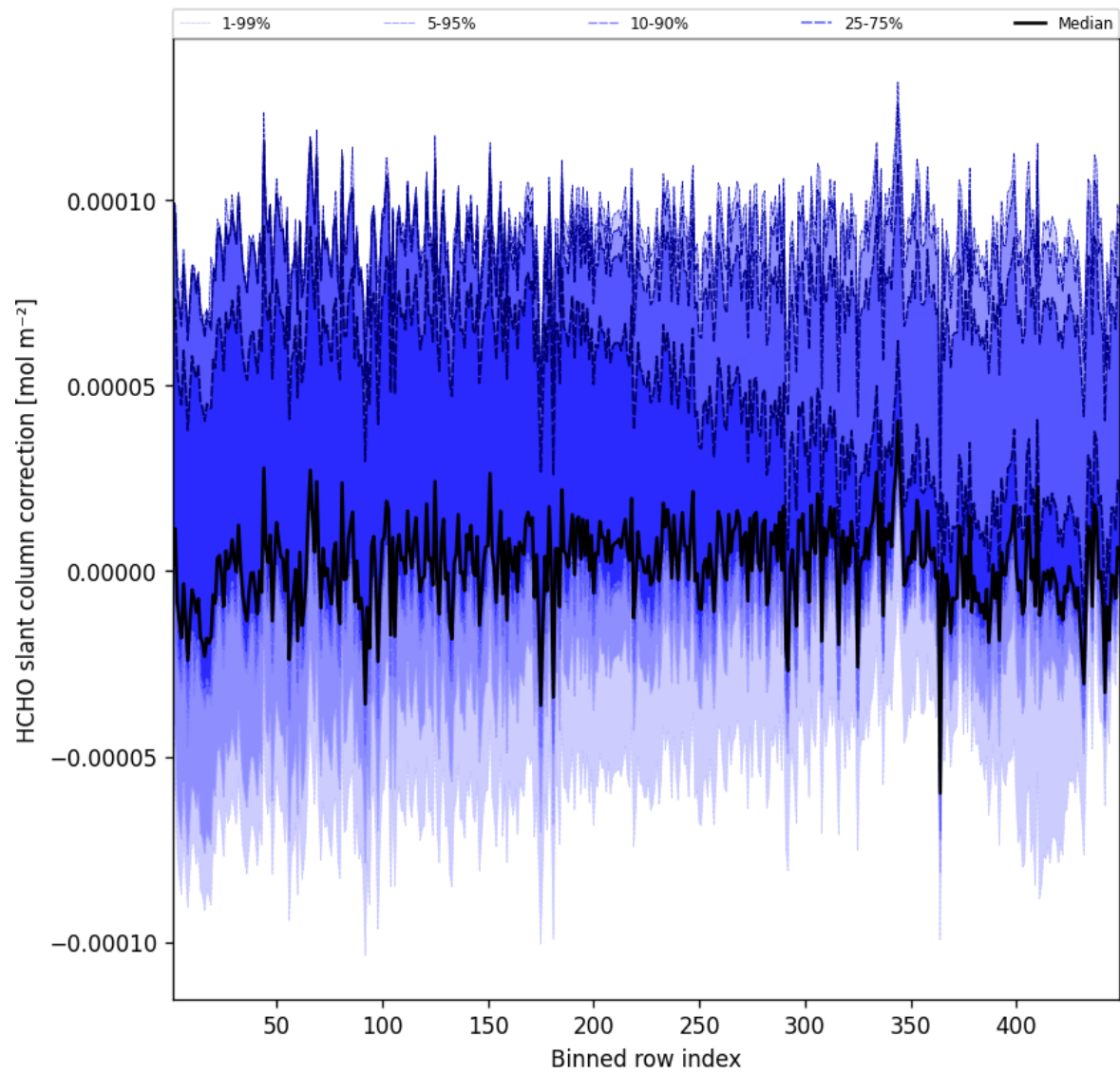
Figure 59: Along track statistics of “HCHO slant column correction” for 2025-04-19 to 2025-04-20
