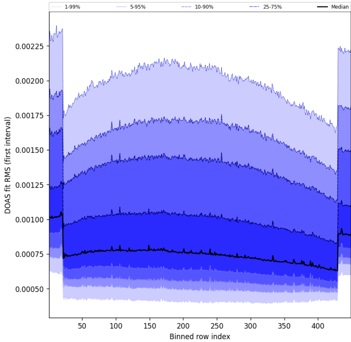
Figure 58: Along track statistics of “DOAS fit RMS (first interval)” for 2025-04-19 to 2025-04-20
