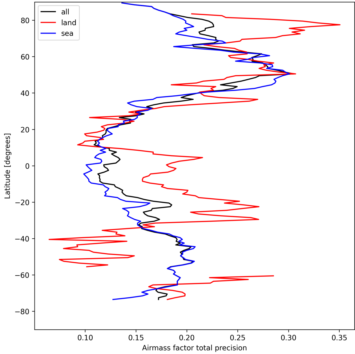
Figure 25: Zonal average of “Airmass factor total precision” for 2025-04-19 to 2025-04-20.
