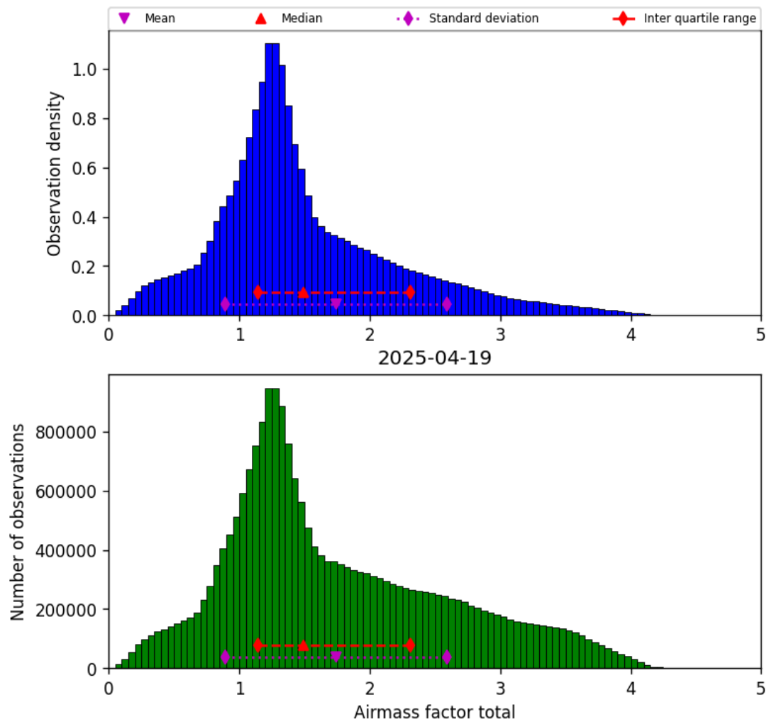
Figure 38: Histogram of “Airmass factor total” for 2025-04-19 to 2025-04-20
