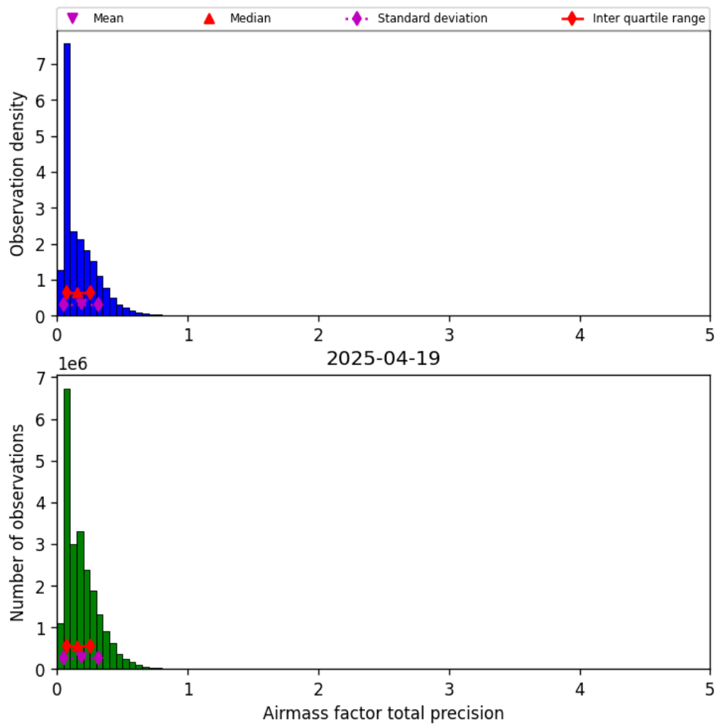
Figure 39: Histogram of “Airmass factor total precision” for 2025-04-19 to 2025-04-20
