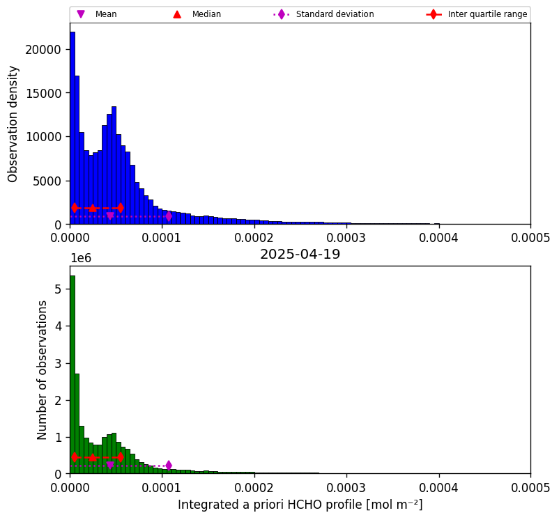
Figure 41: Histogram of “Integrated a priori HCHO profile” for 2025-04-19 to 2025-04-20
