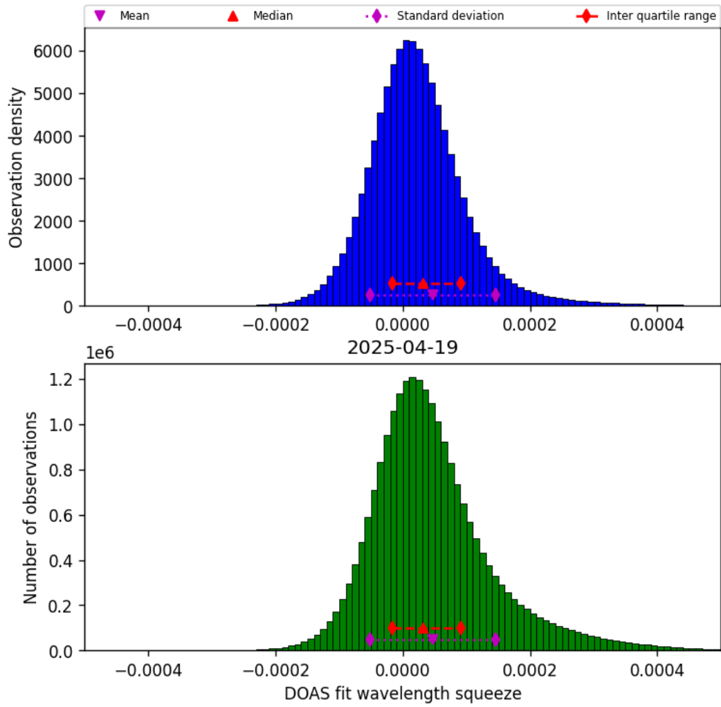
Figure 43: Histogram of “DOAS fit wavelength squeeze” for 2025-04-19 to 2025-04-20
