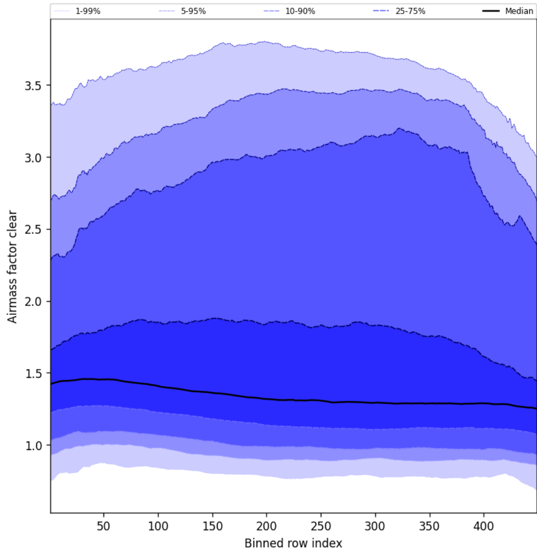
Figure 54: Along track statistics of “Airmass factor clear” for 2025-04-19 to 2025-04-20
