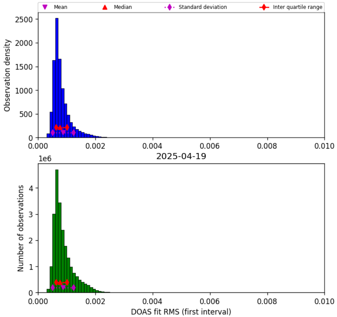
Figure 44: Histogram of “DOAS fit RMS (first interval)” for 2025-04-19 to 2025-04-20
