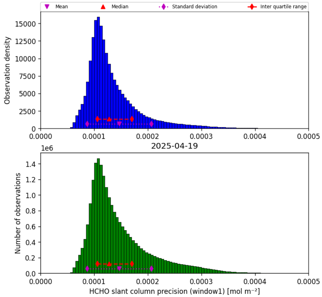
Figure 37: Histogram of “HCHO slant column precision (window1)” for 2025-04-19 to 2025-04-20
