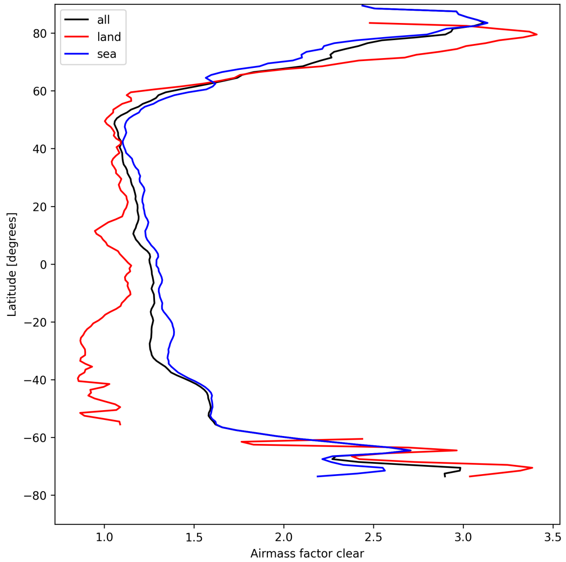
Figure 26: Zonal average of “Airmass factor clear” for 2025-04-19 to 2025-04-20.
