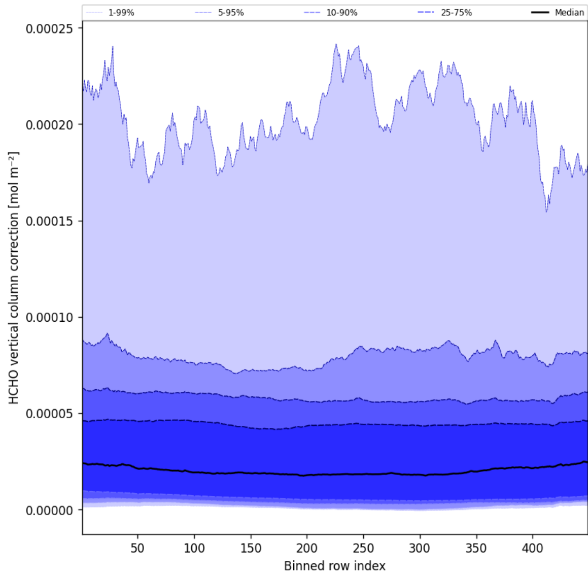
Figure 49: Along track statistics of “HCHO vertical column correction” for 2025-04-19 to 2025-04-20
