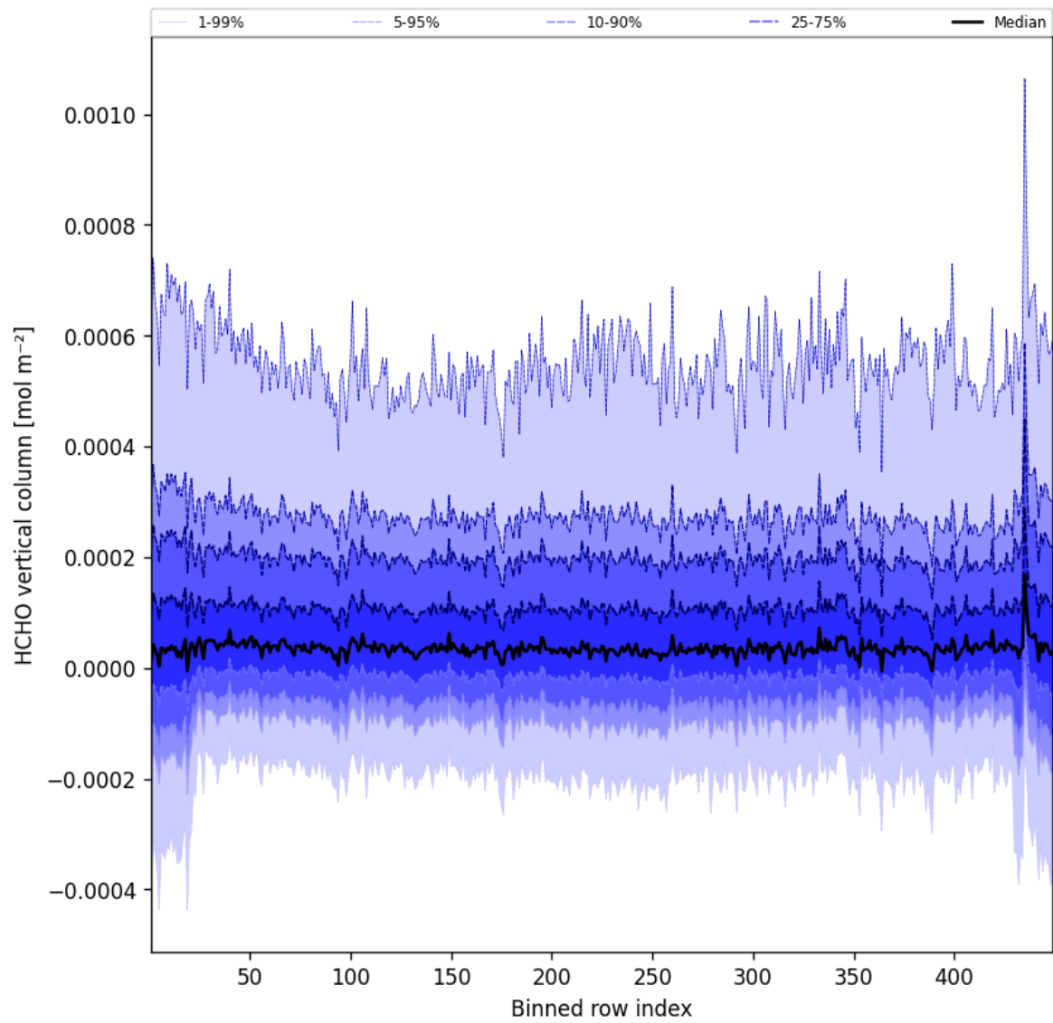
Figure 47: Along track statistics of “HCHO vertical column” for 2025-04-19 to 2025-04-20
