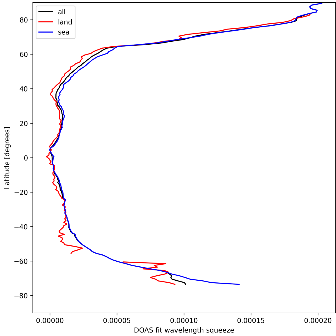
Figure 29: Zonal average of “DOAS fit wavelength squeeze” for 2025-04-19 to 2025-04-20.
