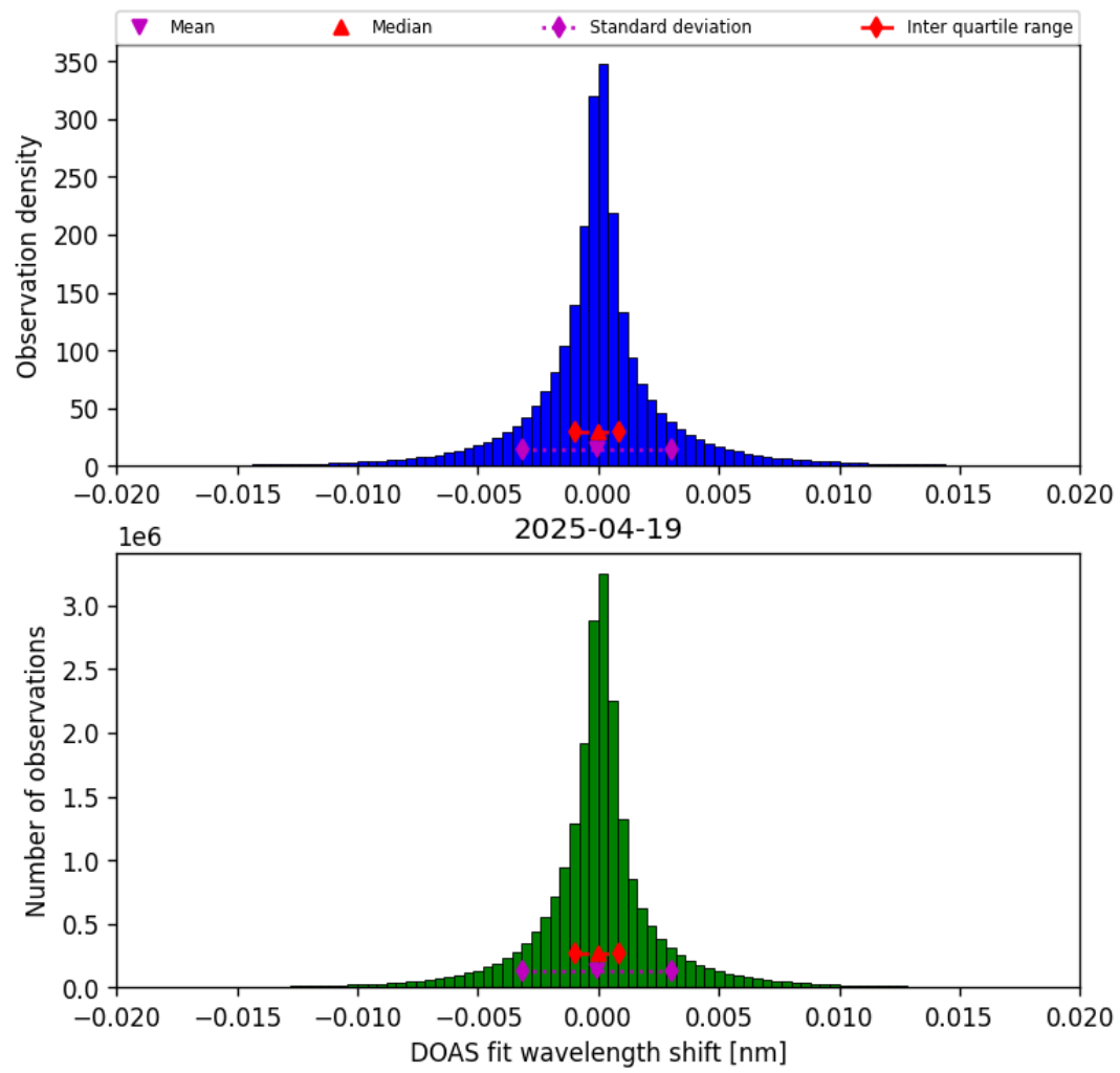
Figure 42: Histogram of “DOAS fit wavelength shift” for 2025-04-19 to 2025-04-20
