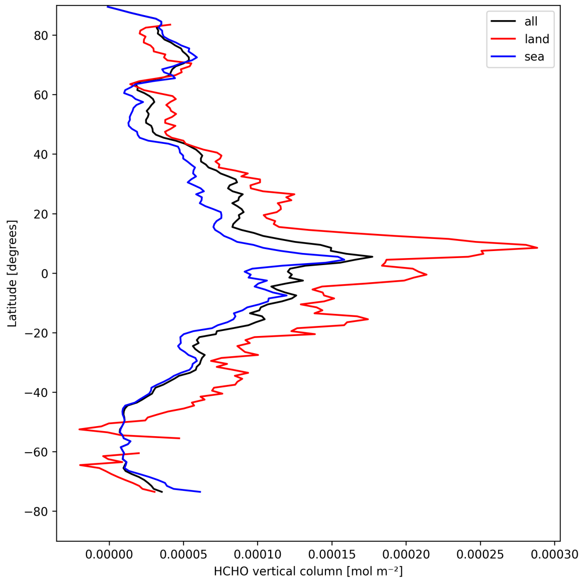
Figure 19: Zonal average of “HCHO vertical column” for 2025-04-19 to 2025-04-20.
