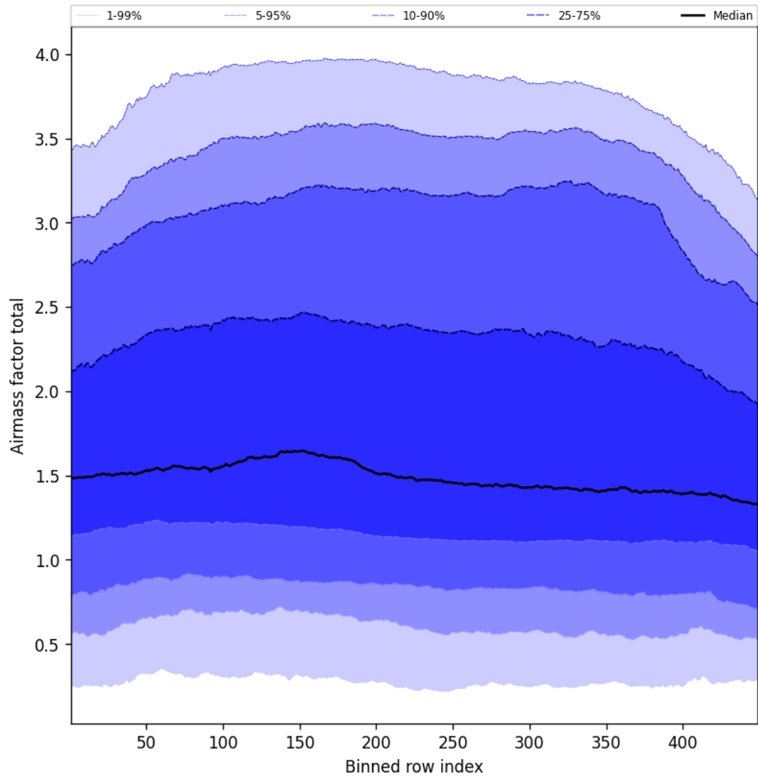
Figure 52: Along track statistics of “Airmass factor total” for 2025-04-19 to 2025-04-20
