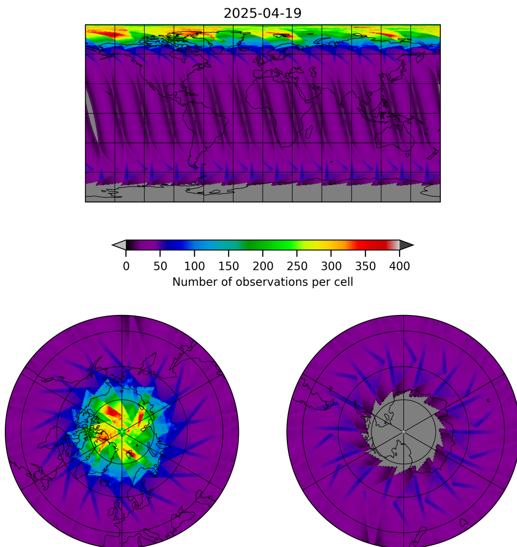
Figure 17: Map of the number of observations for 2025-04-19 to 2025-04-20
