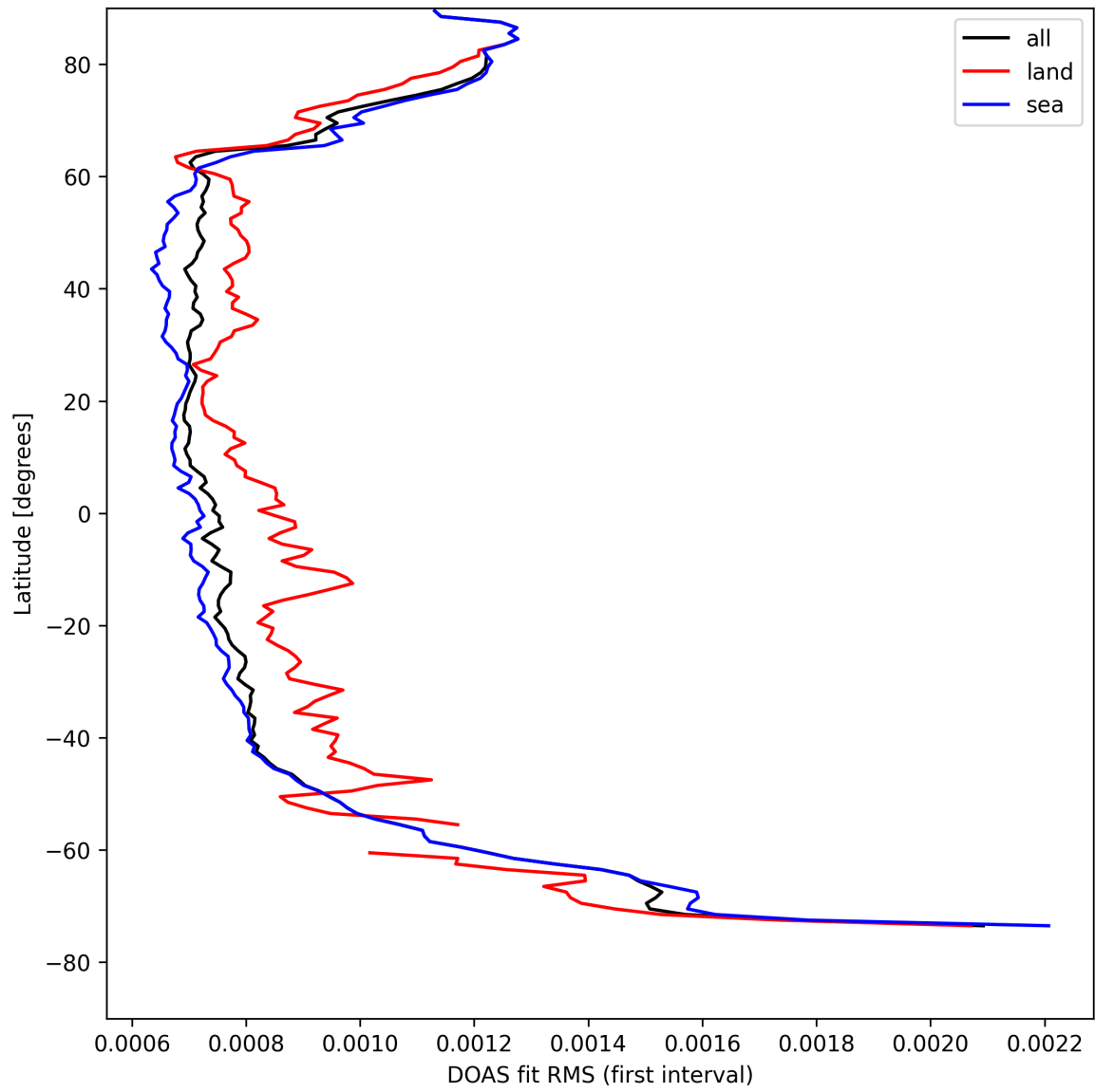
Figure 30: Zonal average of "DOAS fit RMS (first interval)" for 2025-04-19 to 2025-04-20.
