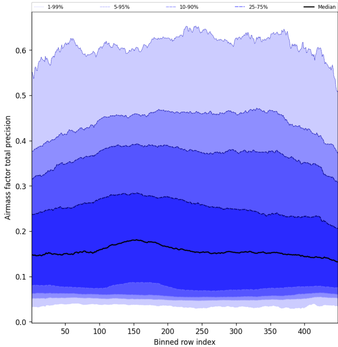
Figure 53: Along track statistics of “Airmass factor total precision” for 2025-04-19 to 2025-04-20
