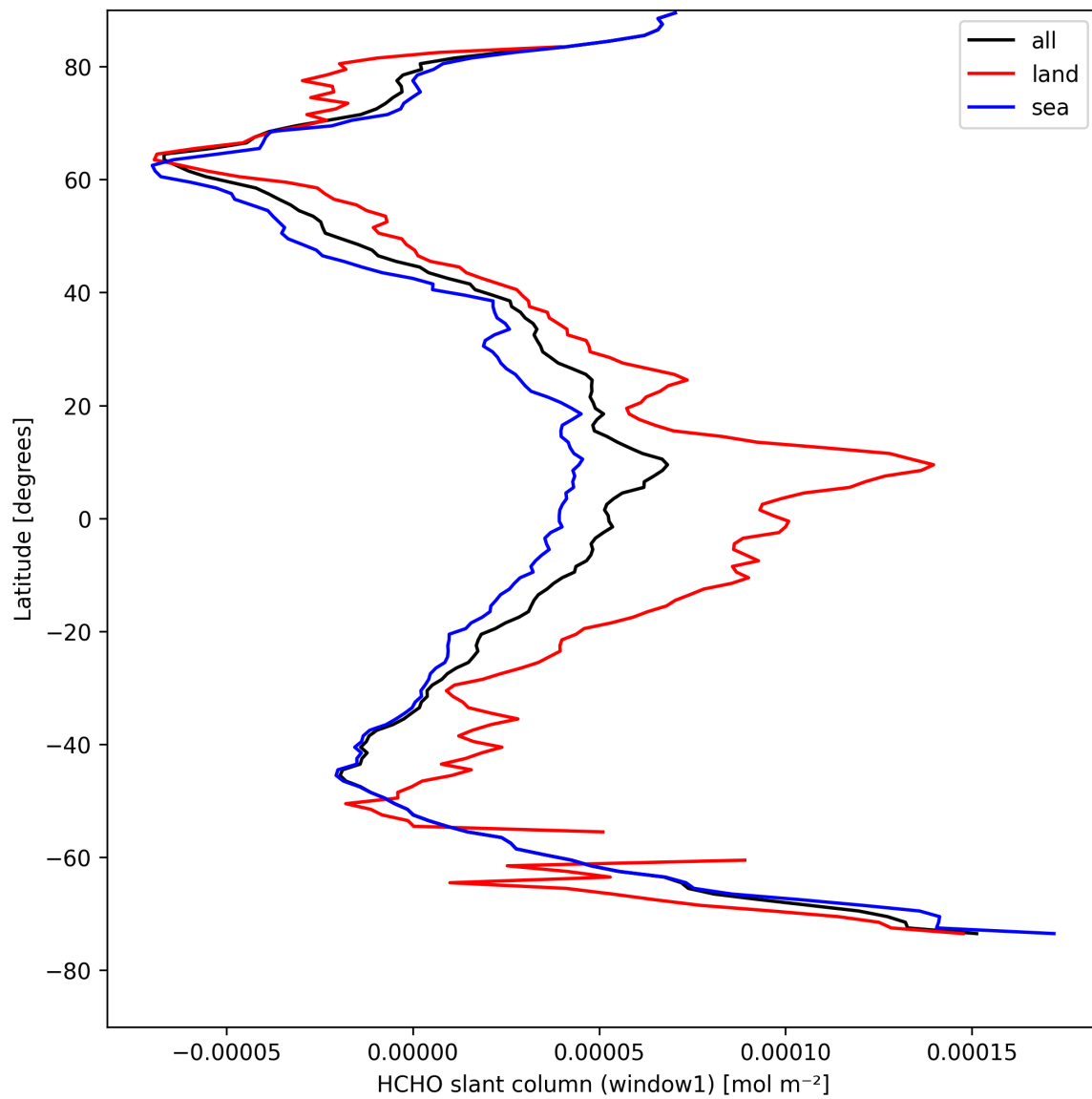
Figure 22: Zonal average of “HCHO slant column (window1)” for 2025-04-19 to 2025-04-20.
