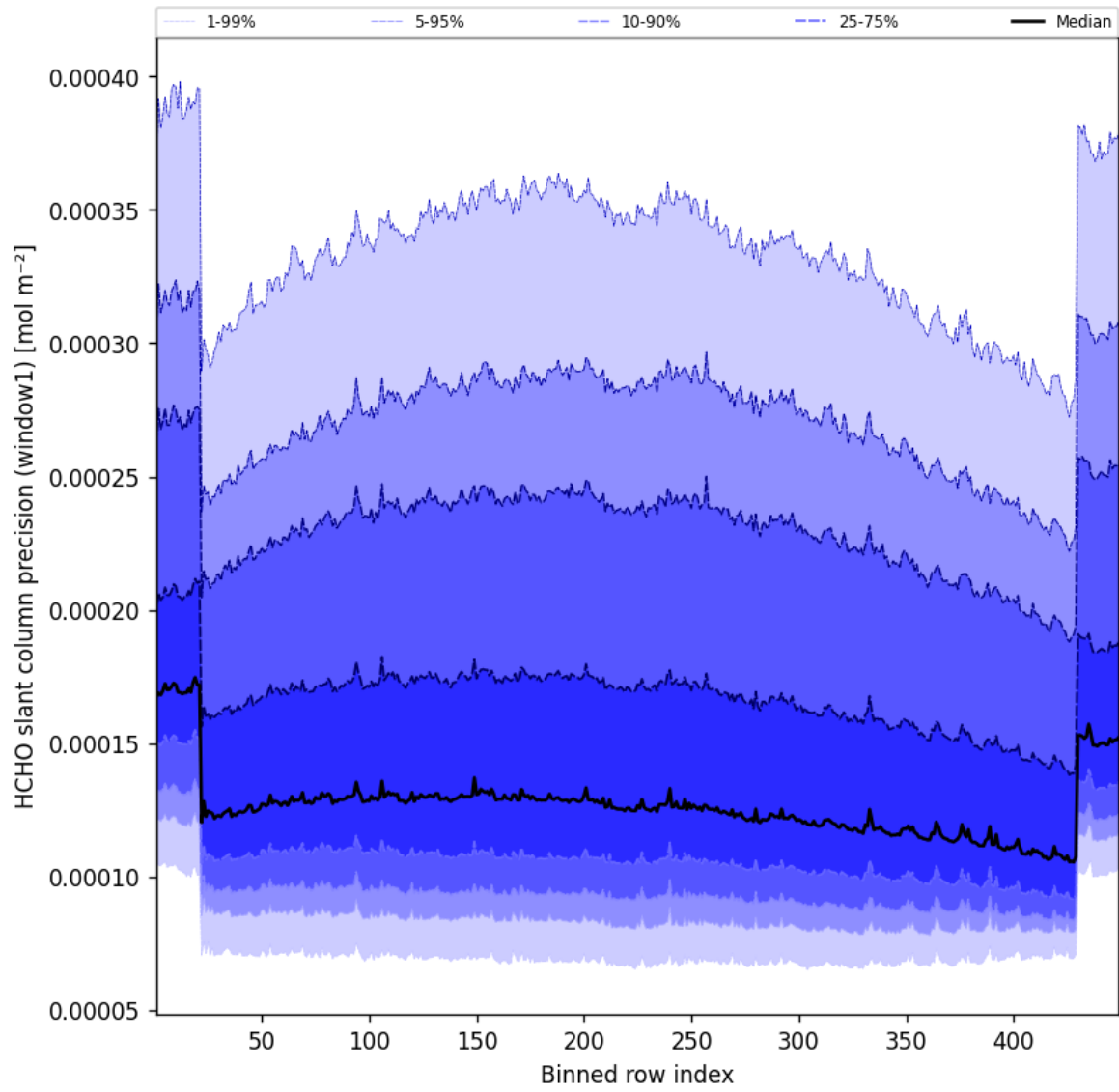
Figure 51: Along track statistics of “HCHO slant column precision (window1)” for 2025-04-19 to 2025-04-20
