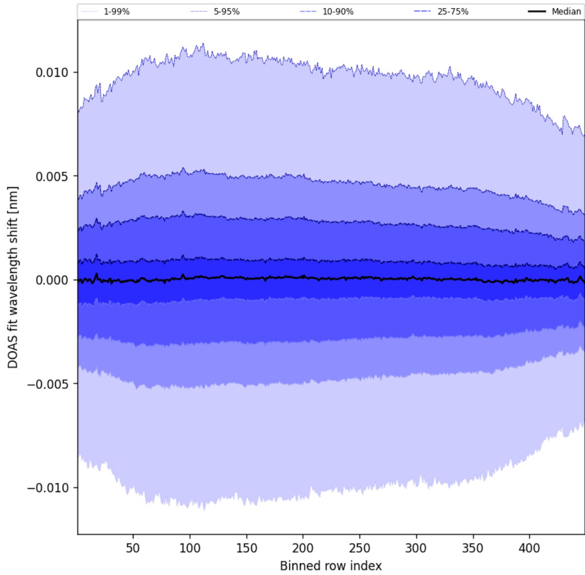
Figure 56: Along track statistics of “DOAS fit wavelength shift” for 2025-04-19 to 2025-04-20
