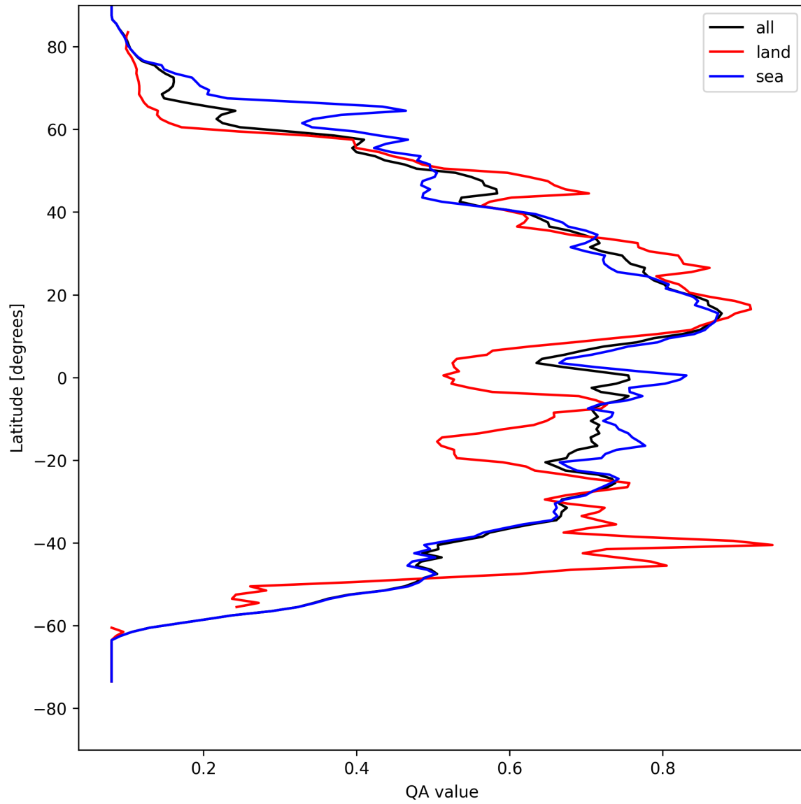
Figure 18: Zonal average of “QA value” for 2025-04-19 to 2025-04-20.
