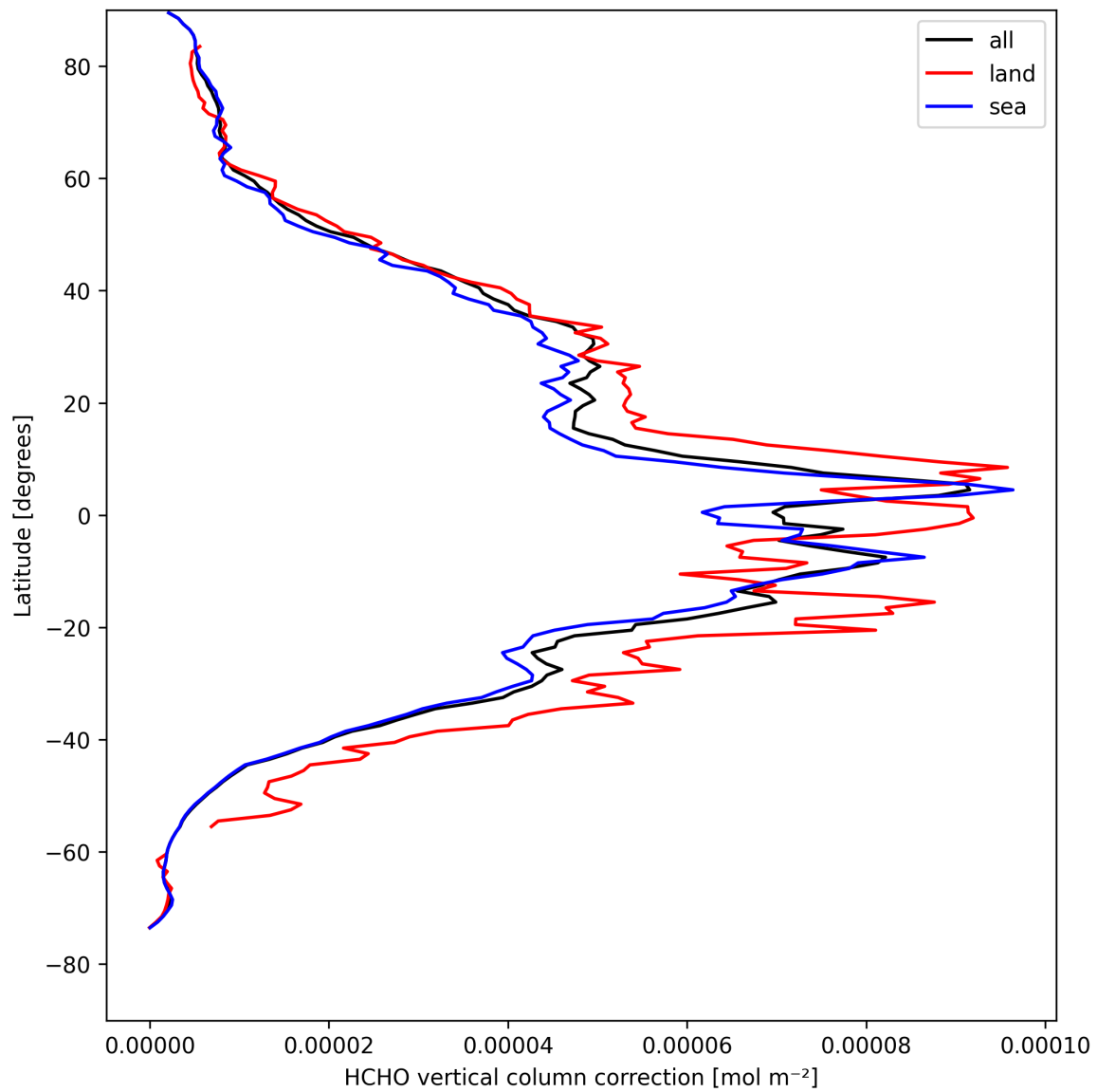
Figure 21: Zonal average of “HCHO vertical column correction” for 2025-04-19 to 2025-04-20.
