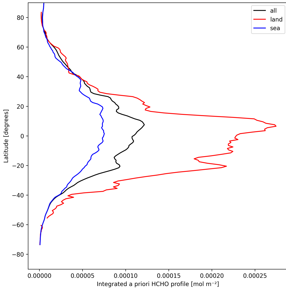
Figure 27: Zonal average of “Integrated a priori HCHO profile” for 2025-04-19 to 2025-04-20.
