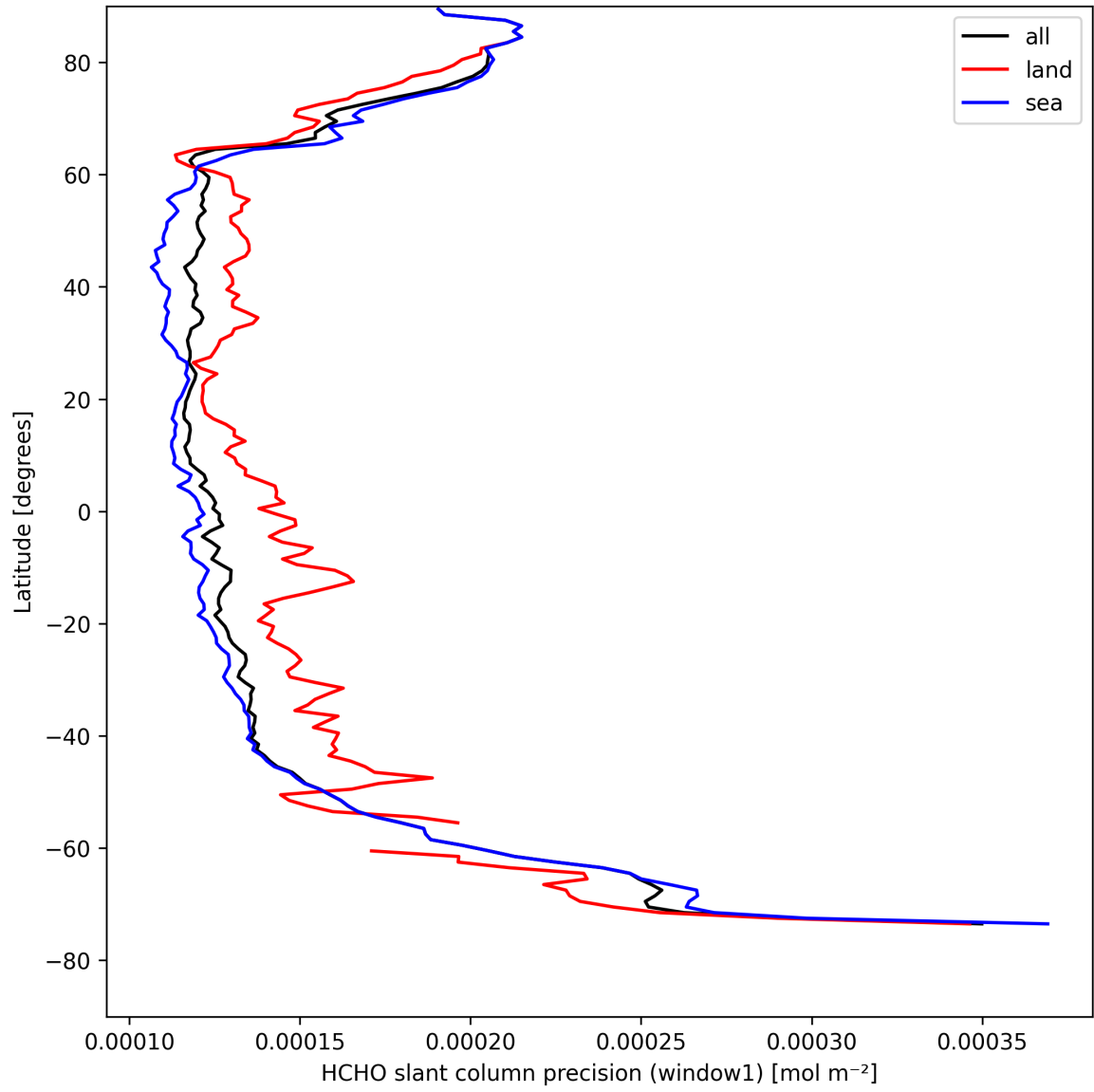
Figure 23: Zonal average of “HCHO slant column precision (window1)” for 2025-04-19 to 2025-04-20.
