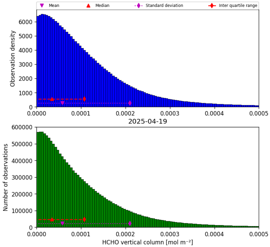
Figure 33: Histogram of “HCHO vertical column” for 2025-04-19 to 2025-04-20
