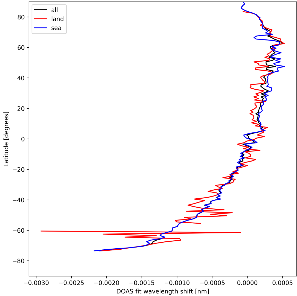
Figure 28: Zonal average of “DOAS fit wavelength shift” for 2025-04-19 to 2025-04-20.
