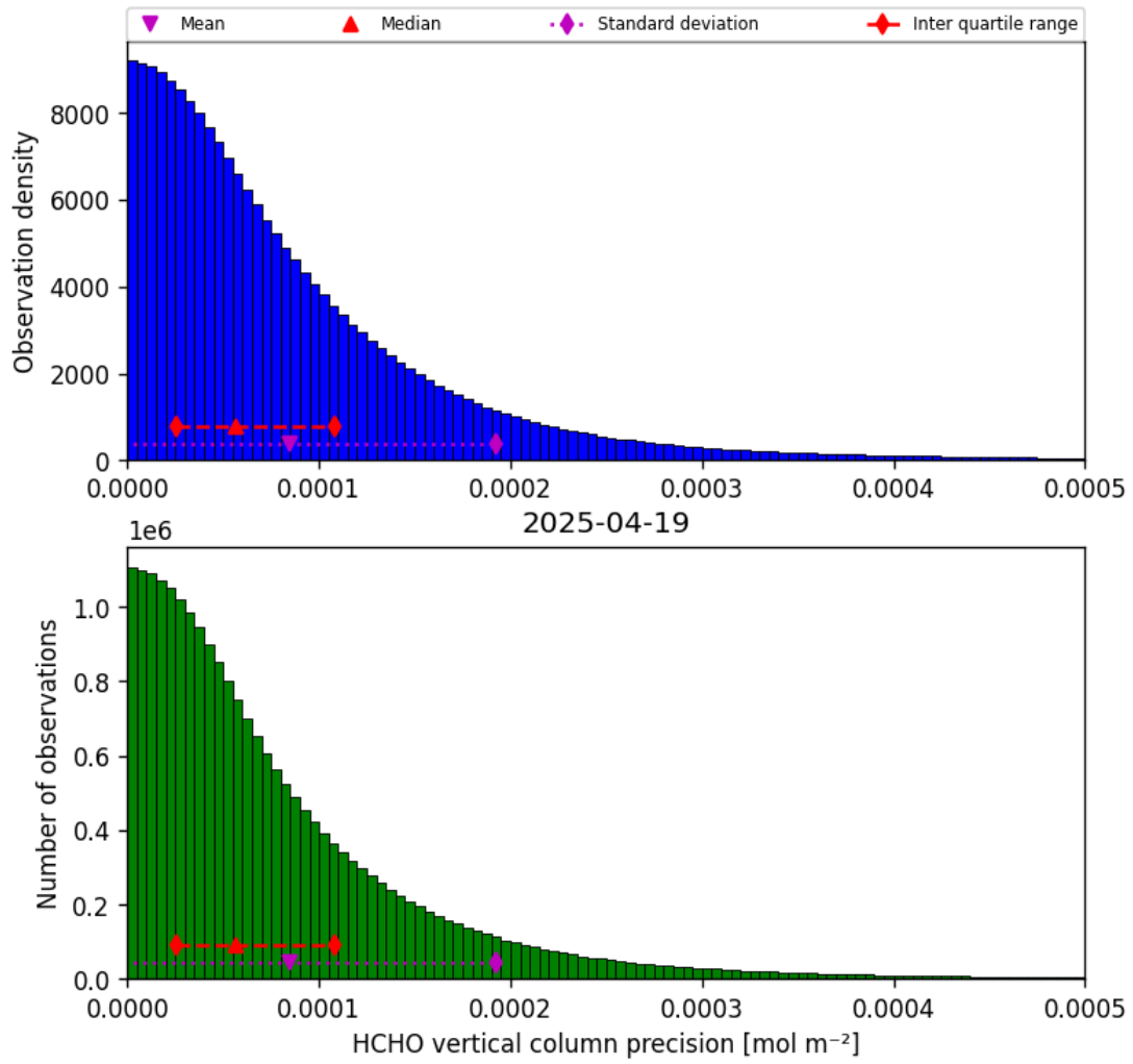
Figure 34: Histogram of “HCHO vertical column precision” for 2025-04-19 to 2025-04-20
