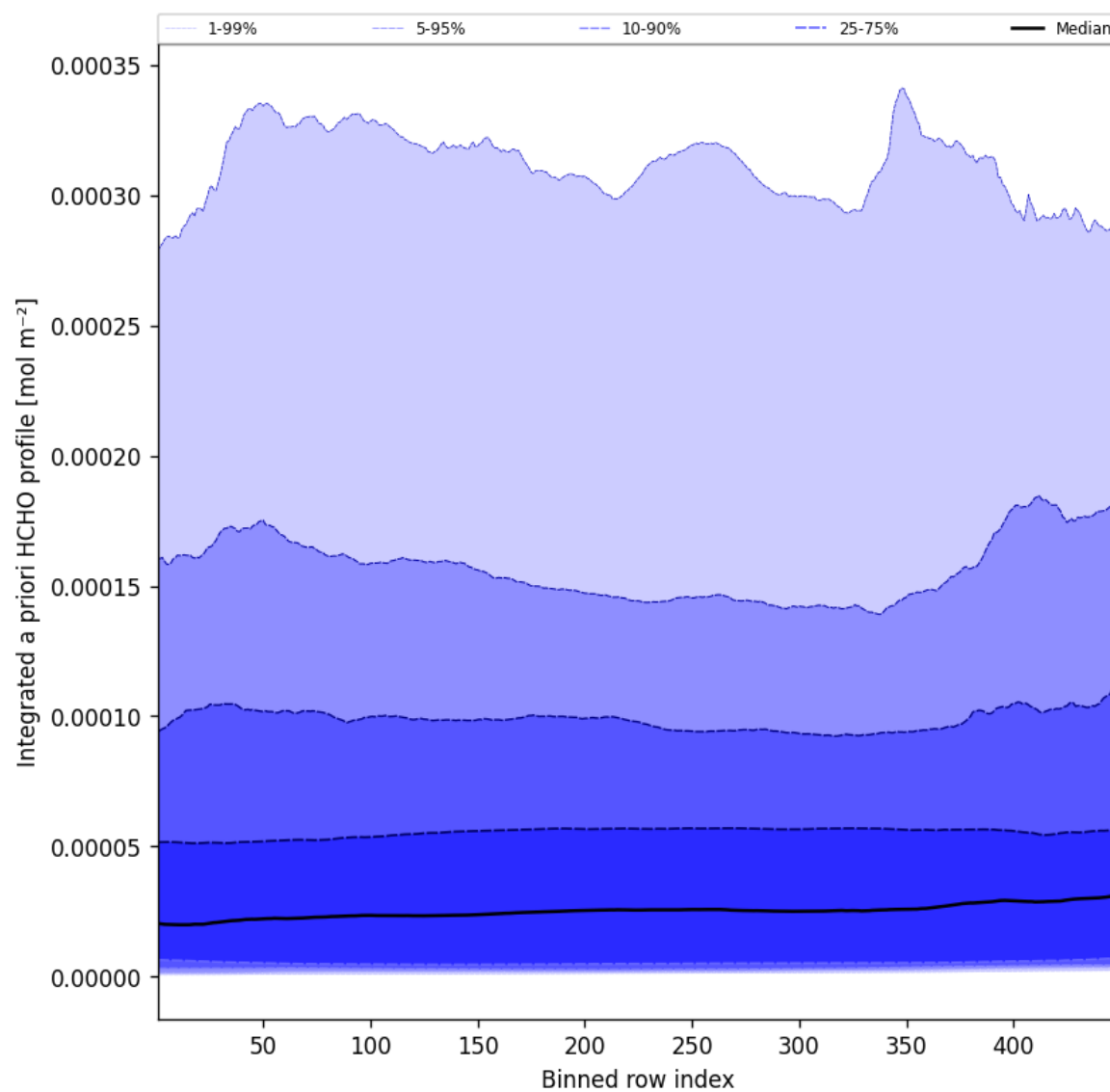
Figure 55: Along track statistics of "Integrated a priori HCHO profile" for 2025-04-19 to 2025-04-20
