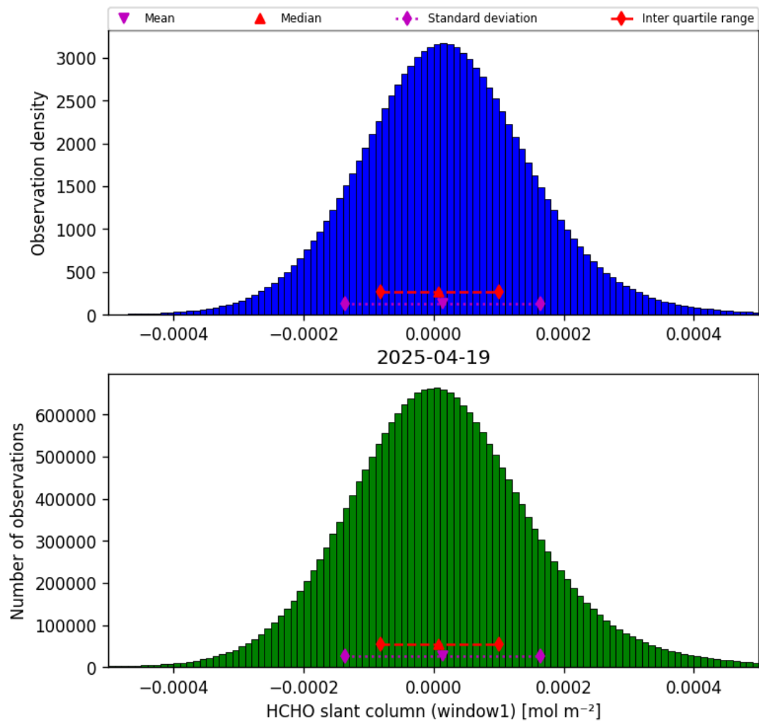
Figure 36: Histogram of “HCHO slant column (window1)” for 2025-04-19 to 2025-04-20
