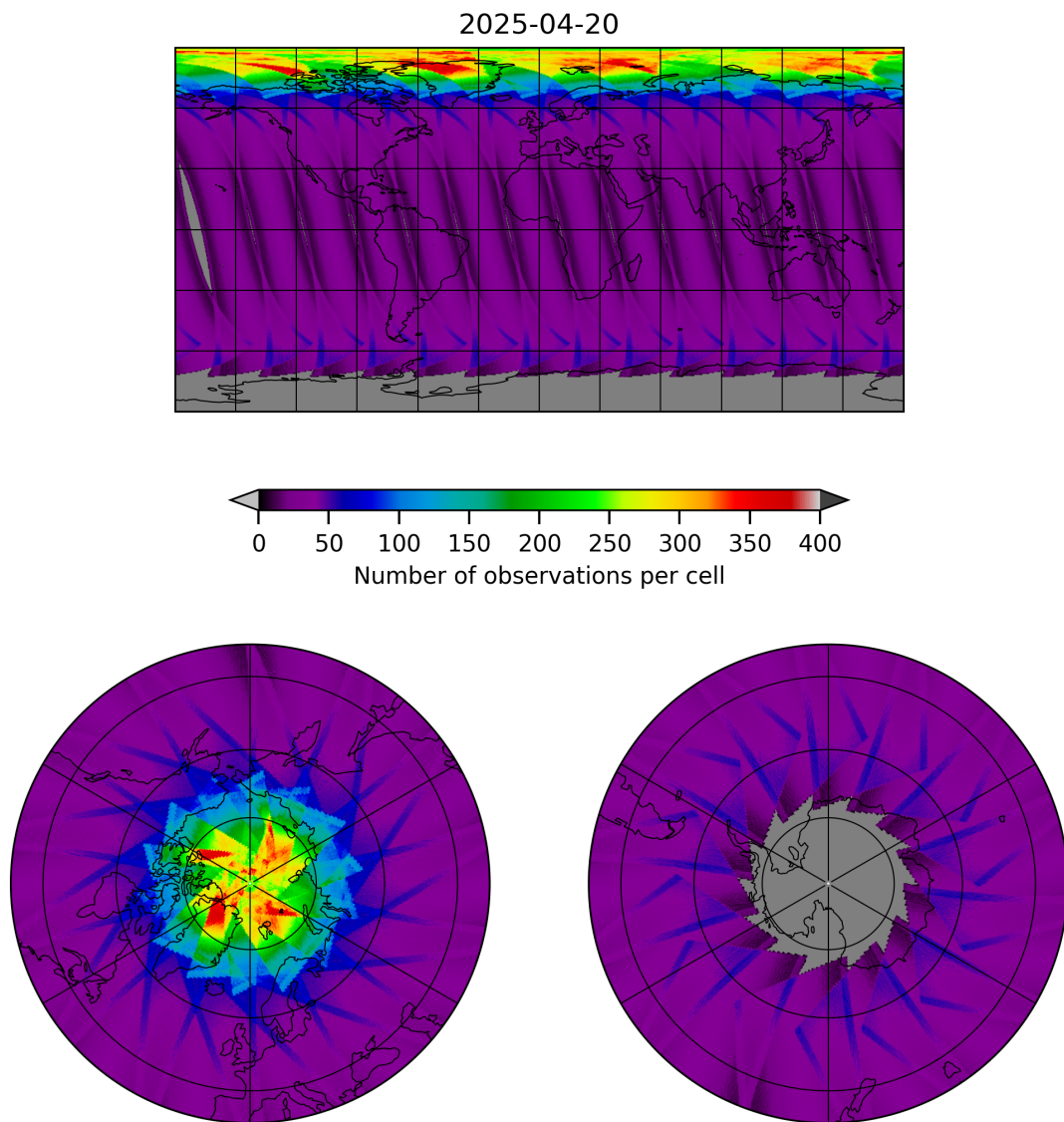
Figure 17: Map of the number of observations for 2025-04-20 to 2025-04-21
