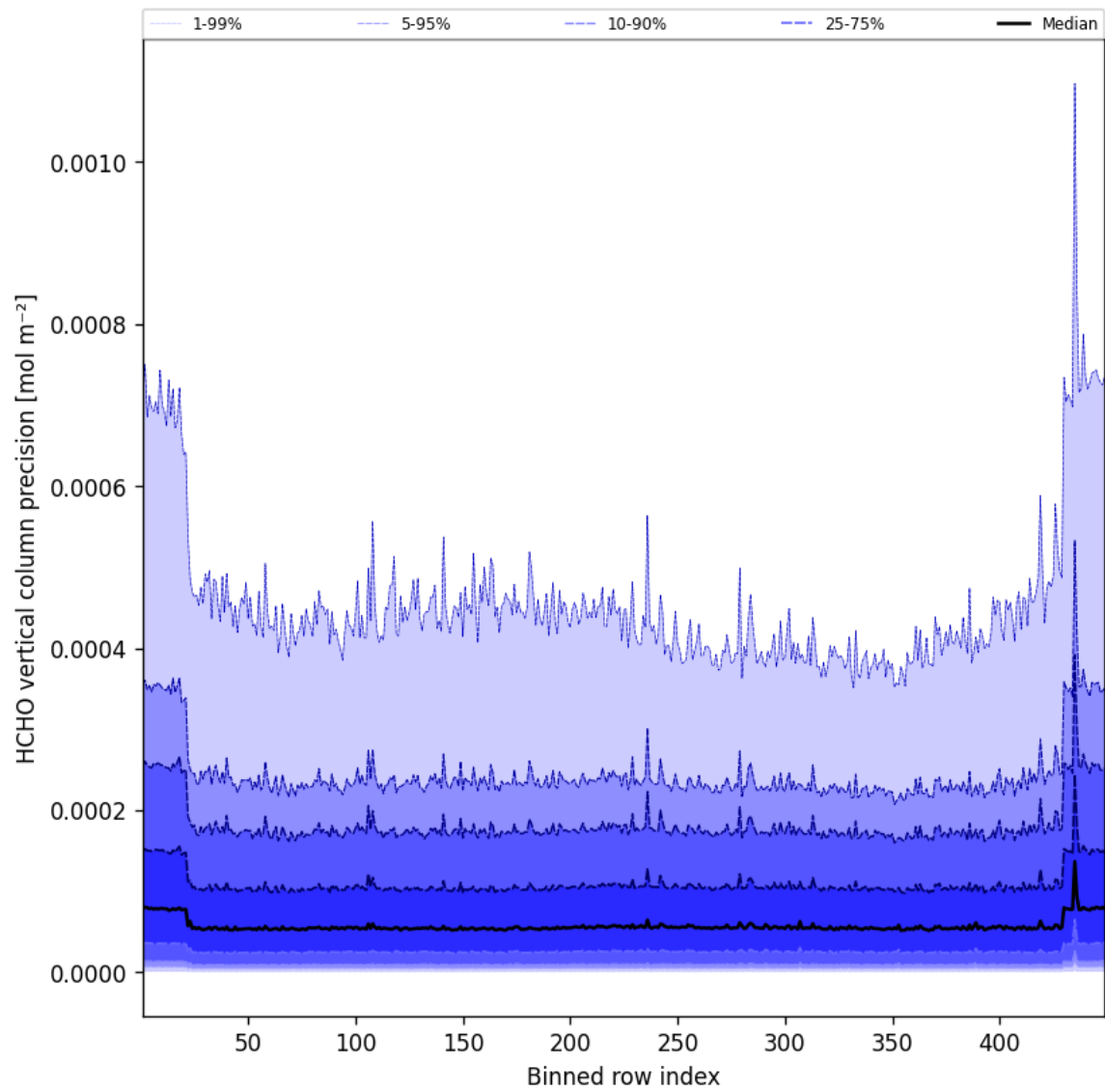
Figure 48: Along track statistics of “HCHO vertical column precision” for 2025-04-20 to 2025-04-21
