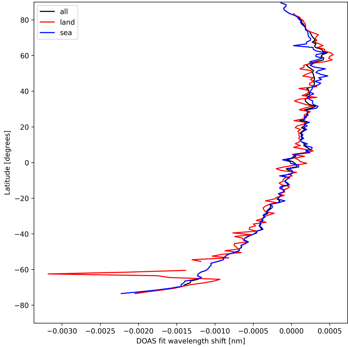
Figure 28: Zonal average of "DOAS fit wavelength shift" for 2025-04-20 to 2025-04-21.
