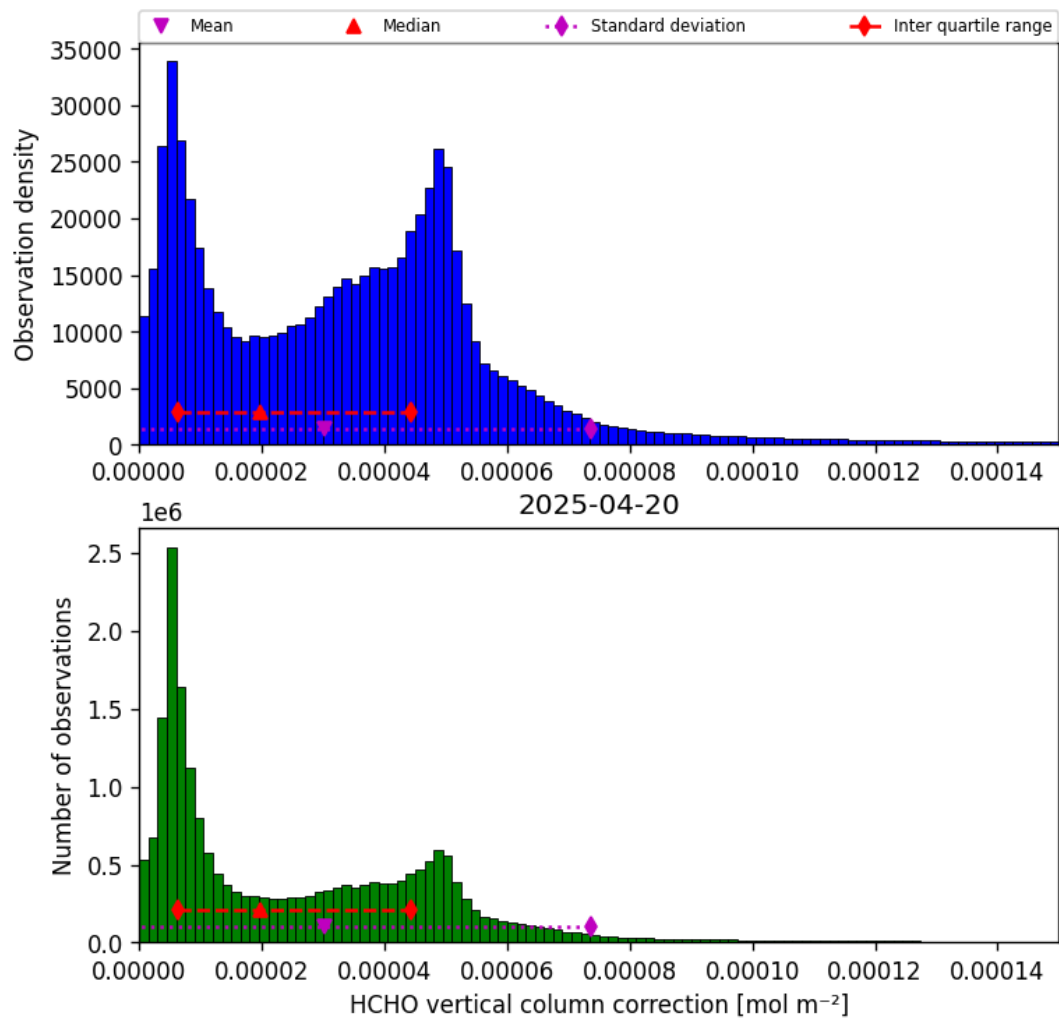
Figure 35: Histogram of “HCHO vertical column correction” for 2025-04-20 to 2025-04-21
