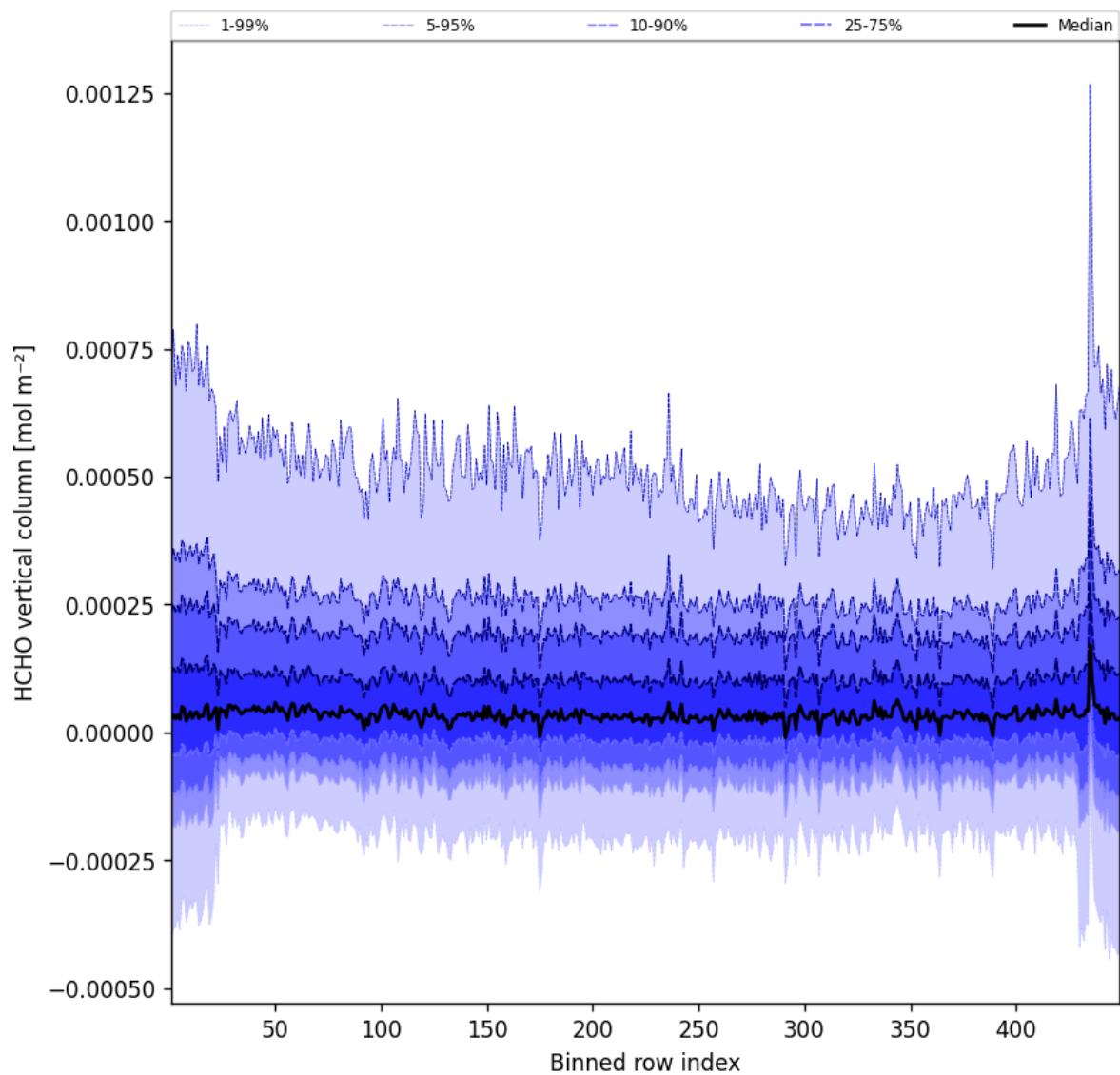
Figure 47: Along track statistics of “HCHO vertical column” for 2025-04-20 to 2025-04-21
