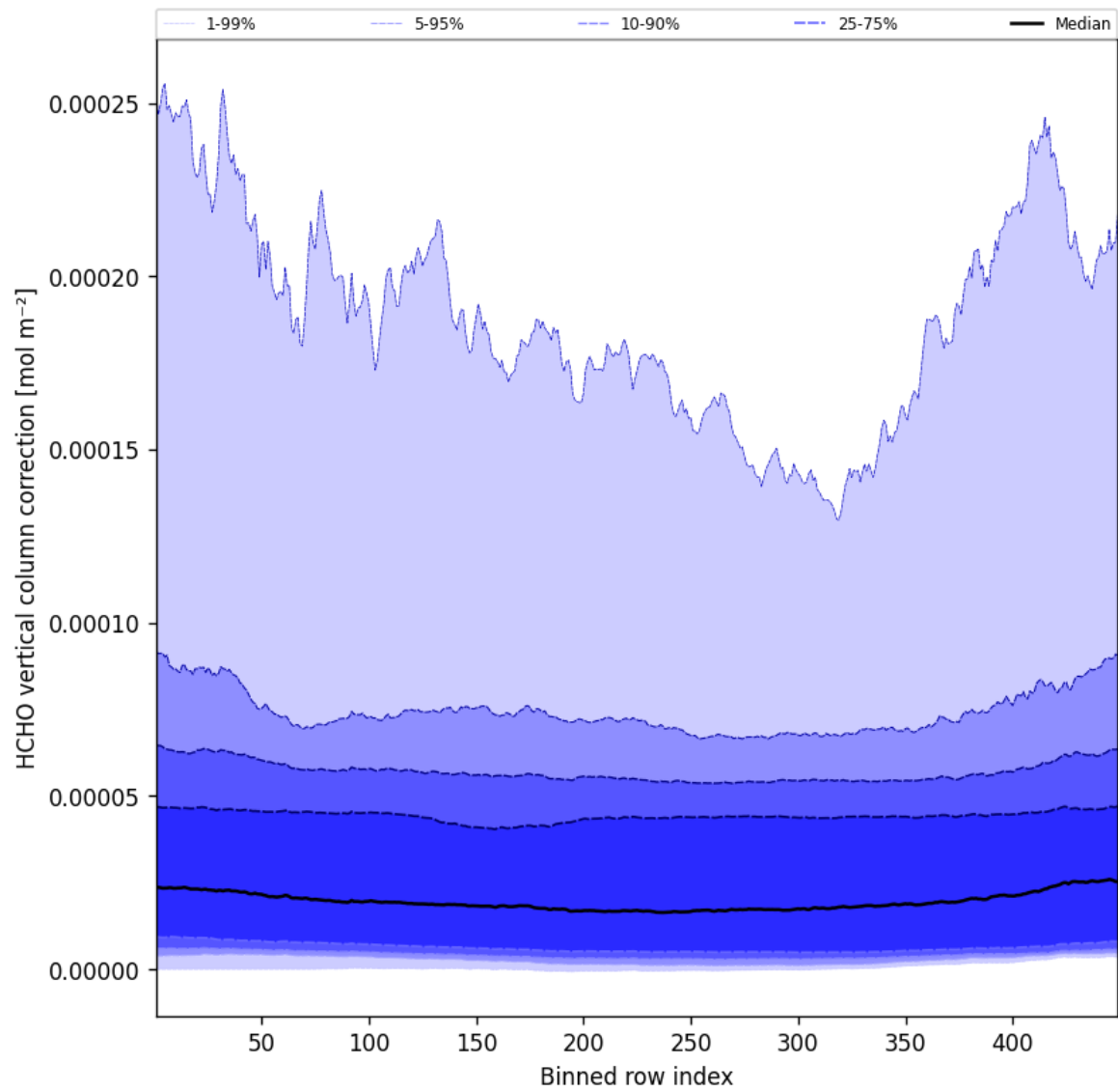
Figure 49: Along track statistics of “HCHO vertical column correction” for 2025-04-20 to 2025-04-21
