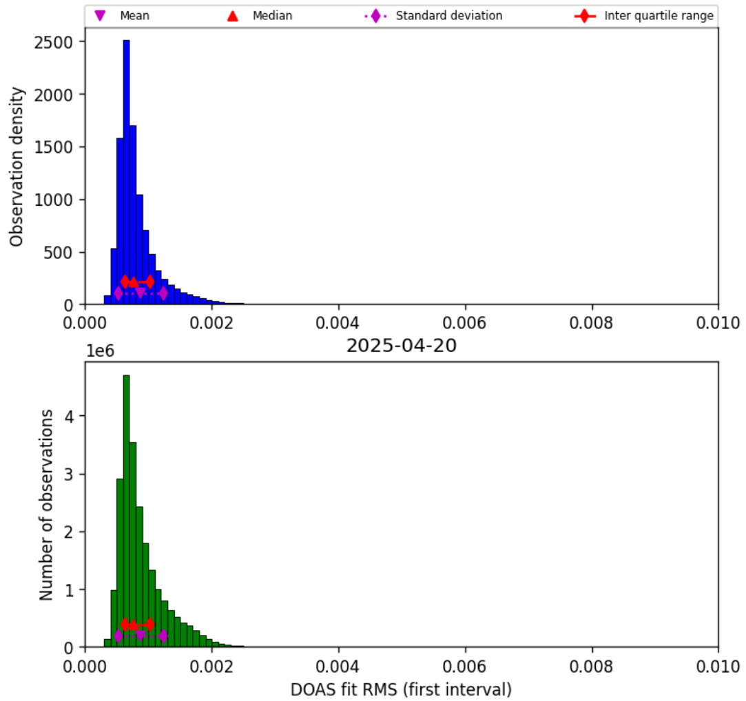
Figure 44: Histogram of “DOAS fit RMS (first interval)” for 2025-04-20 to 2025-04-21
