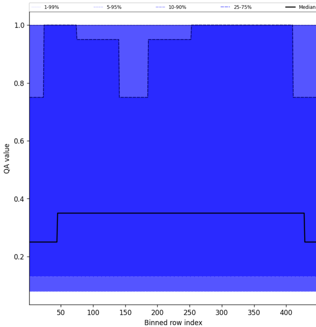
Figure 46: Along track statistics of “QA value” for 2025-04-20 to 2025-04-21
