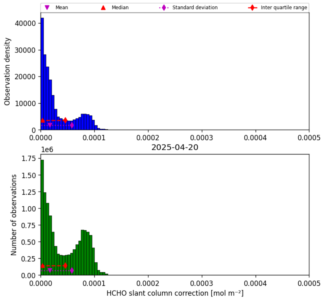
Figure 45: Histogram of “HCHO slant column correction” for 2025-04-20 to 2025-04-21
