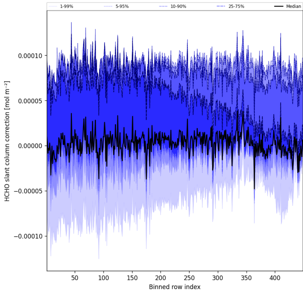
Figure 59: Along track statistics of “HCHO slant column correction” for 2025-04-20 to 2025-04-21
