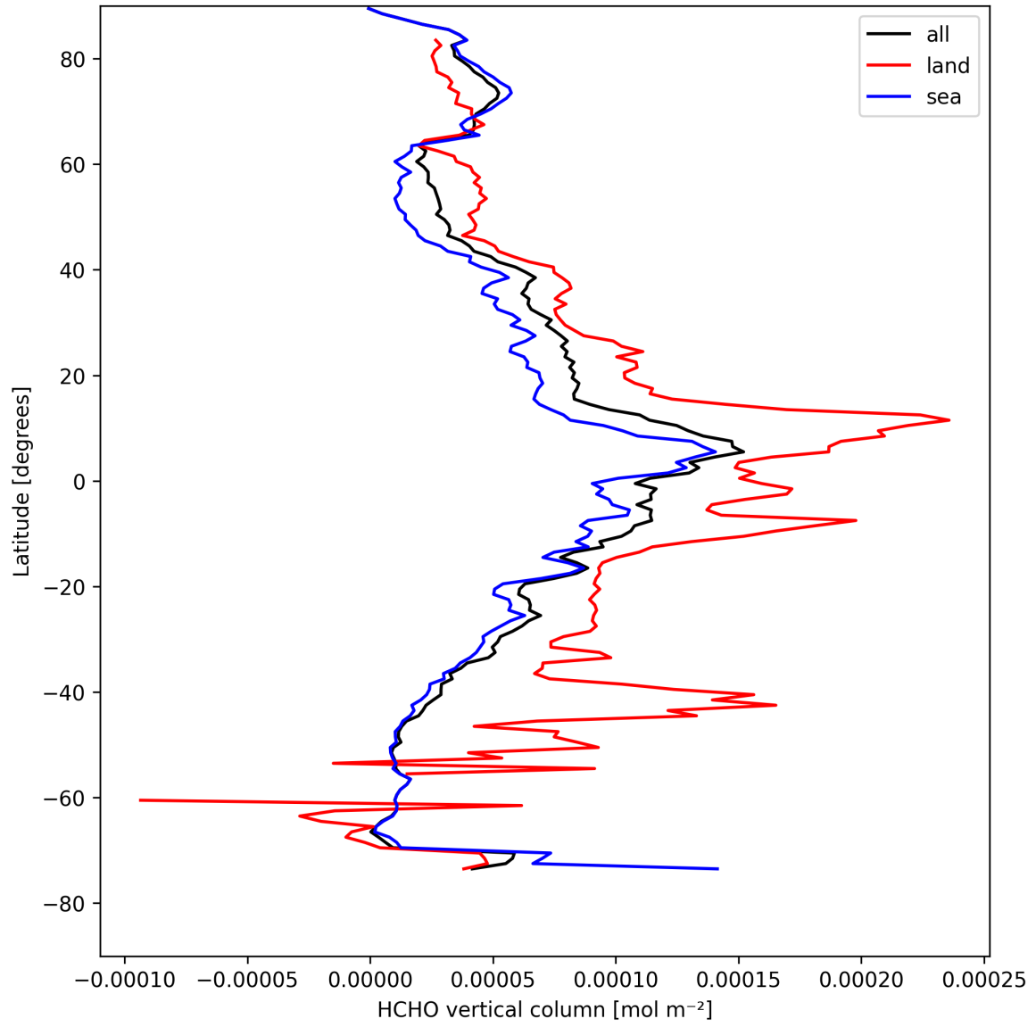
Figure 19: Zonal average of “HCHO vertical column” for 2025-04-20 to 2025-04-21.
