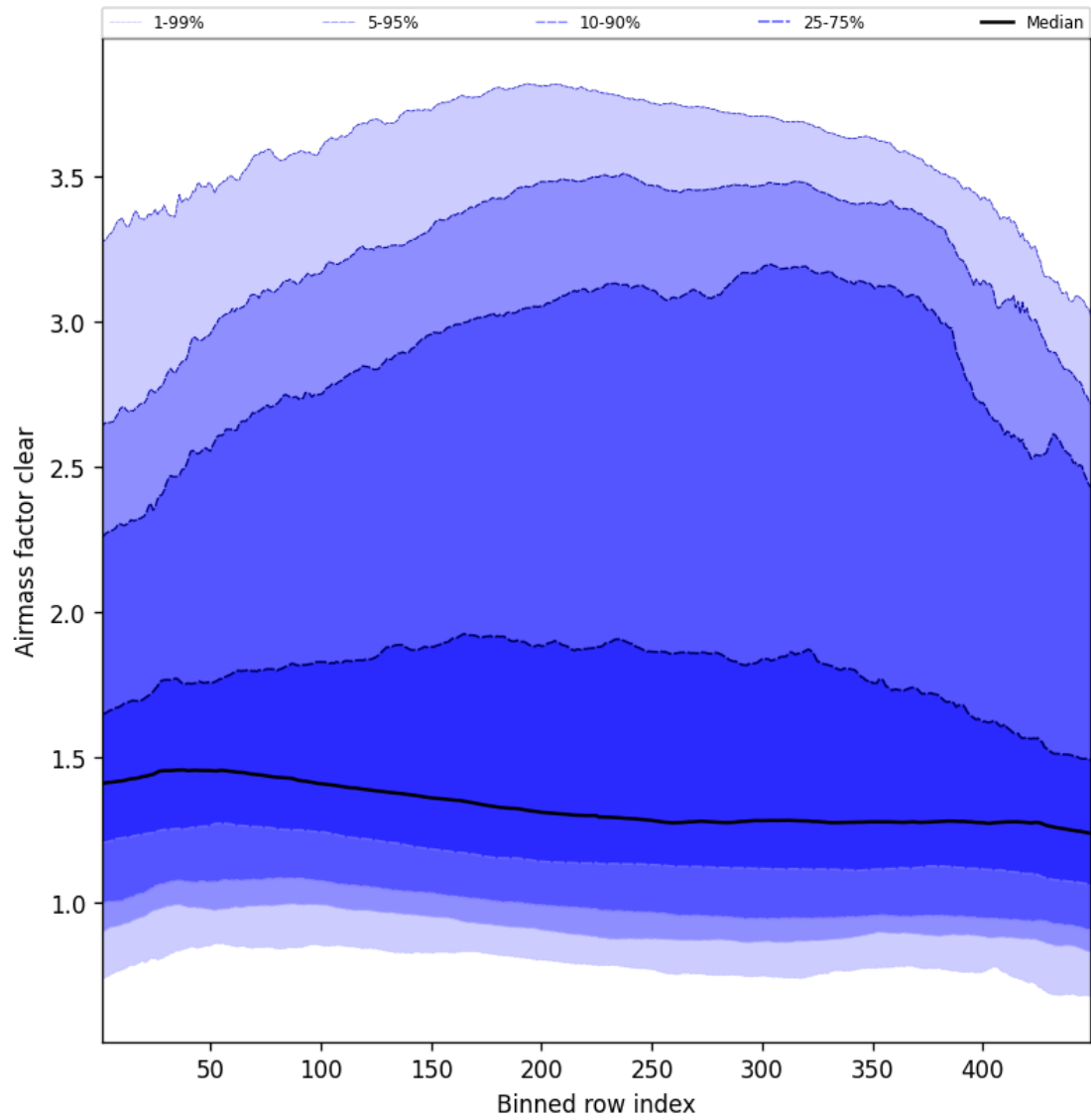
Figure 54: Along track statistics of “Airmass factor clear” for 2025-04-20 to 2025-04-21
