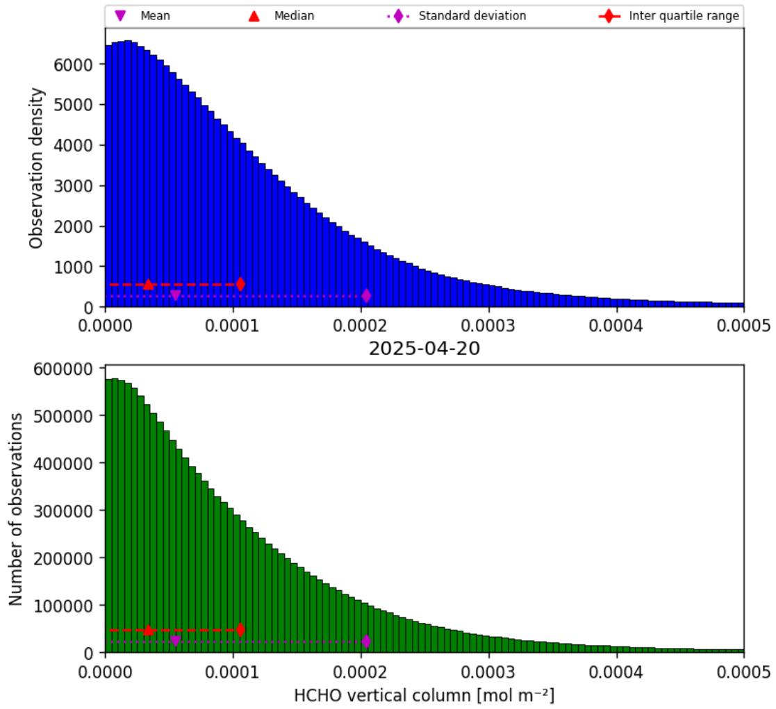
Figure 33: Histogram of “HCHO vertical column” for 2025-04-20 to 2025-04-21
