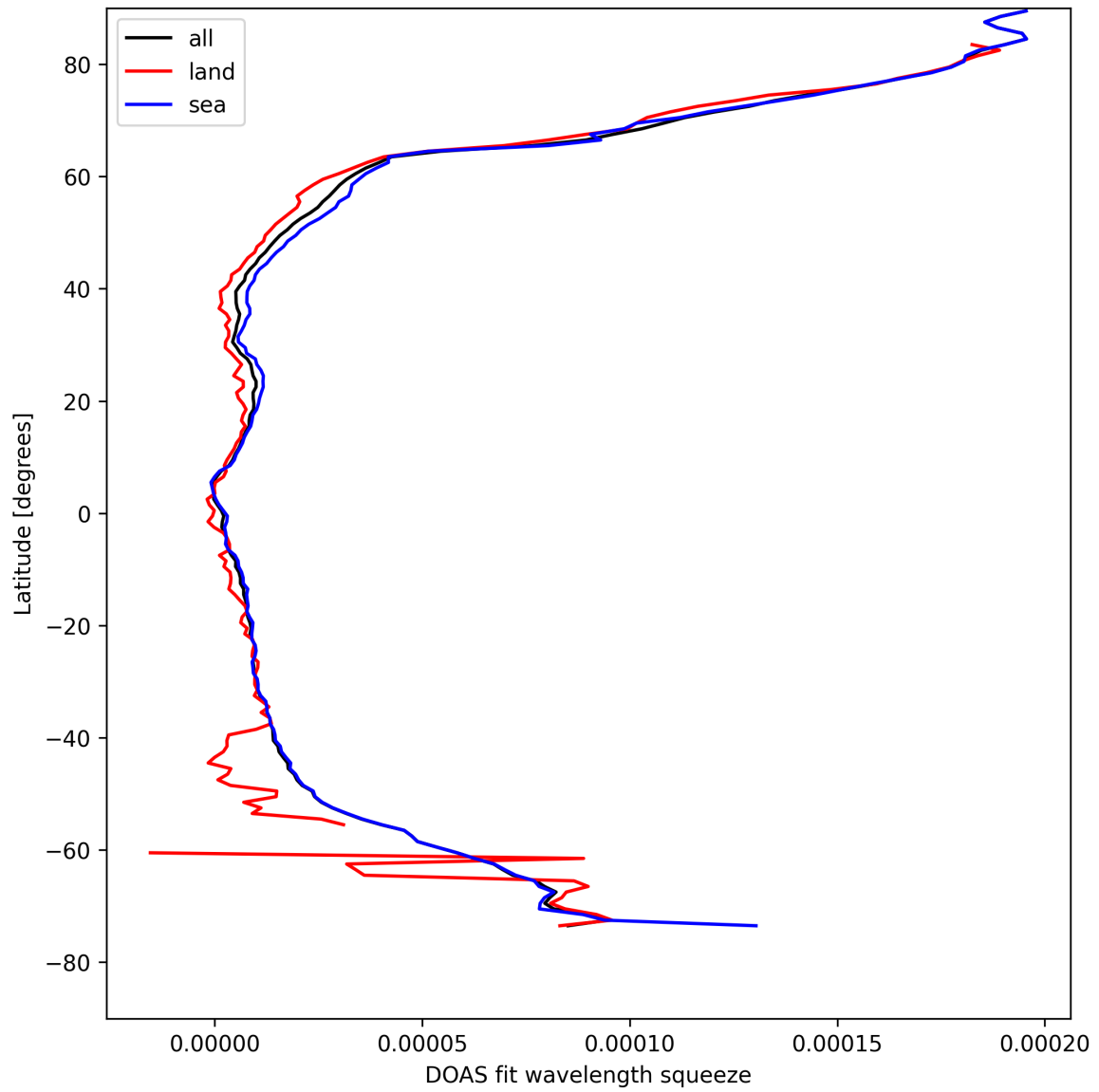
Figure 29: Zonal average of “DOAS fit wavelength squeeze” for 2025-04-20 to 2025-04-21.
