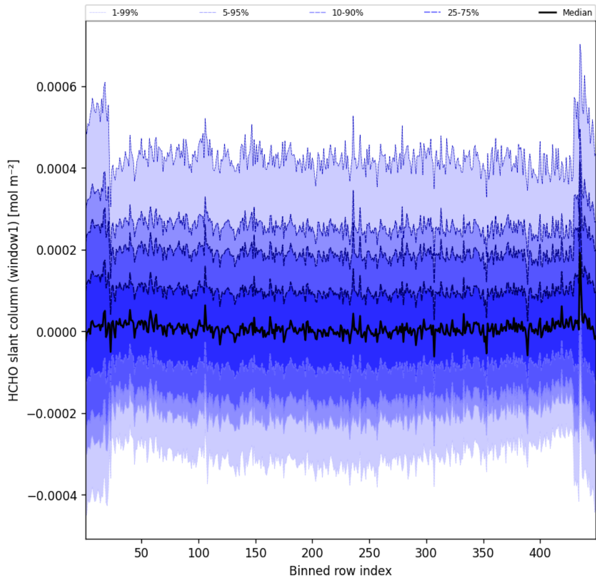
Figure 50: Along track statistics of “HCHO slant column (window1)” for 2025-04-20 to 2025-04-21
