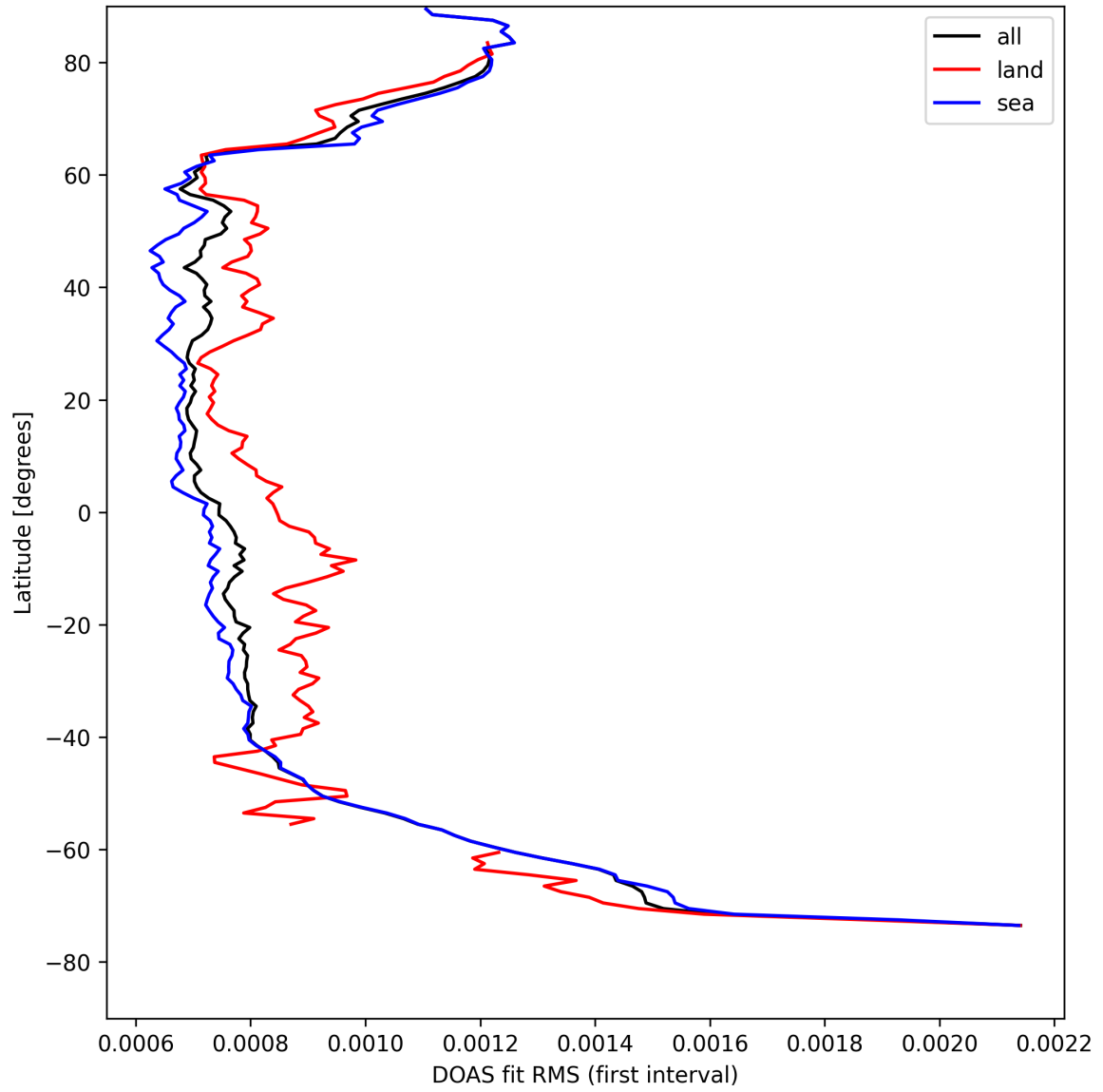
Figure 30: Zonal average of “DOAS fit RMS (first interval)” for 2025-04-20 to 2025-04-21.
