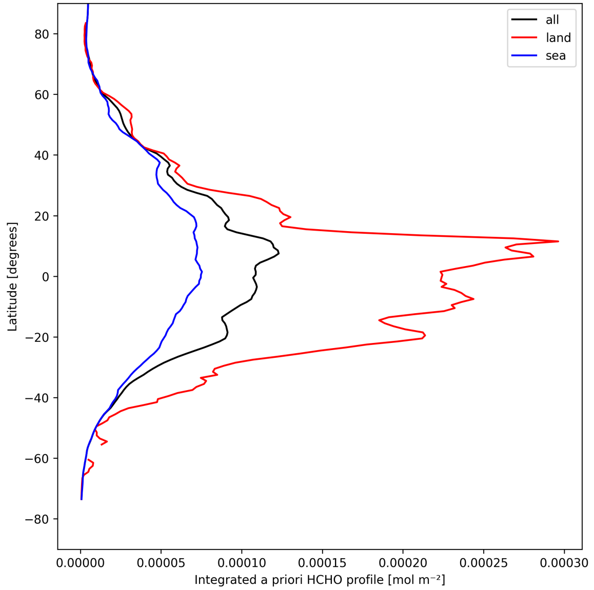
Figure 27: Zonal average of “Integrated a priori HCHO profile” for 2025-04-20 to 2025-04-21.
