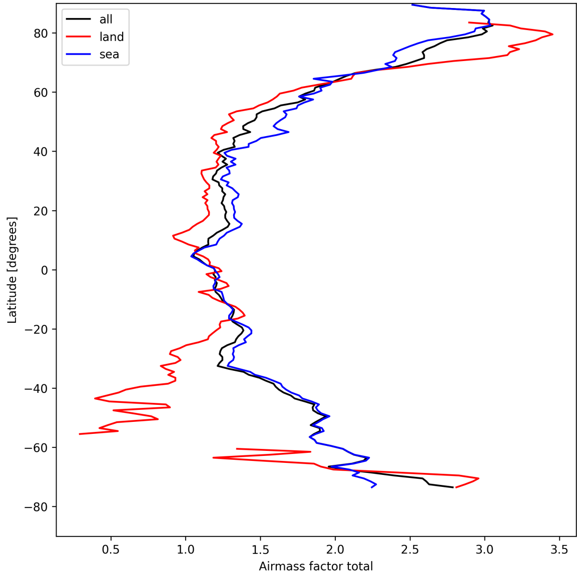
Figure 24: Zonal average of “Airmass factor total” for 2025-04-20 to 2025-04-21.
