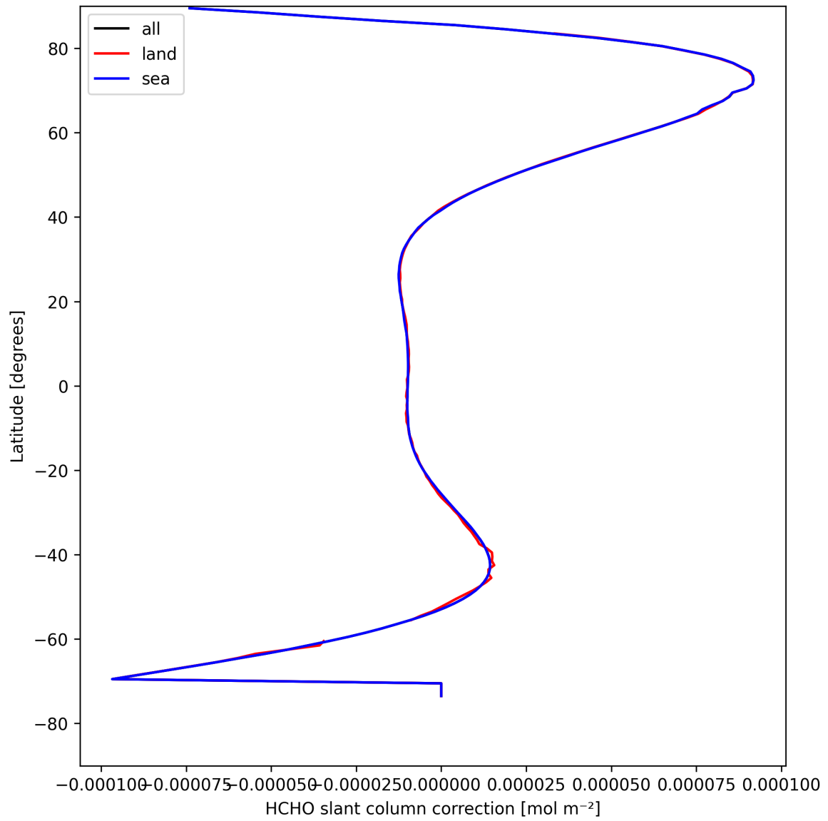
Figure 31: Zonal average of “HCHO slant column correction” for 2025-04-20 to 2025-04-21.
