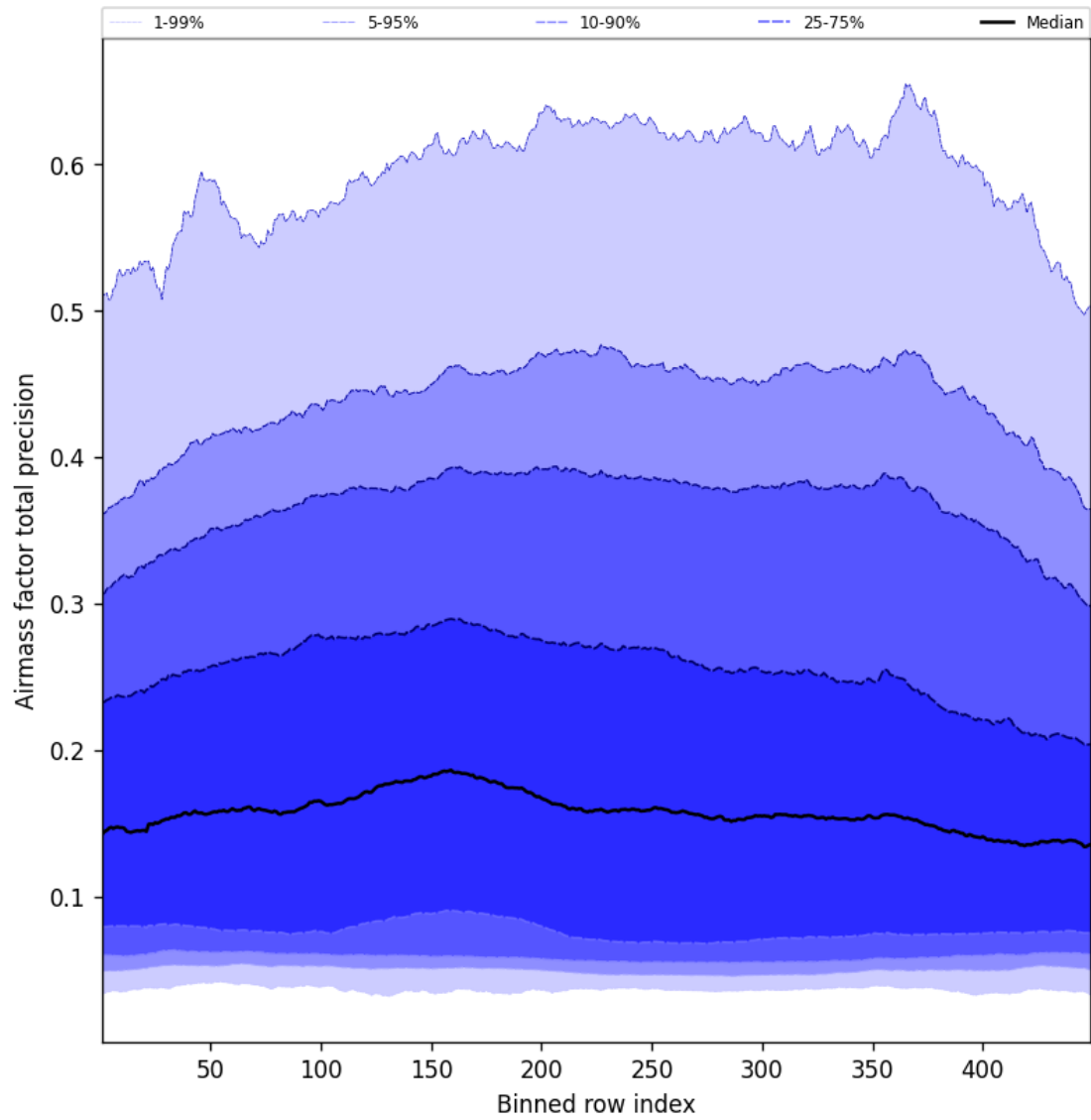
Figure 53: Along track statistics of “Airmass factor total precision” for 2025-04-20 to 2025-04-21
