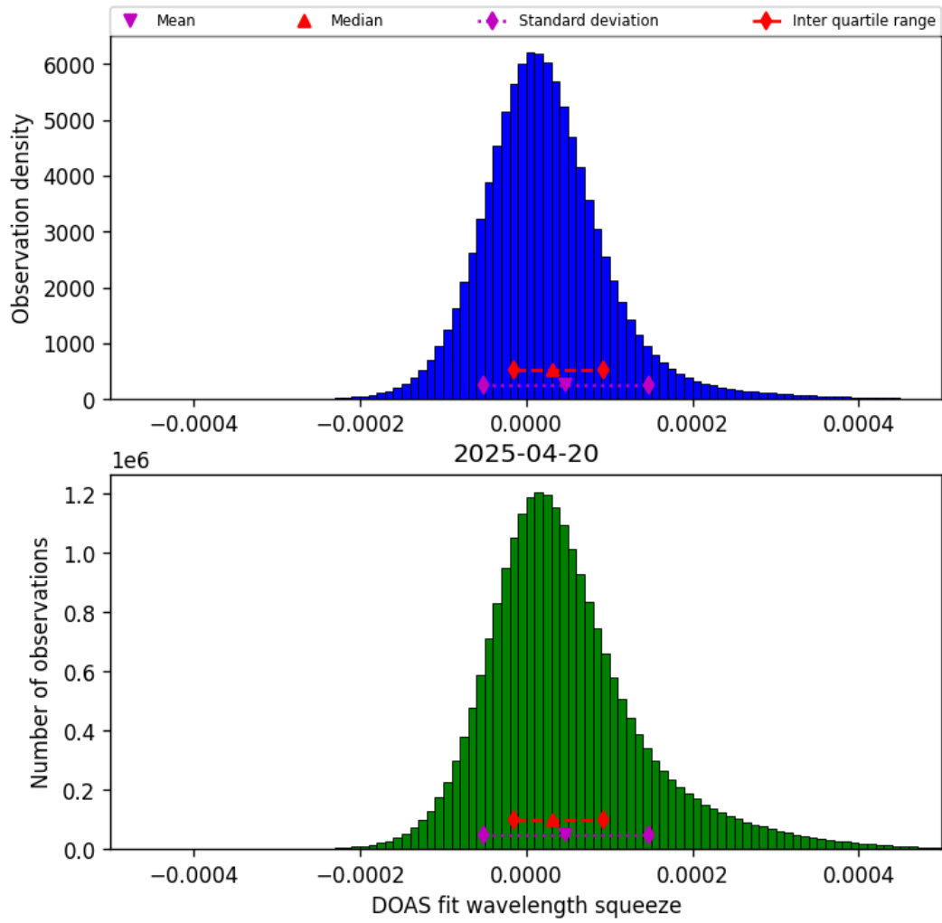
Figure 43: Histogram of “DOAS fit wavelength squeeze” for 2025-04-20 to 2025-04-21
