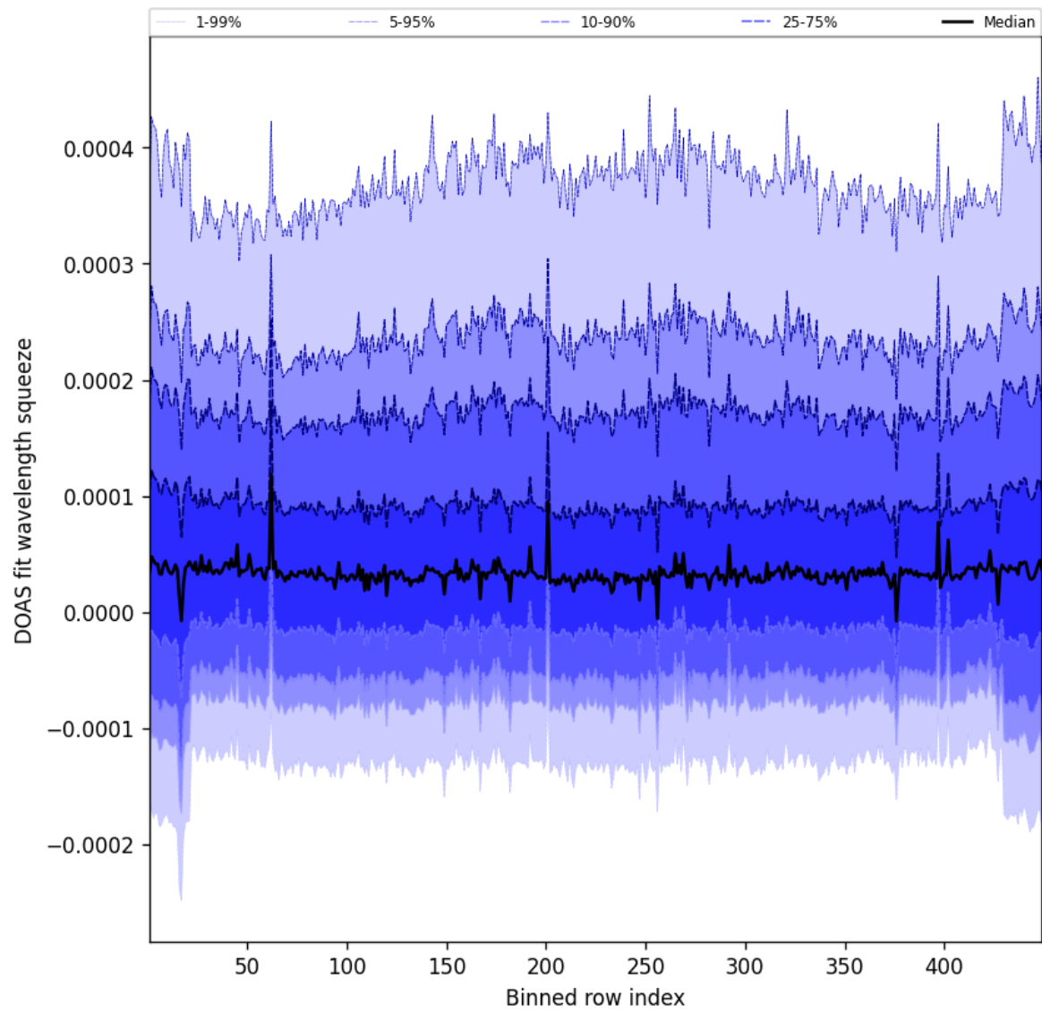
Figure 57: Along track statistics of “DOAS fit wavelength squeeze” for 2025-04-20 to 2025-04-21
