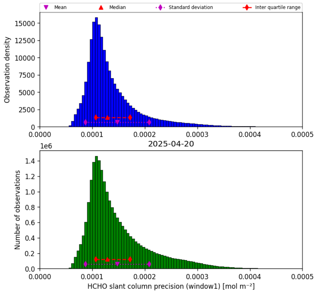
Figure 37: Histogram of “HCHO slant column precision (window1)” for 2025-04-20 to 2025-04-21
