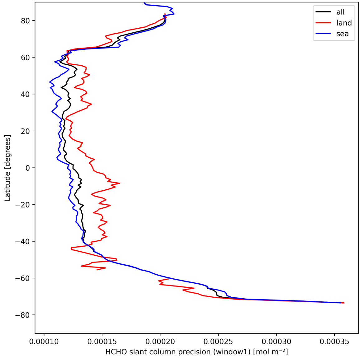
Figure 23: Zonal average of “HCHO slant column precision (window1)” for 2025-04-20 to 2025-04-21.
