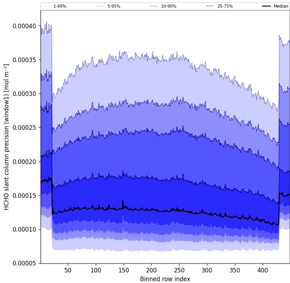
Figure 51: Along track statistics of “HCHO slant column precision (window1)” for 2025-04-20 to 2025-04-21
