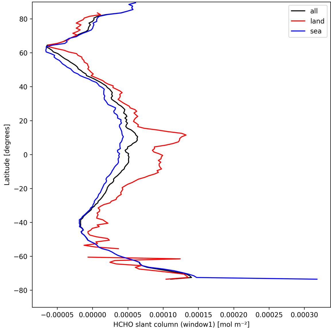
Figure 22: Zonal average of “HCHO slant column (window1)” for 2025-04-20 to 2025-04-21.
