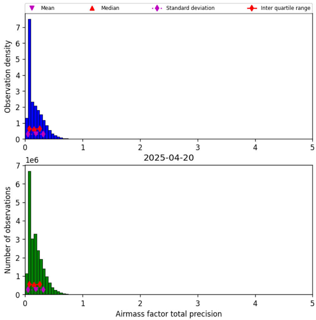
Figure 39: Histogram of “Airmass factor total precision” for 2025-04-20 to 2025-04-21
