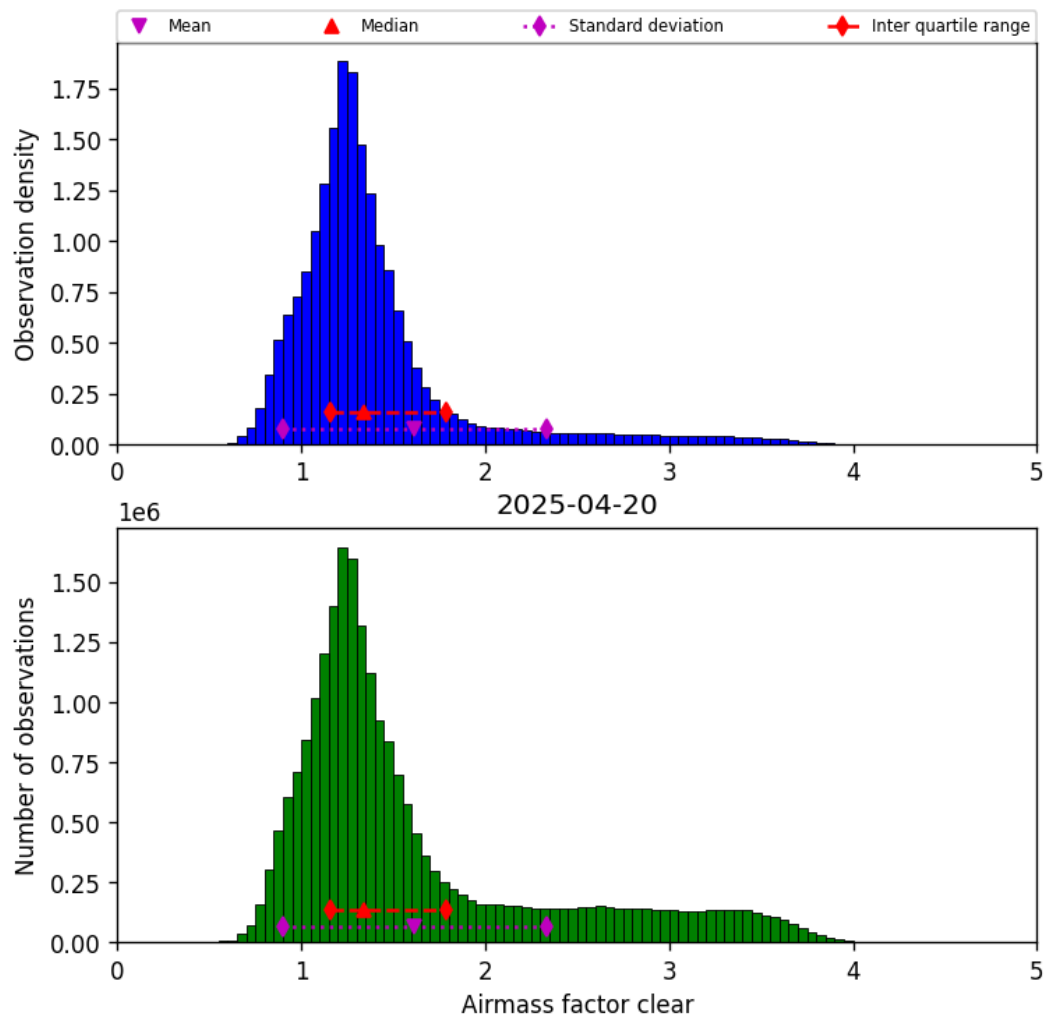
Figure 40: Histogram of “Airmass factor clear” for 2025-04-20 to 2025-04-21
