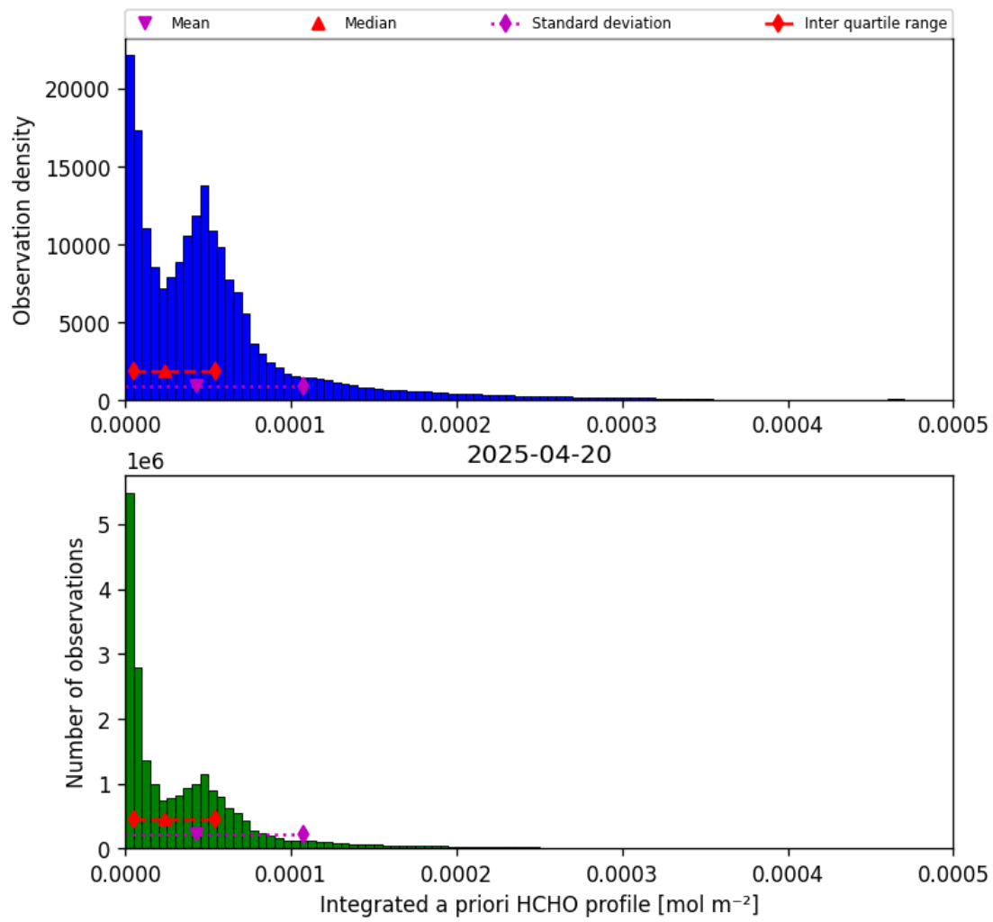
Figure 41: Histogram of “Integrated a priori HCHO profile” for 2025-04-20 to 2025-04-21
