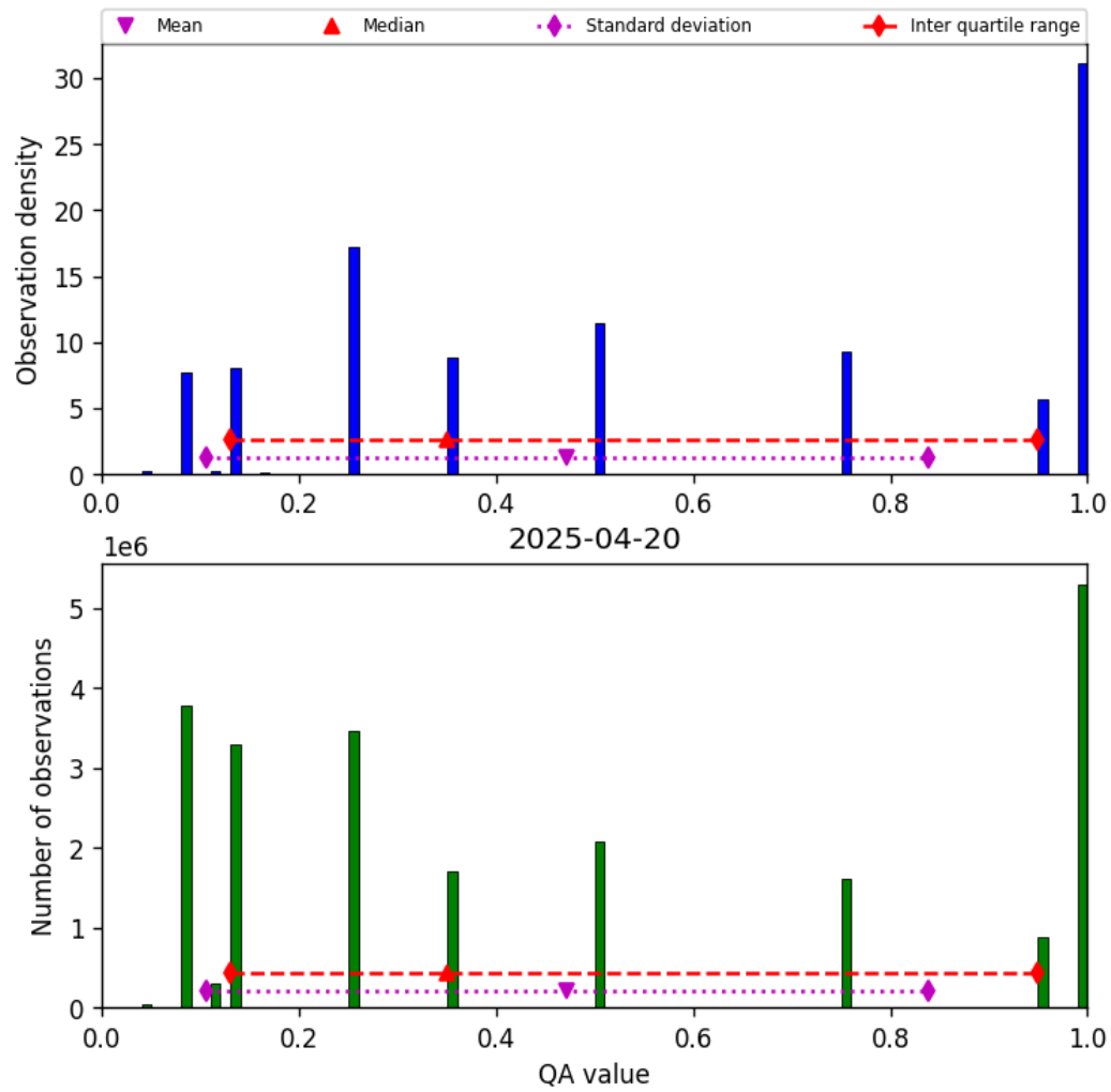
Figure 32: Histogram of “QA value” for 2025-04-20 to 2025-04-21
