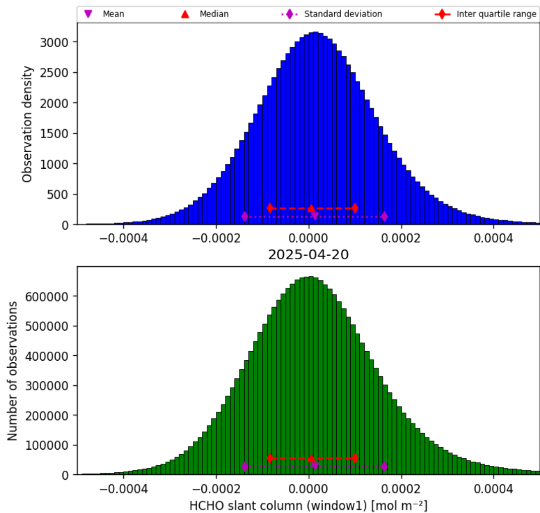
Figure 36: Histogram of “HCHO slant column (window1)” for 2025-04-20 to 2025-04-21
