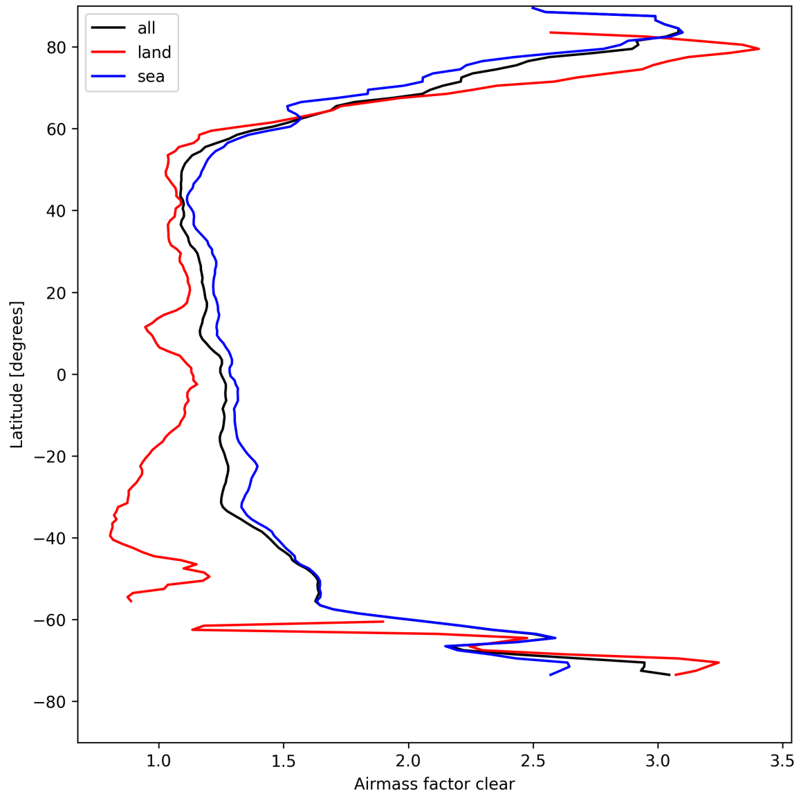
Figure 26: Zonal average of “Airmass factor clear” for 2025-04-20 to 2025-04-21.
