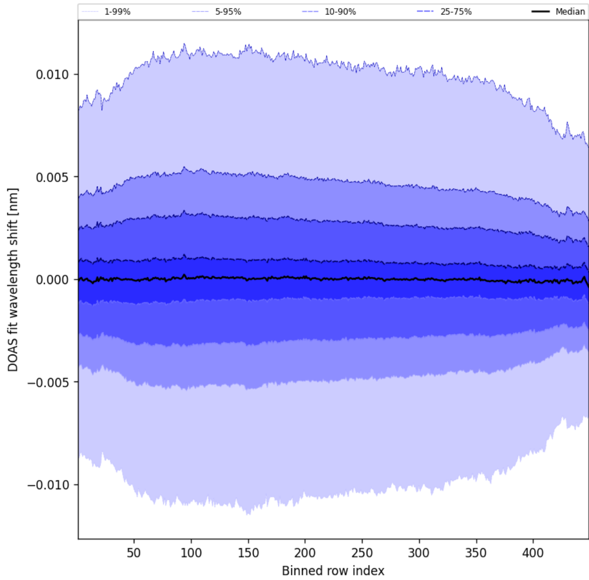
Figure 56: Along track statistics of “DOAS fit wavelength shift” for 2025-04-20 to 2025-04-21
