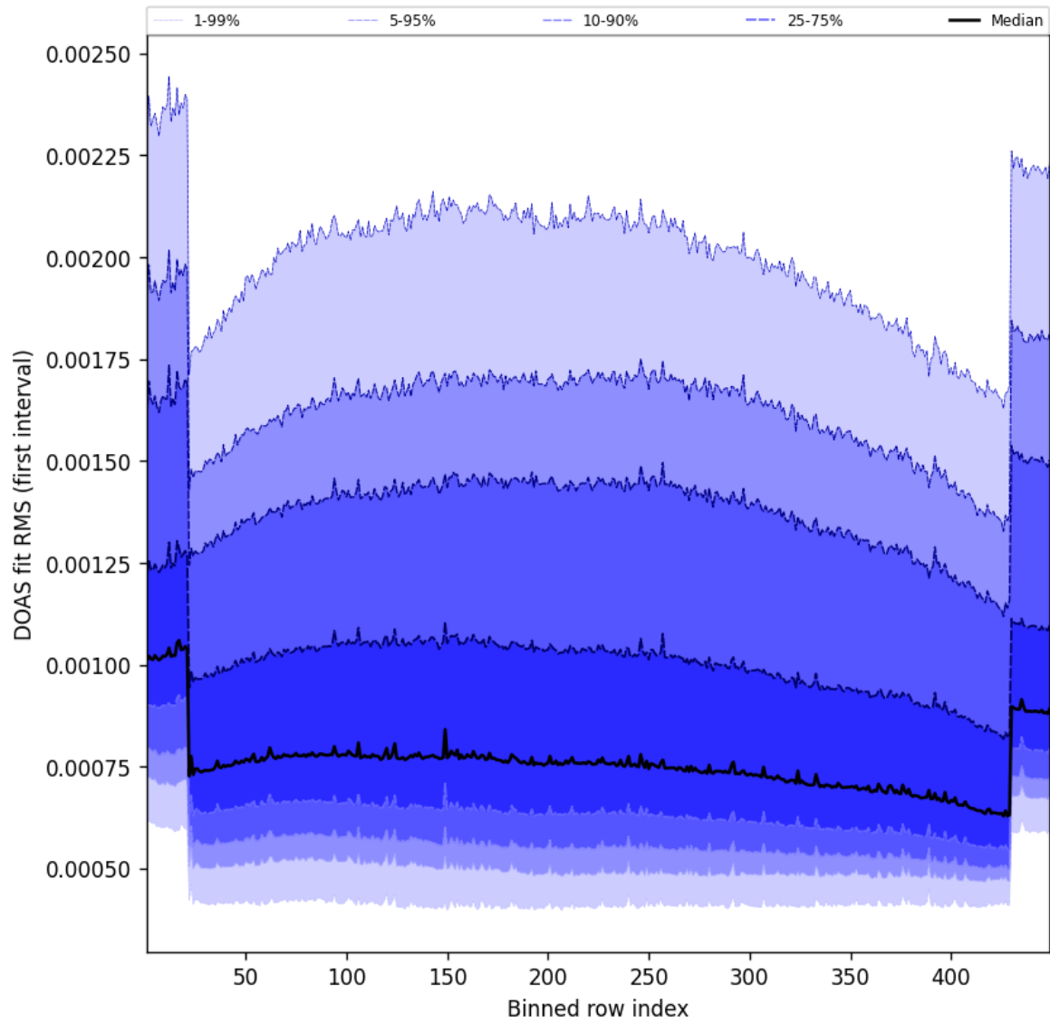
Figure 58: Along track statistics of “DOAS fit RMS (first interval)” for 2025-04-20 to 2025-04-21
