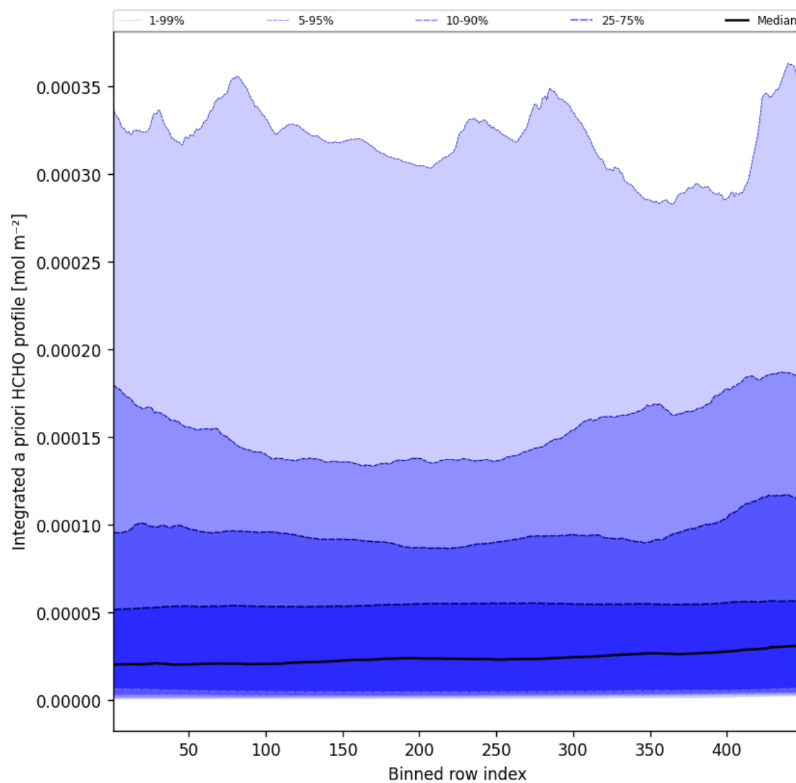
Figure 55: Along track statistics of “Integrated a priori HCHO profile” for 2025-04-20 to 2025-04-21
