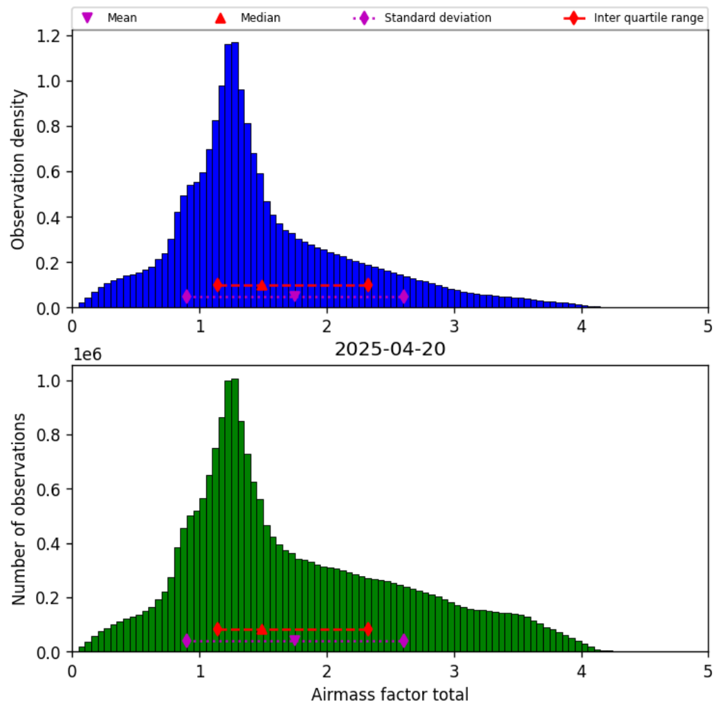
Figure 38: Histogram of “Airmass factor total” for 2025-04-20 to 2025-04-21
