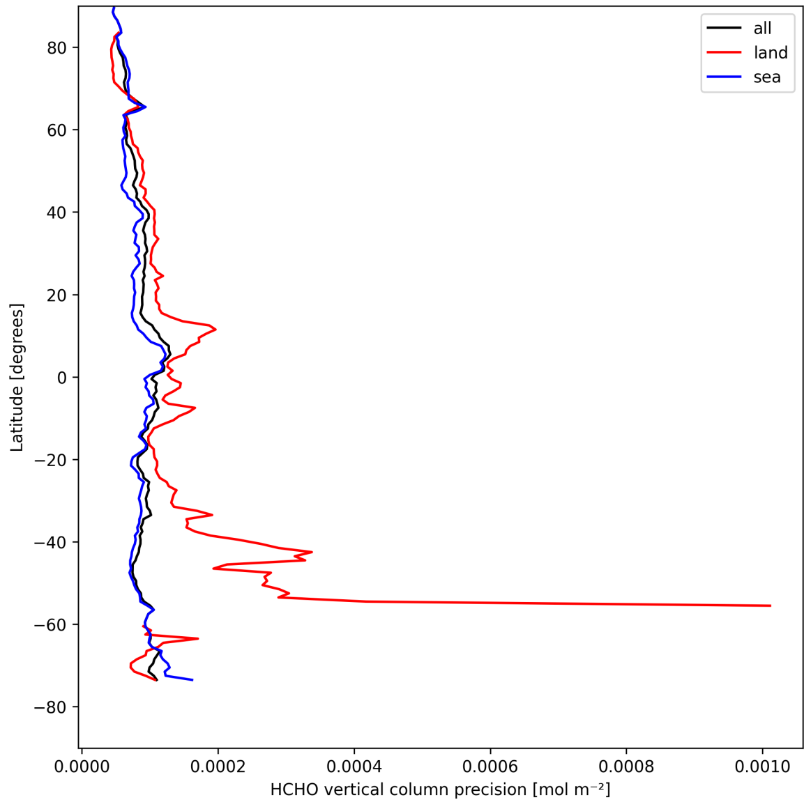
Figure 20: Zonal average of “HCHO vertical column precision” for 2025-04-20 to 2025-04-21.
