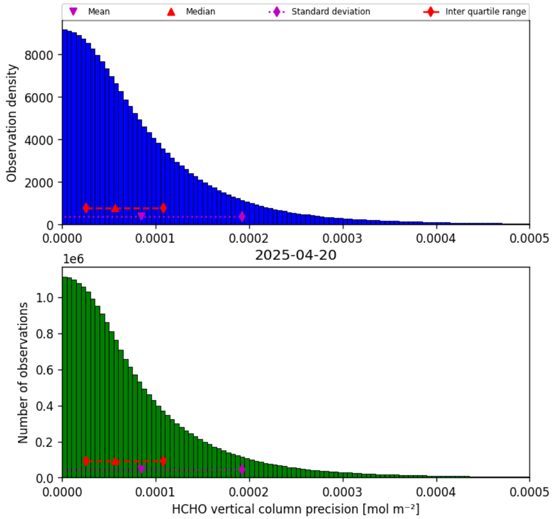
Figure 34: Histogram of “HCHO vertical column precision” for 2025-04-20 to 2025-04-21
