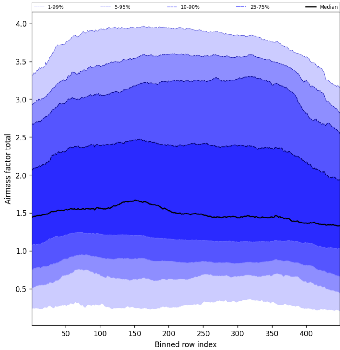
Figure 52: Along track statistics of “Airmass factor total” for 2025-04-20 to 2025-04-21
