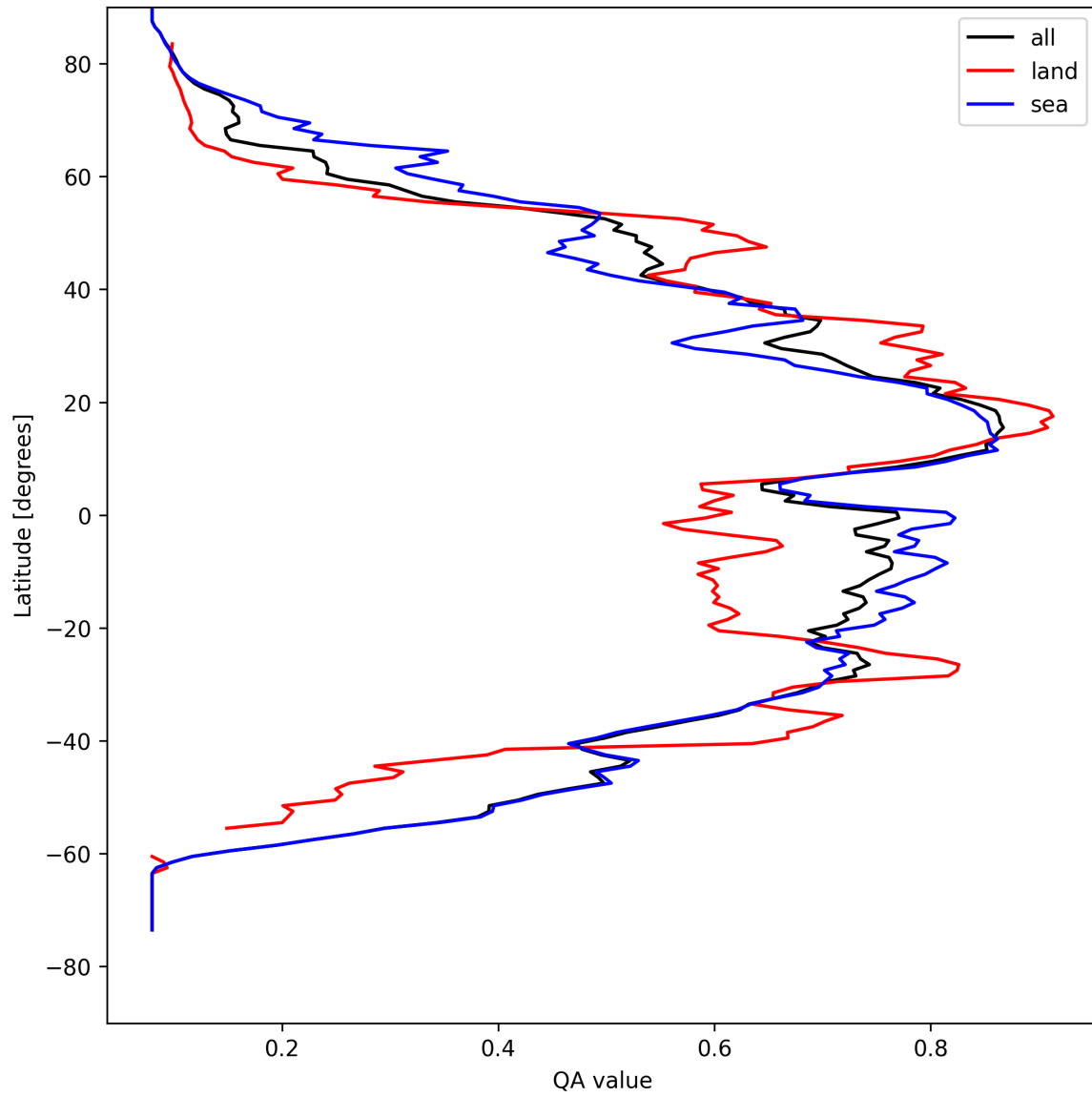
Figure 18: Zonal average of “QA value” for 2025-04-20 to 2025-04-21.
