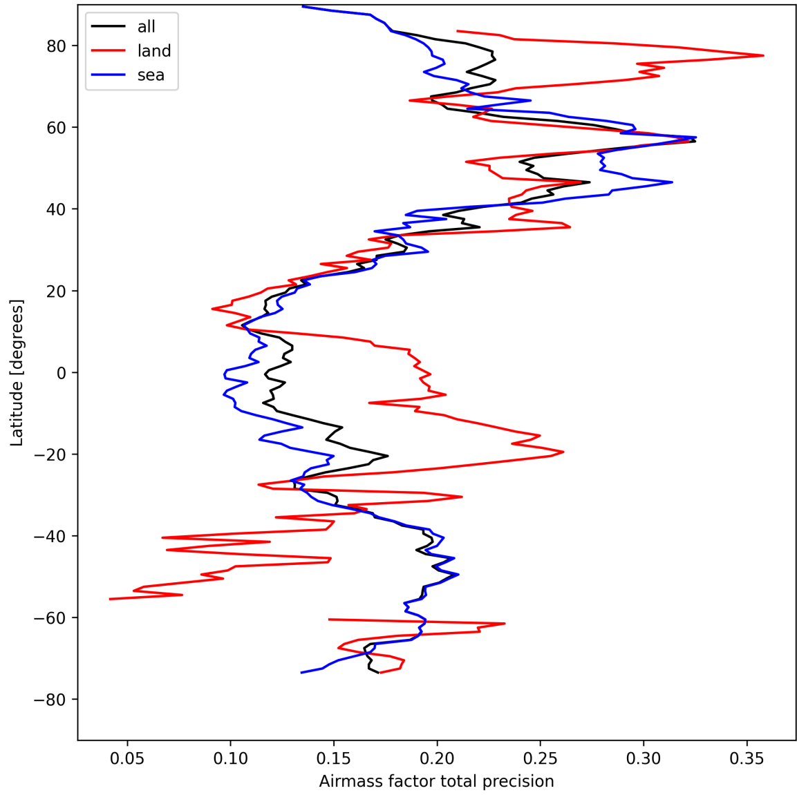
Figure 25: Zonal average of “Airmass factor total precision” for 2025-04-20 to 2025-04-21.
