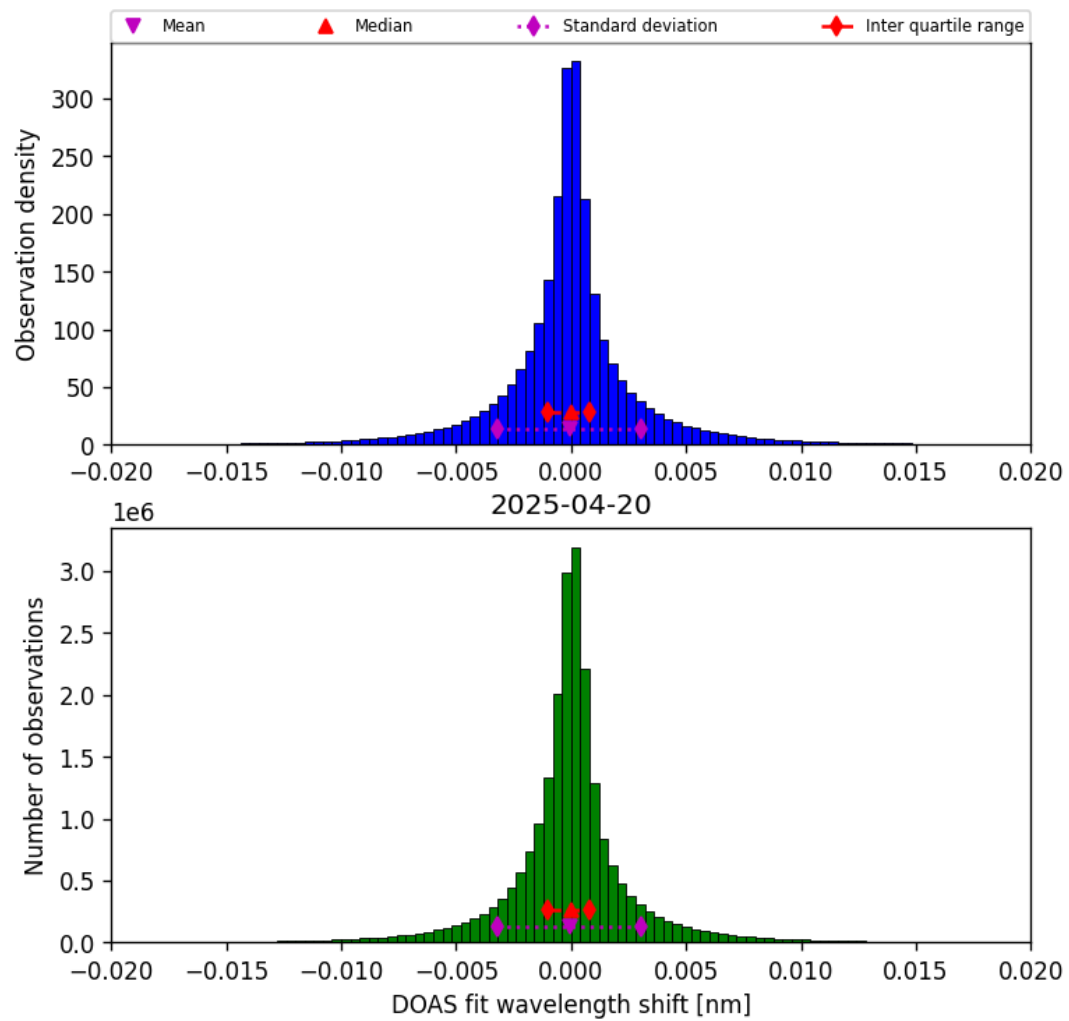
Figure 42: Histogram of “DOAS fit wavelength shift” for 2025-04-20 to 2025-04-21
