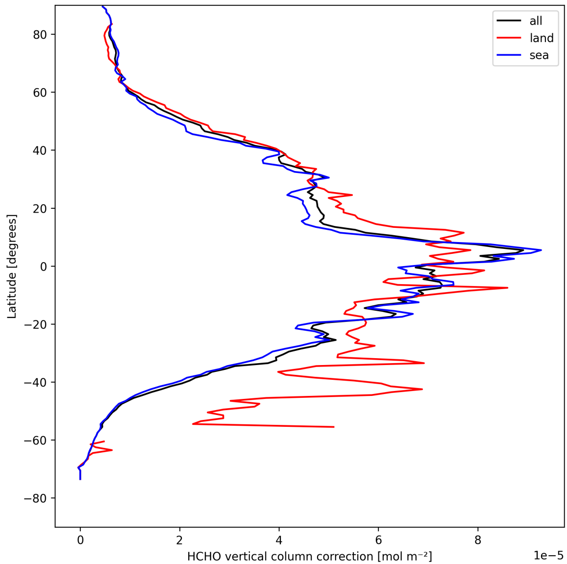
Figure 21: Zonal average of “HCHO vertical column correction” for 2025-04-20 to 2025-04-21.
