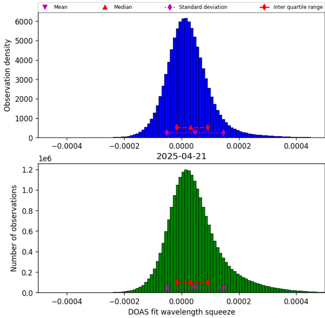
Figure 43: Histogram of “DOAS fit wavelength squeeze” for 2025-04-21 to 2025-04-22
