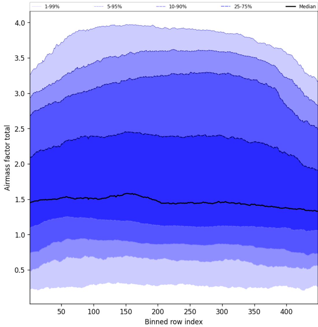
Figure 52: Along track statistics of “Airmass factor total” for 2025-04-21 to 2025-04-22
