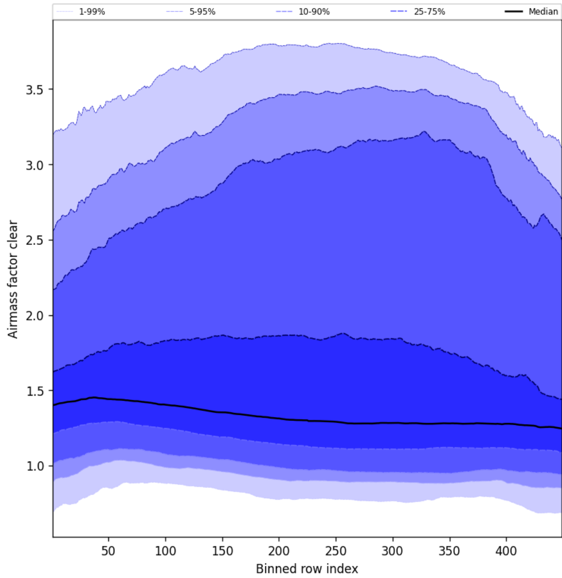
Figure 54: Along track statistics of “Airmass factor clear” for 2025-04-21 to 2025-04-22
