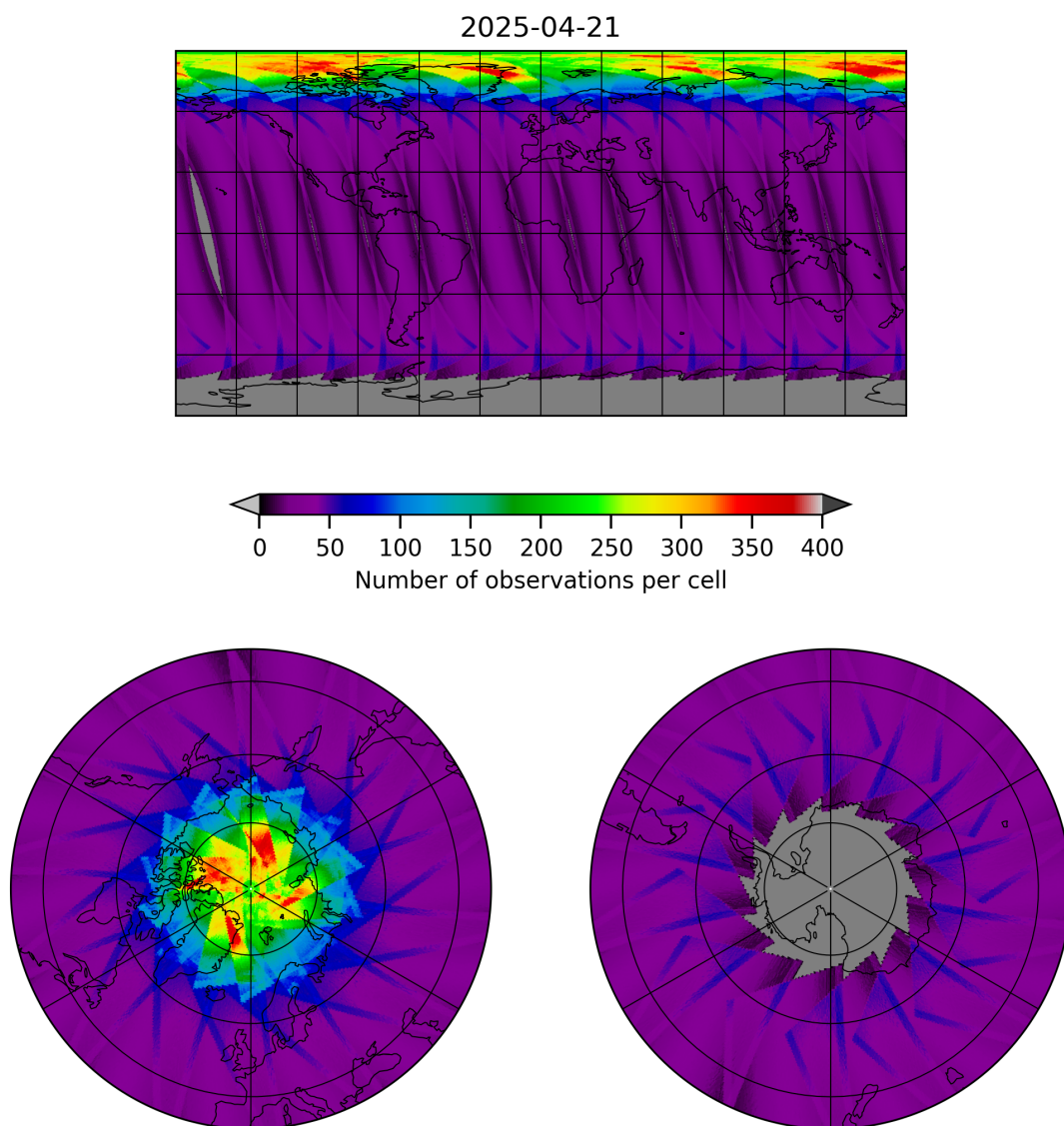
Figure 17: Map of the number of observations for 2025-04-21 to 2025-04-22
