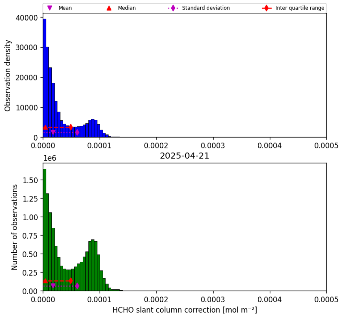
Figure 45: Histogram of “HCHO slant column correction” for 2025-04-21 to 2025-04-22
