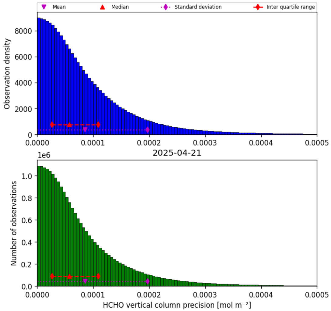
Figure 34: Histogram of “HCHO vertical column precision” for 2025-04-21 to 2025-04-22
