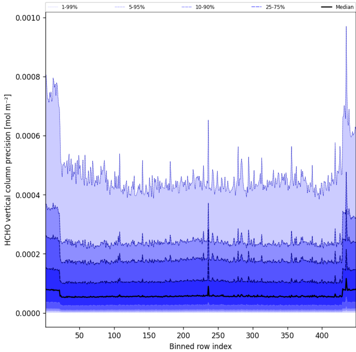
Figure 48: Along track statistics of "HCHO vertical column precision" for 2025-04-21 to 2025-04-22
