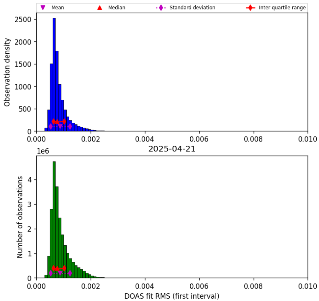
Figure 44: Histogram of "DOAS fit RMS (first interval)" for 2025-04-21 to 2025-04-22
