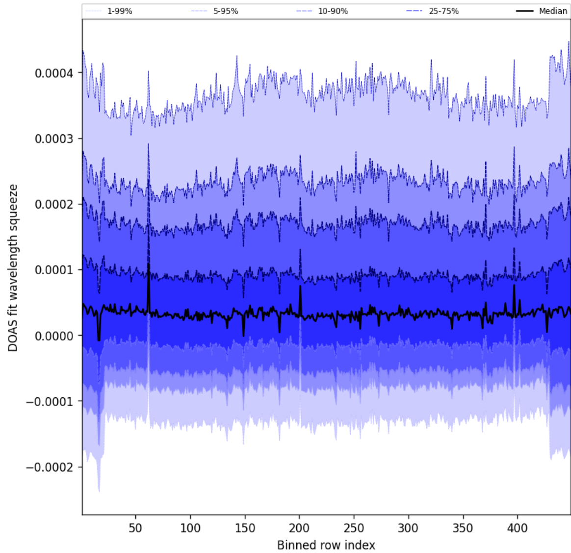
Figure 57: Along track statistics of “DOAS fit wavelength squeeze” for 2025-04-21 to 2025-04-22
