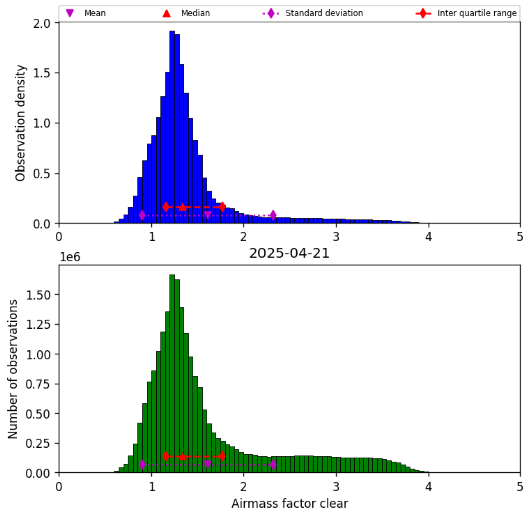
Figure 40: Histogram of “Airmass factor clear” for 2025-04-21 to 2025-04-22
