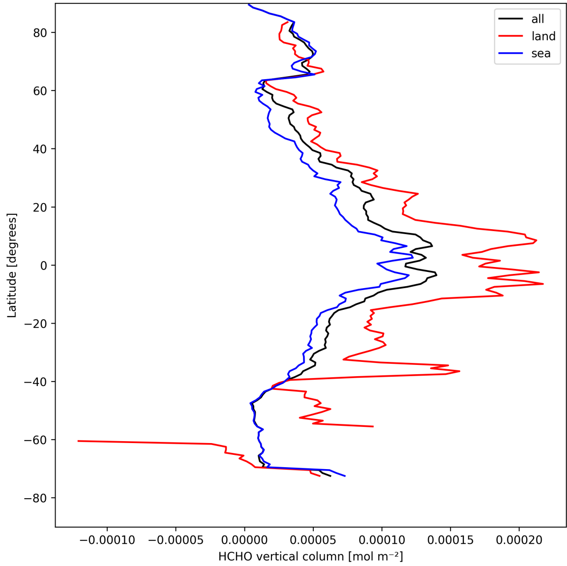
Figure 19: Zonal average of “HCHO vertical column” for 2025-04-21 to 2025-04-22.
