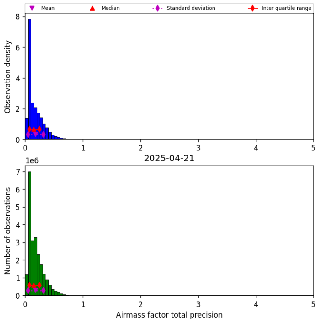
Figure 39: Histogram of “Airmass factor total precision” for 2025-04-21 to 2025-04-22
