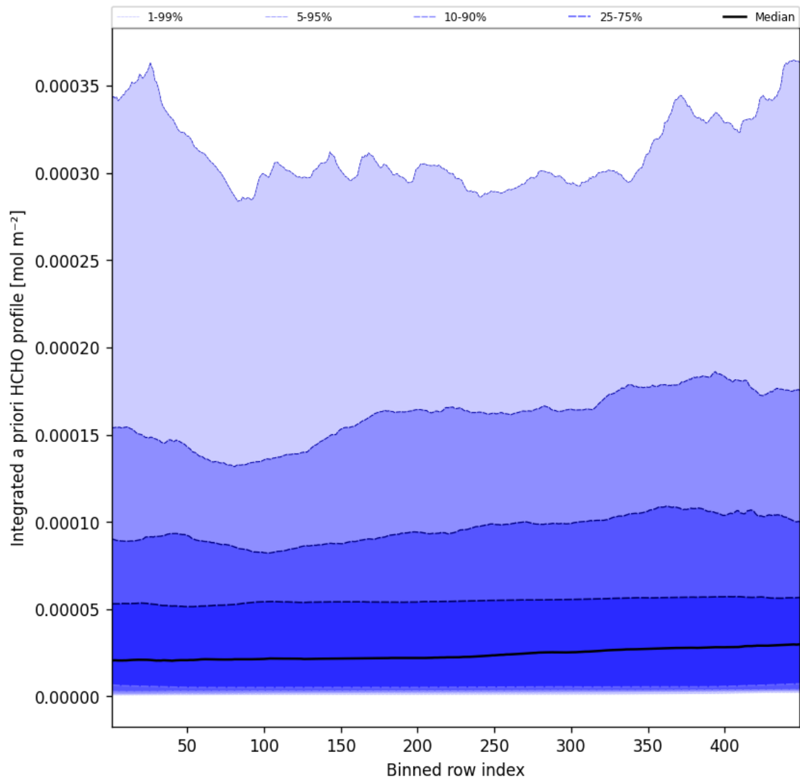
Figure 55: Along track statistics of "Integrated a priori HCHO profile" for 2025-04-21 to 2025-04-22
