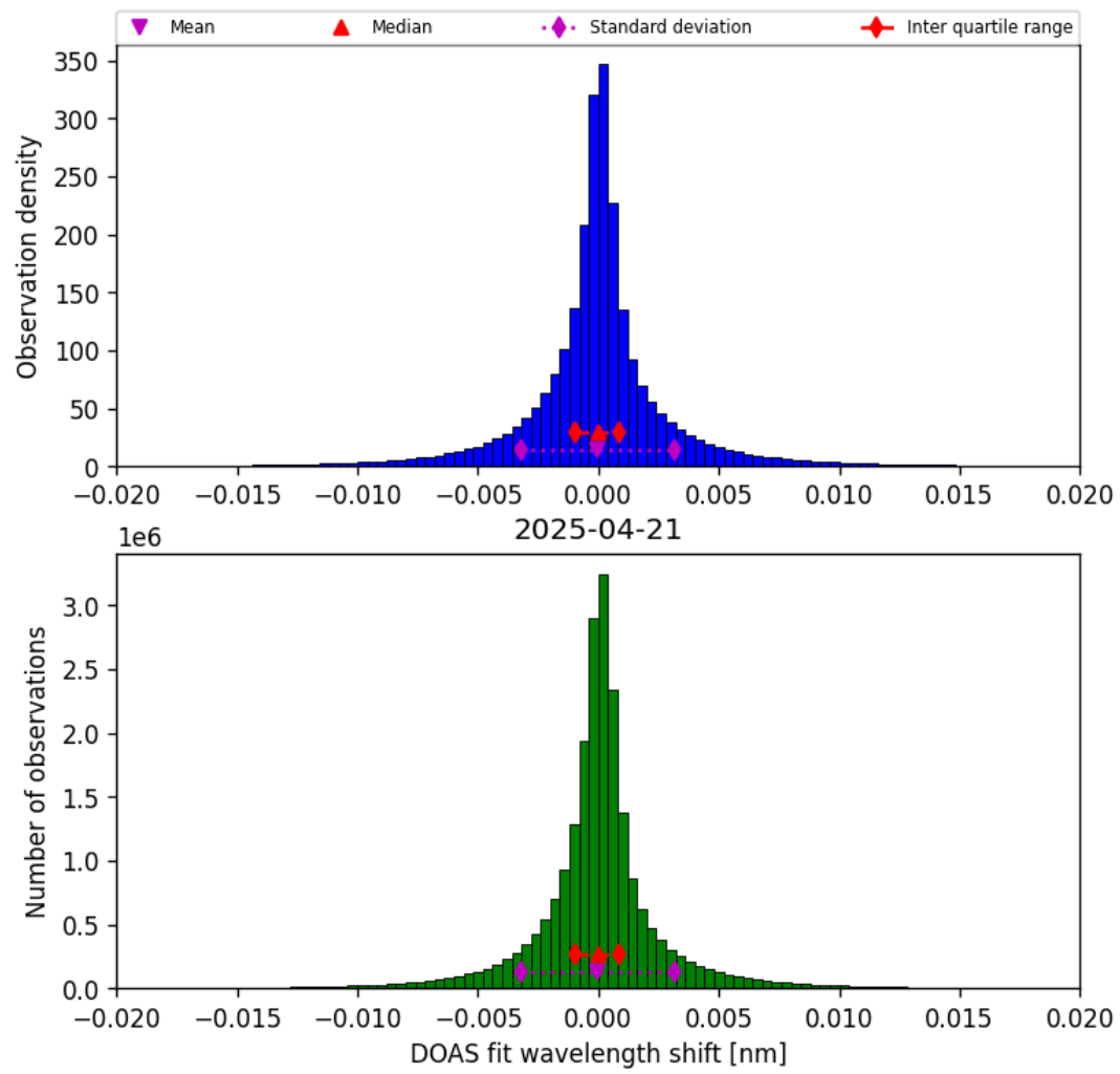
Figure 42: Histogram of “DOAS fit wavelength shift” for 2025-04-21 to 2025-04-22
