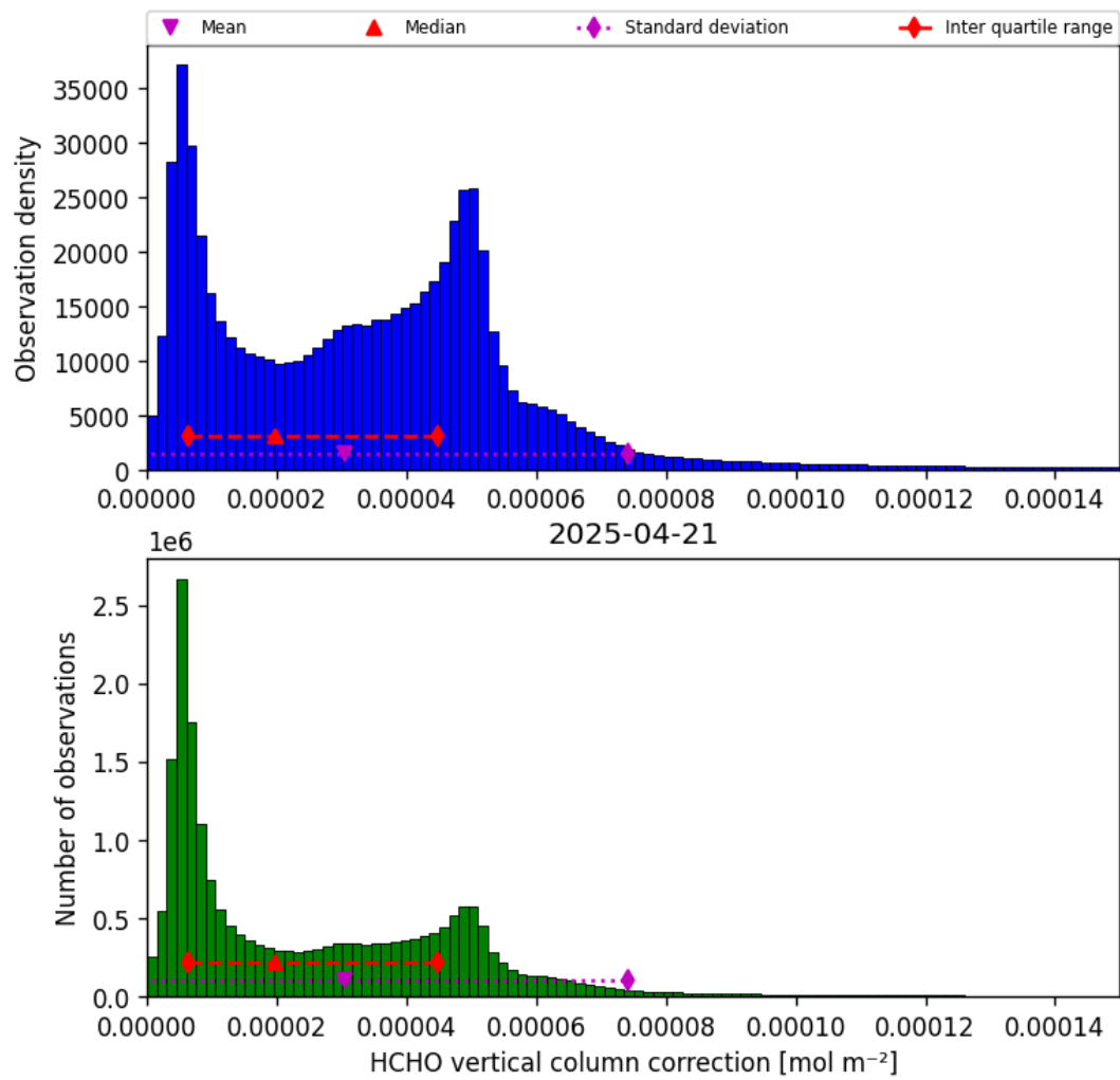
Figure 35: Histogram of “HCHO vertical column correction” for 2025-04-21 to 2025-04-22
