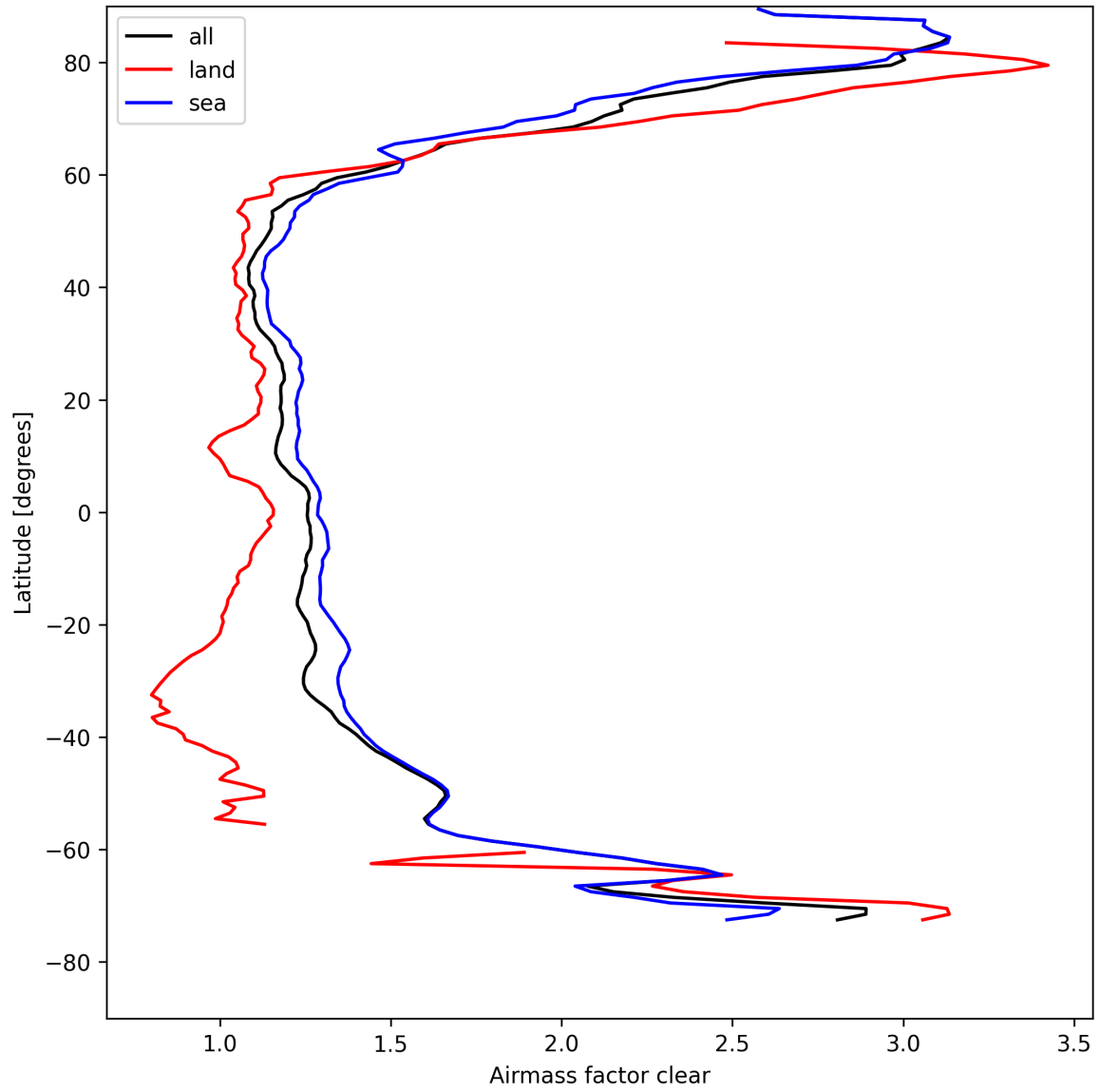
Figure 26: Zonal average of “Airmass factor clear” for 2025-04-21 to 2025-04-22.
