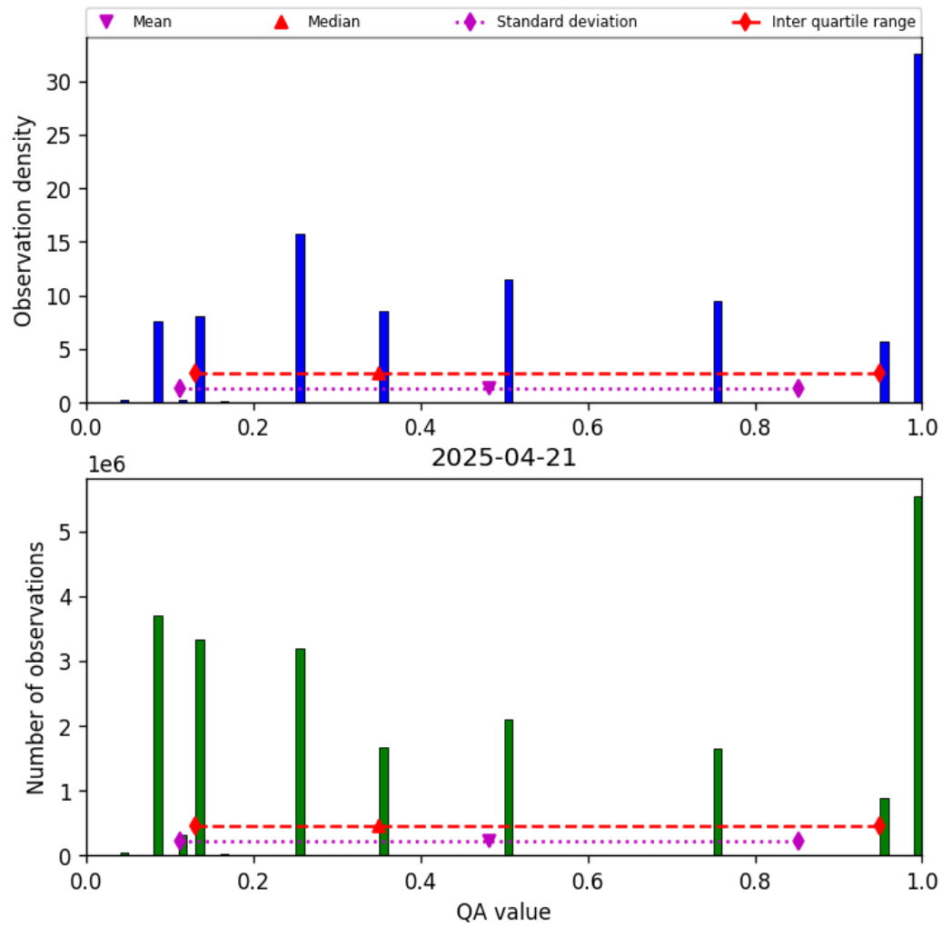
Figure 32: Histogram of “QA value” for 2025-04-21 to 2025-04-22
