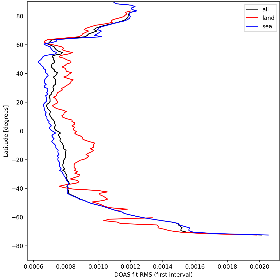
Figure 30: Zonal average of "DOAS fit RMS (first interval)" for 2025-04-21 to 2025-04-22.
