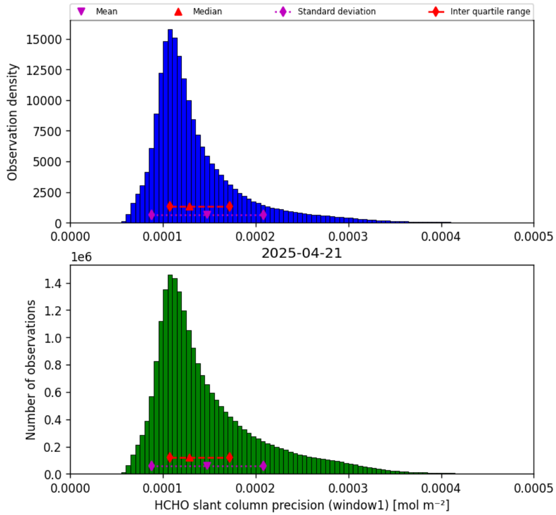
Figure 37: Histogram of “HCHO slant column precision (window1)” for 2025-04-21 to 2025-04-22
