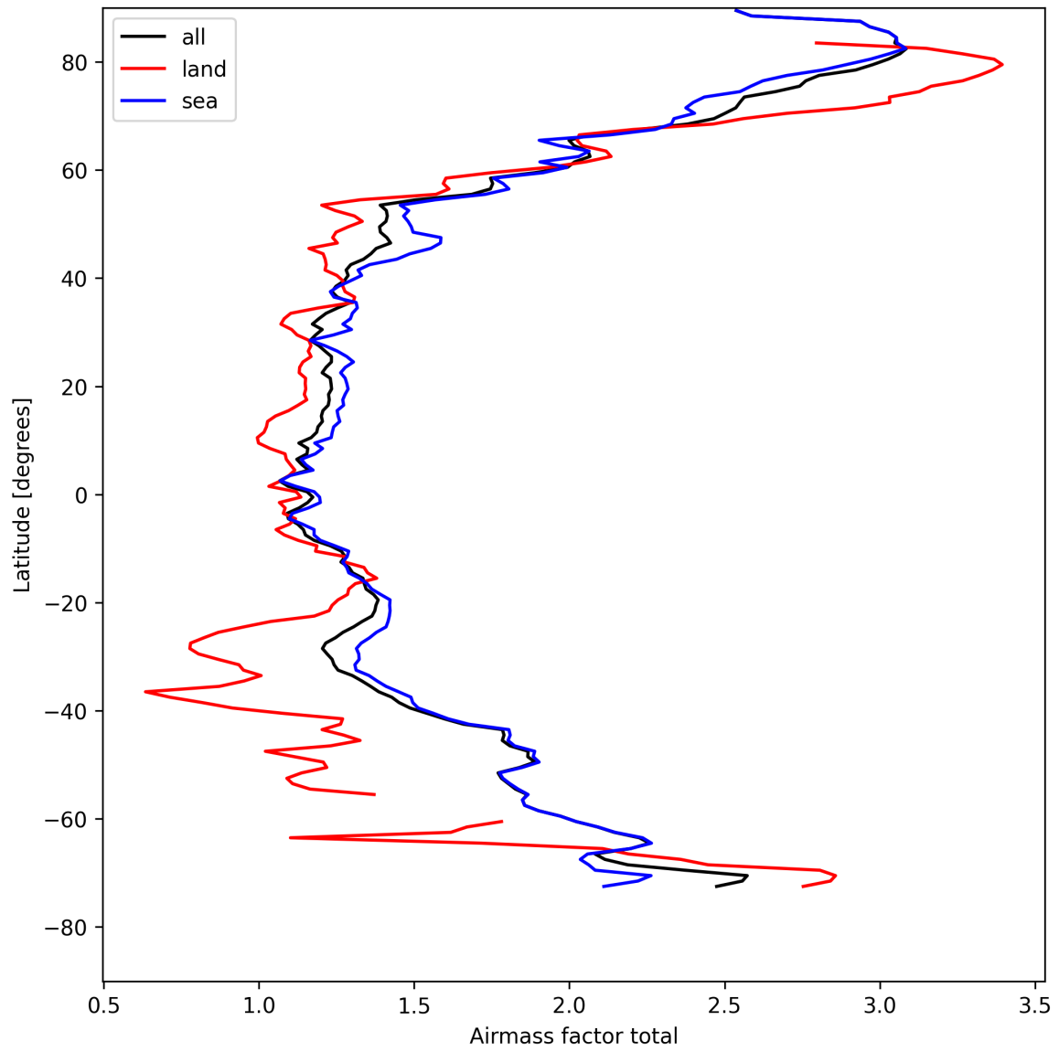
Figure 24: Zonal average of “Airmass factor total” for 2025-04-21 to 2025-04-22.
