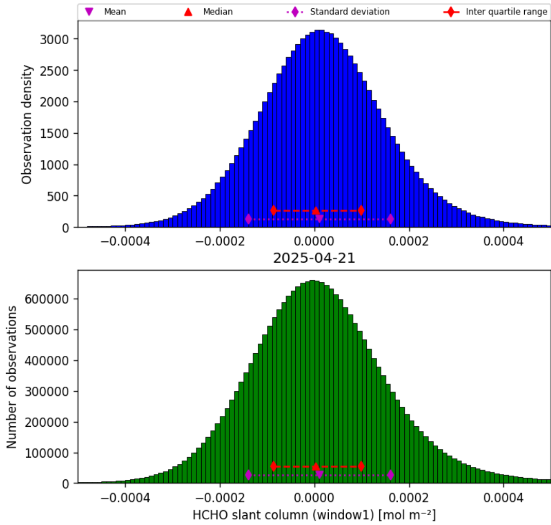
Figure 36: Histogram of “HCHO slant column (window1)” for 2025-04-21 to 2025-04-22
