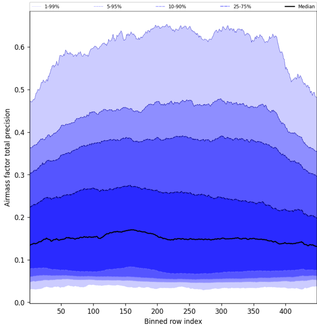
Figure 53: Along track statistics of “Airmass factor total precision” for 2025-04-21 to 2025-04-22
