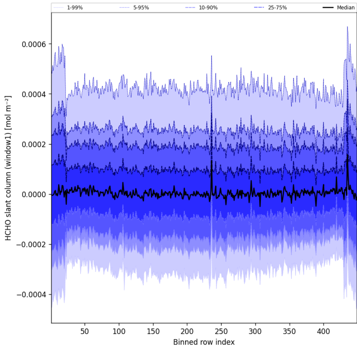
Figure 50: Along track statistics of “HCHO slant column (window1)” for 2025-04-21 to 2025-04-22
