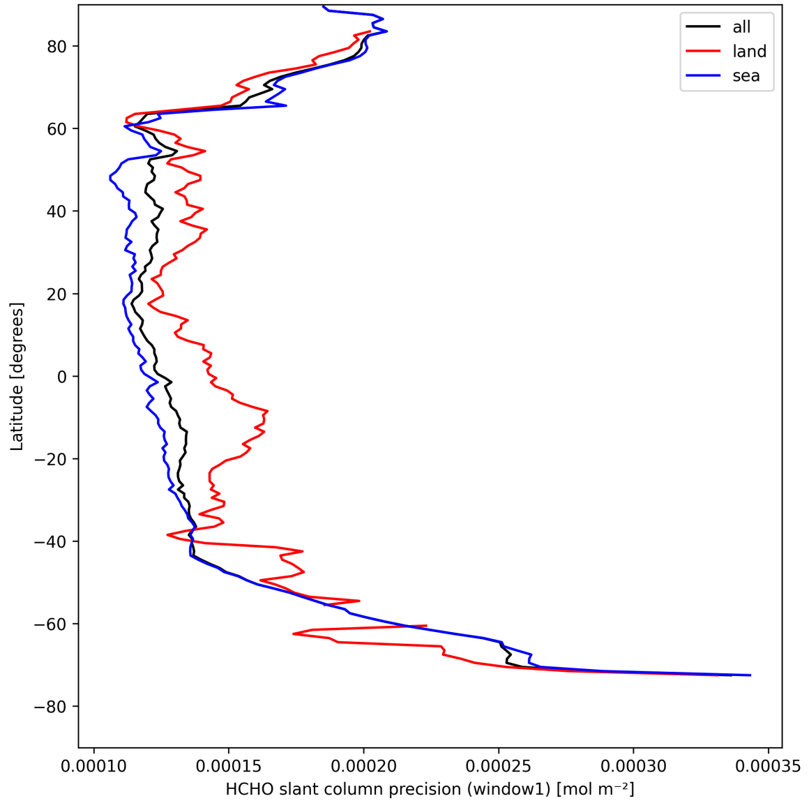
Figure 23: Zonal average of “HCHO slant column precision (window1)” for 2025-04-21 to 2025-04-22.
