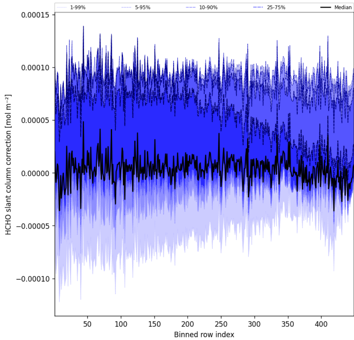
Figure 59: Along track statistics of “HCHO slant column correction” for 2025-04-21 to 2025-04-22
