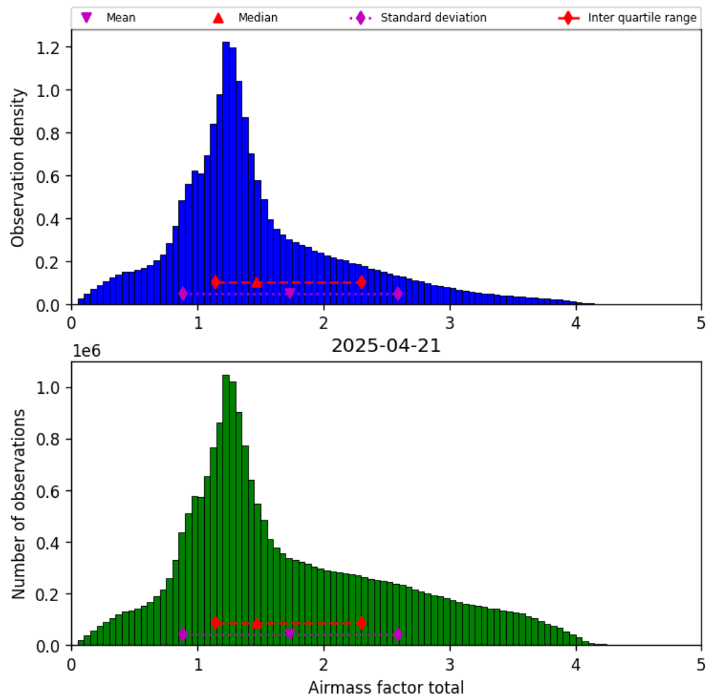
Figure 38: Histogram of “Airmass factor total” for 2025-04-21 to 2025-04-22
