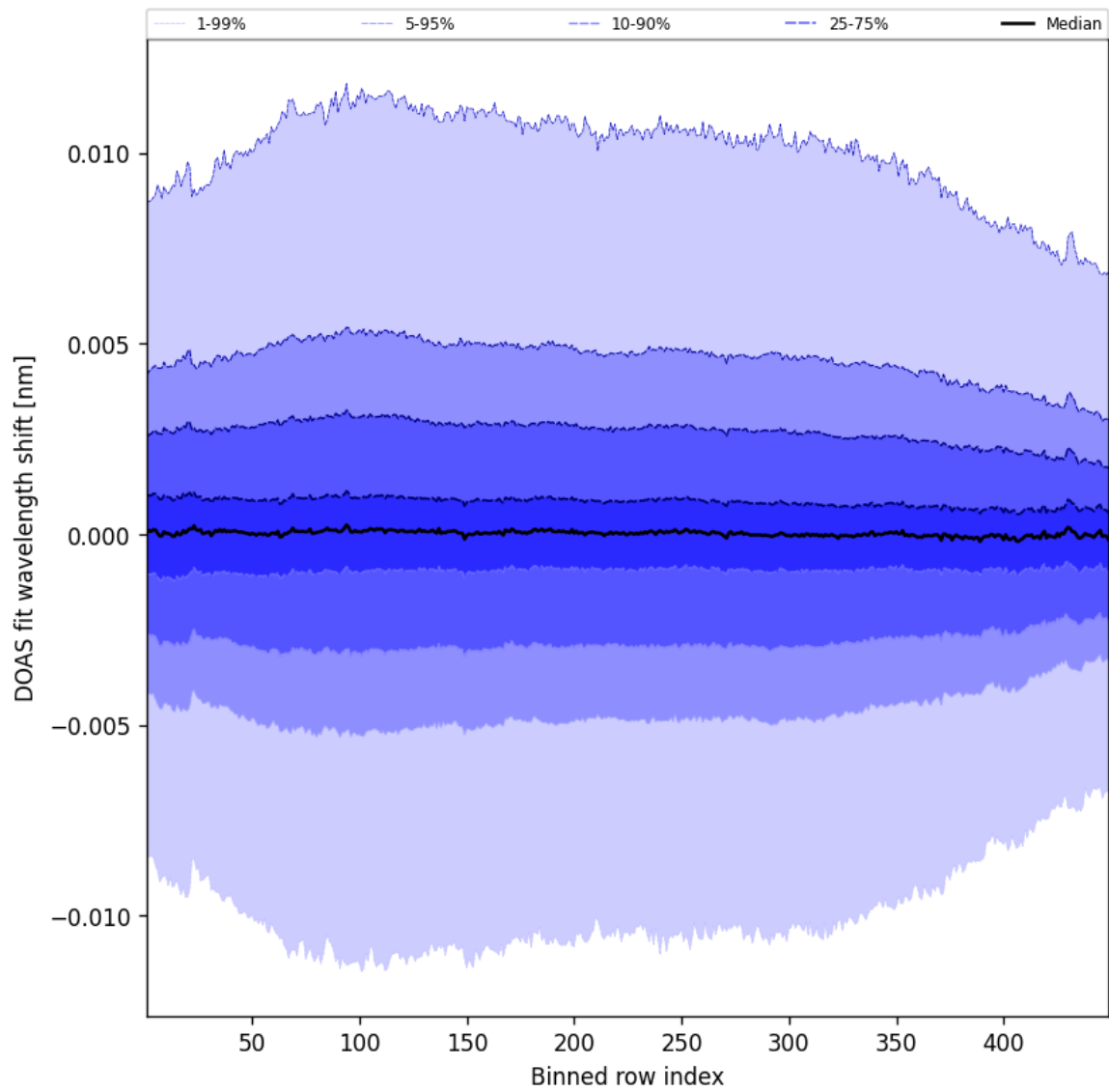
Figure 56: Along track statistics of “DOAS fit wavelength shift” for 2025-04-21 to 2025-04-22
