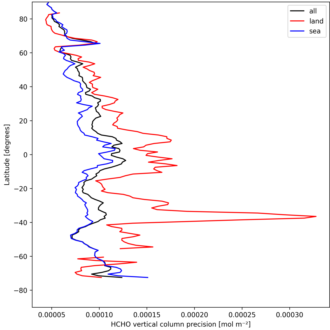
Figure 20: Zonal average of “HCHO vertical column precision” for 2025-04-21 to 2025-04-22.
