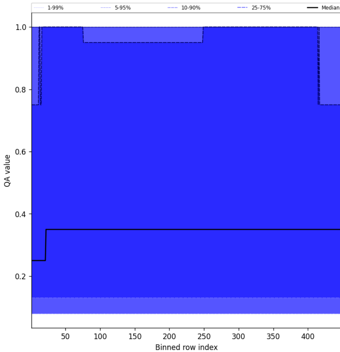
Figure 46: Along track statistics of “QA value” for 2025-04-21 to 2025-04-22
