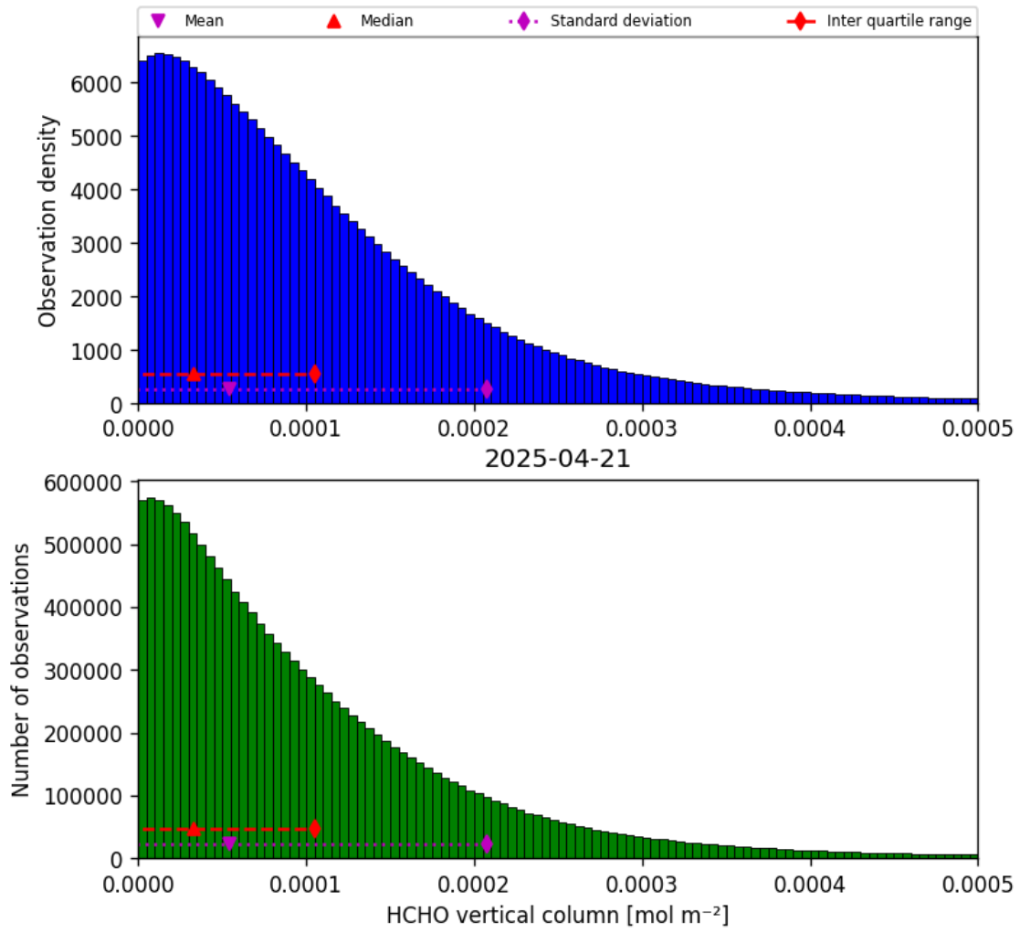
Figure 33: Histogram of “HCHO vertical column” for 2025-04-21 to 2025-04-22
