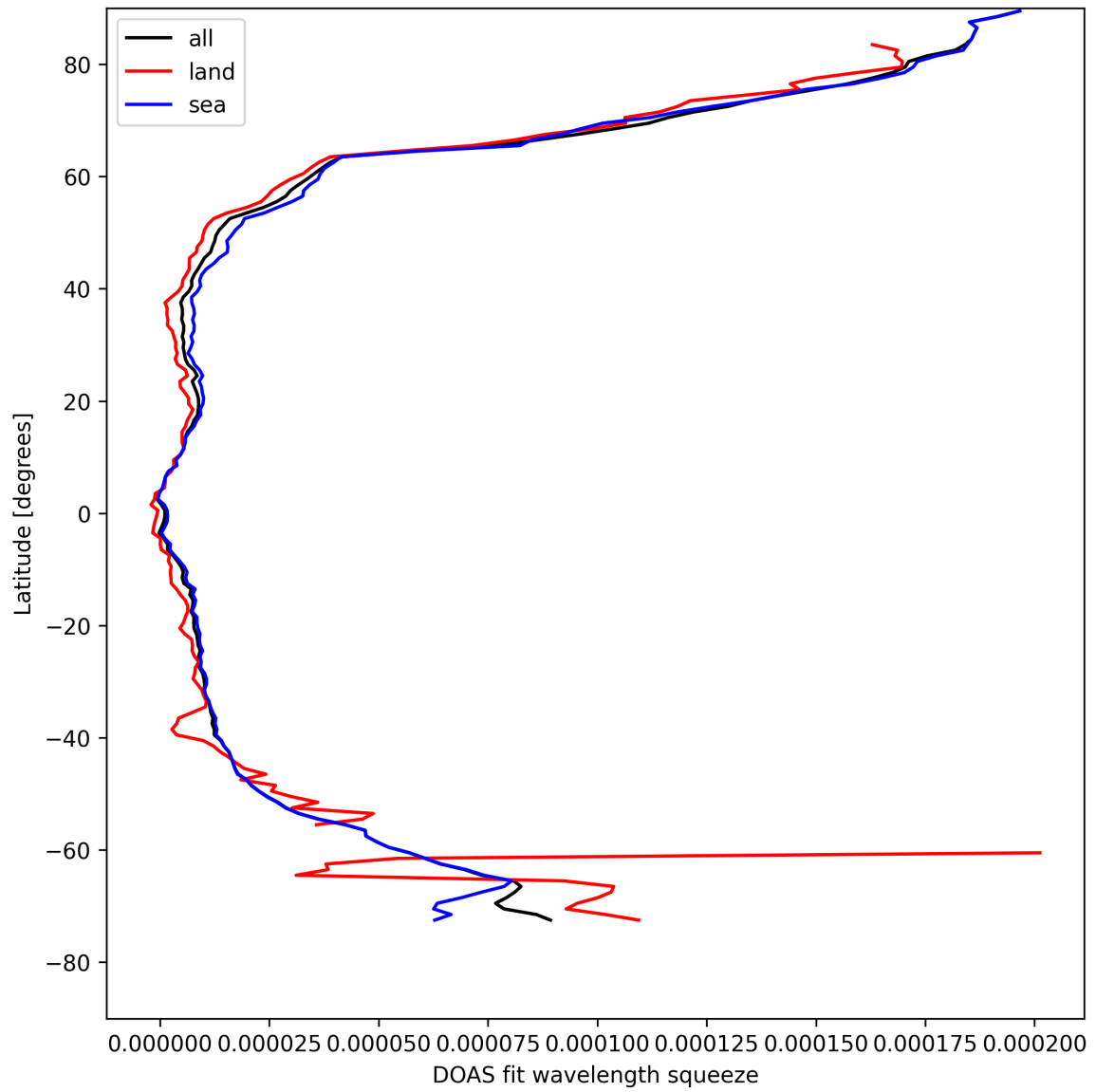
Figure 29: Zonal average of “DOAS fit wavelength squeeze” for 2025-04-21 to 2025-04-22.
