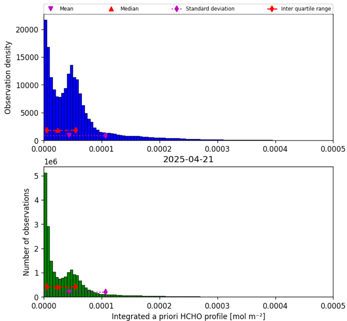
Figure 41: Histogram of “Integrated a priori HCHO profile” for 2025-04-21 to 2025-04-22
