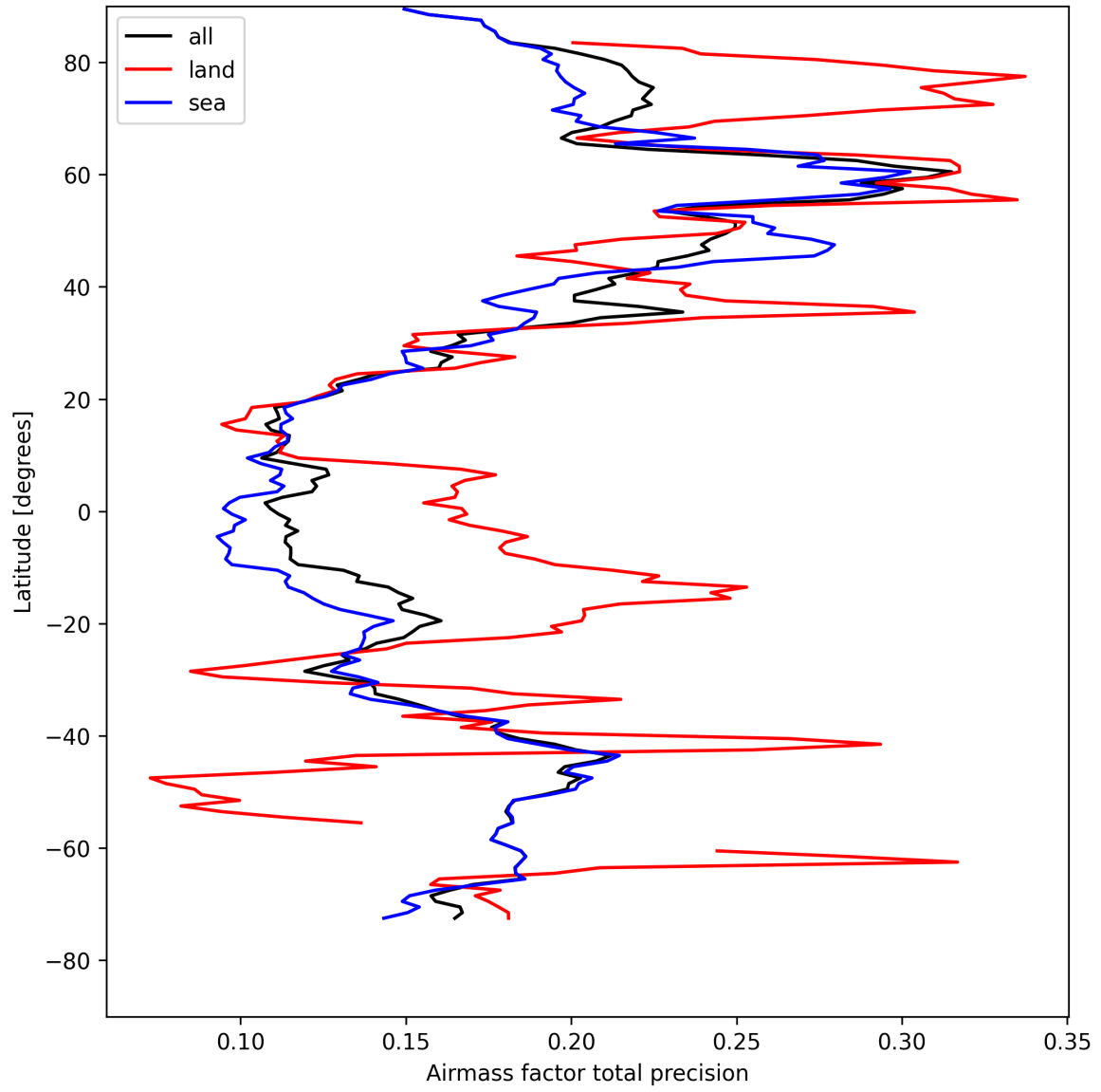
Figure 25: Zonal average of “Airmass factor total precision” for 2025-04-21 to 2025-04-22.
