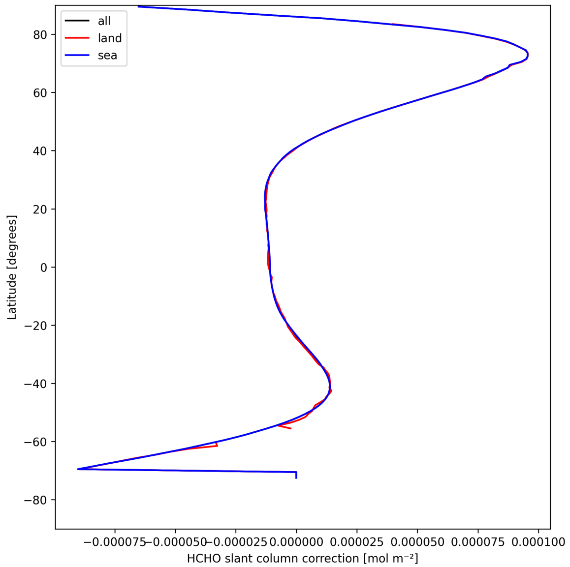
Figure 31: Zonal average of “HCHO slant column correction” for 2025-04-21 to 2025-04-22.
