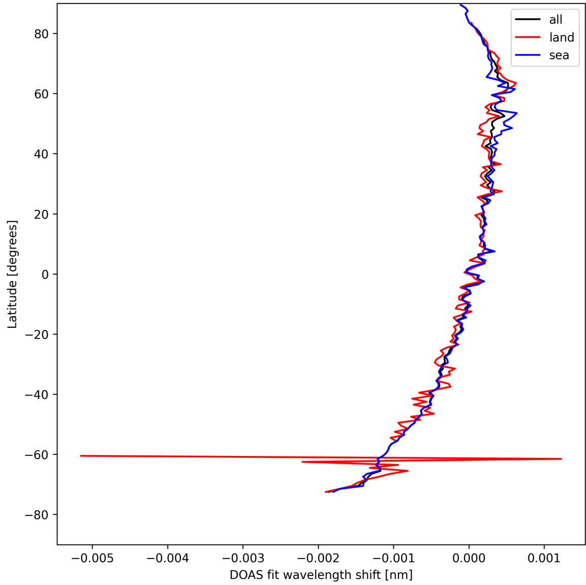
Figure 28: Zonal average of "DOAS fit wavelength shift" for 2025-04-21 to 2025-04-22.
