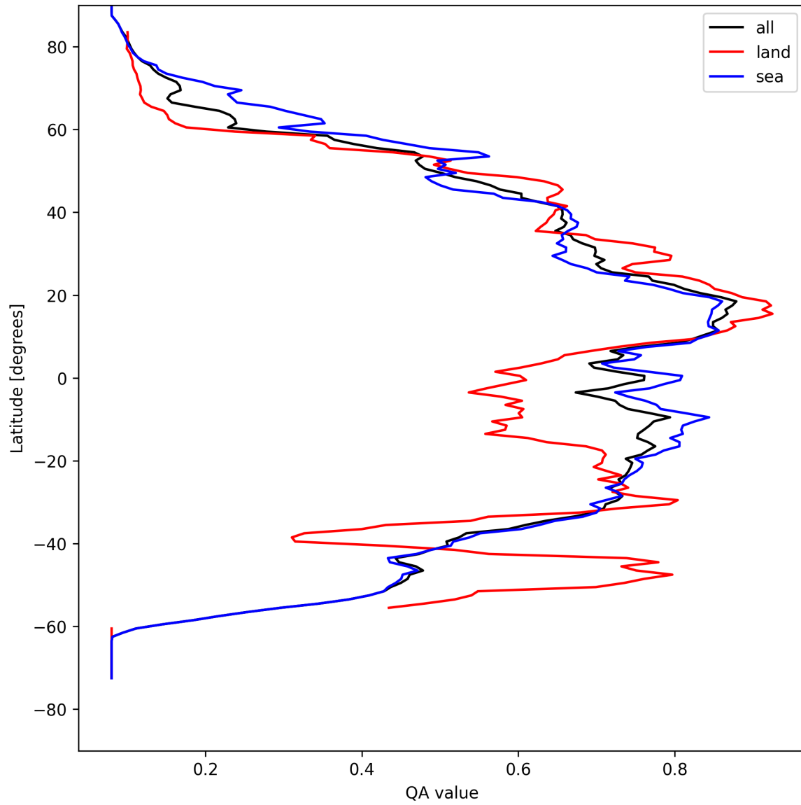
Figure 18: Zonal average of “QA value” for 2025-04-21 to 2025-04-22.
