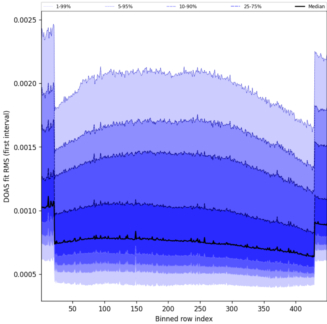
Figure 58: Along track statistics of “DOAS fit RMS (first interval)” for 2025-04-21 to 2025-04-22
