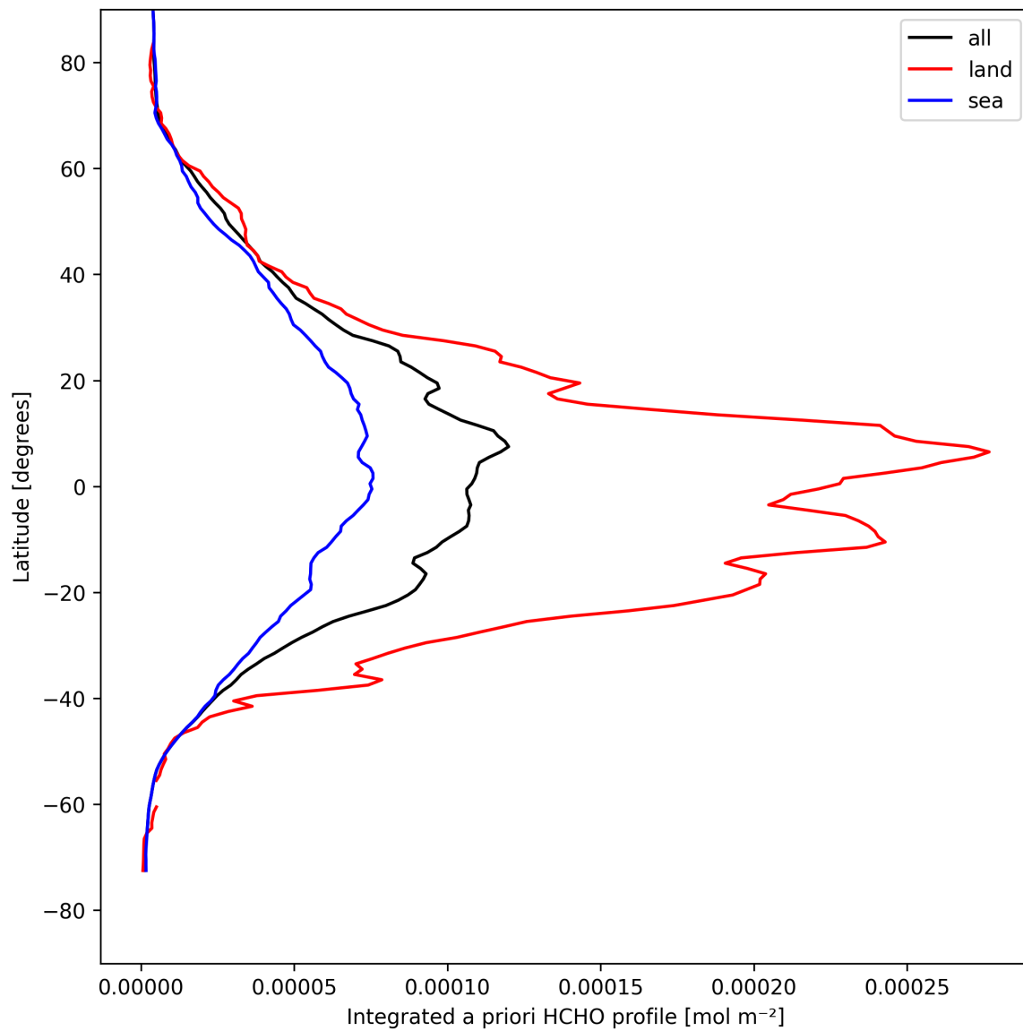
Figure 27: Zonal average of “Integrated a priori HCHO profile” for 2025-04-21 to 2025-04-22.
