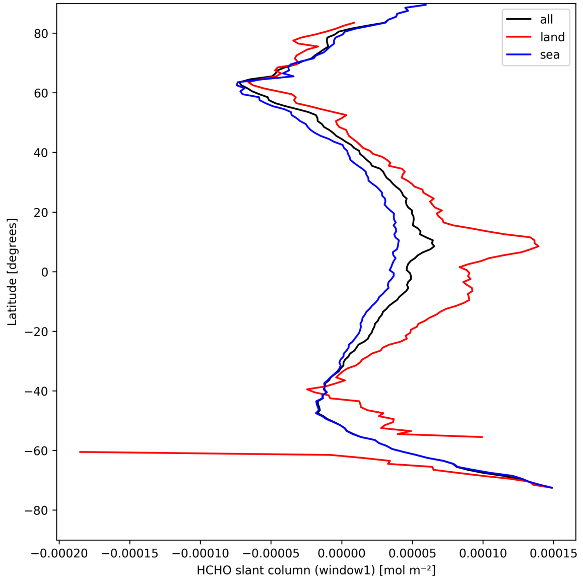
Figure 22: Zonal average of “HCHO slant column (window1)” for 2025-04-21 to 2025-04-22.
