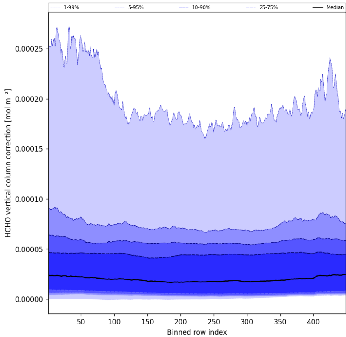
Figure 49: Along track statistics of “HCHO vertical column correction” for 2025-04-21 to 2025-04-22
