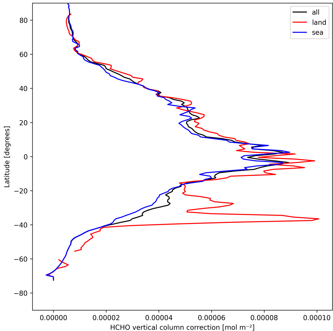
Figure 21: Zonal average of “HCHO vertical column correction” for 2025-04-21 to 2025-04-22.
