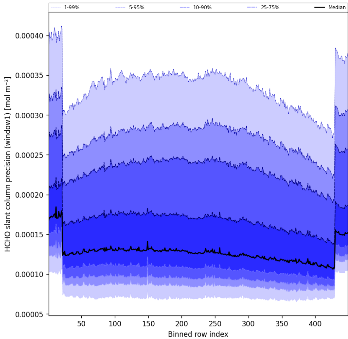
Figure 51: Along track statistics of “HCHO slant column precision (window1)” for 2025-04-21 to 2025-04-22
