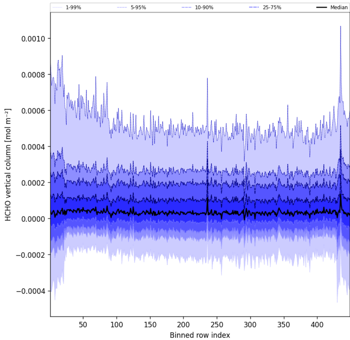
Figure 47: Along track statistics of “HCHO vertical column” for 2025-04-21 to 2025-04-22
