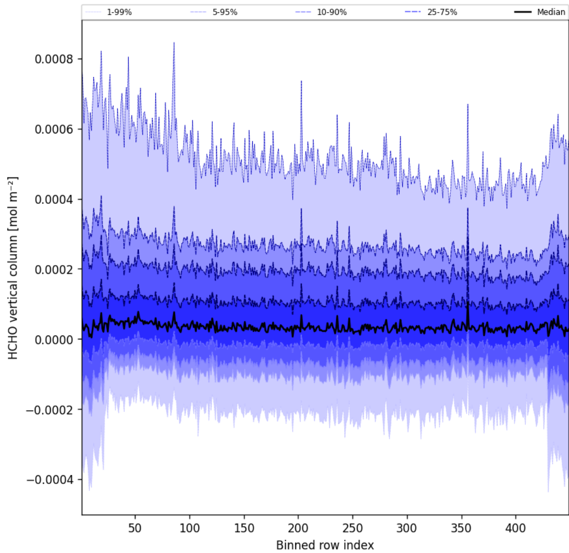
Figure 47: Along track statistics of “HCHO vertical column” for 2025-04-22 to 2025-04-22
