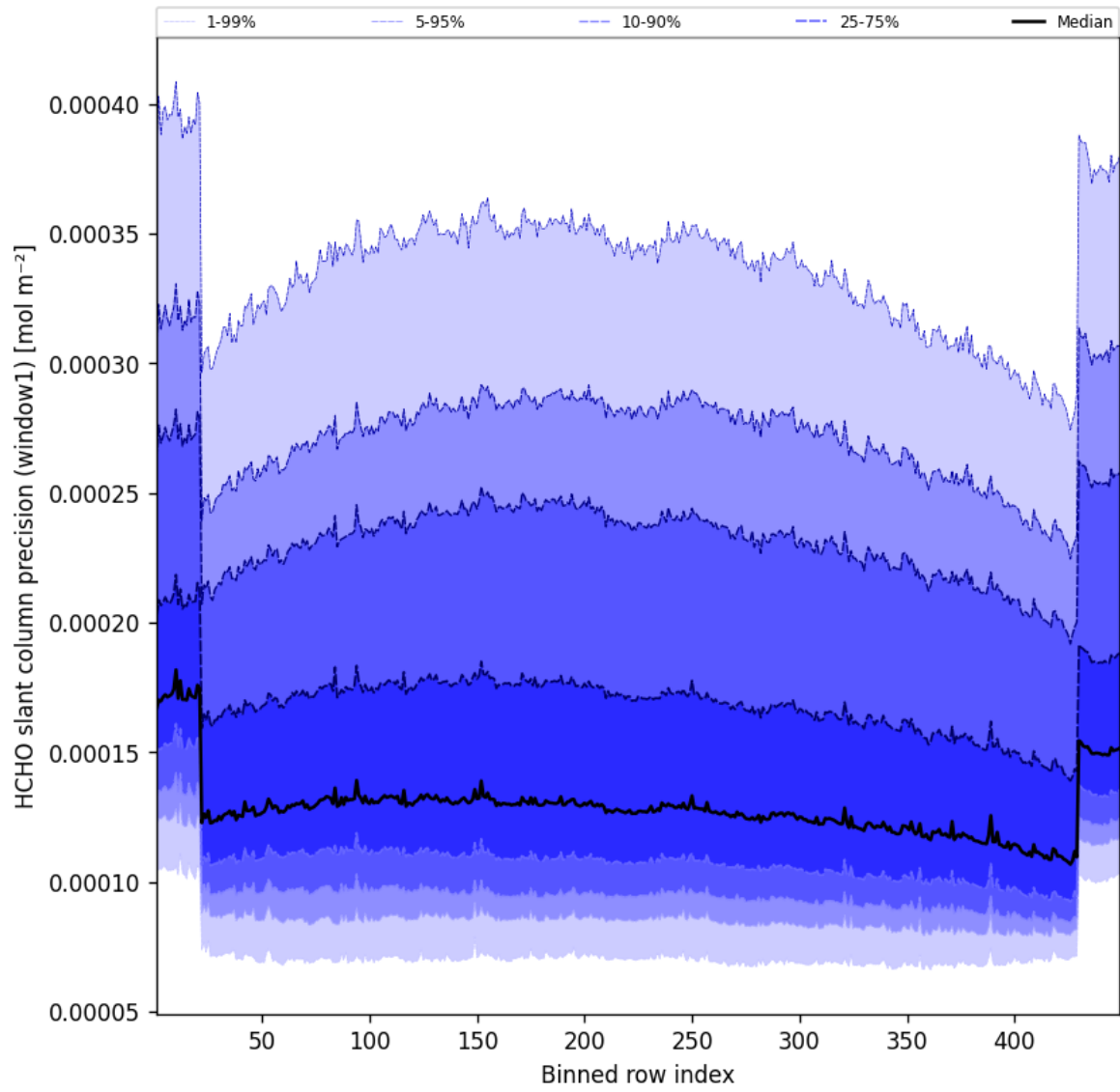
Figure 51: Along track statistics of “HCHO slant column precision (window1)” for 2025-04-22 to 2025-04-22
