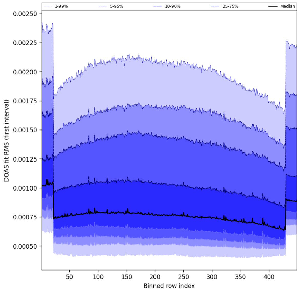
Figure 58: Along track statistics of “DOAS fit RMS (first interval)” for 2025-04-22 to 2025-04-22
