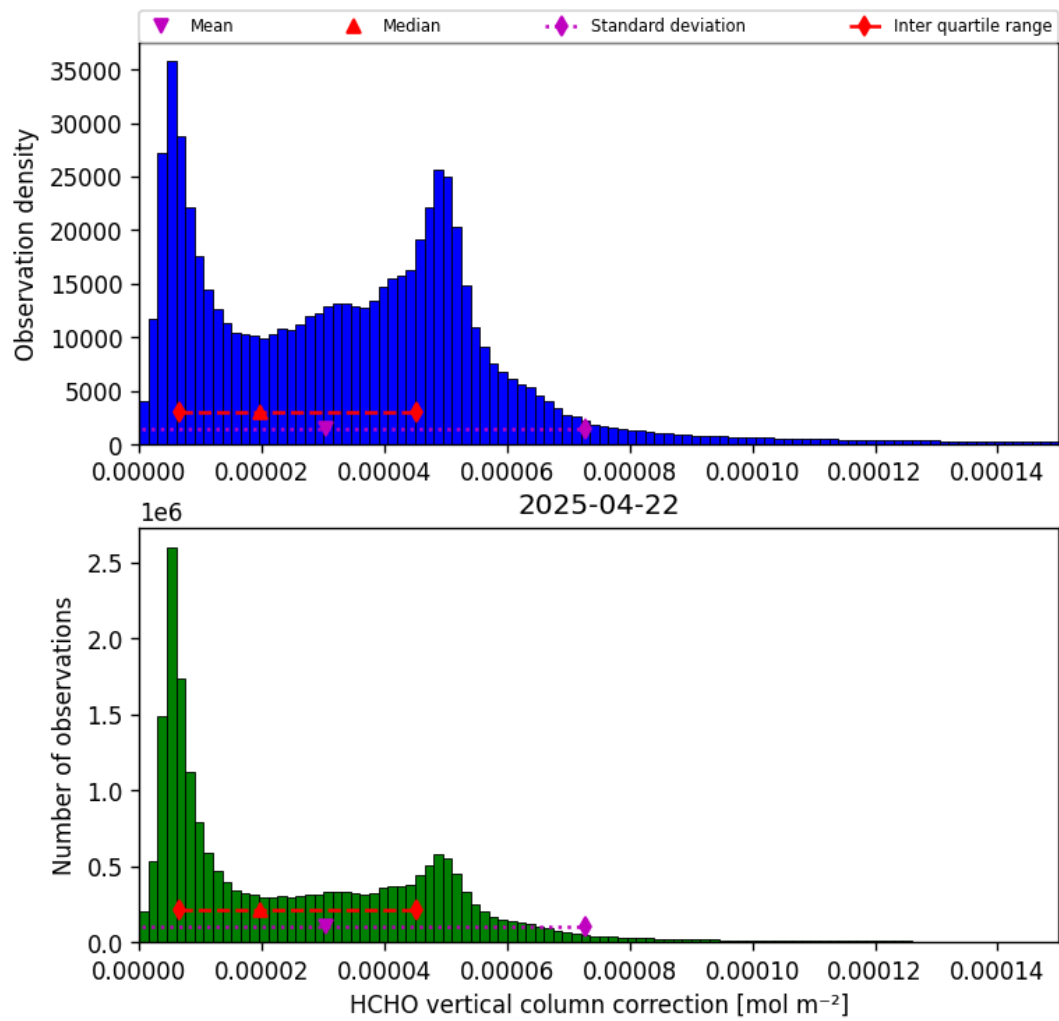
Figure 35: Histogram of “HCHO vertical column correction” for 2025-04-22 to 2025-04-22
