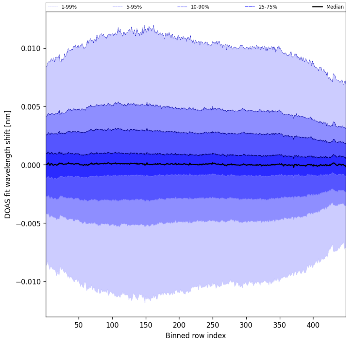
Figure 56: Along track statistics of “DOAS fit wavelength shift” for 2025-04-22 to 2025-04-22
