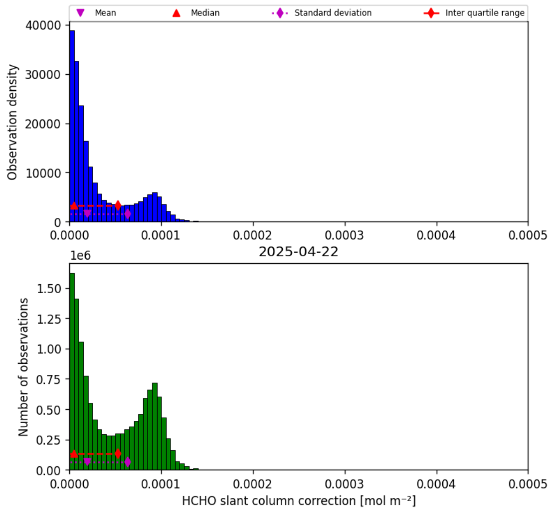
Figure 45: Histogram of “HCHO slant column correction” for 2025-04-22 to 2025-04-22
