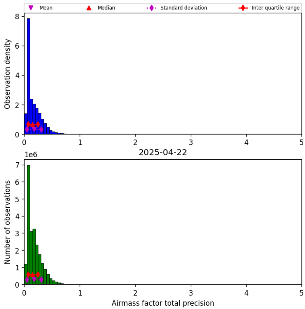
Figure 39: Histogram of “Airmass factor total precision” for 2025-04-22 to 2025-04-22
