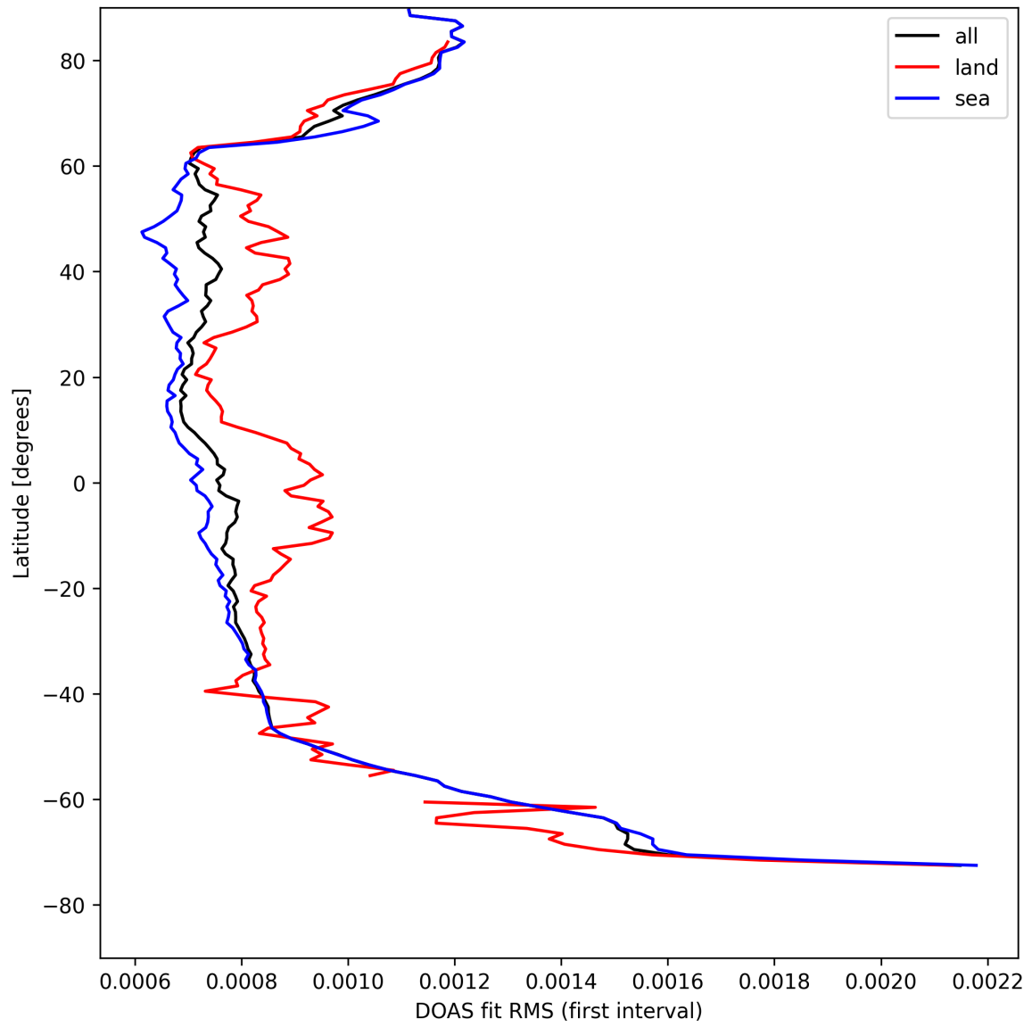
Figure 30: Zonal average of “DOAS fit RMS (first interval)” for 2025-04-22 to 2025-04-22.
