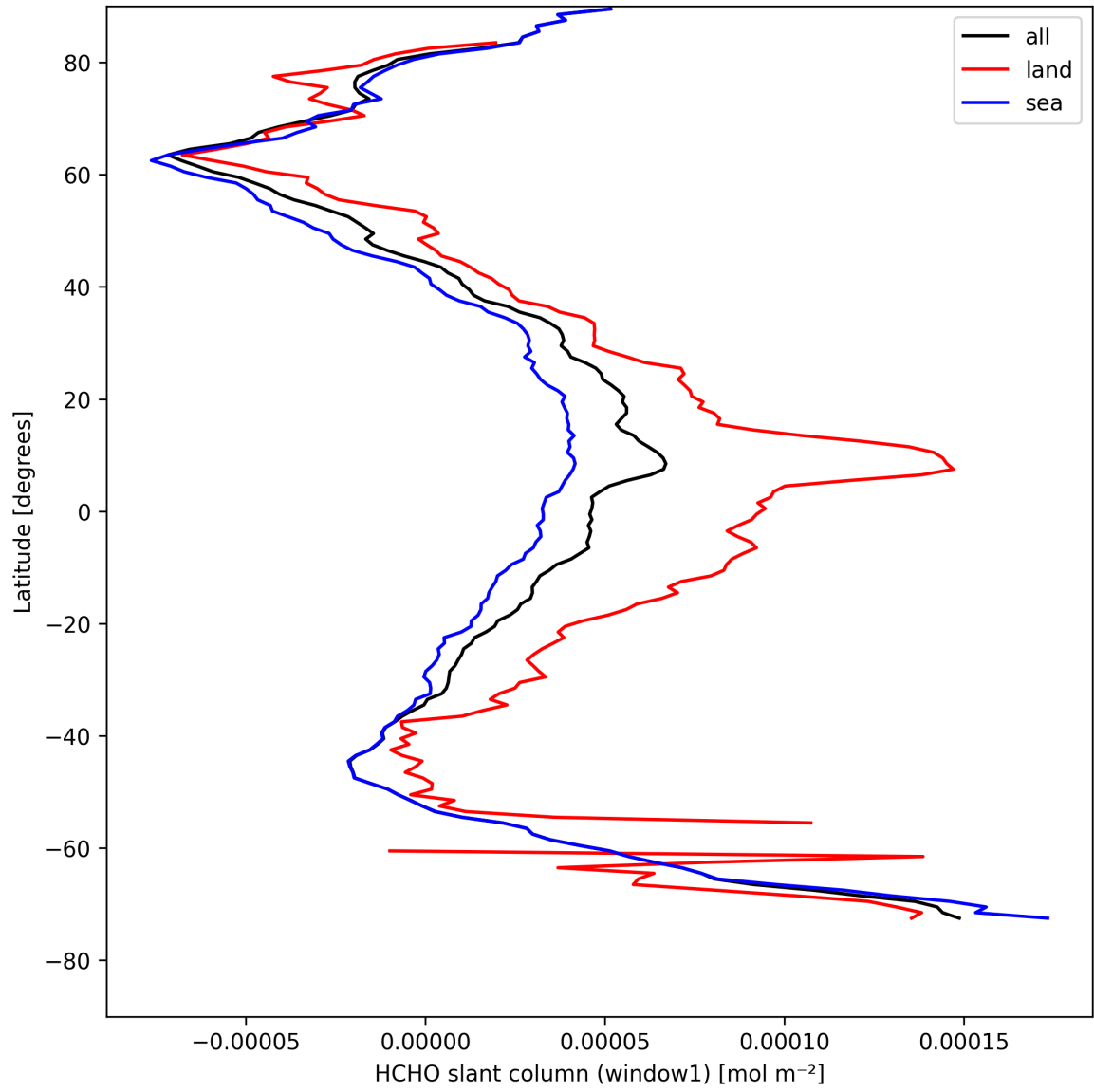
Figure 22: Zonal average of “HCHO slant column (window1)” for 2025-04-22 to 2025-04-22.
