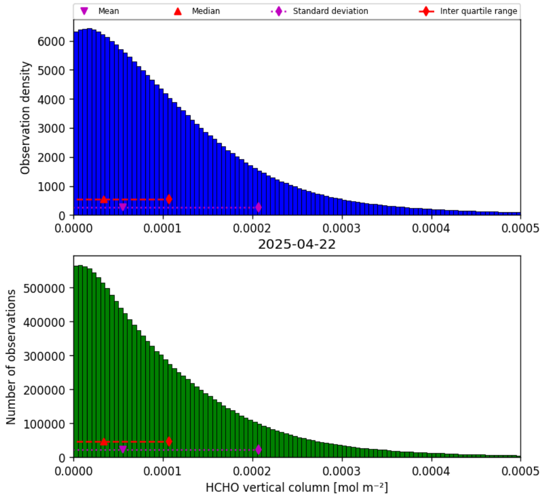
Figure 33: Histogram of “HCHO vertical column” for 2025-04-22 to 2025-04-22
