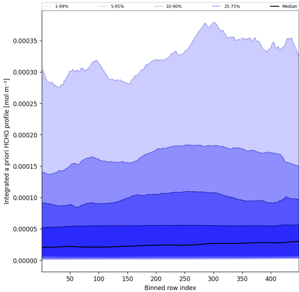
Figure 55: Along track statistics of “Integrated a priori HCHO profile” for 2025-04-22 to 2025-04-22
