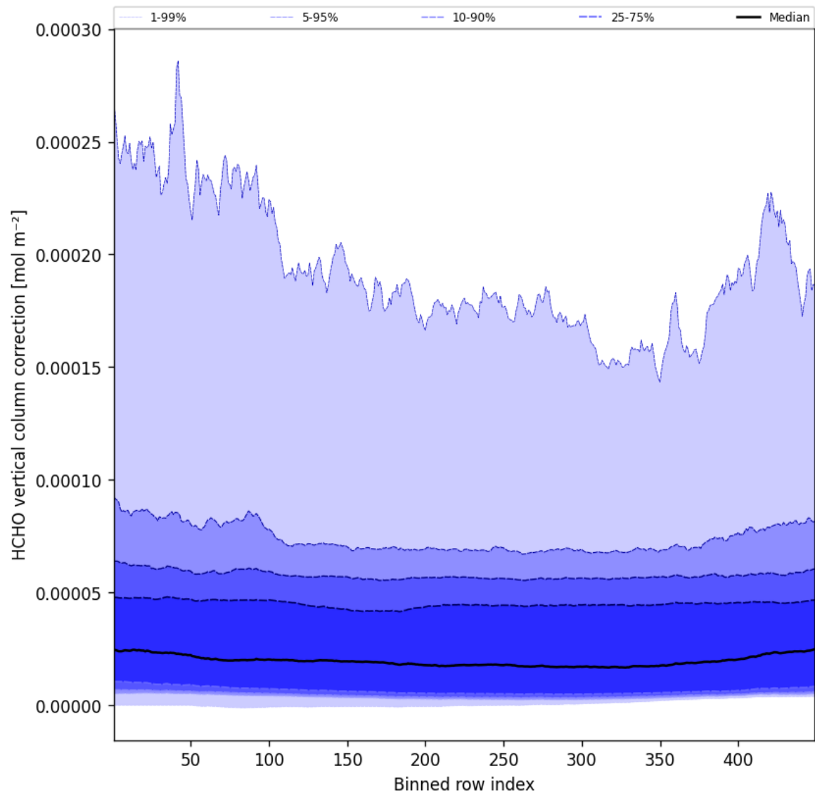
Figure 49: Along track statistics of “HCHO vertical column correction” for 2025-04-22 to 2025-04-22
