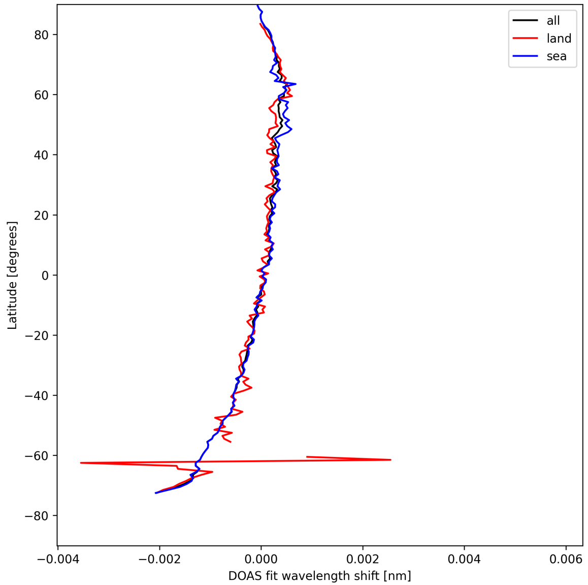
Figure 28: Zonal average of “DOAS fit wavelength shift” for 2025-04-22 to 2025-04-22.
