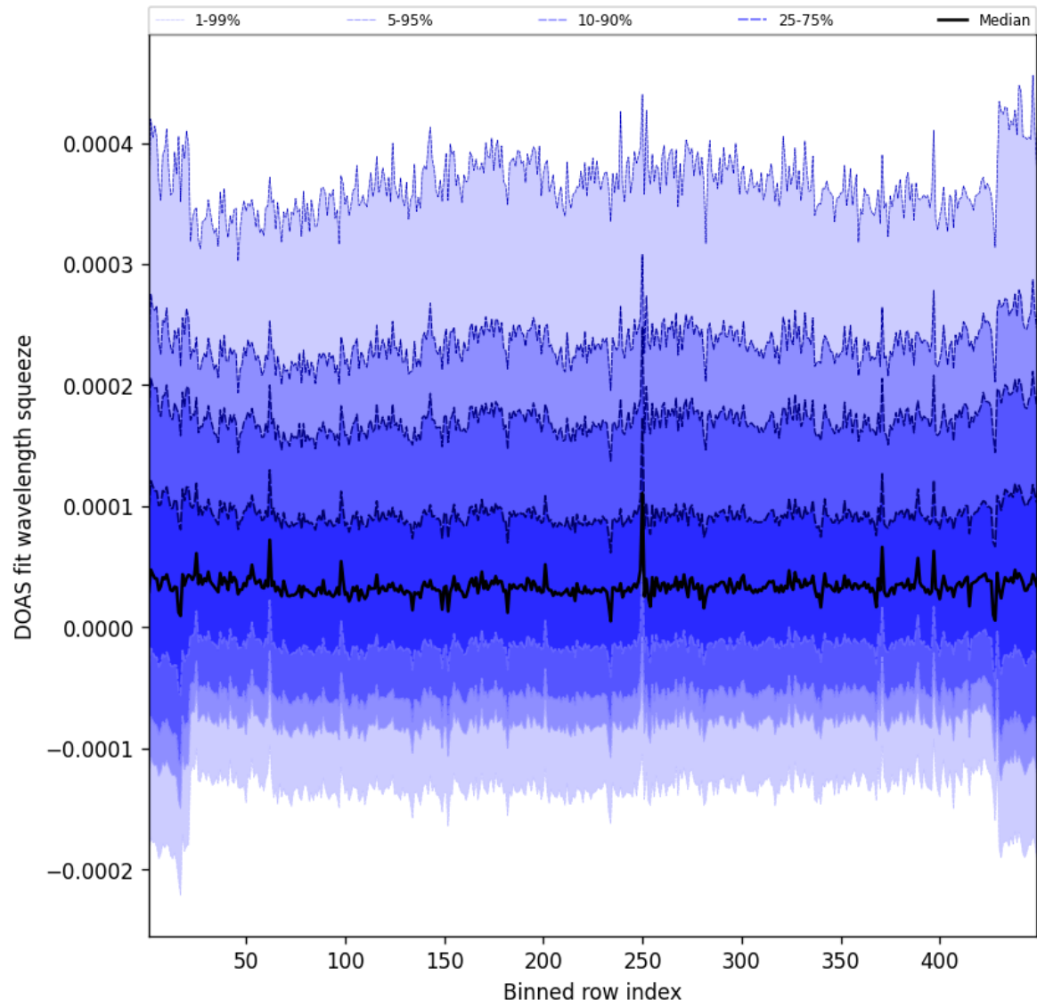
Figure 57: Along track statistics of “DOAS fit wavelength squeeze” for 2025-04-22 to 2025-04-22
