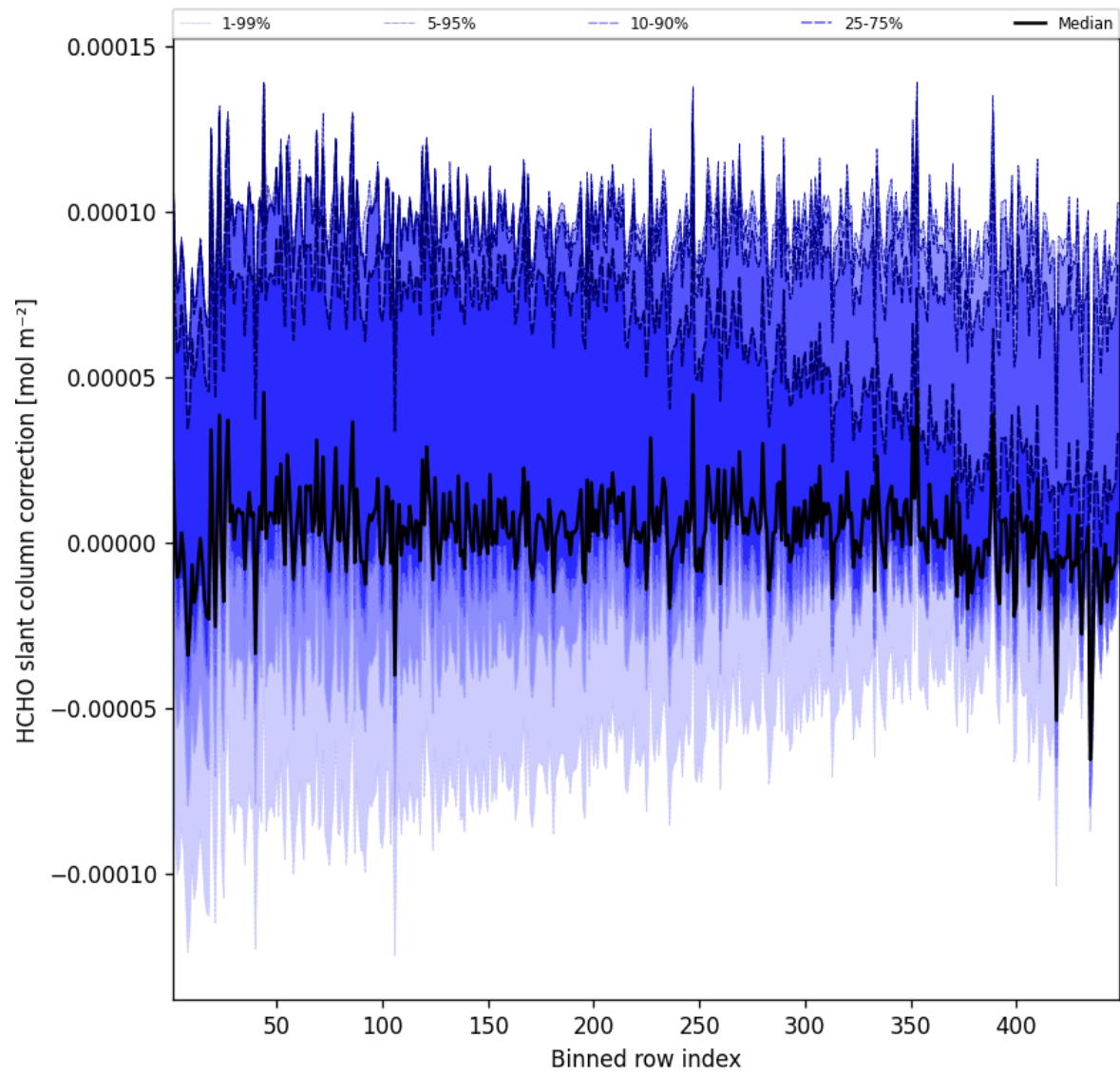
Figure 59: Along track statistics of “HCHO slant column correction” for 2025-04-22 to 2025-04-22
