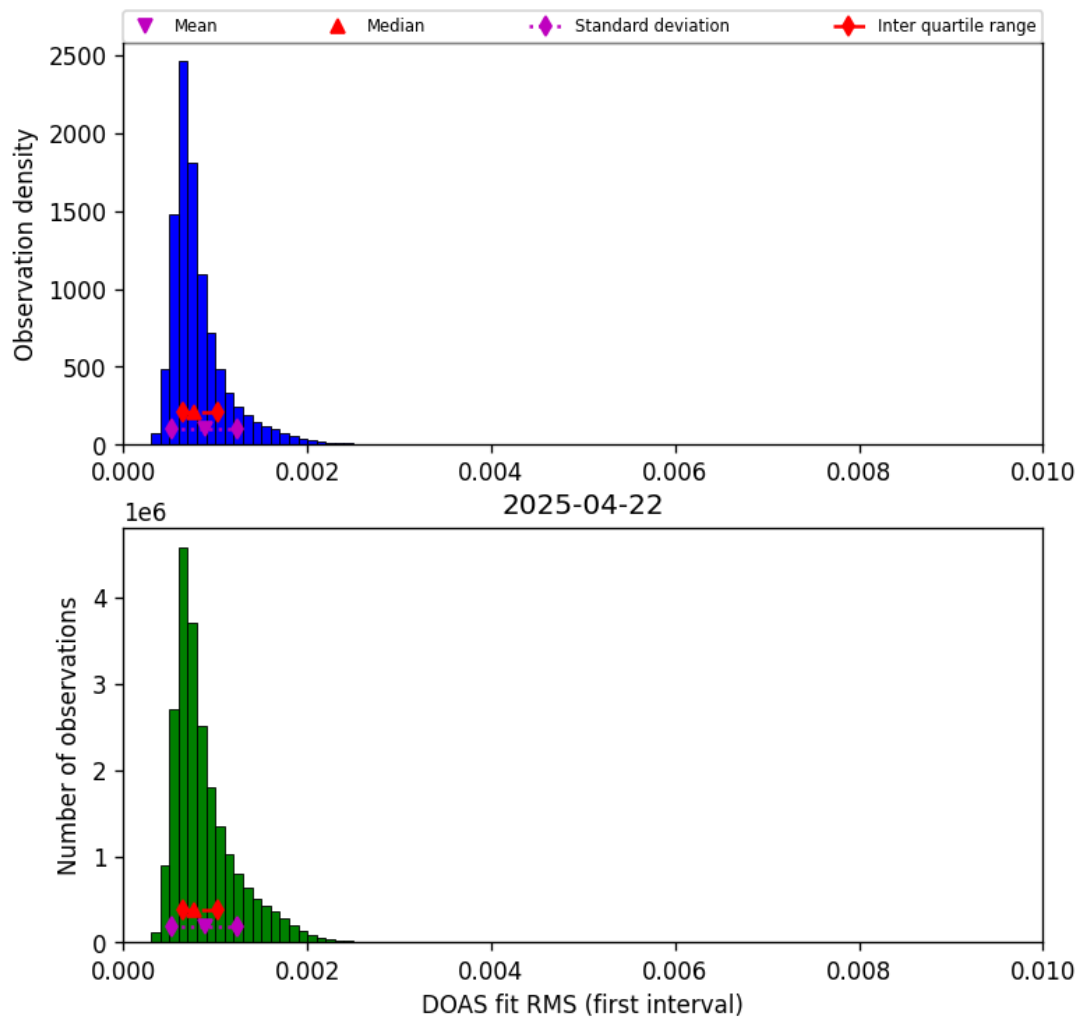
Figure 44: Histogram of “DOAS fit RMS (first interval)” for 2025-04-22 to 2025-04-22
