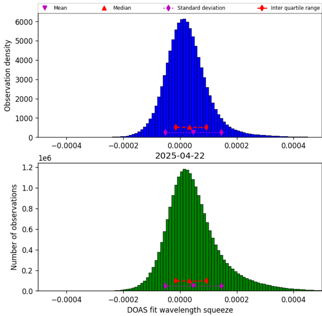
Figure 43: Histogram of “DOAS fit wavelength squeeze” for 2025-04-22 to 2025-04-22
