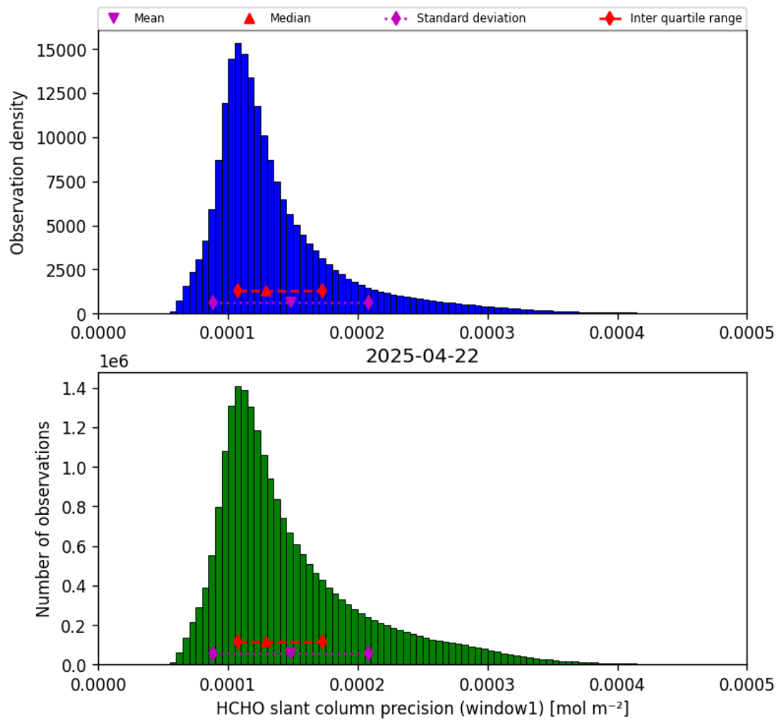
Figure 37: Histogram of “HCHO slant column precision (window1)” for 2025-04-22 to 2025-04-22
