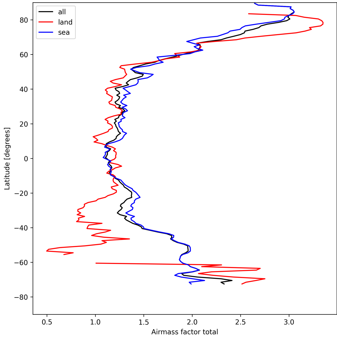
Figure 24: Zonal average of “Airmass factor total” for 2025-04-22 to 2025-04-22.
