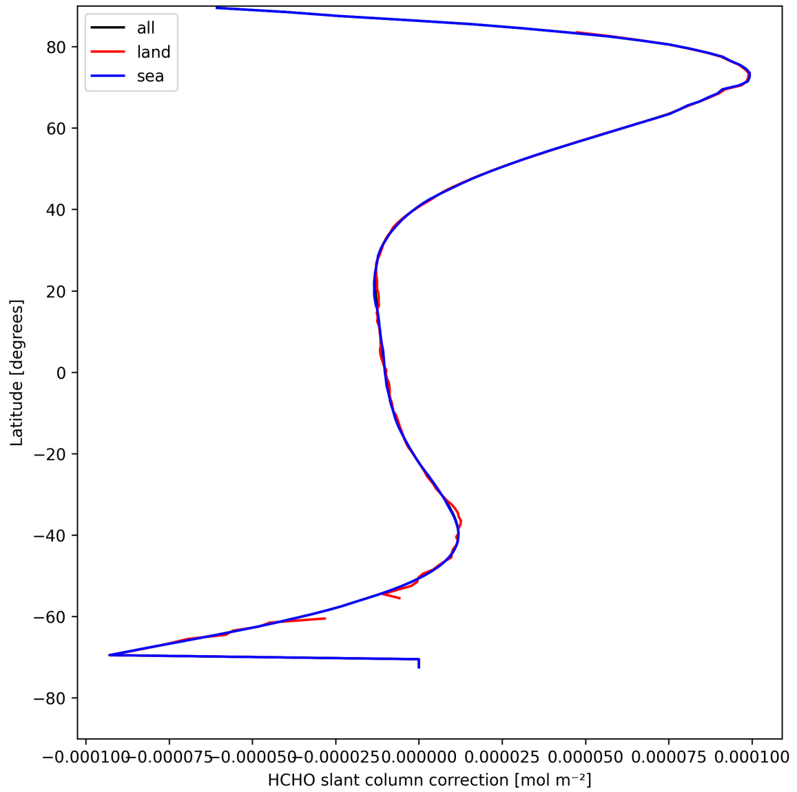
Figure 31: Zonal average of “HCHO slant column correction” for 2025-04-22 to 2025-04-22.
