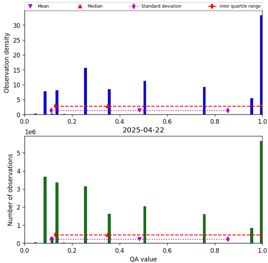
Figure 32: Histogram of “QA value” for 2025-04-22 to 2025-04-22
