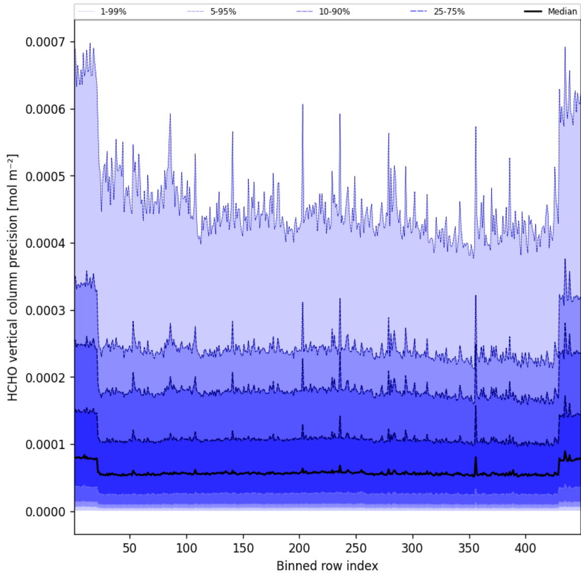
Figure 48: Along track statistics of “HCHO vertical column precision” for 2025-04-22 to 2025-04-22
