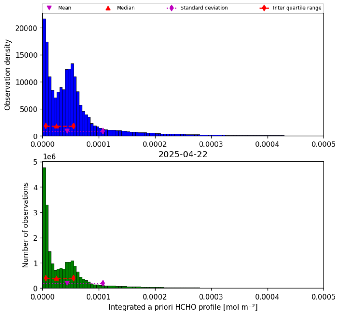
Figure 41: Histogram of “Integrated a priori HCHO profile” for 2025-04-22 to 2025-04-22
