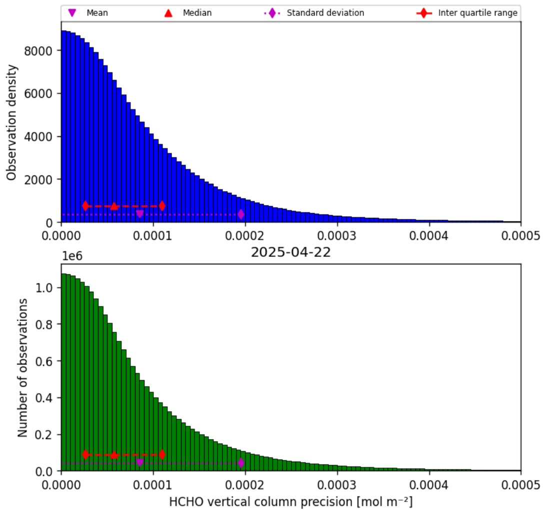
Figure 34: Histogram of “HCHO vertical column precision” for 2025-04-22 to 2025-04-22
