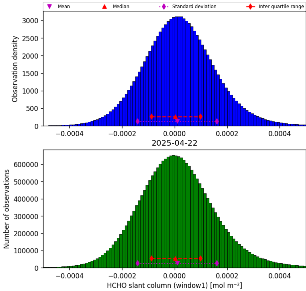
Figure 36: Histogram of “HCHO slant column (window1)” for 2025-04-22 to 2025-04-22
