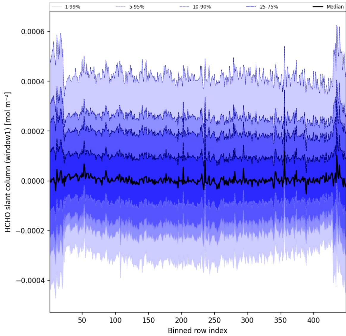
Figure 50: Along track statistics of “HCHO slant column (window1)” for 2025-04-22 to 2025-04-22
