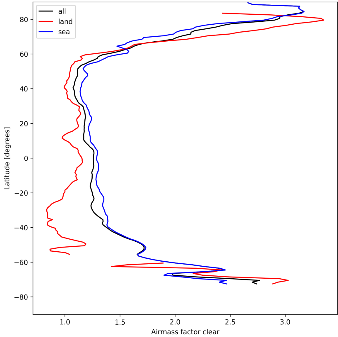
Figure 26: Zonal average of “Airmass factor clear” for 2025-04-22 to 2025-04-22.
