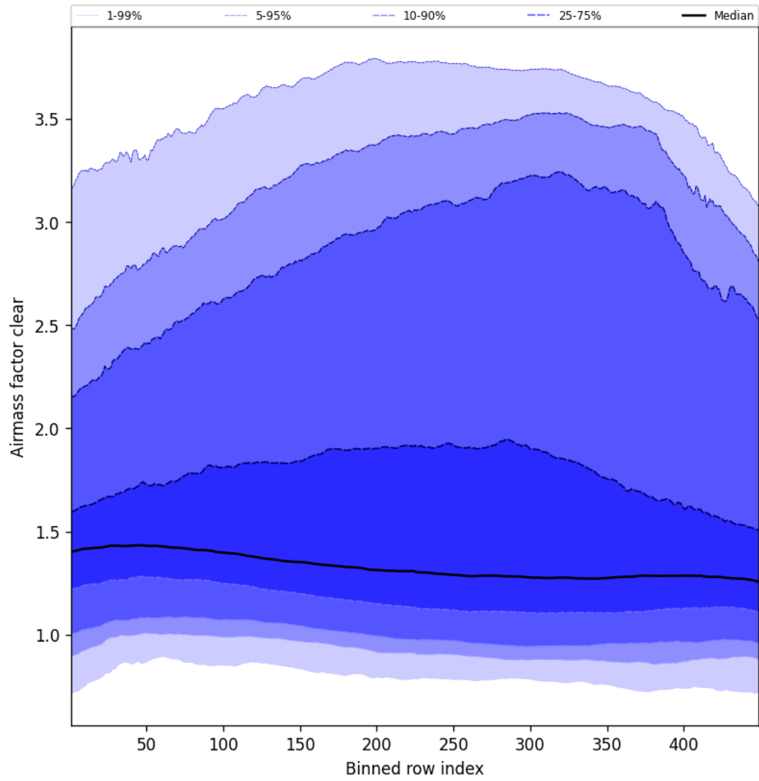
Figure 54: Along track statistics of “Airmass factor clear” for 2025-04-22 to 2025-04-22
