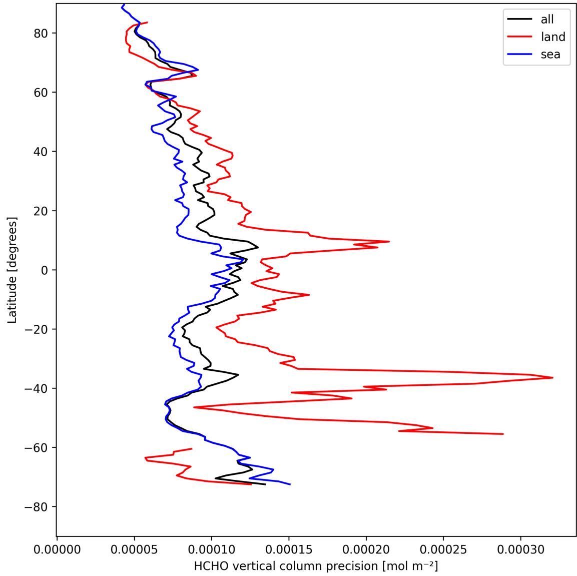
Figure 20: Zonal average of “HCHO vertical column precision” for 2025-04-22 to 2025-04-22.
