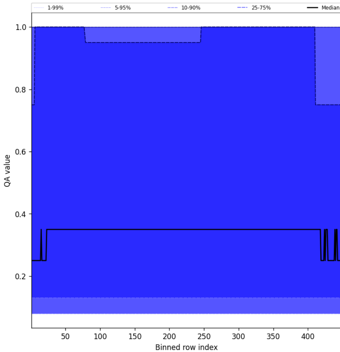
Figure 46: Along track statistics of “QA value” for 2025-04-22 to 2025-04-22
