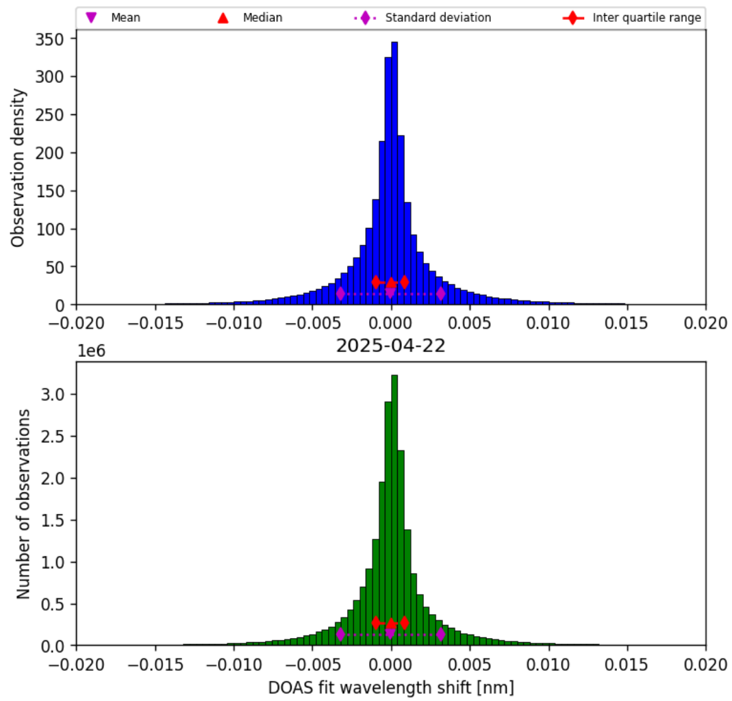
Figure 42: Histogram of “DOAS fit wavelength shift” for 2025-04-22 to 2025-04-22
