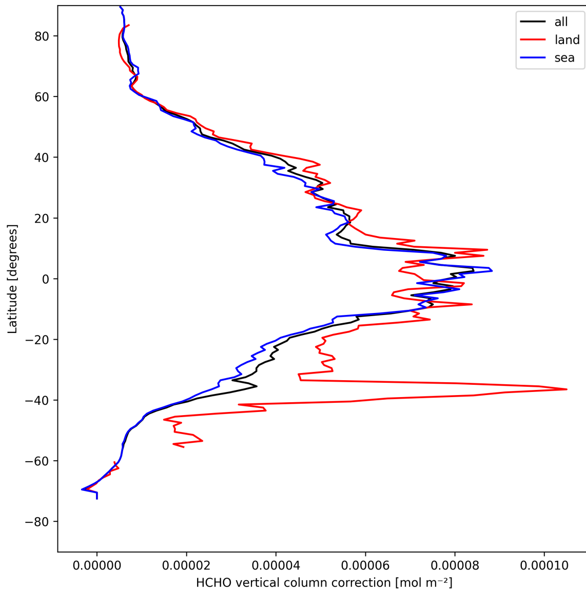
Figure 21: Zonal average of “HCHO vertical column correction” for 2025-04-22 to 2025-04-22.
