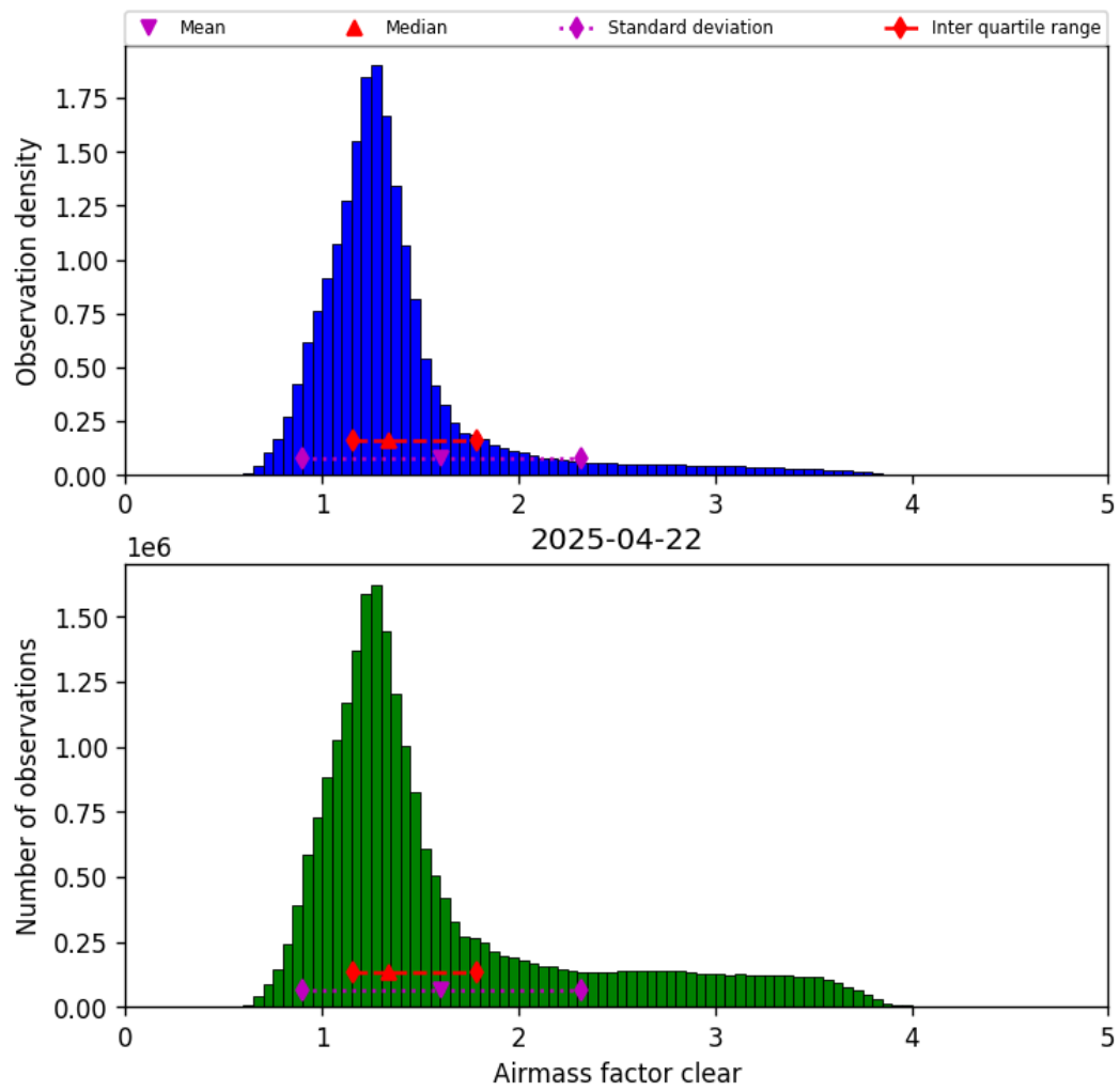
Figure 40: Histogram of “Airmass factor clear” for 2025-04-22 to 2025-04-22
