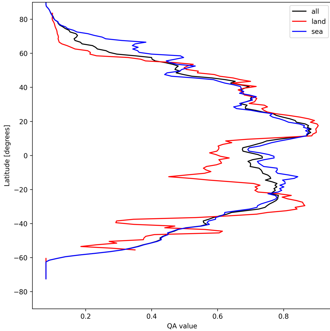
Figure 18: Zonal average of “QA value” for 2025-04-22 to 2025-04-22.
