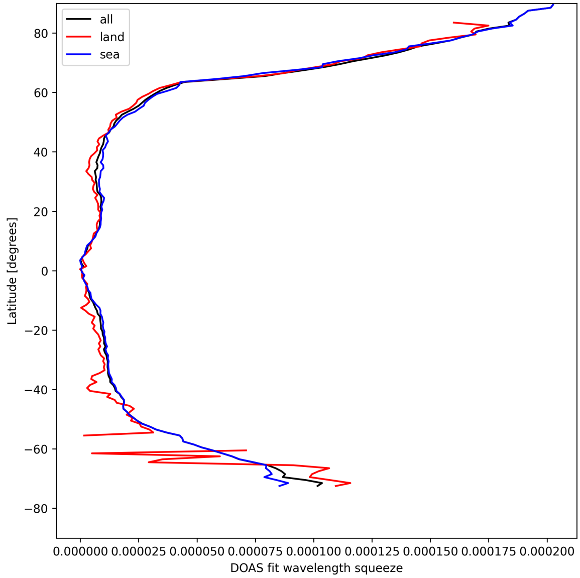
Figure 29: Zonal average of “DOAS fit wavelength squeeze” for 2025-04-22 to 2025-04-22.
