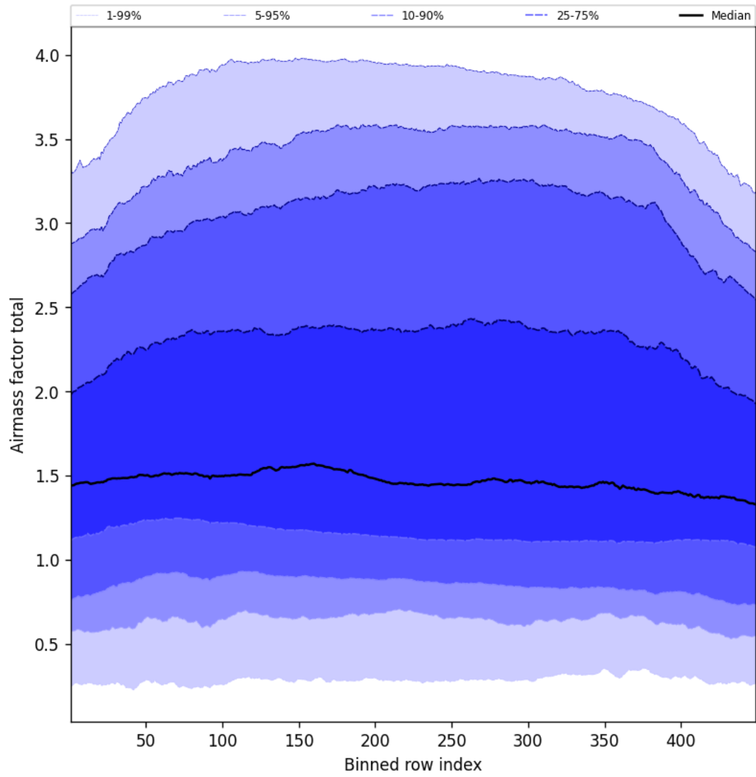
Figure 52: Along track statistics of “Airmass factor total” for 2025-04-22 to 2025-04-22
