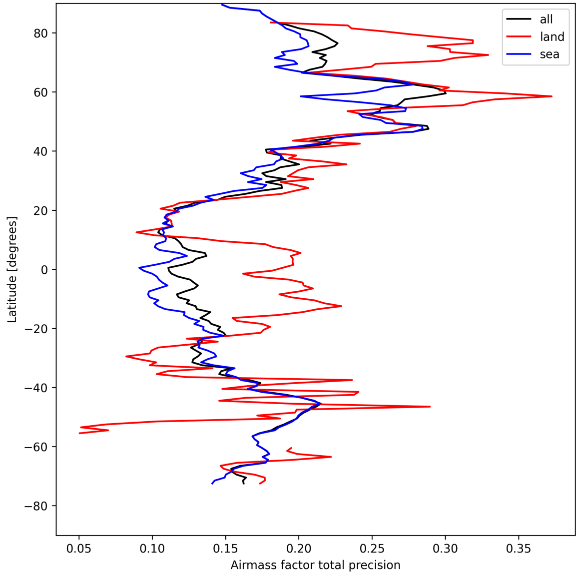
Figure 25: Zonal average of “Airmass factor total precision” for 2025-04-22 to 2025-04-22.
