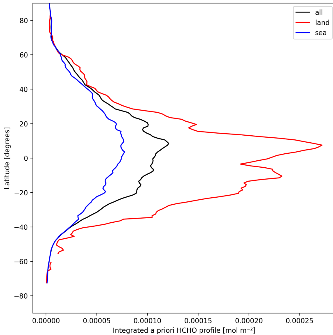
Figure 27: Zonal average of “Integrated a priori HCHO profile” for 2025-04-22 to 2025-04-22.
