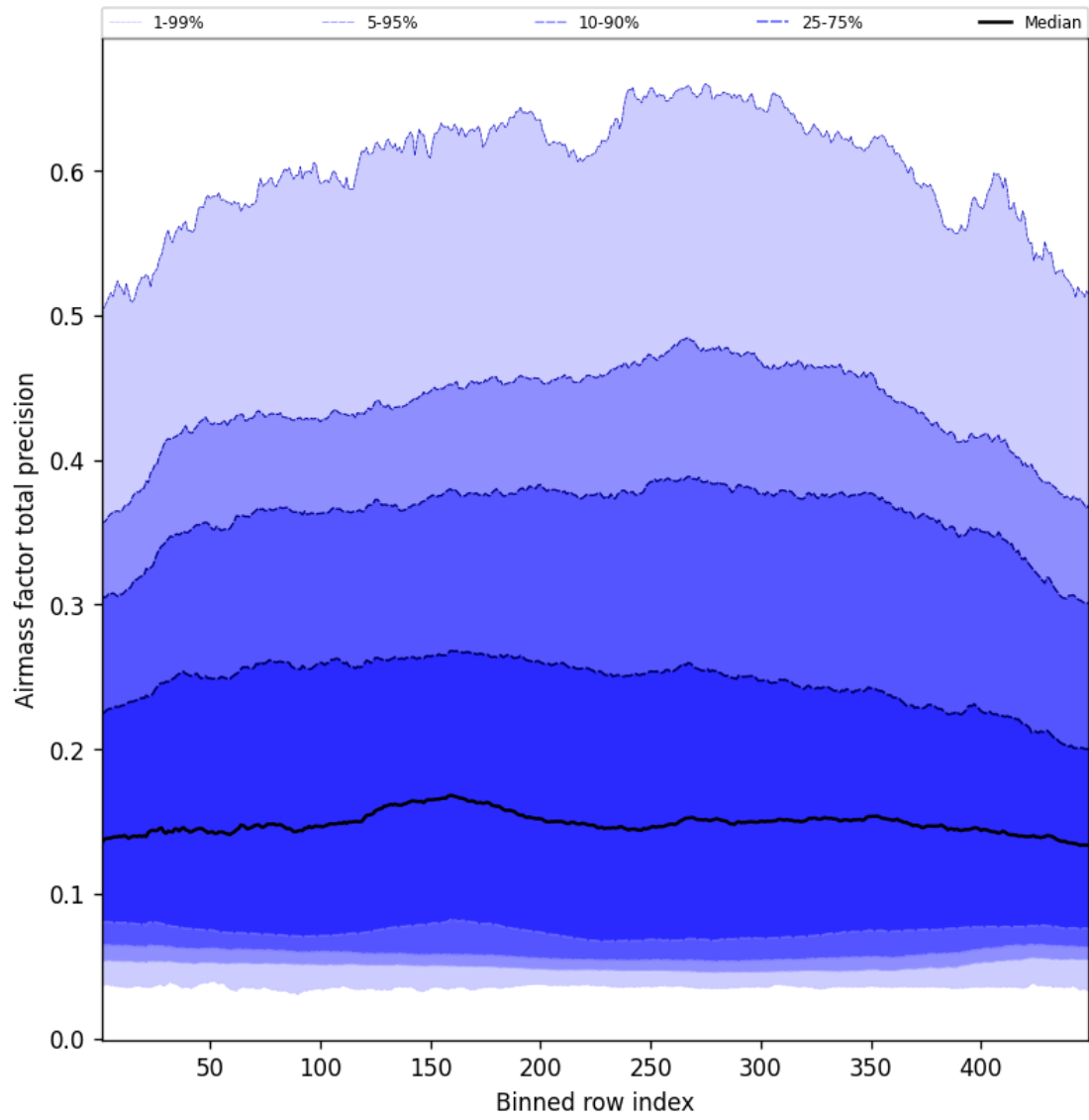
Figure 53: Along track statistics of “Airmass factor total precision” for 2025-04-22 to 2025-04-22
