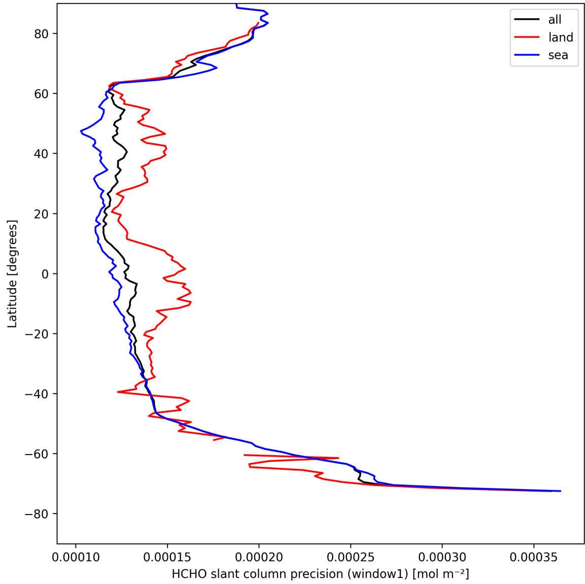
Figure 23: Zonal average of "HCHO slant column precision (window1)" for 2025-04-22 to 2025-04-22.
