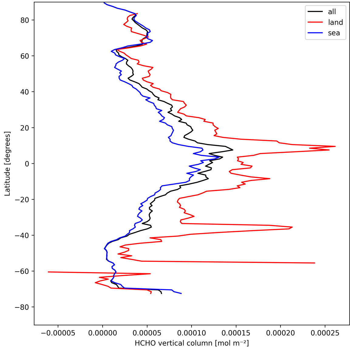
Figure 19: Zonal average of “HCHO vertical column” for 2025-04-22 to 2025-04-22.
