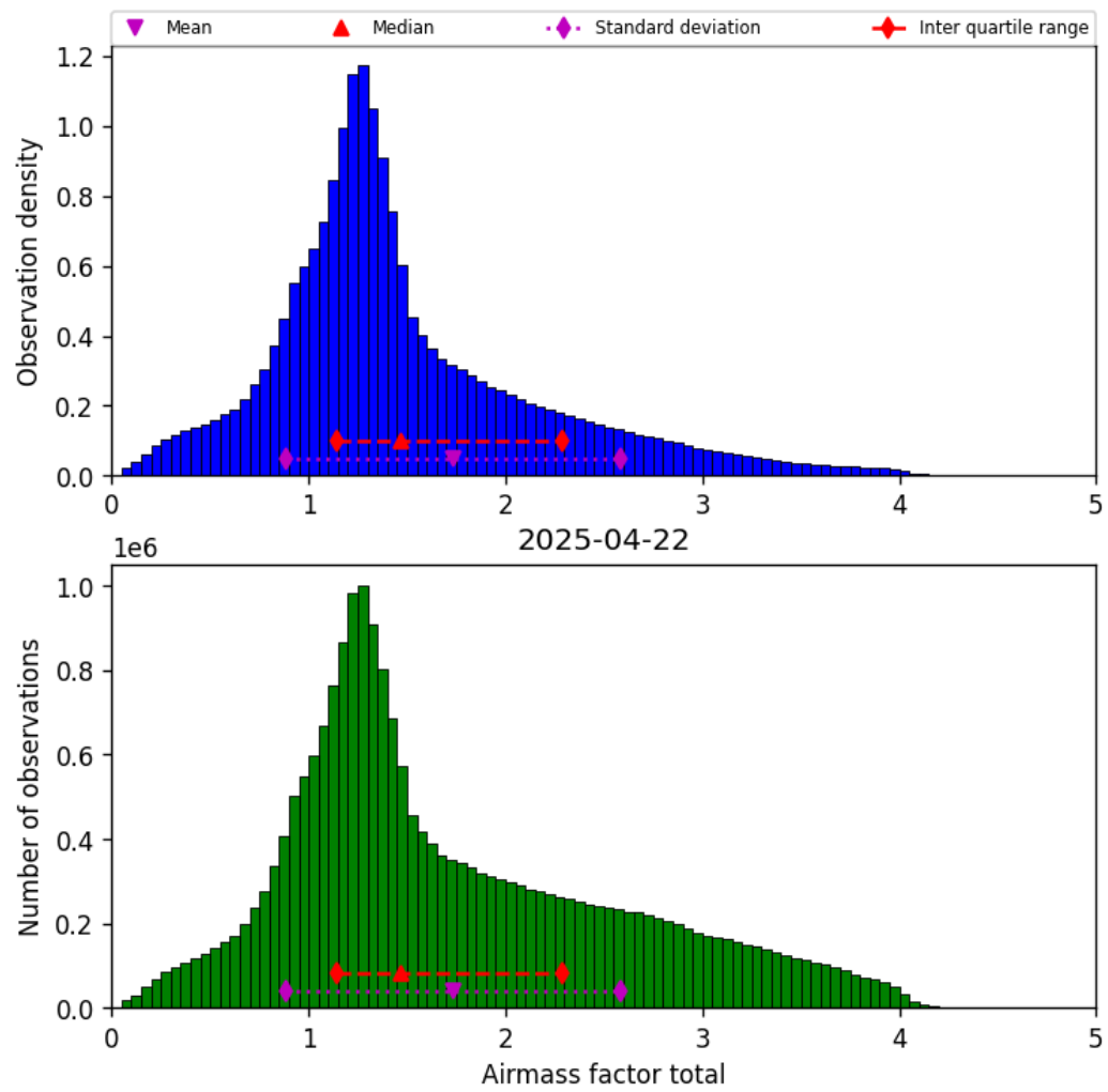
Figure 38: Histogram of “Airmass factor total” for 2025-04-22 to 2025-04-22
