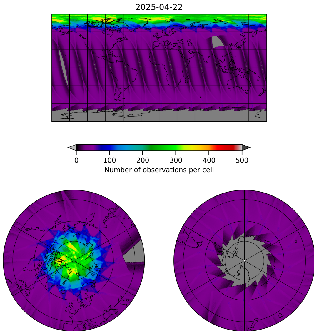
Figure 17: Map of the number of observations for 2025-04-22 to 2025-04-22
