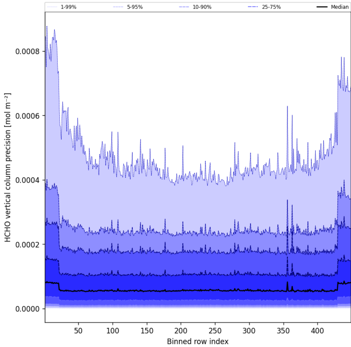
Figure 48: Along track statistics of “HCHO vertical column precision” for 2025-04-23 to 2025-04-24
