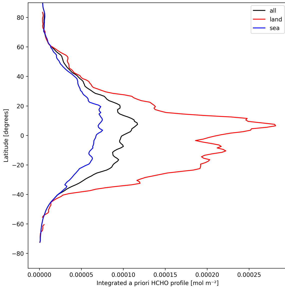
Figure 27: Zonal average of “Integrated a priori HCHO profile” for 2025-04-23 to 2025-04-24.
