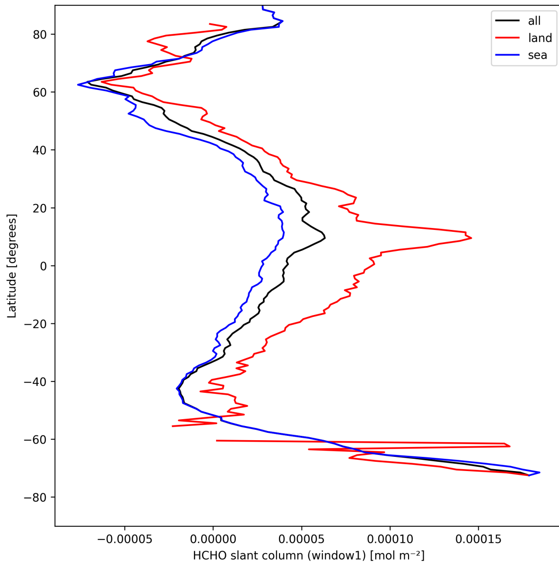
Figure 22: Zonal average of “HCHO slant column (window1)” for 2025-04-23 to 2025-04-24.
