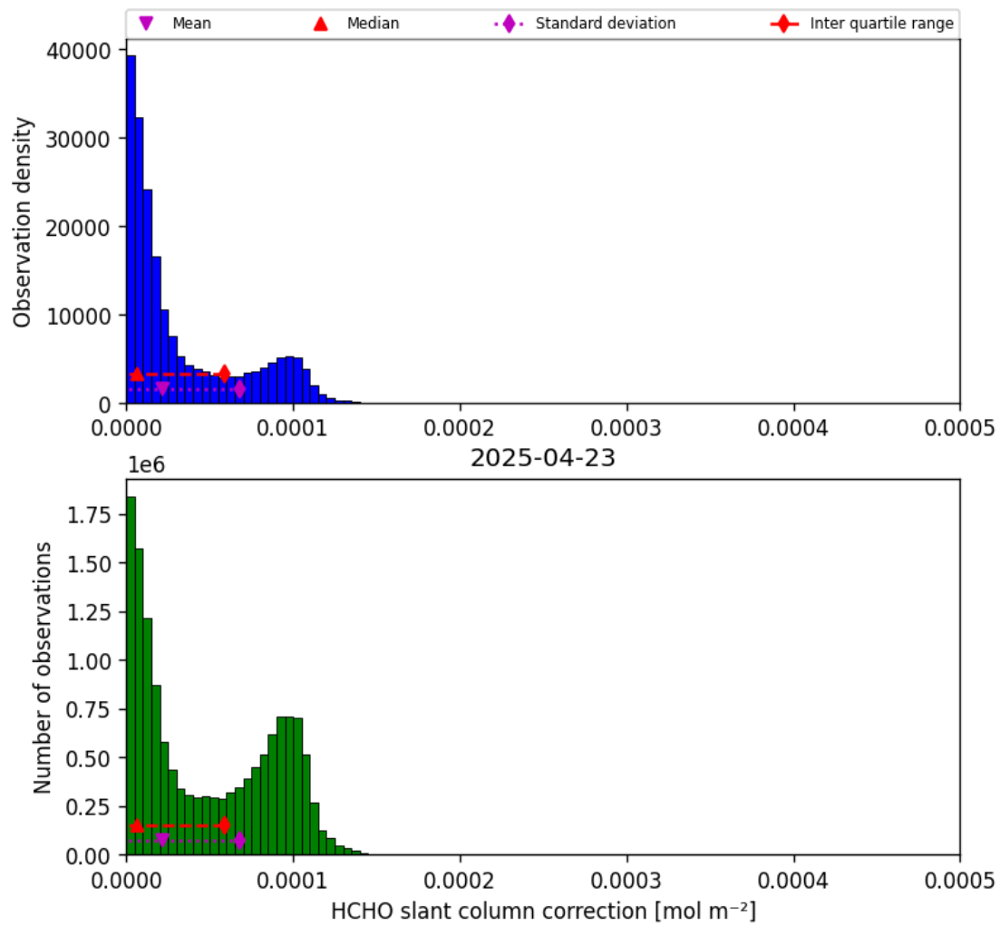
Figure 45: Histogram of “HCHO slant column correction” for 2025-04-23 to 2025-04-24
