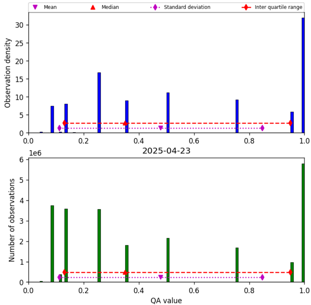
Figure 32: Histogram of “QA value” for 2025-04-23 to 2025-04-24
