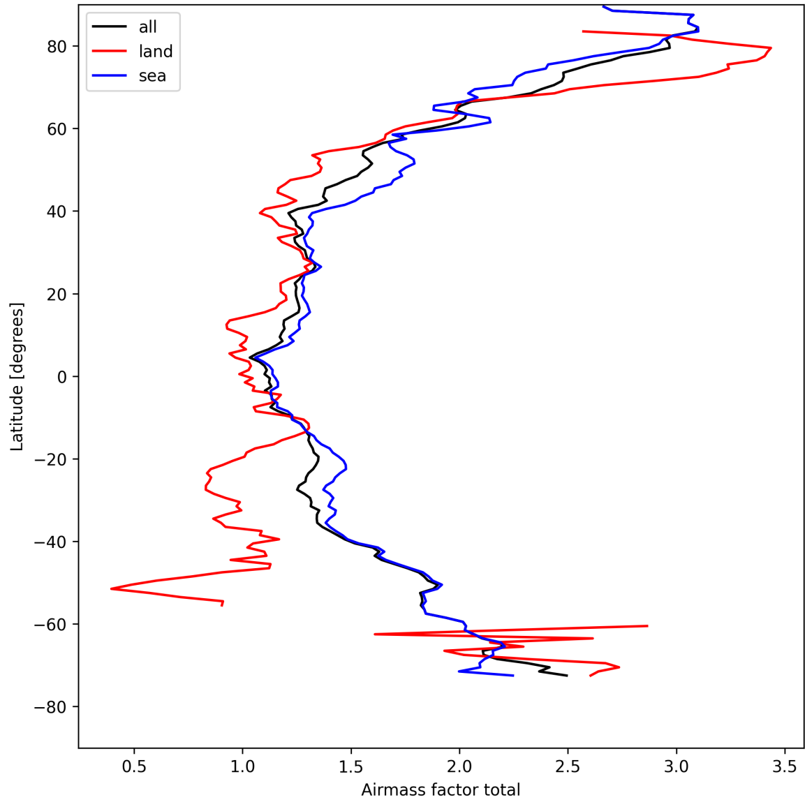
Figure 24: Zonal average of “Airmass factor total” for 2025-04-23 to 2025-04-24.
