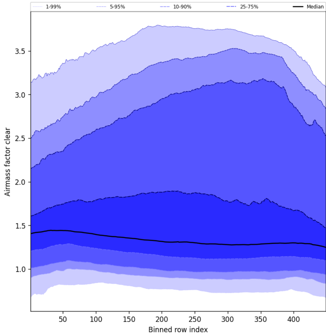
Figure 54: Along track statistics of “Airmass factor clear” for 2025-04-23 to 2025-04-24
