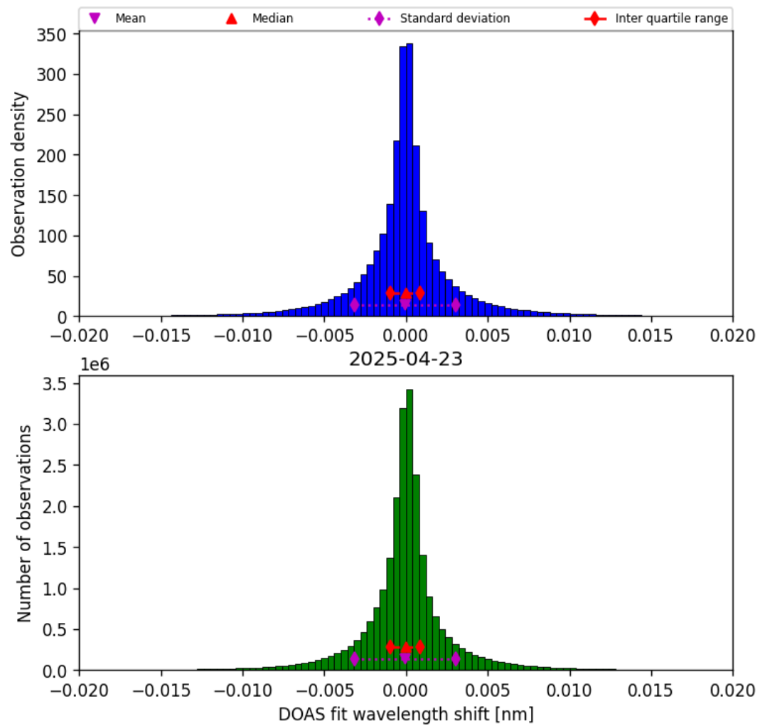
Figure 42: Histogram of “DOAS fit wavelength shift” for 2025-04-23 to 2025-04-24
