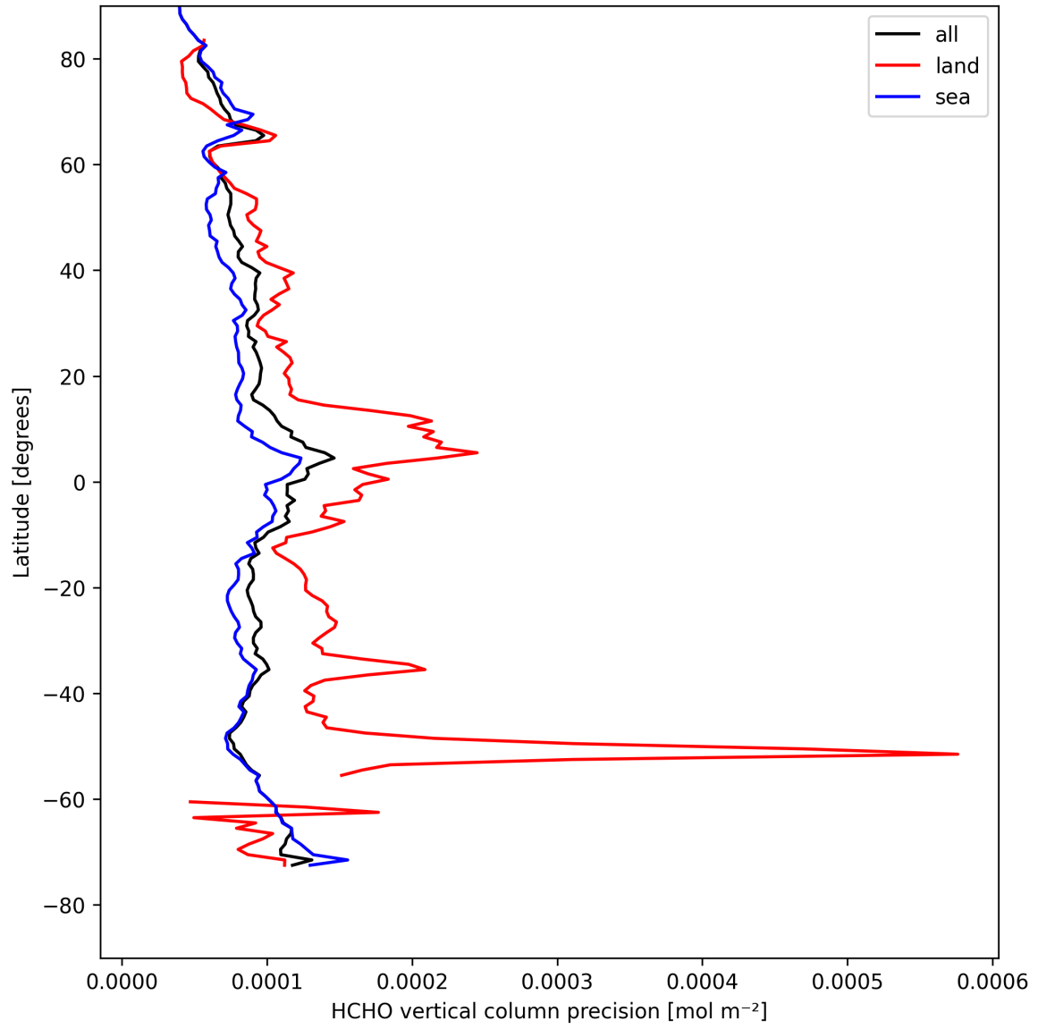
Figure 20: Zonal average of “HCHO vertical column precision” for 2025-04-23 to 2025-04-24.
