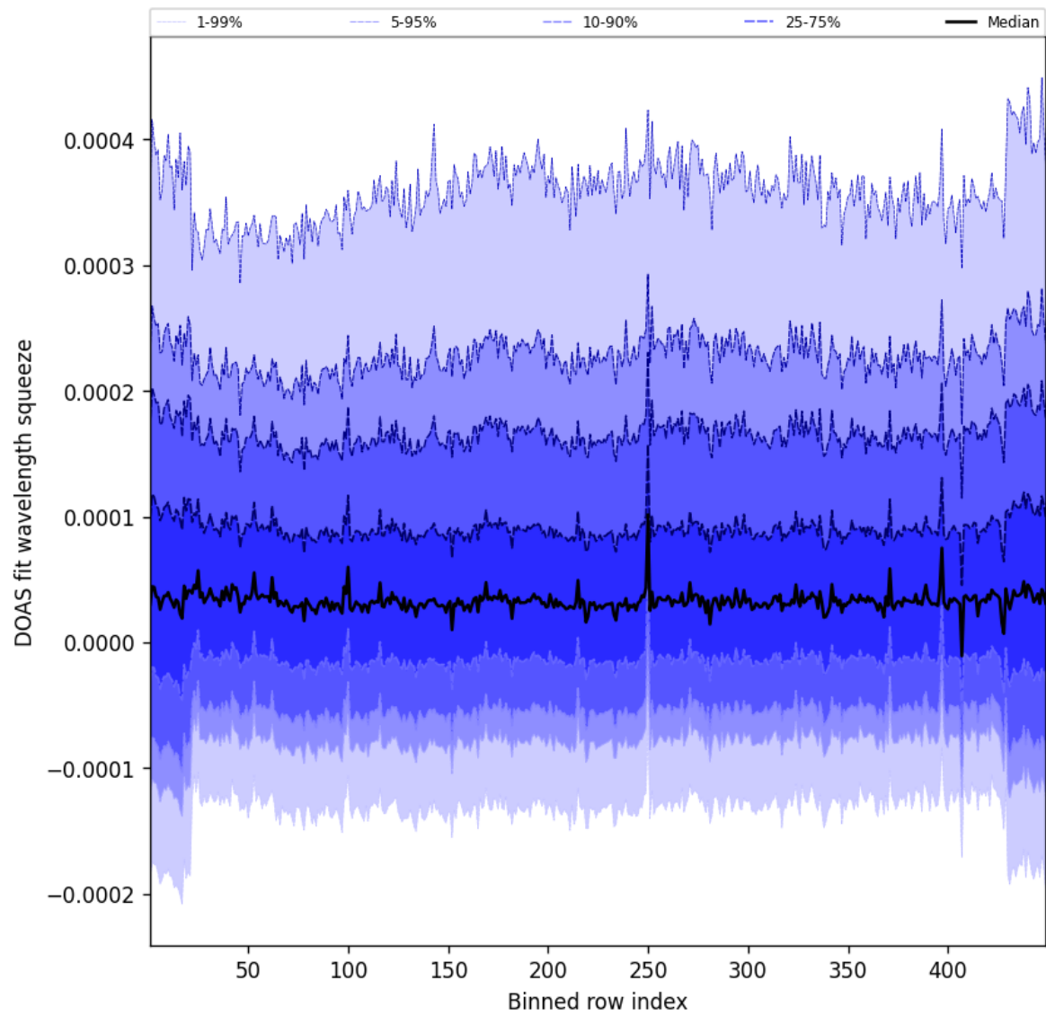
Figure 57: Along track statistics of “DOAS fit wavelength squeeze” for 2025-04-23 to 2025-04-24
