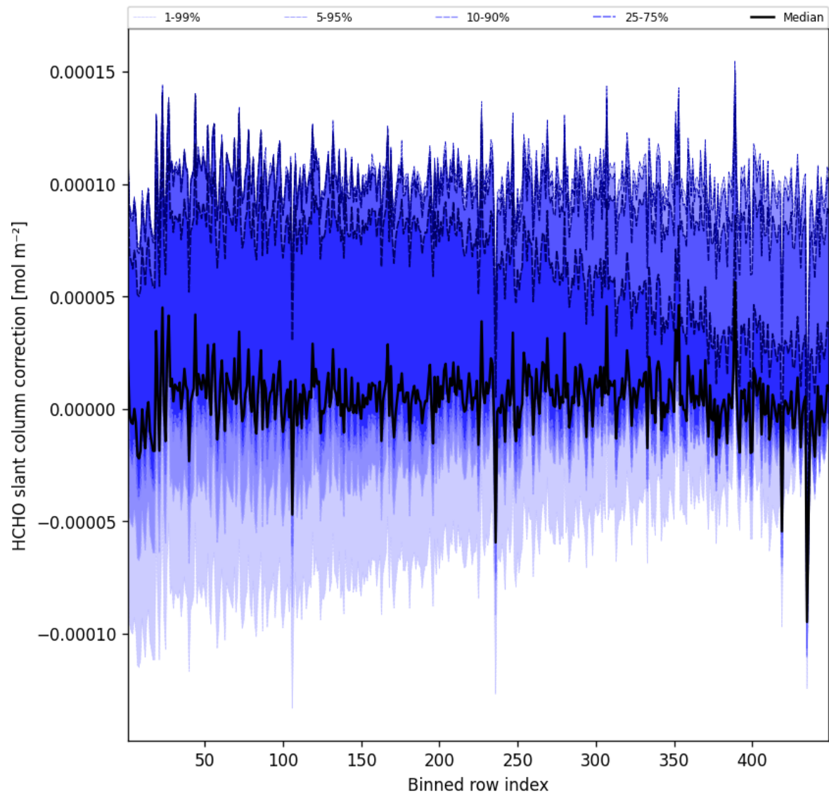
Figure 59: Along track statistics of “HCHO slant column correction” for 2025-04-23 to 2025-04-24
