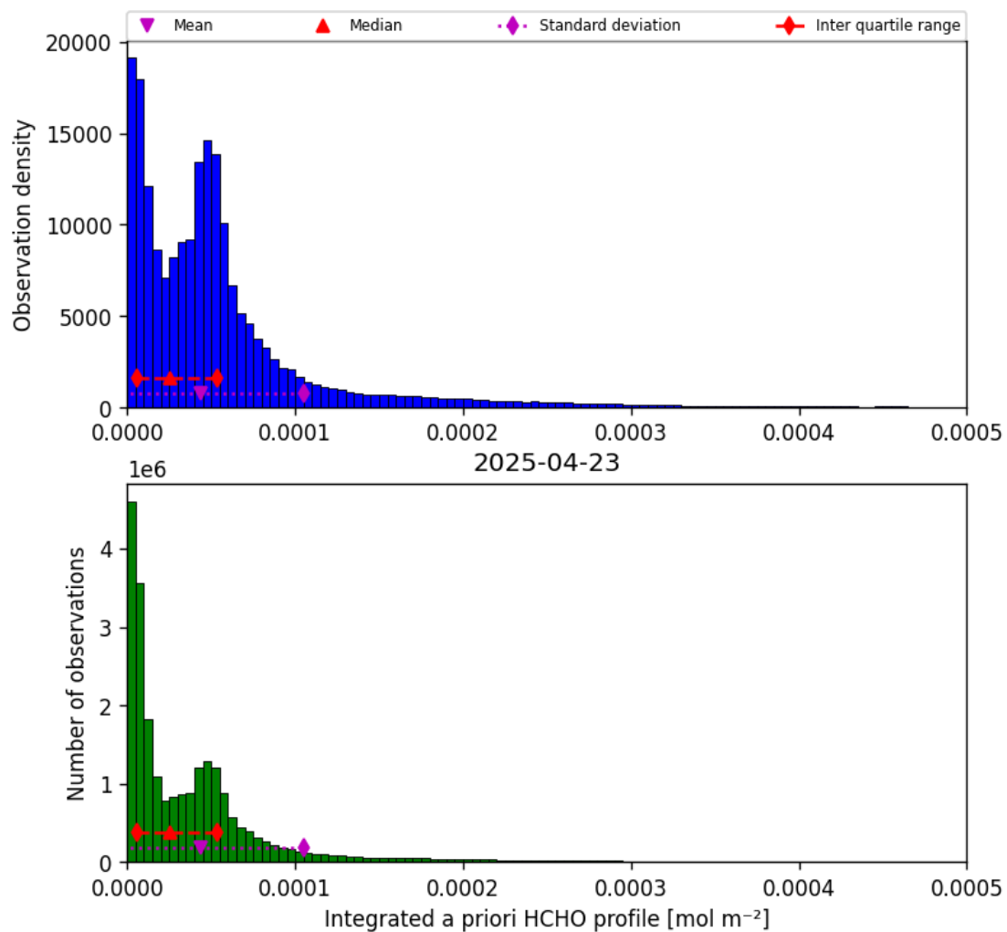
Figure 41: Histogram of “Integrated a priori HCHO profile” for 2025-04-23 to 2025-04-24
