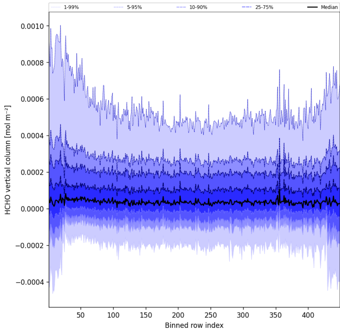
Figure 47: Along track statistics of “HCHO vertical column” for 2025-04-23 to 2025-04-24
