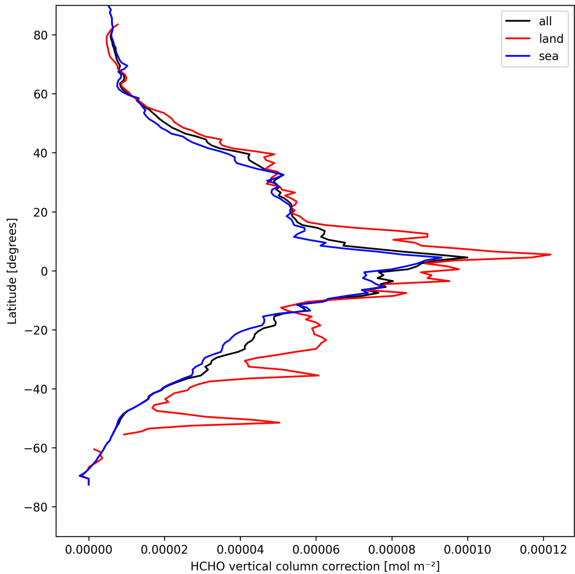
Figure 21: Zonal average of “HCHO vertical column correction” for 2025-04-23 to 2025-04-24.
