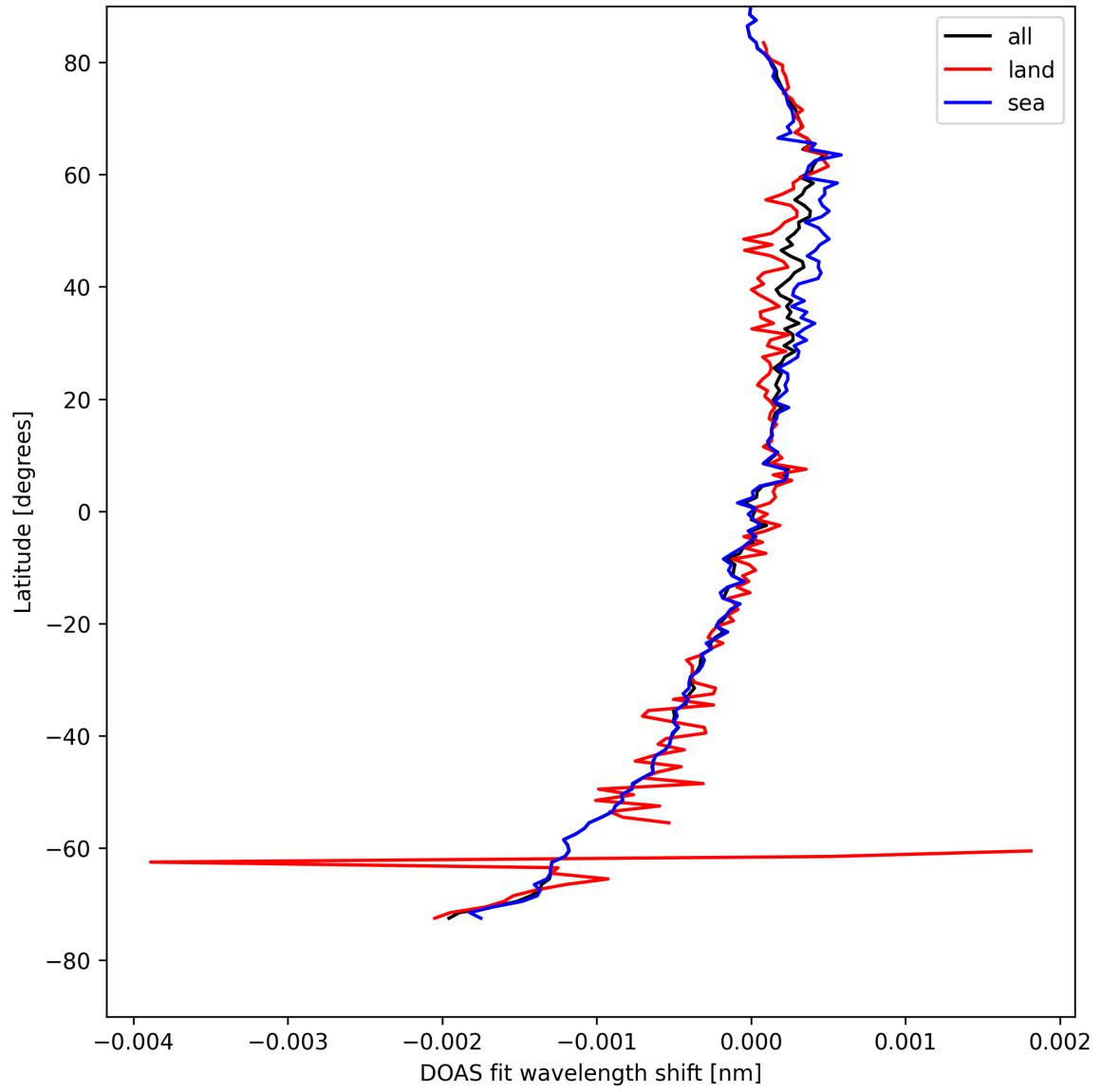
Figure 28: Zonal average of “DOAS fit wavelength shift” for 2025-04-23 to 2025-04-24.
