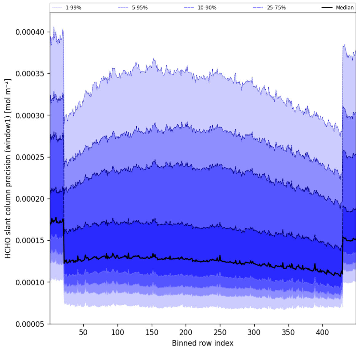
Figure 51: Along track statistics of “HCHO slant column precision (window1)” for 2025-04-23 to 2025-04-24
