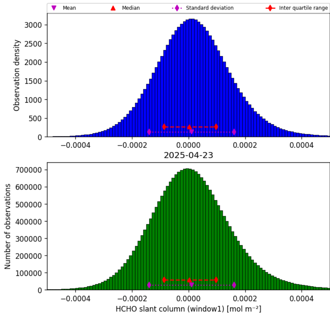
Figure 36: Histogram of “HCHO slant column (window1)” for 2025-04-23 to 2025-04-24
