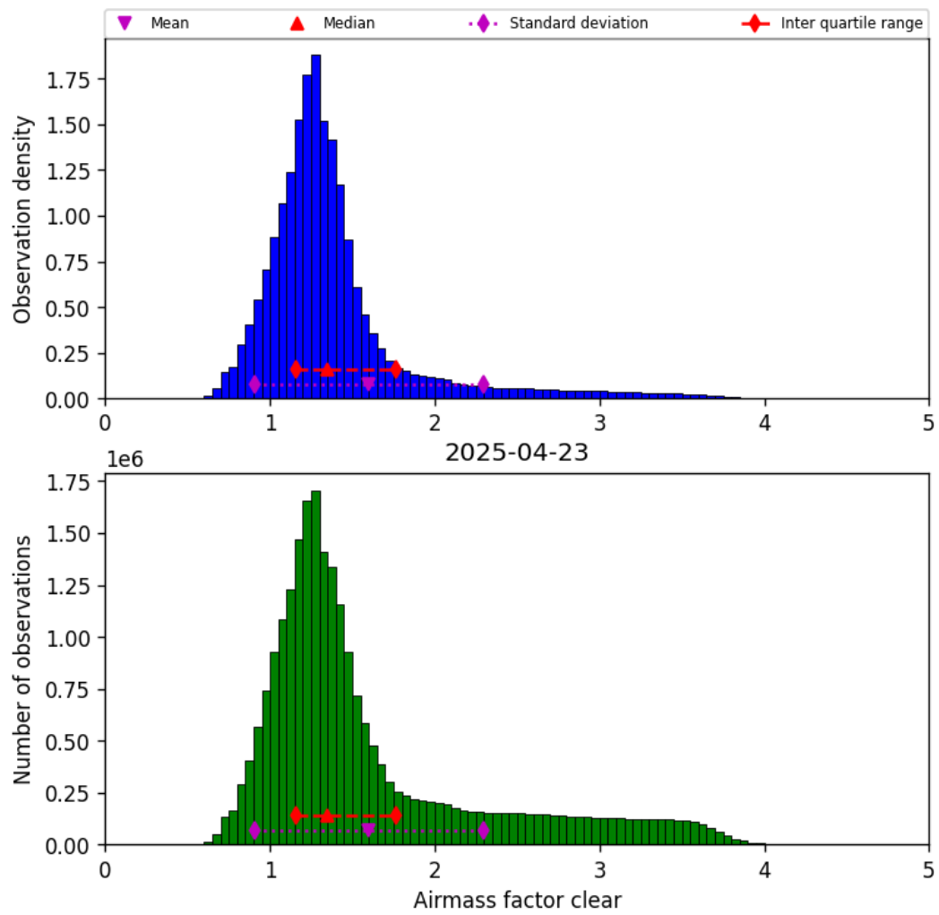
Figure 40: Histogram of “Airmass factor clear” for 2025-04-23 to 2025-04-24
