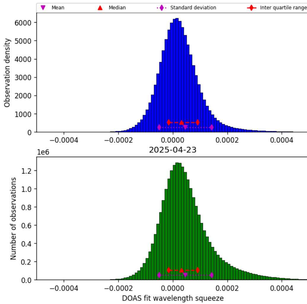
Figure 43: Histogram of “DOAS fit wavelength squeeze” for 2025-04-23 to 2025-04-24
