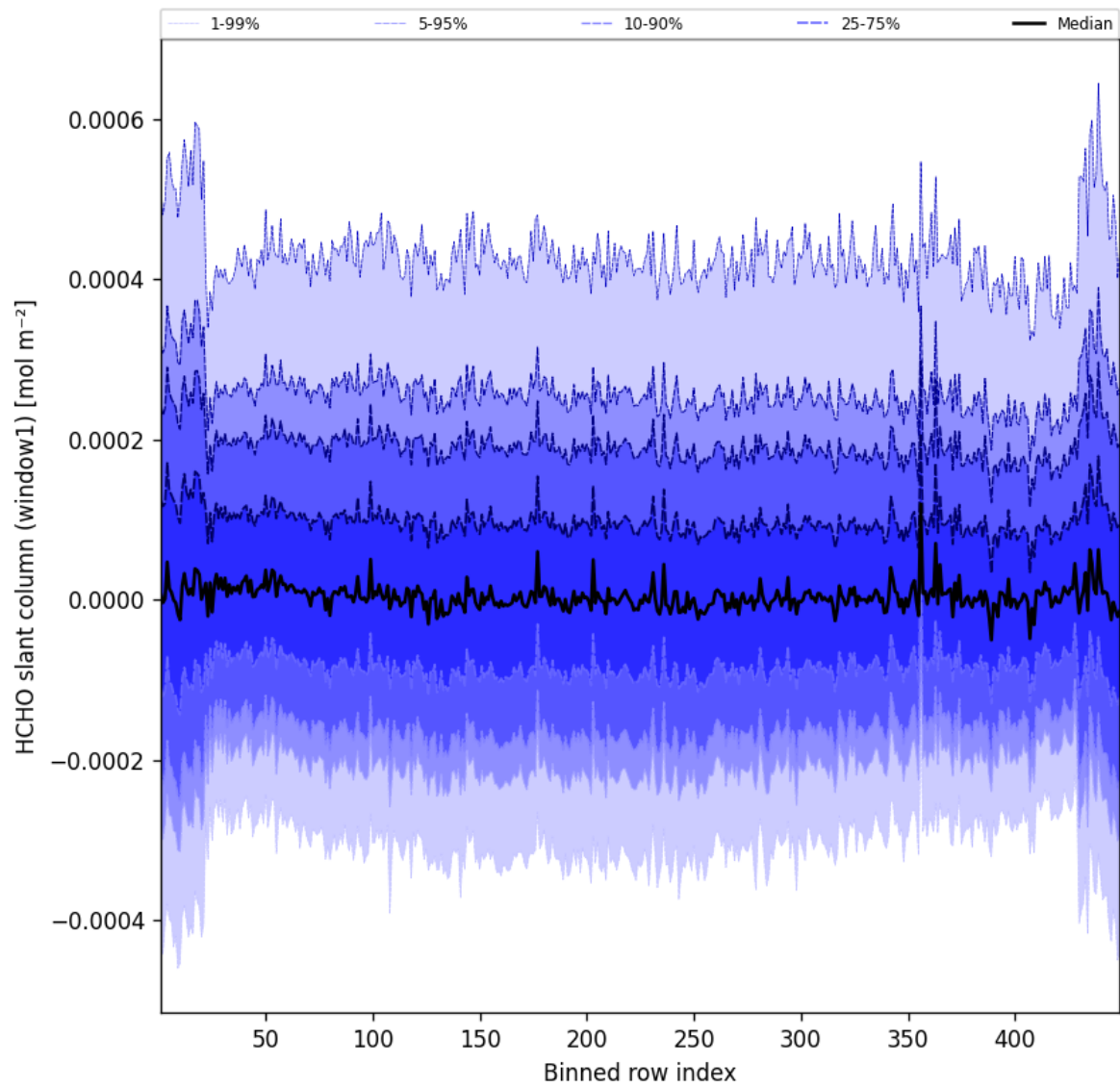
Figure 50: Along track statistics of “HCHO slant column (window1)” for 2025-04-23 to 2025-04-24
