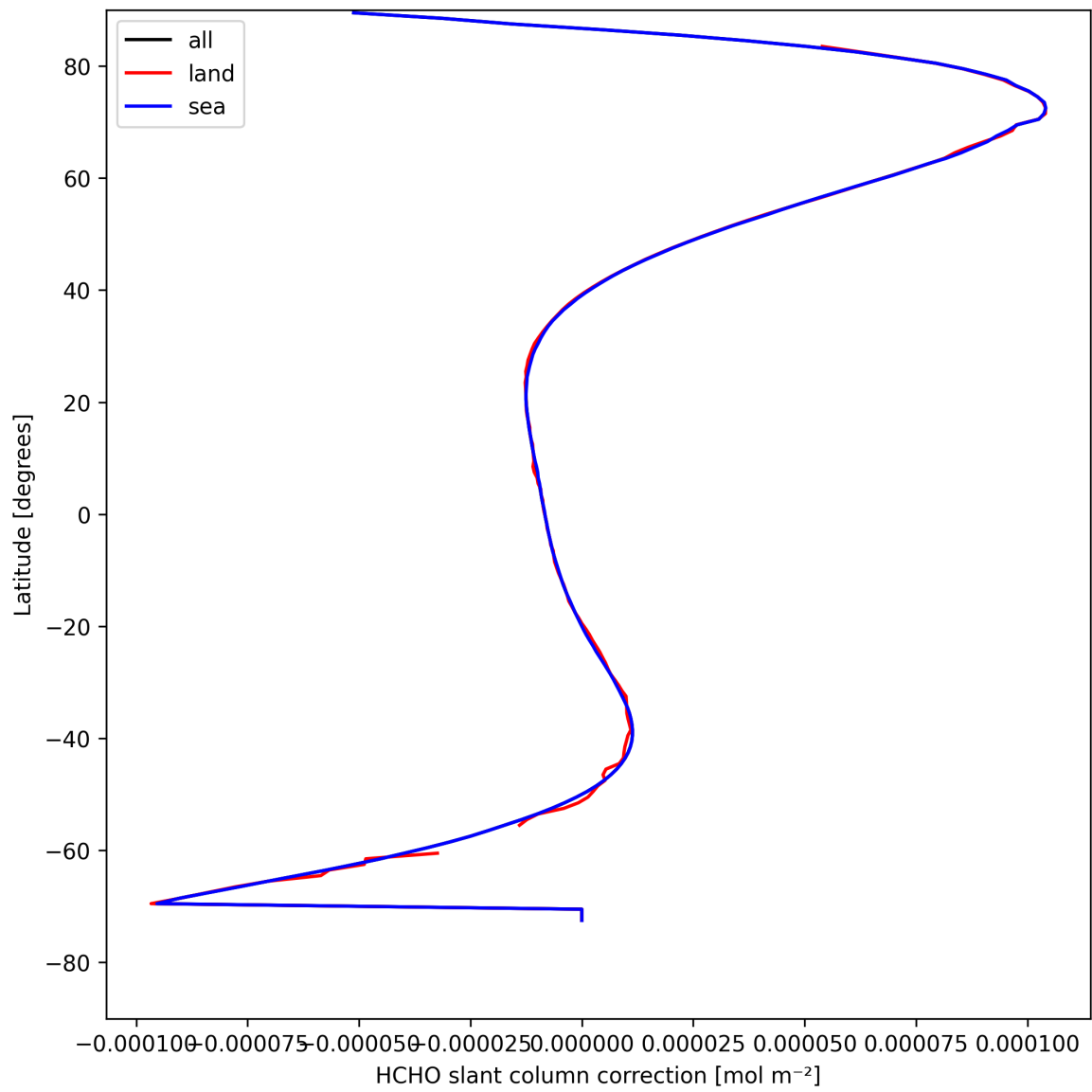
Figure 31: Zonal average of “HCHO slant column correction” for 2025-04-23 to 2025-04-24.
