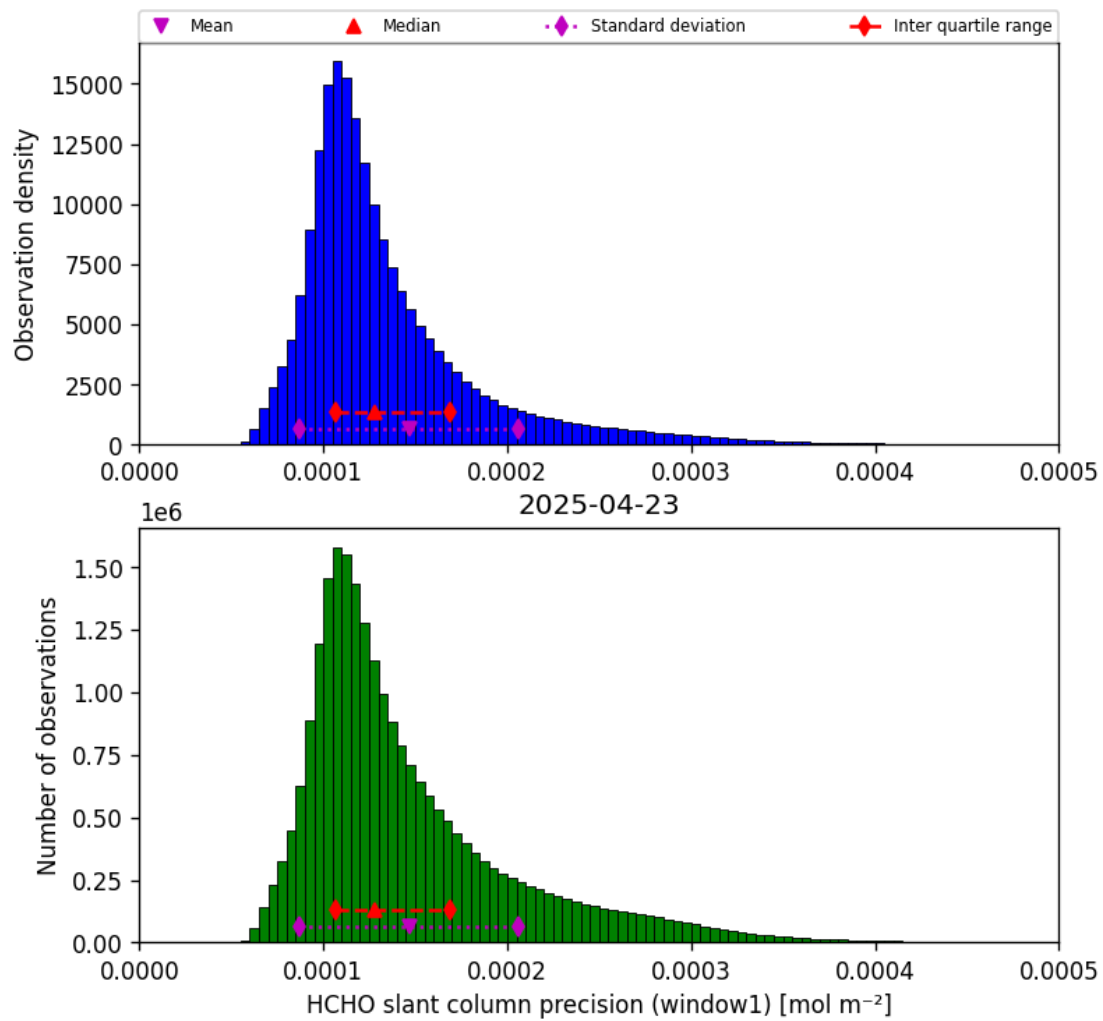
Figure 37: Histogram of “HCHO slant column precision (window1)” for 2025-04-23 to 2025-04-24
