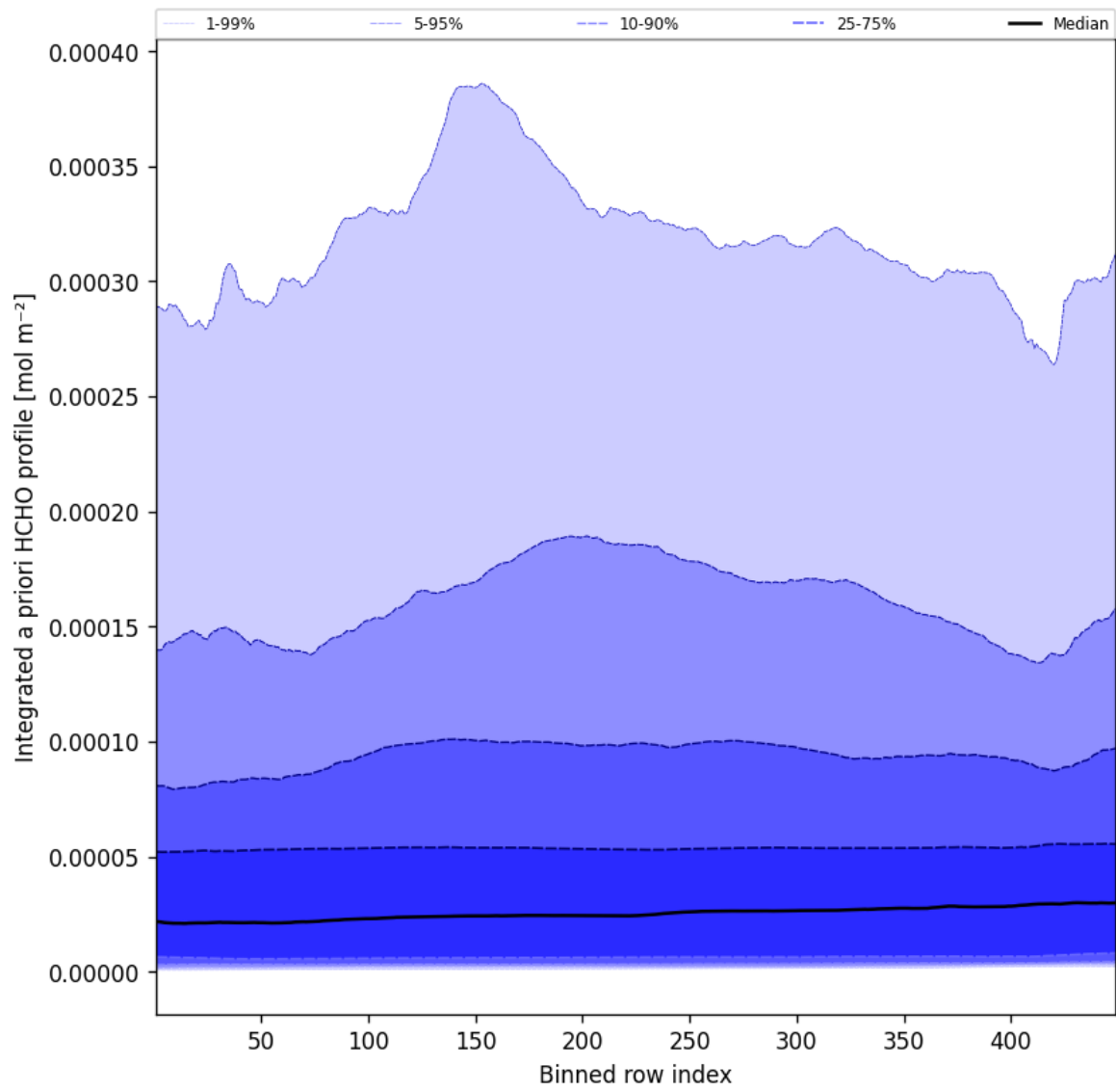
Figure 55: Along track statistics of “Integrated a priori HCHO profile” for 2025-04-23 to 2025-04-24
