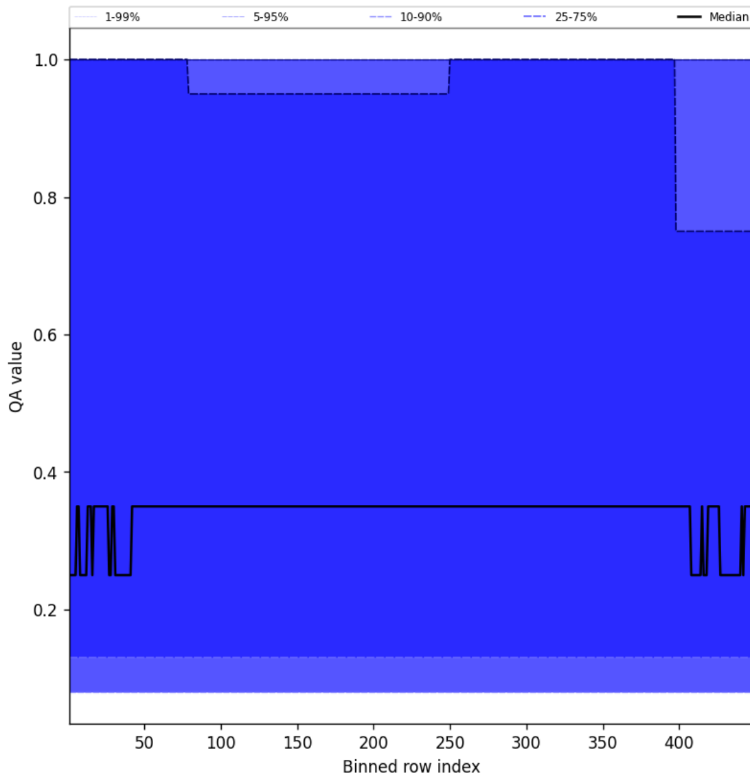
Figure 46: Along track statistics of “QA value” for 2025-04-23 to 2025-04-24
