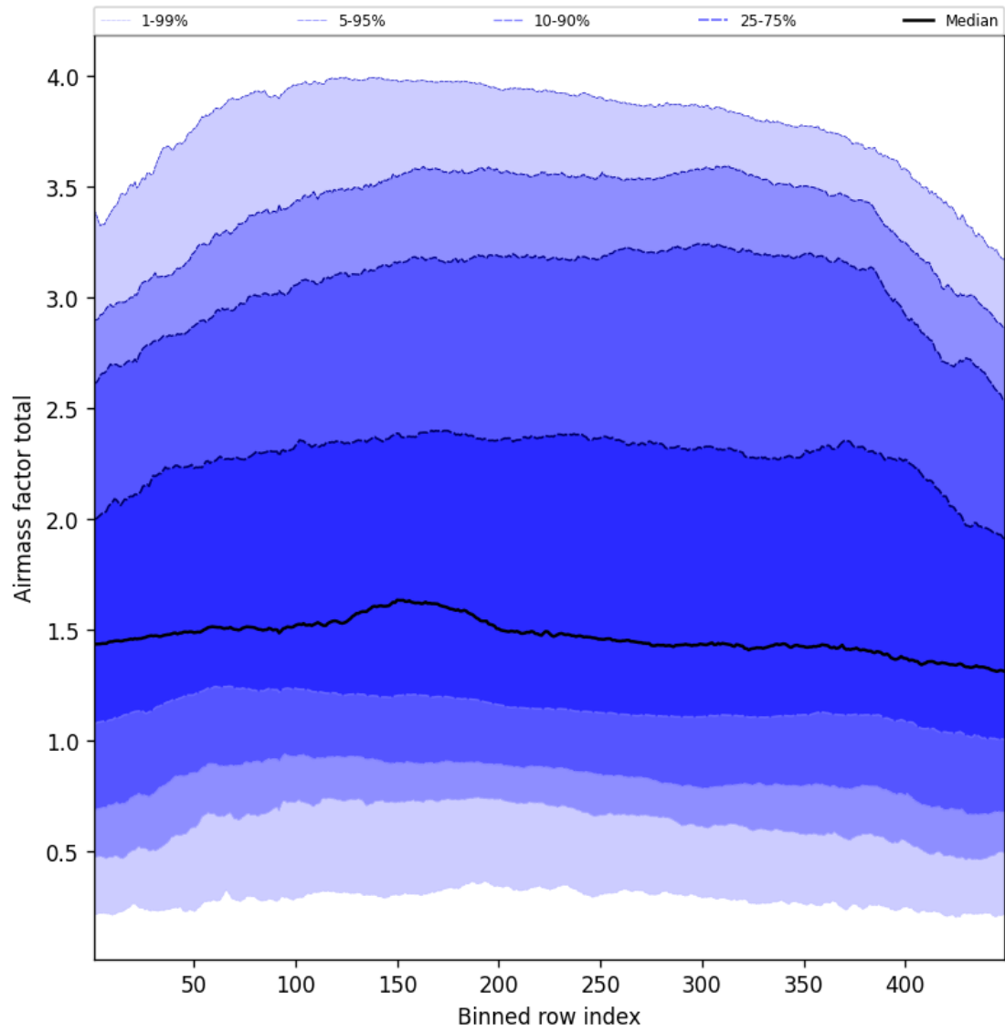
Figure 52: Along track statistics of “Airmass factor total” for 2025-04-23 to 2025-04-24
