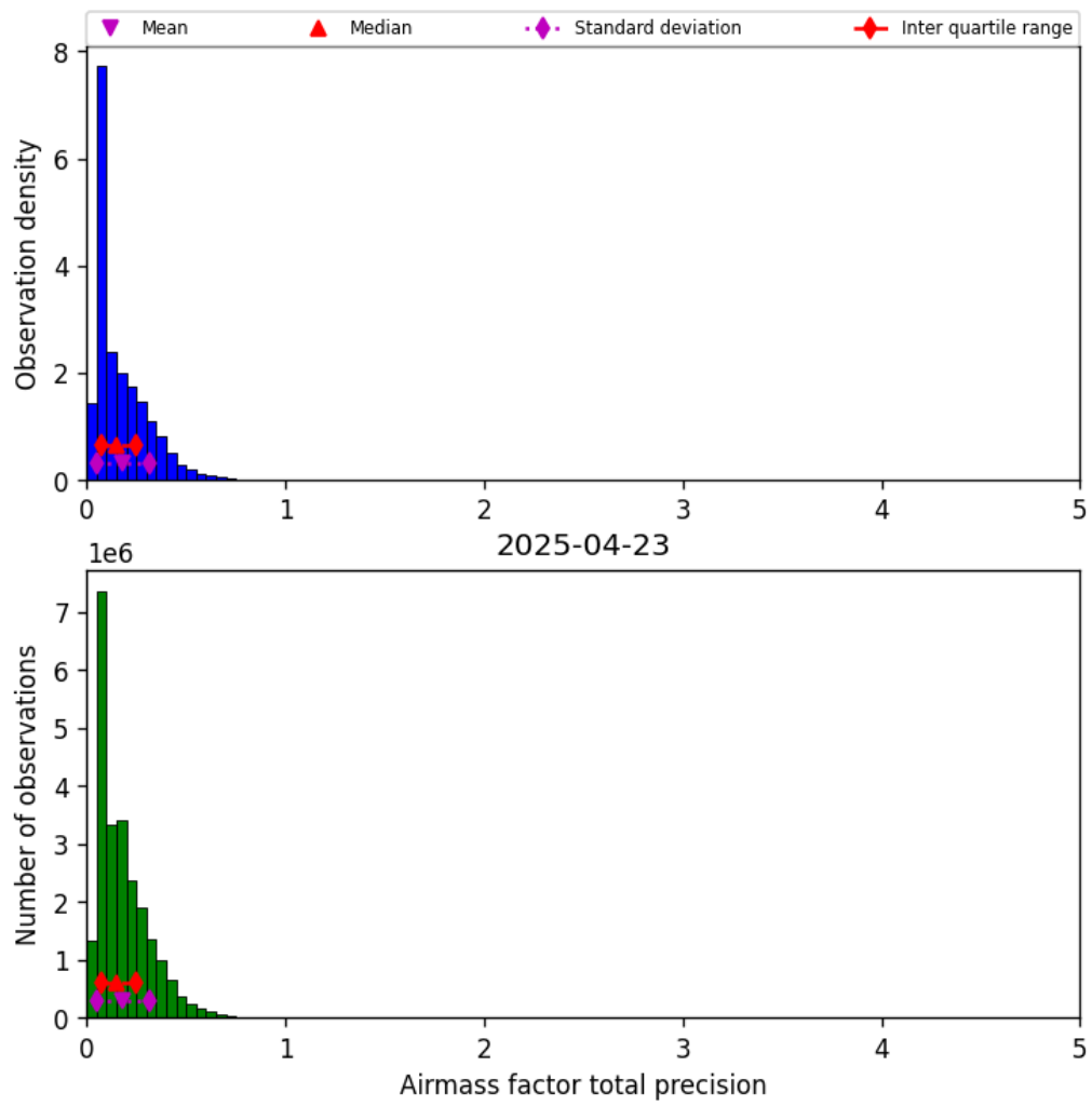
Figure 39: Histogram of “Airmass factor total precision” for 2025-04-23 to 2025-04-24
