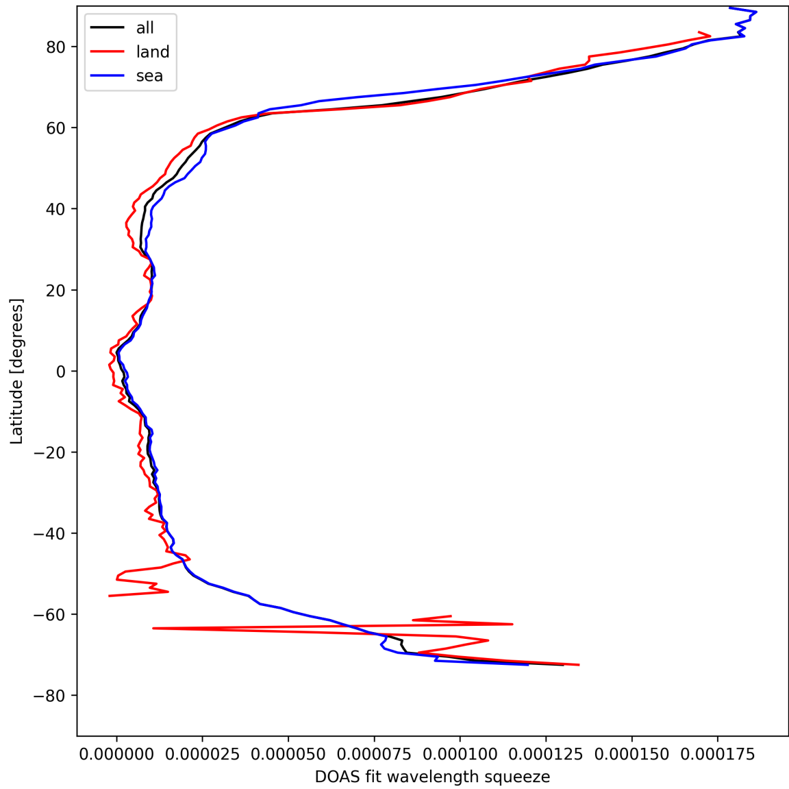
Figure 29: Zonal average of “DOAS fit wavelength squeeze” for 2025-04-23 to 2025-04-24.
