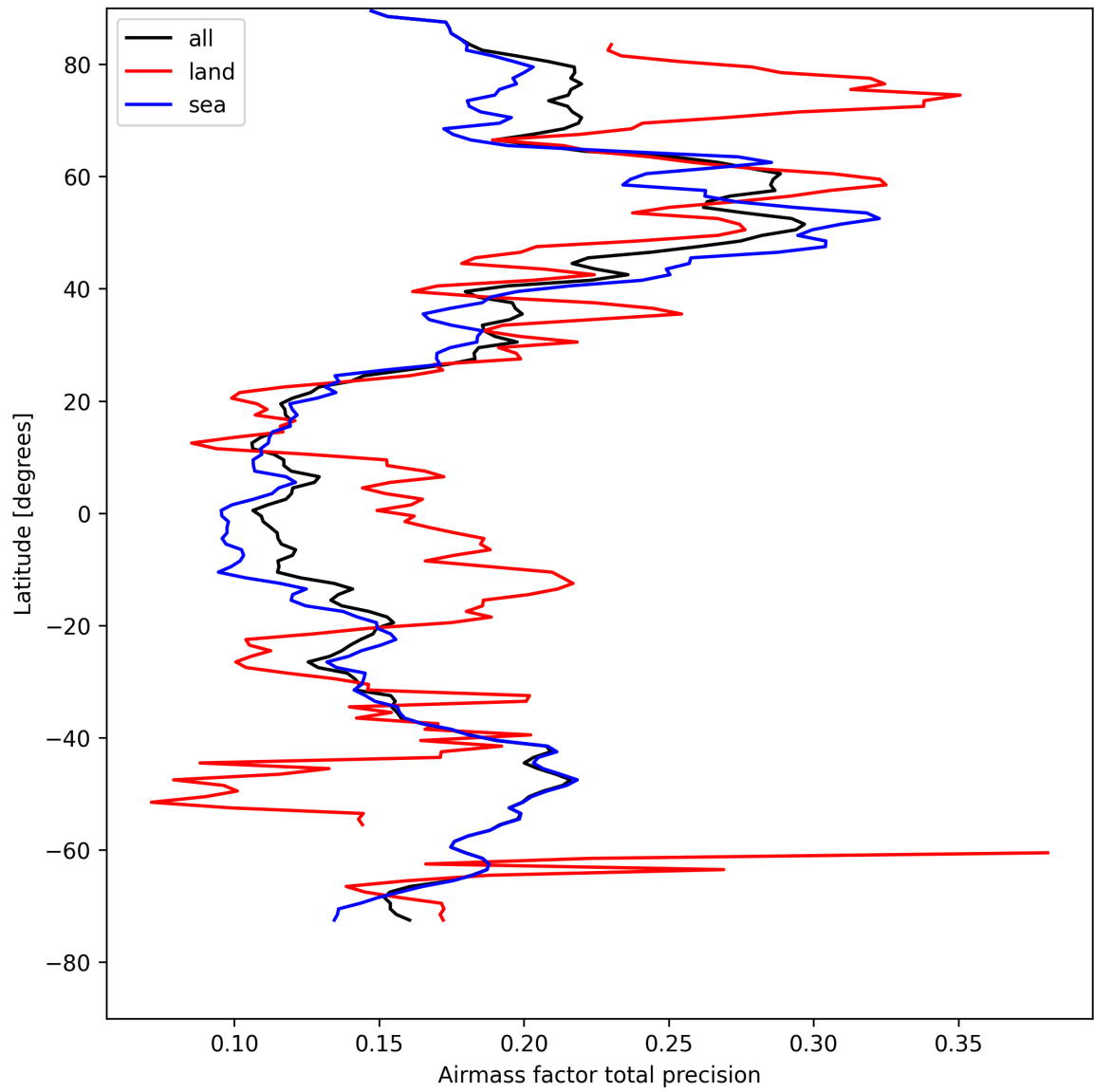
Figure 25: Zonal average of “Airmass factor total precision” for 2025-04-23 to 2025-04-24.
