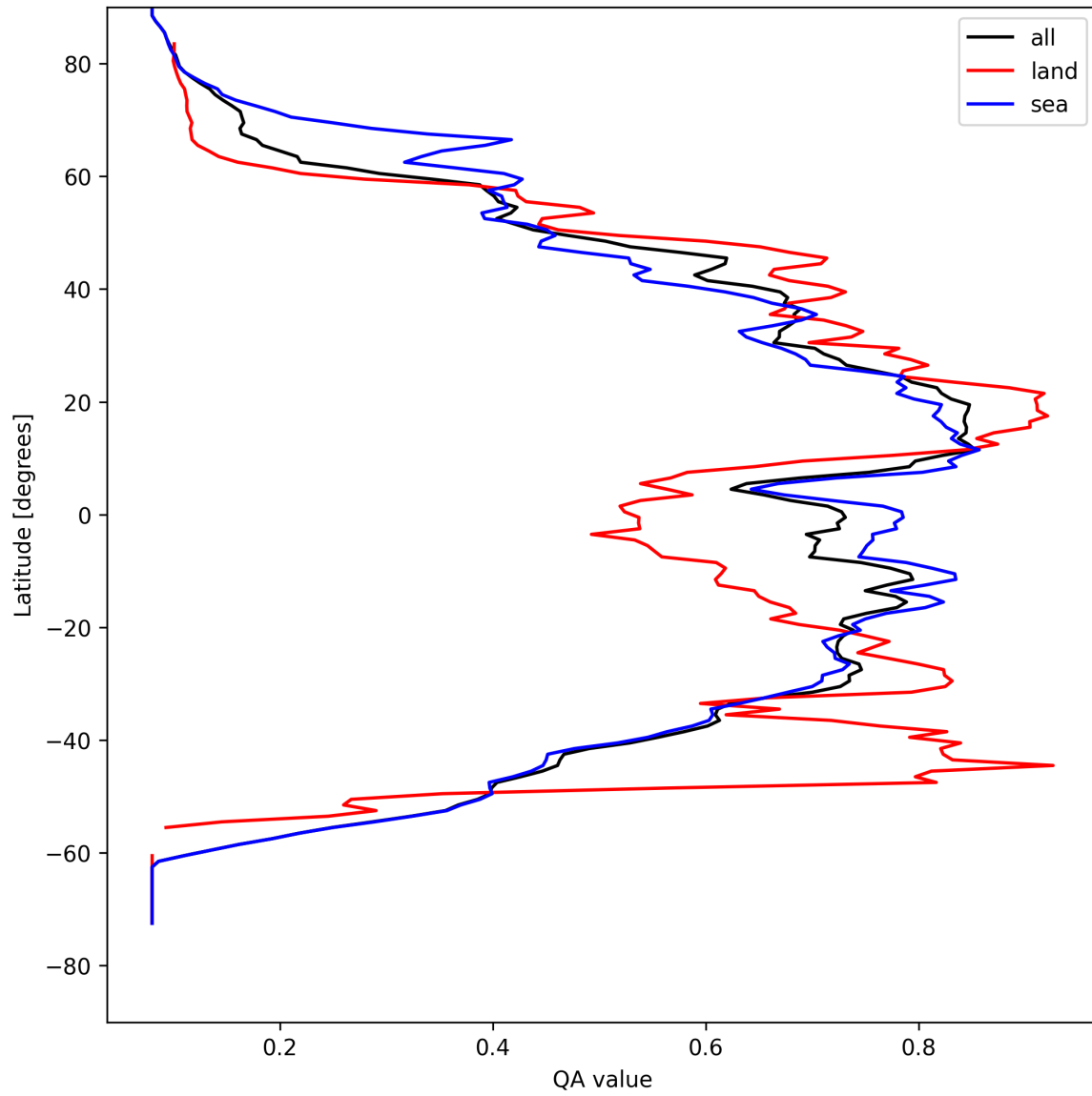
Figure 18: Zonal average of “QA value” for 2025-04-23 to 2025-04-24.
