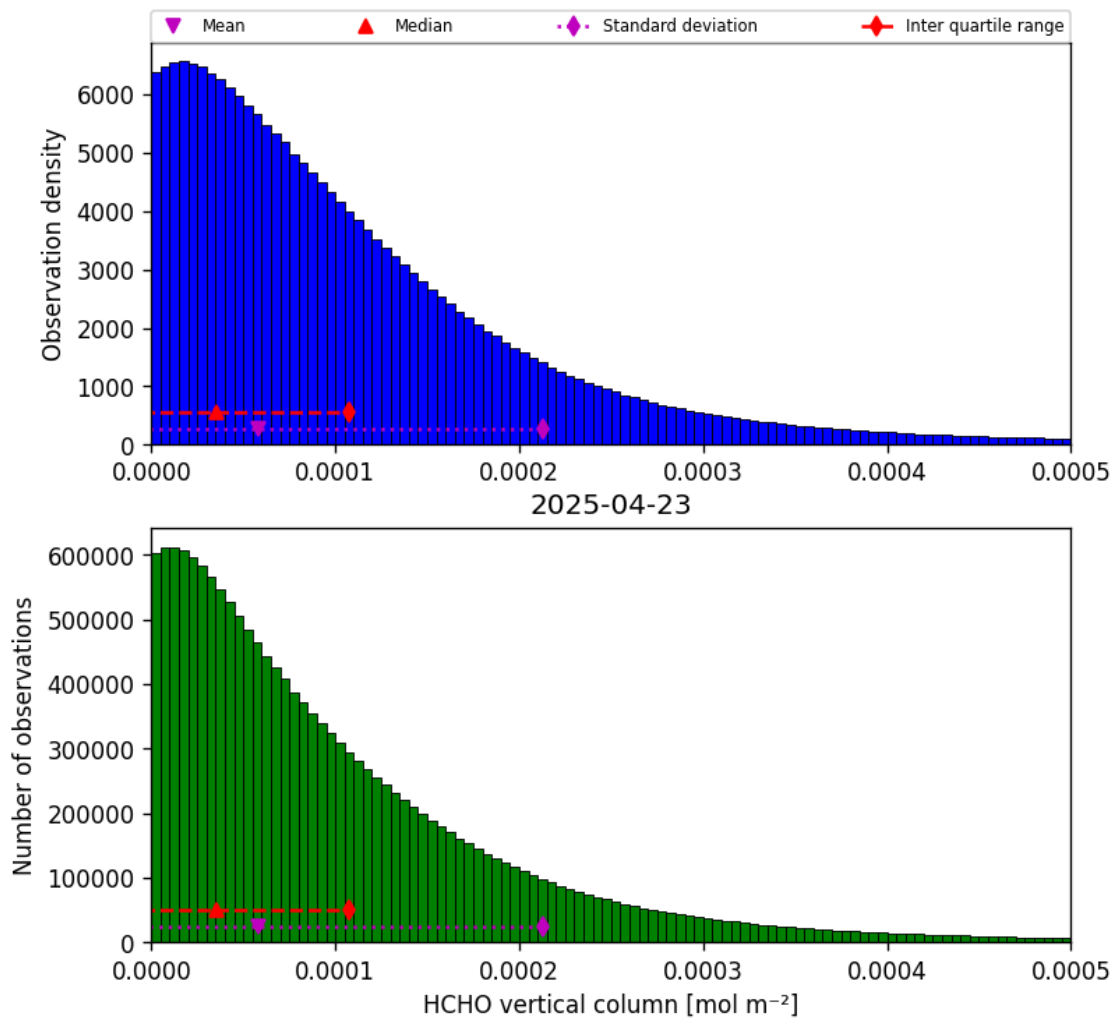
Figure 33: Histogram of “HCHO vertical column” for 2025-04-23 to 2025-04-24
