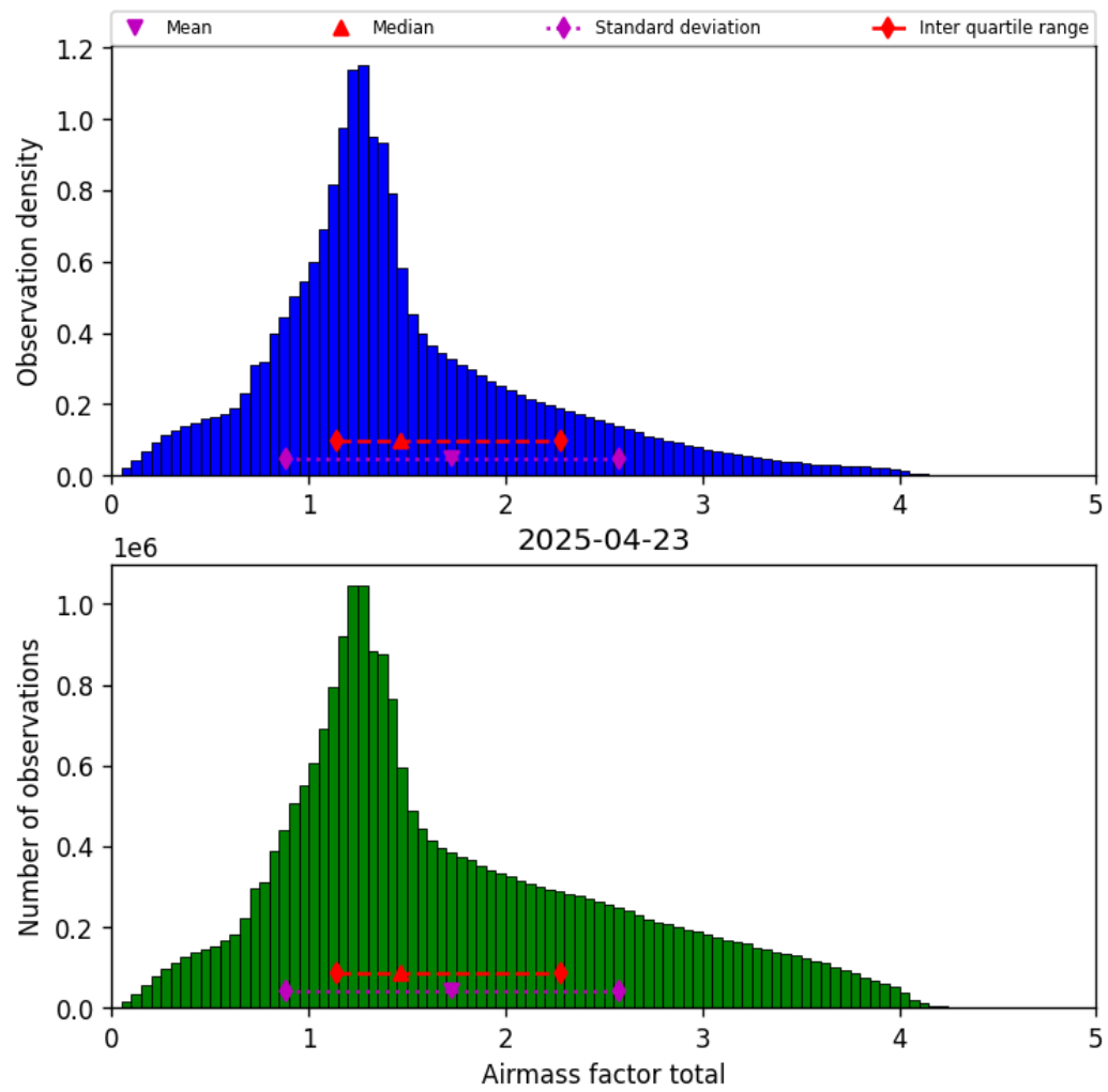
Figure 38: Histogram of “Airmass factor total” for 2025-04-23 to 2025-04-24
