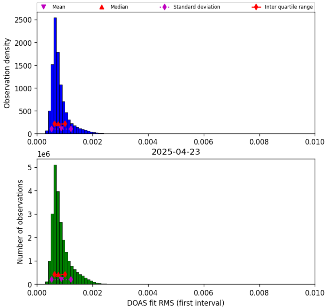
Figure 44: Histogram of “DOAS fit RMS (first interval)” for 2025-04-23 to 2025-04-24
