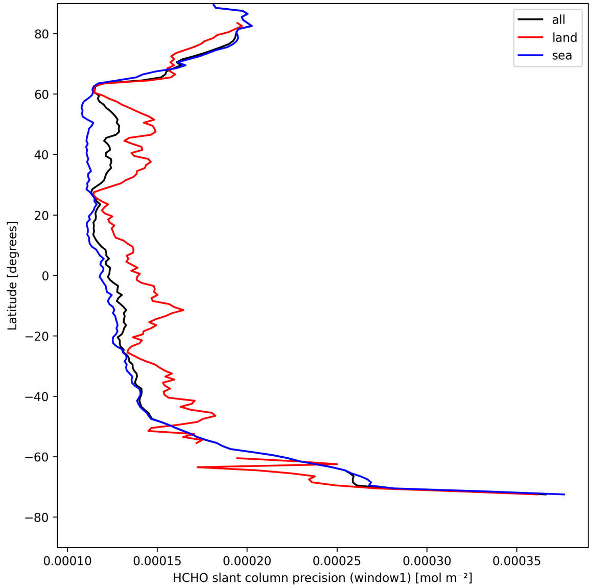
Figure 23: Zonal average of “HCHO slant column precision (window1)” for 2025-04-23 to 2025-04-24.
