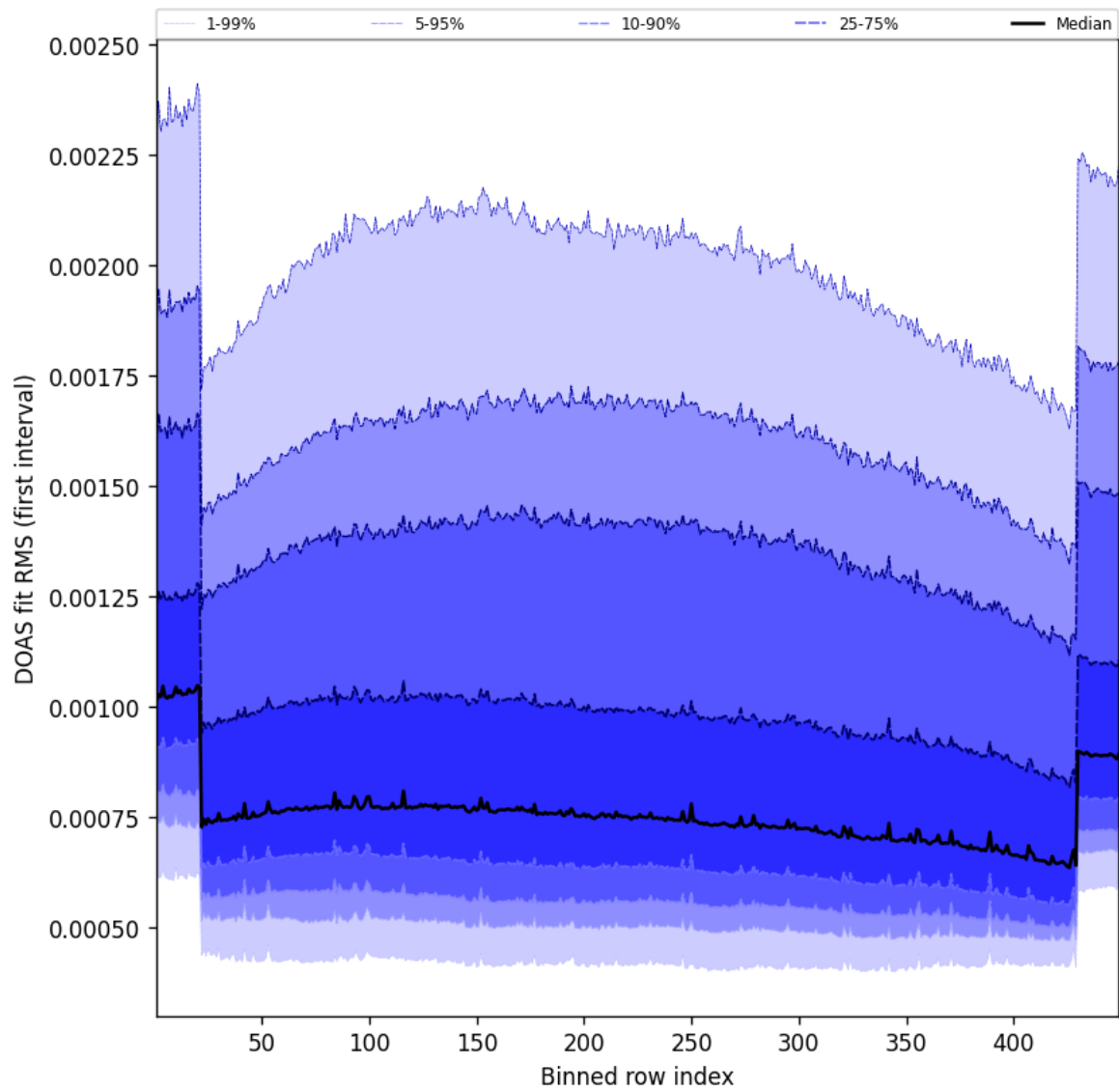
Figure 58: Along track statistics of “DOAS fit RMS (first interval)” for 2025-04-23 to 2025-04-24
