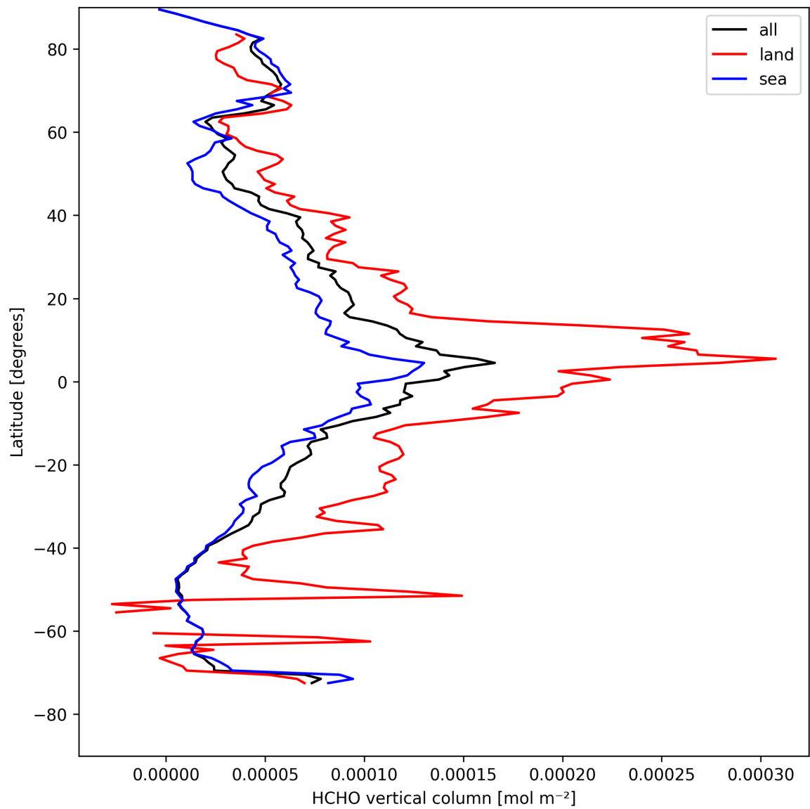
Figure 19: Zonal average of “HCHO vertical column” for 2025-04-23 to 2025-04-24.
