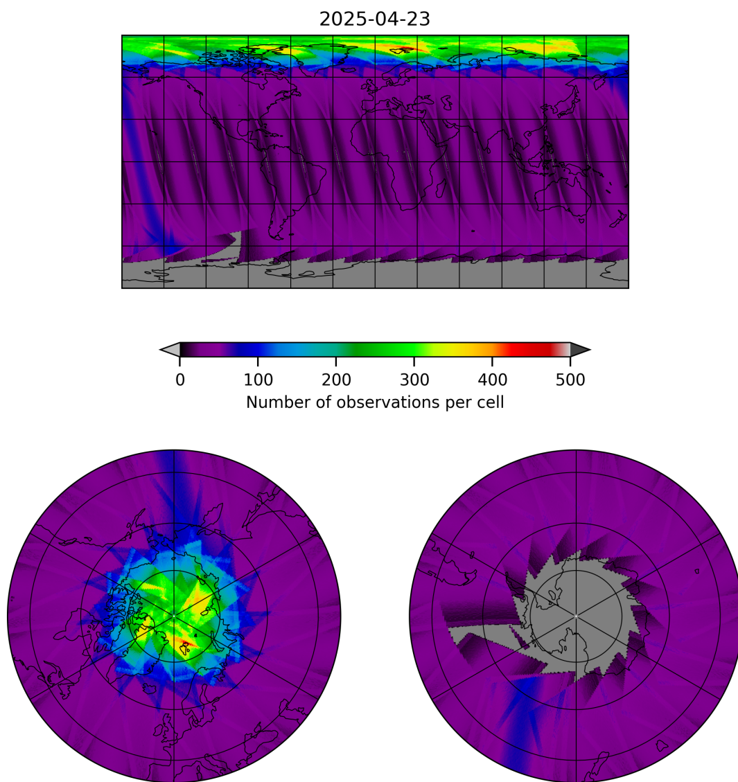
Figure 17: Map of the number of observations for 2025-04-23 to 2025-04-24
