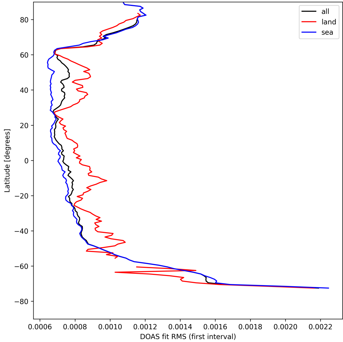
Figure 30: Zonal average of “DOAS fit RMS (first interval)” for 2025-04-23 to 2025-04-24.
