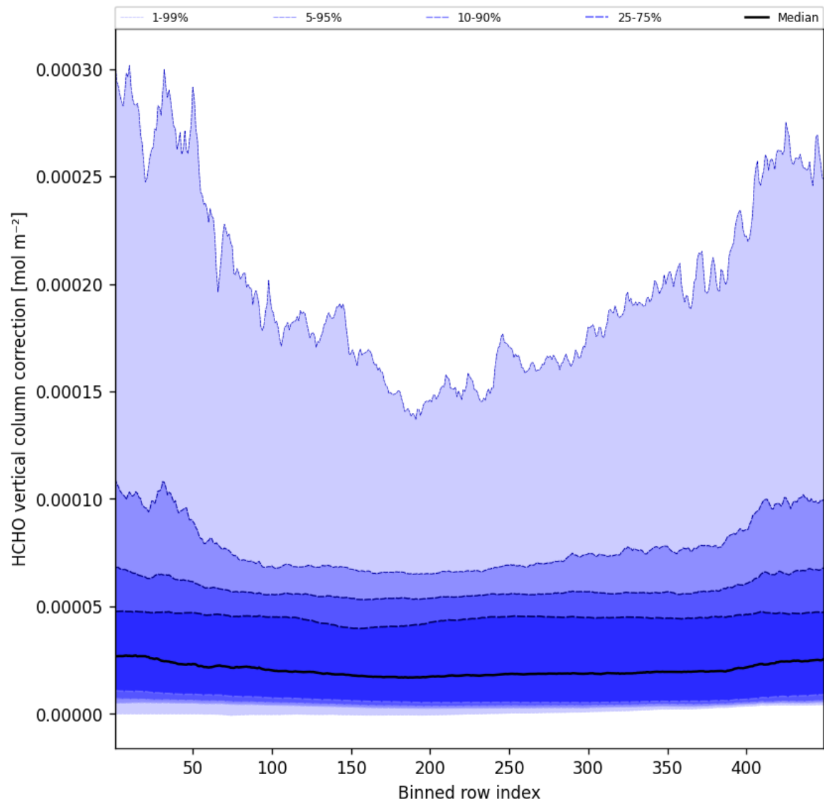
Figure 49: Along track statistics of “HCHO vertical column correction” for 2025-04-23 to 2025-04-24
