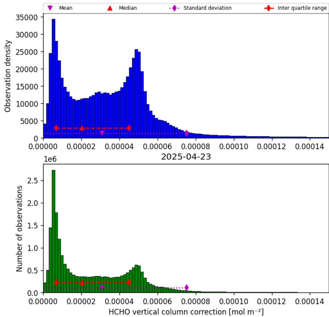
Figure 35: Histogram of “HCHO vertical column correction” for 2025-04-23 to 2025-04-24
