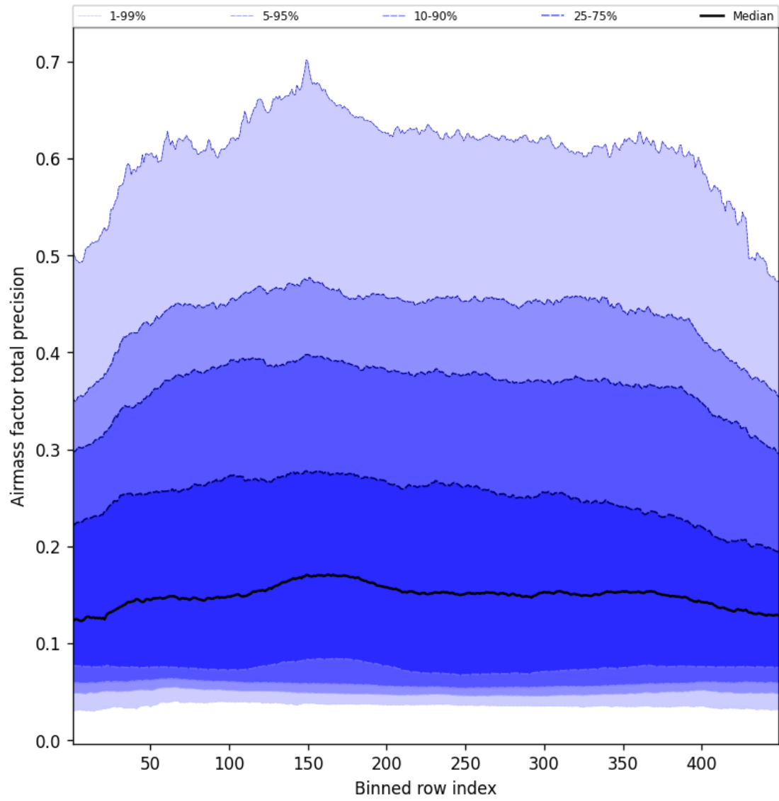
Figure 53: Along track statistics of “Airmass factor total precision” for 2025-04-23 to 2025-04-24
