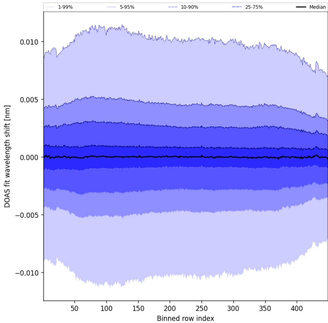
Figure 56: Along track statistics of “DOAS fit wavelength shift” for 2025-04-23 to 2025-04-24
