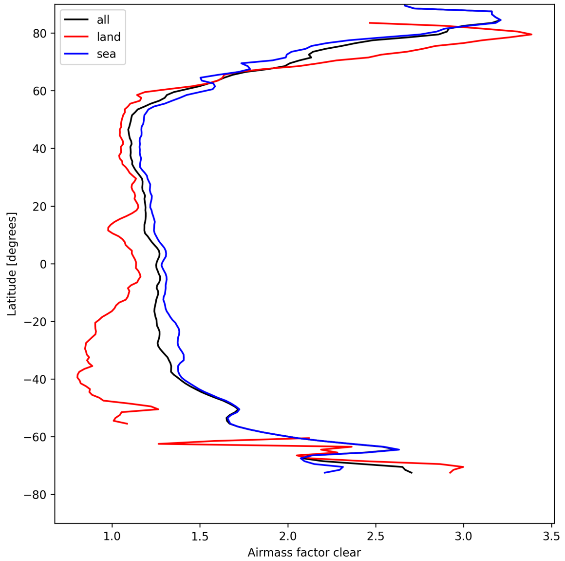
Figure 26: Zonal average of “Airmass factor clear” for 2025-04-23 to 2025-04-24.
