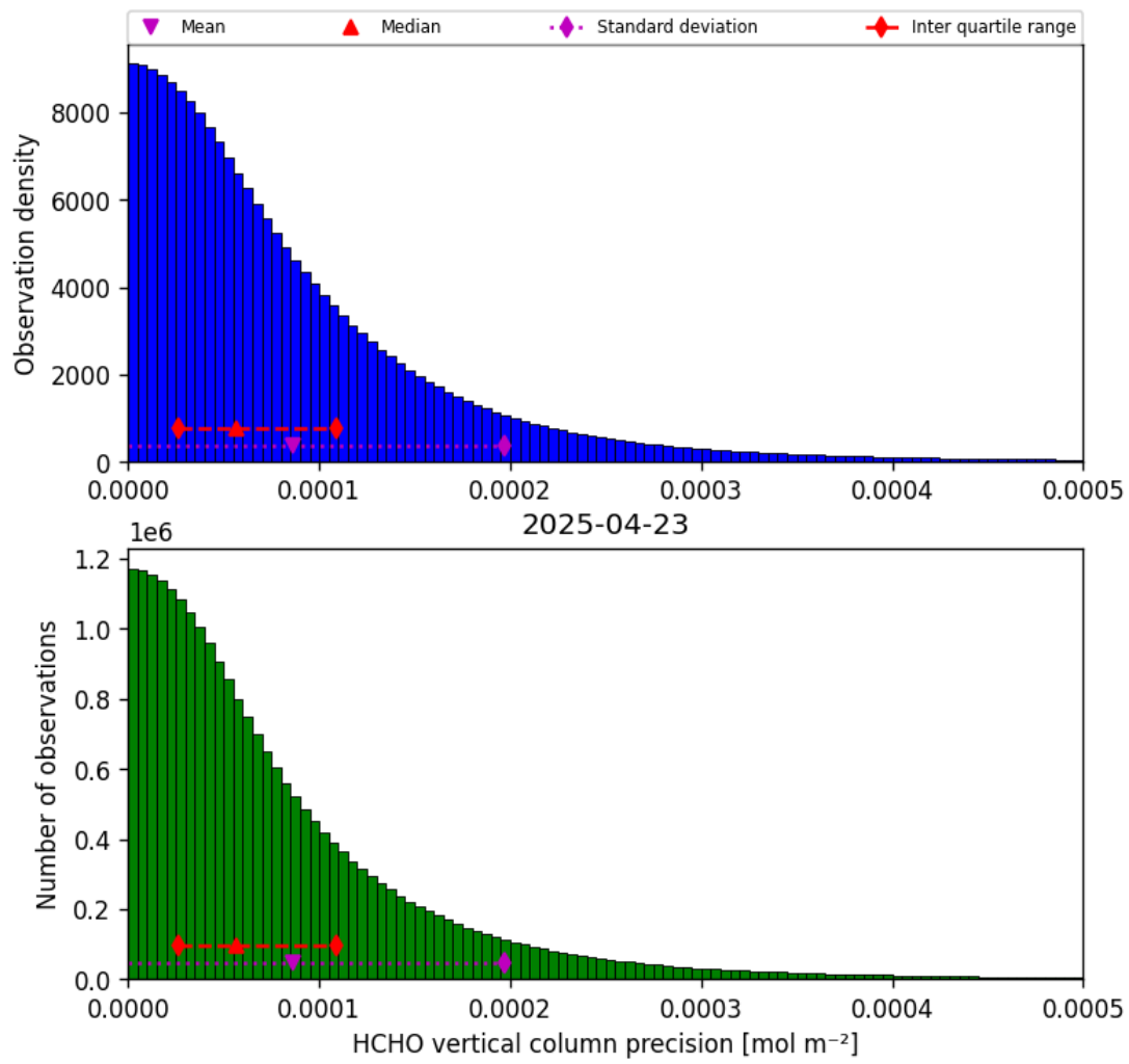
Figure 34: Histogram of “HCHO vertical column precision” for 2025-04-23 to 2025-04-24
