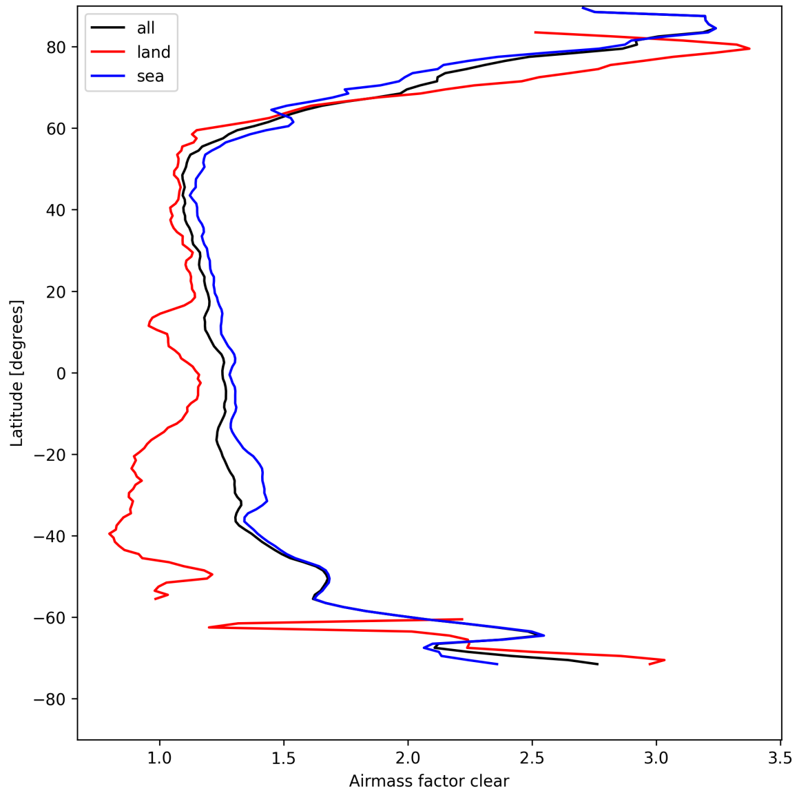
Figure 26: Zonal average of “Airmass factor clear” for 2025-04-24 to 2025-04-25.
