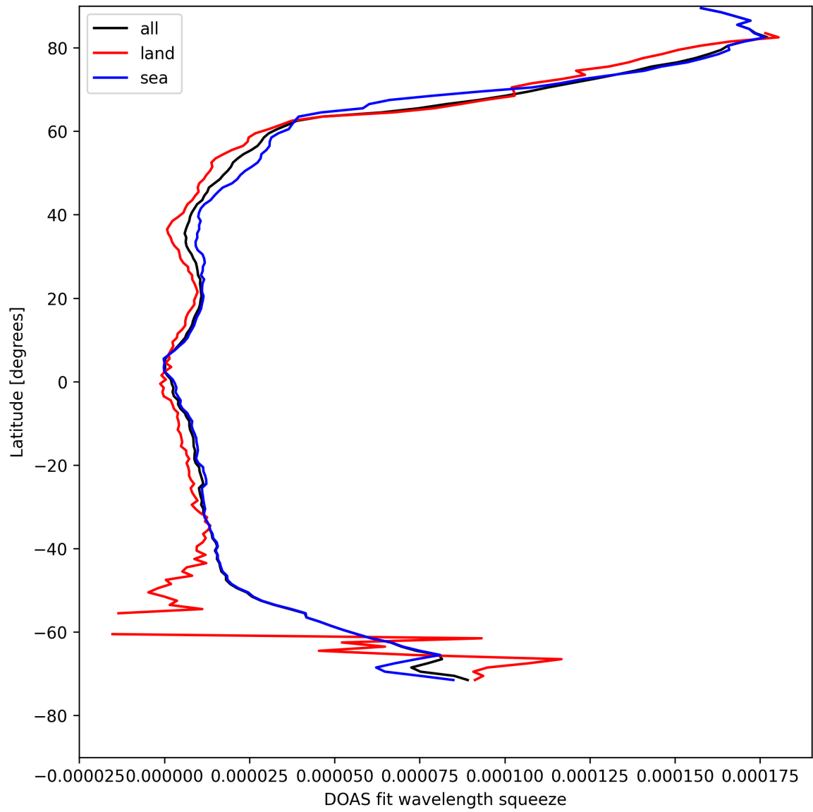
Figure 29: Zonal average of “DOAS fit wavelength squeeze” for 2025-04-24 to 2025-04-25.
