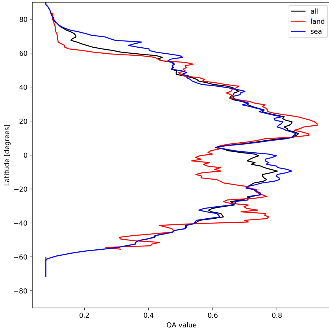
Figure 18: Zonal average of “QA value” for 2025-04-24 to 2025-04-25.
