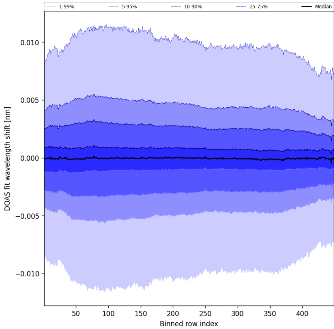
Figure 56: Along track statistics of “DOAS fit wavelength shift” for 2025-04-24 to 2025-04-25
