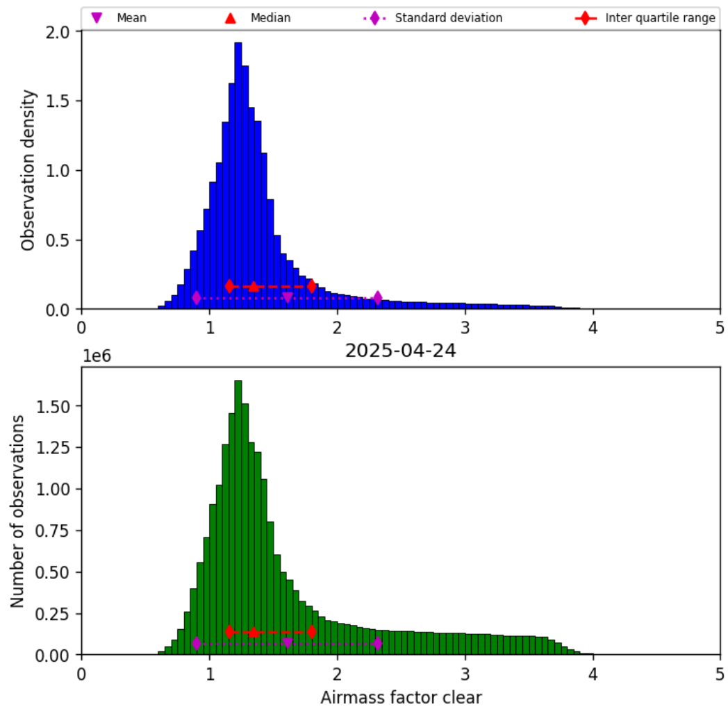
Figure 40: Histogram of “Airmass factor clear” for 2025-04-24 to 2025-04-25
