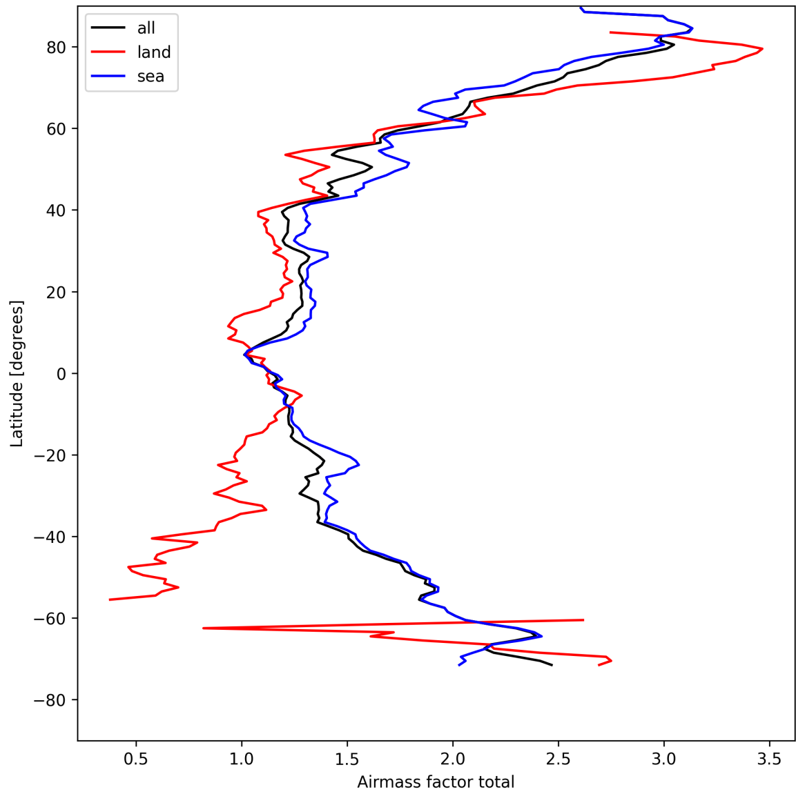
Figure 24: Zonal average of “Airmass factor total” for 2025-04-24 to 2025-04-25.
