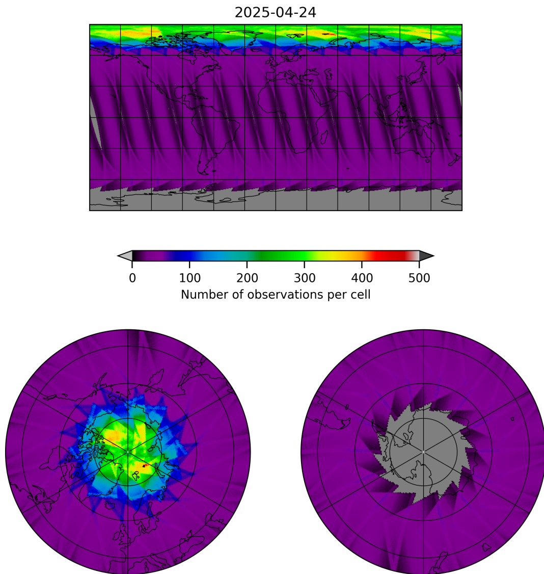
Figure 17: Map of the number of observations for 2025-04-24 to 2025-04-25
