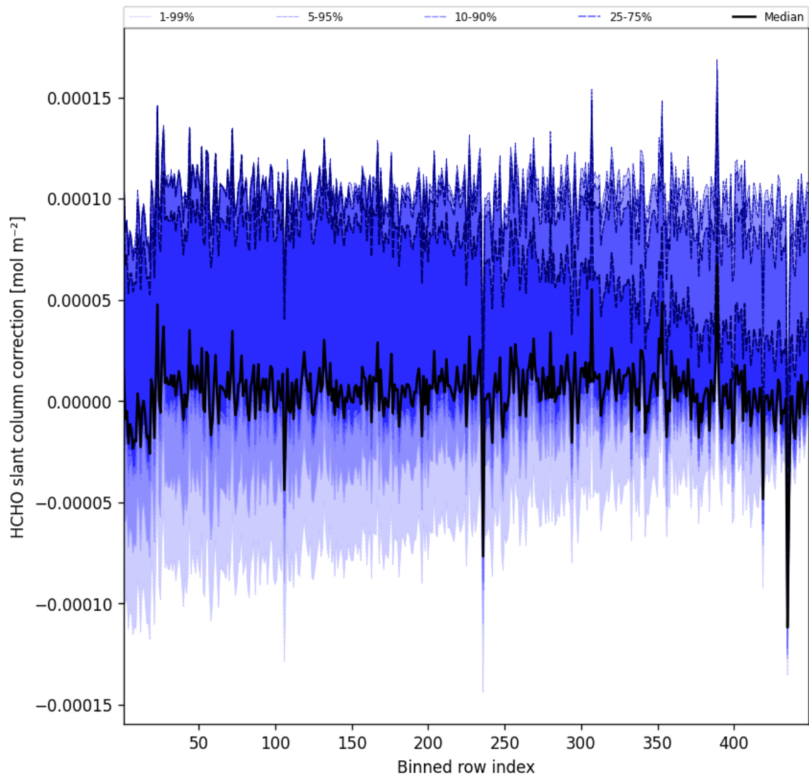
Figure 59: Along track statistics of “HCHO slant column correction” for 2025-04-24 to 2025-04-25
