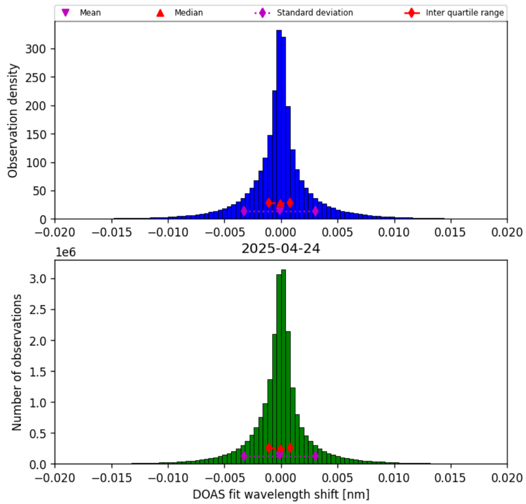
Figure 42: Histogram of “DOAS fit wavelength shift” for 2025-04-24 to 2025-04-25
