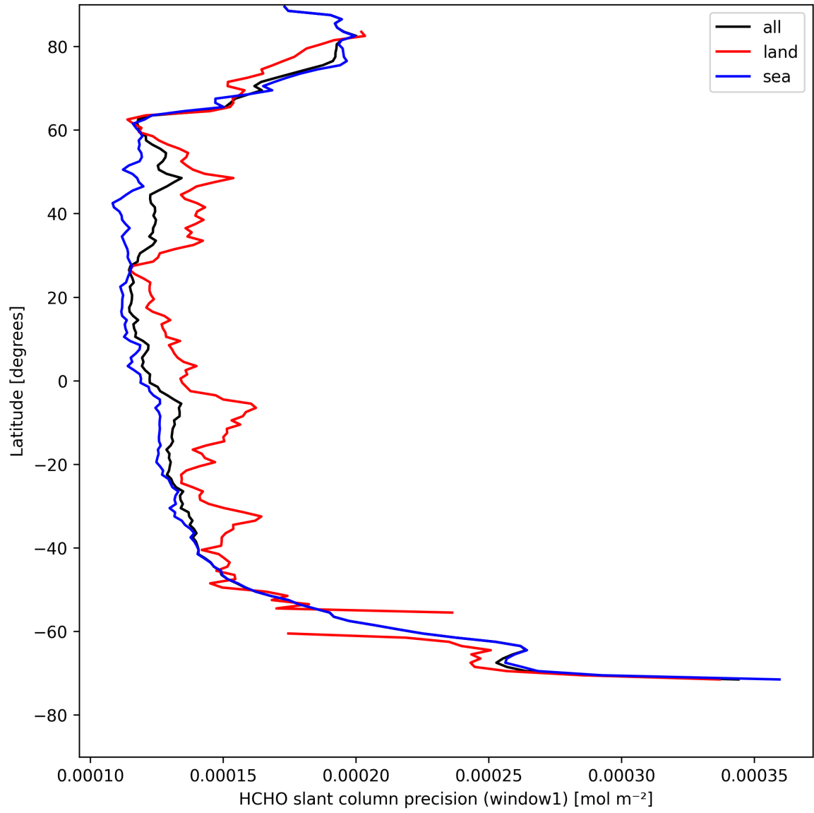
Figure 23: Zonal average of “HCHO slant column precision (window1)” for 2025-04-24 to 2025-04-25.
