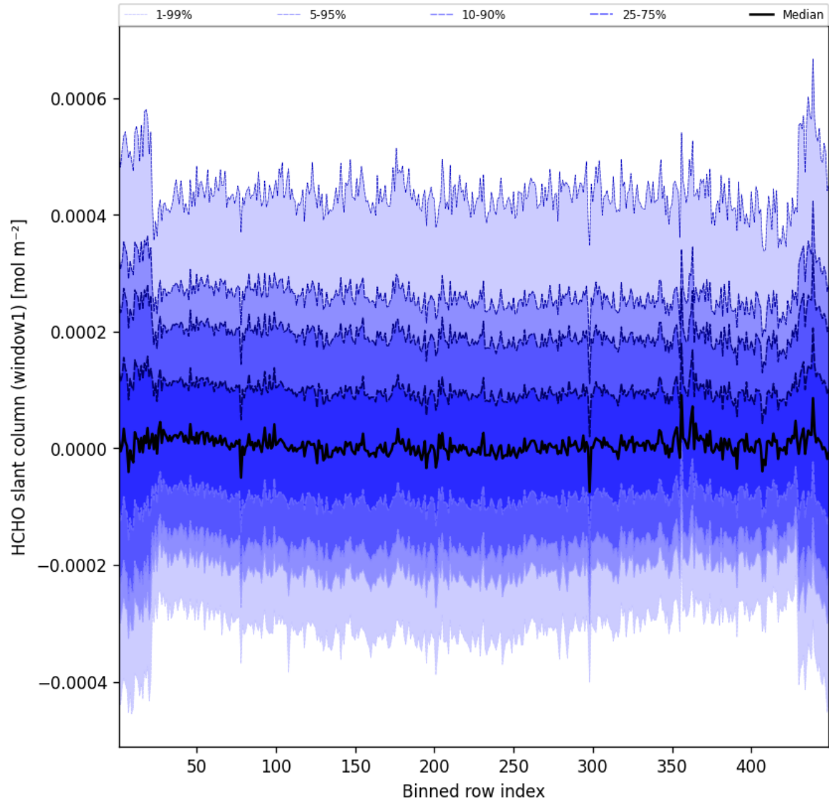
Figure 50: Along track statistics of “HCHO slant column (window1)” for 2025-04-24 to 2025-04-25
