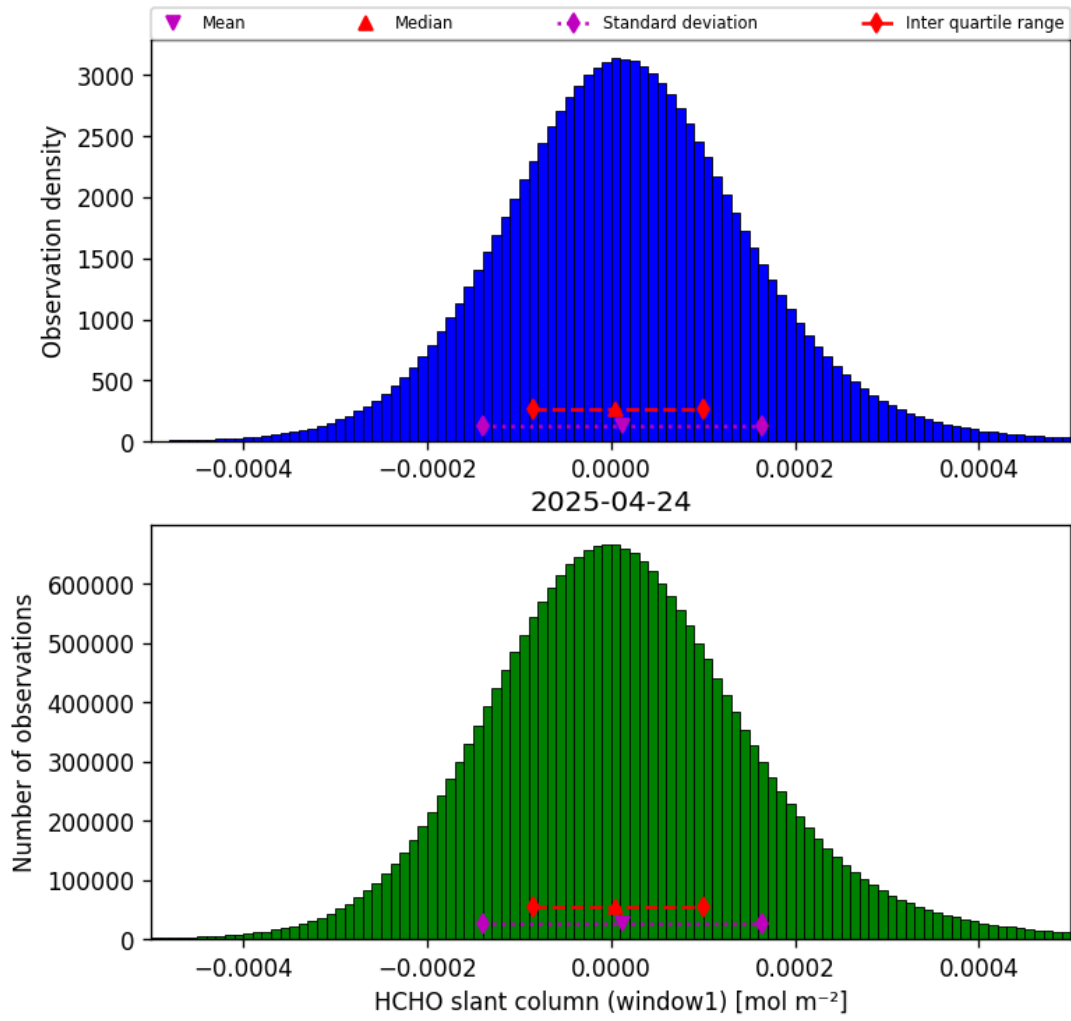
Figure 36: Histogram of “HCHO slant column (window1)” for 2025-04-24 to 2025-04-25
