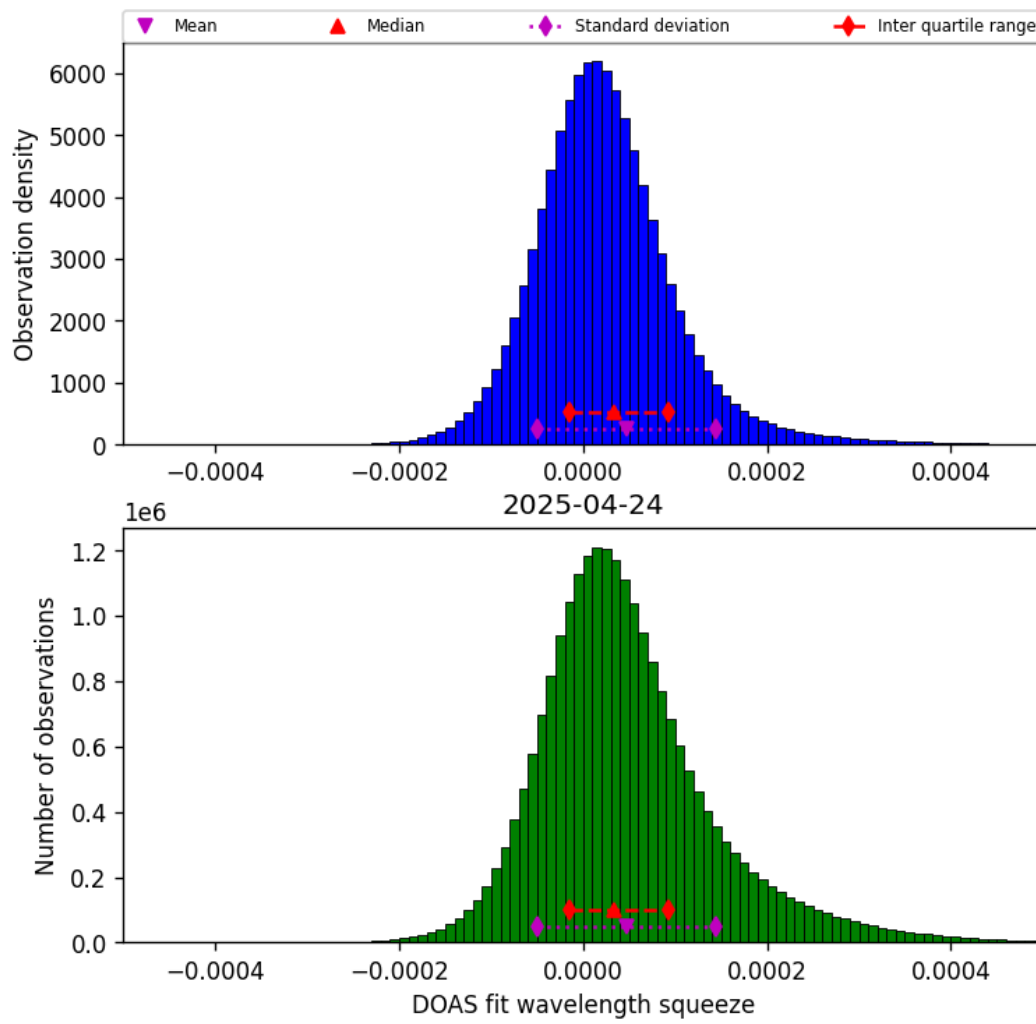
Figure 43: Histogram of “DOAS fit wavelength squeeze” for 2025-04-24 to 2025-04-25
