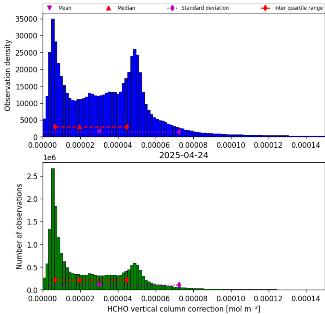
Figure 35: Histogram of “HCHO vertical column correction” for 2025-04-24 to 2025-04-25
