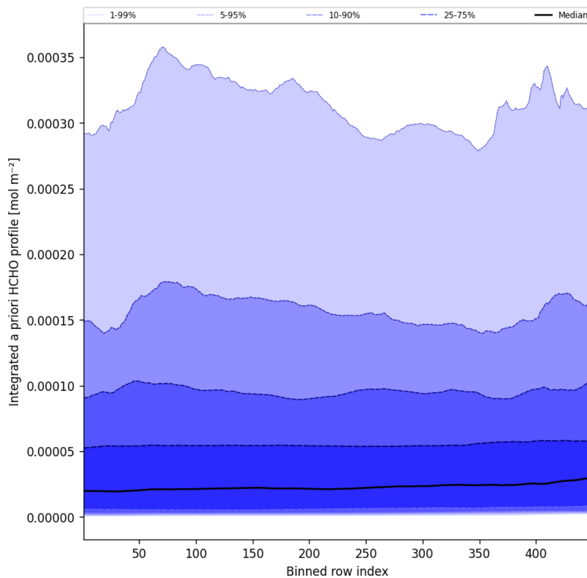
Figure 55: Along track statistics of "Integrated a priori HCHO profile" for 2025-04-24 to 2025-04-25
