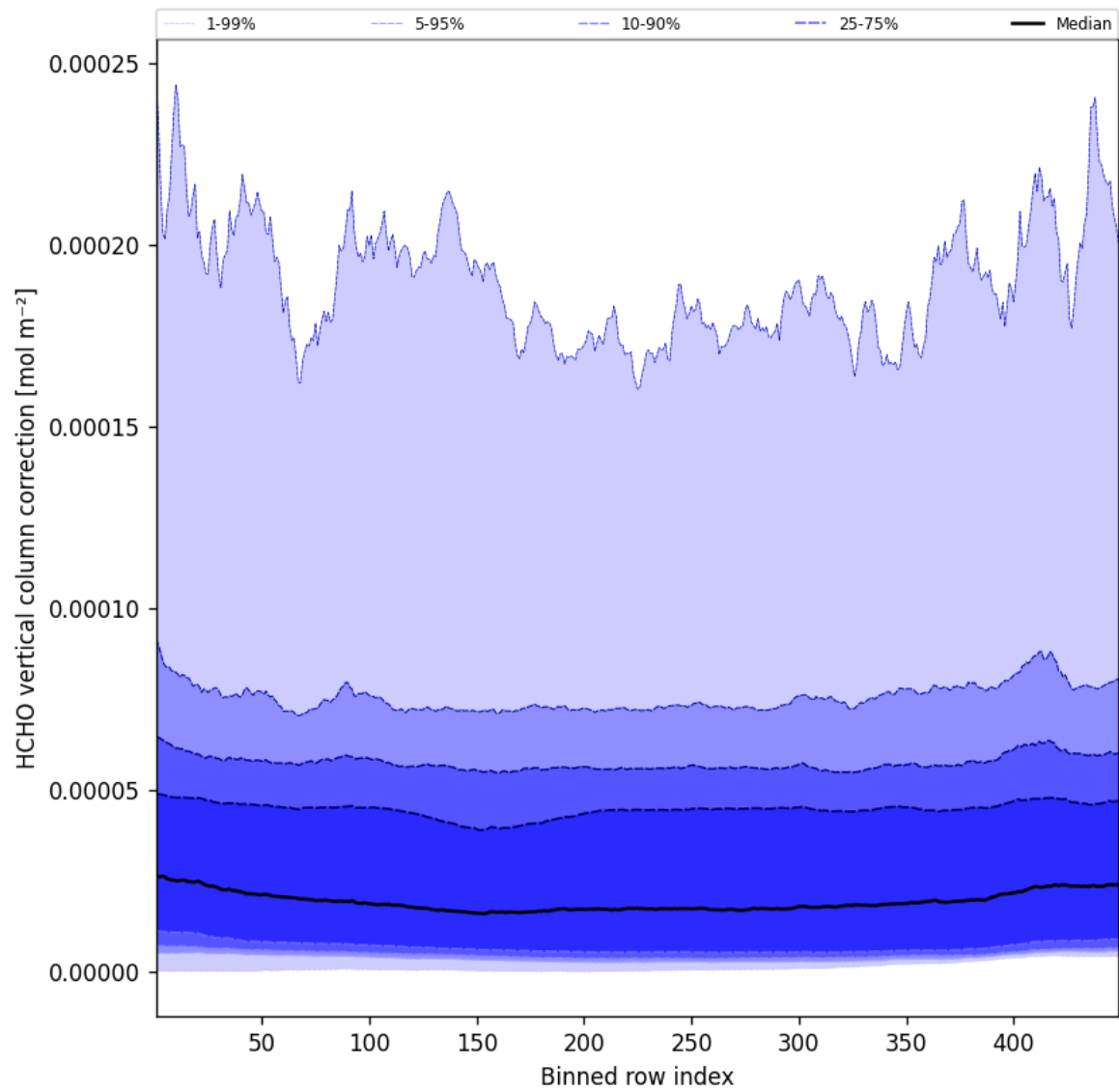
Figure 49: Along track statistics of “HCHO vertical column correction” for 2025-04-24 to 2025-04-25
