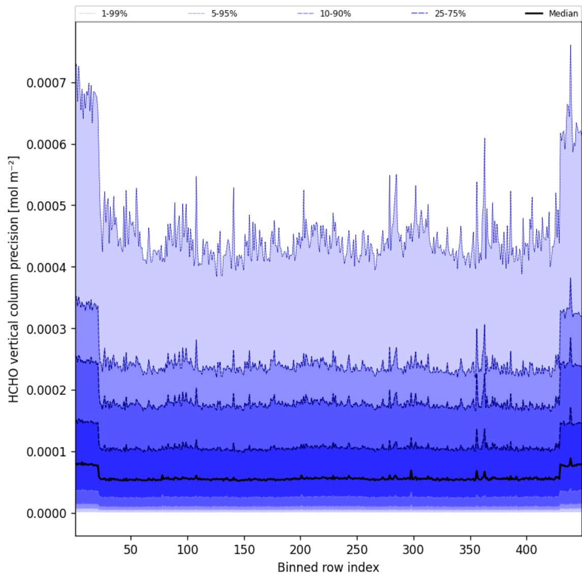
Figure 48: Along track statistics of “HCHO vertical column precision” for 2025-04-24 to 2025-04-25
