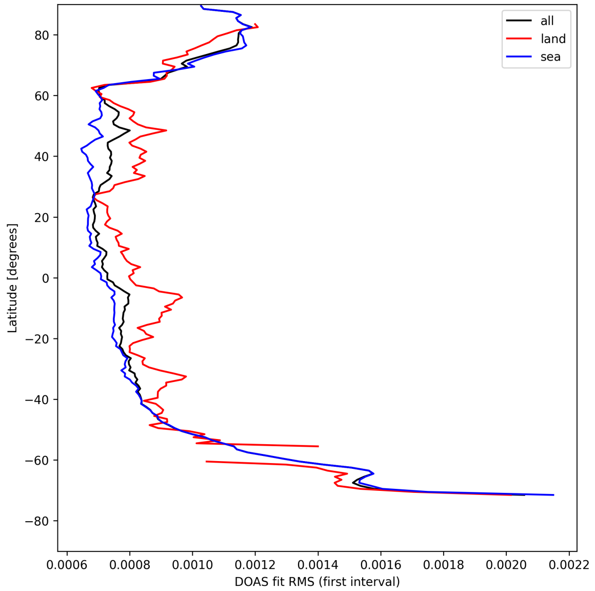
Figure 30: Zonal average of “DOAS fit RMS (first interval)” for 2025-04-24 to 2025-04-25.
