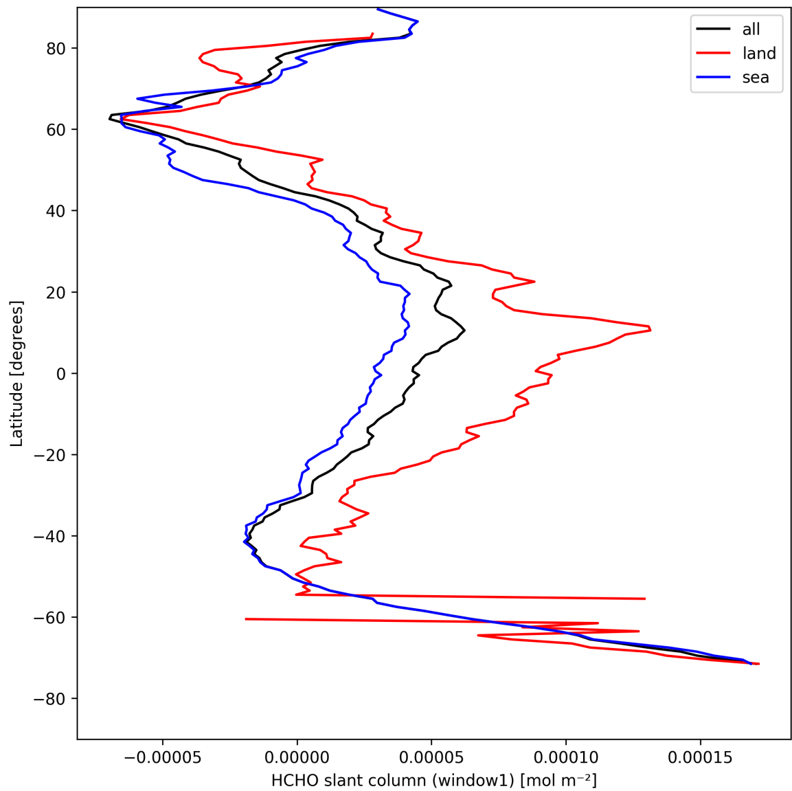
Figure 22: Zonal average of “HCHO slant column (window1)” for 2025-04-24 to 2025-04-25.
