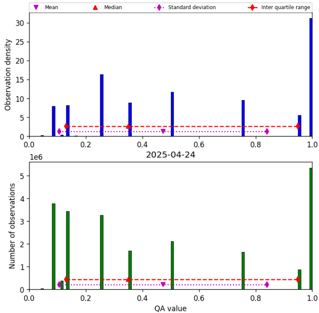
Figure 32: Histogram of “QA value” for 2025-04-24 to 2025-04-25
