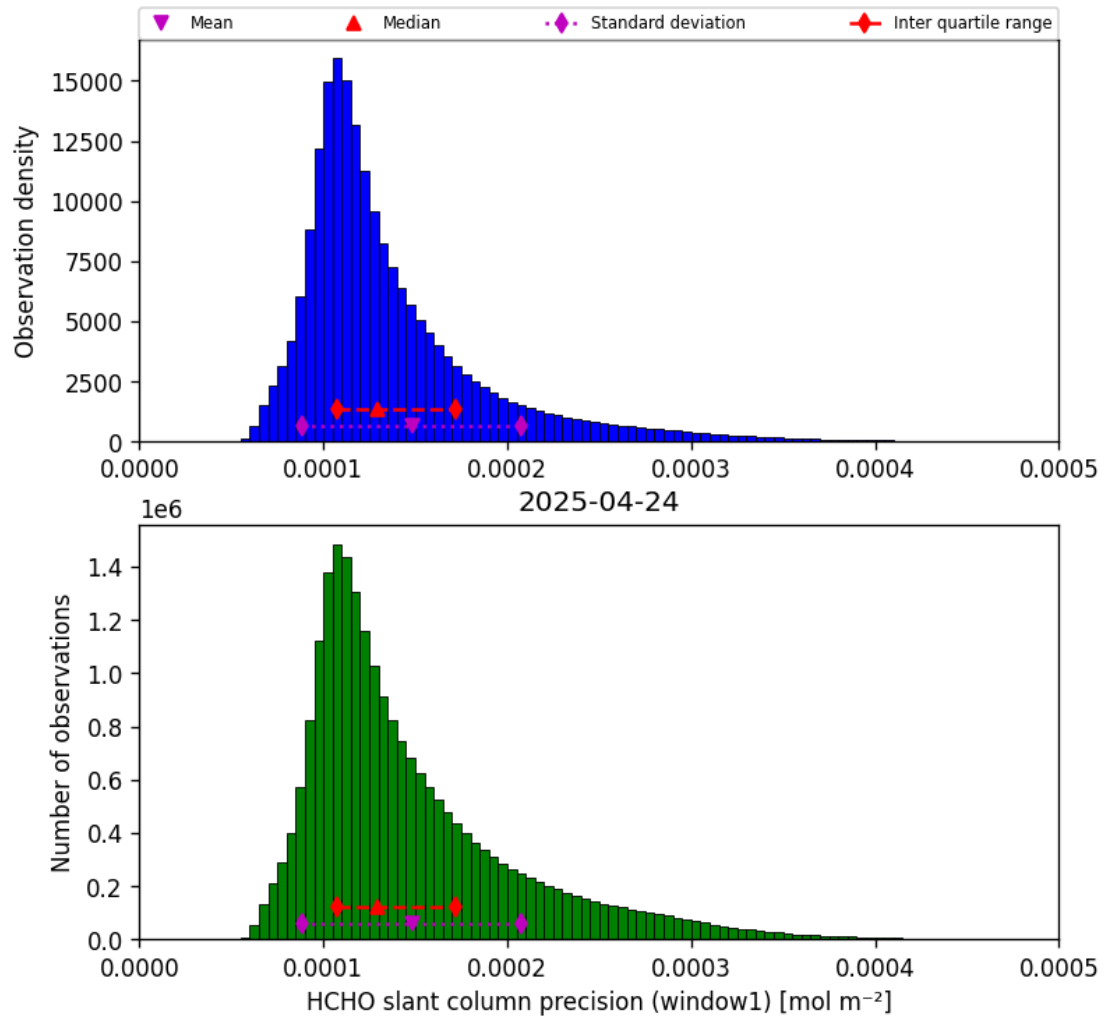
Figure 37: Histogram of “HCHO slant column precision (window1)” for 2025-04-24 to 2025-04-25
