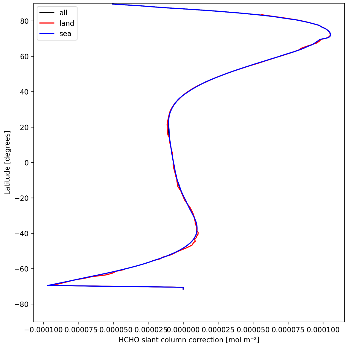
Figure 31: Zonal average of “HCHO slant column correction” for 2025-04-24 to 2025-04-25.
