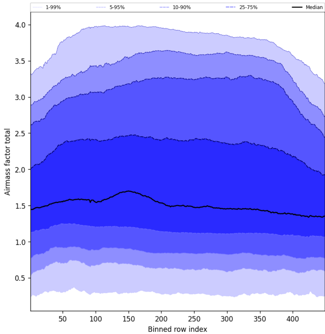
Figure 52: Along track statistics of “Airmass factor total” for 2025-04-24 to 2025-04-25
