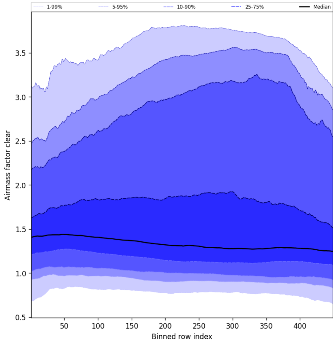
Figure 54: Along track statistics of “Airmass factor clear” for 2025-04-24 to 2025-04-25
