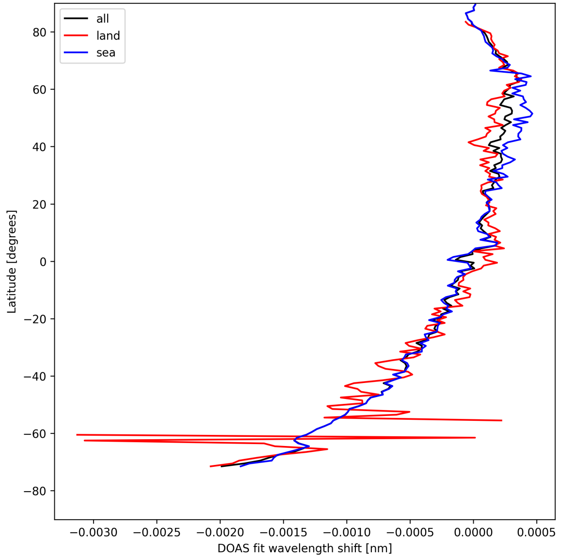
Figure 28: Zonal average of “DOAS fit wavelength shift” for 2025-04-24 to 2025-04-25.
