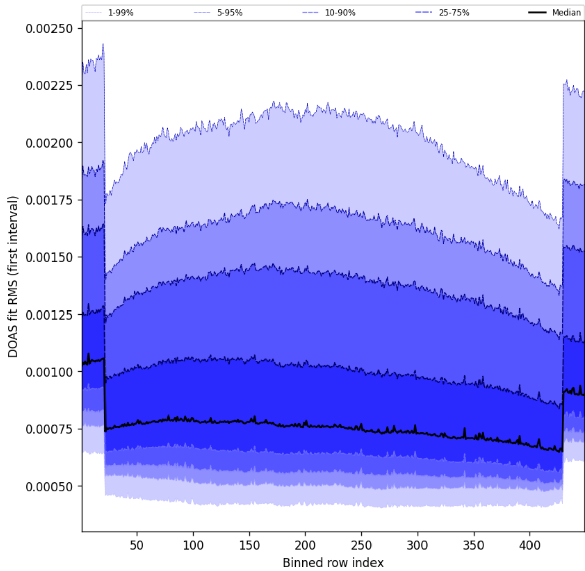
Figure 58: Along track statistics of “DOAS fit RMS (first interval)” for 2025-04-24 to 2025-04-25
