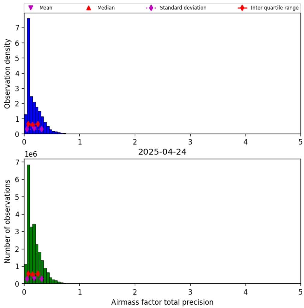
Figure 39: Histogram of “Airmass factor total precision” for 2025-04-24 to 2025-04-25
