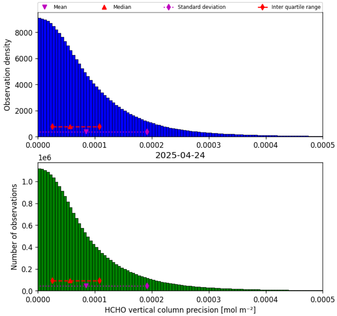
Figure 34: Histogram of “HCHO vertical column precision” for 2025-04-24 to 2025-04-25
