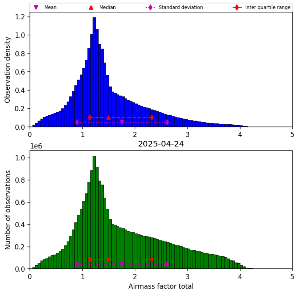
Figure 38: Histogram of “Airmass factor total” for 2025-04-24 to 2025-04-25
