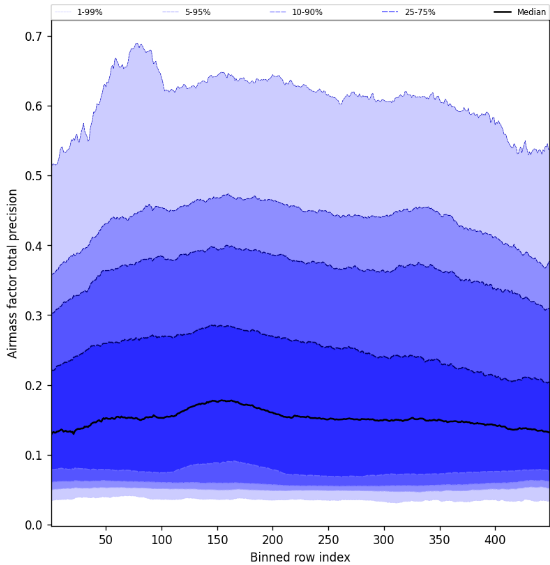
Figure 53: Along track statistics of “Airmass factor total precision” for 2025-04-24 to 2025-04-25
