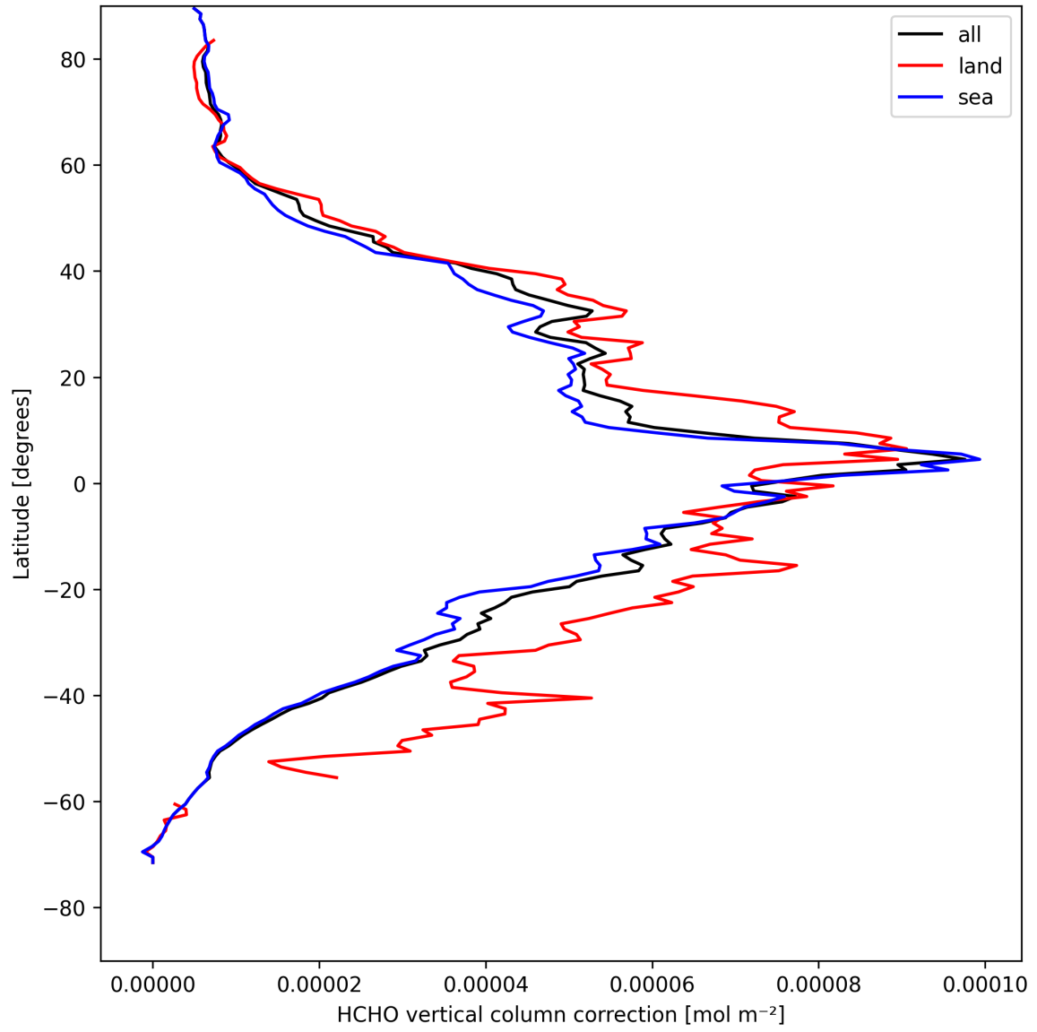
Figure 21: Zonal average of “HCHO vertical column correction” for 2025-04-24 to 2025-04-25.
