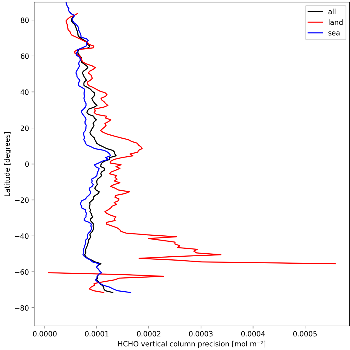
Figure 20: Zonal average of "HCHO vertical column precision" for 2025-04-24 to 2025-04-25.
