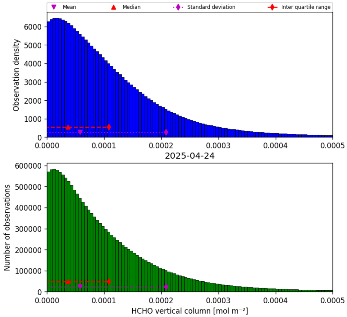
Figure 33: Histogram of “HCHO vertical column” for 2025-04-24 to 2025-04-25
