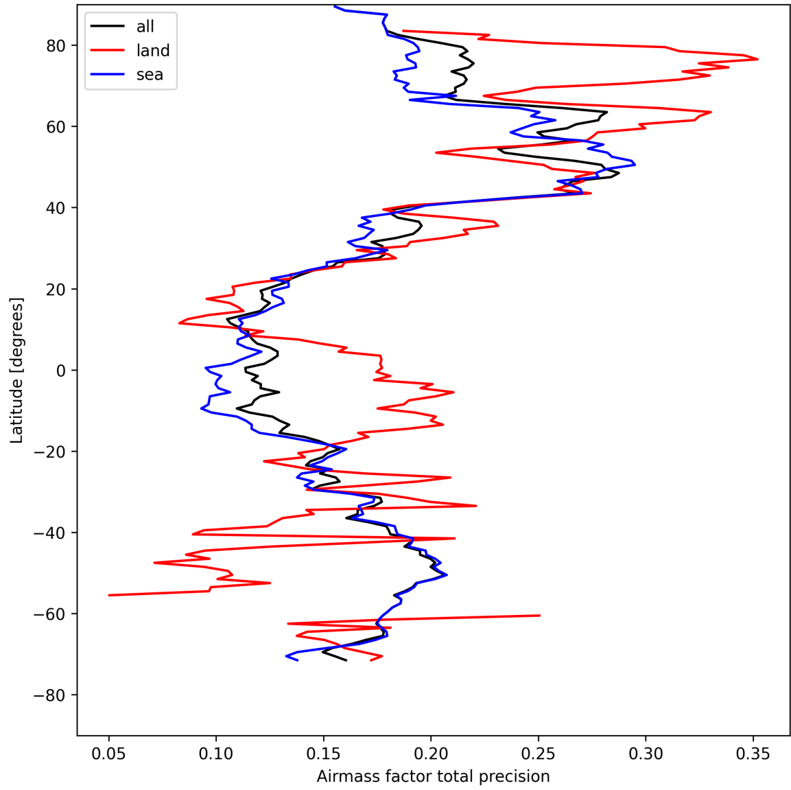
Figure 25: Zonal average of “Airmass factor total precision” for 2025-04-24 to 2025-04-25.
