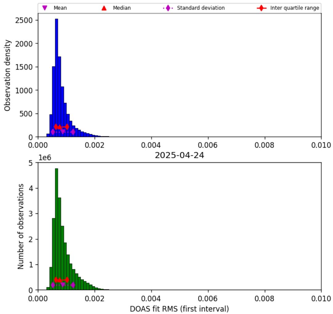
Figure 44: Histogram of “DOAS fit RMS (first interval)” for 2025-04-24 to 2025-04-25
