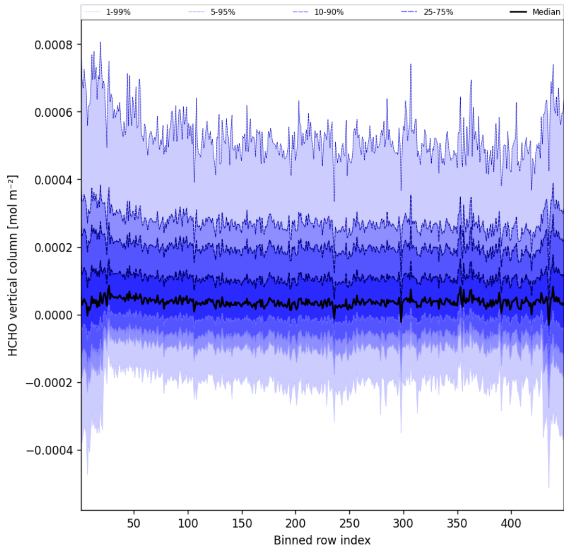
Figure 47: Along track statistics of “HCHO vertical column” for 2025-04-24 to 2025-04-25
