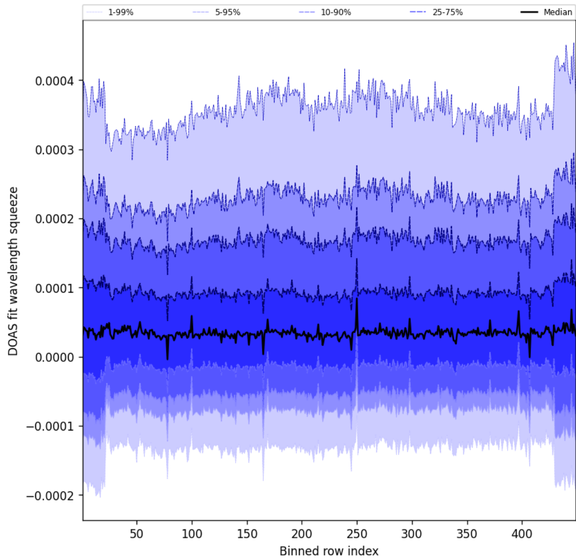
Figure 57: Along track statistics of “DOAS fit wavelength squeeze” for 2025-04-24 to 2025-04-25
