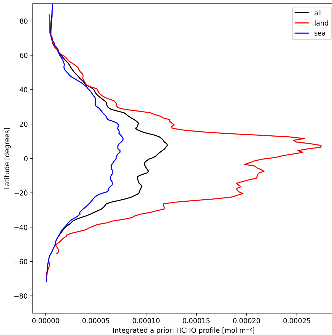
Figure 27: Zonal average of “Integrated a priori HCHO profile” for 2025-04-24 to 2025-04-25.
