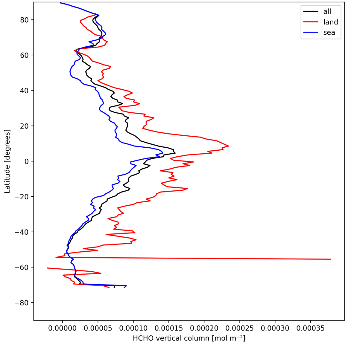
Figure 19: Zonal average of “HCHO vertical column” for 2025-04-24 to 2025-04-25.
