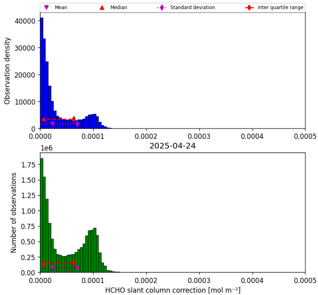
Figure 45: Histogram of “HCHO slant column correction” for 2025-04-24 to 2025-04-25
