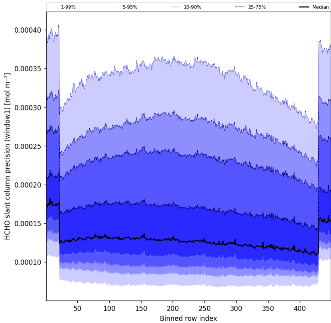
Figure 51: Along track statistics of “HCHO slant column precision (window1)” for 2025-04-24 to 2025-04-25
