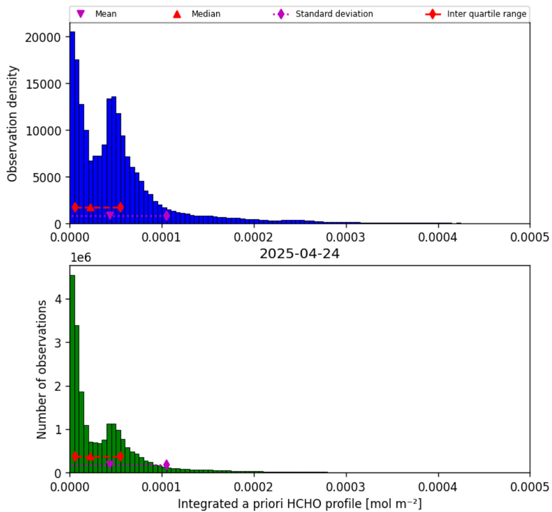
Figure 41: Histogram of “Integrated a priori HCHO profile” for 2025-04-24 to 2025-04-25
