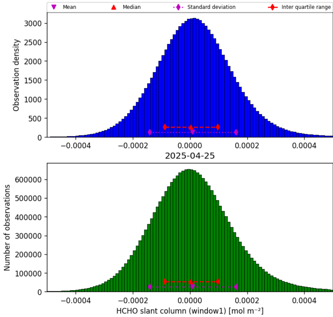
Figure 36: Histogram of “HCHO slant column (window1)” for 2025-04-25 to 2025-04-26
