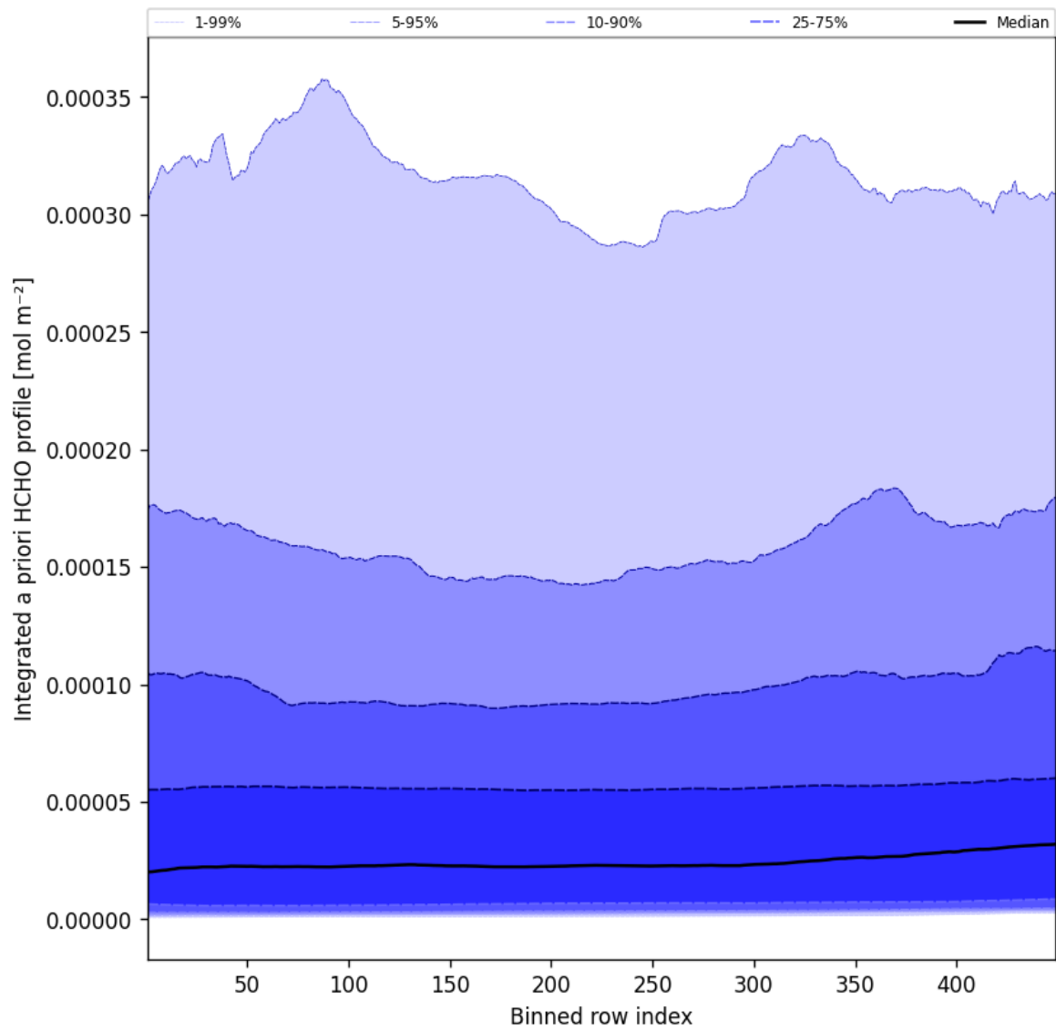
Figure 55: Along track statistics of “Integrated a priori HCHO profile” for 2025-04-25 to 2025-04-26
