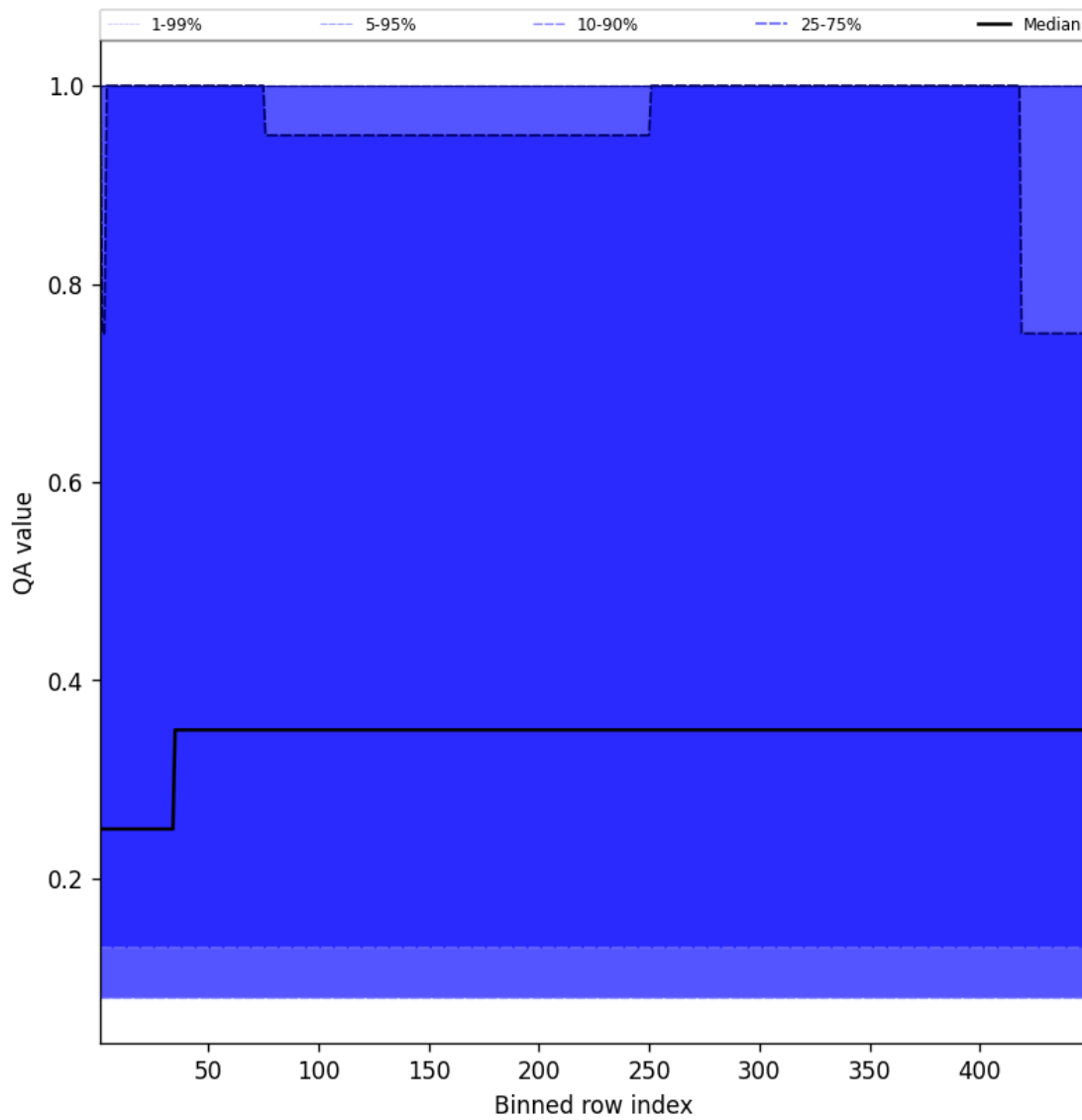
Figure 46: Along track statistics of “QA value” for 2025-04-25 to 2025-04-26
