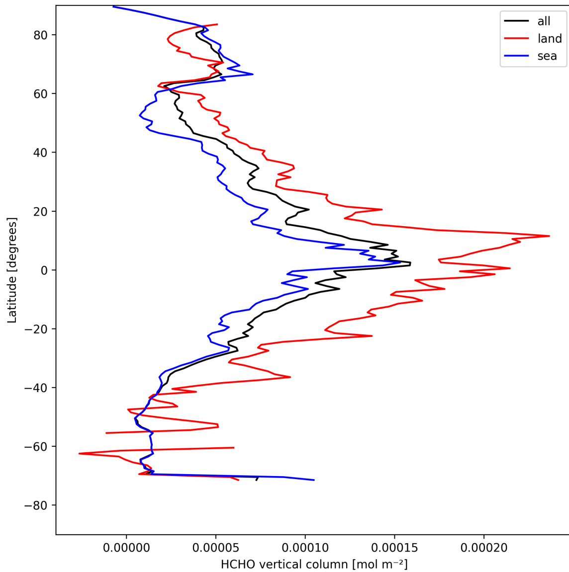
Figure 19: Zonal average of “HCHO vertical column” for 2025-04-25 to 2025-04-26.
