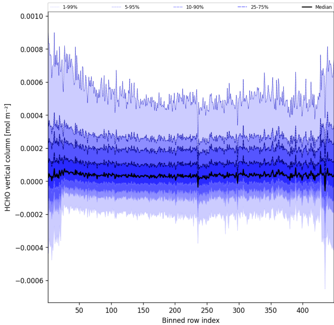
Figure 47: Along track statistics of “HCHO vertical column” for 2025-04-25 to 2025-04-26
