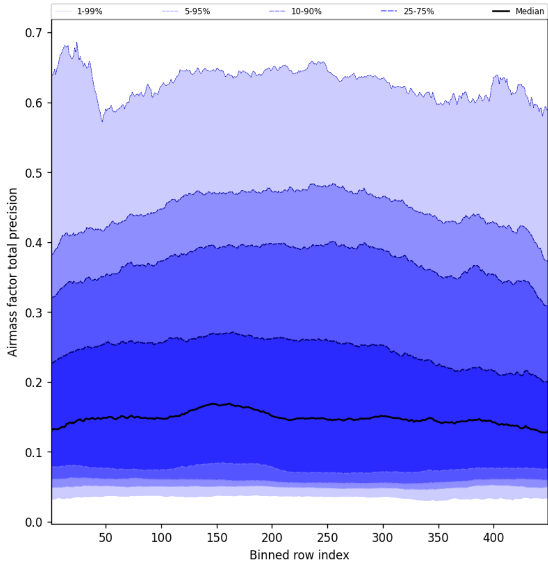
Figure 53: Along track statistics of “Airmass factor total precision” for 2025-04-25 to 2025-04-26
