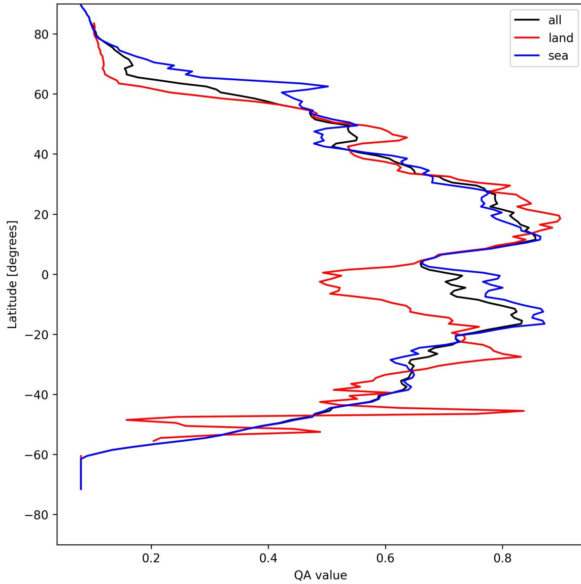
Figure 18: Zonal average of “QA value” for 2025-04-25 to 2025-04-26.
