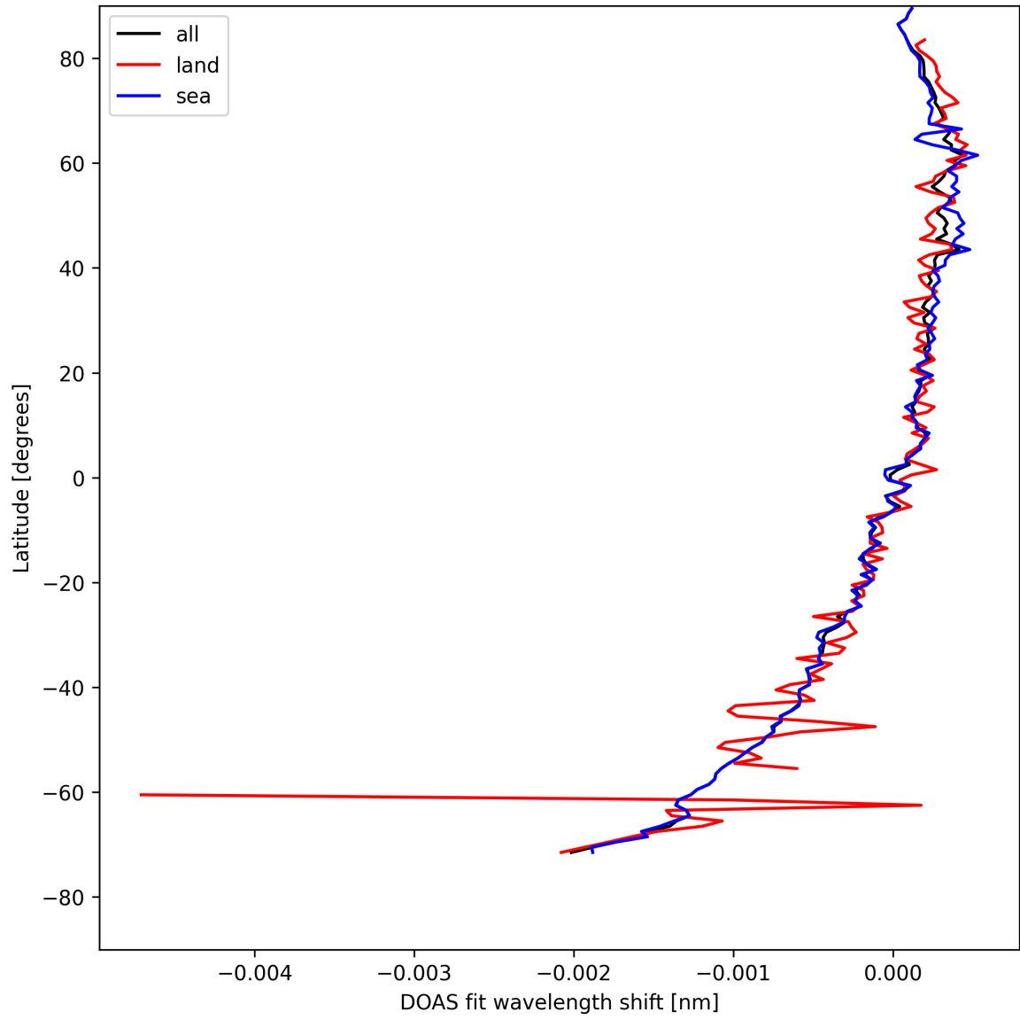
Figure 28: Zonal average of “DOAS fit wavelength shift” for 2025-04-25 to 2025-04-26.
