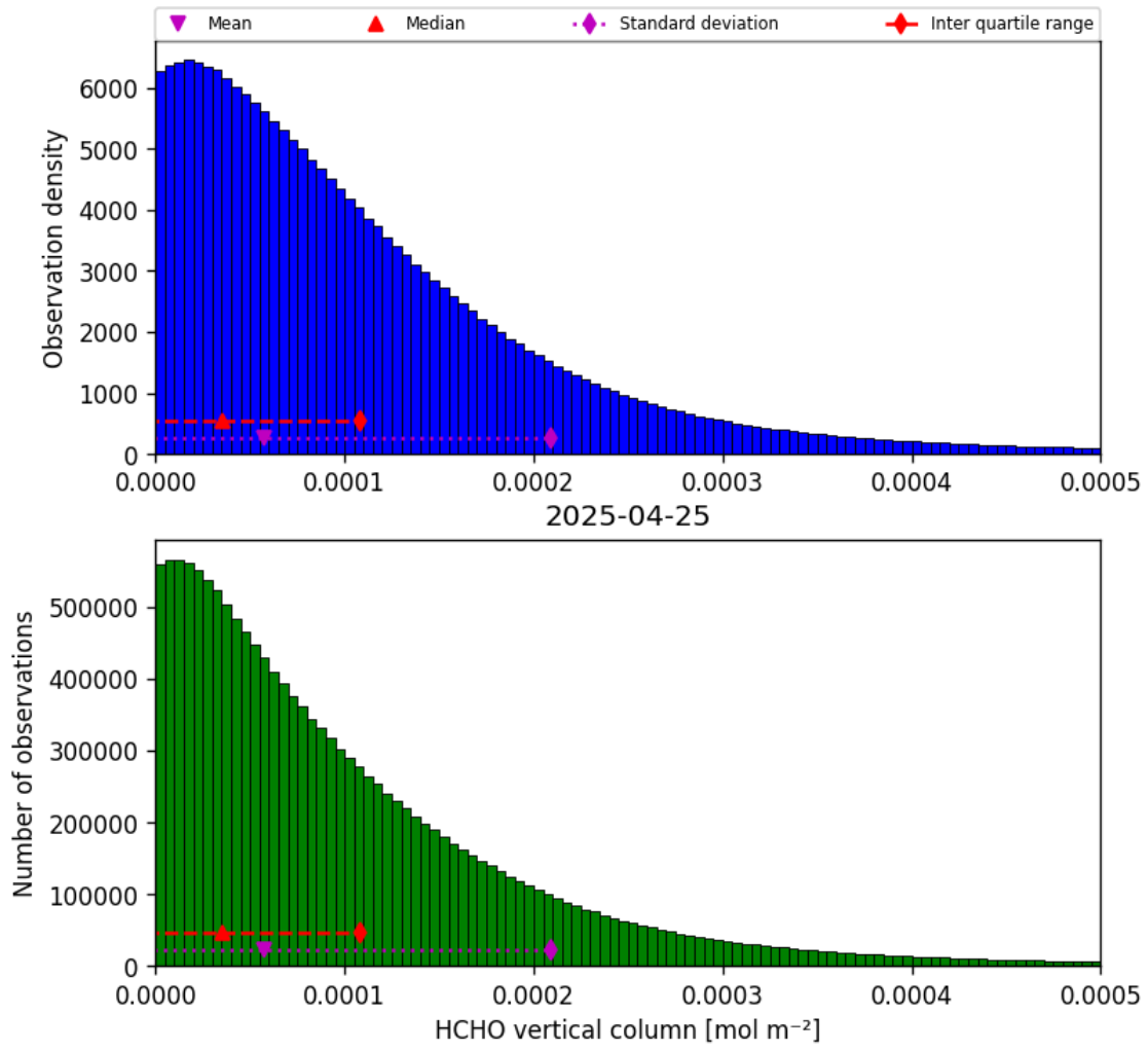
Figure 33: Histogram of “HCHO vertical column” for 2025-04-25 to 2025-04-26
