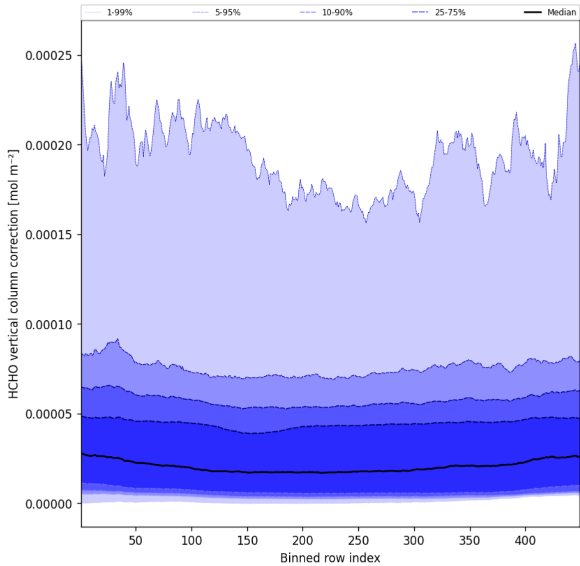
Figure 49: Along track statistics of “HCHO vertical column correction” for 2025-04-25 to 2025-04-26
