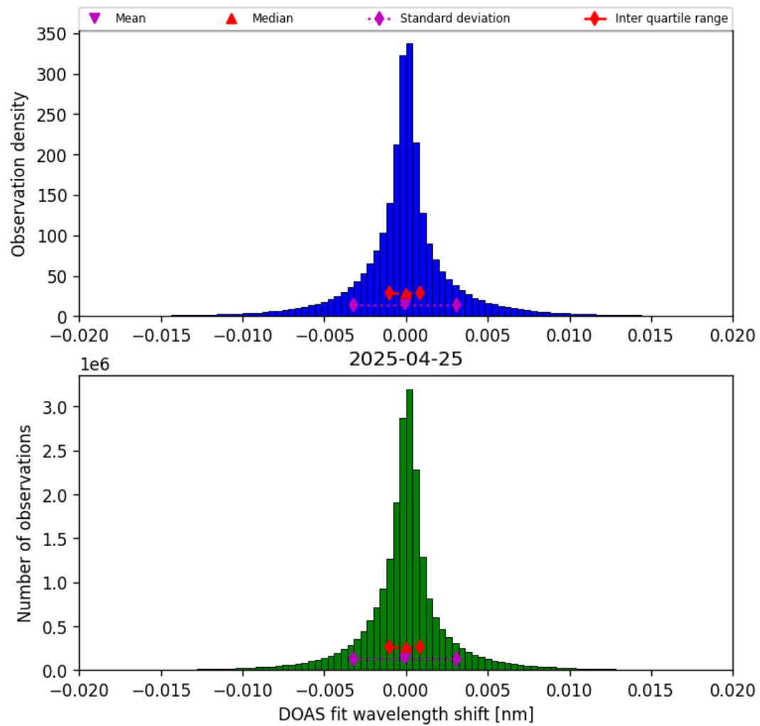
Figure 42: Histogram of “DOAS fit wavelength shift” for 2025-04-25 to 2025-04-26
