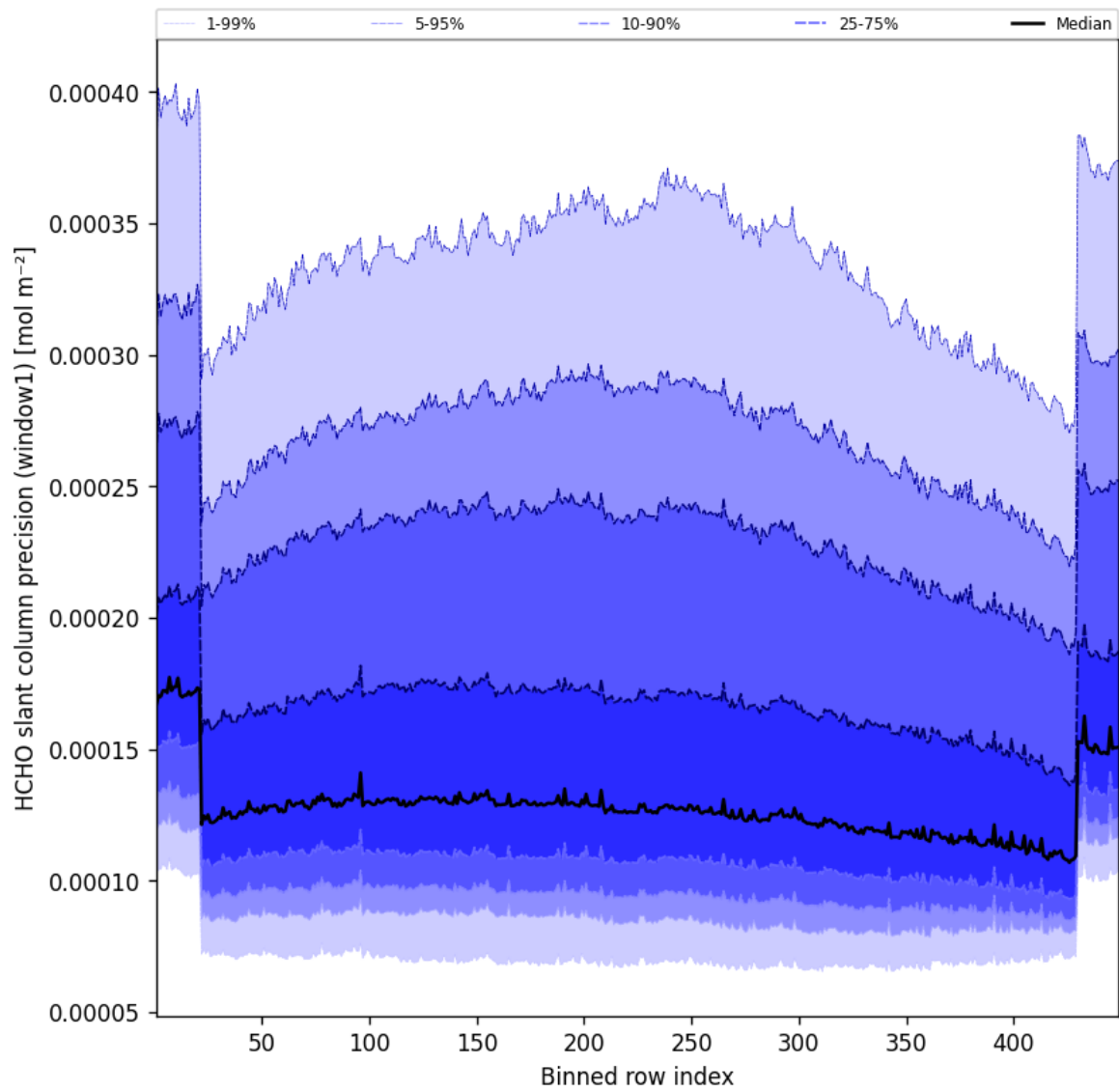
Figure 51: Along track statistics of “HCHO slant column precision (window1)” for 2025-04-25 to 2025-04-26
