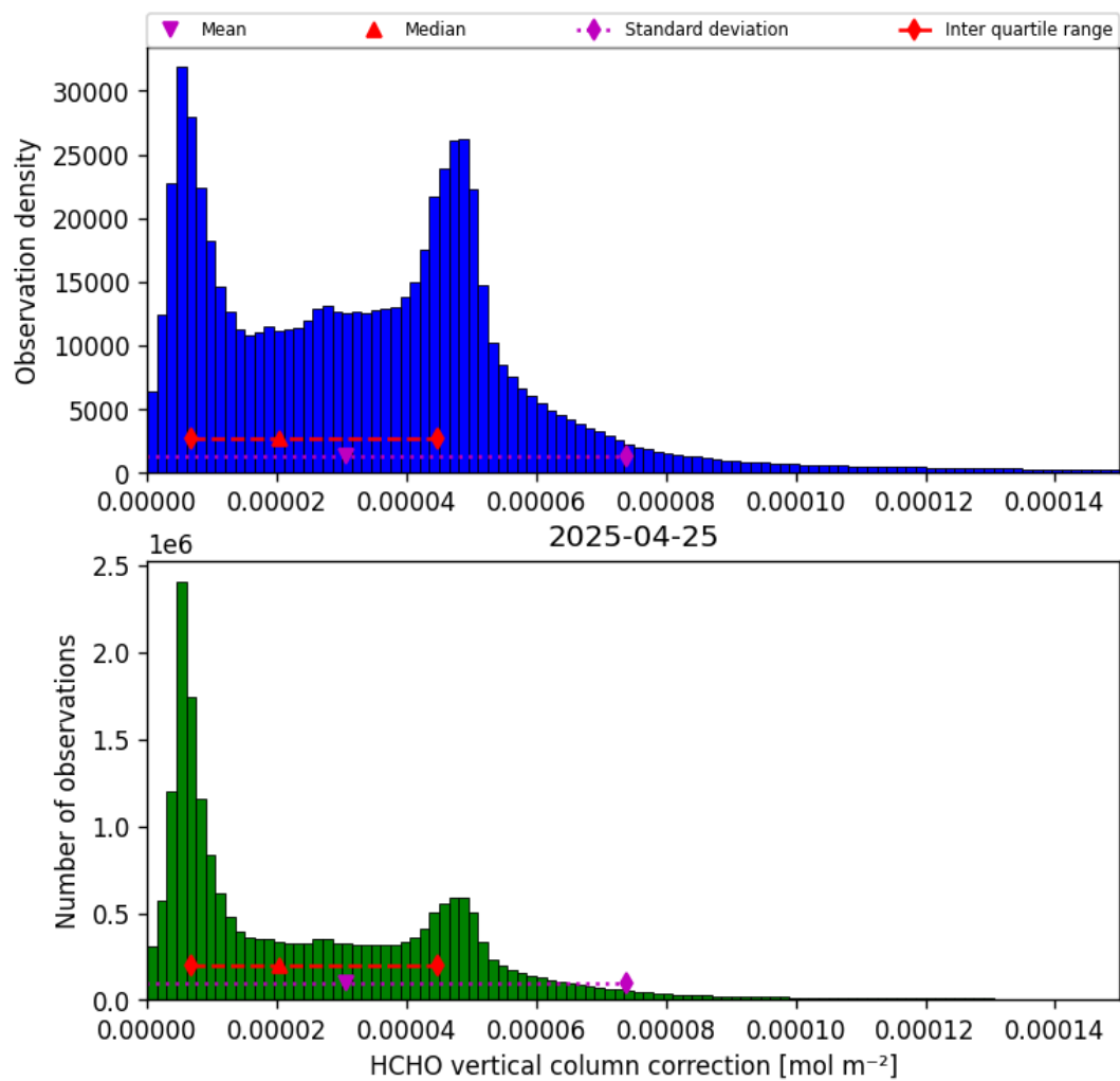
Figure 35: Histogram of “HCHO vertical column correction” for 2025-04-25 to 2025-04-26
