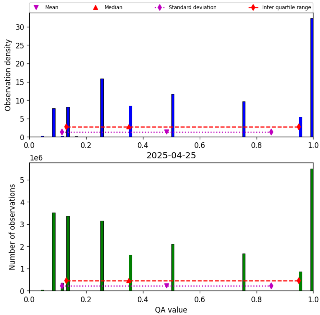
Figure 32: Histogram of “QA value” for 2025-04-25 to 2025-04-26
