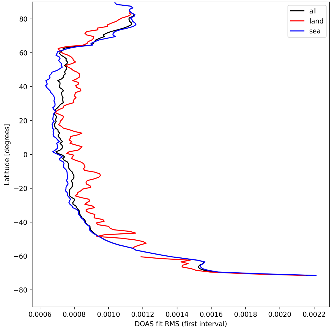
Figure 30: Zonal average of “DOAS fit RMS (first interval)” for 2025-04-25 to 2025-04-26.
