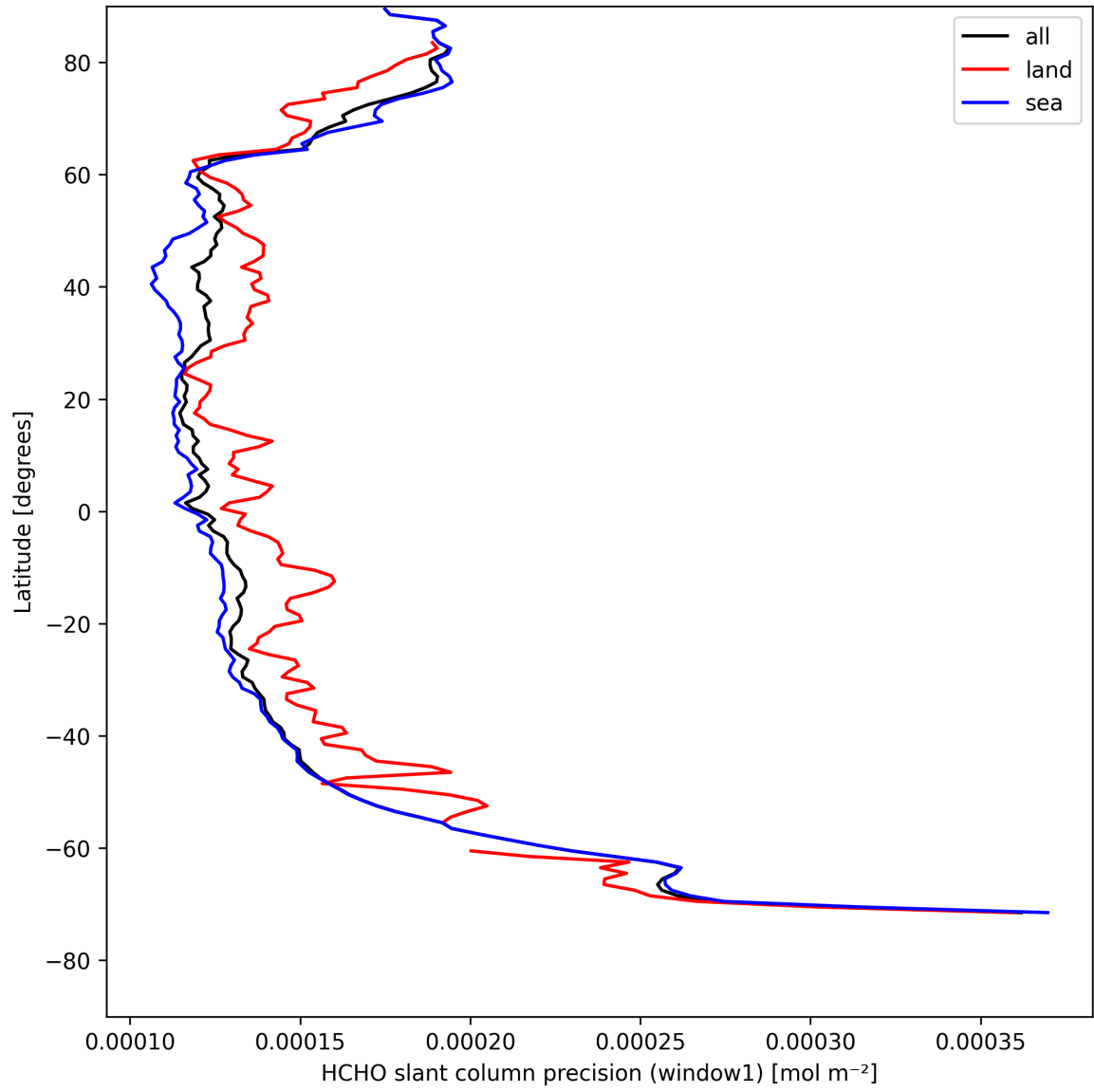
Figure 23: Zonal average of “HCHO slant column precision (window1)” for 2025-04-25 to 2025-04-26.
