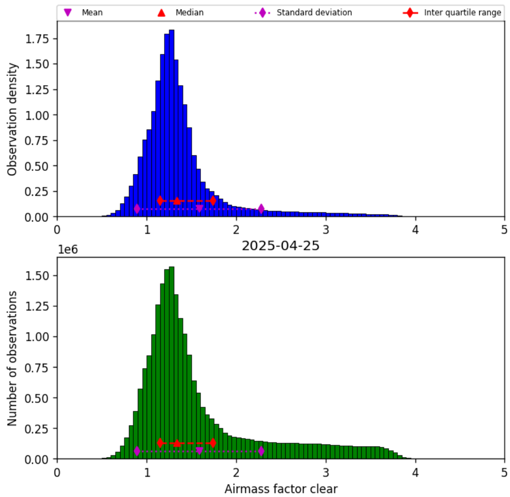
Figure 40: Histogram of “Airmass factor clear” for 2025-04-25 to 2025-04-26
