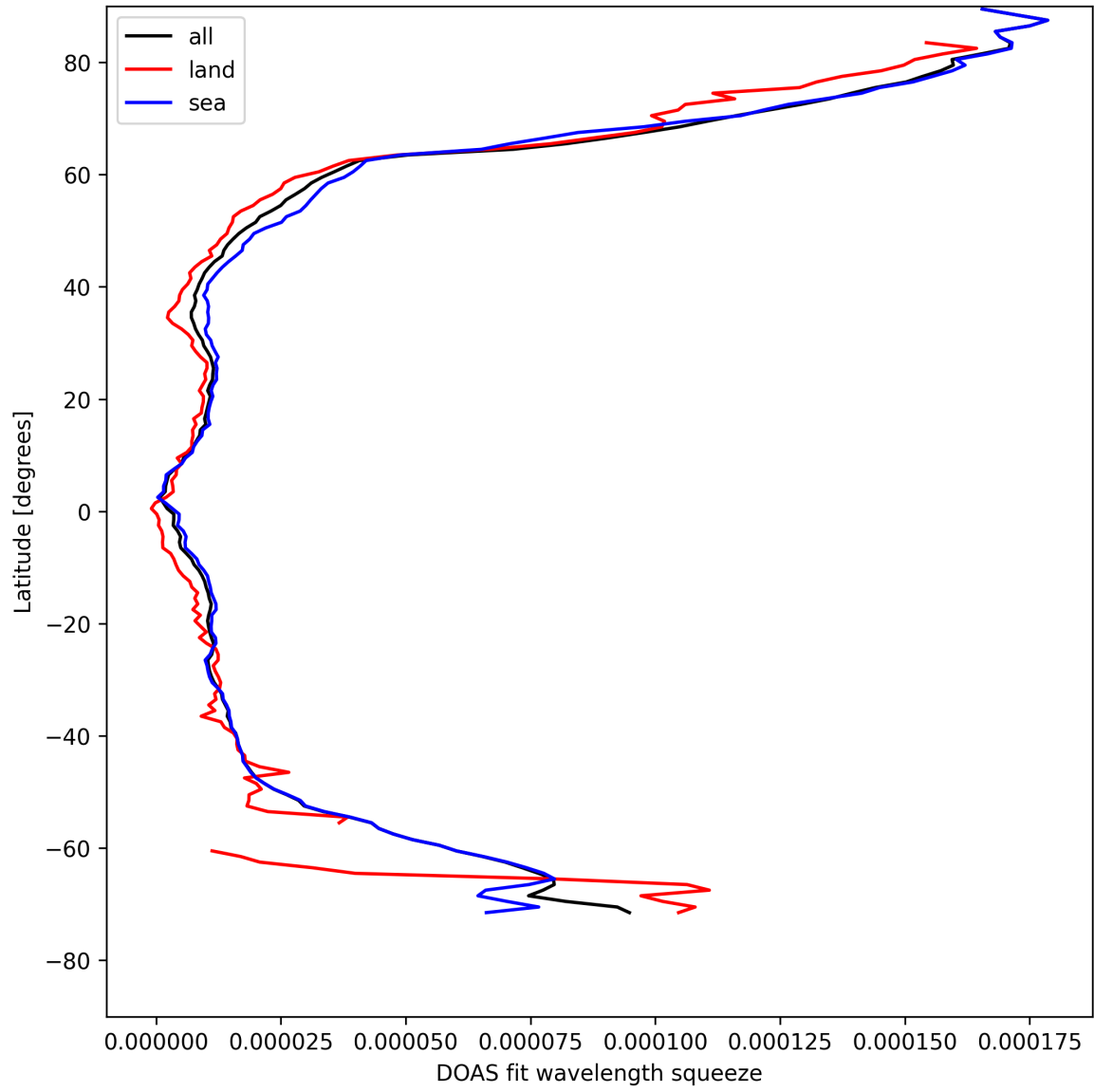
Figure 29: Zonal average of “DOAS fit wavelength squeeze” for 2025-04-25 to 2025-04-26.
