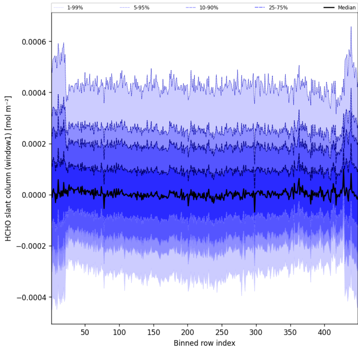
Figure 50: Along track statistics of “HCHO slant column (window1)” for 2025-04-25 to 2025-04-26
