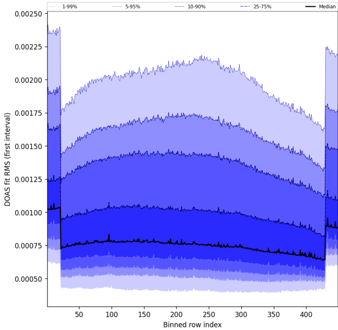
Figure 58: Along track statistics of “DOAS fit RMS (first interval)” for 2025-04-25 to 2025-04-26
