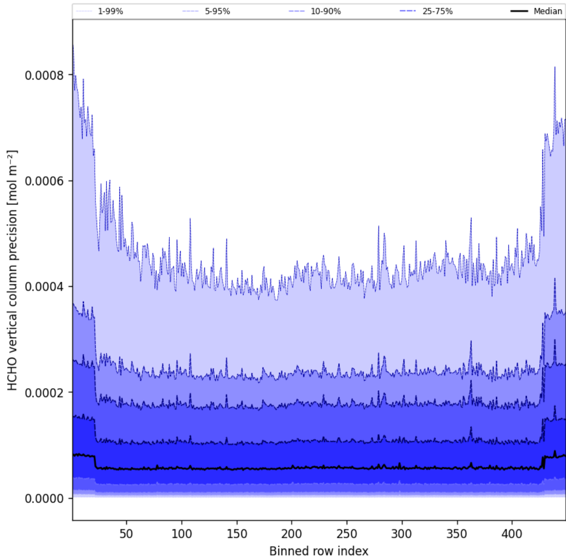
Figure 48: Along track statistics of “HCHO vertical column precision” for 2025-04-25 to 2025-04-26
