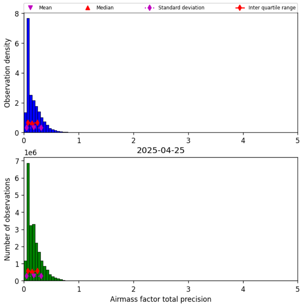
Figure 39: Histogram of “Airmass factor total precision” for 2025-04-25 to 2025-04-26
