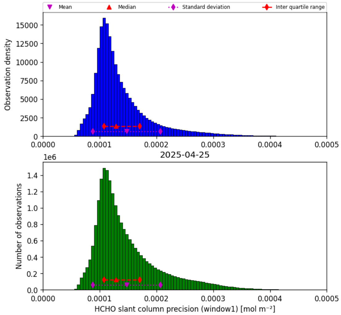
Figure 37: Histogram of “HCHO slant column precision (window1)” for 2025-04-25 to 2025-04-26
