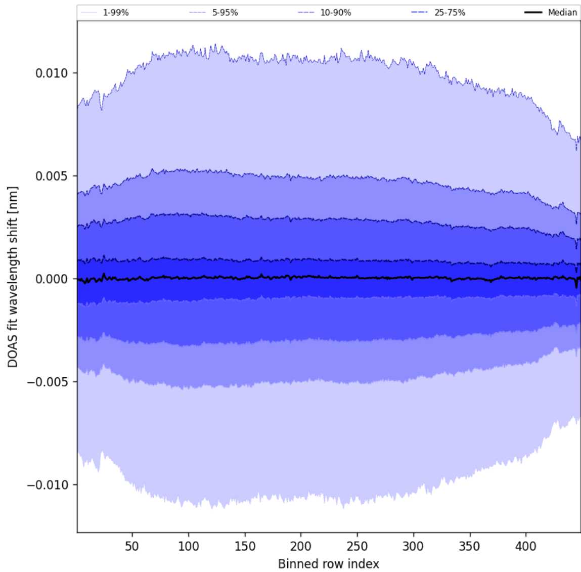
Figure 56: Along track statistics of “DOAS fit wavelength shift” for 2025-04-25 to 2025-04-26
