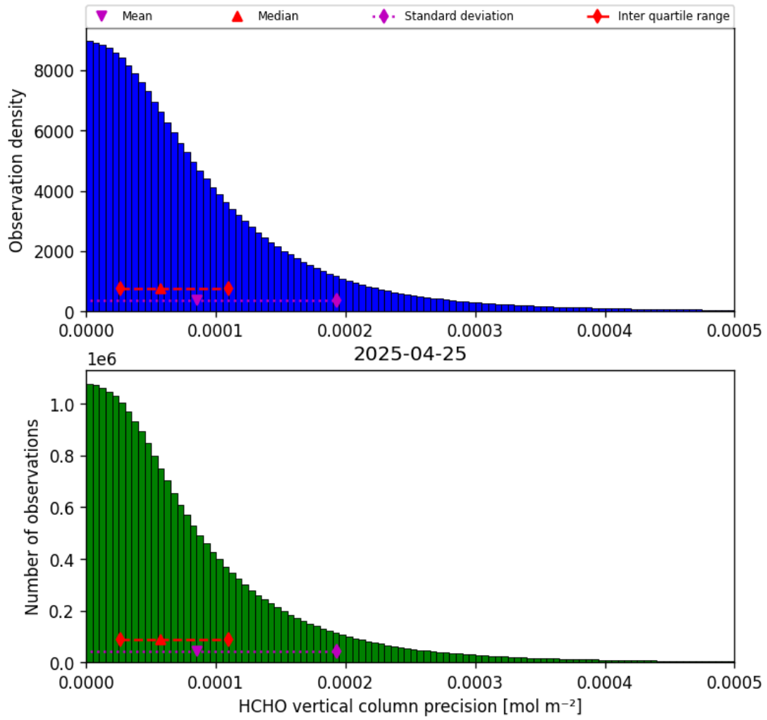
Figure 34: Histogram of “HCHO vertical column precision” for 2025-04-25 to 2025-04-26
