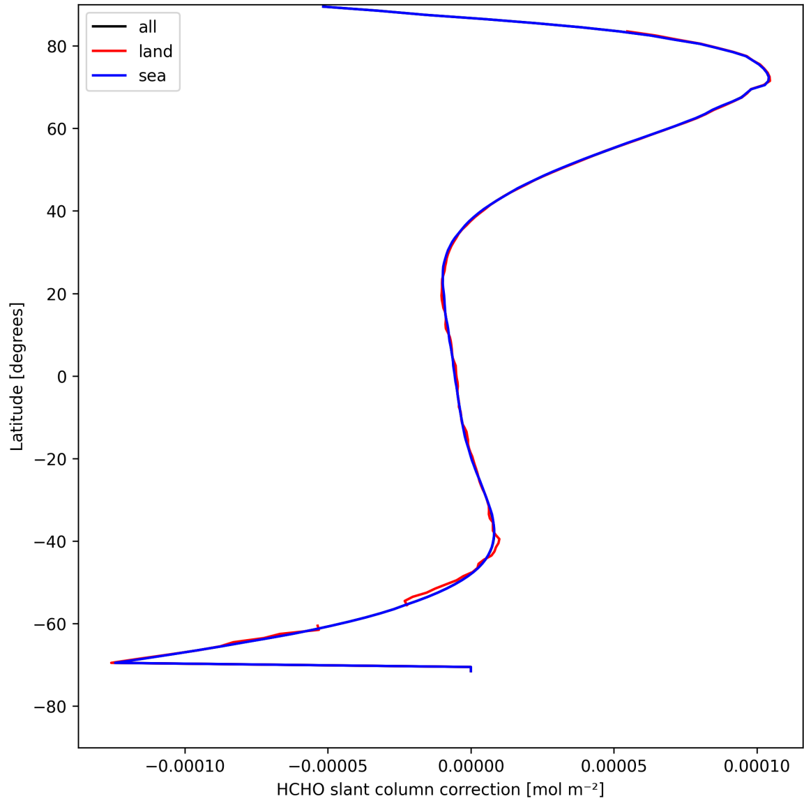
Figure 31: Zonal average of “HCHO slant column correction” for 2025-04-25 to 2025-04-26.
