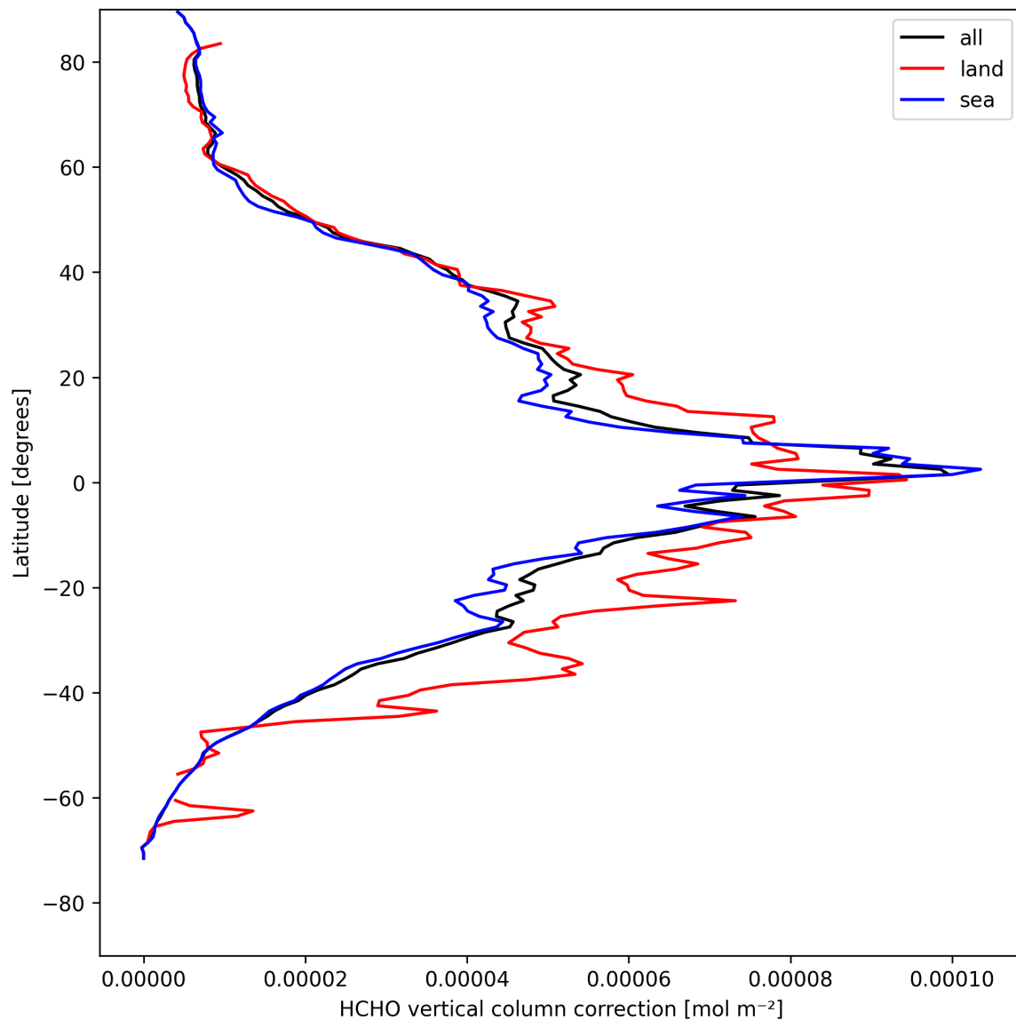
Figure 21: Zonal average of “HCHO vertical column correction” for 2025-04-25 to 2025-04-26.
