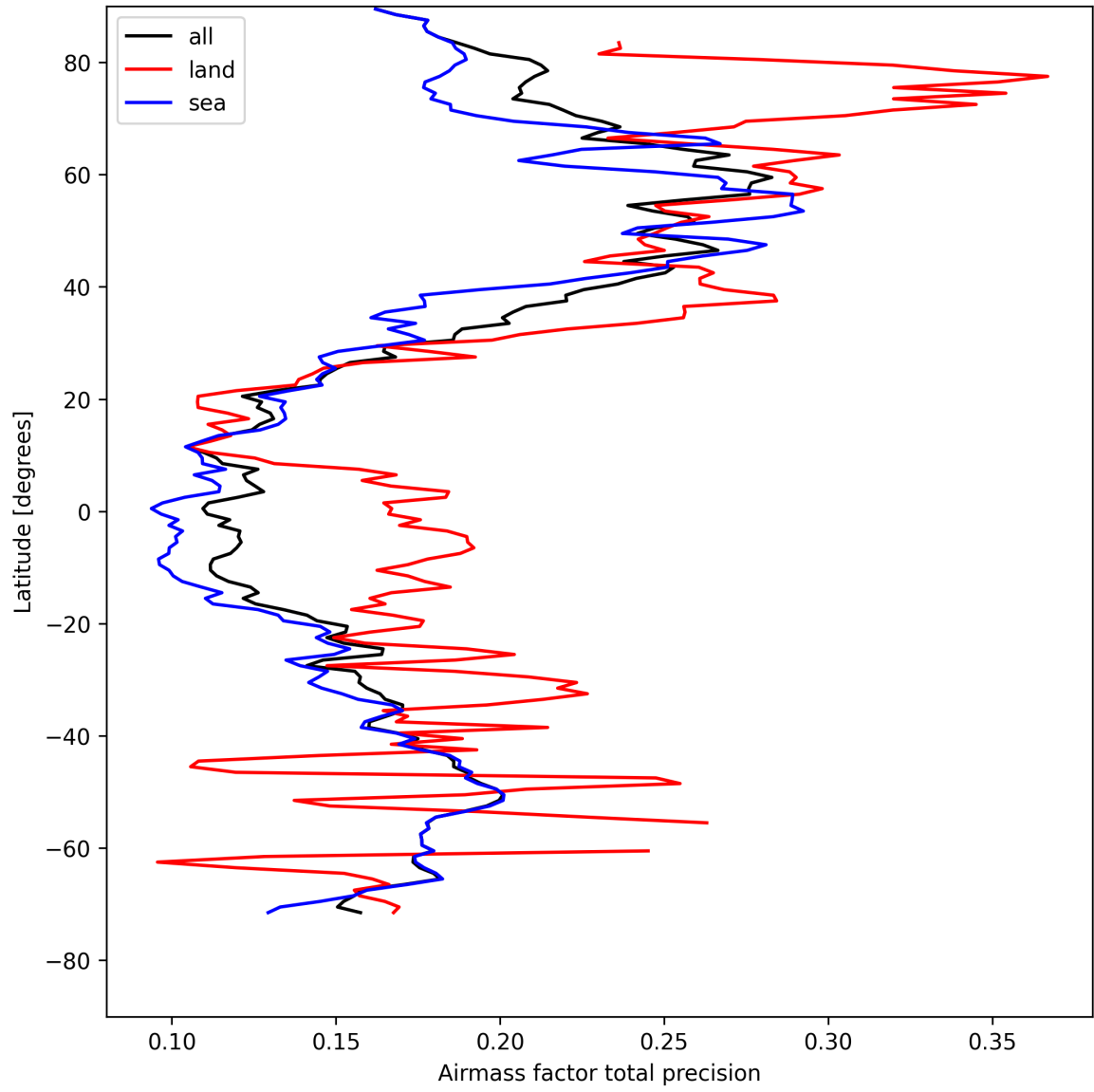
Figure 25: Zonal average of “Airmass factor total precision” for 2025-04-25 to 2025-04-26.
