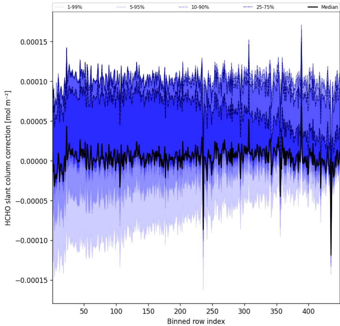
Figure 59: Along track statistics of “HCHO slant column correction” for 2025-04-25 to 2025-04-26
