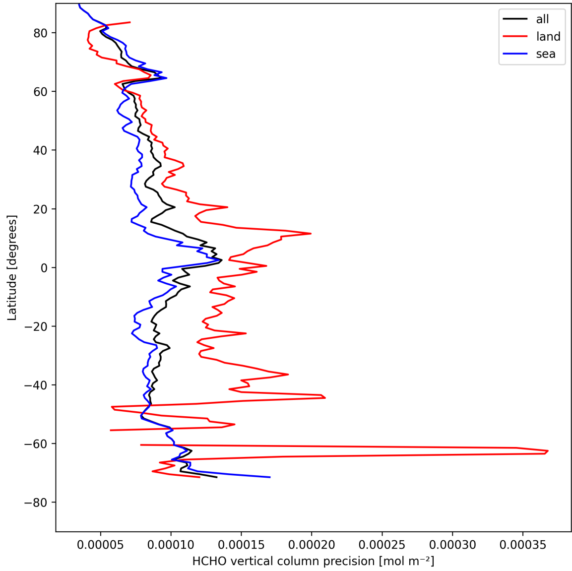
Figure 20: Zonal average of “HCHO vertical column precision” for 2025-04-25 to 2025-04-26.
