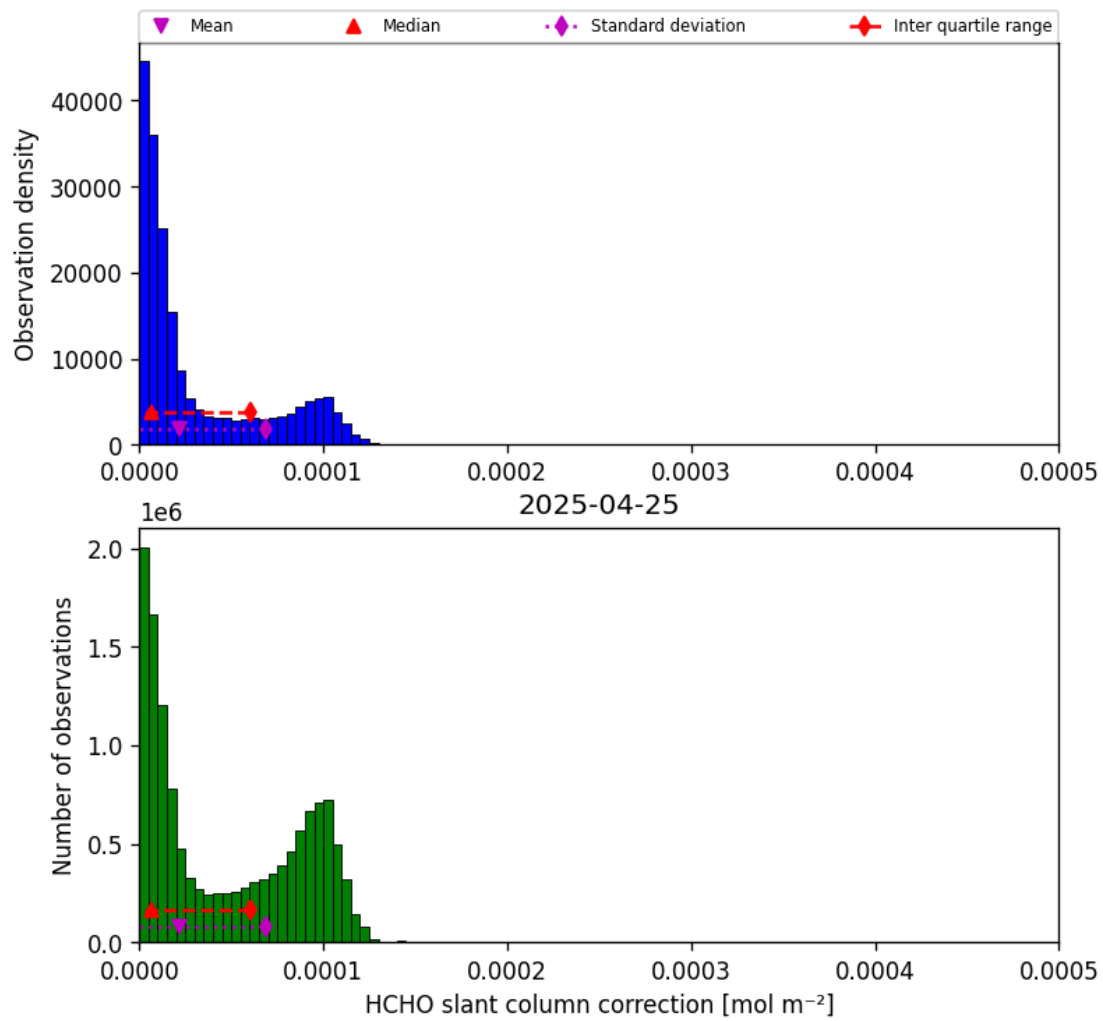
Figure 45: Histogram of “HCHO slant column correction” for 2025-04-25 to 2025-04-26
