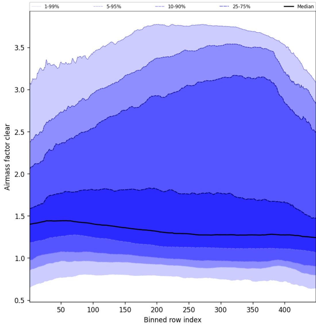
Figure 54: Along track statistics of “Airmass factor clear” for 2025-04-25 to 2025-04-26
