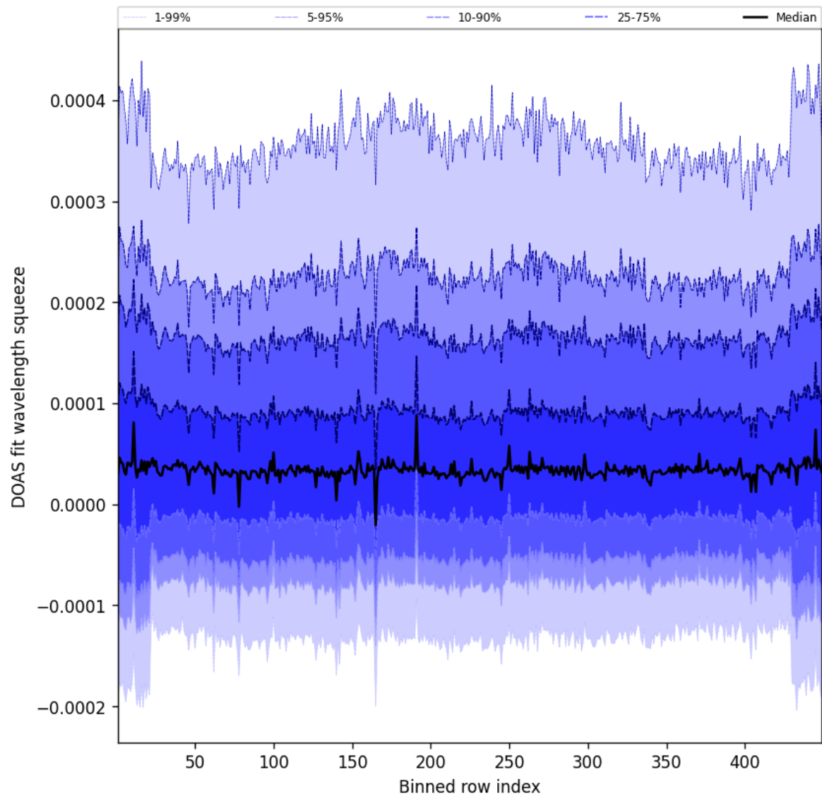
Figure 57: Along track statistics of “DOAS fit wavelength squeeze” for 2025-04-25 to 2025-04-26
