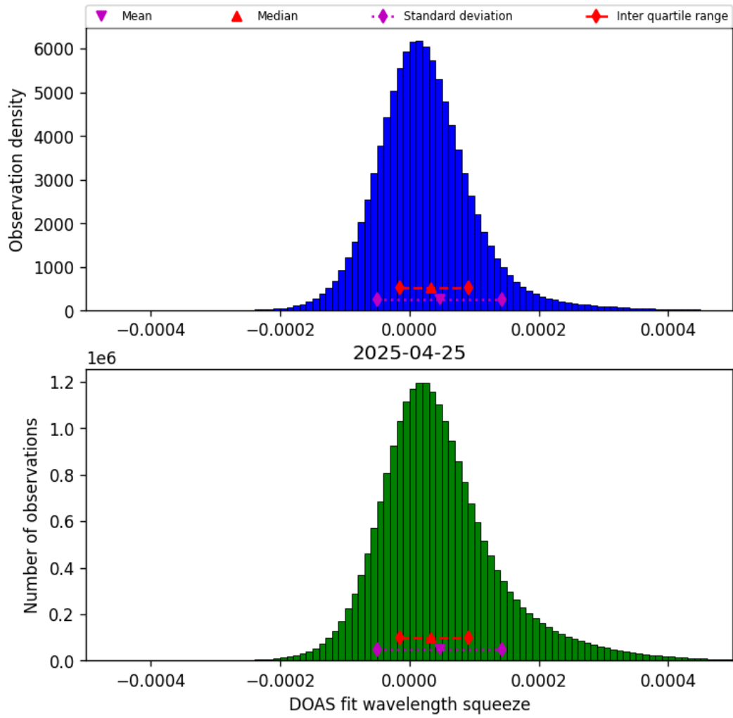
Figure 43: Histogram of “DOAS fit wavelength squeeze” for 2025-04-25 to 2025-04-26
