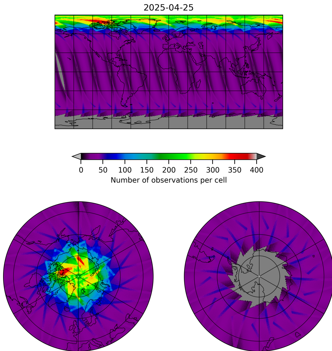
Figure 17: Map of the number of observations for 2025-04-25 to 2025-04-26
