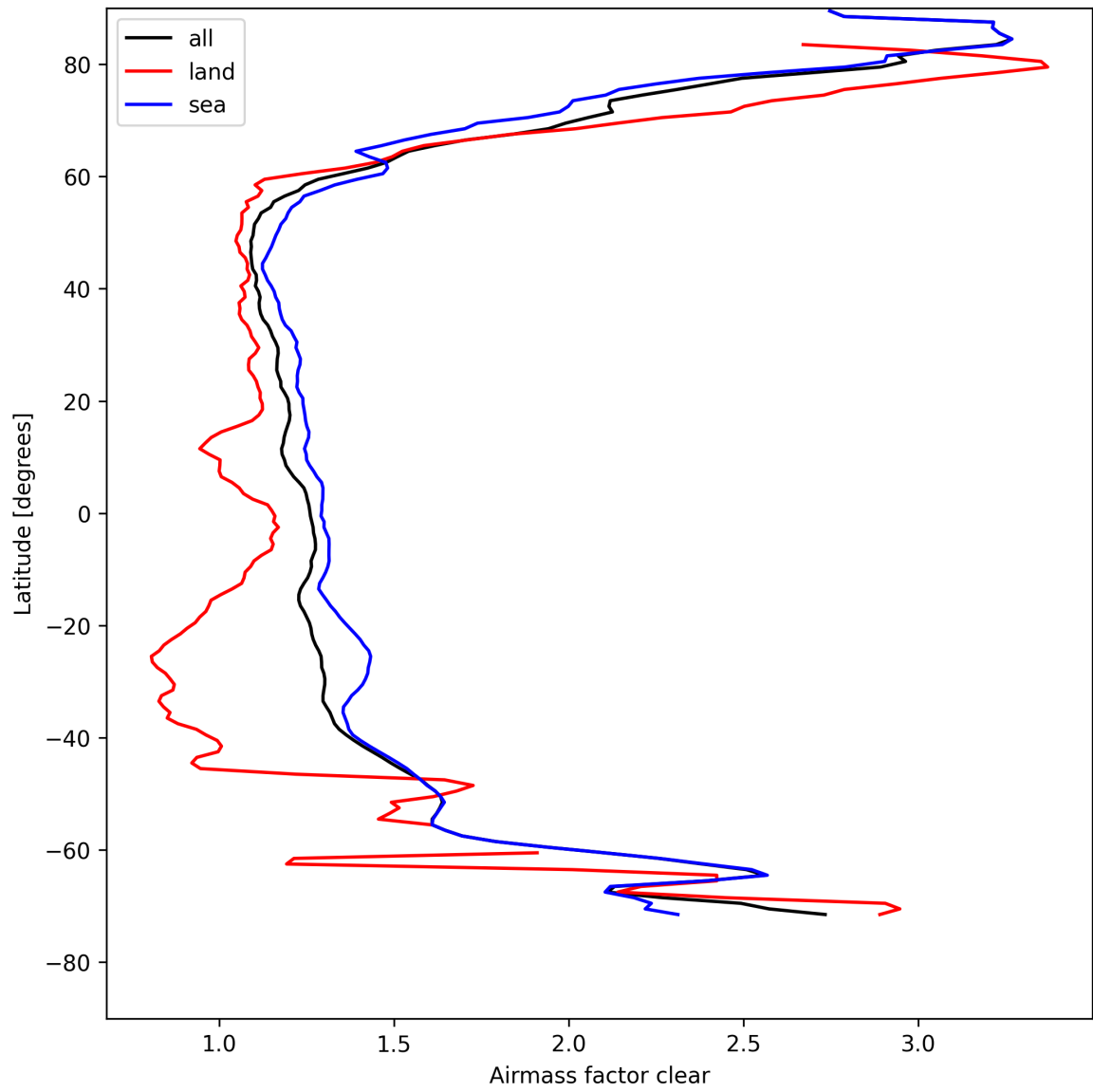
Figure 26: Zonal average of “Airmass factor clear” for 2025-04-25 to 2025-04-26.
