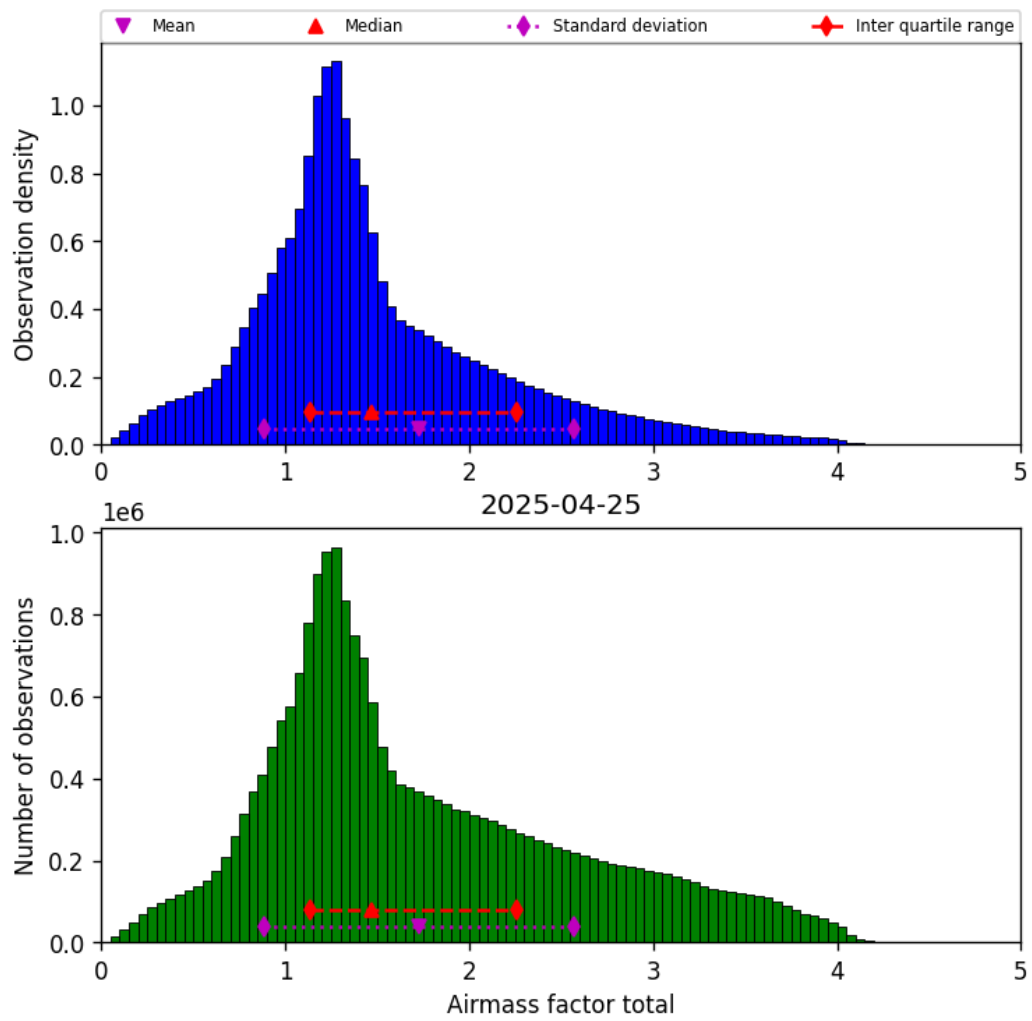
Figure 38: Histogram of “Airmass factor total” for 2025-04-25 to 2025-04-26
