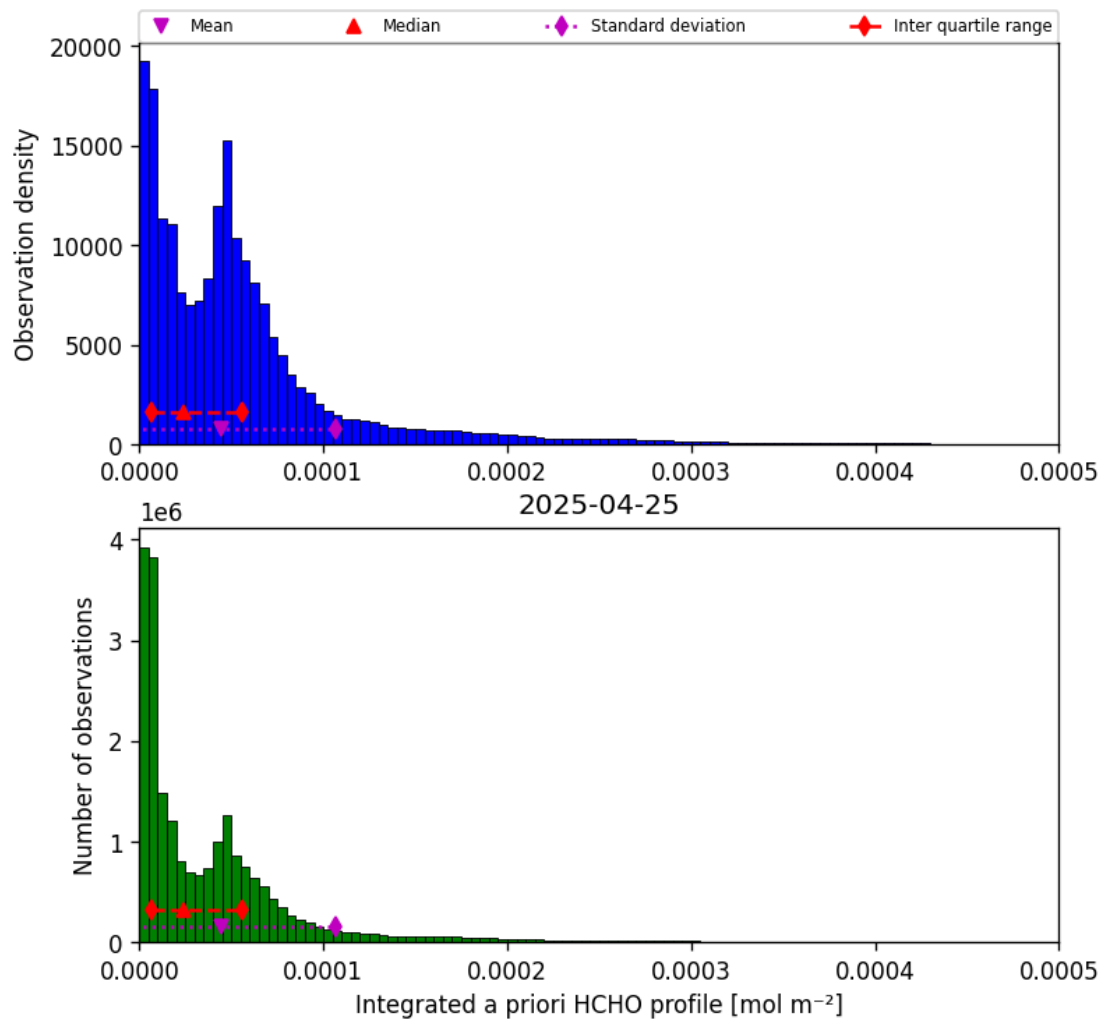
Figure 41: Histogram of “Integrated a priori HCHO profile” for 2025-04-25 to 2025-04-26
