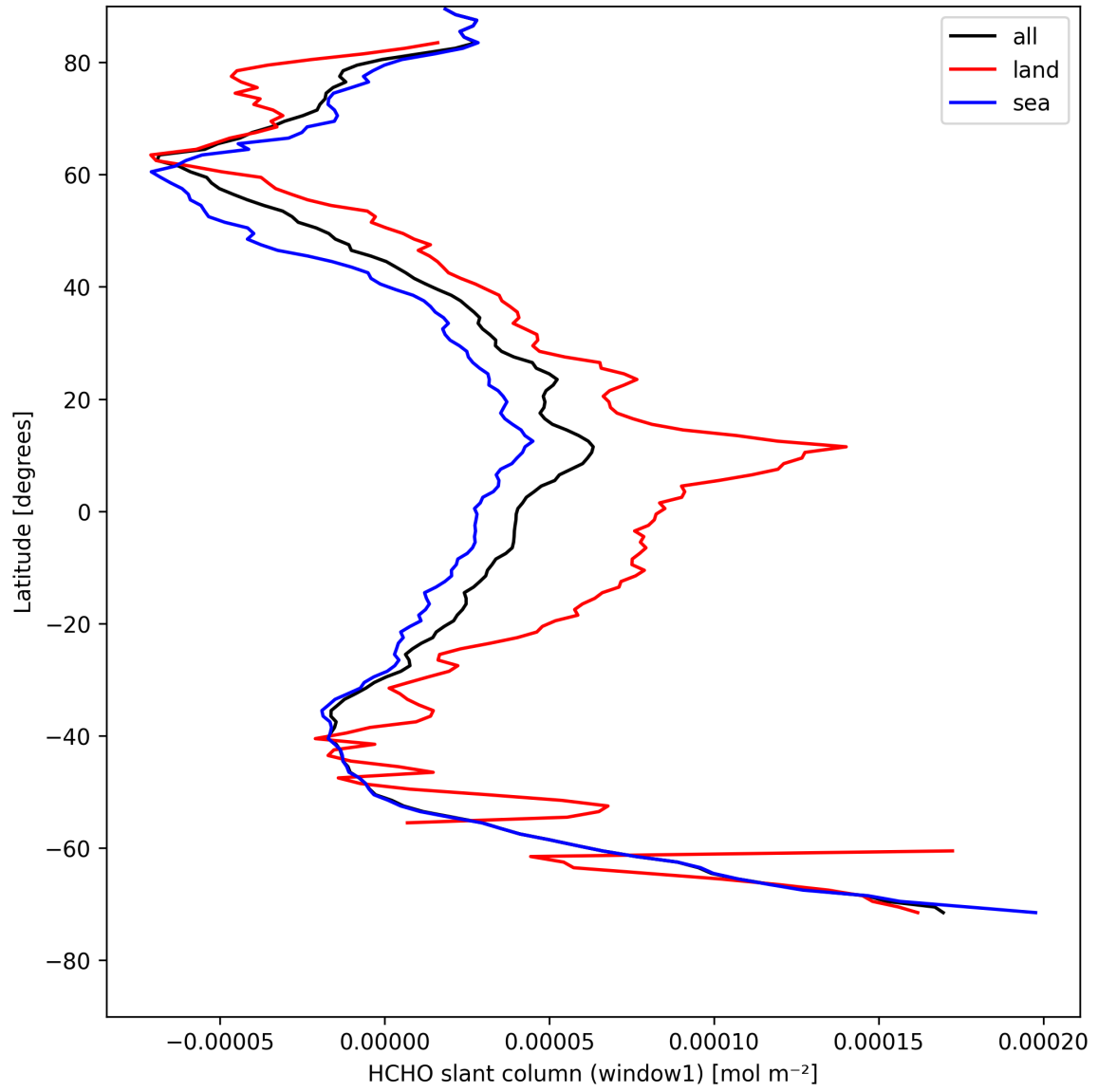
Figure 22: Zonal average of “HCHO slant column (window1)” for 2025-04-25 to 2025-04-26.
