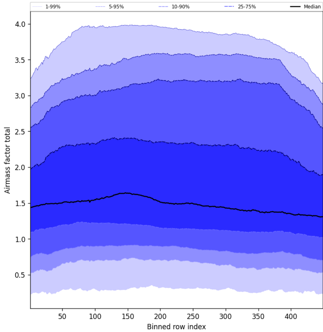
Figure 52: Along track statistics of “Airmass factor total” for 2025-04-25 to 2025-04-26
