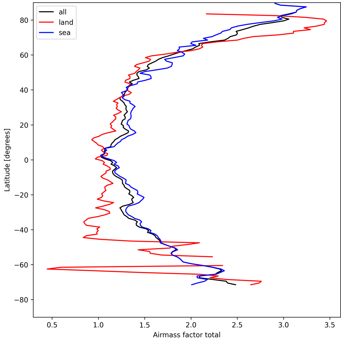
Figure 24: Zonal average of “Airmass factor total” for 2025-04-25 to 2025-04-26.
