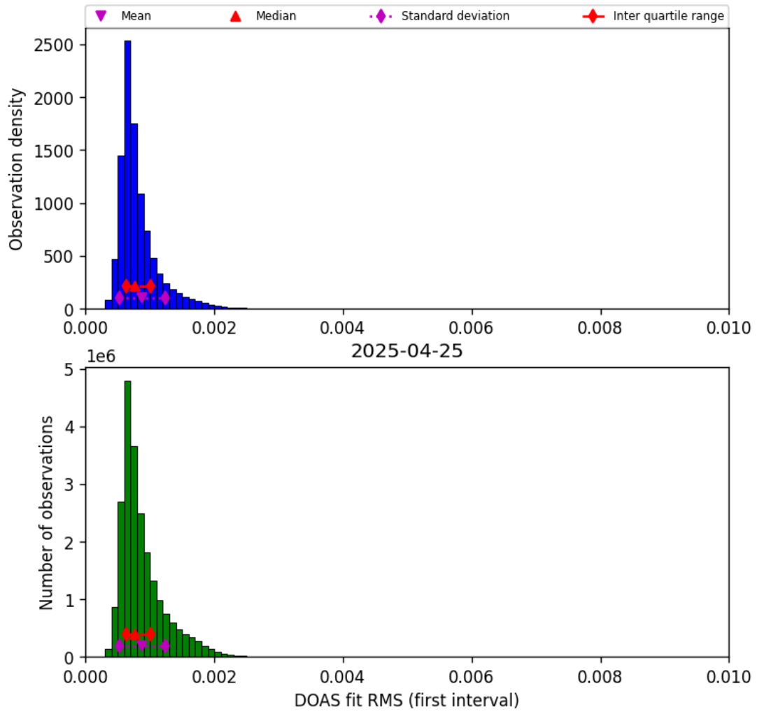
Figure 44: Histogram of “DOAS fit RMS (first interval)” for 2025-04-25 to 2025-04-26
