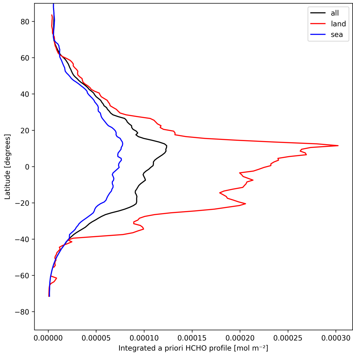
Figure 27: Zonal average of “Integrated a priori HCHO profile” for 2025-04-25 to 2025-04-26.
