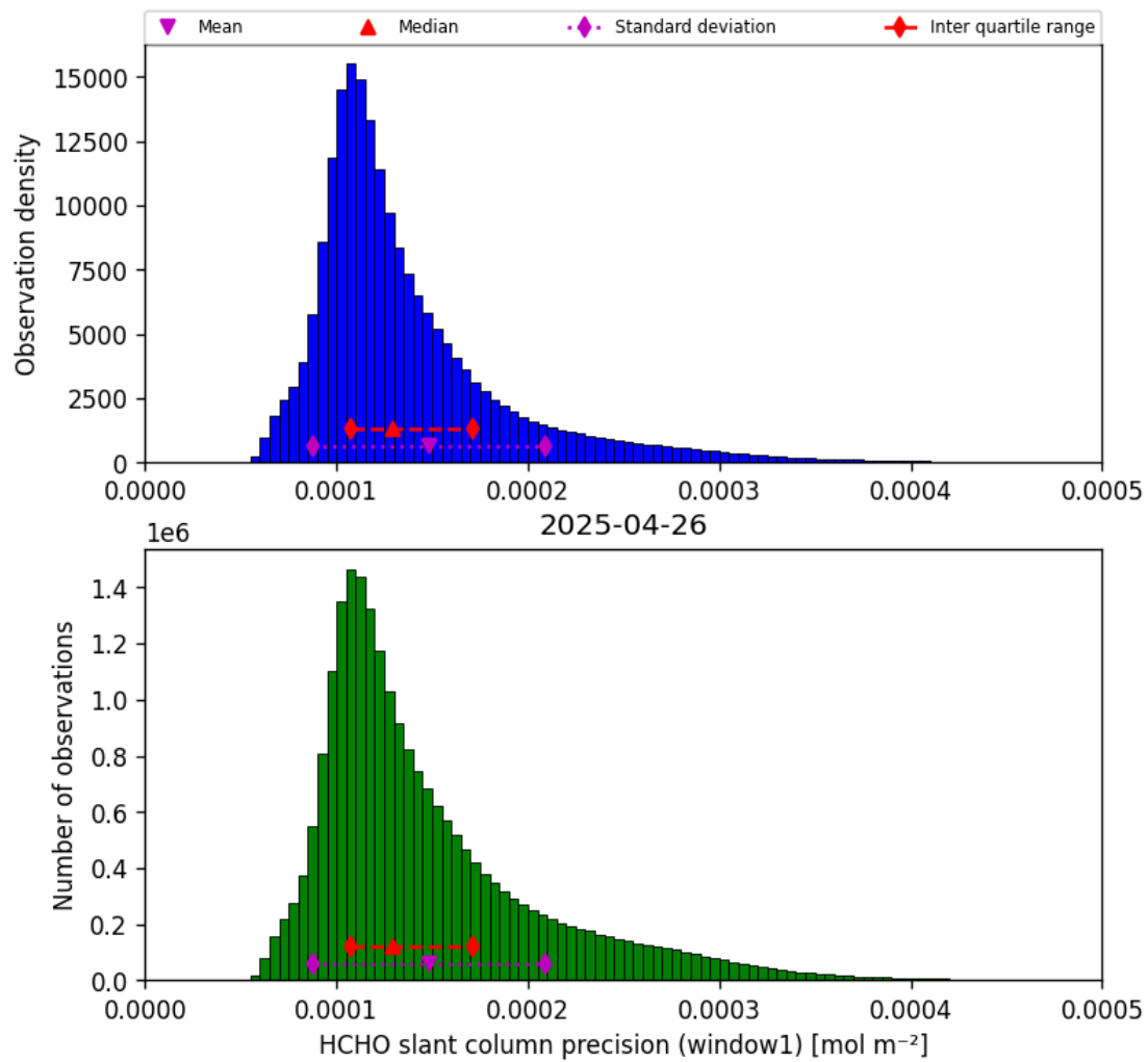
Figure 37: Histogram of “HCHO slant column precision (window1)” for 2025-04-26 to 2025-04-27
