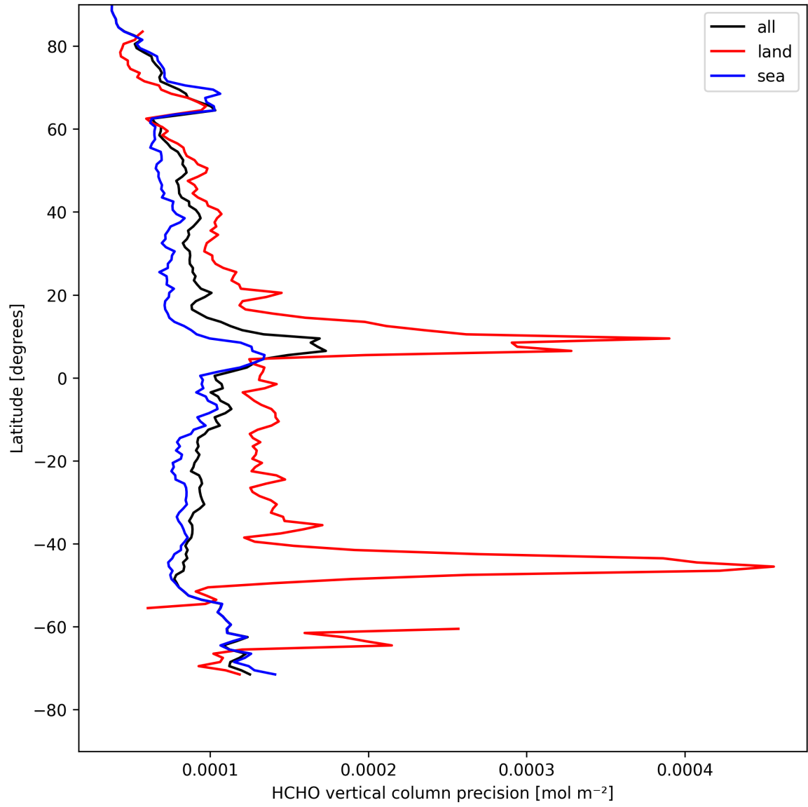
Figure 20: Zonal average of “HCHO vertical column precision” for 2025-04-26 to 2025-04-27.
