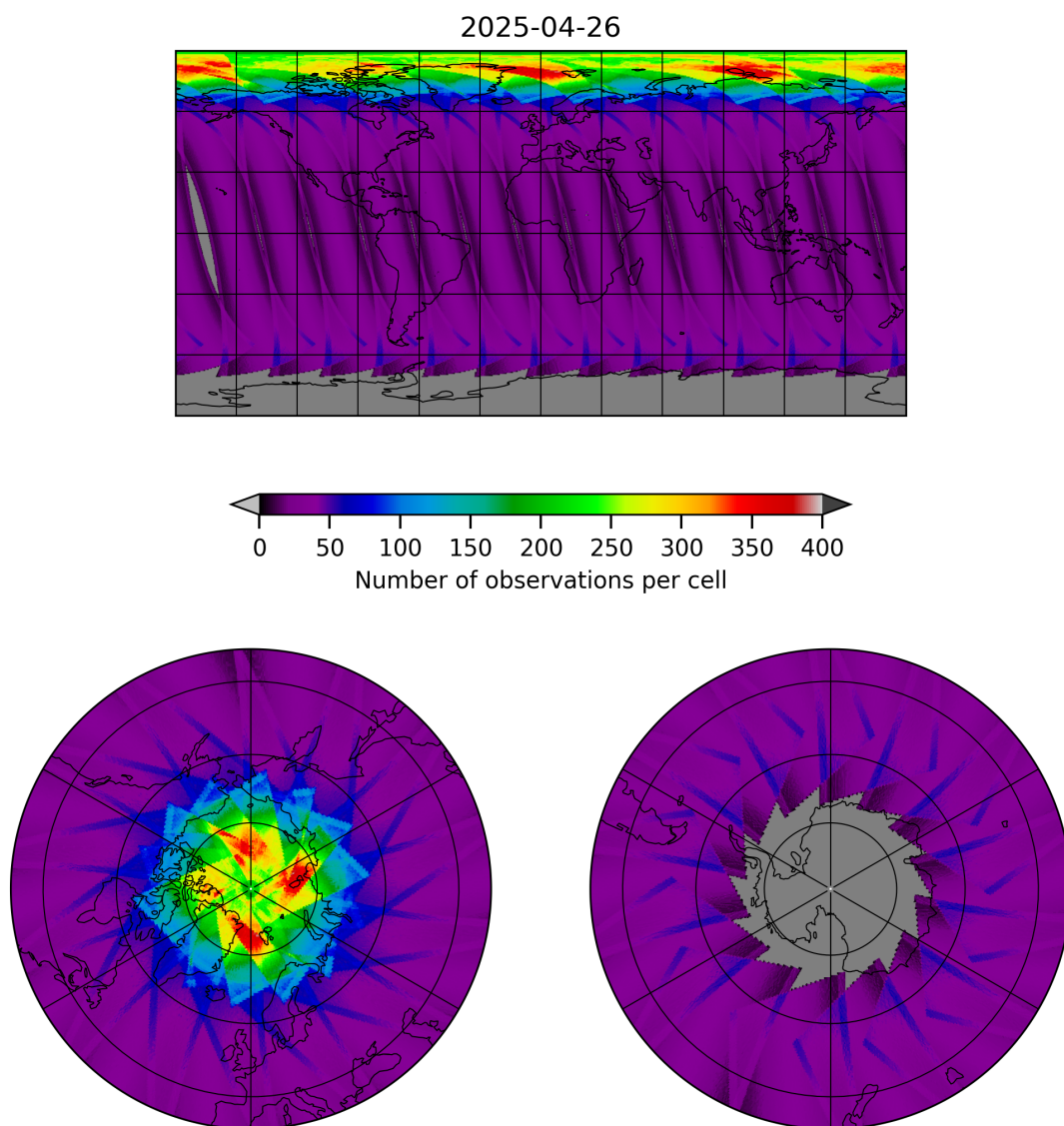
Figure 17: Map of the number of observations for 2025-04-26 to 2025-04-27
