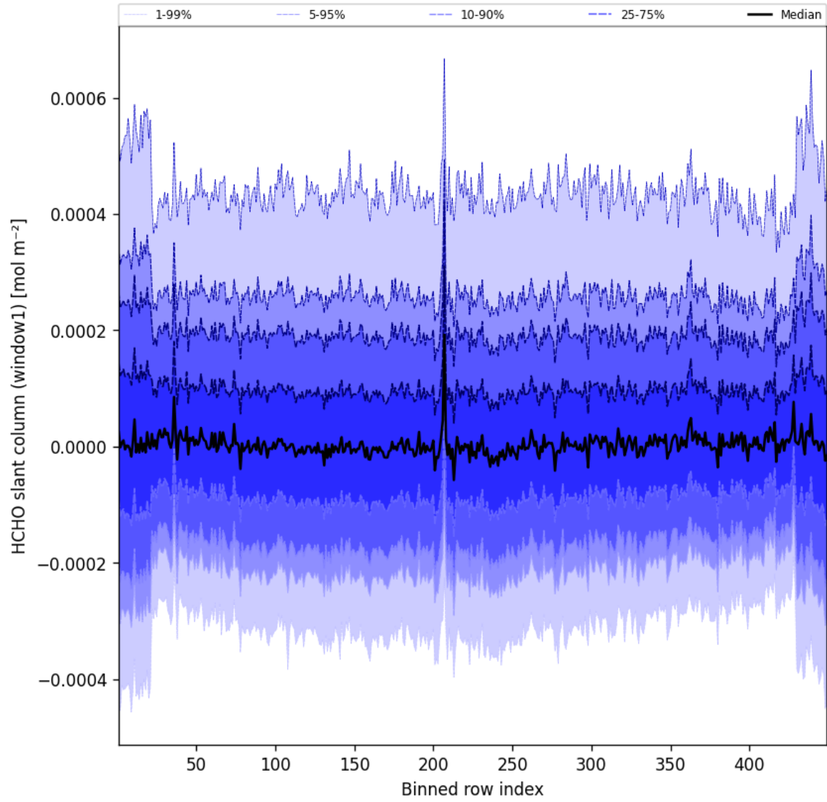
Figure 50: Along track statistics of “HCHO slant column (window1)” for 2025-04-26 to 2025-04-27
