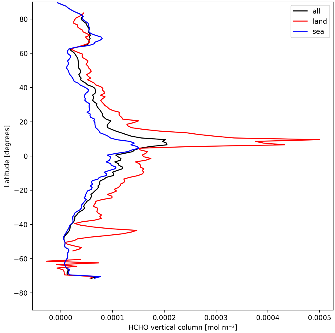
Figure 19: Zonal average of “HCHO vertical column” for 2025-04-26 to 2025-04-27.
