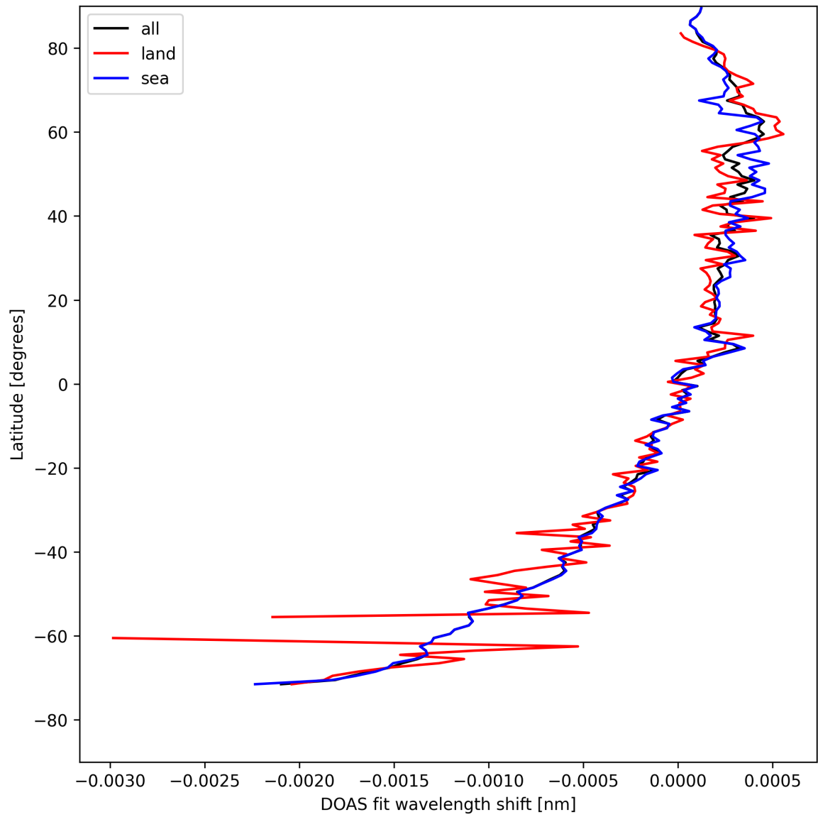
Figure 28: Zonal average of “DOAS fit wavelength shift” for 2025-04-26 to 2025-04-27.
