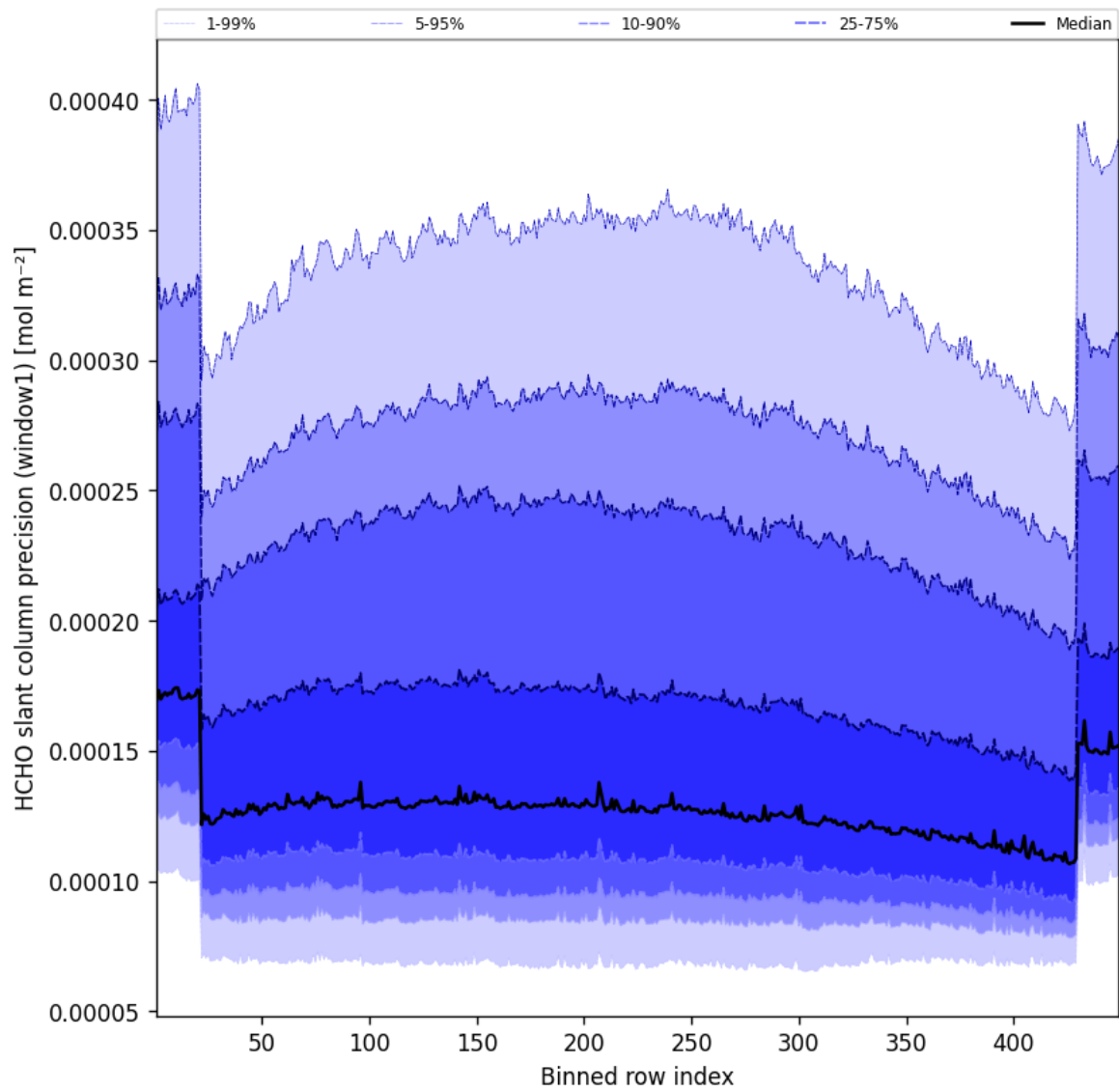
Figure 51: Along track statistics of “HCHO slant column precision (window1)” for 2025-04-26 to 2025-04-27
