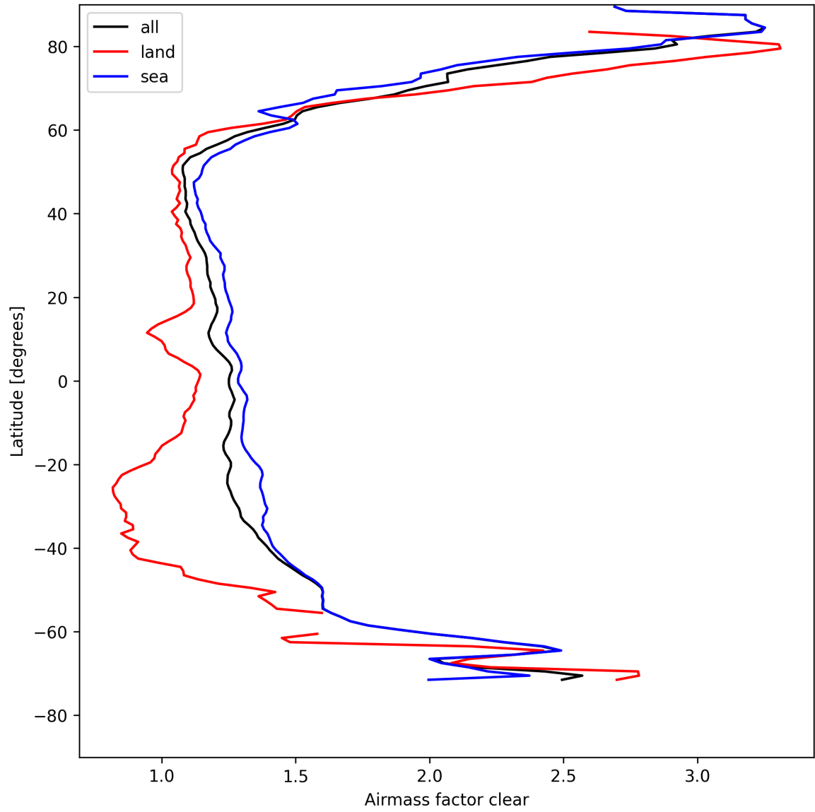
Figure 26: Zonal average of “Airmass factor clear” for 2025-04-26 to 2025-04-27.
