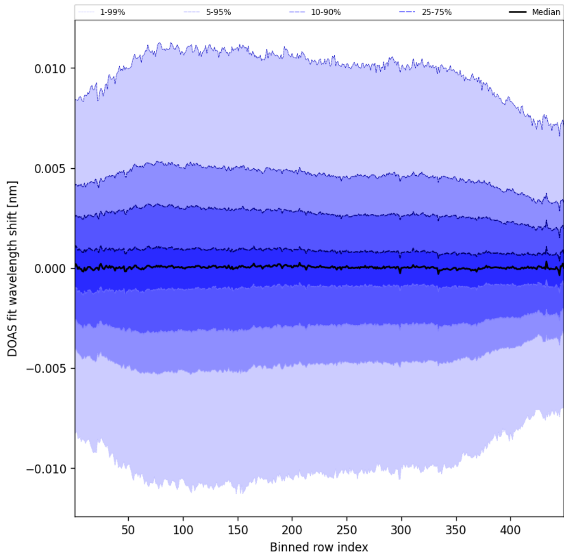
Figure 56: Along track statistics of “DOAS fit wavelength shift” for 2025-04-26 to 2025-04-27
