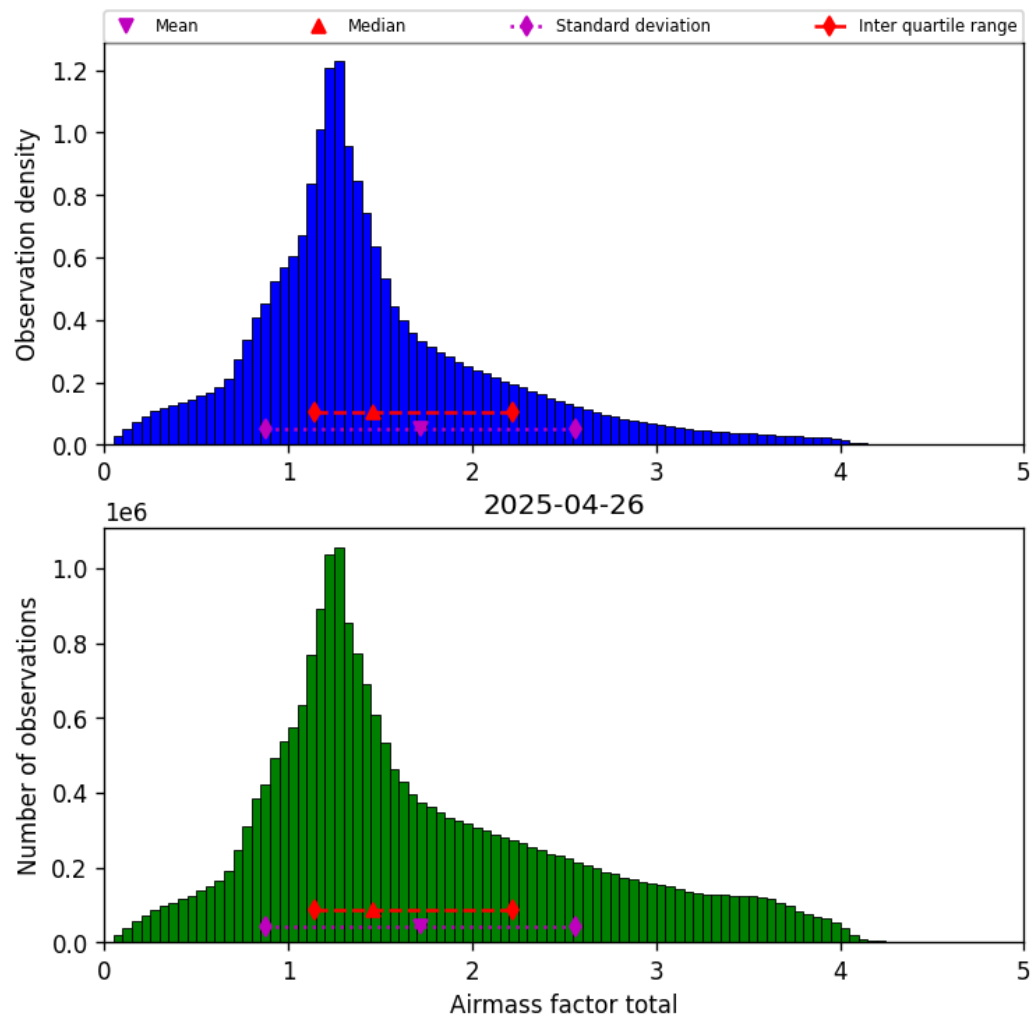
Figure 38: Histogram of “Airmass factor total” for 2025-04-26 to 2025-04-27
