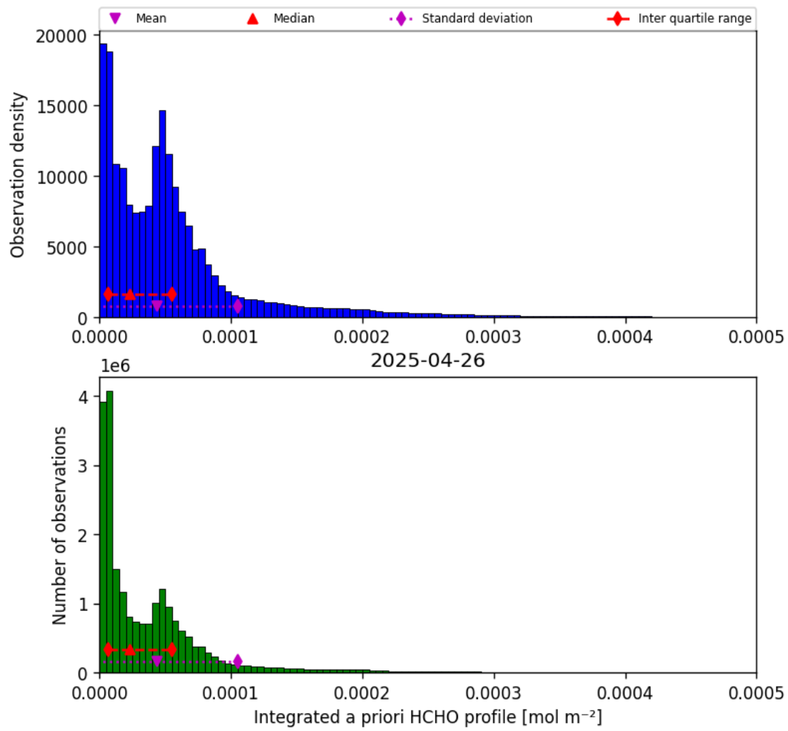
Figure 41: Histogram of “Integrated a priori HCHO profile” for 2025-04-26 to 2025-04-27
