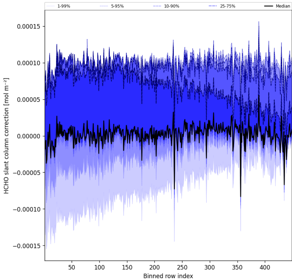
Figure 59: Along track statistics of “HCHO slant column correction” for 2025-04-26 to 2025-04-27
