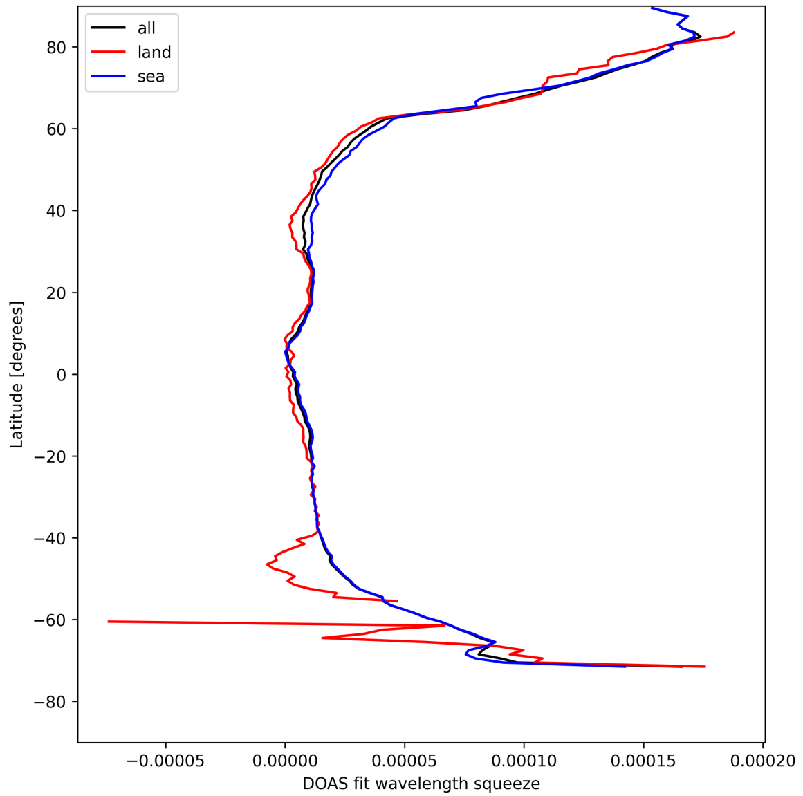
Figure 29: Zonal average of “DOAS fit wavelength squeeze” for 2025-04-26 to 2025-04-27.
