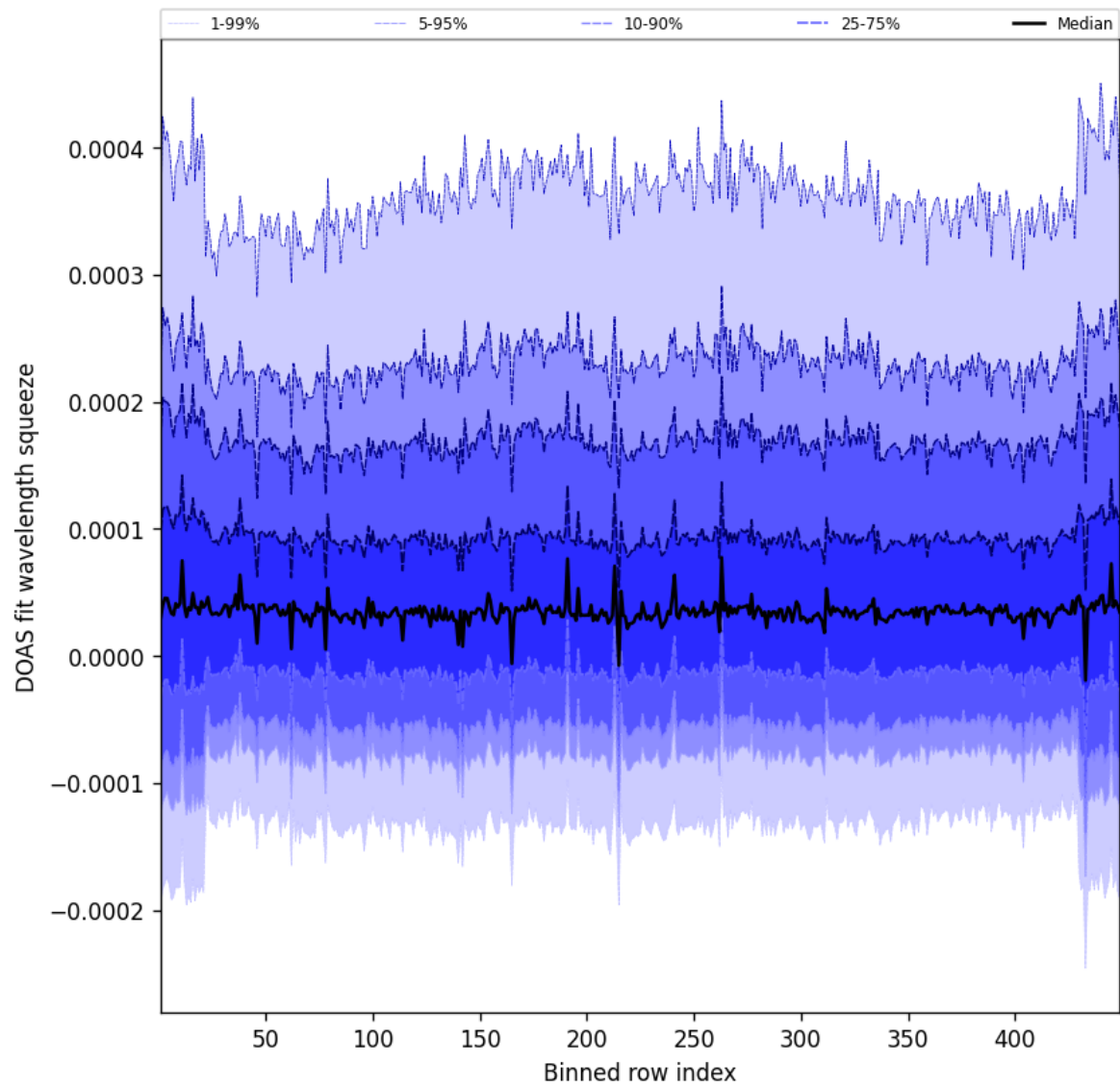
Figure 57: Along track statistics of “DOAS fit wavelength squeeze” for 2025-04-26 to 2025-04-27
