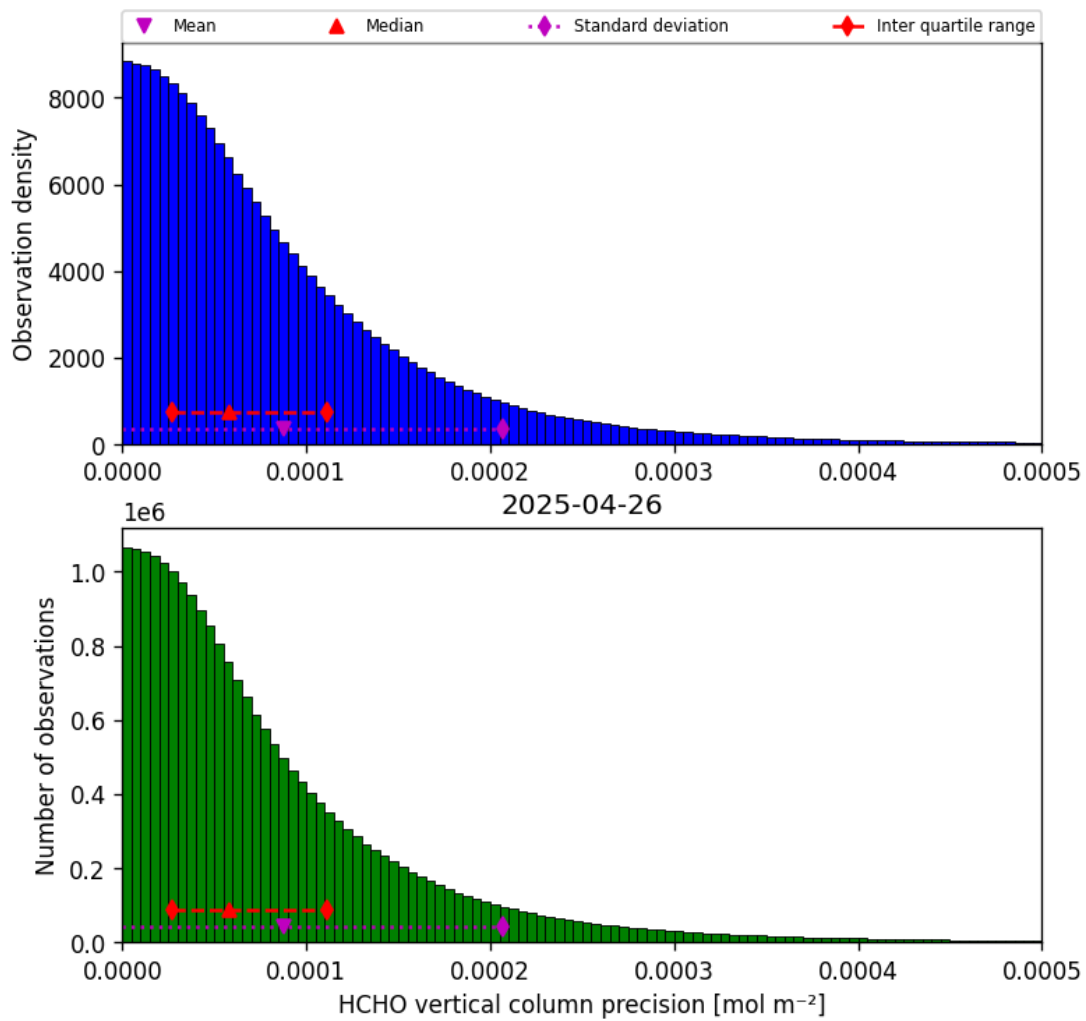
Figure 34: Histogram of “HCHO vertical column precision” for 2025-04-26 to 2025-04-27
