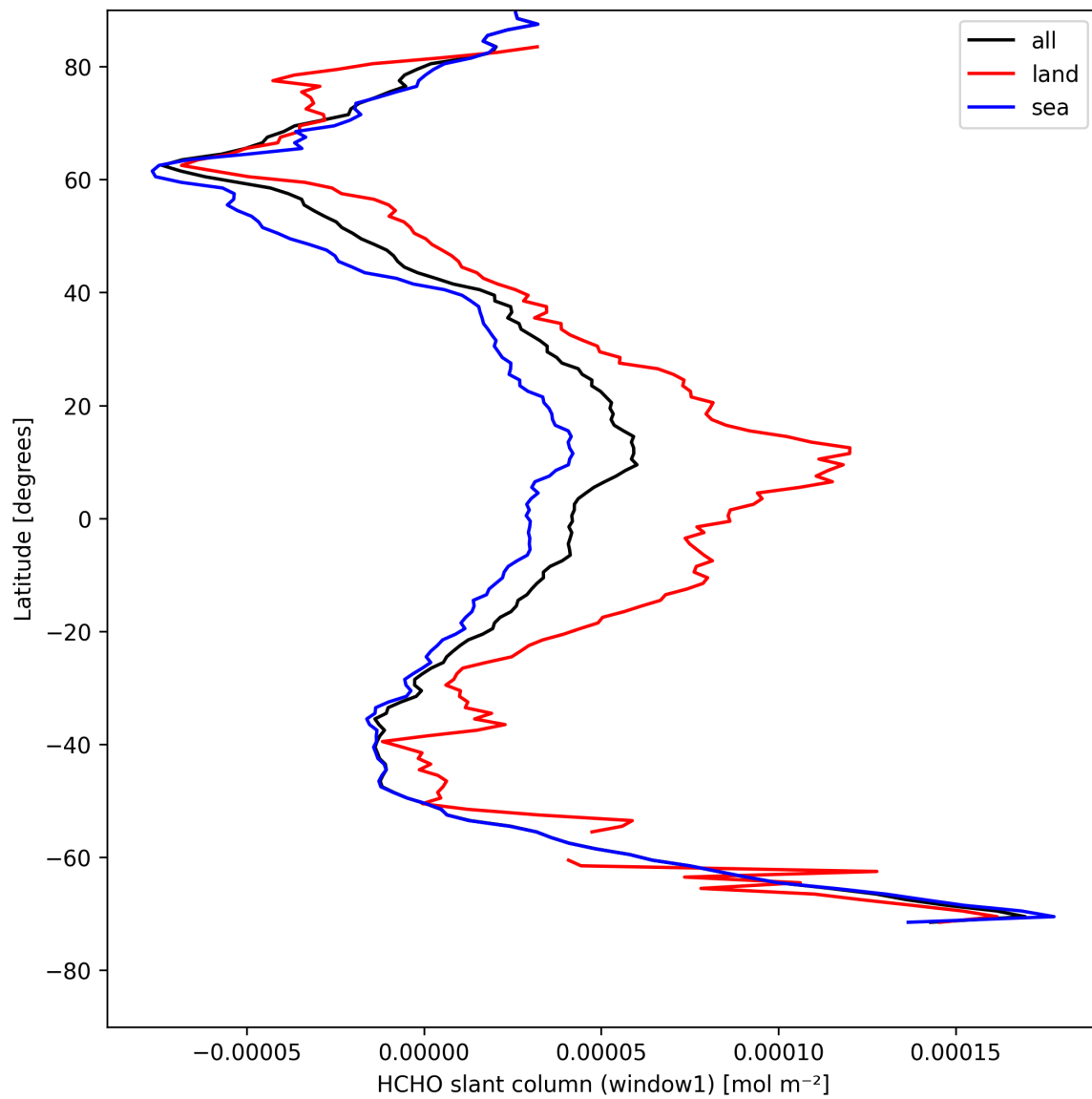
Figure 22: Zonal average of “HCHO slant column (window1)” for 2025-04-26 to 2025-04-27.
