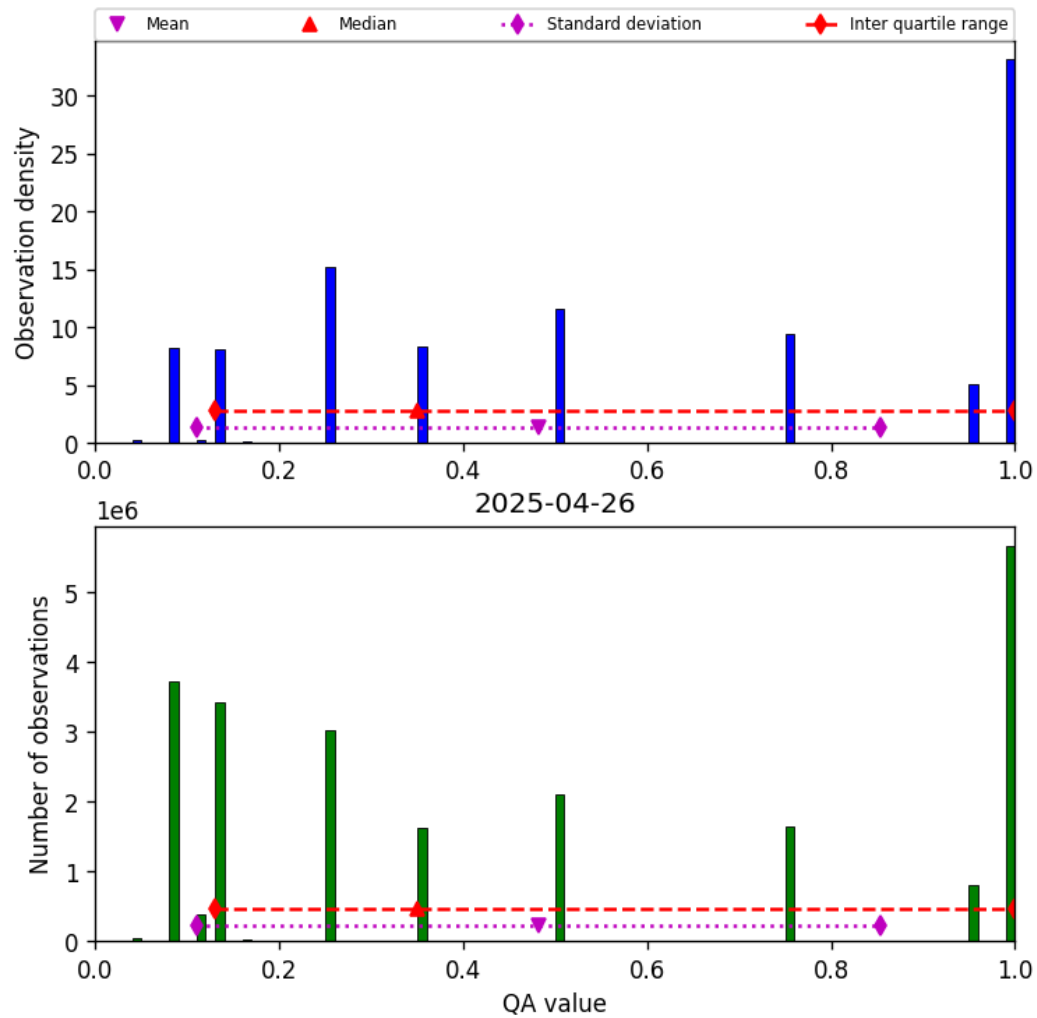
Figure 32: Histogram of “QA value” for 2025-04-26 to 2025-04-27
