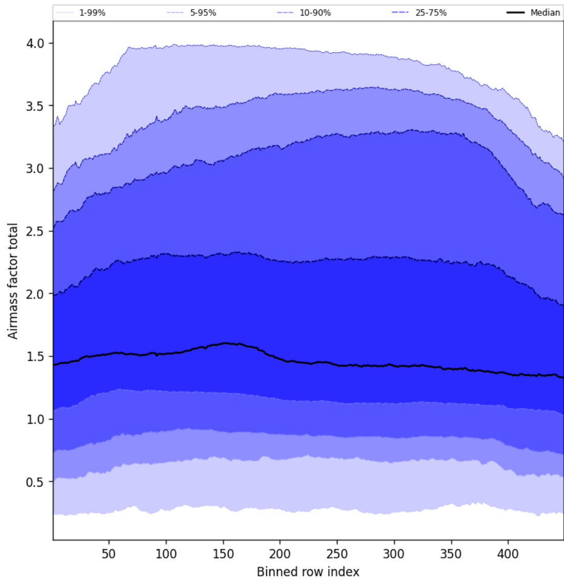
Figure 52: Along track statistics of “Airmass factor total” for 2025-04-26 to 2025-04-27
