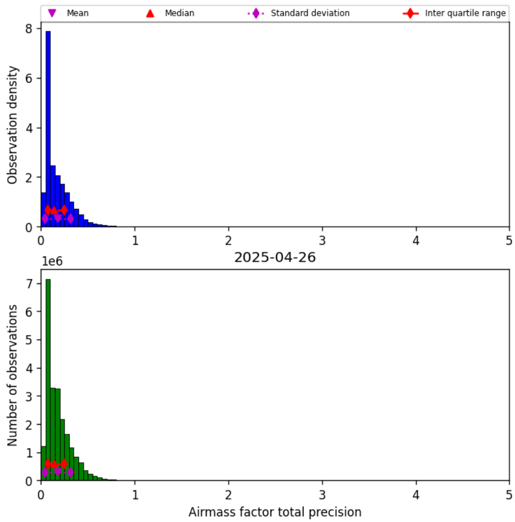
Figure 39: Histogram of “Airmass factor total precision” for 2025-04-26 to 2025-04-27
