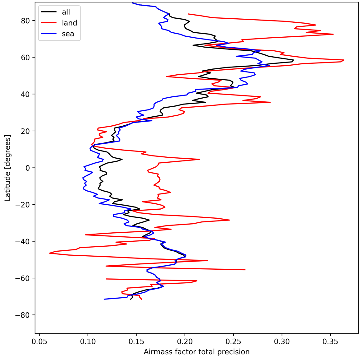
Figure 25: Zonal average of “Airmass factor total precision” for 2025-04-26 to 2025-04-27.
