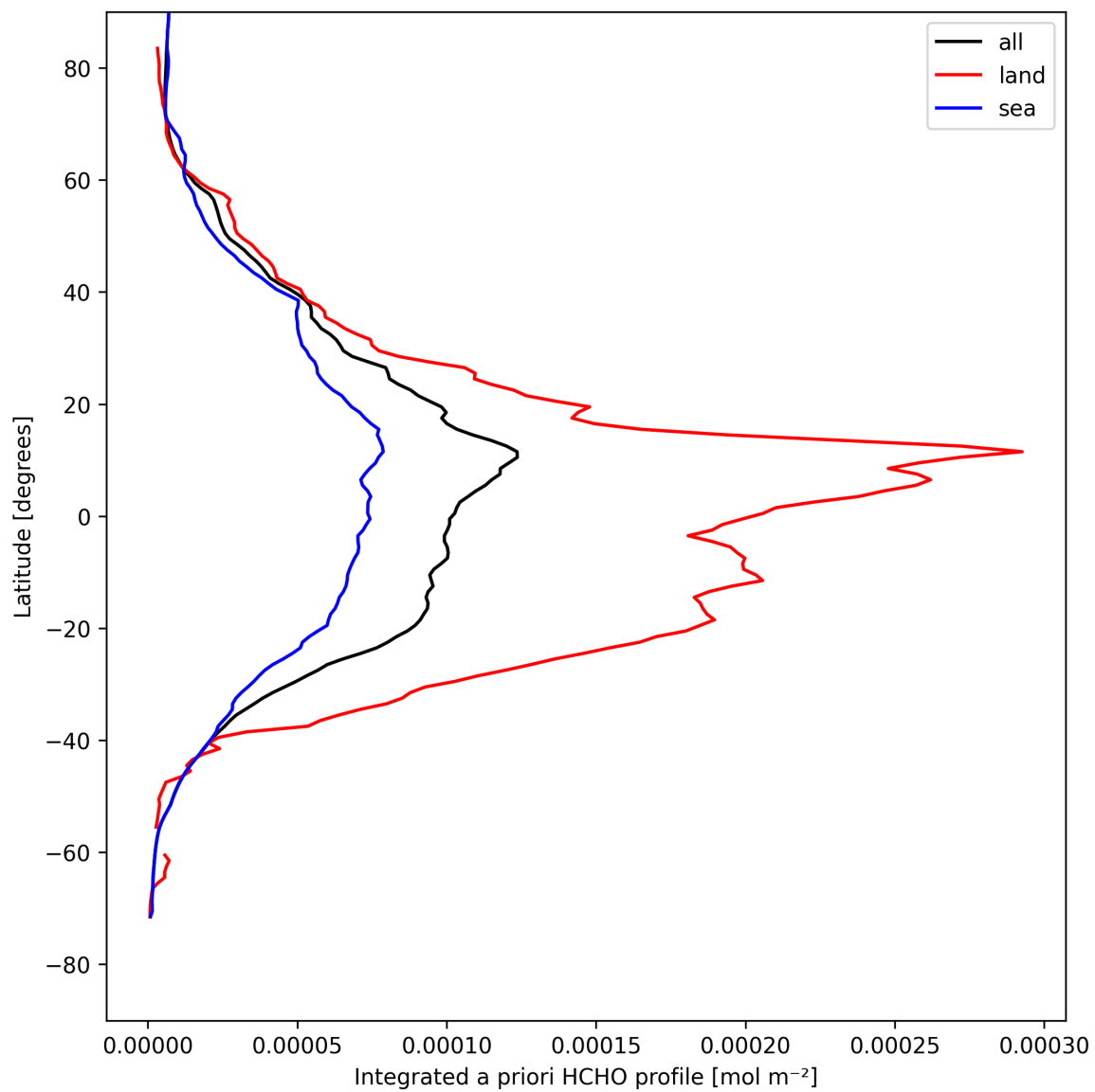
Figure 27: Zonal average of “Integrated a priori HCHO profile” for 2025-04-26 to 2025-04-27.
