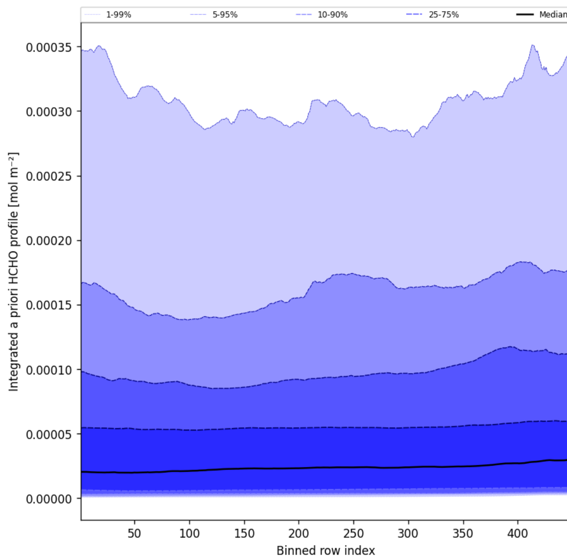
Figure 55: Along track statistics of “Integrated a priori HCHO profile” for 2025-04-26 to 2025-04-27
