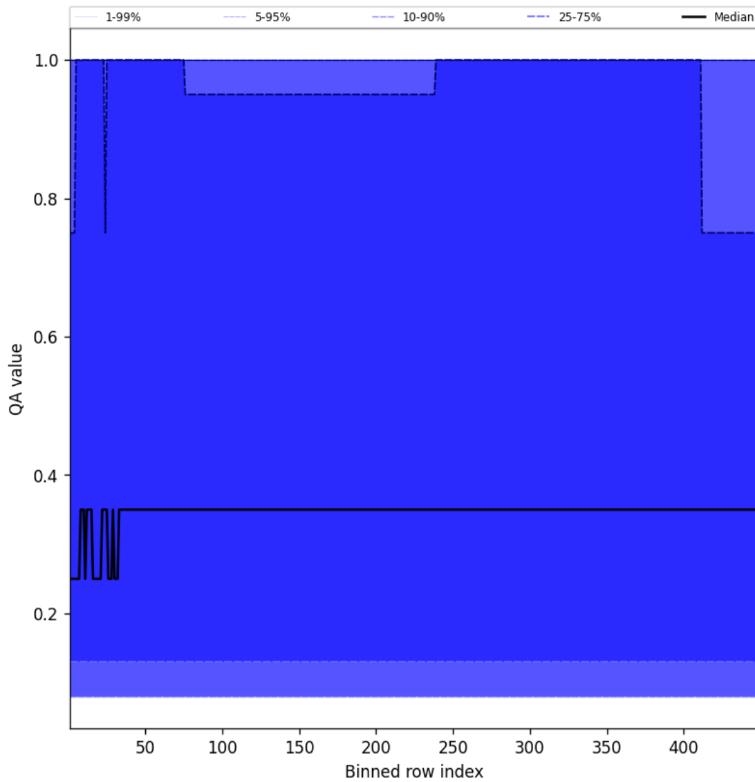
Figure 46: Along track statistics of “QA value” for 2025-04-26 to 2025-04-27
