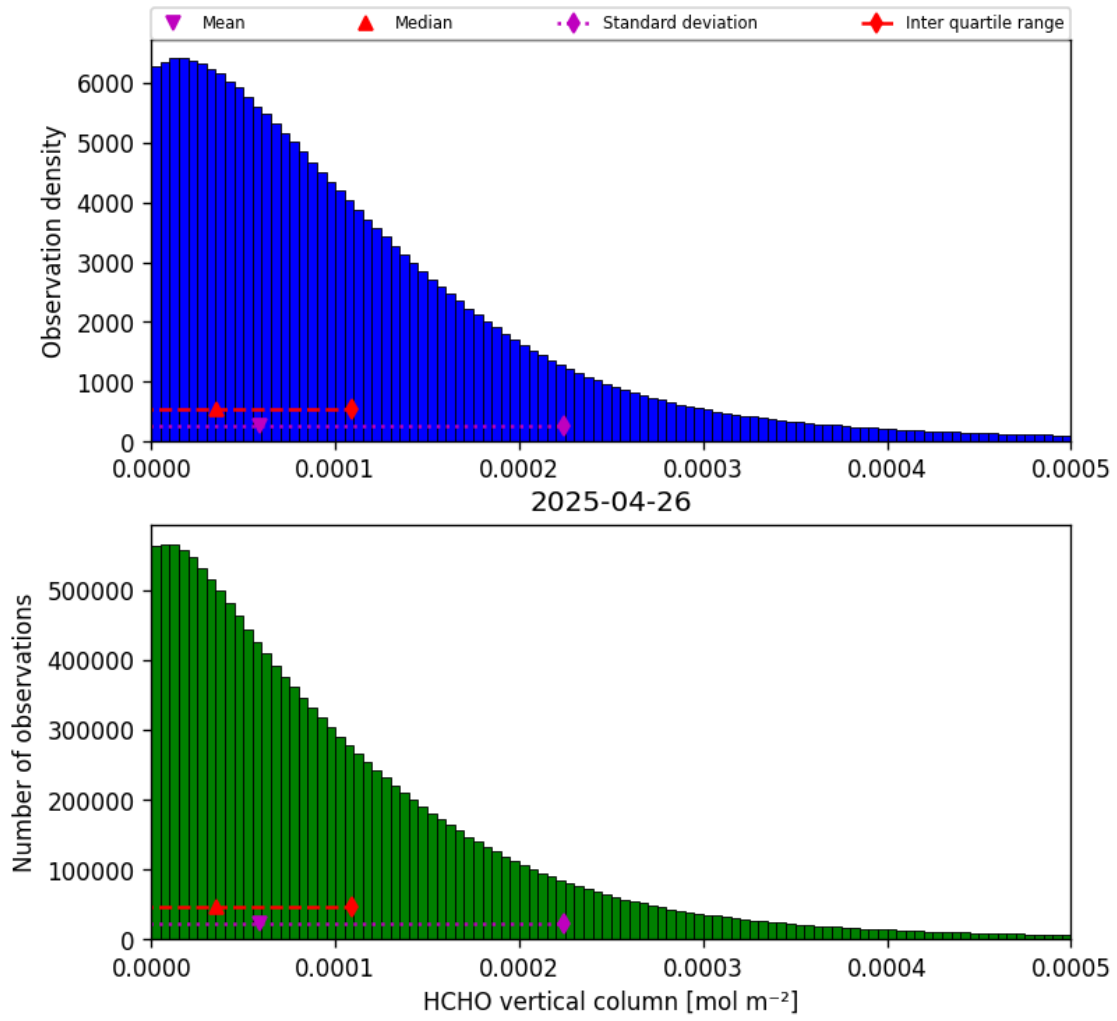
Figure 33: Histogram of “HCHO vertical column” for 2025-04-26 to 2025-04-27
