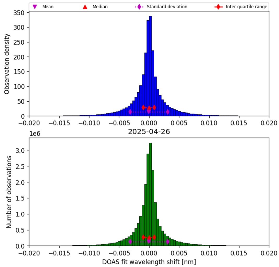
Figure 42: Histogram of “DOAS fit wavelength shift” for 2025-04-26 to 2025-04-27
