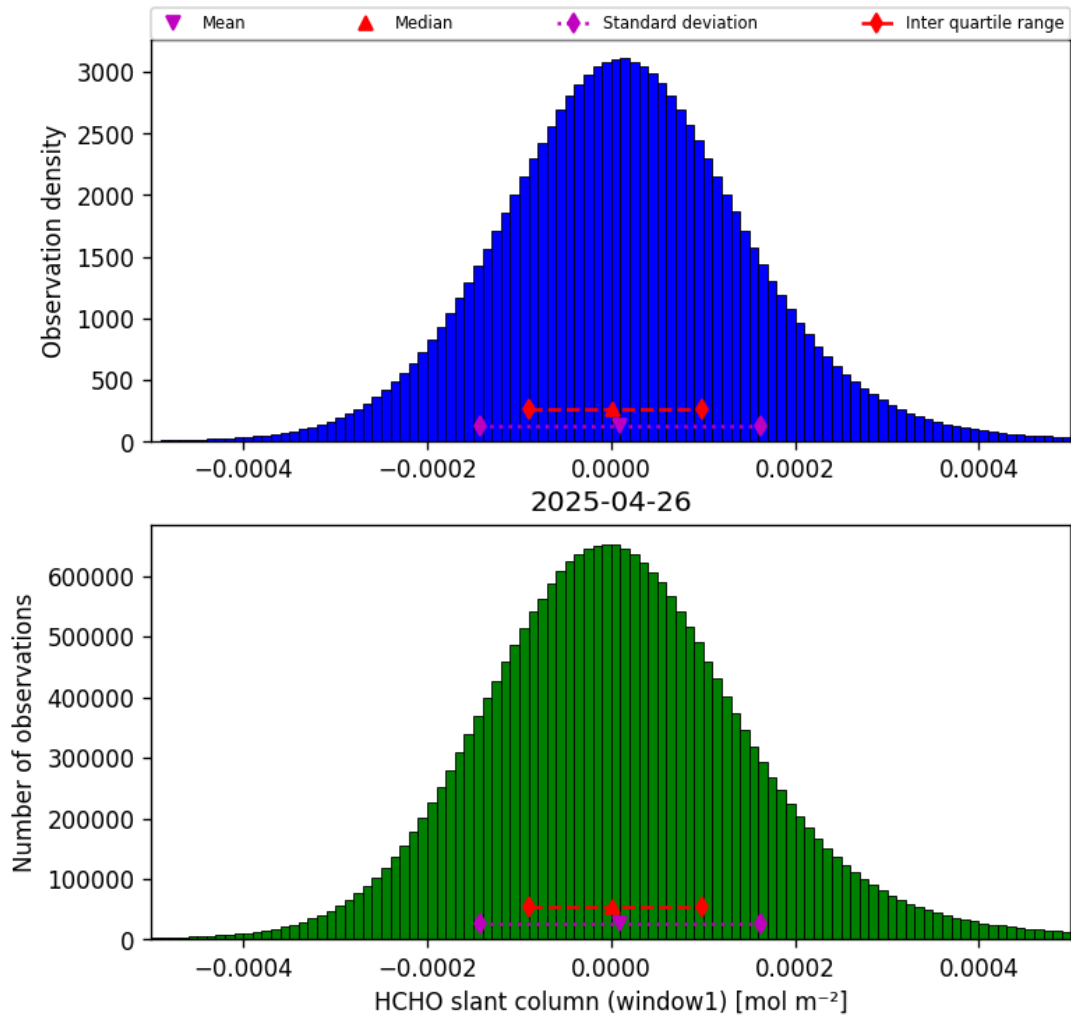
Figure 36: Histogram of “HCHO slant column (window1)” for 2025-04-26 to 2025-04-27
