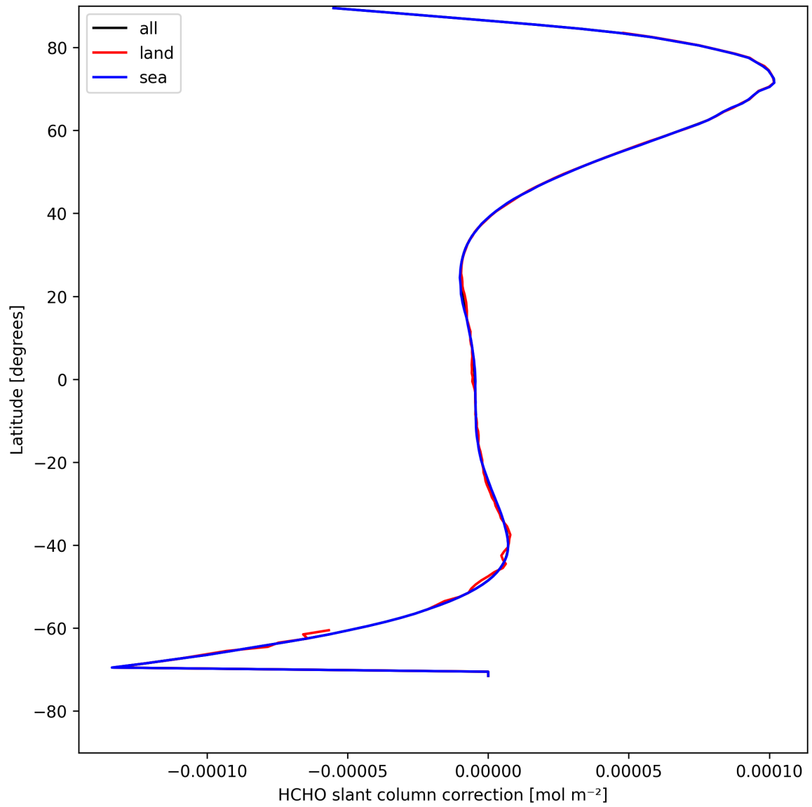
Figure 31: Zonal average of "HCHO slant column correction" for 2025-04-26 to 2025-04-27.
