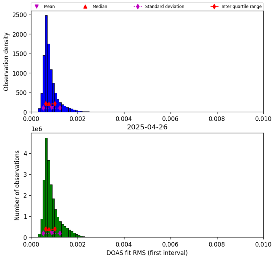
Figure 44: Histogram of “DOAS fit RMS (first interval)” for 2025-04-26 to 2025-04-27
