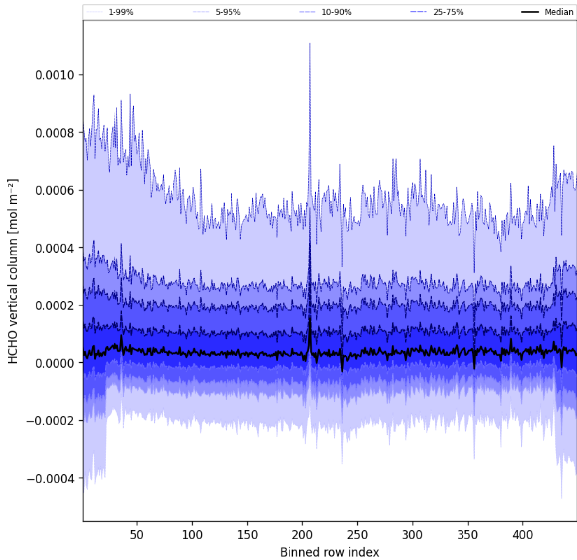
Figure 47: Along track statistics of “HCHO vertical column” for 2025-04-26 to 2025-04-27
