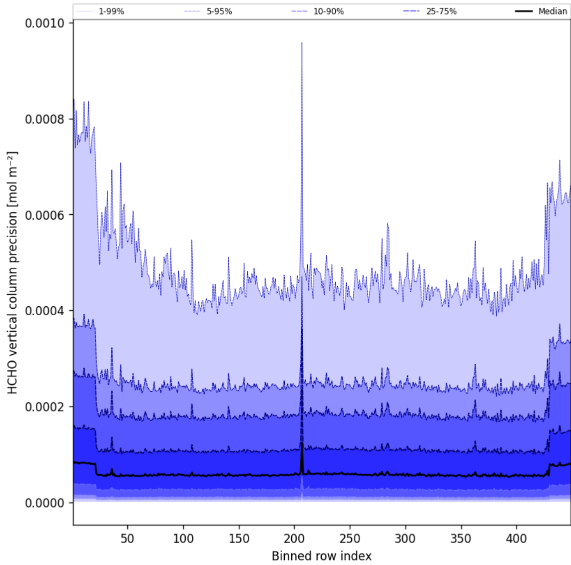
Figure 48: Along track statistics of “HCHO vertical column precision” for 2025-04-26 to 2025-04-27
