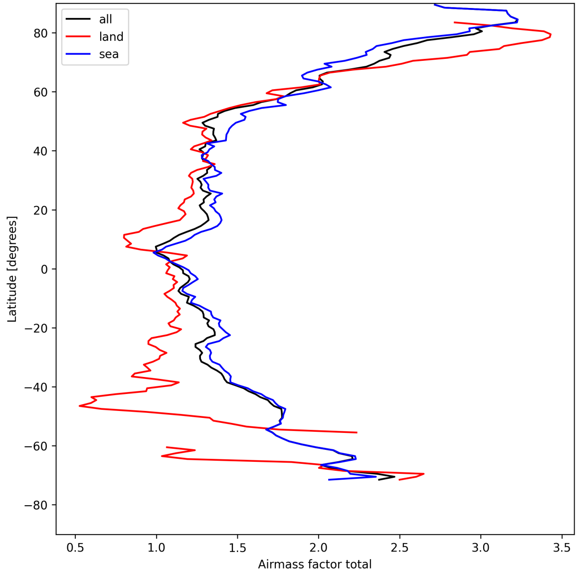
Figure 24: Zonal average of “Airmass factor total” for 2025-04-26 to 2025-04-27.
