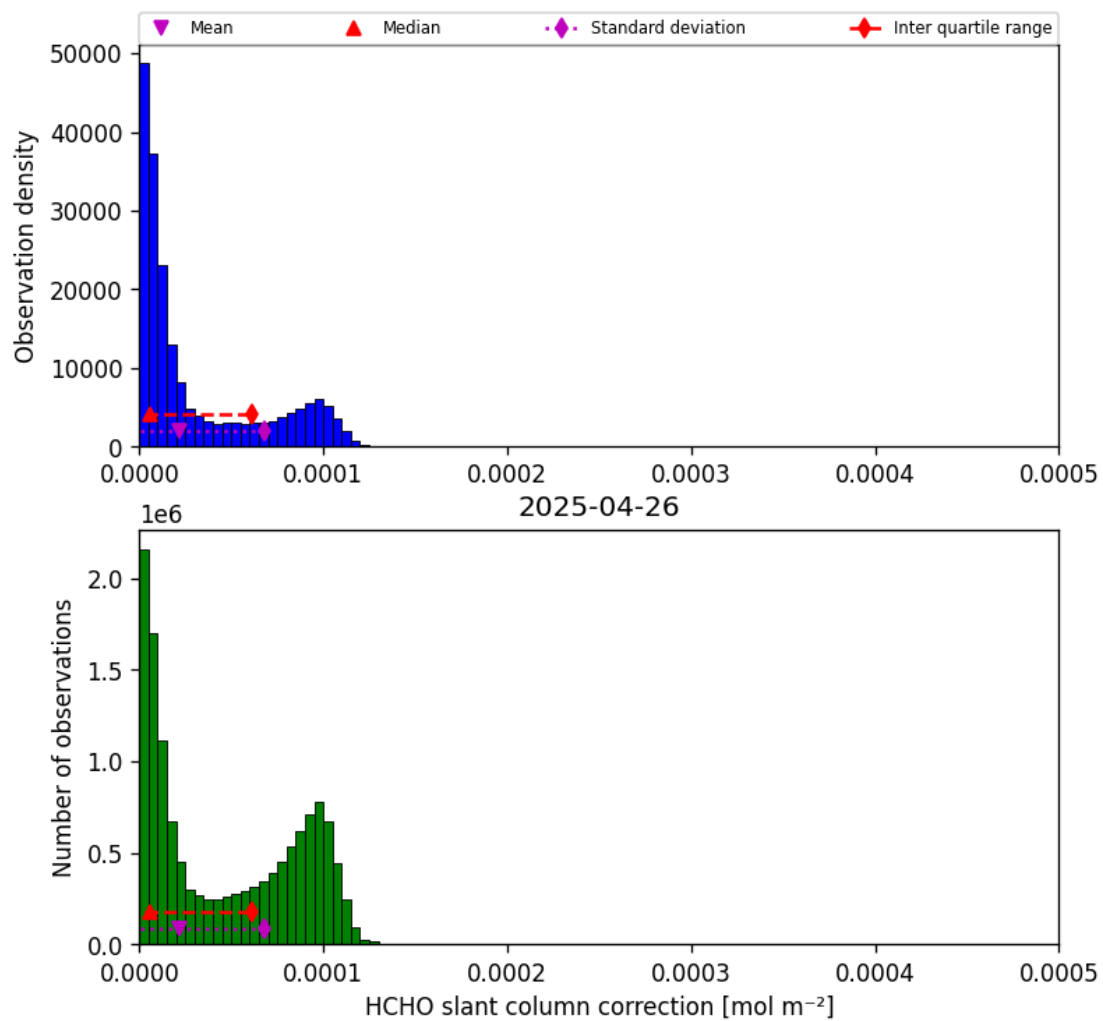
Figure 45: Histogram of “HCHO slant column correction” for 2025-04-26 to 2025-04-27
