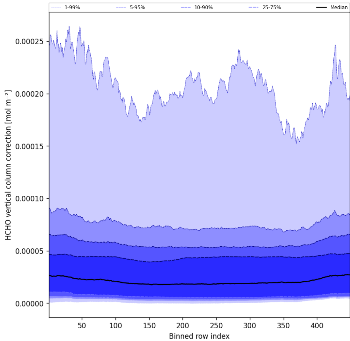
Figure 49: Along track statistics of “HCHO vertical column correction” for 2025-04-26 to 2025-04-27
