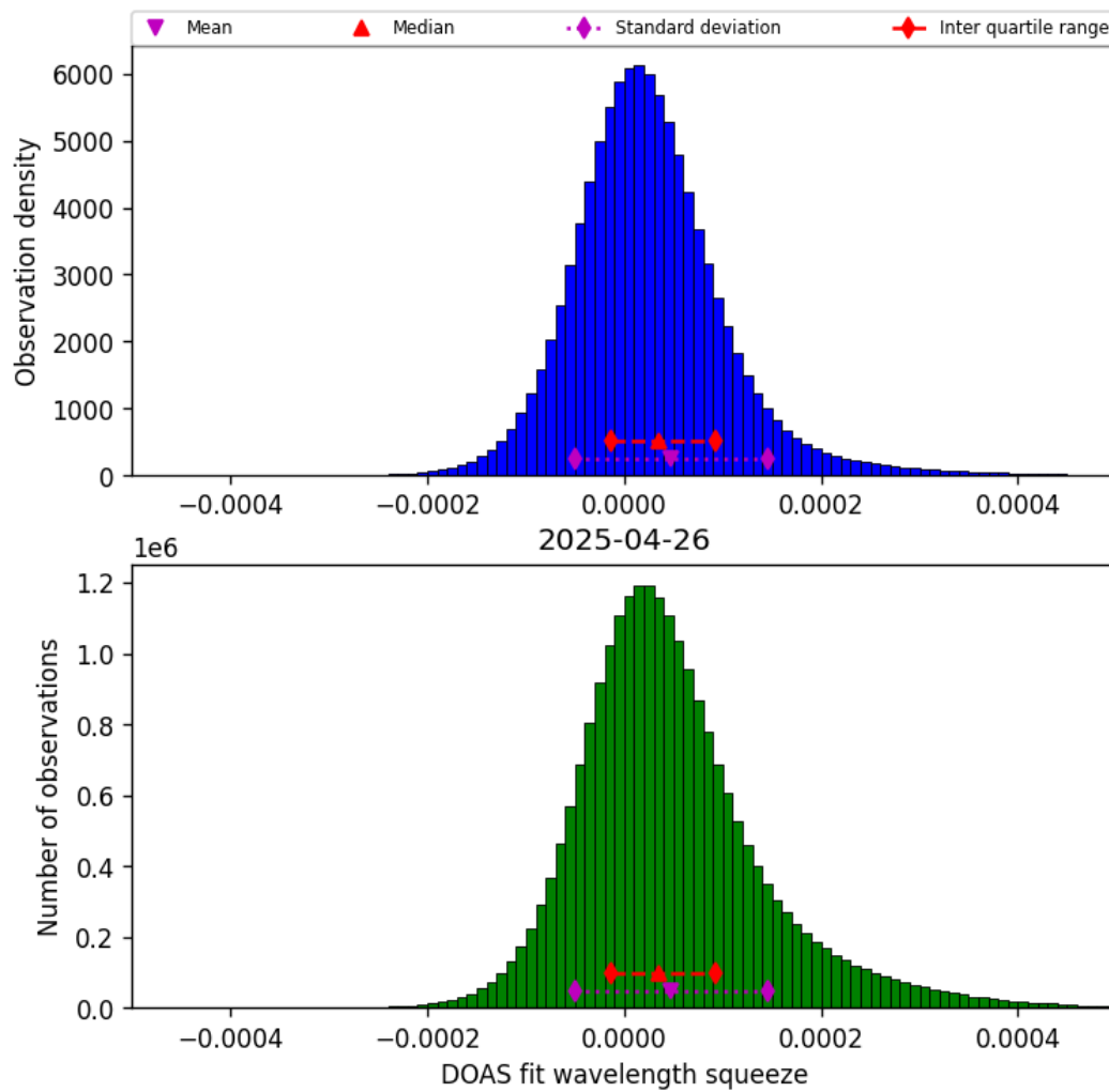
Figure 43: Histogram of “DOAS fit wavelength squeeze” for 2025-04-26 to 2025-04-27
