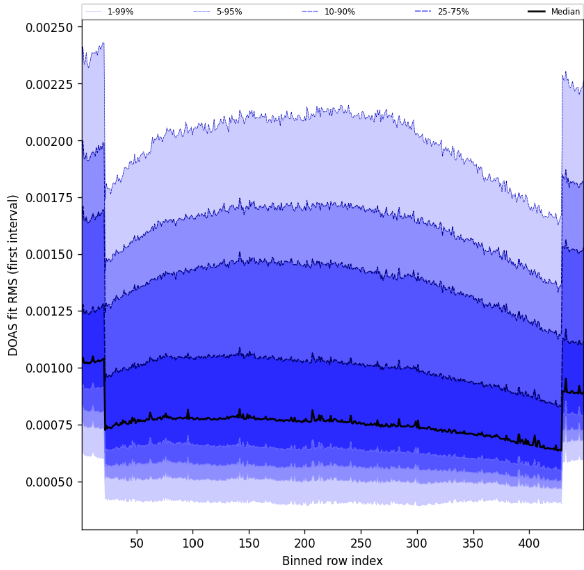
Figure 58: Along track statistics of “DOAS fit RMS (first interval)” for 2025-04-26 to 2025-04-27
