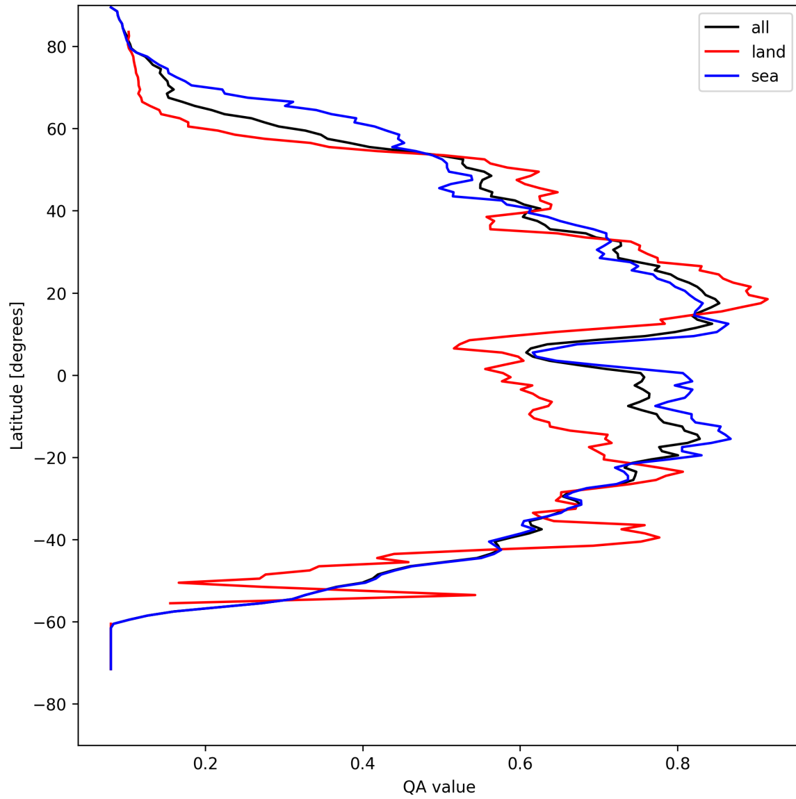
Figure 18: Zonal average of “QA value” for 2025-04-26 to 2025-04-27.
