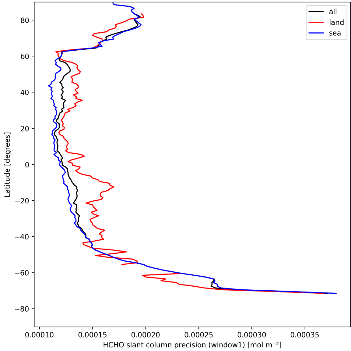
Figure 23: Zonal average of “HCHO slant column precision (window1)” for 2025-04-26 to 2025-04-27.
