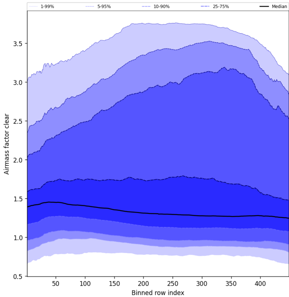
Figure 54: Along track statistics of “Airmass factor clear” for 2025-04-26 to 2025-04-27
