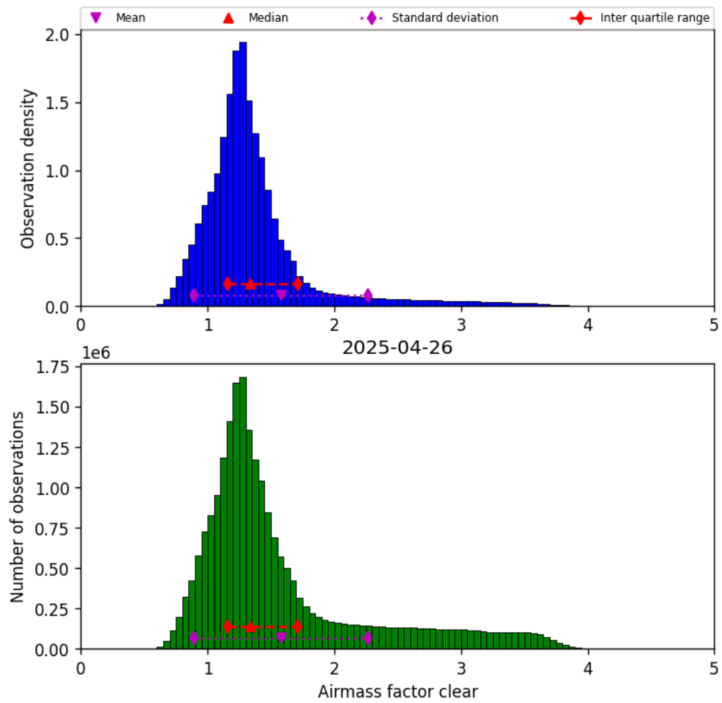
Figure 40: Histogram of “Airmass factor clear” for 2025-04-26 to 2025-04-27
