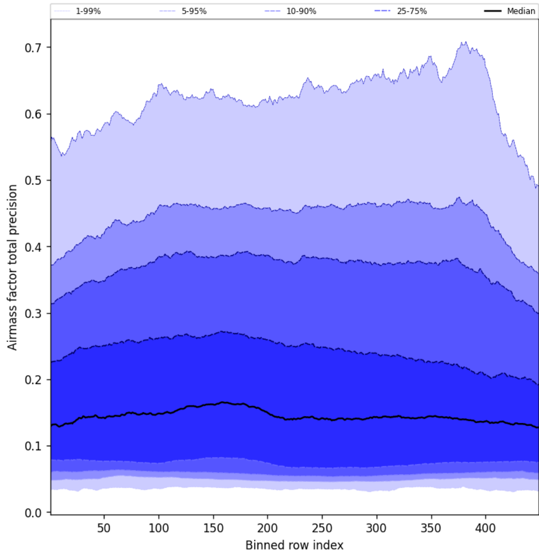
Figure 53: Along track statistics of “Airmass factor total precision” for 2025-04-26 to 2025-04-27
