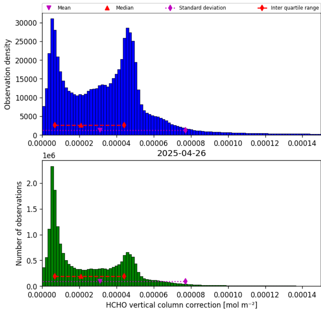
Figure 35: Histogram of “HCHO vertical column correction” for 2025-04-26 to 2025-04-27
