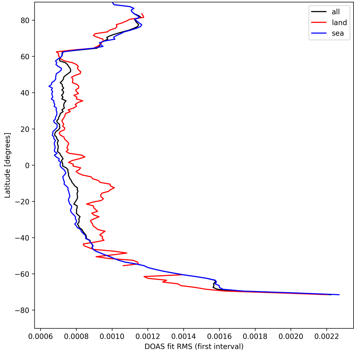
Figure 30: Zonal average of "DOAS fit RMS (first interval)" for 2025-04-26 to 2025-04-27.
