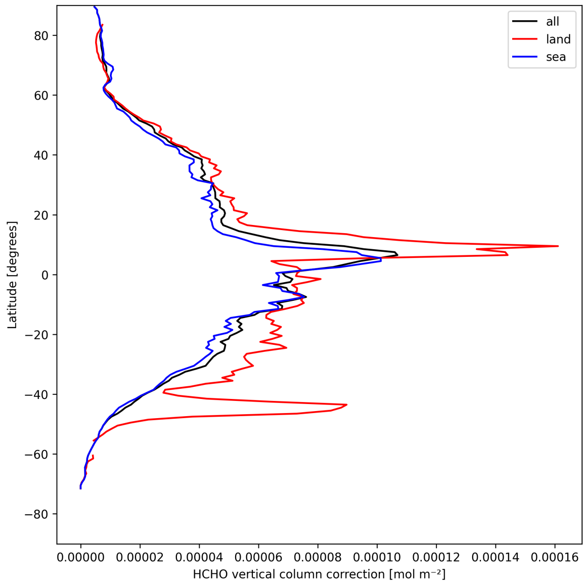
Figure 21: Zonal average of “HCHO vertical column correction” for 2025-04-26 to 2025-04-27.
