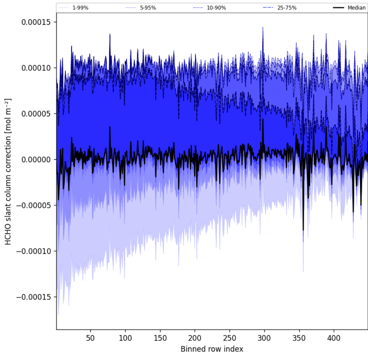
Figure 59: Along track statistics of “HCHO slant column correction” for 2025-04-27 to 2025-04-27
