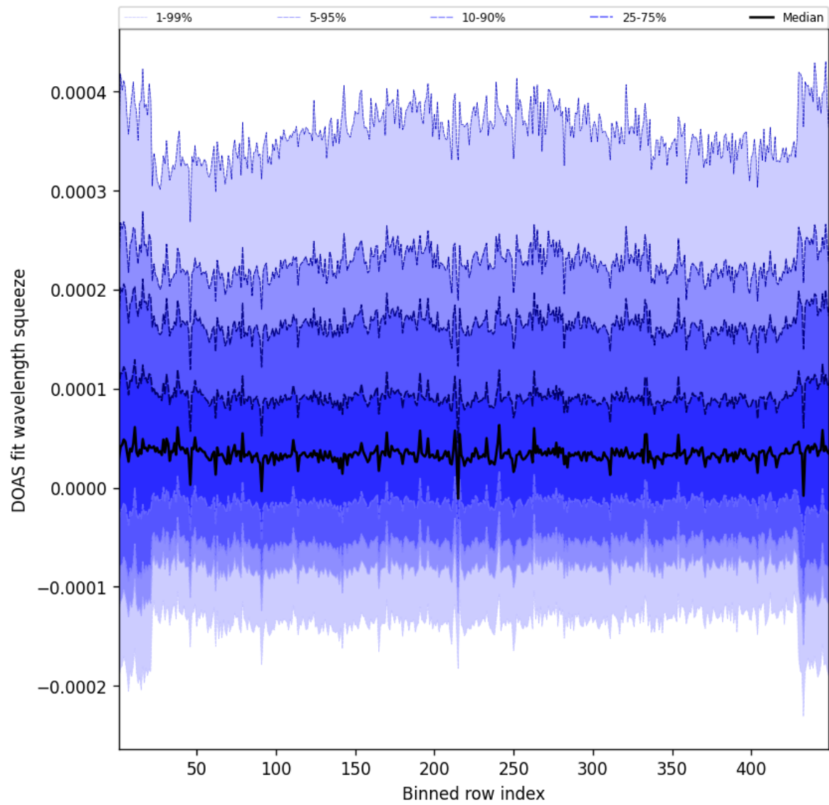
Figure 57: Along track statistics of “DOAS fit wavelength squeeze” for 2025-04-27 to 2025-04-27
