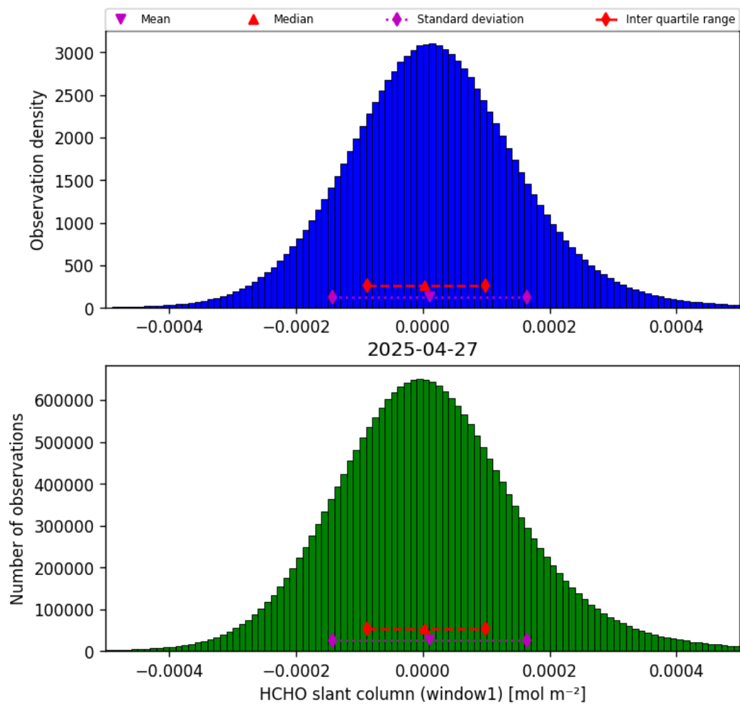
Figure 36: Histogram of “HCHO slant column (window1)” for 2025-04-27 to 2025-04-27
