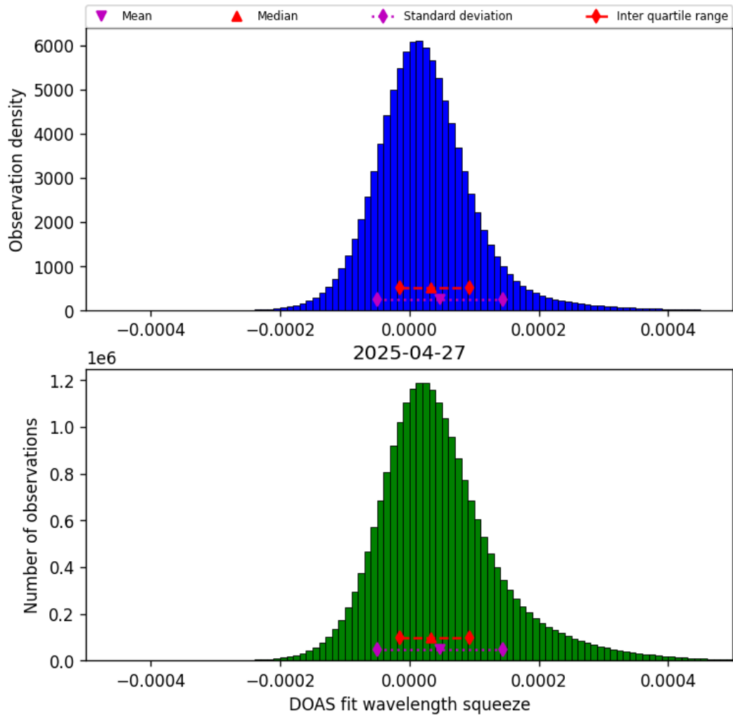
Figure 43: Histogram of “DOAS fit wavelength squeeze” for 2025-04-27 to 2025-04-27
