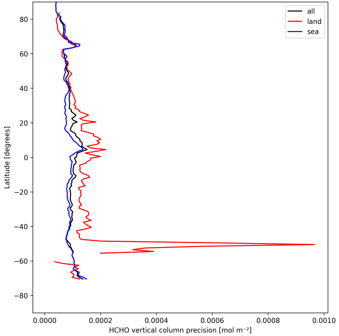
Figure 20: Zonal average of “HCHO vertical column precision” for 2025-04-27 to 2025-04-27.
