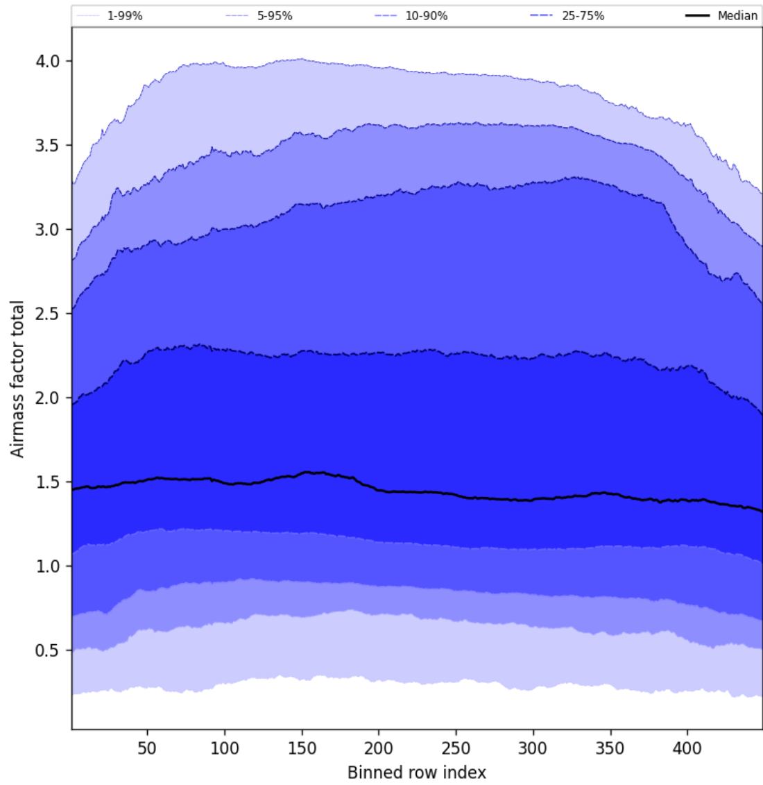
Figure 52: Along track statistics of “Airmass factor total” for 2025-04-27 to 2025-04-27
