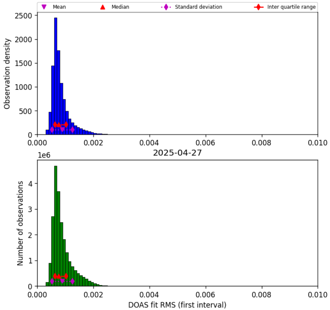
Figure 44: Histogram of “DOAS fit RMS (first interval)” for 2025-04-27 to 2025-04-27
