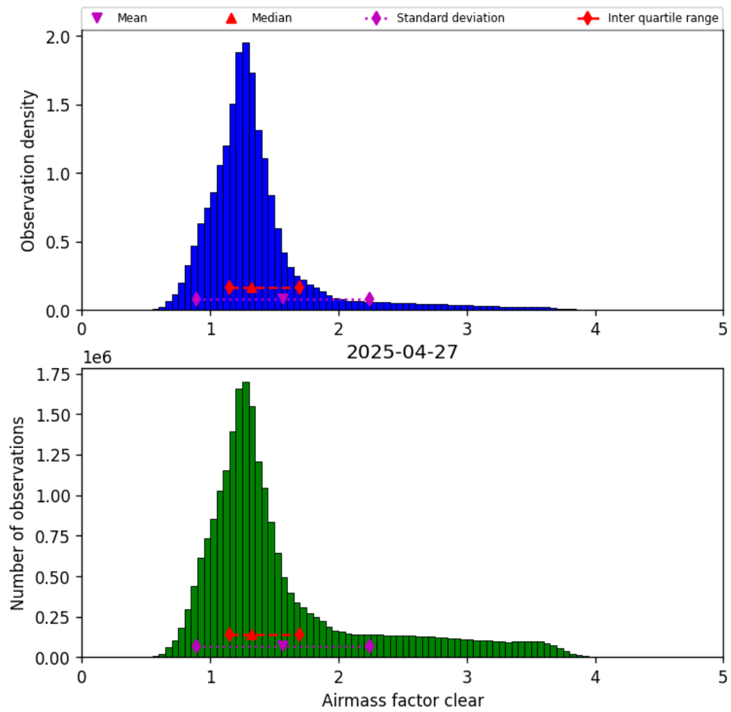
Figure 40: Histogram of “Airmass factor clear” for 2025-04-27 to 2025-04-27
