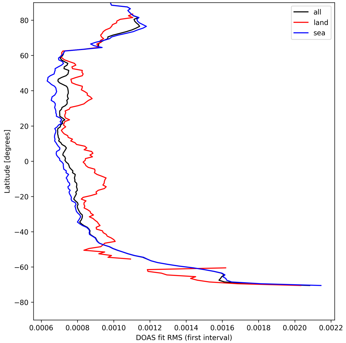
Figure 30: Zonal average of “DOAS fit RMS (first interval)” for 2025-04-27 to 2025-04-27.
