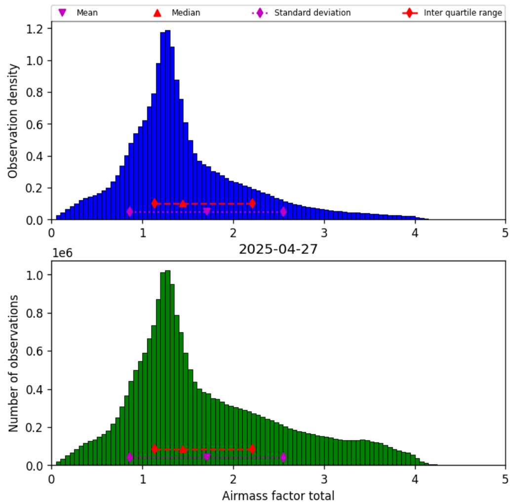
Figure 38: Histogram of “Airmass factor total” for 2025-04-27 to 2025-04-27
