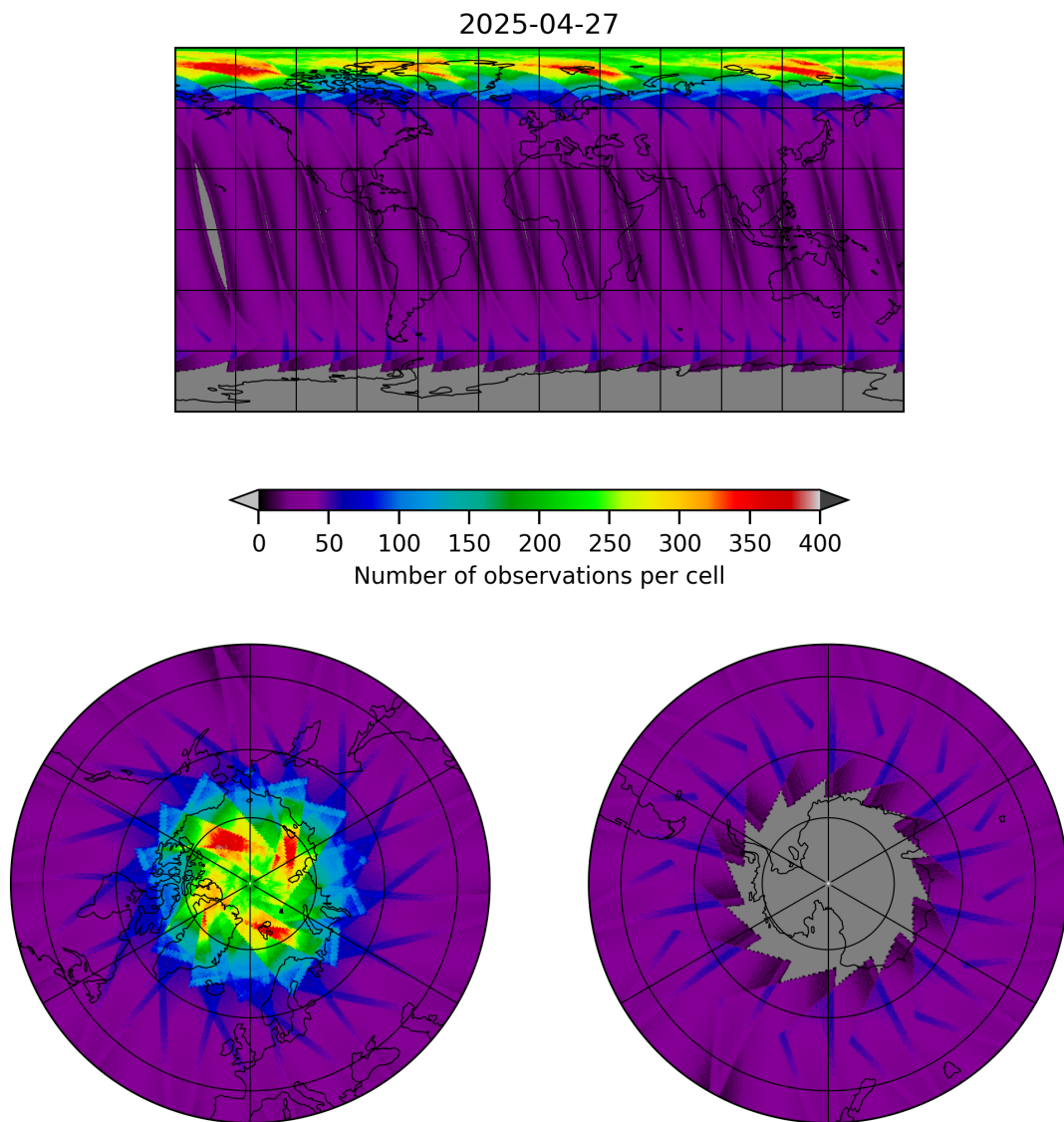
Figure 17: Map of the number of observations for 2025-04-27 to 2025-04-27
