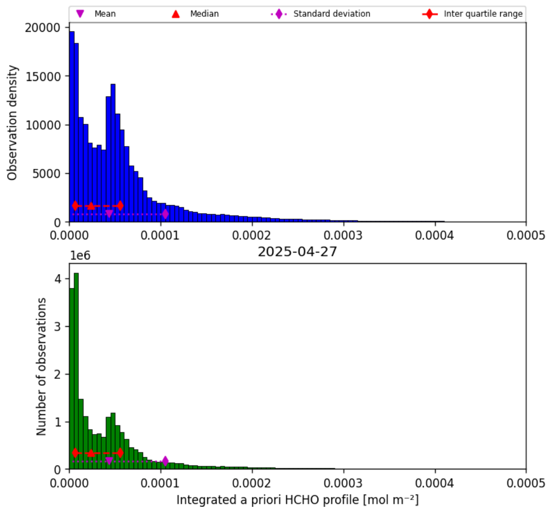
Figure 41: Histogram of “Integrated a priori HCHO profile” for 2025-04-27 to 2025-04-27
