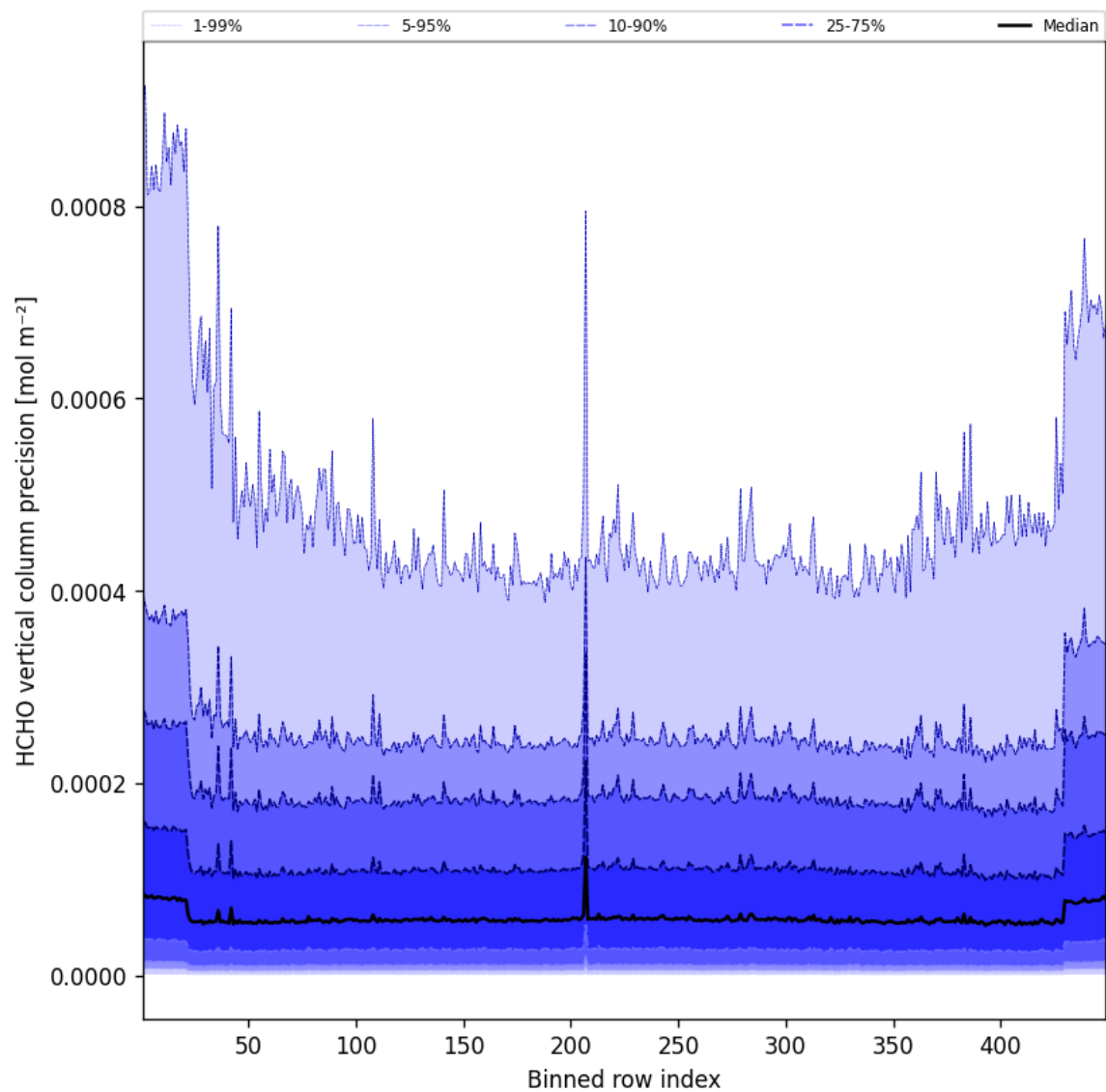
Figure 48: Along track statistics of “HCHO vertical column precision” for 2025-04-27 to 2025-04-27
