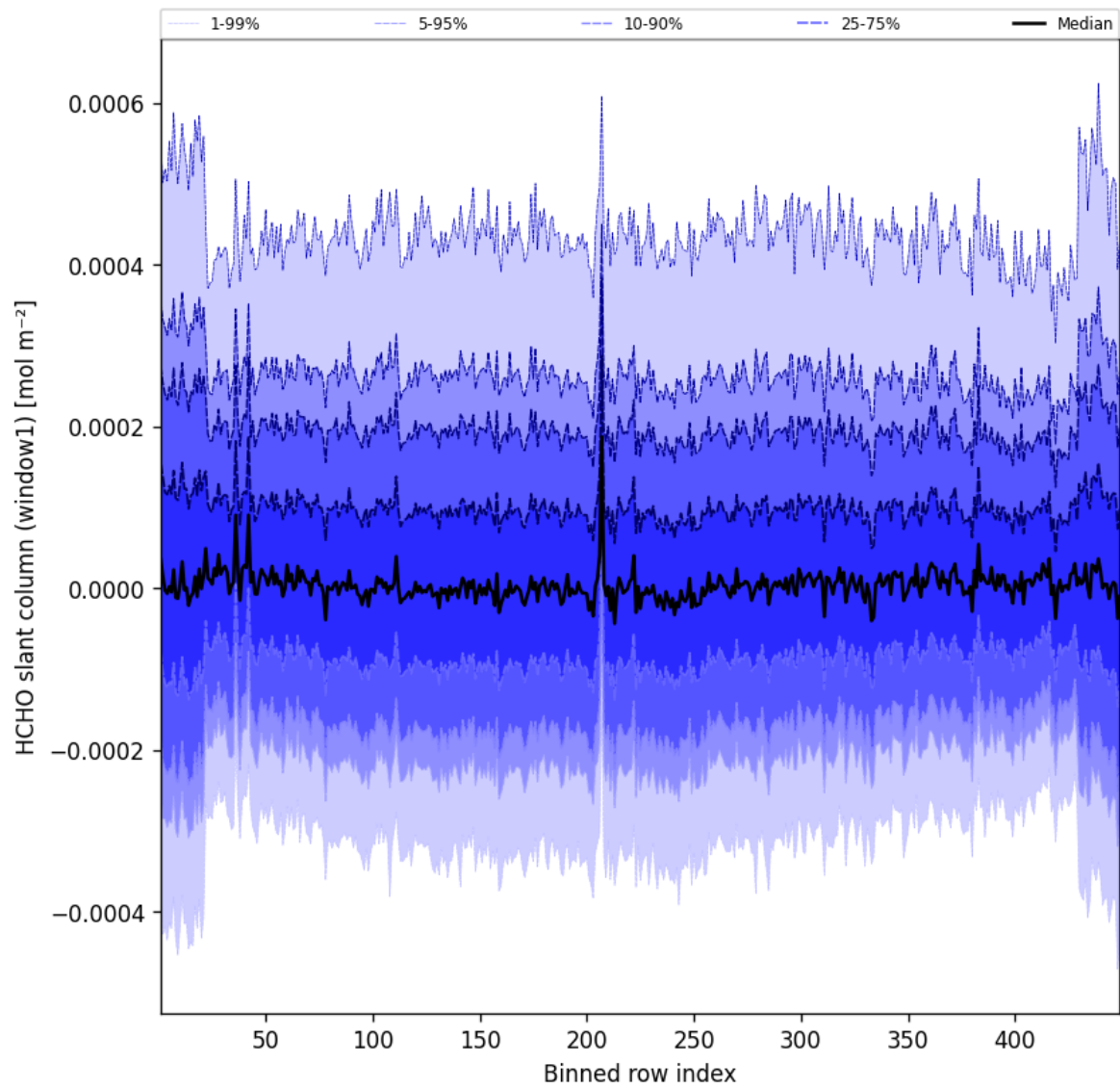
Figure 50: Along track statistics of “HCHO slant column (window1)” for 2025-04-27 to 2025-04-27
