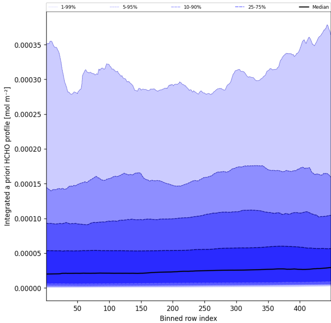
Figure 55: Along track statistics of “Integrated a priori HCHO profile” for 2025-04-27 to 2025-04-27
