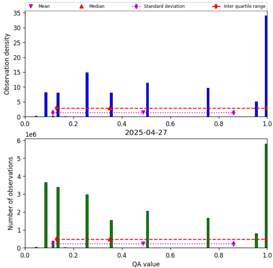
Figure 32: Histogram of “QA value” for 2025-04-27 to 2025-04-27
