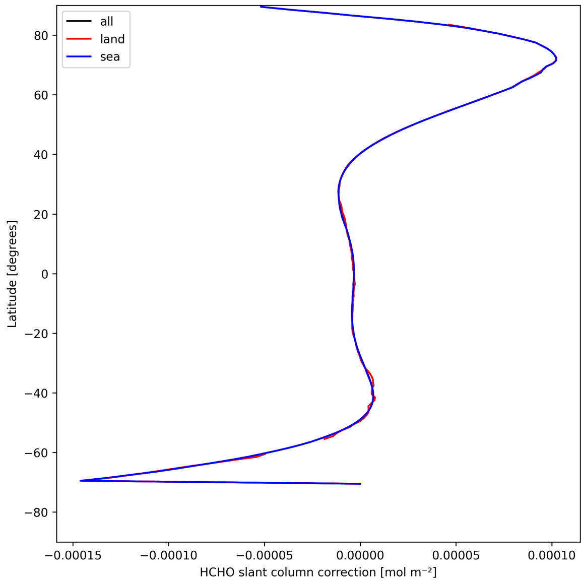
Figure 31: Zonal average of “HCHO slant column correction” for 2025-04-27 to 2025-04-27.
