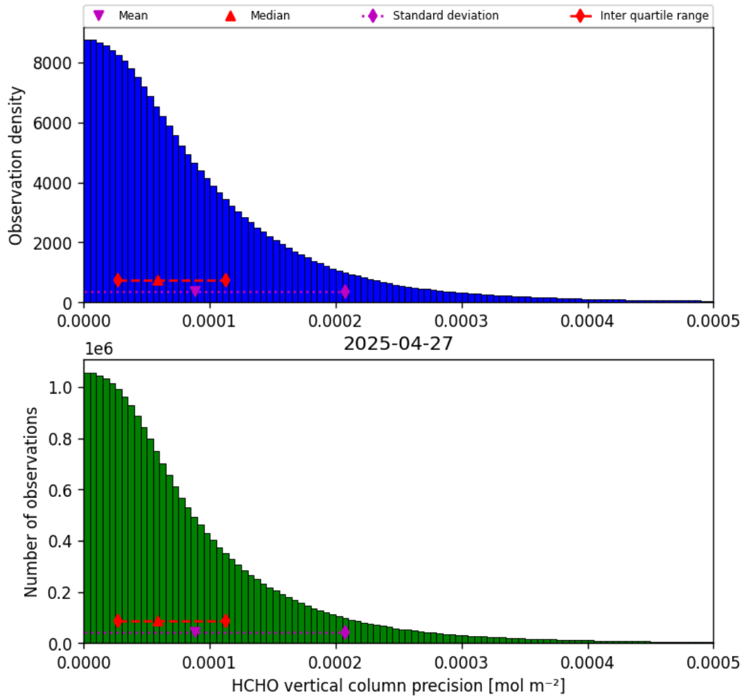
Figure 34: Histogram of “HCHO vertical column precision” for 2025-04-27 to 2025-04-27
