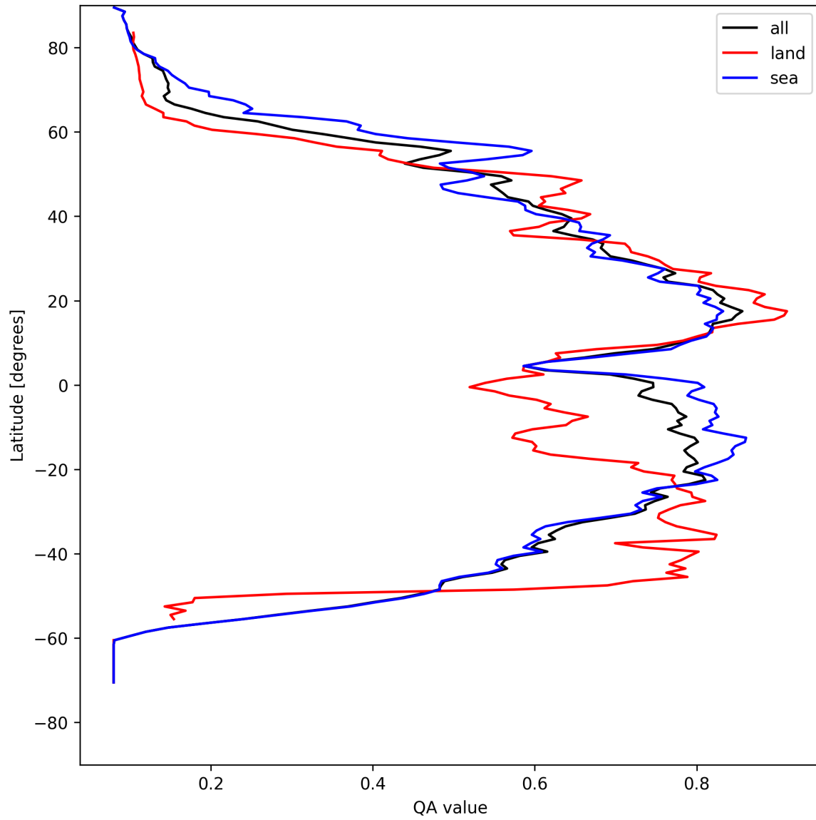
Figure 18: Zonal average of “QA value” for 2025-04-27 to 2025-04-27.
