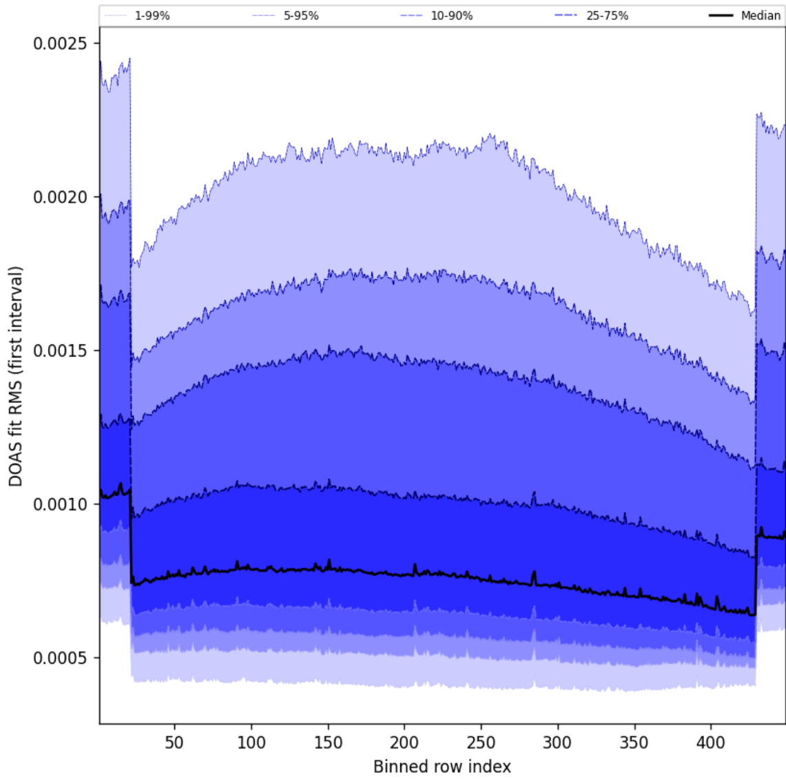
Figure 58: Along track statistics of “DOAS fit RMS (first interval)” for 2025-04-27 to 2025-04-27
