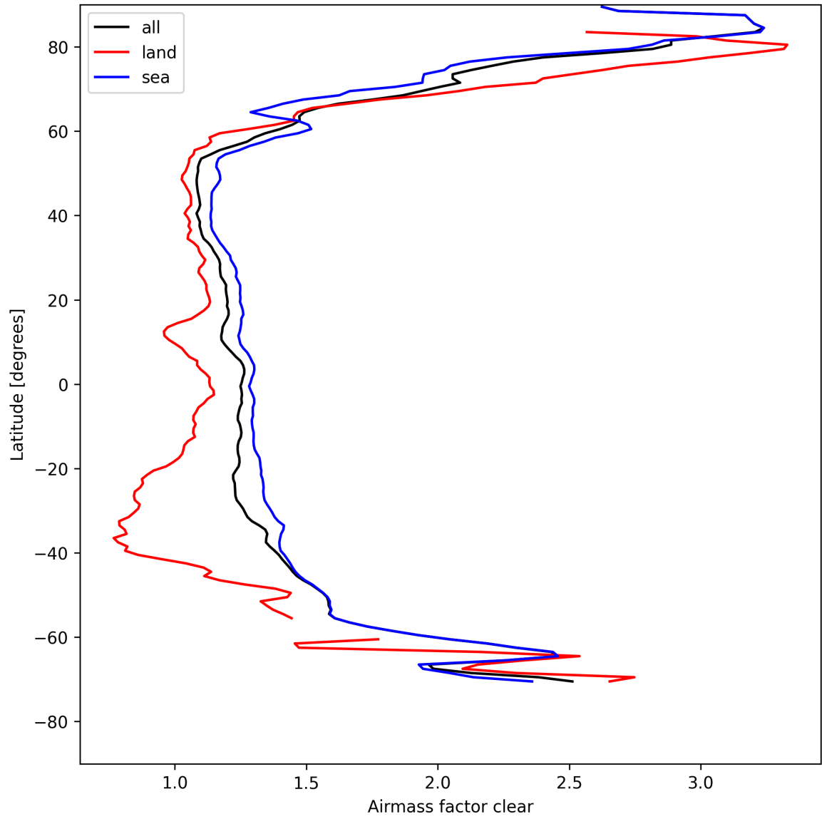
Figure 26: Zonal average of “Airmass factor clear” for 2025-04-27 to 2025-04-27.
