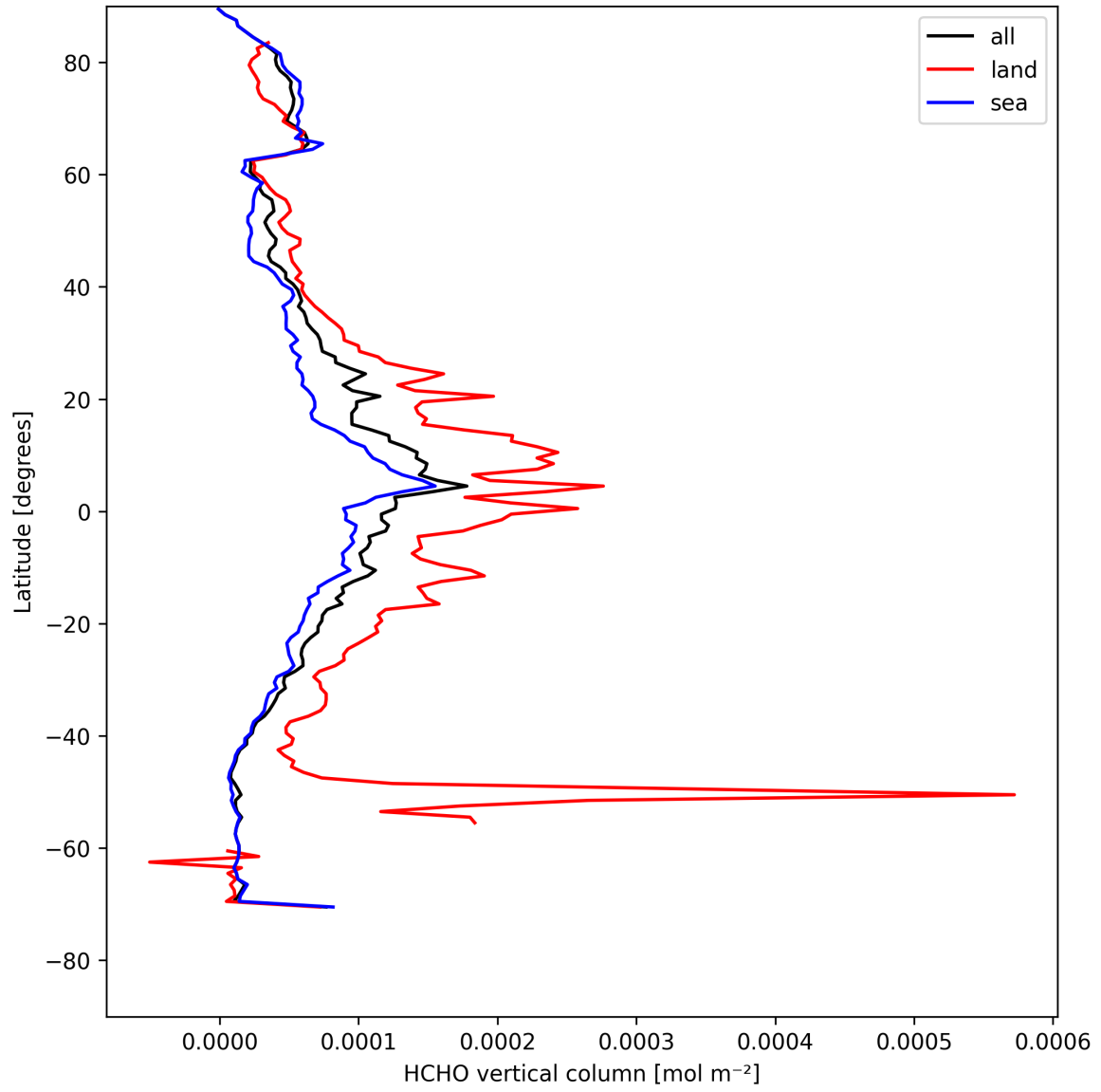
Figure 19: Zonal average of “HCHO vertical column” for 2025-04-27 to 2025-04-27.
