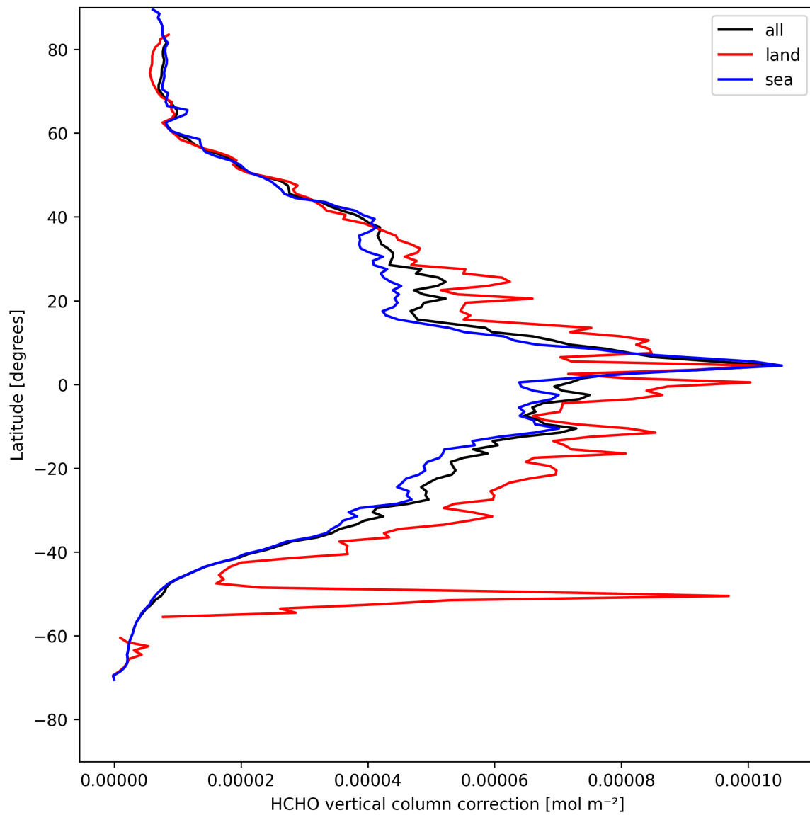
Figure 21: Zonal average of “HCHO vertical column correction” for 2025-04-27 to 2025-04-27.
