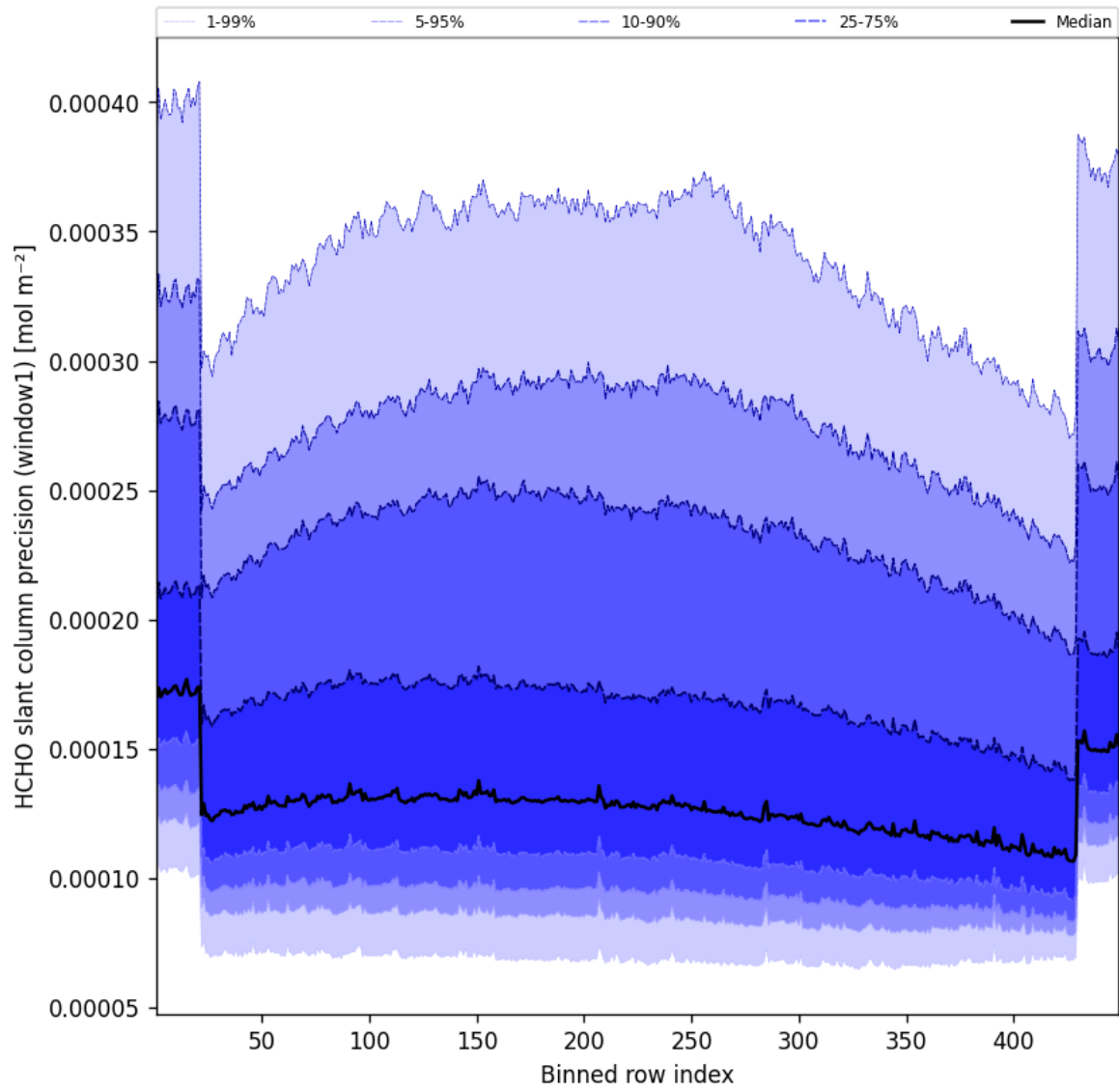
Figure 51: Along track statistics of “HCHO slant column precision (window1)” for 2025-04-27 to 2025-04-27
