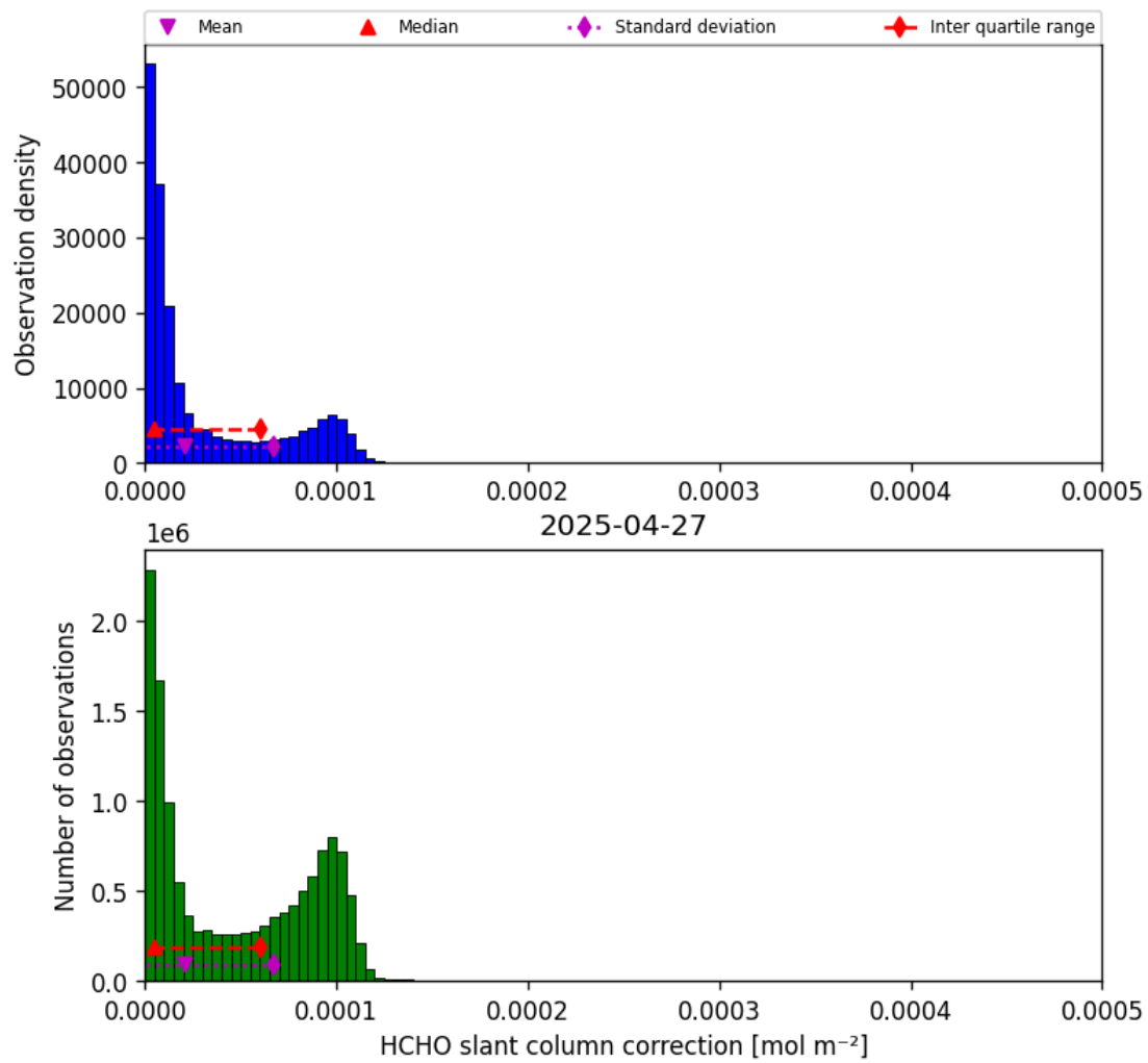
Figure 45: Histogram of “HCHO slant column correction” for 2025-04-27 to 2025-04-27
