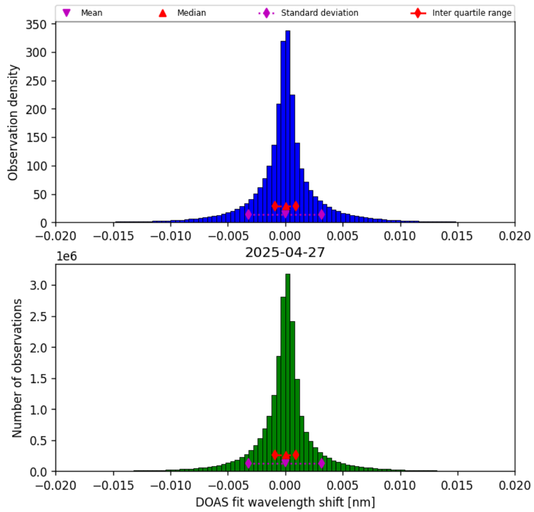
Figure 42: Histogram of “DOAS fit wavelength shift” for 2025-04-27 to 2025-04-27
