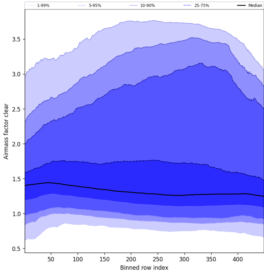
Figure 54: Along track statistics of “Airmass factor clear” for 2025-04-27 to 2025-04-27
