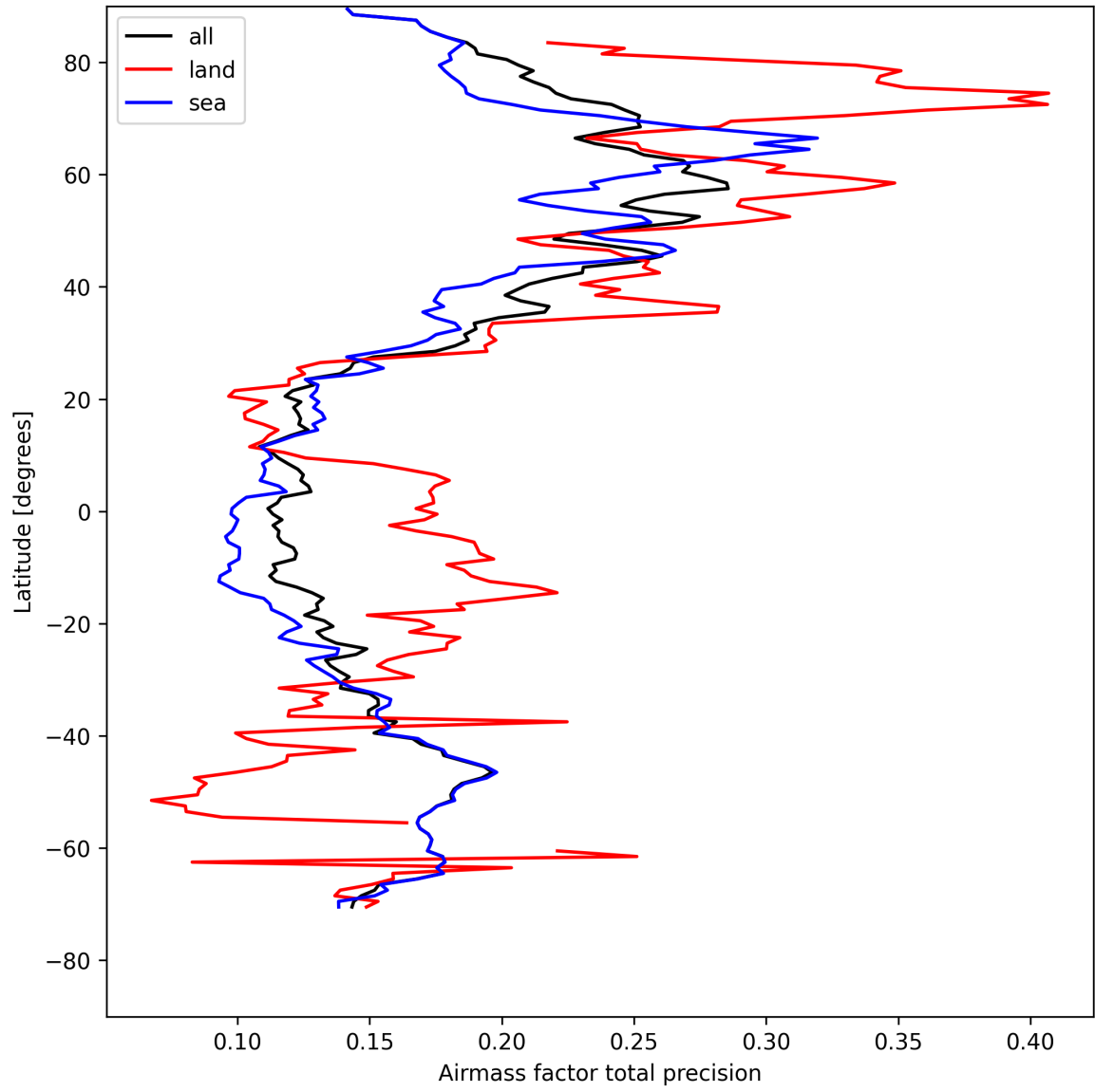
Figure 25: Zonal average of “Airmass factor total precision” for 2025-04-27 to 2025-04-27.
