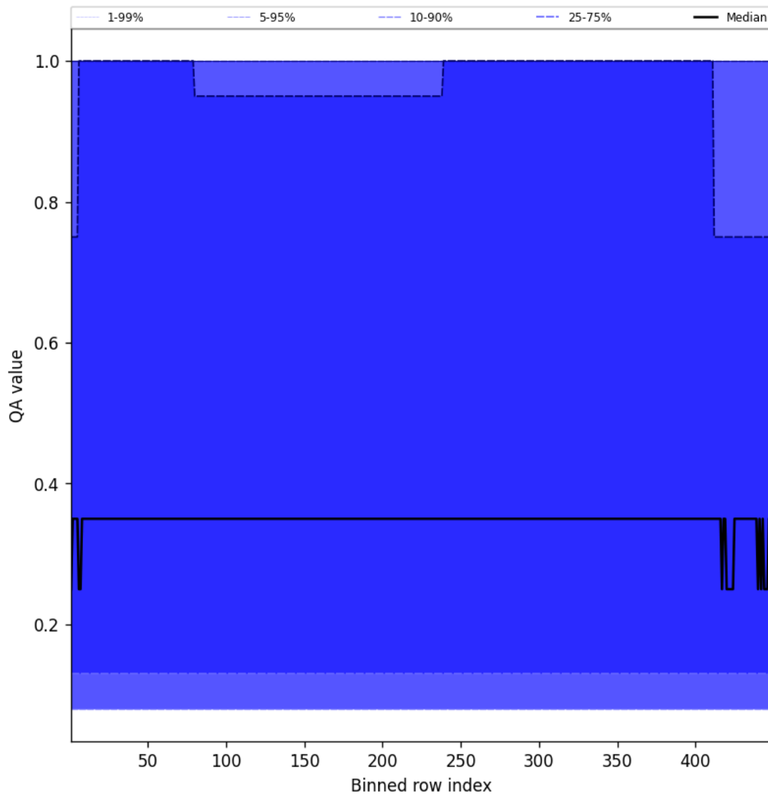
Figure 46: Along track statistics of "QA value" for 2025-04-27 to 2025-04-27
