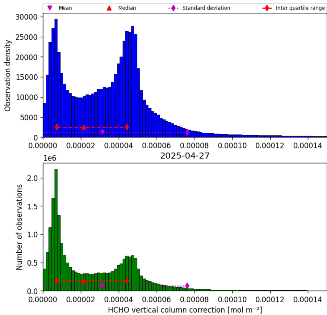
Figure 35: Histogram of “HCHO vertical column correction” for 2025-04-27 to 2025-04-27
