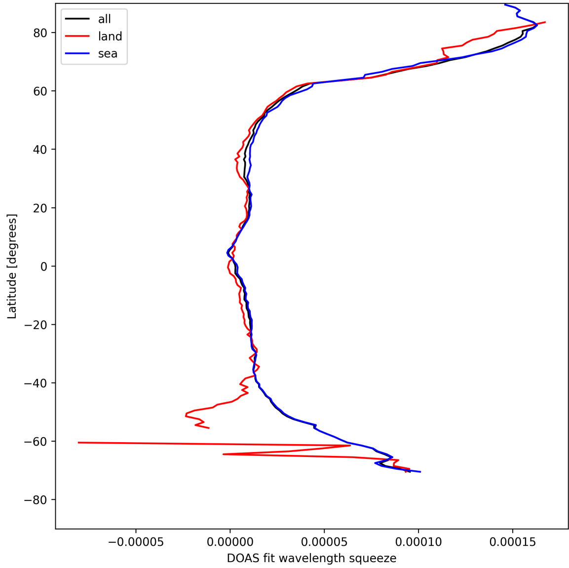
Figure 29: Zonal average of “DOAS fit wavelength squeeze” for 2025-04-27 to 2025-04-27.
