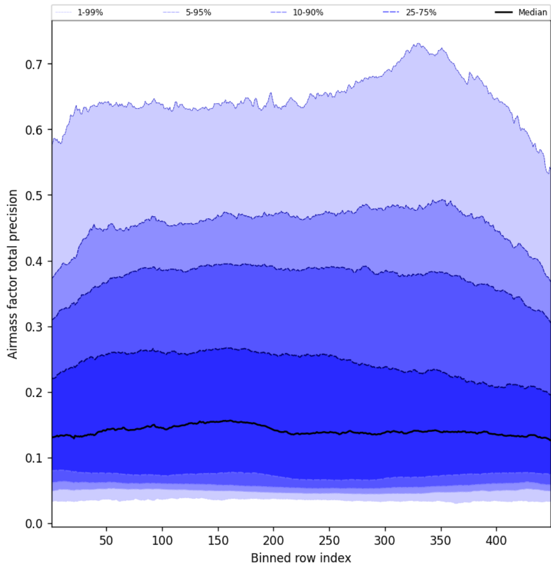
Figure 53: Along track statistics of “Airmass factor total precision” for 2025-04-27 to 2025-04-27
