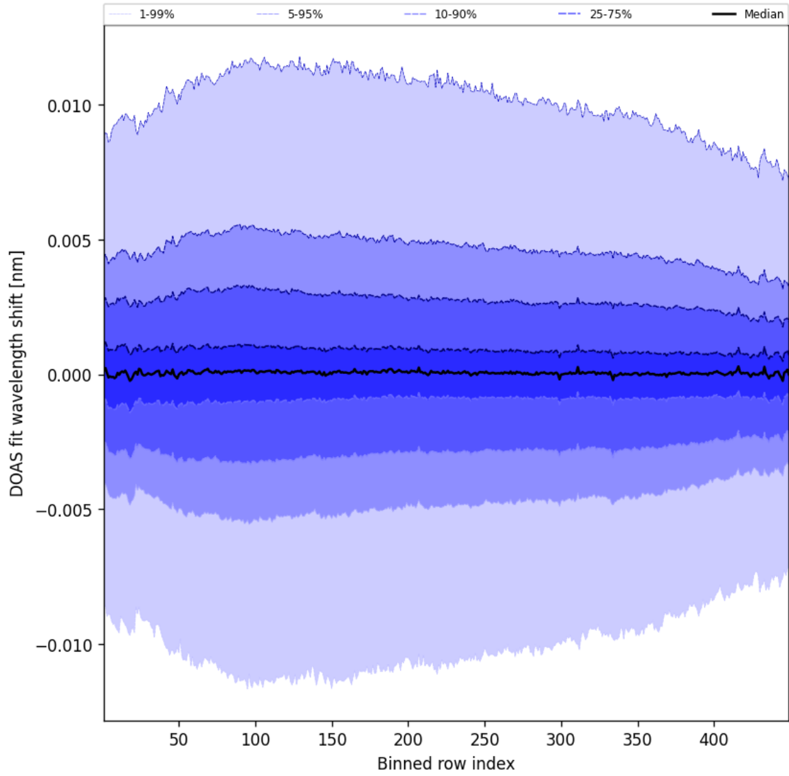
Figure 56: Along track statistics of “DOAS fit wavelength shift” for 2025-04-27 to 2025-04-27
