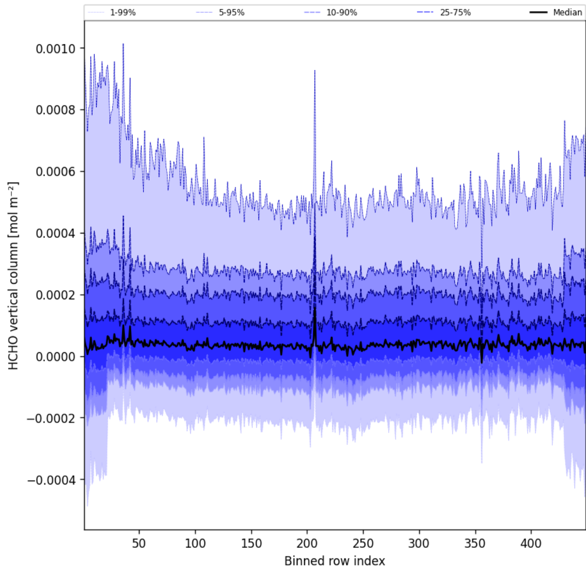
Figure 47: Along track statistics of “HCHO vertical column” for 2025-04-27 to 2025-04-27
