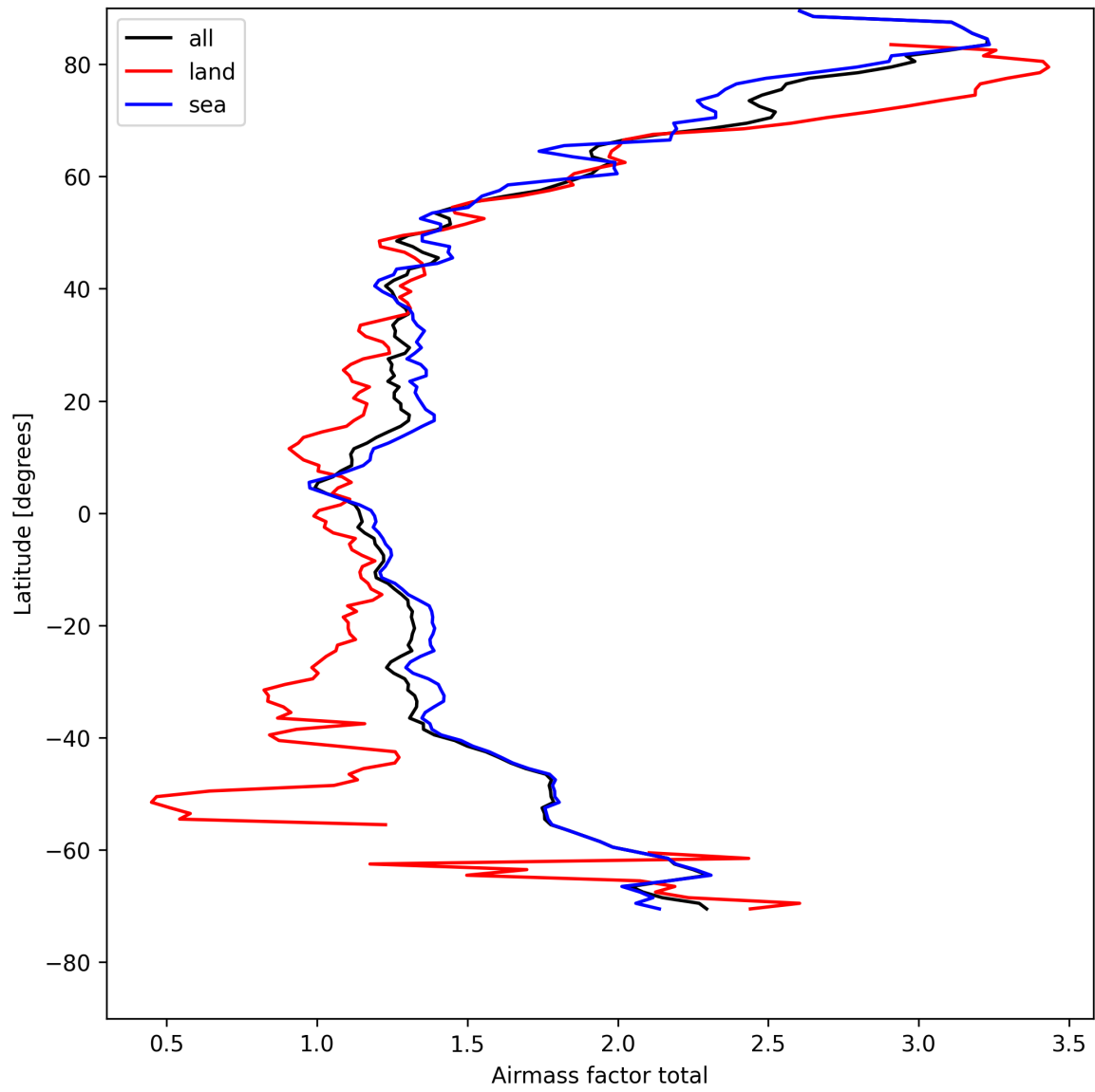
Figure 24: Zonal average of “Airmass factor total” for 2025-04-27 to 2025-04-27.
