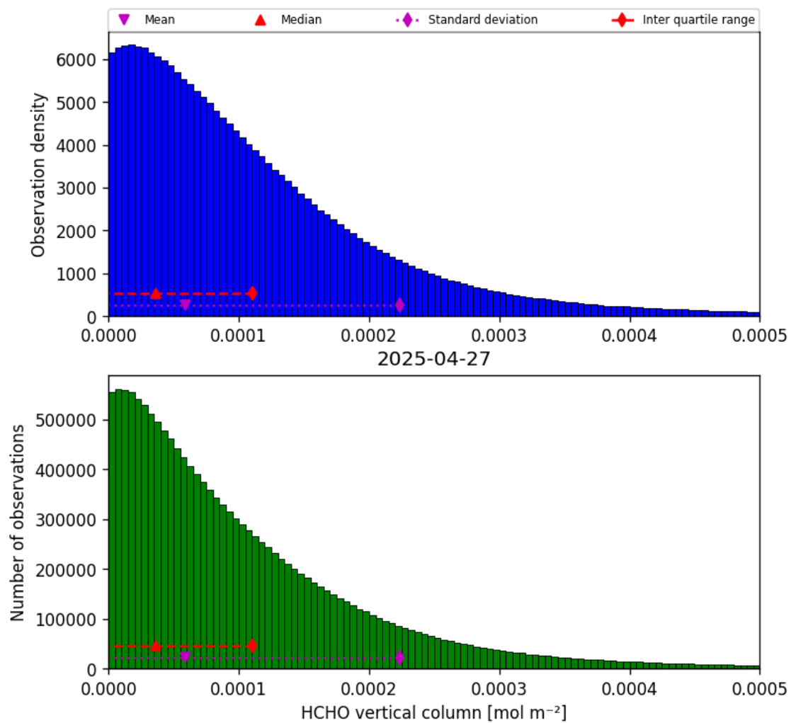
Figure 33: Histogram of “HCHO vertical column” for 2025-04-27 to 2025-04-27
