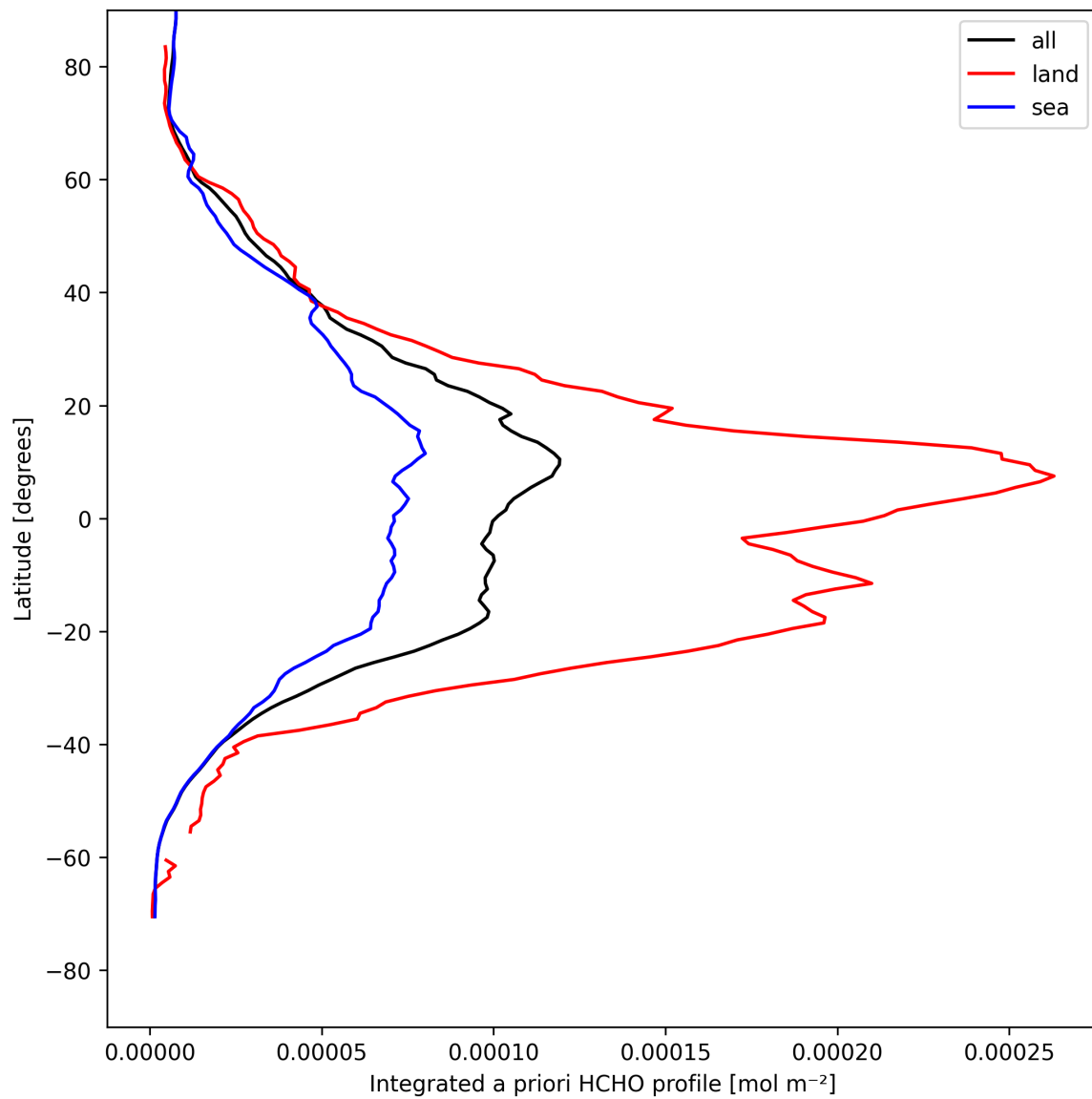
Figure 27: Zonal average of “Integrated a priori HCHO profile” for 2025-04-27 to 2025-04-27.
