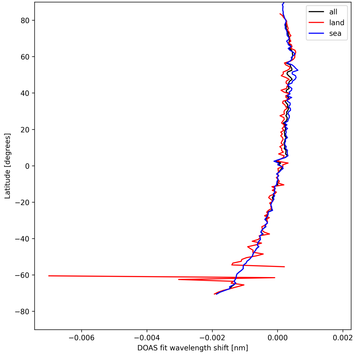
Figure 28: Zonal average of “DOAS fit wavelength shift” for 2025-04-27 to 2025-04-27.
