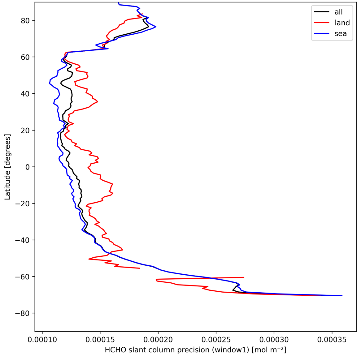
Figure 23: Zonal average of “HCHO slant column precision (window1)” for 2025-04-27 to 2025-04-27.
