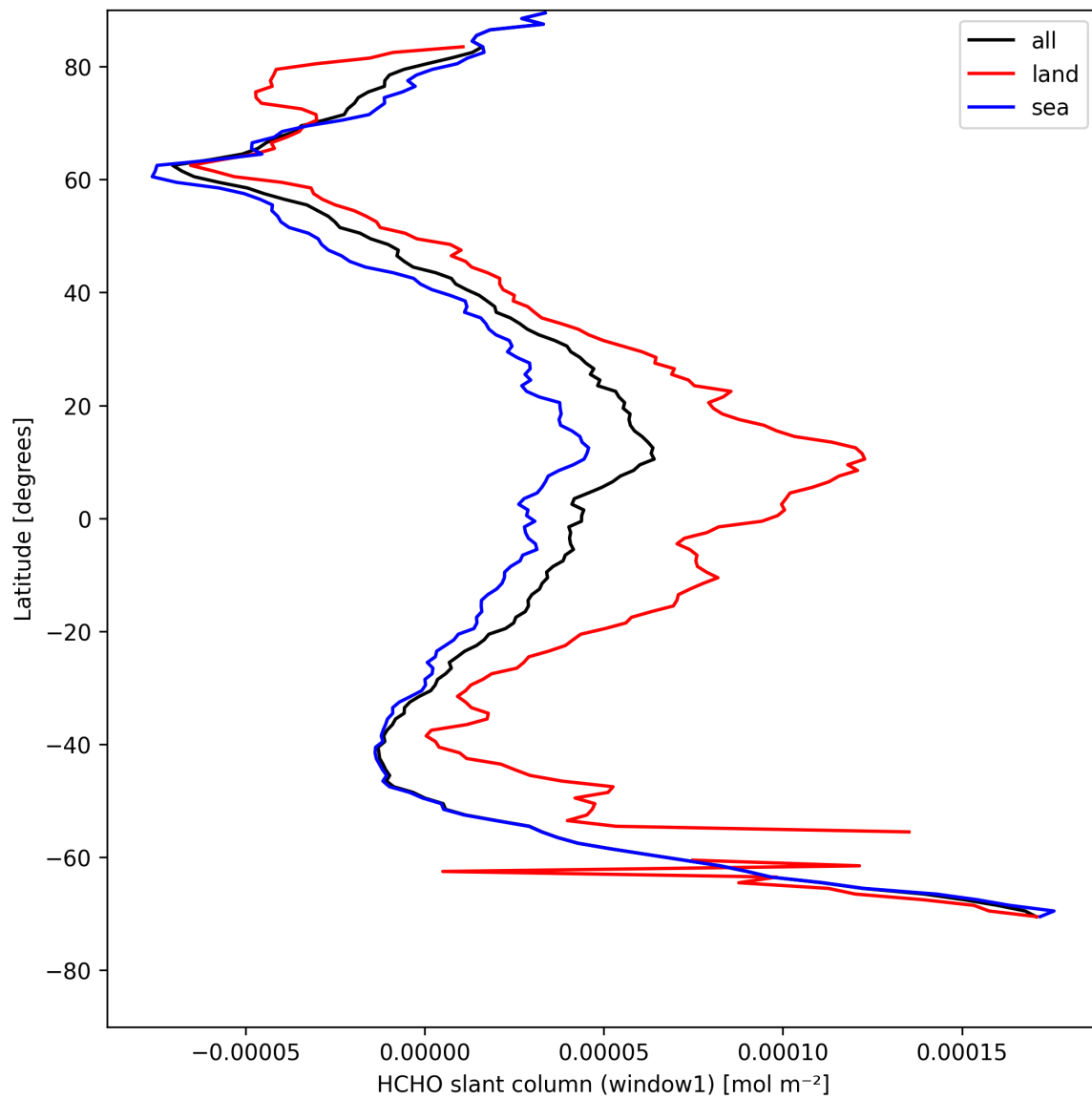
Figure 22: Zonal average of “HCHO slant column (window1)” for 2025-04-27 to 2025-04-27.
