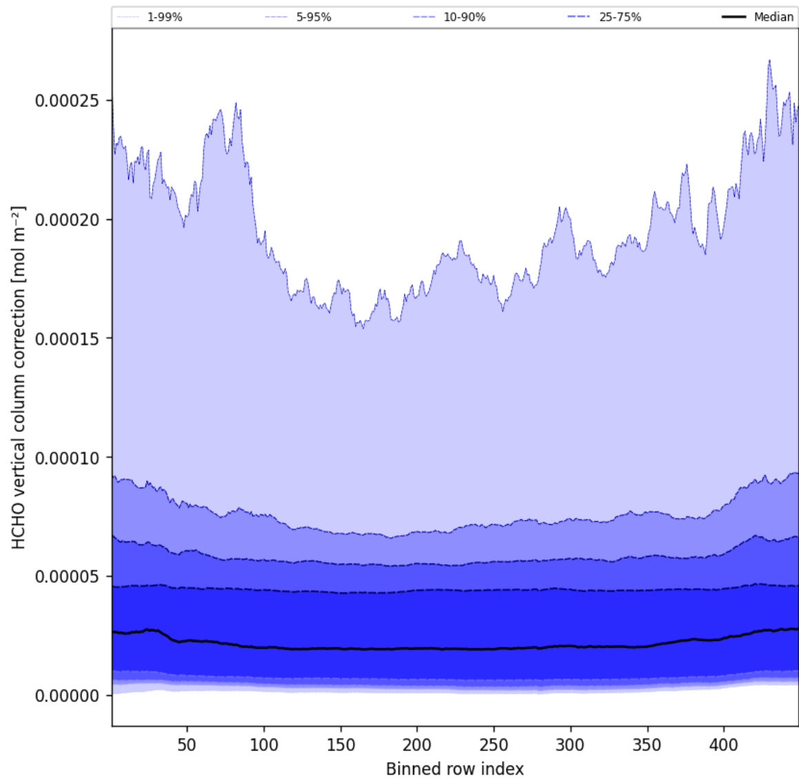
Figure 49: Along track statistics of “HCHO vertical column correction” for 2025-04-27 to 2025-04-27
