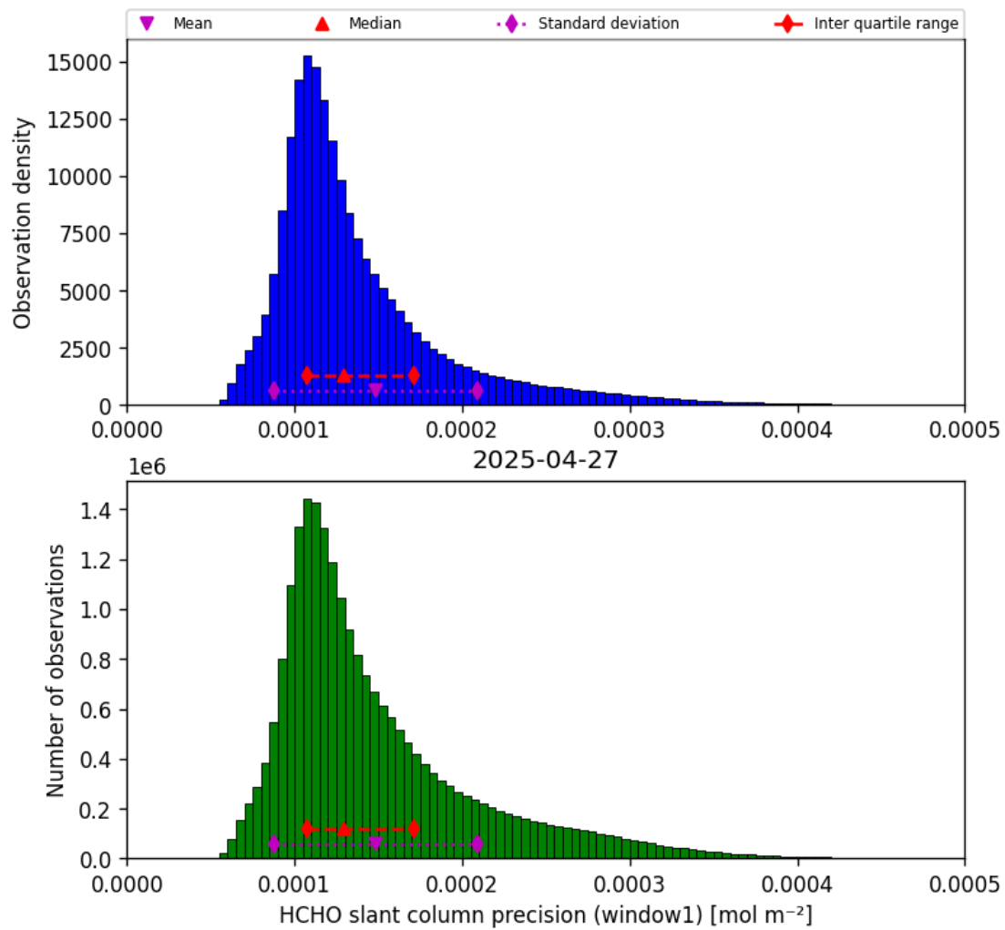
Figure 37: Histogram of “HCHO slant column precision (window1)” for 2025-04-27 to 2025-04-27
