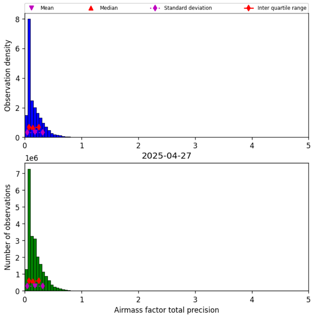
Figure 39: Histogram of “Airmass factor total precision” for 2025-04-27 to 2025-04-27
