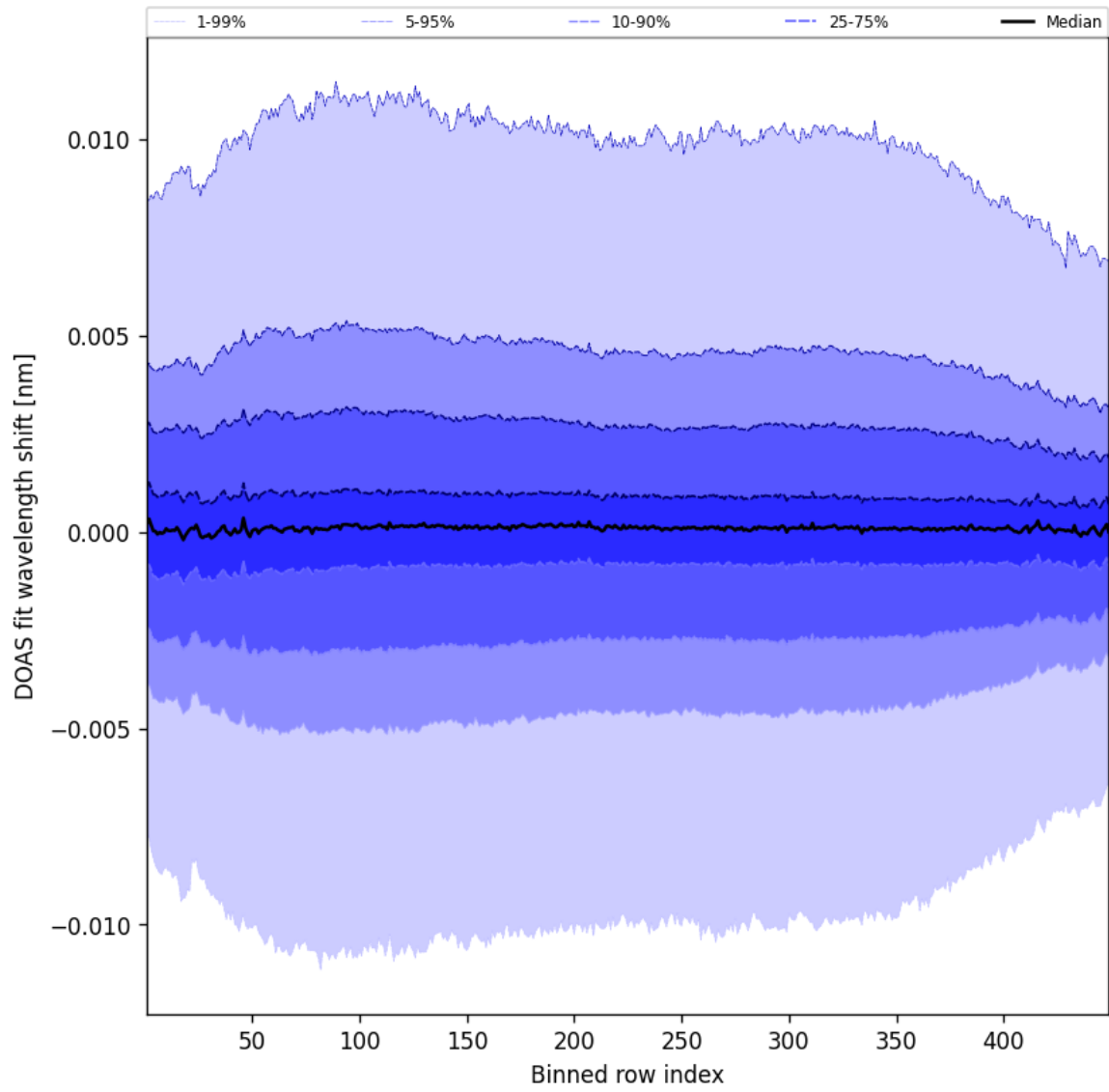
Figure 56: Along track statistics of “DOAS fit wavelength shift” for 2025-04-28 to 2025-04-29
