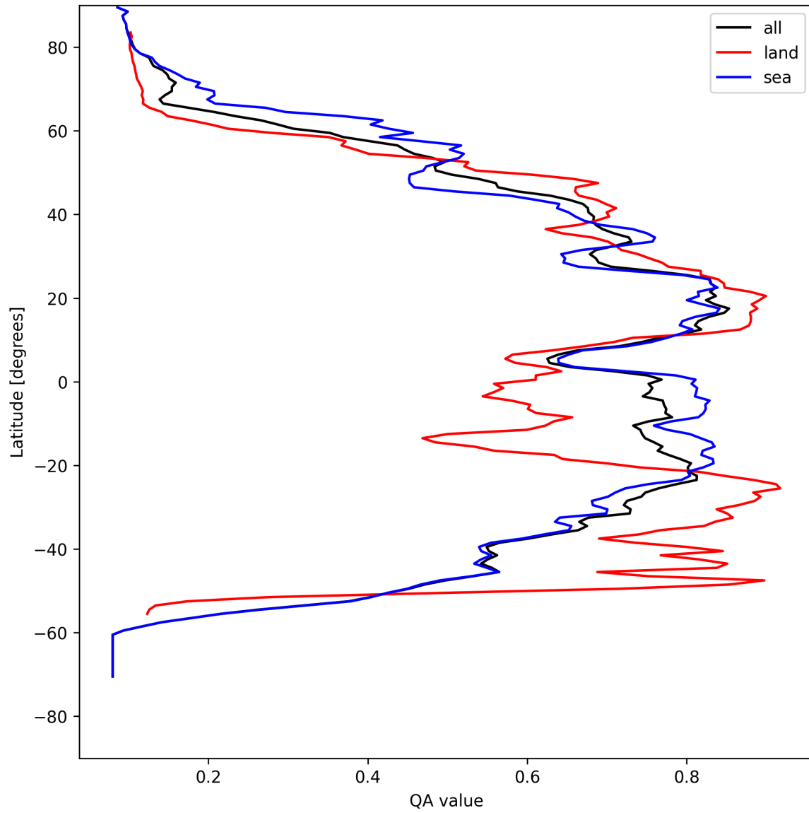
Figure 18: Zonal average of “QA value” for 2025-04-28 to 2025-04-29.
