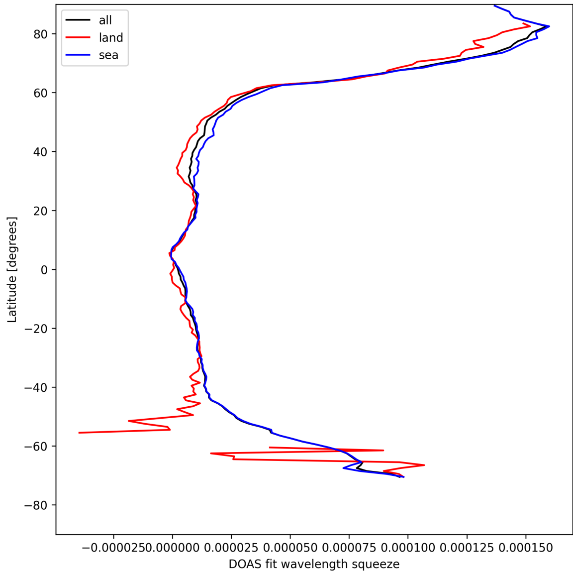
Figure 29: Zonal average of “DOAS fit wavelength squeeze” for 2025-04-28 to 2025-04-29.
