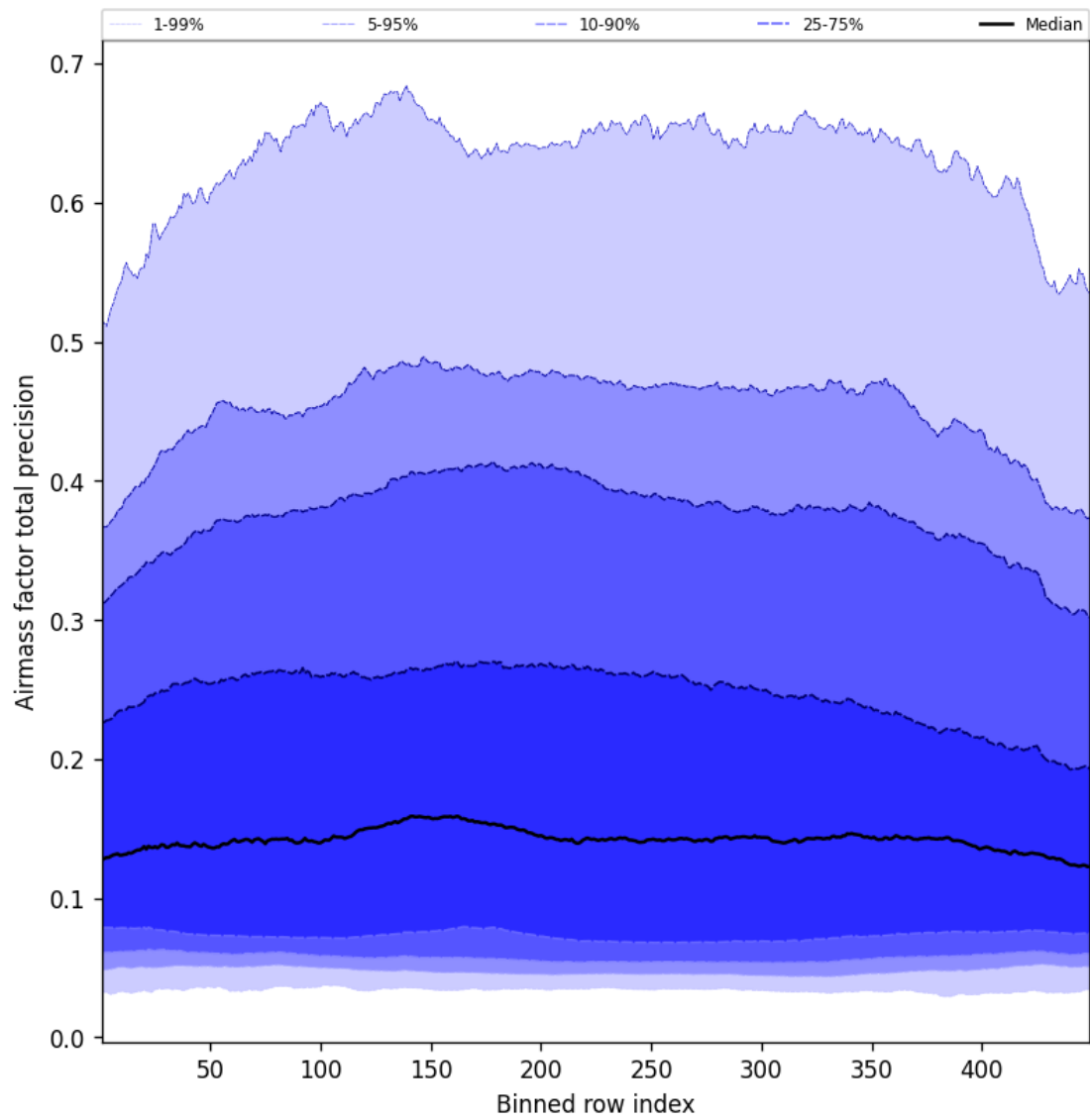
Figure 53: Along track statistics of “Airmass factor total precision” for 2025-04-28 to 2025-04-29
