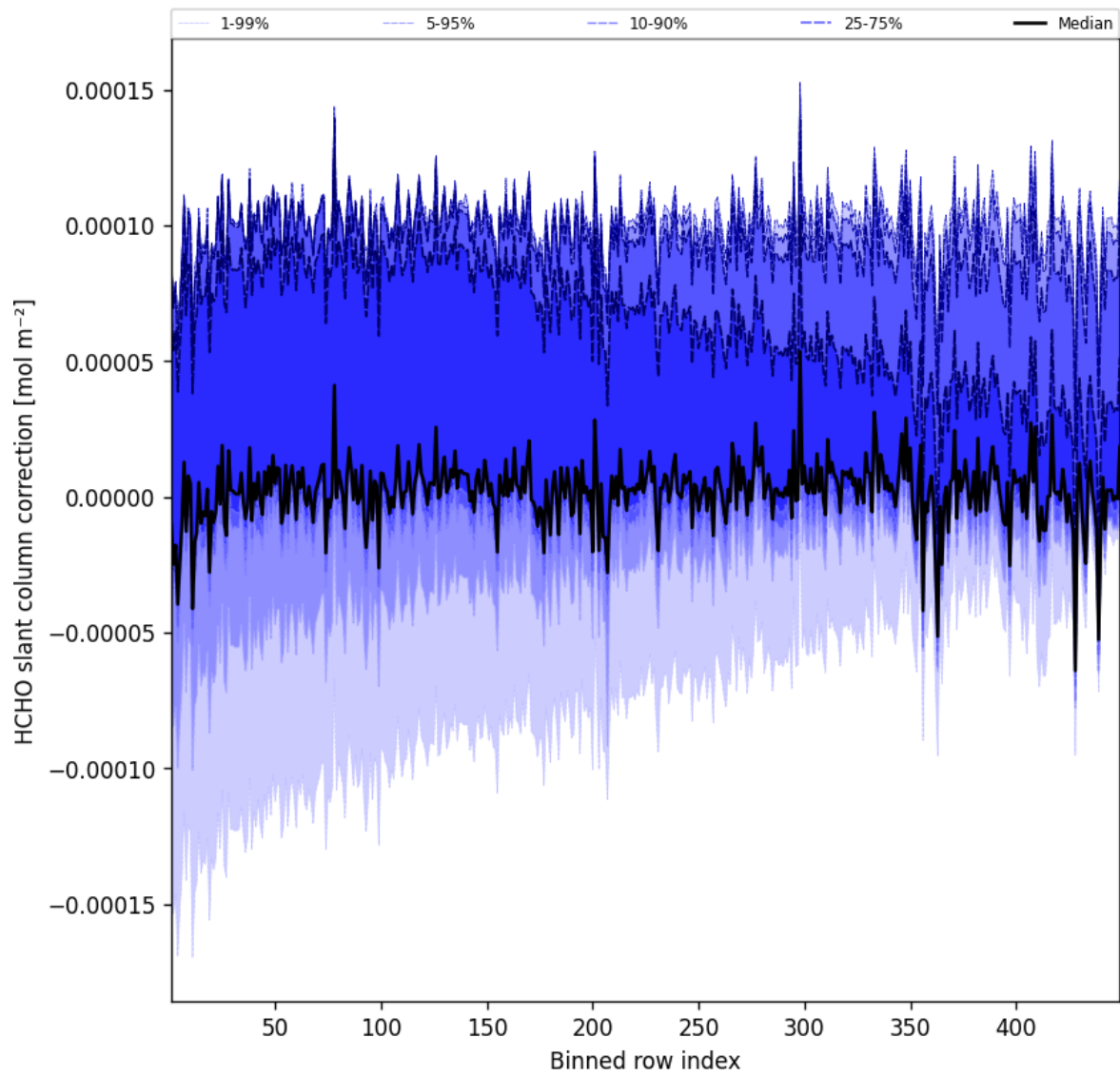
Figure 59: Along track statistics of “HCHO slant column correction” for 2025-04-28 to 2025-04-29
