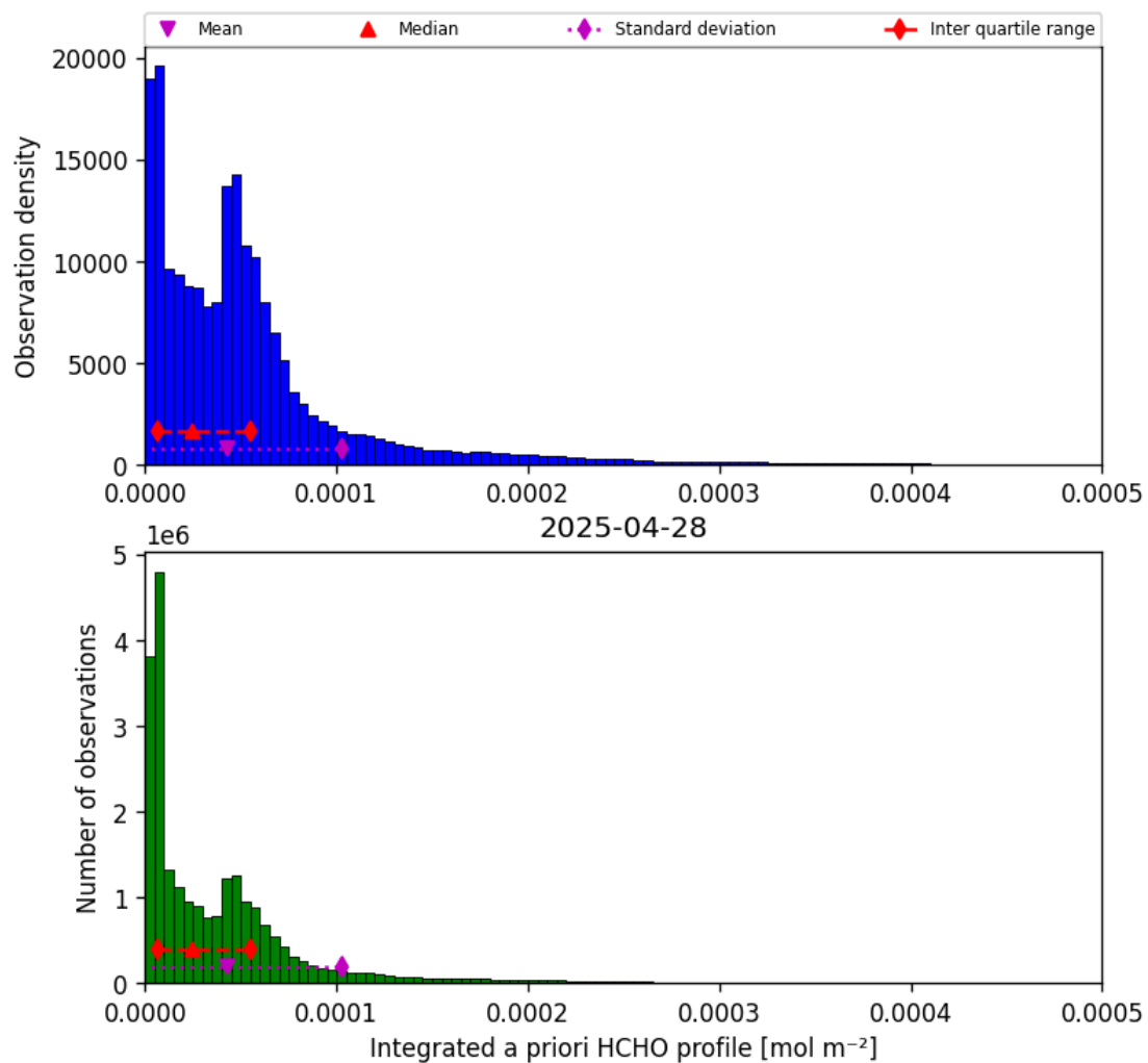
Figure 41: Histogram of “Integrated a priori HCHO profile” for 2025-04-28 to 2025-04-29
