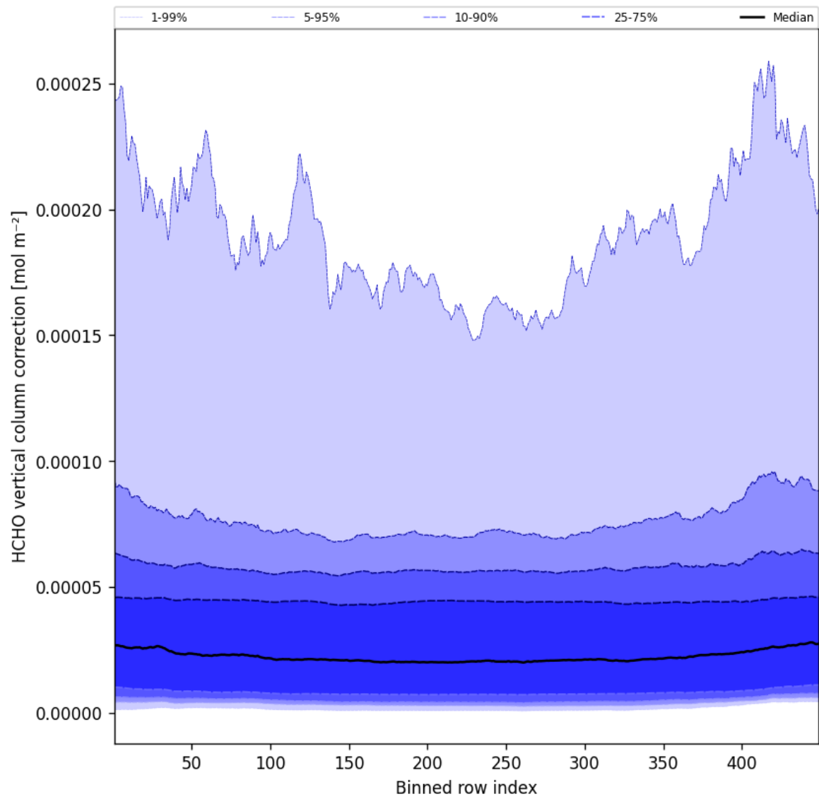
Figure 49: Along track statistics of “HCHO vertical column correction” for 2025-04-28 to 2025-04-29
