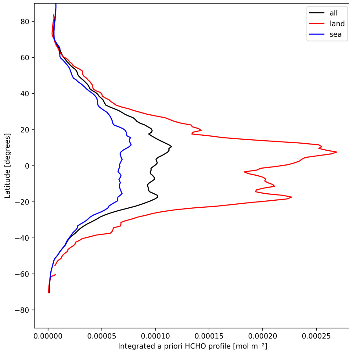
Figure 27: Zonal average of “Integrated a priori HCHO profile” for 2025-04-28 to 2025-04-29.
