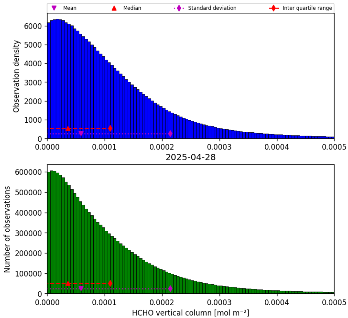
Figure 33: Histogram of “HCHO vertical column” for 2025-04-28 to 2025-04-29
