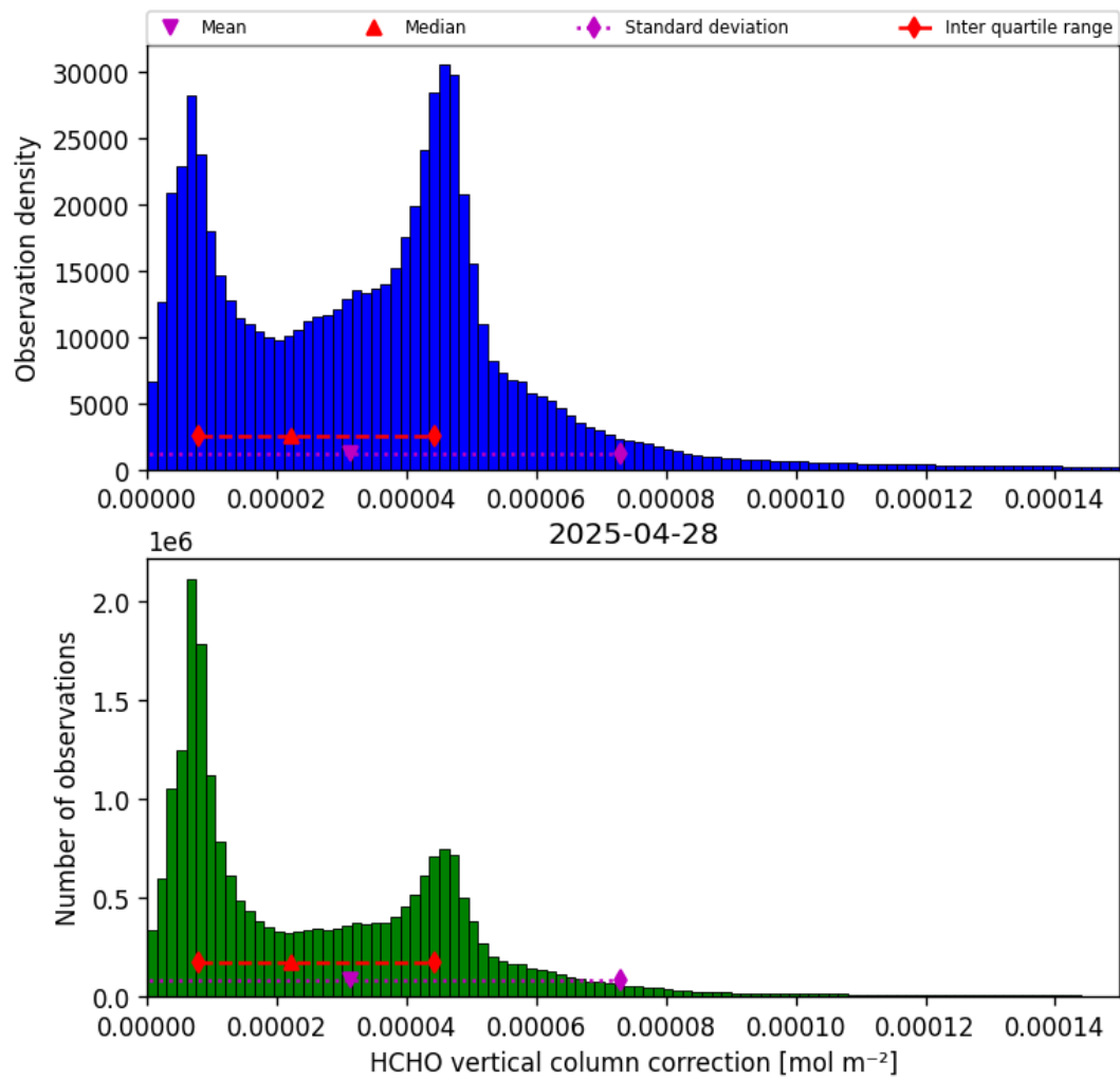
Figure 35: Histogram of “HCHO vertical column correction” for 2025-04-28 to 2025-04-29
