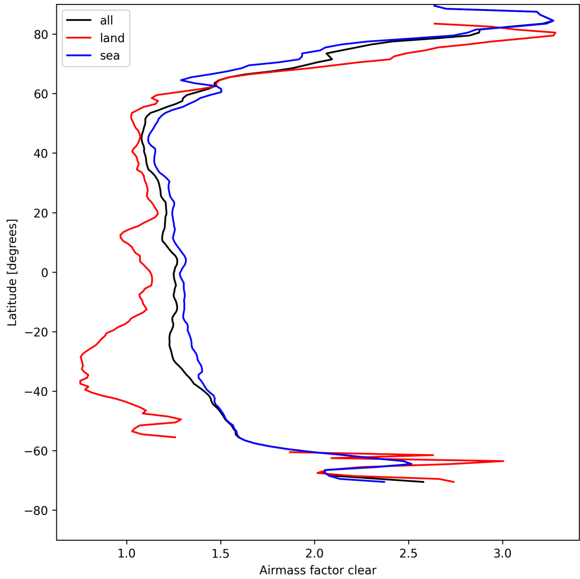
Figure 26: Zonal average of “Airmass factor clear” for 2025-04-28 to 2025-04-29.
