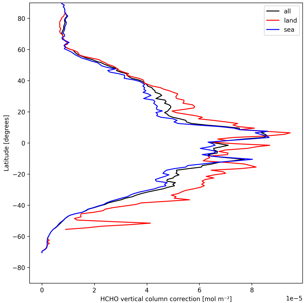
Figure 21: Zonal average of “HCHO vertical column correction” for 2025-04-28 to 2025-04-29.
