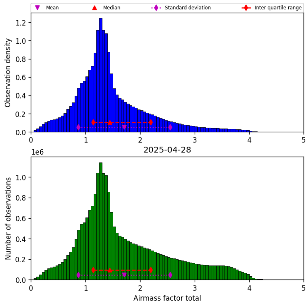
Figure 38: Histogram of “Airmass factor total” for 2025-04-28 to 2025-04-29
