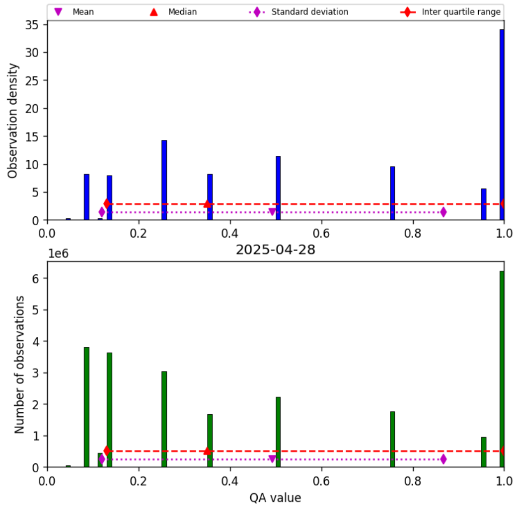
Figure 32: Histogram of “QA value” for 2025-04-28 to 2025-04-29
