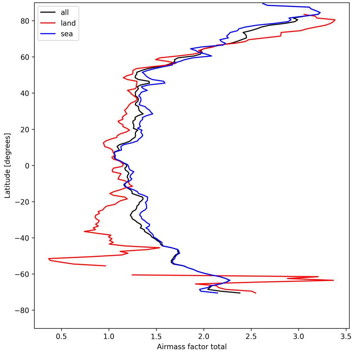
Figure 24: Zonal average of “Airmass factor total” for 2025-04-28 to 2025-04-29.
