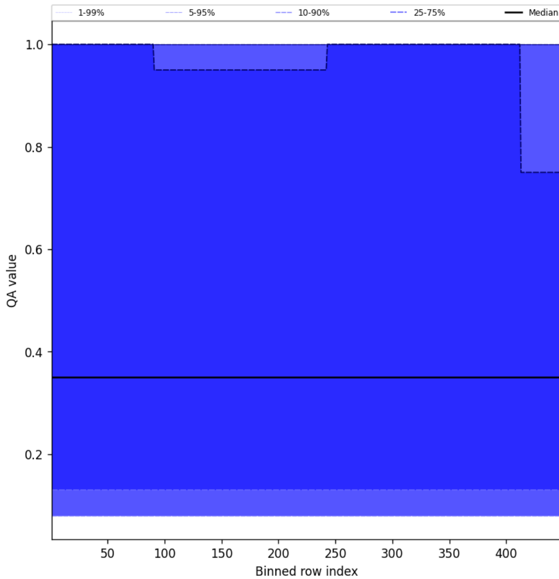
Figure 46: Along track statistics of “QA value” for 2025-04-28 to 2025-04-29
