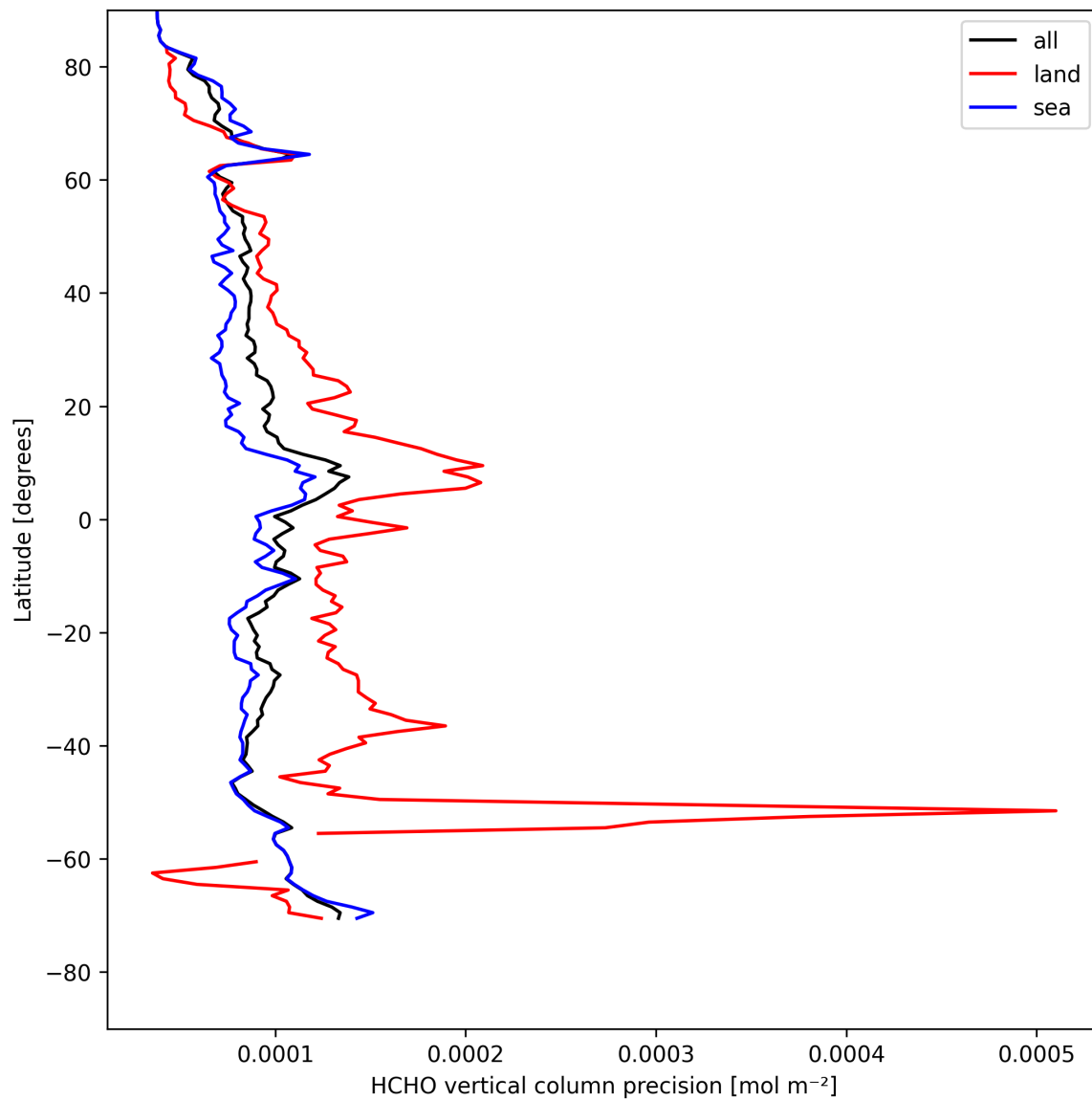
Figure 20: Zonal average of “HCHO vertical column precision” for 2025-04-28 to 2025-04-29.
