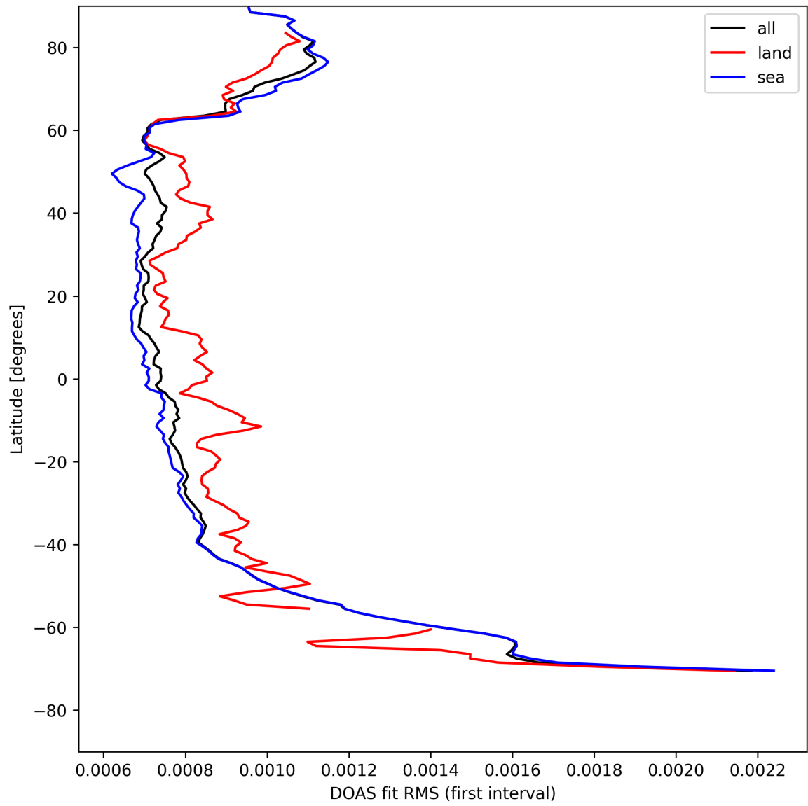
Figure 30: Zonal average of "DOAS fit RMS (first interval)" for 2025-04-28 to 2025-04-29.
