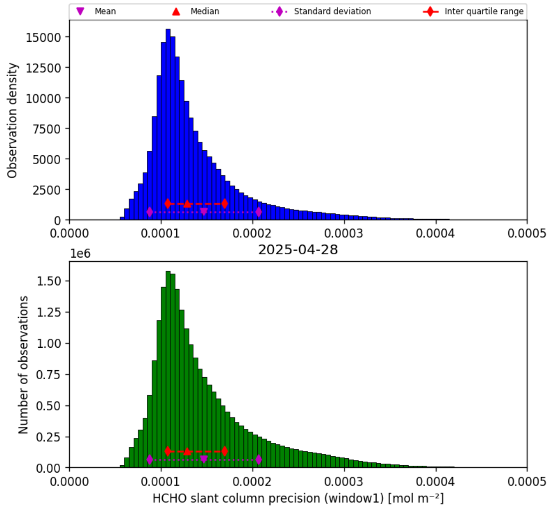
Figure 37: Histogram of “HCHO slant column precision (window1)” for 2025-04-28 to 2025-04-29
