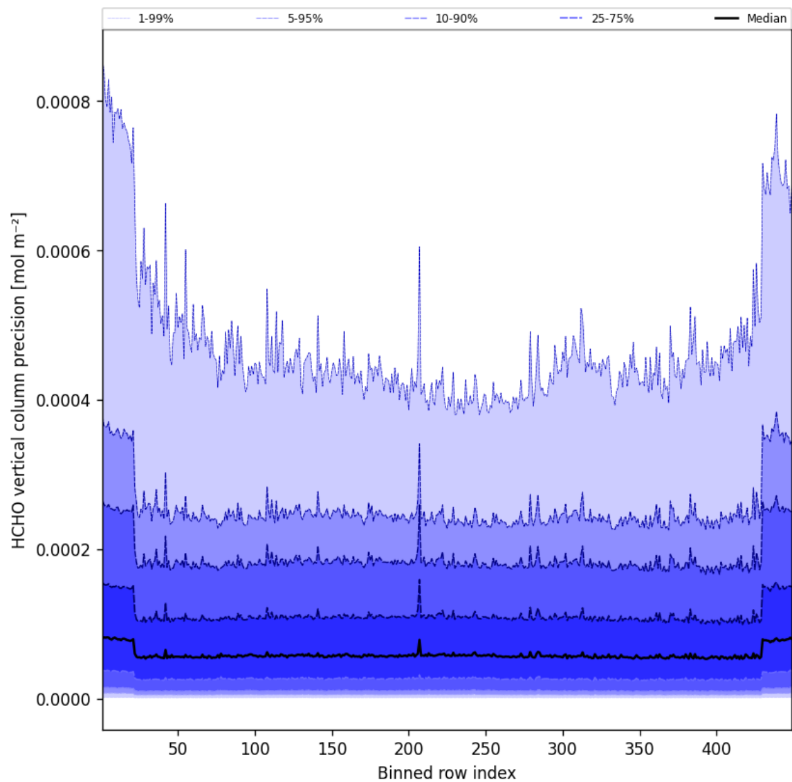
Figure 48: Along track statistics of “HCHO vertical column precision” for 2025-04-28 to 2025-04-29
