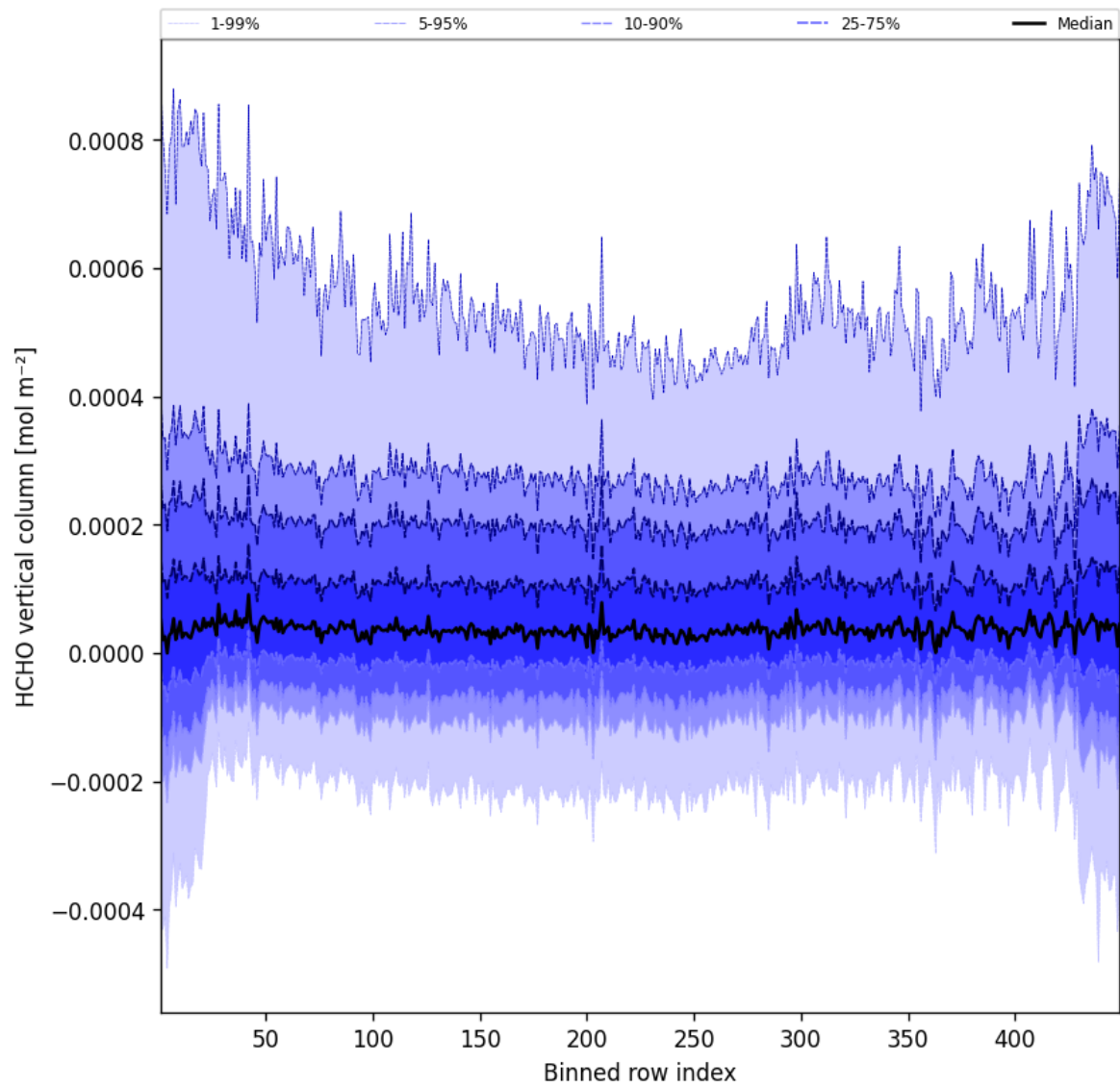
Figure 47: Along track statistics of “HCHO vertical column” for 2025-04-28 to 2025-04-29
