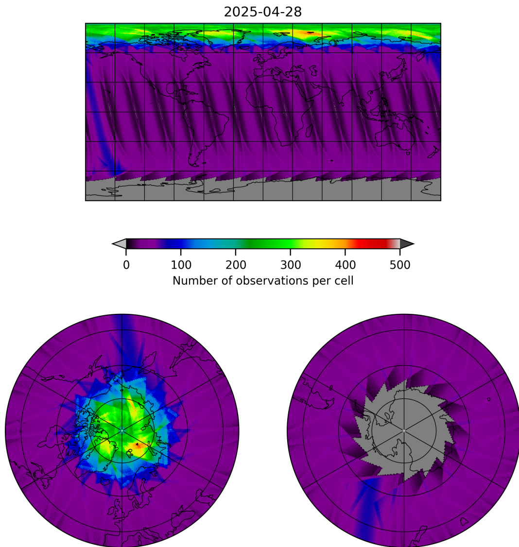
Figure 17: Map of the number of observations for 2025-04-28 to 2025-04-29
