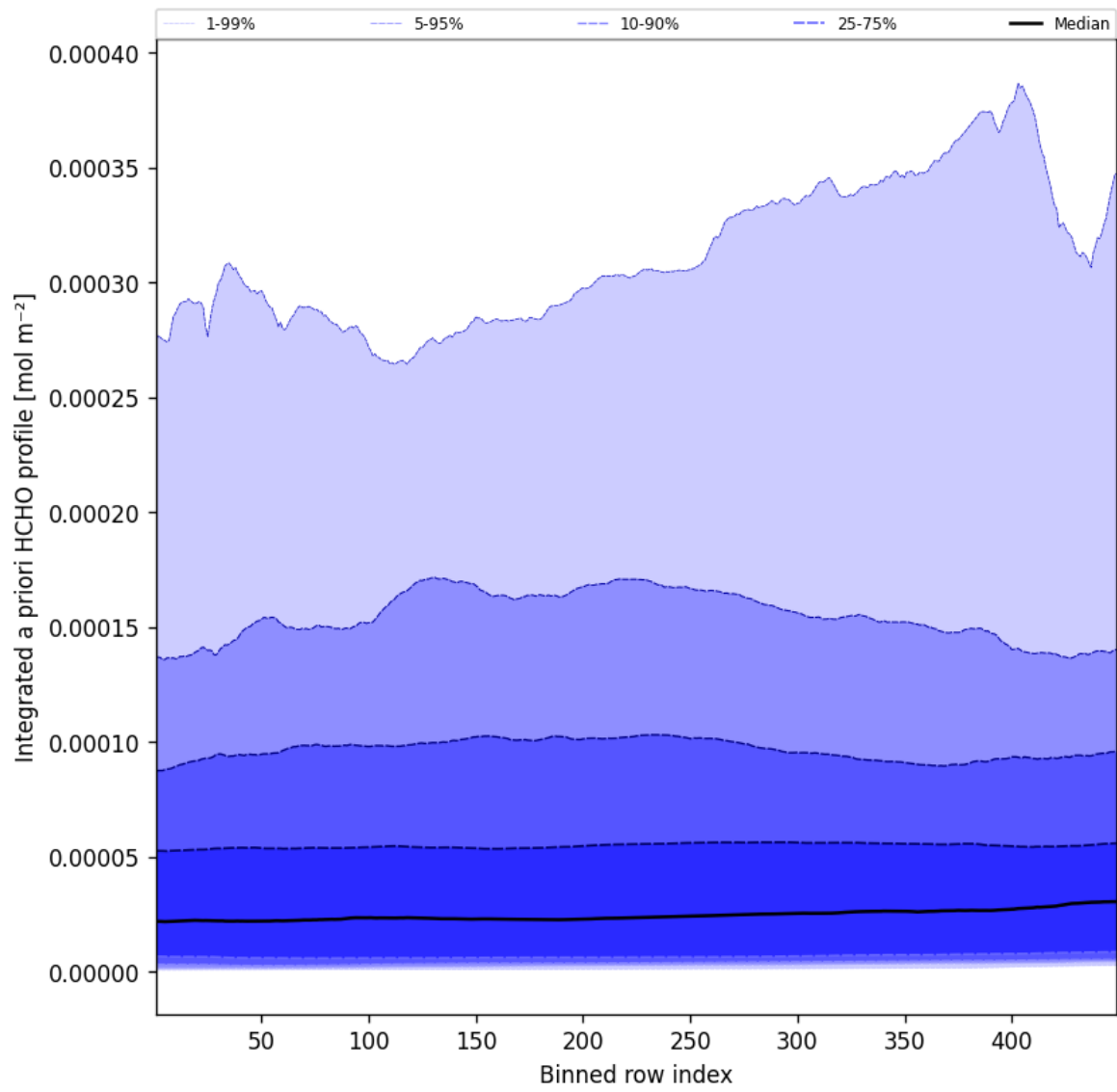
Figure 55: Along track statistics of "Integrated a priori HCHO profile" for 2025-04-28 to 2025-04-29
