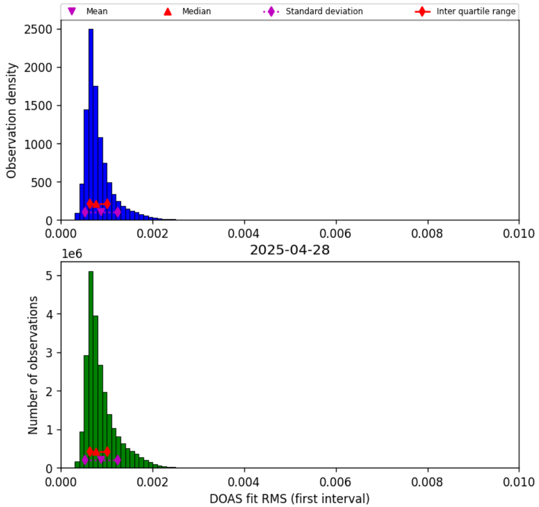
Figure 44: Histogram of “DOAS fit RMS (first interval)” for 2025-04-28 to 2025-04-29
