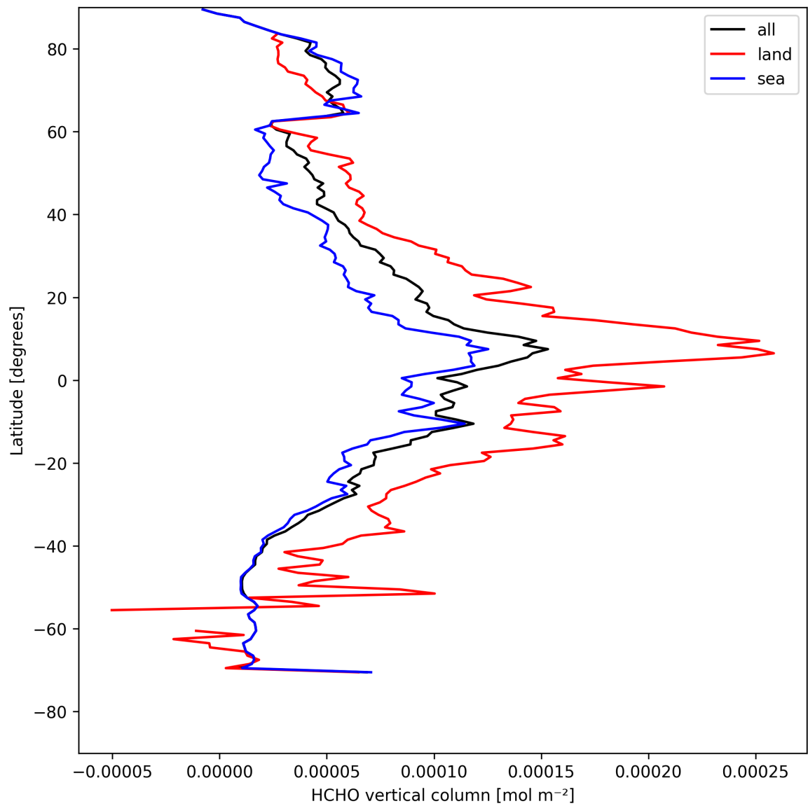
Figure 19: Zonal average of “HCHO vertical column” for 2025-04-28 to 2025-04-29.
