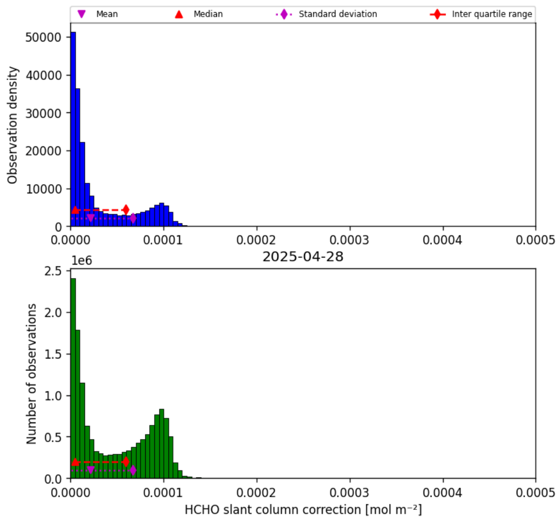
Figure 45: Histogram of “HCHO slant column correction” for 2025-04-28 to 2025-04-29
