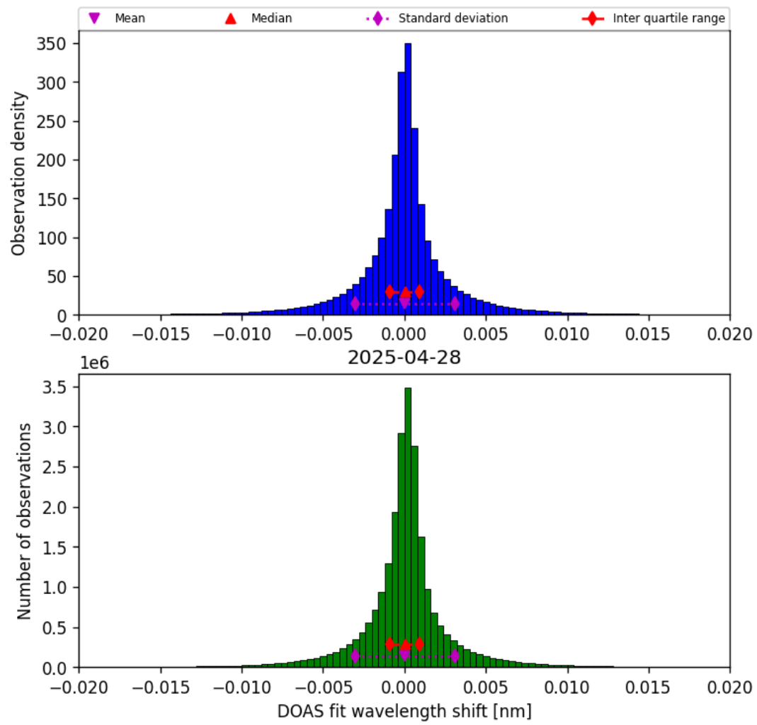
Figure 42: Histogram of “DOAS fit wavelength shift” for 2025-04-28 to 2025-04-29
