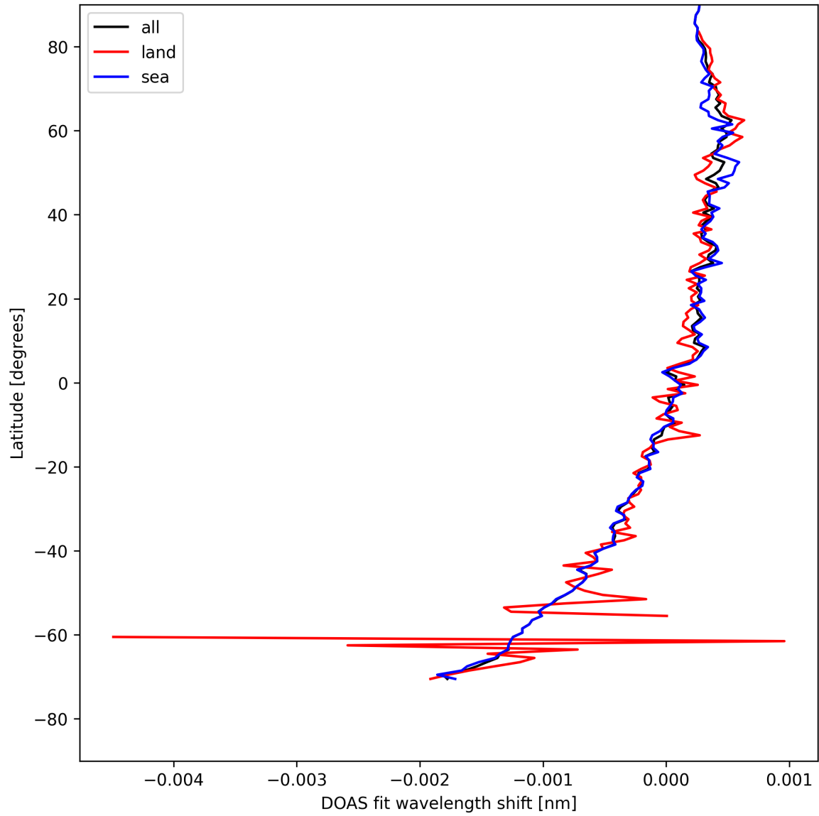
Figure 28: Zonal average of “DOAS fit wavelength shift” for 2025-04-28 to 2025-04-29.
