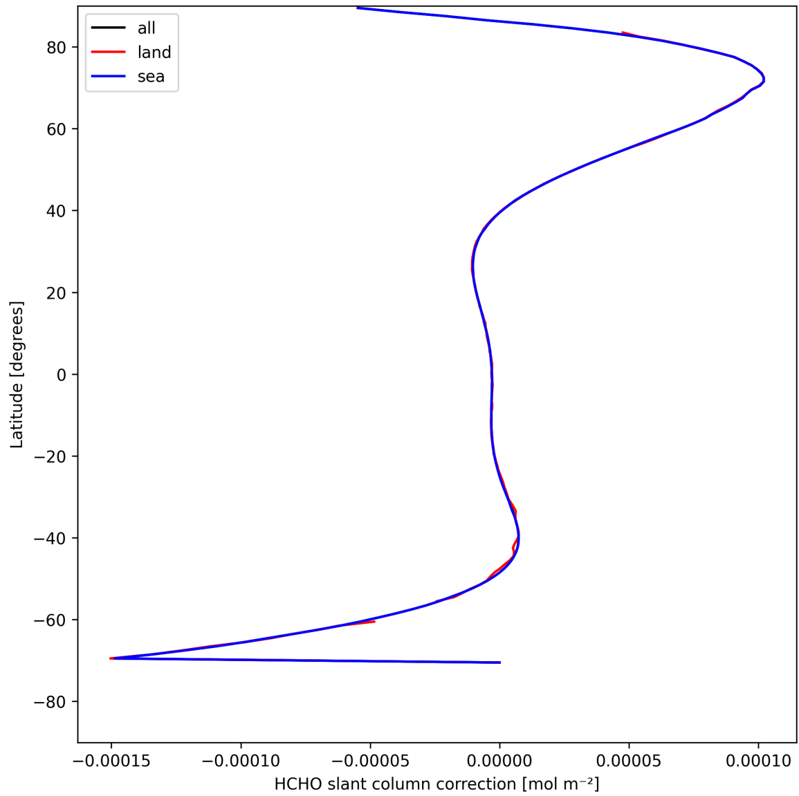
Figure 31: Zonal average of “HCHO slant column correction” for 2025-04-28 to 2025-04-29.
