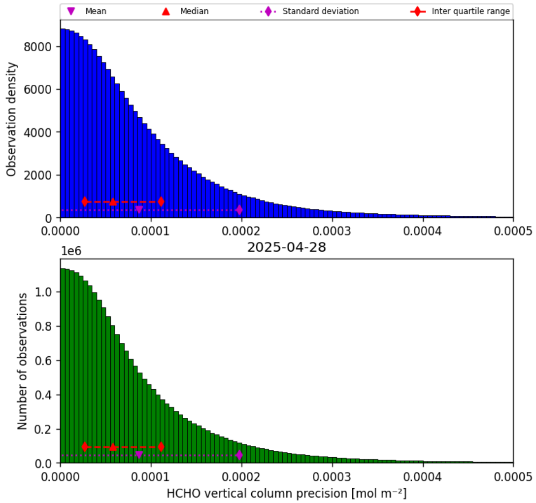
Figure 34: Histogram of “HCHO vertical column precision” for 2025-04-28 to 2025-04-29
