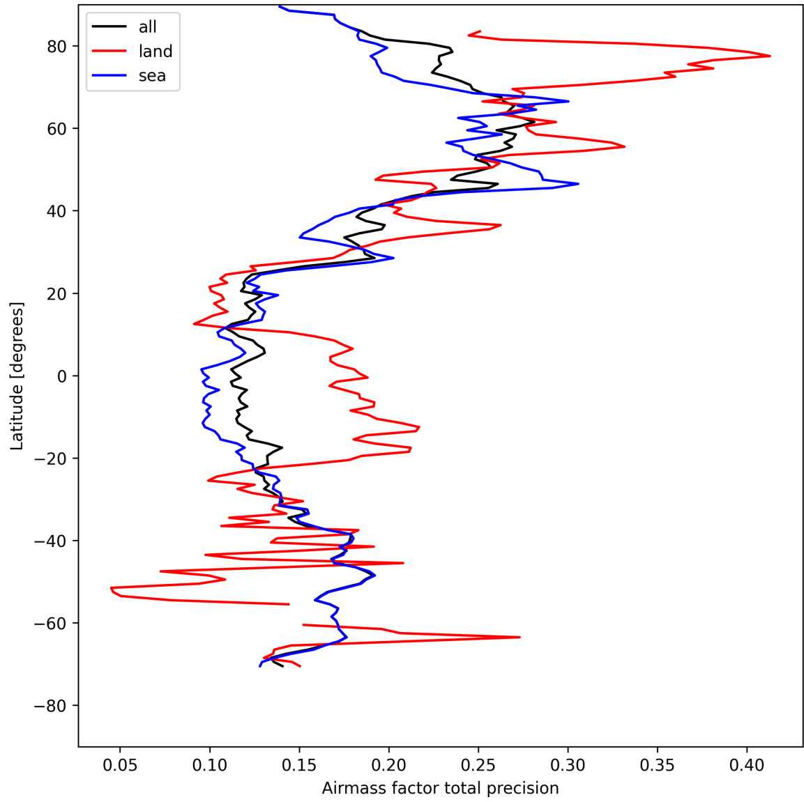
Figure 25: Zonal average of “Airmass factor total precision” for 2025-04-28 to 2025-04-29.
