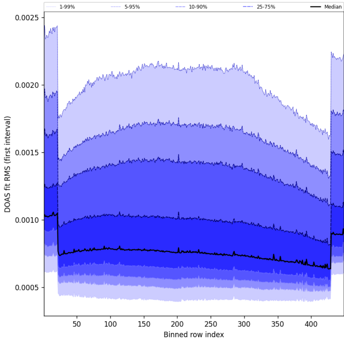
Figure 58: Along track statistics of “DOAS fit RMS (first interval)” for 2025-04-28 to 2025-04-29
