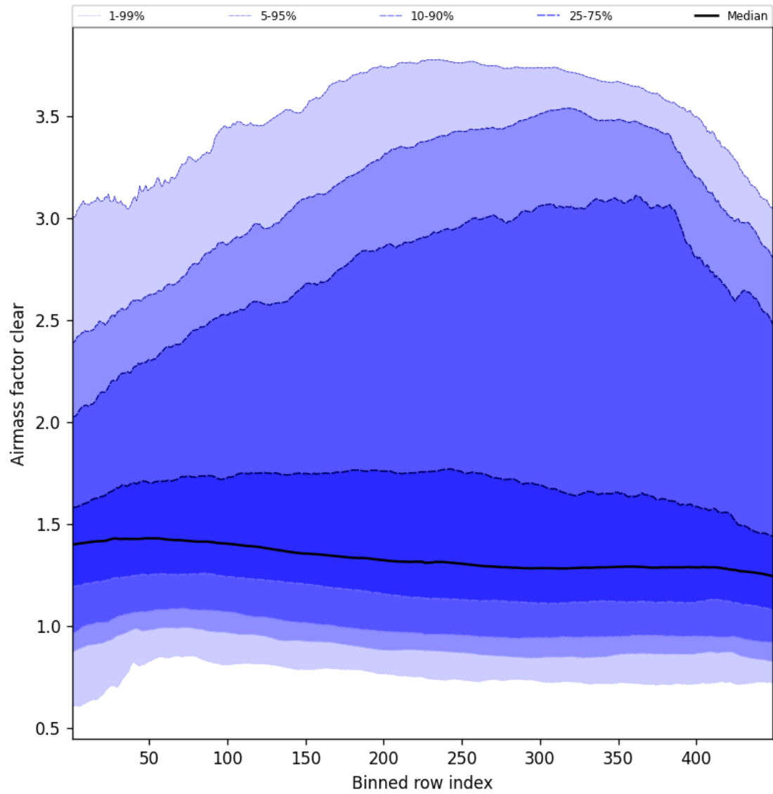
Figure 54: Along track statistics of “Airmass factor clear” for 2025-04-28 to 2025-04-29
