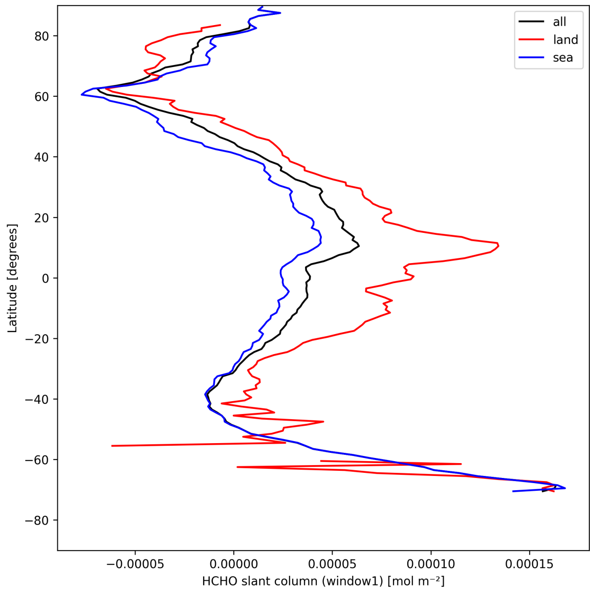
Figure 22: Zonal average of “HCHO slant column (window1)” for 2025-04-28 to 2025-04-29.
