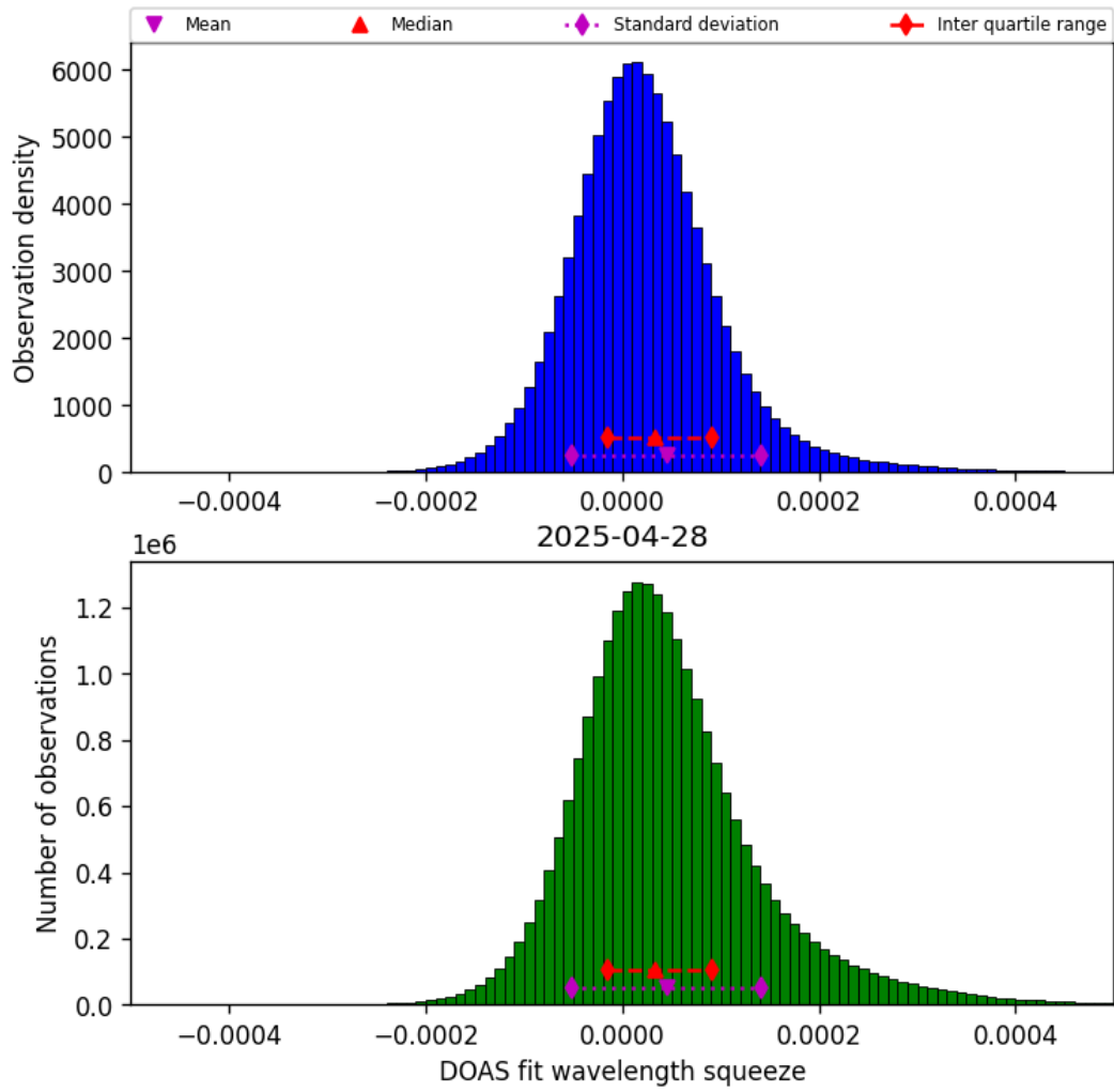
Figure 43: Histogram of “DOAS fit wavelength squeeze” for 2025-04-28 to 2025-04-29
