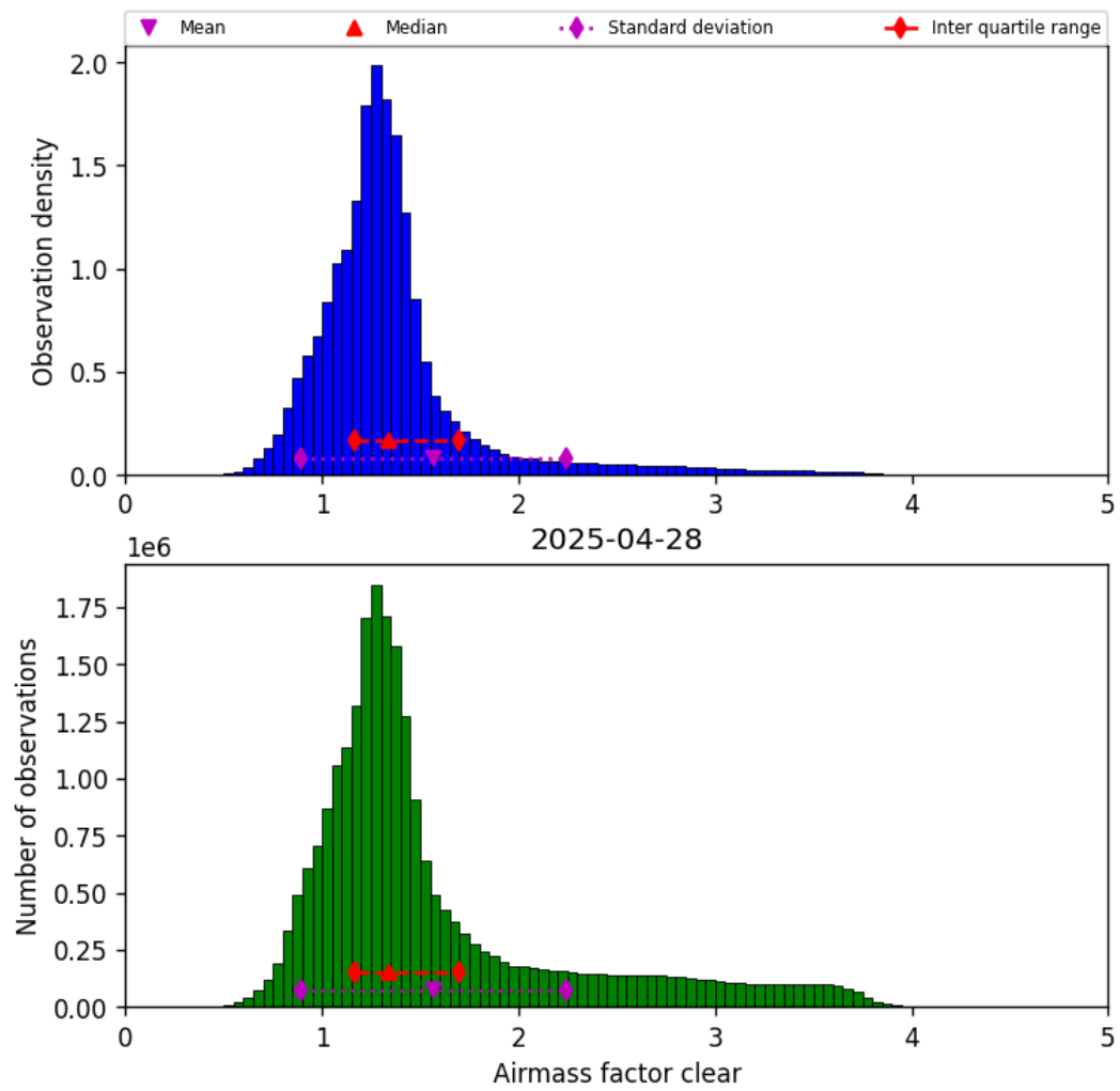
Figure 40: Histogram of “Airmass factor clear” for 2025-04-28 to 2025-04-29
