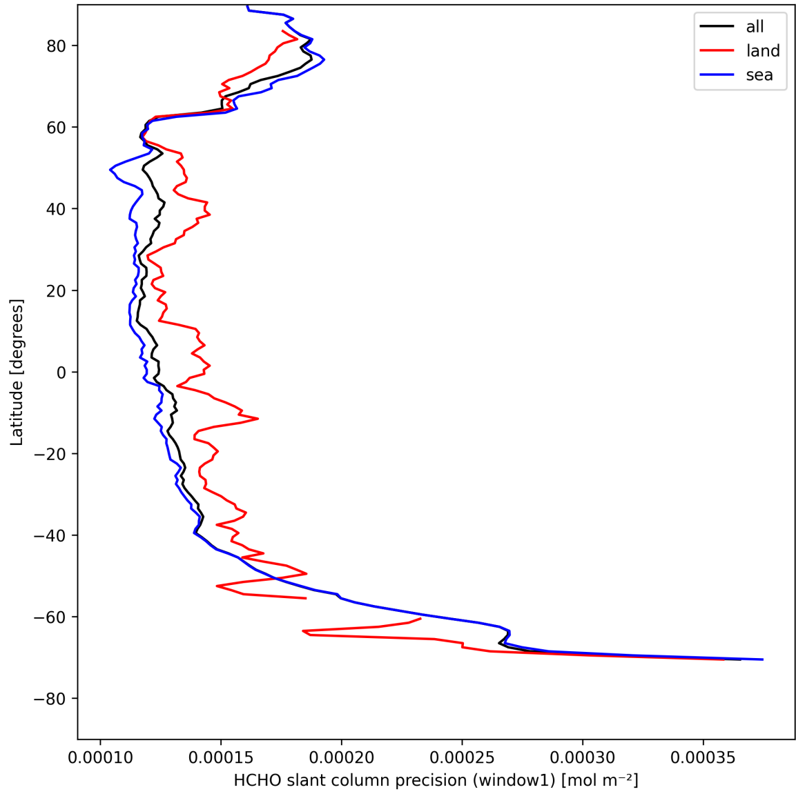
Figure 23: Zonal average of “HCHO slant column precision (window1)” for 2025-04-28 to 2025-04-29.
