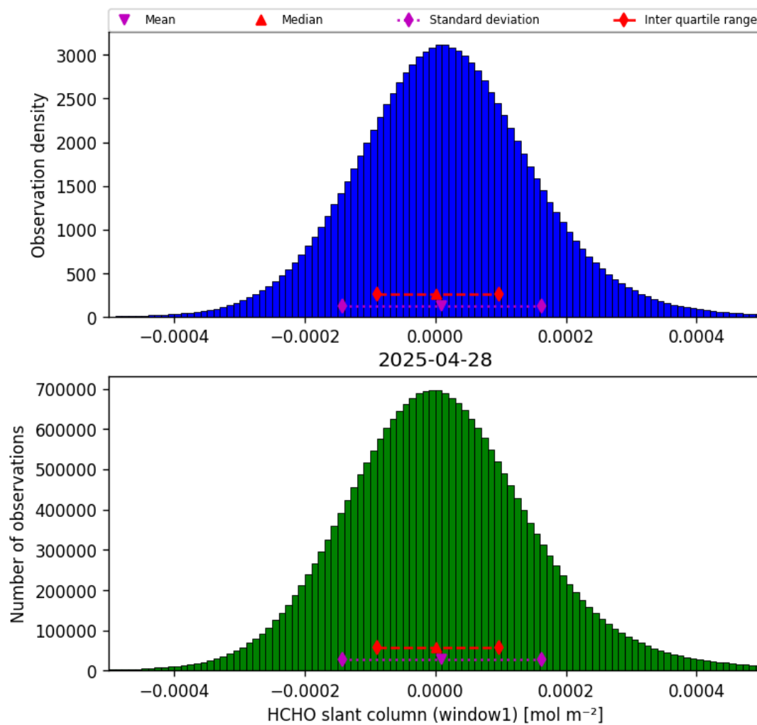
Figure 36: Histogram of “HCHO slant column (window1)” for 2025-04-28 to 2025-04-29
