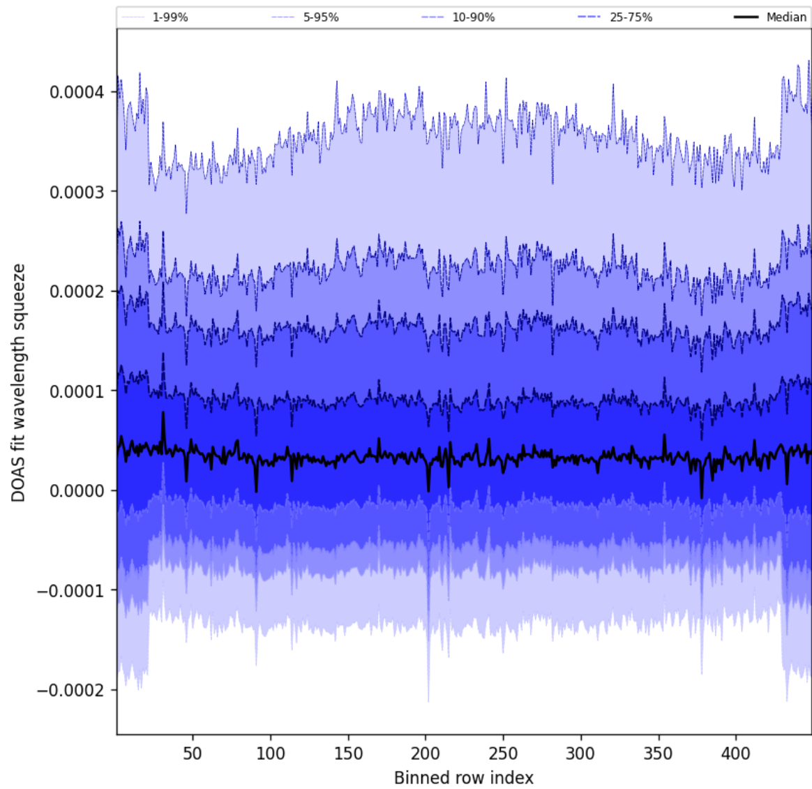
Figure 57: Along track statistics of “DOAS fit wavelength squeeze” for 2025-04-28 to 2025-04-29
