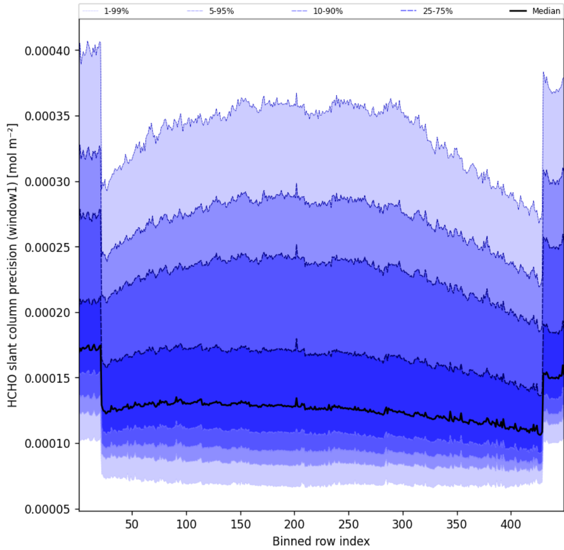
Figure 51: Along track statistics of “HCHO slant column precision (window1)” for 2025-04-28 to 2025-04-29
