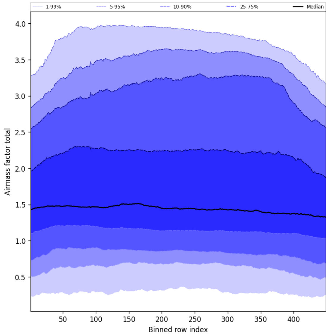
Figure 52: Along track statistics of “Airmass factor total” for 2025-04-28 to 2025-04-29
