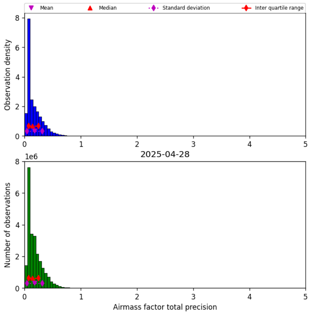
Figure 39: Histogram of “Airmass factor total precision” for 2025-04-28 to 2025-04-29
