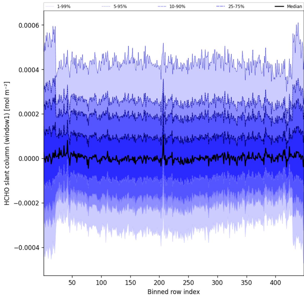
Figure 50: Along track statistics of “HCHO slant column (window1)” for 2025-04-28 to 2025-04-29
