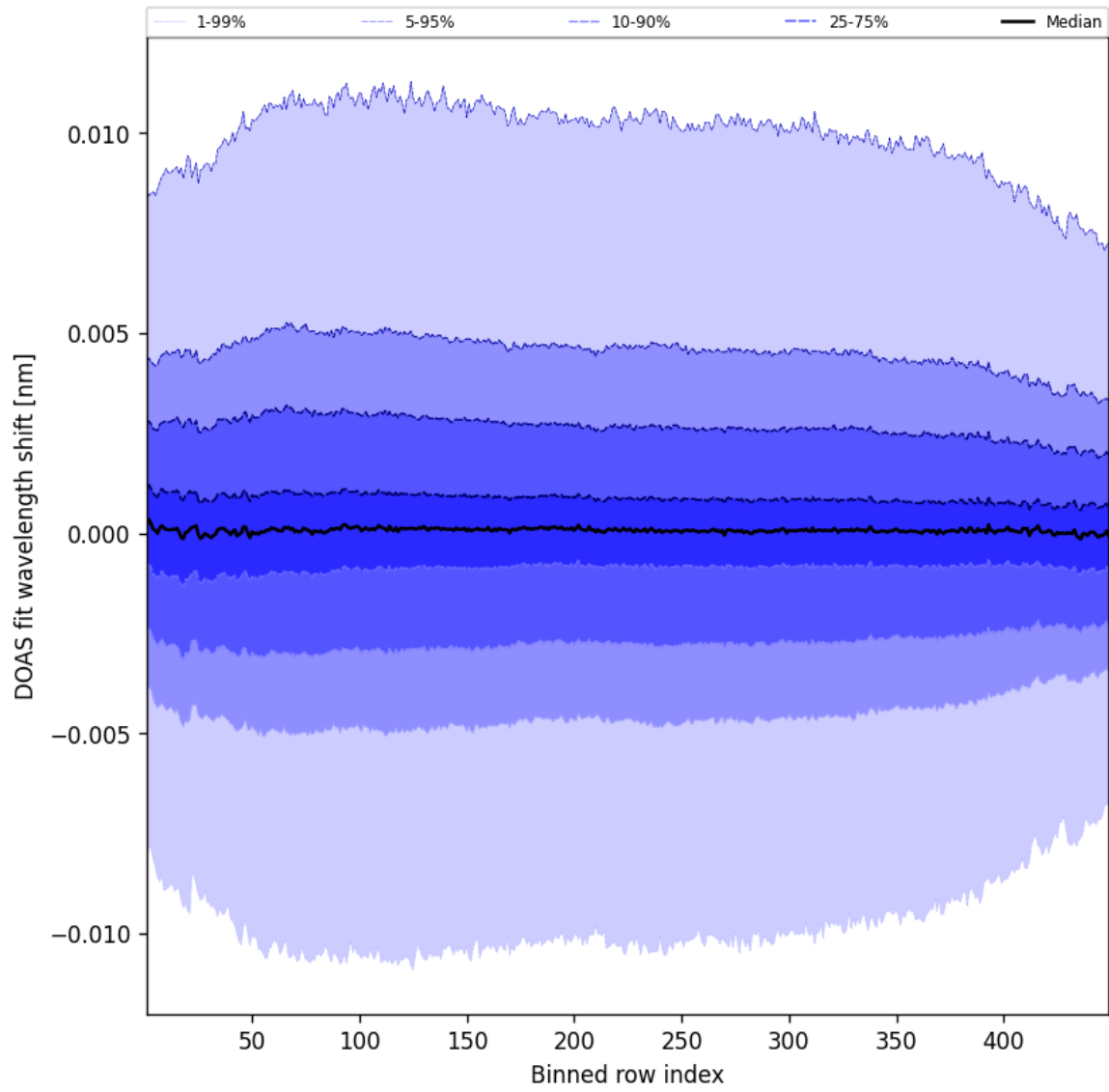
Figure 56: Along track statistics of “DOAS fit wavelength shift” for 2025-04-29 to 2025-04-30
