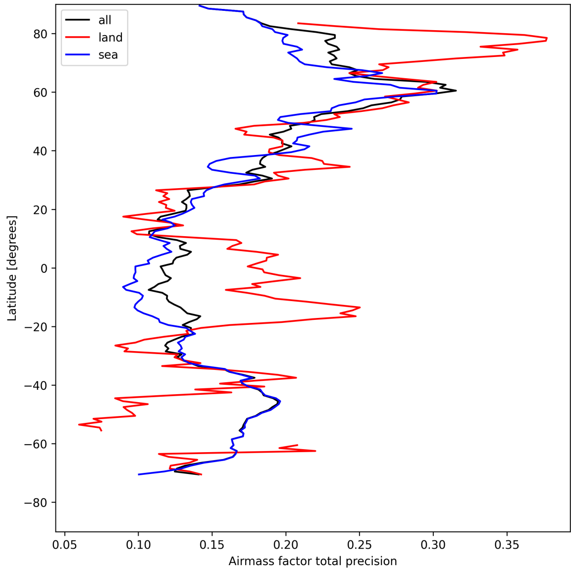
Figure 25: Zonal average of “Airmass factor total precision” for 2025-04-29 to 2025-04-30.
