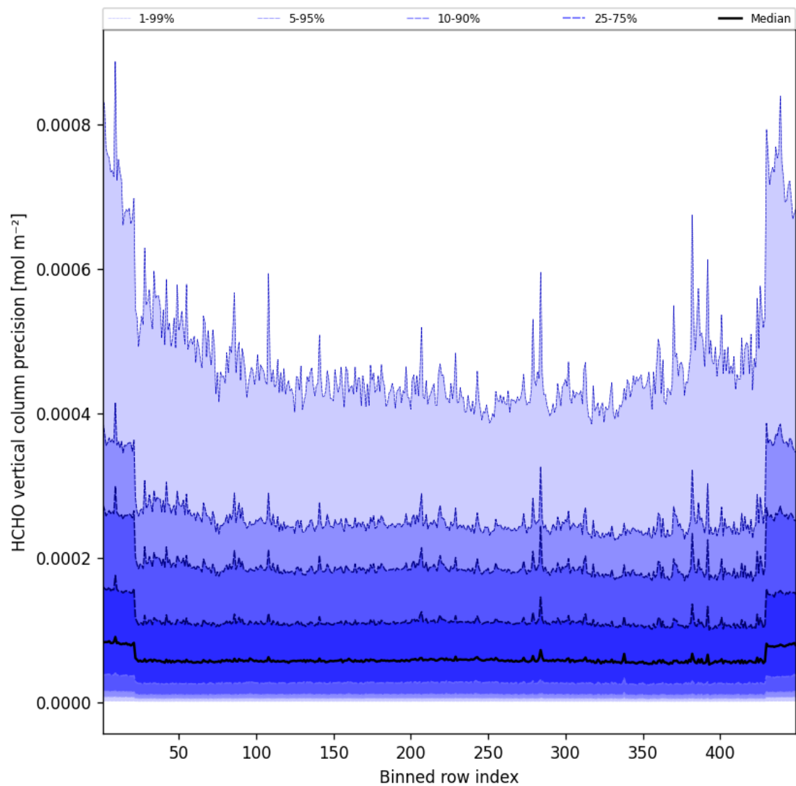
Figure 48: Along track statistics of “HCHO vertical column precision” for 2025-04-29 to 2025-04-30
