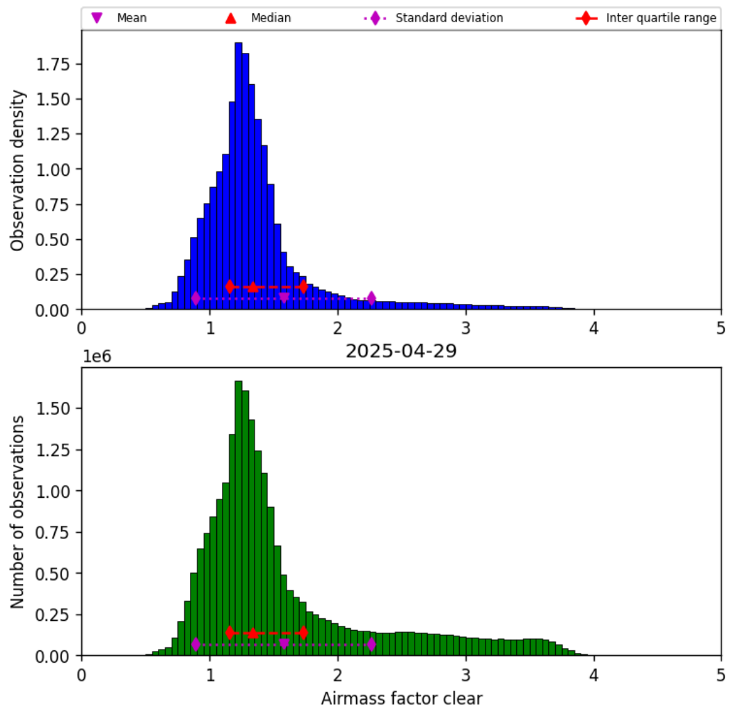
Figure 40: Histogram of “Airmass factor clear” for 2025-04-29 to 2025-04-30
