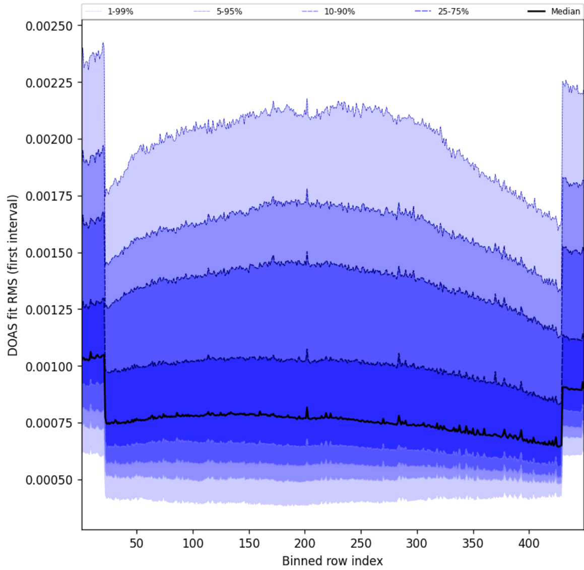
Figure 58: Along track statistics of “DOAS fit RMS (first interval)” for 2025-04-29 to 2025-04-30
