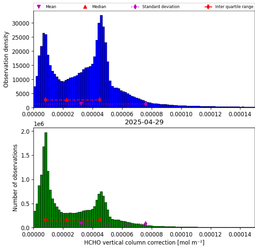
Figure 35: Histogram of “HCHO vertical column correction” for 2025-04-29 to 2025-04-30
