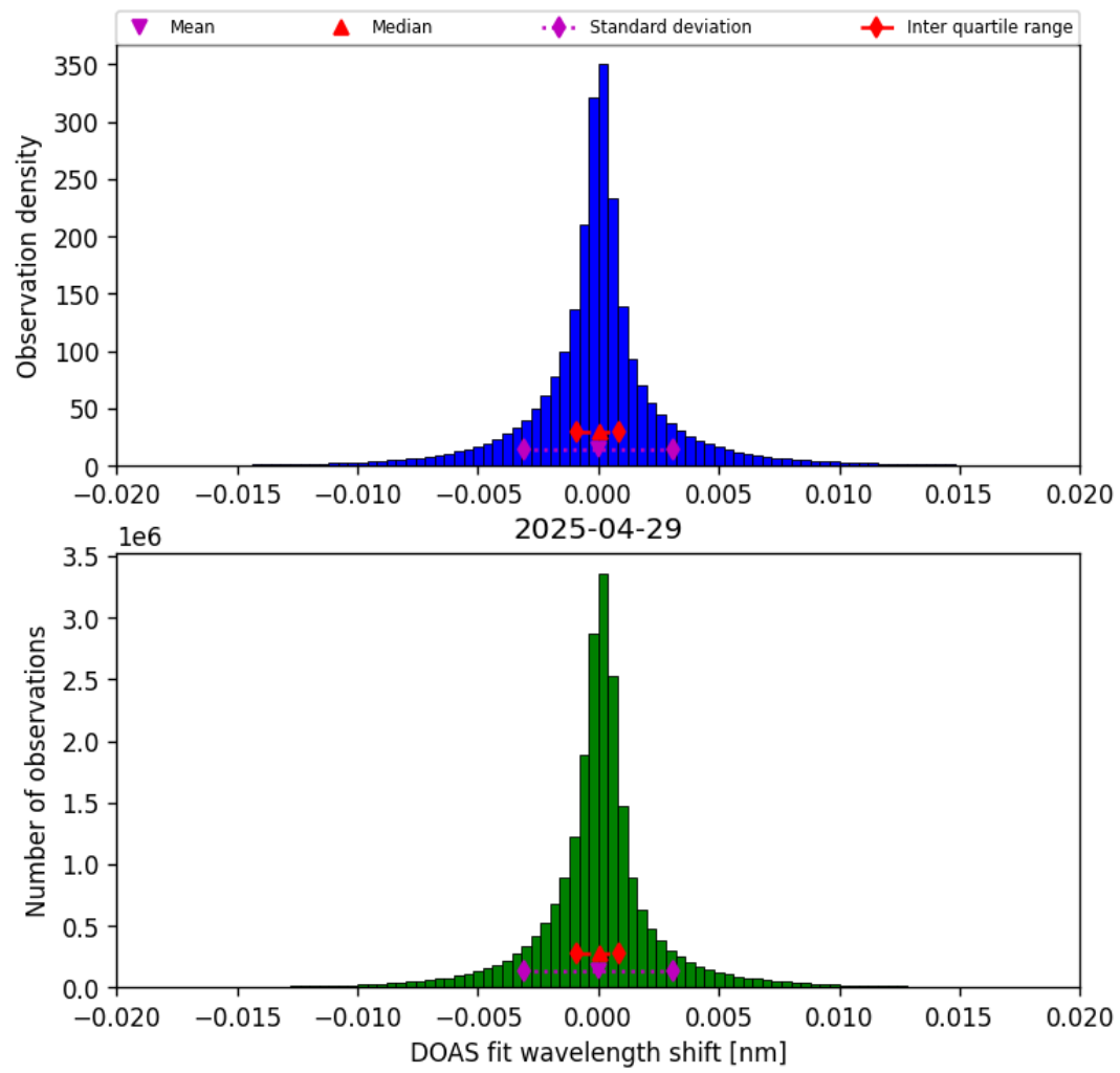
Figure 42: Histogram of “DOAS fit wavelength shift” for 2025-04-29 to 2025-04-30
