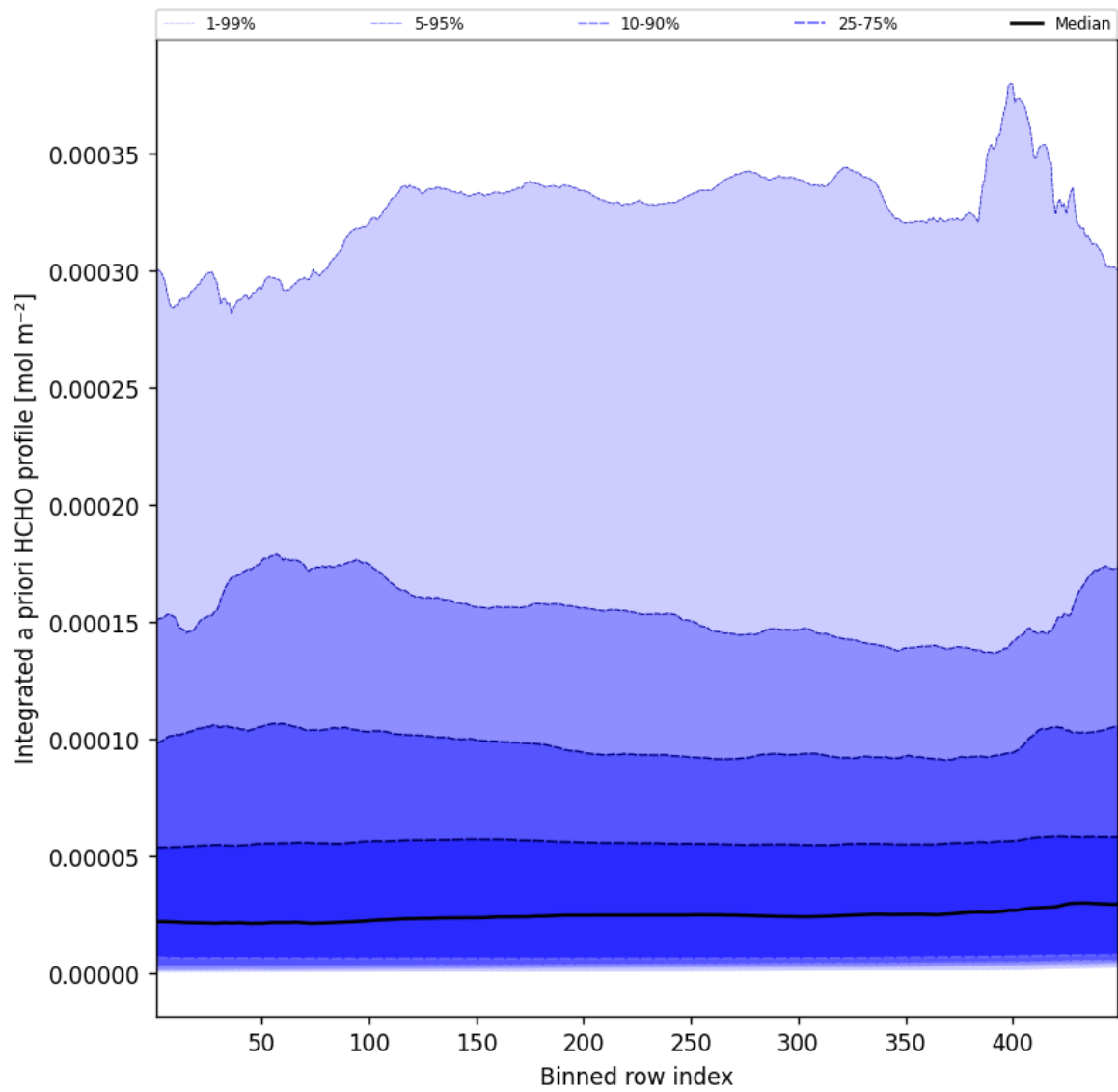
Figure 55: Along track statistics of "Integrated a priori HCHO profile" for 2025-04-29 to 2025-04-30
