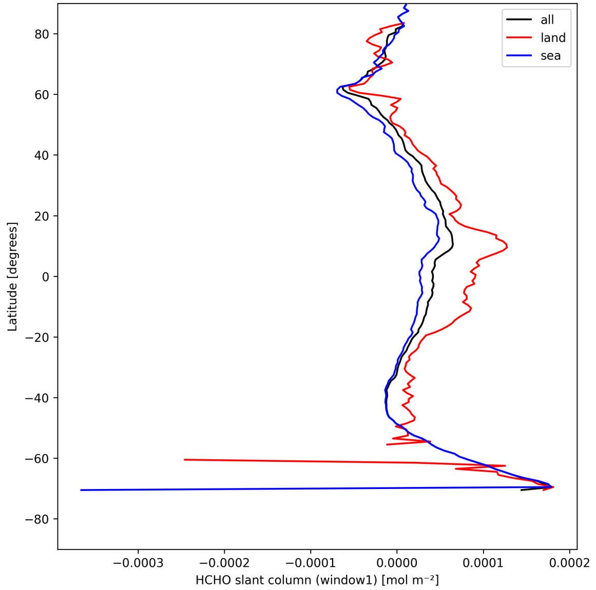
Figure 22: Zonal average of “HCHO slant column (window1)” for 2025-04-29 to 2025-04-30.
