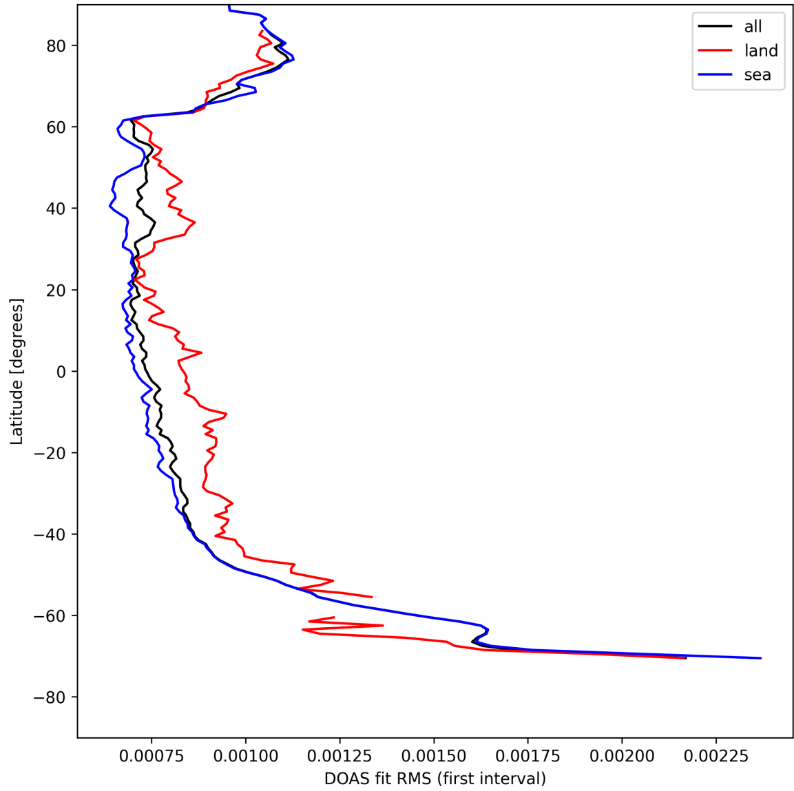
Figure 30: Zonal average of “DOAS fit RMS (first interval)” for 2025-04-29 to 2025-04-30.
