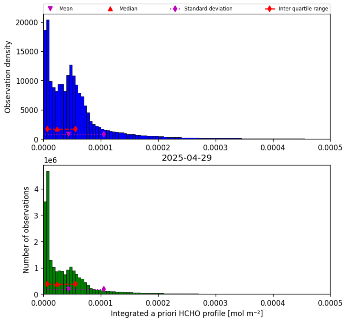
Figure 41: Histogram of “Integrated a priori HCHO profile” for 2025-04-29 to 2025-04-30
