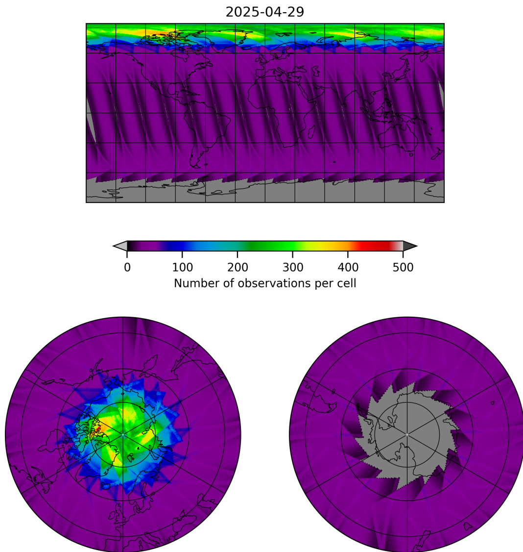
Figure 17: Map of the number of observations for 2025-04-29 to 2025-04-30
