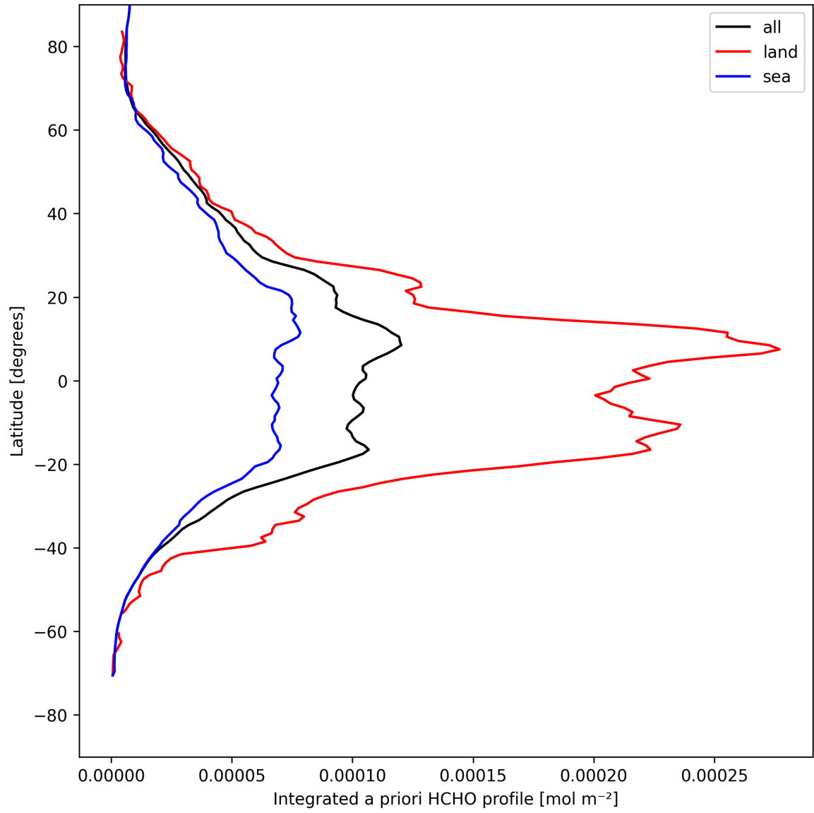
Figure 27: Zonal average of “Integrated a priori HCHO profile” for 2025-04-29 to 2025-04-30.
