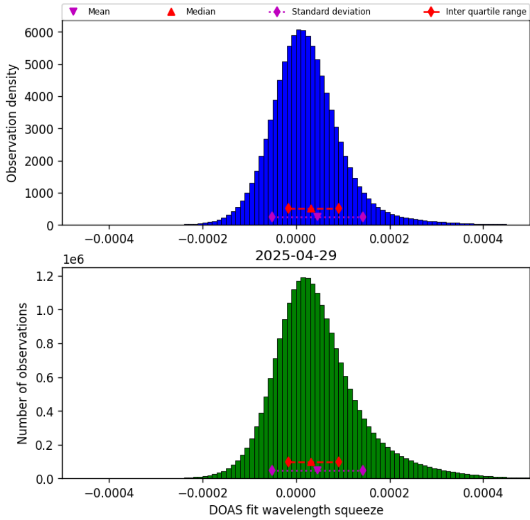
Figure 43: Histogram of “DOAS fit wavelength squeeze” for 2025-04-29 to 2025-04-30
