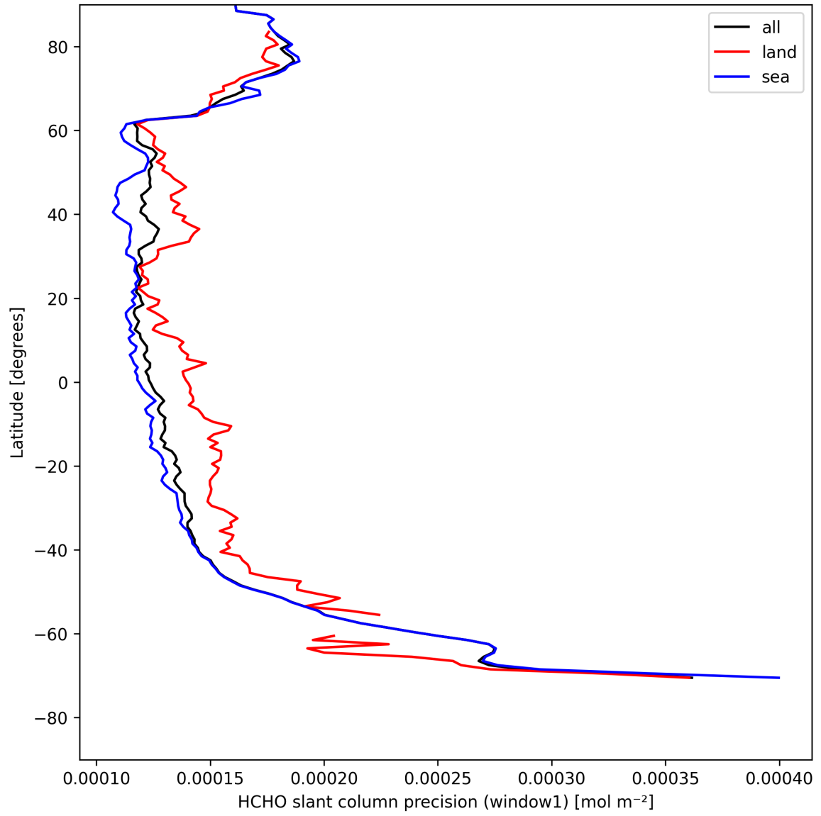
Figure 23: Zonal average of “HCHO slant column precision (window1)” for 2025-04-29 to 2025-04-30.
