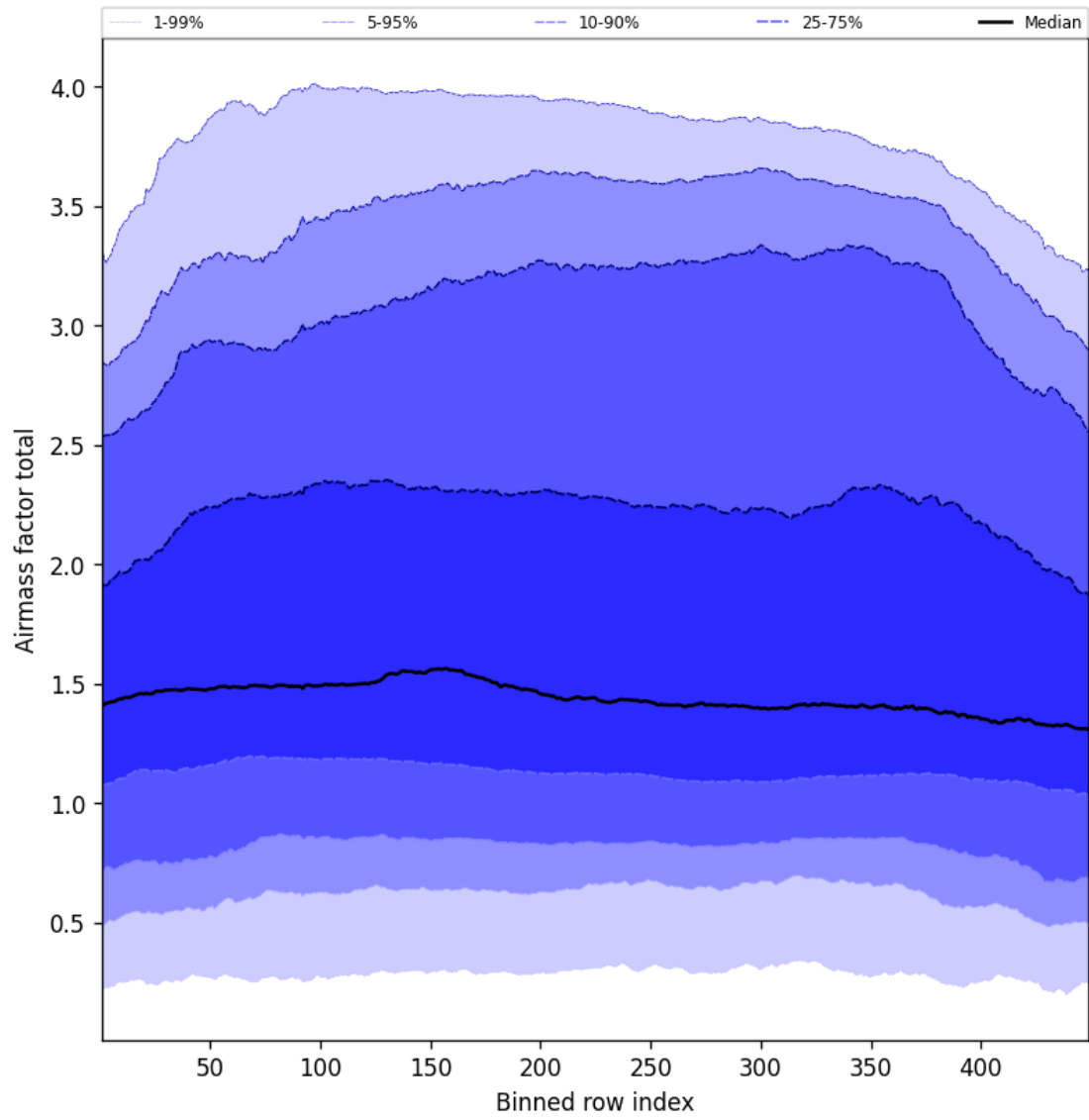
Figure 52: Along track statistics of “Airmass factor total” for 2025-04-29 to 2025-04-30
