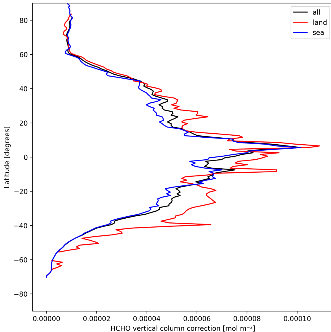
Figure 21: Zonal average of “HCHO vertical column correction” for 2025-04-29 to 2025-04-30.
