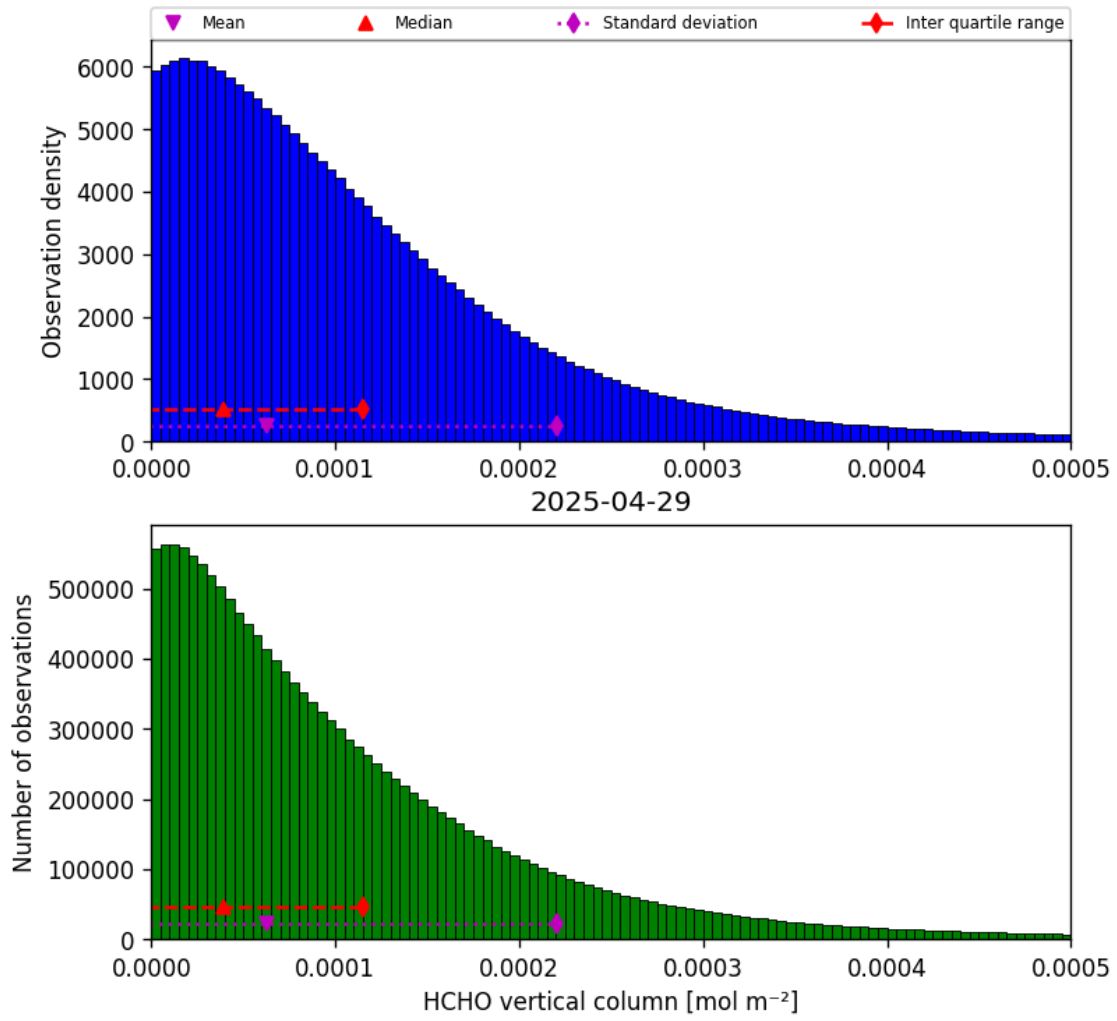
Figure 33: Histogram of “HCHO vertical column” for 2025-04-29 to 2025-04-30
