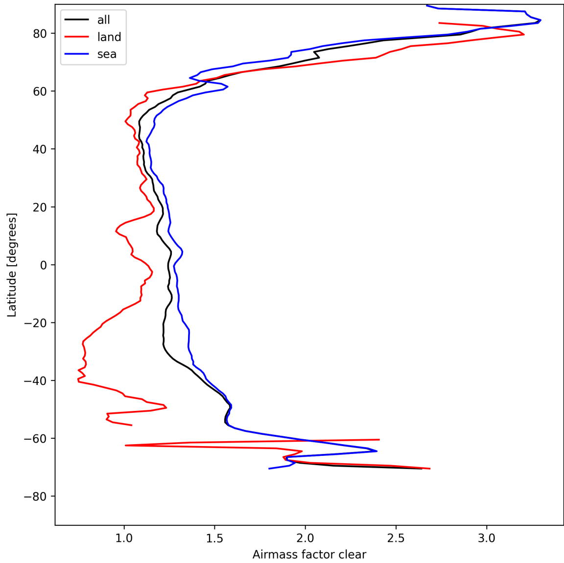
Figure 26: Zonal average of “Airmass factor clear” for 2025-04-29 to 2025-04-30.
