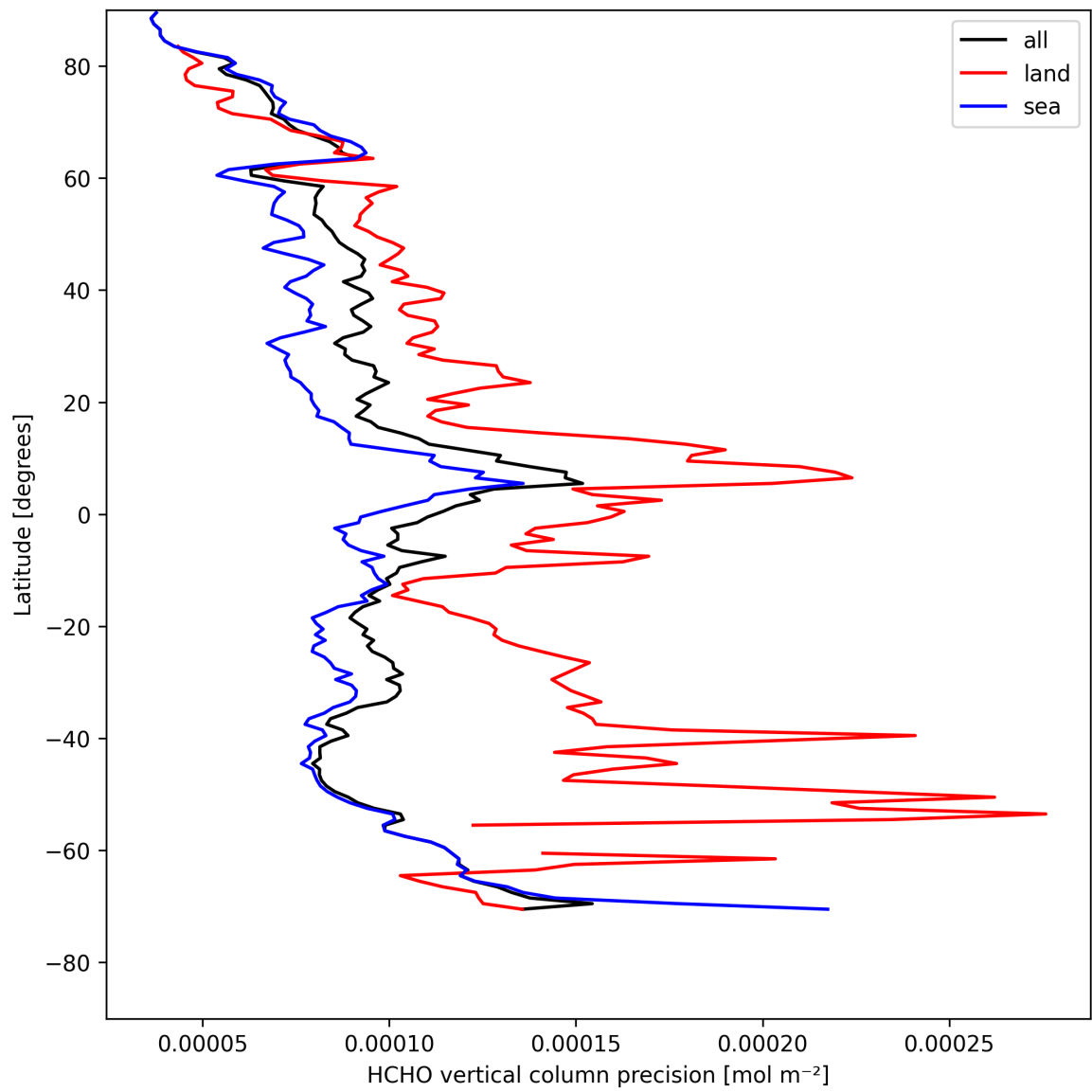
Figure 20: Zonal average of “HCHO vertical column precision” for 2025-04-29 to 2025-04-30.
