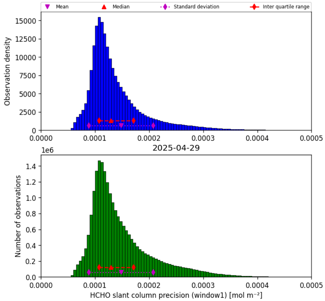
Figure 37: Histogram of “HCHO slant column precision (window1)” for 2025-04-29 to 2025-04-30
