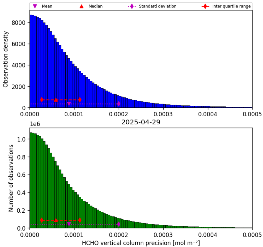
Figure 34: Histogram of “HCHO vertical column precision” for 2025-04-29 to 2025-04-30
