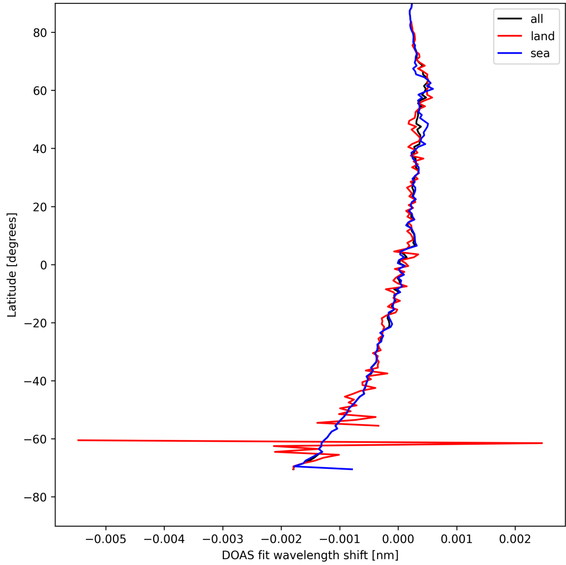
Figure 28: Zonal average of “DOAS fit wavelength shift” for 2025-04-29 to 2025-04-30.
