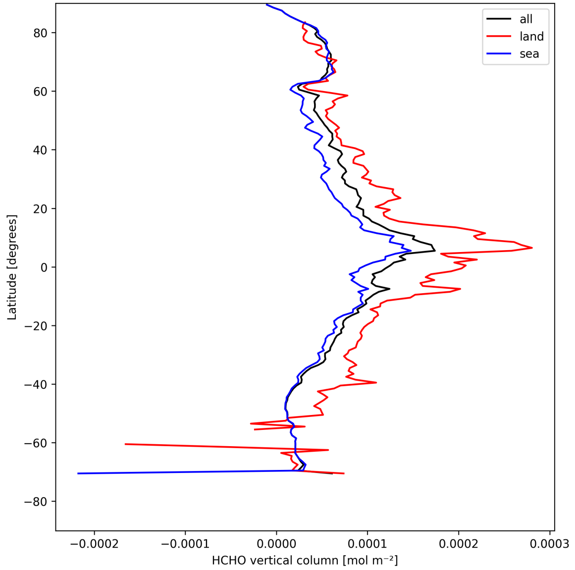
Figure 19: Zonal average of “HCHO vertical column” for 2025-04-29 to 2025-04-30.
