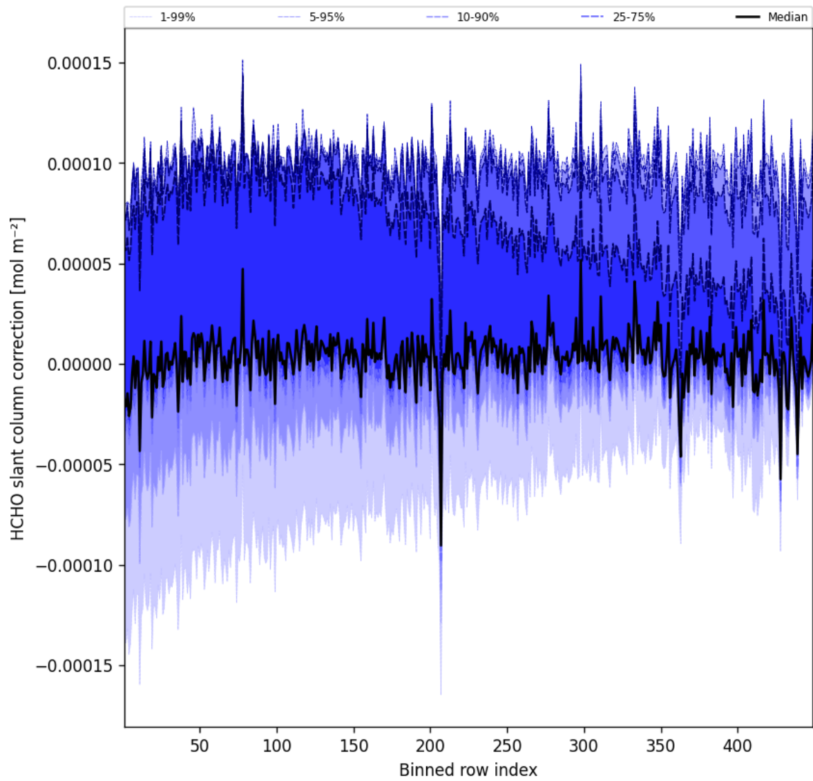
Figure 59: Along track statistics of “HCHO slant column correction” for 2025-04-29 to 2025-04-30
