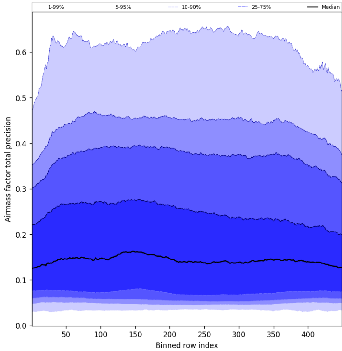
Figure 53: Along track statistics of “Airmass factor total precision” for 2025-04-29 to 2025-04-30
