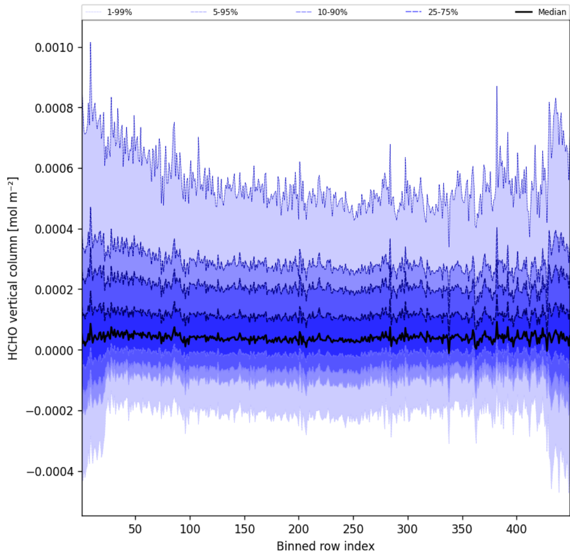
Figure 47: Along track statistics of “HCHO vertical column” for 2025-04-29 to 2025-04-30
