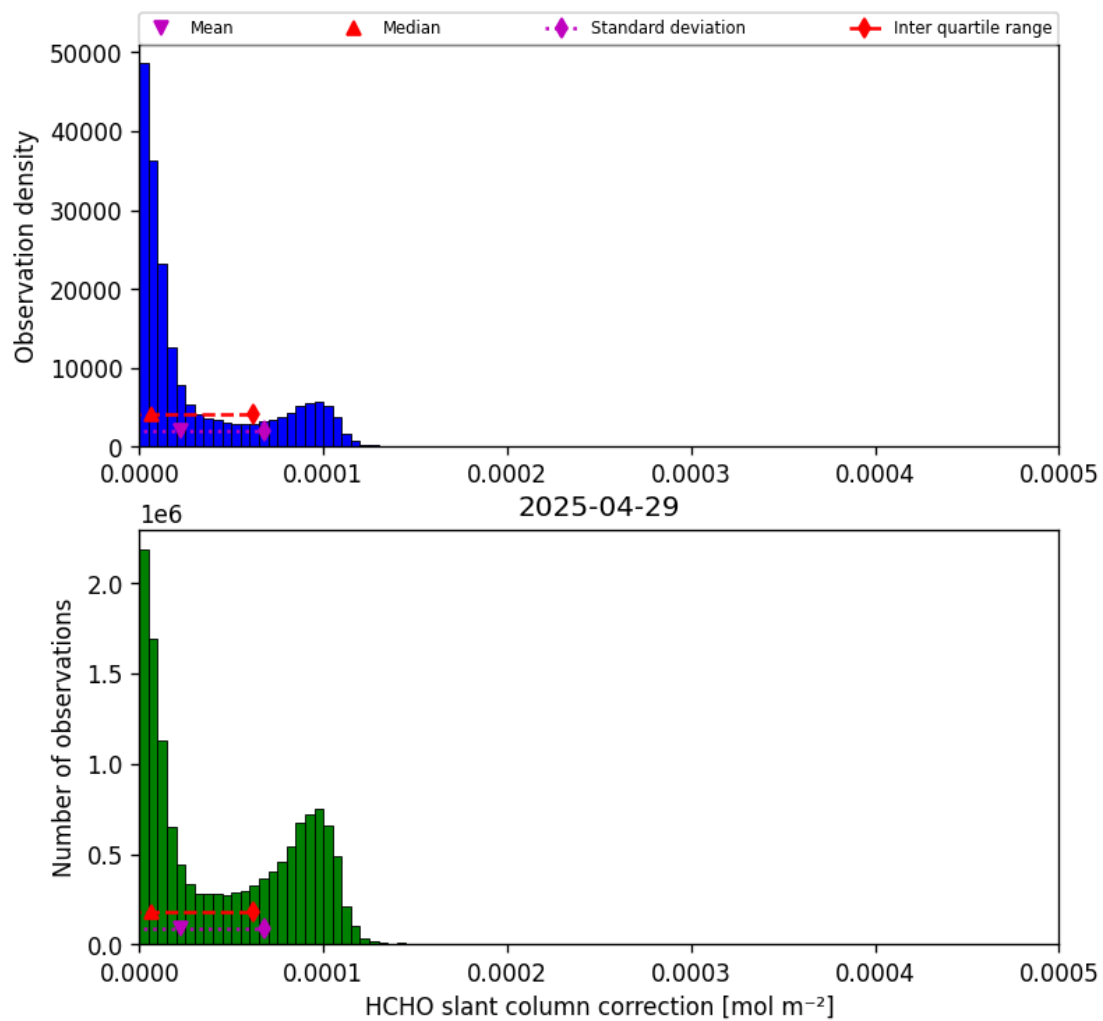
Figure 45: Histogram of “HCHO slant column correction” for 2025-04-29 to 2025-04-30
