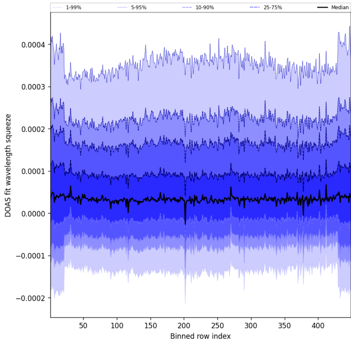
Figure 57: Along track statistics of “DOAS fit wavelength squeeze” for 2025-04-29 to 2025-04-30
