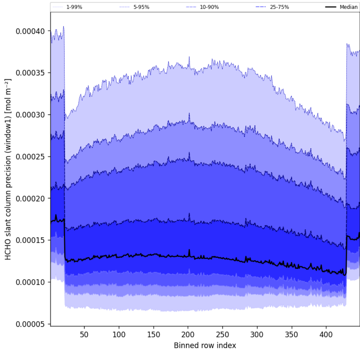
Figure 51: Along track statistics of “HCHO slant column precision (window1)” for 2025-04-29 to 2025-04-30
