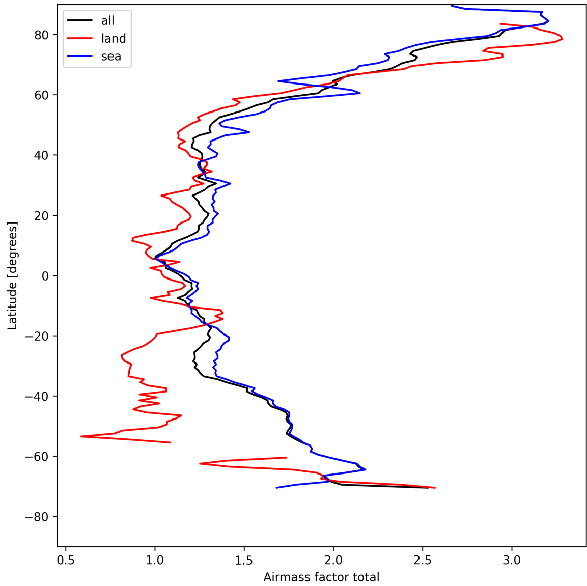
Figure 24: Zonal average of “Airmass factor total” for 2025-04-29 to 2025-04-30.
