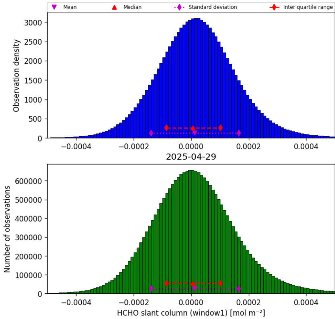
Figure 36: Histogram of “HCHO slant column (window1)” for 2025-04-29 to 2025-04-30
