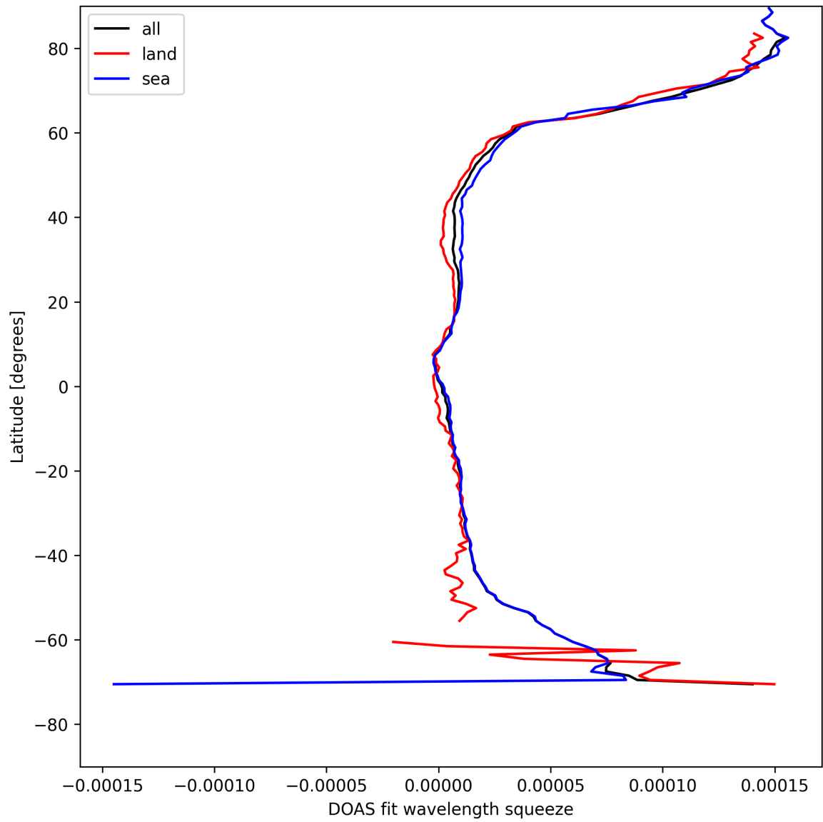
Figure 29: Zonal average of “DOAS fit wavelength squeeze” for 2025-04-29 to 2025-04-30.
