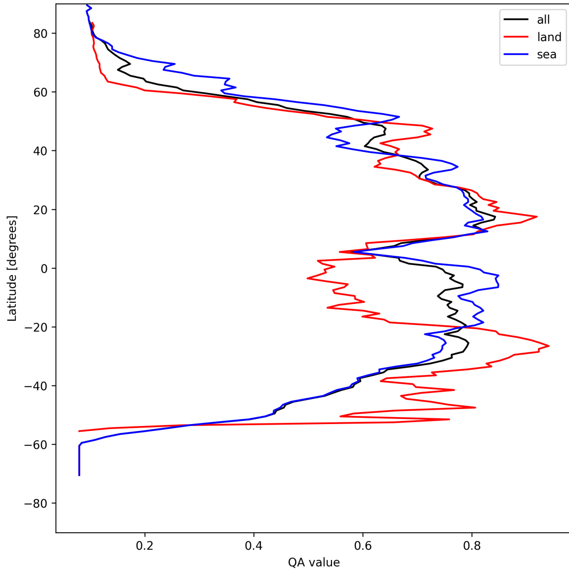
Figure 18: Zonal average of “QA value” for 2025-04-29 to 2025-04-30.
