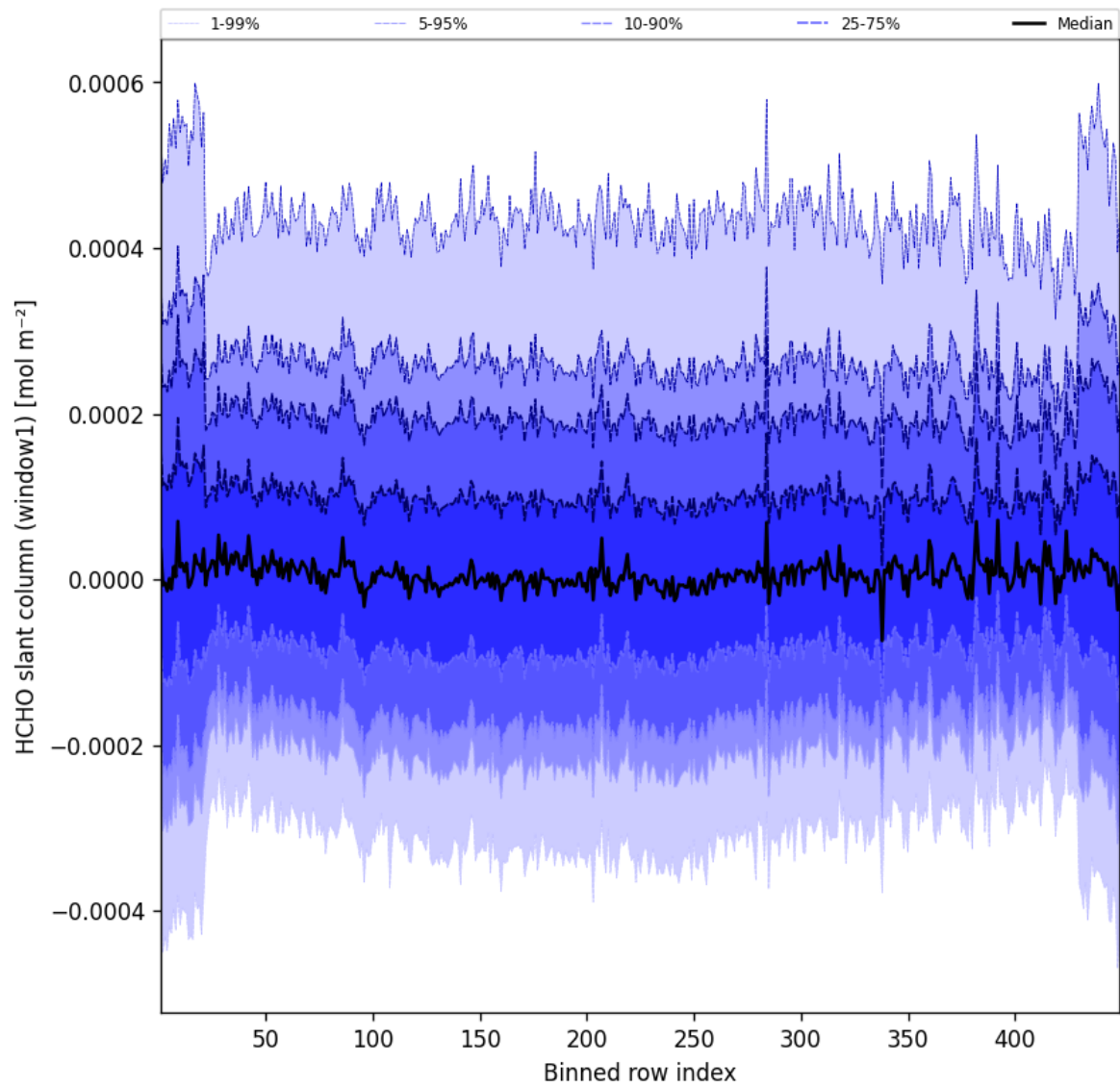
Figure 50: Along track statistics of “HCHO slant column (window1)” for 2025-04-29 to 2025-04-30
