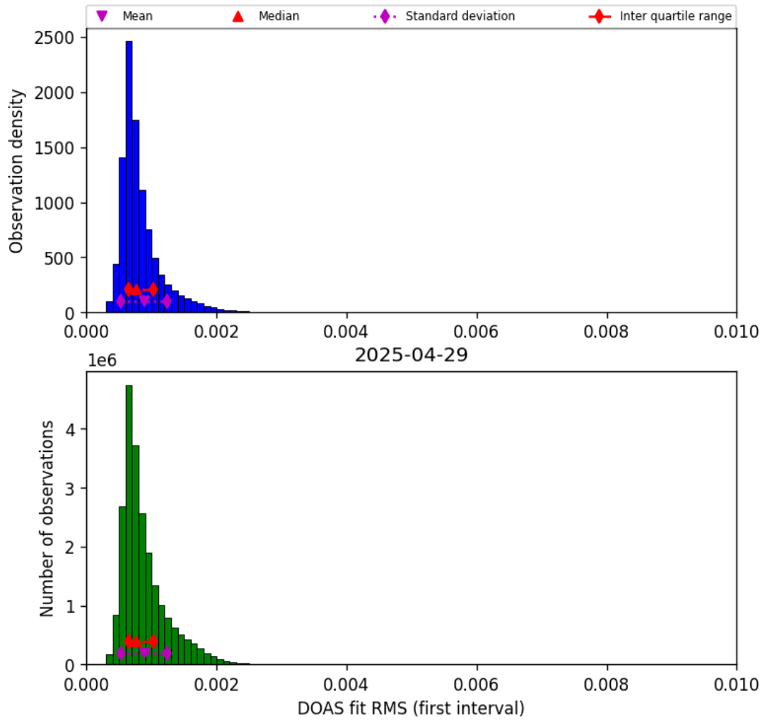
Figure 44: Histogram of “DOAS fit RMS (first interval)” for 2025-04-29 to 2025-04-30
