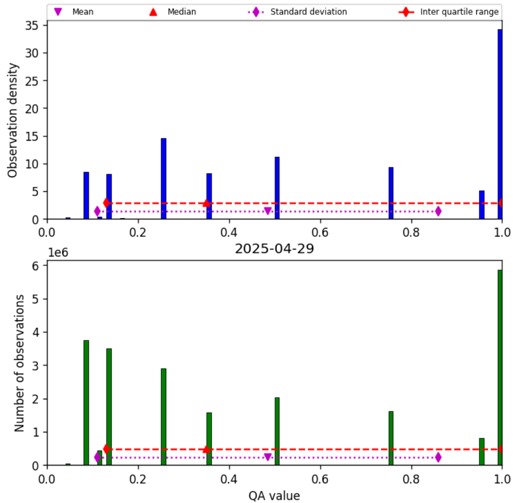
Figure 32: Histogram of “QA value” for 2025-04-29 to 2025-04-30
