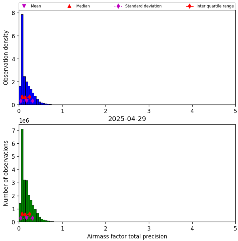
Figure 39: Histogram of “Airmass factor total precision” for 2025-04-29 to 2025-04-30
