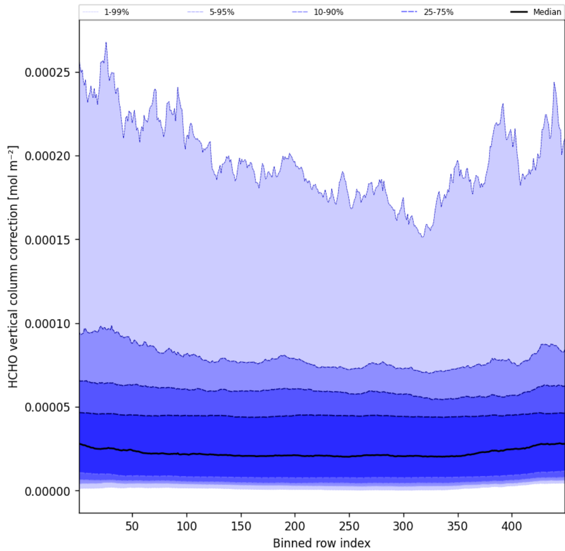
Figure 49: Along track statistics of “HCHO vertical column correction” for 2025-04-29 to 2025-04-30
