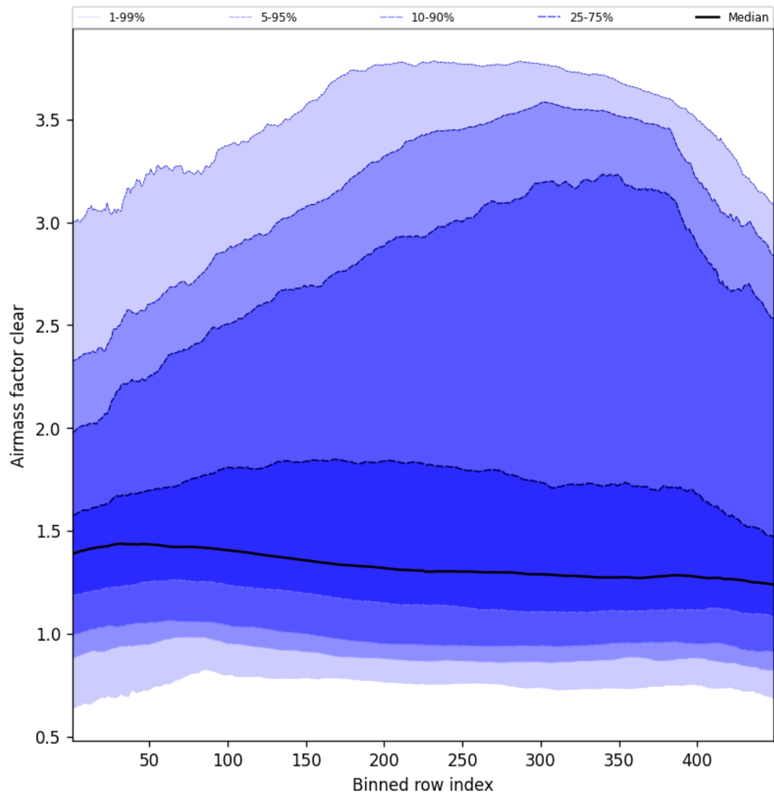
Figure 54: Along track statistics of “Airmass factor clear” for 2025-04-29 to 2025-04-30
