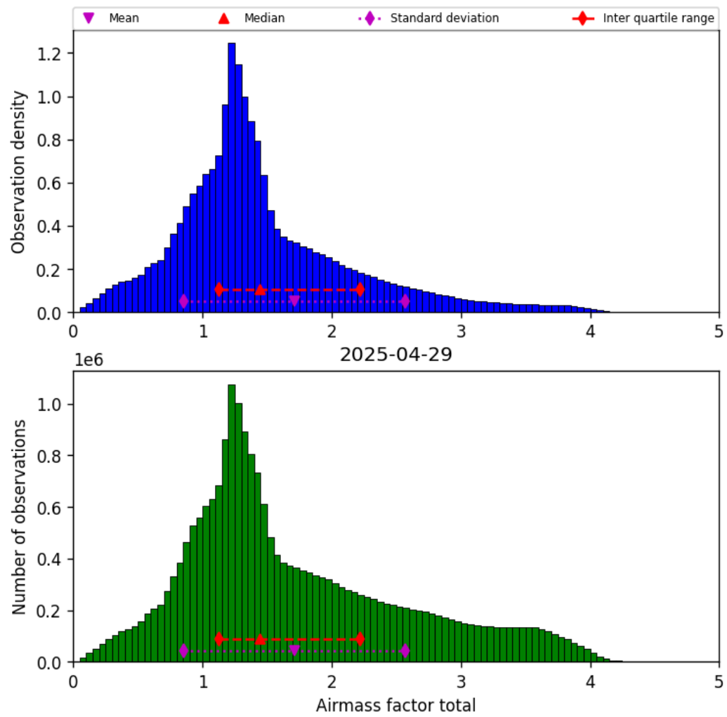
Figure 38: Histogram of “Airmass factor total” for 2025-04-29 to 2025-04-30
