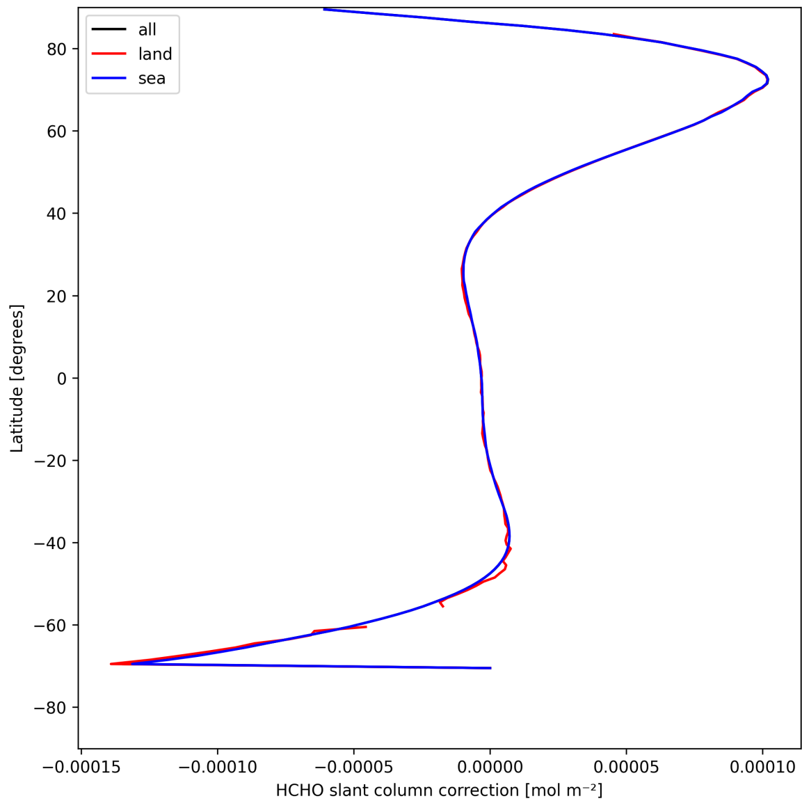
Figure 31: Zonal average of “HCHO slant column correction” for 2025-04-29 to 2025-04-30.
