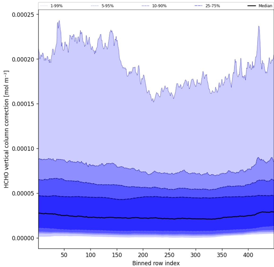
Figure 49: Along track statistics of “HCHO vertical column correction” for 2025-04-30 to 2025-05-01
