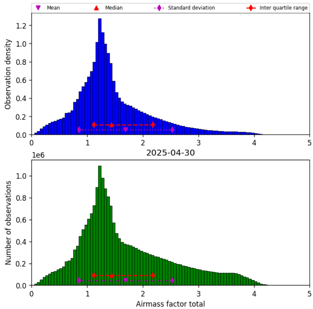
Figure 38: Histogram of “Airmass factor total” for 2025-04-30 to 2025-05-01
