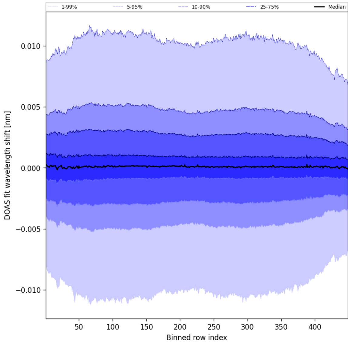
Figure 56: Along track statistics of “DOAS fit wavelength shift” for 2025-04-30 to 2025-05-01
