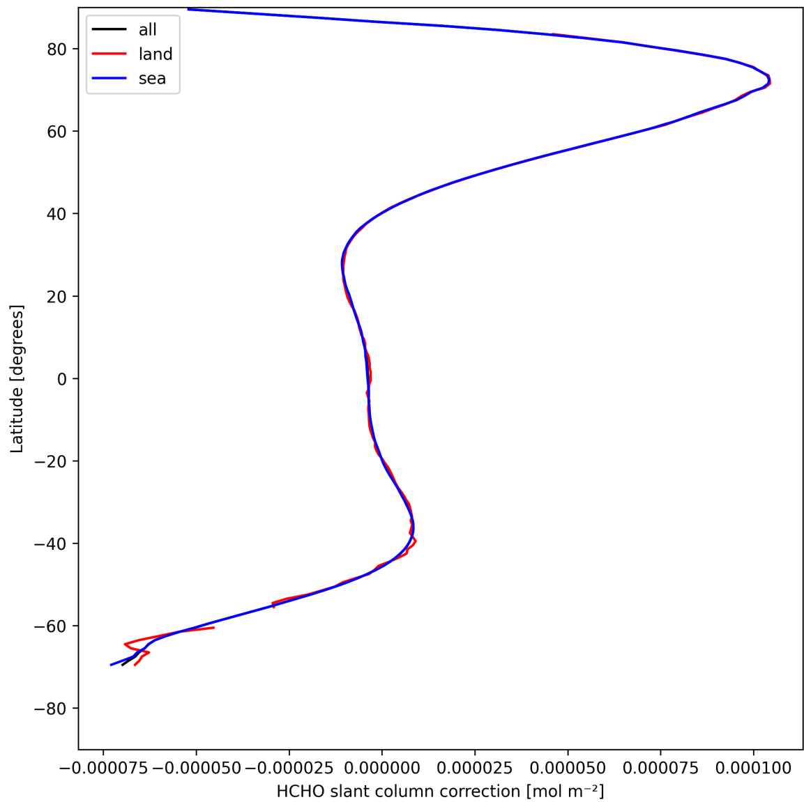
Figure 31: Zonal average of “HCHO slant column correction” for 2025-04-30 to 2025-05-01.
