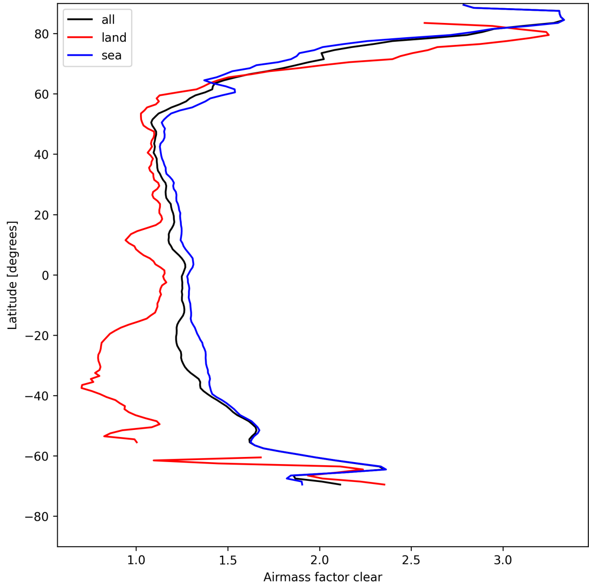
Figure 26: Zonal average of “Airmass factor clear” for 2025-04-30 to 2025-05-01.
