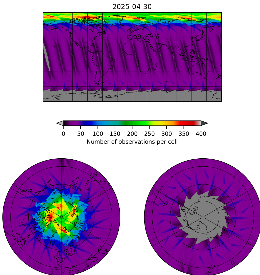
Figure 17: Map of the number of observations for 2025-04-30 to 2025-05-01
