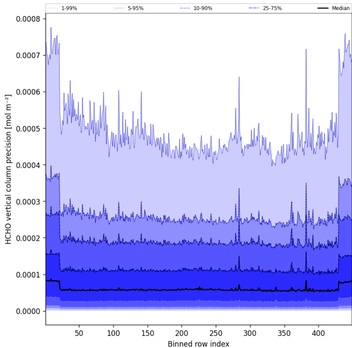
Figure 48: Along track statistics of “HCHO vertical column precision” for 2025-04-30 to 2025-05-01
