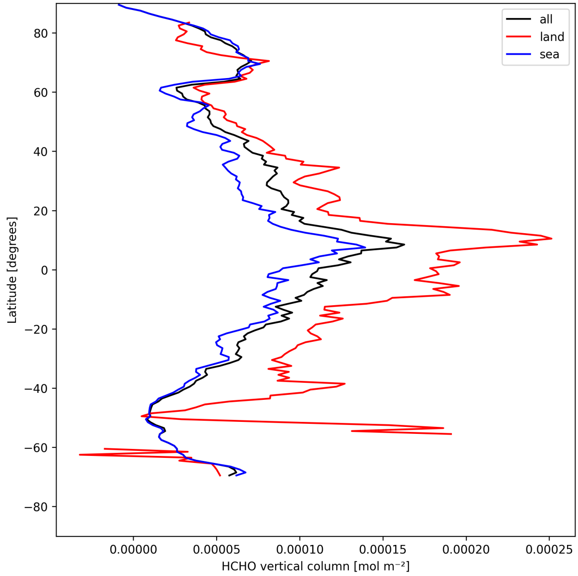
Figure 19: Zonal average of “HCHO vertical column” for 2025-04-30 to 2025-05-01.
