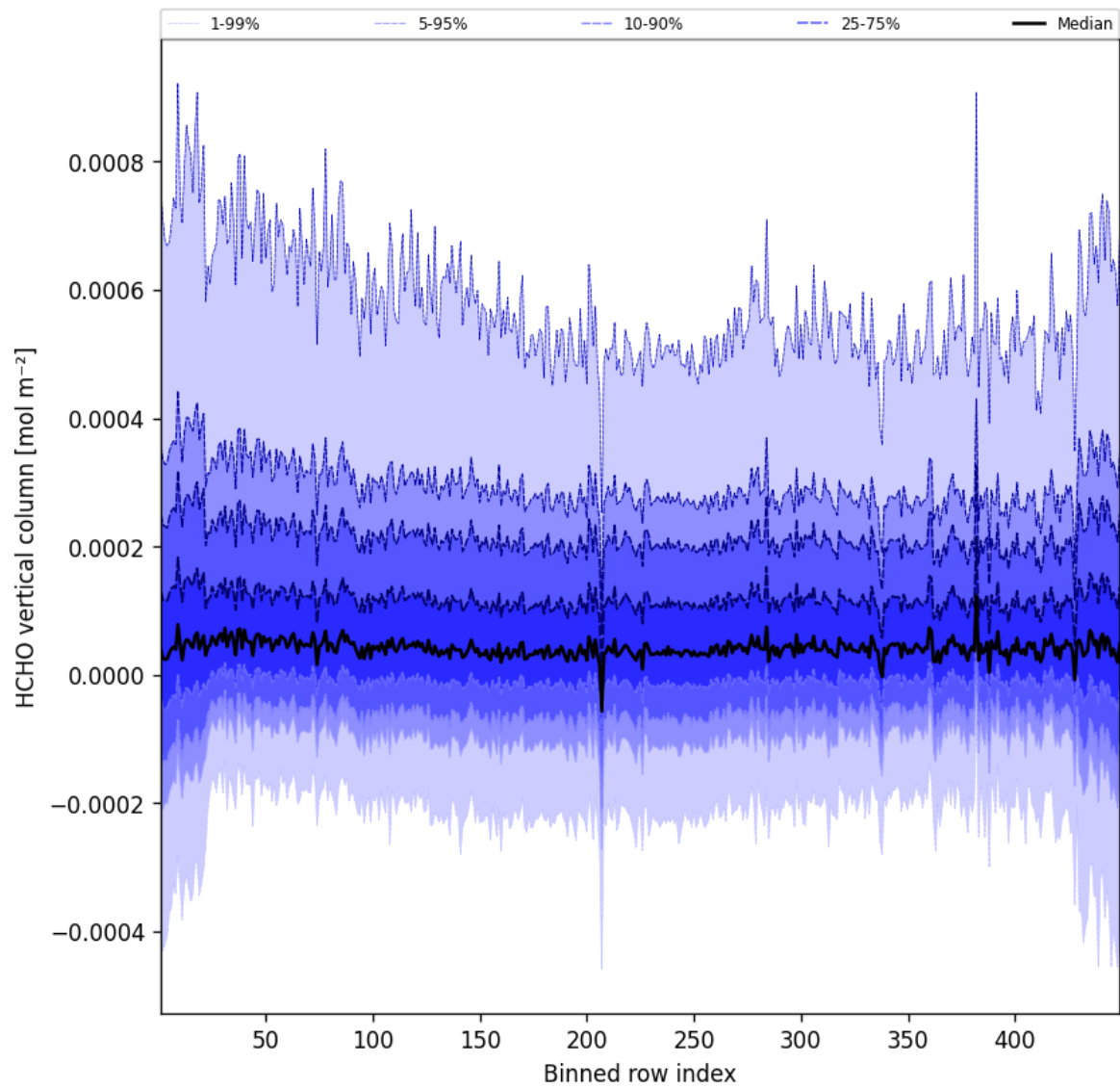
Figure 47: Along track statistics of “HCHO vertical column” for 2025-04-30 to 2025-05-01
