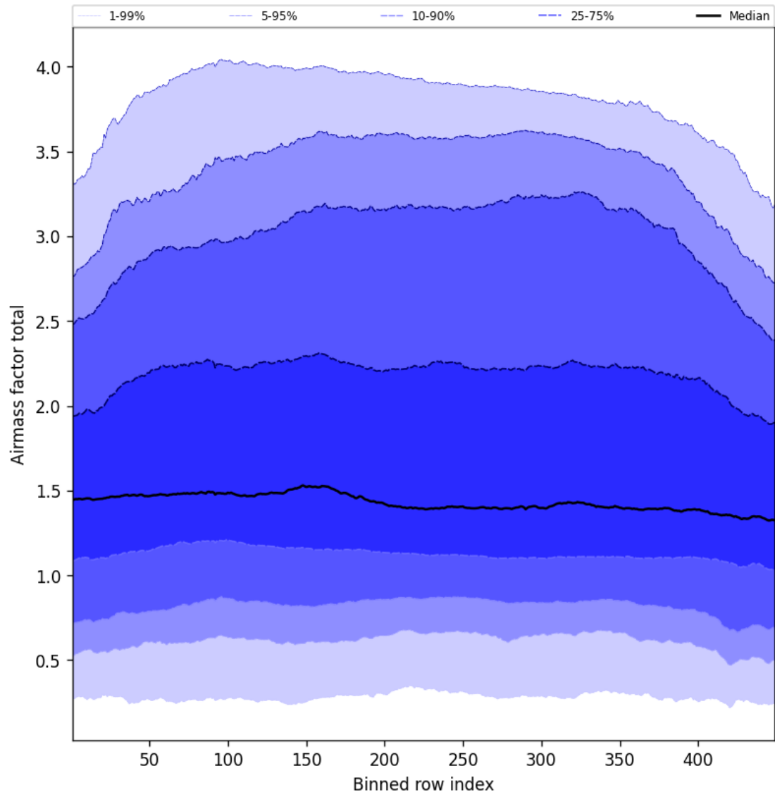
Figure 52: Along track statistics of “Airmass factor total” for 2025-04-30 to 2025-05-01
