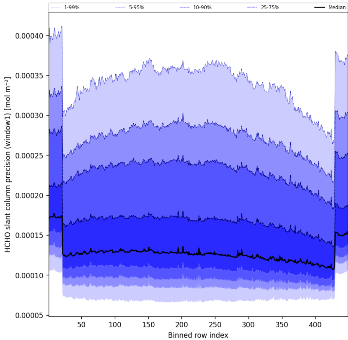
Figure 51: Along track statistics of “HCHO slant column precision (window1)” for 2025-04-30 to 2025-05-01
