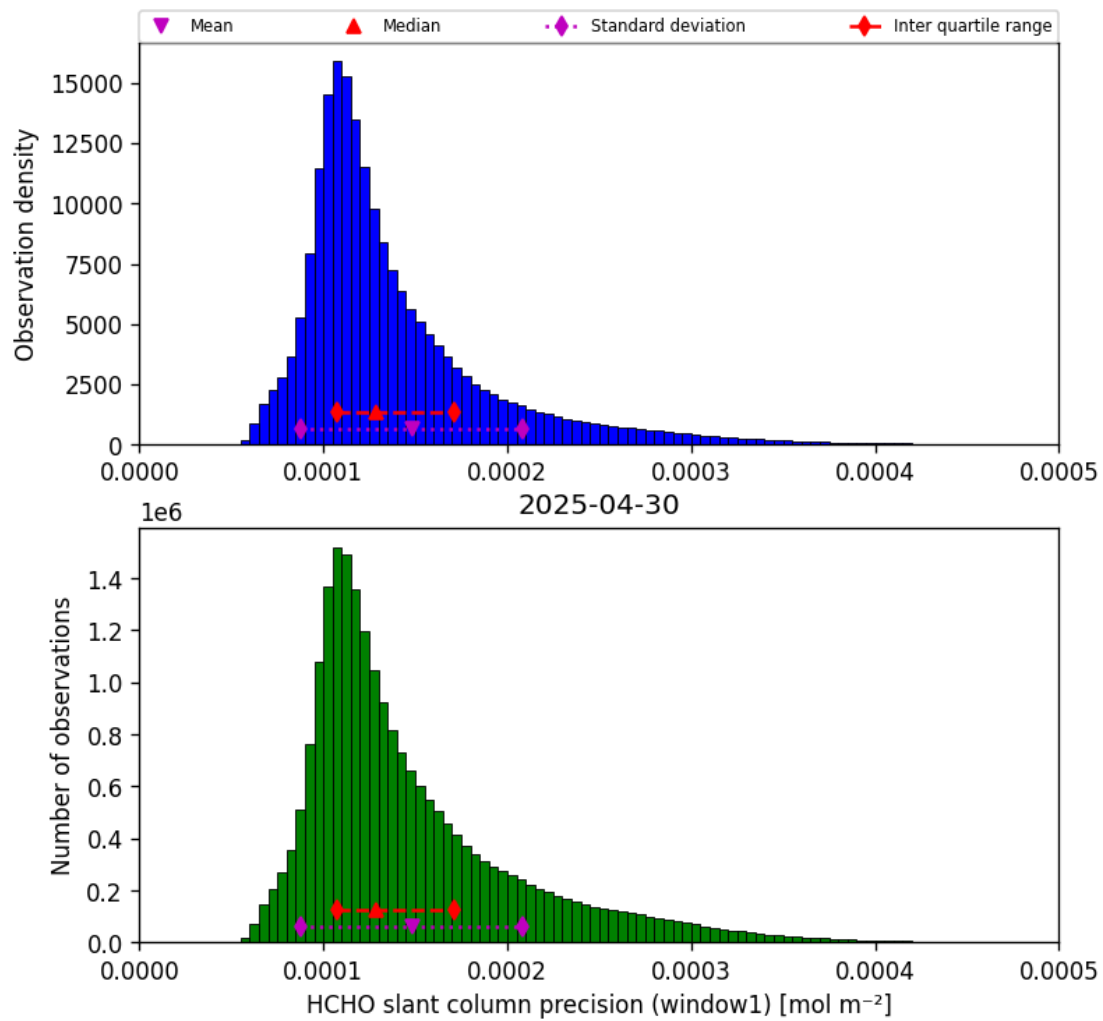
Figure 37: Histogram of “HCHO slant column precision (window1)” for 2025-04-30 to 2025-05-01
