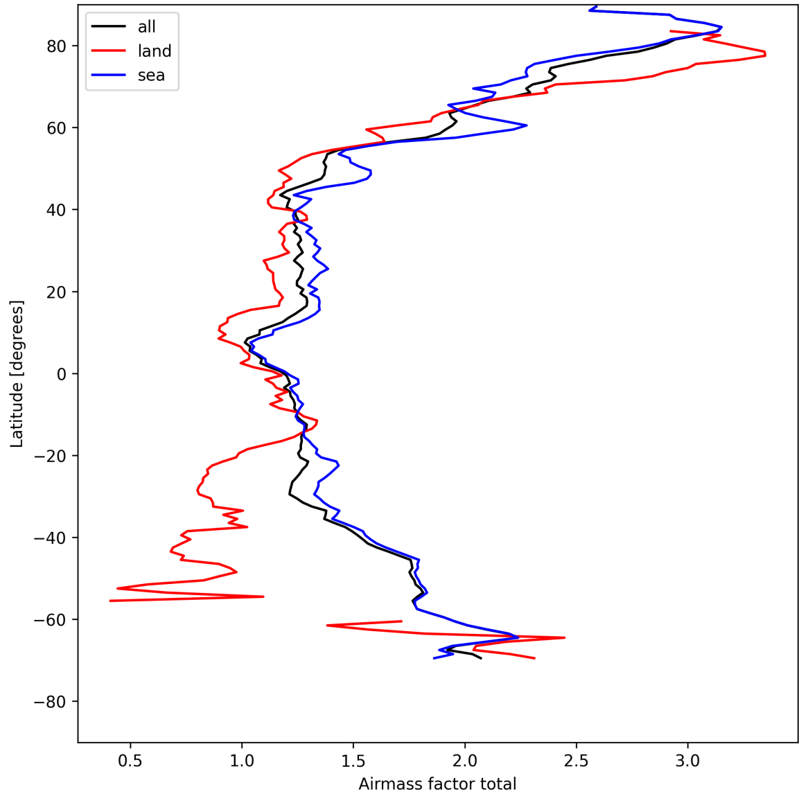
Figure 24: Zonal average of “Airmass factor total” for 2025-04-30 to 2025-05-01.
