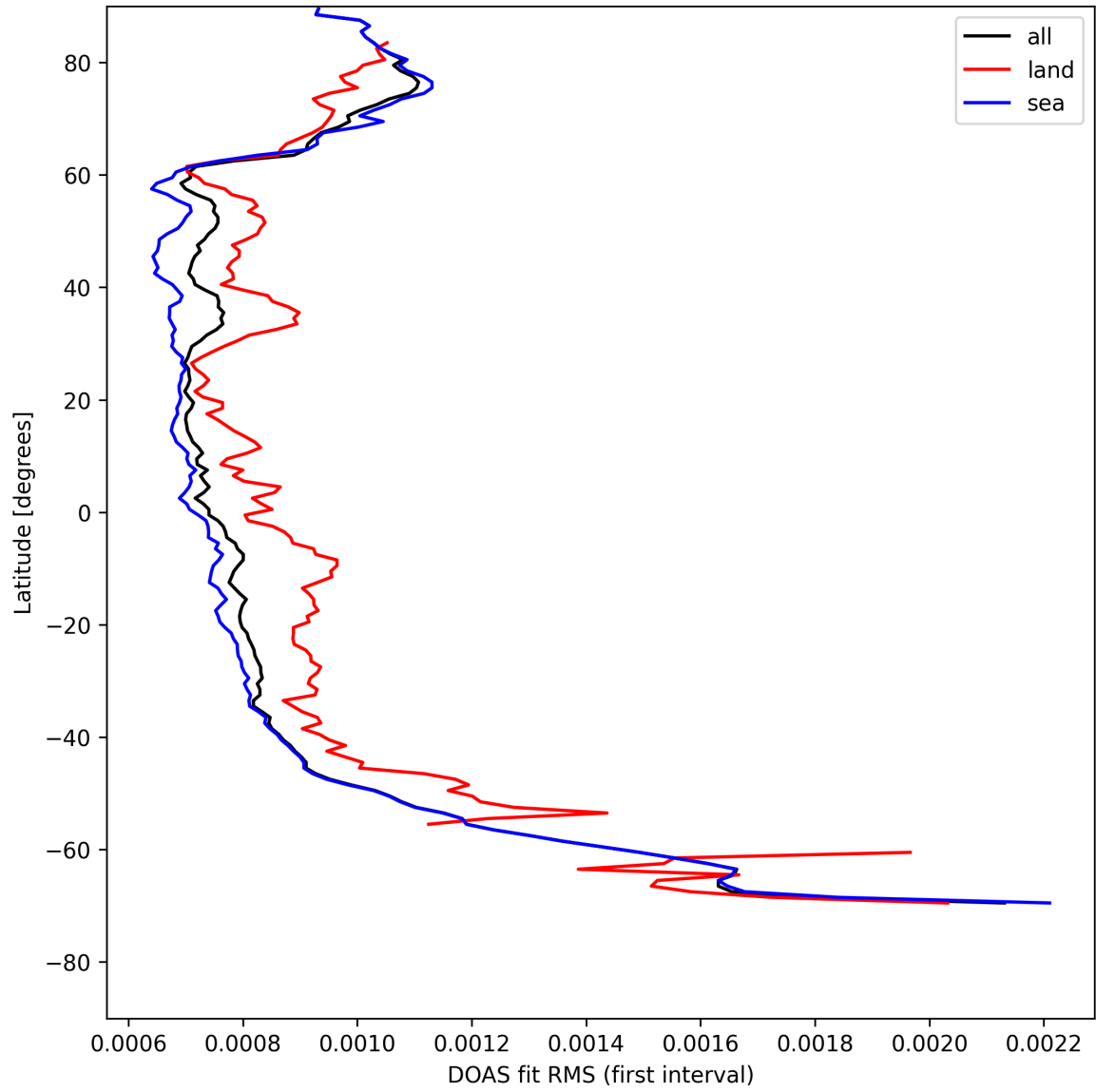
Figure 30: Zonal average of "DOAS fit RMS (first interval)" for 2025-04-30 to 2025-05-01.
