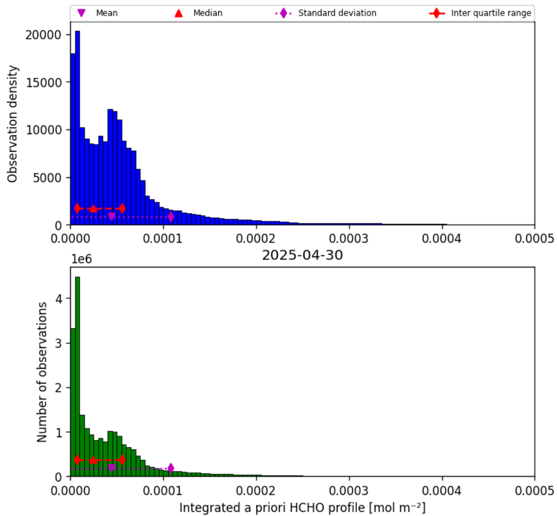
Figure 41: Histogram of “Integrated a priori HCHO profile” for 2025-04-30 to 2025-05-01
