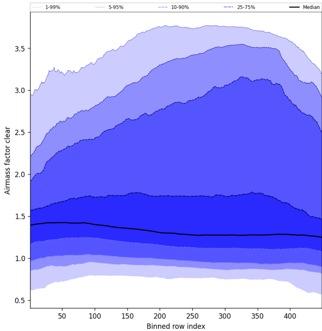
Figure 54: Along track statistics of “Airmass factor clear” for 2025-04-30 to 2025-05-01
