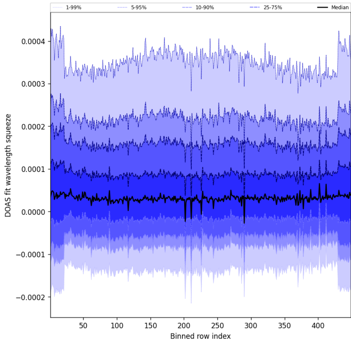
Figure 57: Along track statistics of “DOAS fit wavelength squeeze” for 2025-04-30 to 2025-05-01
