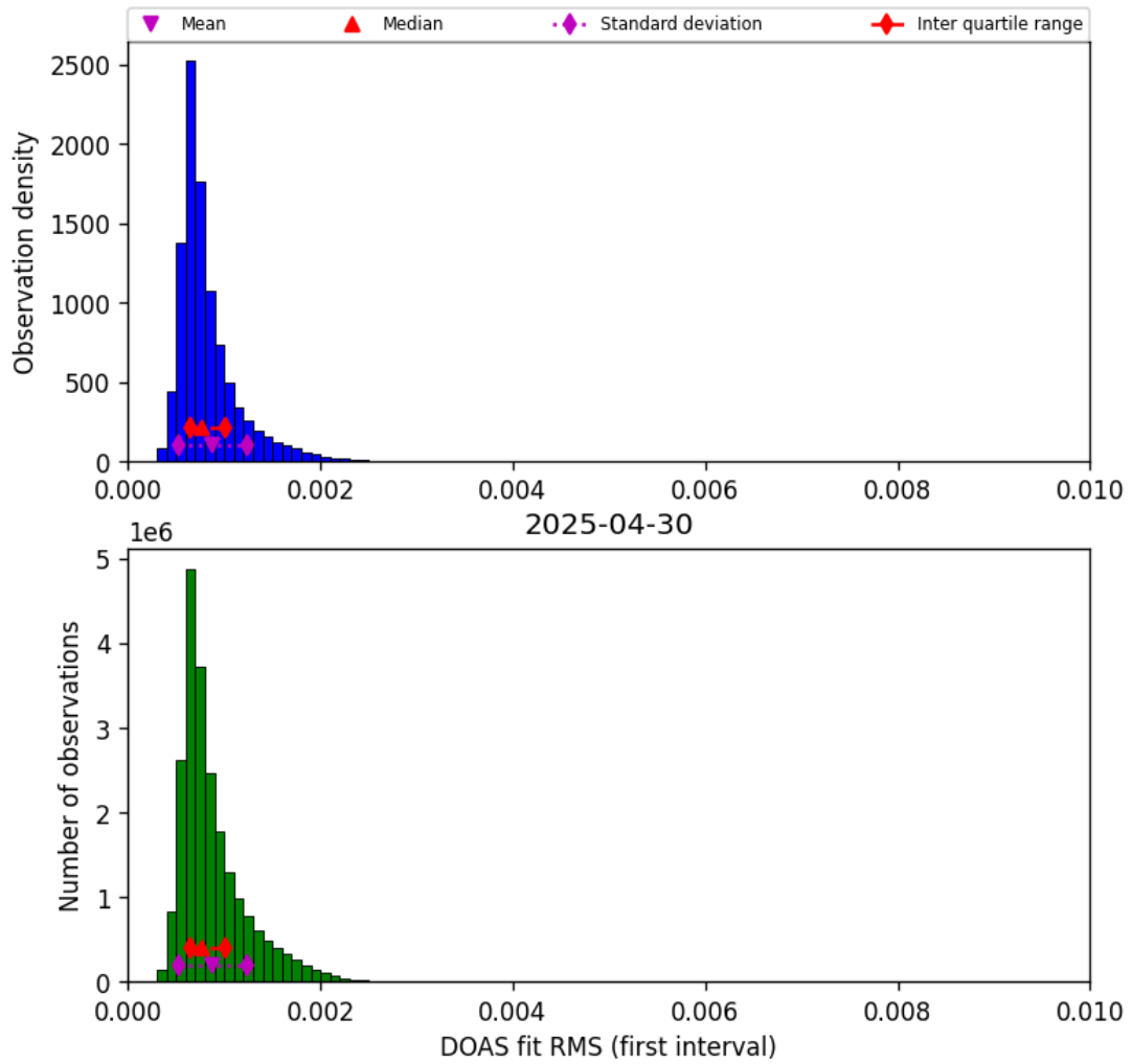
Figure 44: Histogram of “DOAS fit RMS (first interval)” for 2025-04-30 to 2025-05-01
