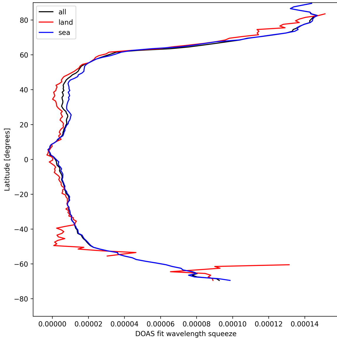
Figure 29: Zonal average of “DOAS fit wavelength squeeze” for 2025-04-30 to 2025-05-01.
