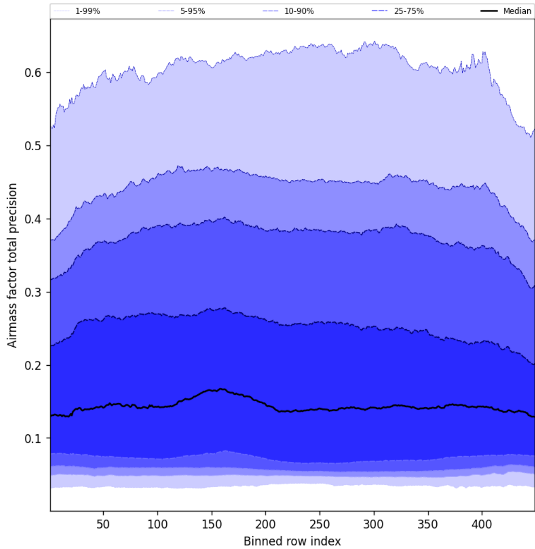
Figure 53: Along track statistics of “Airmass factor total precision” for 2025-04-30 to 2025-05-01
