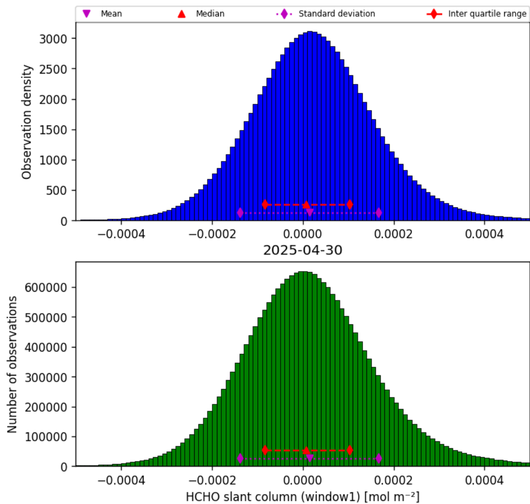
Figure 36: Histogram of “HCHO slant column (window1)” for 2025-04-30 to 2025-05-01
