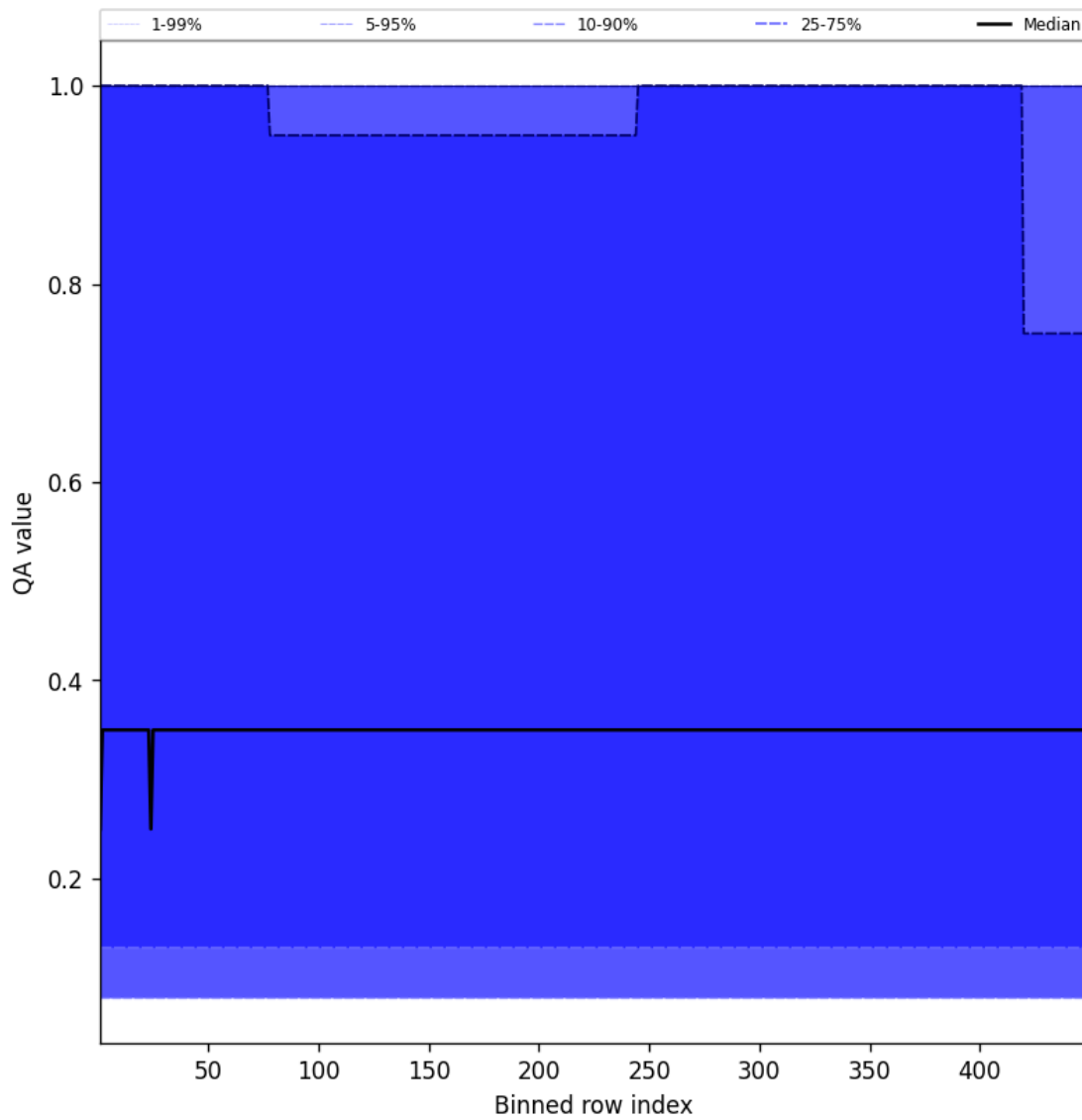
Figure 46: Along track statistics of “QA value” for 2025-04-30 to 2025-05-01
