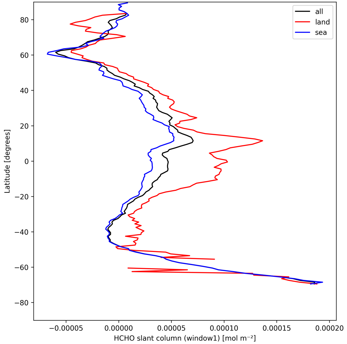
Figure 22: Zonal average of “HCHO slant column (window1)” for 2025-04-30 to 2025-05-01.
