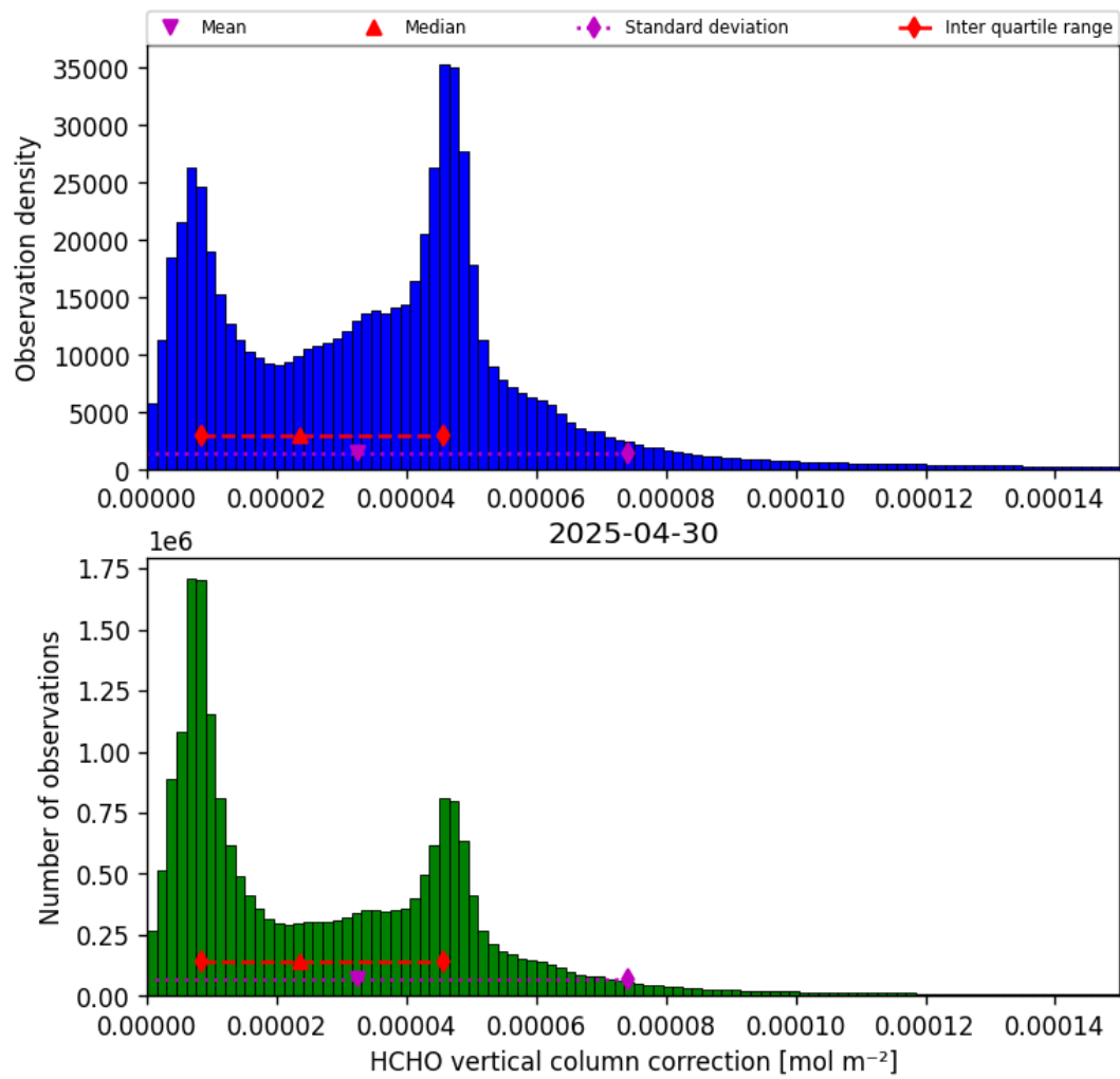
Figure 35: Histogram of “HCHO vertical column correction” for 2025-04-30 to 2025-05-01
