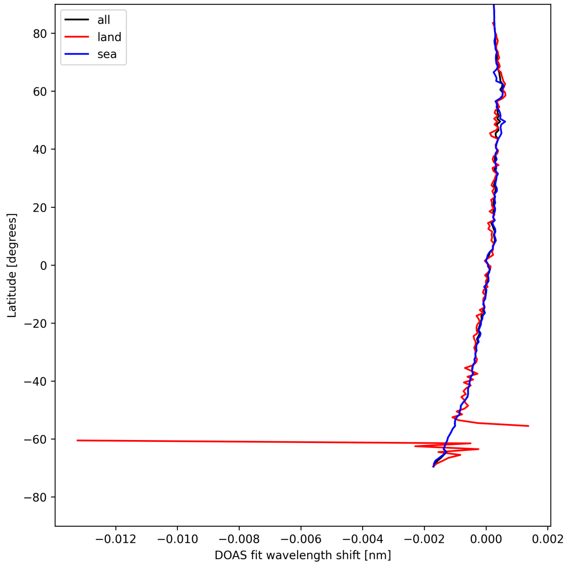
Figure 28: Zonal average of “DOAS fit wavelength shift” for 2025-04-30 to 2025-05-01.
