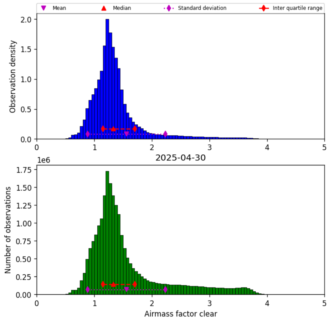
Figure 40: Histogram of “Airmass factor clear” for 2025-04-30 to 2025-05-01
