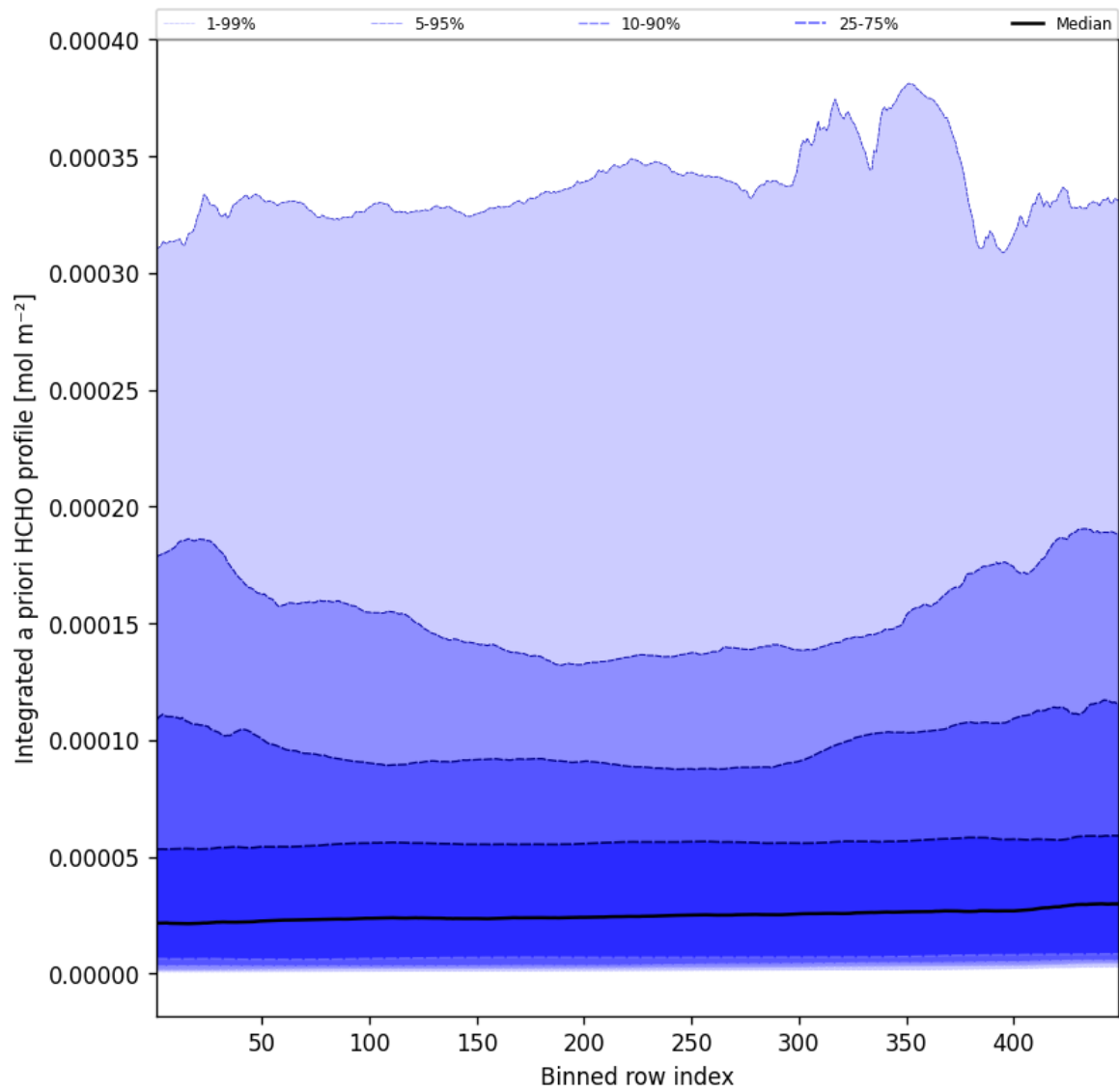
Figure 55: Along track statistics of "Integrated a priori HCHO profile" for 2025-04-30 to 2025-05-01
