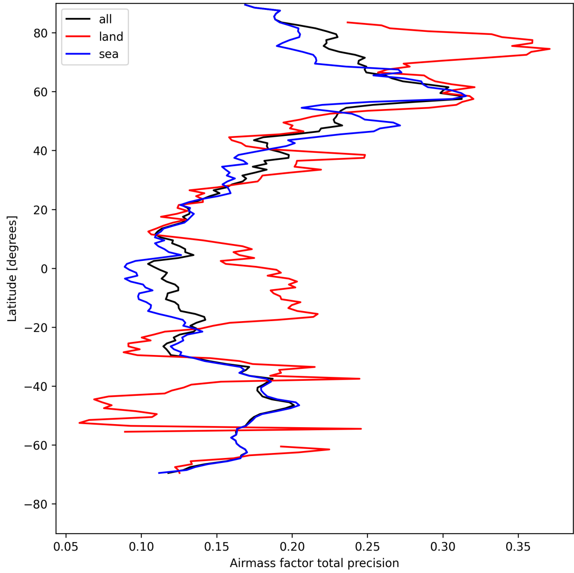
Figure 25: Zonal average of “Airmass factor total precision” for 2025-04-30 to 2025-05-01.
