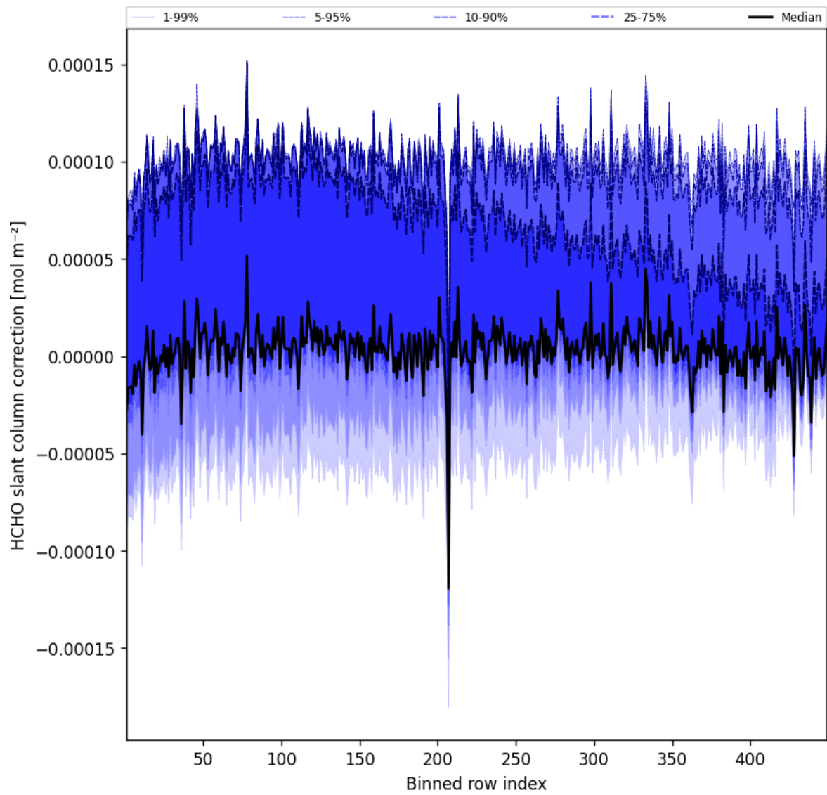
Figure 59: Along track statistics of “HCHO slant column correction” for 2025-04-30 to 2025-05-01
