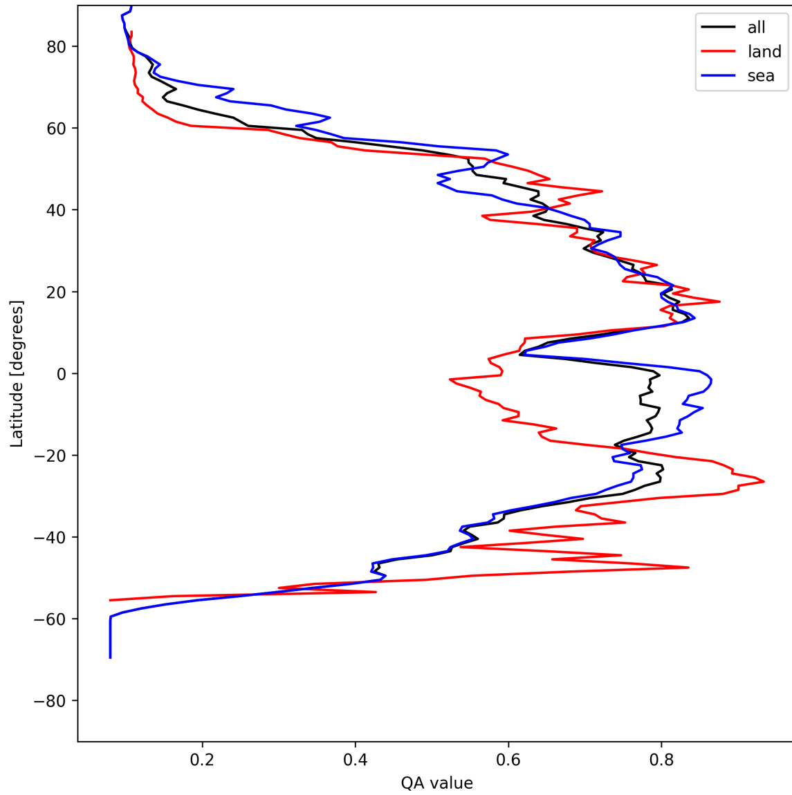
Figure 18: Zonal average of “QA value” for 2025-04-30 to 2025-05-01.
