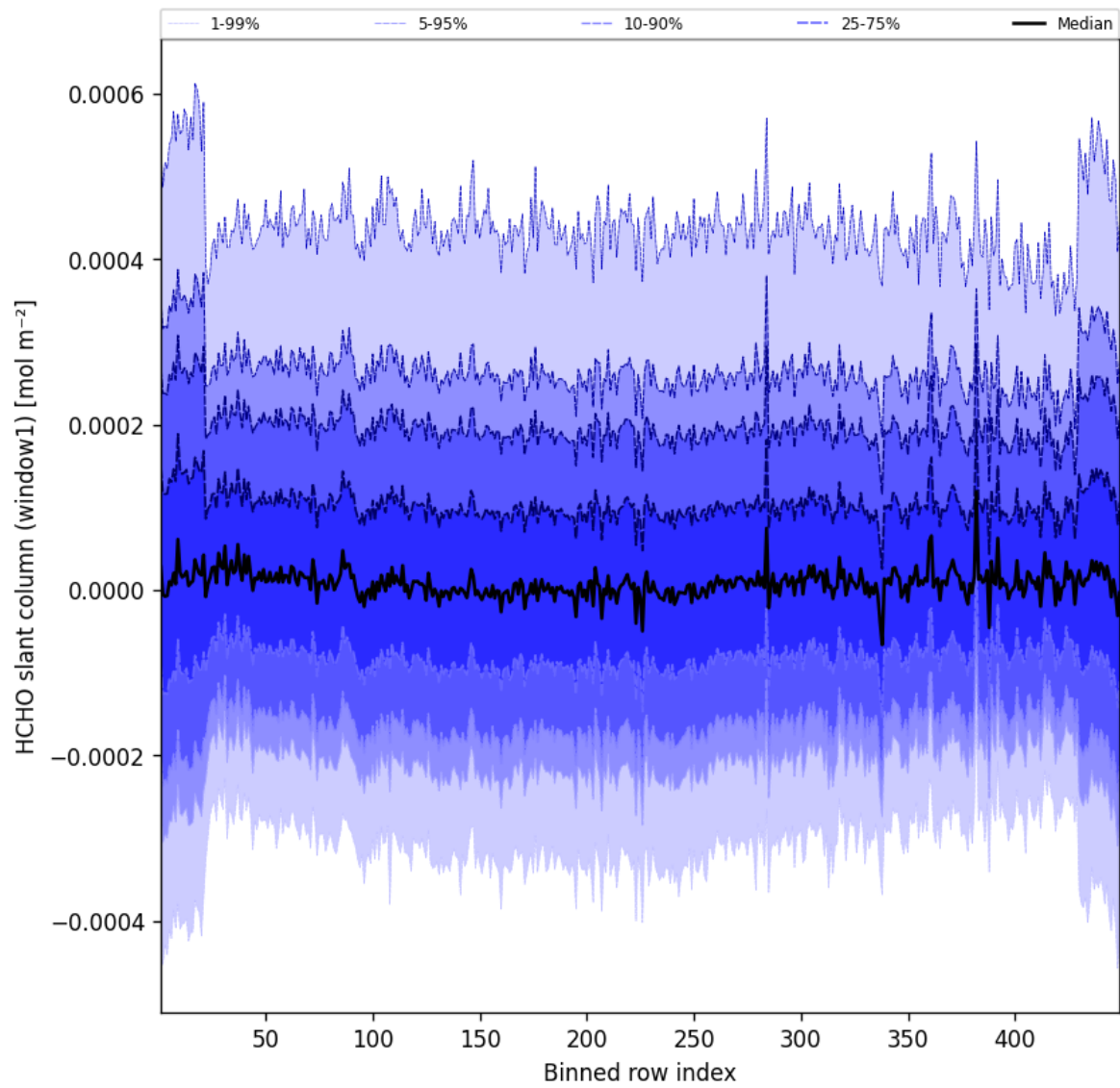
Figure 50: Along track statistics of “HCHO slant column (window1)” for 2025-04-30 to 2025-05-01
