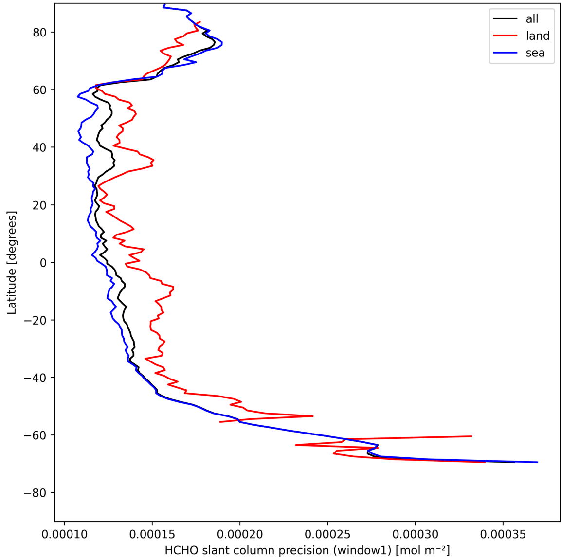
Figure 23: Zonal average of "HCHO slant column precision (window1)" for 2025-04-30 to 2025-05-01.
