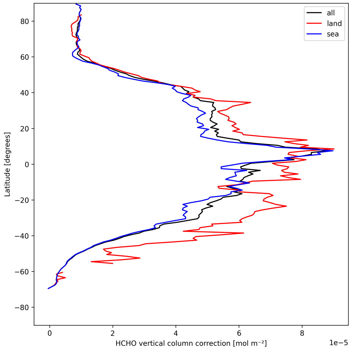
Figure 21: Zonal average of “HCHO vertical column correction” for 2025-04-30 to 2025-05-01.
