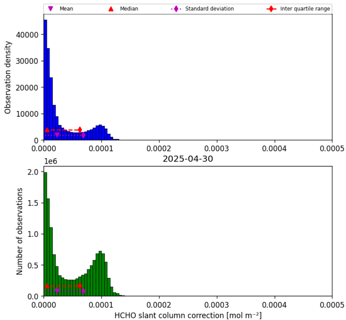
Figure 45: Histogram of “HCHO slant column correction” for 2025-04-30 to 2025-05-01
