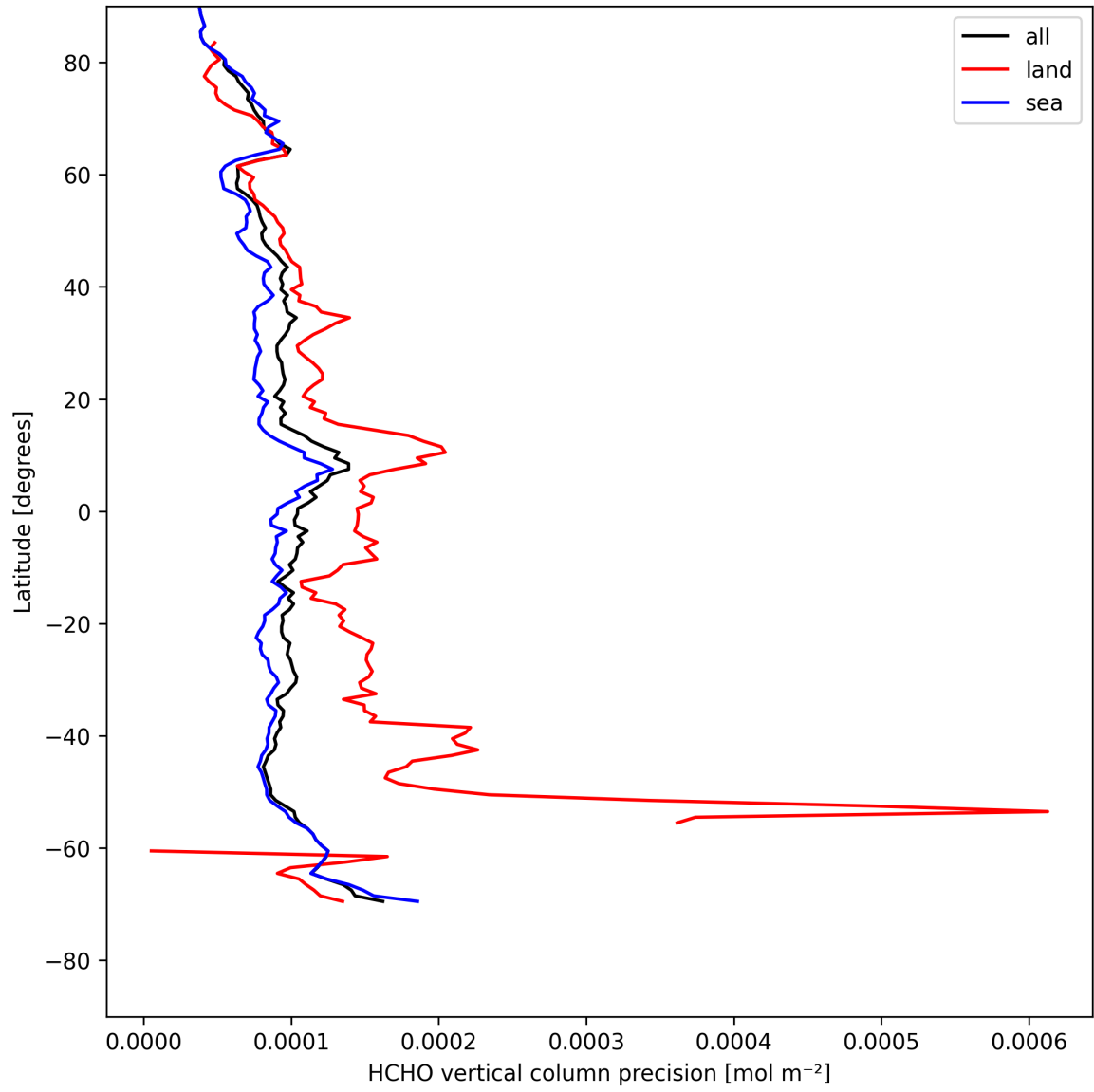
Figure 20: Zonal average of “HCHO vertical column precision” for 2025-04-30 to 2025-05-01.
