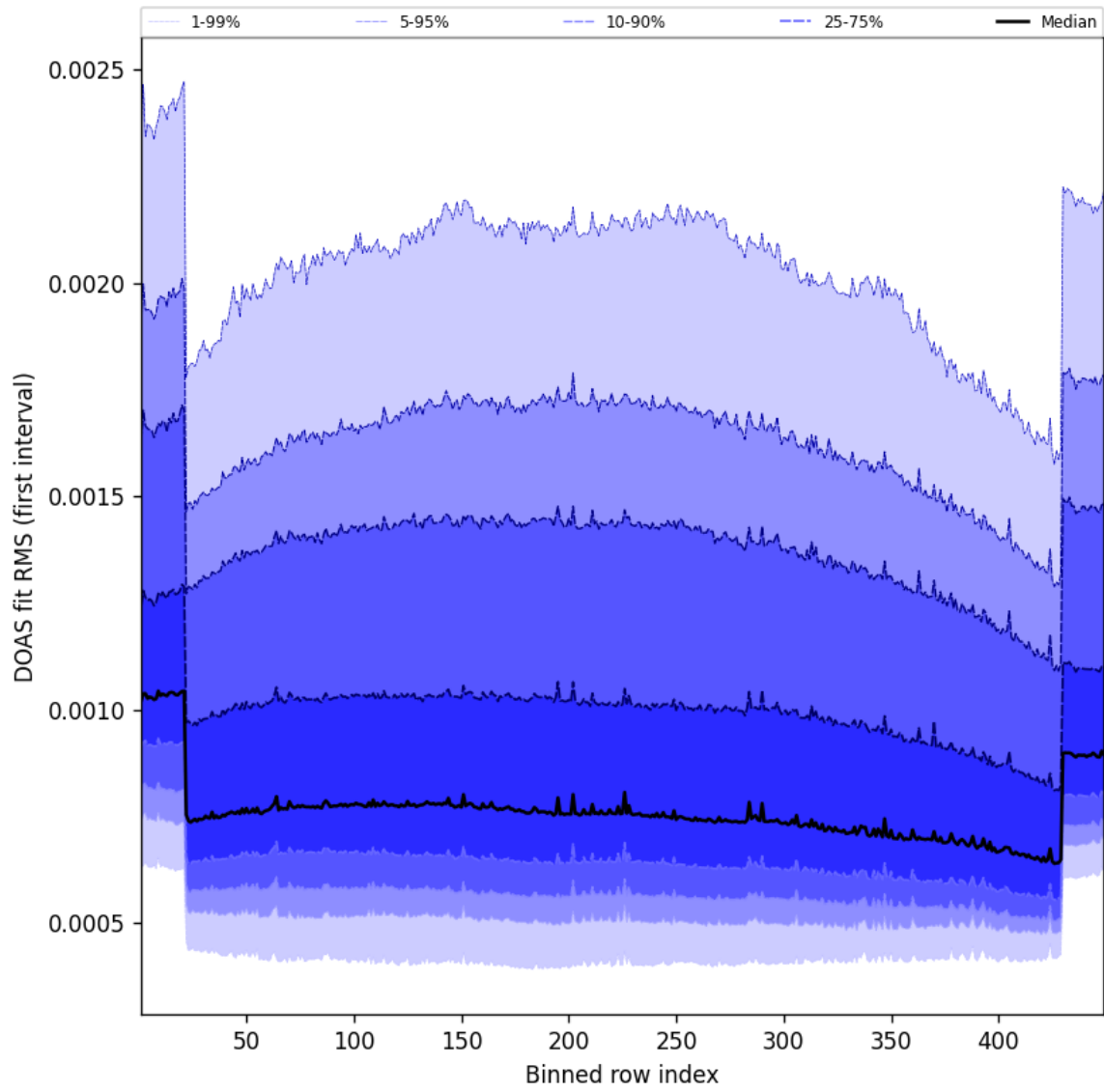
Figure 58: Along track statistics of “DOAS fit RMS (first interval)” for 2025-04-30 to 2025-05-01
