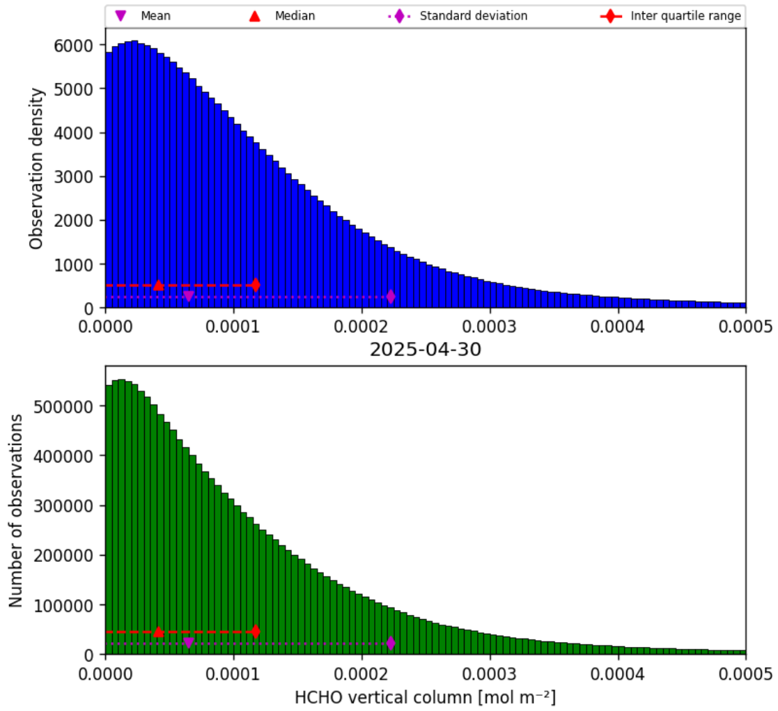
Figure 33: Histogram of “HCHO vertical column” for 2025-04-30 to 2025-05-01
