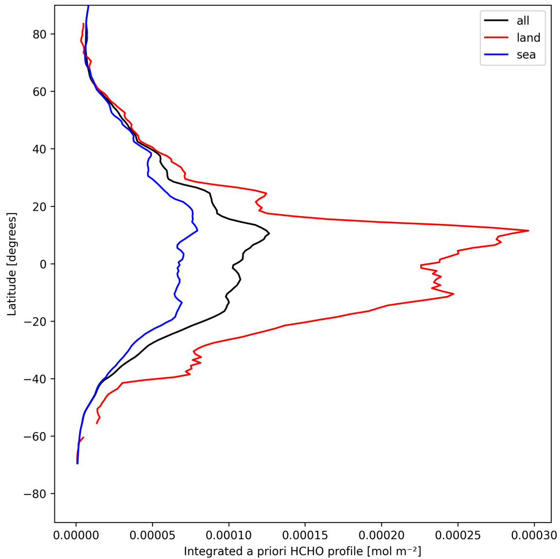
Figure 27: Zonal average of “Integrated a priori HCHO profile” for 2025-04-30 to 2025-05-01.
