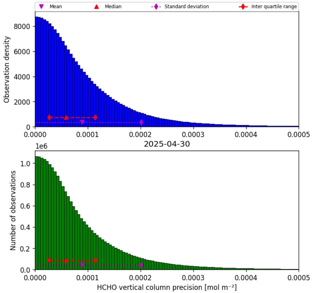
Figure 34: Histogram of “HCHO vertical column precision” for 2025-04-30 to 2025-05-01
