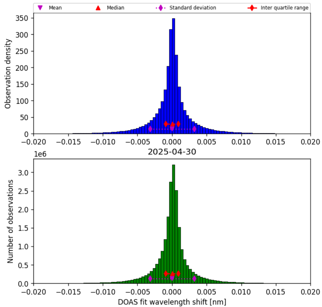
Figure 42: Histogram of “DOAS fit wavelength shift” for 2025-04-30 to 2025-05-01
