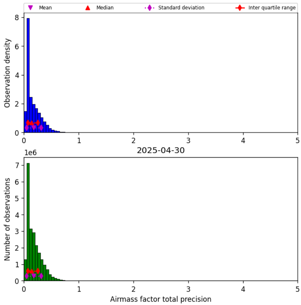
Figure 39: Histogram of “Airmass factor total precision” for 2025-04-30 to 2025-05-01
