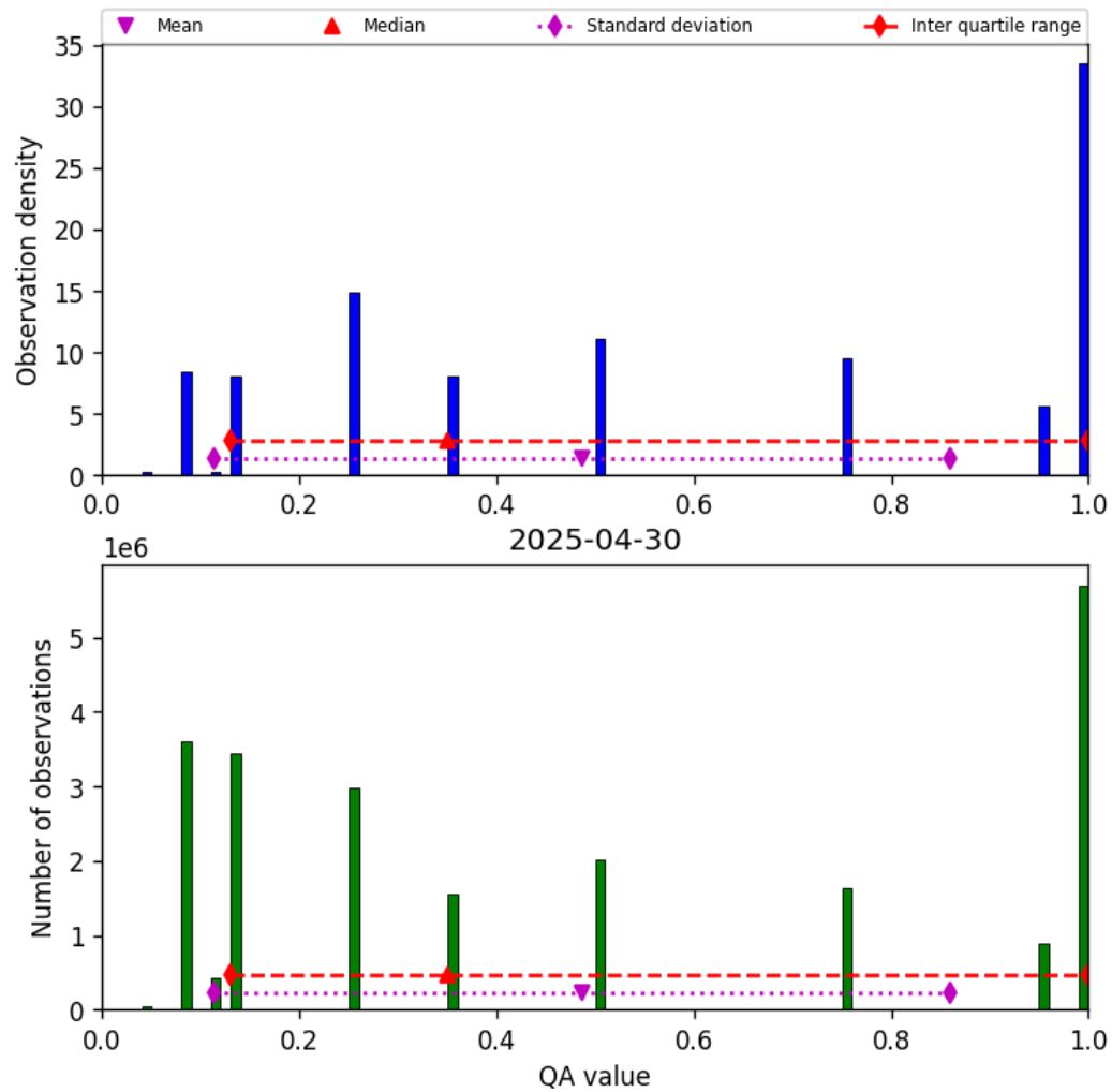
Figure 32: Histogram of “QA value” for 2025-04-30 to 2025-05-01
