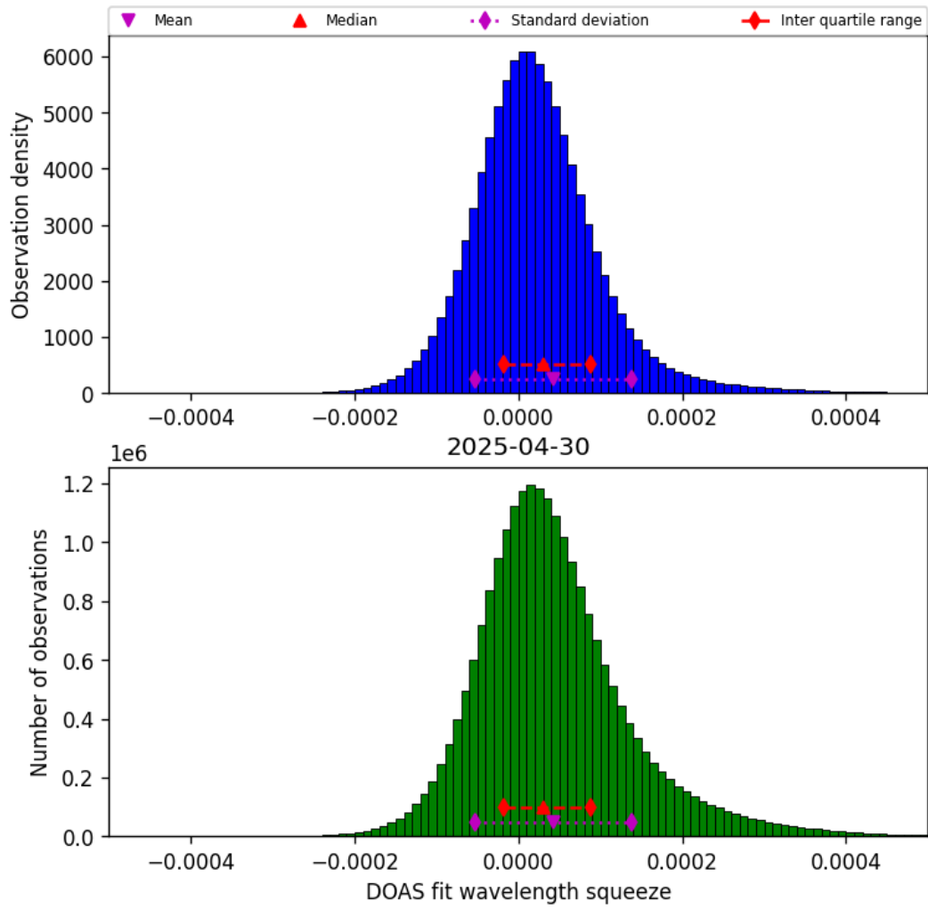
Figure 43: Histogram of “DOAS fit wavelength squeeze” for 2025-04-30 to 2025-05-01
