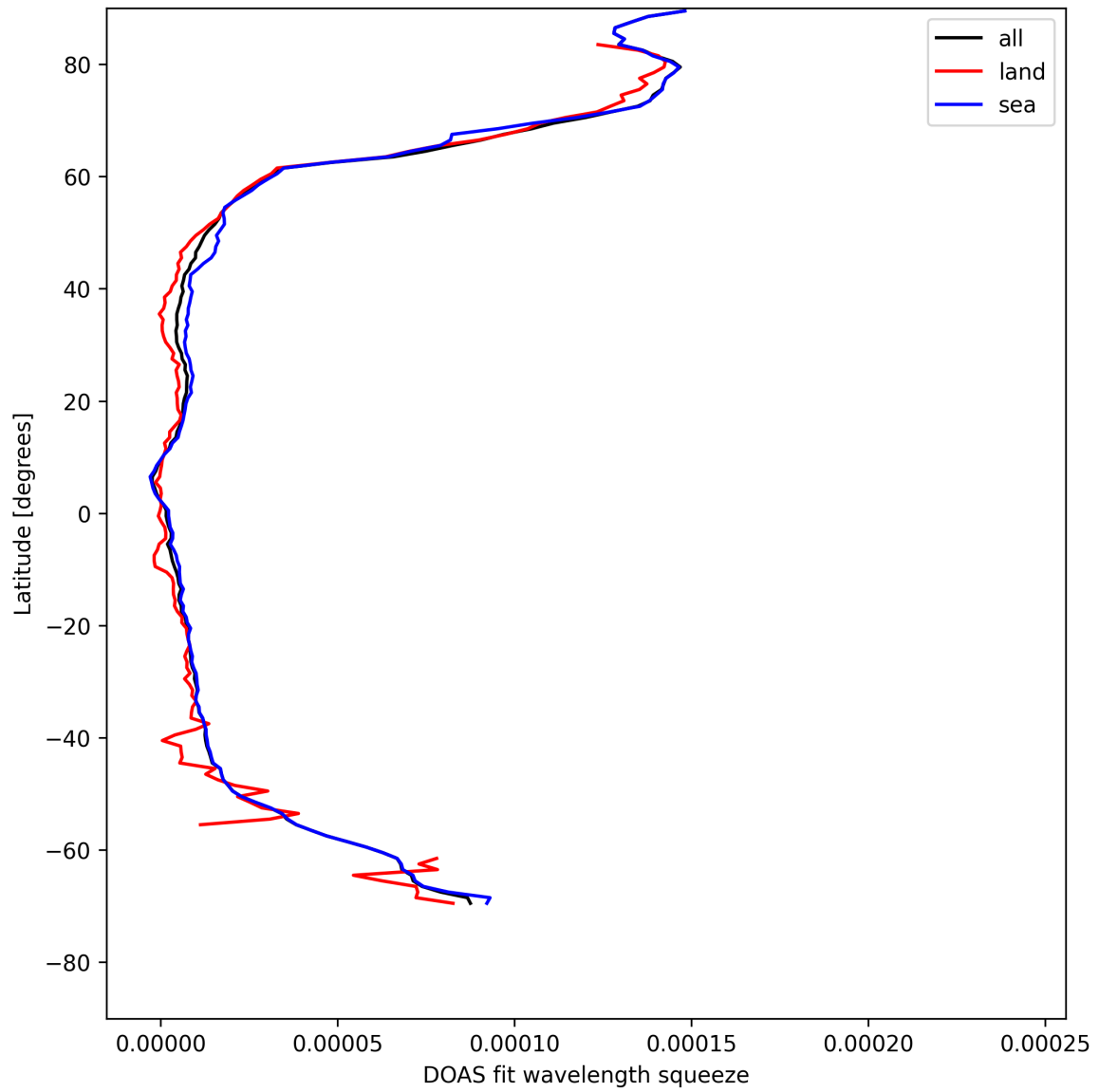
Figure 29: Zonal average of “DOAS fit wavelength squeeze” for 2025-05-01 to 2025-05-02.
