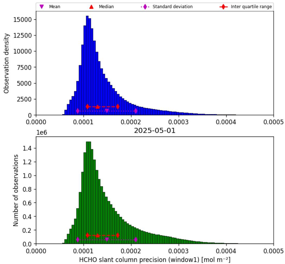
Figure 37: Histogram of “HCHO slant column precision (window1)” for 2025-05-01 to 2025-05-02
