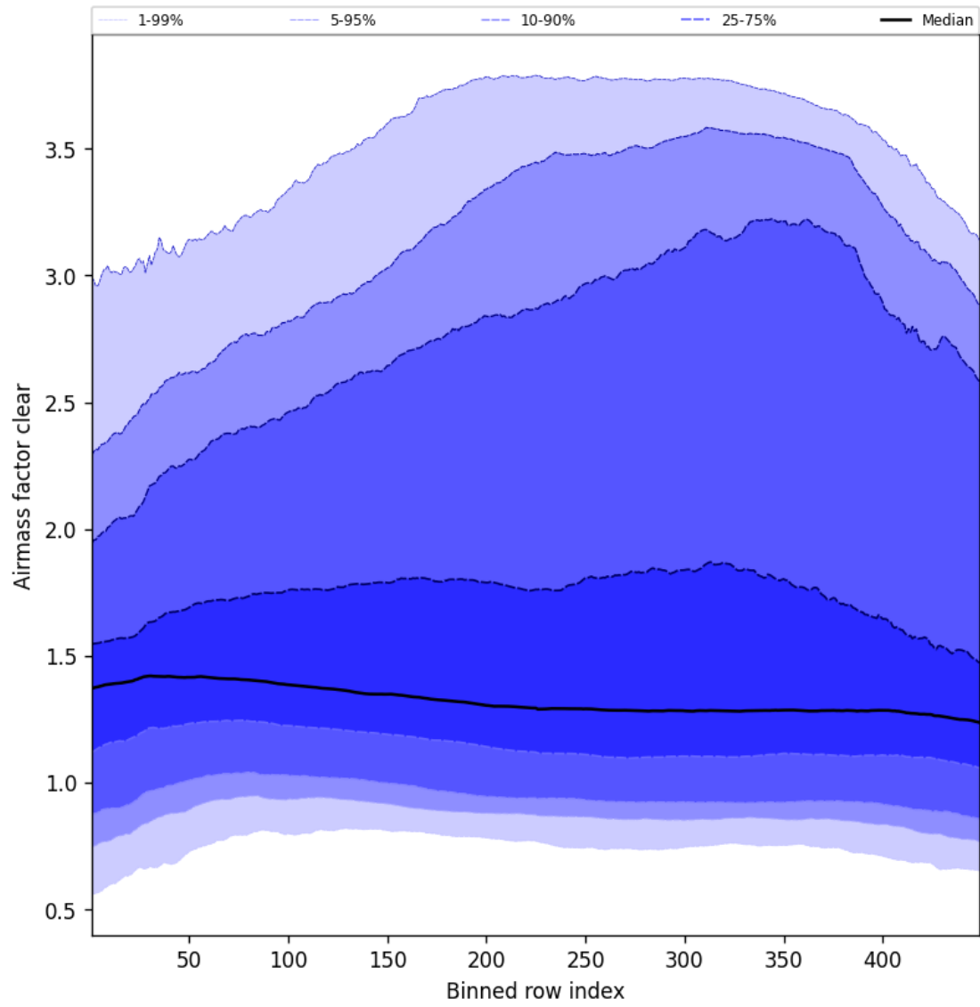
Figure 54: Along track statistics of “Airmass factor clear” for 2025-05-01 to 2025-05-02
