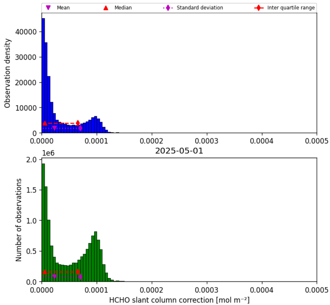
Figure 45: Histogram of “HCHO slant column correction” for 2025-05-01 to 2025-05-02
