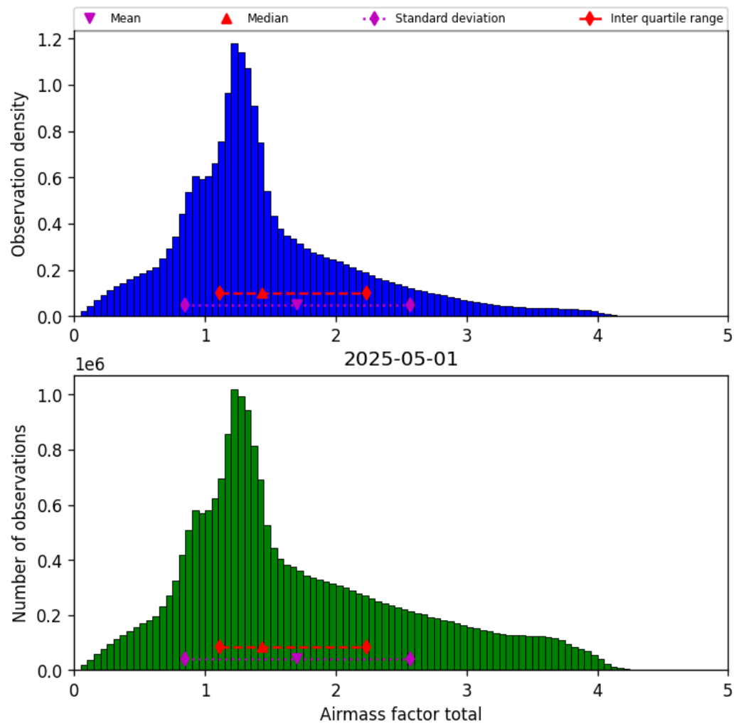
Figure 38: Histogram of “Airmass factor total” for 2025-05-01 to 2025-05-02
