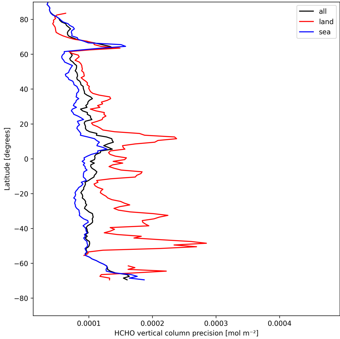
Figure 20: Zonal average of “HCHO vertical column precision” for 2025-05-01 to 2025-05-02.
