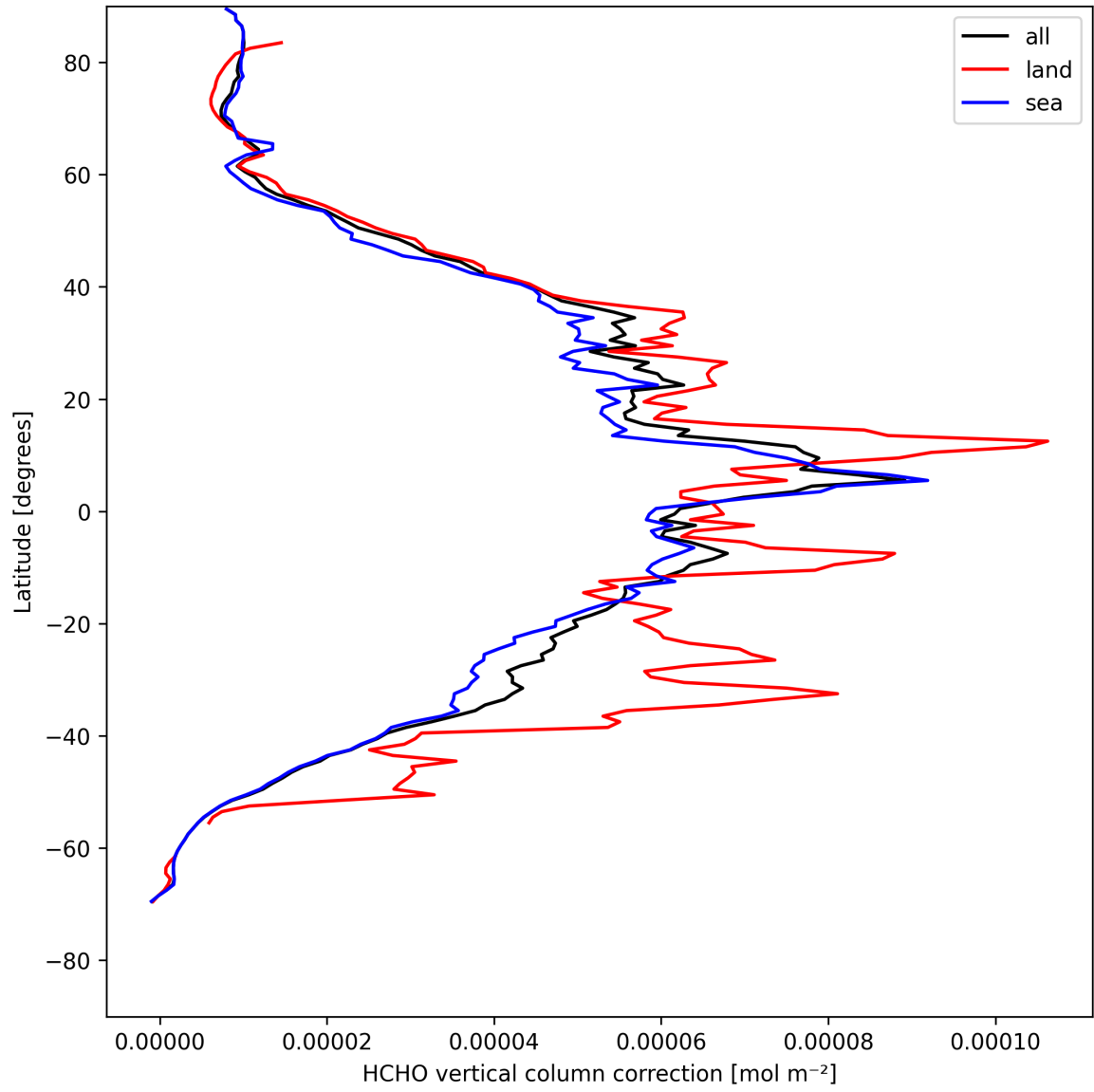
Figure 21: Zonal average of “HCHO vertical column correction” for 2025-05-01 to 2025-05-02.
