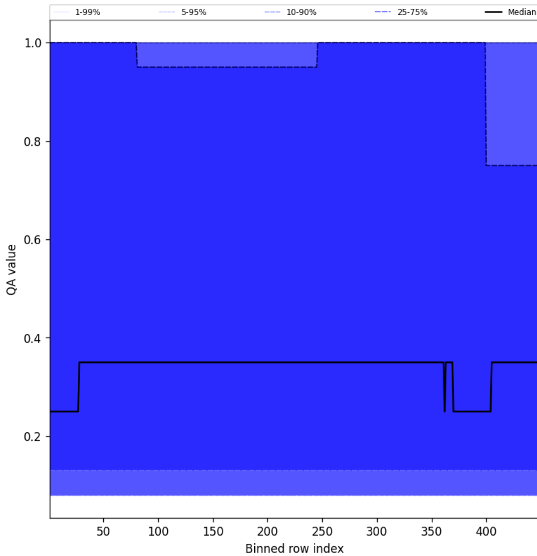
Figure 46: Along track statistics of “QA value” for 2025-05-01 to 2025-05-02
