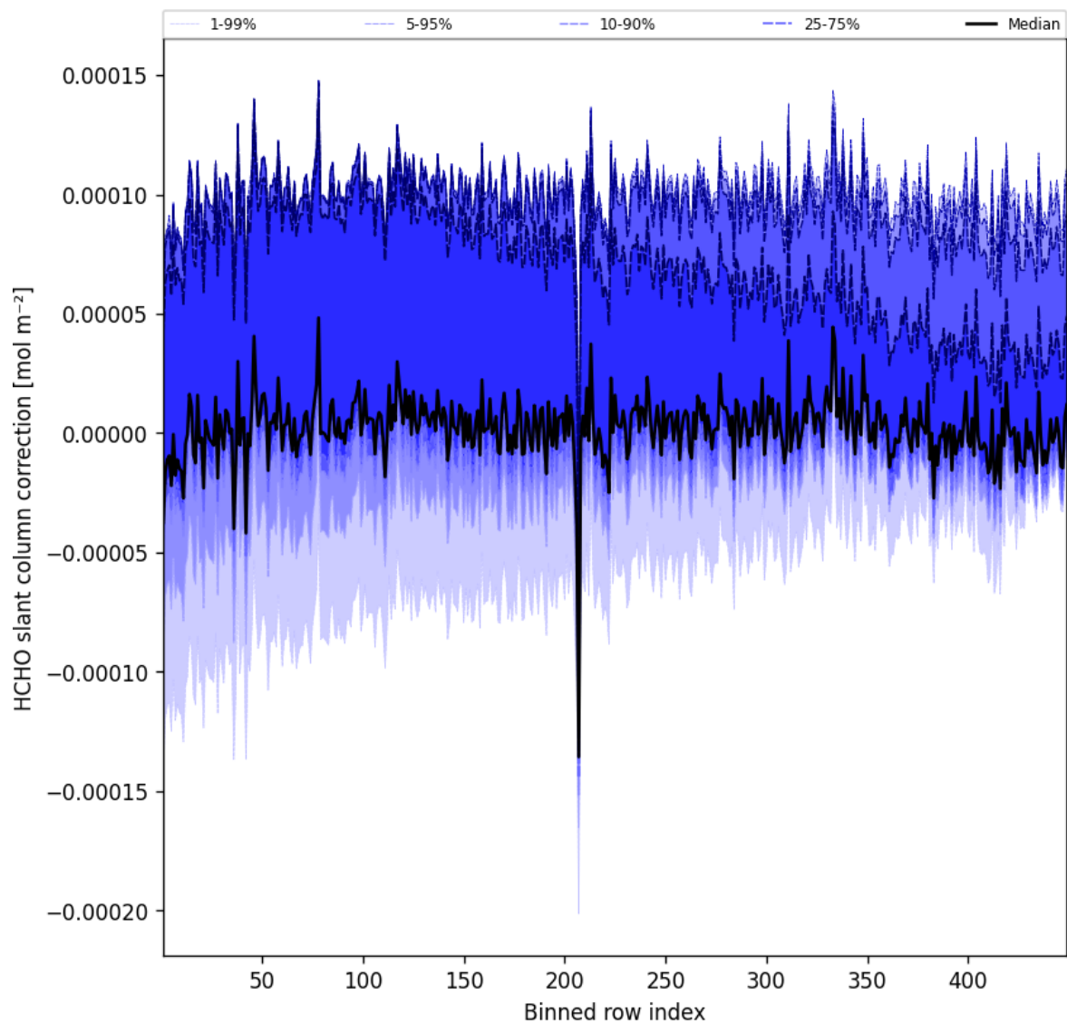
Figure 59: Along track statistics of “HCHO slant column correction” for 2025-05-01 to 2025-05-02
