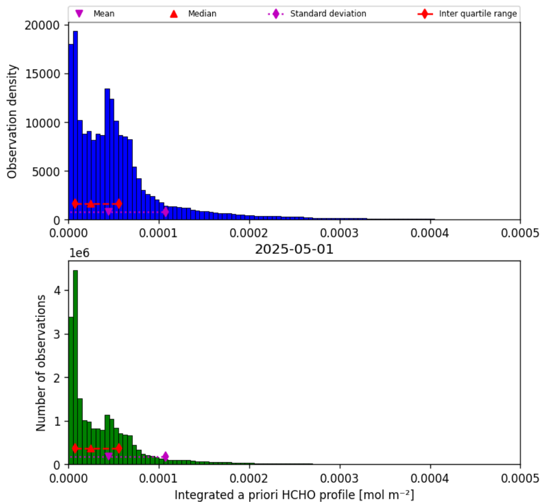
Figure 41: Histogram of “Integrated a priori HCHO profile” for 2025-05-01 to 2025-05-02
