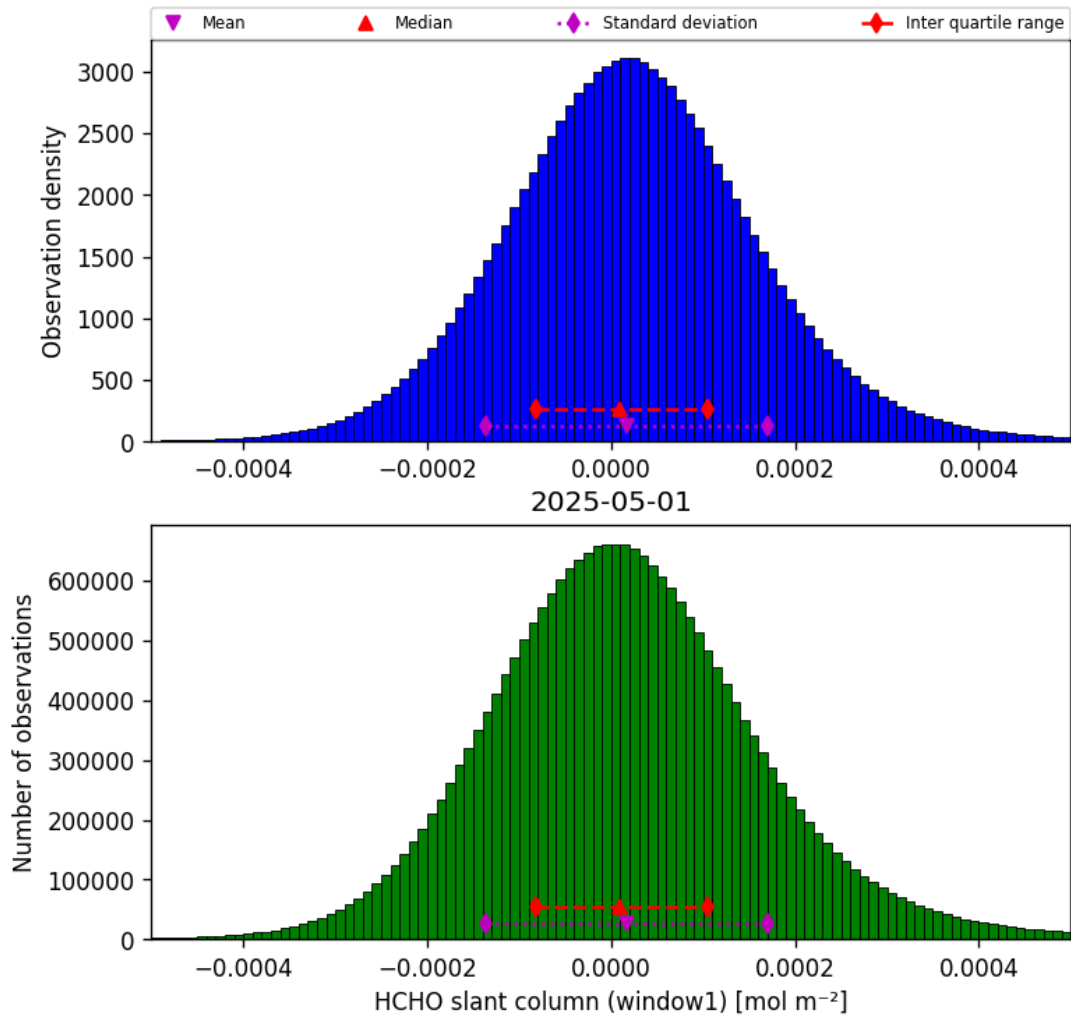
Figure 36: Histogram of “HCHO slant column (window1)” for 2025-05-01 to 2025-05-02
