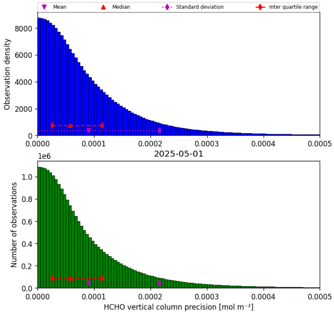
Figure 34: Histogram of “HCHO vertical column precision” for 2025-05-01 to 2025-05-02
