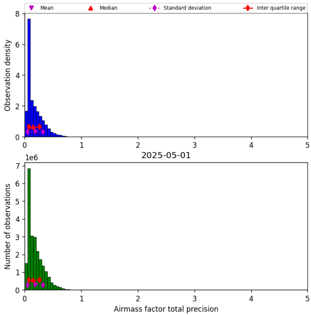
Figure 39: Histogram of “Airmass factor total precision” for 2025-05-01 to 2025-05-02
