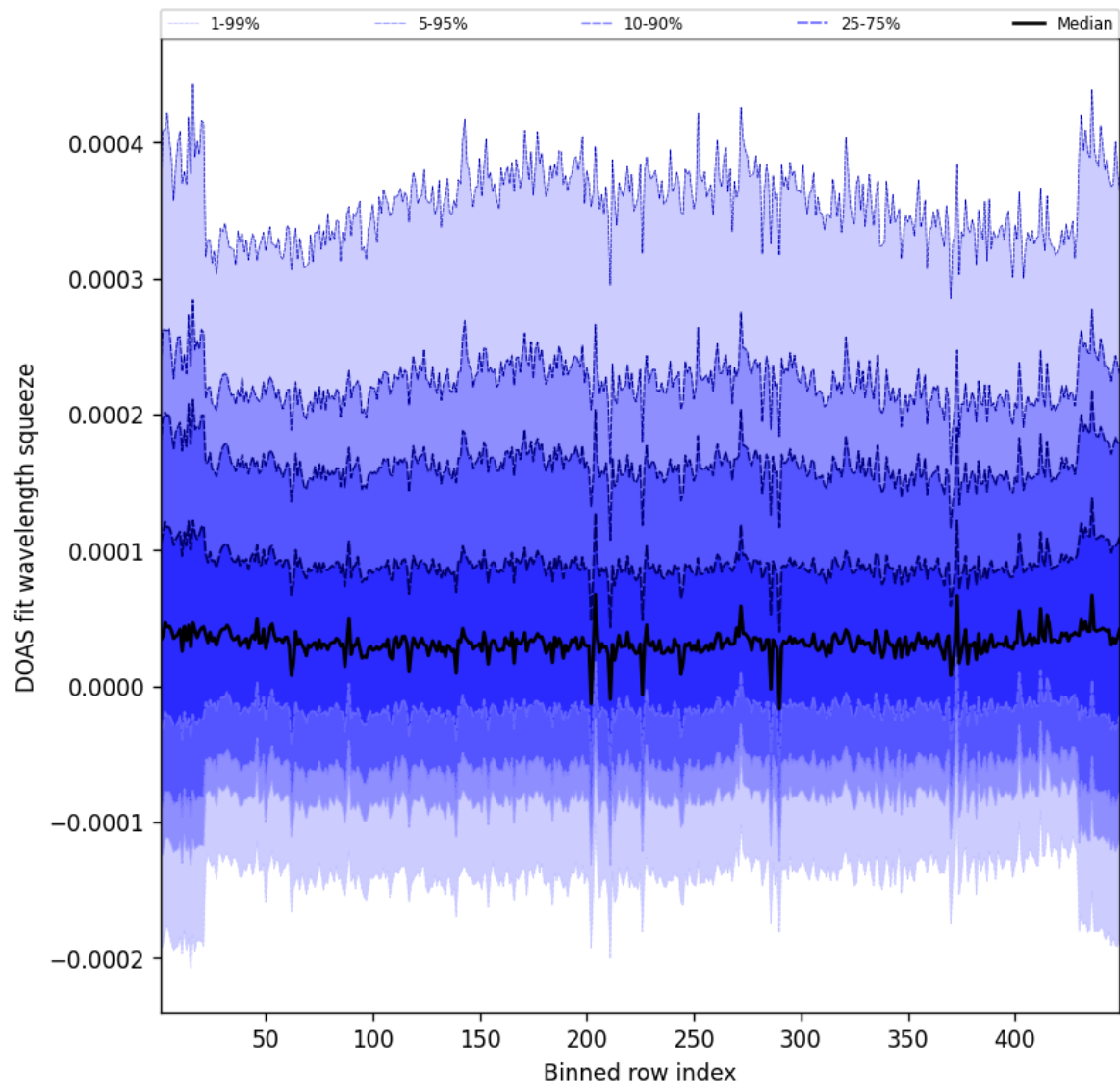
Figure 57: Along track statistics of “DOAS fit wavelength squeeze” for 2025-05-01 to 2025-05-02
