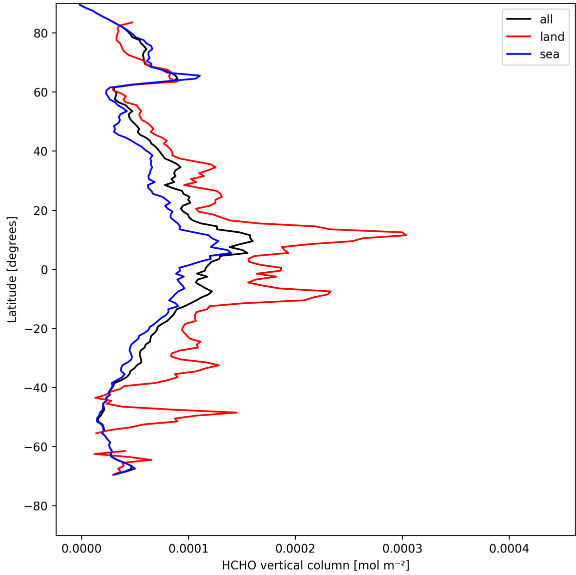
Figure 19: Zonal average of “HCHO vertical column” for 2025-05-01 to 2025-05-02.
