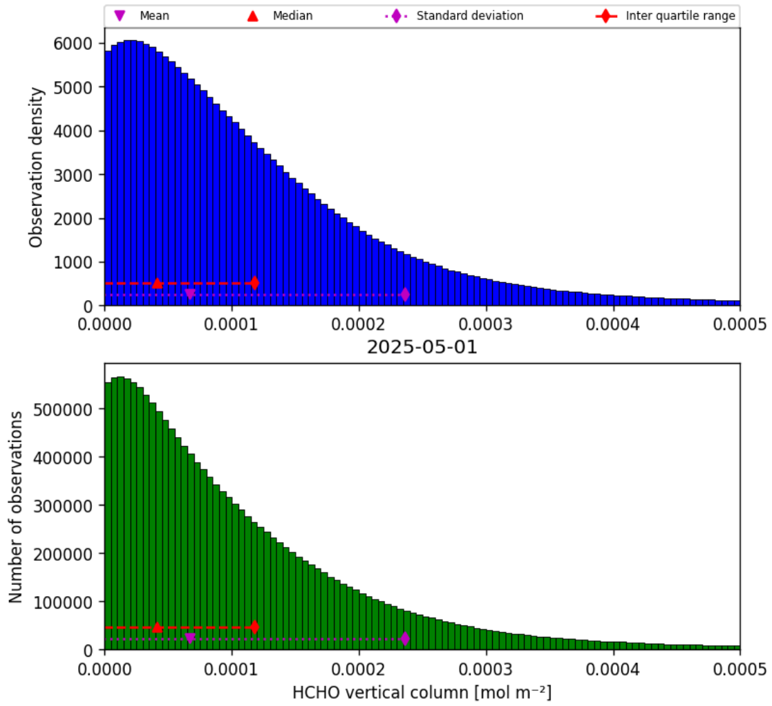
Figure 33: Histogram of “HCHO vertical column” for 2025-05-01 to 2025-05-02
