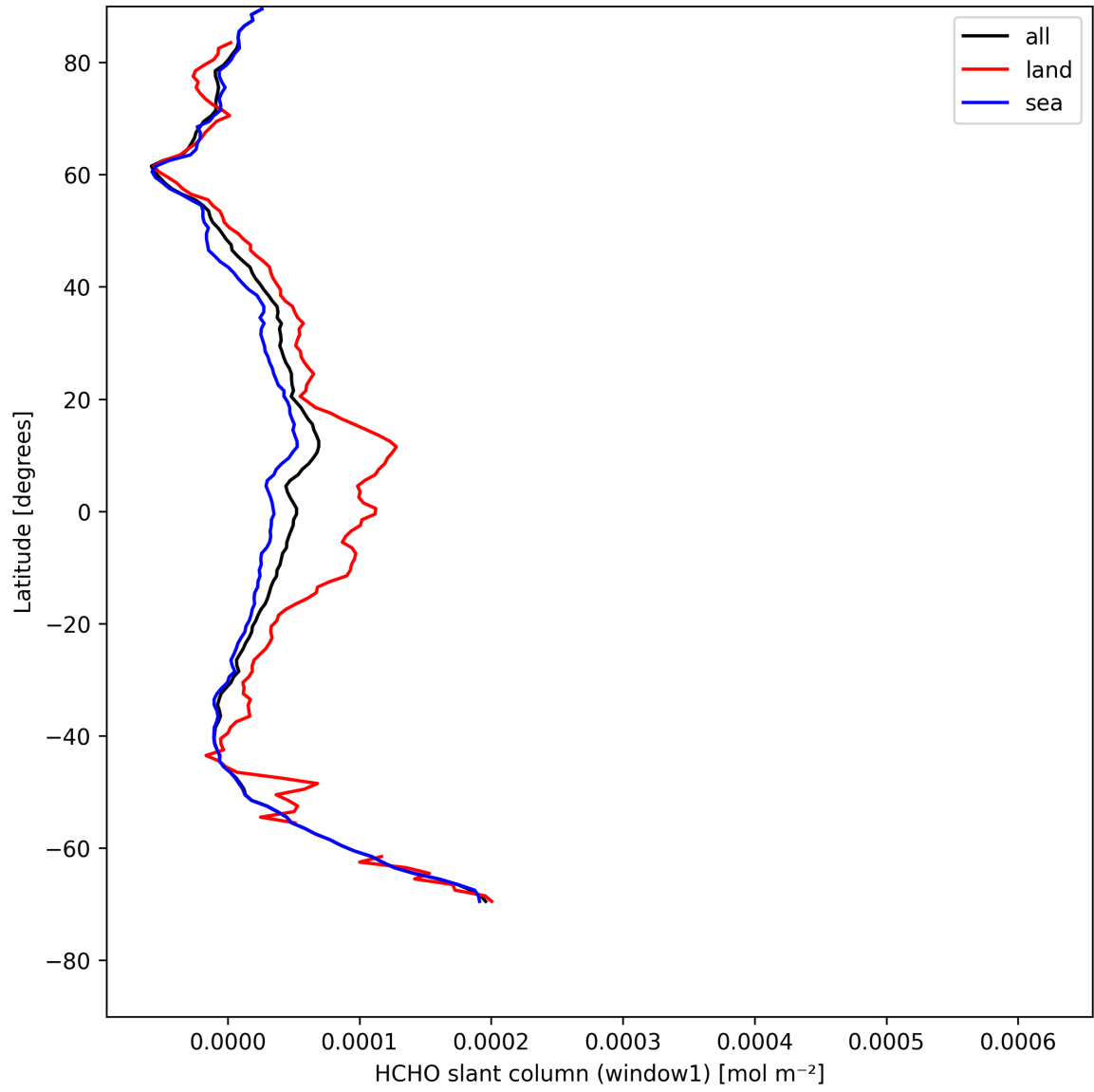
Figure 22: Zonal average of “HCHO slant column (window1)” for 2025-05-01 to 2025-05-02.
