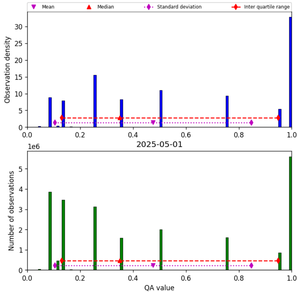
Figure 32: Histogram of “QA value” for 2025-05-01 to 2025-05-02
