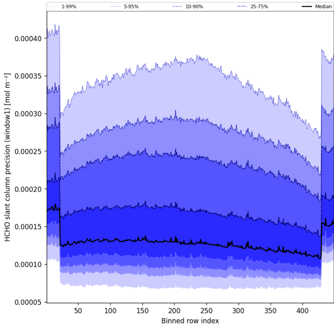
Figure 51: Along track statistics of “HCHO slant column precision (window1)” for 2025-05-01 to 2025-05-02
