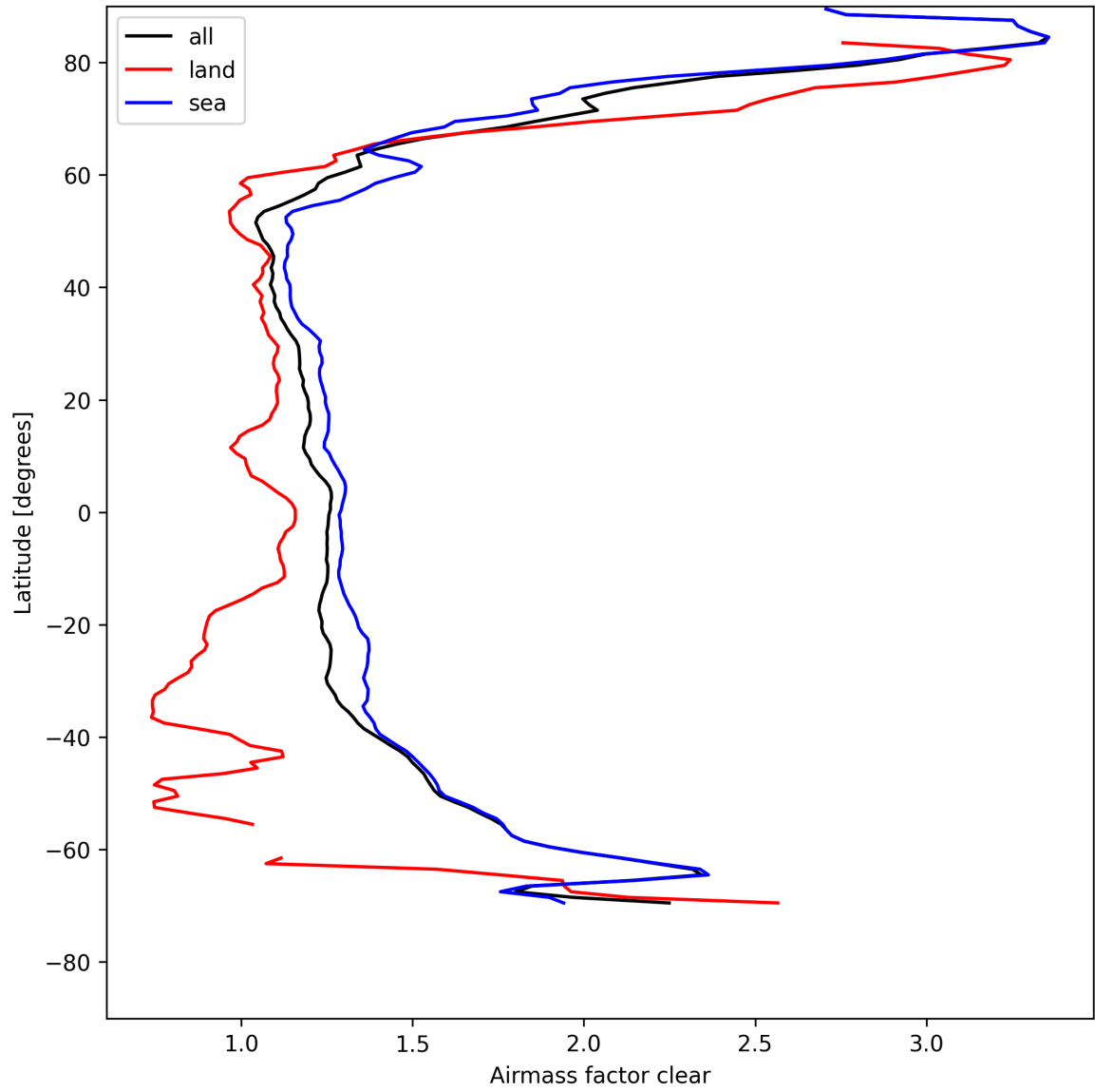
Figure 26: Zonal average of “Airmass factor clear” for 2025-05-01 to 2025-05-02.
