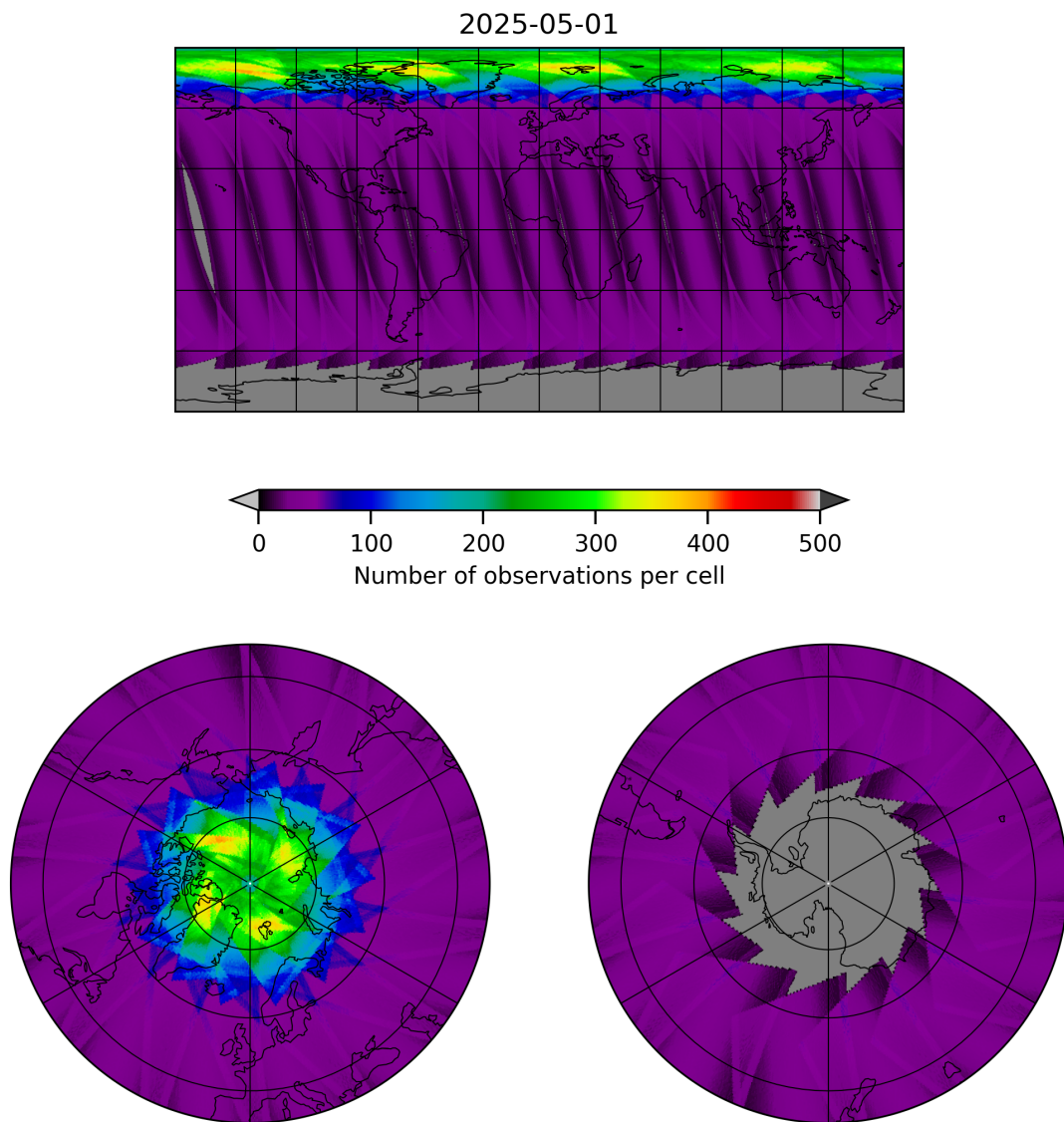
Figure 17: Map of the number of observations for 2025-05-01 to 2025-05-02
