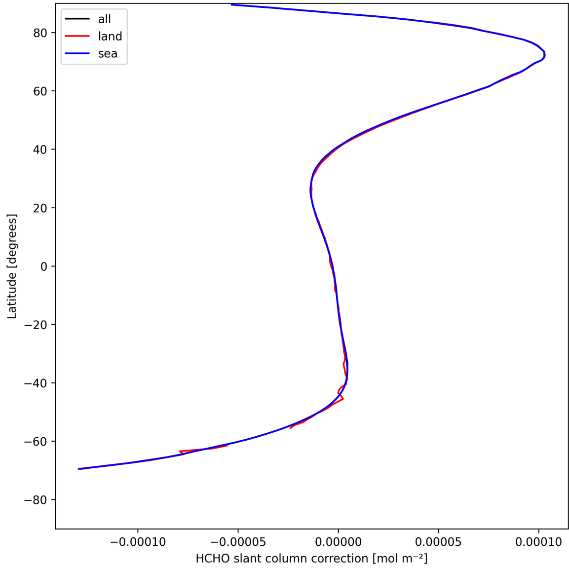
Figure 31: Zonal average of “HCHO slant column correction” for 2025-05-01 to 2025-05-02.
