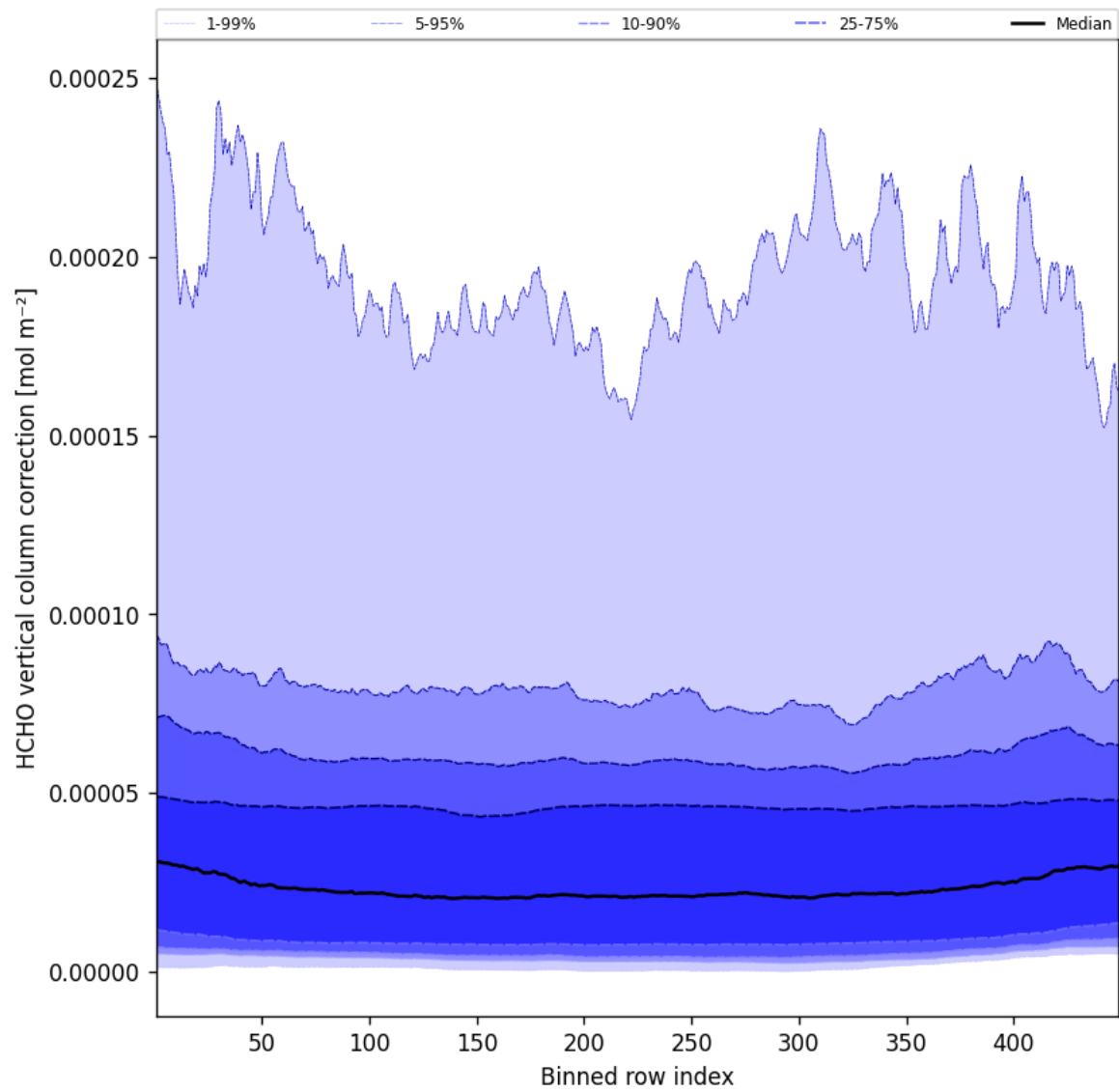
Figure 49: Along track statistics of “HCHO vertical column correction” for 2025-05-01 to 2025-05-02
