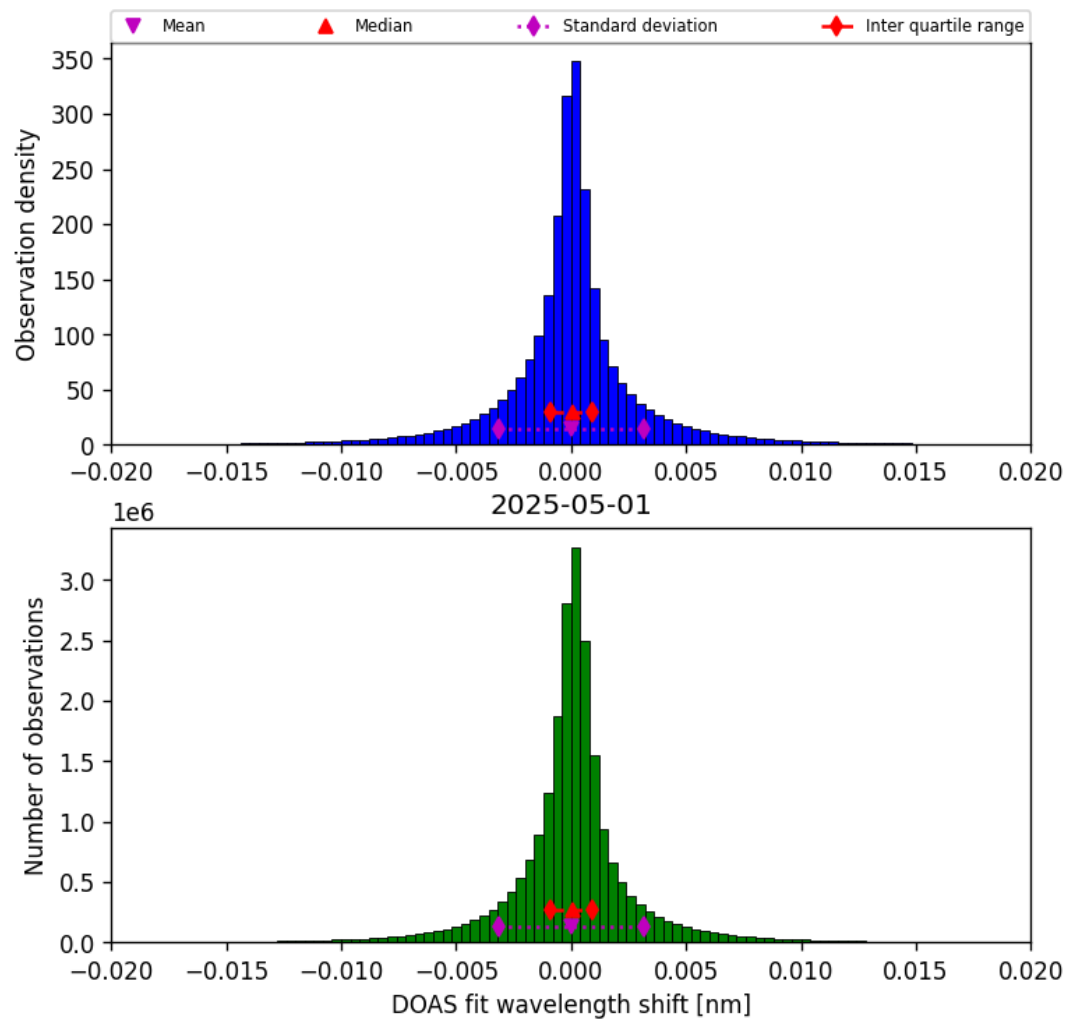
Figure 42: Histogram of “DOAS fit wavelength shift” for 2025-05-01 to 2025-05-02
