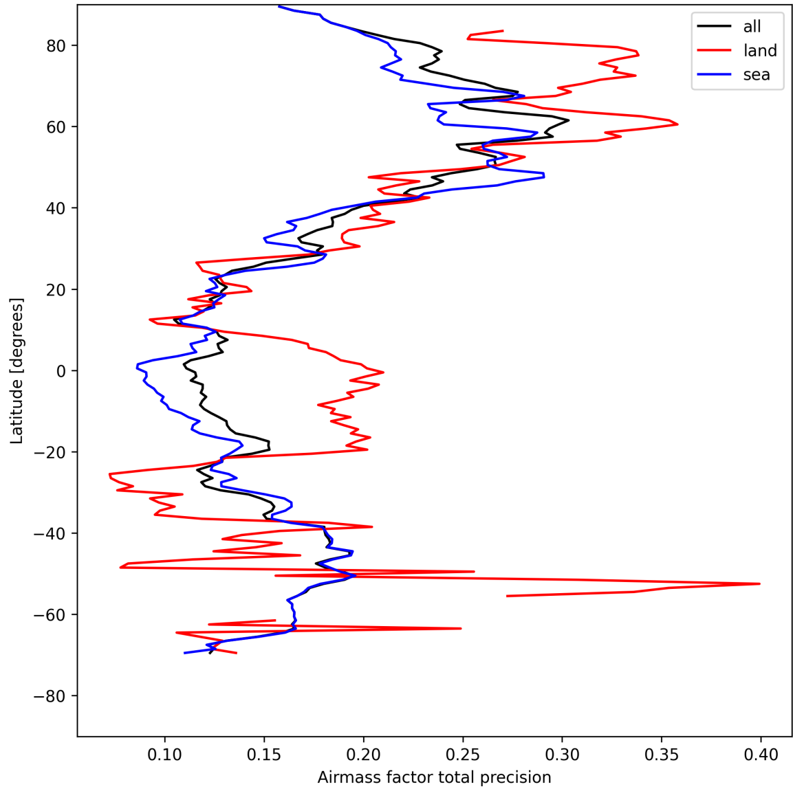
Figure 25: Zonal average of “Airmass factor total precision” for 2025-05-01 to 2025-05-02.
