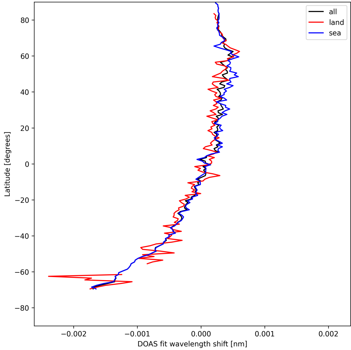
Figure 28: Zonal average of “DOAS fit wavelength shift” for 2025-05-01 to 2025-05-02.
