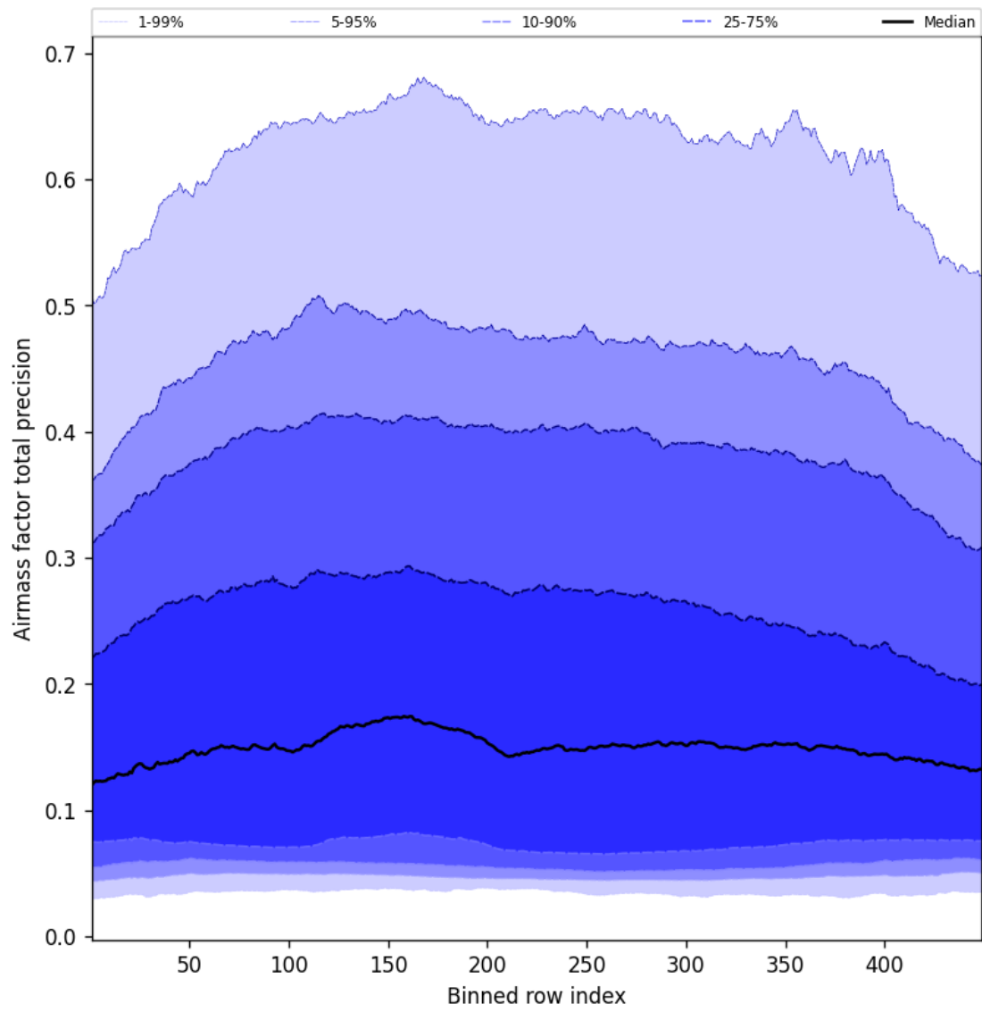
Figure 53: Along track statistics of “Airmass factor total precision” for 2025-05-01 to 2025-05-02
