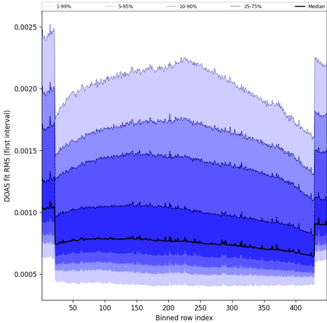
Figure 58: Along track statistics of “DOAS fit RMS (first interval)” for 2025-05-01 to 2025-05-02
