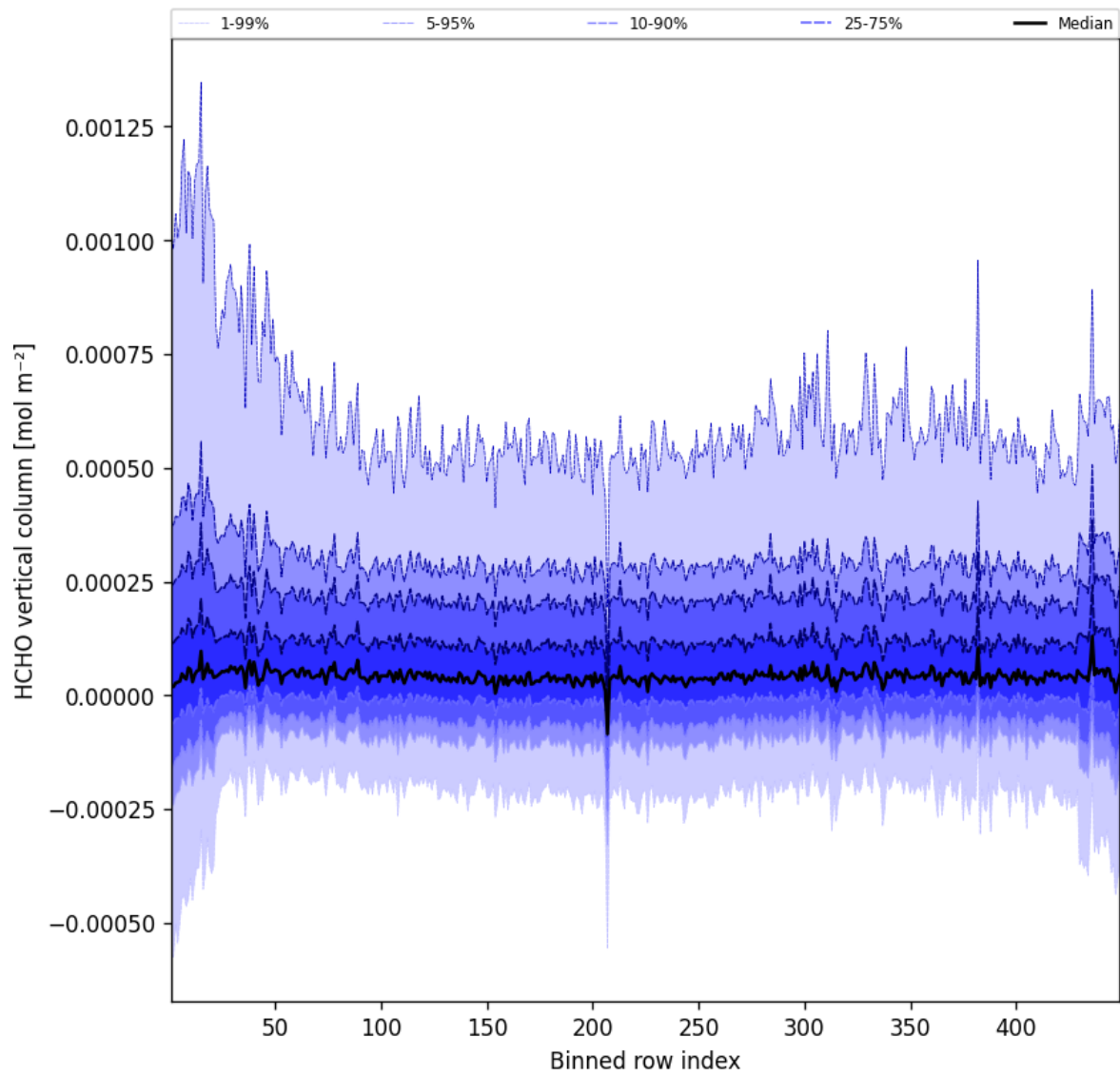
Figure 47: Along track statistics of “HCHO vertical column” for 2025-05-01 to 2025-05-02
