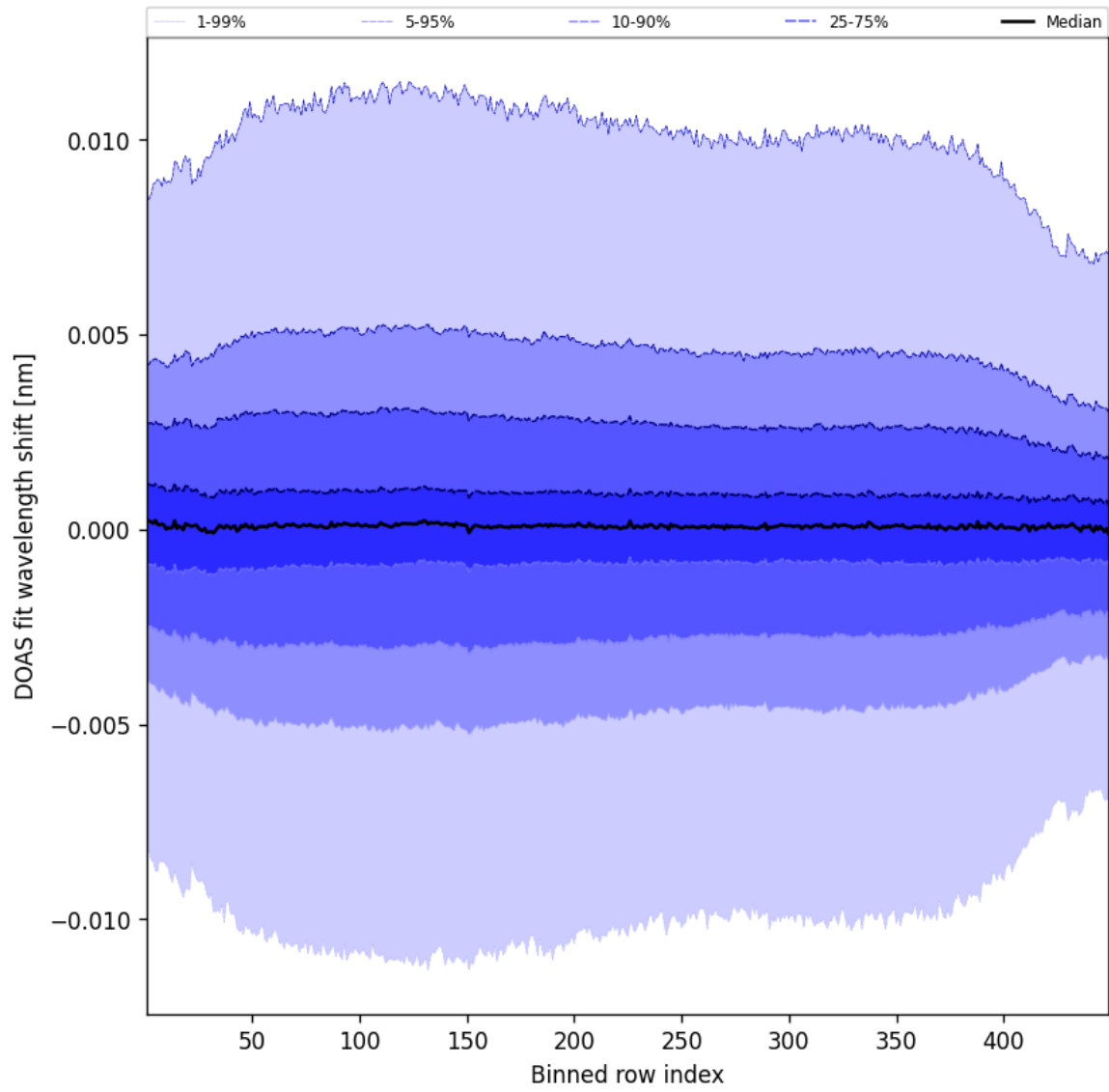
Figure 56: Along track statistics of “DOAS fit wavelength shift” for 2025-05-01 to 2025-05-02
