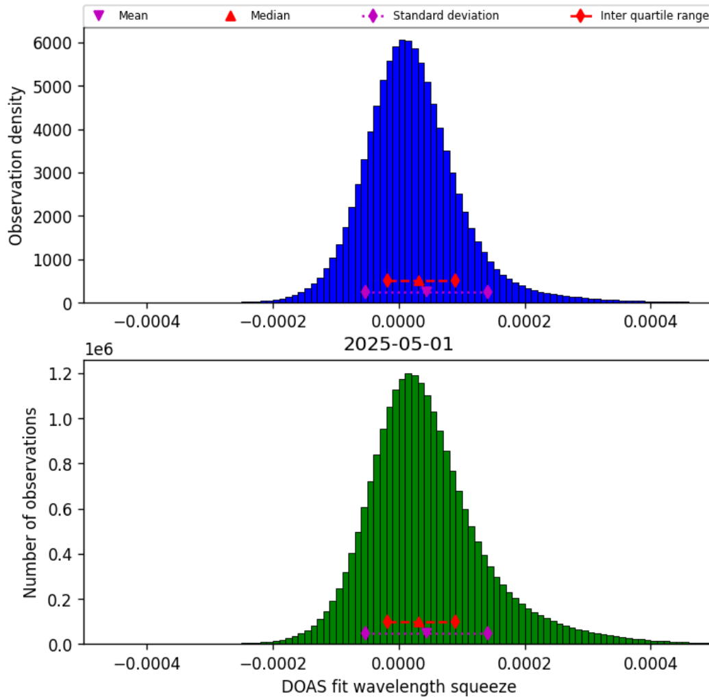
Figure 43: Histogram of “DOAS fit wavelength squeeze” for 2025-05-01 to 2025-05-02
