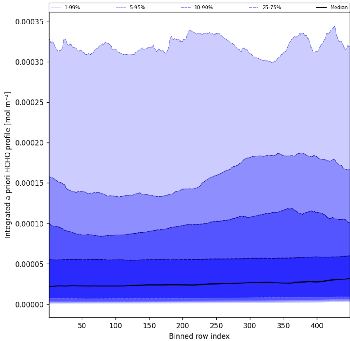
Figure 55: Along track statistics of “Integrated a priori HCHO profile” for 2025-05-01 to 2025-05-02
