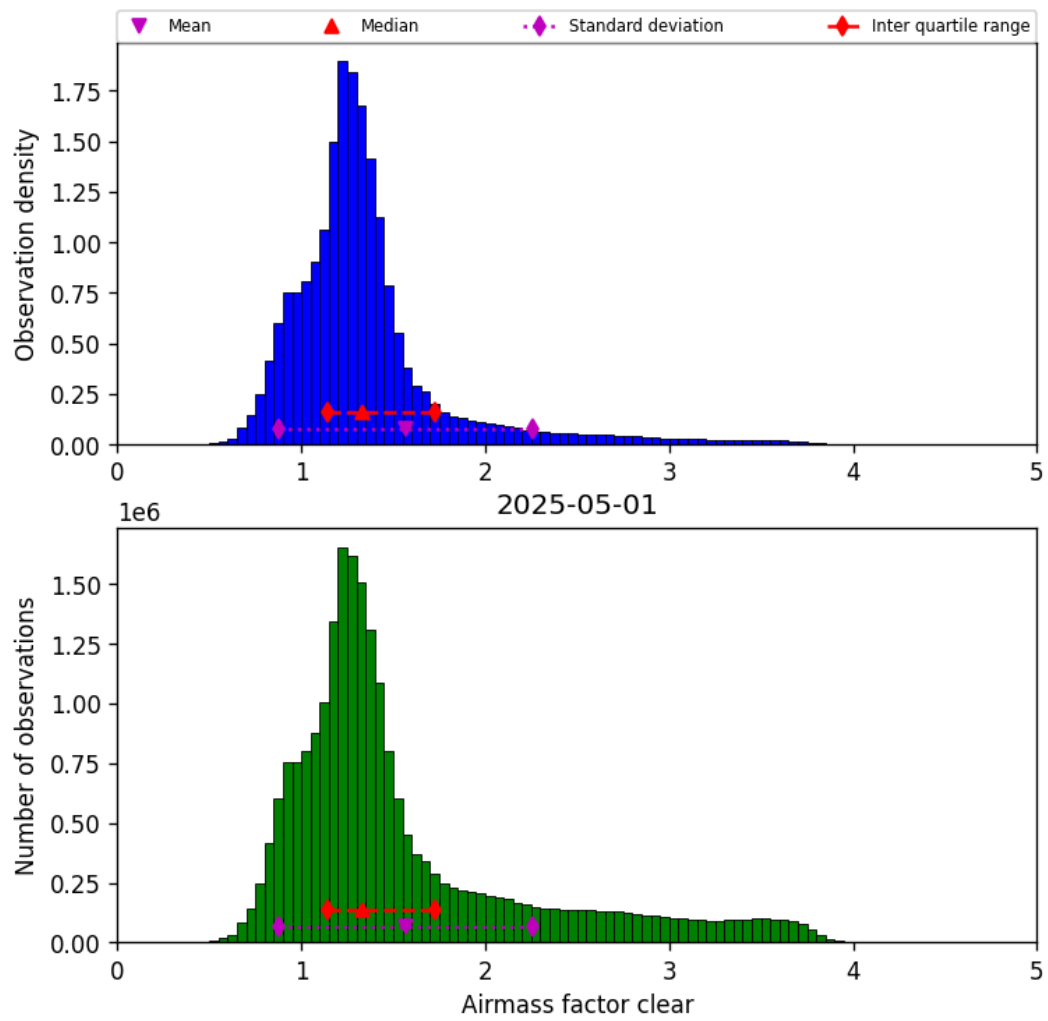
Figure 40: Histogram of “Airmass factor clear” for 2025-05-01 to 2025-05-02
