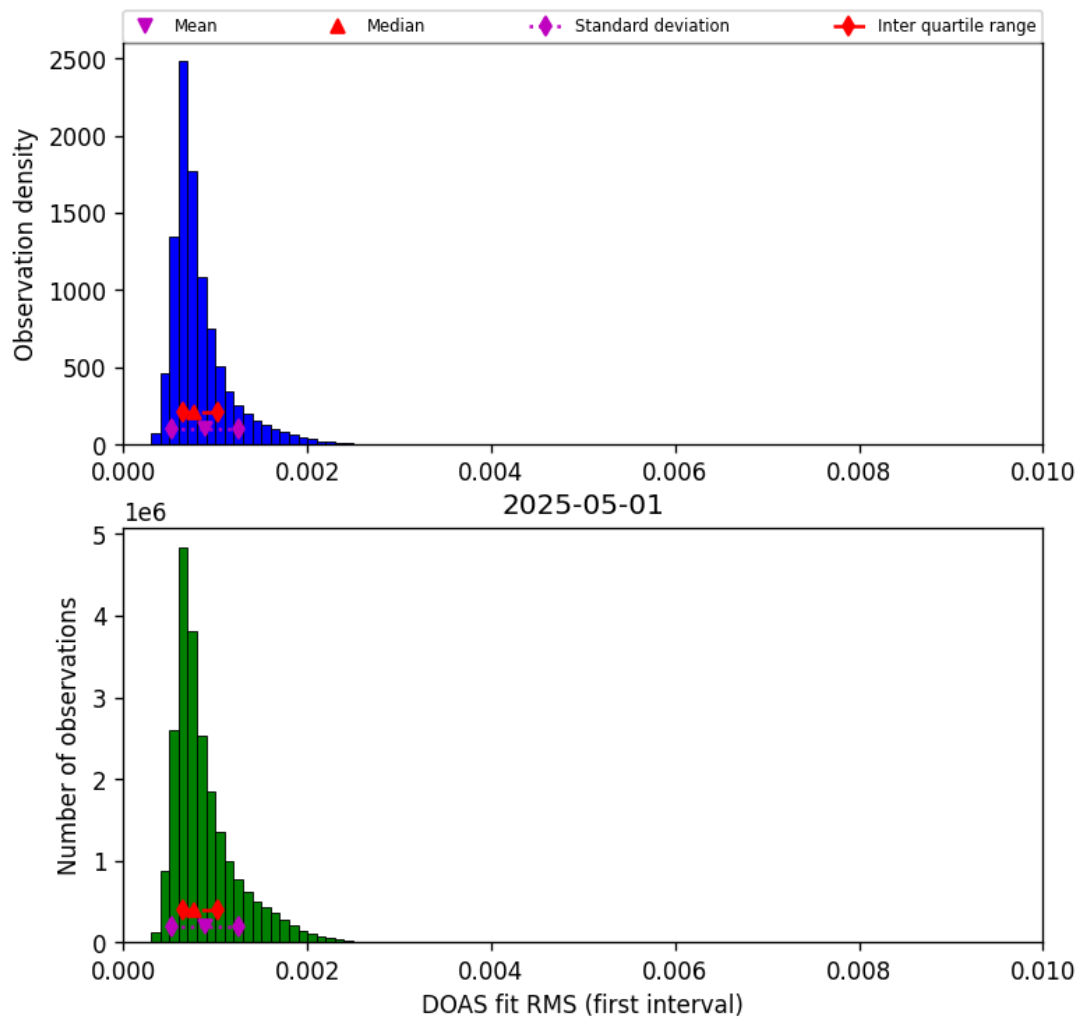
Figure 44: Histogram of “DOAS fit RMS (first interval)” for 2025-05-01 to 2025-05-02
