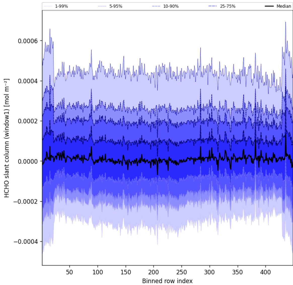
Figure 50: Along track statistics of “HCHO slant column (window1)” for 2025-05-01 to 2025-05-02
