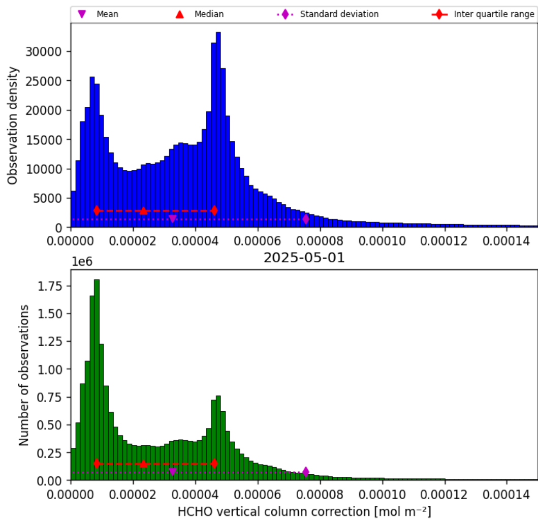
Figure 35: Histogram of “HCHO vertical column correction” for 2025-05-01 to 2025-05-02
