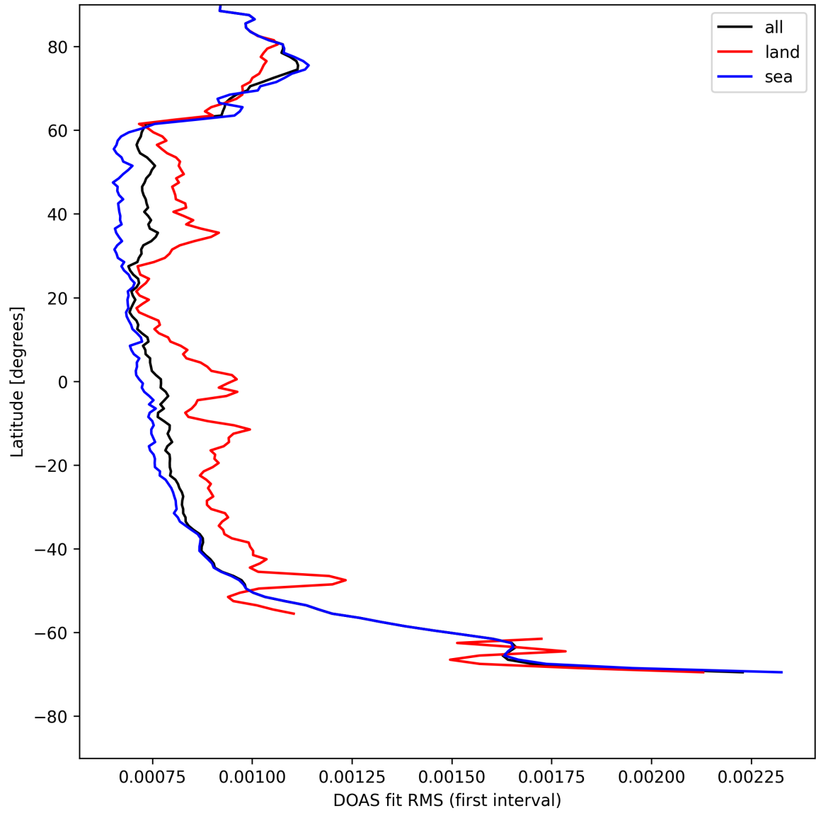
Figure 30: Zonal average of “DOAS fit RMS (first interval)” for 2025-05-01 to 2025-05-02.
