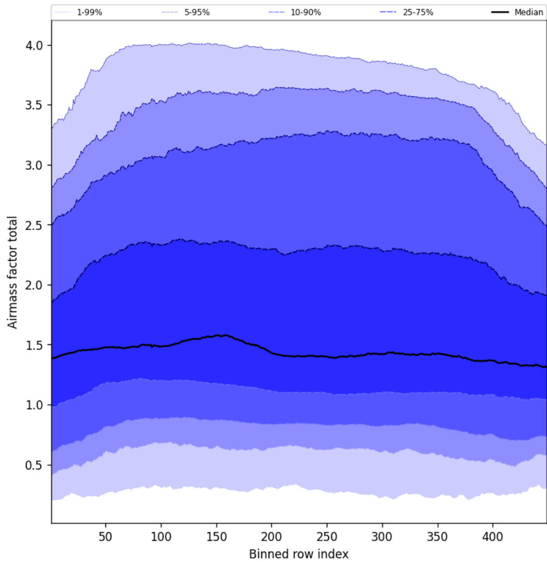
Figure 52: Along track statistics of “Airmass factor total” for 2025-05-01 to 2025-05-02
