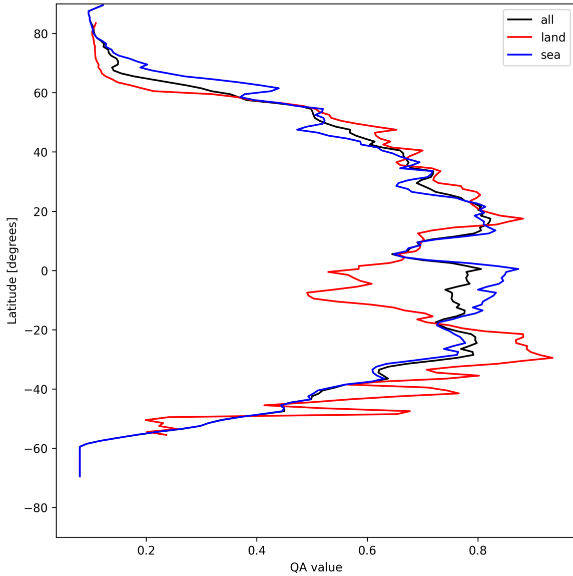
Figure 18: Zonal average of “QA value” for 2025-05-01 to 2025-05-02.
