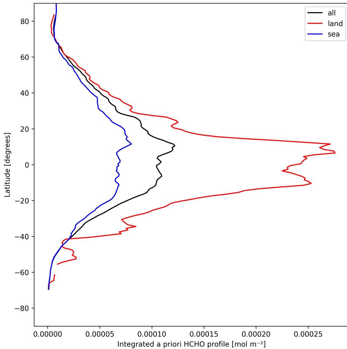
Figure 27: Zonal average of “Integrated a priori HCHO profile” for 2025-05-01 to 2025-05-02.
