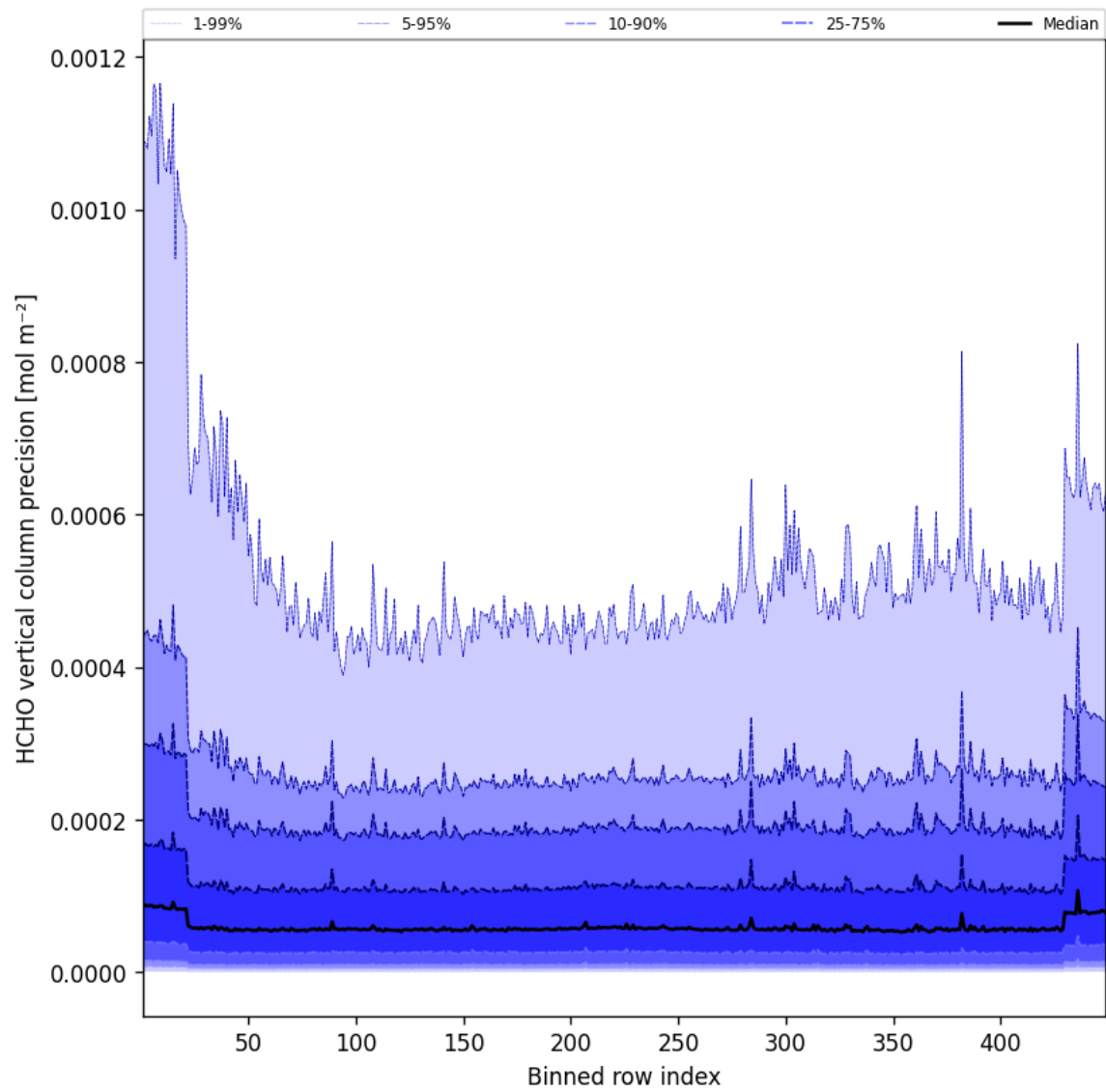
Figure 48: Along track statistics of “HCHO vertical column precision” for 2025-05-01 to 2025-05-02
