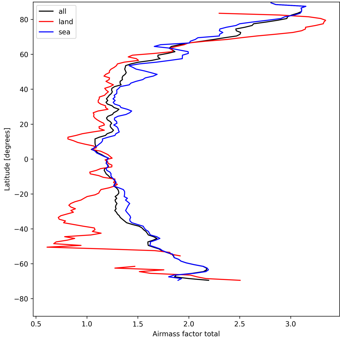
Figure 24: Zonal average of “Airmass factor total” for 2025-05-01 to 2025-05-02.
