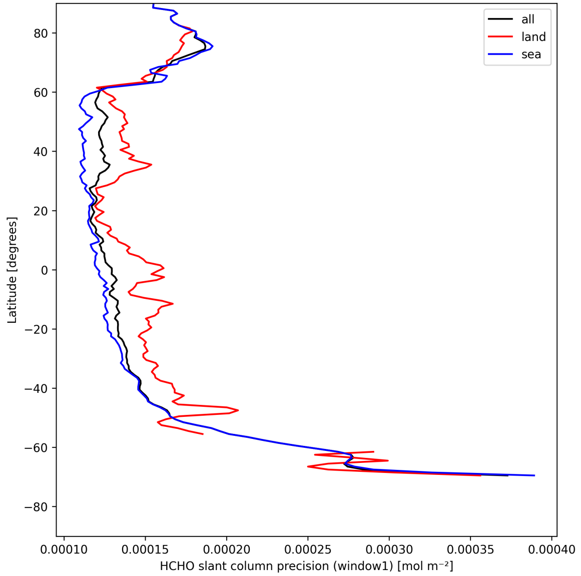
Figure 23: Zonal average of “HCHO slant column precision (window1)” for 2025-05-01 to 2025-05-02.
