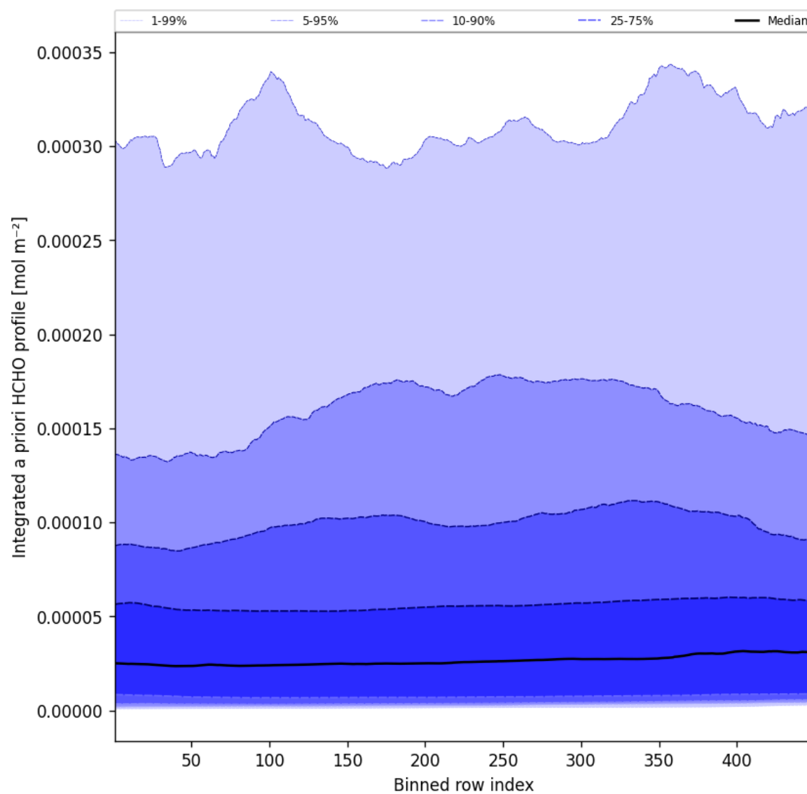
Figure 55: Along track statistics of “Integrated a priori HCHO profile” for 2025-05-02 to 2025-05-02
