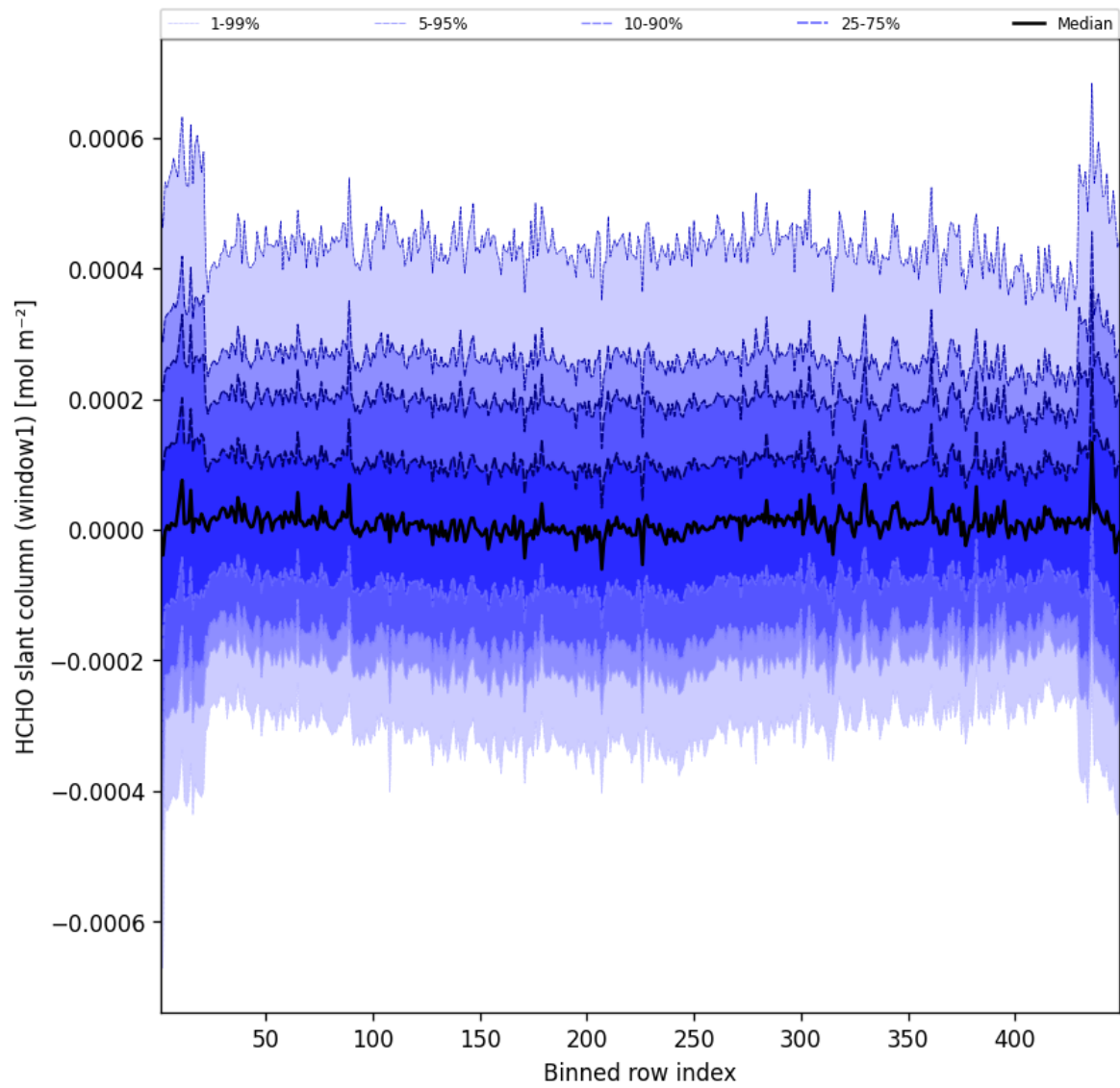
Figure 50: Along track statistics of “HCHO slant column (window1)” for 2025-05-02 to 2025-05-02
