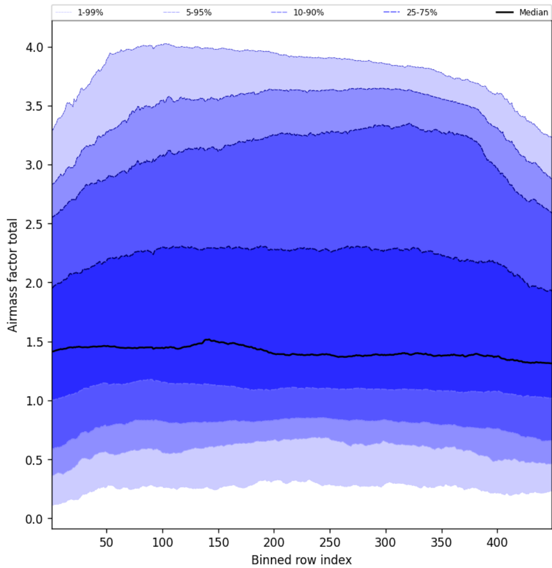
Figure 52: Along track statistics of “Airmass factor total” for 2025-05-02 to 2025-05-02
