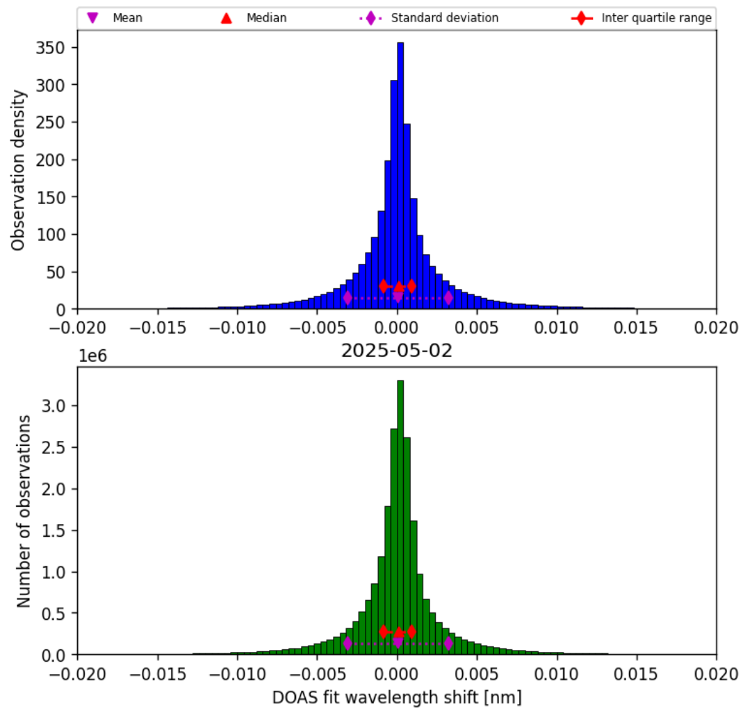
Figure 42: Histogram of “DOAS fit wavelength shift” for 2025-05-02 to 2025-05-02
