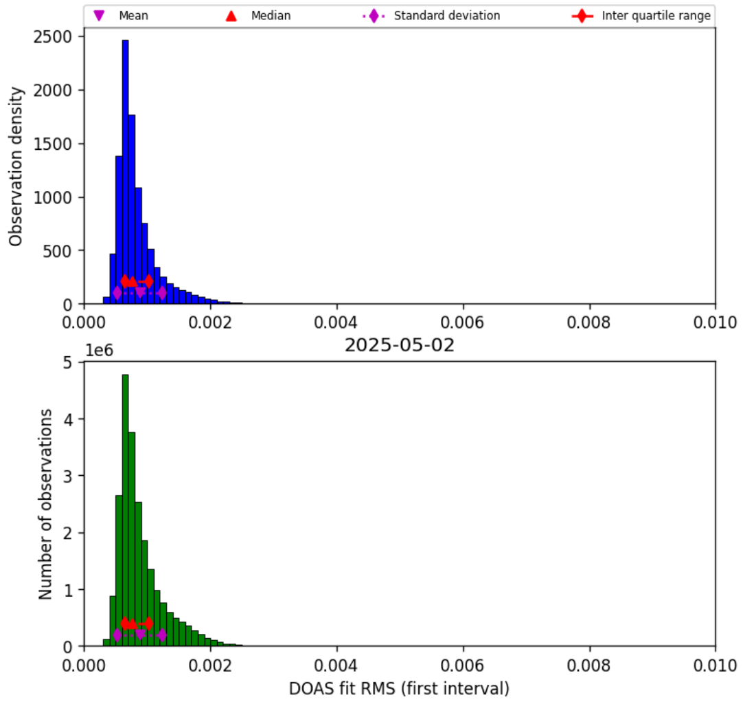
Figure 44: Histogram of “DOAS fit RMS (first interval)” for 2025-05-02 to 2025-05-02
