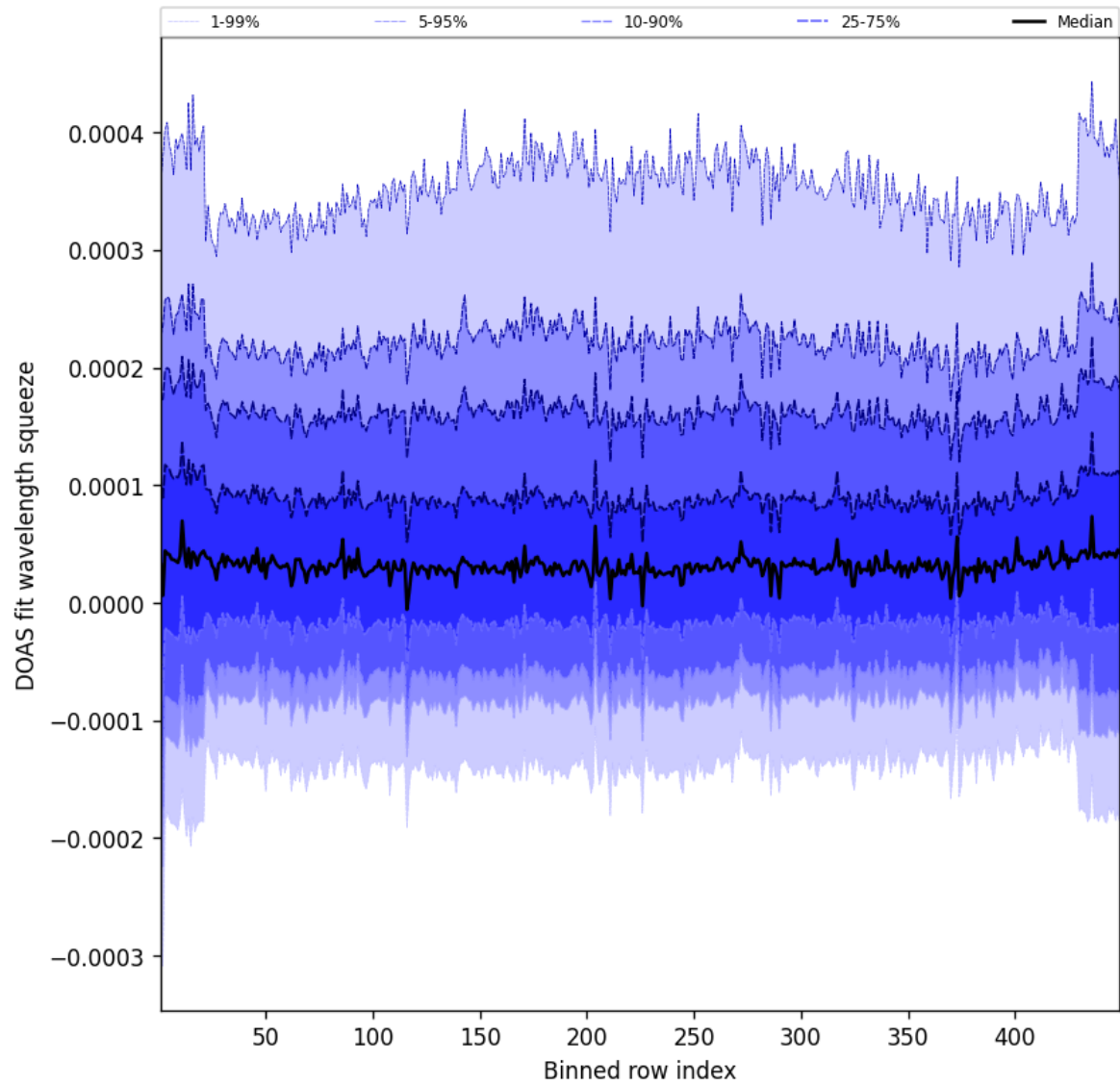
Figure 57: Along track statistics of “DOAS fit wavelength squeeze” for 2025-05-02 to 2025-05-02
