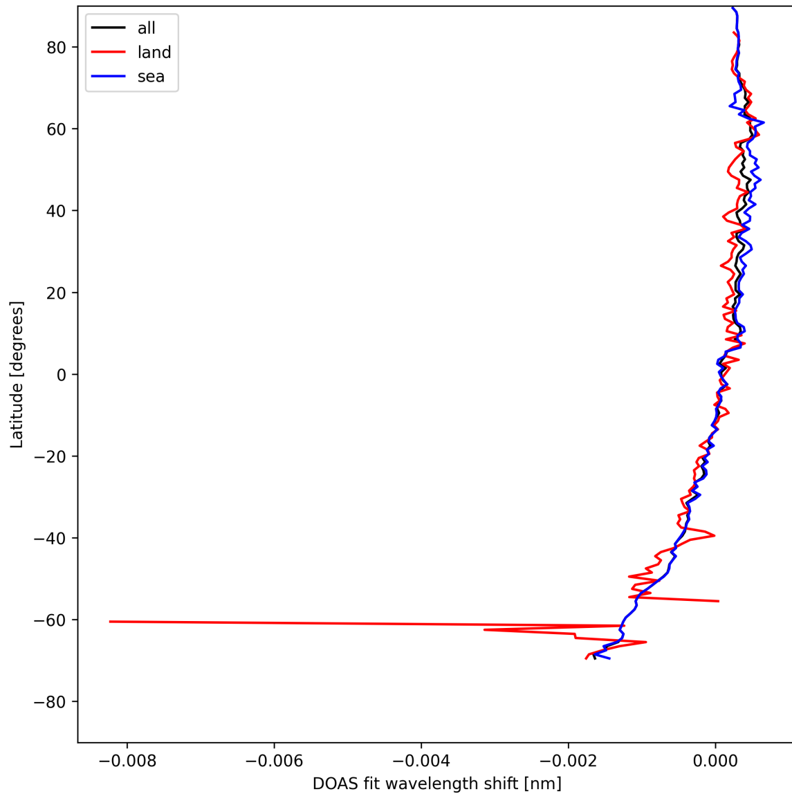
Figure 28: Zonal average of “DOAS fit wavelength shift” for 2025-05-02 to 2025-05-02.
