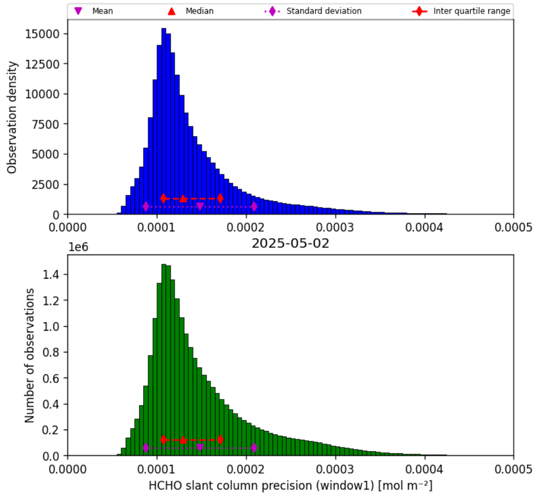
Figure 37: Histogram of “HCHO slant column precision (window1)” for 2025-05-02 to 2025-05-02
