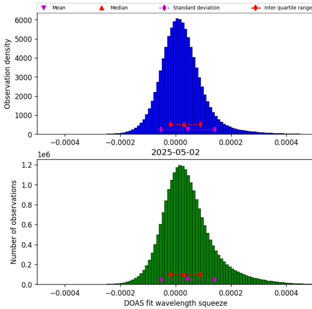
Figure 43: Histogram of “DOAS fit wavelength squeeze” for 2025-05-02 to 2025-05-02
