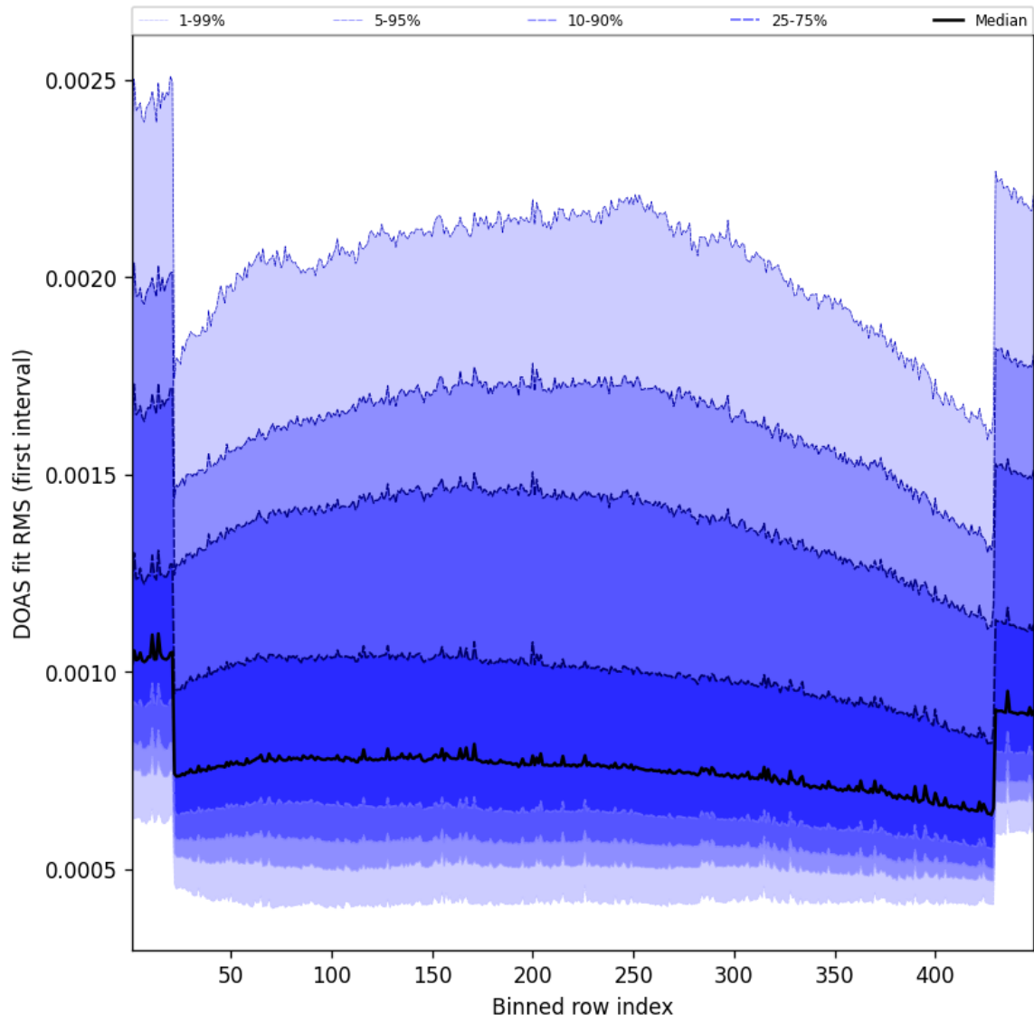
Figure 58: Along track statistics of “DOAS fit RMS (first interval)” for 2025-05-02 to 2025-05-02
