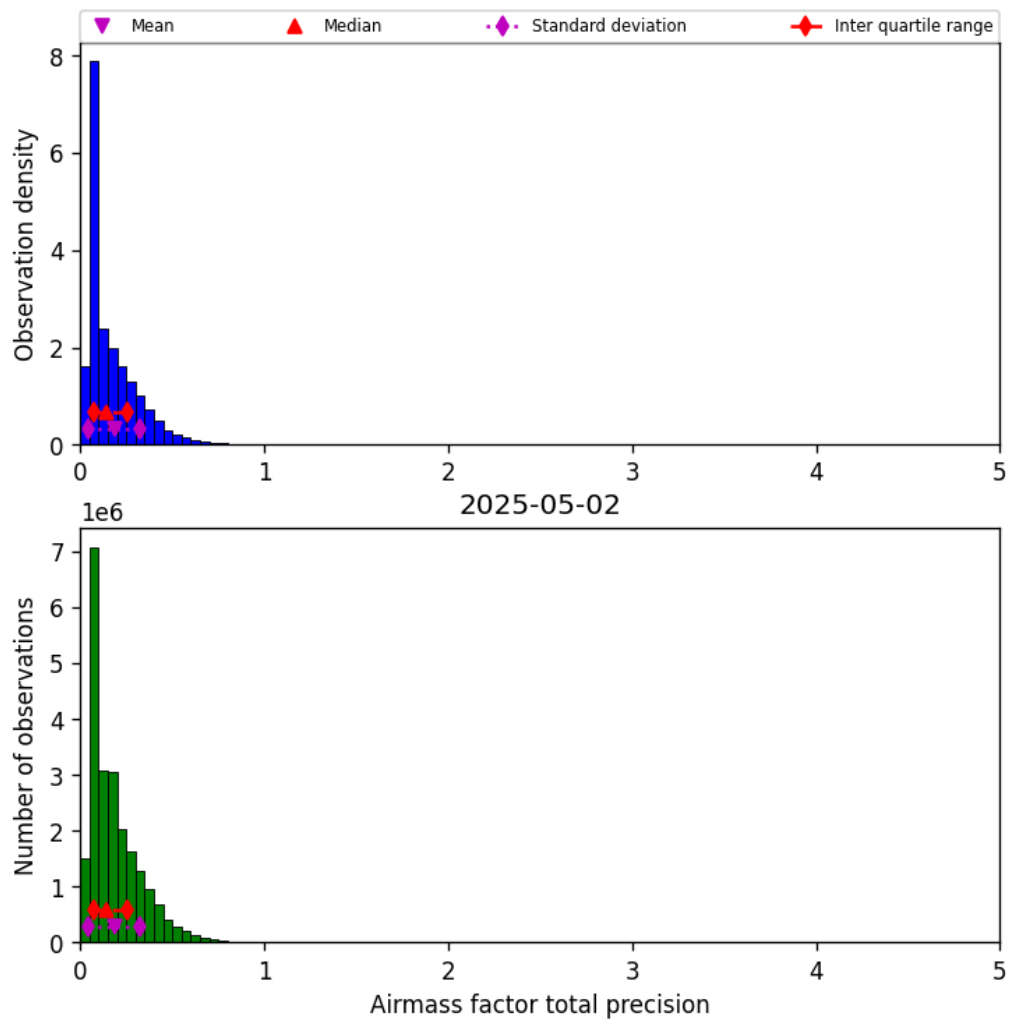
Figure 39: Histogram of “Airmass factor total precision” for 2025-05-02 to 2025-05-02
