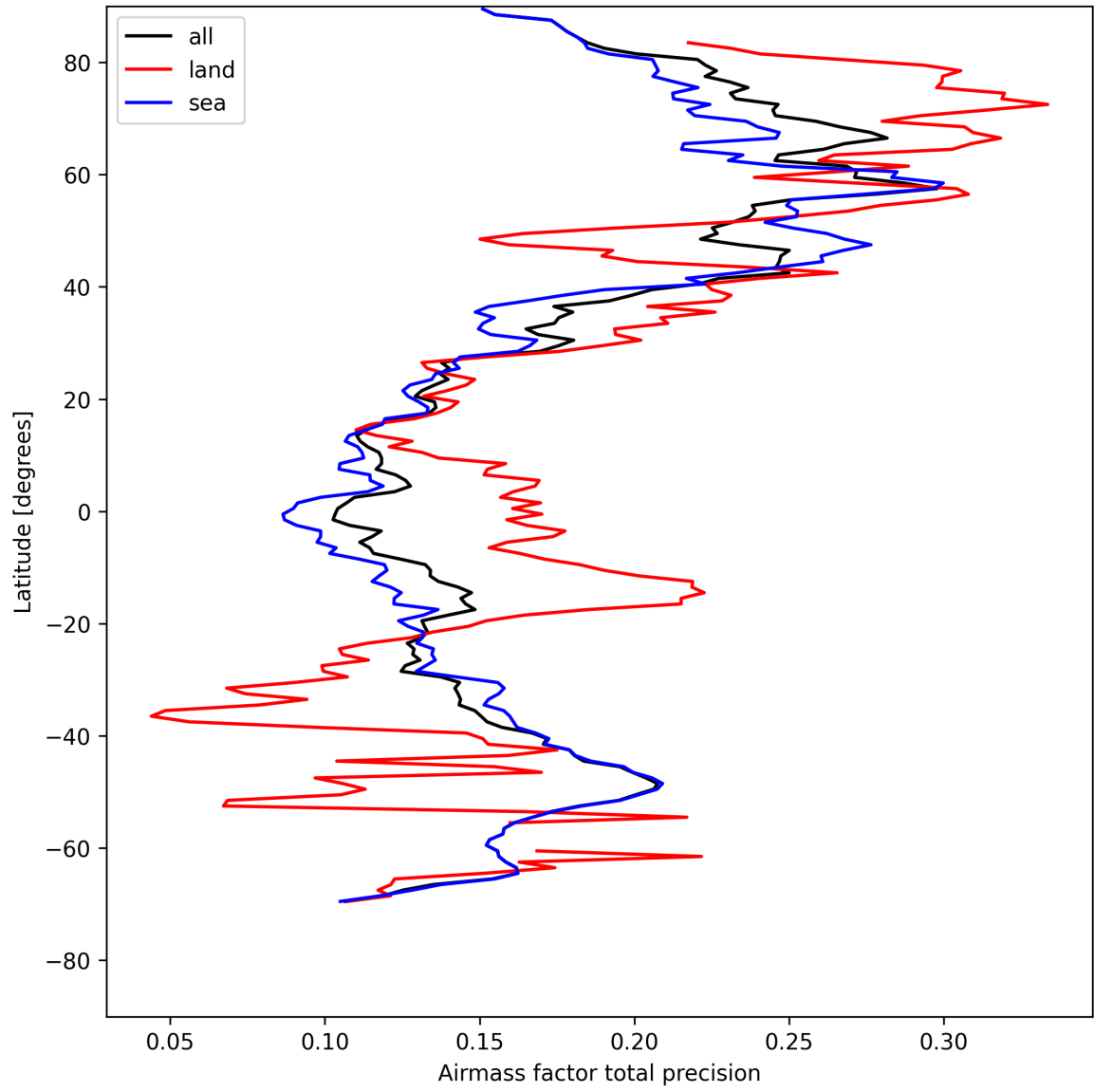
Figure 25: Zonal average of “Airmass factor total precision” for 2025-05-02 to 2025-05-02.
