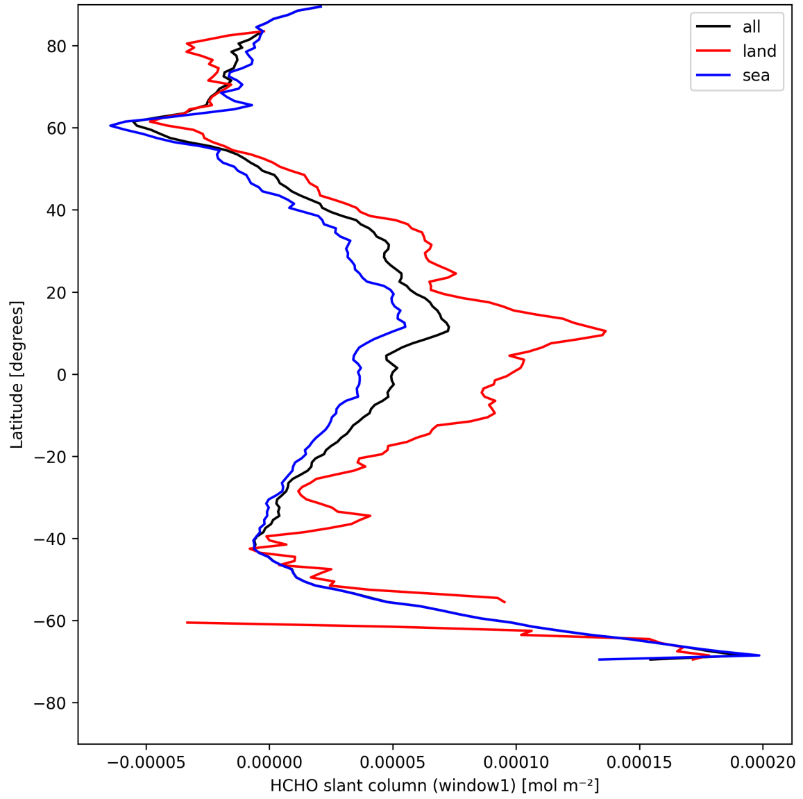
Figure 22: Zonal average of “HCHO slant column (window1)” for 2025-05-02 to 2025-05-02.
