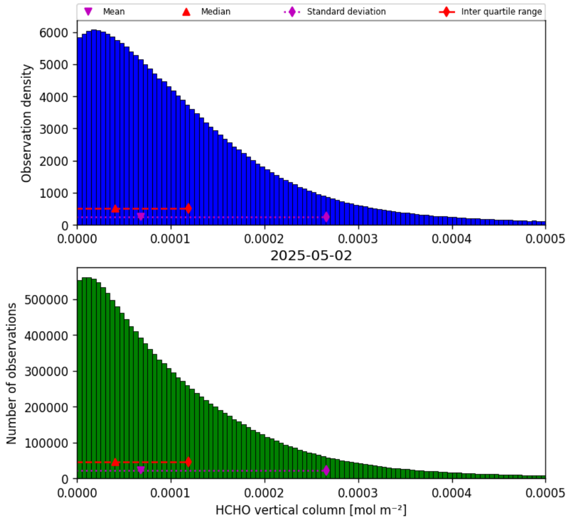
Figure 33: Histogram of “HCHO vertical column” for 2025-05-02 to 2025-05-02
