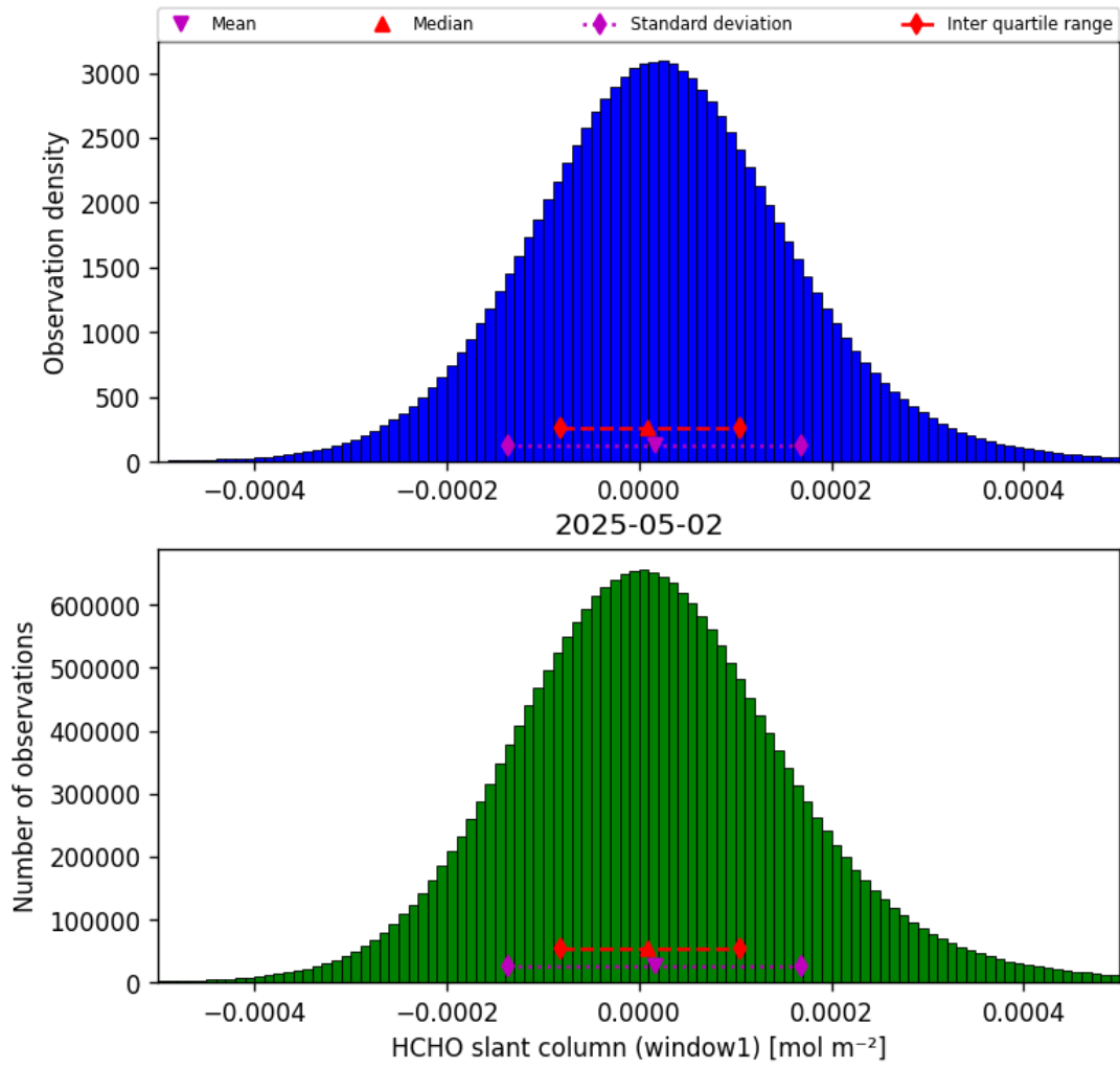
Figure 36: Histogram of “HCHO slant column (window1)” for 2025-05-02 to 2025-05-02
