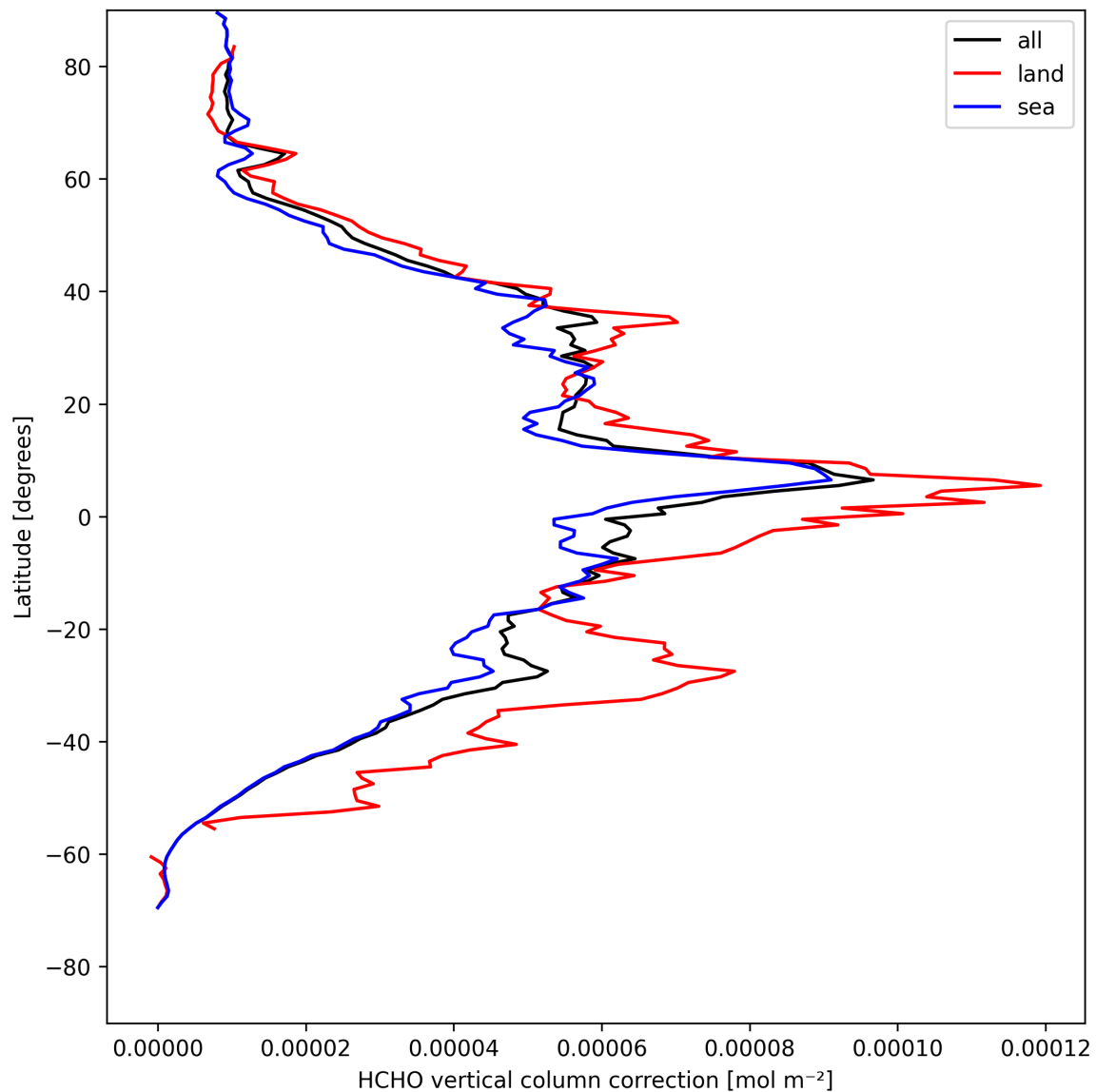
Figure 21: Zonal average of “HCHO vertical column correction” for 2025-05-02 to 2025-05-02.
