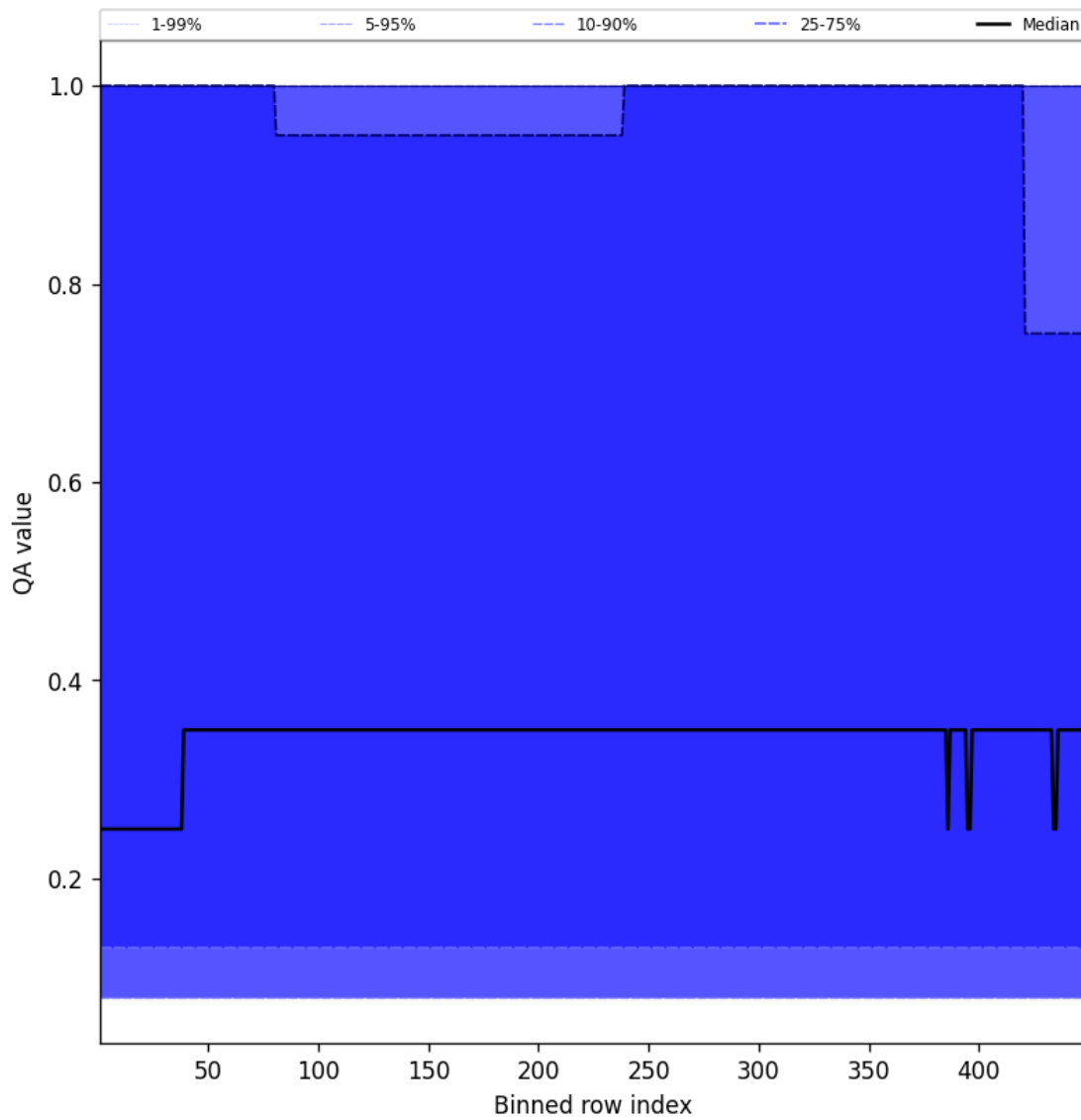
Figure 46: Along track statistics of “QA value” for 2025-05-02 to 2025-05-02
