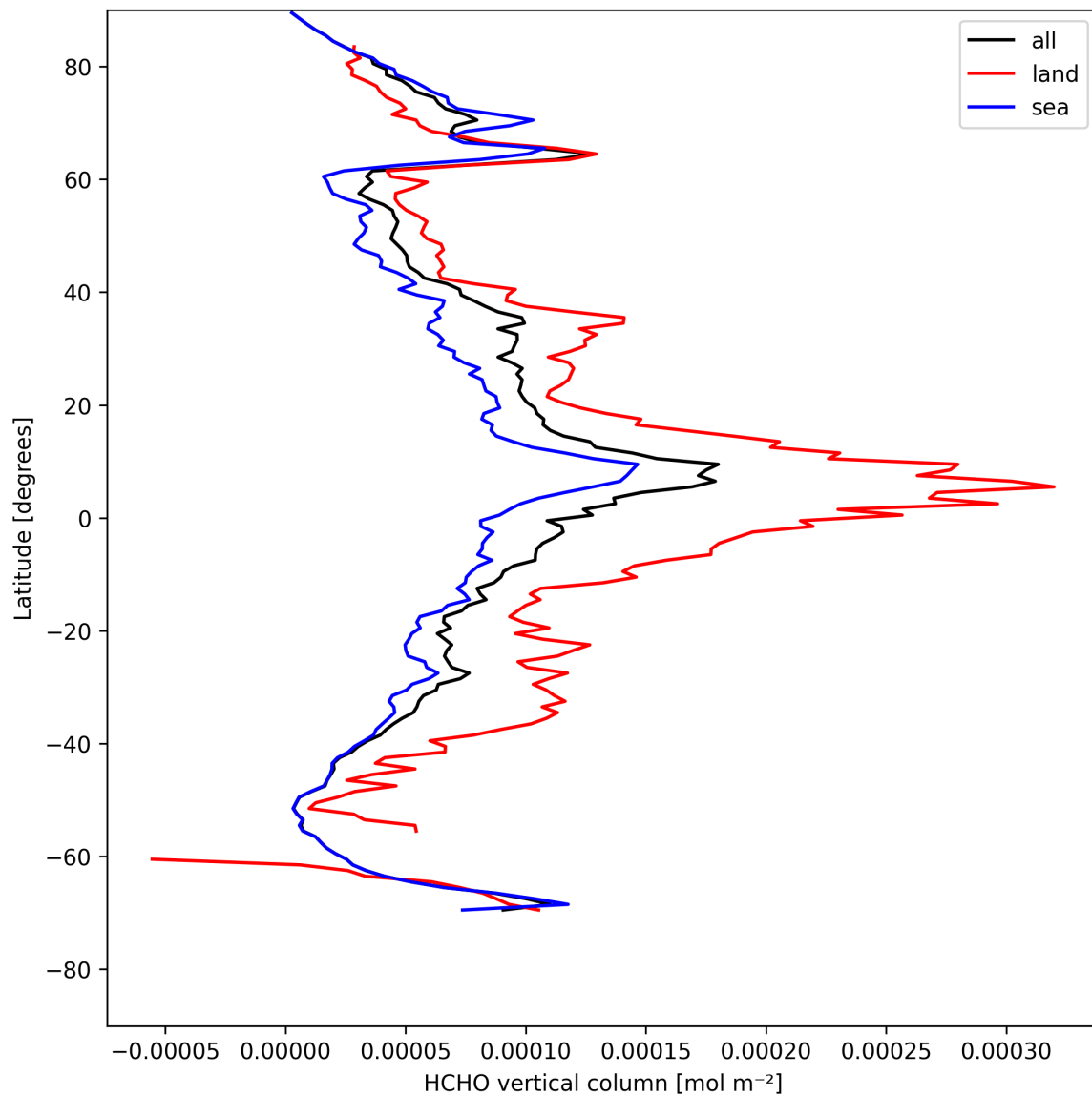
Figure 19: Zonal average of “HCHO vertical column” for 2025-05-02 to 2025-05-02.
