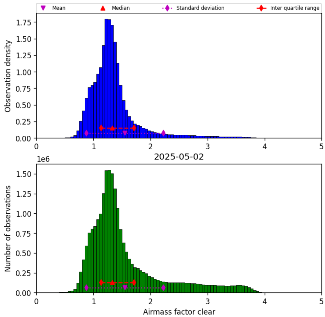
Figure 40: Histogram of “Airmass factor clear” for 2025-05-02 to 2025-05-02
