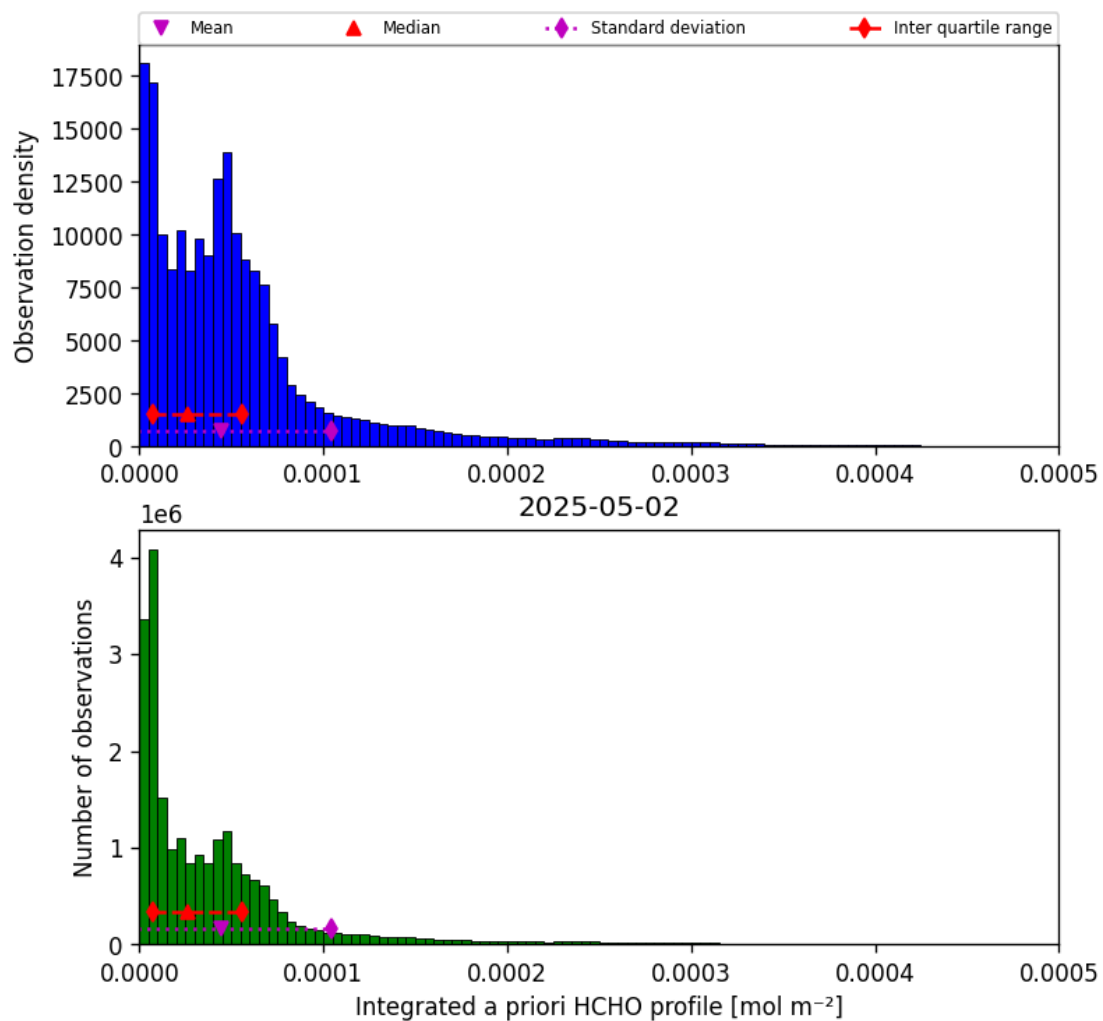
Figure 41: Histogram of “Integrated a priori HCHO profile” for 2025-05-02 to 2025-05-02
