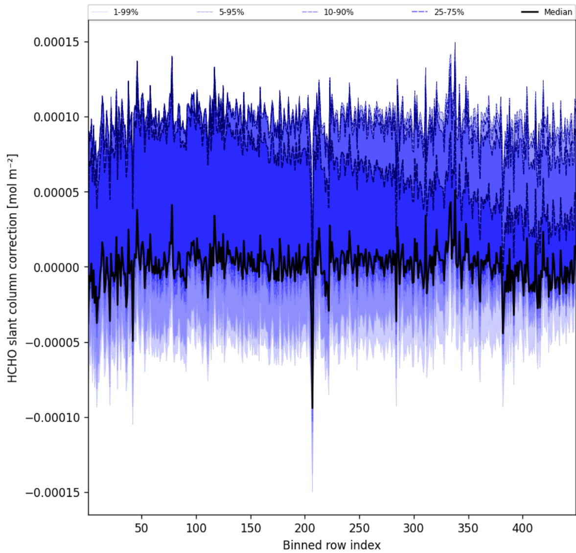
Figure 59: Along track statistics of “HCHO slant column correction” for 2025-05-02 to 2025-05-02
