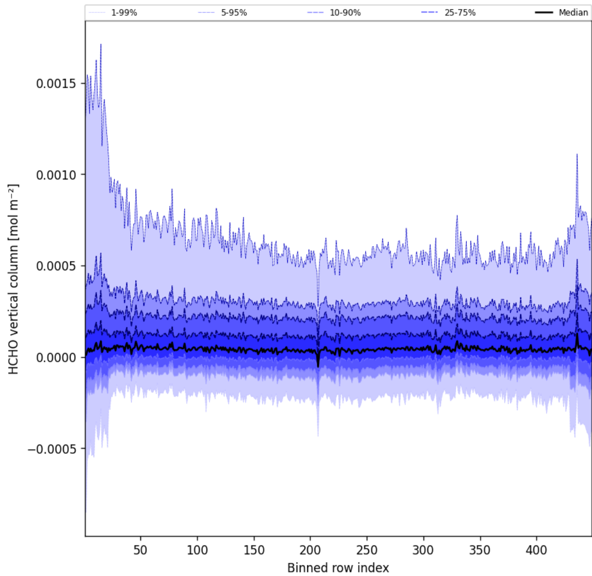
Figure 47: Along track statistics of “HCHO vertical column” for 2025-05-02 to 2025-05-02
