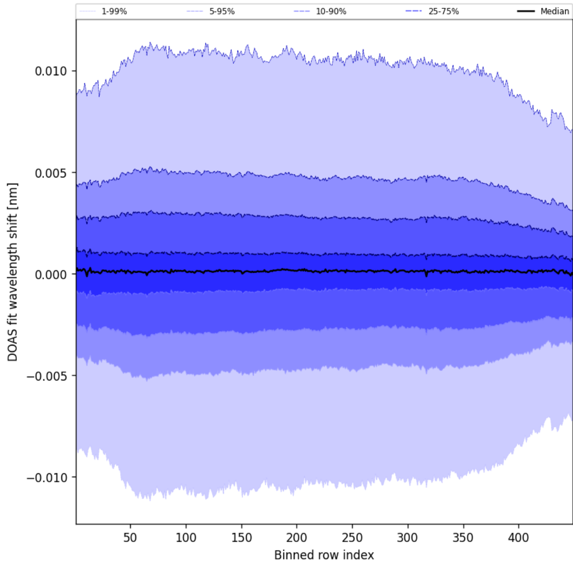
Figure 56: Along track statistics of “DOAS fit wavelength shift” for 2025-05-02 to 2025-05-02
