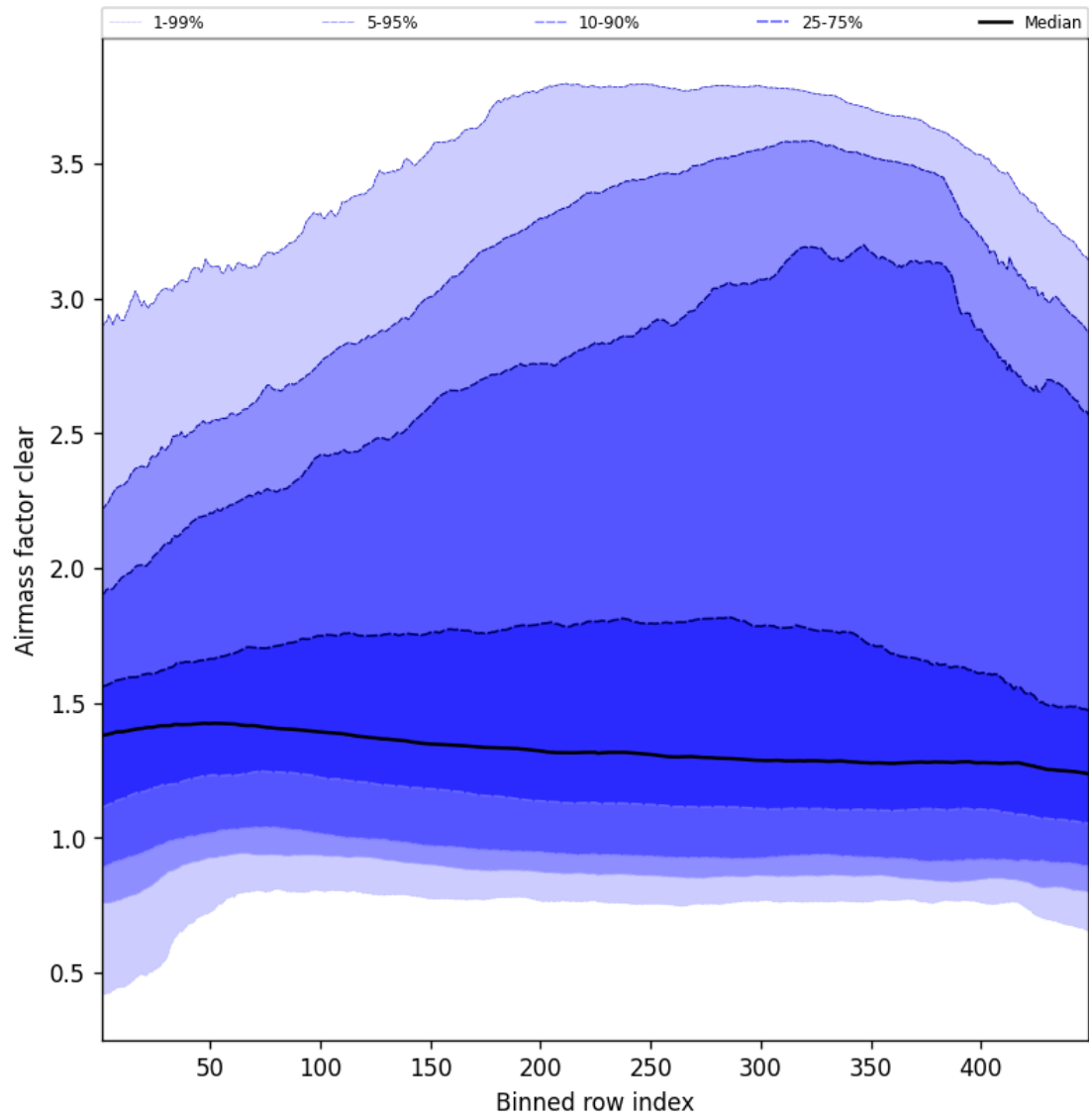
Figure 54: Along track statistics of “Airmass factor clear” for 2025-05-02 to 2025-05-02
