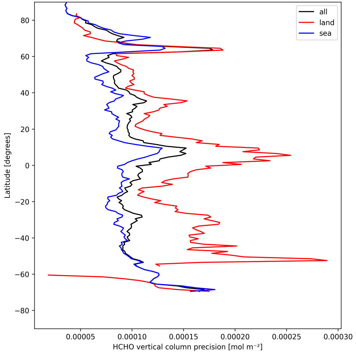
Figure 20: Zonal average of “HCHO vertical column precision” for 2025-05-02 to 2025-05-02.
