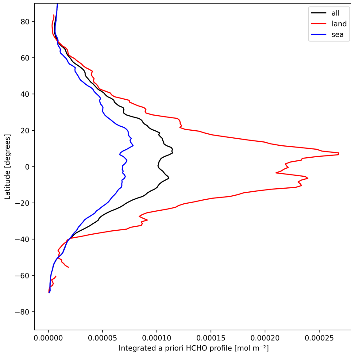
Figure 27: Zonal average of “Integrated a priori HCHO profile” for 2025-05-02 to 2025-05-02.
