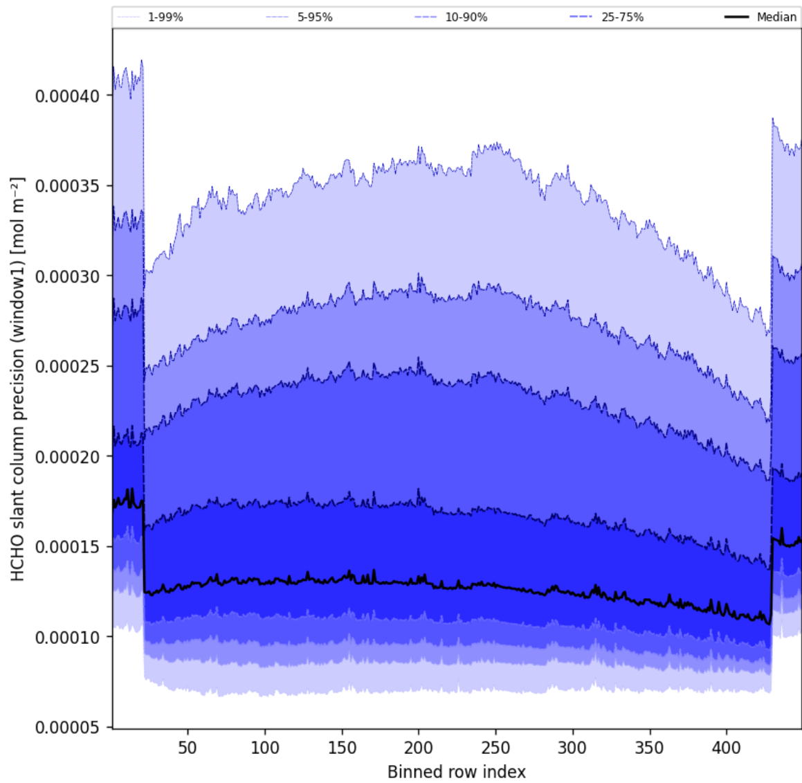
Figure 51: Along track statistics of “HCHO slant column precision (window1)” for 2025-05-02 to 2025-05-02
