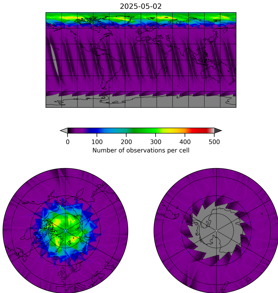
Figure 17: Map of the number of observations for 2025-05-02 to 2025-05-02
