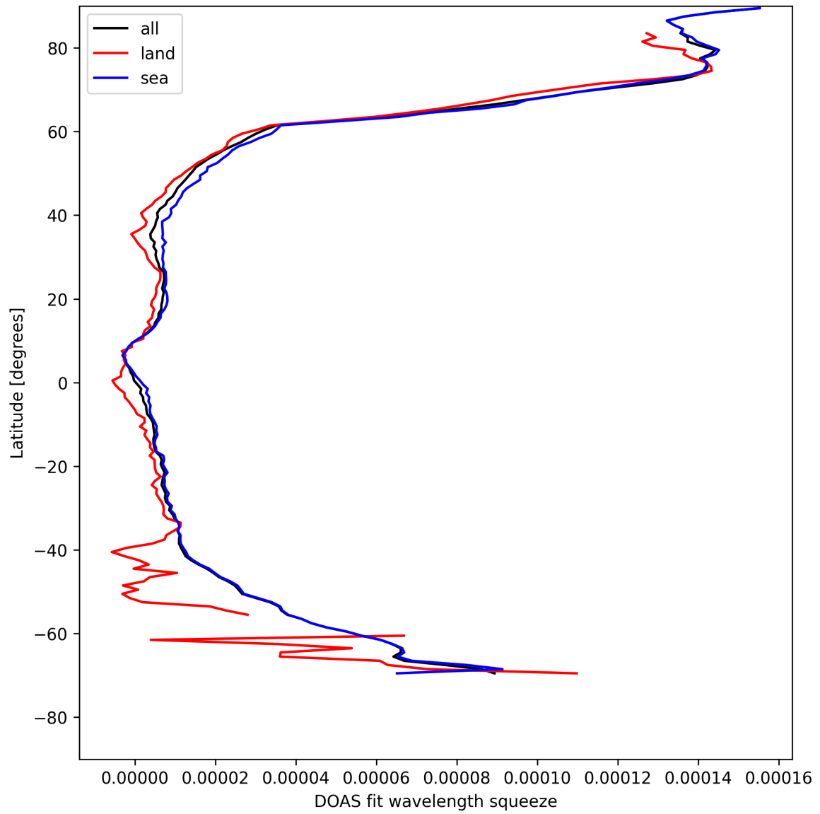
Figure 29: Zonal average of “DOAS fit wavelength squeeze” for 2025-05-02 to 2025-05-02.
