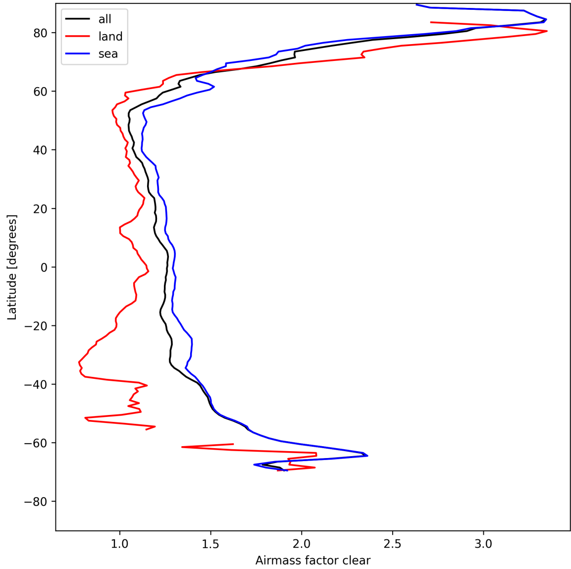
Figure 26: Zonal average of “Airmass factor clear” for 2025-05-02 to 2025-05-02.
