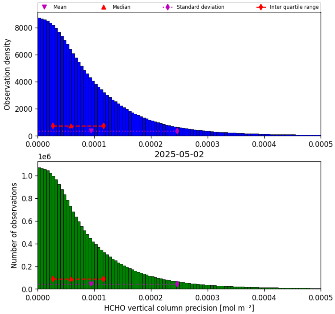
Figure 34: Histogram of “HCHO vertical column precision” for 2025-05-02 to 2025-05-02
