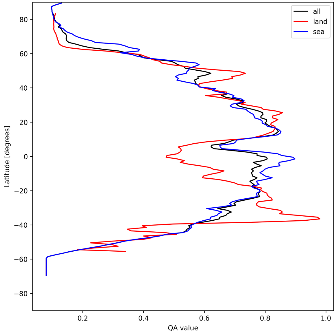
Figure 18: Zonal average of “QA value” for 2025-05-02 to 2025-05-02.
