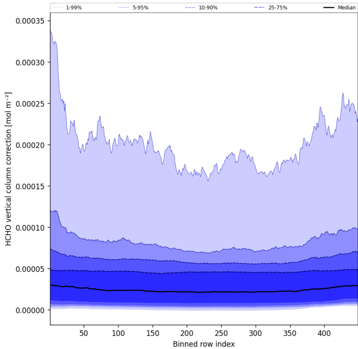
Figure 49: Along track statistics of “HCHO vertical column correction” for 2025-05-02 to 2025-05-02
