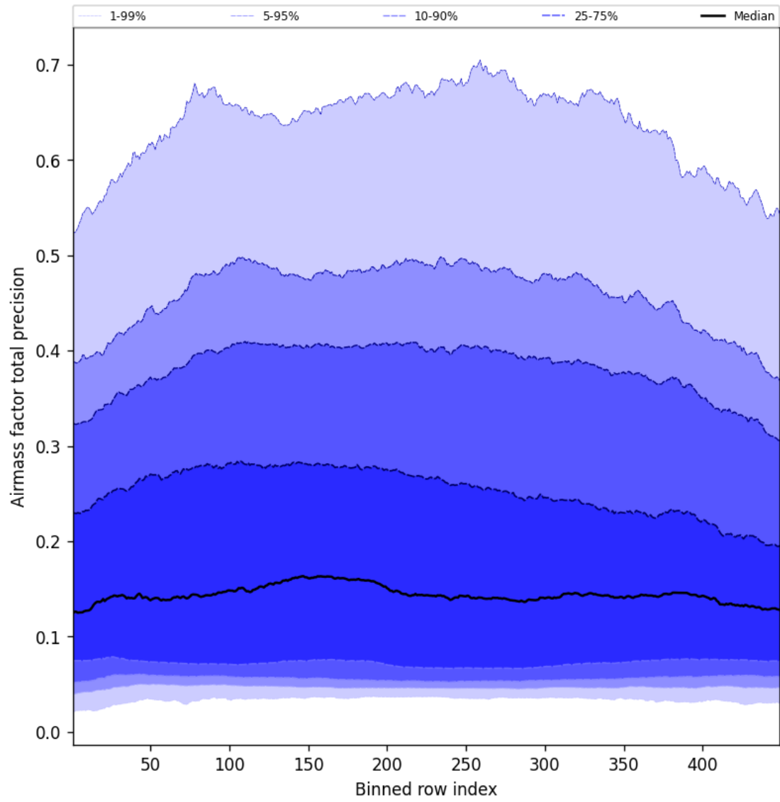
Figure 53: Along track statistics of “Airmass factor total precision” for 2025-05-02 to 2025-05-02
