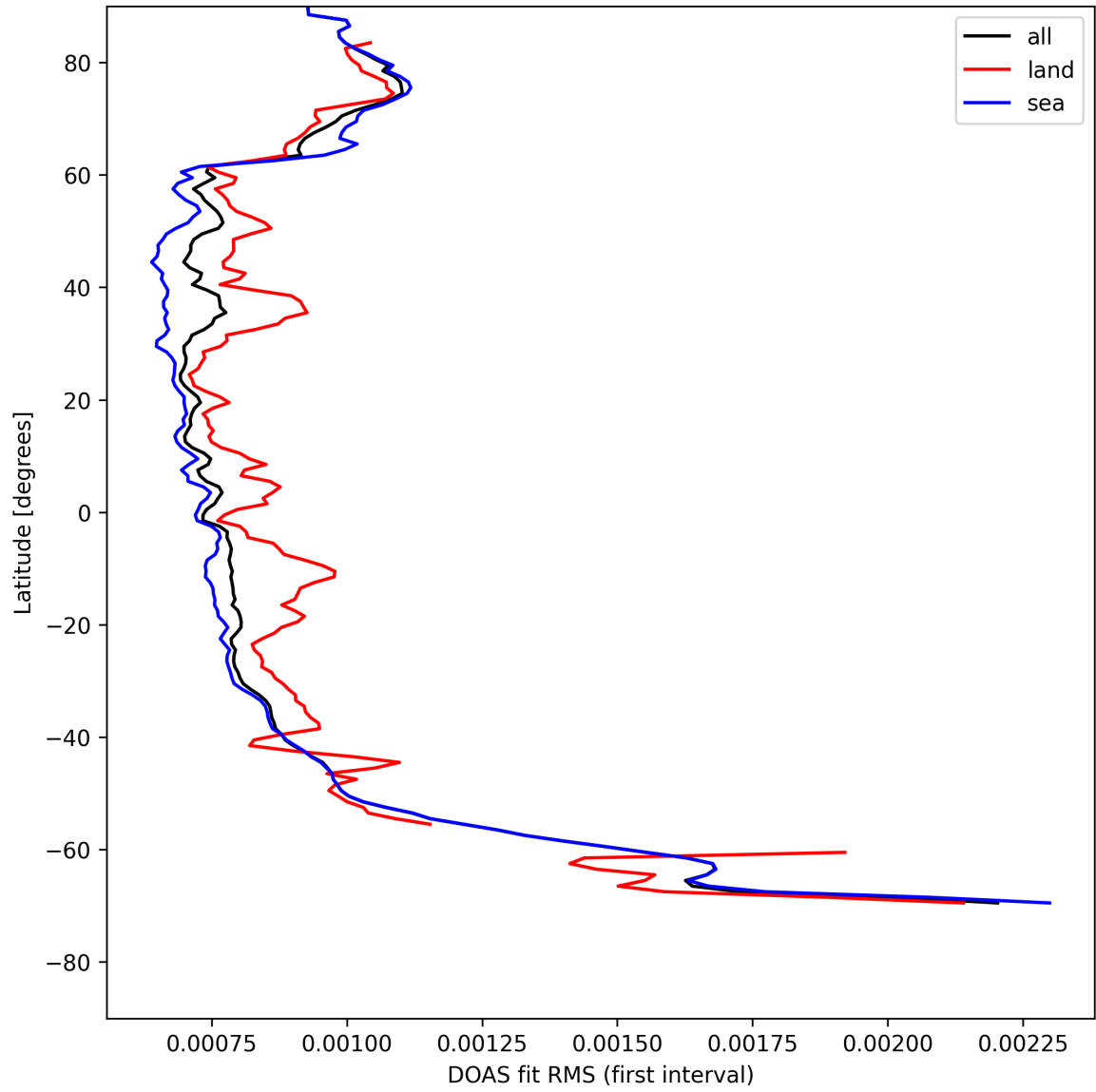
Figure 30: Zonal average of "DOAS fit RMS (first interval)" for 2025-05-02 to 2025-05-02.
