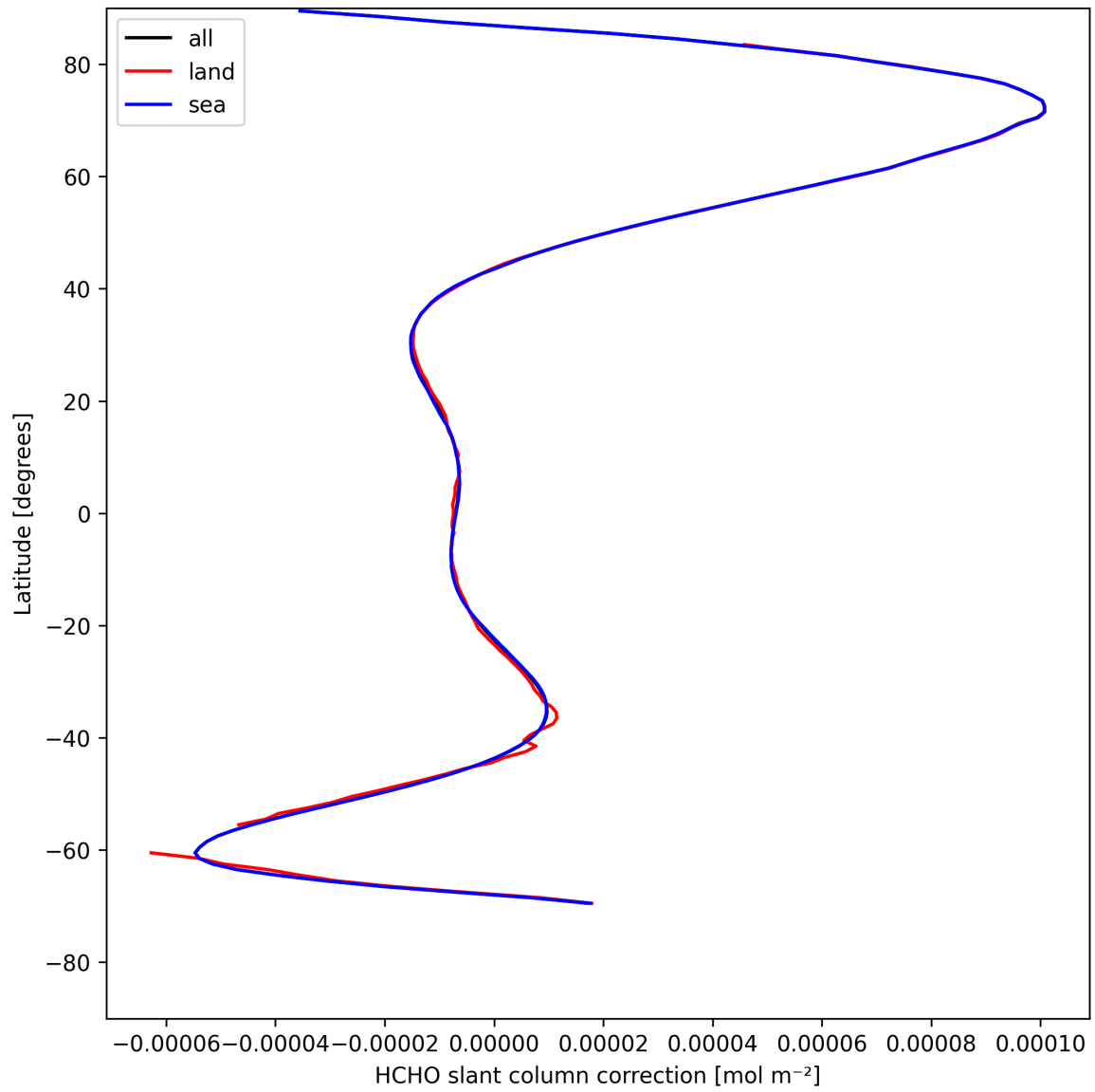
Figure 31: Zonal average of “HCHO slant column correction” for 2025-05-02 to 2025-05-02.
