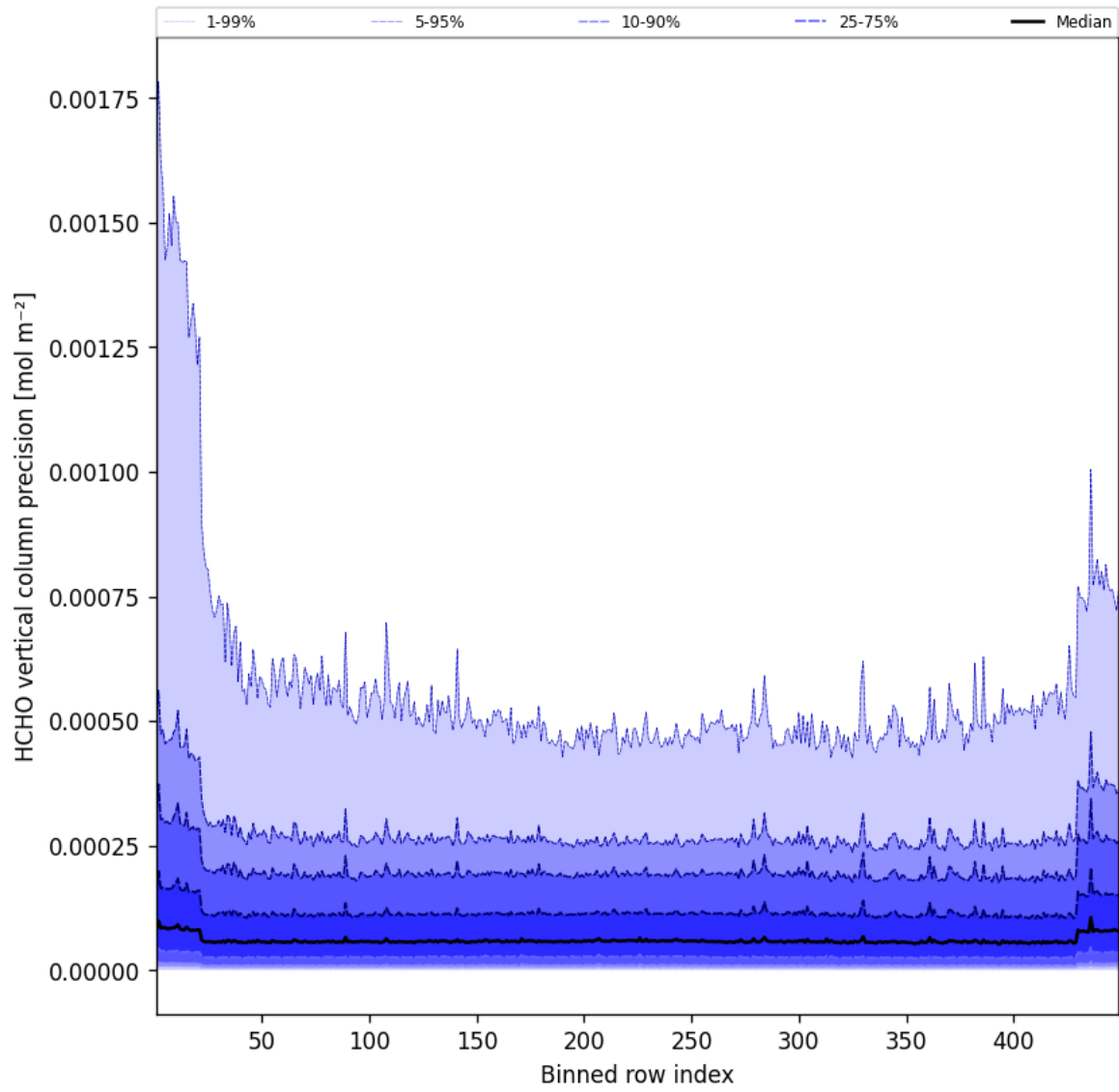
Figure 48: Along track statistics of “HCHO vertical column precision” for 2025-05-02 to 2025-05-02
