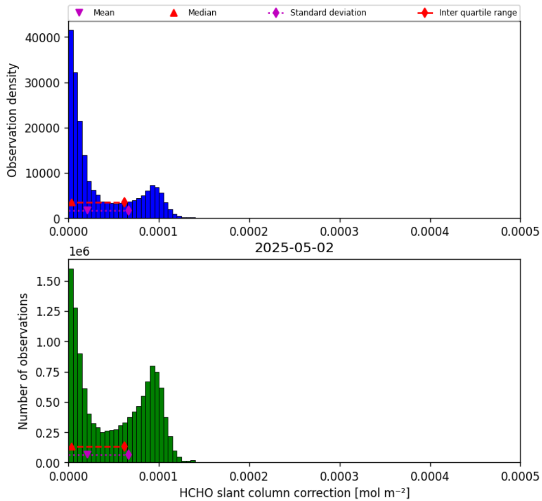
Figure 45: Histogram of “HCHO slant column correction” for 2025-05-02 to 2025-05-02
