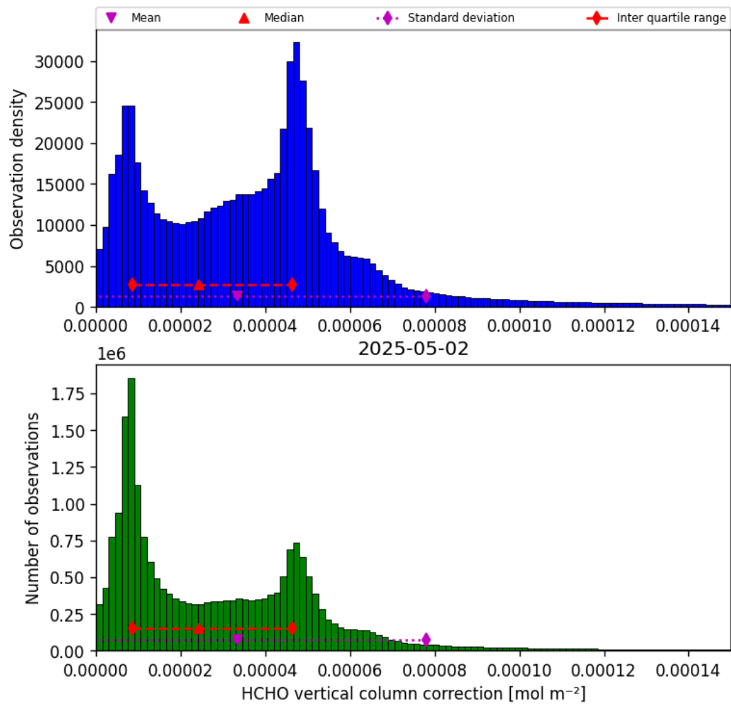
Figure 35: Histogram of “HCHO vertical column correction” for 2025-05-02 to 2025-05-02
