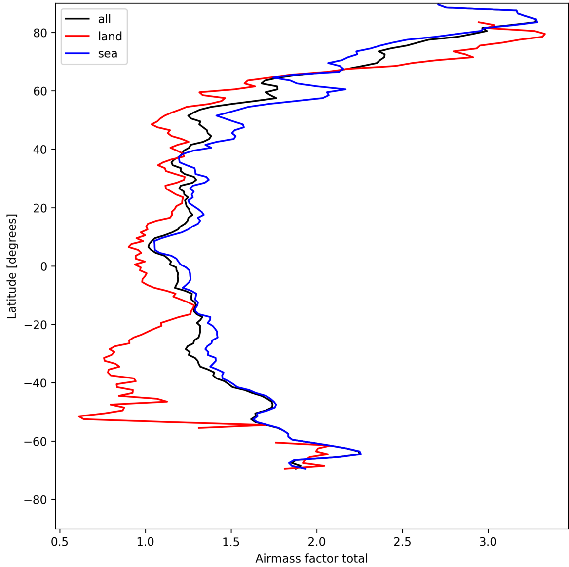
Figure 24: Zonal average of “Airmass factor total” for 2025-05-02 to 2025-05-02.
