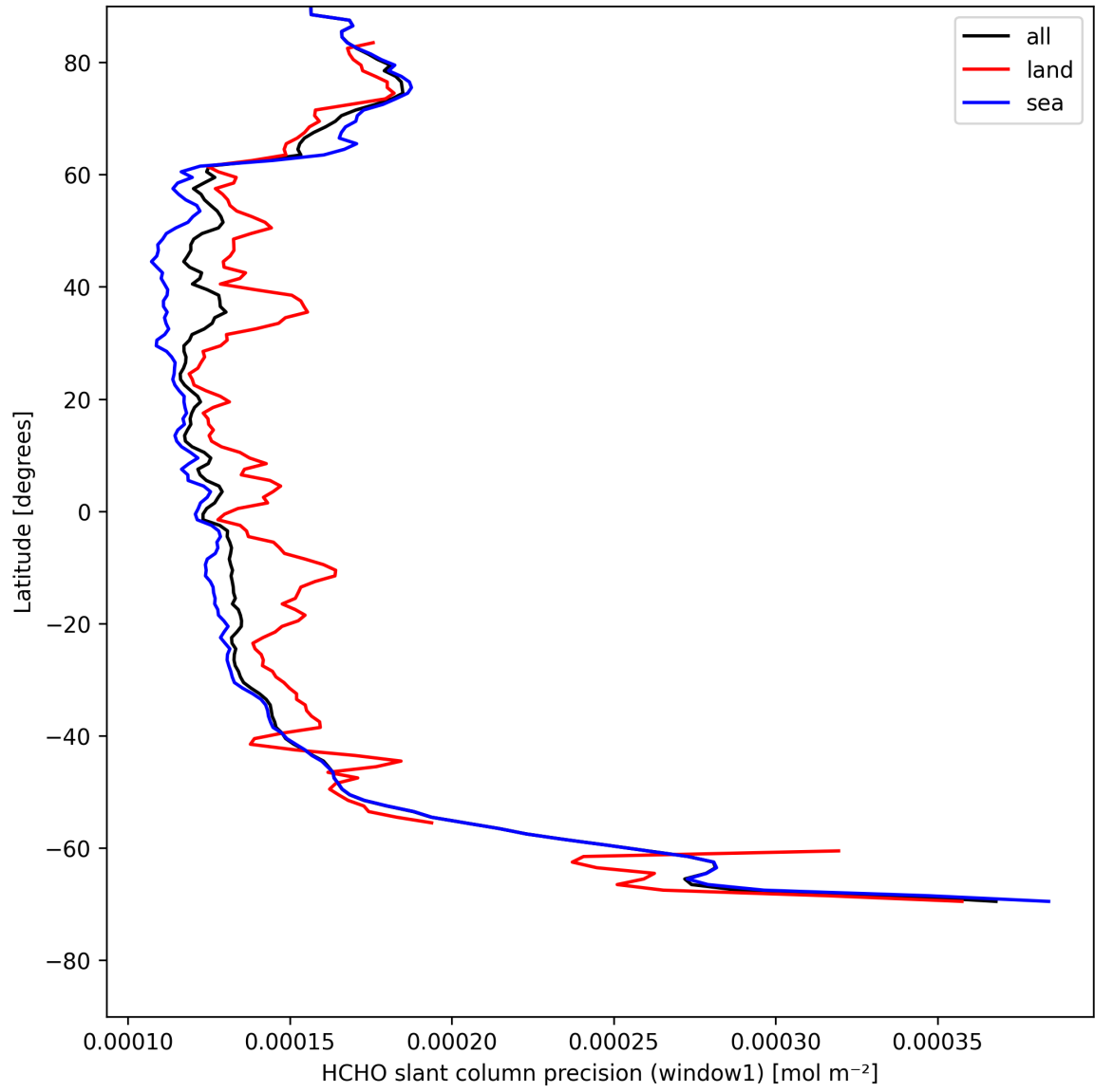
Figure 23: Zonal average of “HCHO slant column precision (window1)” for 2025-05-02 to 2025-05-02.
