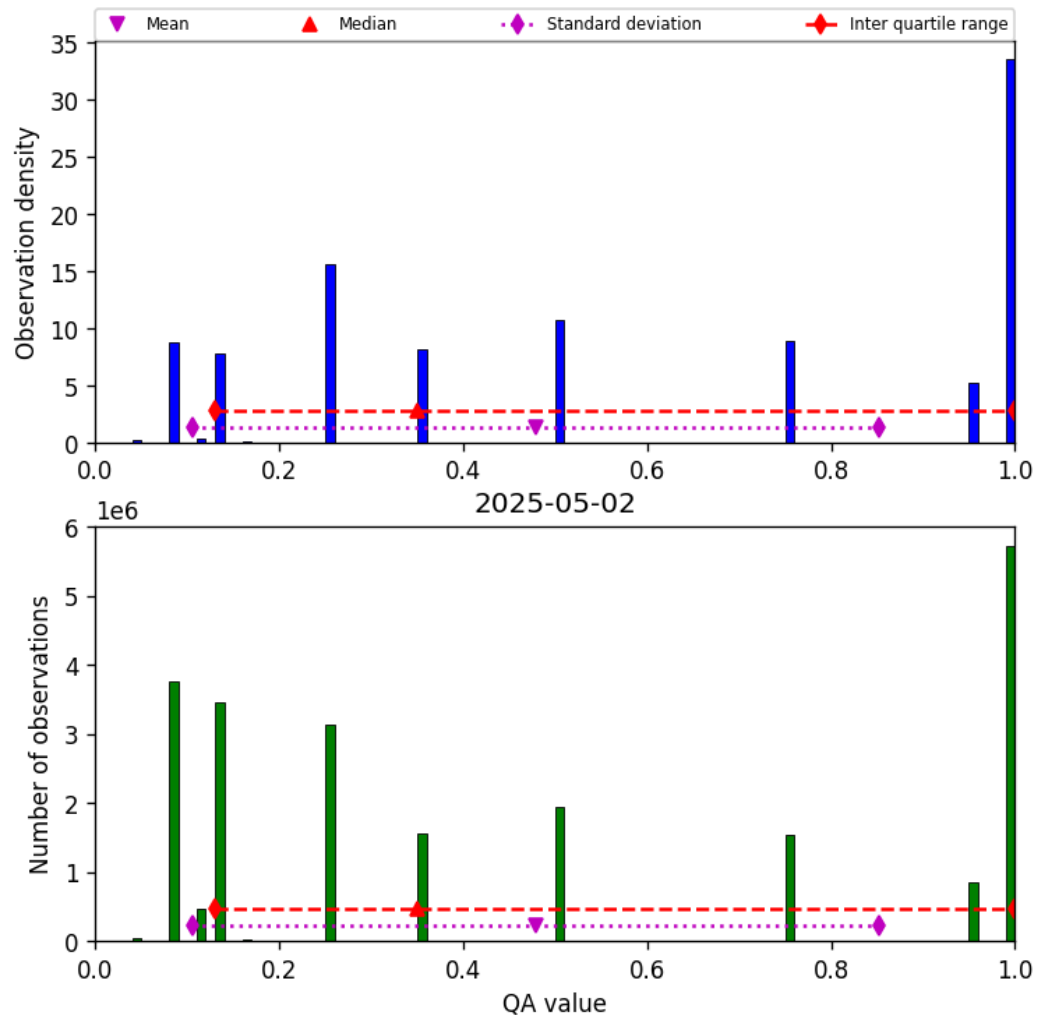
Figure 32: Histogram of “QA value” for 2025-05-02 to 2025-05-02
