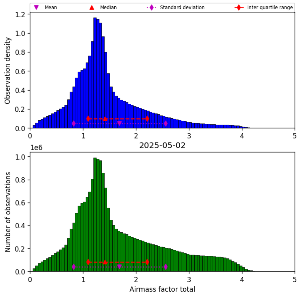
Figure 38: Histogram of “Airmass factor total” for 2025-05-02 to 2025-05-02
