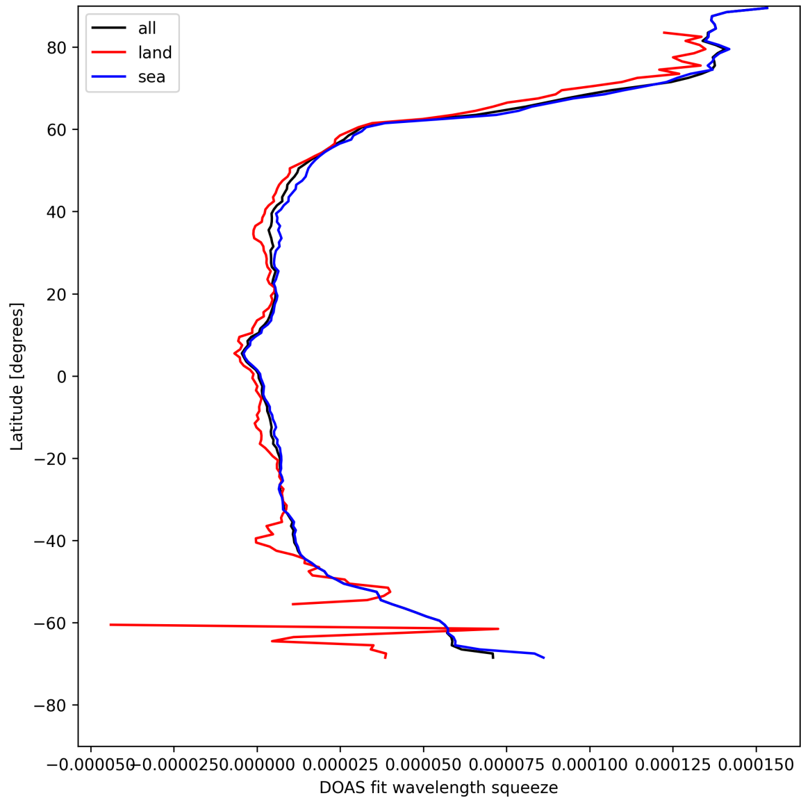
Figure 29: Zonal average of “DOAS fit wavelength squeeze” for 2025-05-03 to 2025-05-03.
