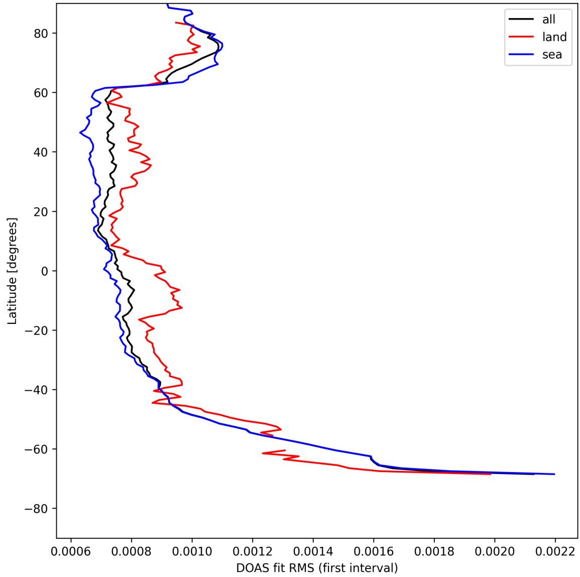
Figure 30: Zonal average of “DOAS fit RMS (first interval)” for 2025-05-03 to 2025-05-03.
