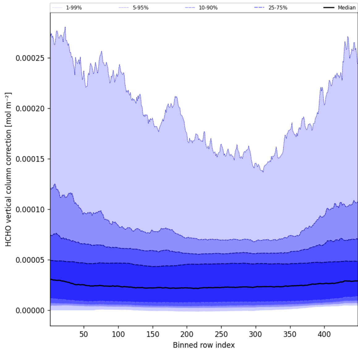
Figure 49: Along track statistics of “HCHO vertical column correction” for 2025-05-03 to 2025-05-03
