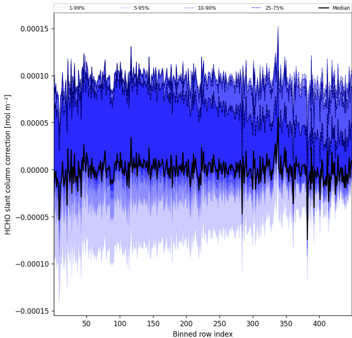
Figure 59: Along track statistics of "HCHO slant column correction" for 2025-05-03 to 2025-05-03
