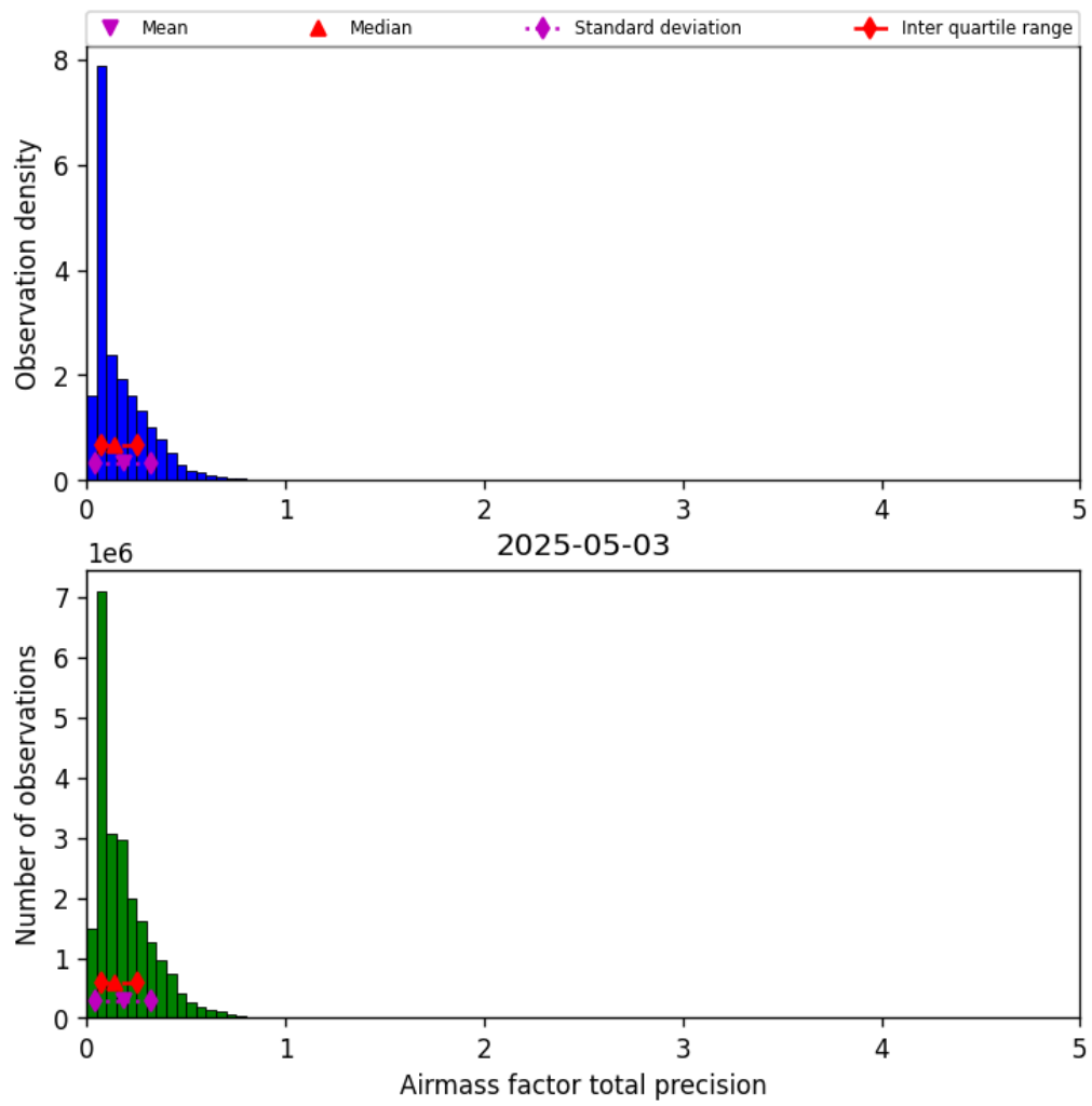
Figure 39: Histogram of “Airmass factor total precision” for 2025-05-03 to 2025-05-03
