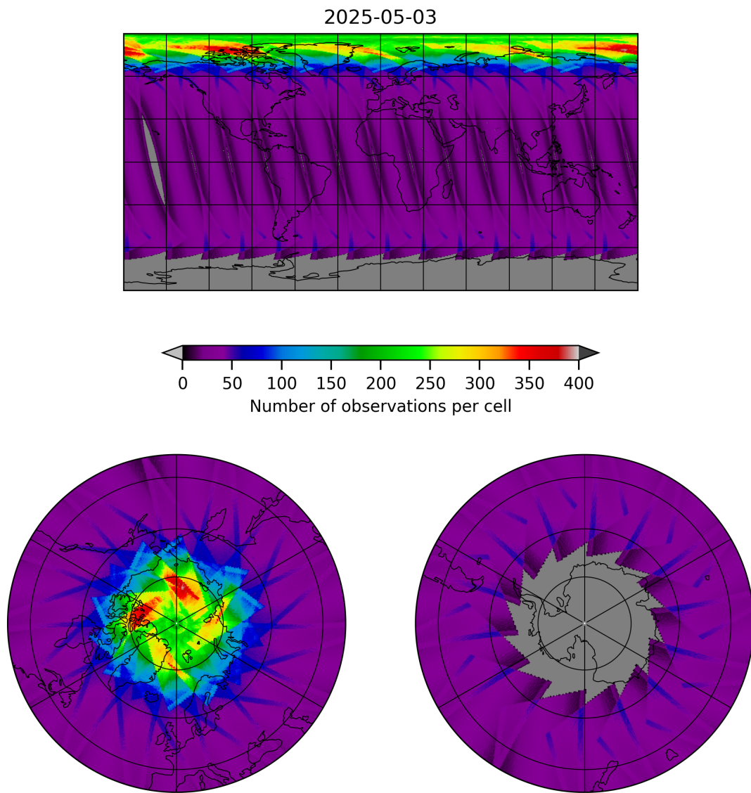
Figure 17: Map of the number of observations for 2025-05-03 to 2025-05-03
