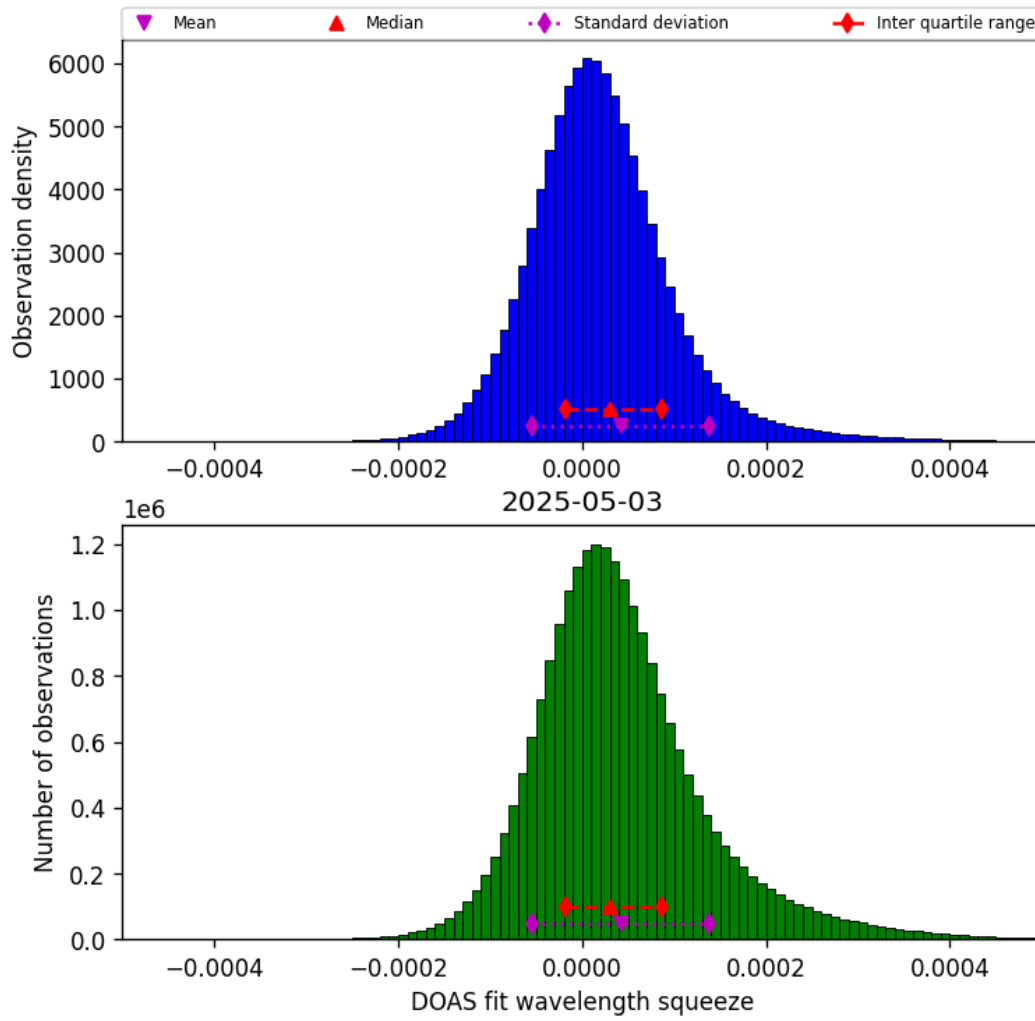
Figure 43: Histogram of “DOAS fit wavelength squeeze” for 2025-05-03 to 2025-05-03
