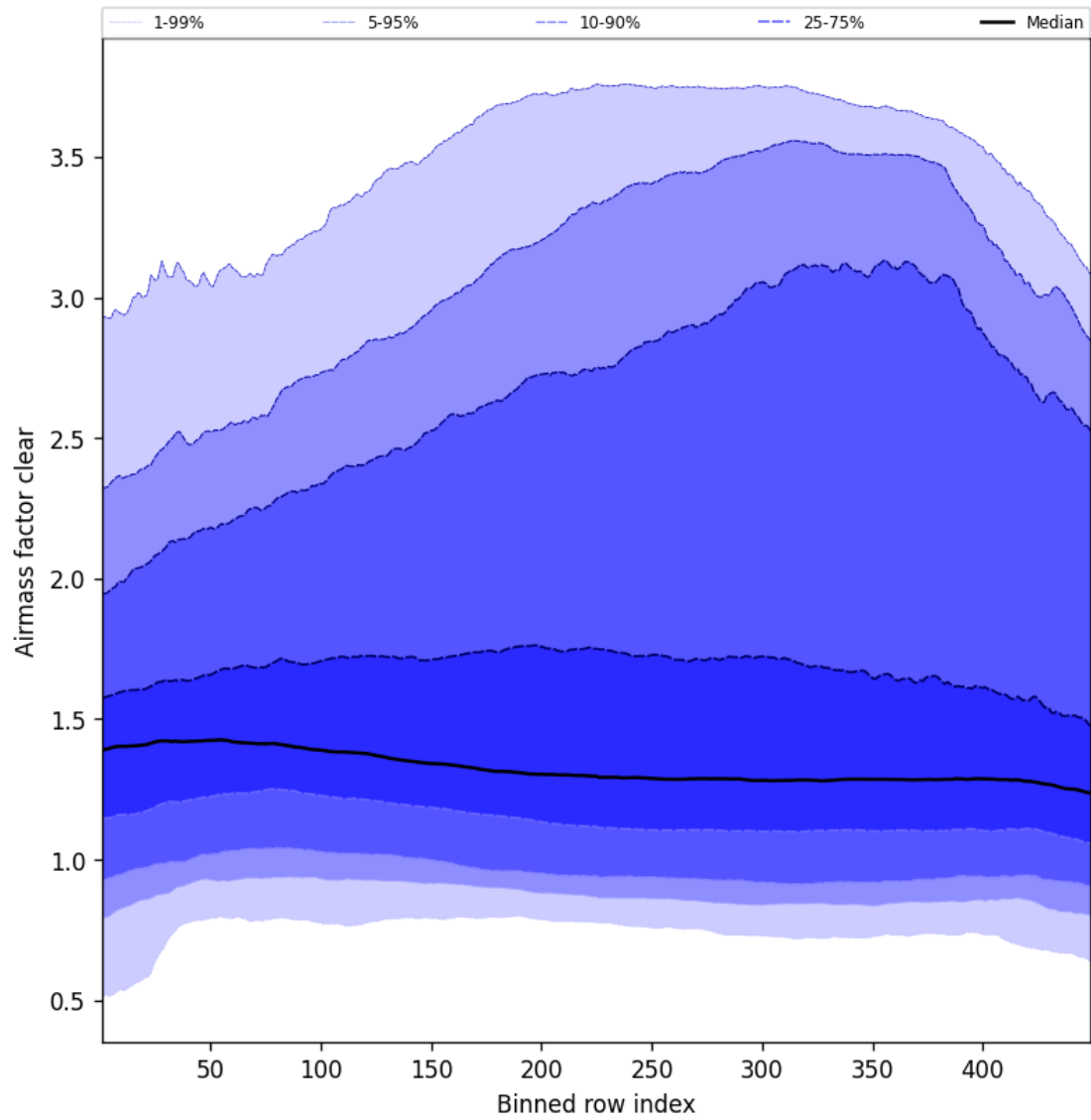
Figure 54: Along track statistics of “Airmass factor clear” for 2025-05-03 to 2025-05-03
