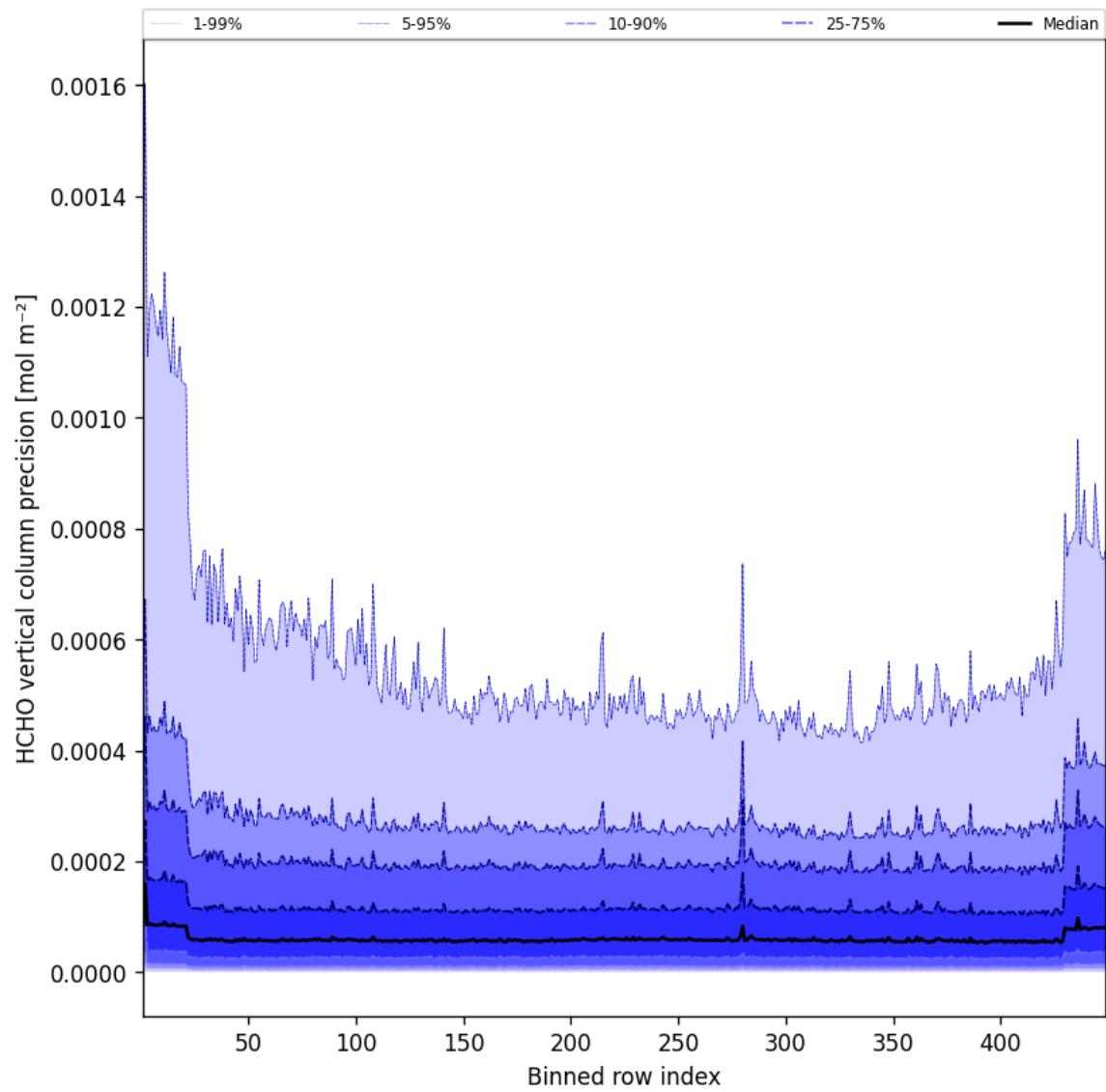
Figure 48: Along track statistics of “HCHO vertical column precision” for 2025-05-03 to 2025-05-03
