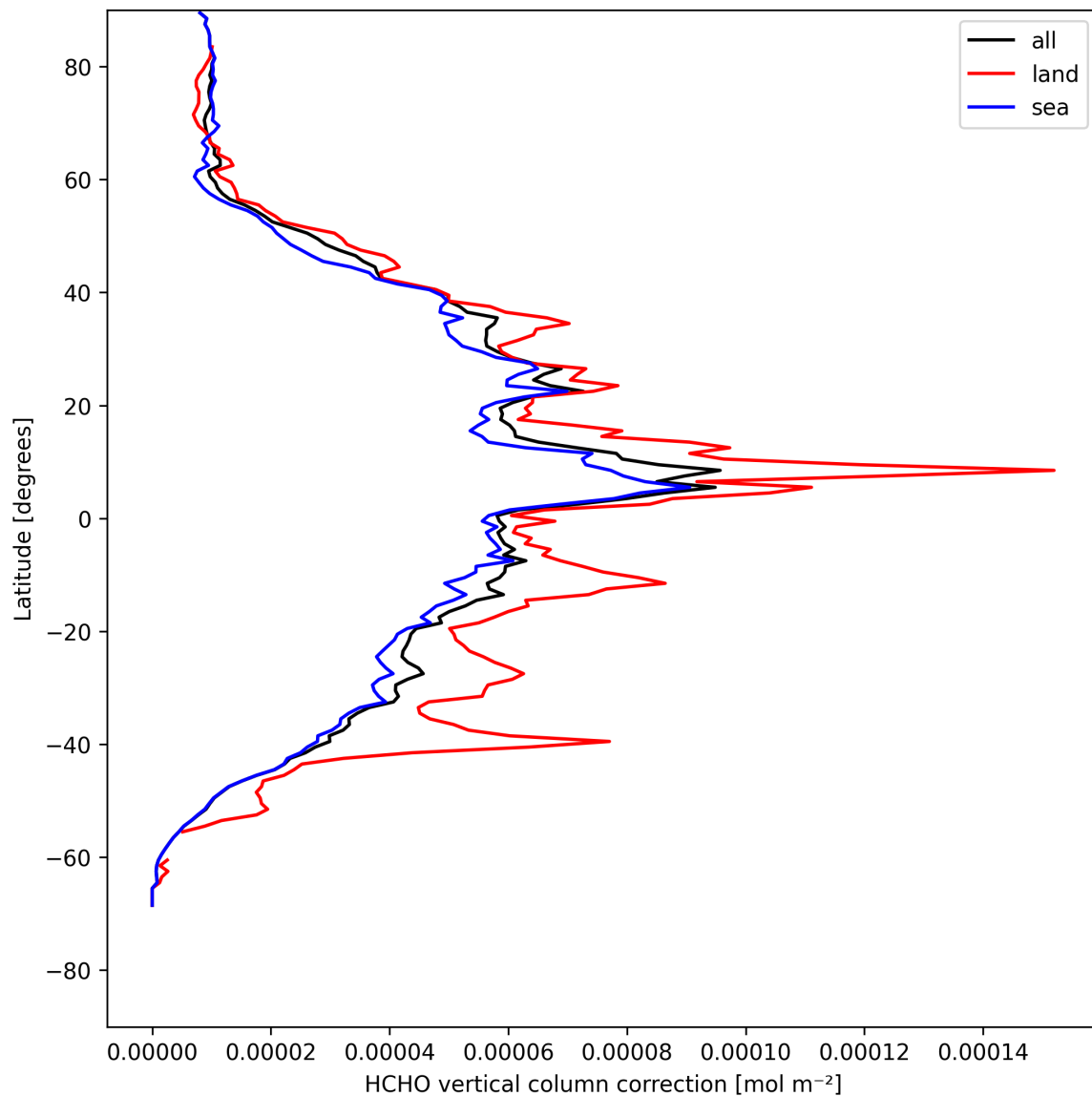
Figure 21: Zonal average of “HCHO vertical column correction” for 2025-05-03 to 2025-05-03.
