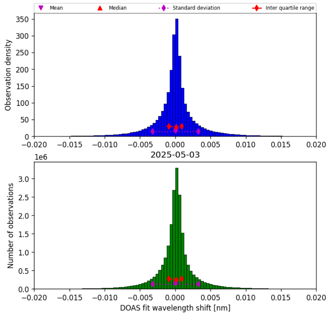
Figure 42: Histogram of “DOAS fit wavelength shift” for 2025-05-03 to 2025-05-03
