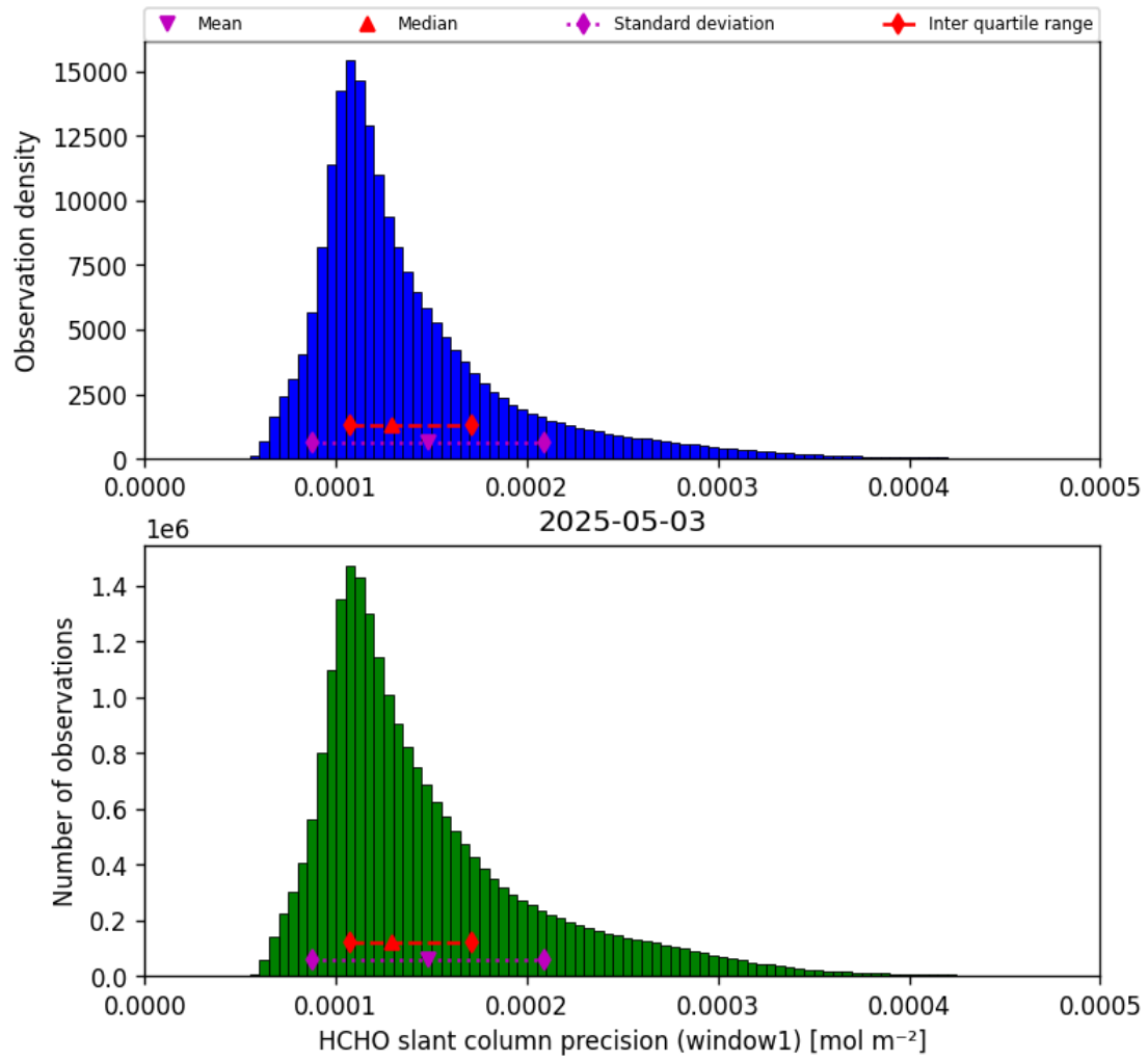
Figure 37: Histogram of “HCHO slant column precision (window1)” for 2025-05-03 to 2025-05-03
