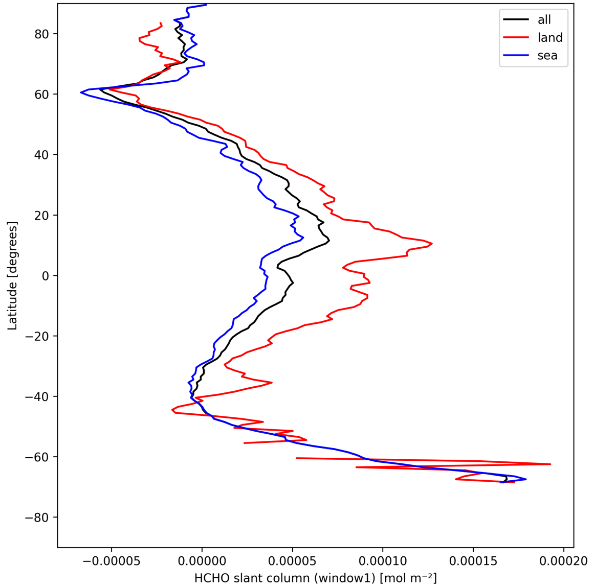
Figure 22: Zonal average of “HCHO slant column (window1)” for 2025-05-03 to 2025-05-03.
