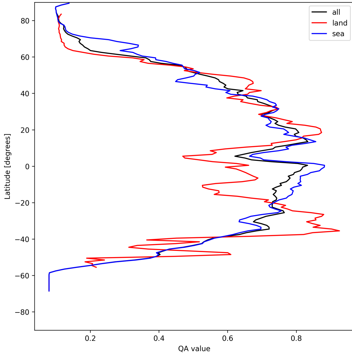
Figure 18: Zonal average of “QA value” for 2025-05-03 to 2025-05-03.
