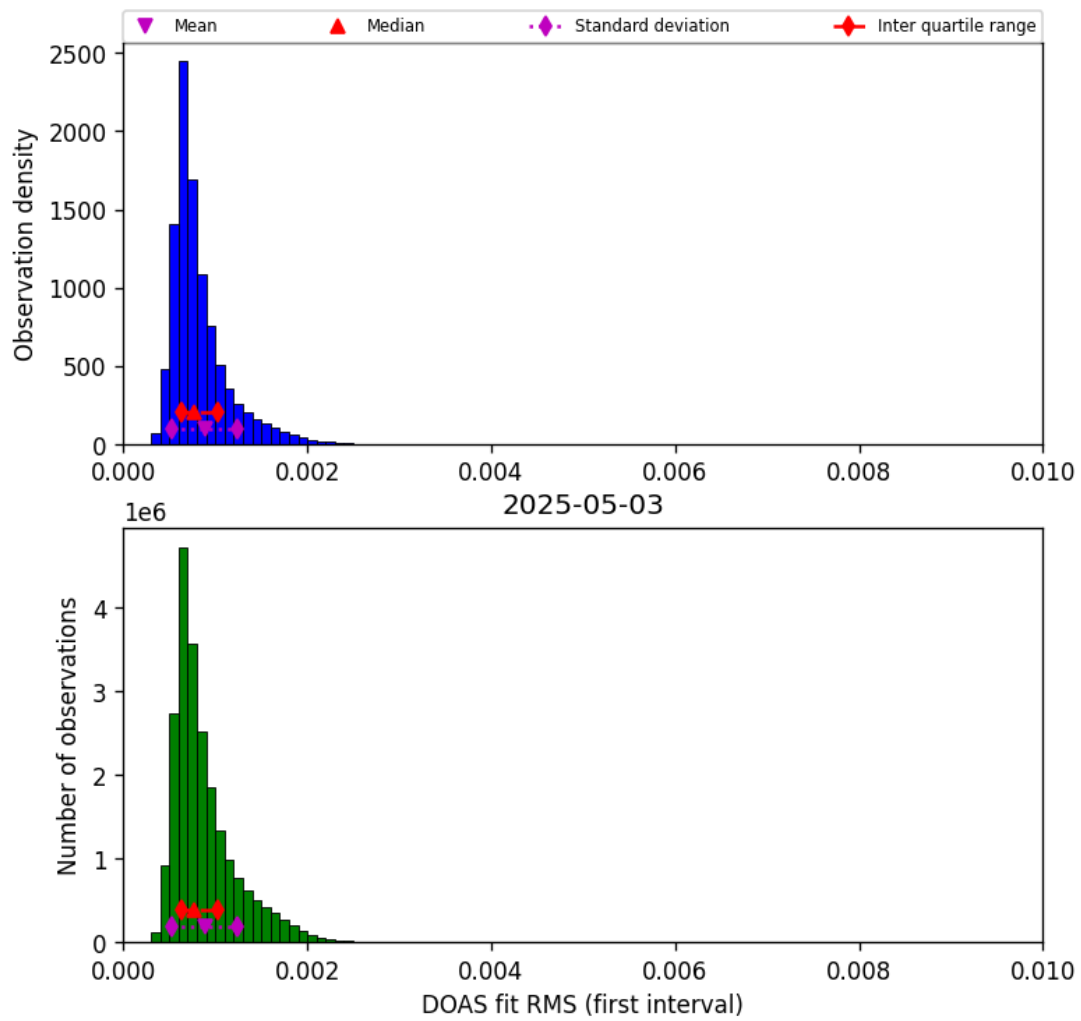
Figure 44: Histogram of “DOAS fit RMS (first interval)” for 2025-05-03 to 2025-05-03
