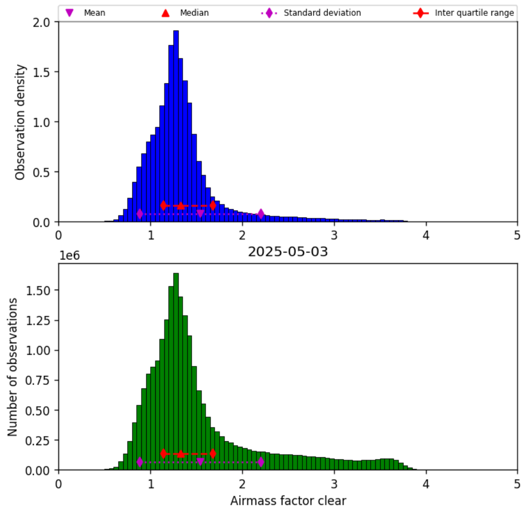
Figure 40: Histogram of “Airmass factor clear” for 2025-05-03 to 2025-05-03
