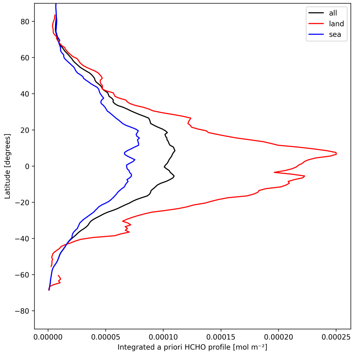
Figure 27: Zonal average of “Integrated a priori HCHO profile” for 2025-05-03 to 2025-05-03.
