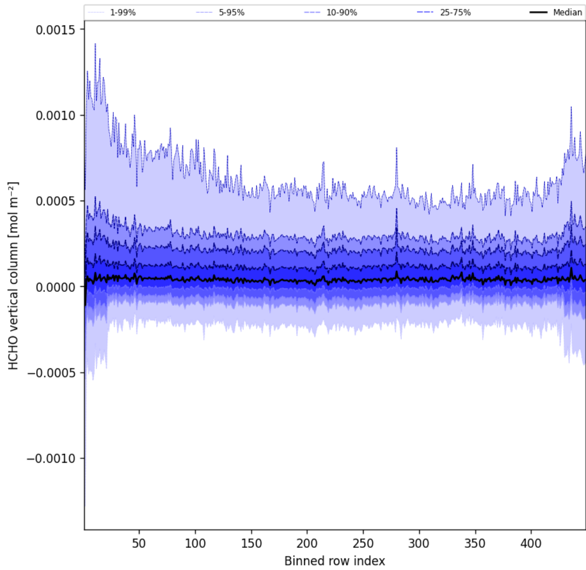
Figure 47: Along track statistics of “HCHO vertical column” for 2025-05-03 to 2025-05-03
