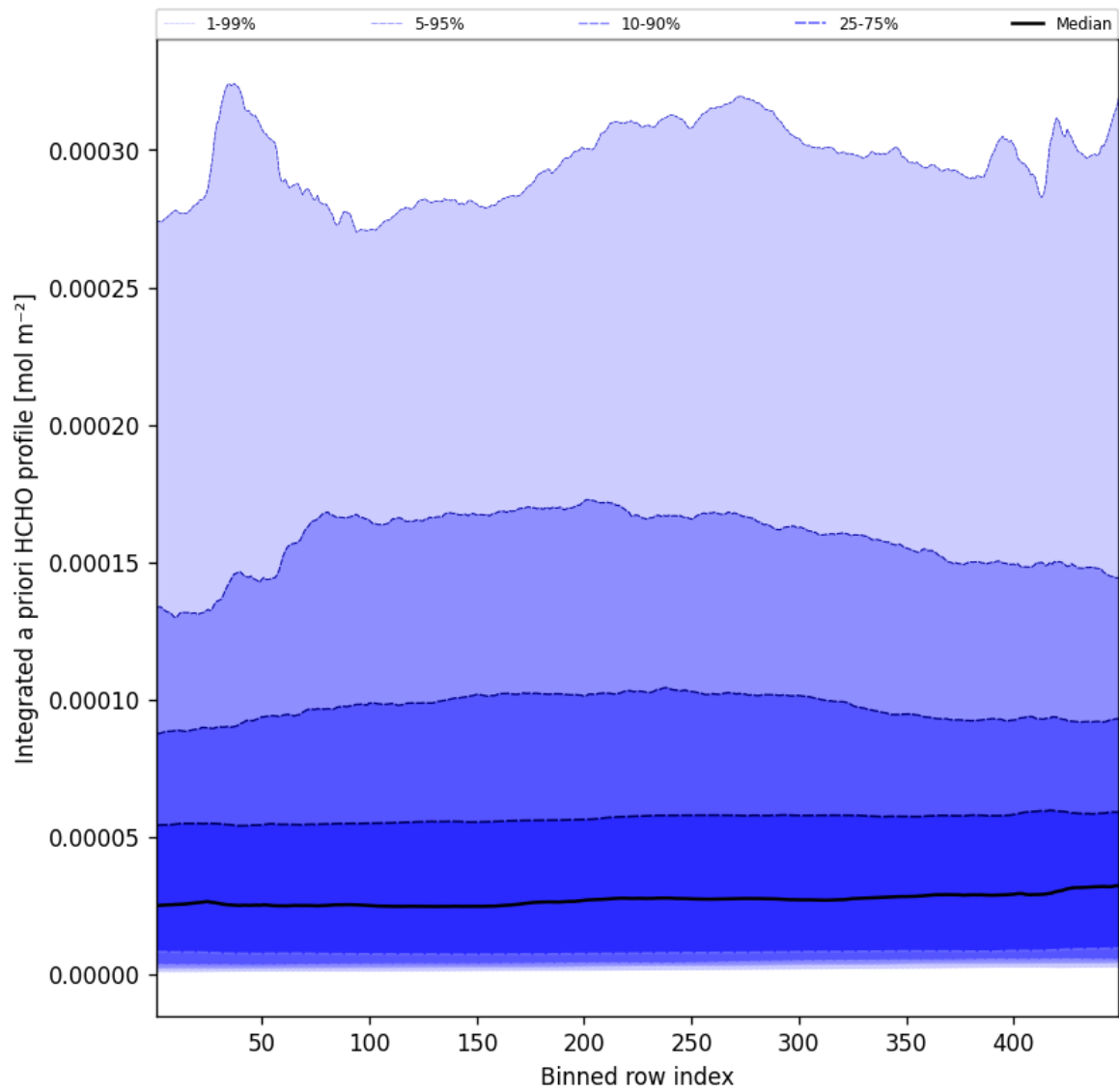
Figure 55: Along track statistics of “Integrated a priori HCHO profile” for 2025-05-03 to 2025-05-03
