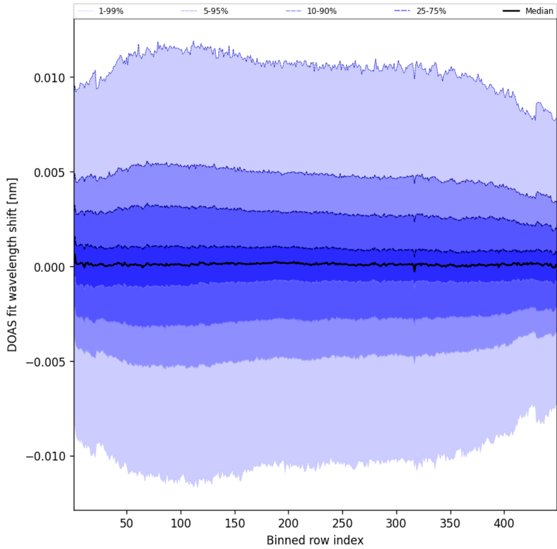
Figure 56: Along track statistics of “DOAS fit wavelength shift” for 2025-05-03 to 2025-05-03
