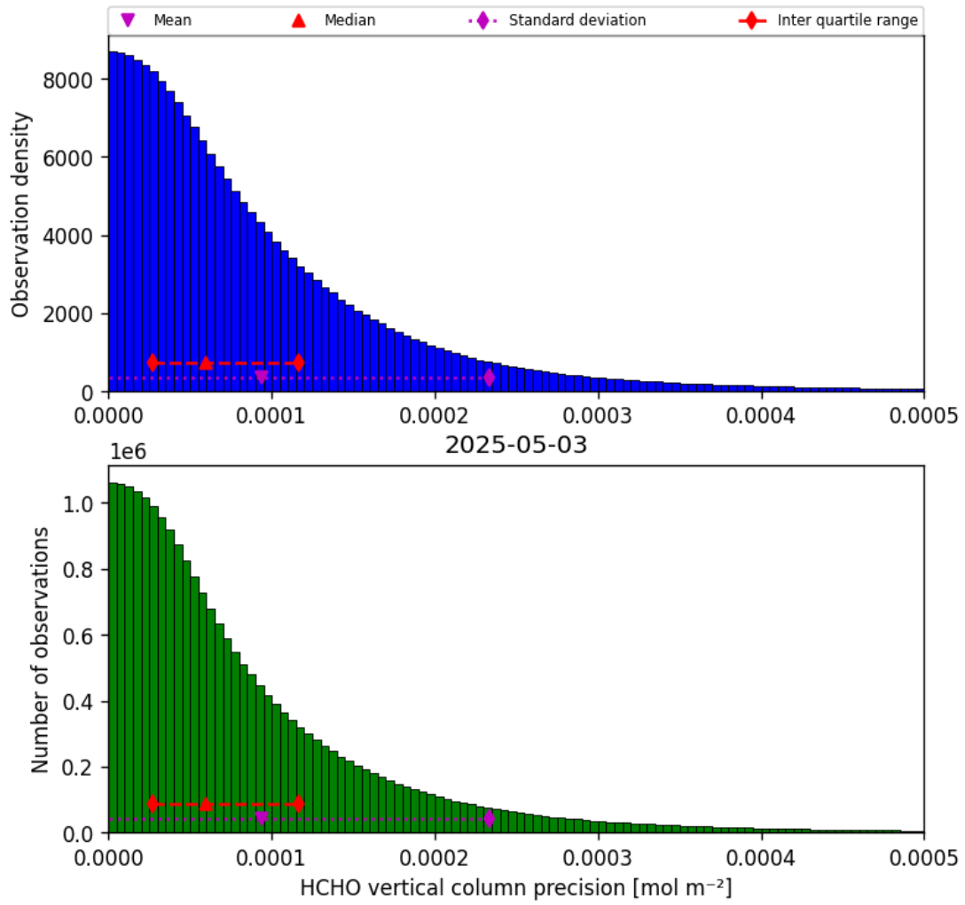
Figure 34: Histogram of “HCHO vertical column precision” for 2025-05-03 to 2025-05-03
