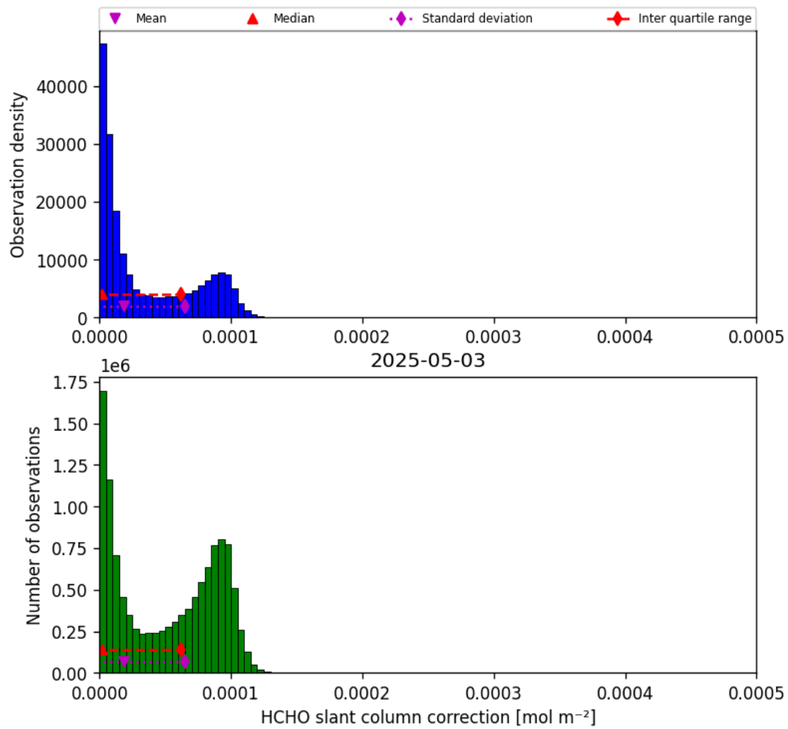
Figure 45: Histogram of “HCHO slant column correction” for 2025-05-03 to 2025-05-03
