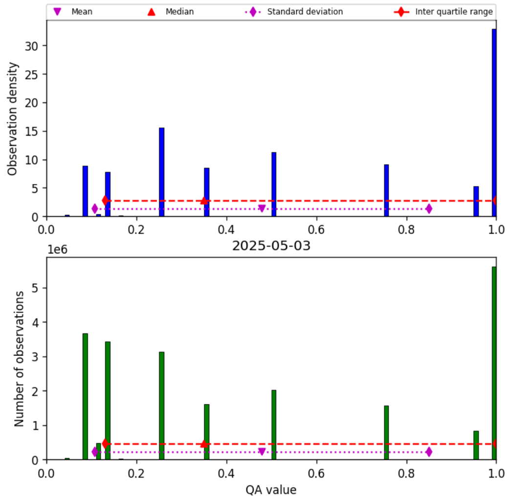
Figure 32: Histogram of “QA value” for 2025-05-03 to 2025-05-03
