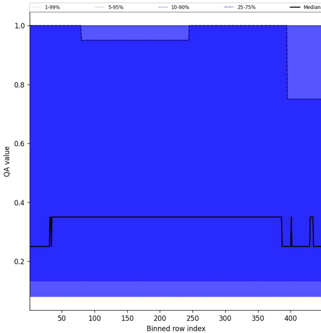
Figure 46: Along track statistics of “QA value” for 2025-05-03 to 2025-05-03
