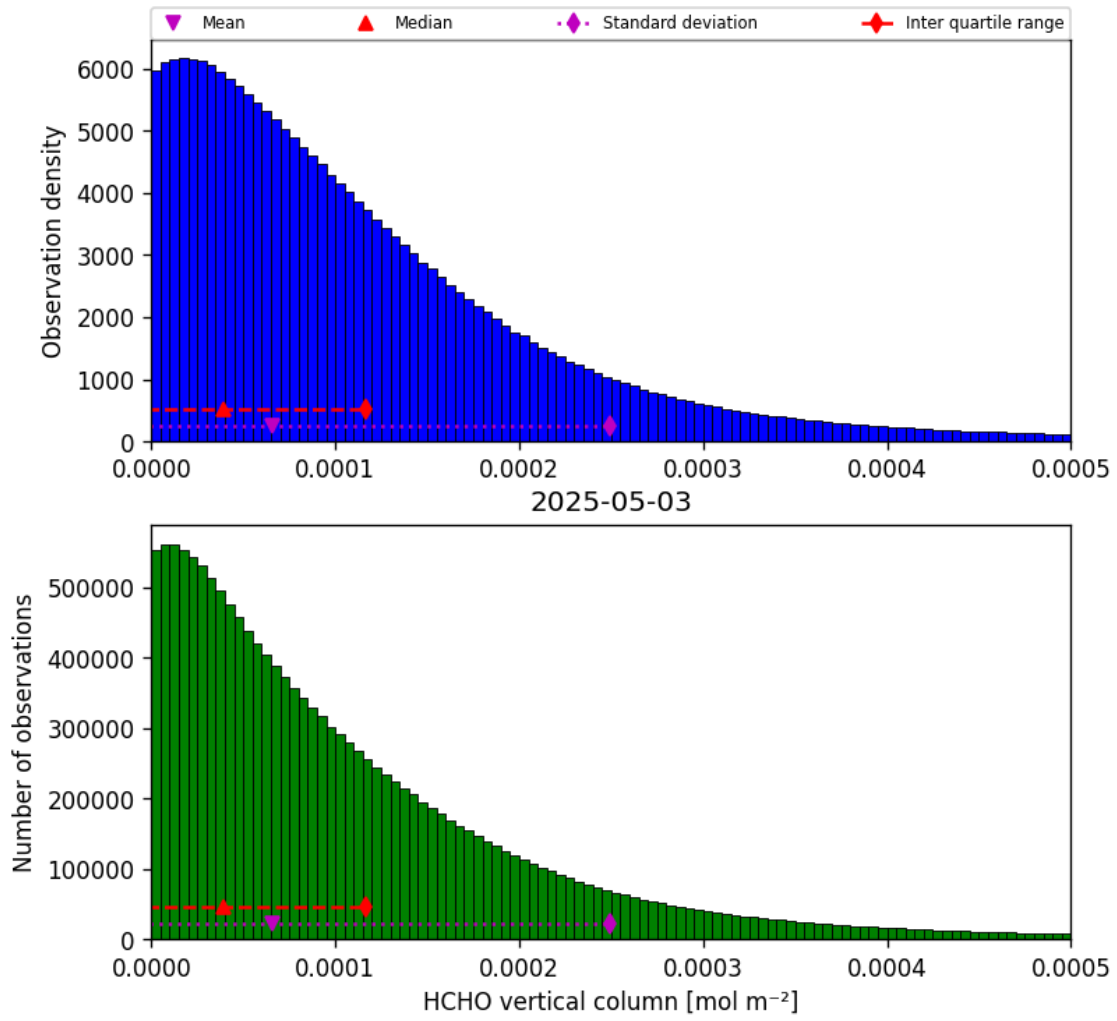
Figure 33: Histogram of “HCHO vertical column” for 2025-05-03 to 2025-05-03
