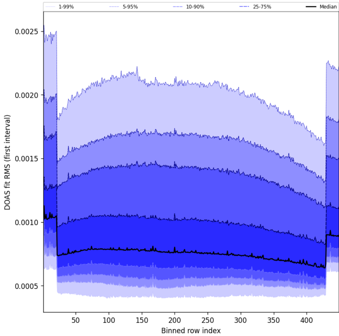
Figure 58: Along track statistics of “DOAS fit RMS (first interval)” for 2025-05-03 to 2025-05-03
