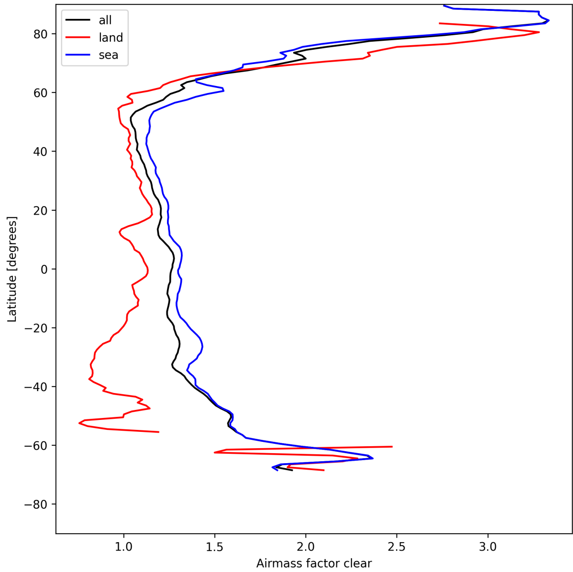
Figure 26: Zonal average of “Airmass factor clear” for 2025-05-03 to 2025-05-03.
