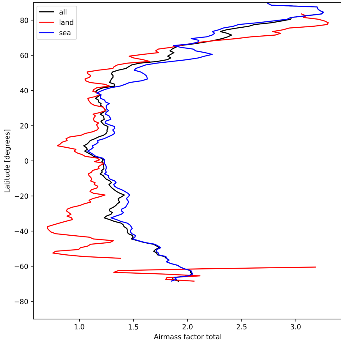
Figure 24: Zonal average of “Airmass factor total” for 2025-05-03 to 2025-05-03.
