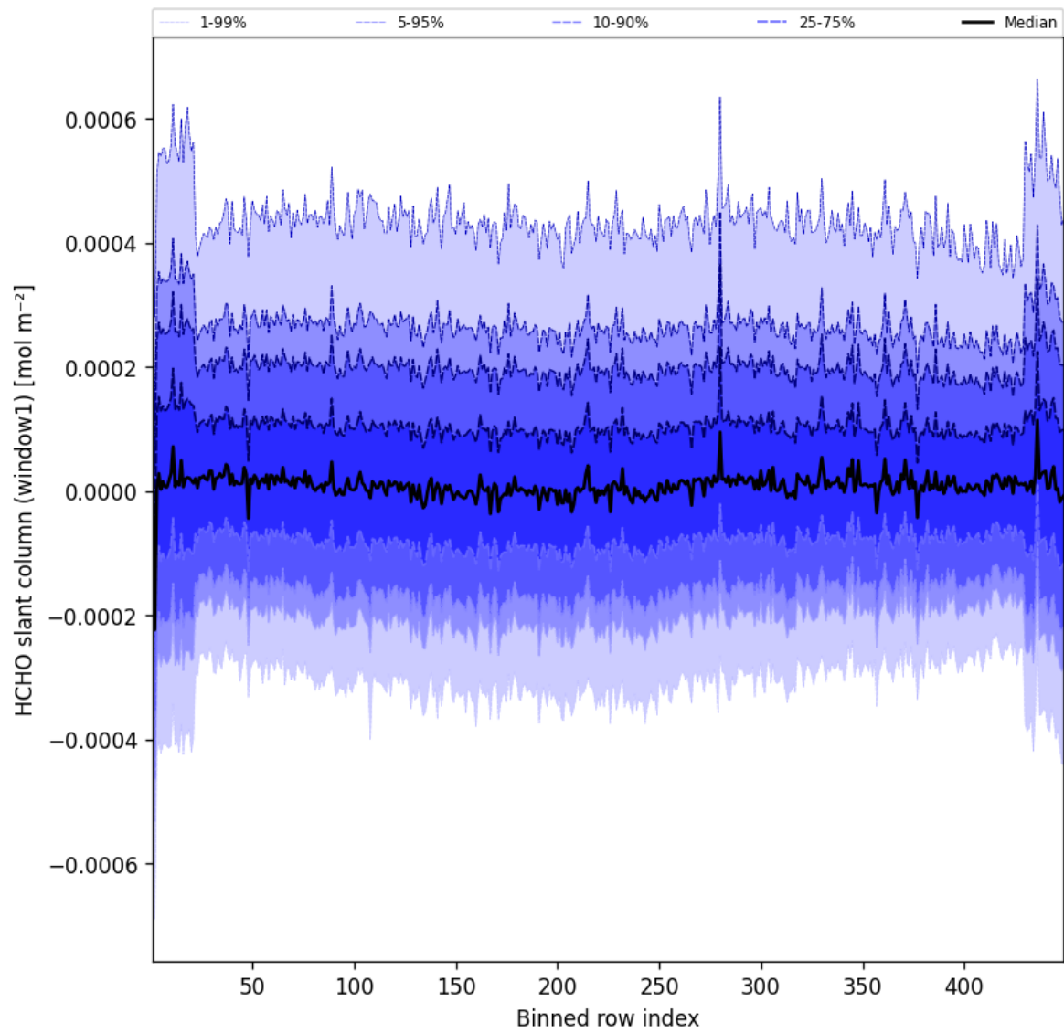
Figure 50: Along track statistics of “HCHO slant column (window1)” for 2025-05-03 to 2025-05-03
