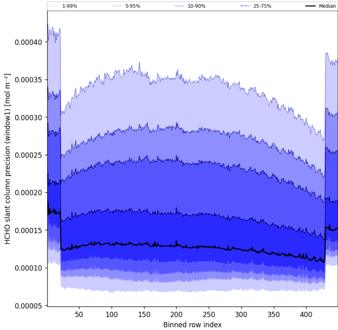
Figure 51: Along track statistics of “HCHO slant column precision (window1)” for 2025-05-03 to 2025-05-03
