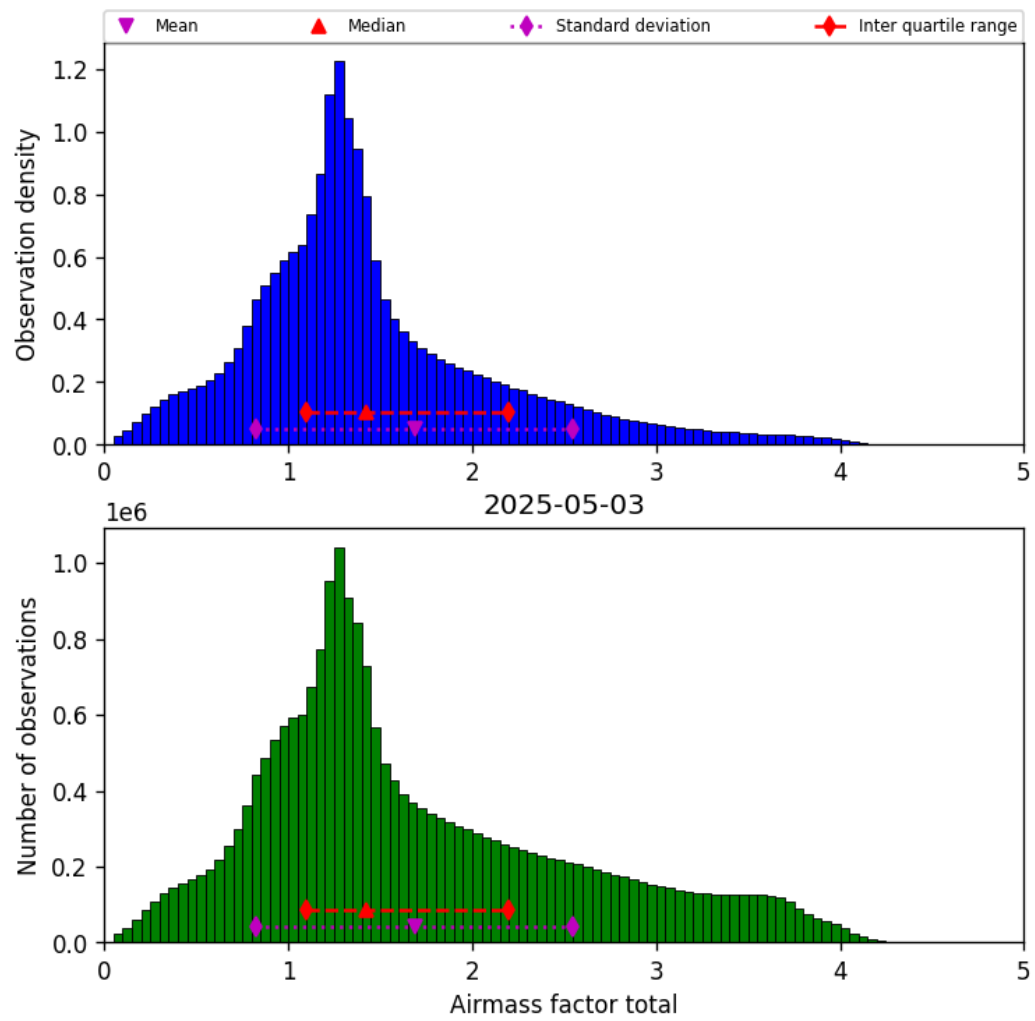
Figure 38: Histogram of “Airmass factor total” for 2025-05-03 to 2025-05-03
