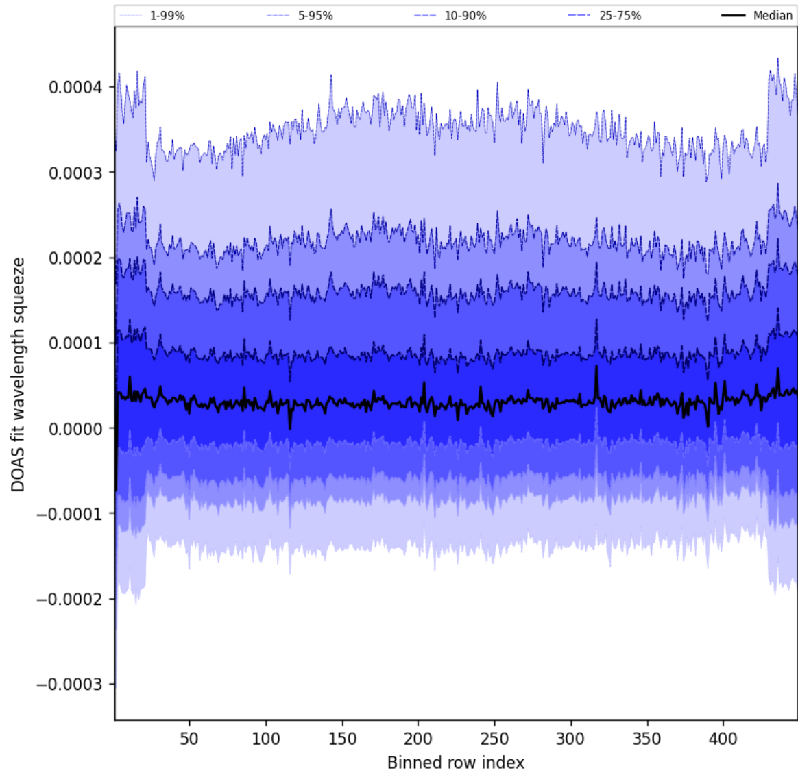
Figure 57: Along track statistics of “DOAS fit wavelength squeeze” for 2025-05-03 to 2025-05-03
