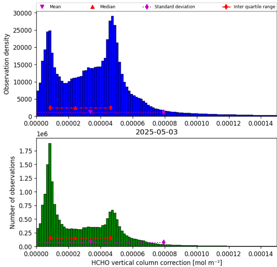
Figure 35: Histogram of “HCHO vertical column correction” for 2025-05-03 to 2025-05-03
