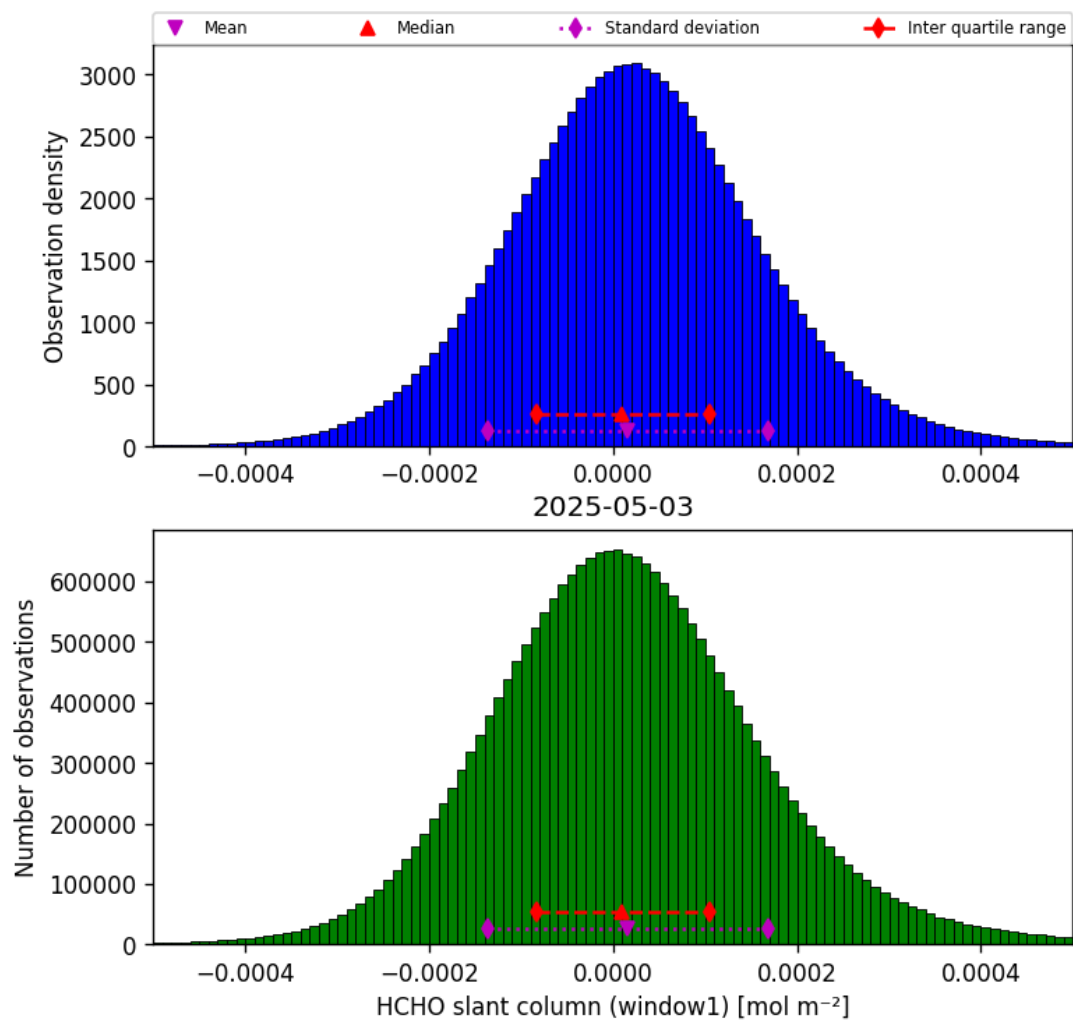
Figure 36: Histogram of “HCHO slant column (window1)” for 2025-05-03 to 2025-05-03
