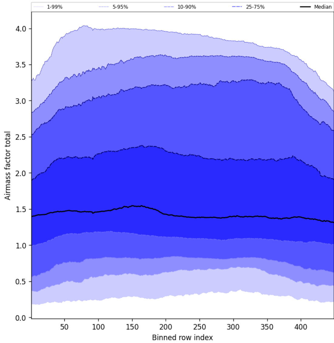
Figure 52: Along track statistics of “Airmass factor total” for 2025-05-03 to 2025-05-03
