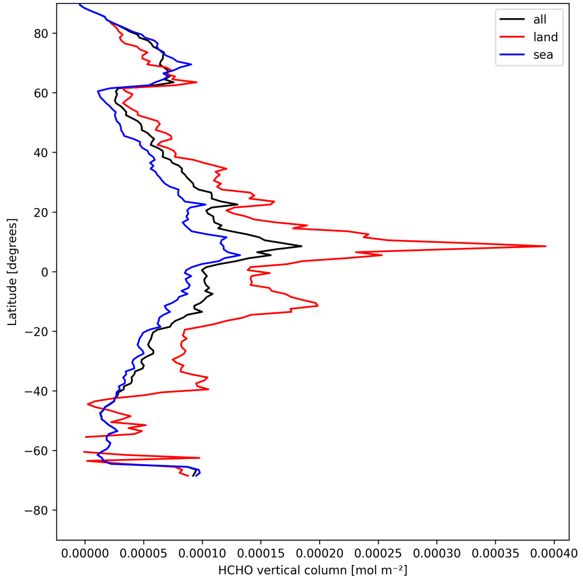
Figure 19: Zonal average of “HCHO vertical column” for 2025-05-03 to 2025-05-03.
