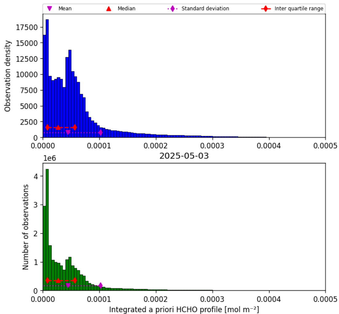
Figure 41: Histogram of “Integrated a priori HCHO profile” for 2025-05-03 to 2025-05-03
