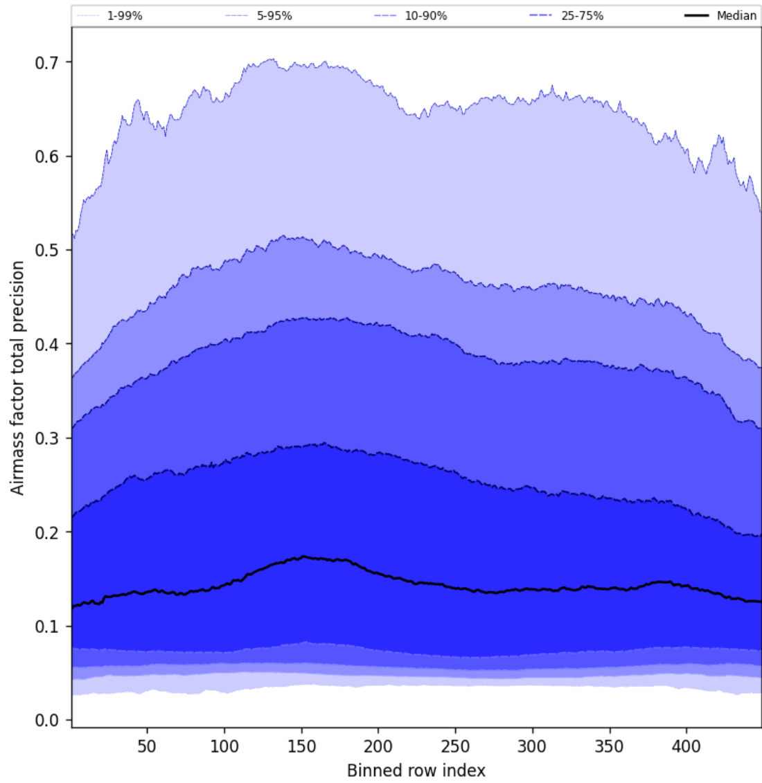
Figure 53: Along track statistics of “Airmass factor total precision” for 2025-05-03 to 2025-05-03
