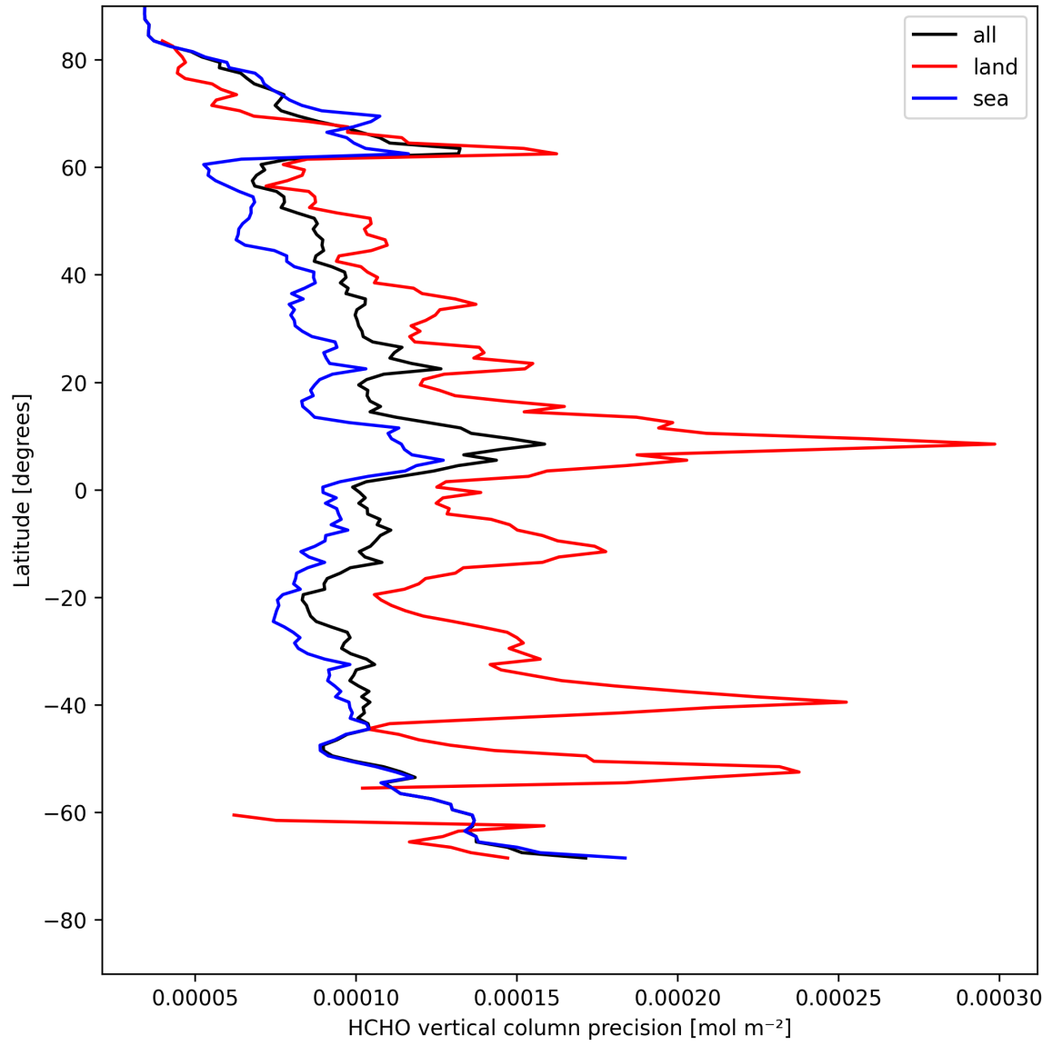
Figure 20: Zonal average of “HCHO vertical column precision” for 2025-05-03 to 2025-05-03.
