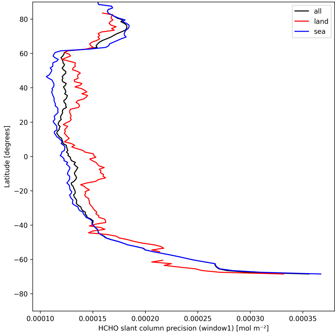
Figure 23: Zonal average of "HCHO slant column precision (window1)" for 2025-05-03 to 2025-05-03.
