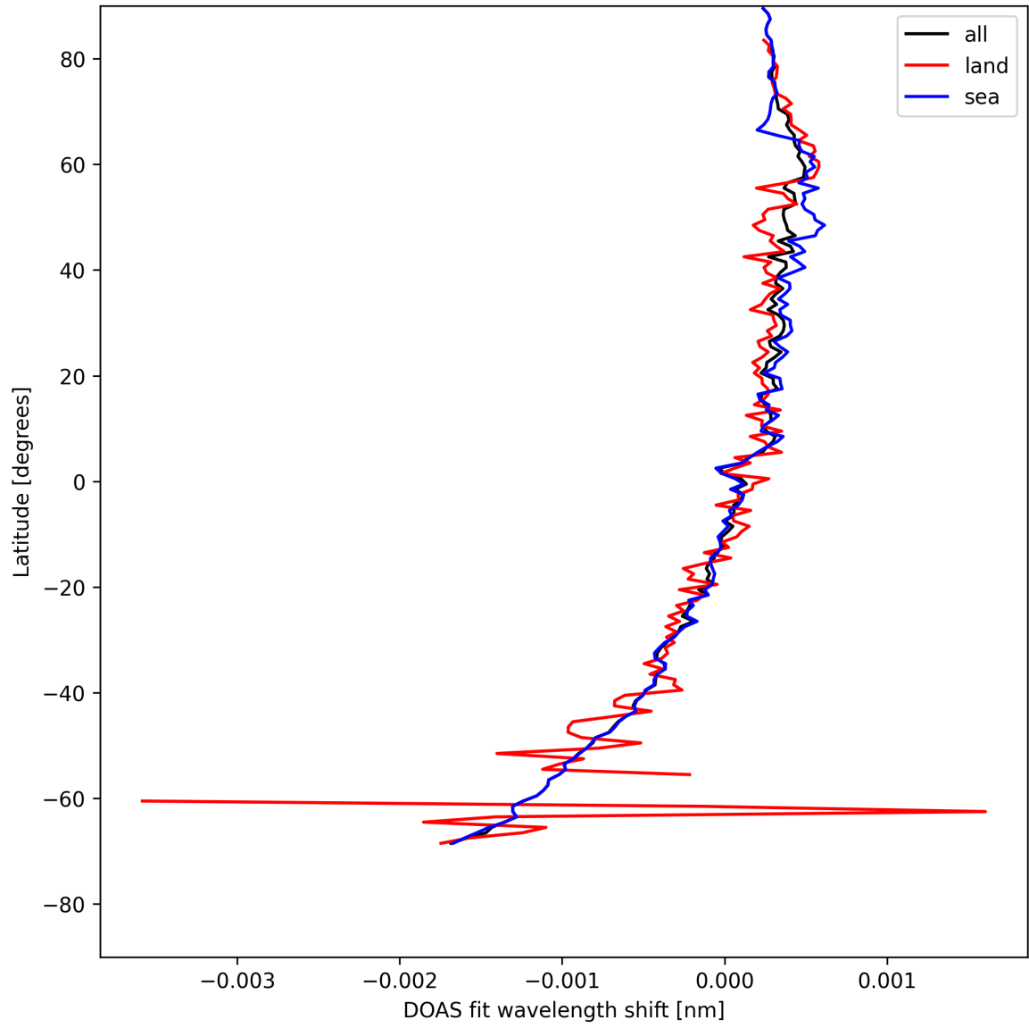
Figure 28: Zonal average of "DOAS fit wavelength shift" for 2025-05-03 to 2025-05-03.
