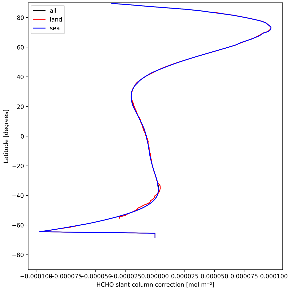
Figure 31: Zonal average of “HCHO slant column correction” for 2025-05-03 to 2025-05-03.
