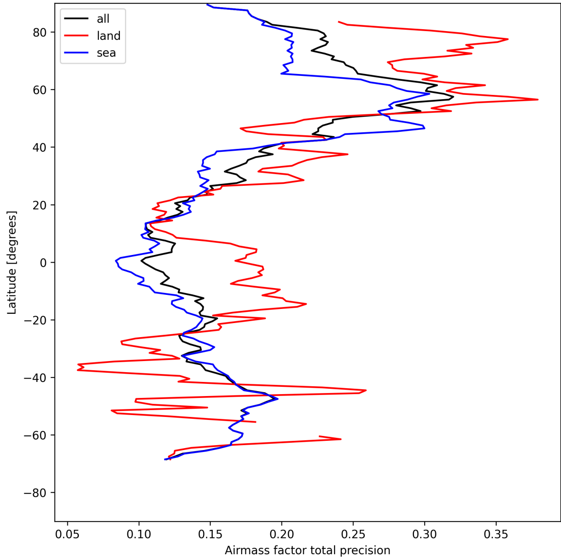
Figure 25: Zonal average of “Airmass factor total precision” for 2025-05-03 to 2025-05-03.
