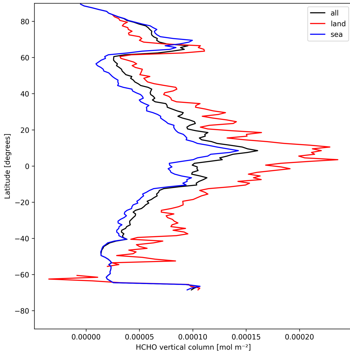
Figure 19: Zonal average of “HCHO vertical column” for 2025-05-04 to 2025-05-05.
