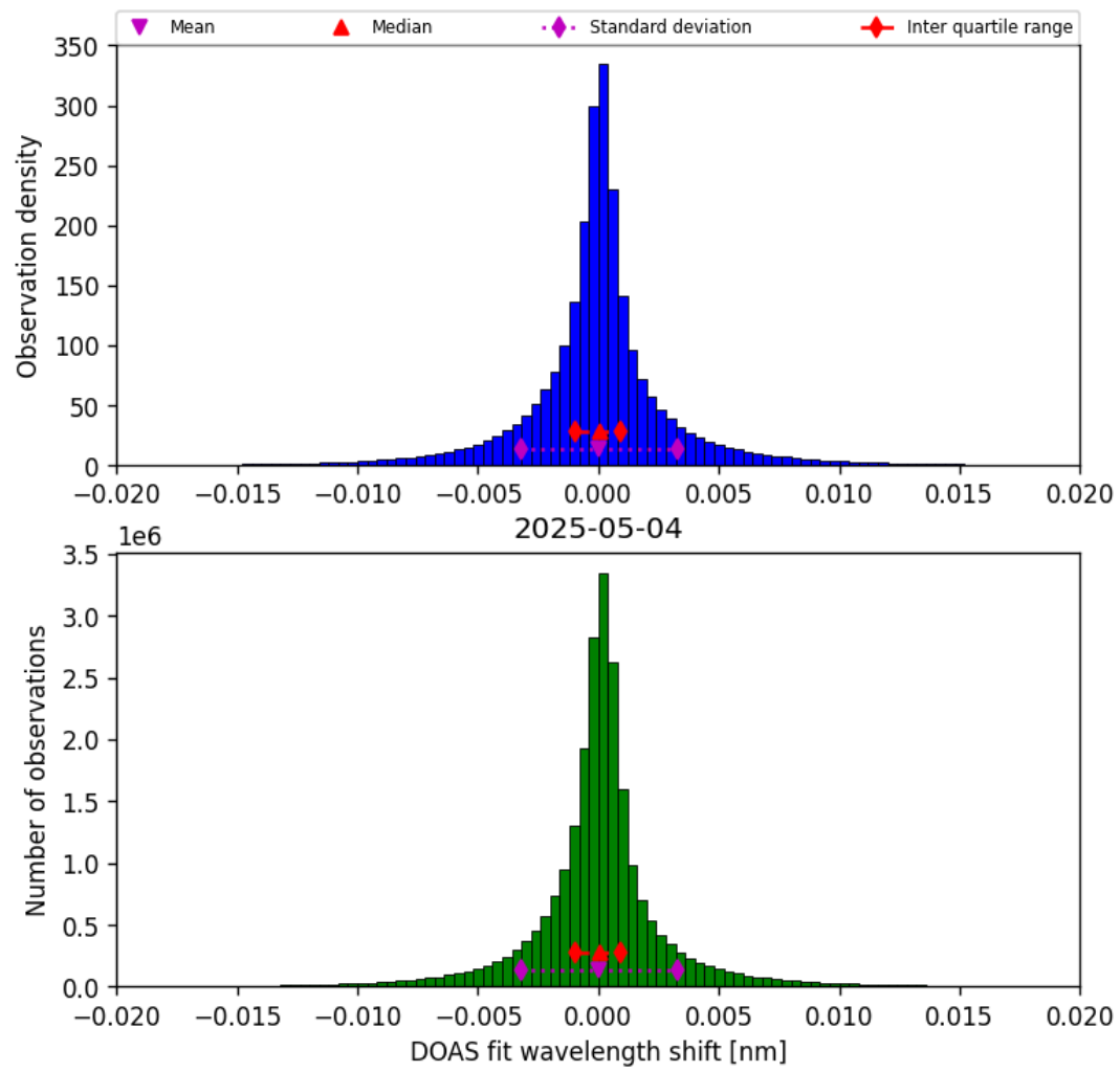
Figure 42: Histogram of “DOAS fit wavelength shift” for 2025-05-04 to 2025-05-05
