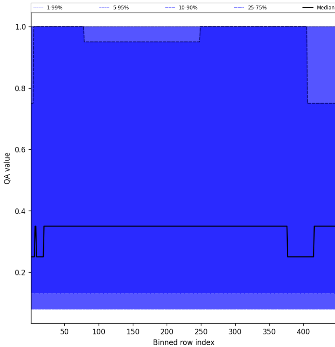
Figure 46: Along track statistics of “QA value” for 2025-05-04 to 2025-05-05
