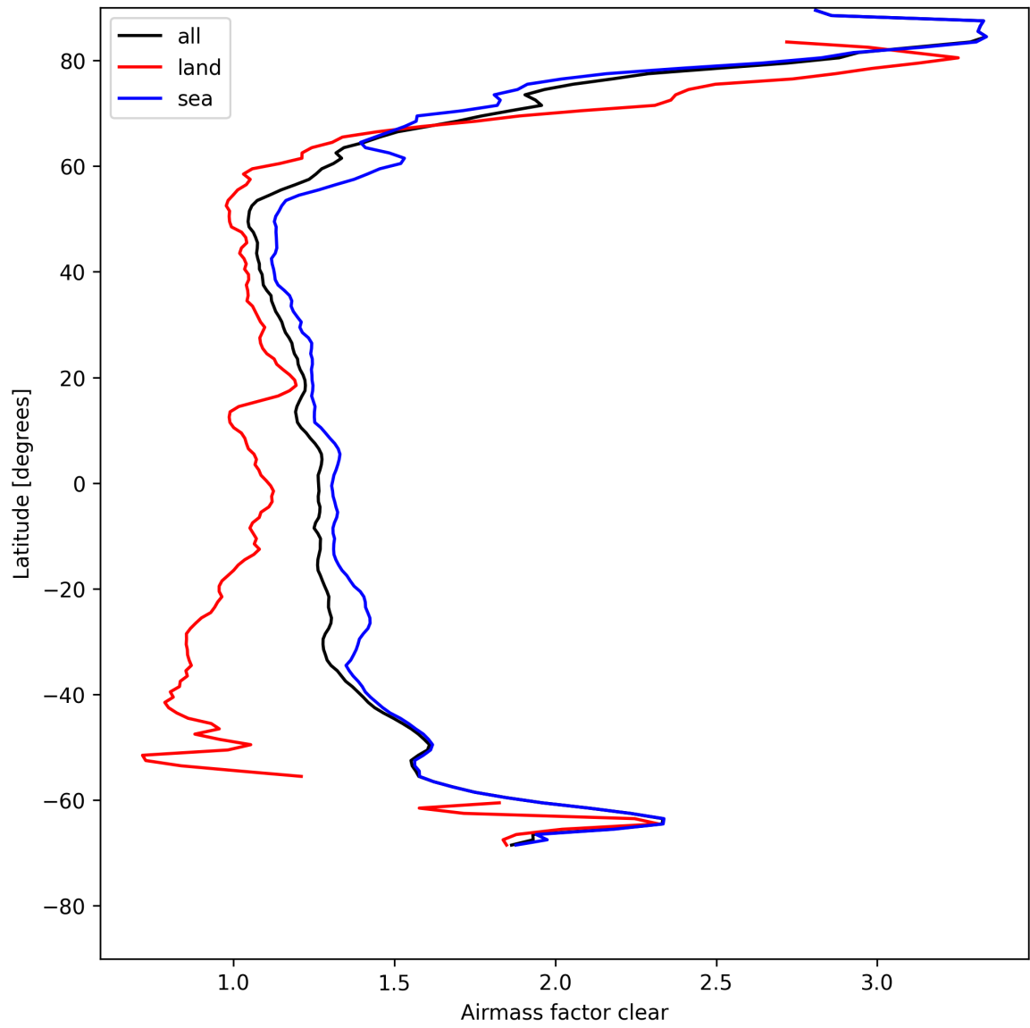
Figure 26: Zonal average of “Airmass factor clear” for 2025-05-04 to 2025-05-05.
