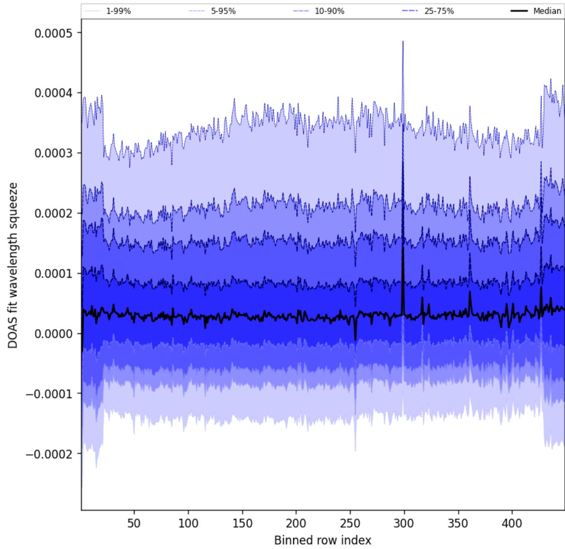
Figure 57: Along track statistics of “DOAS fit wavelength squeeze” for 2025-05-04 to 2025-05-05
