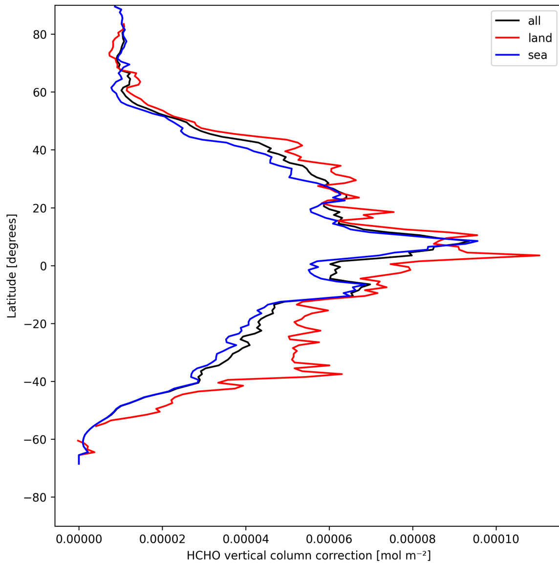
Figure 21: Zonal average of “HCHO vertical column correction” for 2025-05-04 to 2025-05-05.
