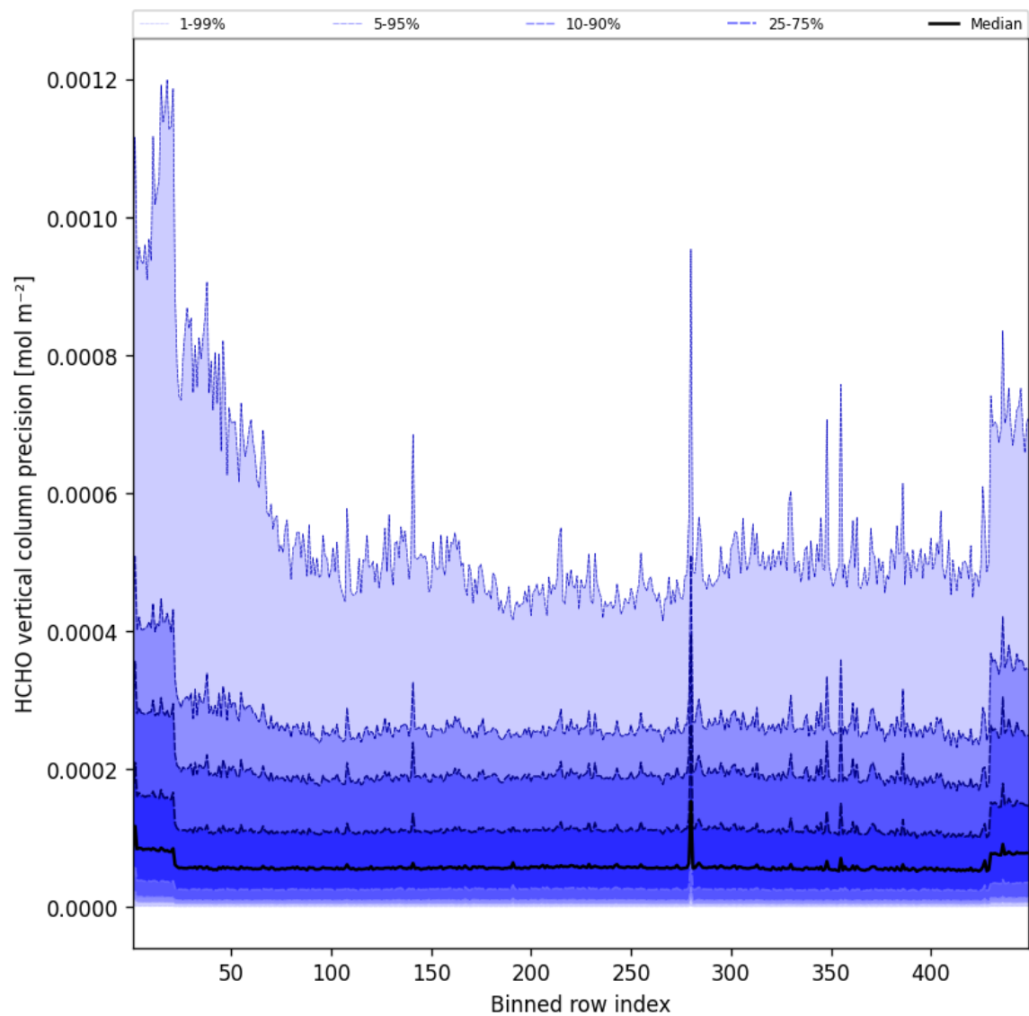
Figure 48: Along track statistics of “HCHO vertical column precision” for 2025-05-04 to 2025-05-05
