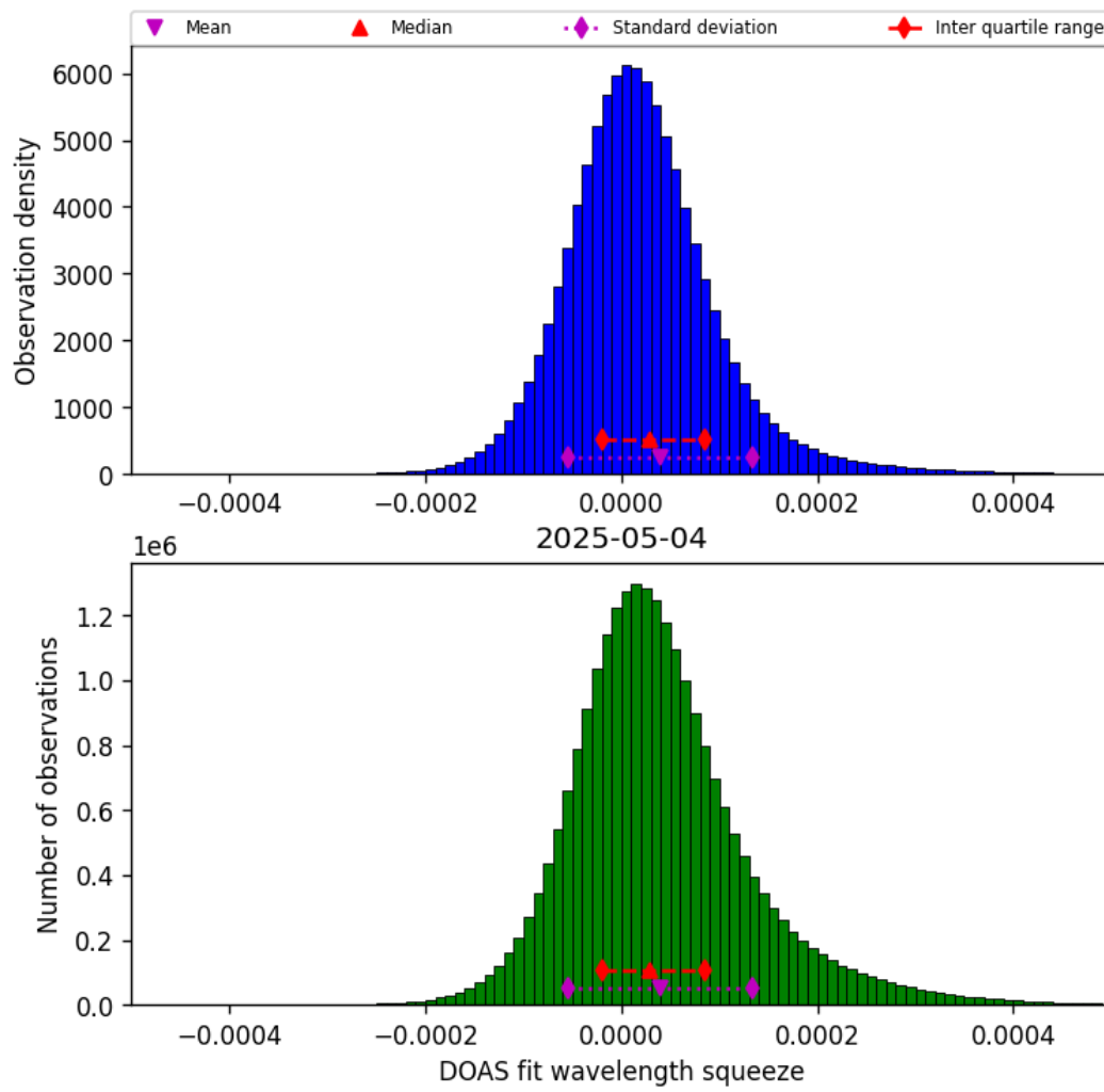
Figure 43: Histogram of “DOAS fit wavelength squeeze” for 2025-05-04 to 2025-05-05
