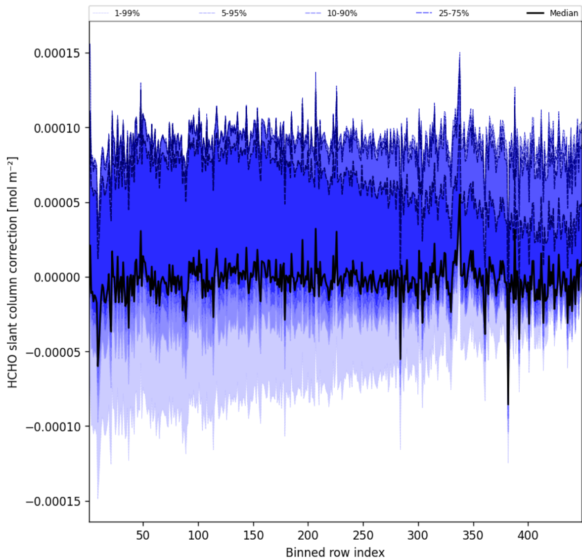
Figure 59: Along track statistics of “HCHO slant column correction” for 2025-05-04 to 2025-05-05
