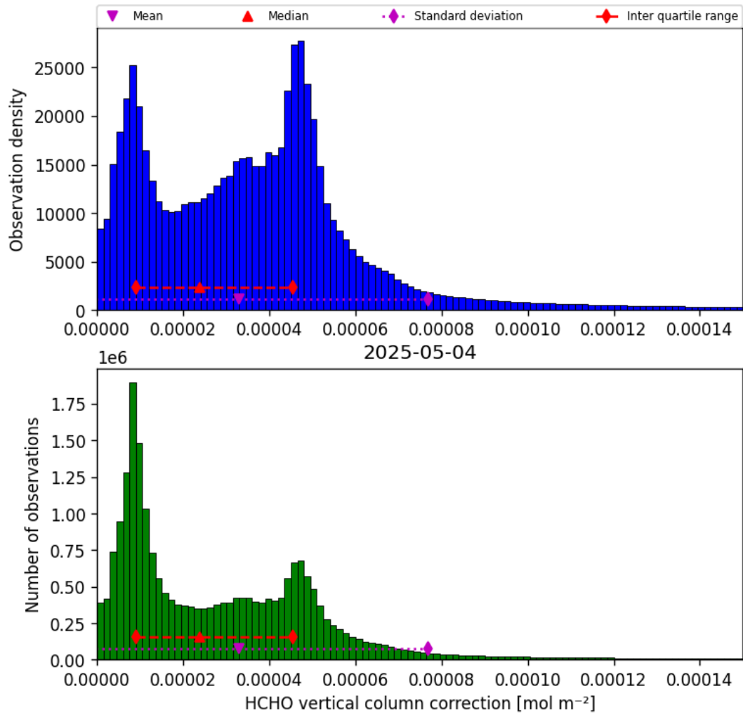
Figure 35: Histogram of “HCHO vertical column correction” for 2025-05-04 to 2025-05-05
