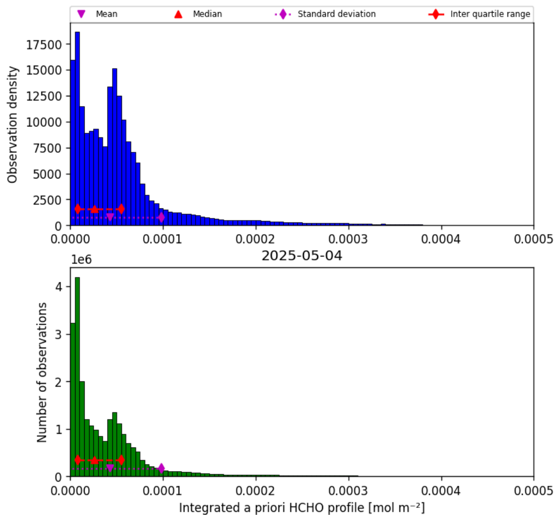
Figure 41: Histogram of “Integrated a priori HCHO profile” for 2025-05-04 to 2025-05-05
