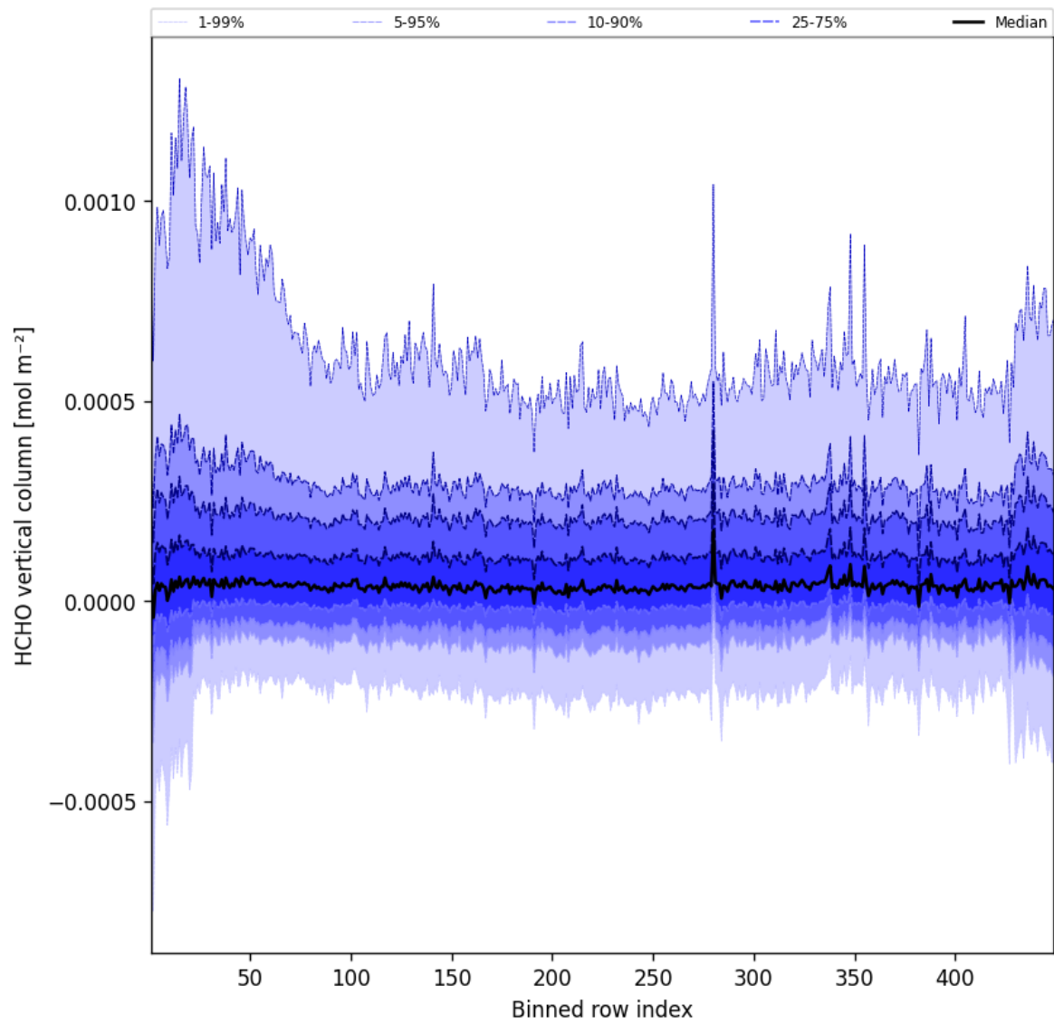
Figure 47: Along track statistics of “HCHO vertical column” for 2025-05-04 to 2025-05-05
