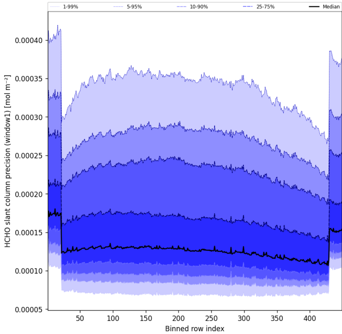
Figure 51: Along track statistics of “HCHO slant column precision (window1)” for 2025-05-04 to 2025-05-05
