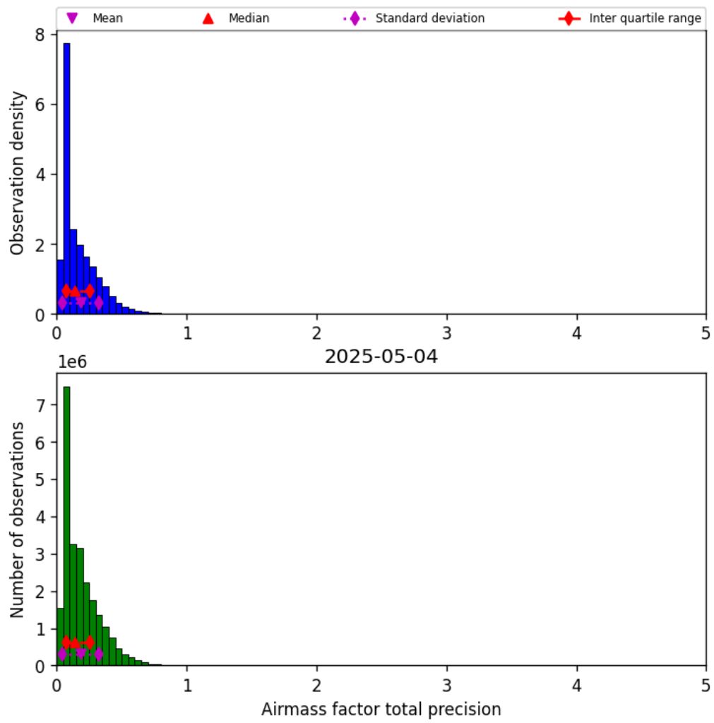
Figure 39: Histogram of “Airmass factor total precision” for 2025-05-04 to 2025-05-05
