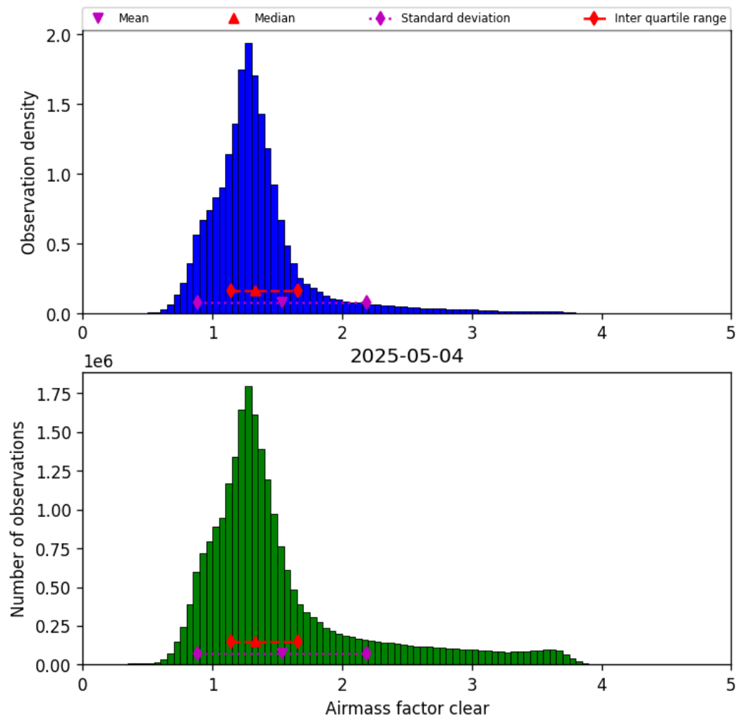
Figure 40: Histogram of “Airmass factor clear” for 2025-05-04 to 2025-05-05
