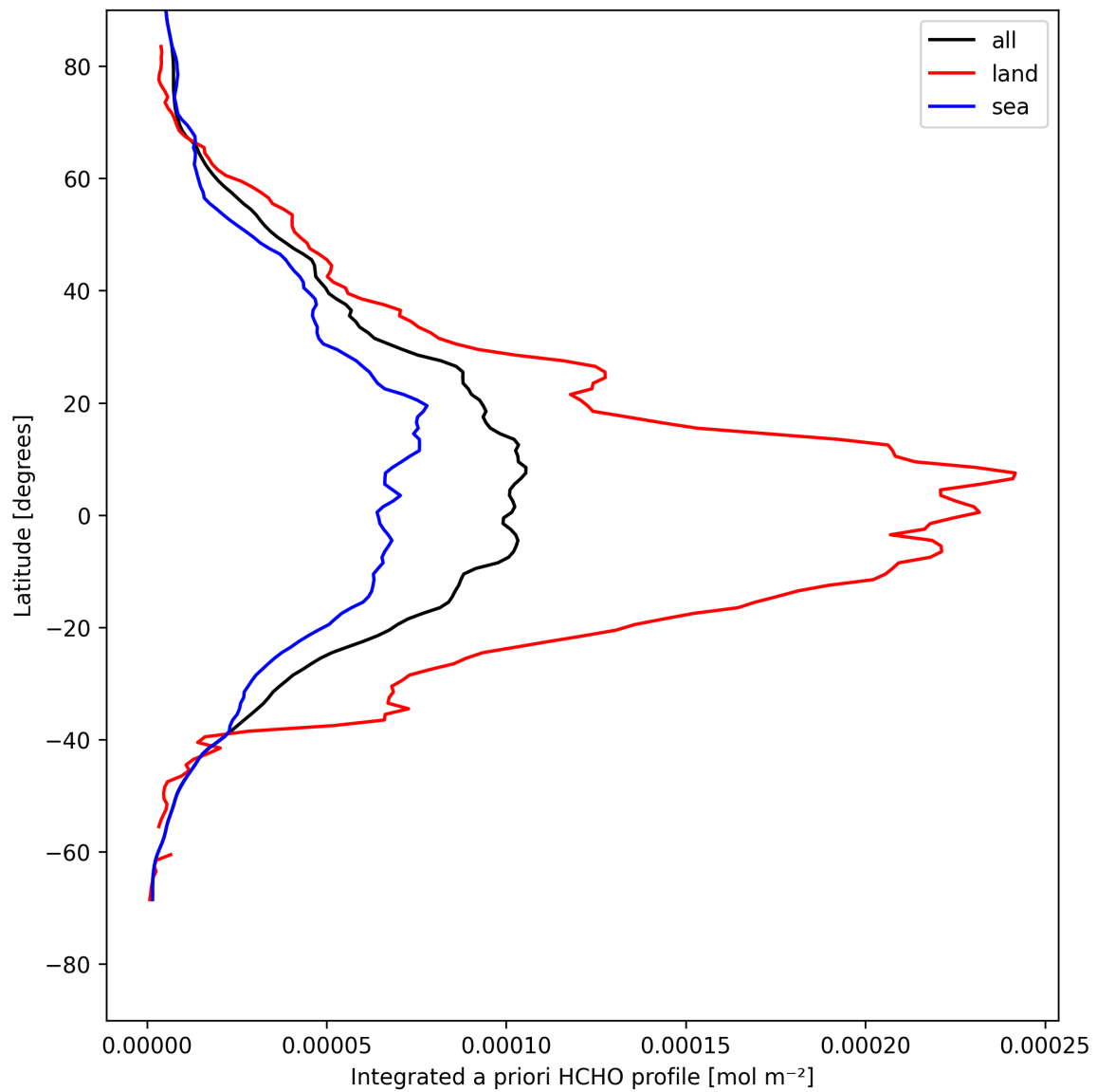
Figure 27: Zonal average of “Integrated a priori HCHO profile” for 2025-05-04 to 2025-05-05.
