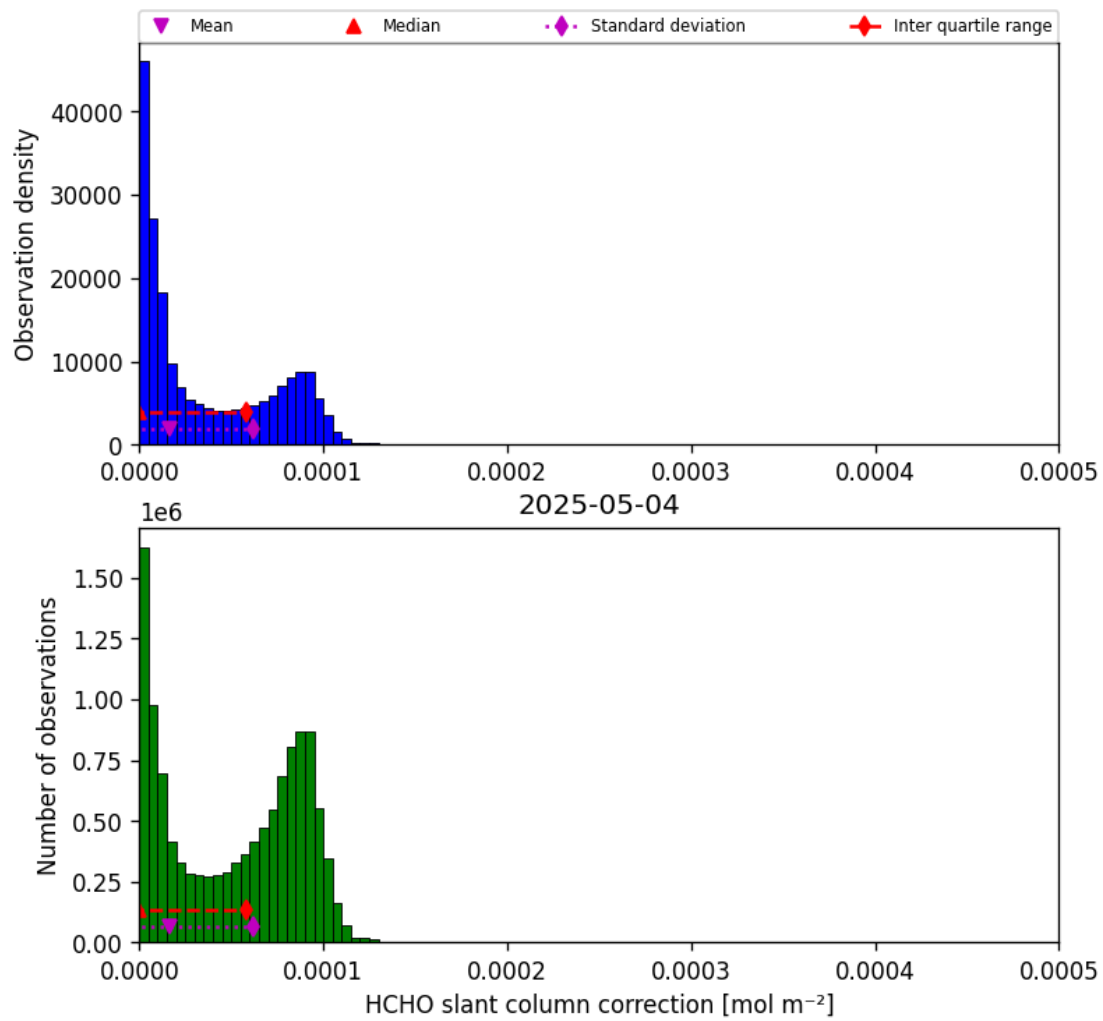
Figure 45: Histogram of “HCHO slant column correction” for 2025-05-04 to 2025-05-05
