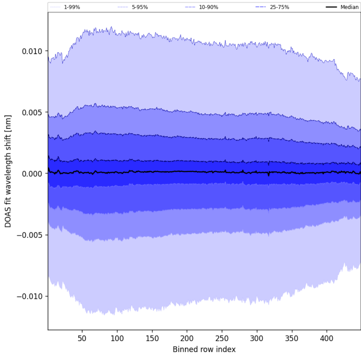
Figure 56: Along track statistics of “DOAS fit wavelength shift” for 2025-05-04 to 2025-05-05
