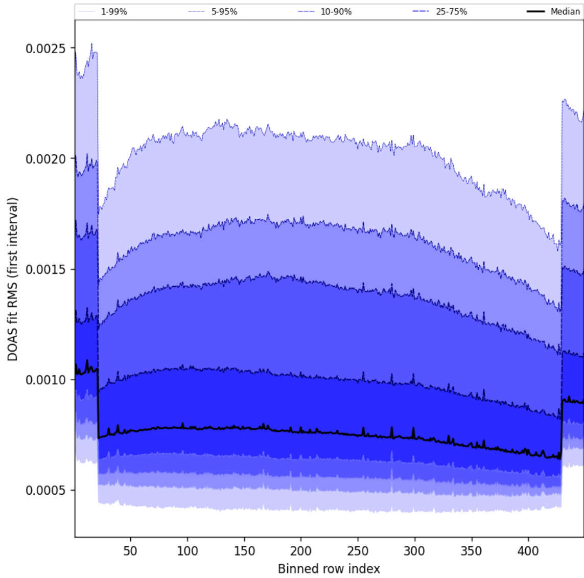
Figure 58: Along track statistics of “DOAS fit RMS (first interval)” for 2025-05-04 to 2025-05-05
