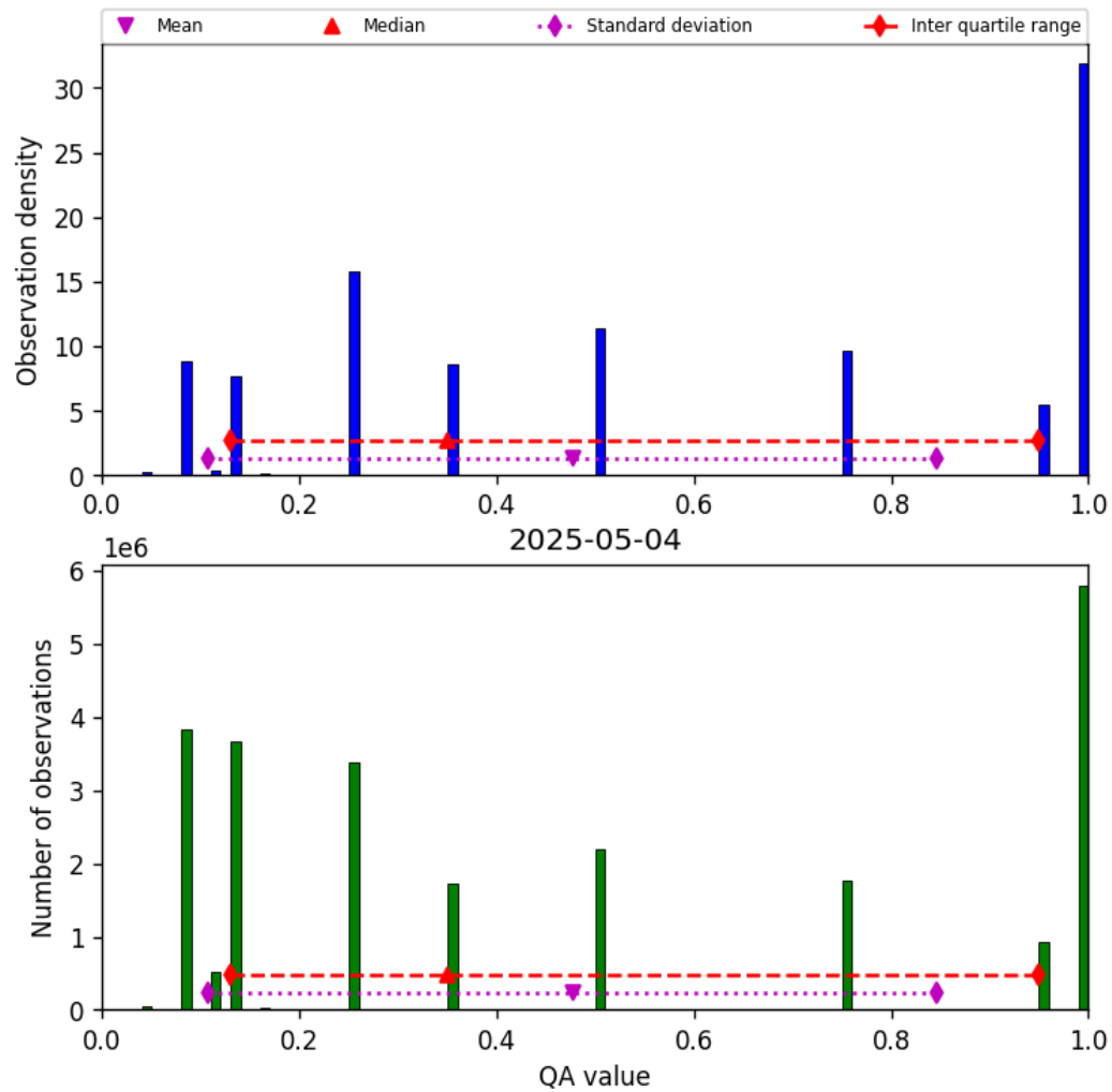
Figure 32: Histogram of “QA value” for 2025-05-04 to 2025-05-05
