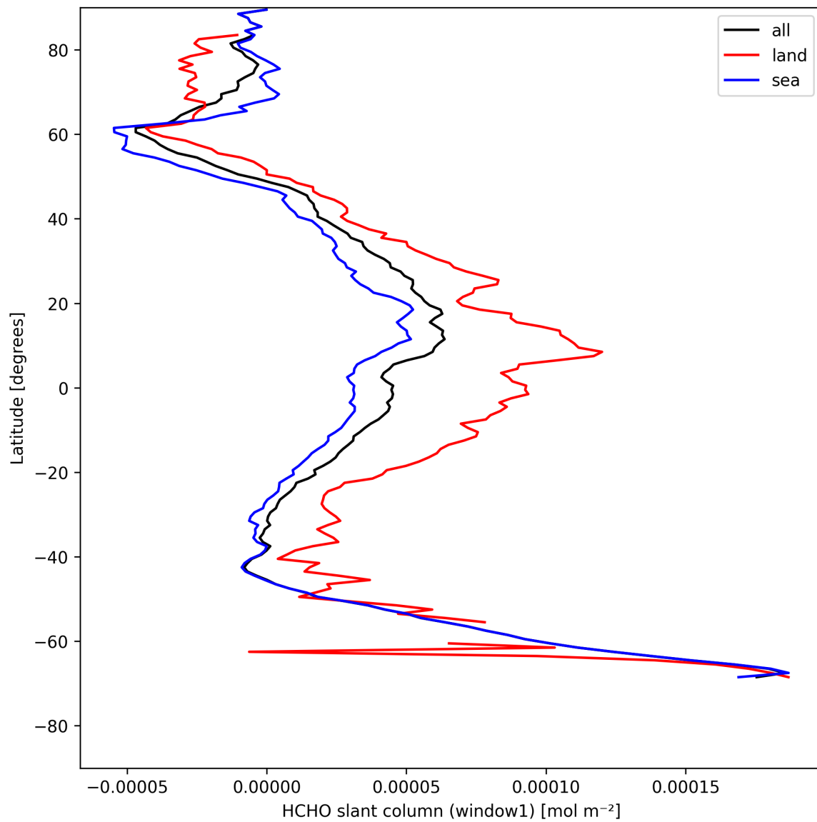
Figure 22: Zonal average of “HCHO slant column (window1)” for 2025-05-04 to 2025-05-05.
