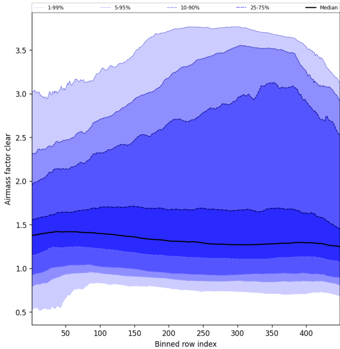
Figure 54: Along track statistics of “Airmass factor clear” for 2025-05-04 to 2025-05-05
