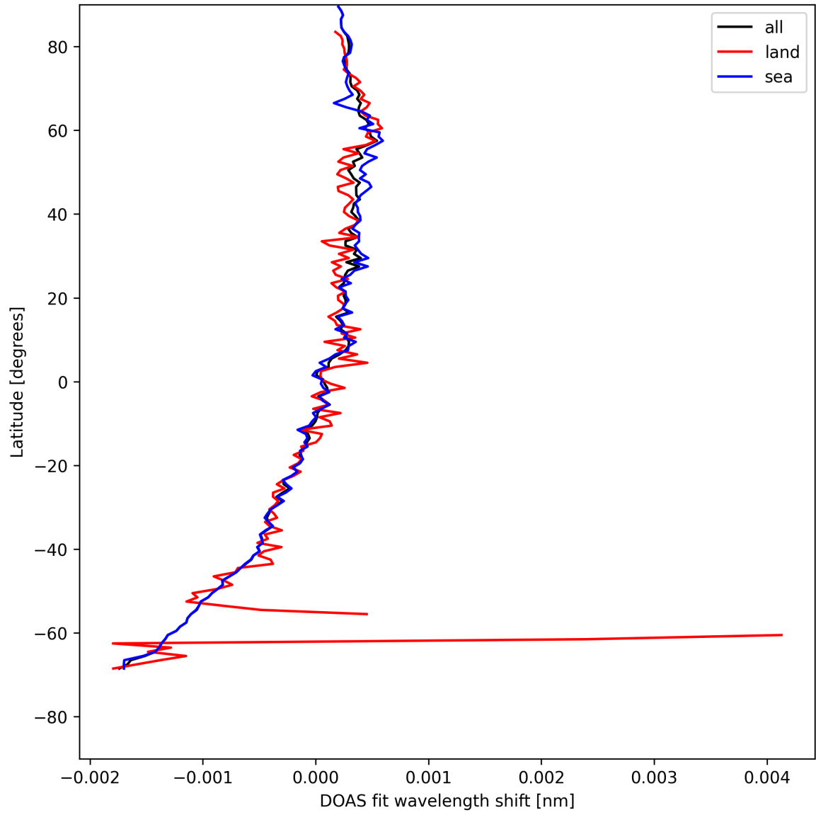
Figure 28: Zonal average of “DOAS fit wavelength shift” for 2025-05-04 to 2025-05-05.
