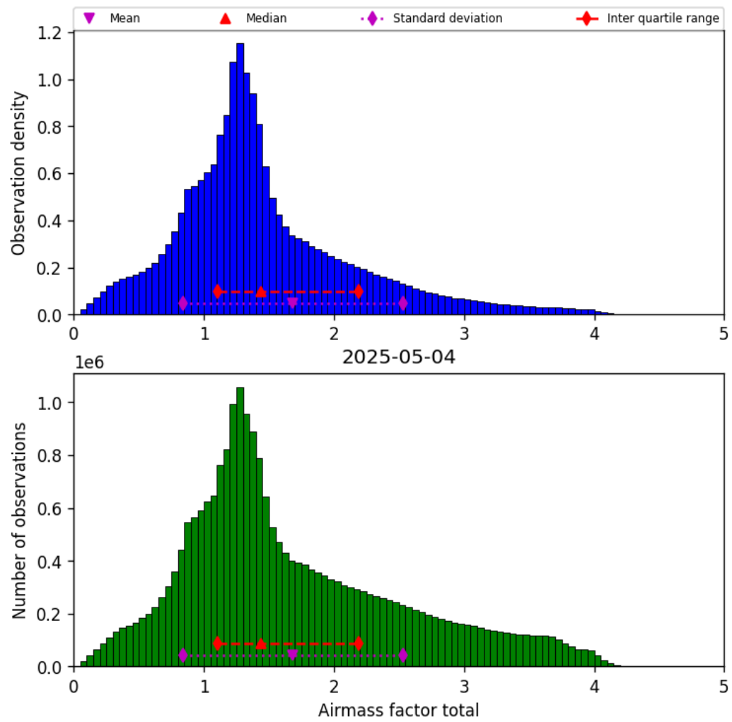
Figure 38: Histogram of “Airmass factor total” for 2025-05-04 to 2025-05-05
