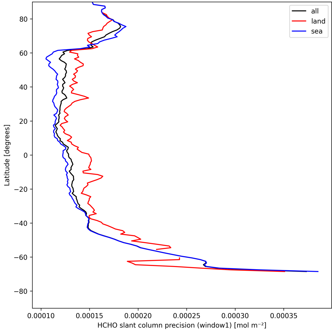
Figure 23: Zonal average of “HCHO slant column precision (window1)” for 2025-05-04 to 2025-05-05.
