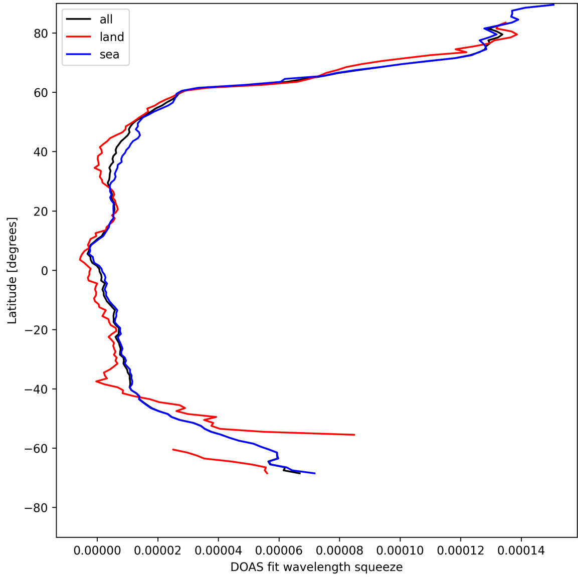
Figure 29: Zonal average of “DOAS fit wavelength squeeze” for 2025-05-04 to 2025-05-05.
