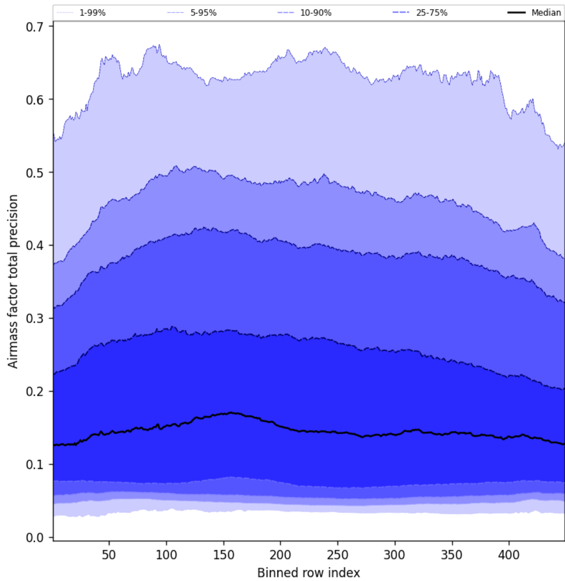
Figure 53: Along track statistics of “Airmass factor total precision” for 2025-05-04 to 2025-05-05
