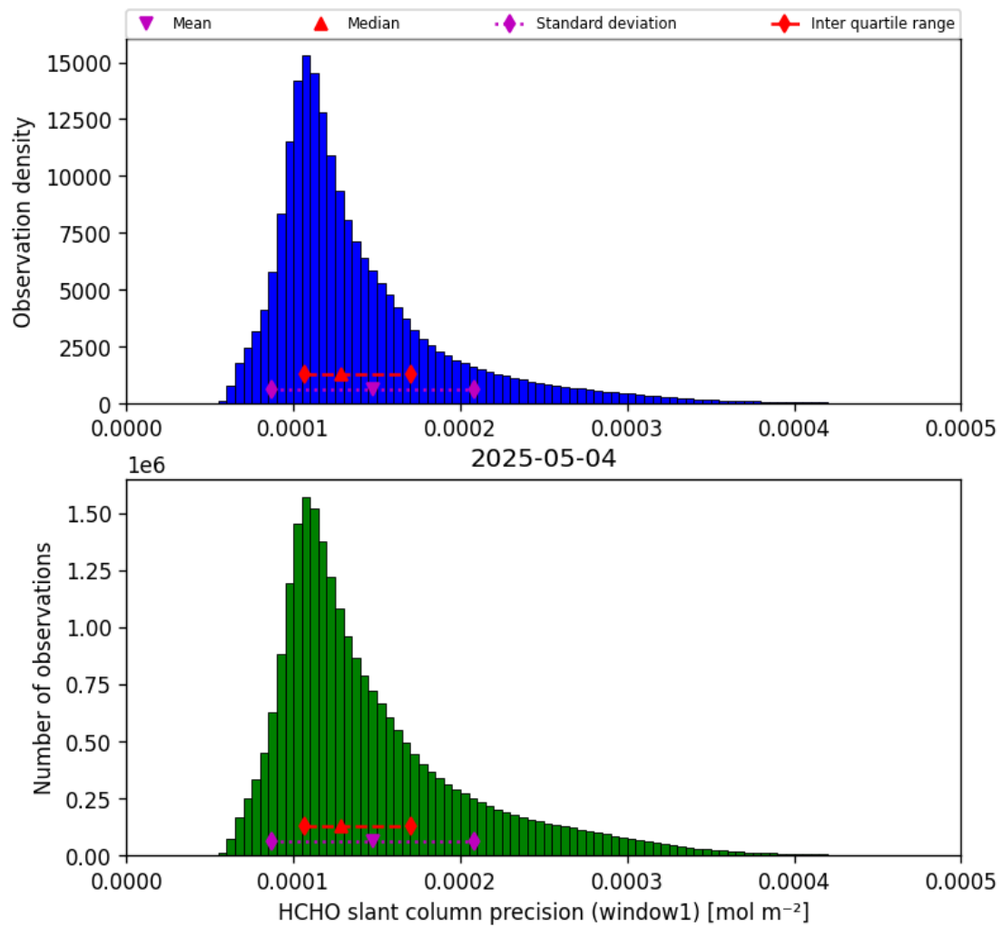
Figure 37: Histogram of “HCHO slant column precision (window1)” for 2025-05-04 to 2025-05-05
