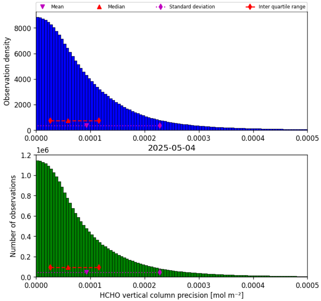
Figure 34: Histogram of “HCHO vertical column precision” for 2025-05-04 to 2025-05-05
