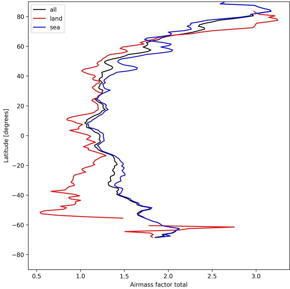
Figure 24: Zonal average of “Airmass factor total” for 2025-05-04 to 2025-05-05.
