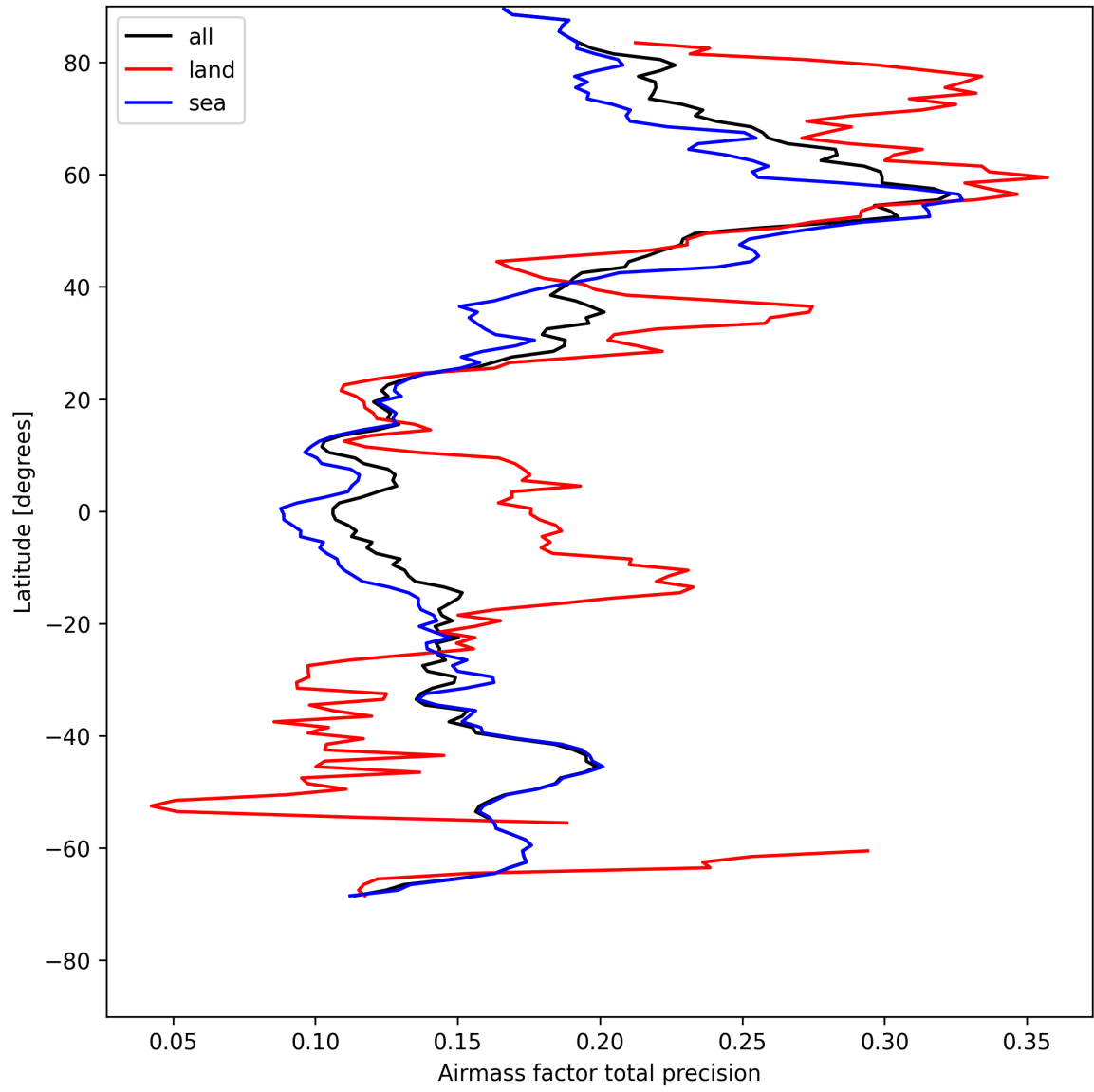
Figure 25: Zonal average of “Airmass factor total precision” for 2025-05-04 to 2025-05-05.
