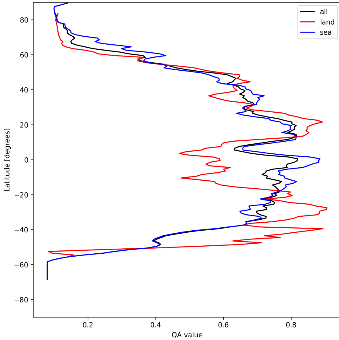
Figure 18: Zonal average of “QA value” for 2025-05-04 to 2025-05-05.
