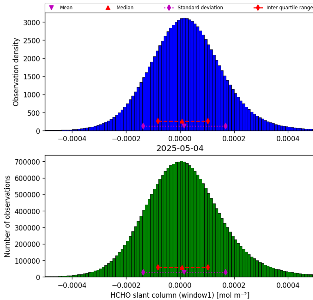
Figure 36: Histogram of “HCHO slant column (window1)” for 2025-05-04 to 2025-05-05
