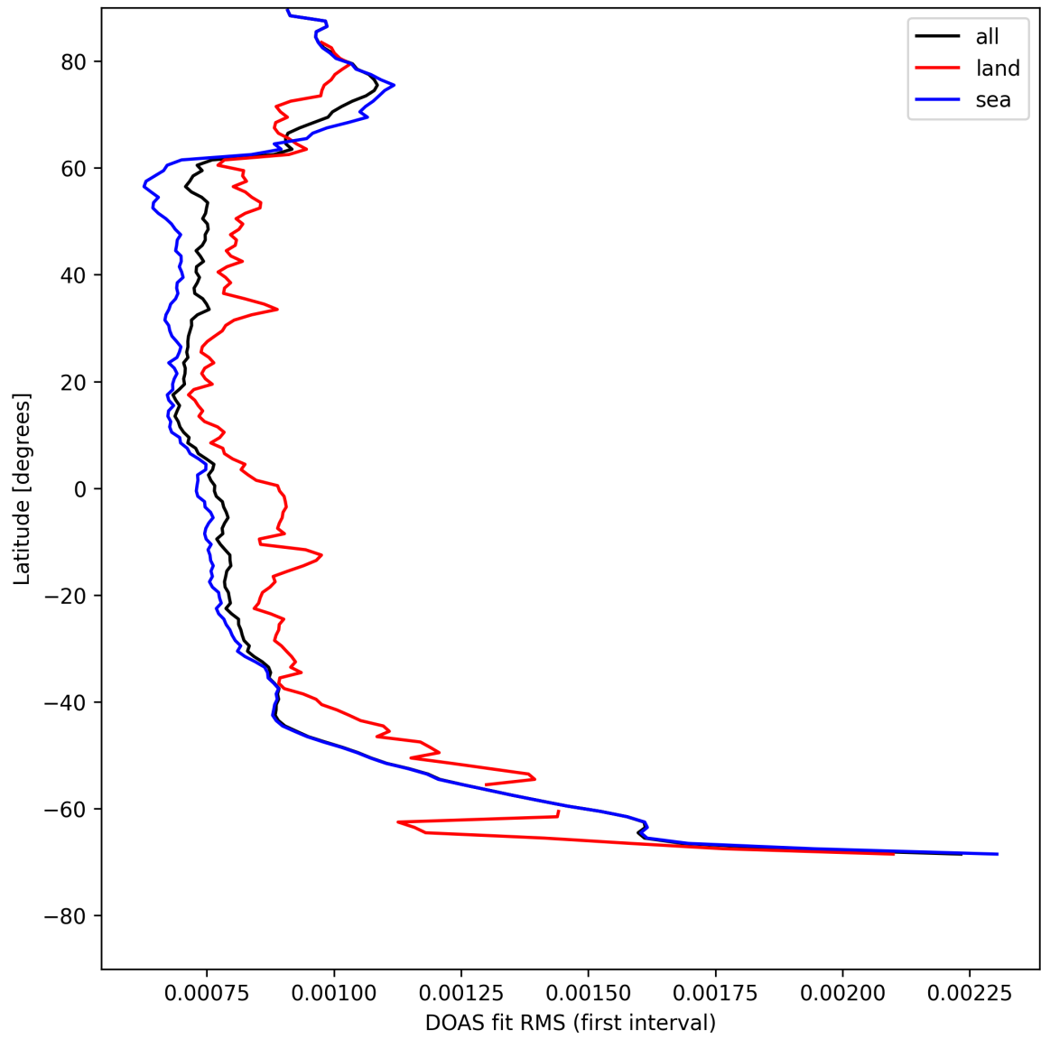
Figure 30: Zonal average of "DOAS fit RMS (first interval)" for 2025-05-04 to 2025-05-05.
