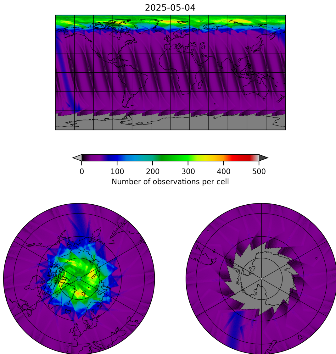
Figure 17: Map of the number of observations for 2025-05-04 to 2025-05-05
