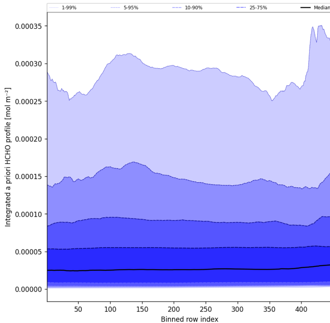
Figure 55: Along track statistics of “Integrated a priori HCHO profile” for 2025-05-04 to 2025-05-05
