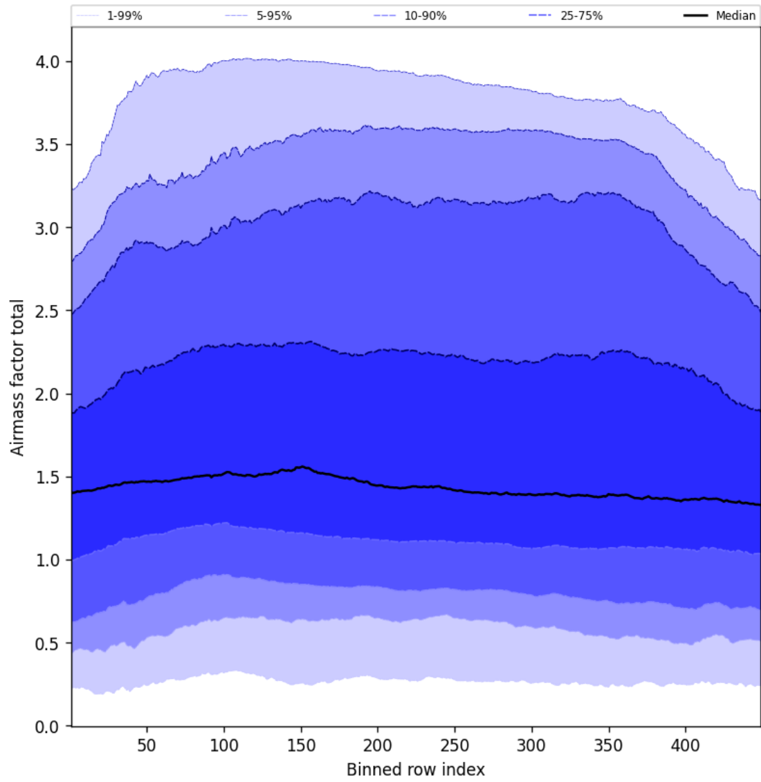
Figure 52: Along track statistics of “Airmass factor total” for 2025-05-04 to 2025-05-05
