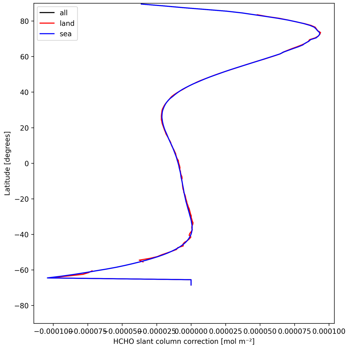
Figure 31: Zonal average of “HCHO slant column correction” for 2025-05-04 to 2025-05-05.
