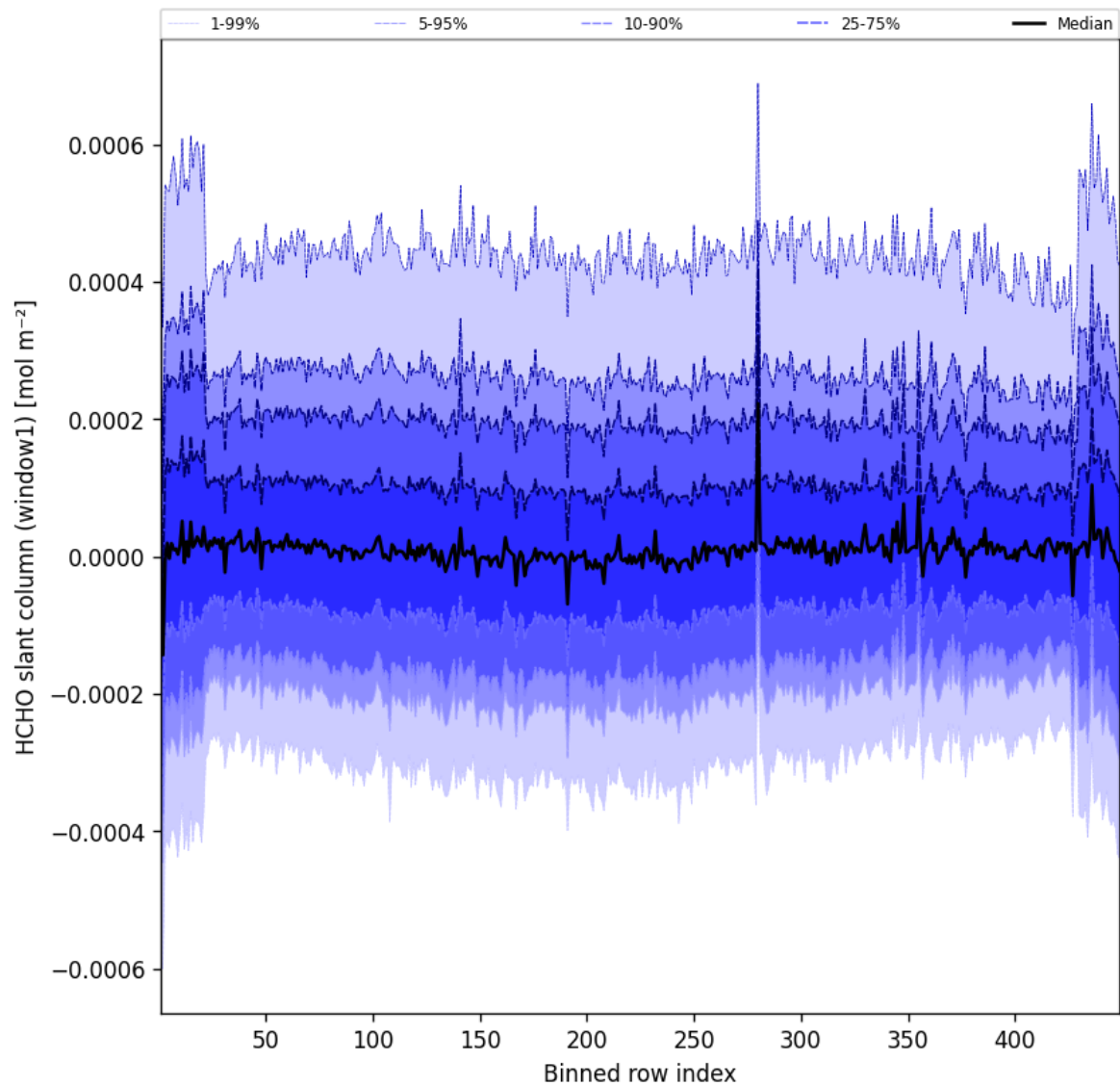
Figure 50: Along track statistics of “HCHO slant column (window1)” for 2025-05-04 to 2025-05-05
