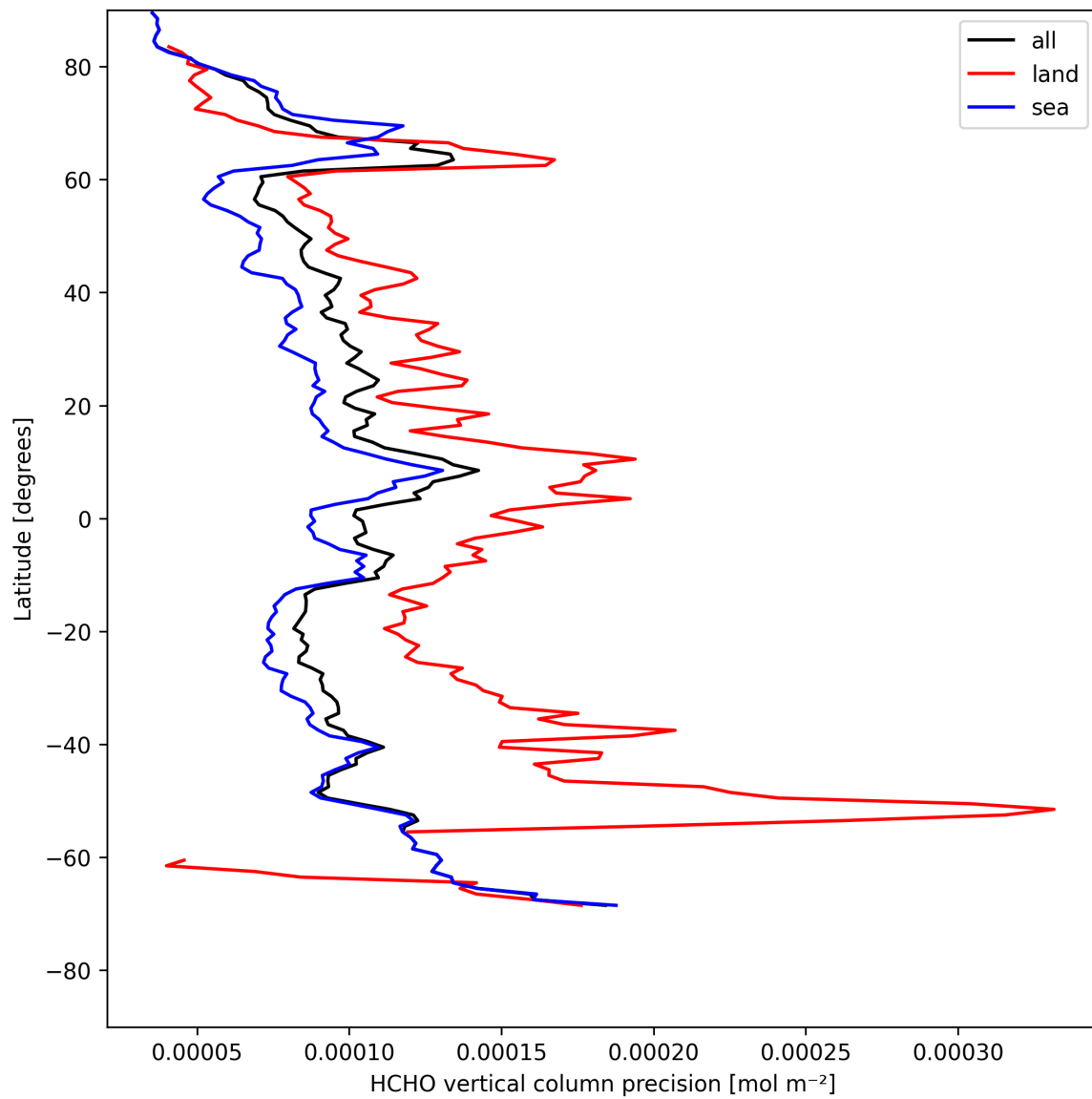
Figure 20: Zonal average of “HCHO vertical column precision” for 2025-05-04 to 2025-05-05.
