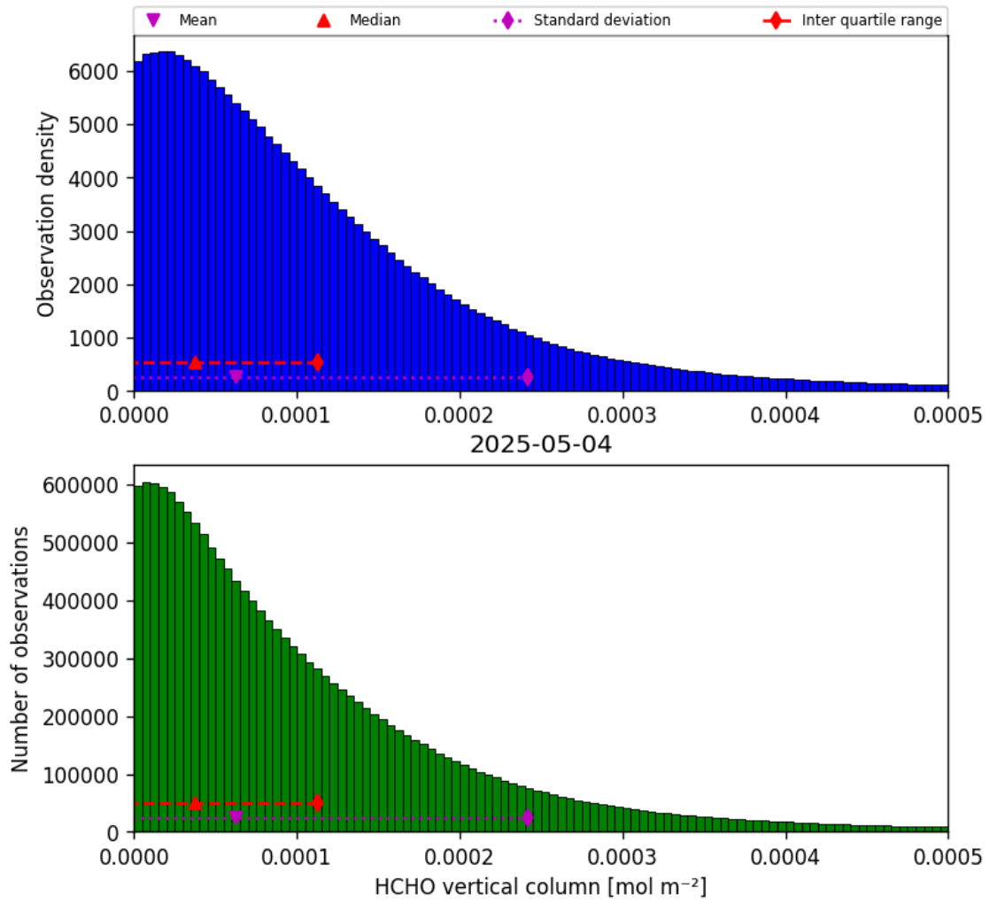
Figure 33: Histogram of “HCHO vertical column” for 2025-05-04 to 2025-05-05
