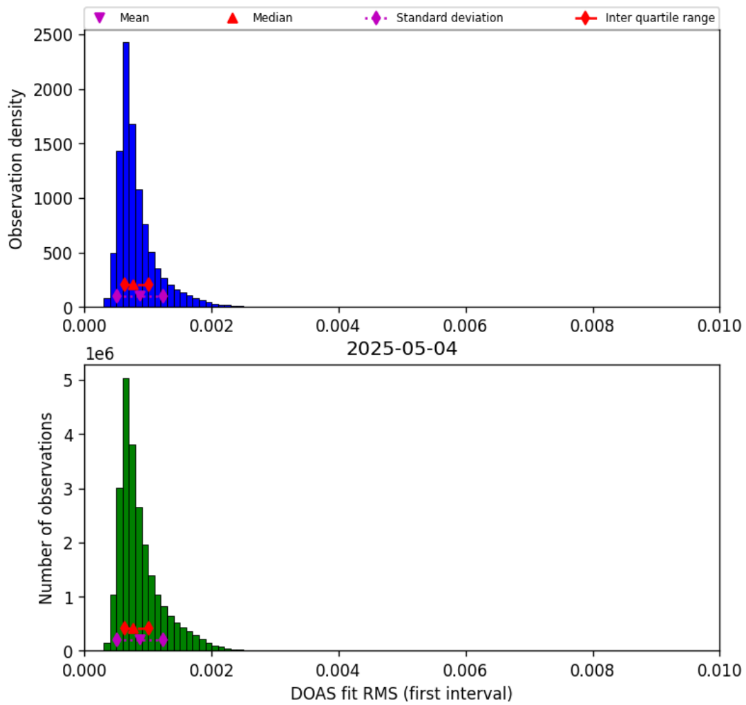
Figure 44: Histogram of “DOAS fit RMS (first interval)” for 2025-05-04 to 2025-05-05
