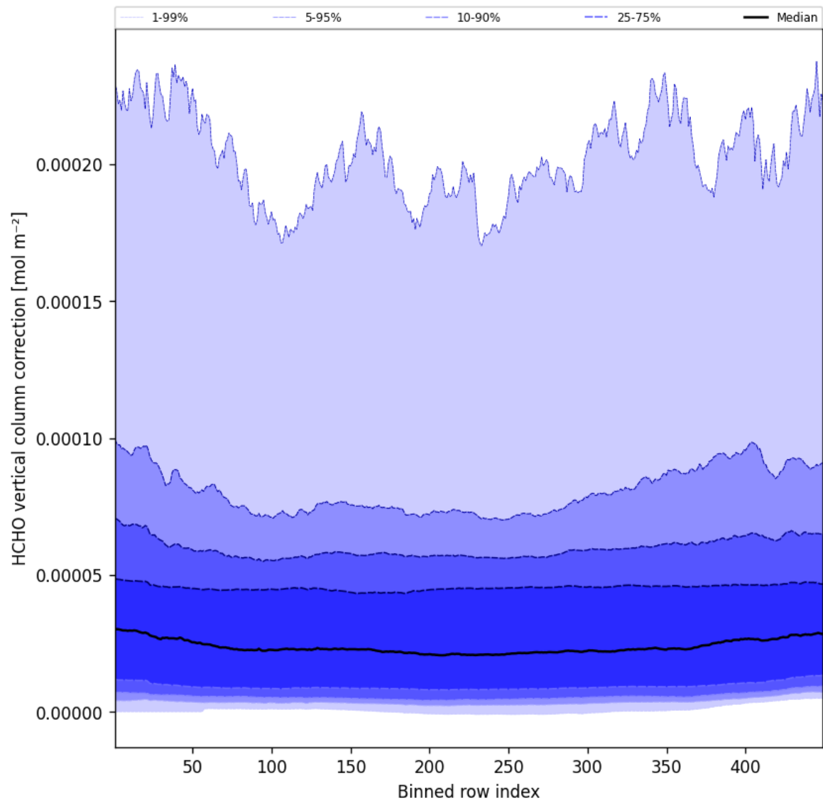
Figure 49: Along track statistics of “HCHO vertical column correction” for 2025-05-04 to 2025-05-05
