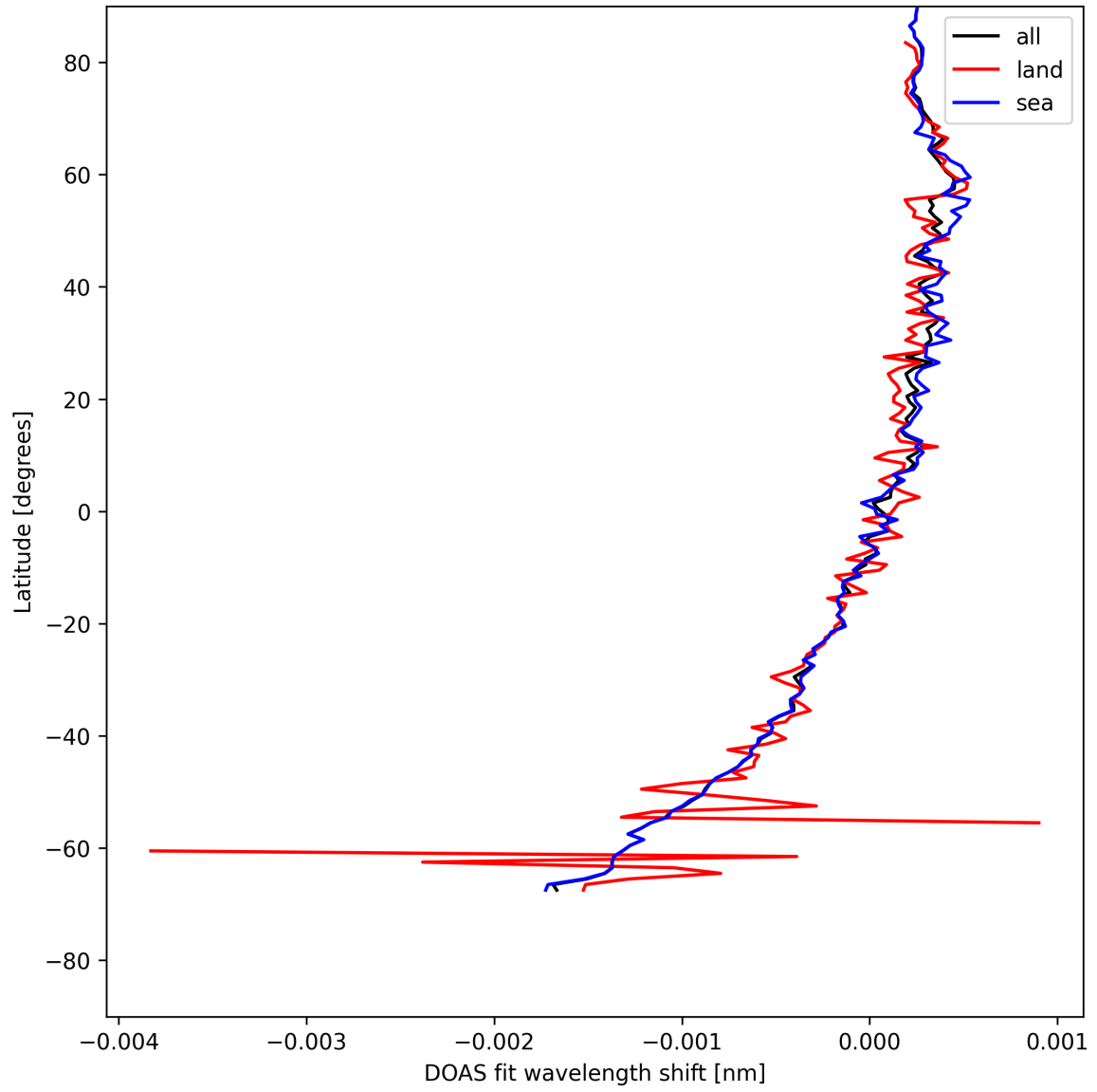
Figure 28: Zonal average of “DOAS fit wavelength shift” for 2025-05-06 to 2025-05-07.
