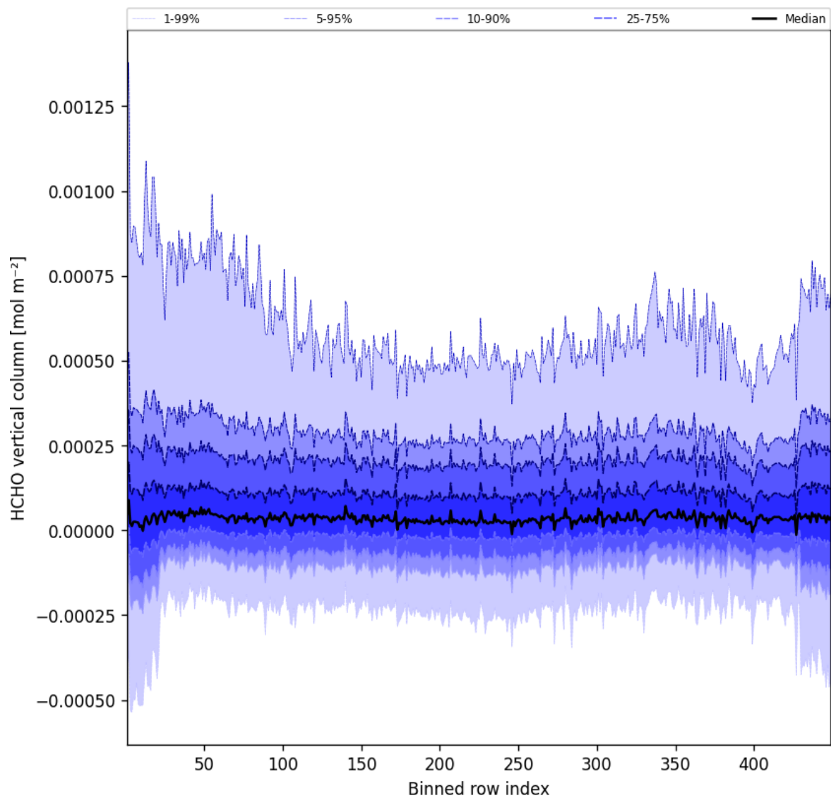
Figure 47: Along track statistics of “HCHO vertical column” for 2025-05-06 to 2025-05-07
