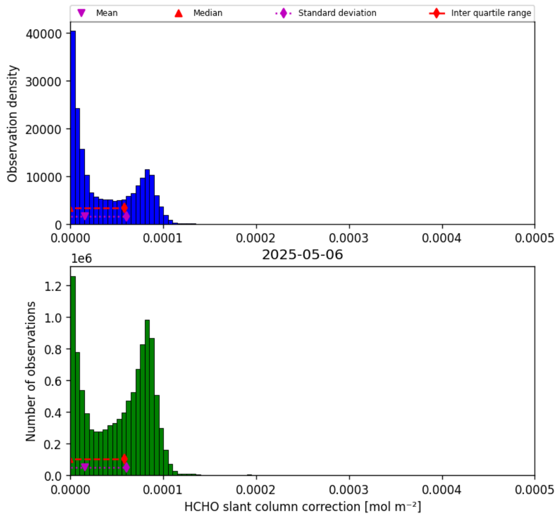
Figure 45: Histogram of “HCHO slant column correction” for 2025-05-06 to 2025-05-07
