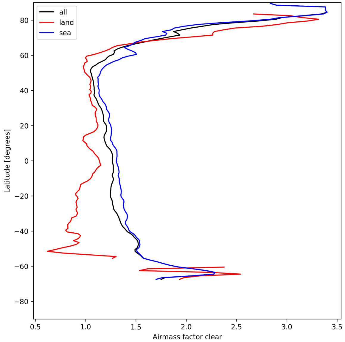
Figure 26: Zonal average of “Airmass factor clear” for 2025-05-06 to 2025-05-07.
