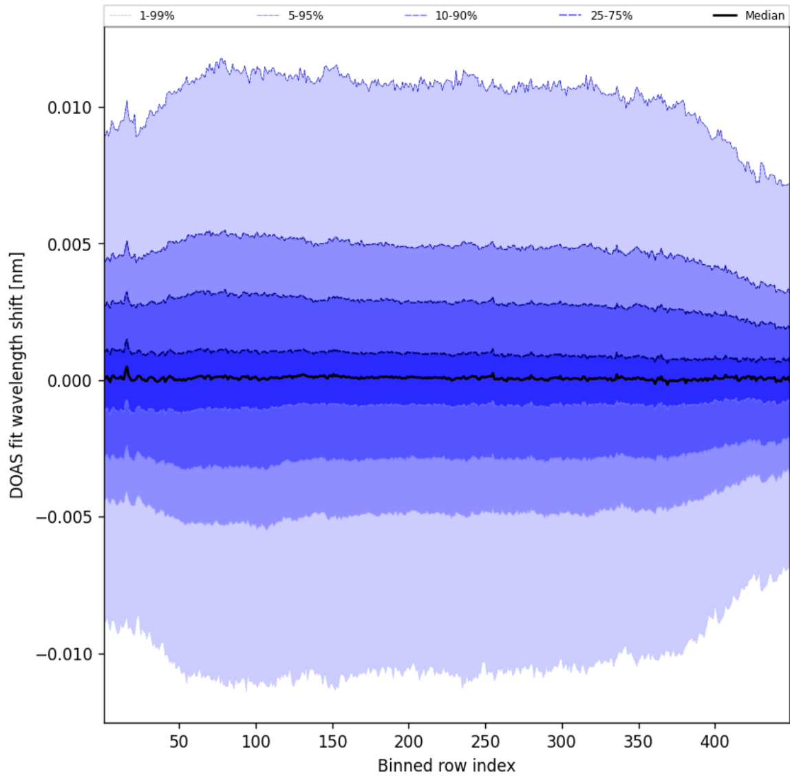
Figure 56: Along track statistics of “DOAS fit wavelength shift” for 2025-05-06 to 2025-05-07
