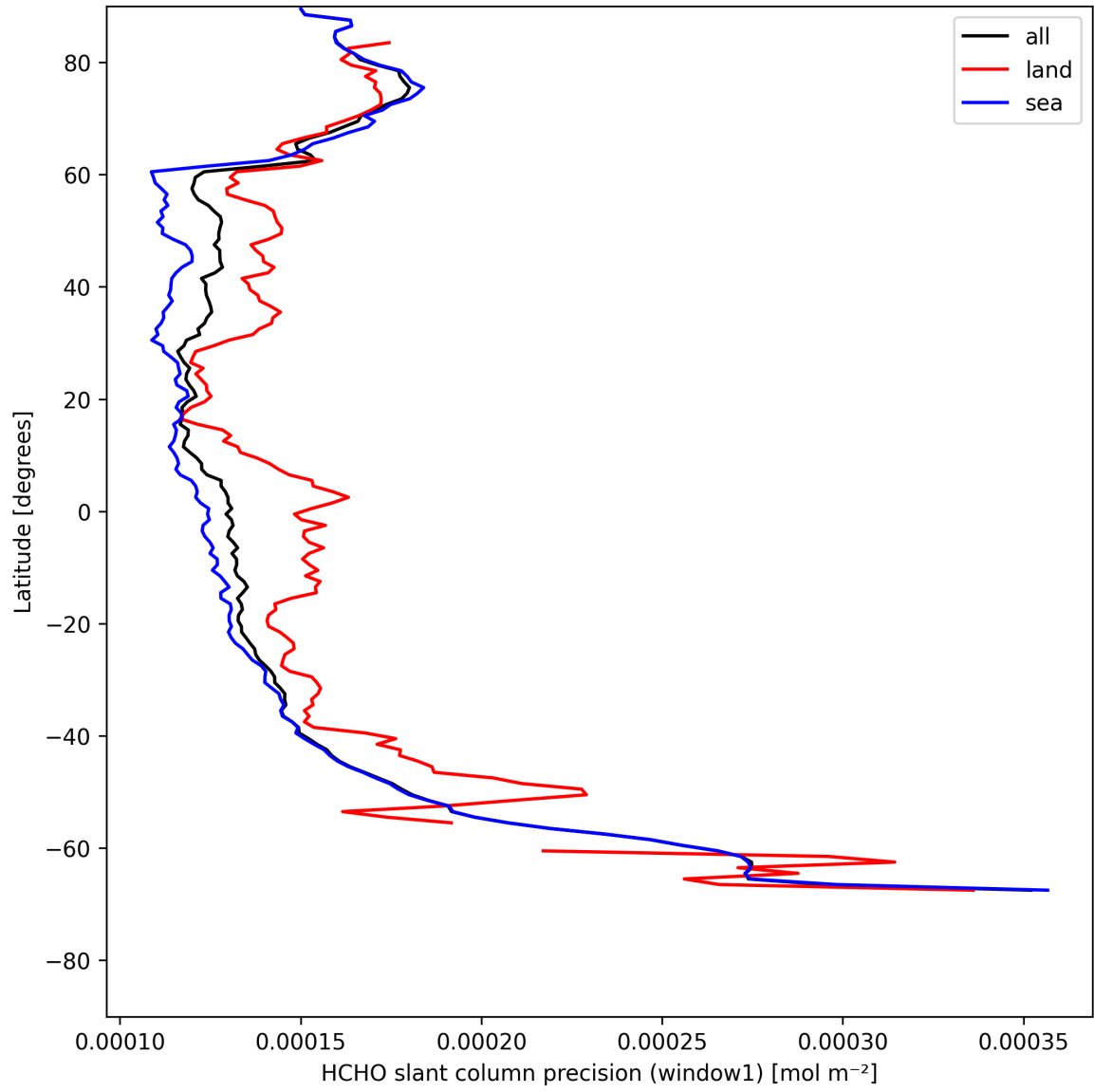
Figure 23: Zonal average of “HCHO slant column precision (window1)” for 2025-05-06 to 2025-05-07.
