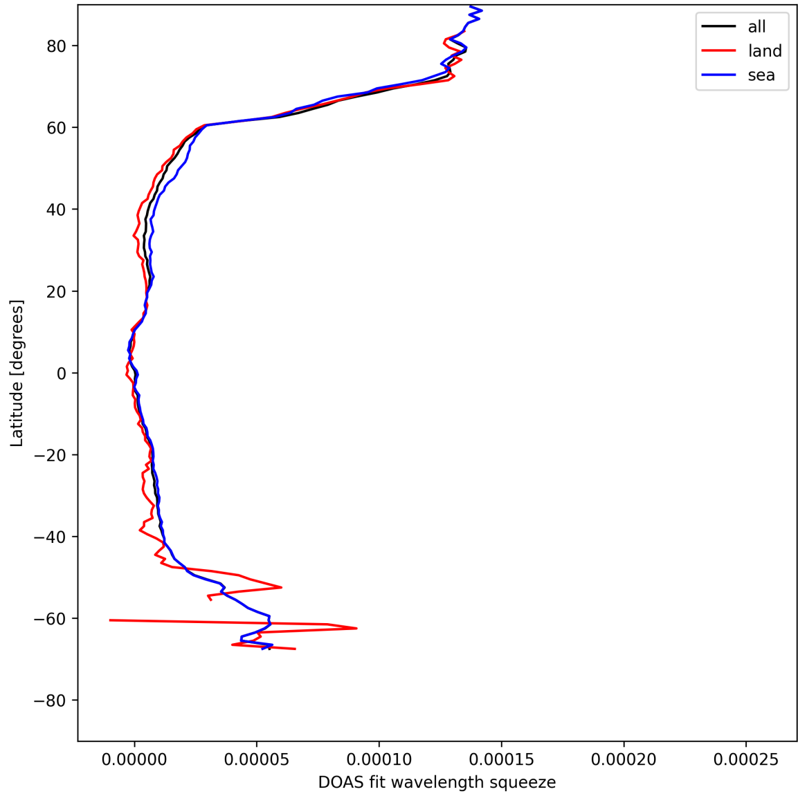
Figure 29: Zonal average of “DOAS fit wavelength squeeze” for 2025-05-06 to 2025-05-07.
