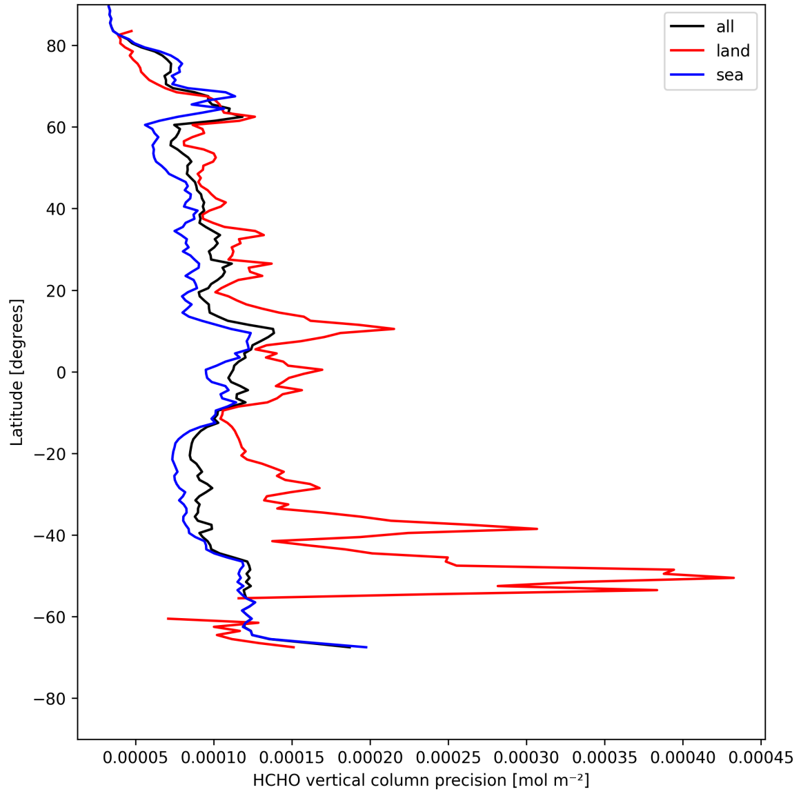
Figure 20: Zonal average of “HCHO vertical column precision” for 2025-05-06 to 2025-05-07.
