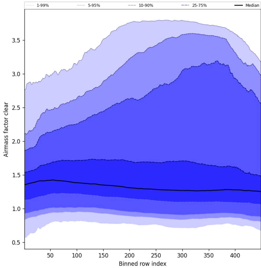
Figure 54: Along track statistics of “Airmass factor clear” for 2025-05-06 to 2025-05-07
