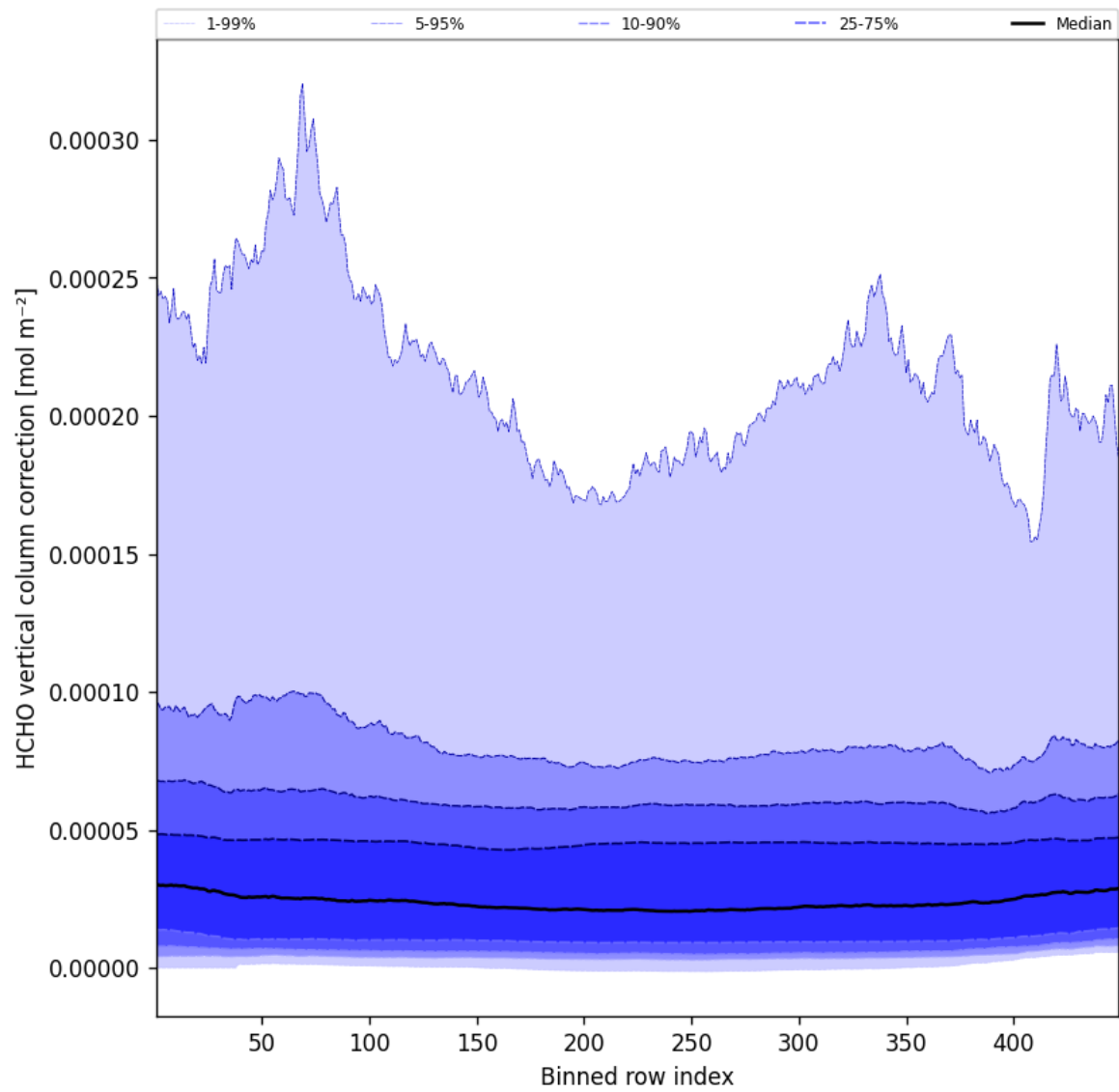
Figure 49: Along track statistics of “HCHO vertical column correction” for 2025-05-06 to 2025-05-07
