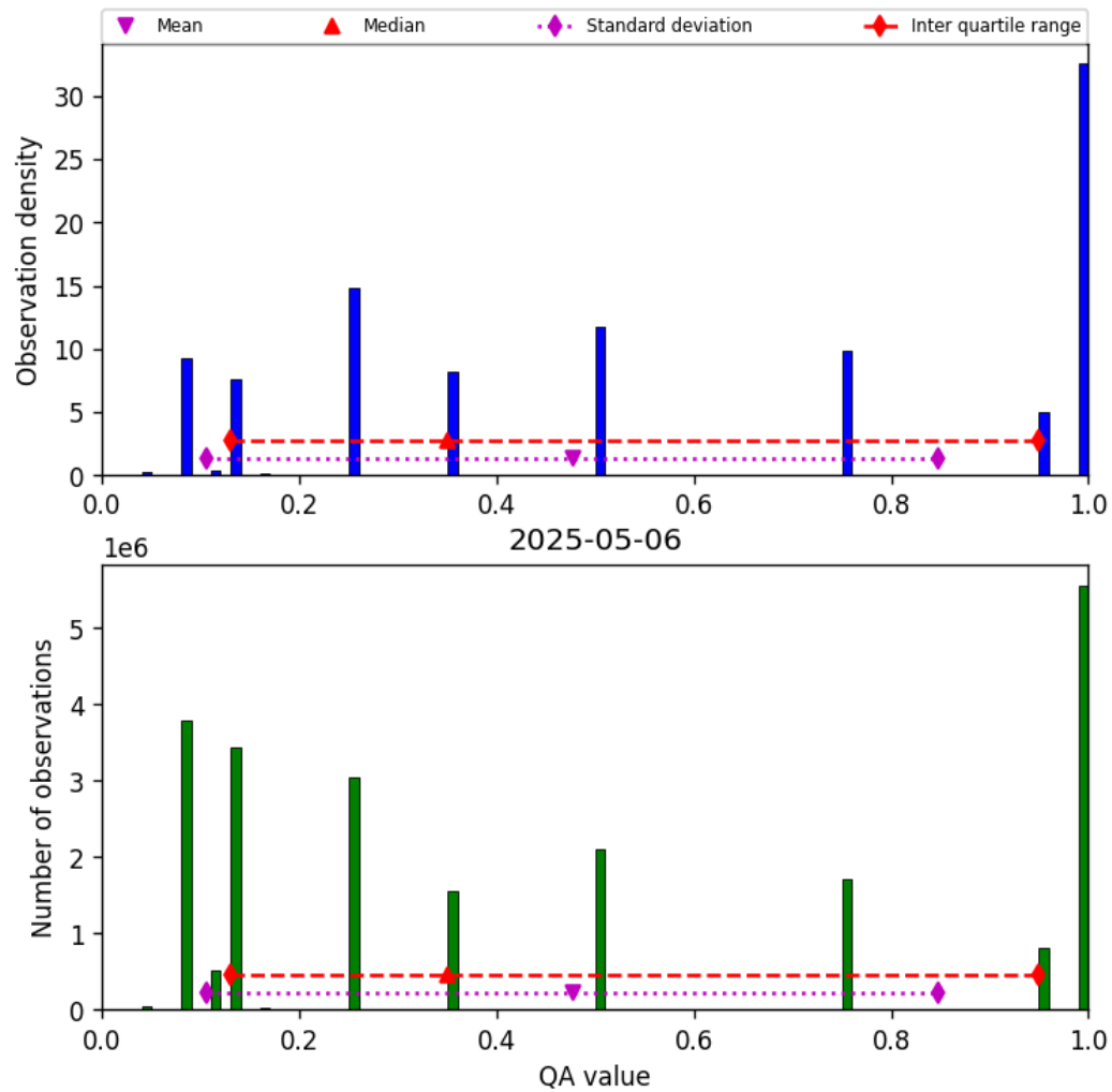
Figure 32: Histogram of “QA value” for 2025-05-06 to 2025-05-07
