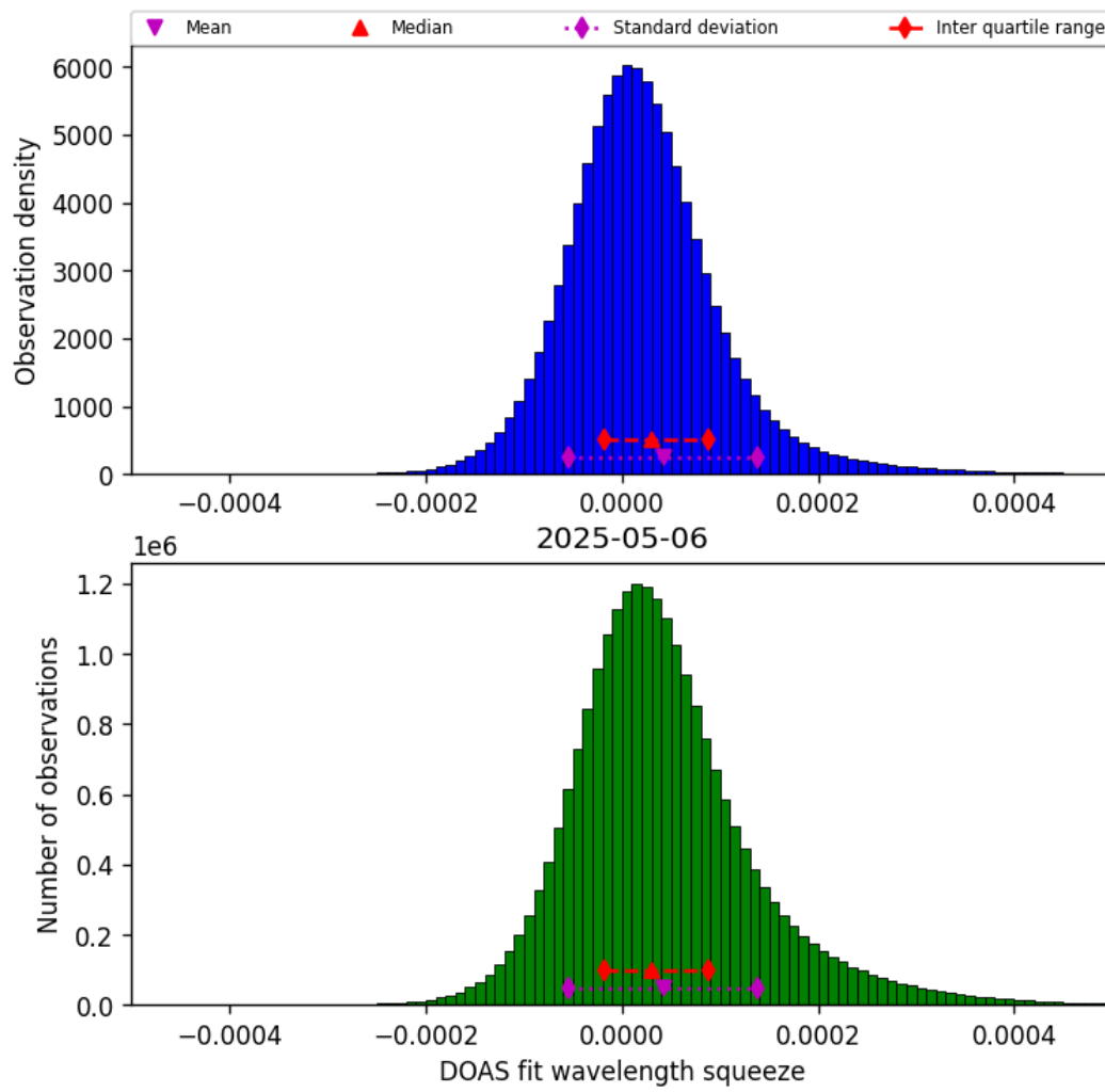
Figure 43: Histogram of “DOAS fit wavelength squeeze” for 2025-05-06 to 2025-05-07
