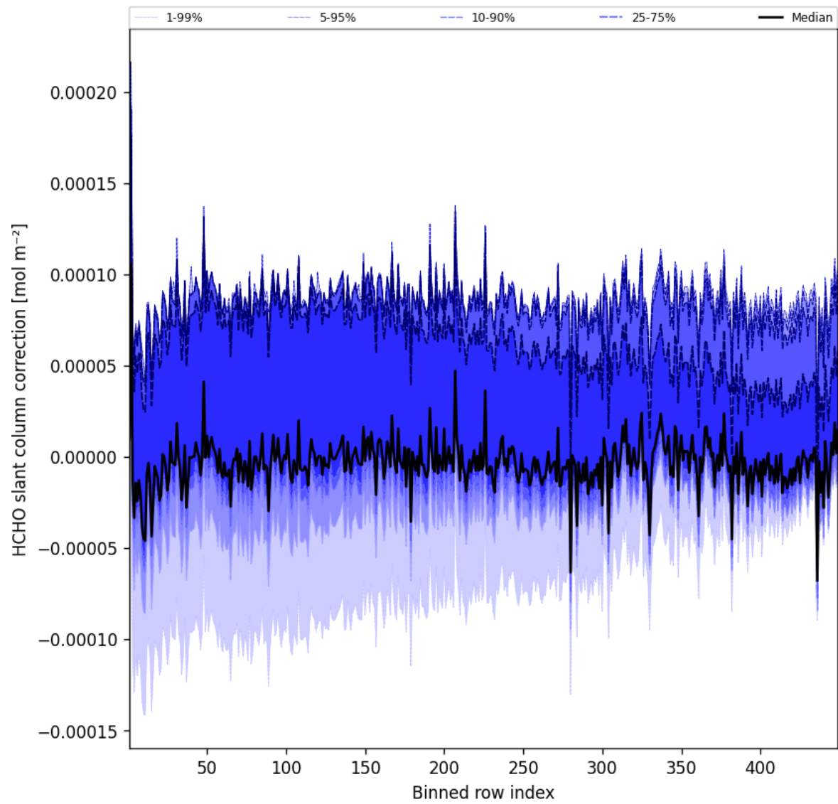
Figure 59: Along track statistics of “HCHO slant column correction” for 2025-05-06 to 2025-05-07
