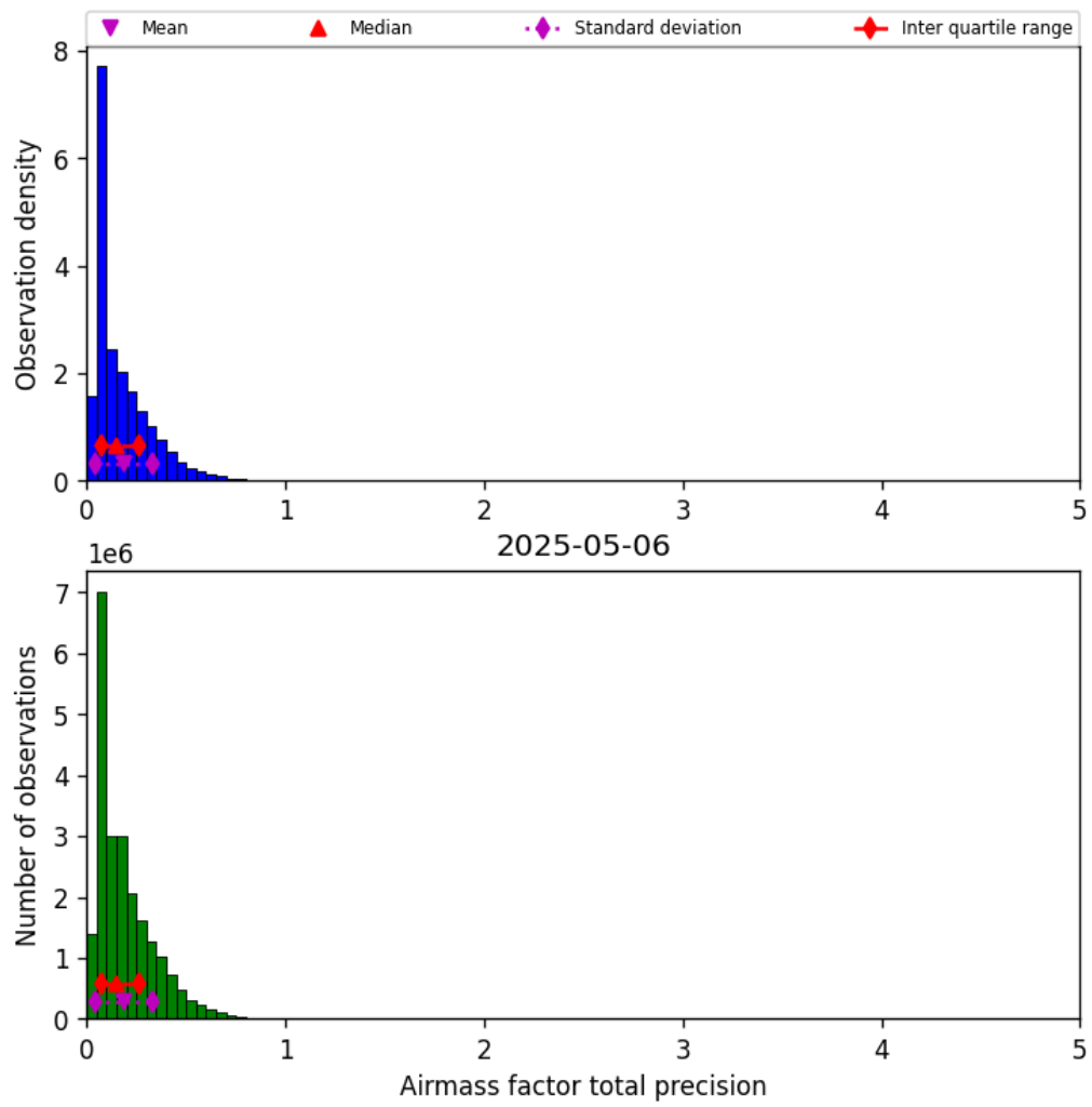
Figure 39: Histogram of “Airmass factor total precision” for 2025-05-06 to 2025-05-07
