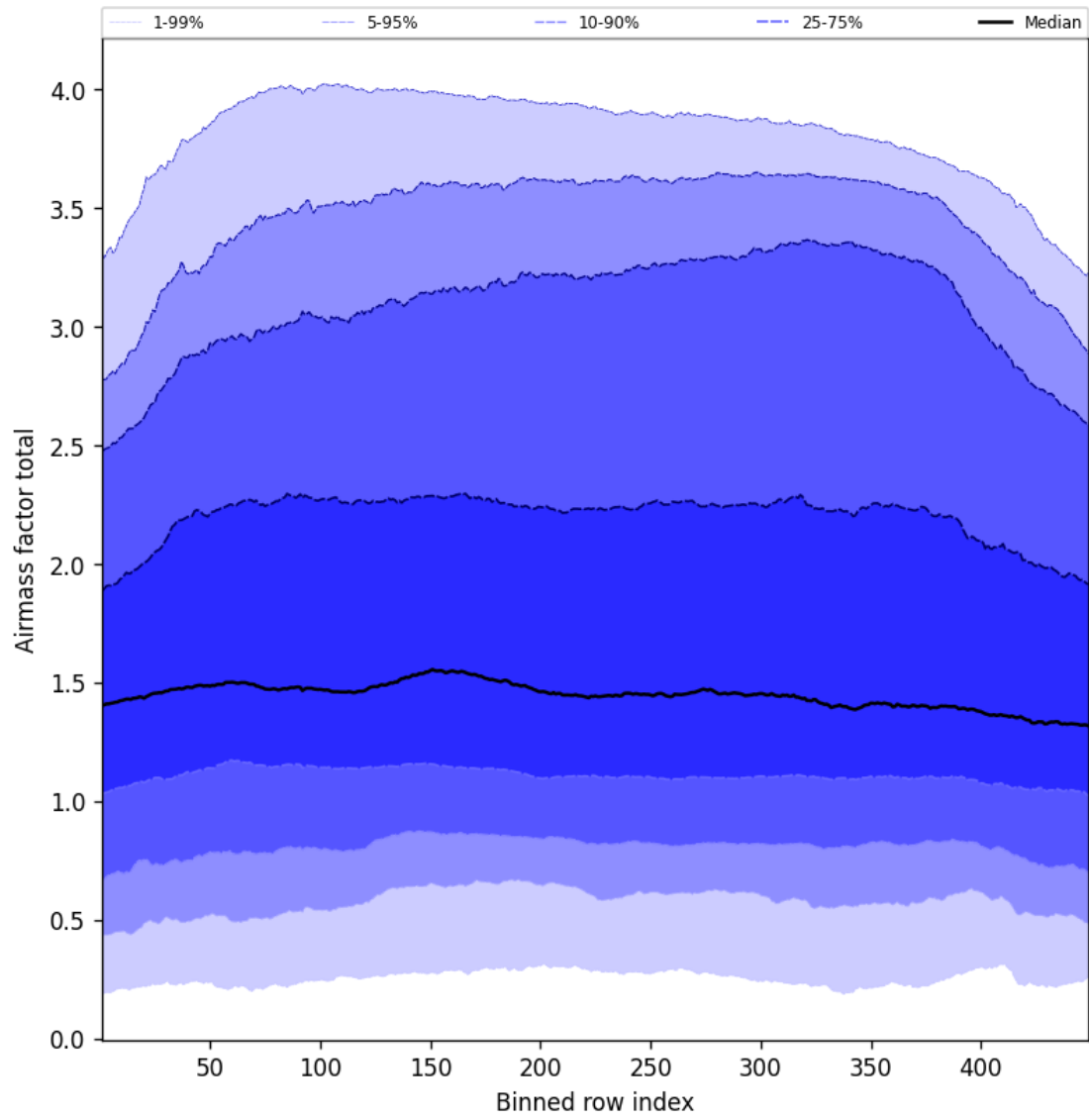
Figure 52: Along track statistics of “Airmass factor total” for 2025-05-06 to 2025-05-07
