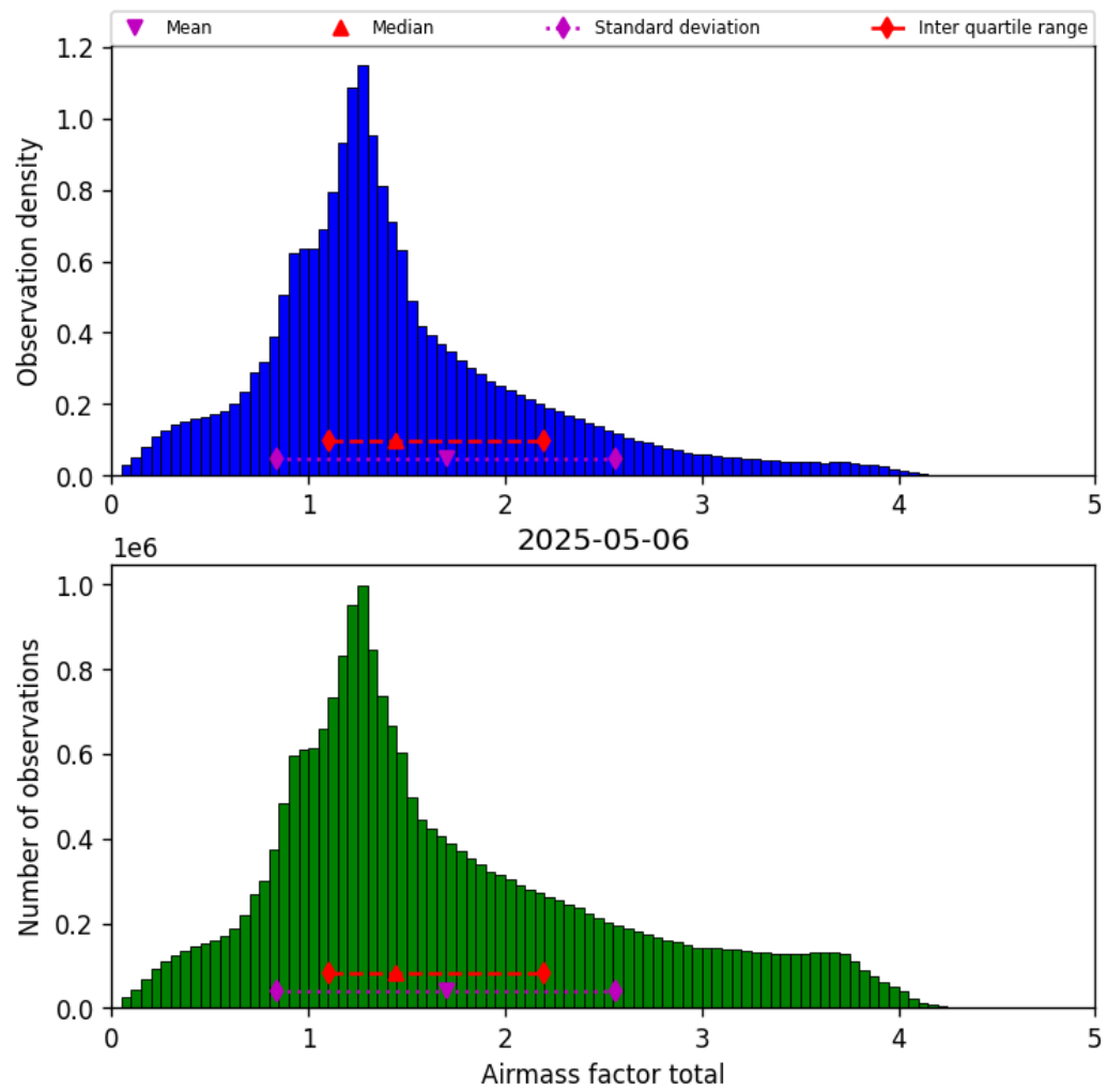
Figure 38: Histogram of “Airmass factor total” for 2025-05-06 to 2025-05-07
