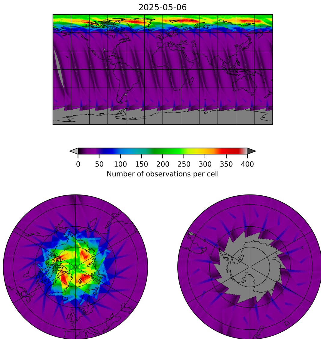
Figure 17: Map of the number of observations for 2025-05-06 to 2025-05-07
