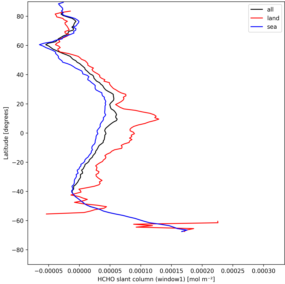
Figure 22: Zonal average of “HCHO slant column (window1)” for 2025-05-06 to 2025-05-07.
