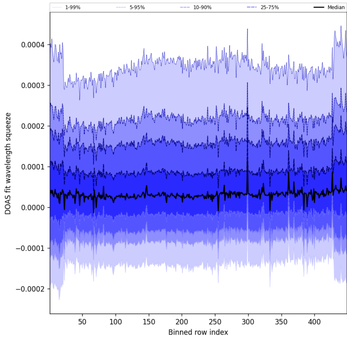
Figure 57: Along track statistics of “DOAS fit wavelength squeeze” for 2025-05-06 to 2025-05-07
