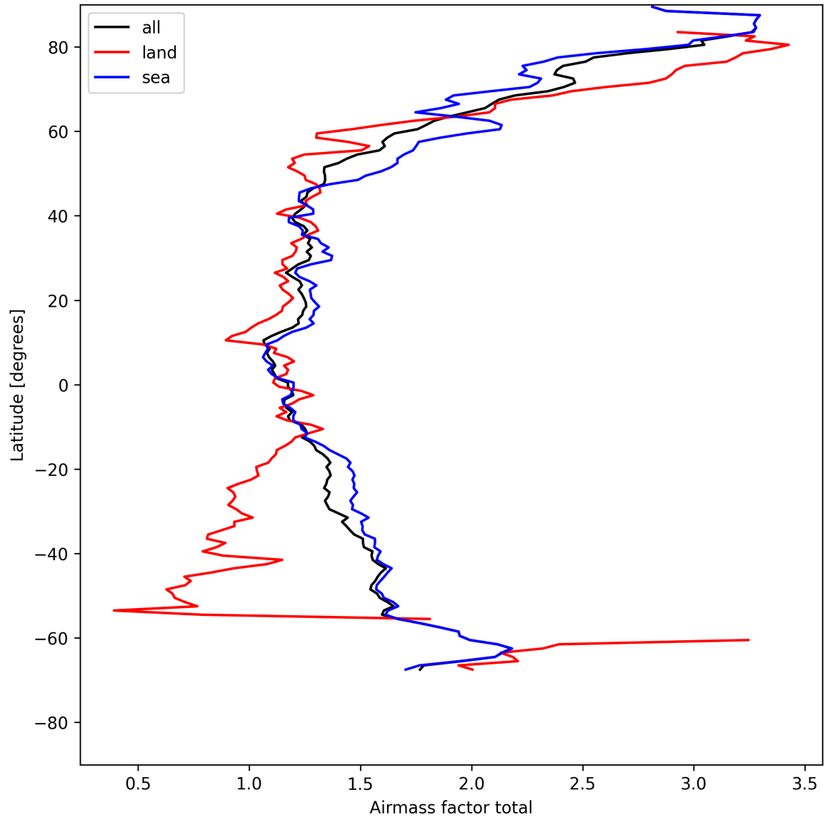
Figure 24: Zonal average of “Airmass factor total” for 2025-05-06 to 2025-05-07.
