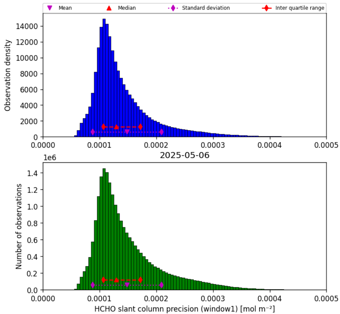
Figure 37: Histogram of “HCHO slant column precision (window1)” for 2025-05-06 to 2025-05-07
