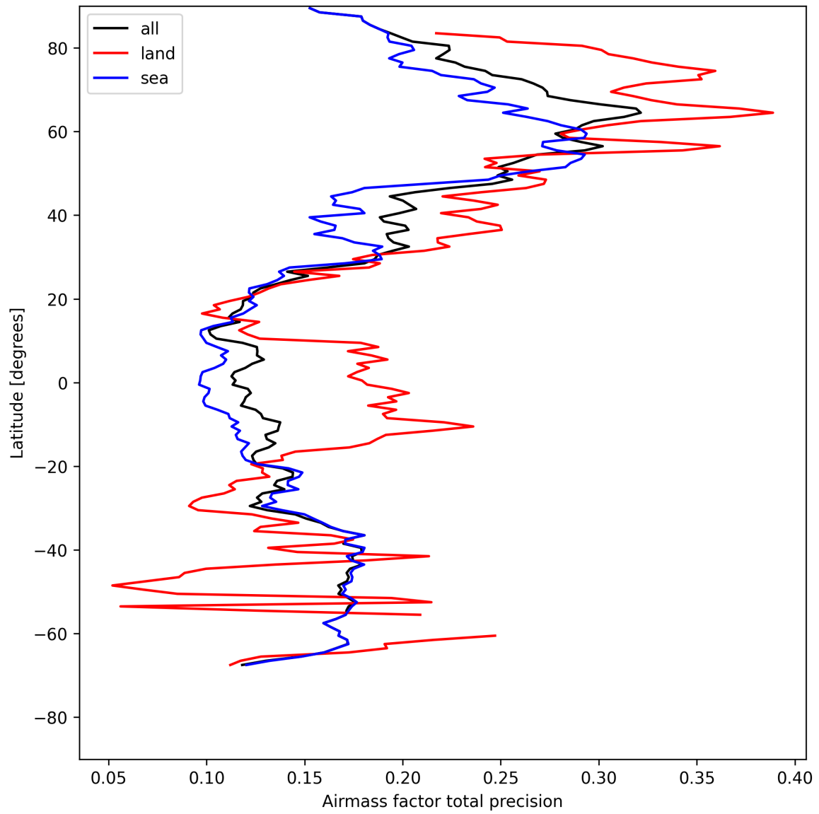
Figure 25: Zonal average of “Airmass factor total precision” for 2025-05-06 to 2025-05-07.
