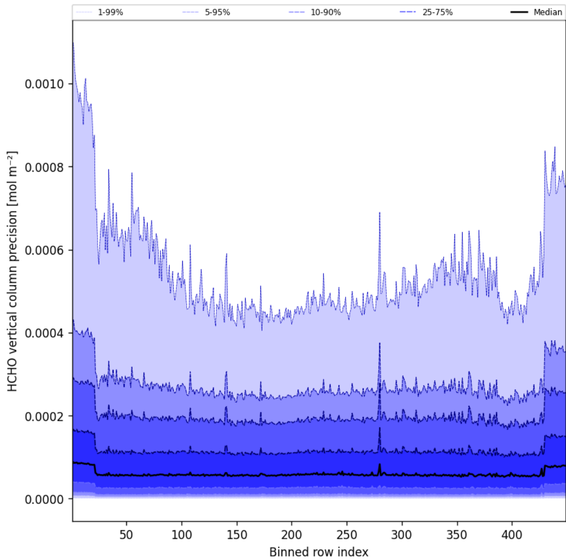
Figure 48: Along track statistics of “HCHO vertical column precision” for 2025-05-06 to 2025-05-07
