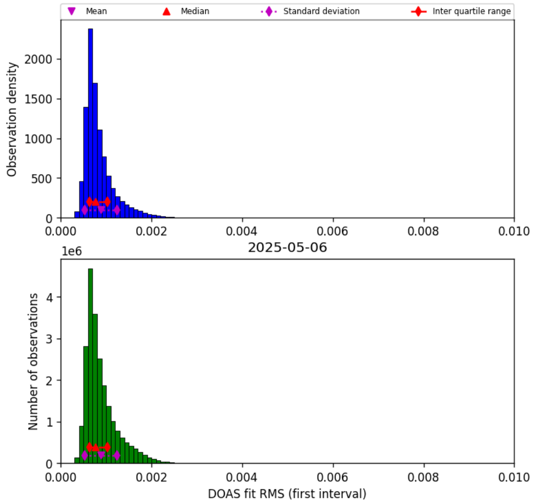
Figure 44: Histogram of “DOAS fit RMS (first interval)” for 2025-05-06 to 2025-05-07
