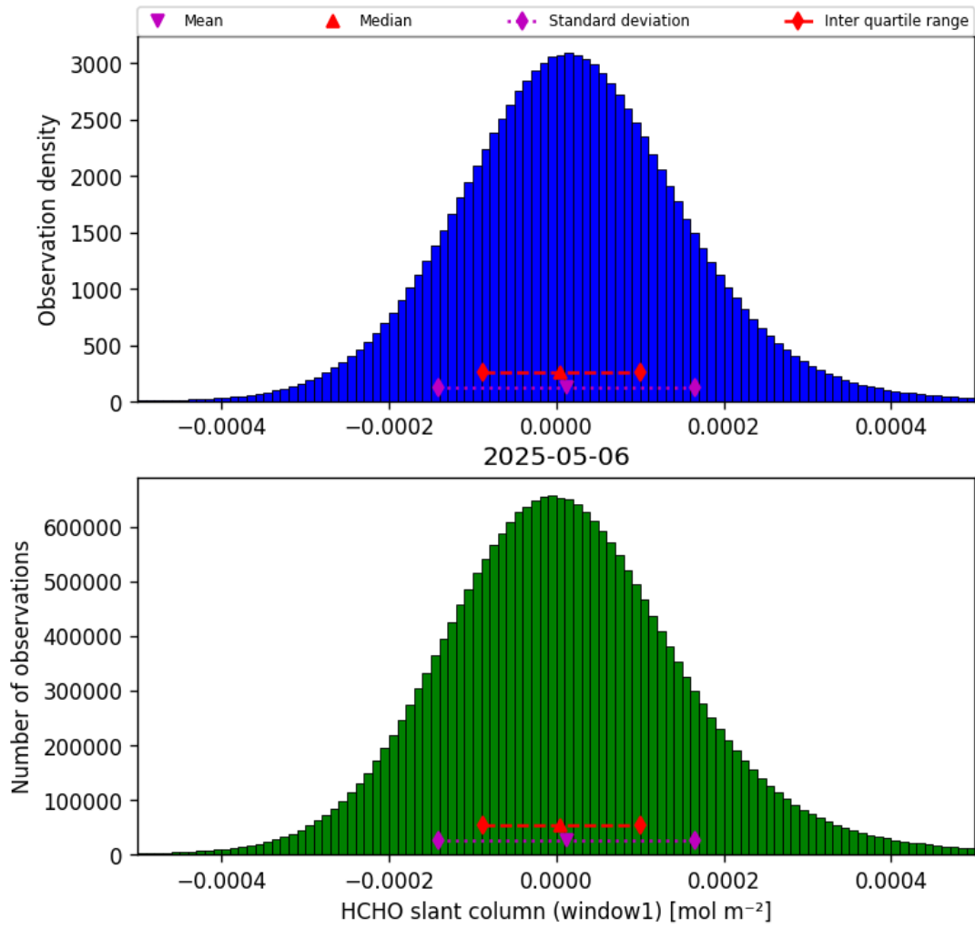
Figure 36: Histogram of “HCHO slant column (window1)” for 2025-05-06 to 2025-05-07
