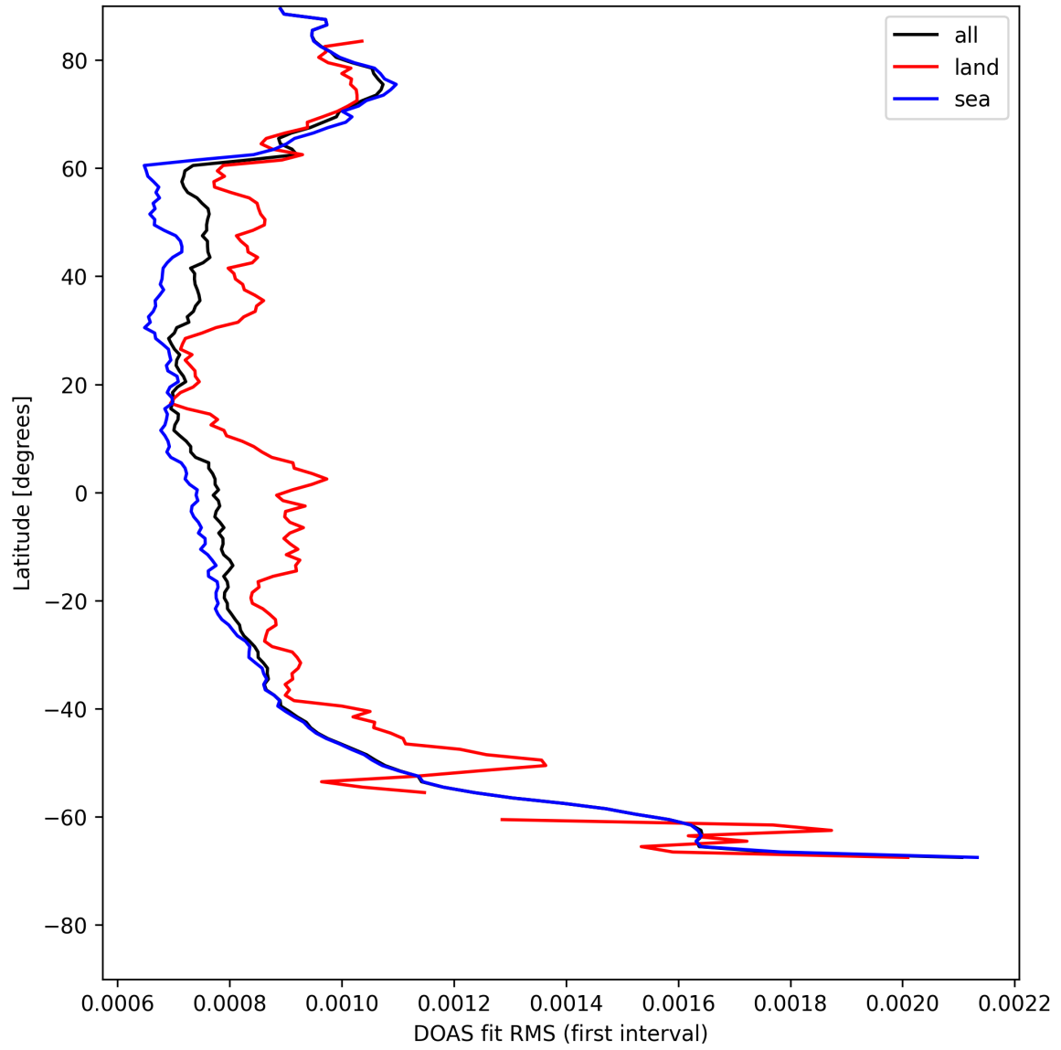
Figure 30: Zonal average of “DOAS fit RMS (first interval)” for 2025-05-06 to 2025-05-07.
