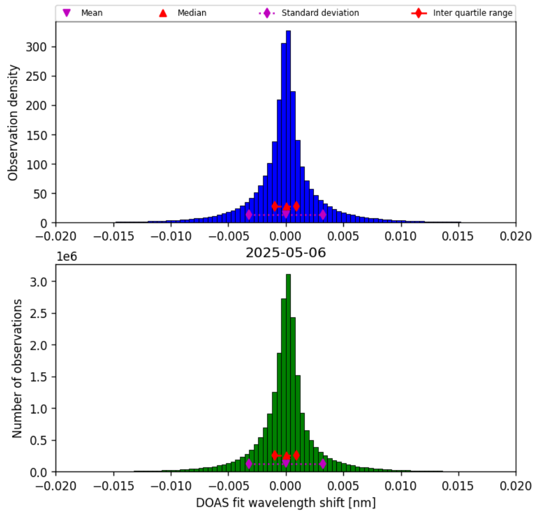
Figure 42: Histogram of “DOAS fit wavelength shift” for 2025-05-06 to 2025-05-07
