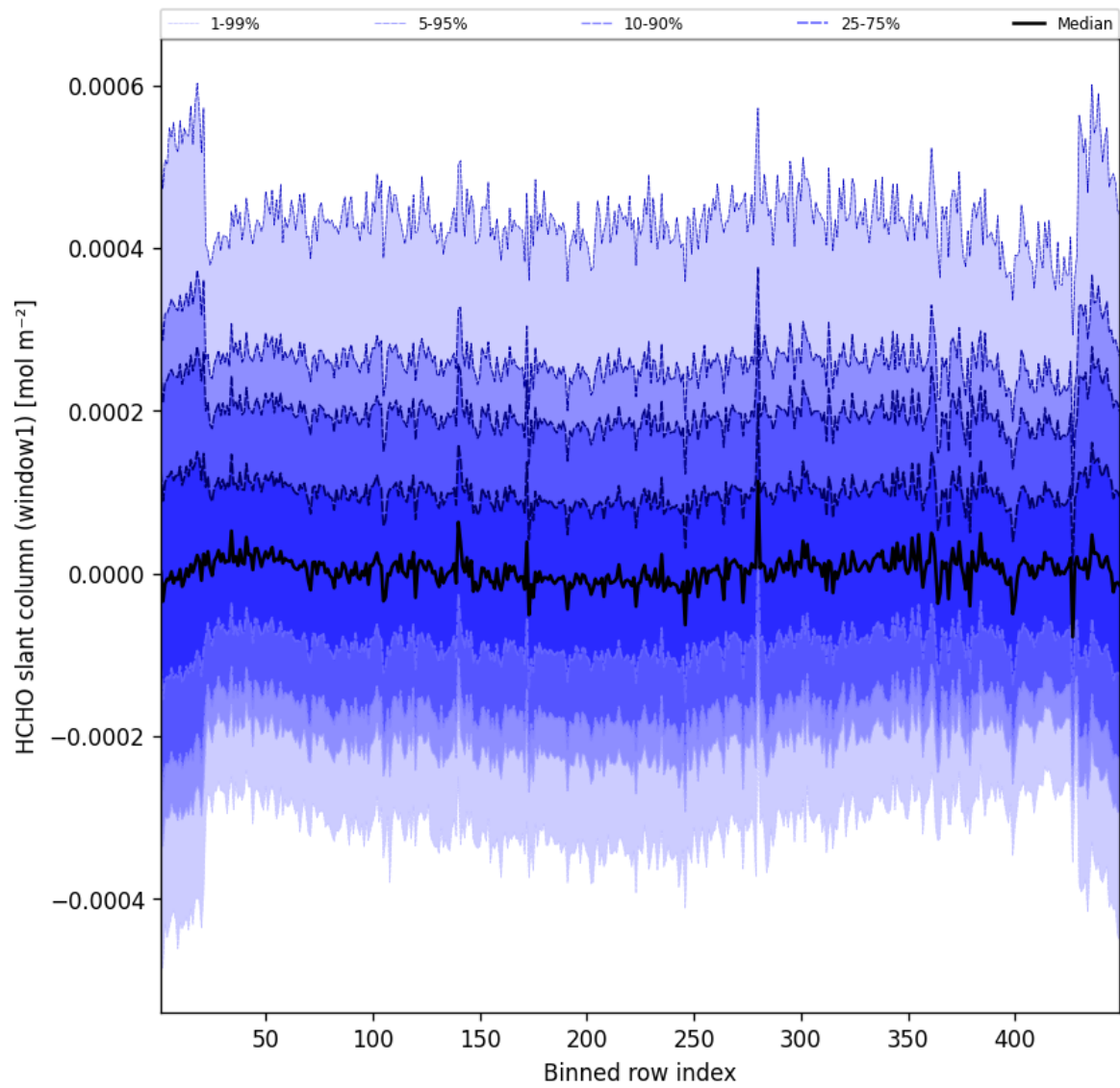
Figure 50: Along track statistics of “HCHO slant column (window1)” for 2025-05-06 to 2025-05-07
