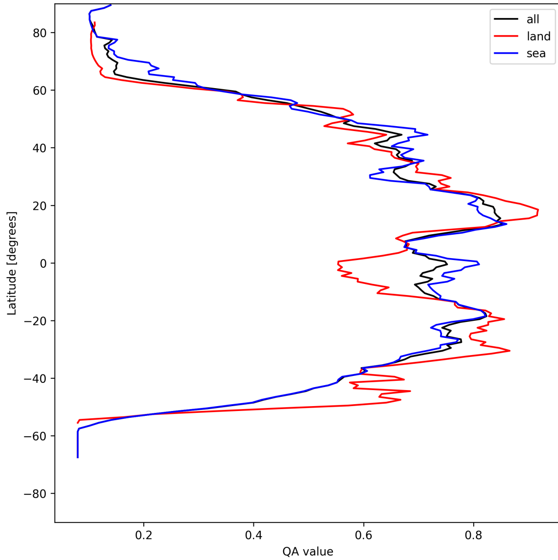
Figure 18: Zonal average of “QA value” for 2025-05-06 to 2025-05-07.
