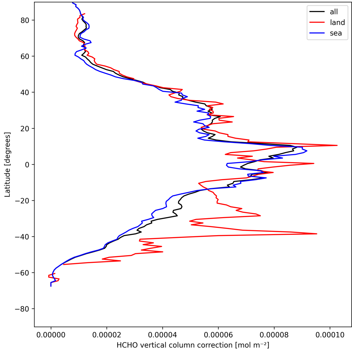
Figure 21: Zonal average of “HCHO vertical column correction” for 2025-05-06 to 2025-05-07.
