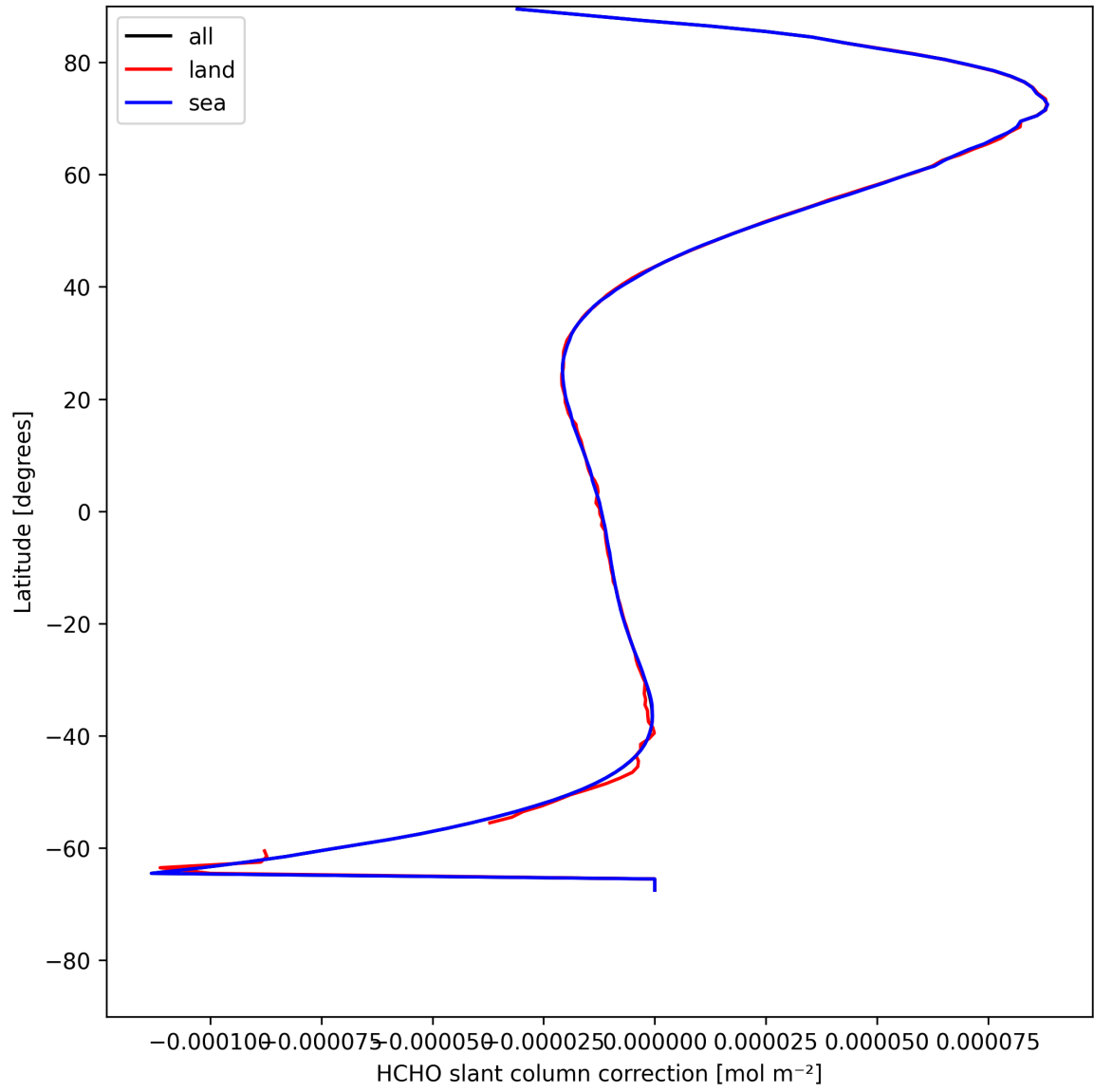
Figure 31: Zonal average of “HCHO slant column correction” for 2025-05-06 to 2025-05-07.
