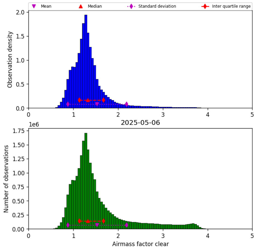
Figure 40: Histogram of “Airmass factor clear” for 2025-05-06 to 2025-05-07
