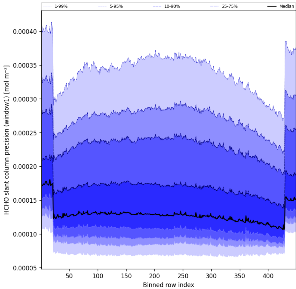
Figure 51: Along track statistics of “HCHO slant column precision (window1)” for 2025-05-06 to 2025-05-07
