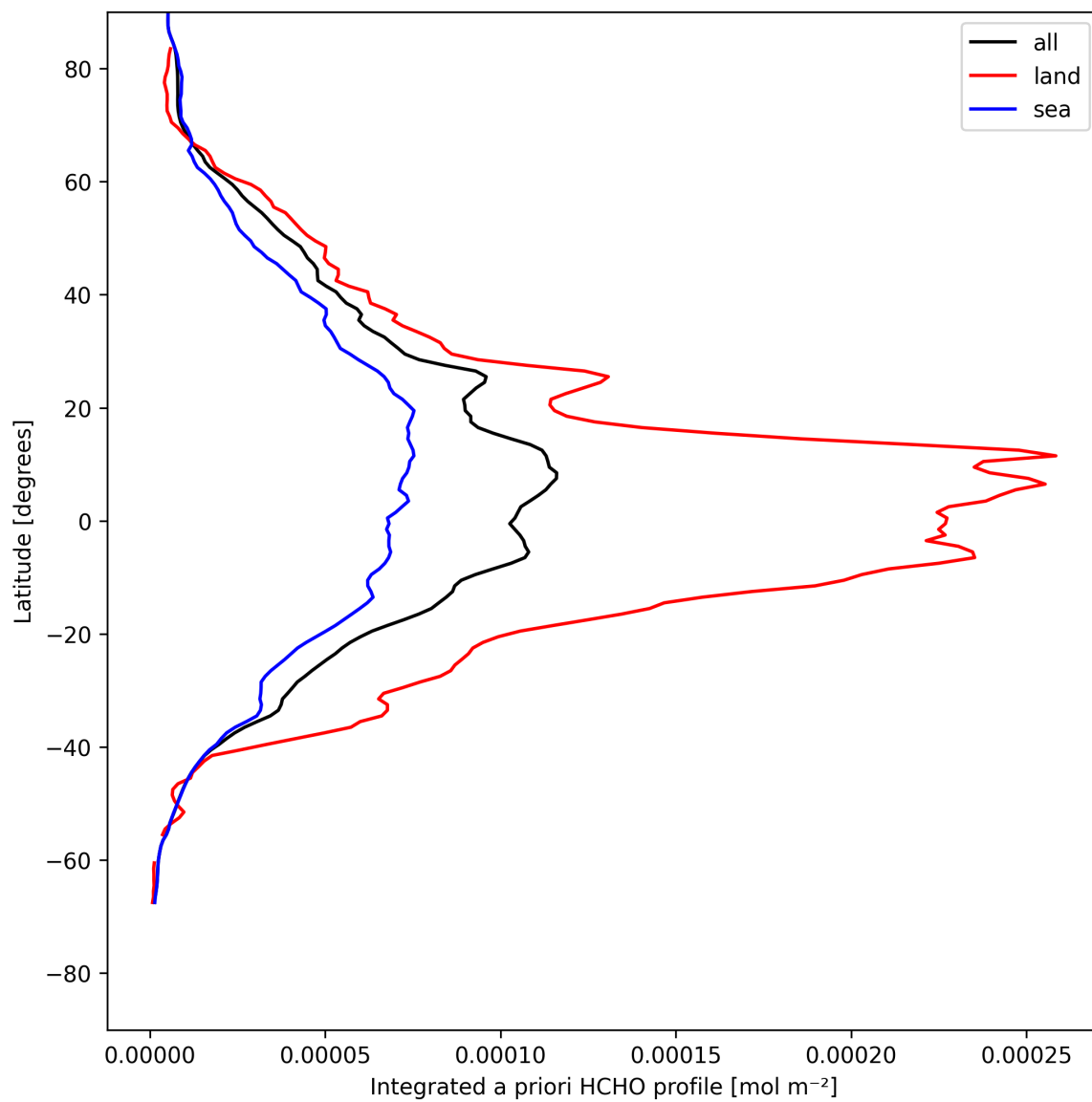
Figure 27: Zonal average of “Integrated a priori HCHO profile” for 2025-05-06 to 2025-05-07.
