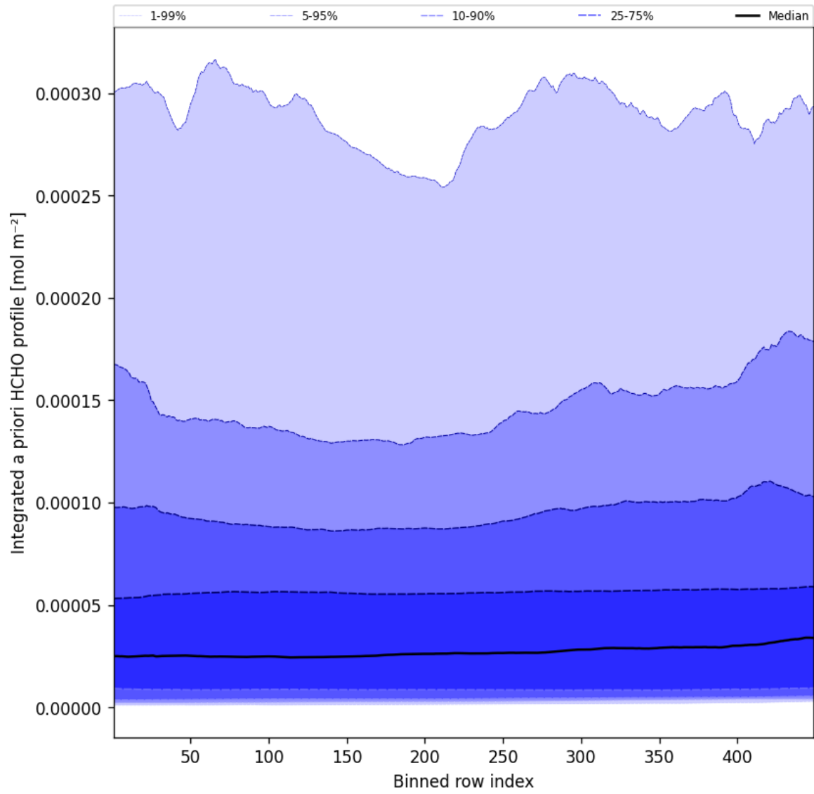
Figure 55: Along track statistics of "Integrated a priori HCHO profile" for 2025-05-06 to 2025-05-07
