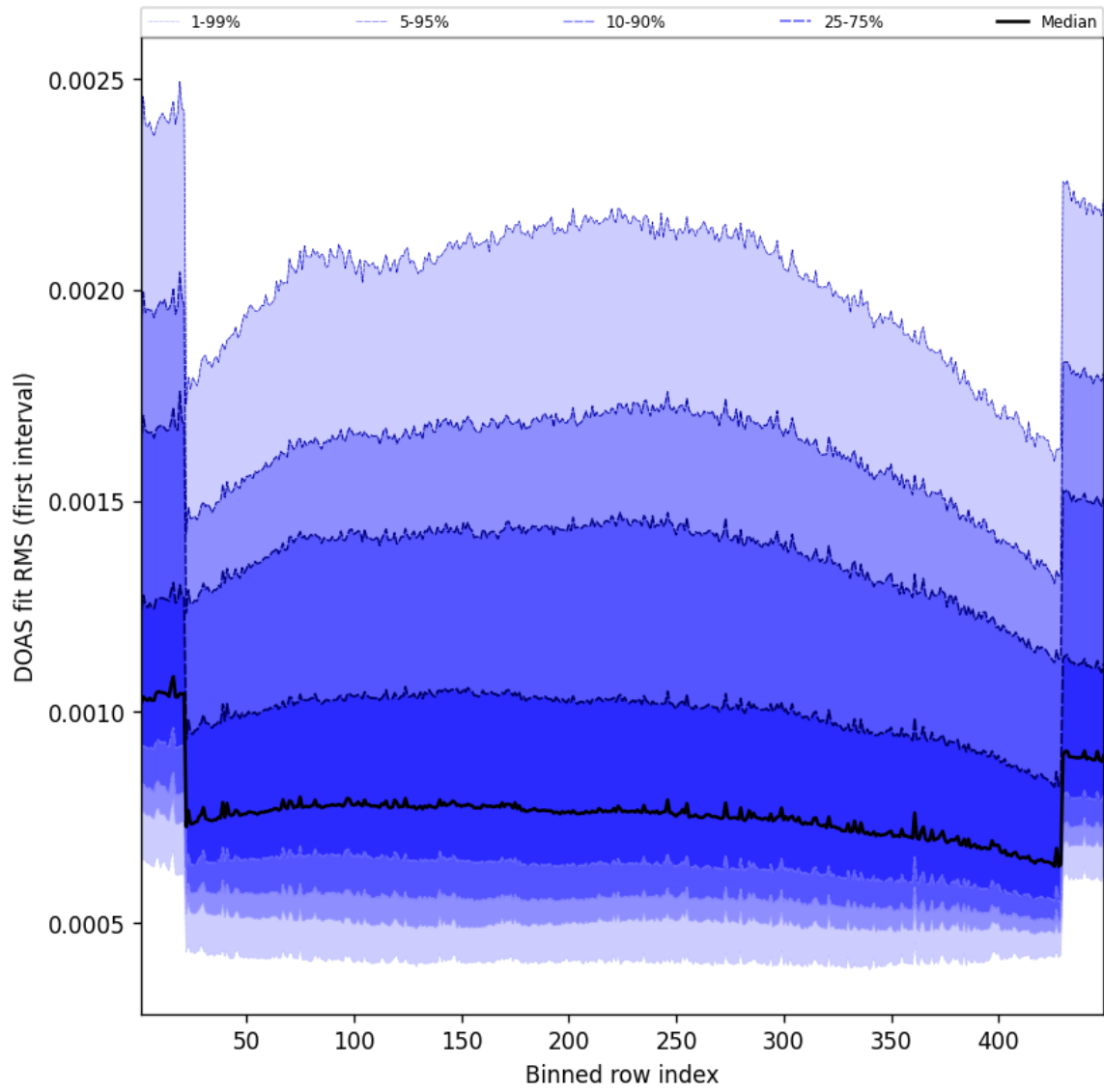
Figure 58: Along track statistics of “DOAS fit RMS (first interval)” for 2025-05-06 to 2025-05-07
