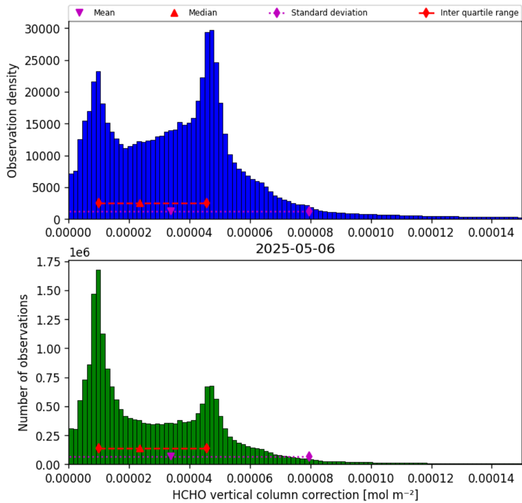
Figure 35: Histogram of “HCHO vertical column correction” for 2025-05-06 to 2025-05-07
