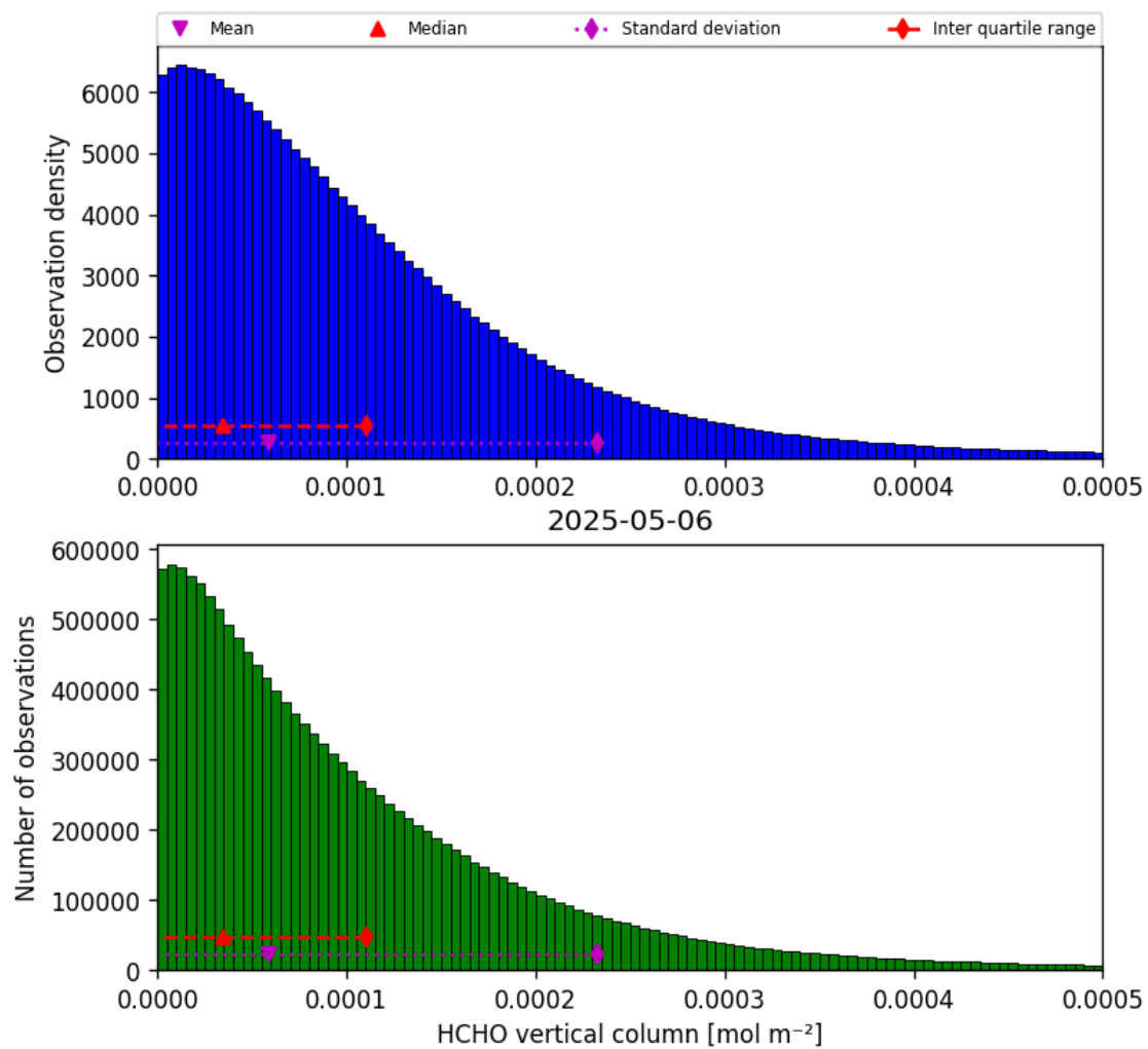
Figure 33: Histogram of “HCHO vertical column” for 2025-05-06 to 2025-05-07
