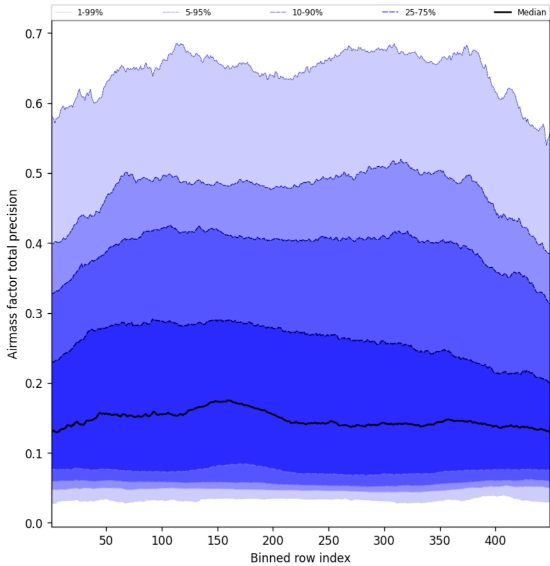
Figure 53: Along track statistics of “Airmass factor total precision” for 2025-05-06 to 2025-05-07
