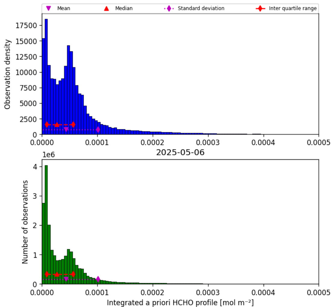
Figure 41: Histogram of “Integrated a priori HCHO profile” for 2025-05-06 to 2025-05-07
