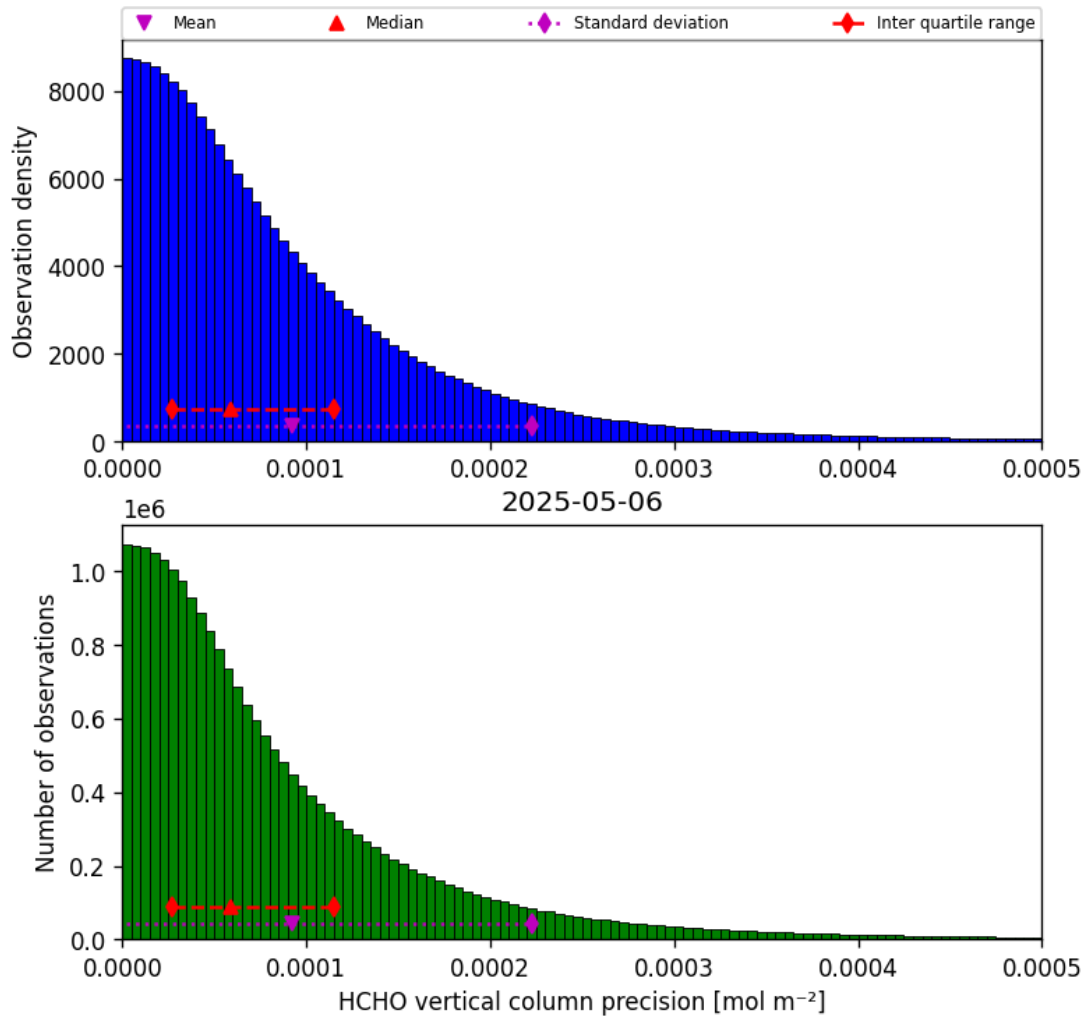
Figure 34: Histogram of “HCHO vertical column precision” for 2025-05-06 to 2025-05-07
