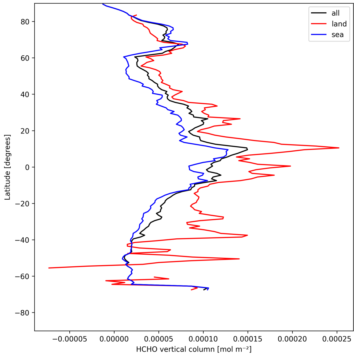
Figure 19: Zonal average of “HCHO vertical column” for 2025-05-06 to 2025-05-07.
