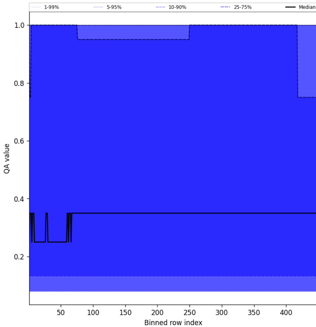
Figure 46: Along track statistics of “QA value” for 2025-05-06 to 2025-05-07
