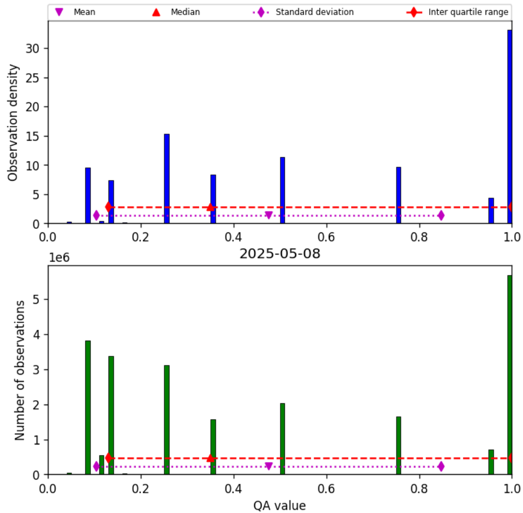
Figure 32: Histogram of “QA value” for 2025-05-08 to 2025-05-08
