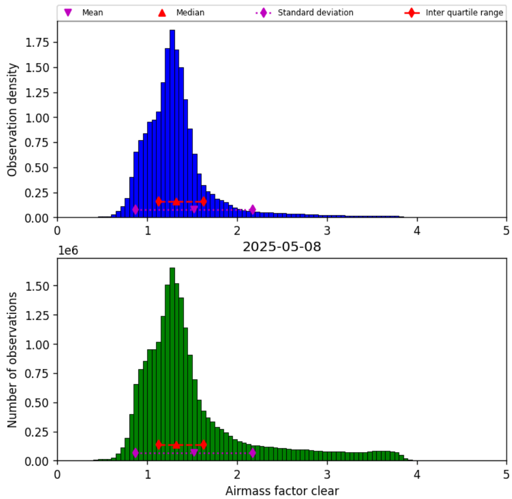
Figure 40: Histogram of “Airmass factor clear” for 2025-05-08 to 2025-05-08
