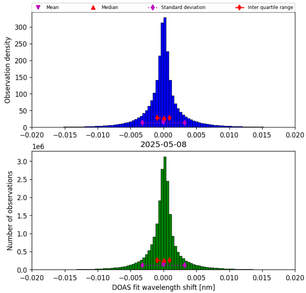
Figure 42: Histogram of “DOAS fit wavelength shift” for 2025-05-08 to 2025-05-08
