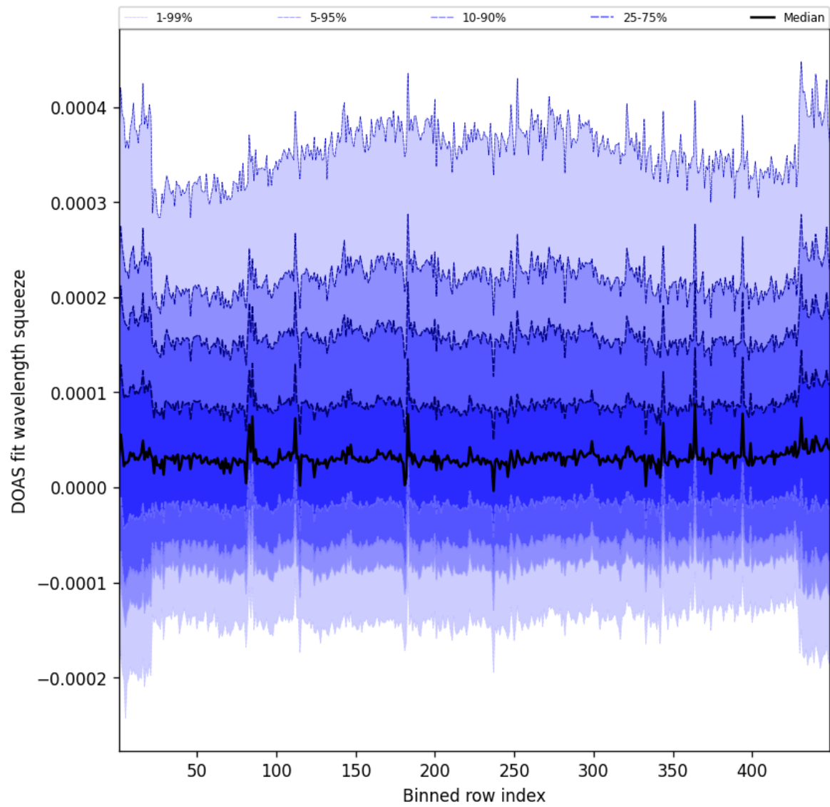
Figure 57: Along track statistics of “DOAS fit wavelength squeeze” for 2025-05-08 to 2025-05-08
