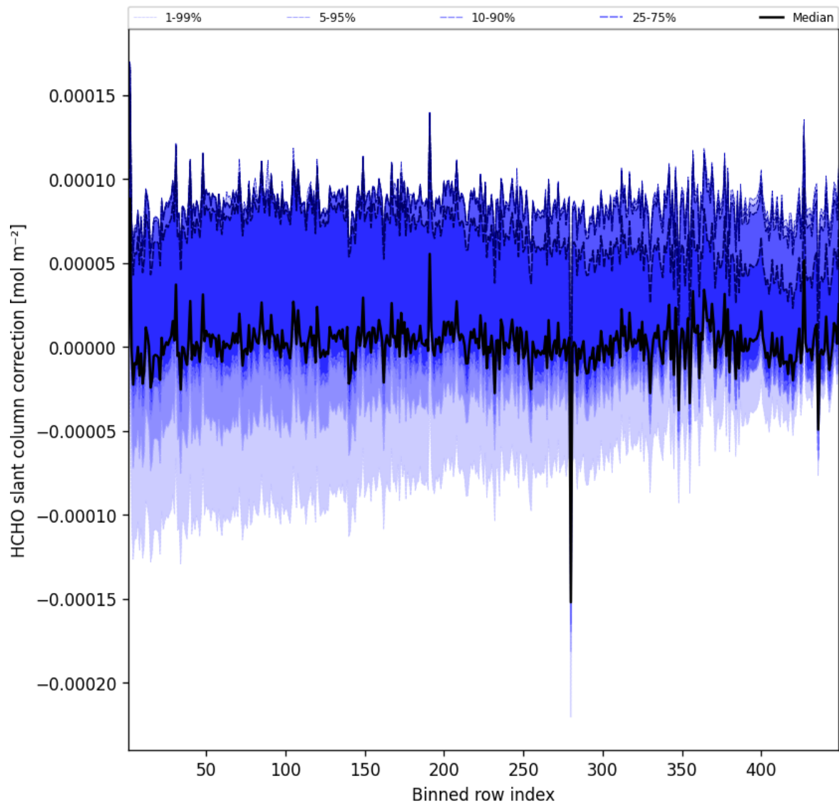
Figure 59: Along track statistics of “HCHO slant column correction” for 2025-05-08 to 2025-05-08
