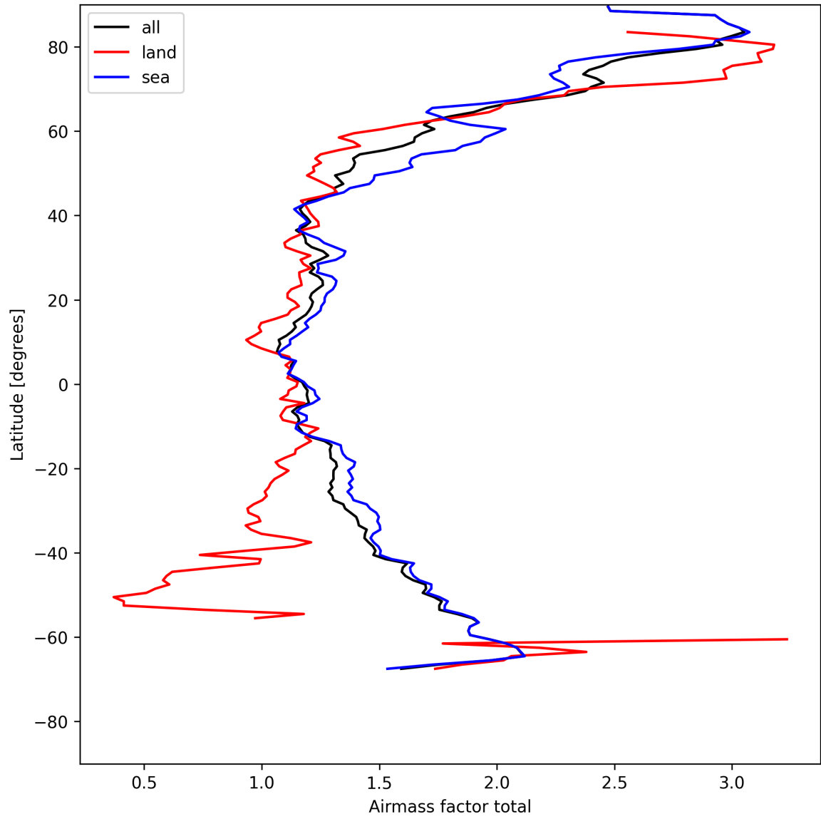
Figure 24: Zonal average of “Airmass factor total” for 2025-05-08 to 2025-05-08.
