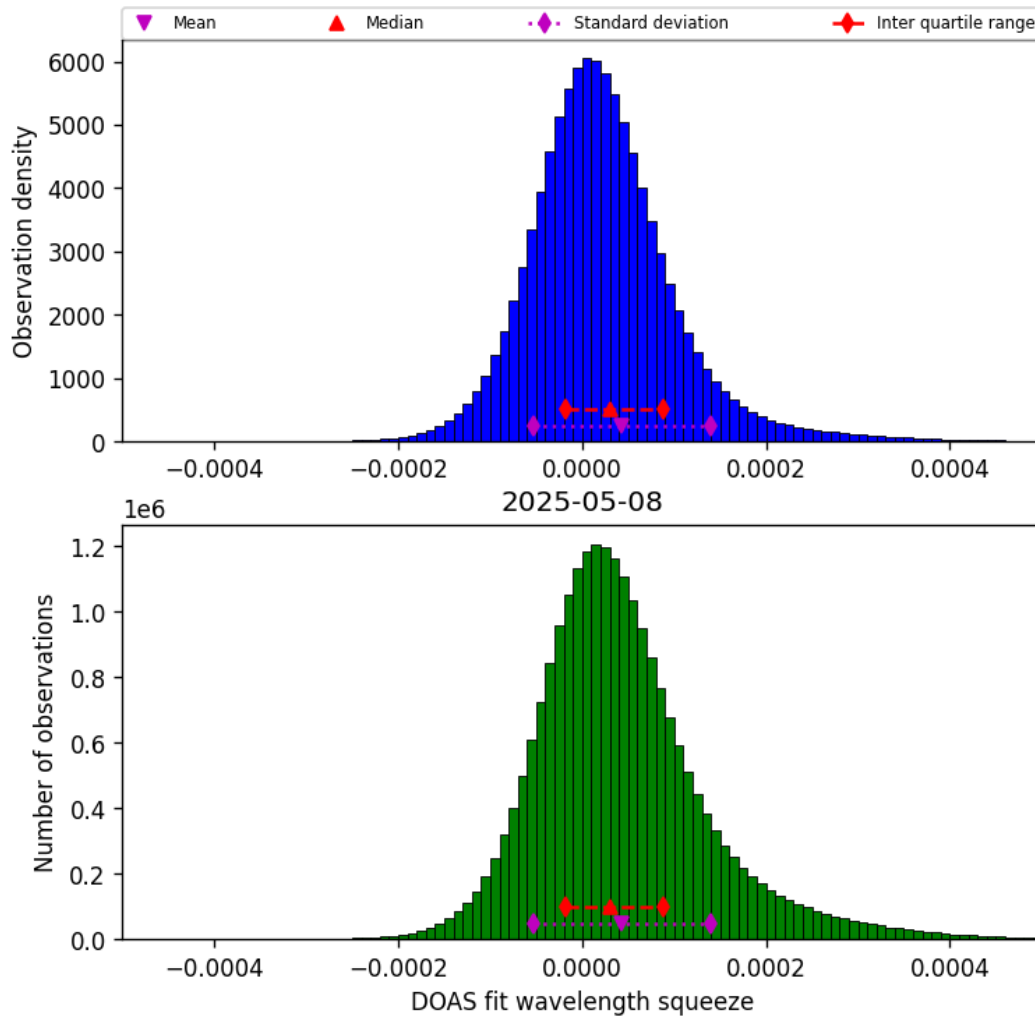
Figure 43: Histogram of “DOAS fit wavelength squeeze” for 2025-05-08 to 2025-05-08
