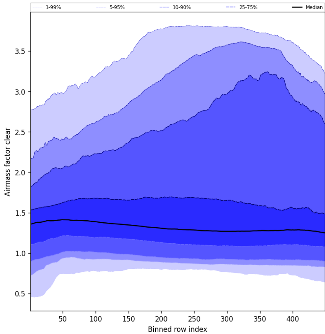
Figure 54: Along track statistics of “Airmass factor clear” for 2025-05-08 to 2025-05-08
