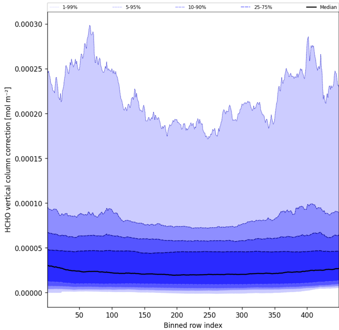
Figure 49: Along track statistics of “HCHO vertical column correction” for 2025-05-08 to 2025-05-08
