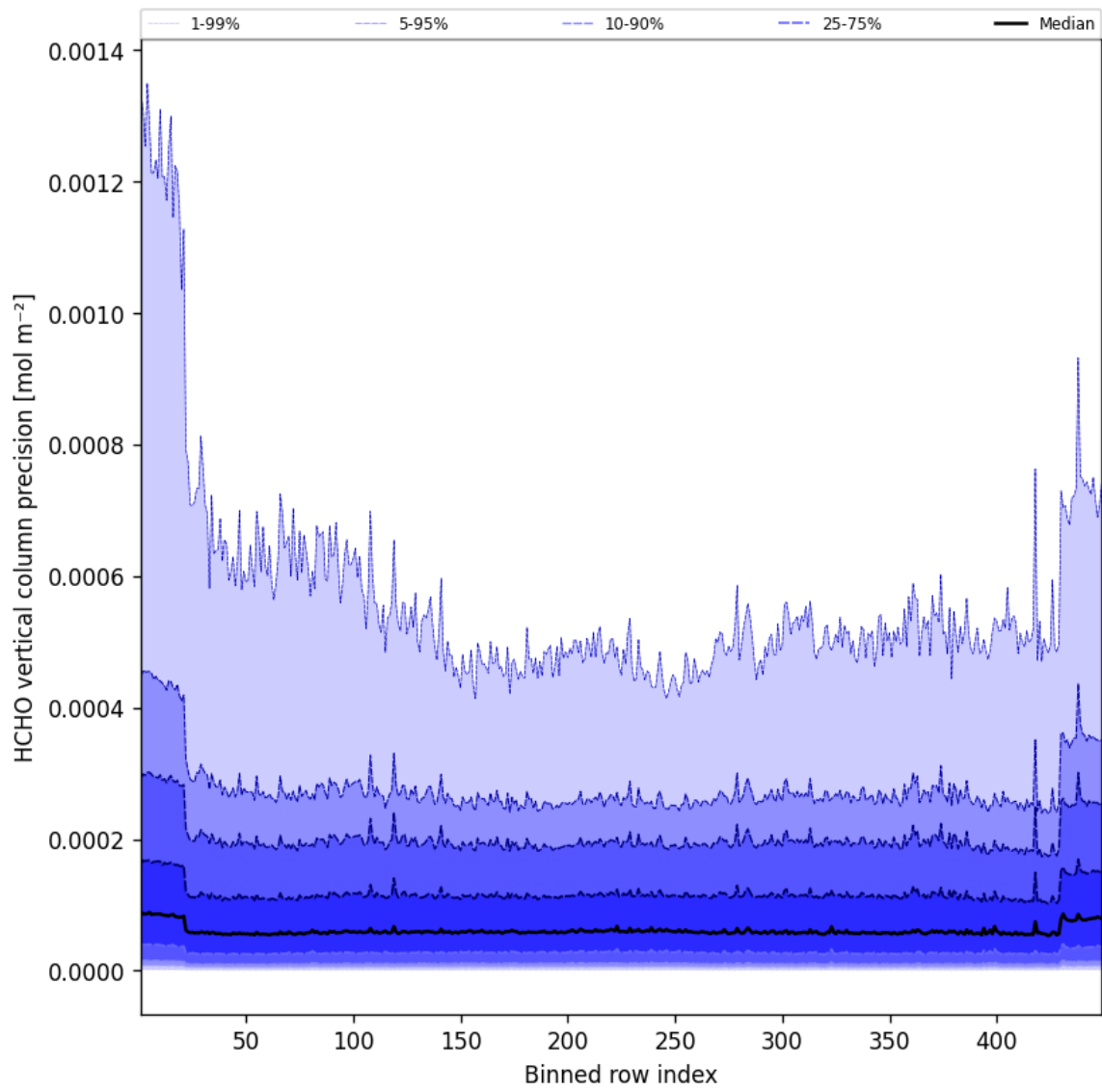
Figure 48: Along track statistics of “HCHO vertical column precision” for 2025-05-08 to 2025-05-08
