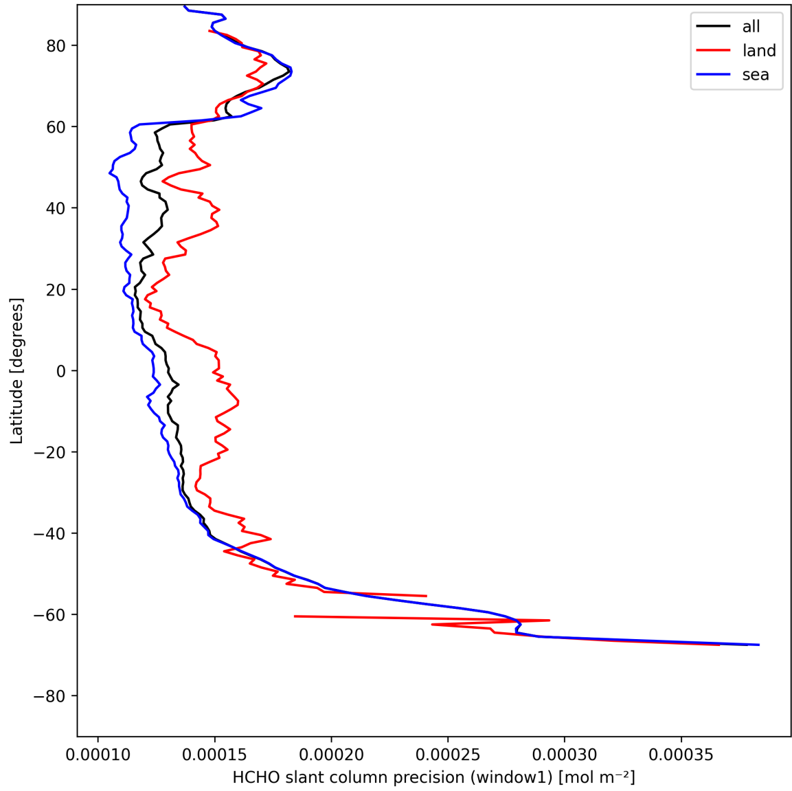
Figure 23: Zonal average of "HCHO slant column precision (window1)" for 2025-05-08 to 2025-05-08.
