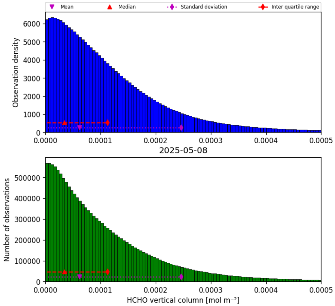
Figure 33: Histogram of “HCHO vertical column” for 2025-05-08 to 2025-05-08
