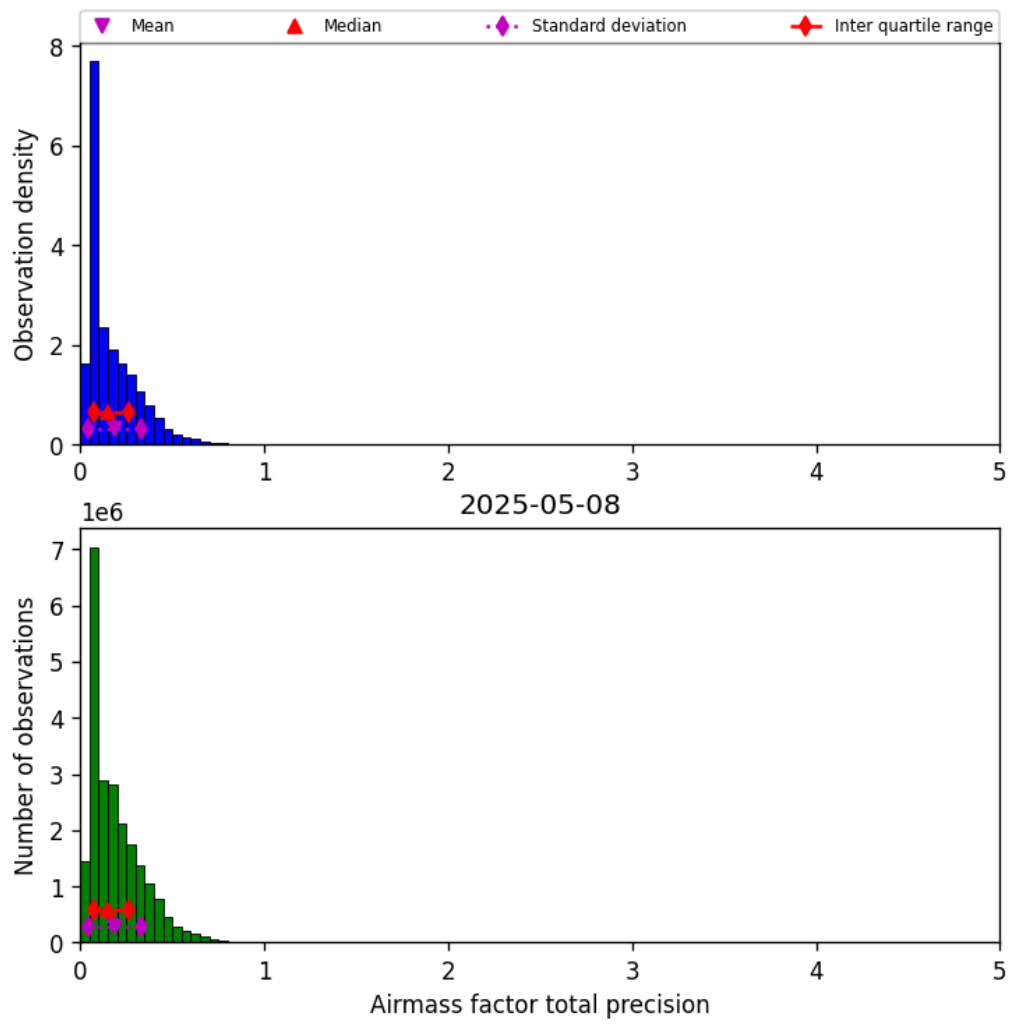
Figure 39: Histogram of “Airmass factor total precision” for 2025-05-08 to 2025-05-08
