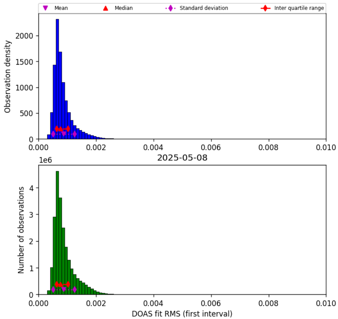
Figure 44: Histogram of “DOAS fit RMS (first interval)” for 2025-05-08 to 2025-05-08
