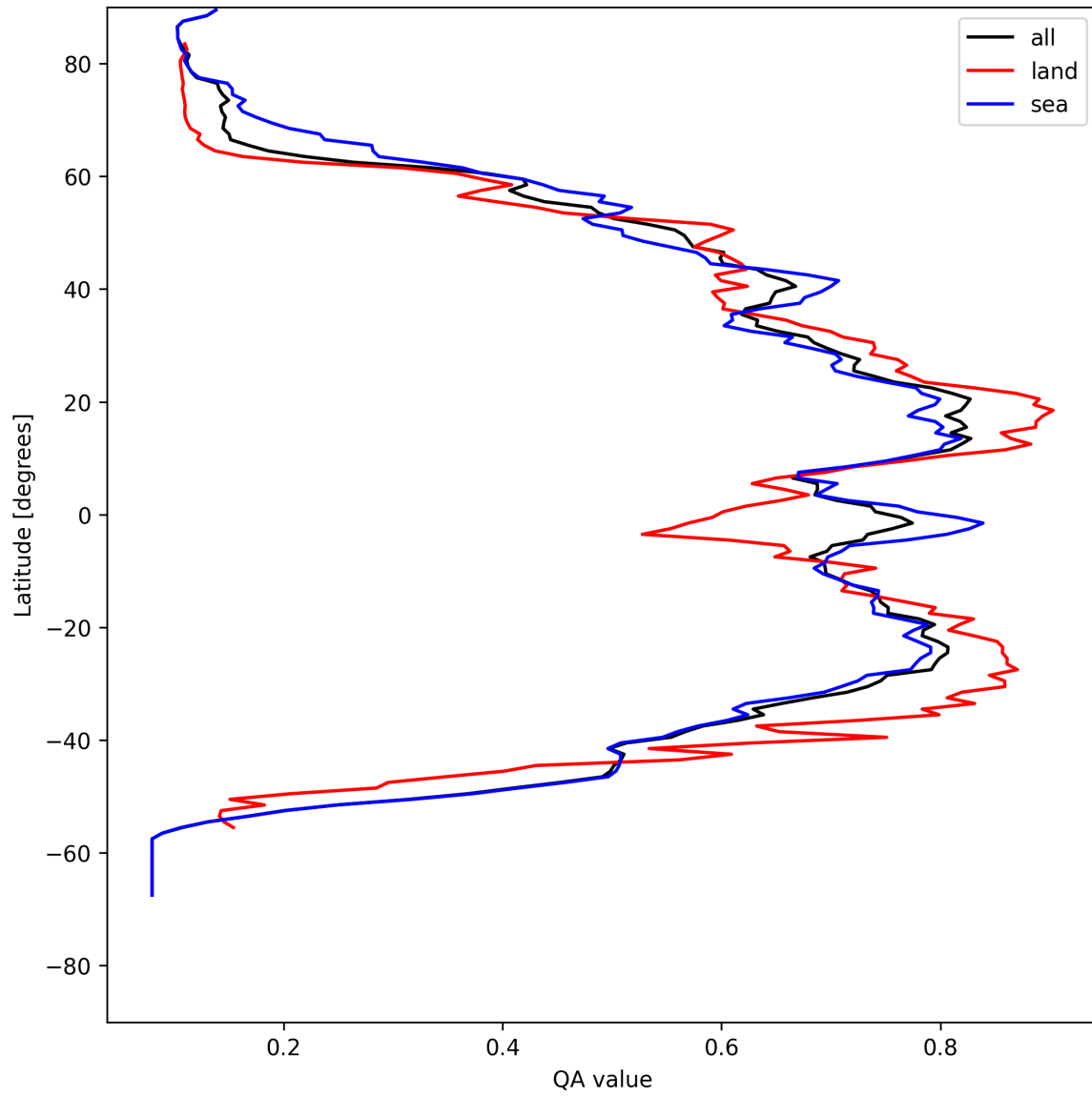
Figure 18: Zonal average of “QA value” for 2025-05-08 to 2025-05-08.
