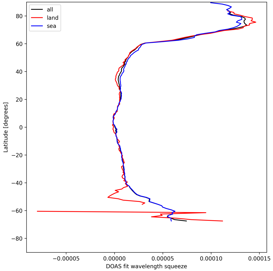
Figure 29: Zonal average of “DOAS fit wavelength squeeze” for 2025-05-08 to 2025-05-08.
