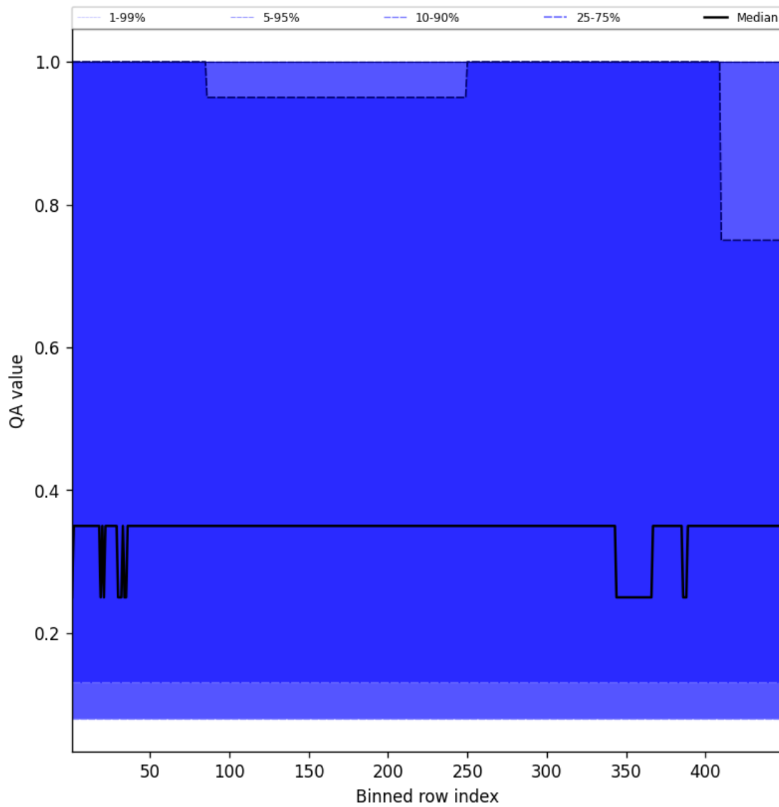
Figure 46: Along track statistics of “QA value” for 2025-05-08 to 2025-05-08
