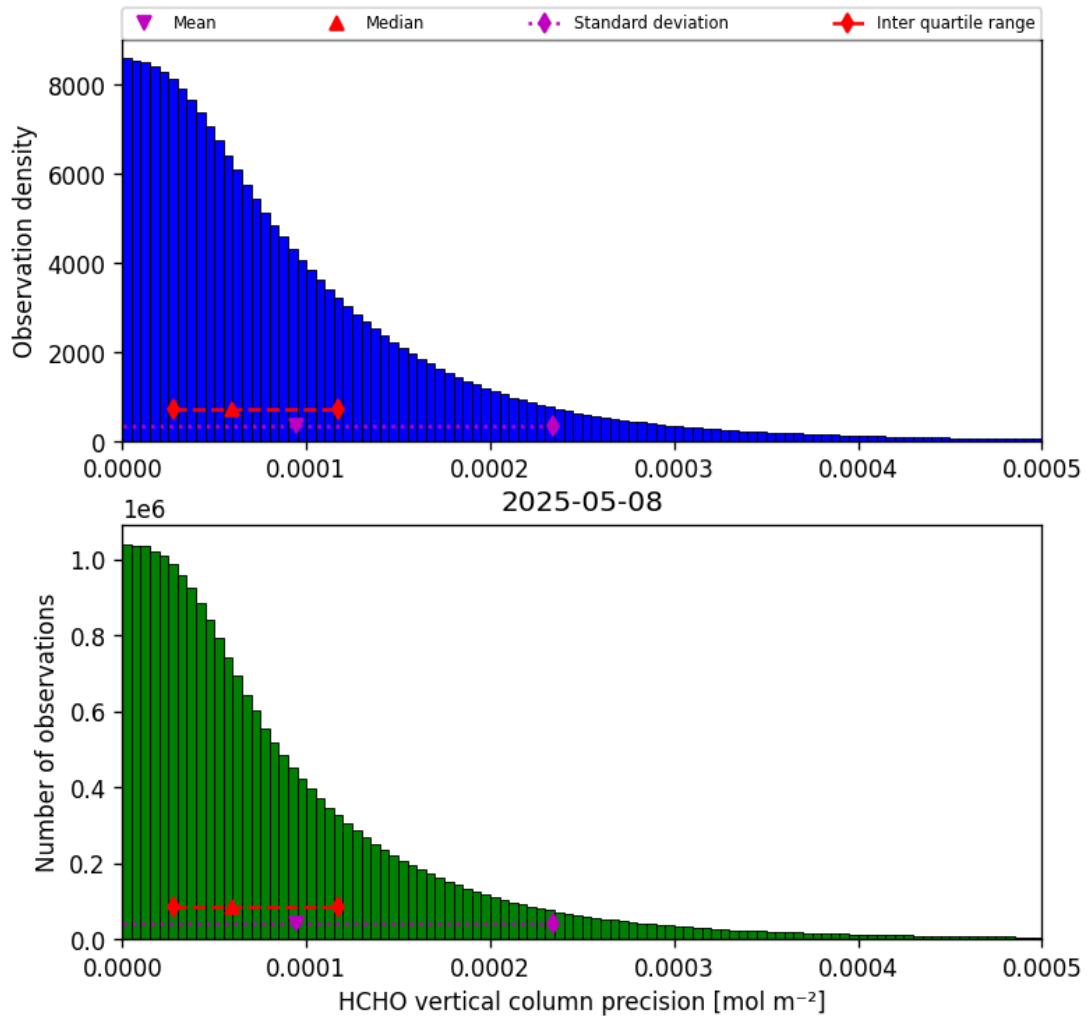
Figure 34: Histogram of “HCHO vertical column precision” for 2025-05-08 to 2025-05-08
