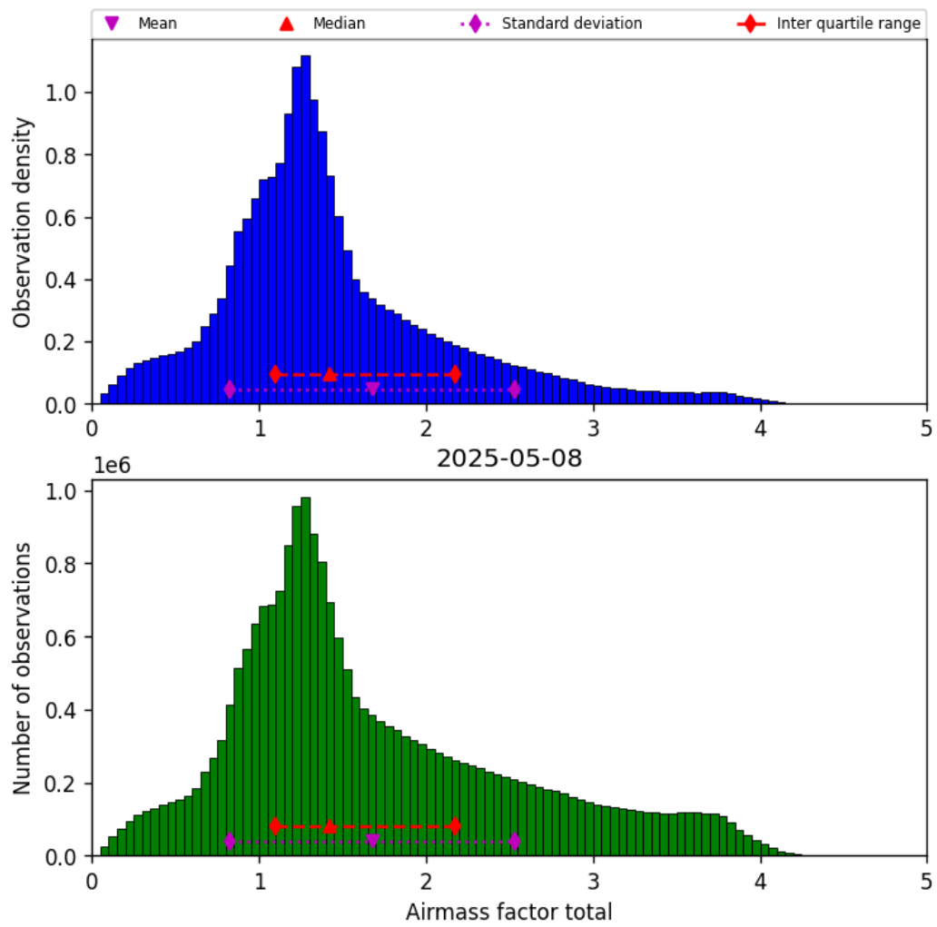
Figure 38: Histogram of “Airmass factor total” for 2025-05-08 to 2025-05-08
