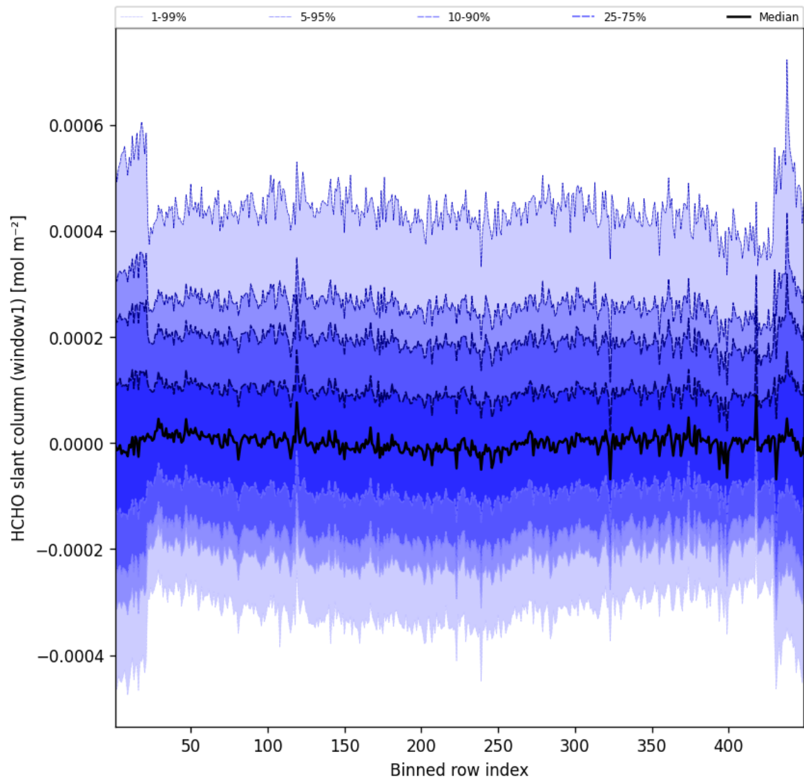
Figure 50: Along track statistics of “HCHO slant column (window1)” for 2025-05-08 to 2025-05-08
