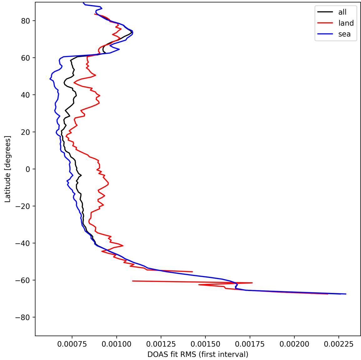
Figure 30: Zonal average of “DOAS fit RMS (first interval)” for 2025-05-08 to 2025-05-08.
