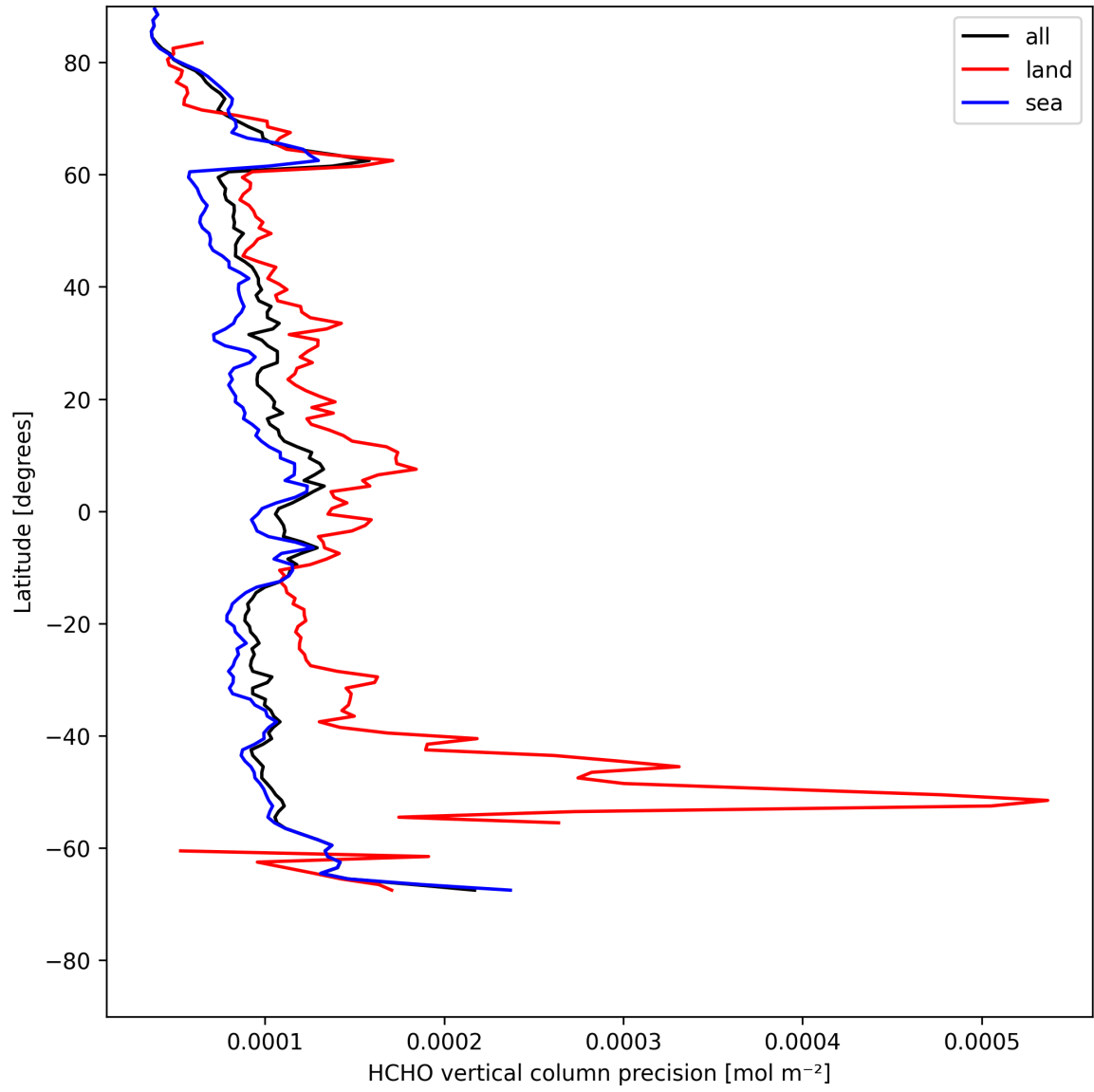
Figure 20: Zonal average of “HCHO vertical column precision” for 2025-05-08 to 2025-05-08.
