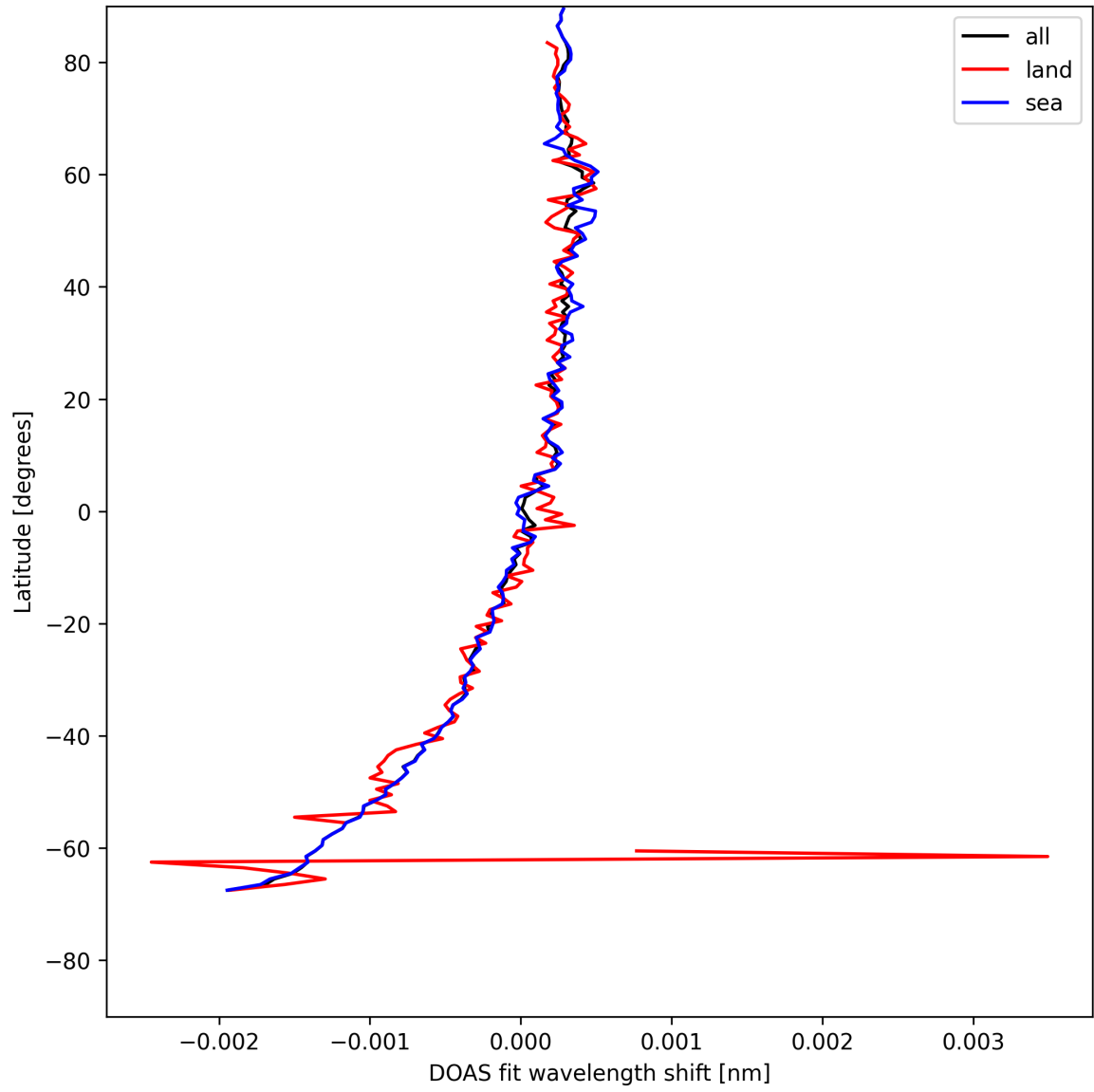
Figure 28: Zonal average of “DOAS fit wavelength shift” for 2025-05-08 to 2025-05-08.
