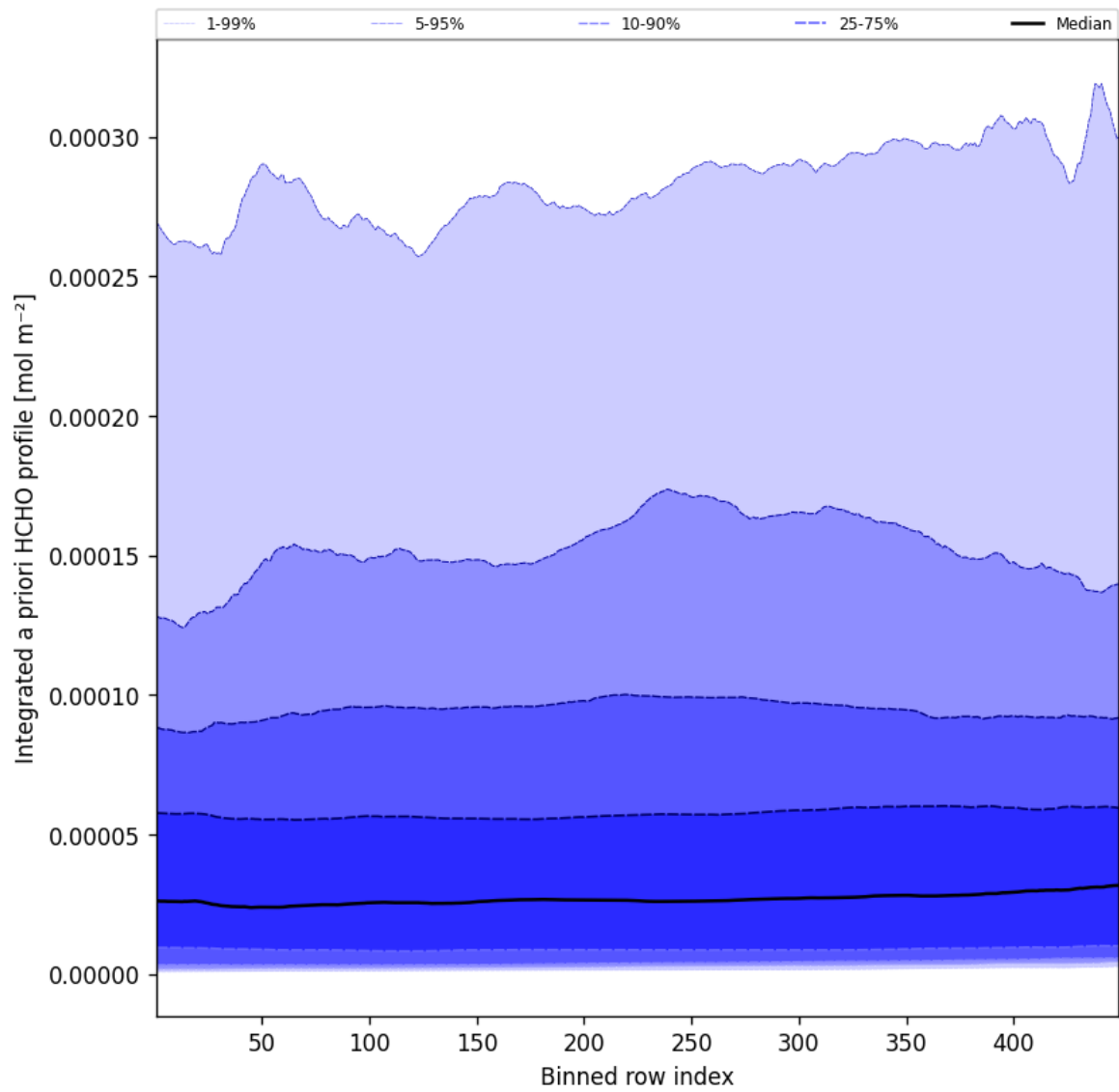
Figure 55: Along track statistics of “Integrated a priori HCHO profile” for 2025-05-08 to 2025-05-08
