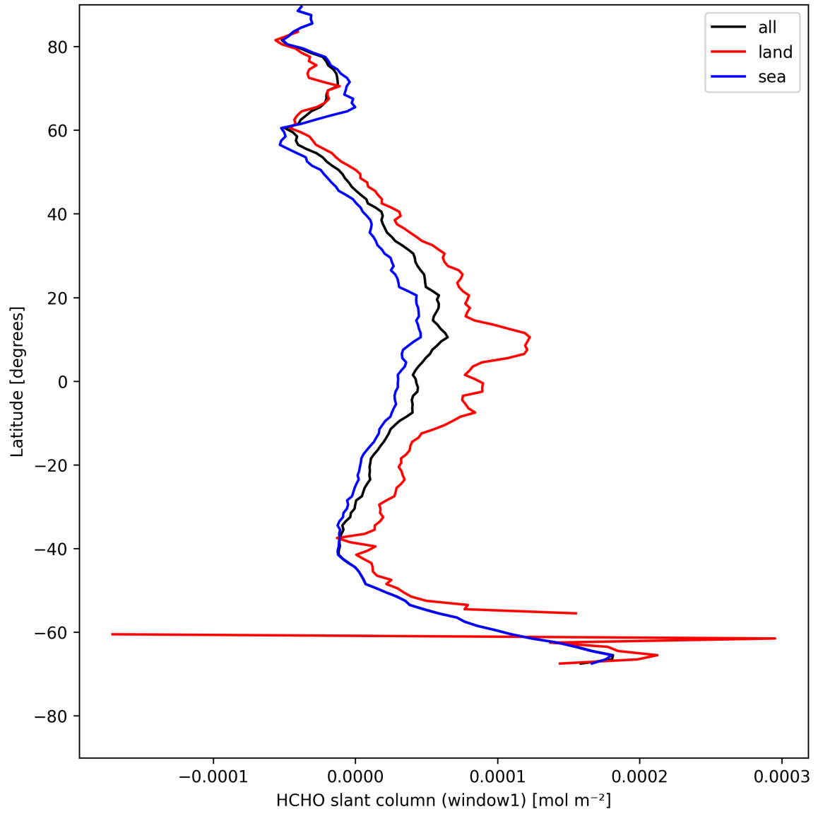
Figure 22: Zonal average of “HCHO slant column (window1)” for 2025-05-08 to 2025-05-08.
