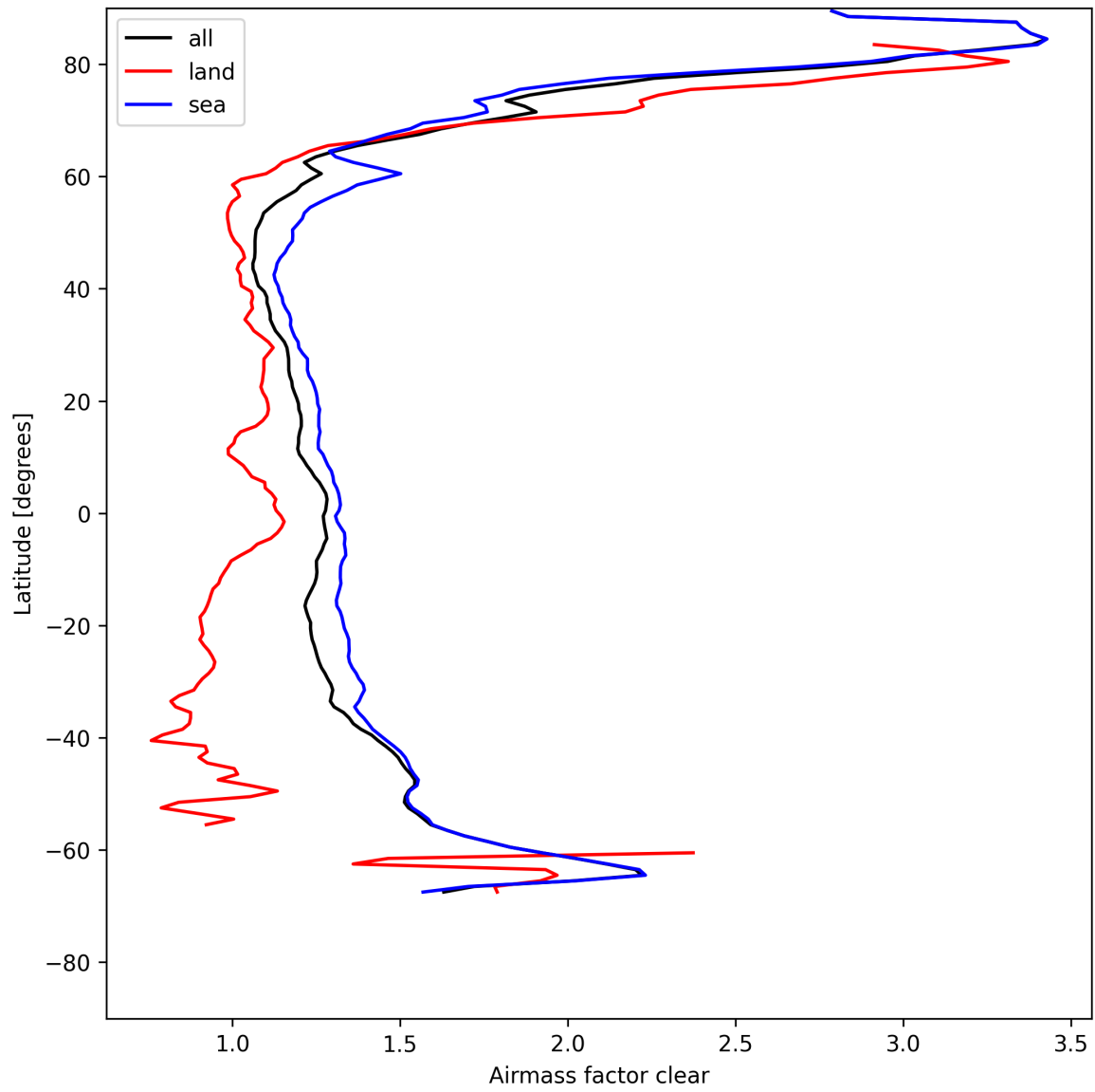
Figure 26: Zonal average of “Airmass factor clear” for 2025-05-08 to 2025-05-08.
