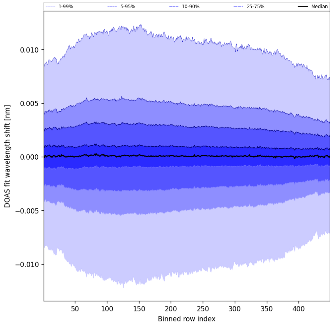
Figure 56: Along track statistics of “DOAS fit wavelength shift” for 2025-05-08 to 2025-05-08
