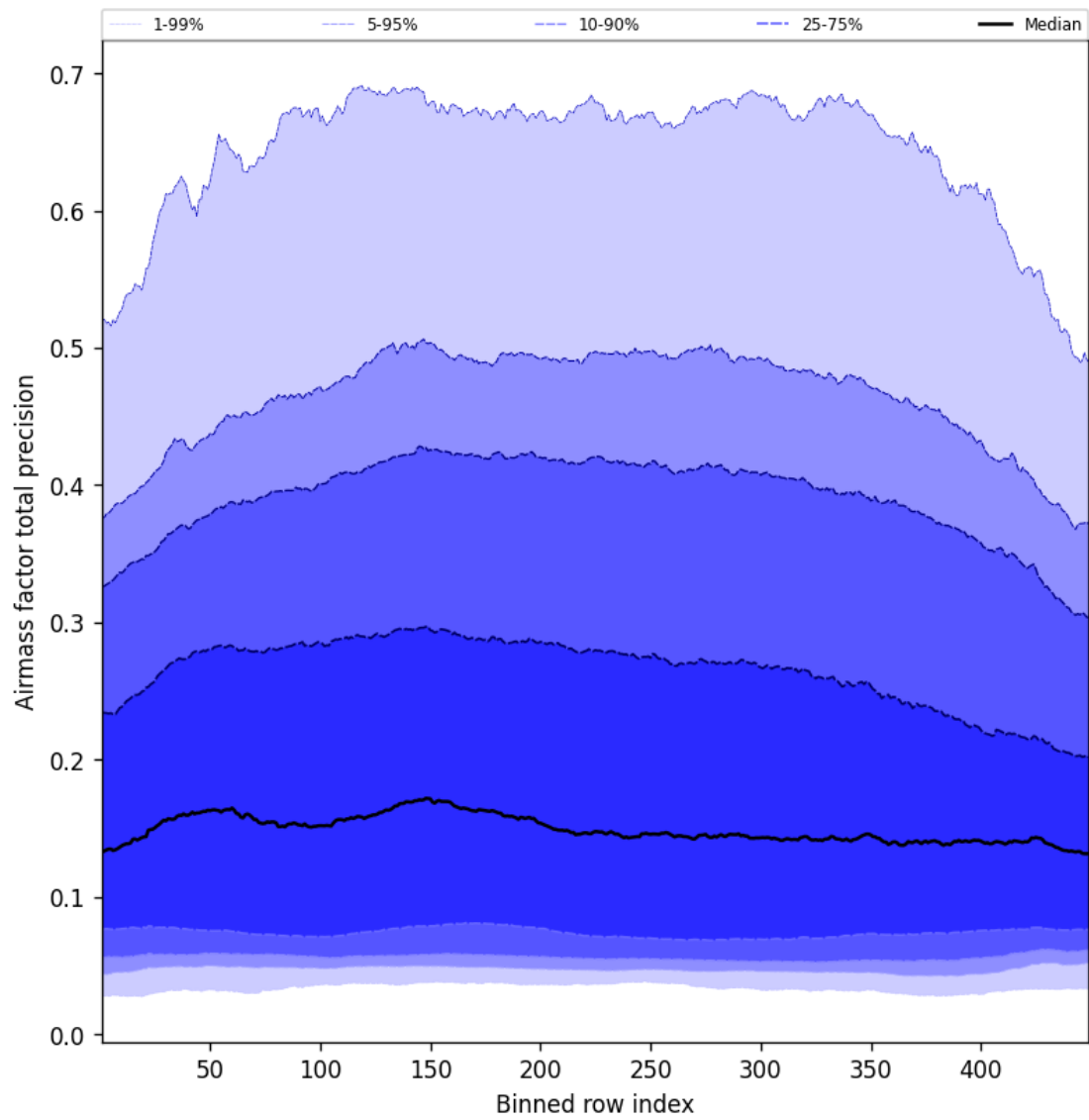
Figure 53: Along track statistics of “Airmass factor total precision” for 2025-05-08 to 2025-05-08
