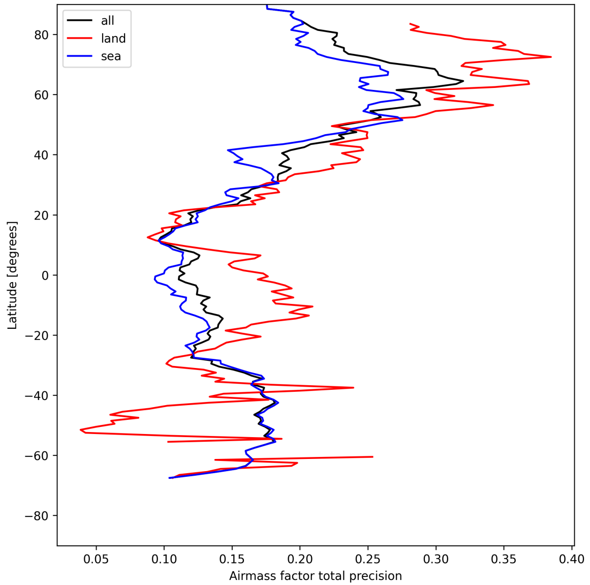
Figure 25: Zonal average of “Airmass factor total precision” for 2025-05-08 to 2025-05-08.
