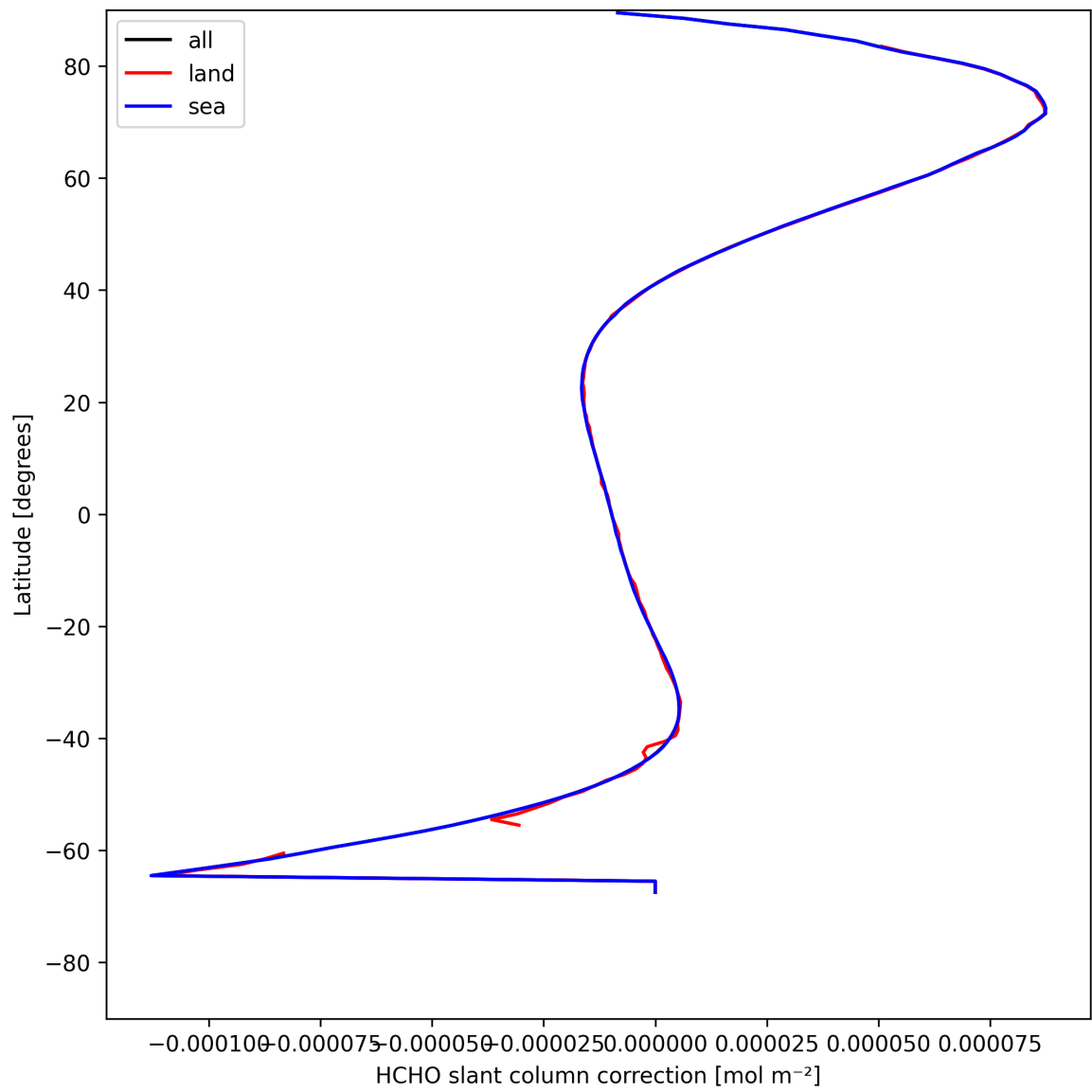
Figure 31: Zonal average of “HCHO slant column correction” for 2025-05-08 to 2025-05-08.
