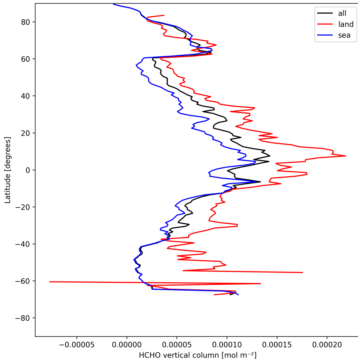
Figure 19: Zonal average of “HCHO vertical column” for 2025-05-08 to 2025-05-08.
