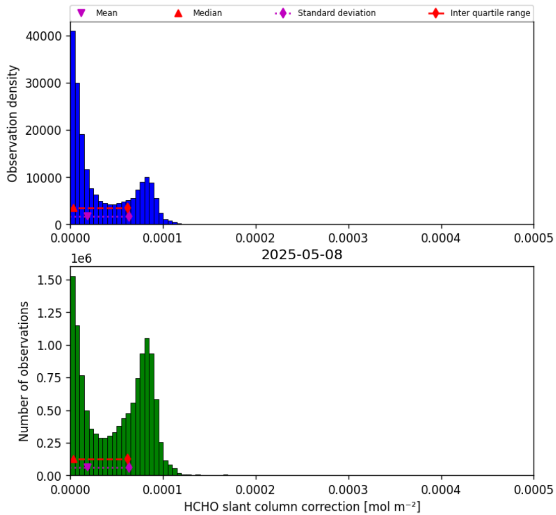
Figure 45: Histogram of “HCHO slant column correction” for 2025-05-08 to 2025-05-08
