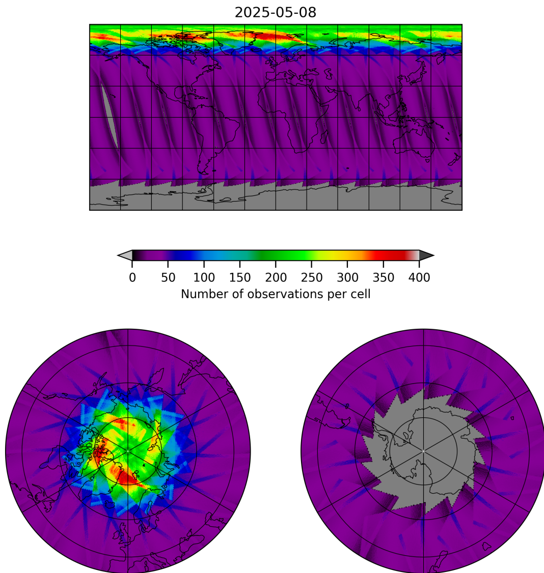
Figure 17: Map of the number of observations for 2025-05-08 to 2025-05-08
