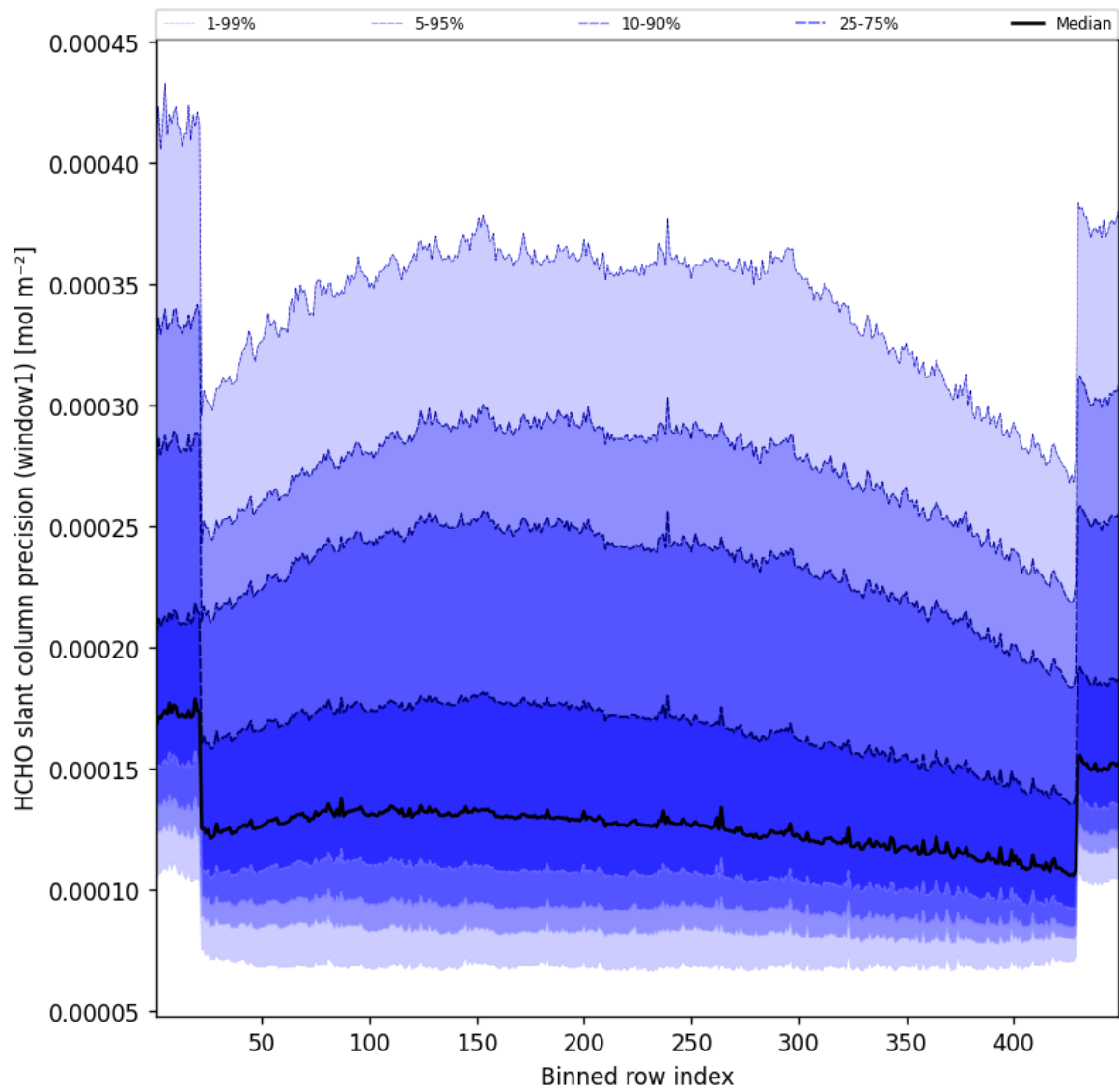
Figure 51: Along track statistics of “HCHO slant column precision (window1)” for 2025-05-08 to 2025-05-08
