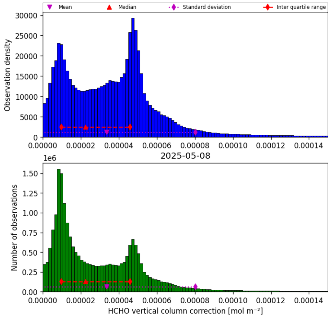
Figure 35: Histogram of “HCHO vertical column correction” for 2025-05-08 to 2025-05-08
