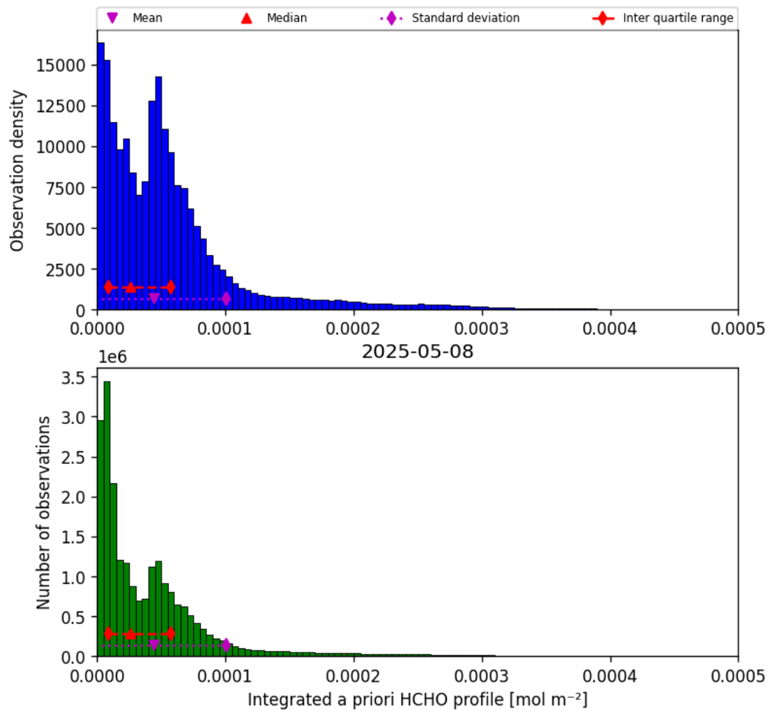
Figure 41: Histogram of “Integrated a priori HCHO profile” for 2025-05-08 to 2025-05-08
