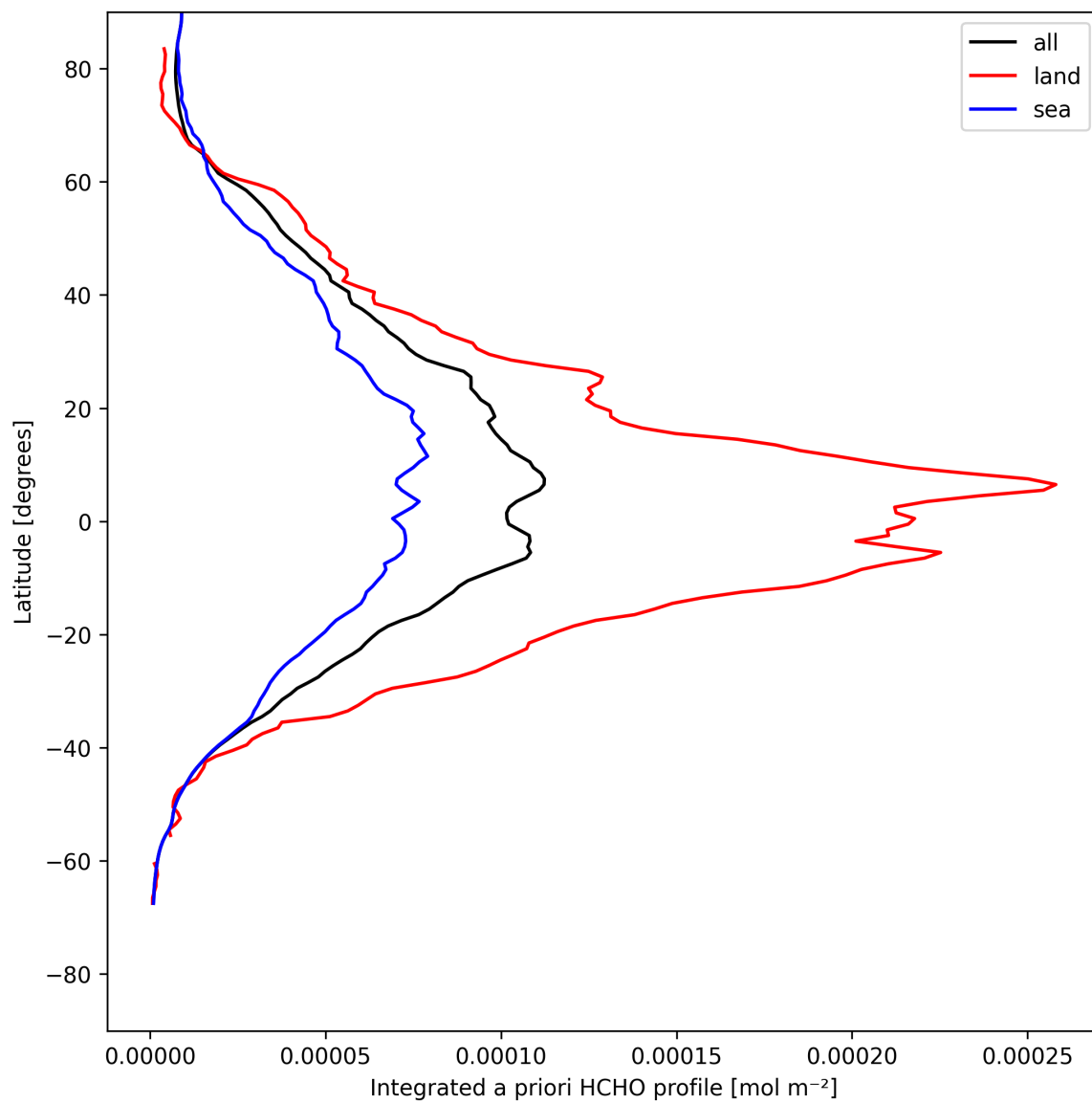
Figure 27: Zonal average of “Integrated a priori HCHO profile” for 2025-05-08 to 2025-05-08.
