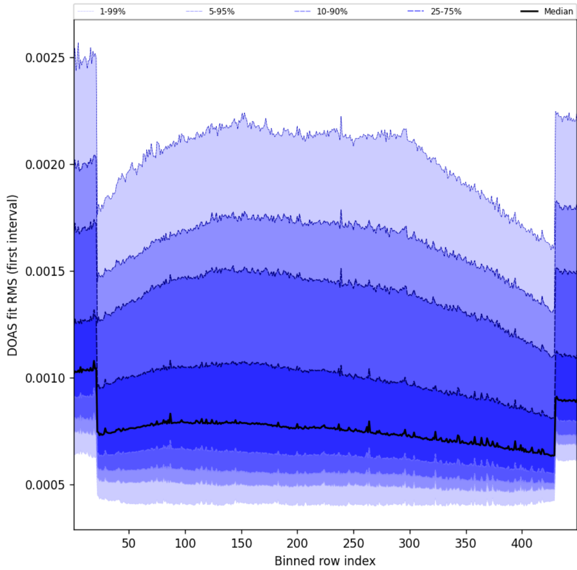
Figure 58: Along track statistics of “DOAS fit RMS (first interval)” for 2025-05-08 to 2025-05-08
