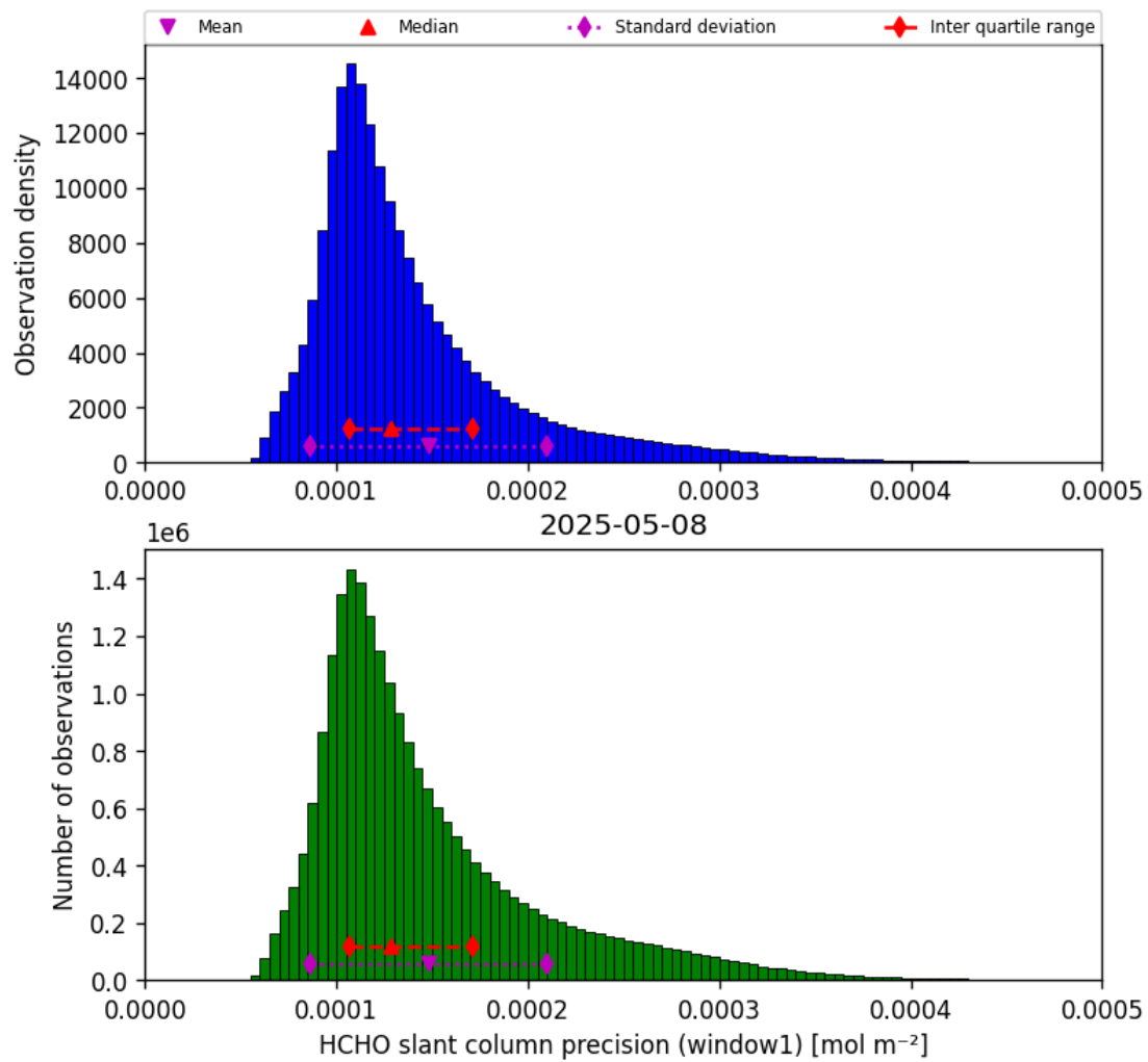
Figure 37: Histogram of “HCHO slant column precision (window1)” for 2025-05-08 to 2025-05-08
