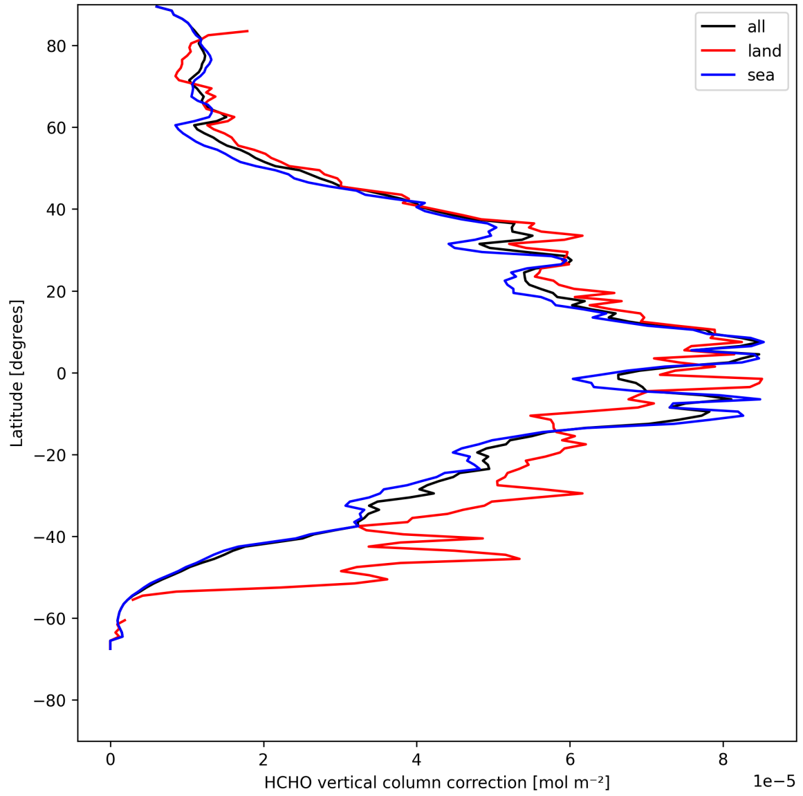
Figure 21: Zonal average of “HCHO vertical column correction” for 2025-05-08 to 2025-05-08.
