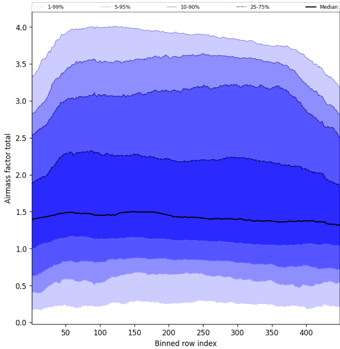
Figure 52: Along track statistics of “Airmass factor total” for 2025-05-08 to 2025-05-08
