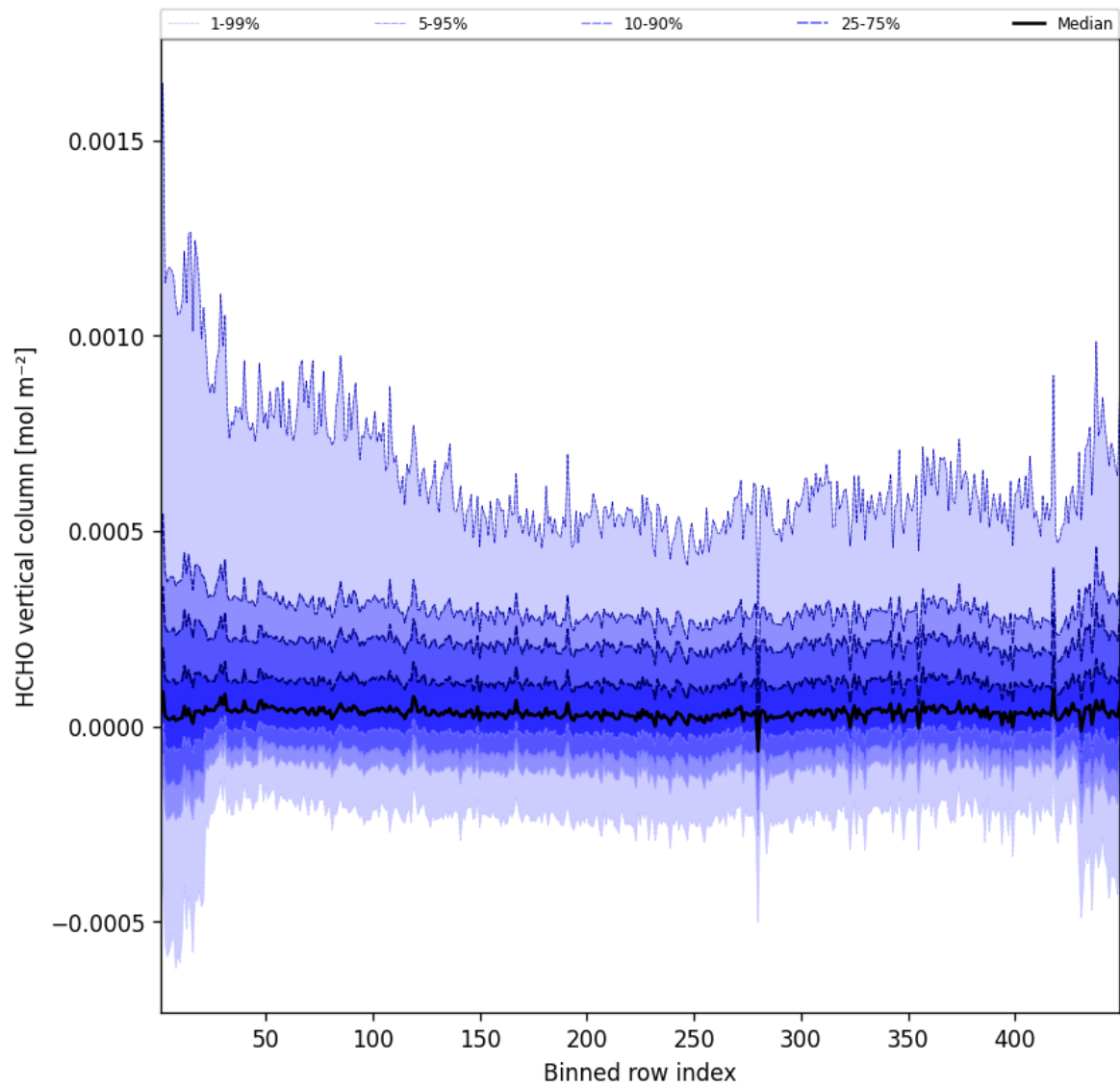
Figure 47: Along track statistics of “HCHO vertical column” for 2025-05-08 to 2025-05-08
