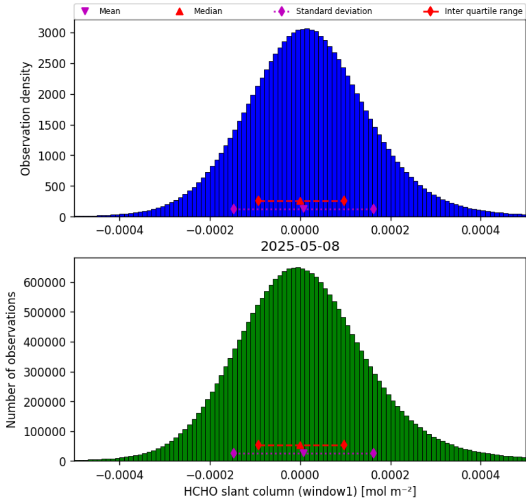
Figure 36: Histogram of “HCHO slant column (window1)” for 2025-05-08 to 2025-05-08
