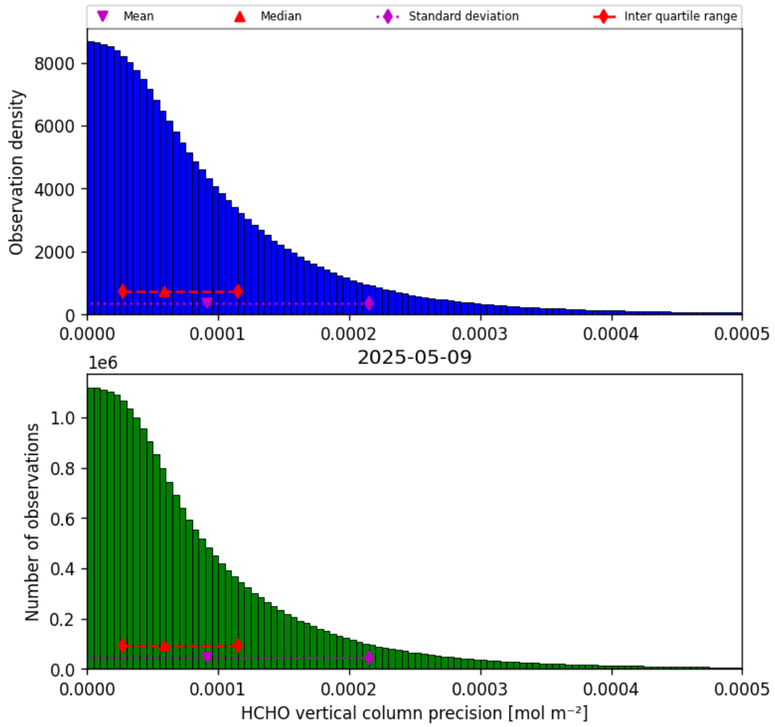
Figure 34: Histogram of “HCHO vertical column precision” for 2025-05-09 to 2025-05-10
