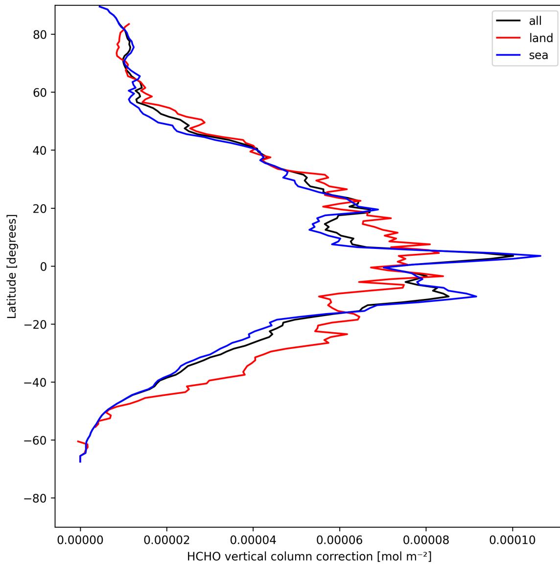
Figure 21: Zonal average of “HCHO vertical column correction” for 2025-05-09 to 2025-05-10.
