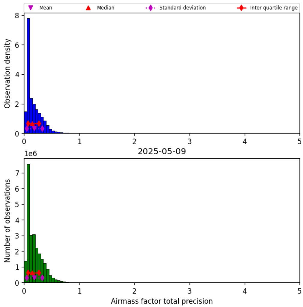
Figure 39: Histogram of “Airmass factor total precision” for 2025-05-09 to 2025-05-10
