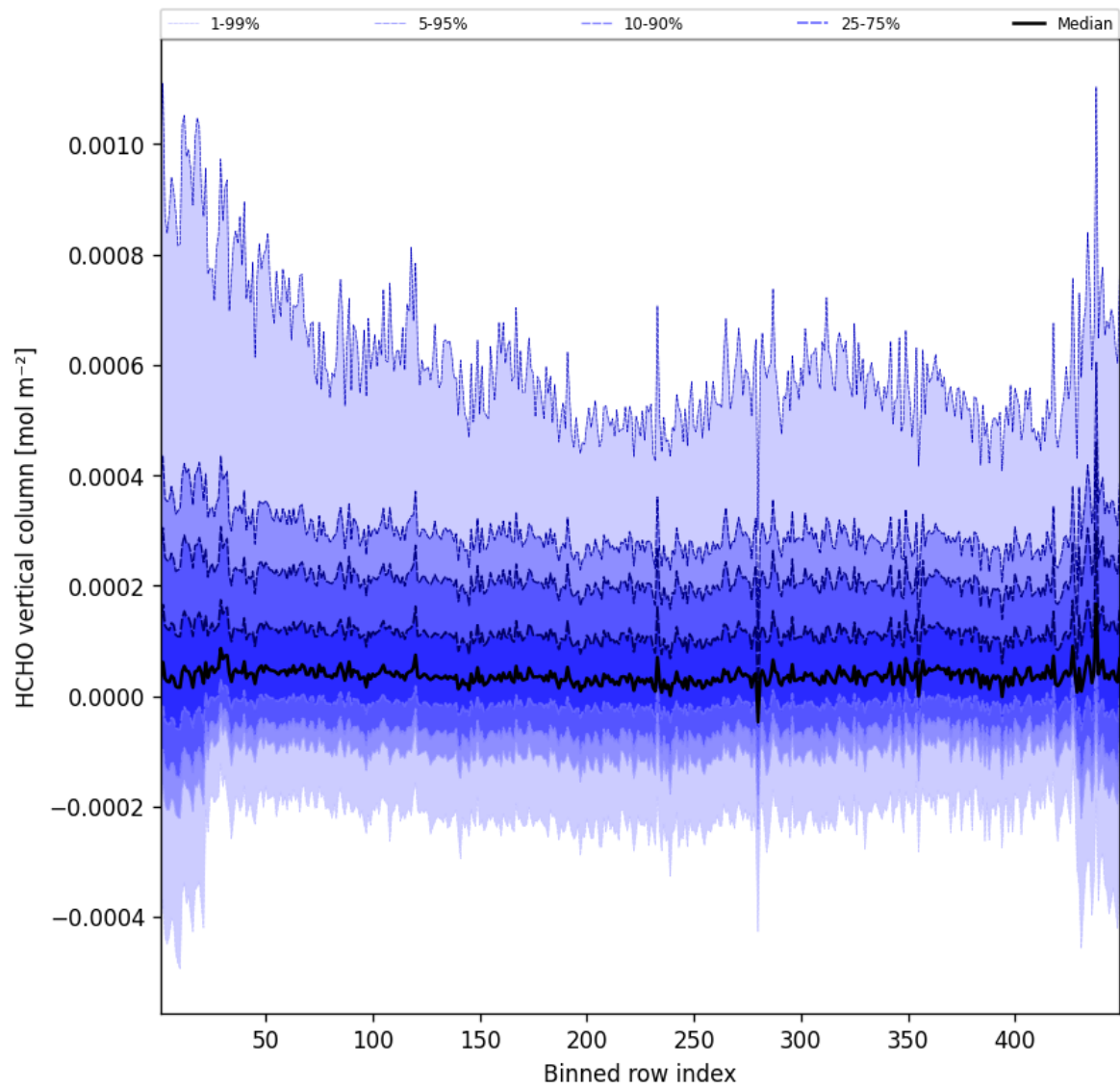
Figure 47: Along track statistics of “HCHO vertical column” for 2025-05-09 to 2025-05-10
