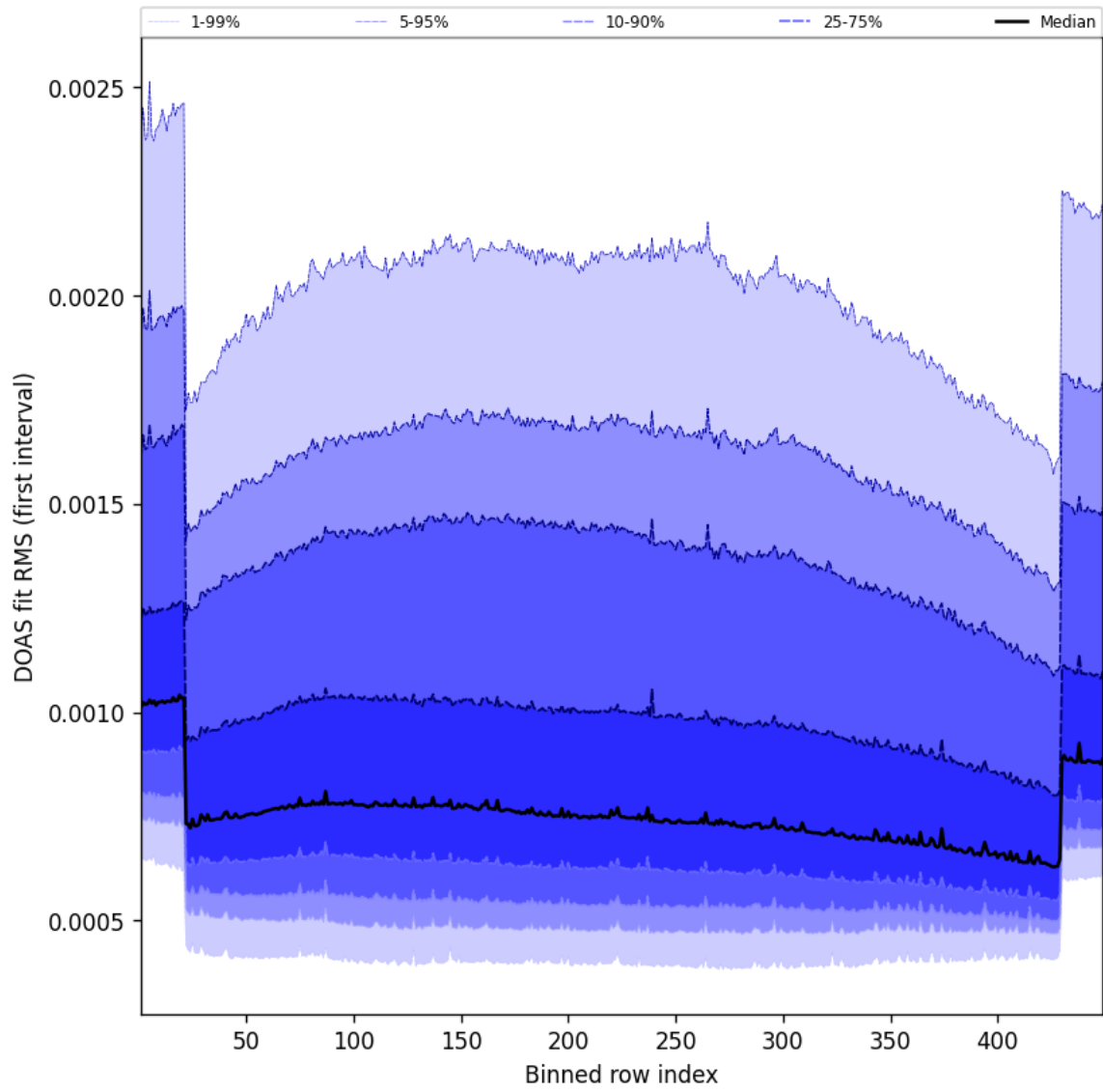
Figure 58: Along track statistics of “DOAS fit RMS (first interval)” for 2025-05-09 to 2025-05-10
