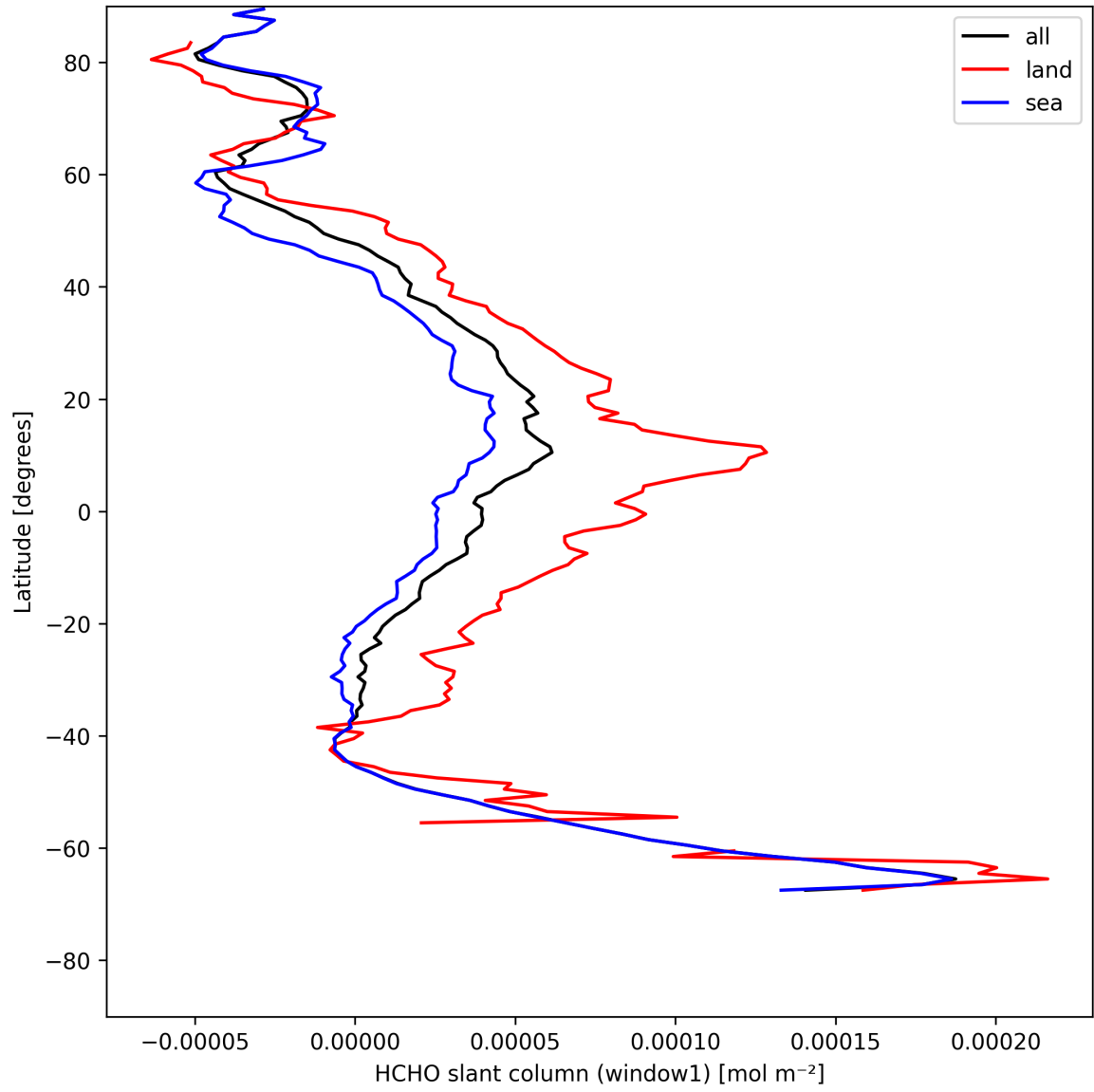
Figure 22: Zonal average of “HCHO slant column (window1)” for 2025-05-09 to 2025-05-10.
