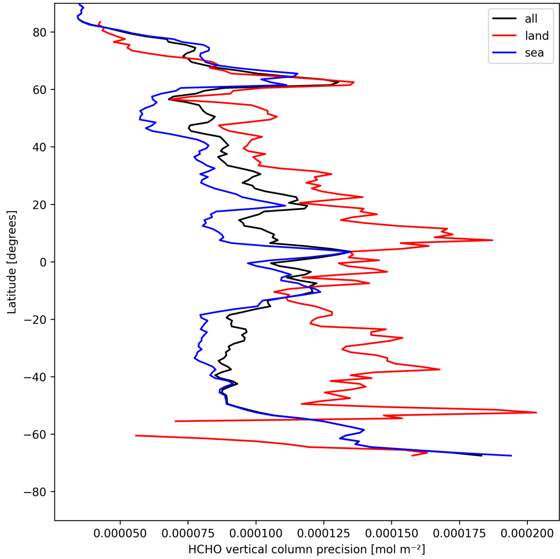
Figure 20: Zonal average of “HCHO vertical column precision” for 2025-05-09 to 2025-05-10.
