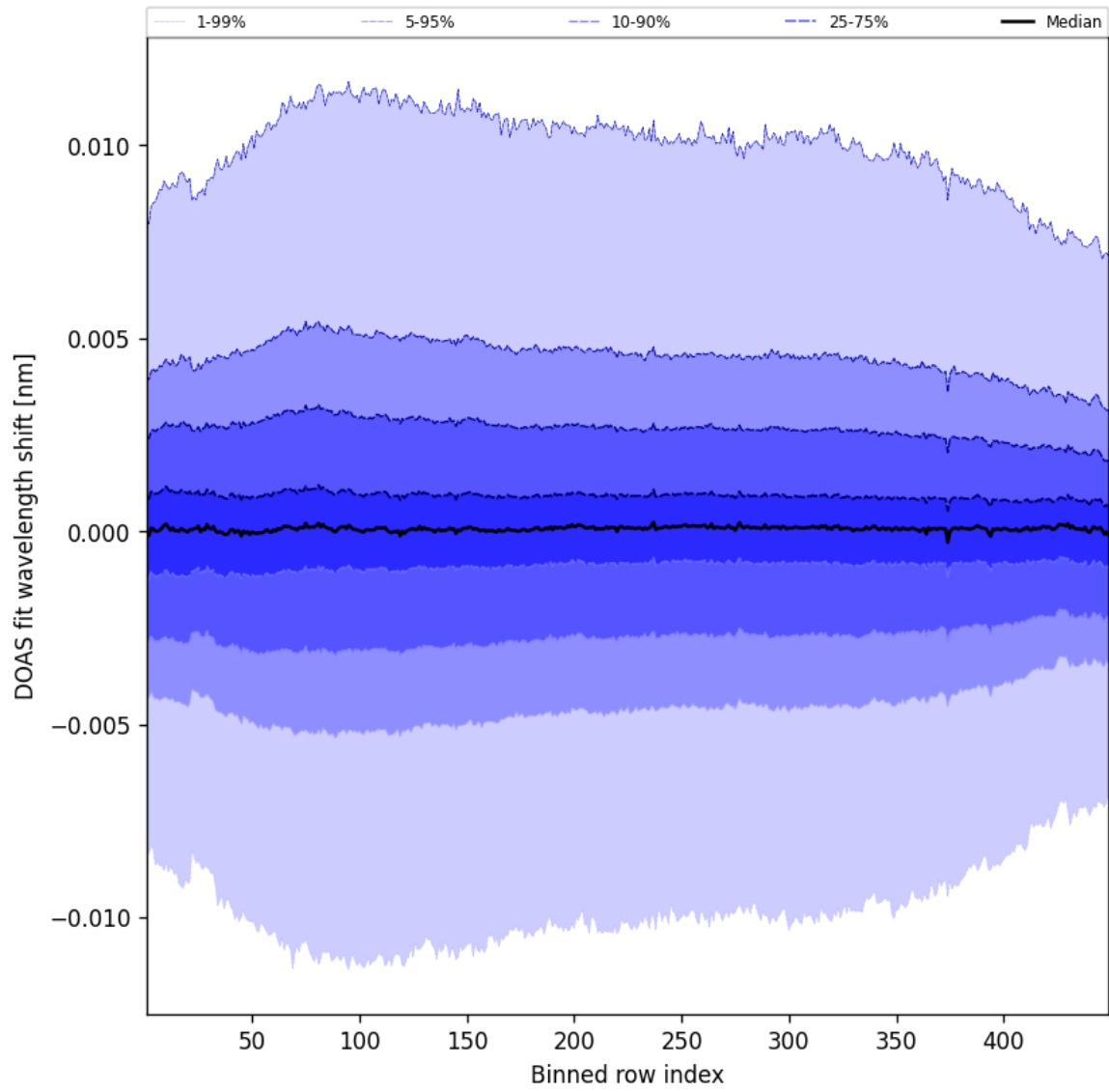
Figure 56: Along track statistics of “DOAS fit wavelength shift” for 2025-05-09 to 2025-05-10
