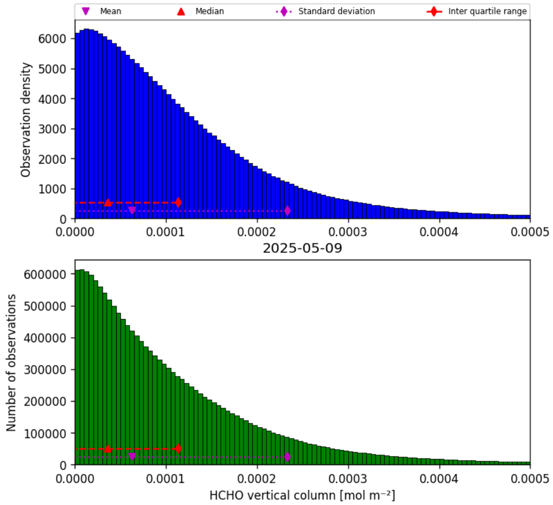
Figure 33: Histogram of “HCHO vertical column” for 2025-05-09 to 2025-05-10
