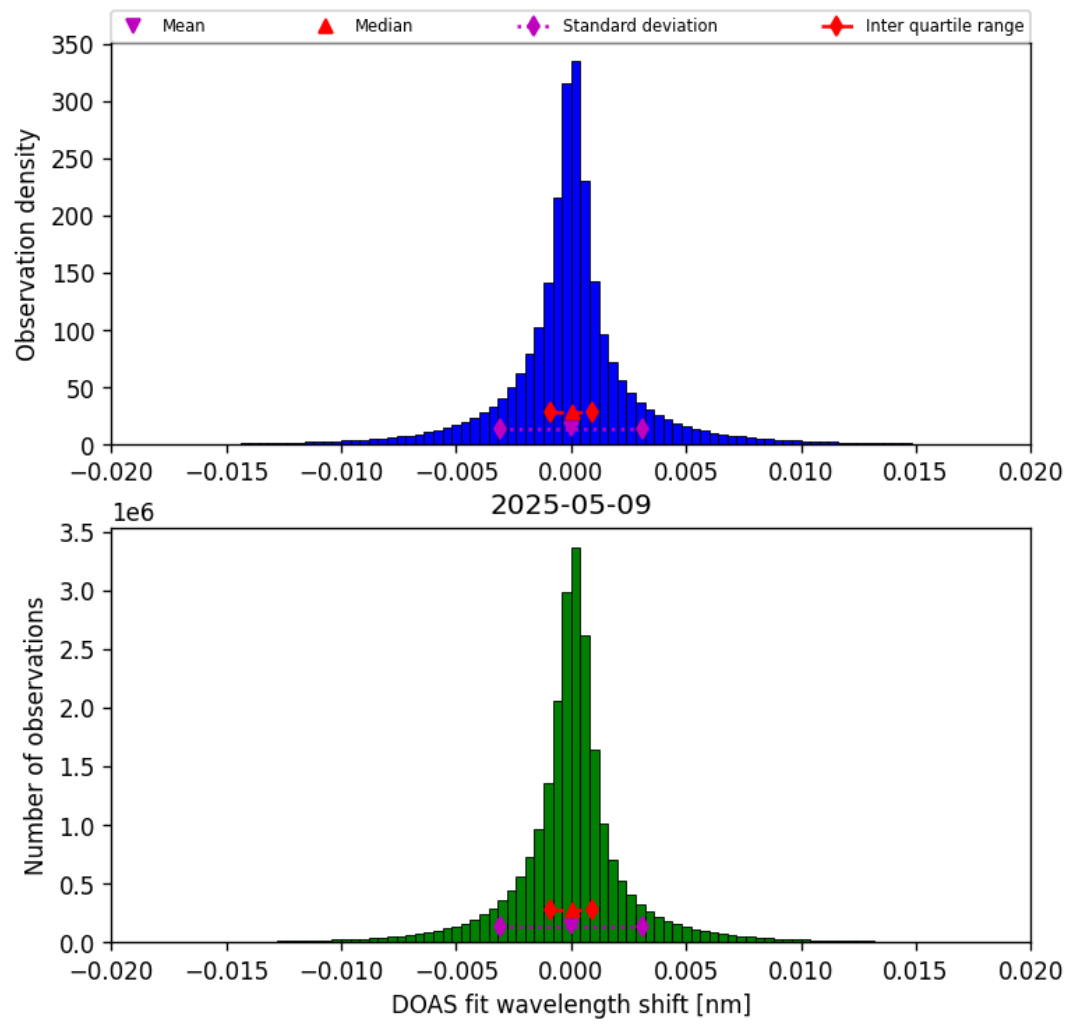
Figure 42: Histogram of “DOAS fit wavelength shift” for 2025-05-09 to 2025-05-10
