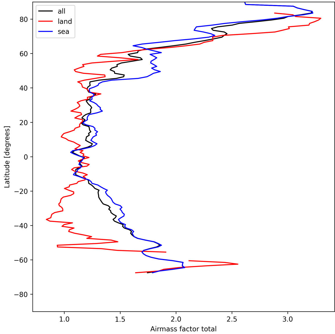
Figure 24: Zonal average of “Airmass factor total” for 2025-05-09 to 2025-05-10.
