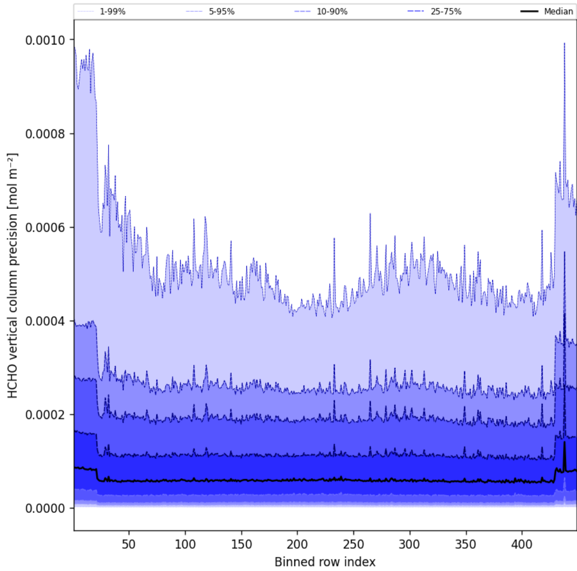
Figure 48: Along track statistics of “HCHO vertical column precision” for 2025-05-09 to 2025-05-10
