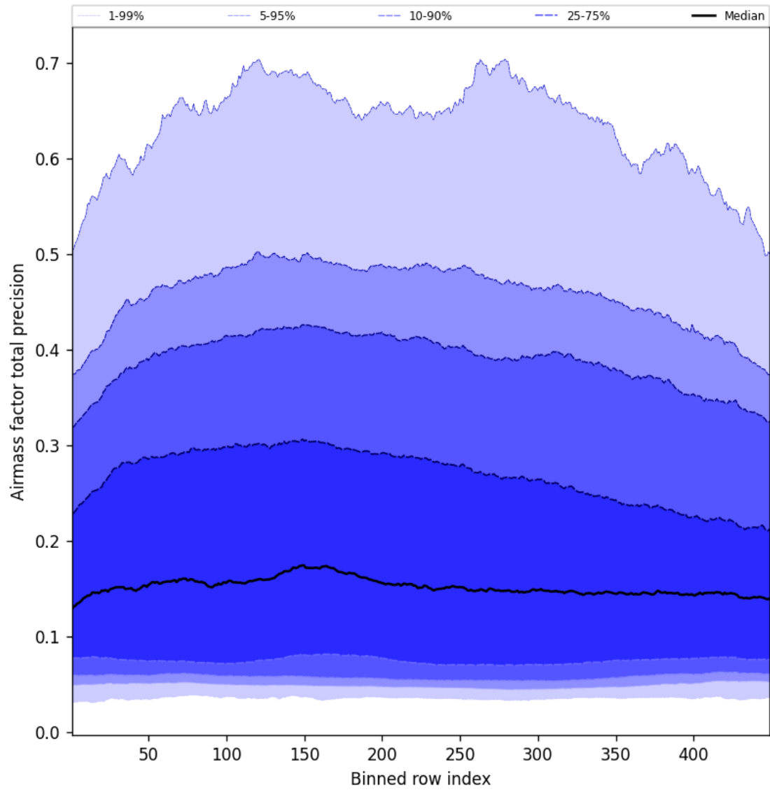
Figure 53: Along track statistics of “Airmass factor total precision” for 2025-05-09 to 2025-05-10
