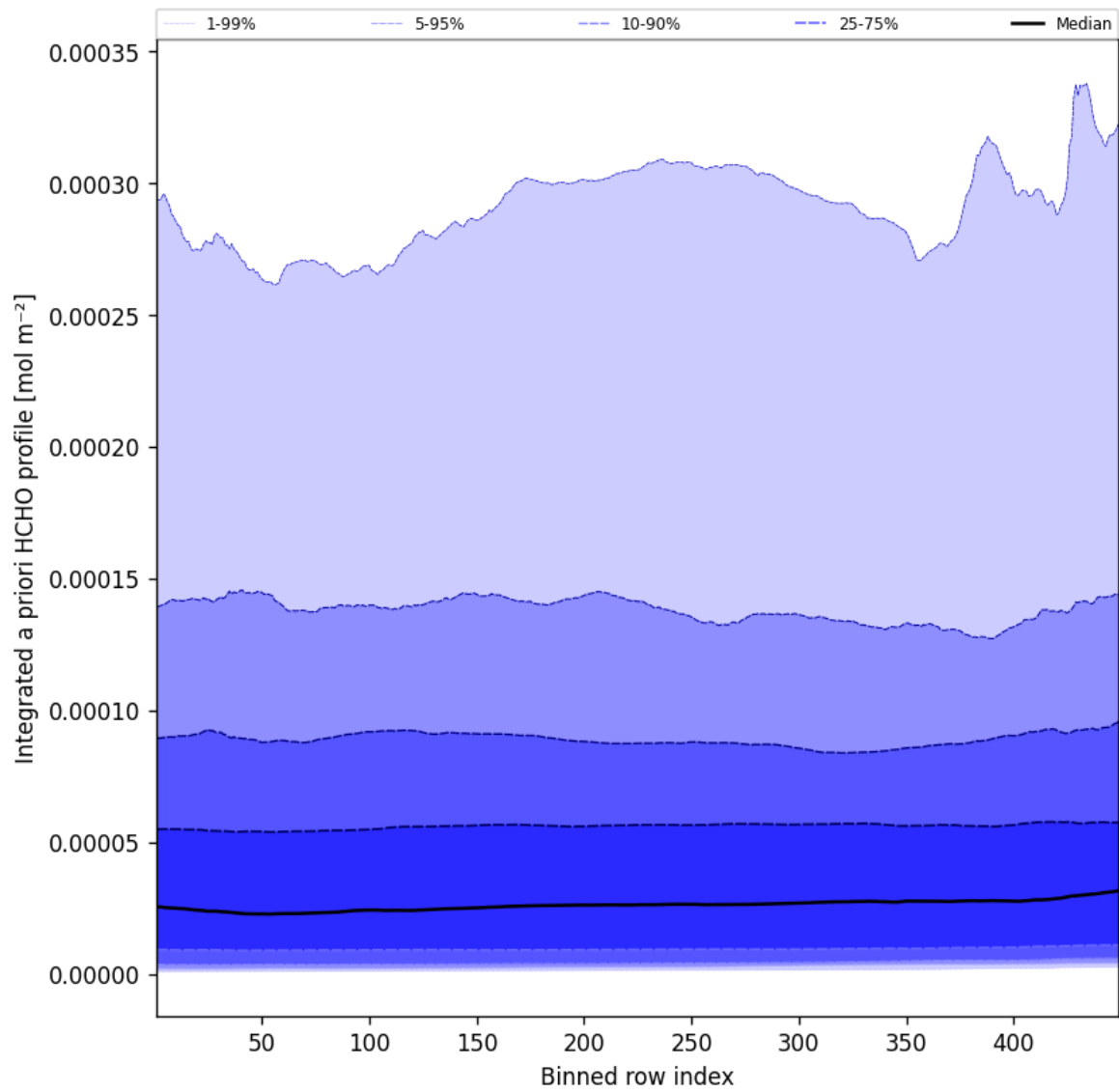
Figure 55: Along track statistics of “Integrated a priori HCHO profile” for 2025-05-09 to 2025-05-10
