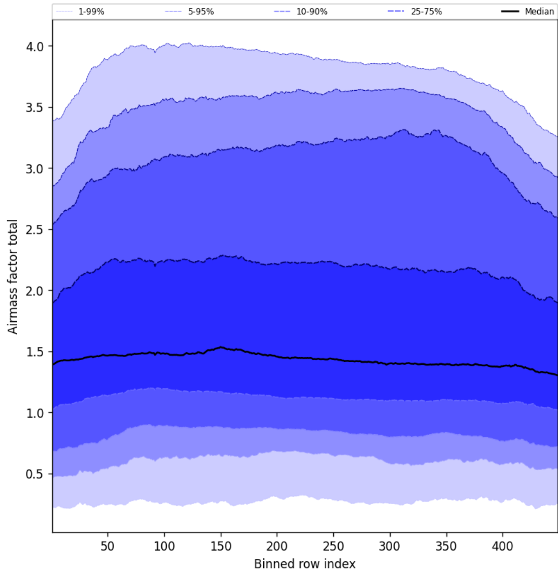
Figure 52: Along track statistics of “Airmass factor total” for 2025-05-09 to 2025-05-10
