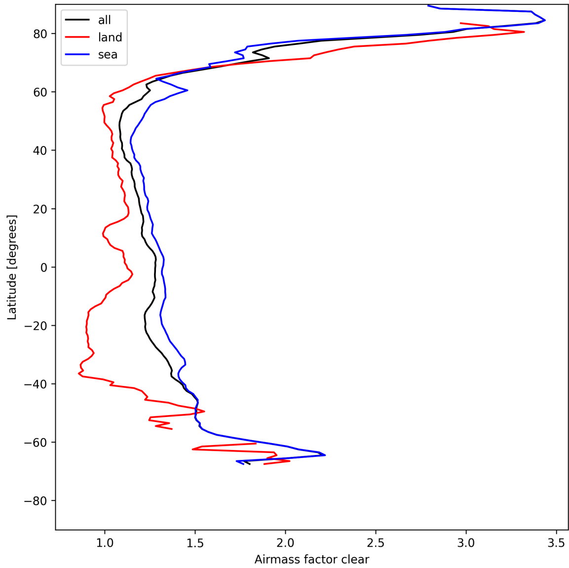
Figure 26: Zonal average of “Airmass factor clear” for 2025-05-09 to 2025-05-10.
