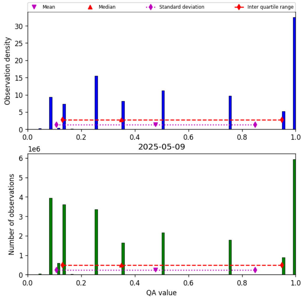
Figure 32: Histogram of “QA value” for 2025-05-09 to 2025-05-10
