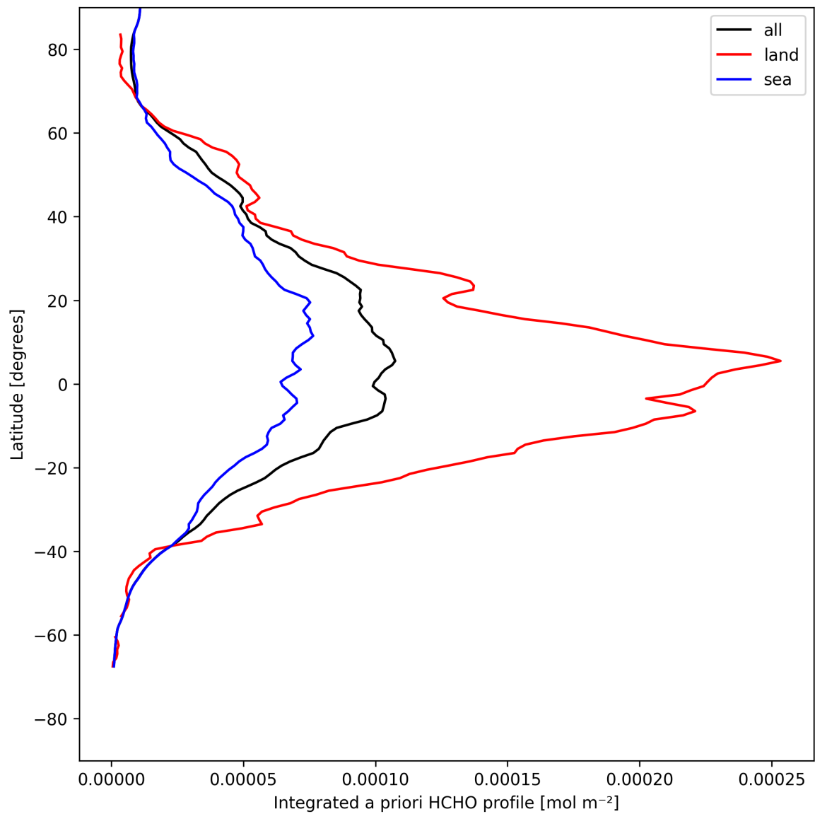
Figure 27: Zonal average of “Integrated a priori HCHO profile” for 2025-05-09 to 2025-05-10.
