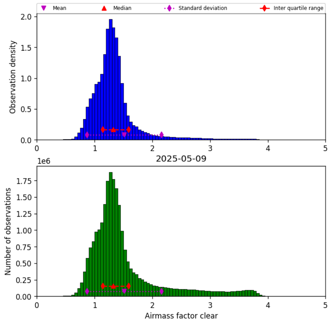
Figure 40: Histogram of “Airmass factor clear” for 2025-05-09 to 2025-05-10
