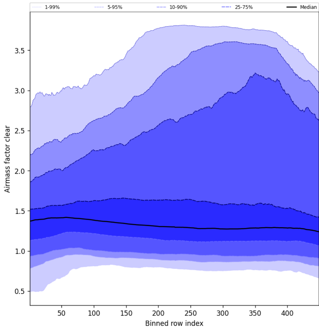
Figure 54: Along track statistics of “Airmass factor clear” for 2025-05-09 to 2025-05-10
