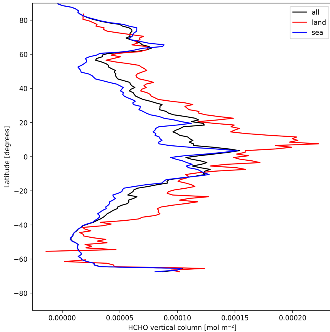
Figure 19: Zonal average of “HCHO vertical column” for 2025-05-09 to 2025-05-10.
