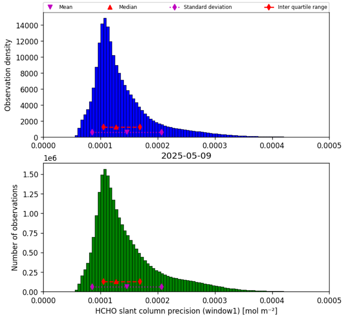
Figure 37: Histogram of “HCHO slant column precision (window1)” for 2025-05-09 to 2025-05-10
