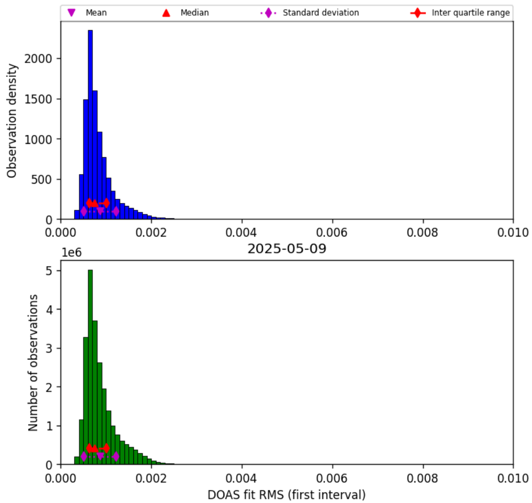
Figure 44: Histogram of “DOAS fit RMS (first interval)” for 2025-05-09 to 2025-05-10
