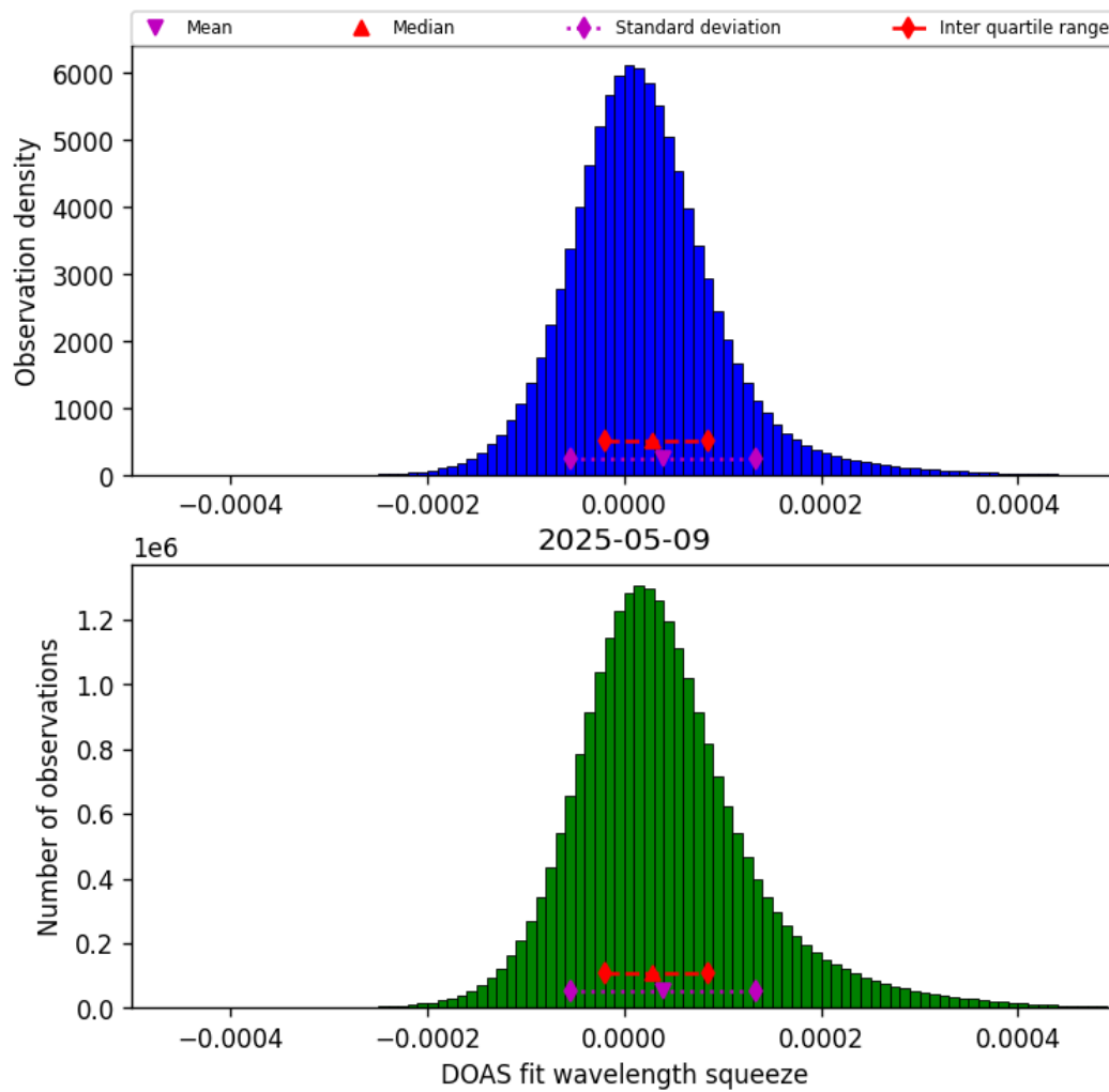
Figure 43: Histogram of “DOAS fit wavelength squeeze” for 2025-05-09 to 2025-05-10
