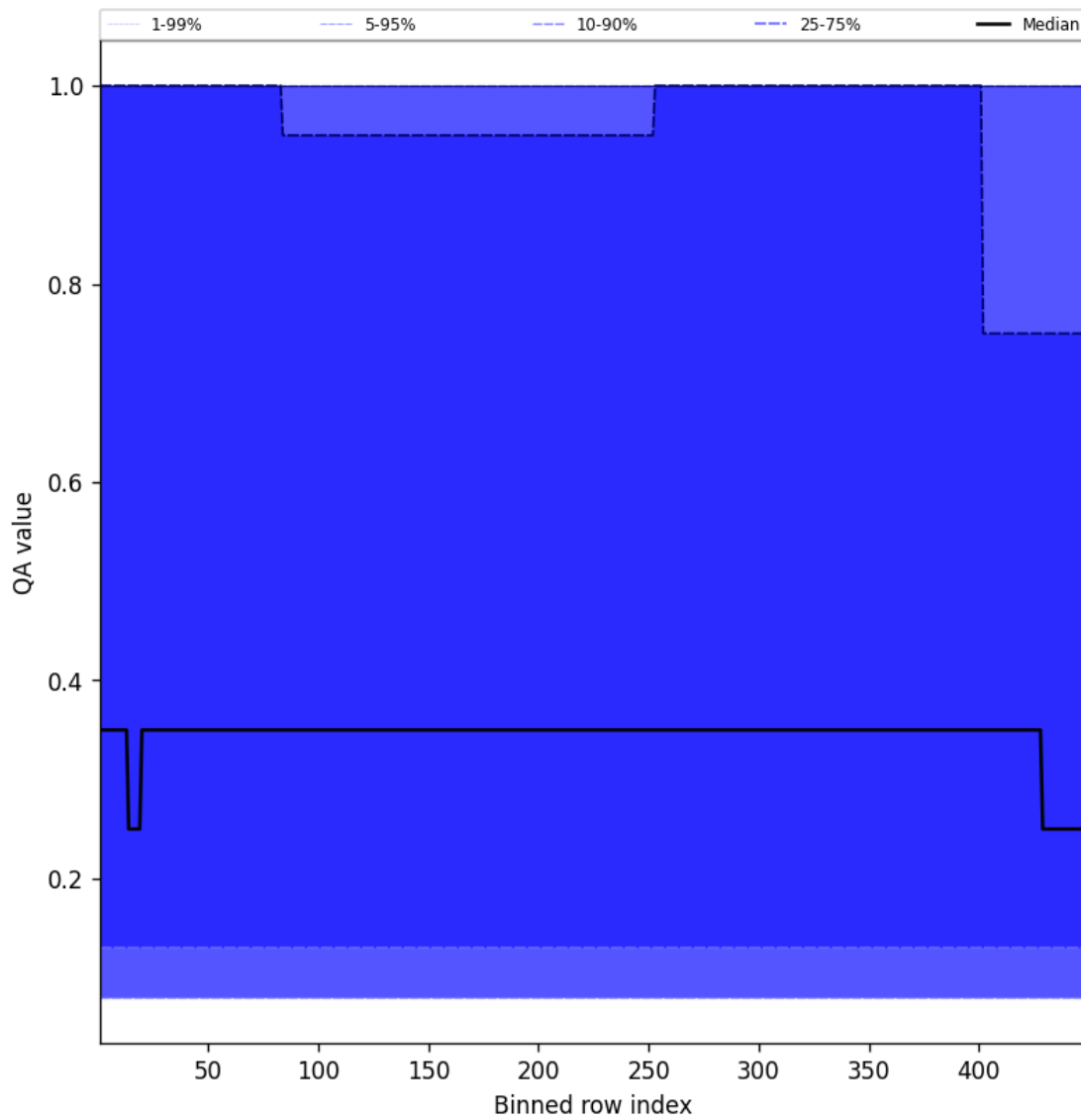
Figure 46: Along track statistics of “QA value” for 2025-05-09 to 2025-05-10
