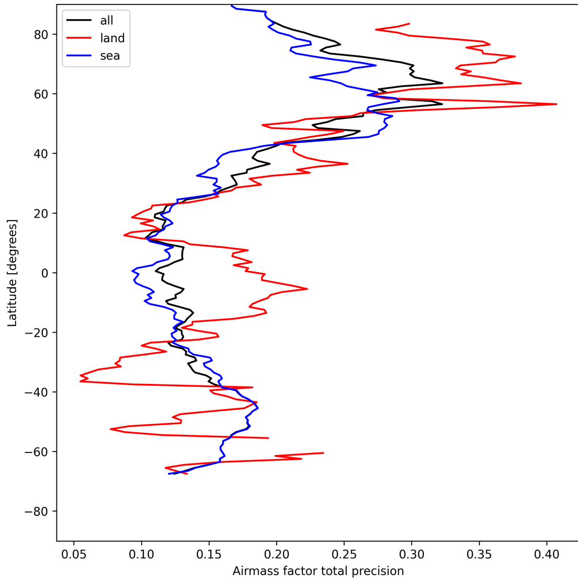
Figure 25: Zonal average of “Airmass factor total precision” for 2025-05-09 to 2025-05-10.
