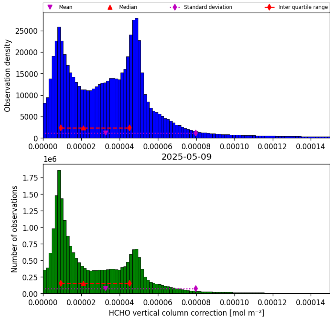
Figure 35: Histogram of “HCHO vertical column correction” for 2025-05-09 to 2025-05-10
