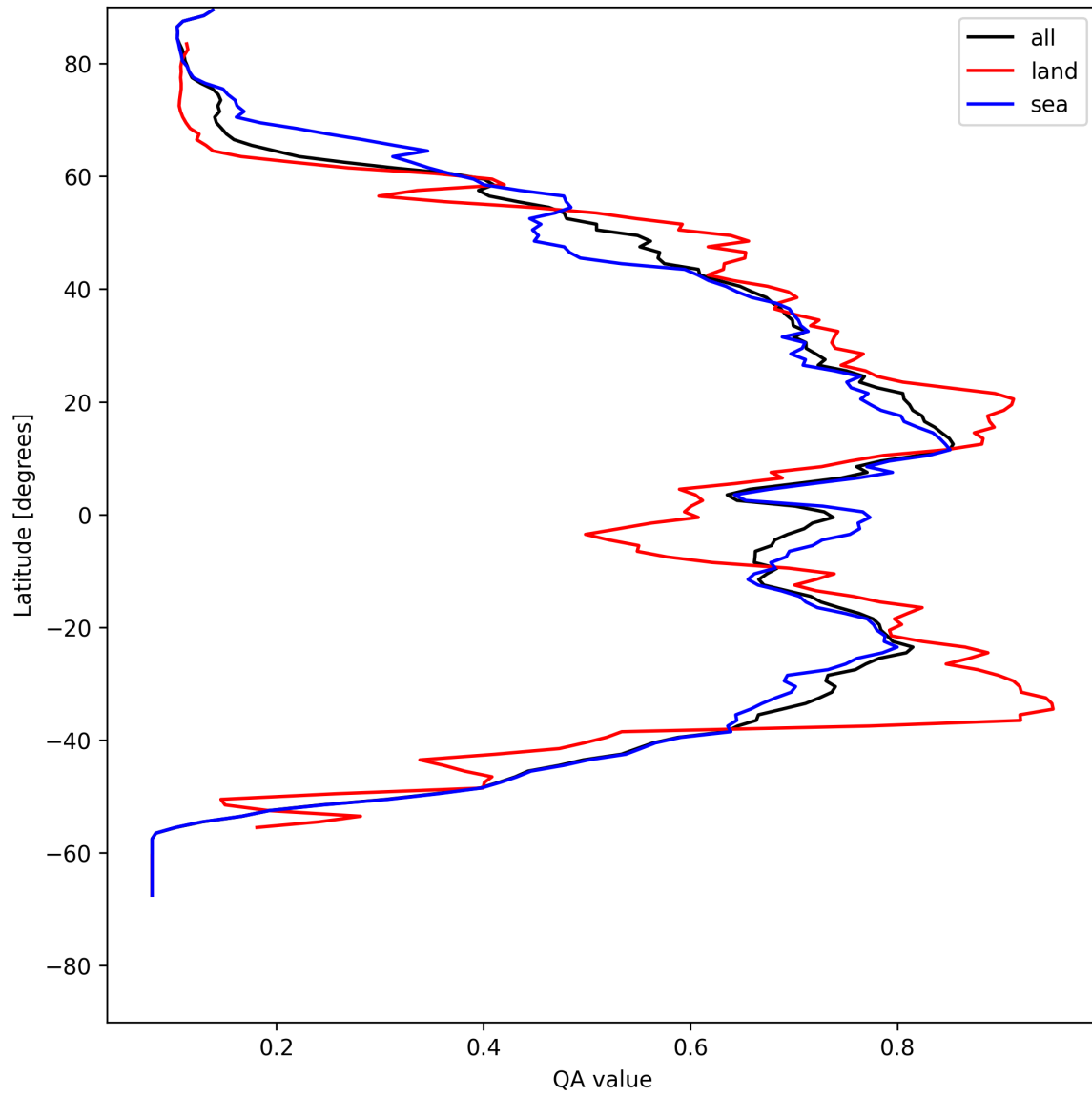
Figure 18: Zonal average of “QA value” for 2025-05-09 to 2025-05-10.
