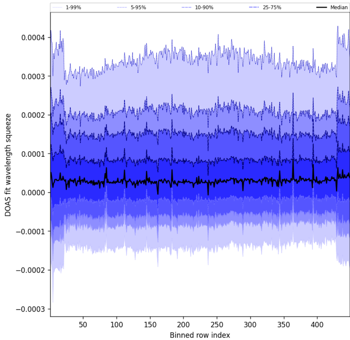
Figure 57: Along track statistics of “DOAS fit wavelength squeeze” for 2025-05-09 to 2025-05-10
