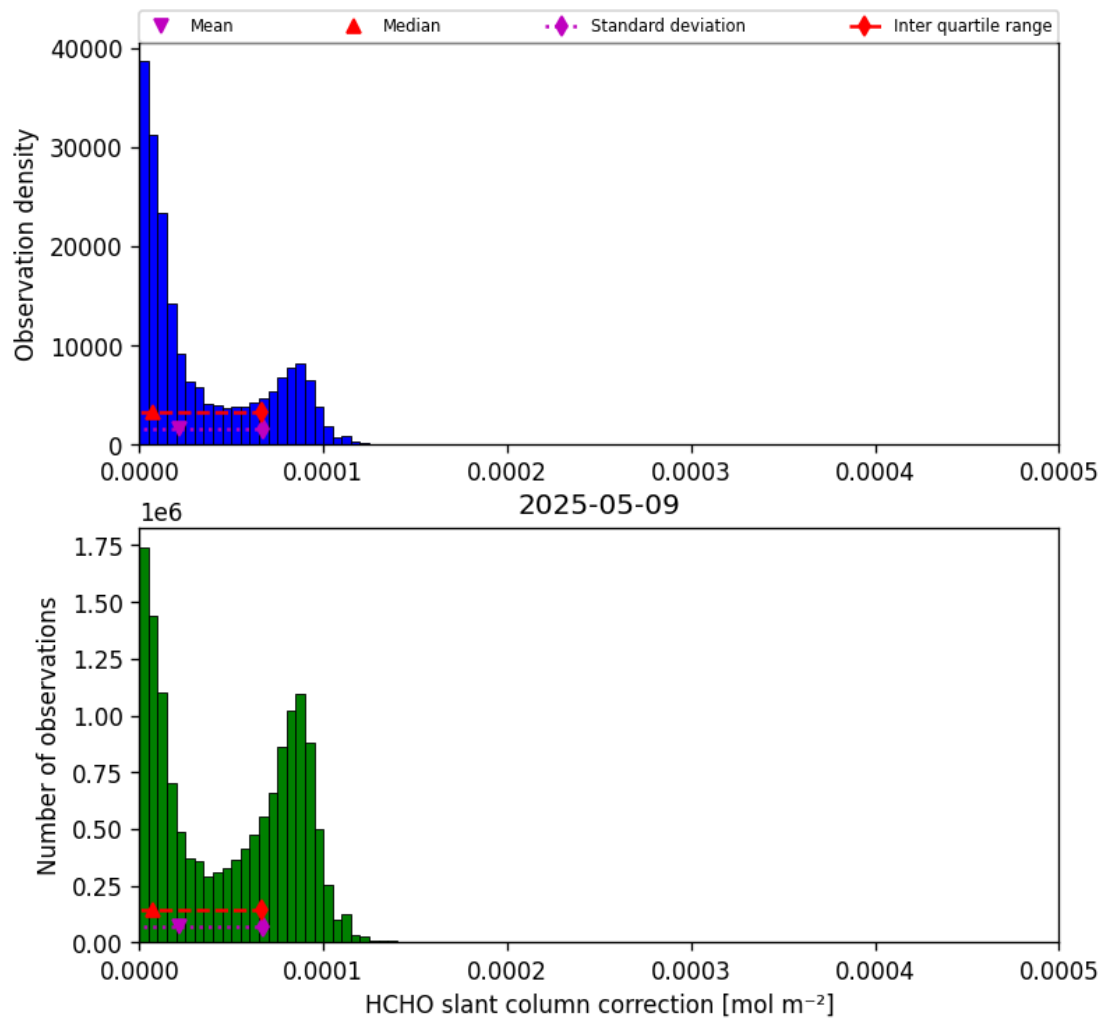
Figure 45: Histogram of “HCHO slant column correction” for 2025-05-09 to 2025-05-10
