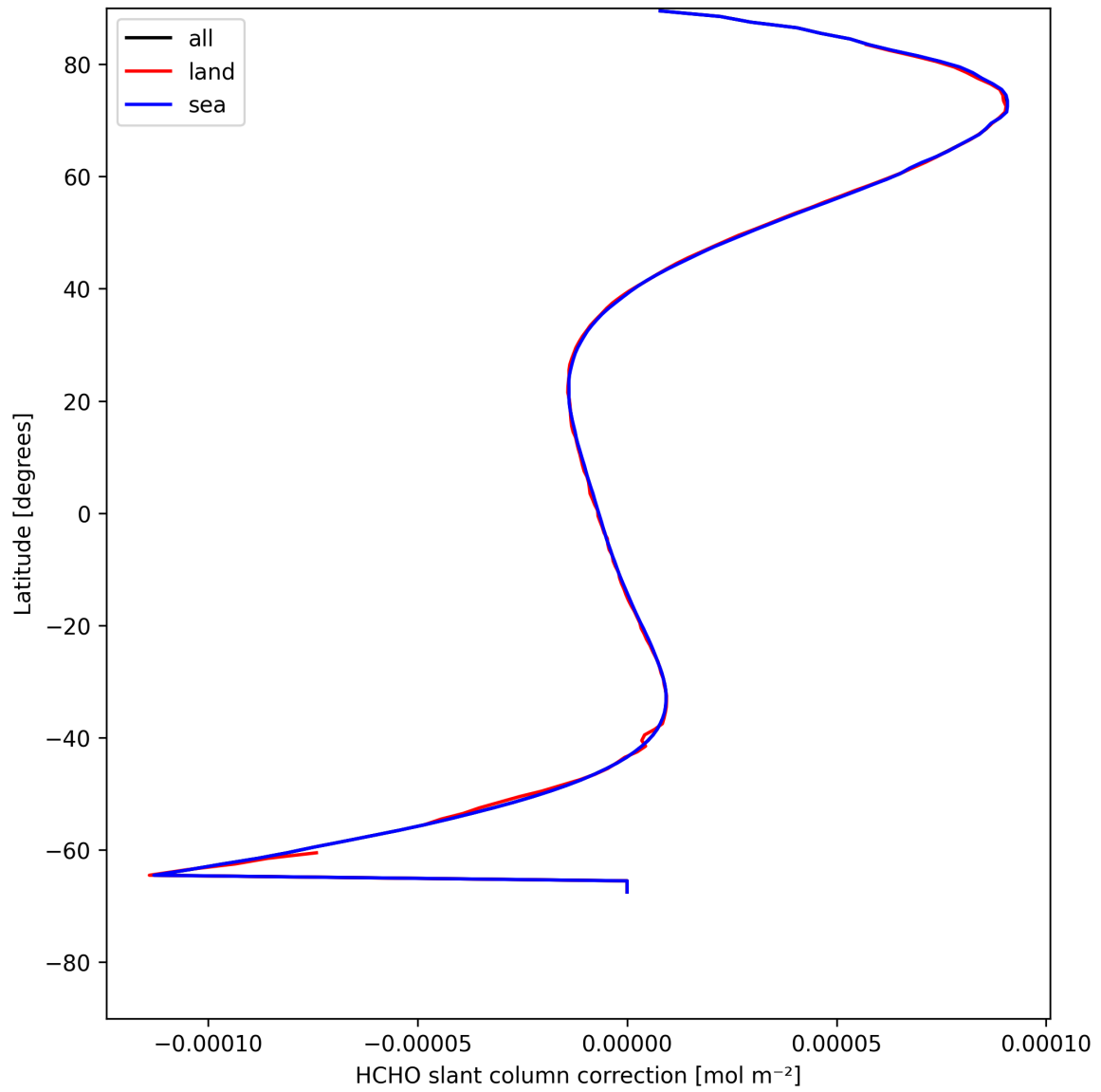
Figure 31: Zonal average of “HCHO slant column correction” for 2025-05-09 to 2025-05-10.
