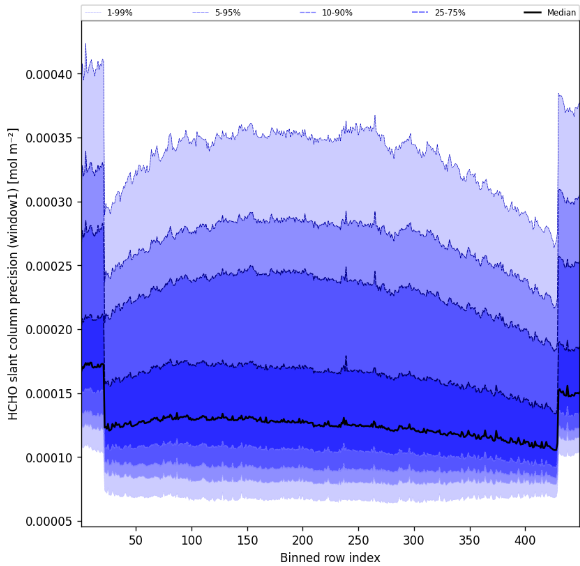
Figure 51: Along track statistics of “HCHO slant column precision (window1)” for 2025-05-09 to 2025-05-10
