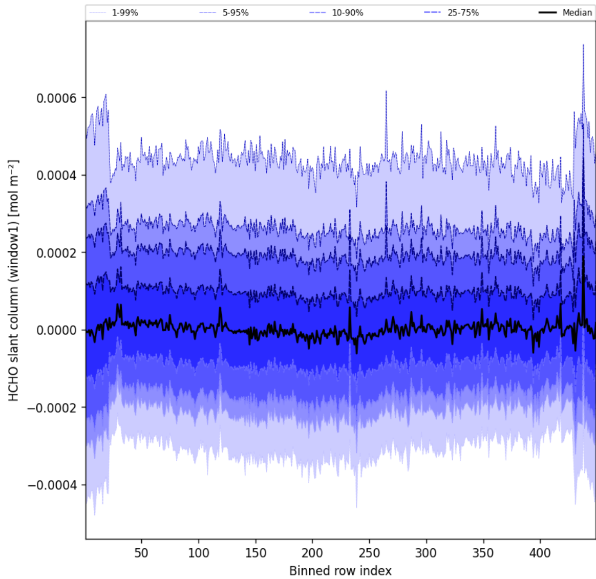
Figure 50: Along track statistics of “HCHO slant column (window1)” for 2025-05-09 to 2025-05-10
