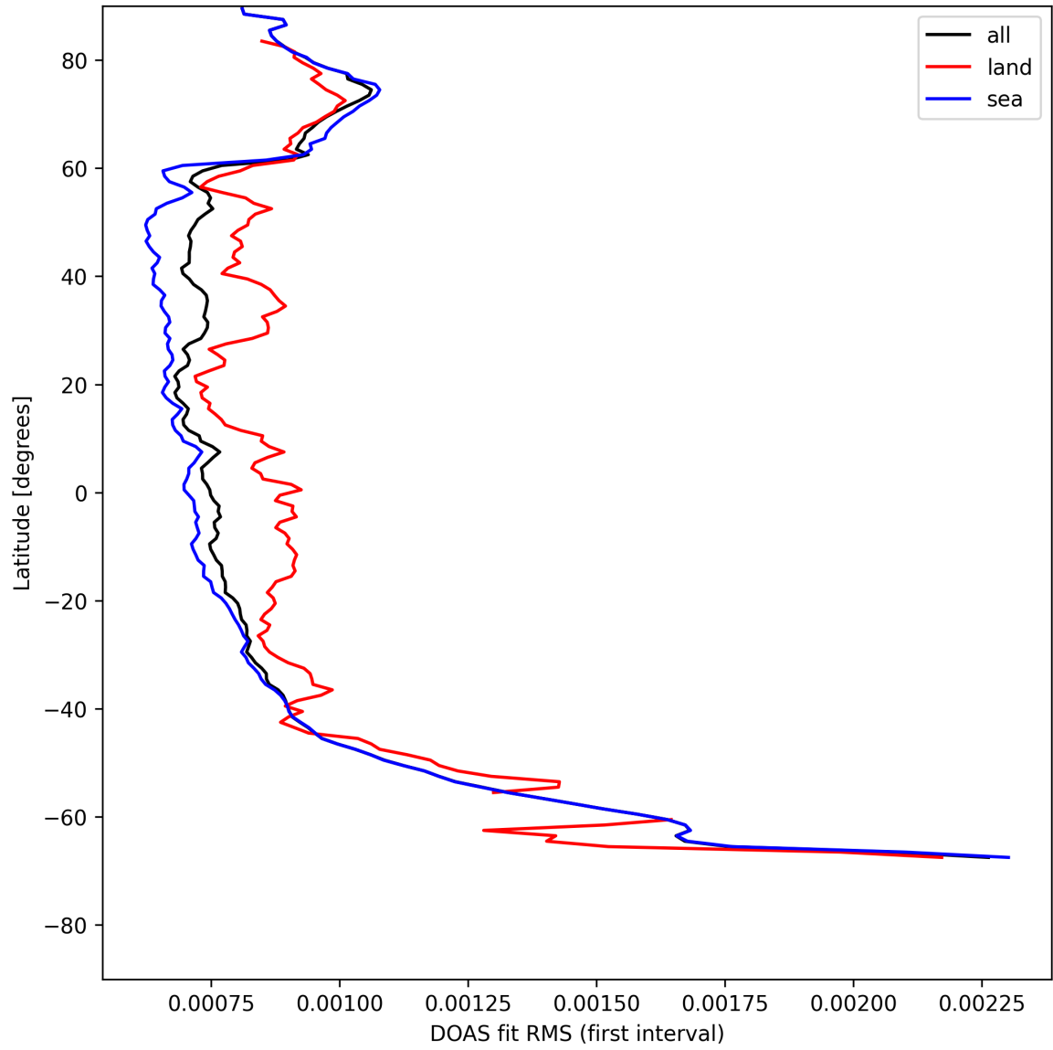
Figure 30: Zonal average of “DOAS fit RMS (first interval)” for 2025-05-09 to 2025-05-10.
