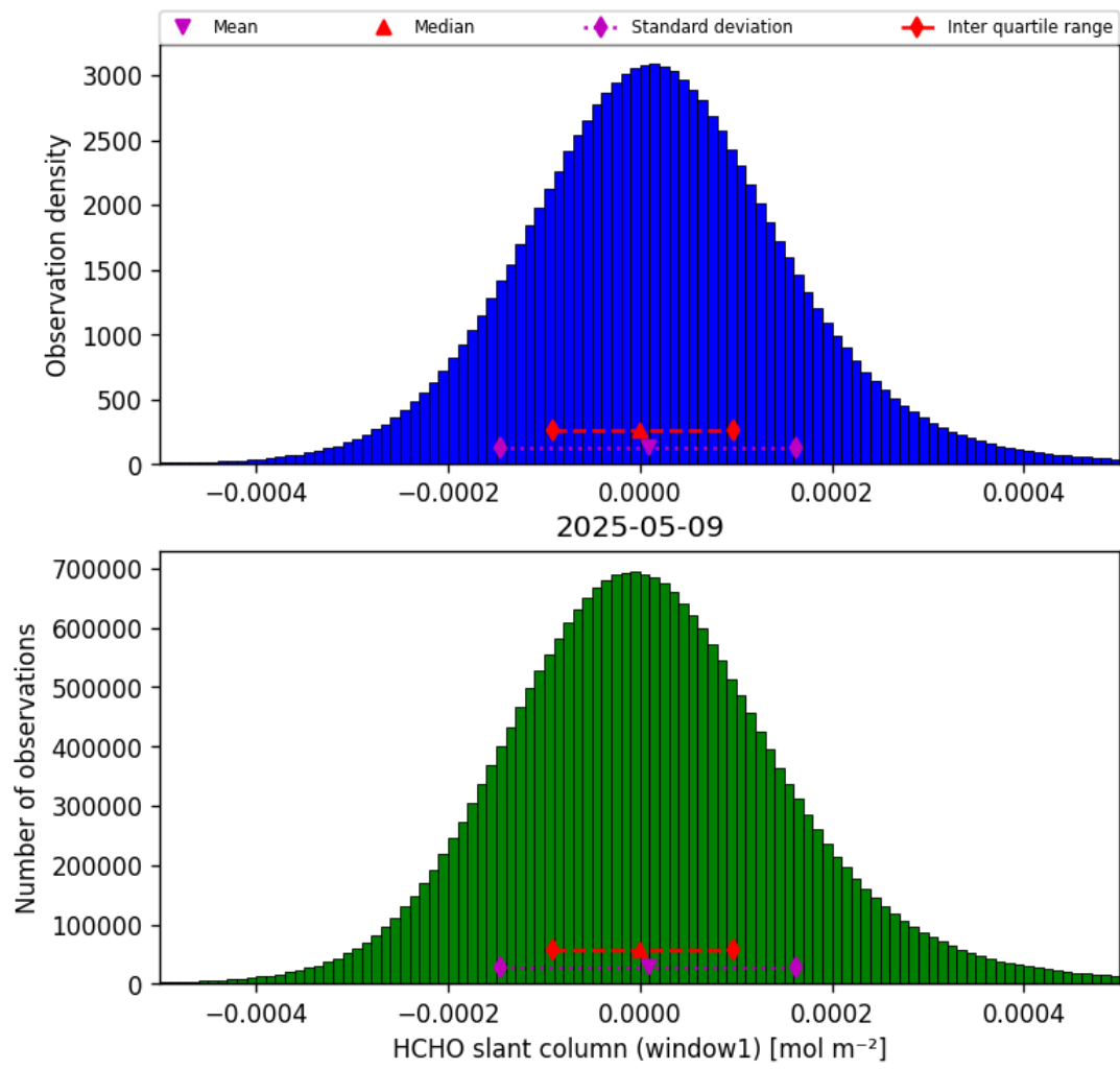
Figure 36: Histogram of "HCHO slant column (window1)" for 2025-05-09 to 2025-05-10
