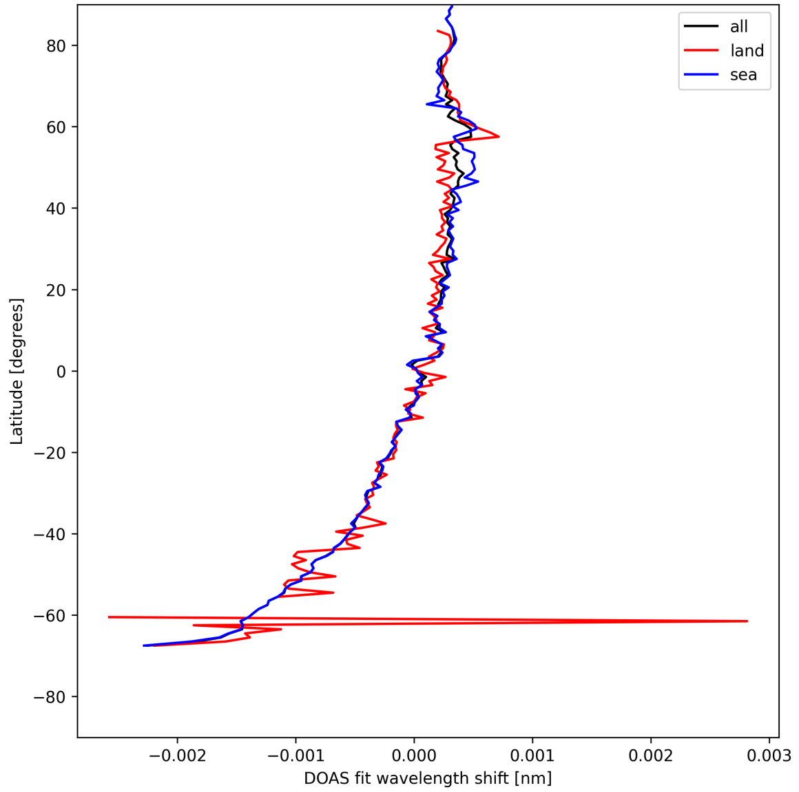
Figure 28: Zonal average of “DOAS fit wavelength shift” for 2025-05-09 to 2025-05-10.
