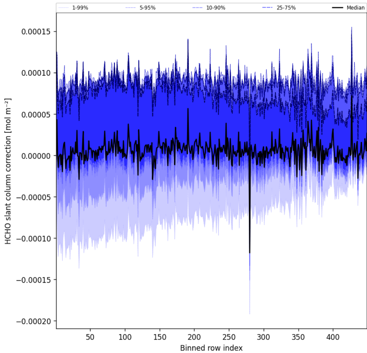
Figure 59: Along track statistics of “HCHO slant column correction” for 2025-05-09 to 2025-05-10
