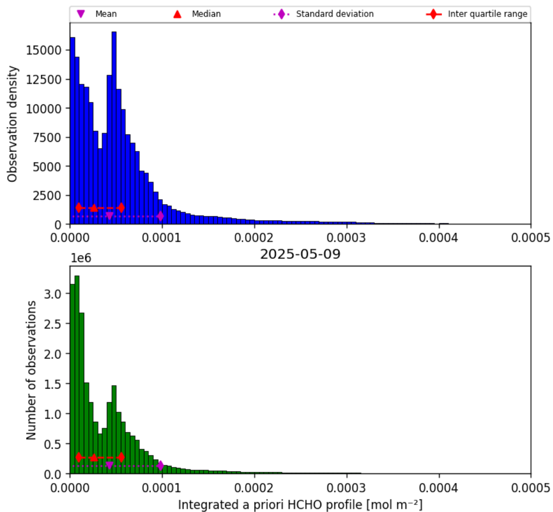
Figure 41: Histogram of “Integrated a priori HCHO profile” for 2025-05-09 to 2025-05-10
