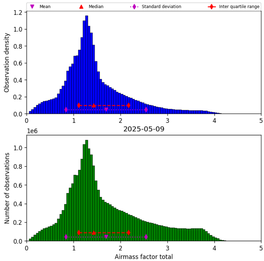
Figure 38: Histogram of “Airmass factor total” for 2025-05-09 to 2025-05-10
