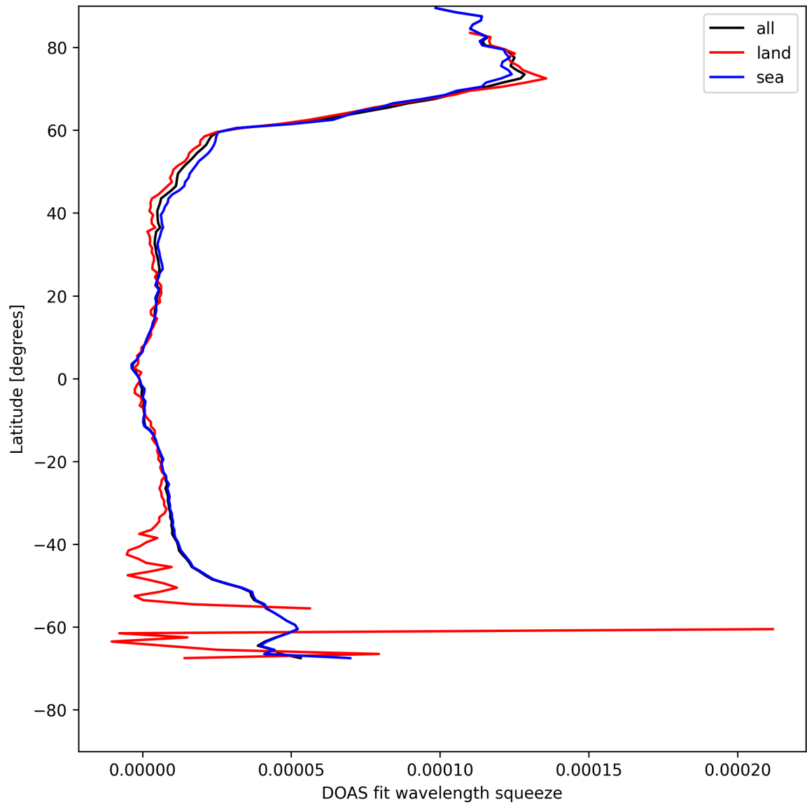
Figure 29: Zonal average of “DOAS fit wavelength squeeze” for 2025-05-09 to 2025-05-10.
