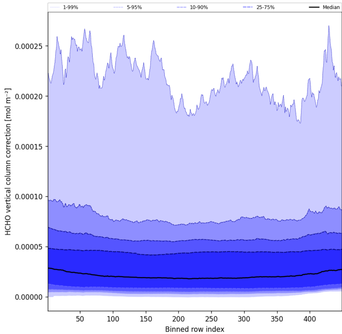
Figure 49: Along track statistics of “HCHO vertical column correction” for 2025-05-09 to 2025-05-10
