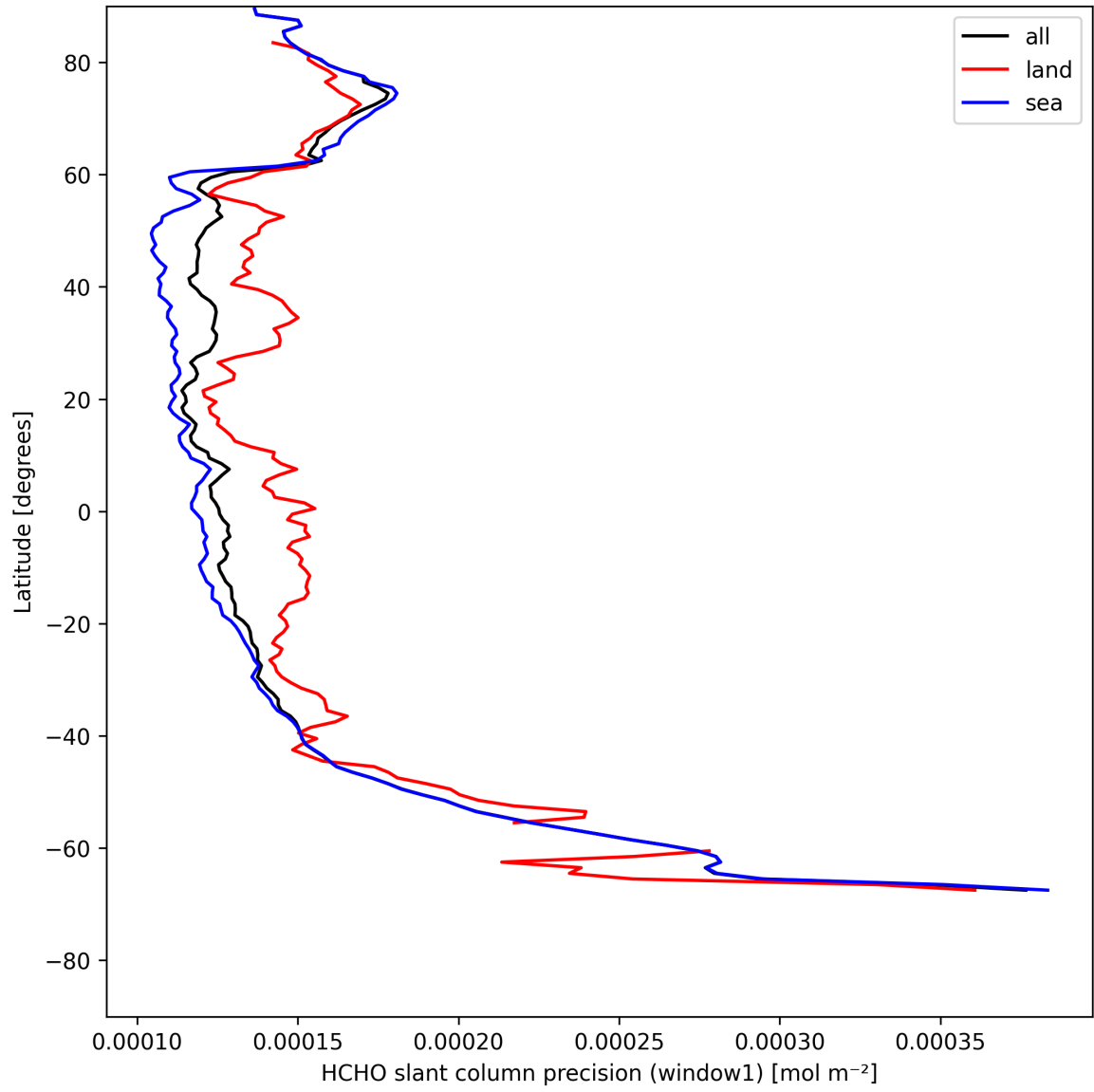
Figure 23: Zonal average of “HCHO slant column precision (window1)” for 2025-05-09 to 2025-05-10.
