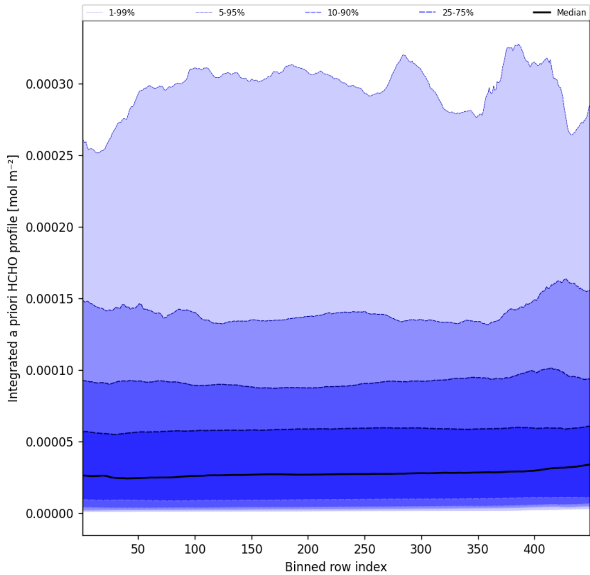
Figure 55: Along track statistics of “Integrated a priori HCHO profile” for 2025-05-10 to 2025-05-11
