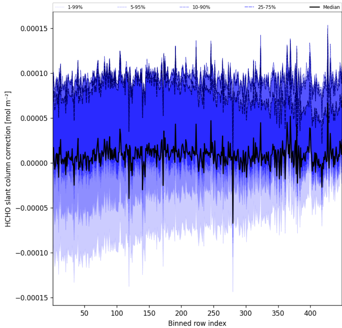
Figure 59: Along track statistics of “HCHO slant column correction” for 2025-05-10 to 2025-05-11
