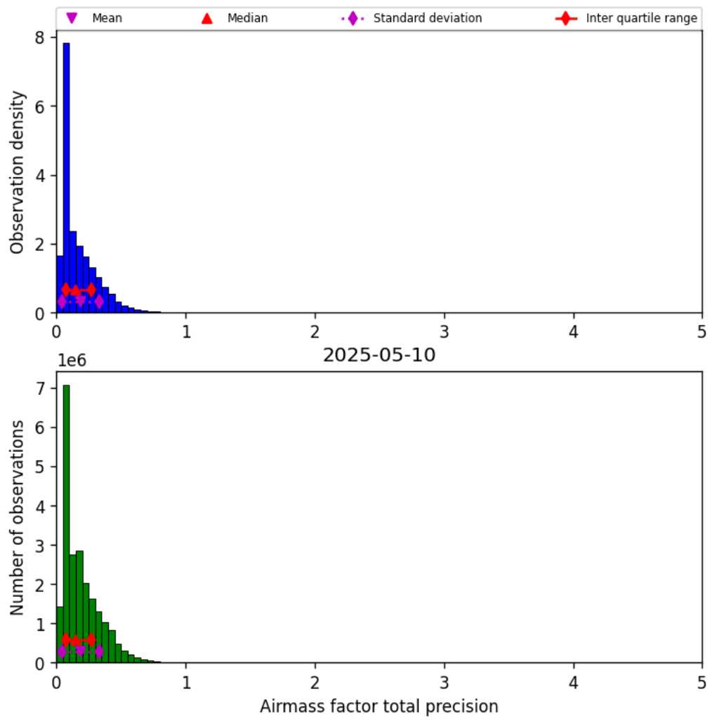
Figure 39: Histogram of “Airmass factor total precision” for 2025-05-10 to 2025-05-11
