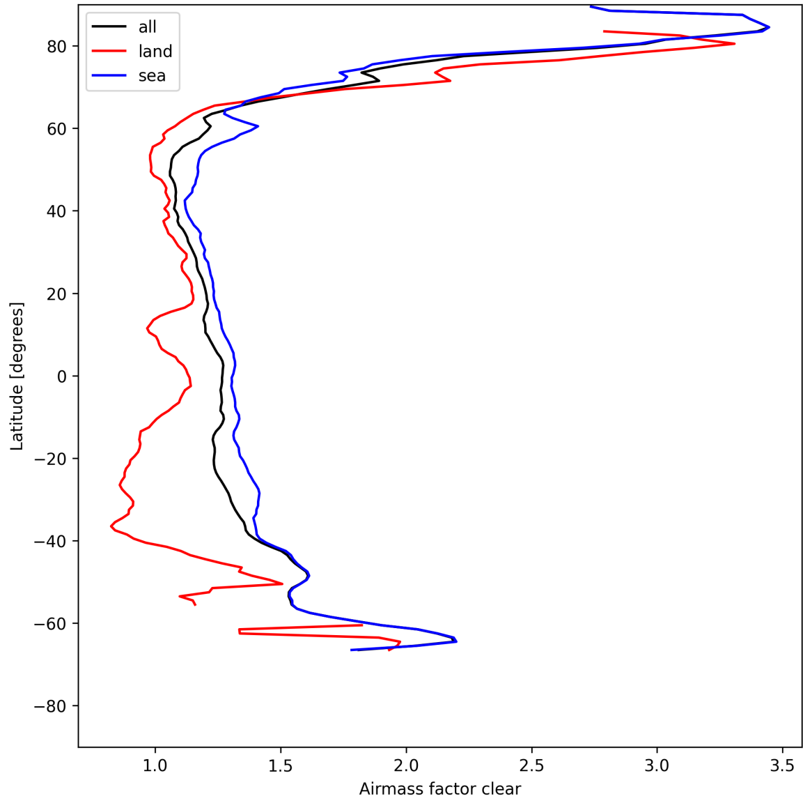
Figure 26: Zonal average of “Airmass factor clear” for 2025-05-10 to 2025-05-11.
