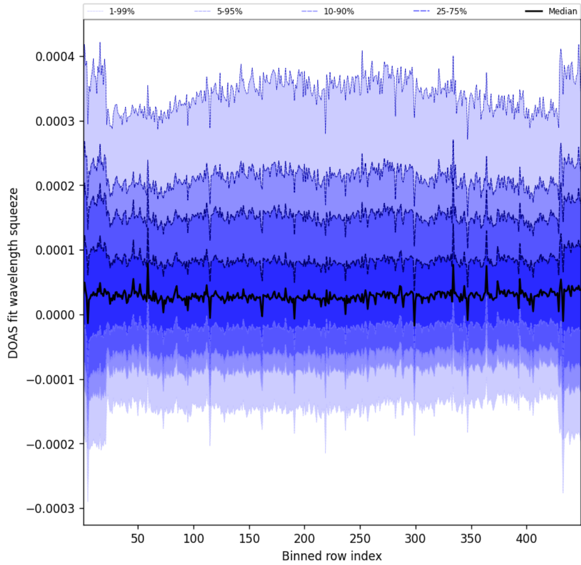
Figure 57: Along track statistics of “DOAS fit wavelength squeeze” for 2025-05-10 to 2025-05-11
