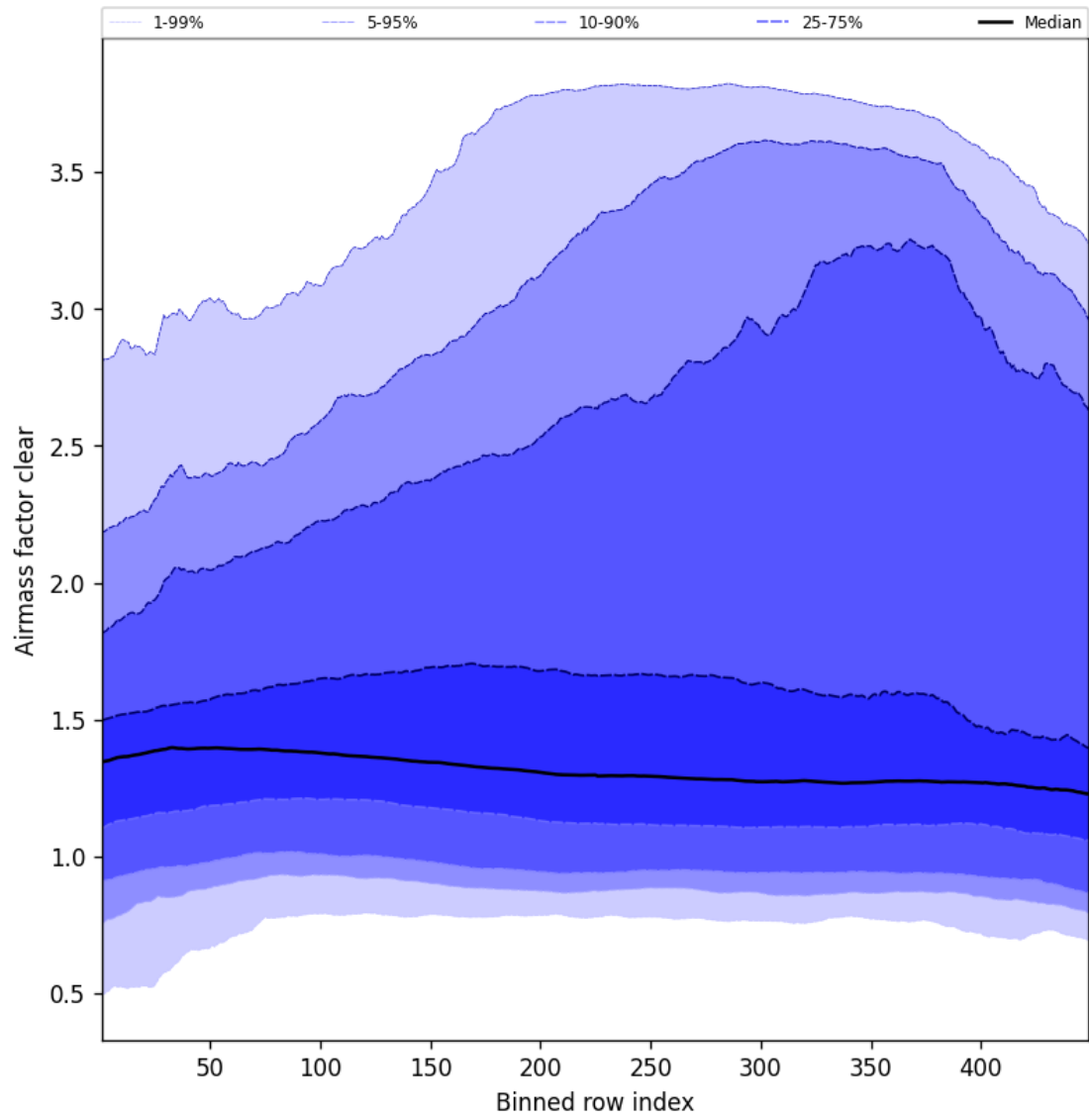
Figure 54: Along track statistics of “Airmass factor clear” for 2025-05-10 to 2025-05-11
