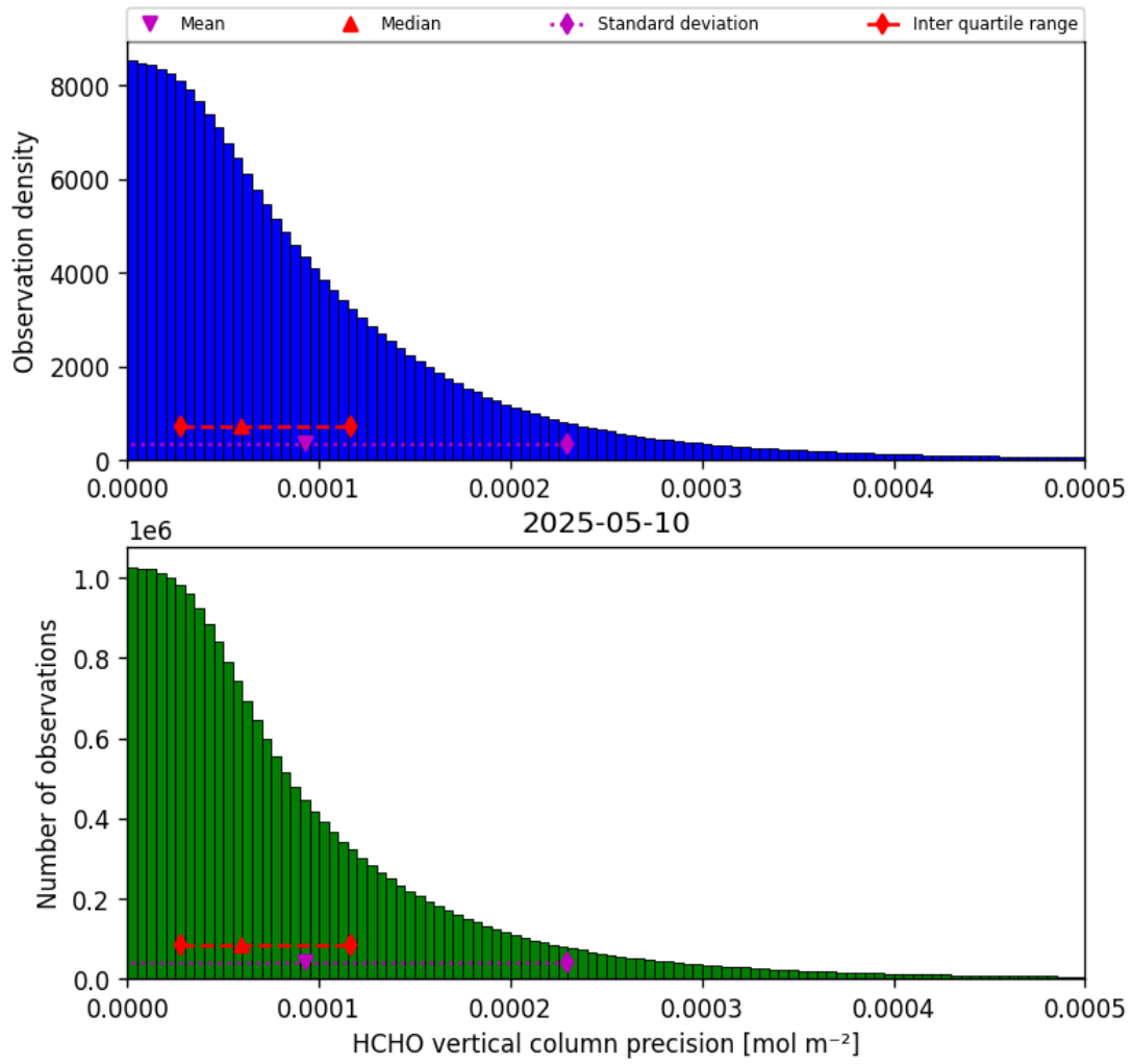
Figure 34: Histogram of “HCHO vertical column precision” for 2025-05-10 to 2025-05-11
