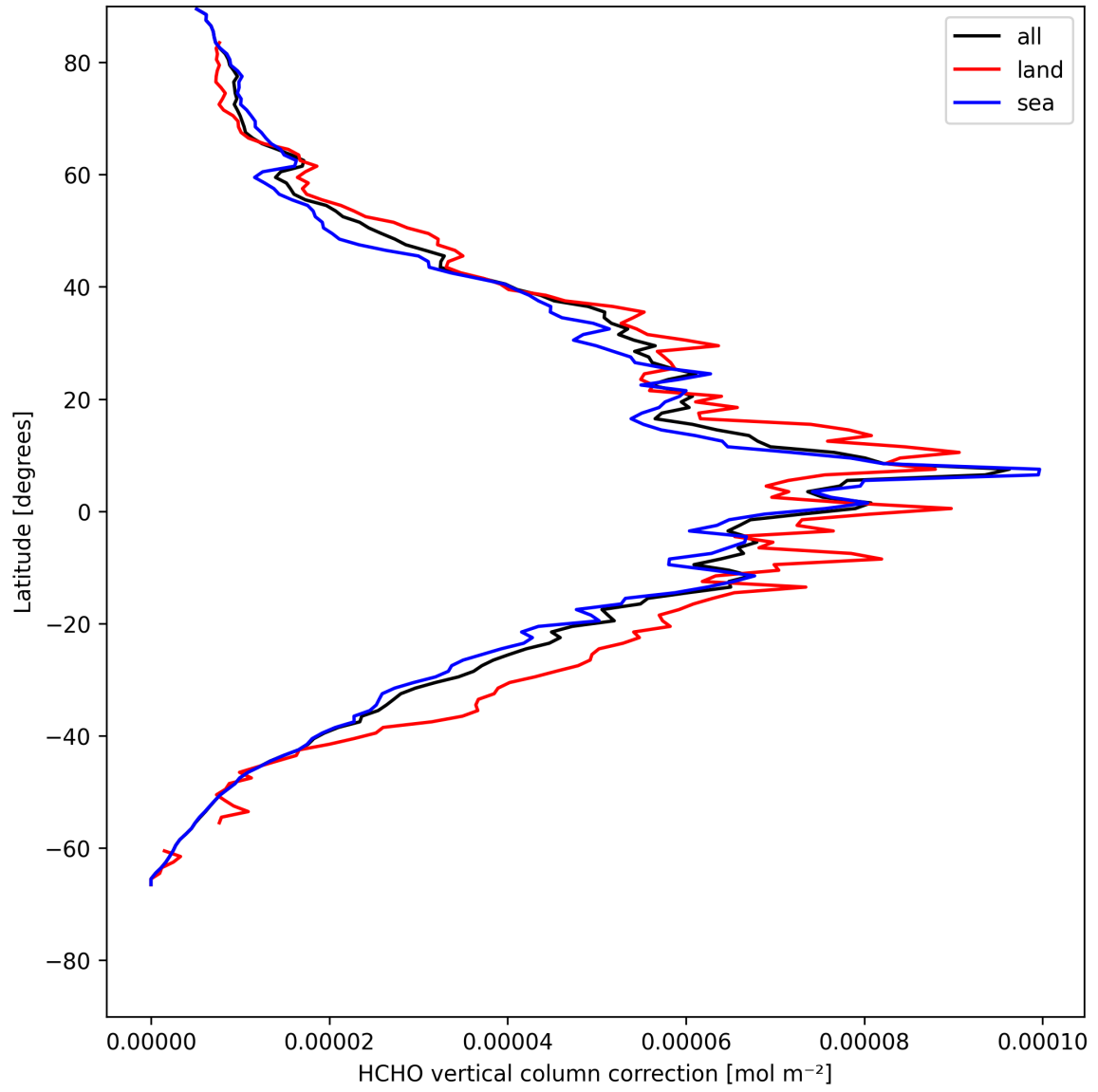
Figure 21: Zonal average of “HCHO vertical column correction” for 2025-05-10 to 2025-05-11.
