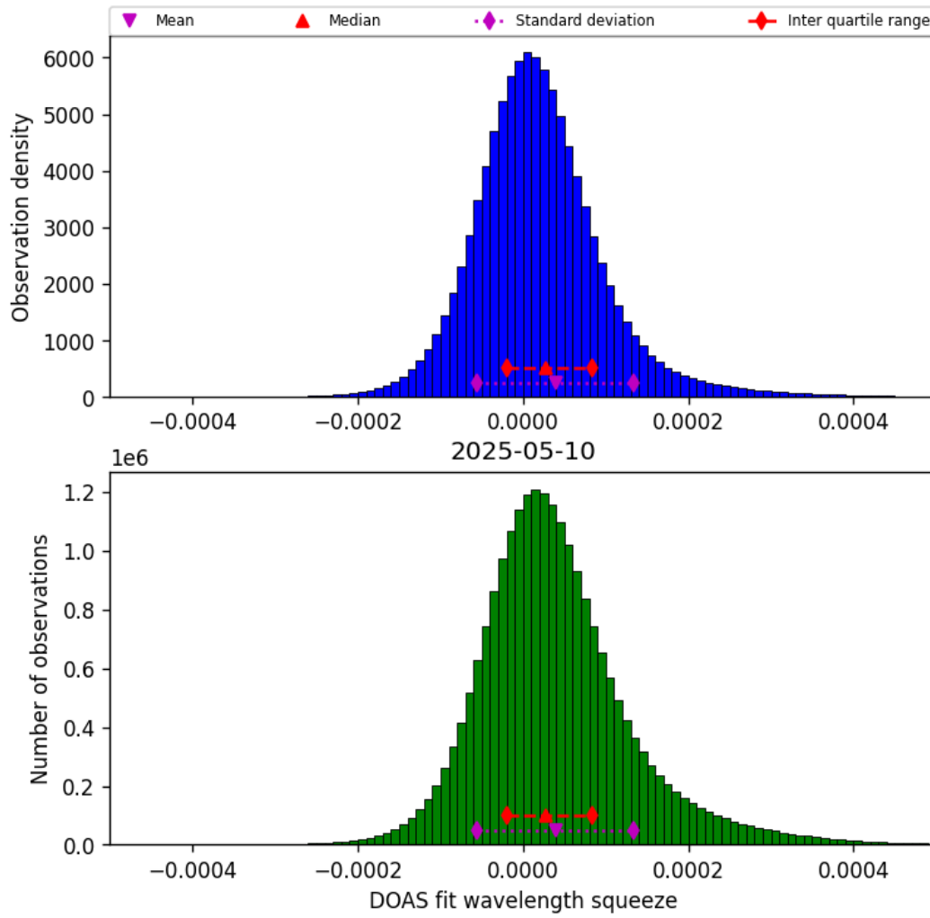
Figure 43: Histogram of “DOAS fit wavelength squeeze” for 2025-05-10 to 2025-05-11
