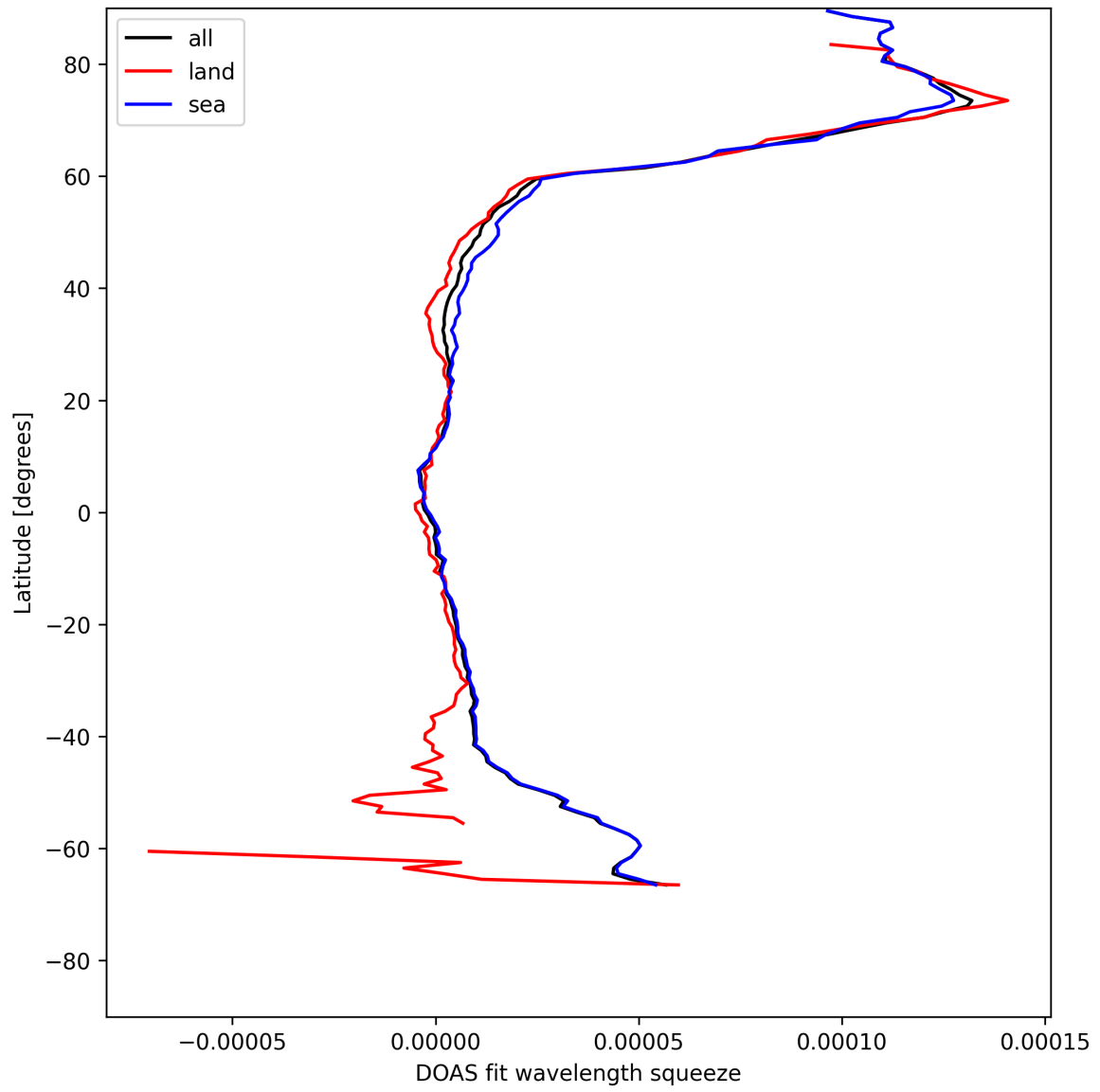
Figure 29: Zonal average of "DOAS fit wavelength squeeze" for 2025-05-10 to 2025-05-11.
