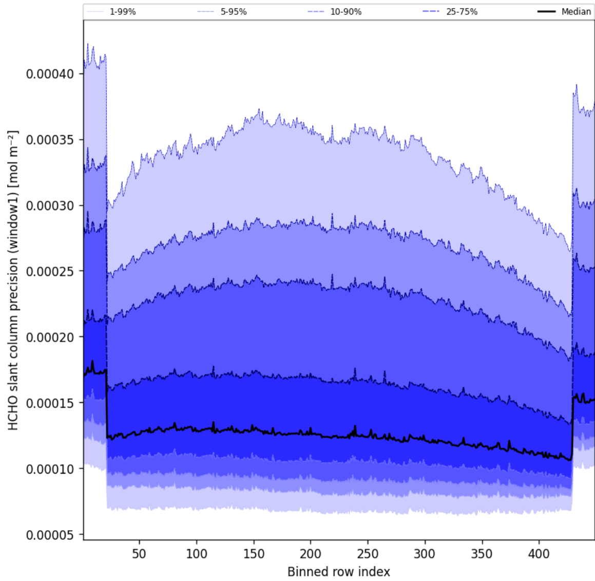
Figure 51: Along track statistics of “HCHO slant column precision (window1)” for 2025-05-10 to 2025-05-11
