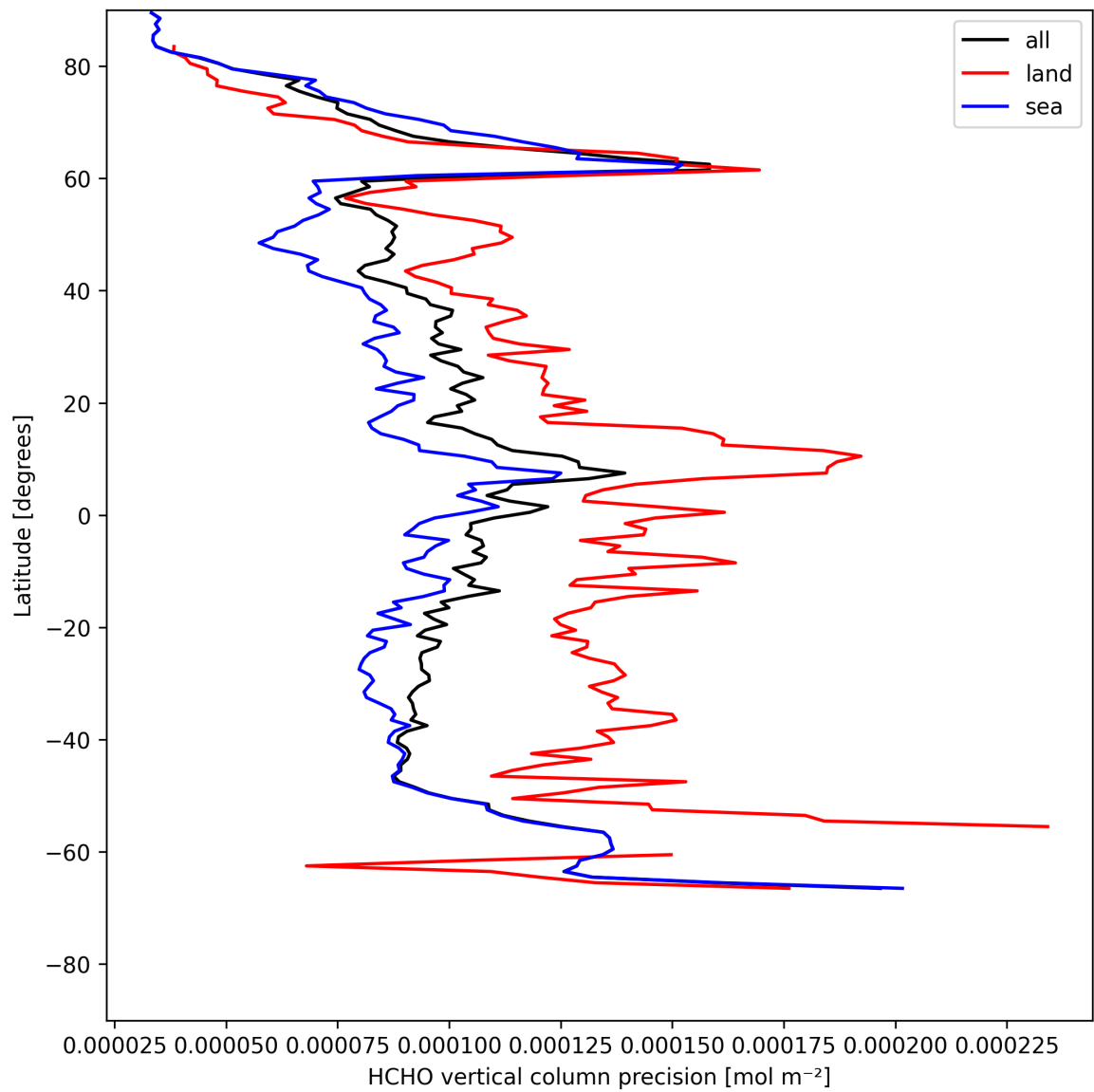
Figure 20: Zonal average of “HCHO vertical column precision” for 2025-05-10 to 2025-05-11.
