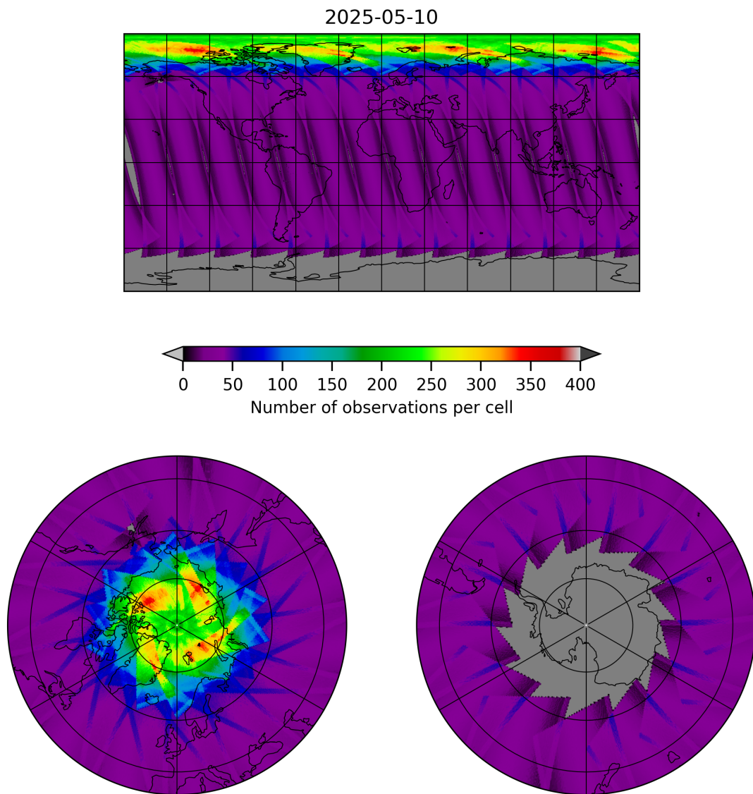
Figure 17: Map of the number of observations for 2025-05-10 to 2025-05-11
