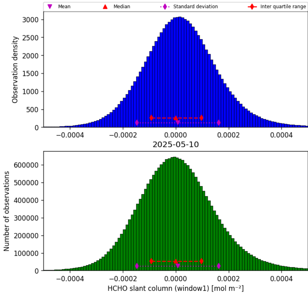
Figure 36: Histogram of “HCHO slant column (window1)” for 2025-05-10 to 2025-05-11
