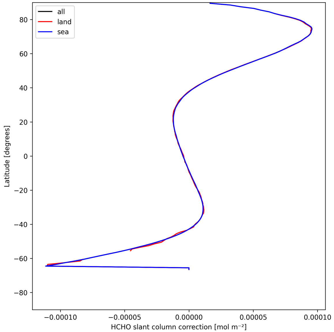
Figure 31: Zonal average of "HCHO slant column correction" for 2025-05-10 to 2025-05-11.
