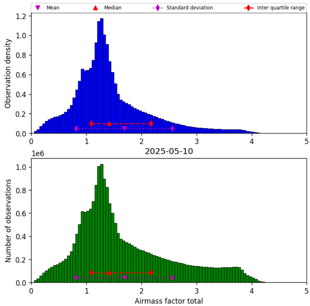
Figure 38: Histogram of “Airmass factor total” for 2025-05-10 to 2025-05-11
