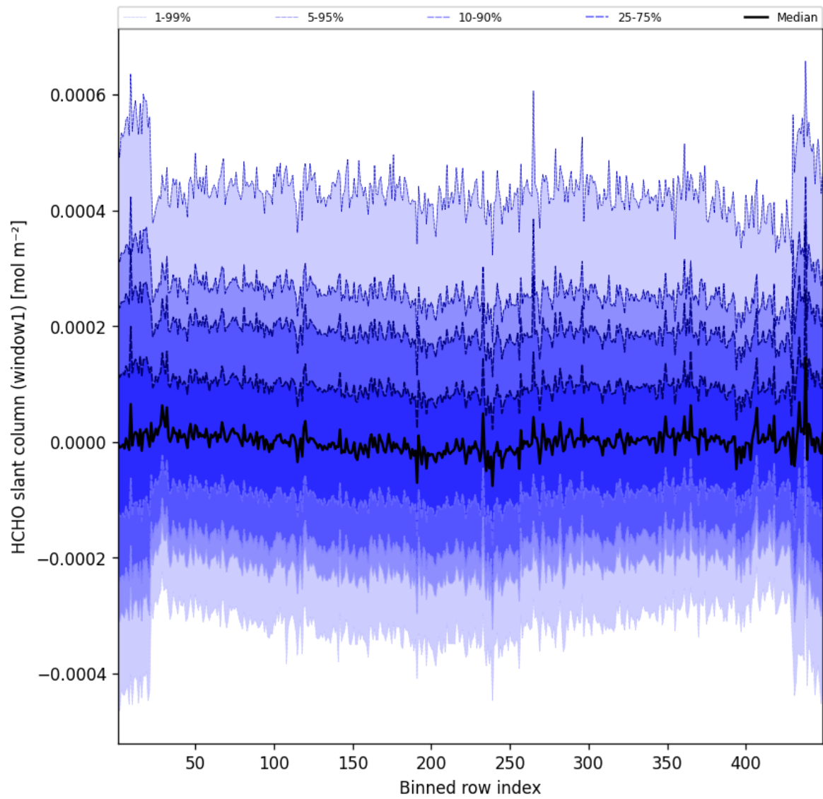
Figure 50: Along track statistics of “HCHO slant column (window1)” for 2025-05-10 to 2025-05-11
