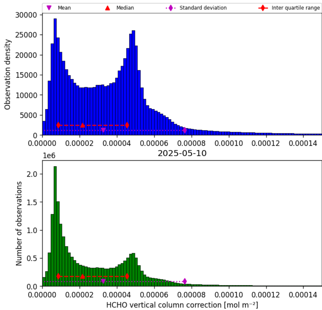
Figure 35: Histogram of “HCHO vertical column correction” for 2025-05-10 to 2025-05-11
