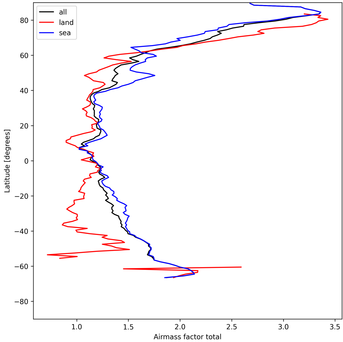
Figure 24: Zonal average of “Airmass factor total” for 2025-05-10 to 2025-05-11.
