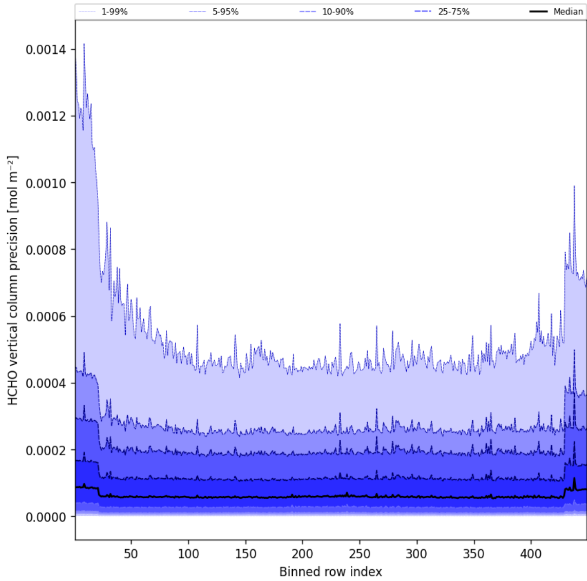
Figure 48: Along track statistics of “HCHO vertical column precision” for 2025-05-10 to 2025-05-11
