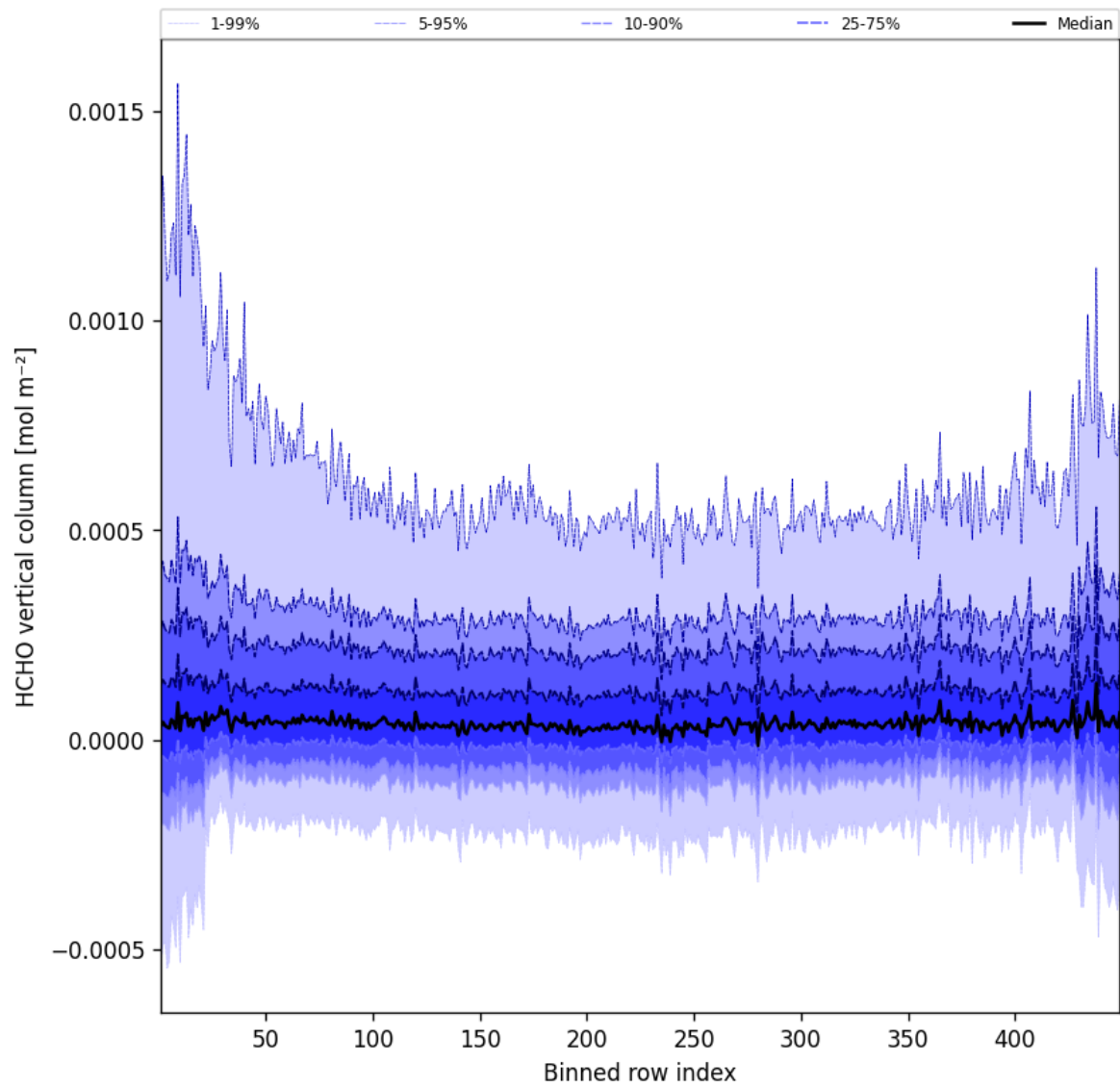
Figure 47: Along track statistics of “HCHO vertical column” for 2025-05-10 to 2025-05-11
