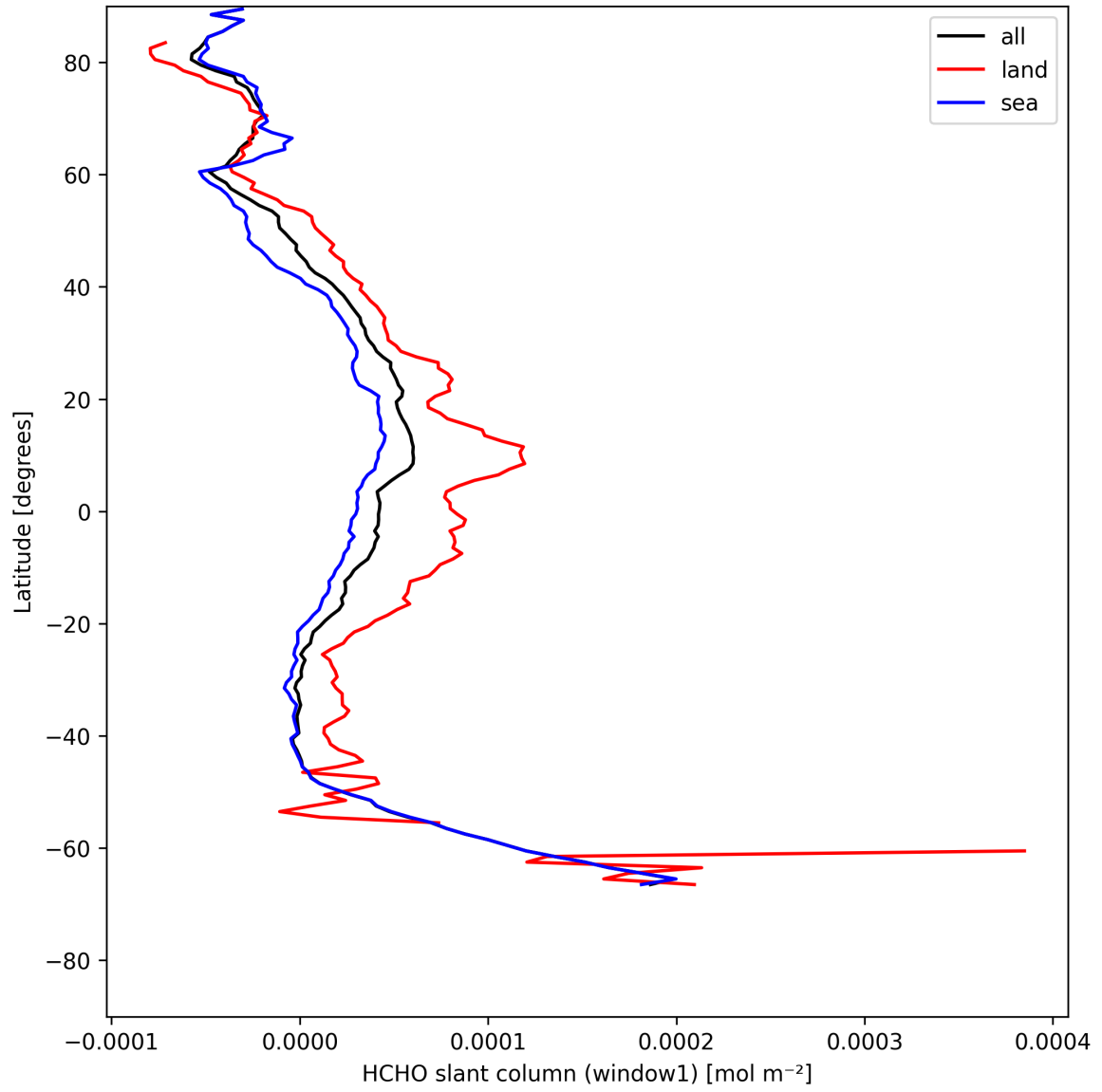
Figure 22: Zonal average of “HCHO slant column (window1)” for 2025-05-10 to 2025-05-11.
