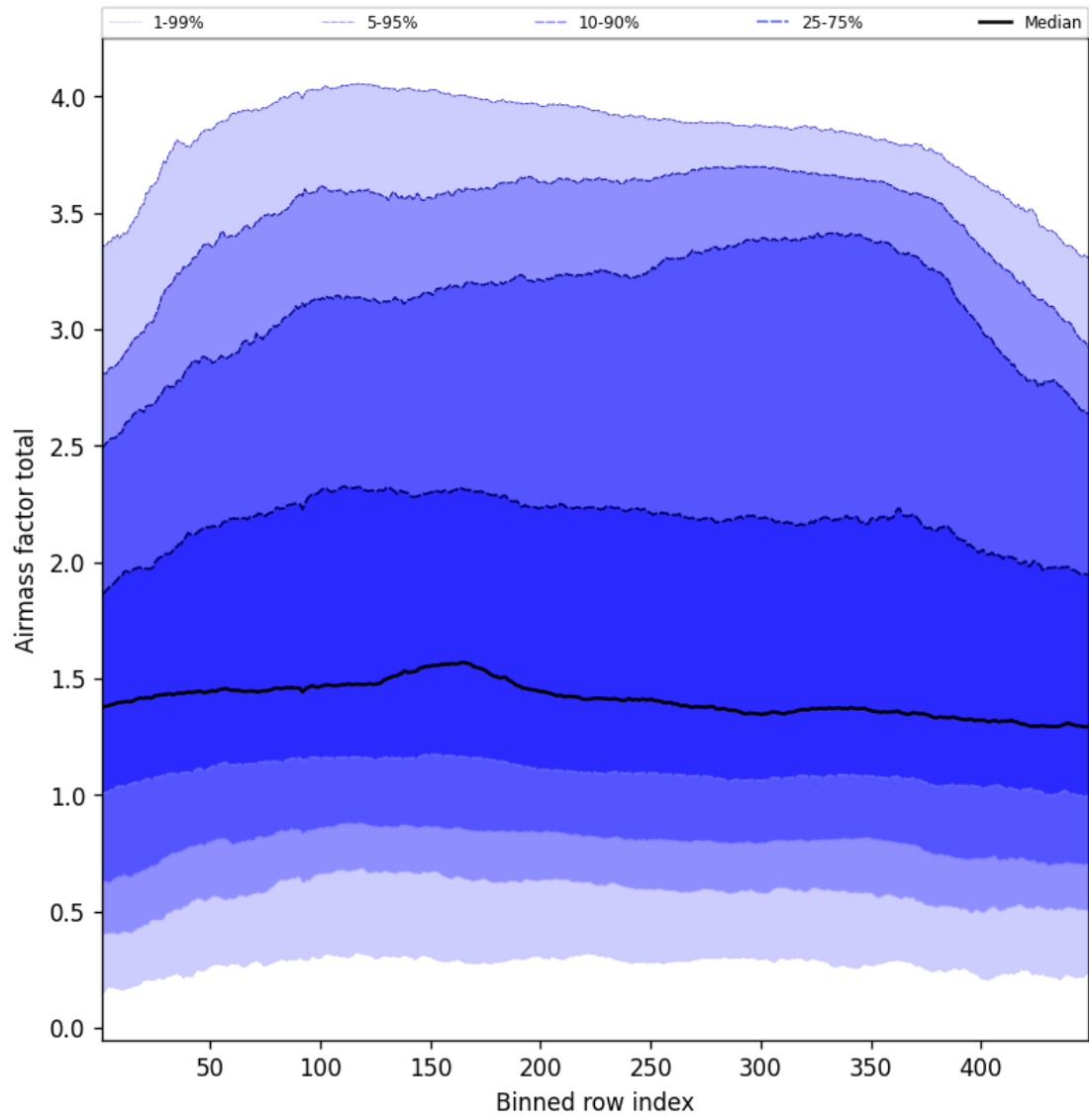
Figure 52: Along track statistics of “Airmass factor total” for 2025-05-10 to 2025-05-11
