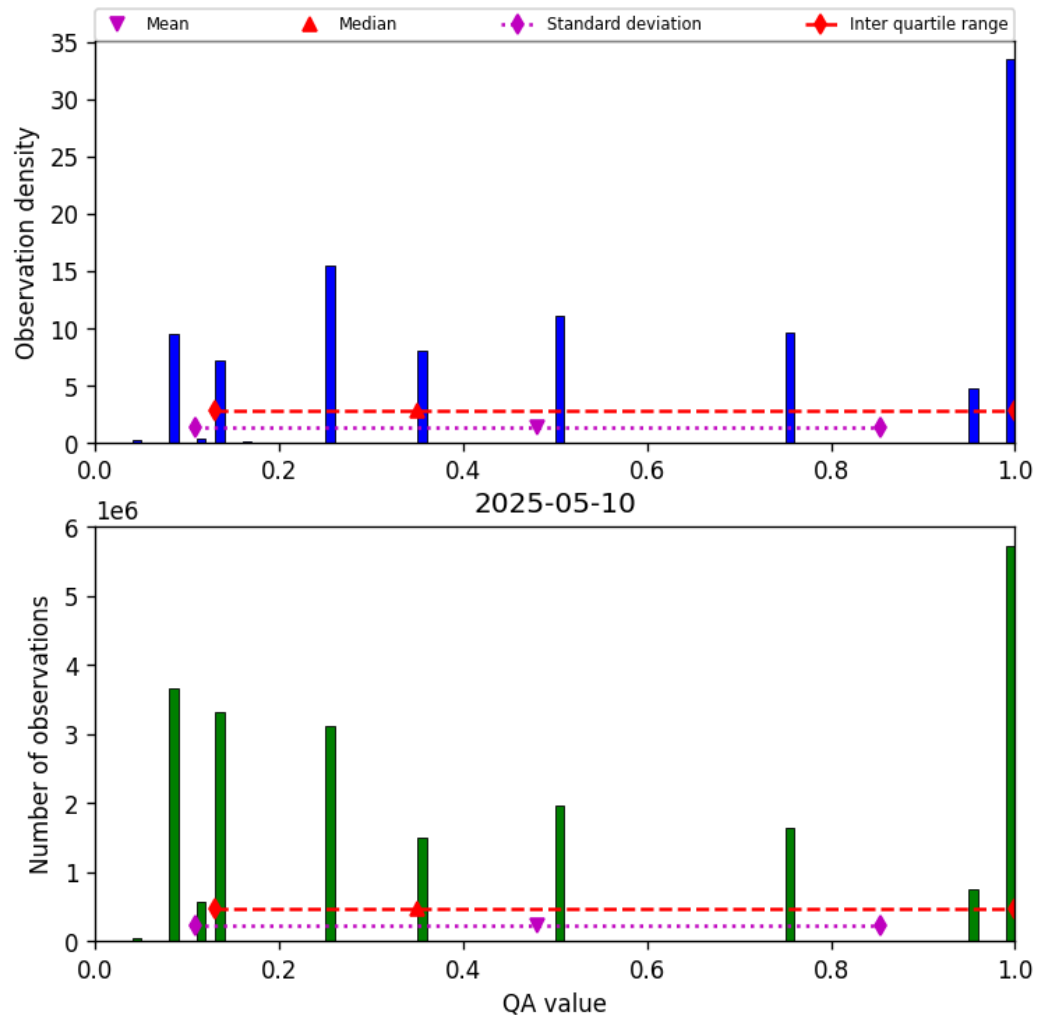
Figure 32: Histogram of “QA value” for 2025-05-10 to 2025-05-11
