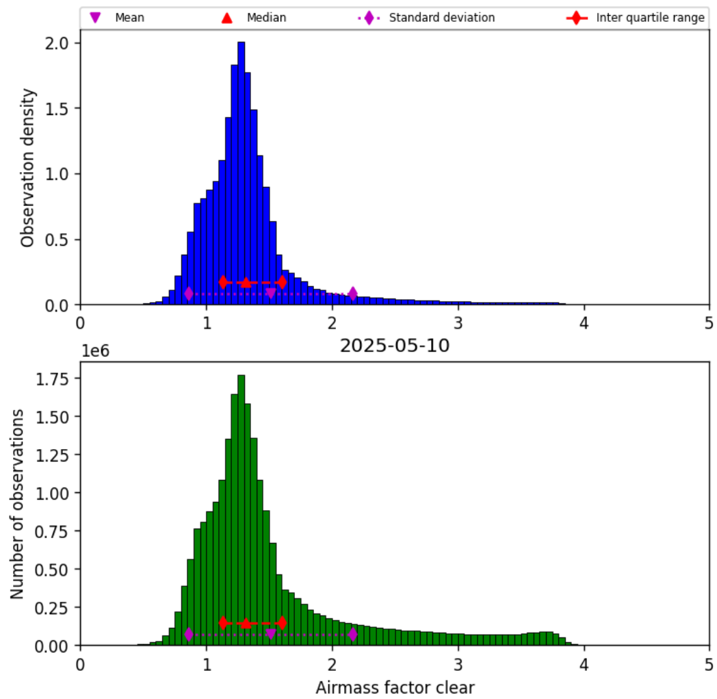
Figure 40: Histogram of “Airmass factor clear” for 2025-05-10 to 2025-05-11
