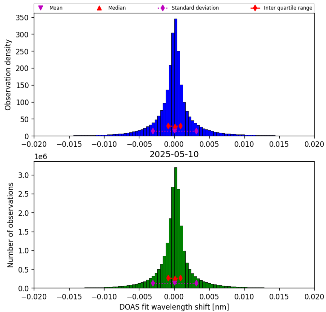
Figure 42: Histogram of “DOAS fit wavelength shift” for 2025-05-10 to 2025-05-11
