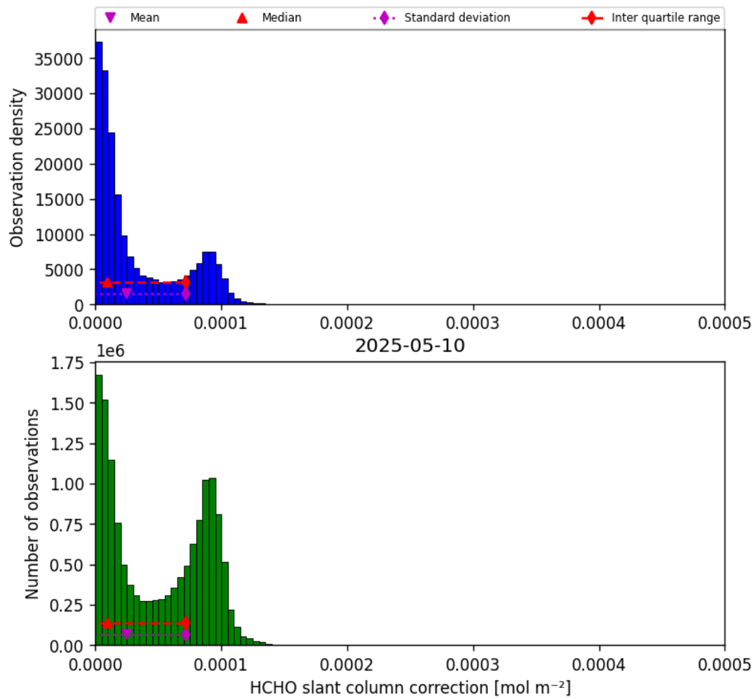
Figure 45: Histogram of “HCHO slant column correction” for 2025-05-10 to 2025-05-11
