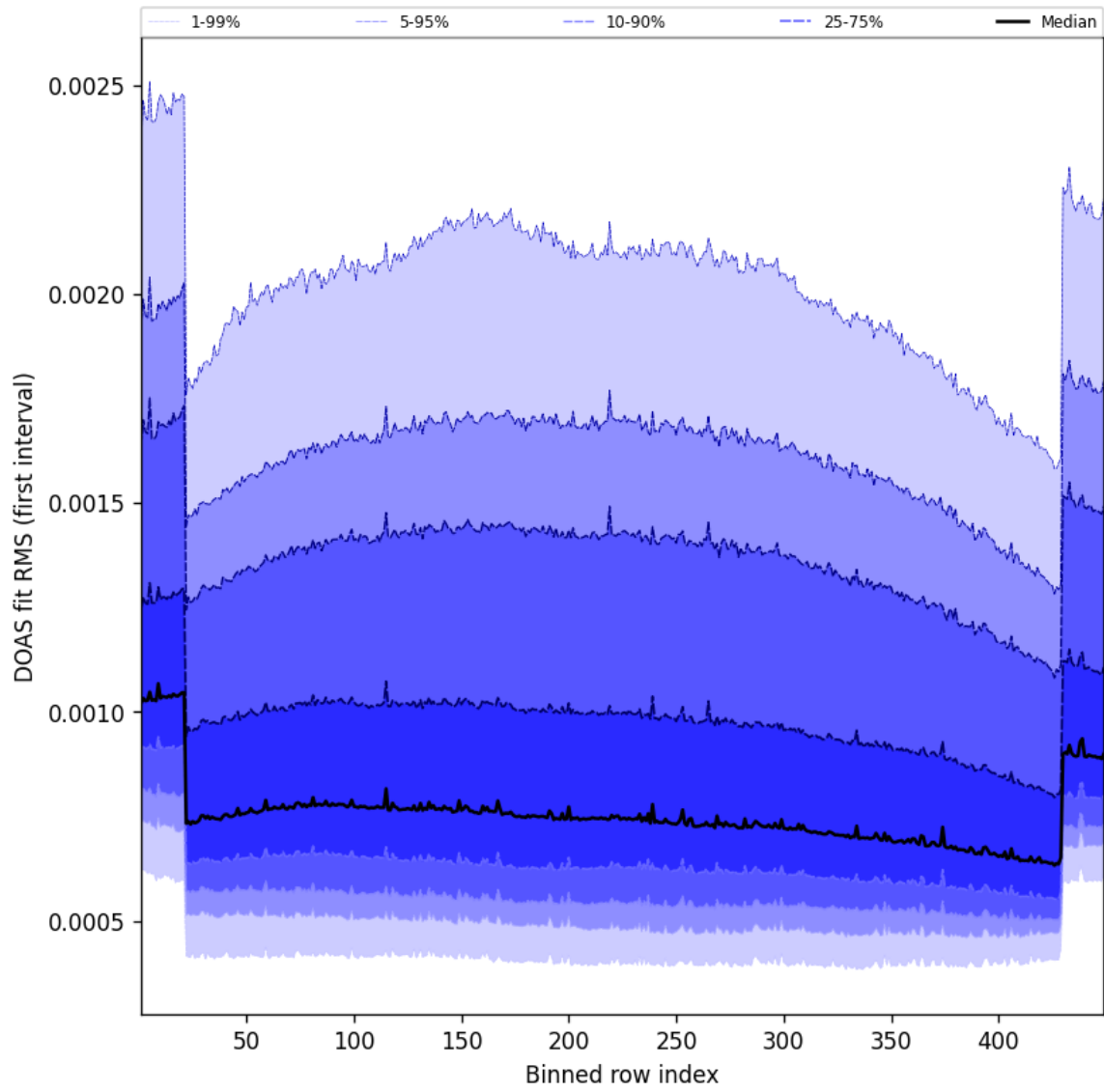
Figure 58: Along track statistics of “DOAS fit RMS (first interval)” for 2025-05-10 to 2025-05-11
