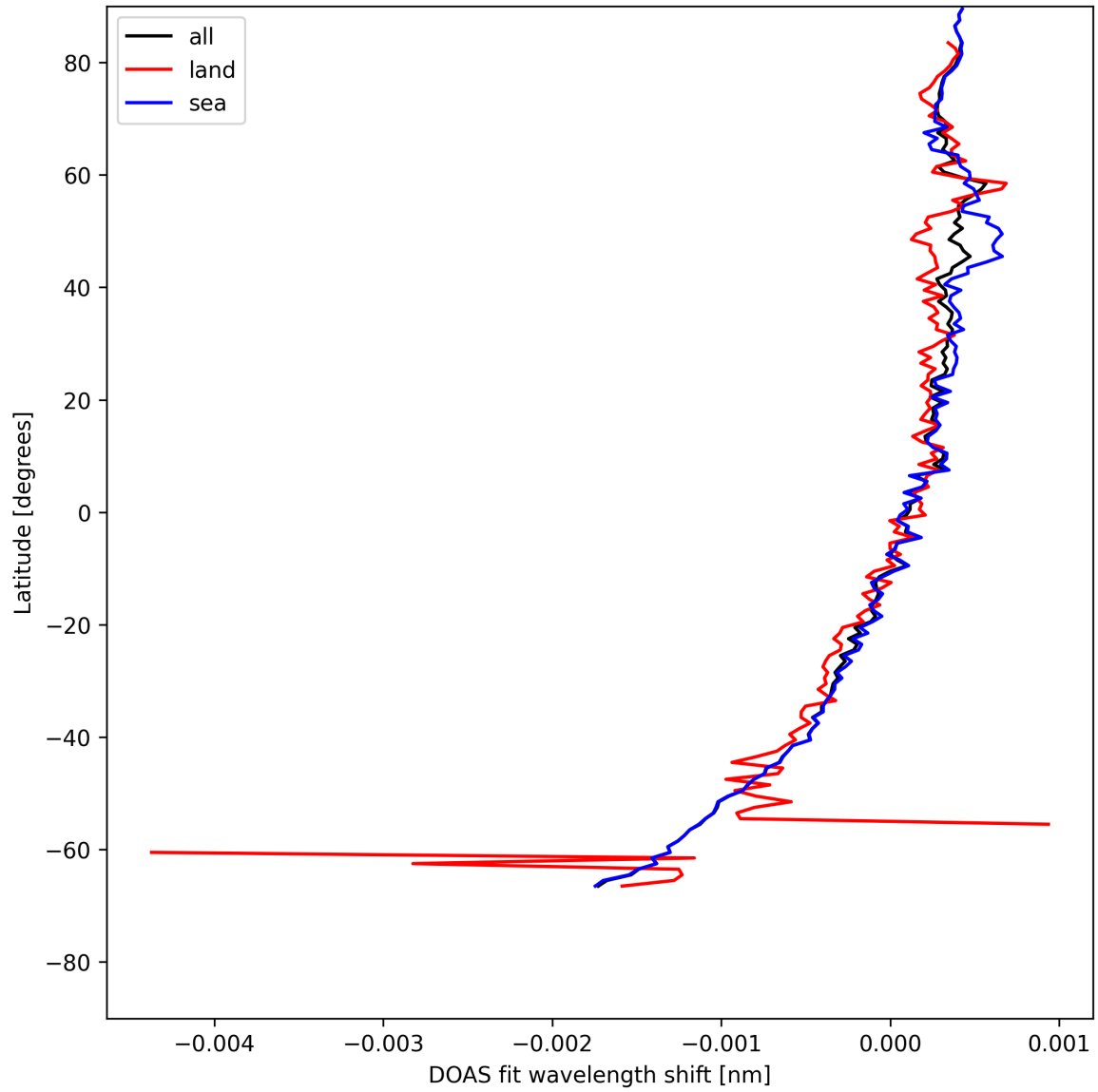
Figure 28: Zonal average of “DOAS fit wavelength shift” for 2025-05-10 to 2025-05-11.
