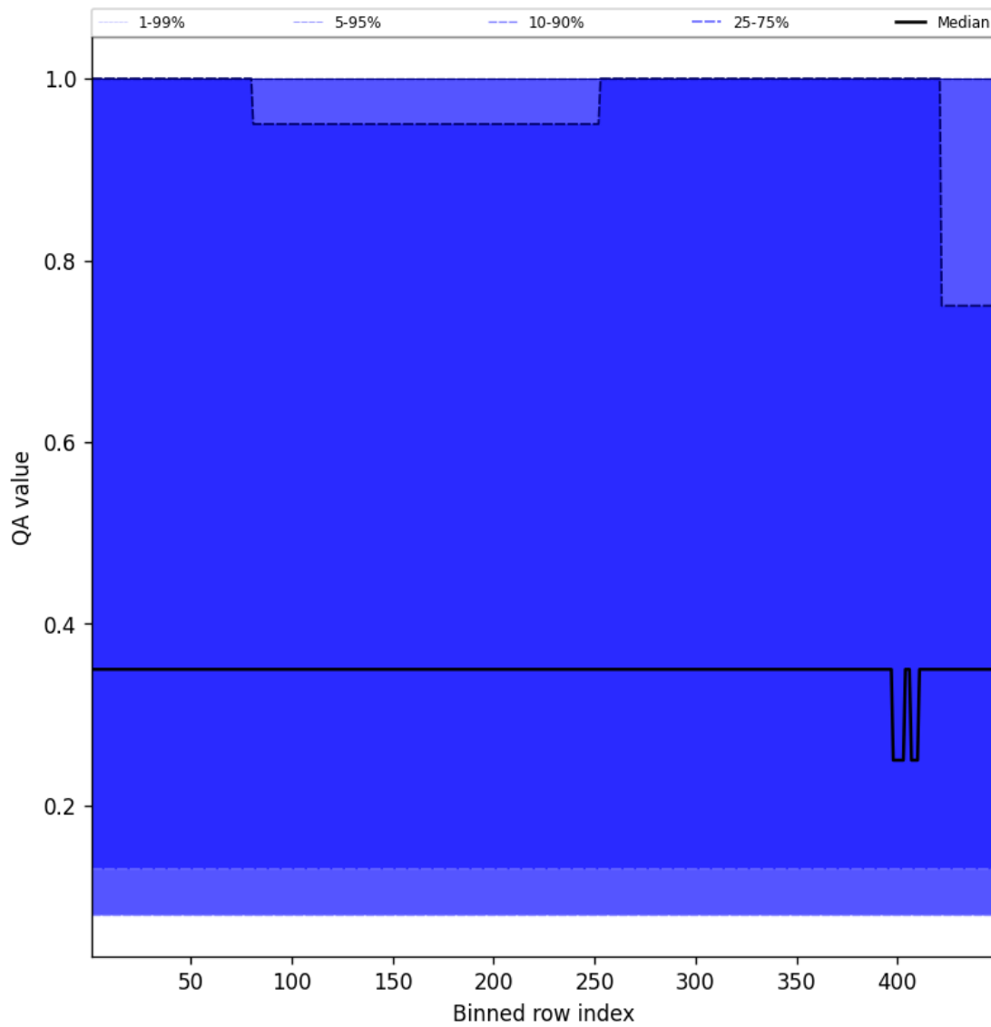
Figure 46: Along track statistics of “QA value” for 2025-05-10 to 2025-05-11
