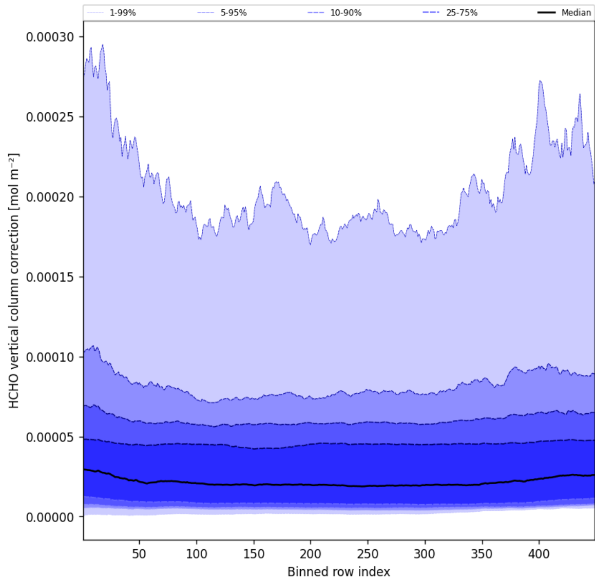
Figure 49: Along track statistics of “HCHO vertical column correction” for 2025-05-10 to 2025-05-11
