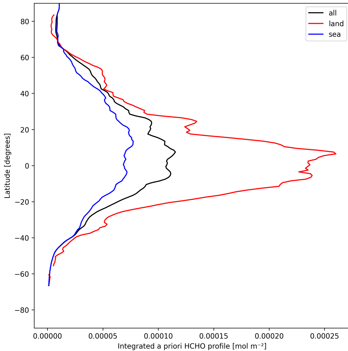
Figure 27: Zonal average of “Integrated a priori HCHO profile” for 2025-05-10 to 2025-05-11.
