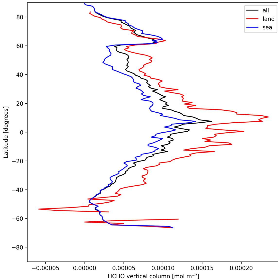
Figure 19: Zonal average of “HCHO vertical column” for 2025-05-10 to 2025-05-11.
