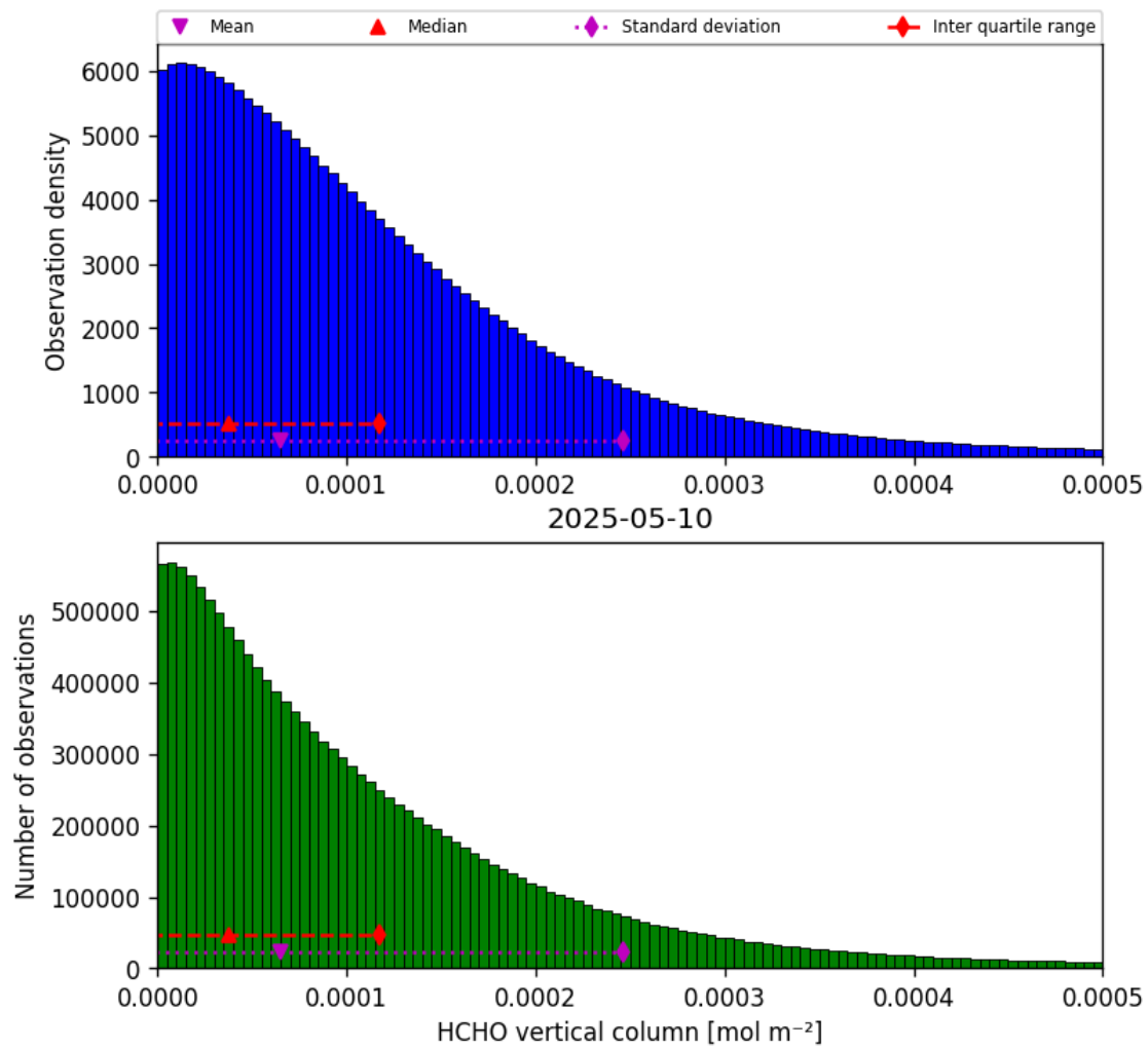
Figure 33: Histogram of “HCHO vertical column” for 2025-05-10 to 2025-05-11
