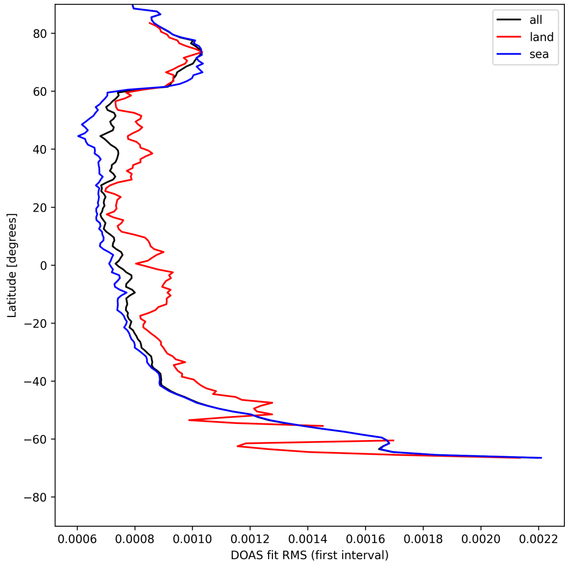
Figure 30: Zonal average of “DOAS fit RMS (first interval)” for 2025-05-10 to 2025-05-11.
