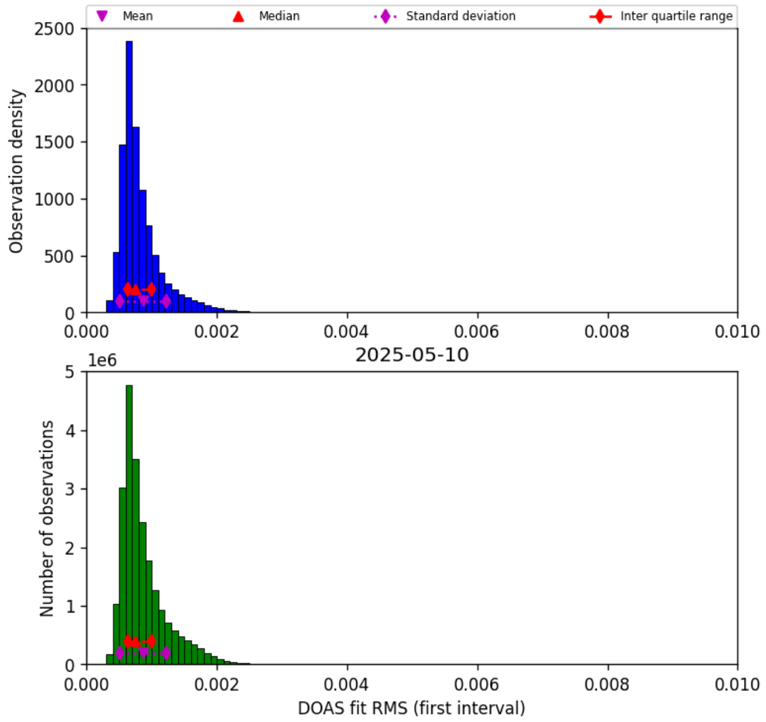
Figure 44: Histogram of “DOAS fit RMS (first interval)” for 2025-05-10 to 2025-05-11
