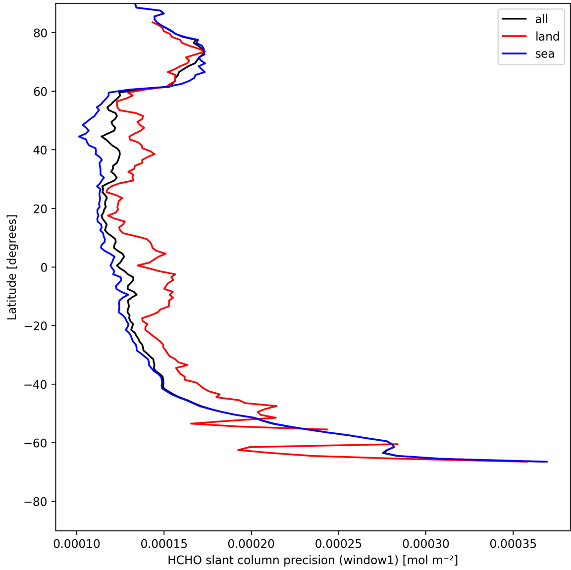
Figure 23: Zonal average of “HCHO slant column precision (window1)” for 2025-05-10 to 2025-05-11.
