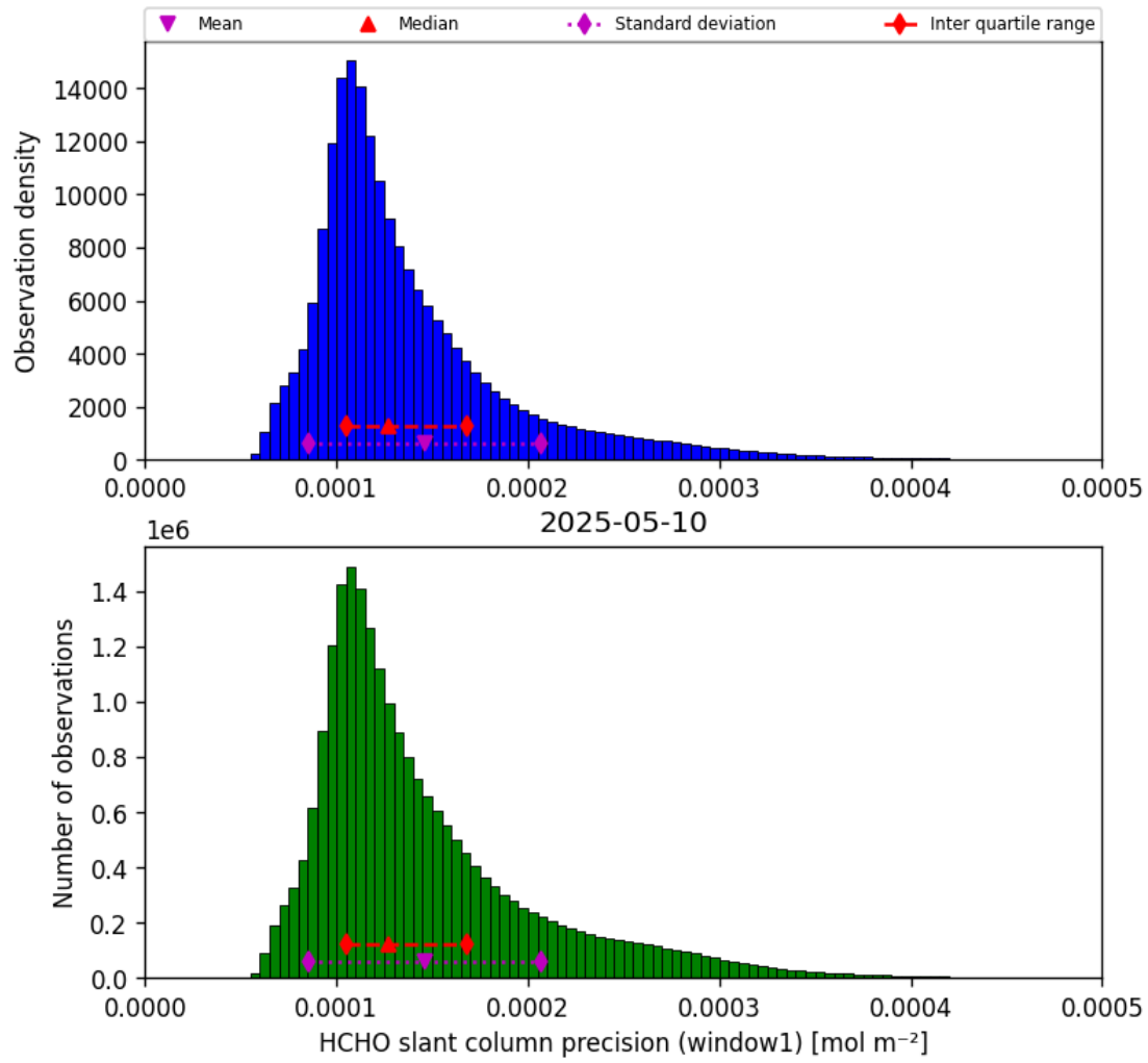
Figure 37: Histogram of “HCHO slant column precision (window1)” for 2025-05-10 to 2025-05-11
