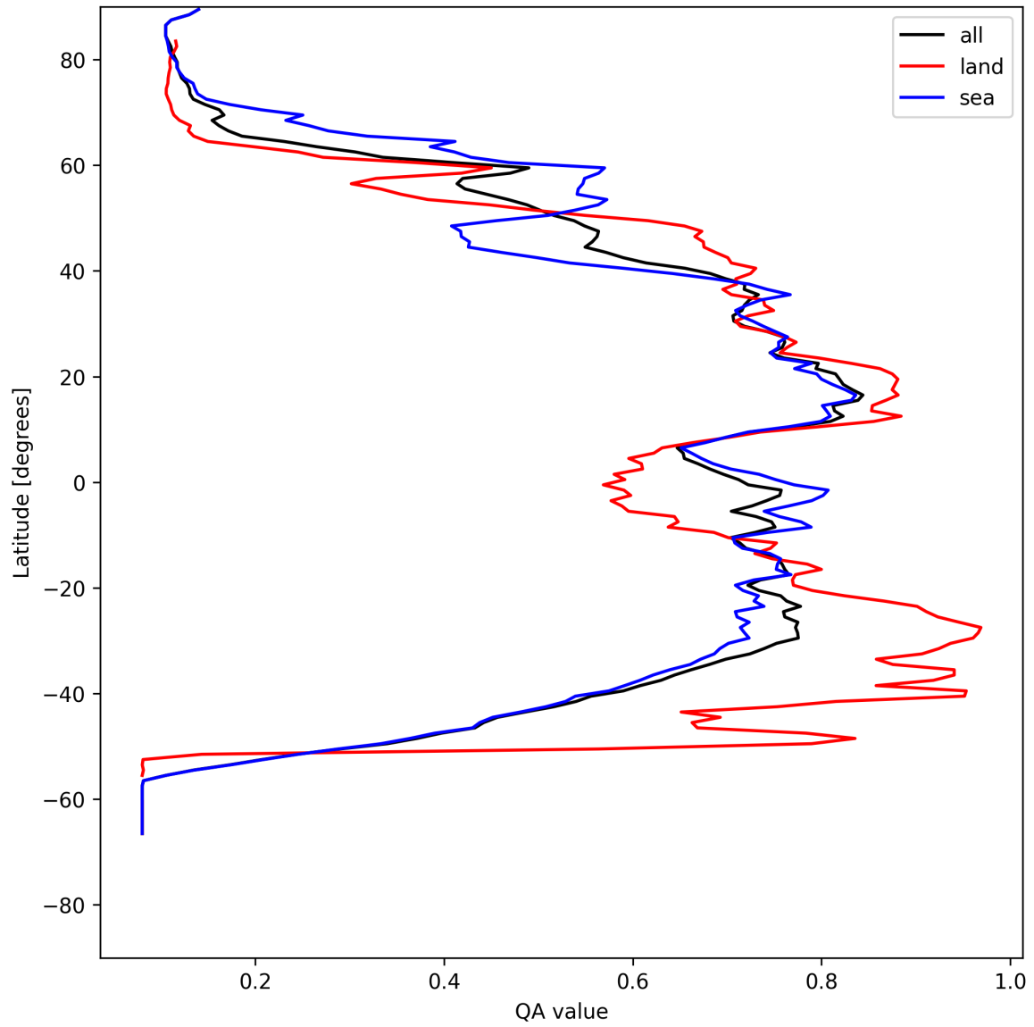
Figure 18: Zonal average of “QA value” for 2025-05-10 to 2025-05-11.
