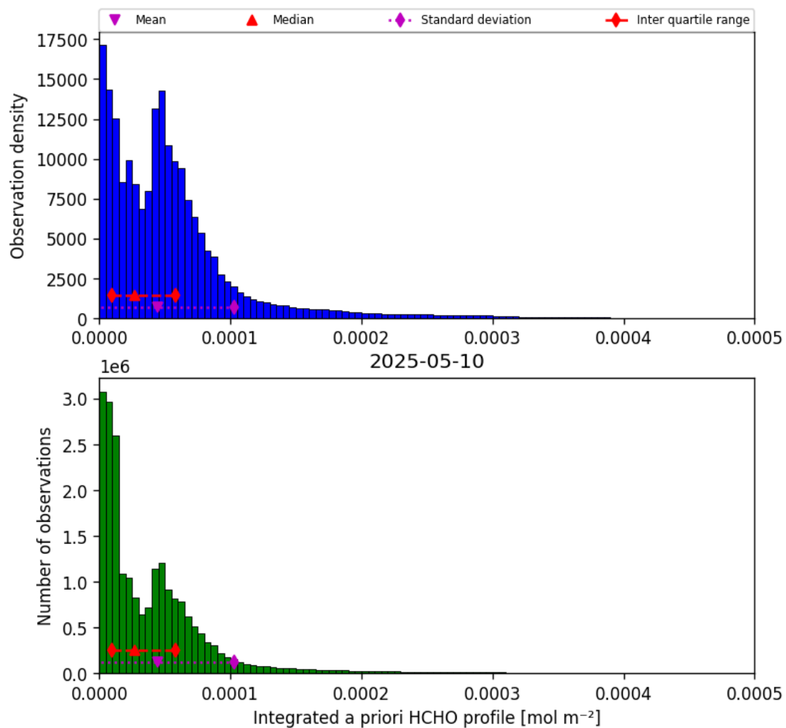
Figure 41: Histogram of “Integrated a priori HCHO profile” for 2025-05-10 to 2025-05-11
