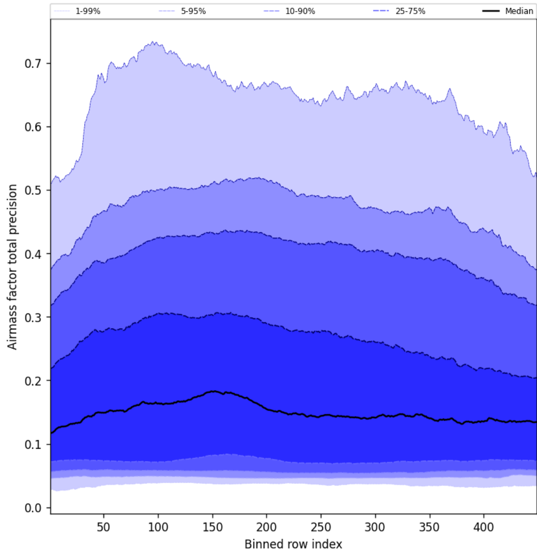
Figure 53: Along track statistics of “Airmass factor total precision” for 2025-05-10 to 2025-05-11
