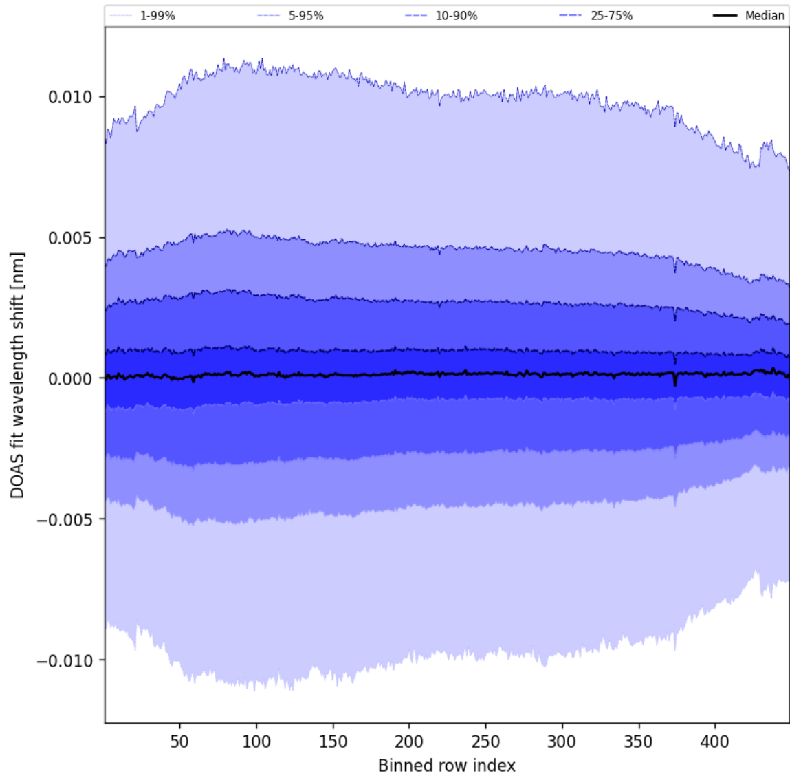
Figure 56: Along track statistics of “DOAS fit wavelength shift” for 2025-05-10 to 2025-05-11
