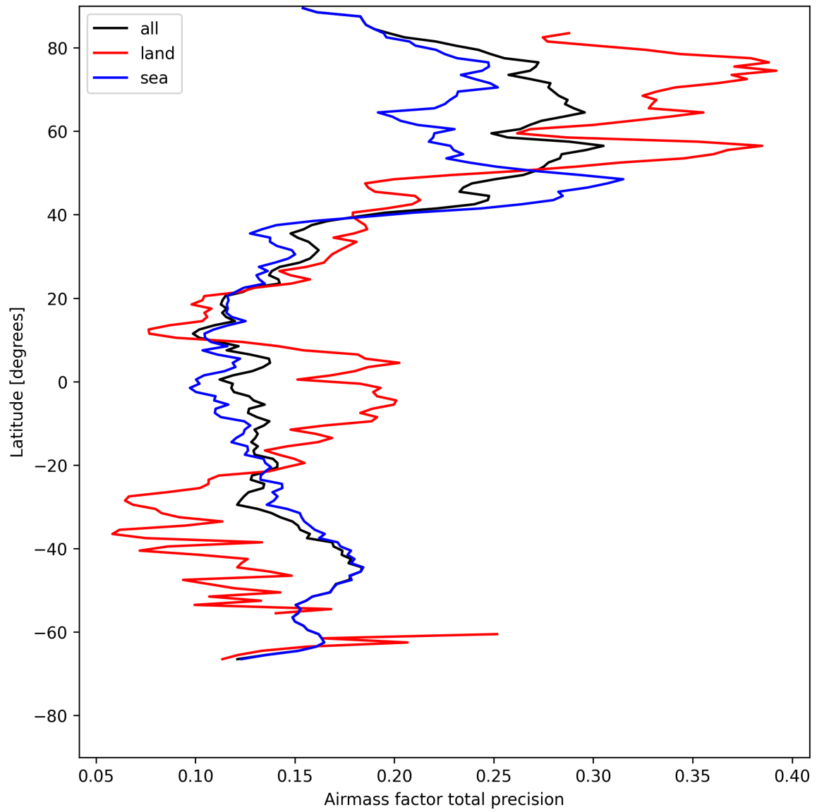
Figure 25: Zonal average of “Airmass factor total precision” for 2025-05-10 to 2025-05-11.
