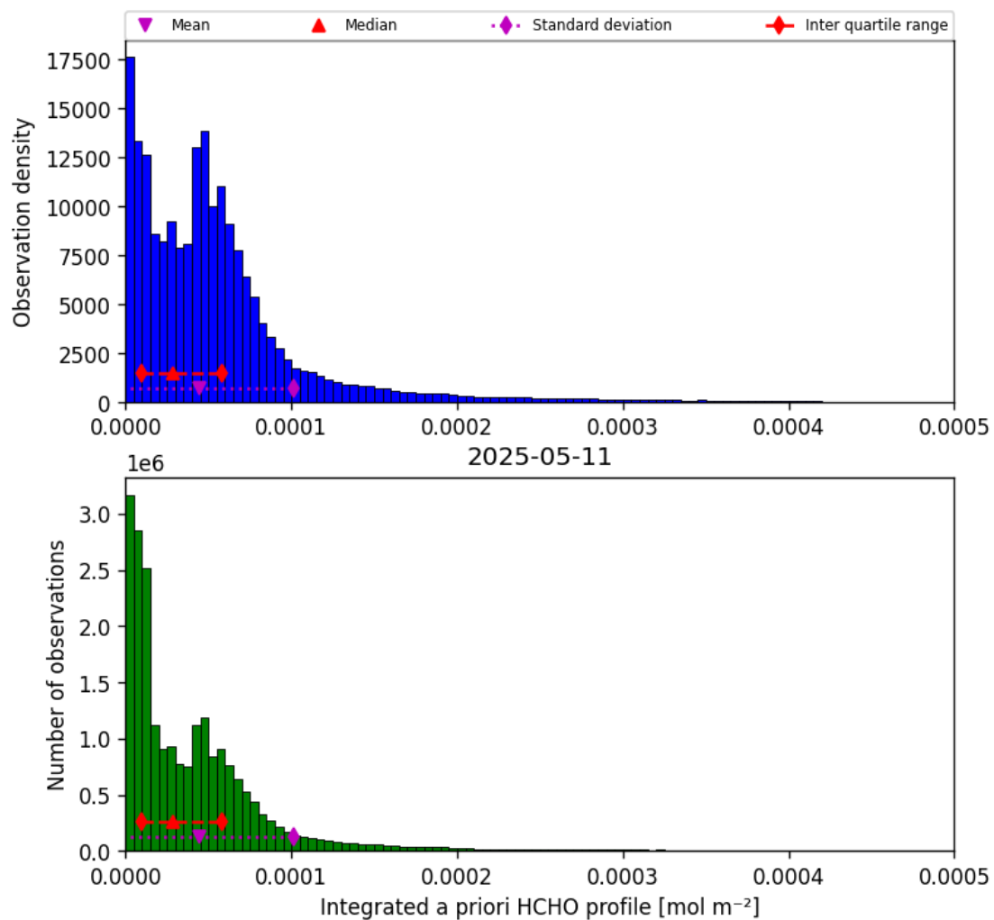
Figure 41: Histogram of “Integrated a priori HCHO profile” for 2025-05-11 to 2025-05-12
