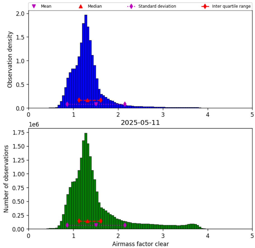
Figure 40: Histogram of “Airmass factor clear” for 2025-05-11 to 2025-05-12
