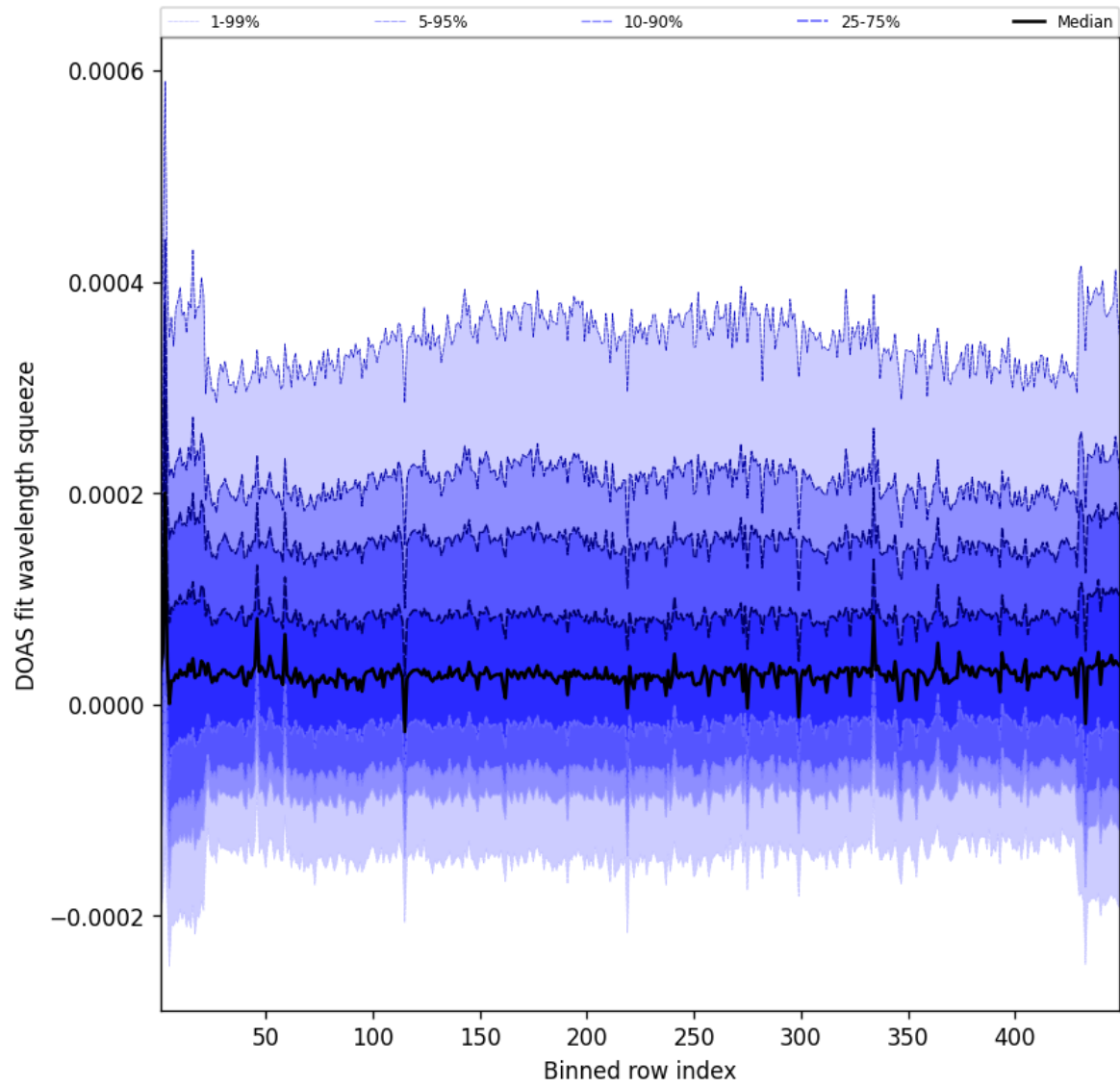
Figure 57: Along track statistics of “DOAS fit wavelength squeeze” for 2025-05-11 to 2025-05-12
