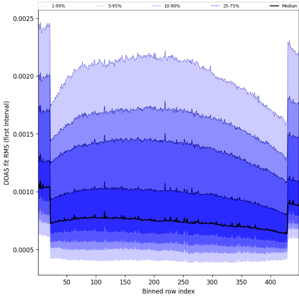
Figure 58: Along track statistics of “DOAS fit RMS (first interval)” for 2025-05-11 to 2025-05-12
