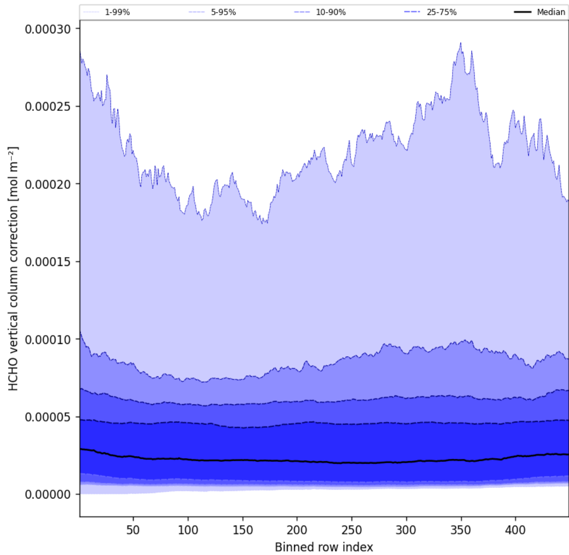
Figure 49: Along track statistics of “HCHO vertical column correction” for 2025-05-11 to 2025-05-12
