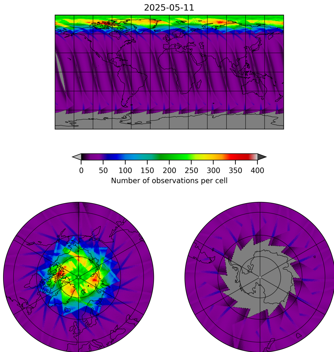
Figure 17: Map of the number of observations for 2025-05-11 to 2025-05-12
