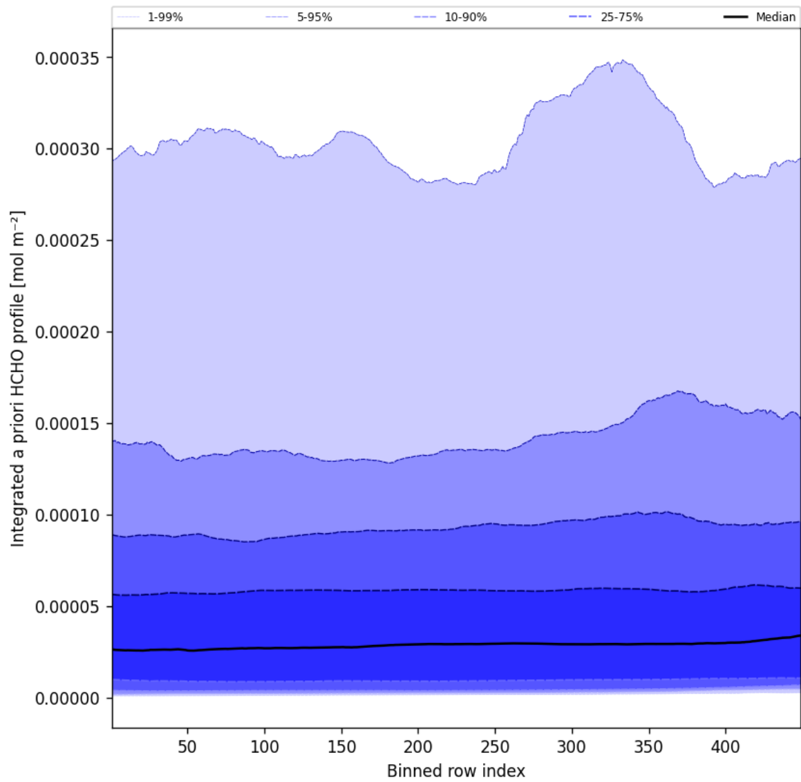
Figure 55: Along track statistics of “Integrated a priori HCHO profile” for 2025-05-11 to 2025-05-12
