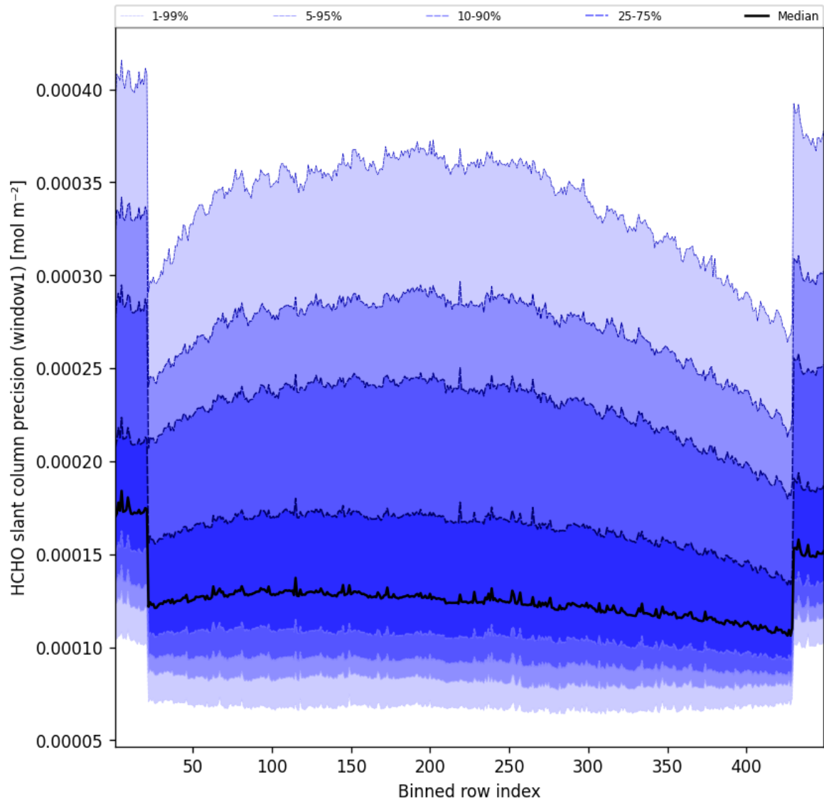
Figure 51: Along track statistics of “HCHO slant column precision (window1)” for 2025-05-11 to 2025-05-12
