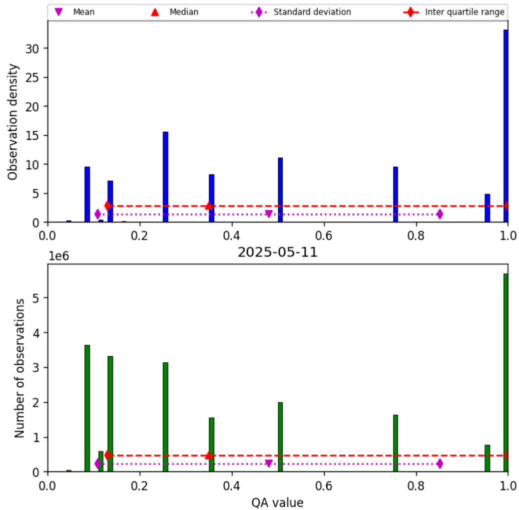
Figure 32: Histogram of “QA value” for 2025-05-11 to 2025-05-12
