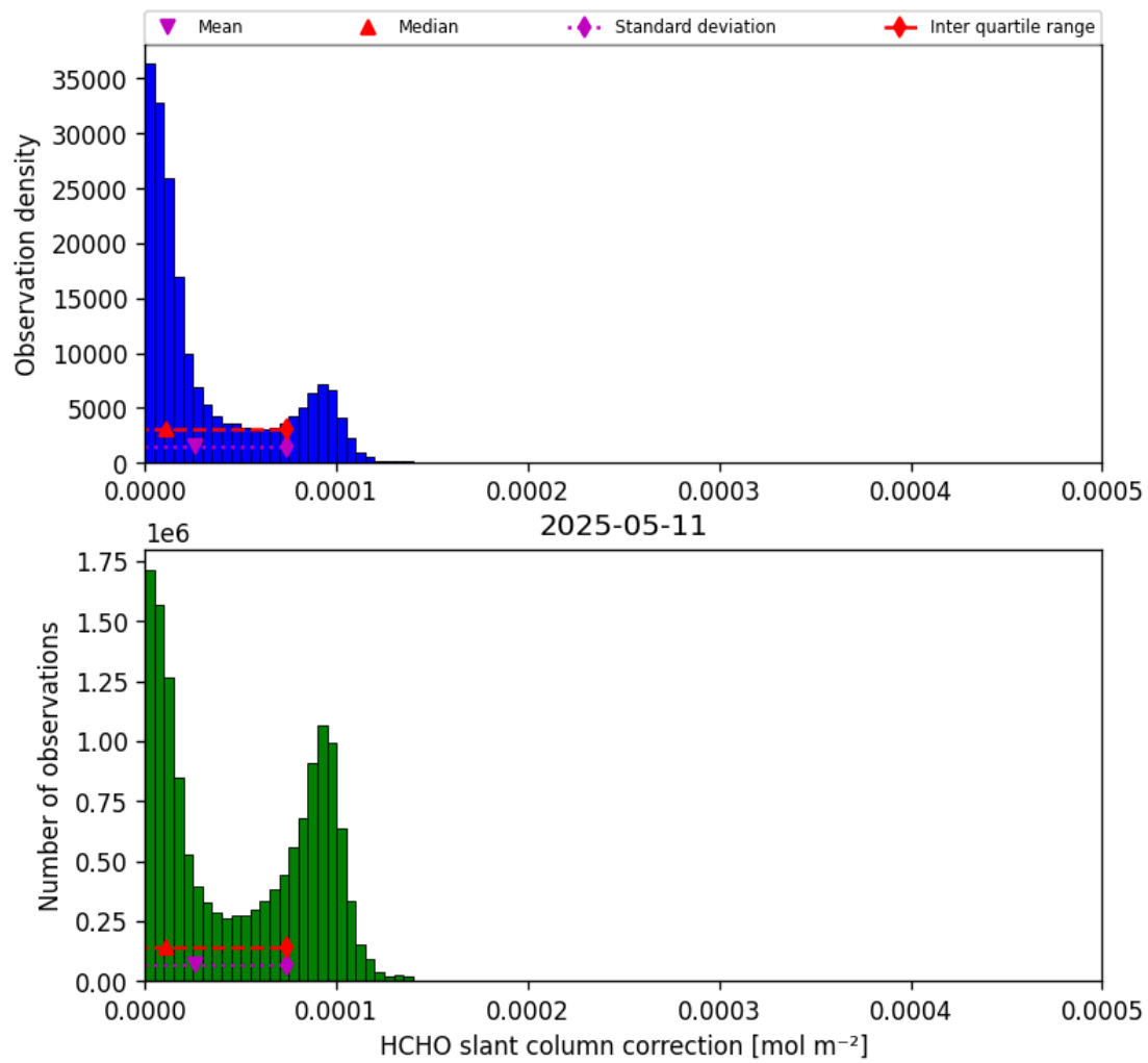
Figure 45: Histogram of “HCHO slant column correction” for 2025-05-11 to 2025-05-12
