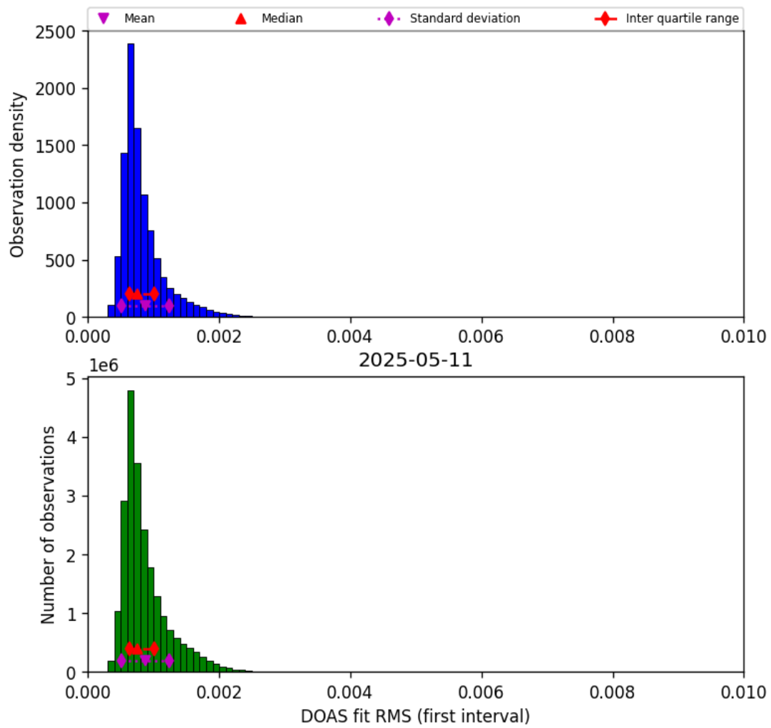
Figure 44: Histogram of “DOAS fit RMS (first interval)” for 2025-05-11 to 2025-05-12
