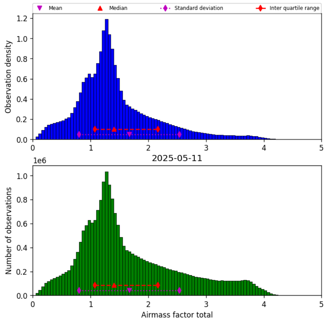
Figure 38: Histogram of “Airmass factor total” for 2025-05-11 to 2025-05-12
