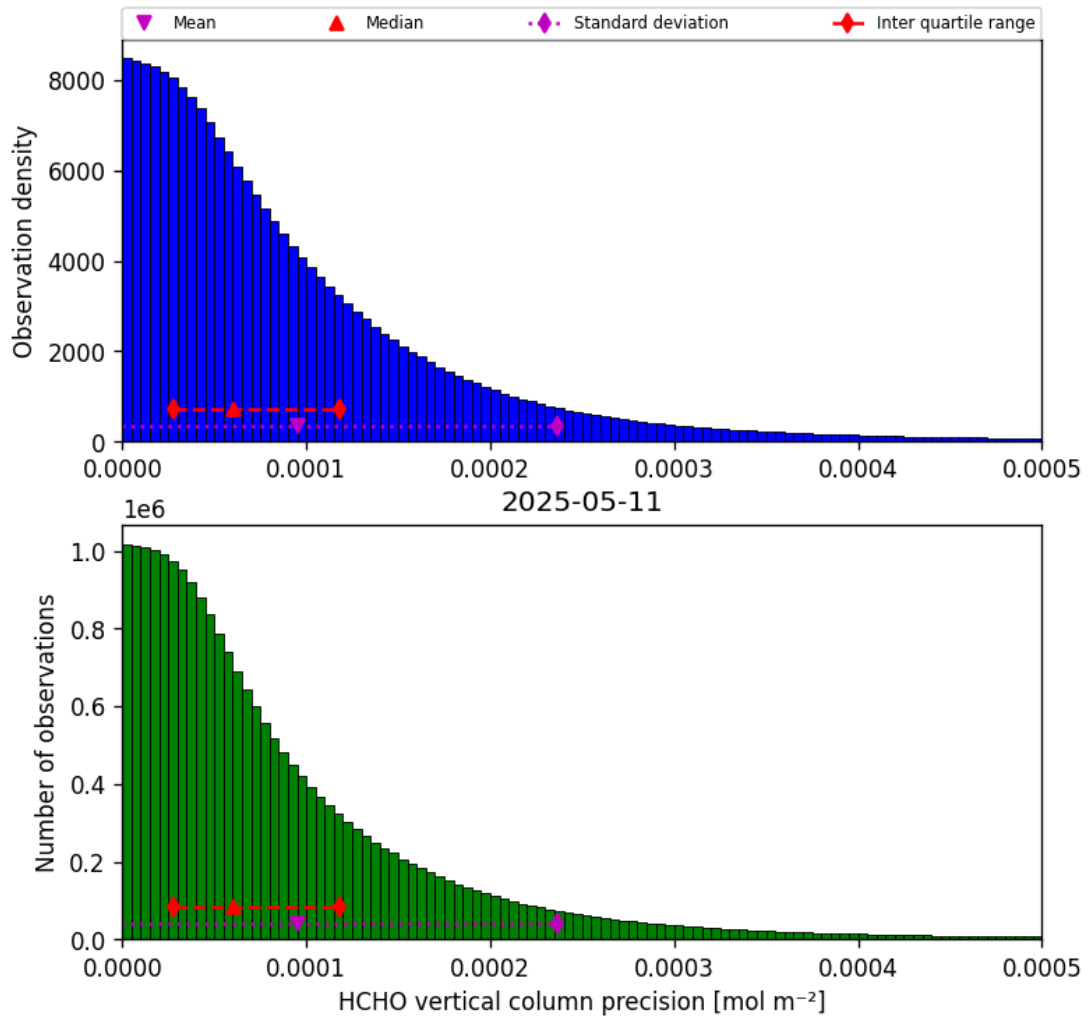
Figure 34: Histogram of “HCHO vertical column precision” for 2025-05-11 to 2025-05-12
