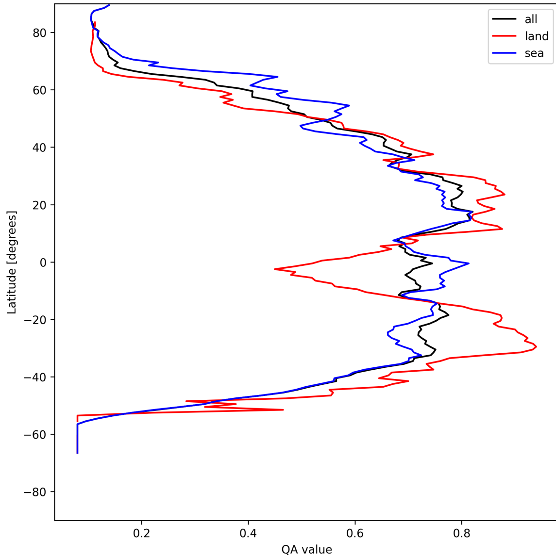
Figure 18: Zonal average of “QA value” for 2025-05-11 to 2025-05-12.
