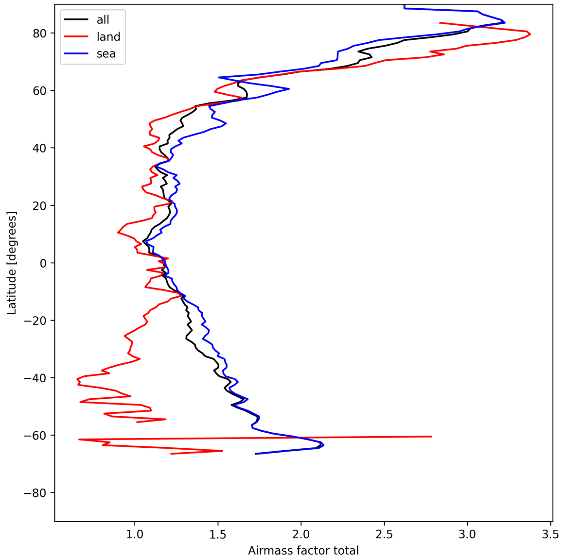
Figure 24: Zonal average of “Airmass factor total” for 2025-05-11 to 2025-05-12.
