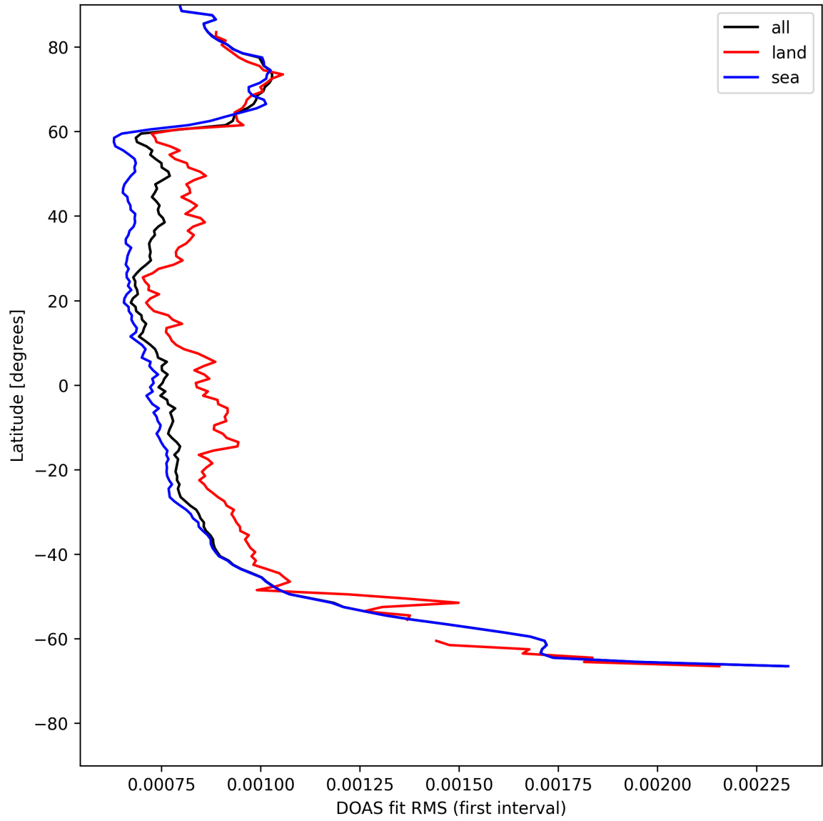
Figure 30: Zonal average of “DOAS fit RMS (first interval)” for 2025-05-11 to 2025-05-12.
