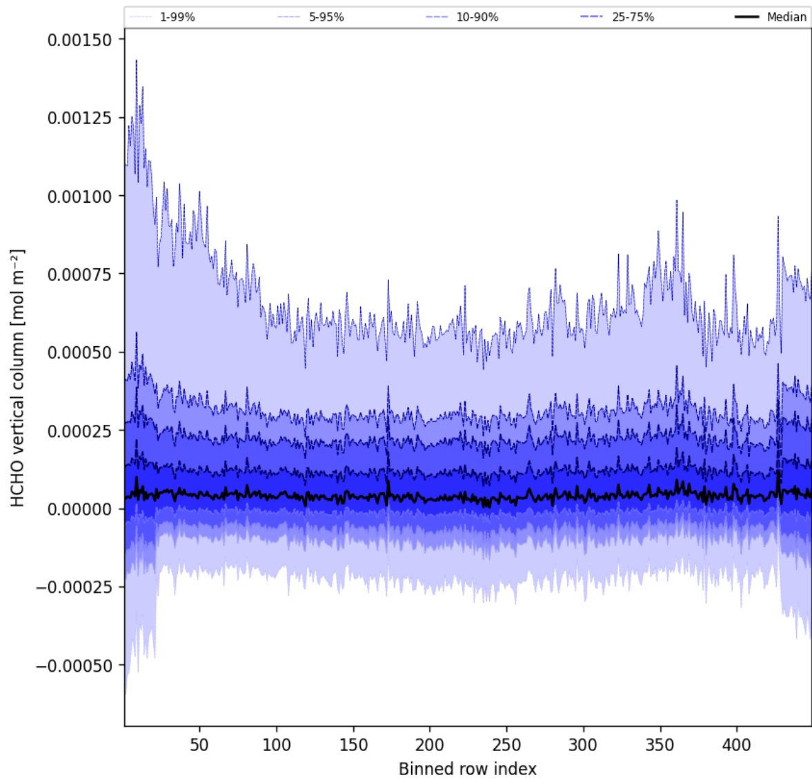
Figure 47: Along track statistics of “HCHO vertical column” for 2025-05-11 to 2025-05-12
