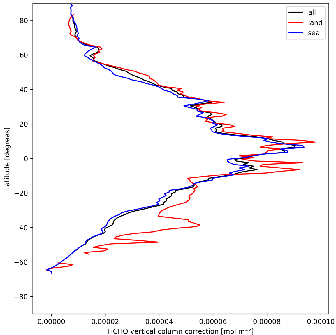
Figure 21: Zonal average of “HCHO vertical column correction” for 2025-05-11 to 2025-05-12.
