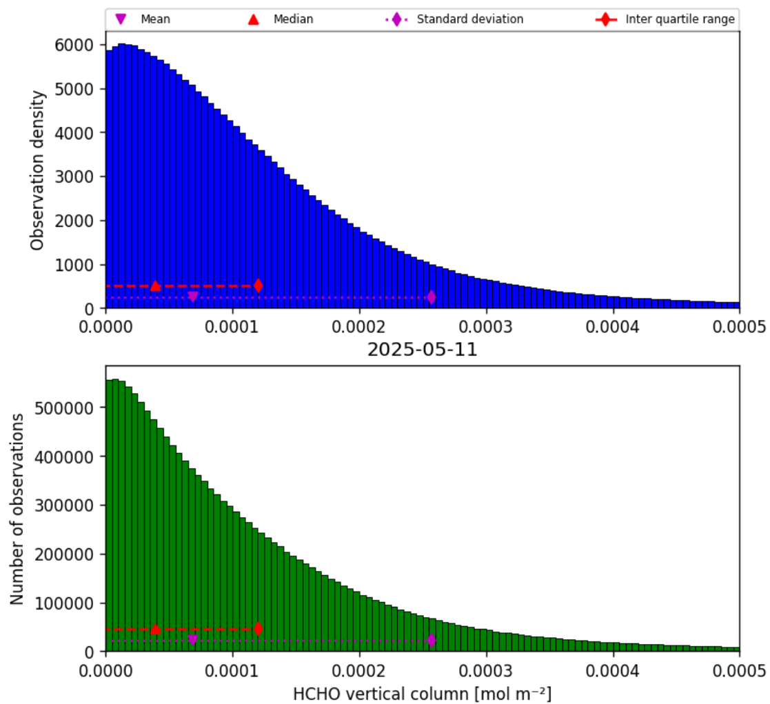
Figure 33: Histogram of “HCHO vertical column” for 2025-05-11 to 2025-05-12
