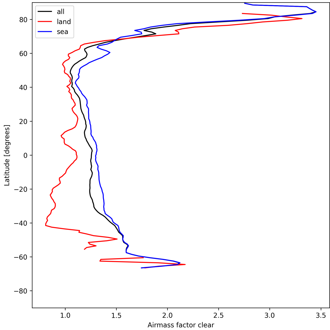
Figure 26: Zonal average of “Airmass factor clear” for 2025-05-11 to 2025-05-12.
