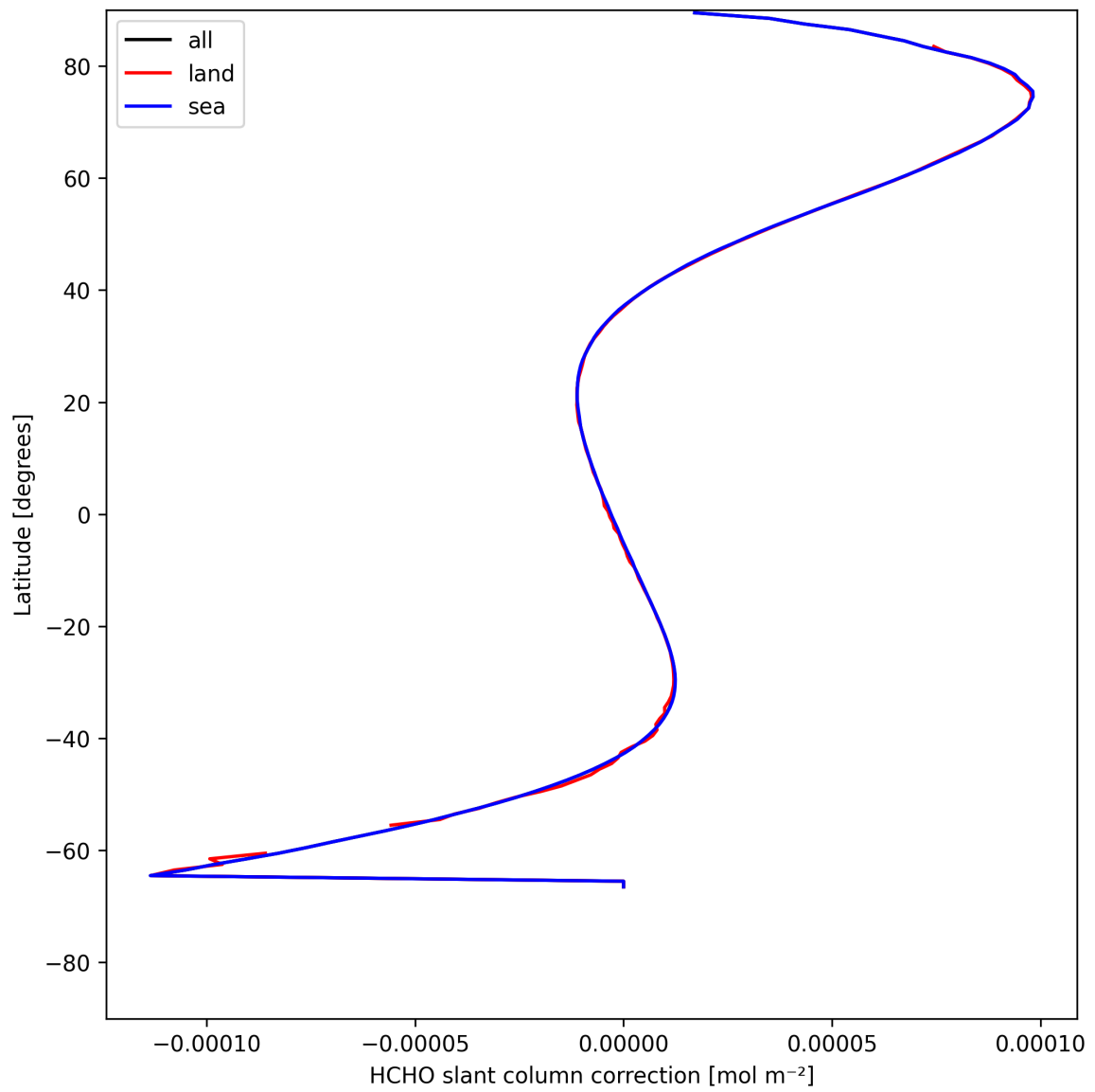
Figure 31: Zonal average of “HCHO slant column correction” for 2025-05-11 to 2025-05-12.
