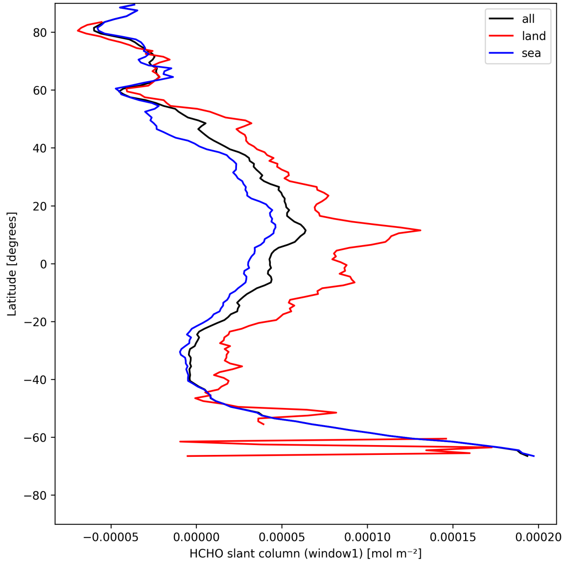
Figure 22: Zonal average of “HCHO slant column (window1)” for 2025-05-11 to 2025-05-12.
