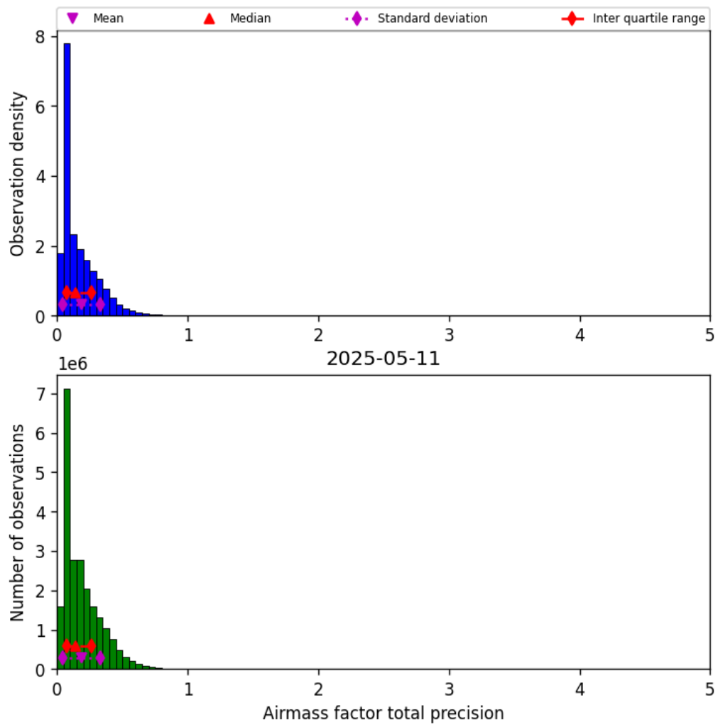
Figure 39: Histogram of “Airmass factor total precision” for 2025-05-11 to 2025-05-12
