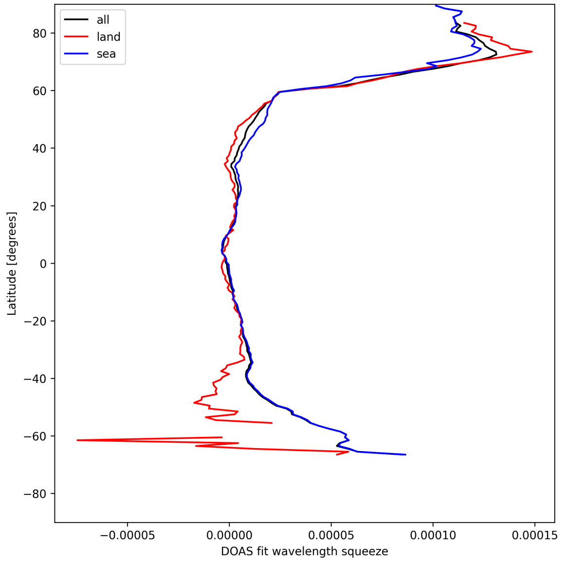
Figure 29: Zonal average of “DOAS fit wavelength squeeze” for 2025-05-11 to 2025-05-12.
