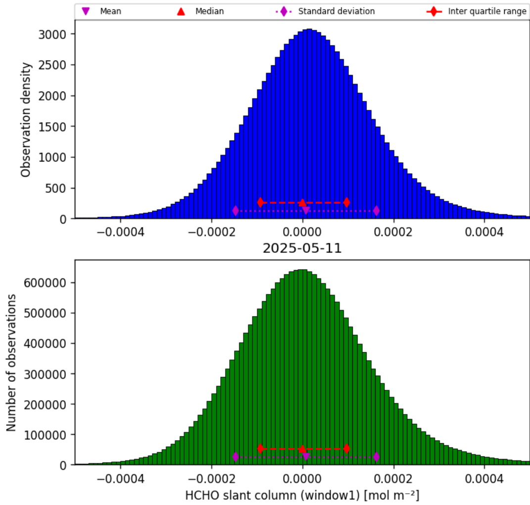
Figure 36: Histogram of “HCHO slant column (window1)” for 2025-05-11 to 2025-05-12
