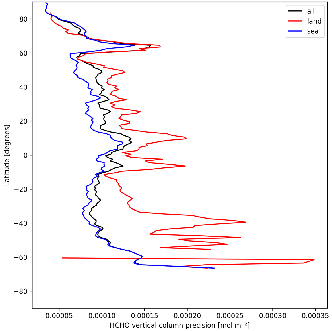
Figure 20: Zonal average of “HCHO vertical column precision” for 2025-05-11 to 2025-05-12.
