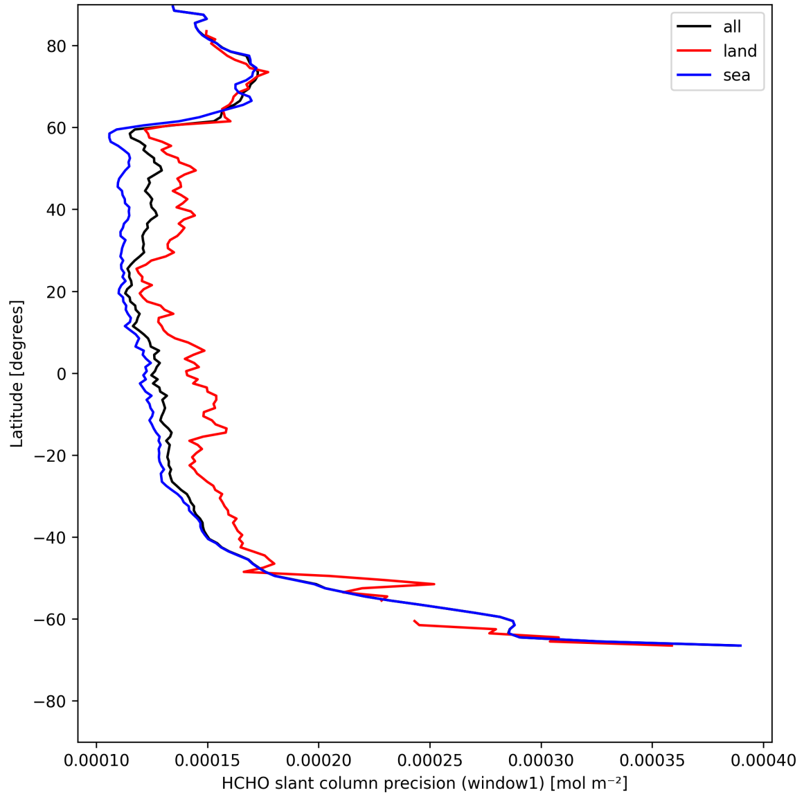
Figure 23: Zonal average of “HCHO slant column precision (window1)” for 2025-05-11 to 2025-05-12.
