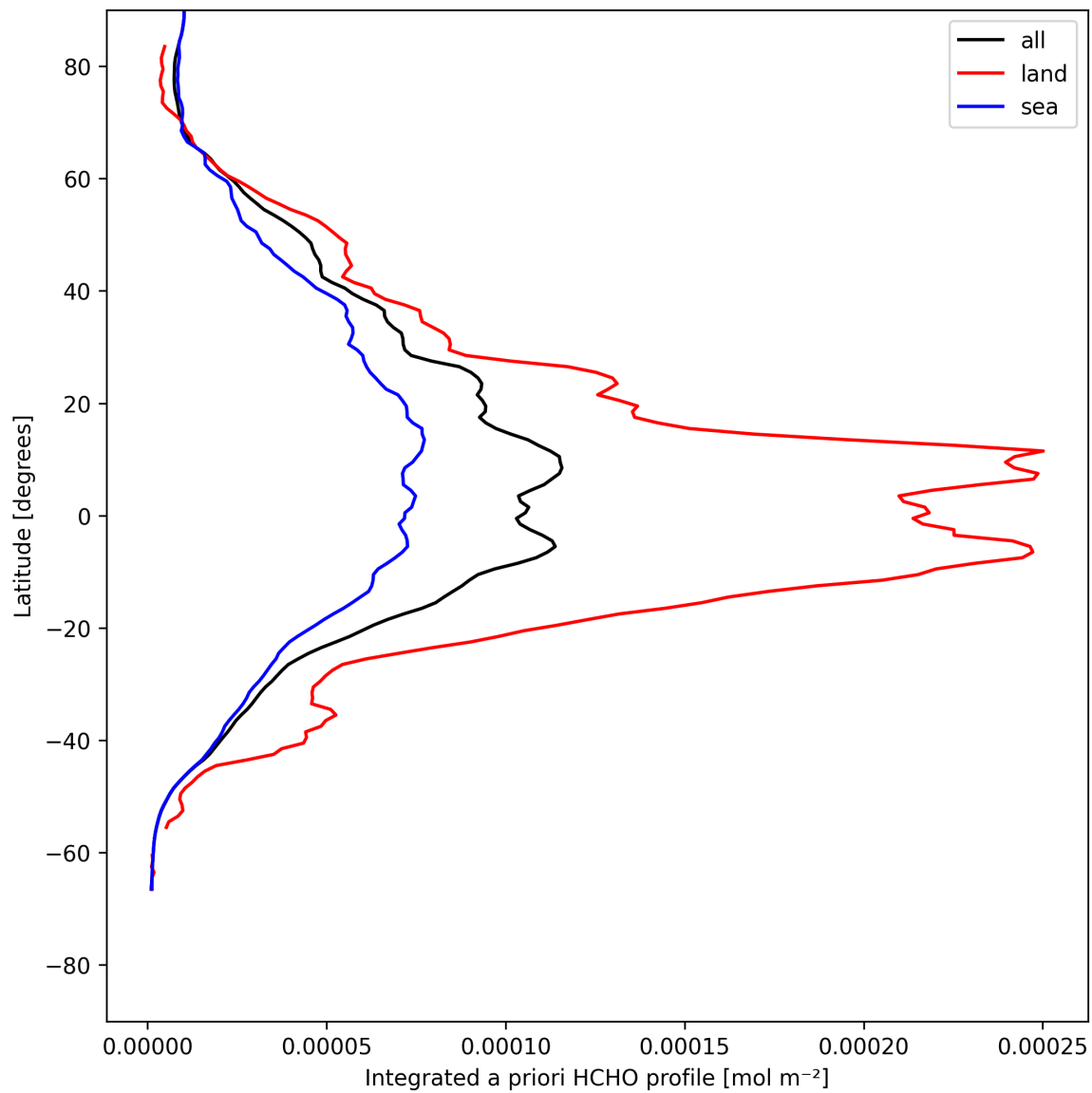
Figure 27: Zonal average of “Integrated a priori HCHO profile” for 2025-05-11 to 2025-05-12.
