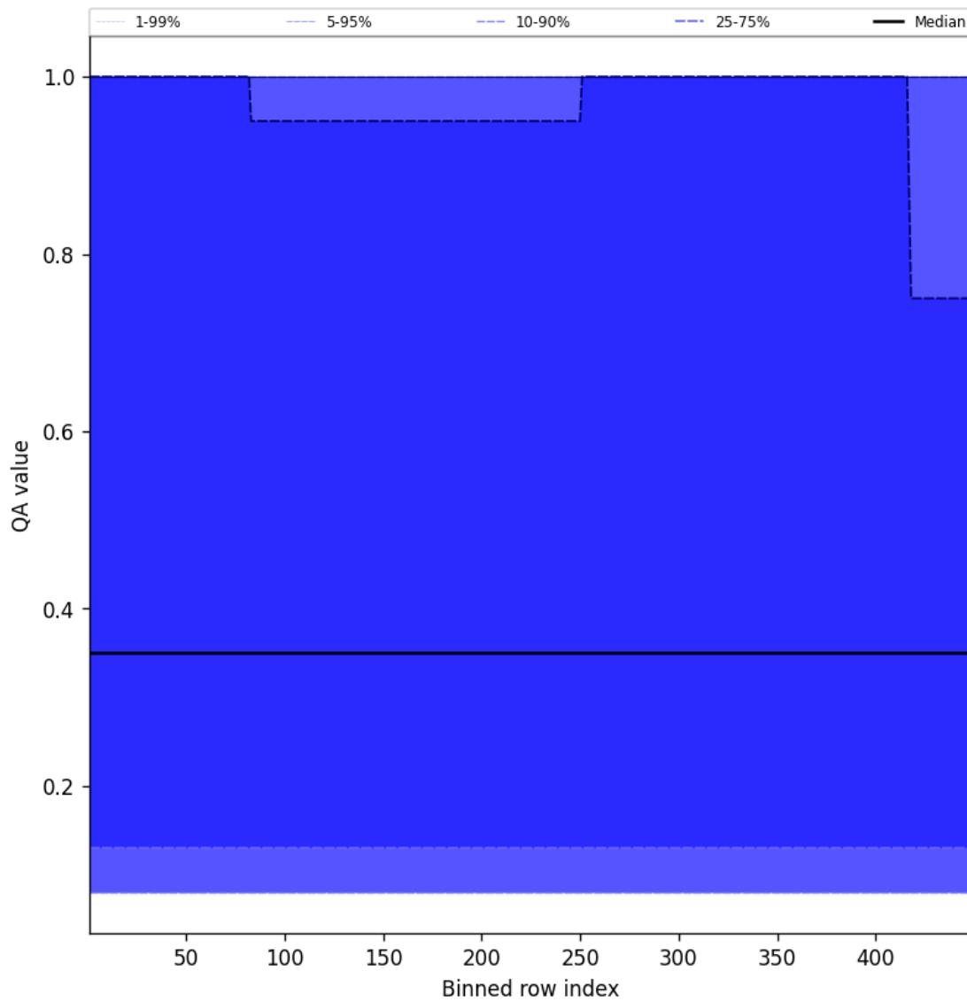
Figure 46: Along track statistics of “QA value” for 2025-05-11 to 2025-05-12
