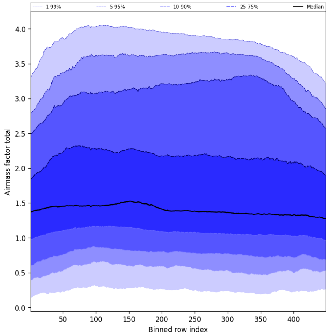
Figure 52: Along track statistics of “Airmass factor total” for 2025-05-11 to 2025-05-12
