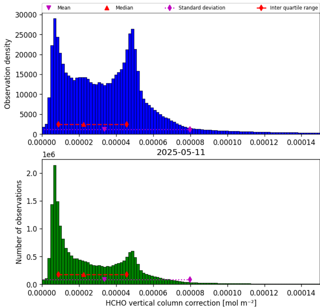
Figure 35: Histogram of “HCHO vertical column correction” for 2025-05-11 to 2025-05-12
