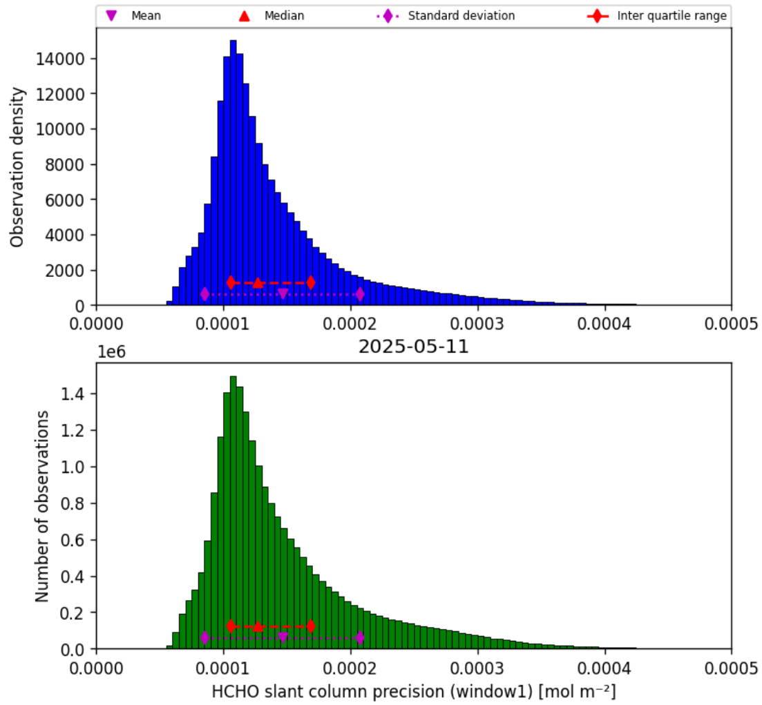
Figure 37: Histogram of “HCHO slant column precision (window1)” for 2025-05-11 to 2025-05-12
