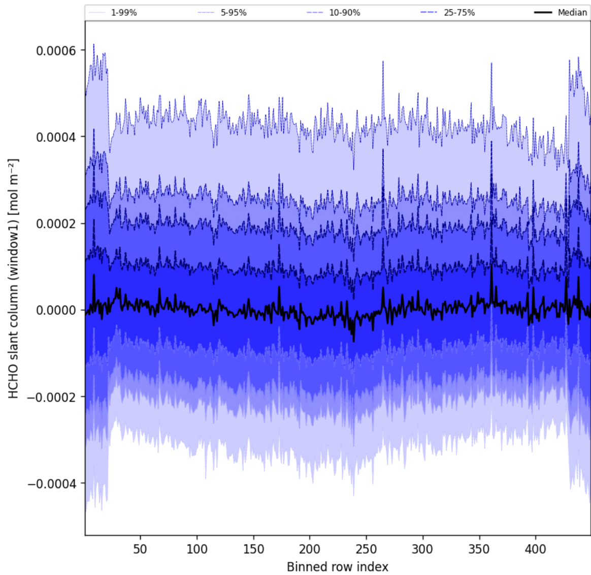
Figure 50: Along track statistics of “HCHO slant column (window1)” for 2025-05-11 to 2025-05-12
