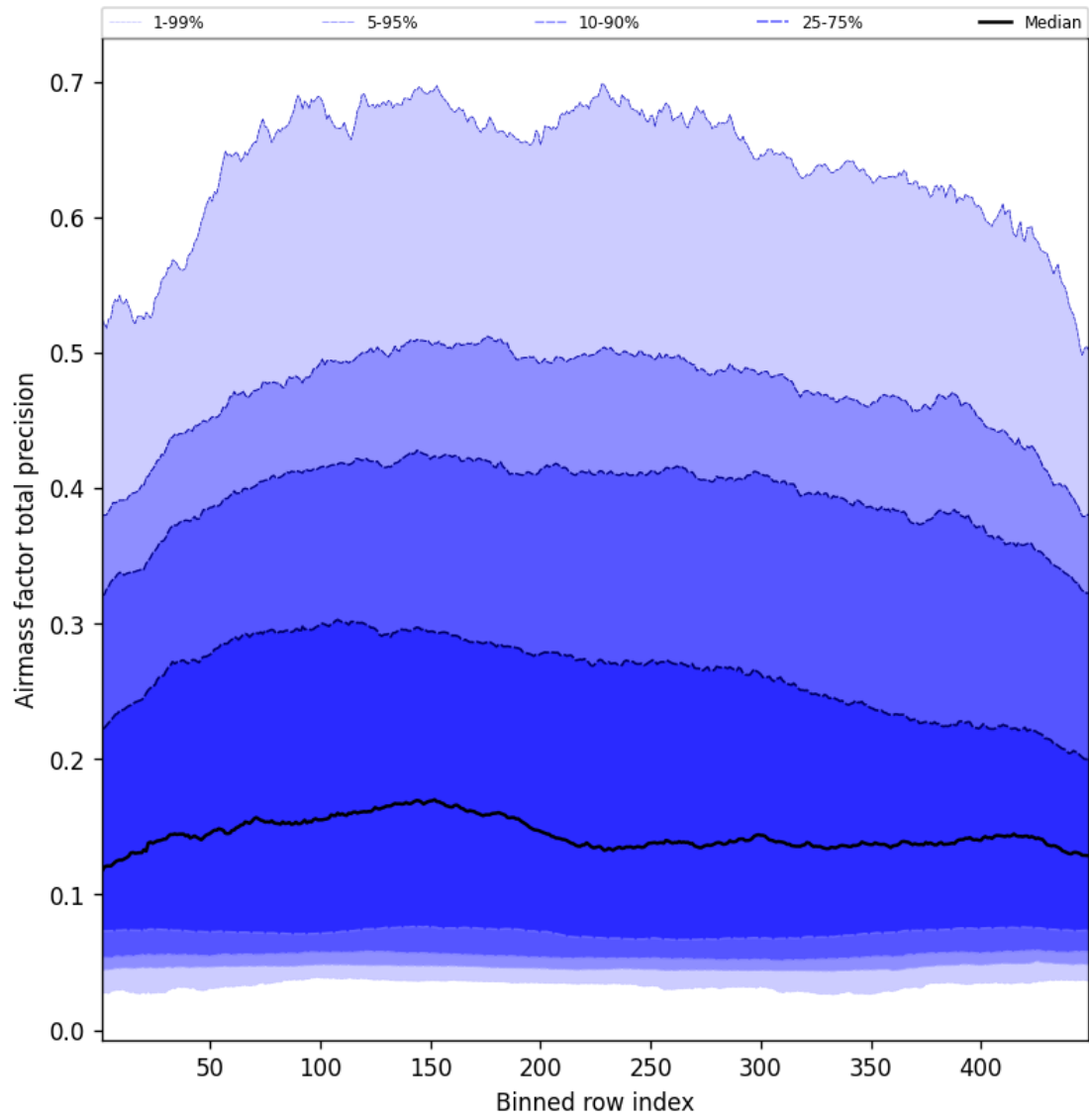
Figure 53: Along track statistics of “Airmass factor total precision” for 2025-05-11 to 2025-05-12
