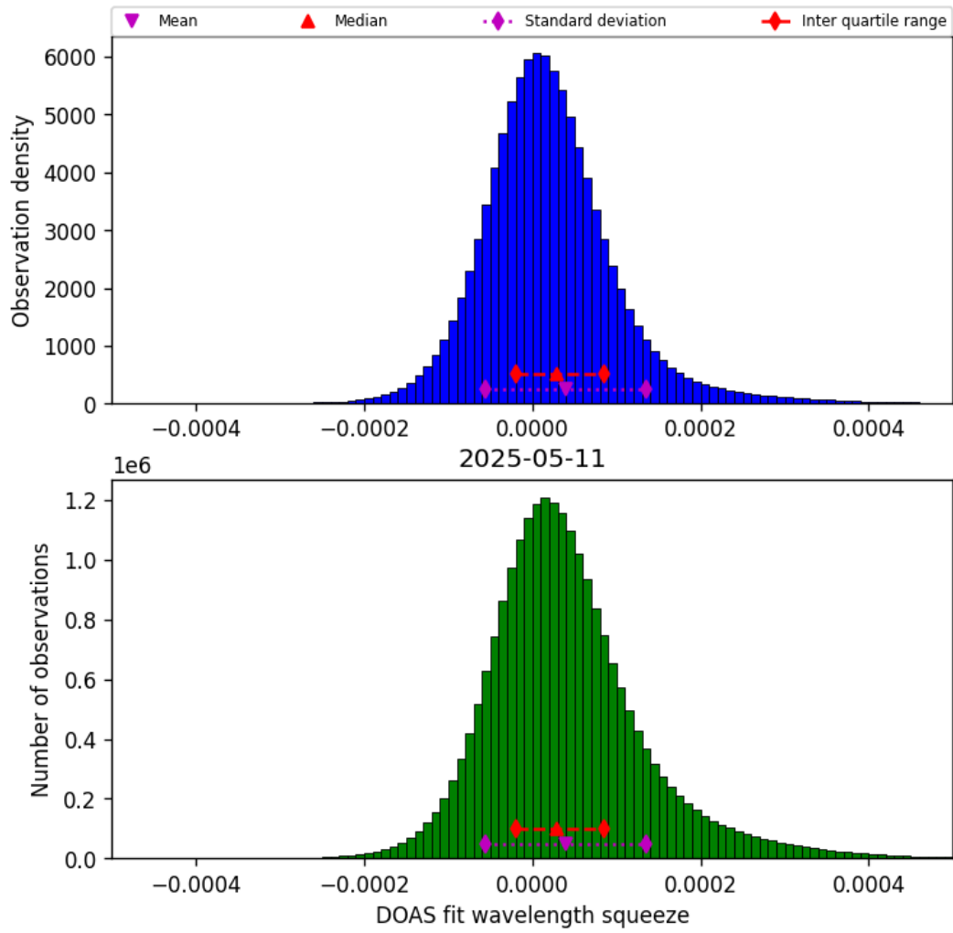
Figure 43: Histogram of “DOAS fit wavelength squeeze” for 2025-05-11 to 2025-05-12
