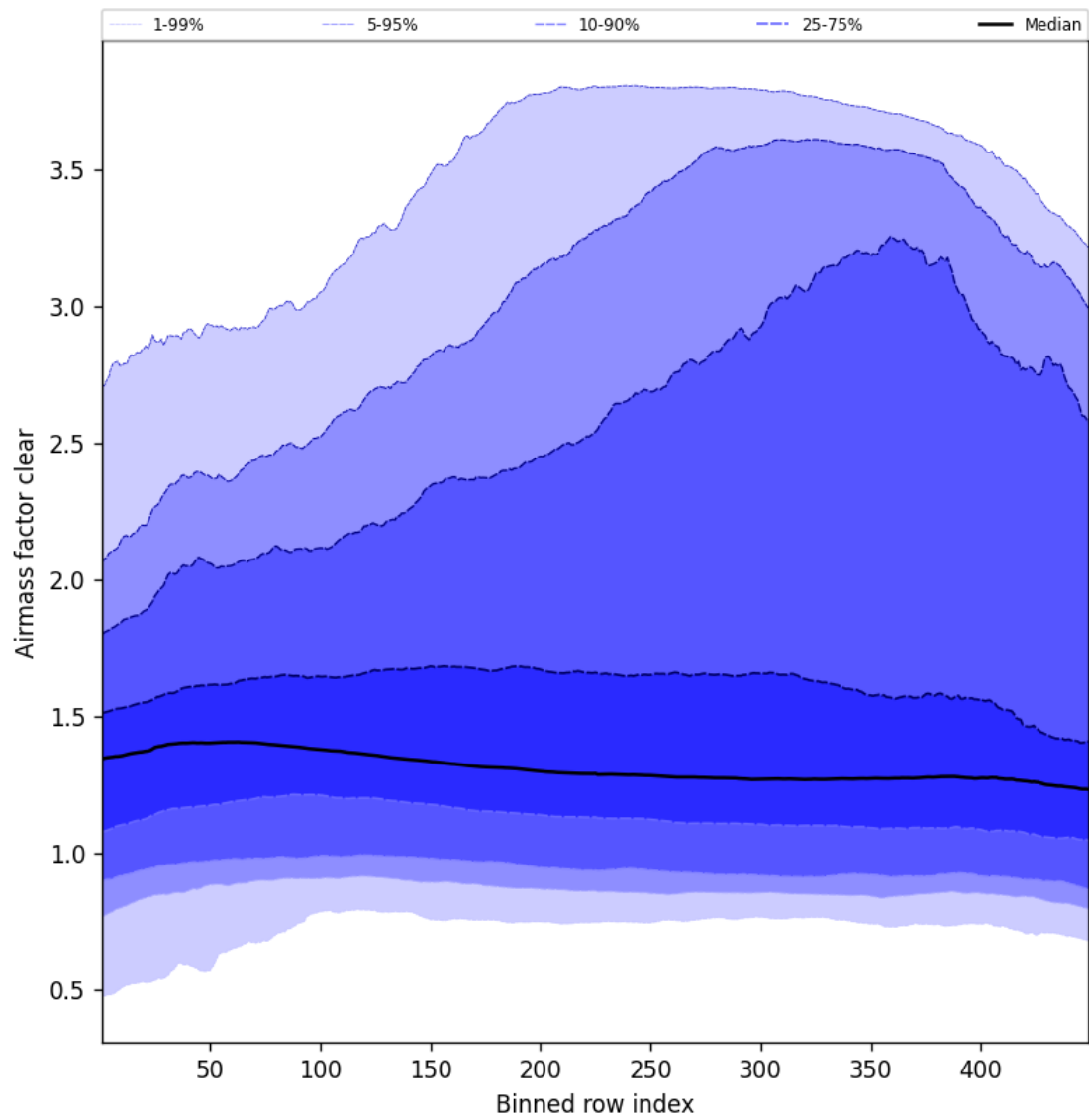
Figure 54: Along track statistics of “Airmass factor clear” for 2025-05-11 to 2025-05-12
