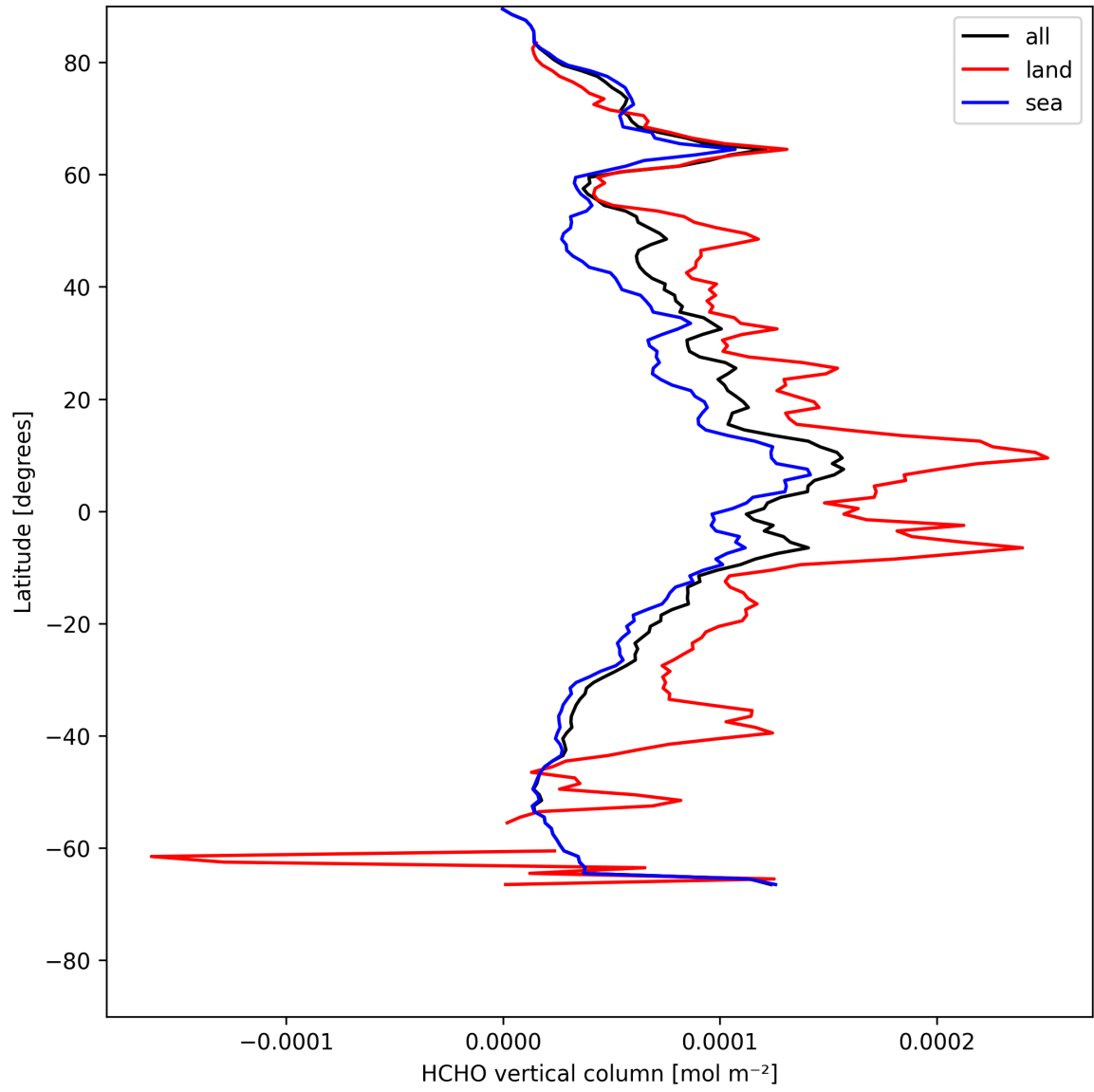
Figure 19: Zonal average of “HCHO vertical column” for 2025-05-11 to 2025-05-12.
