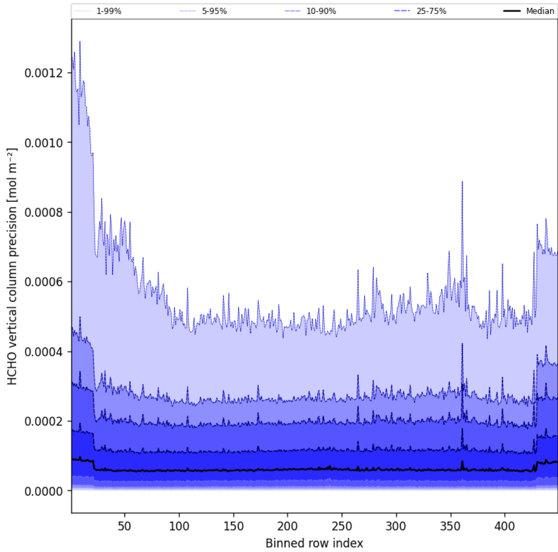
Figure 48: Along track statistics of “HCHO vertical column precision” for 2025-05-11 to 2025-05-12
