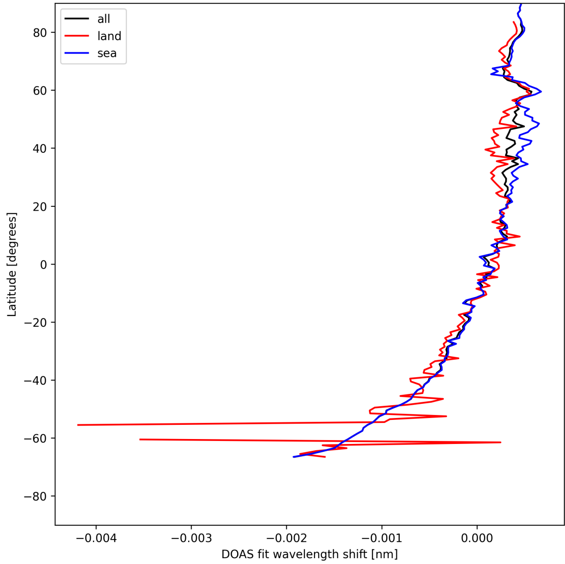
Figure 28: Zonal average of “DOAS fit wavelength shift” for 2025-05-11 to 2025-05-12.
