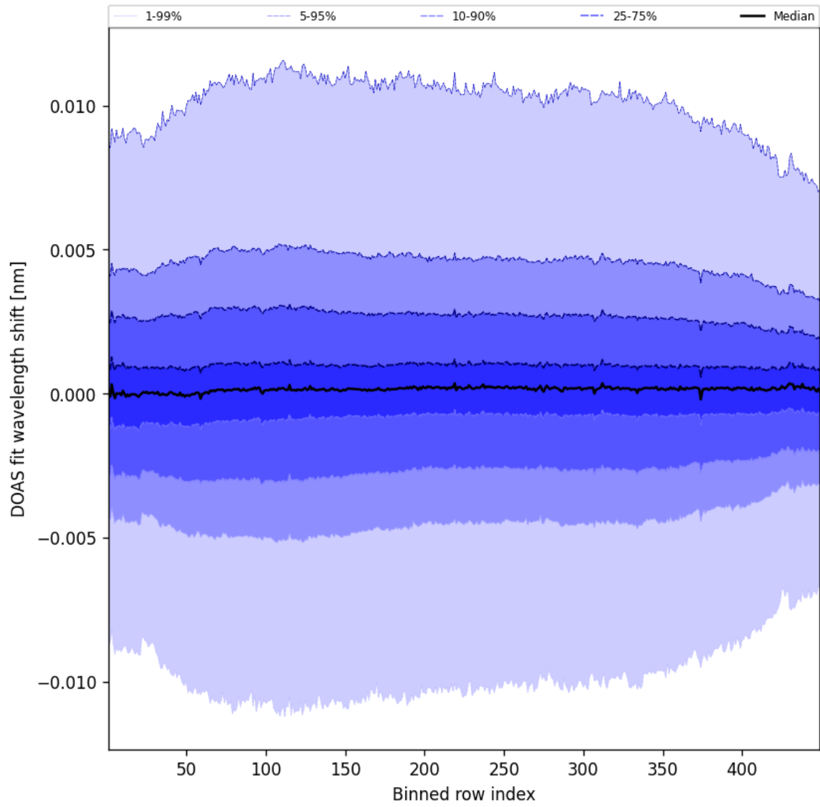
Figure 56: Along track statistics of “DOAS fit wavelength shift” for 2025-05-11 to 2025-05-12
