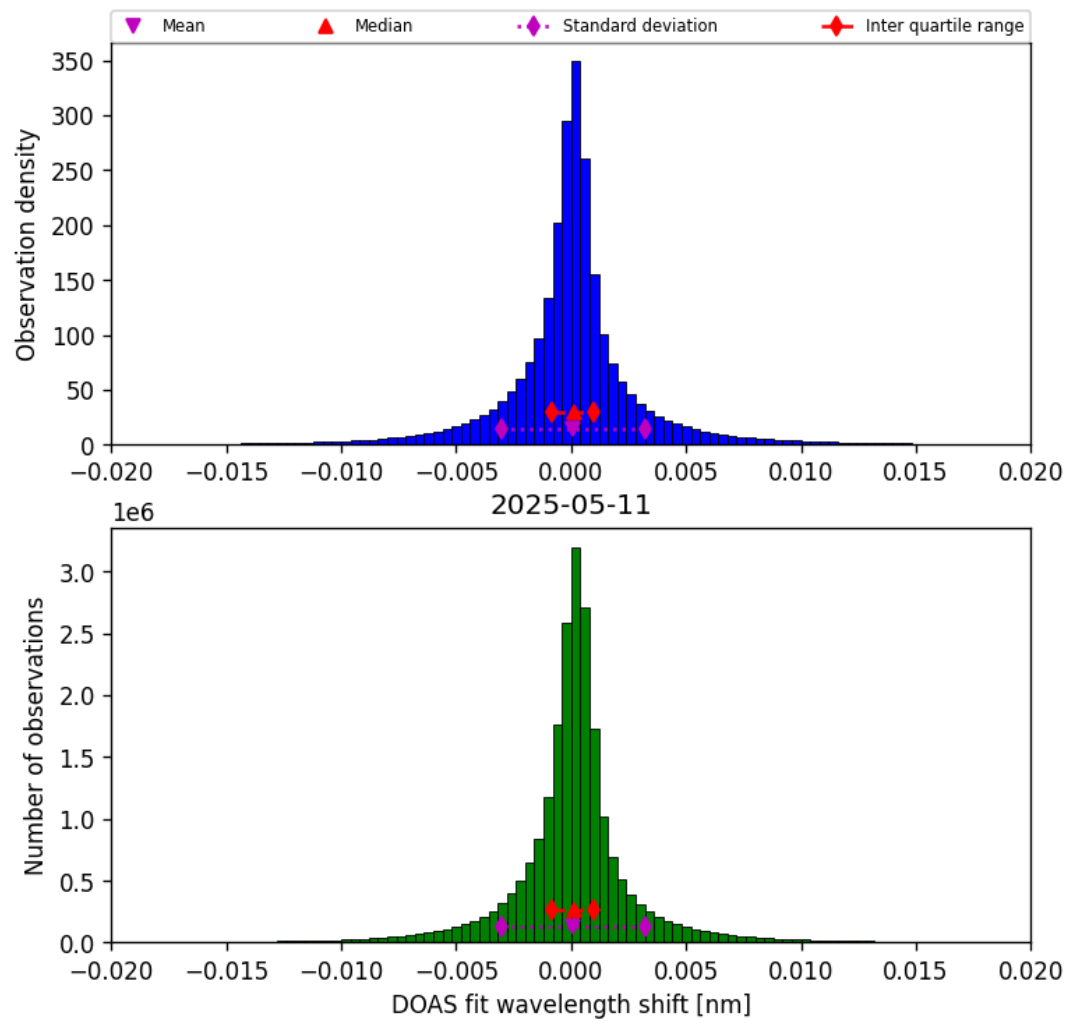
Figure 42: Histogram of “DOAS fit wavelength shift” for 2025-05-11 to 2025-05-12
