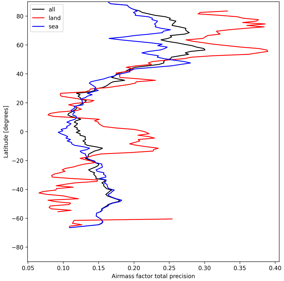
Figure 25: Zonal average of “Airmass factor total precision” for 2025-05-11 to 2025-05-12.
