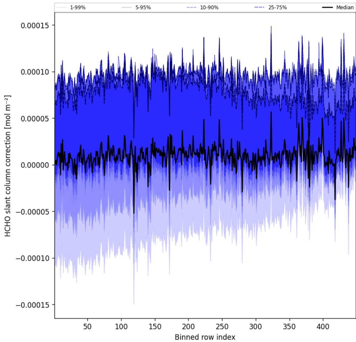
Figure 59: Along track statistics of “HCHO slant column correction” for 2025-05-11 to 2025-05-12
