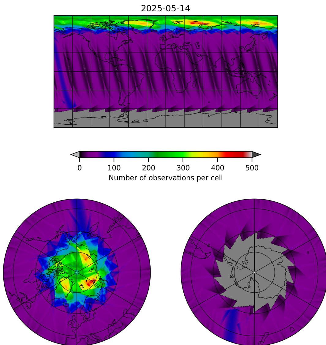
Figure 17: Map of the number of observations for 2025-05-14 to 2025-05-15
