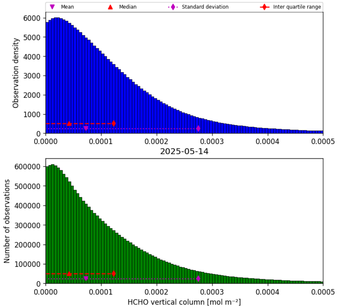
Figure 33: Histogram of “HCHO vertical column” for 2025-05-14 to 2025-05-15
