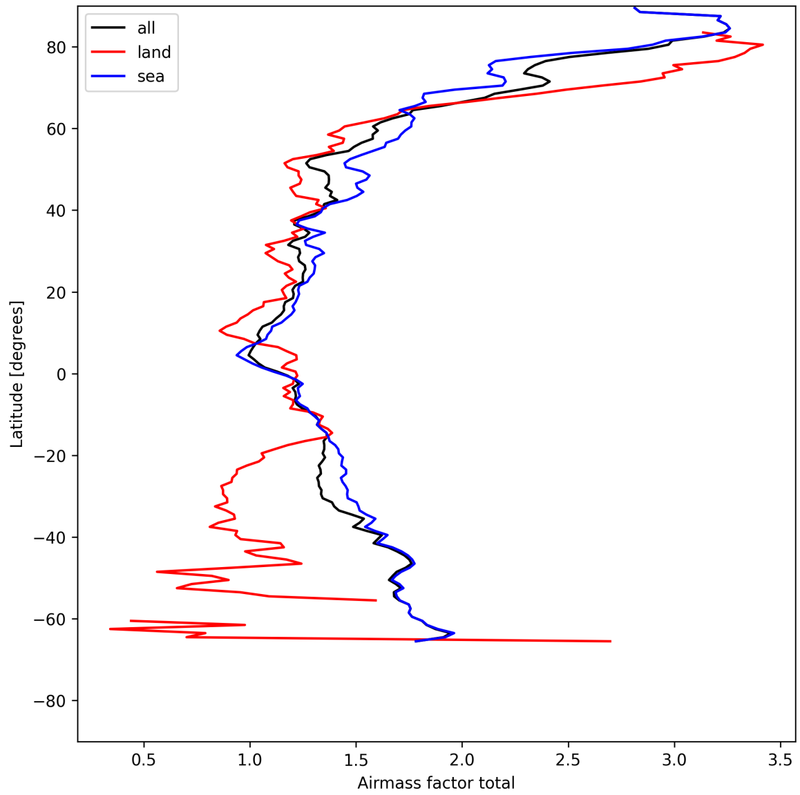
Figure 24: Zonal average of “Airmass factor total” for 2025-05-14 to 2025-05-15.
