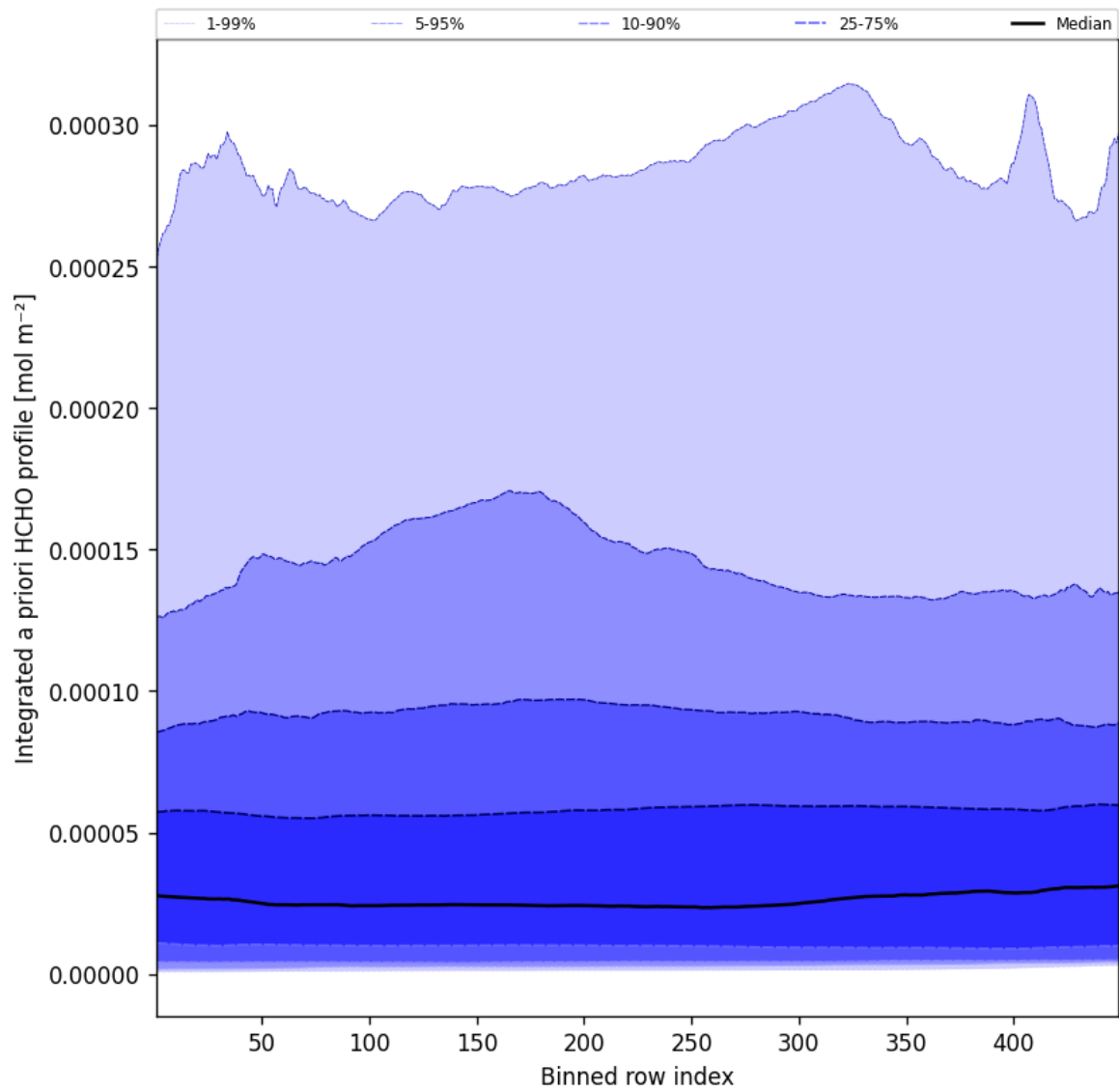
Figure 55: Along track statistics of “Integrated a priori HCHO profile” for 2025-05-14 to 2025-05-15
