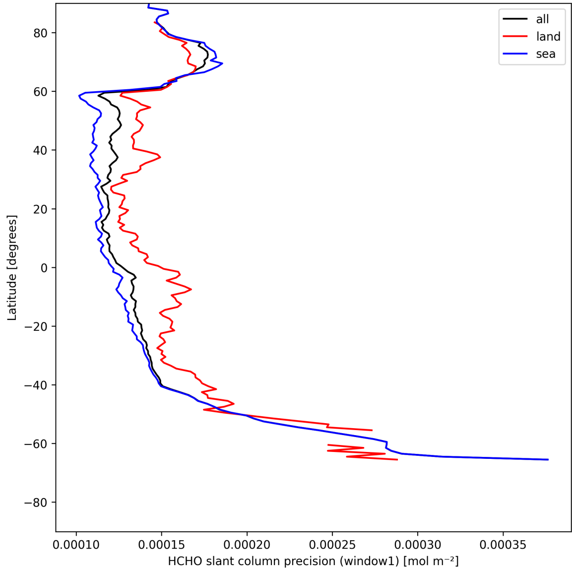
Figure 23: Zonal average of “HCHO slant column precision (window1)” for 2025-05-14 to 2025-05-15.
