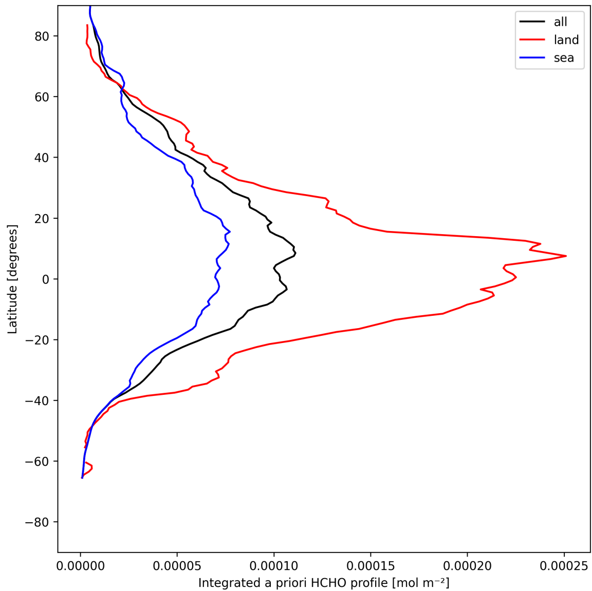
Figure 27: Zonal average of “Integrated a priori HCHO profile” for 2025-05-14 to 2025-05-15.
