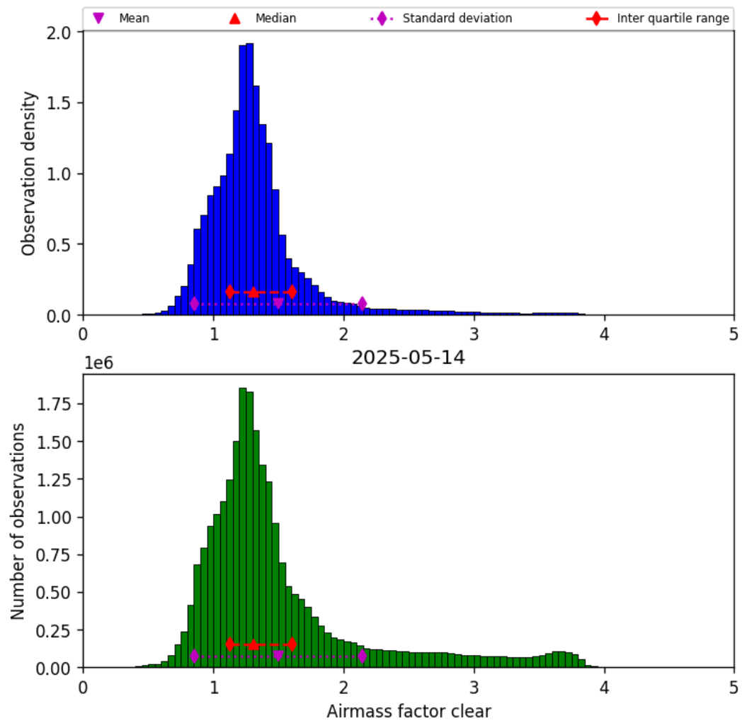
Figure 40: Histogram of “Airmass factor clear” for 2025-05-14 to 2025-05-15
