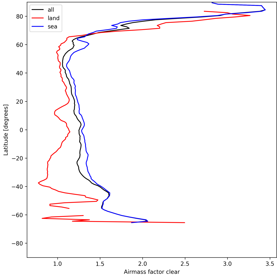
Figure 26: Zonal average of “Airmass factor clear” for 2025-05-14 to 2025-05-15.
