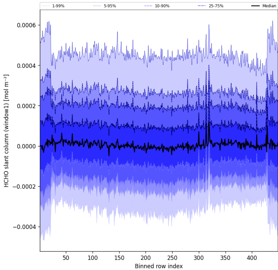
Figure 50: Along track statistics of “HCHO slant column (window1)” for 2025-05-14 to 2025-05-15
