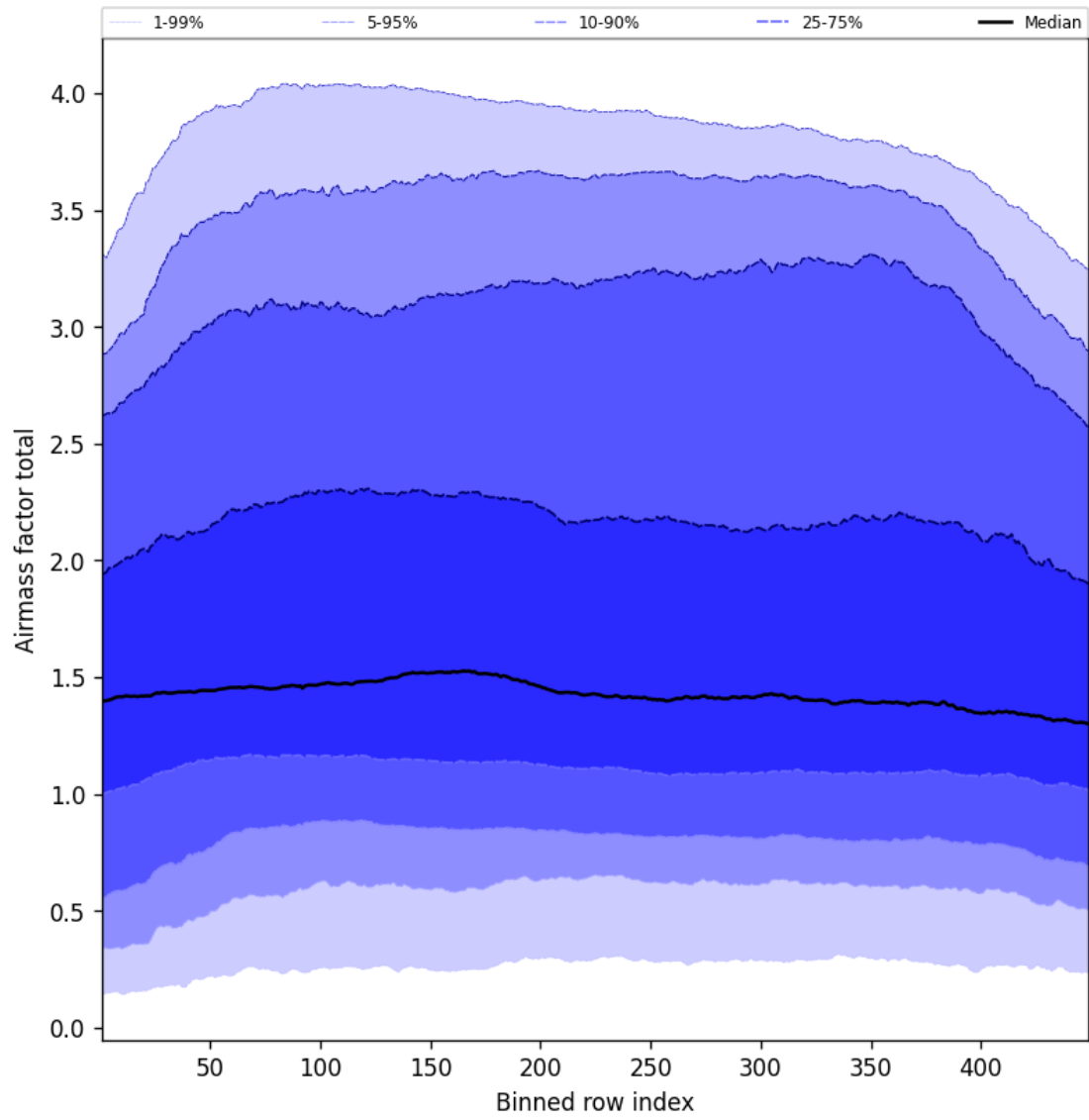
Figure 52: Along track statistics of “Airmass factor total” for 2025-05-14 to 2025-05-15
