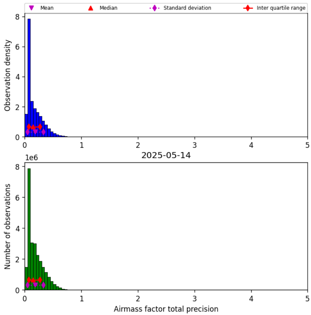
Figure 39: Histogram of “Airmass factor total precision” for 2025-05-14 to 2025-05-15
