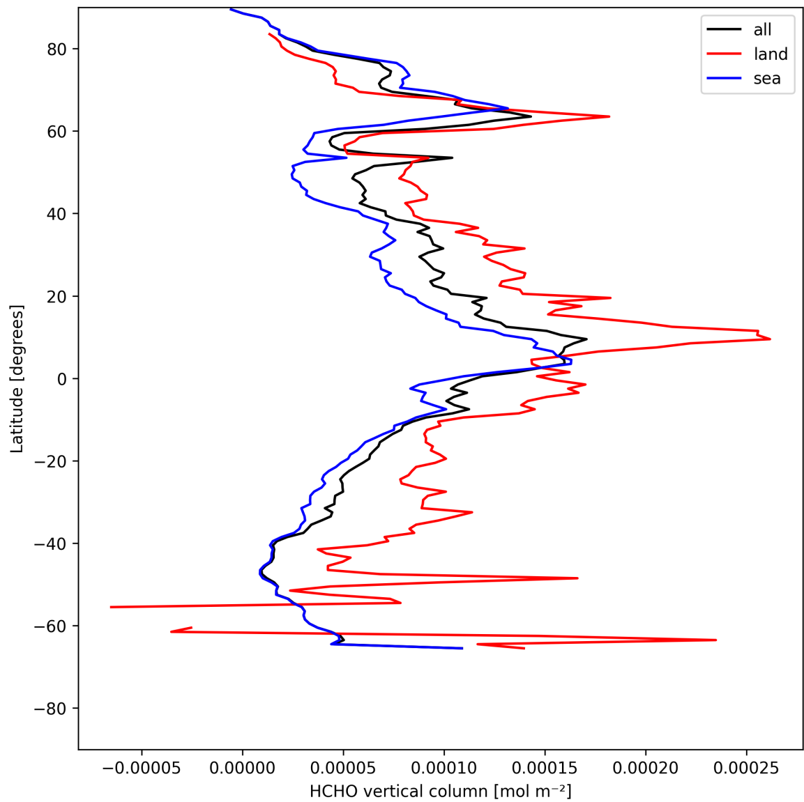
Figure 19: Zonal average of “HCHO vertical column” for 2025-05-14 to 2025-05-15.
