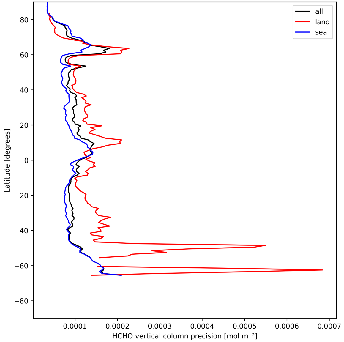
Figure 20: Zonal average of “HCHO vertical column precision” for 2025-05-14 to 2025-05-15.
