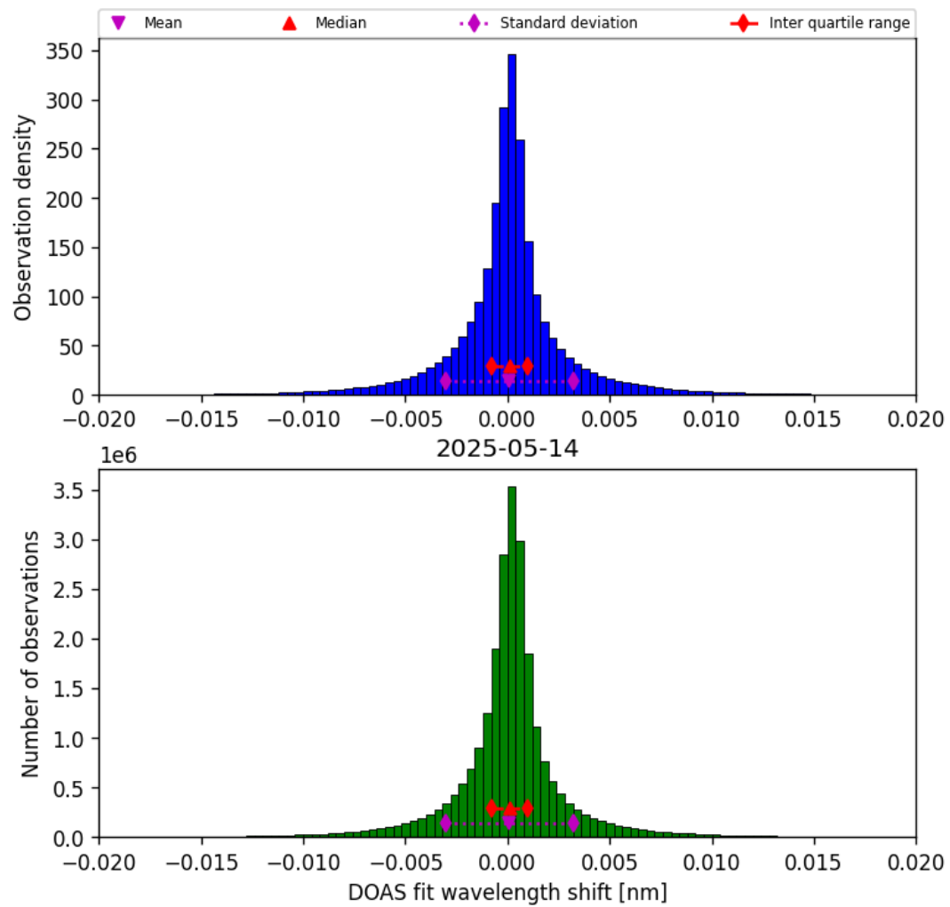
Figure 42: Histogram of “DOAS fit wavelength shift” for 2025-05-14 to 2025-05-15
