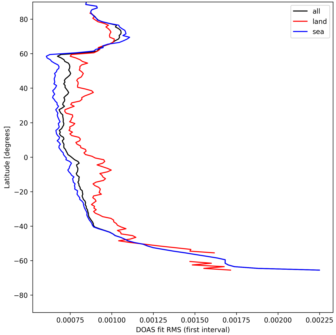
Figure 30: Zonal average of "DOAS fit RMS (first interval)" for 2025-05-14 to 2025-05-15.
