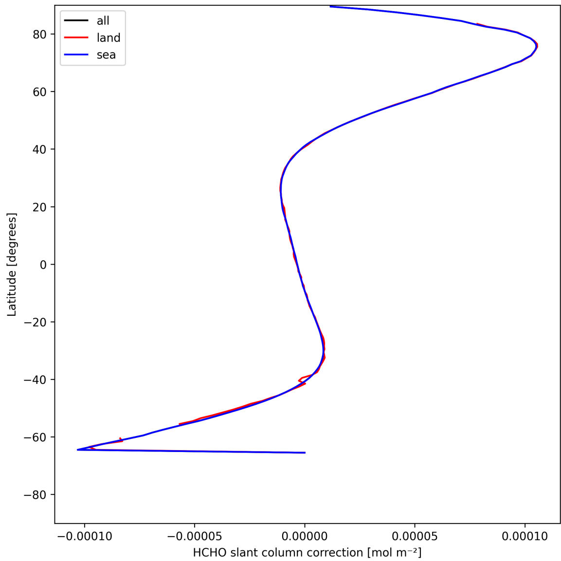
Figure 31: Zonal average of “HCHO slant column correction” for 2025-05-14 to 2025-05-15.
