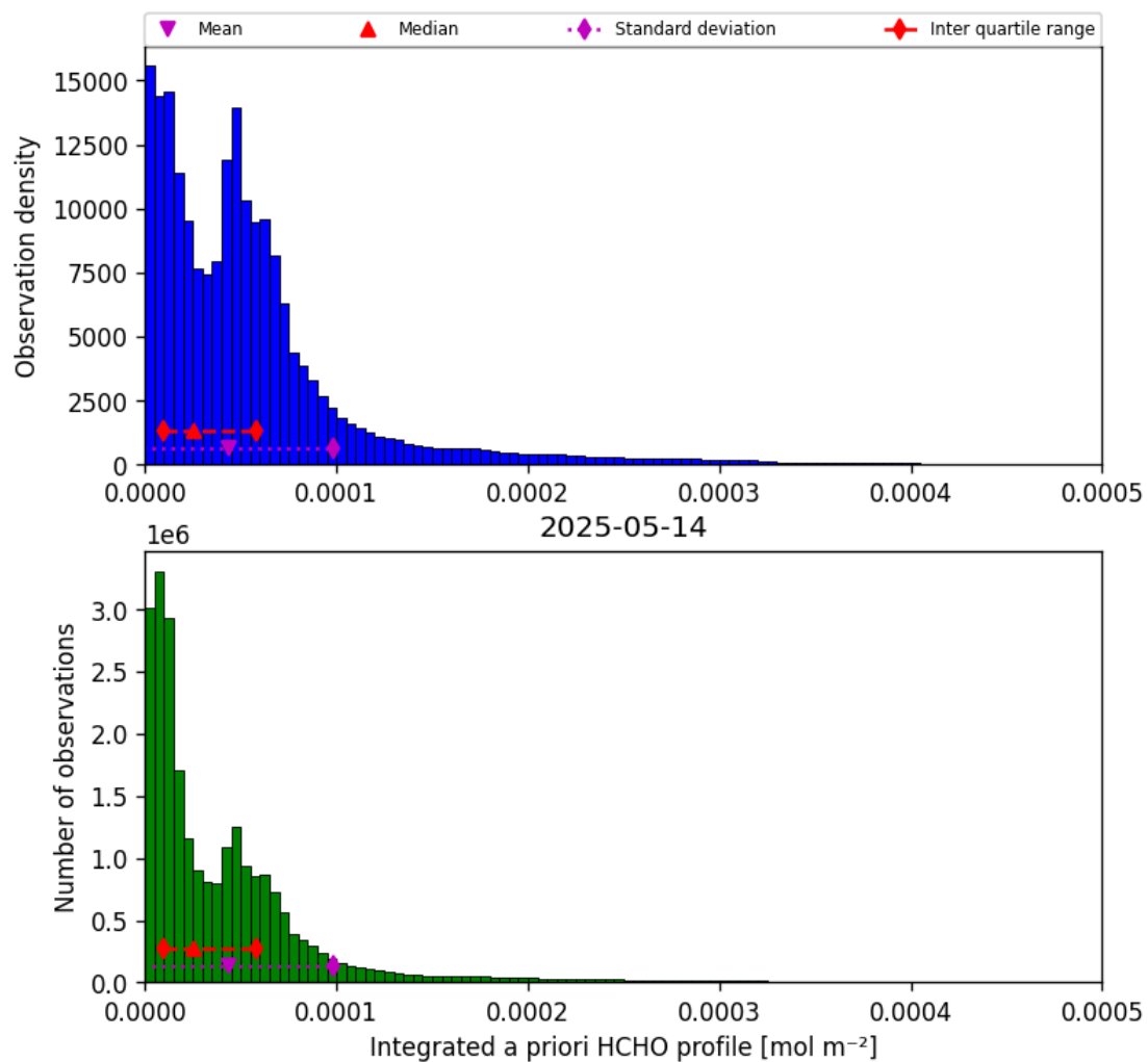
Figure 41: Histogram of “Integrated a priori HCHO profile” for 2025-05-14 to 2025-05-15
