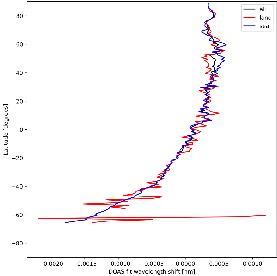
Figure 28: Zonal average of “DOAS fit wavelength shift” for 2025-05-14 to 2025-05-15.
