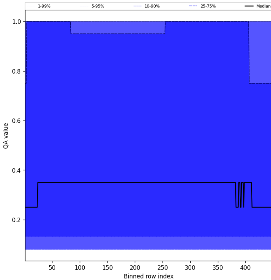
Figure 46: Along track statistics of “QA value” for 2025-05-14 to 2025-05-15
