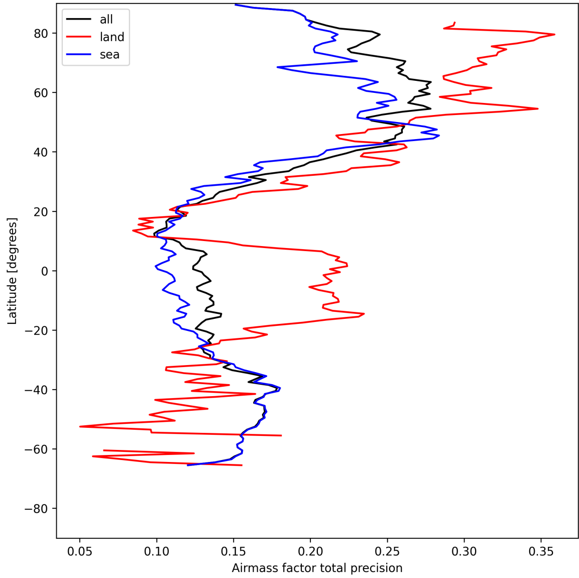
Figure 25: Zonal average of “Airmass factor total precision” for 2025-05-14 to 2025-05-15.
