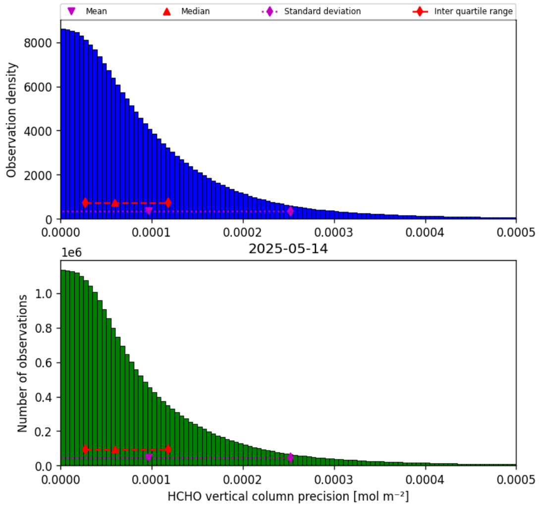
Figure 34: Histogram of “HCHO vertical column precision” for 2025-05-14 to 2025-05-15
