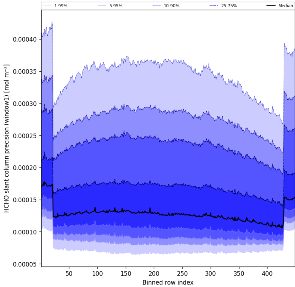
Figure 51: Along track statistics of “HCHO slant column precision (window1)” for 2025-05-14 to 2025-05-15
