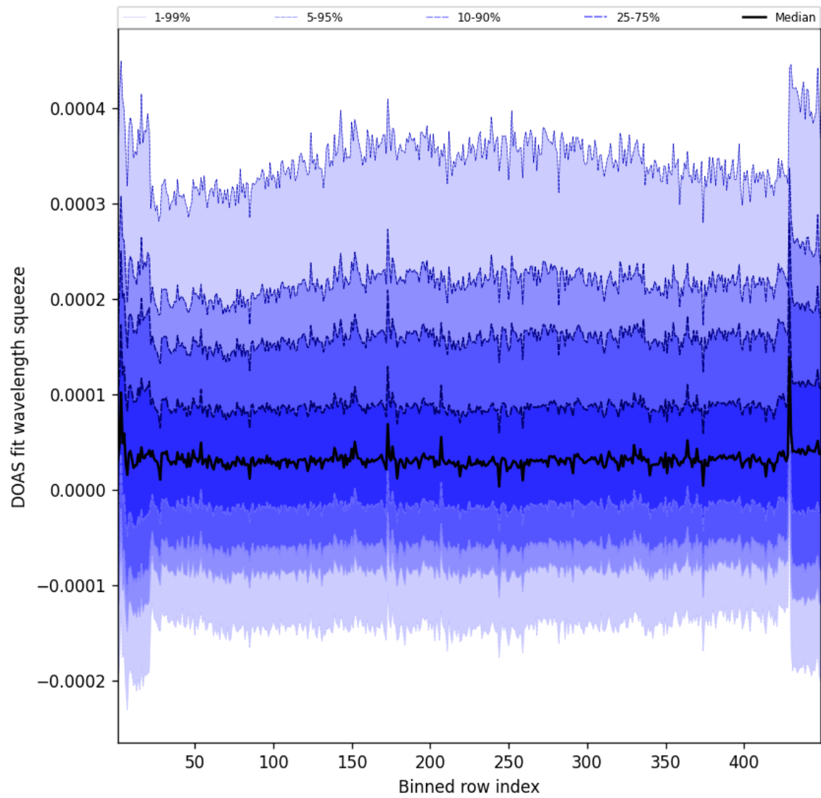
Figure 57: Along track statistics of “DOAS fit wavelength squeeze” for 2025-05-14 to 2025-05-15
