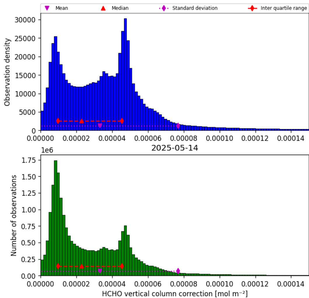
Figure 35: Histogram of “HCHO vertical column correction” for 2025-05-14 to 2025-05-15
