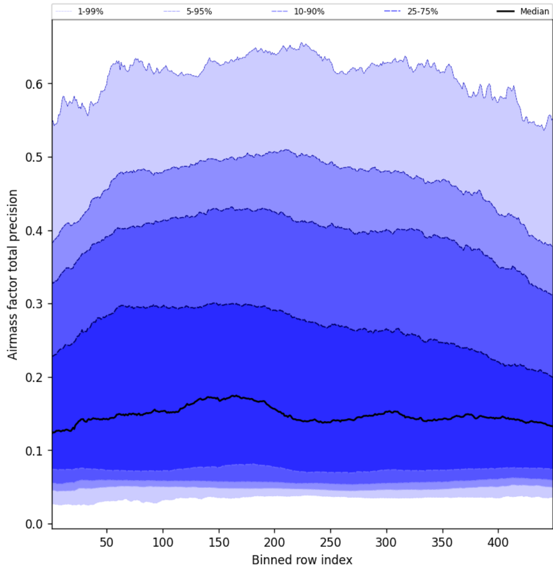
Figure 53: Along track statistics of “Airmass factor total precision” for 2025-05-14 to 2025-05-15
