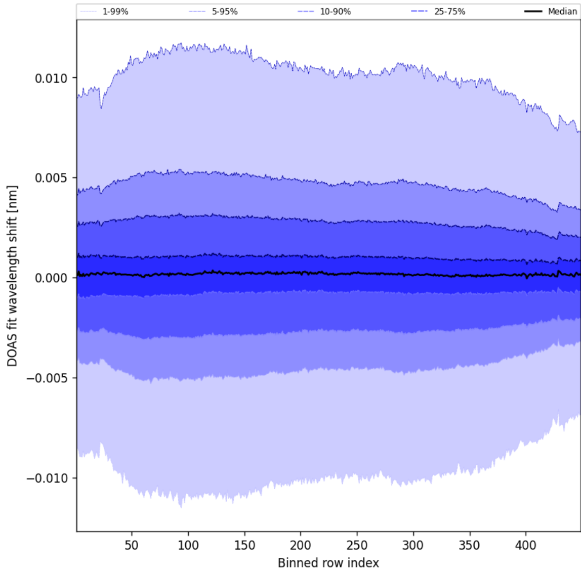
Figure 56: Along track statistics of “DOAS fit wavelength shift” for 2025-05-14 to 2025-05-15
