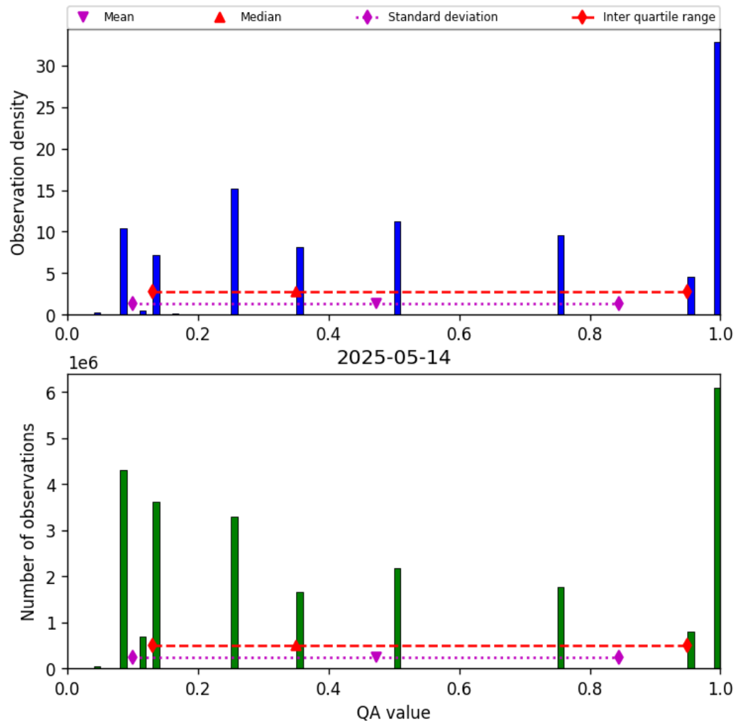
Figure 32: Histogram of “QA value” for 2025-05-14 to 2025-05-15
