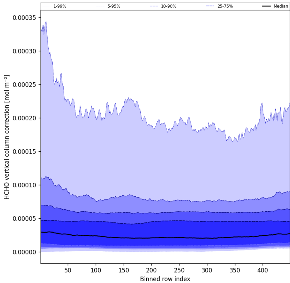
Figure 49: Along track statistics of “HCHO vertical column correction” for 2025-05-14 to 2025-05-15
