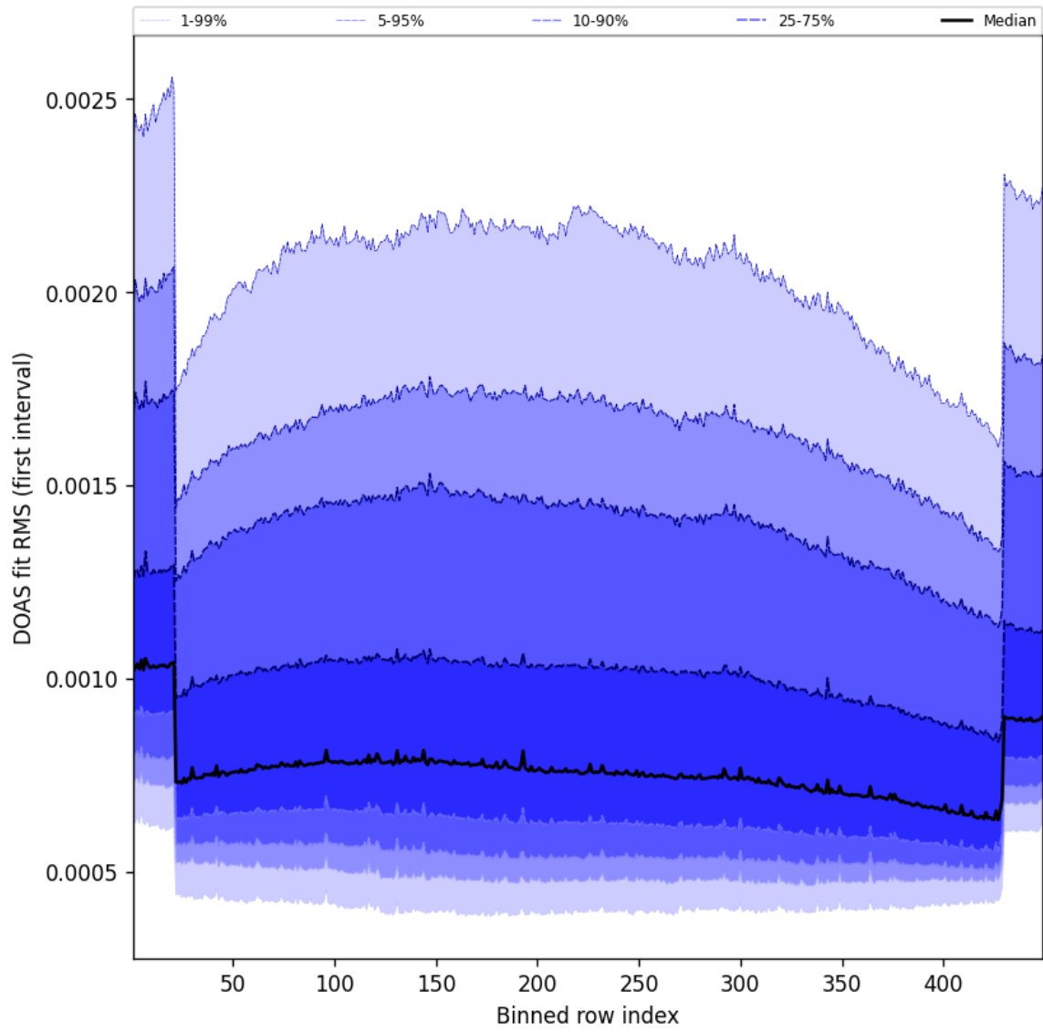
Figure 58: Along track statistics of “DOAS fit RMS (first interval)” for 2025-05-14 to 2025-05-15
