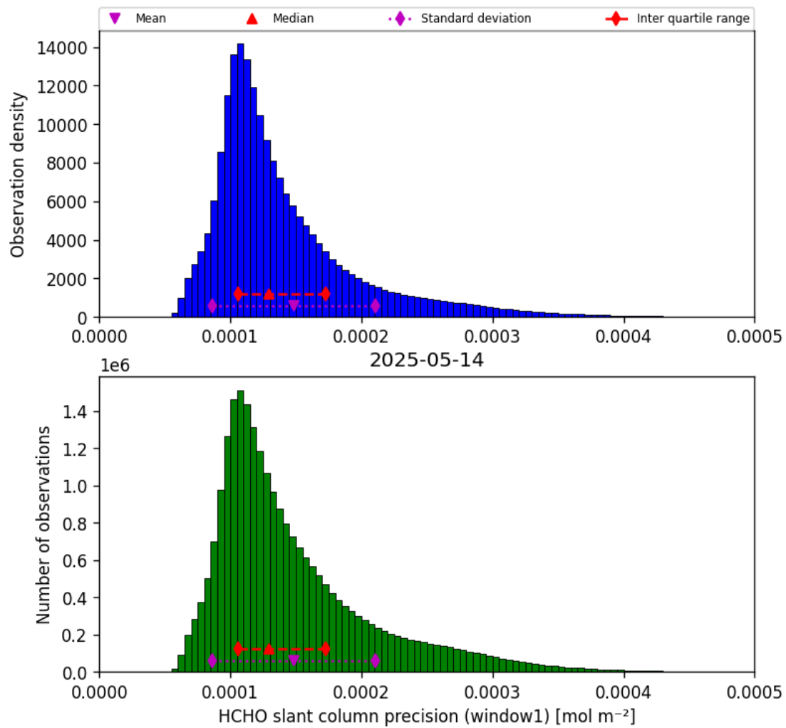
Figure 37: Histogram of “HCHO slant column precision (window1)” for 2025-05-14 to 2025-05-15
