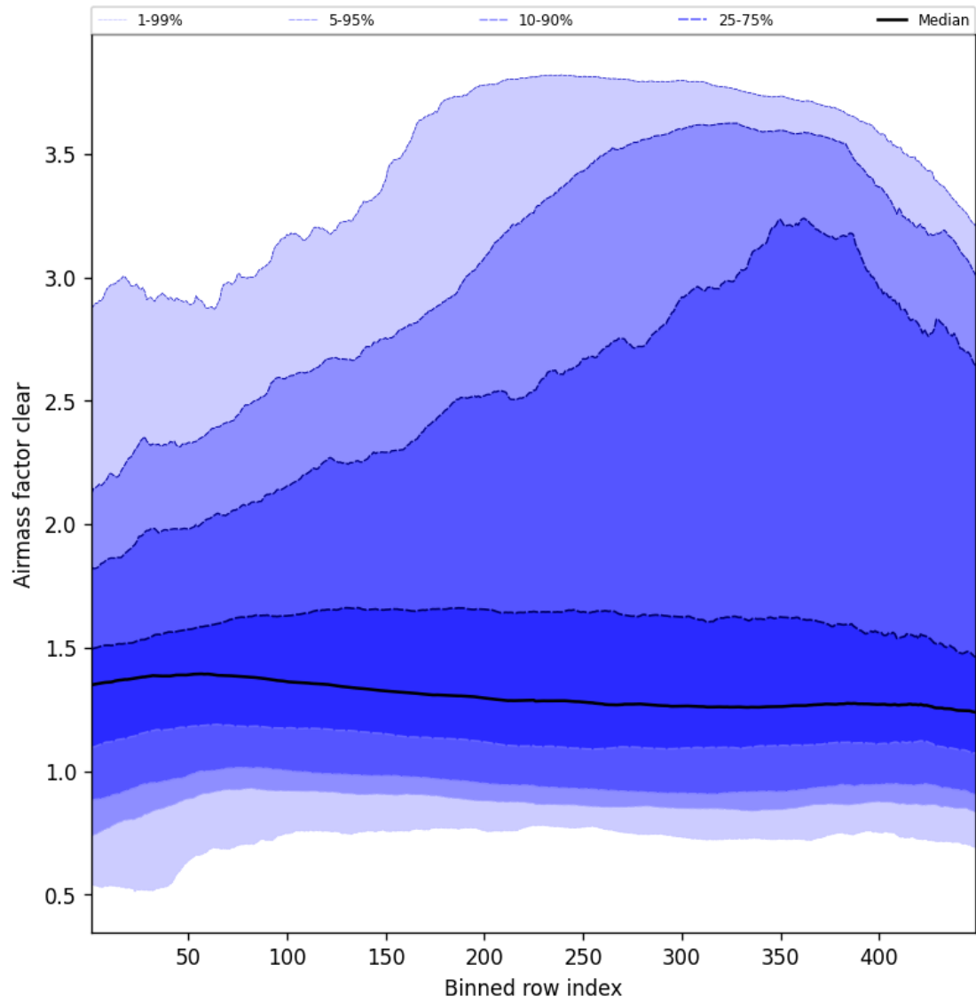
Figure 54: Along track statistics of “Airmass factor clear” for 2025-05-14 to 2025-05-15
