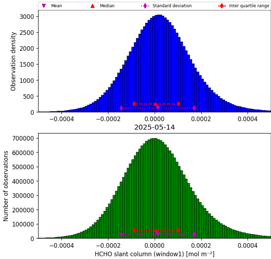
Figure 36: Histogram of “HCHO slant column (window1)” for 2025-05-14 to 2025-05-15
