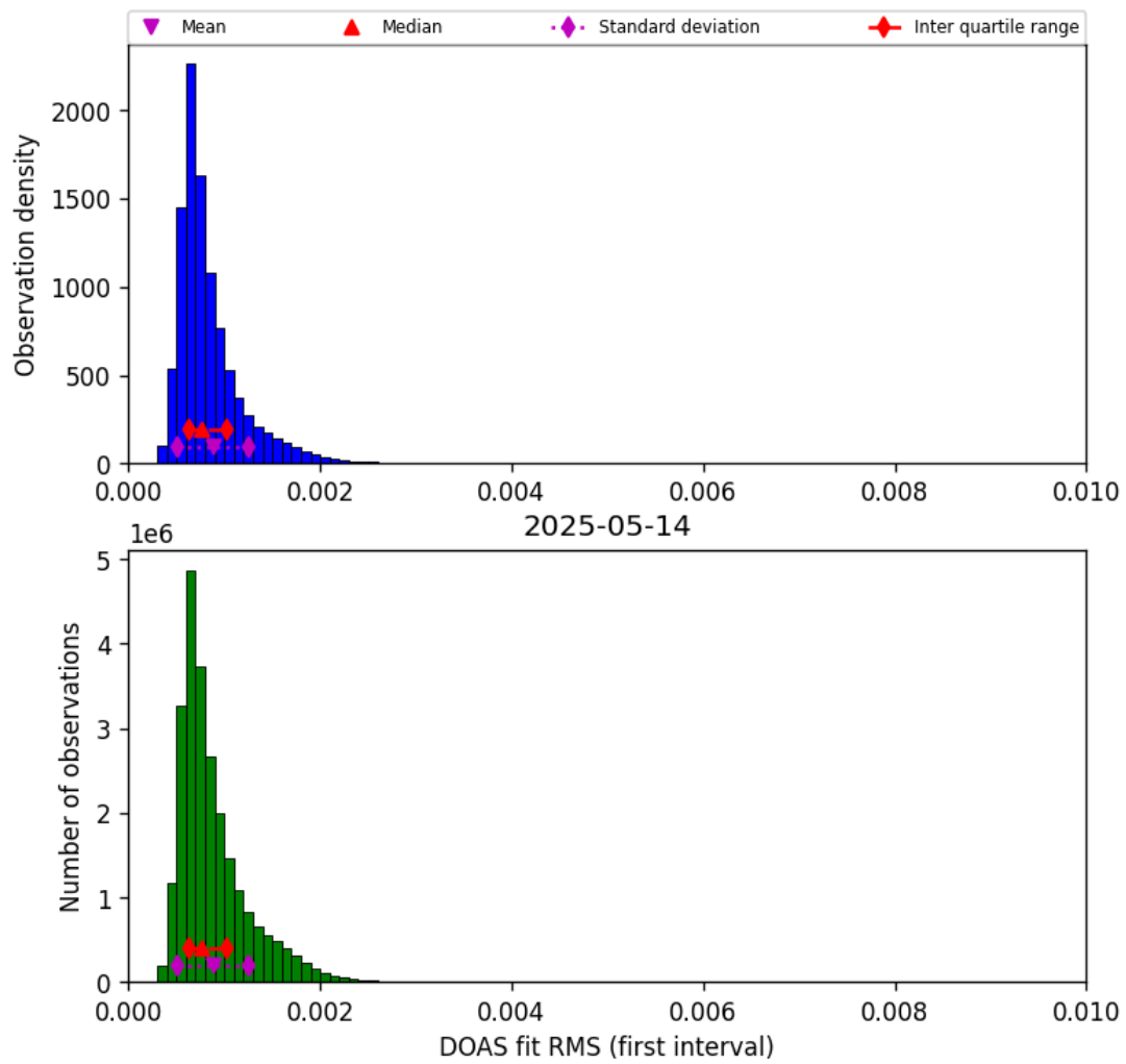
Figure 44: Histogram of “DOAS fit RMS (first interval)” for 2025-05-14 to 2025-05-15
