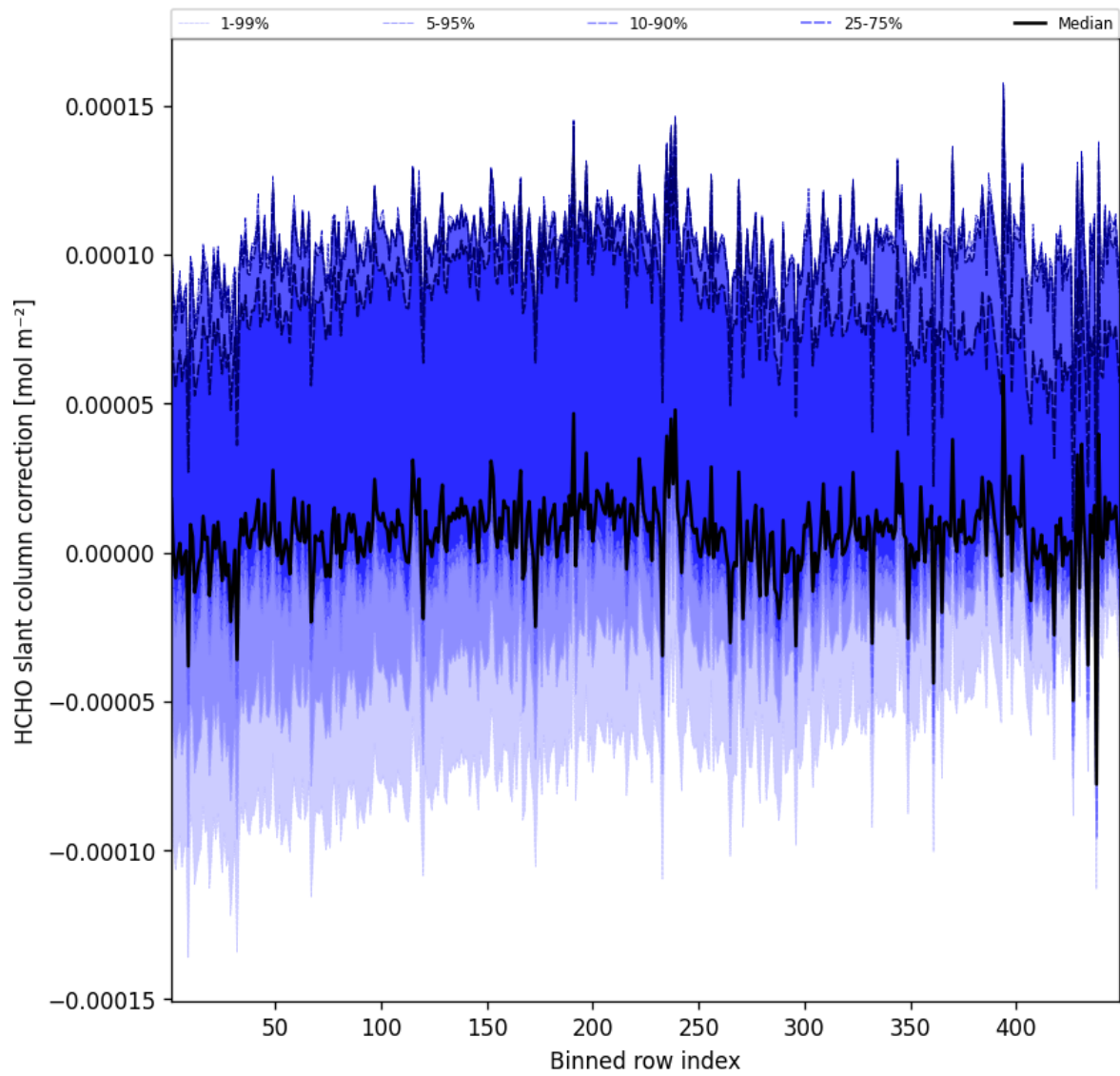
Figure 59: Along track statistics of “HCHO slant column correction” for 2025-05-14 to 2025-05-15
