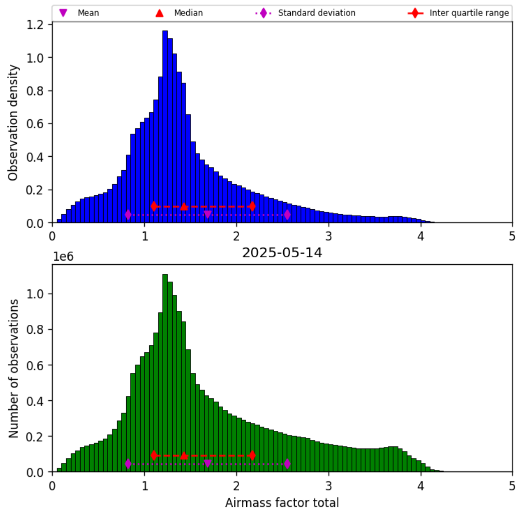
Figure 38: Histogram of “Airmass factor total” for 2025-05-14 to 2025-05-15
