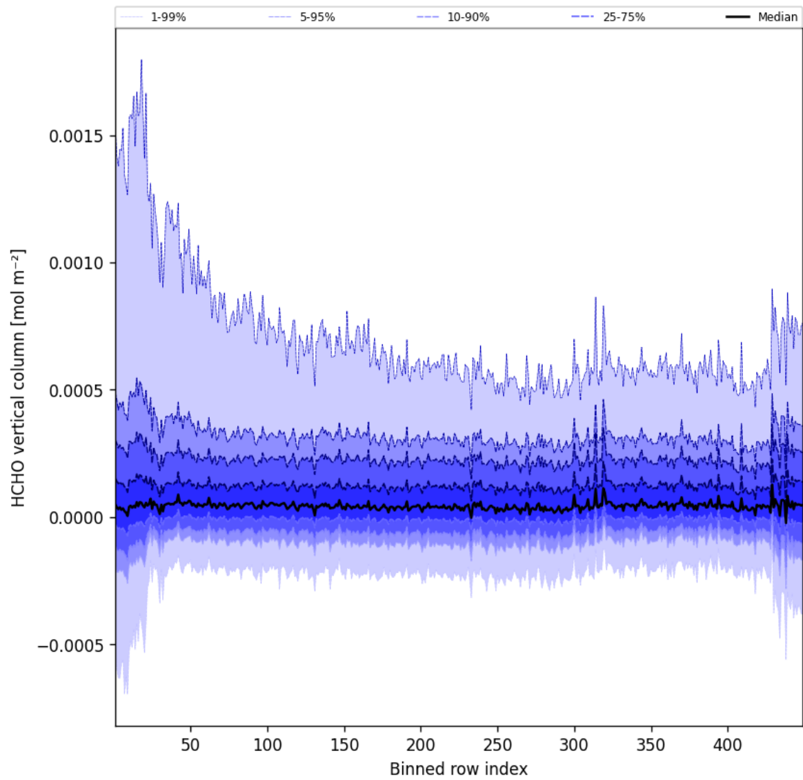
Figure 47: Along track statistics of “HCHO vertical column” for 2025-05-14 to 2025-05-15
