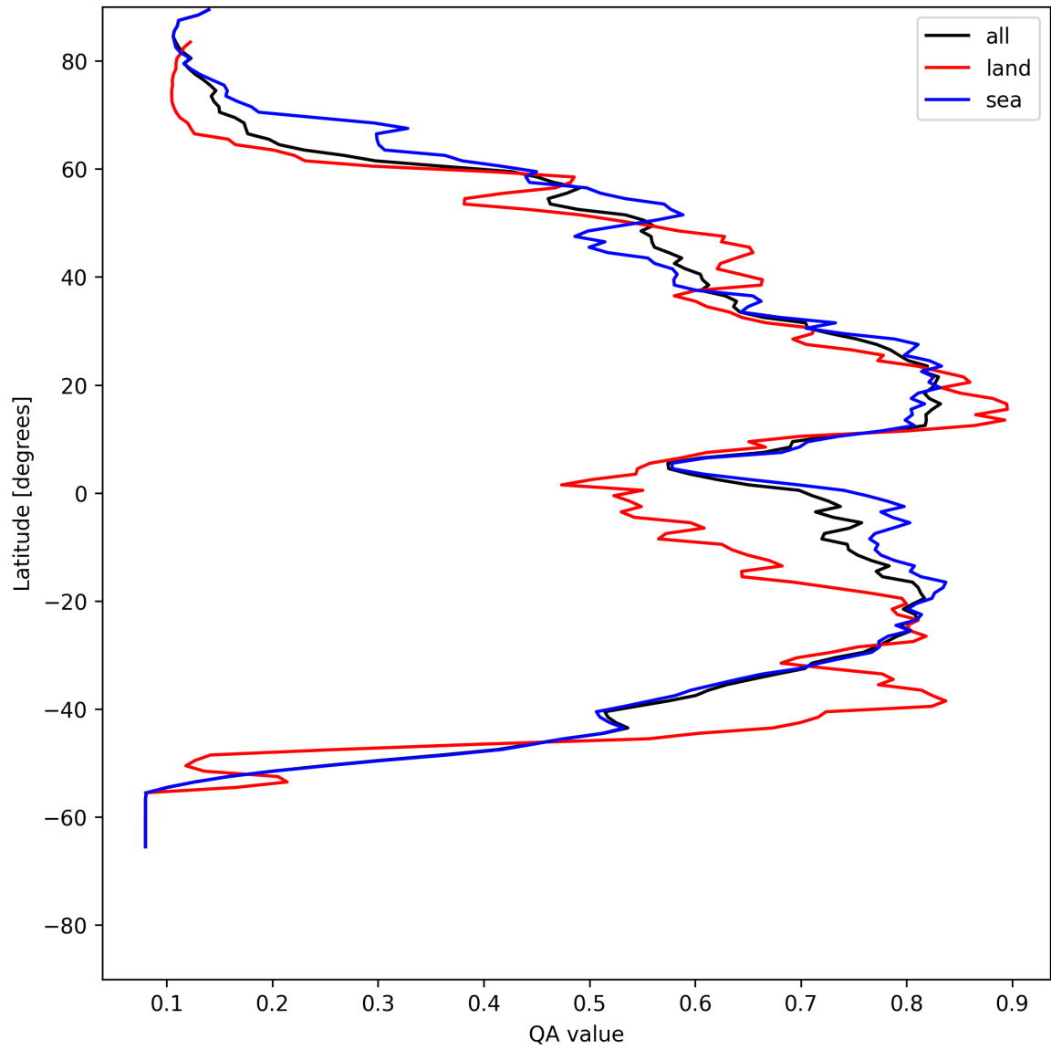
Figure 18: Zonal average of “QA value” for 2025-05-14 to 2025-05-15.
