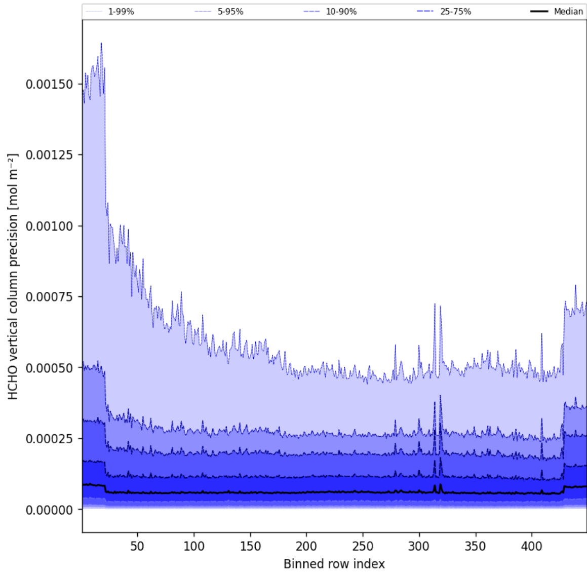
Figure 48: Along track statistics of “HCHO vertical column precision” for 2025-05-14 to 2025-05-15
