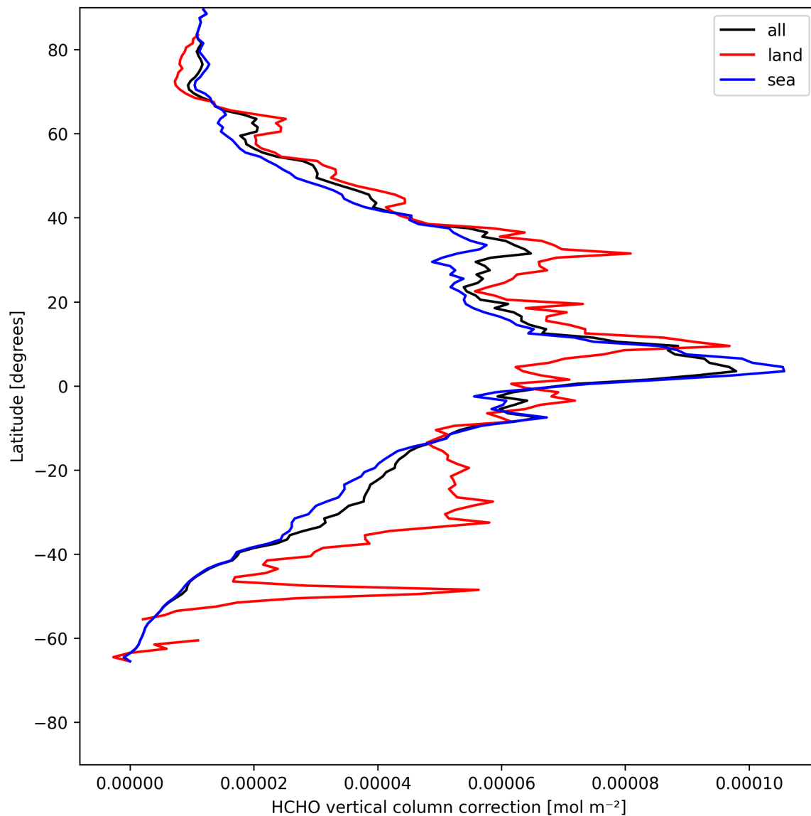
Figure 21: Zonal average of “HCHO vertical column correction” for 2025-05-14 to 2025-05-15.
