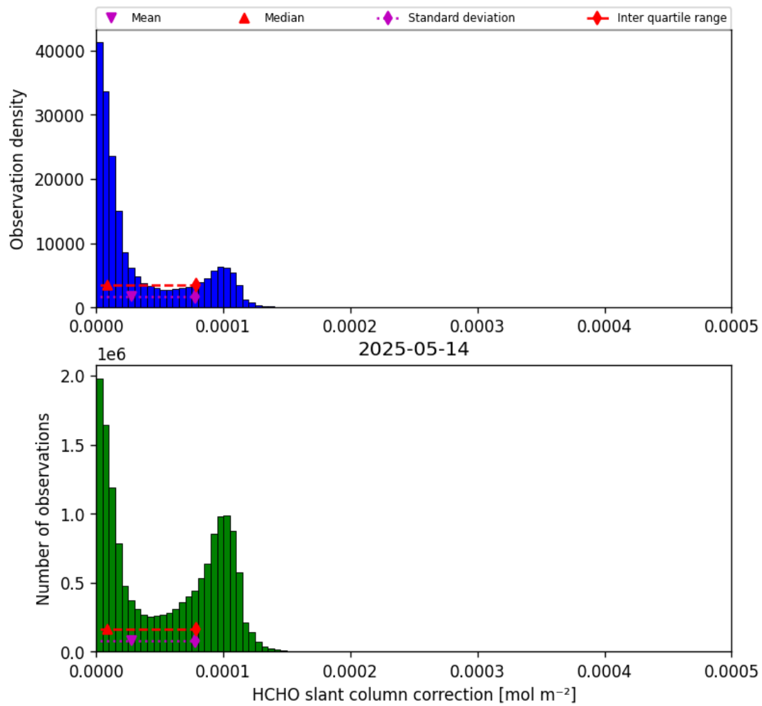
Figure 45: Histogram of “HCHO slant column correction” for 2025-05-14 to 2025-05-15
