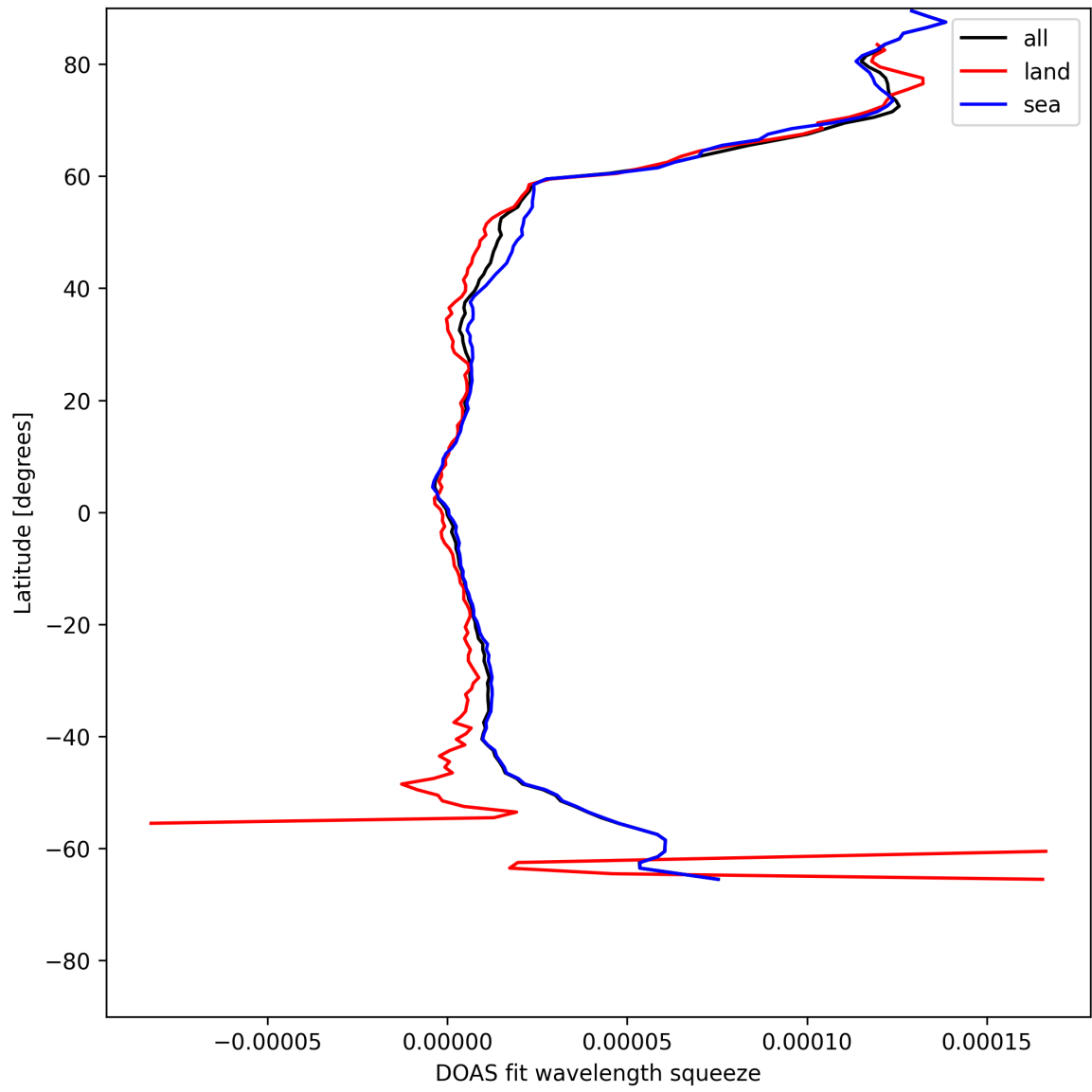
Figure 29: Zonal average of “DOAS fit wavelength squeeze” for 2025-05-14 to 2025-05-15.
