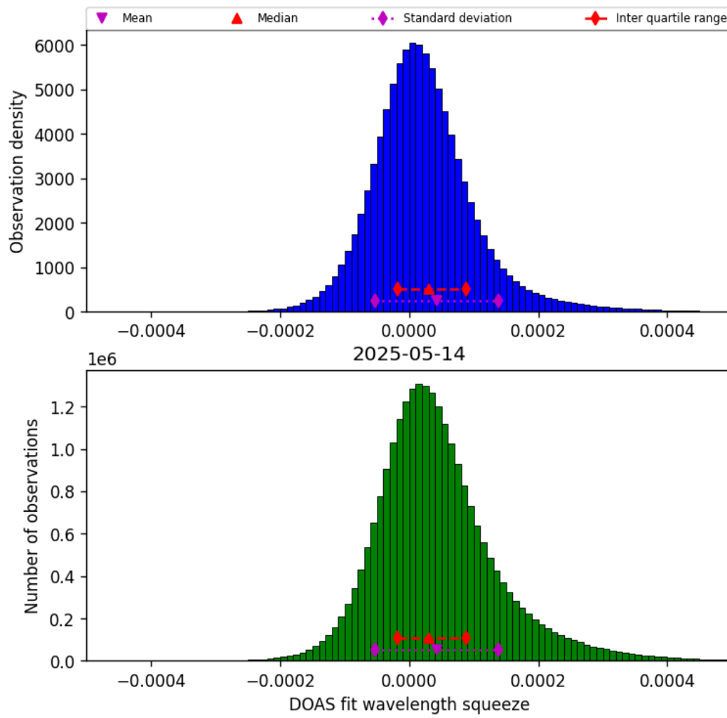
Figure 43: Histogram of “DOAS fit wavelength squeeze” for 2025-05-14 to 2025-05-15
