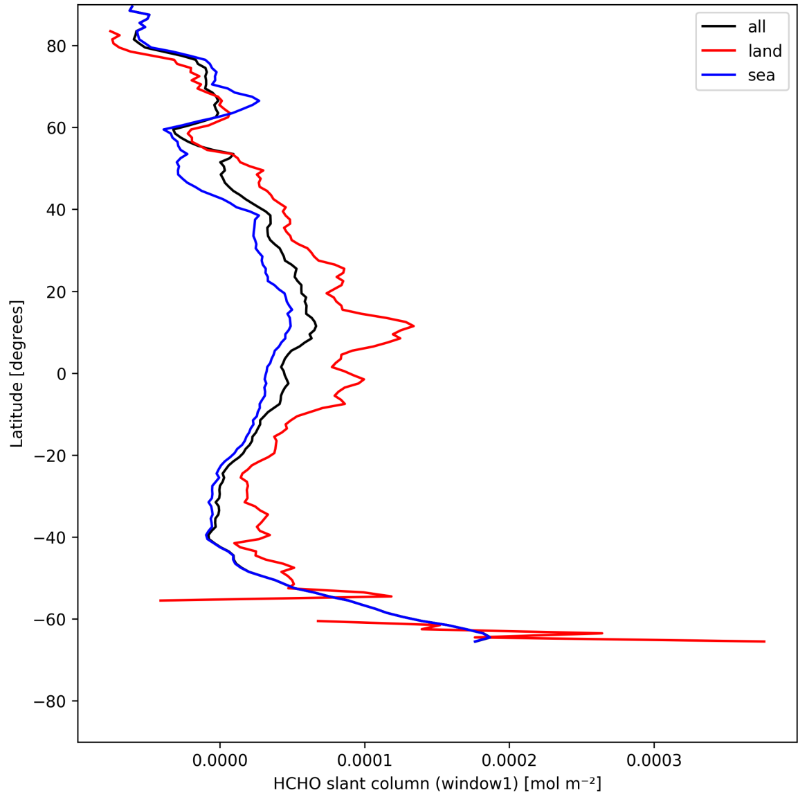
Figure 22: Zonal average of “HCHO slant column (window1)” for 2025-05-14 to 2025-05-15.
