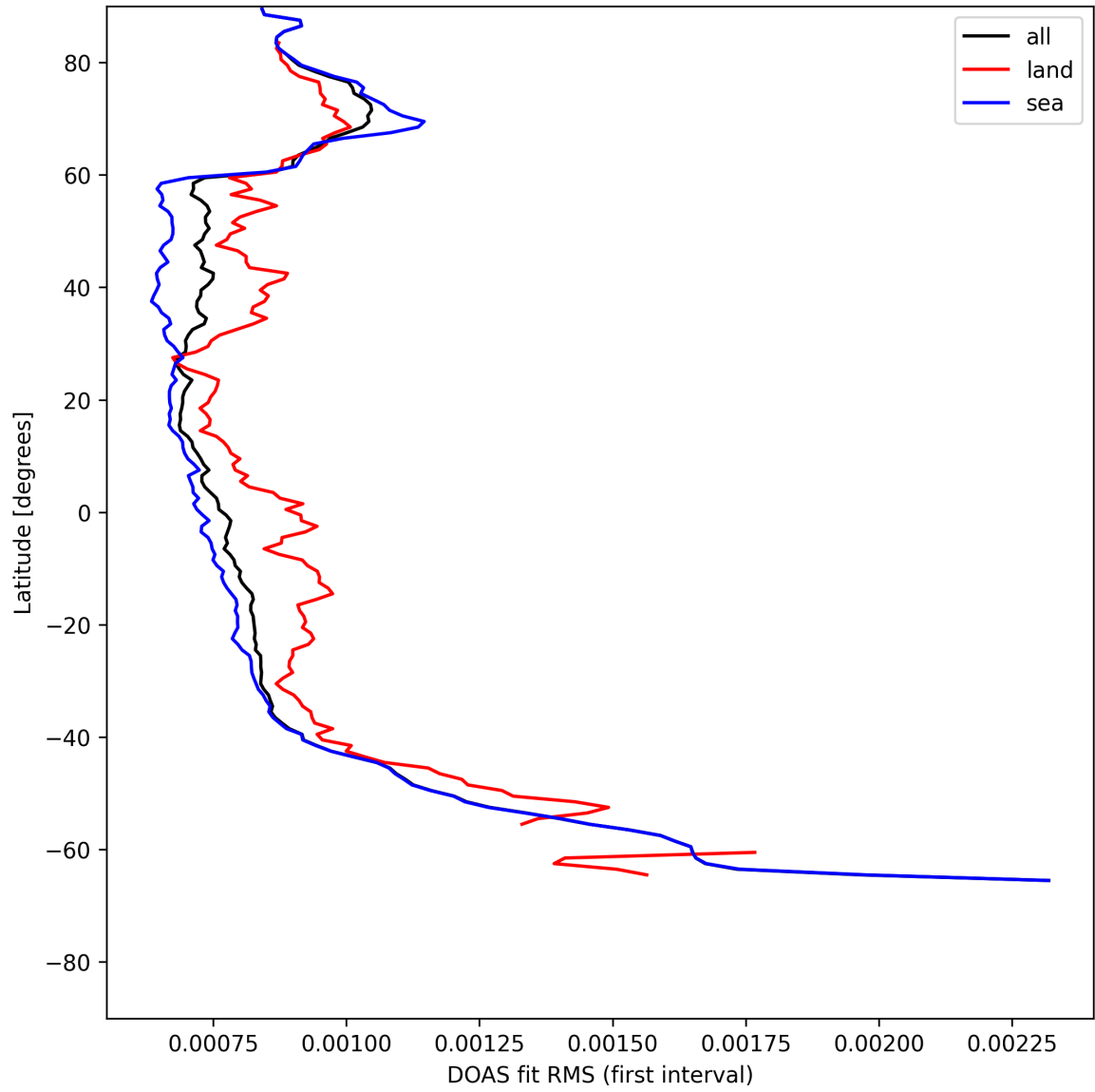
Figure 30: Zonal average of “DOAS fit RMS (first interval)” for 2025-05-15 to 2025-05-16.
