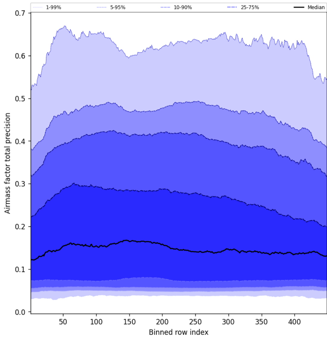
Figure 53: Along track statistics of “Airmass factor total precision” for 2025-05-15 to 2025-05-16
