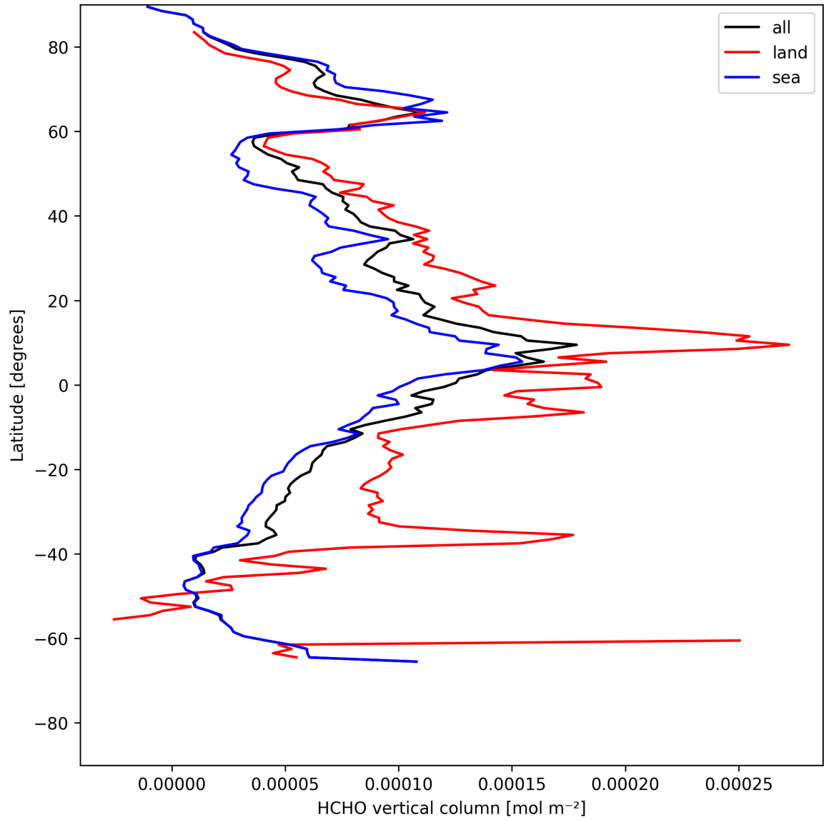
Figure 19: Zonal average of “HCHO vertical column” for 2025-05-15 to 2025-05-16.
