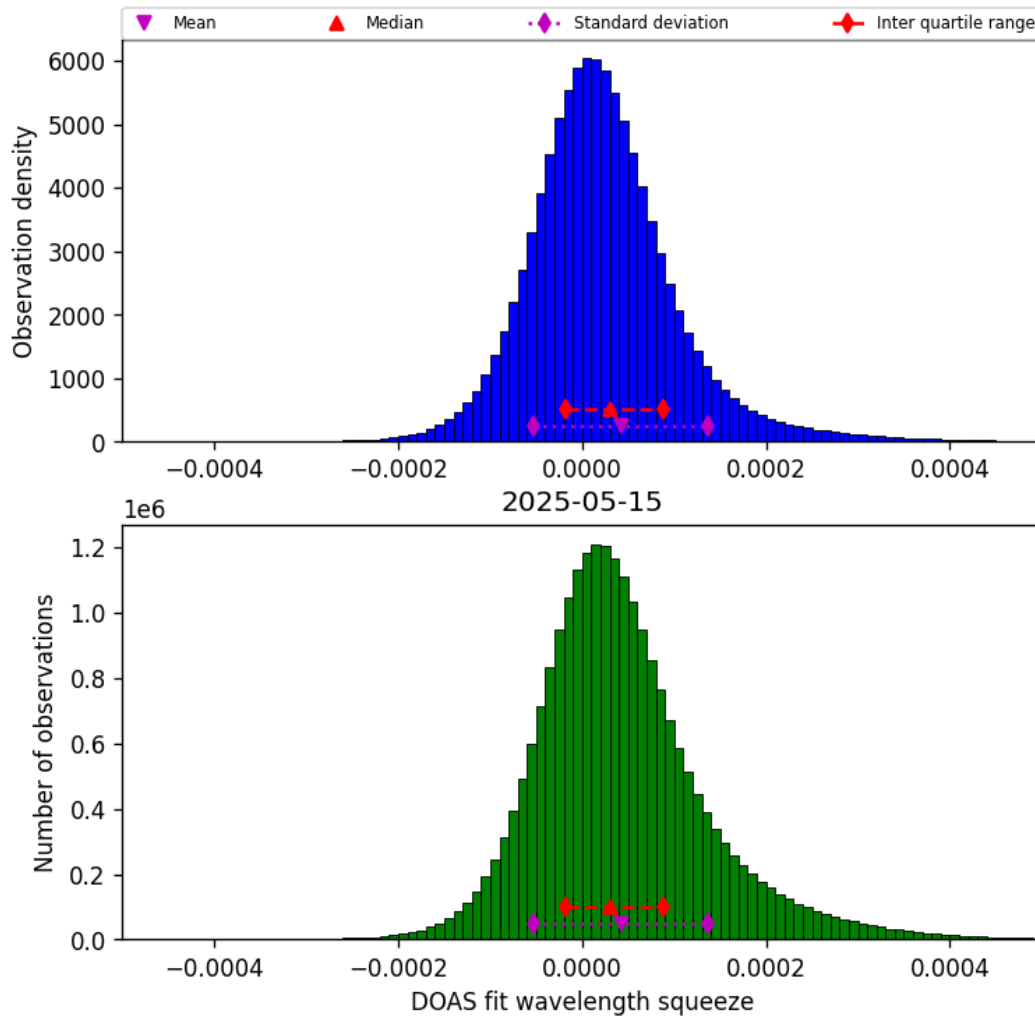
Figure 43: Histogram of “DOAS fit wavelength squeeze” for 2025-05-15 to 2025-05-16
