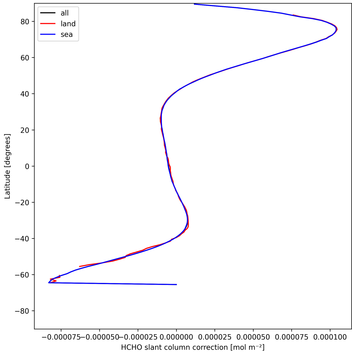
Figure 31: Zonal average of “HCHO slant column correction” for 2025-05-15 to 2025-05-16.
