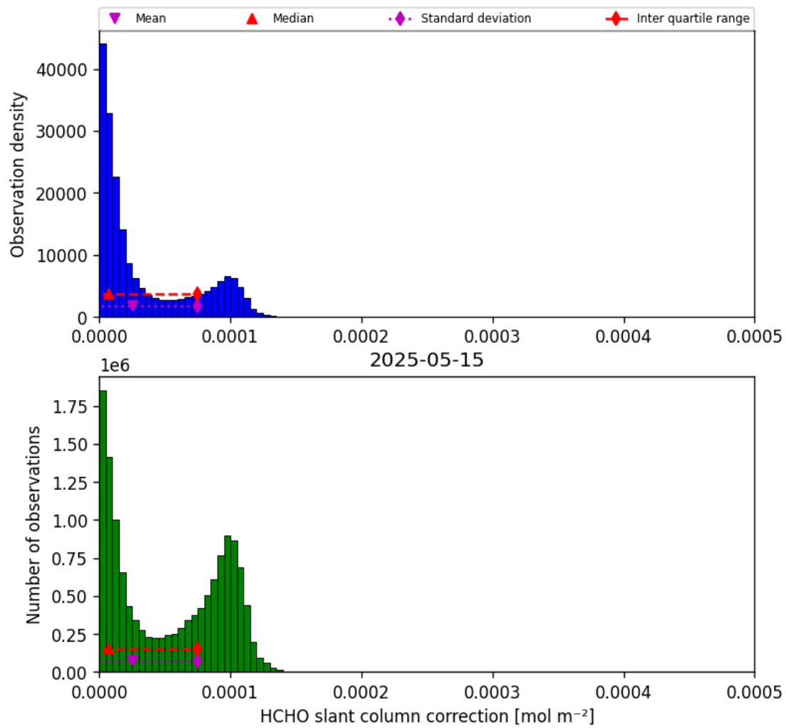
Figure 45: Histogram of “HCHO slant column correction” for 2025-05-15 to 2025-05-16
