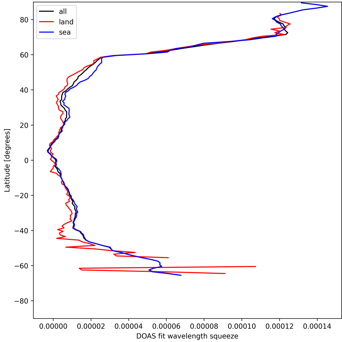
Figure 29: Zonal average of “DOAS fit wavelength squeeze” for 2025-05-15 to 2025-05-16.
