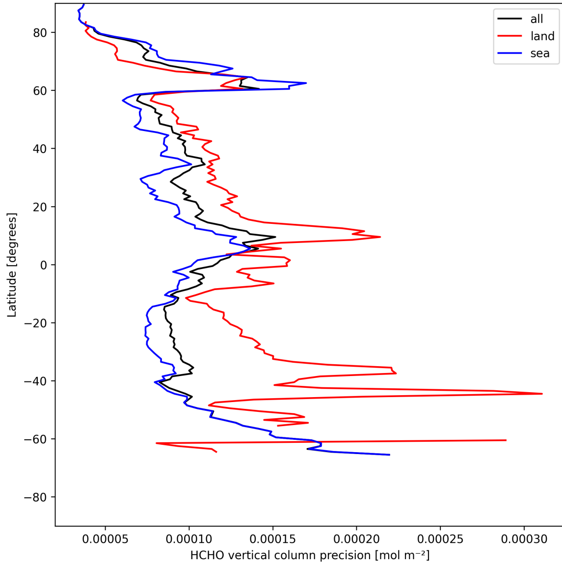
Figure 20: Zonal average of “HCHO vertical column precision” for 2025-05-15 to 2025-05-16.
