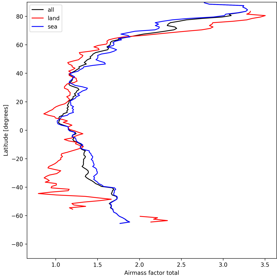
Figure 24: Zonal average of “Airmass factor total” for 2025-05-15 to 2025-05-16.
