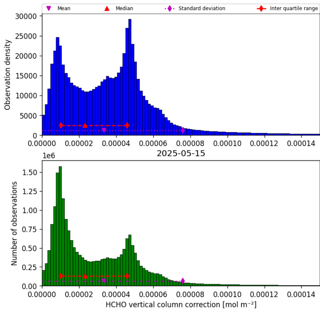
Figure 35: Histogram of “HCHO vertical column correction” for 2025-05-15 to 2025-05-16
