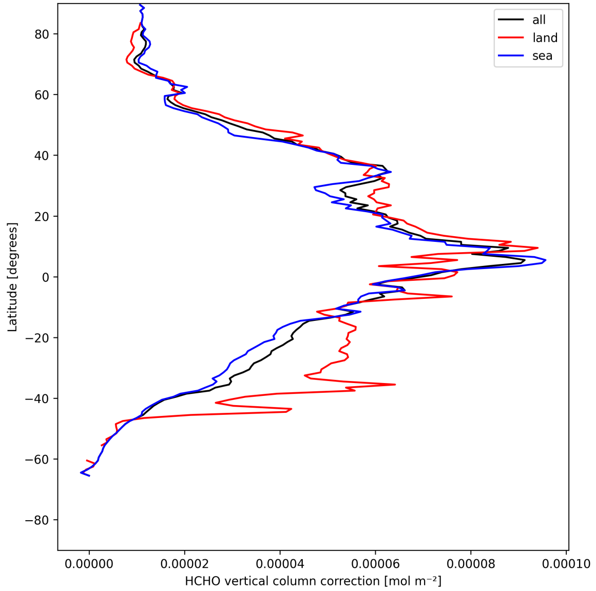
Figure 21: Zonal average of “HCHO vertical column correction” for 2025-05-15 to 2025-05-16.
