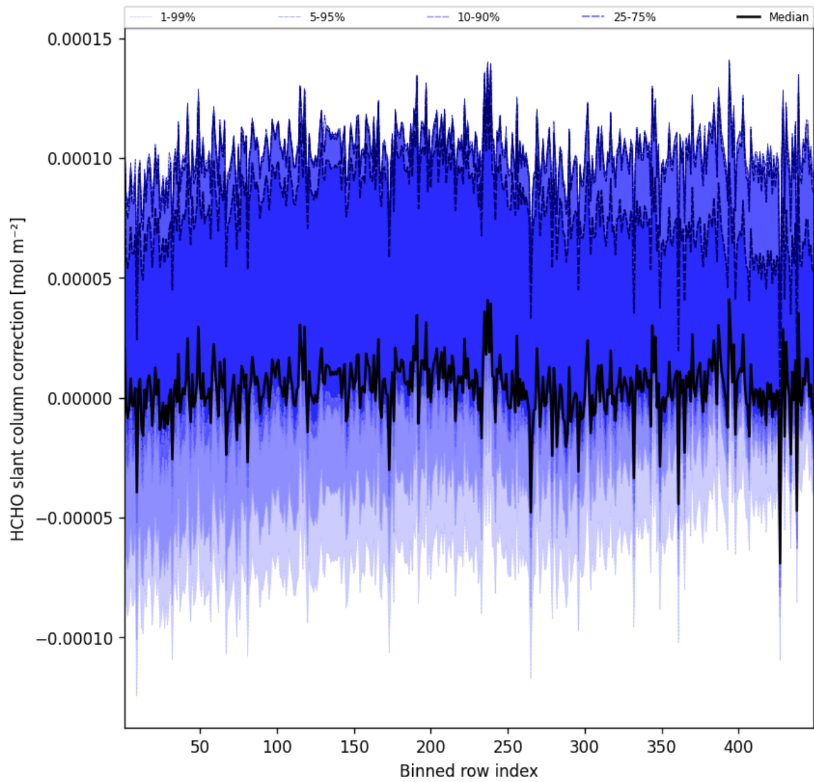
Figure 59: Along track statistics of “HCHO slant column correction” for 2025-05-15 to 2025-05-16
