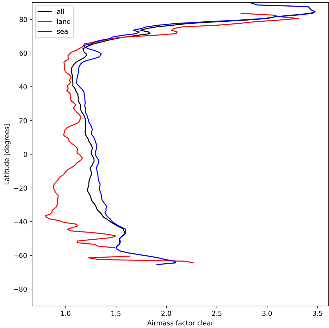
Figure 26: Zonal average of “Airmass factor clear” for 2025-05-15 to 2025-05-16.
