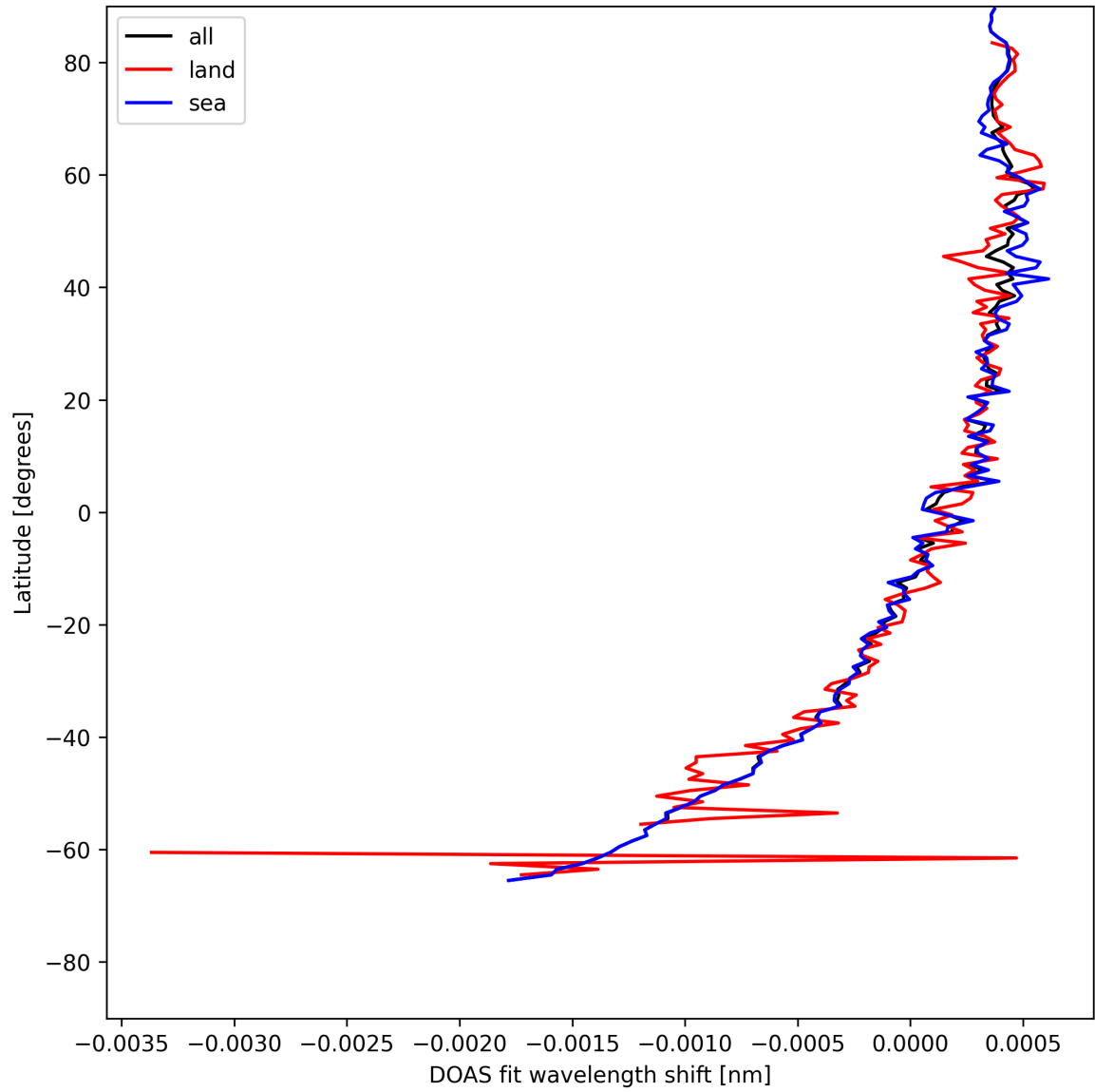
Figure 28: Zonal average of “DOAS fit wavelength shift” for 2025-05-15 to 2025-05-16.
