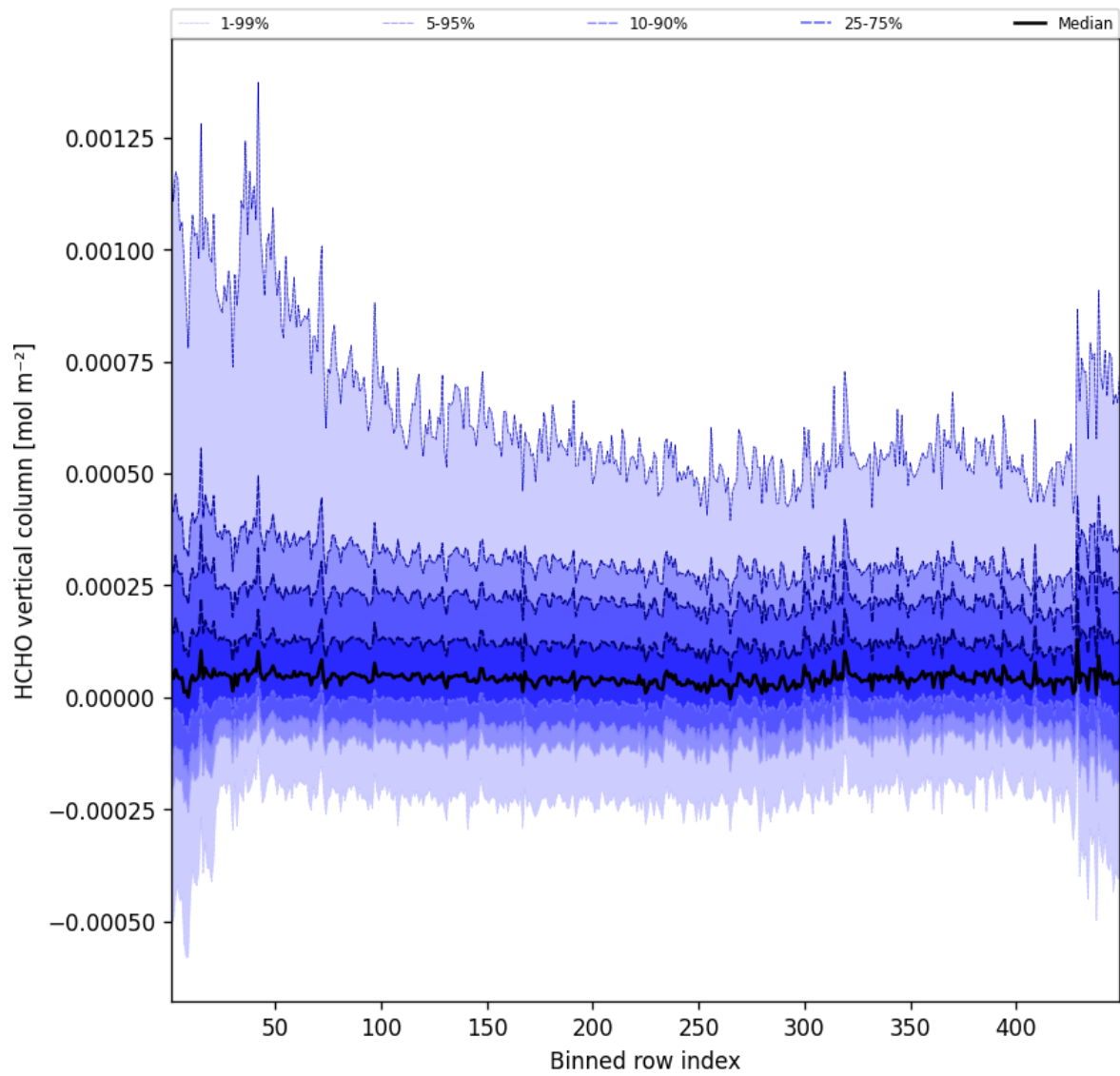
Figure 47: Along track statistics of “HCHO vertical column” for 2025-05-15 to 2025-05-16
