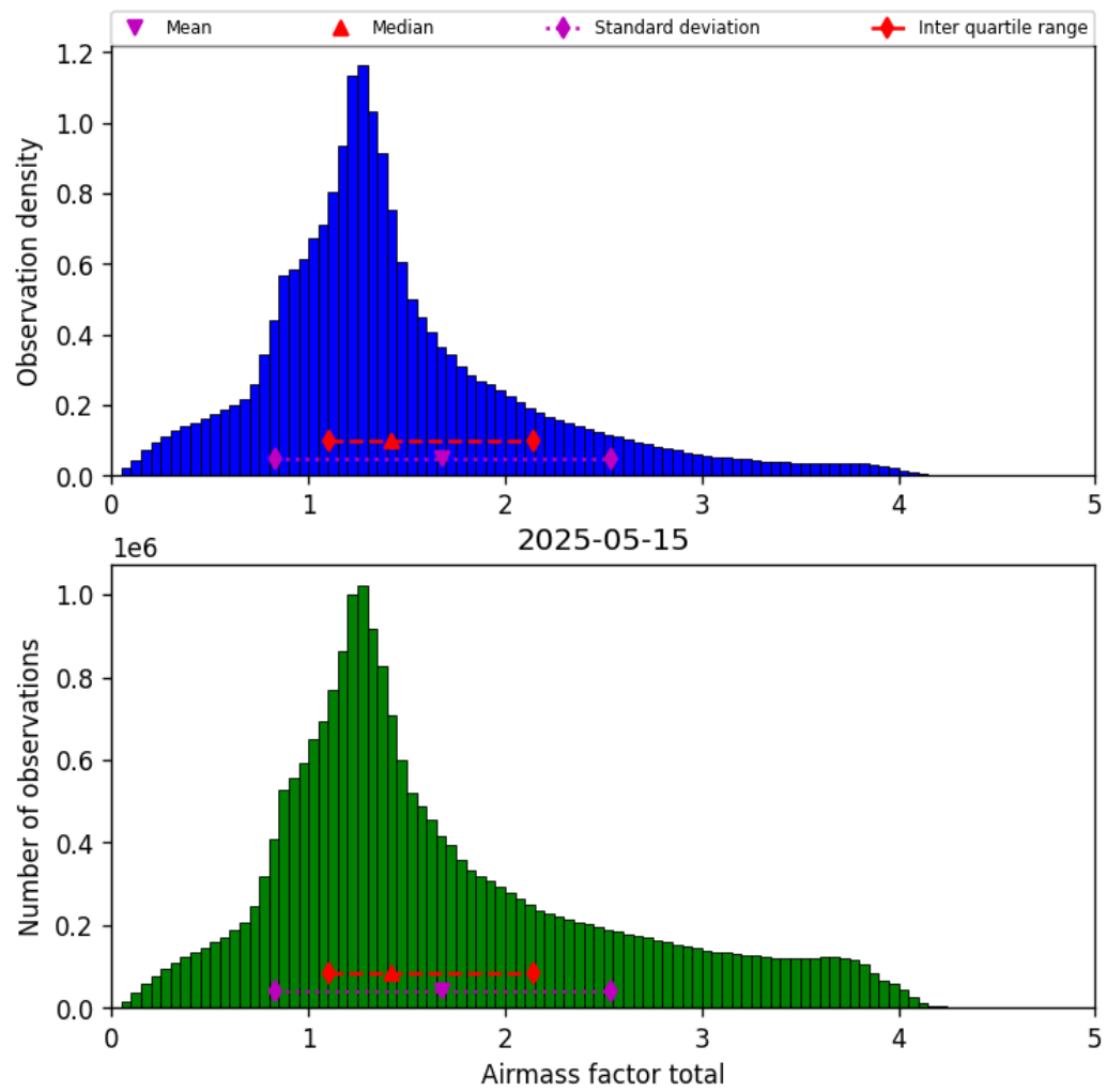
Figure 38: Histogram of “Airmass factor total” for 2025-05-15 to 2025-05-16
