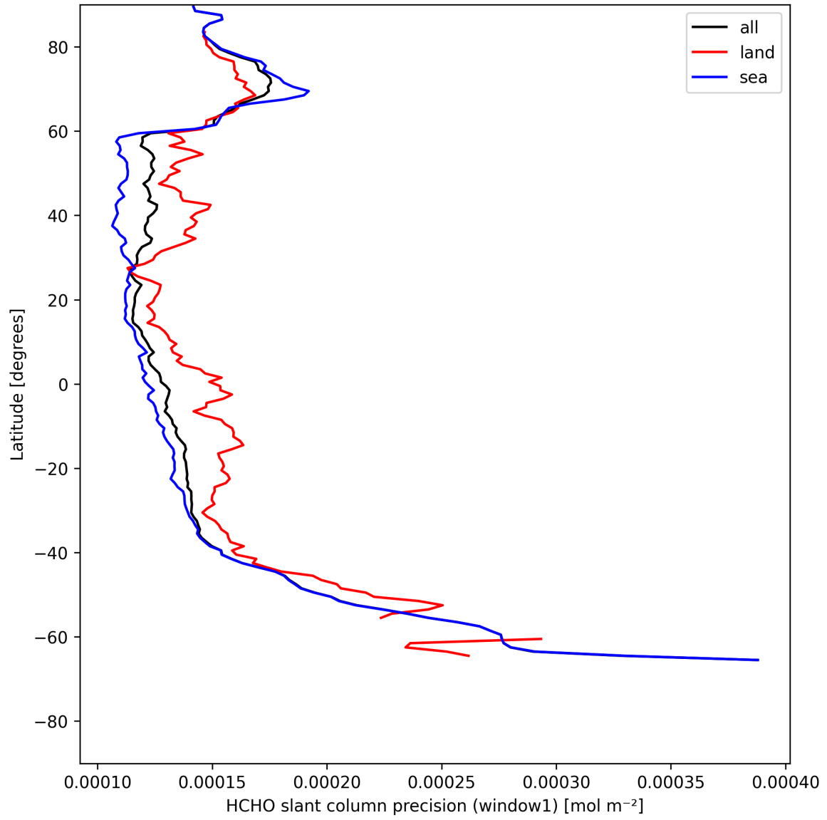
Figure 23: Zonal average of “HCHO slant column precision (window1)” for 2025-05-15 to 2025-05-16.
