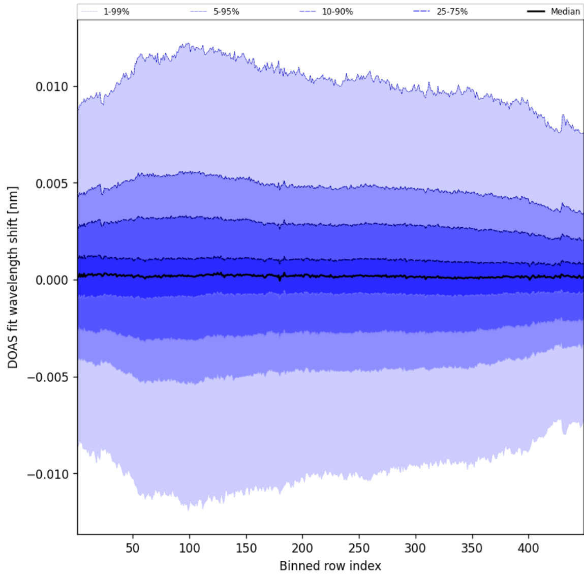
Figure 56: Along track statistics of “DOAS fit wavelength shift” for 2025-05-15 to 2025-05-16
