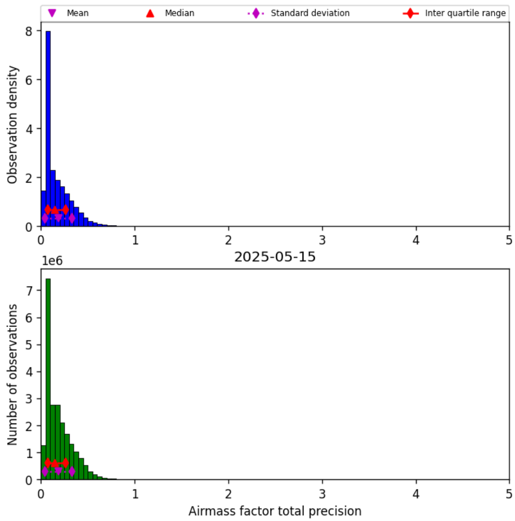
Figure 39: Histogram of “Airmass factor total precision” for 2025-05-15 to 2025-05-16
