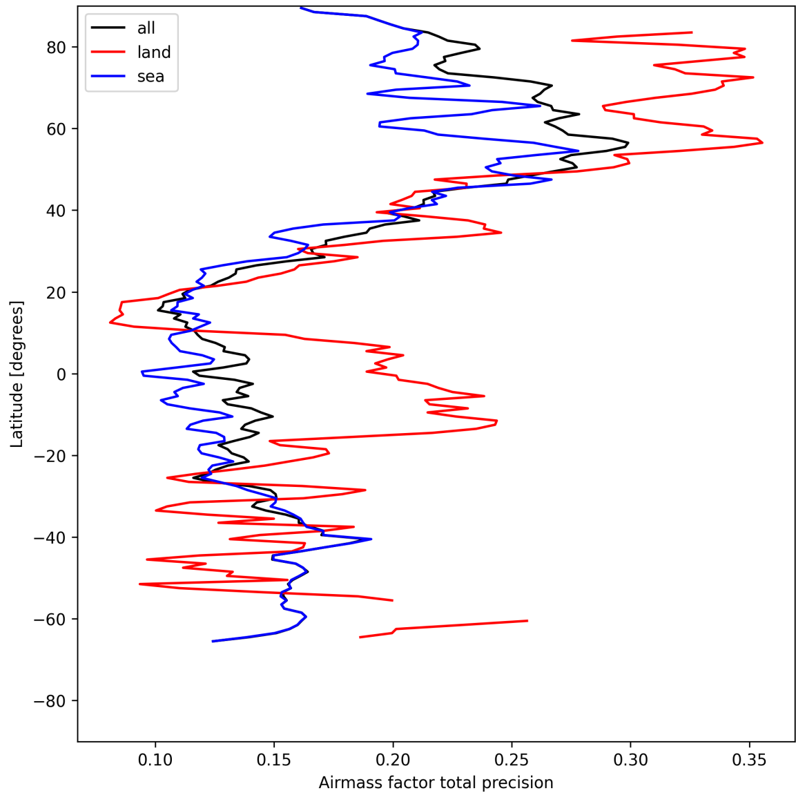
Figure 25: Zonal average of “Airmass factor total precision” for 2025-05-15 to 2025-05-16.
