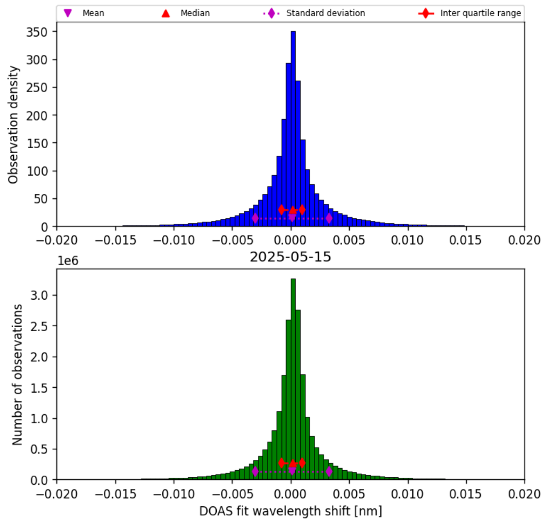
Figure 42: Histogram of “DOAS fit wavelength shift” for 2025-05-15 to 2025-05-16
