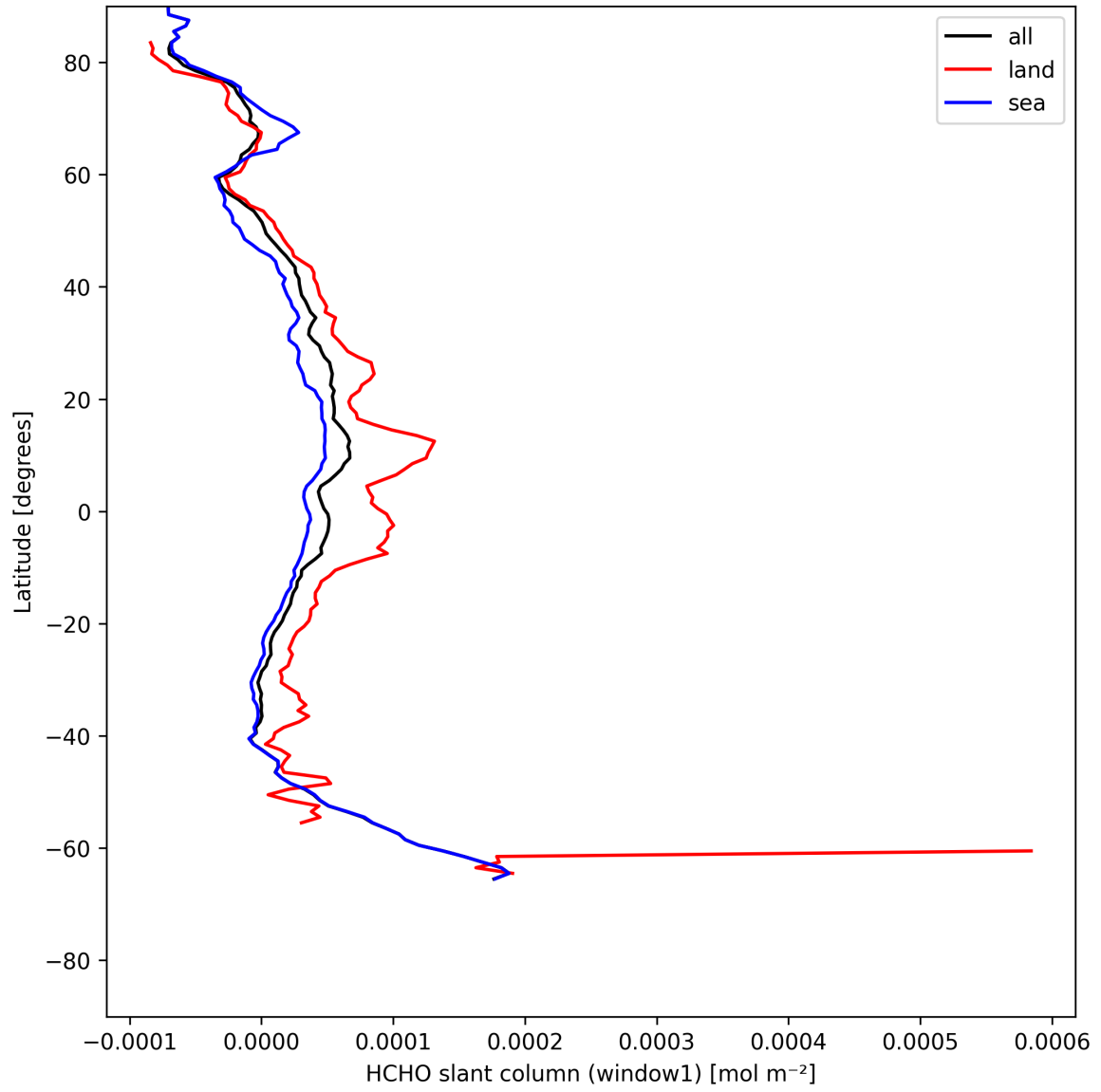
Figure 22: Zonal average of “HCHO slant column (window1)” for 2025-05-15 to 2025-05-16.
