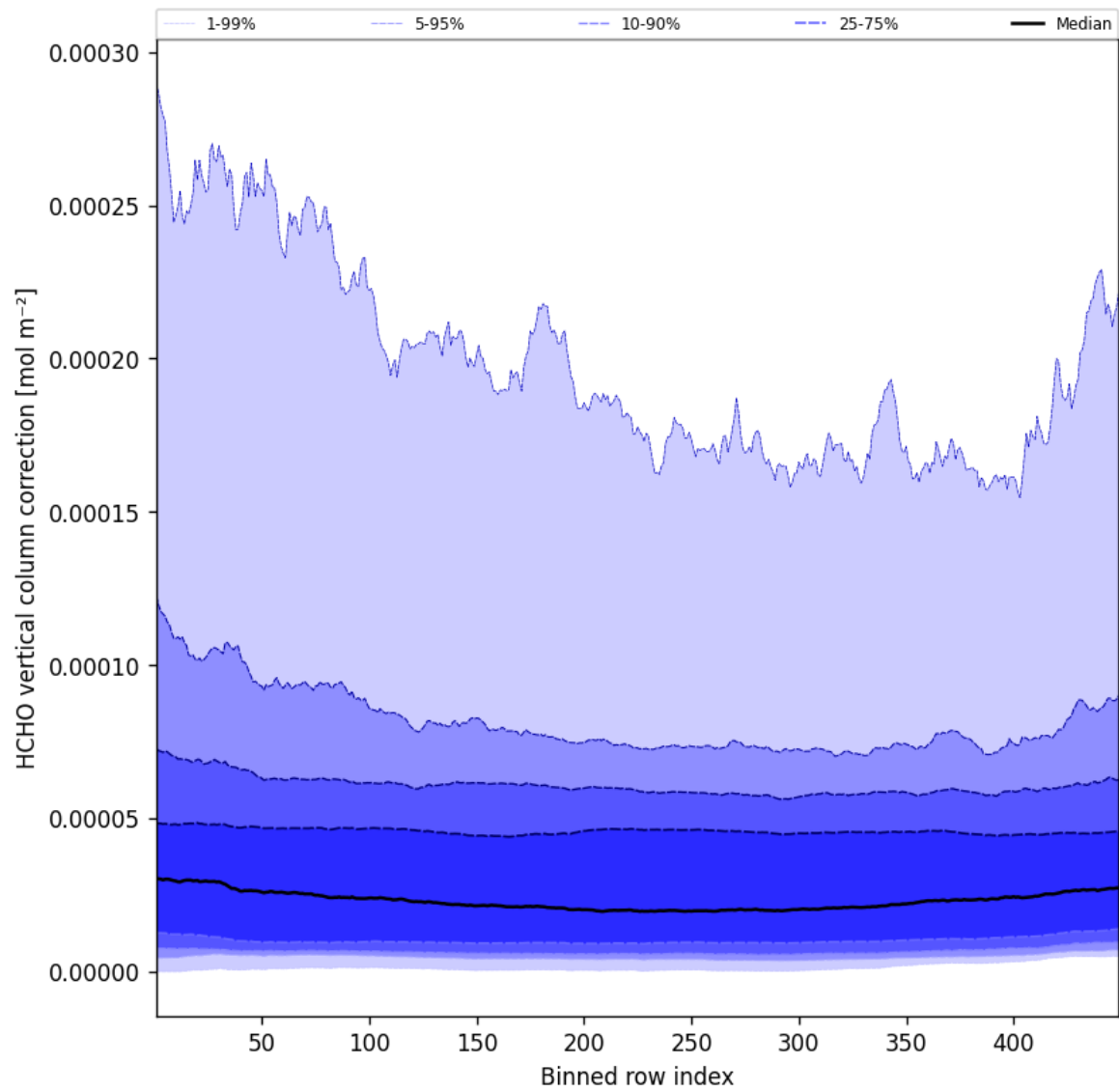
Figure 49: Along track statistics of “HCHO vertical column correction” for 2025-05-15 to 2025-05-16
