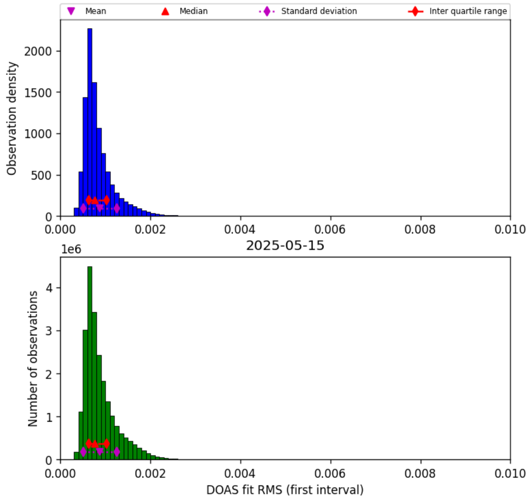
Figure 44: Histogram of “DOAS fit RMS (first interval)” for 2025-05-15 to 2025-05-16
