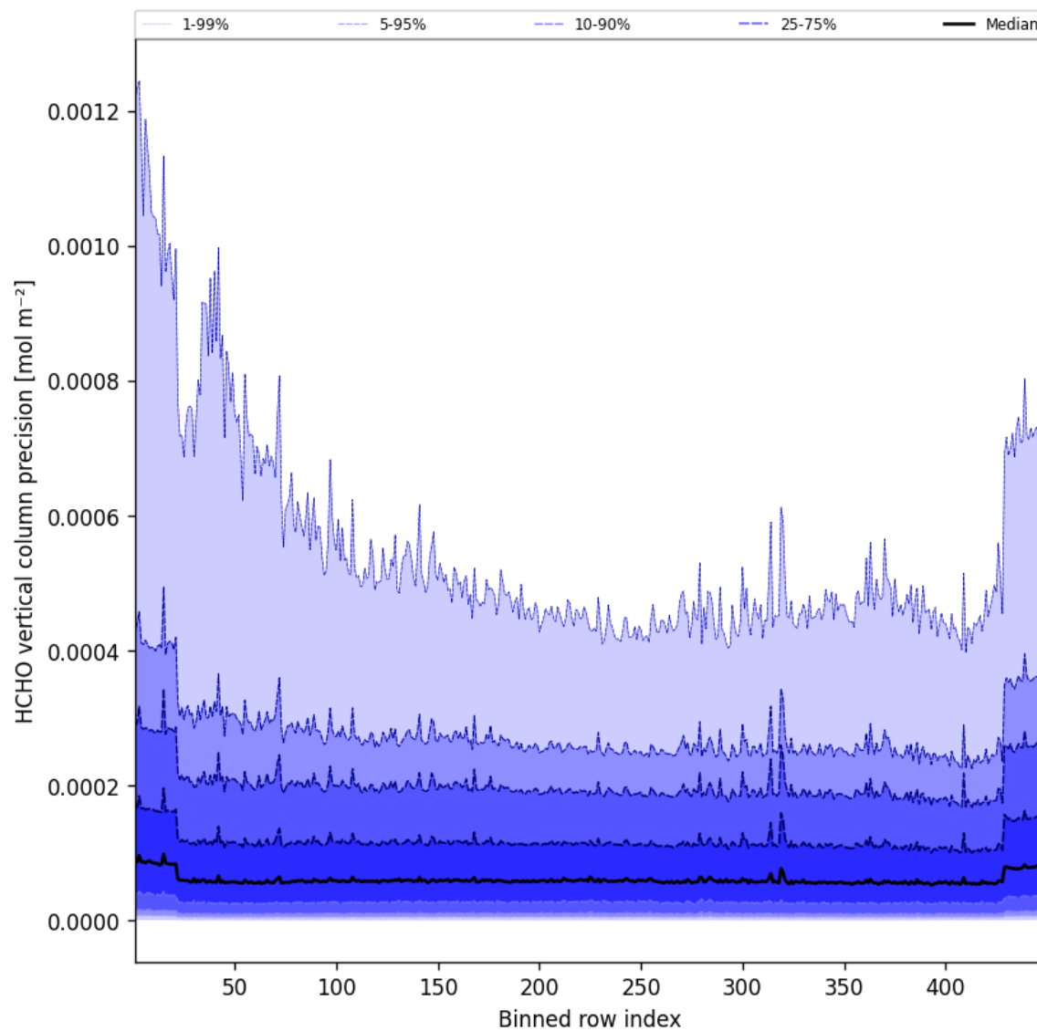
Figure 48: Along track statistics of “HCHO vertical column precision” for 2025-05-15 to 2025-05-16
