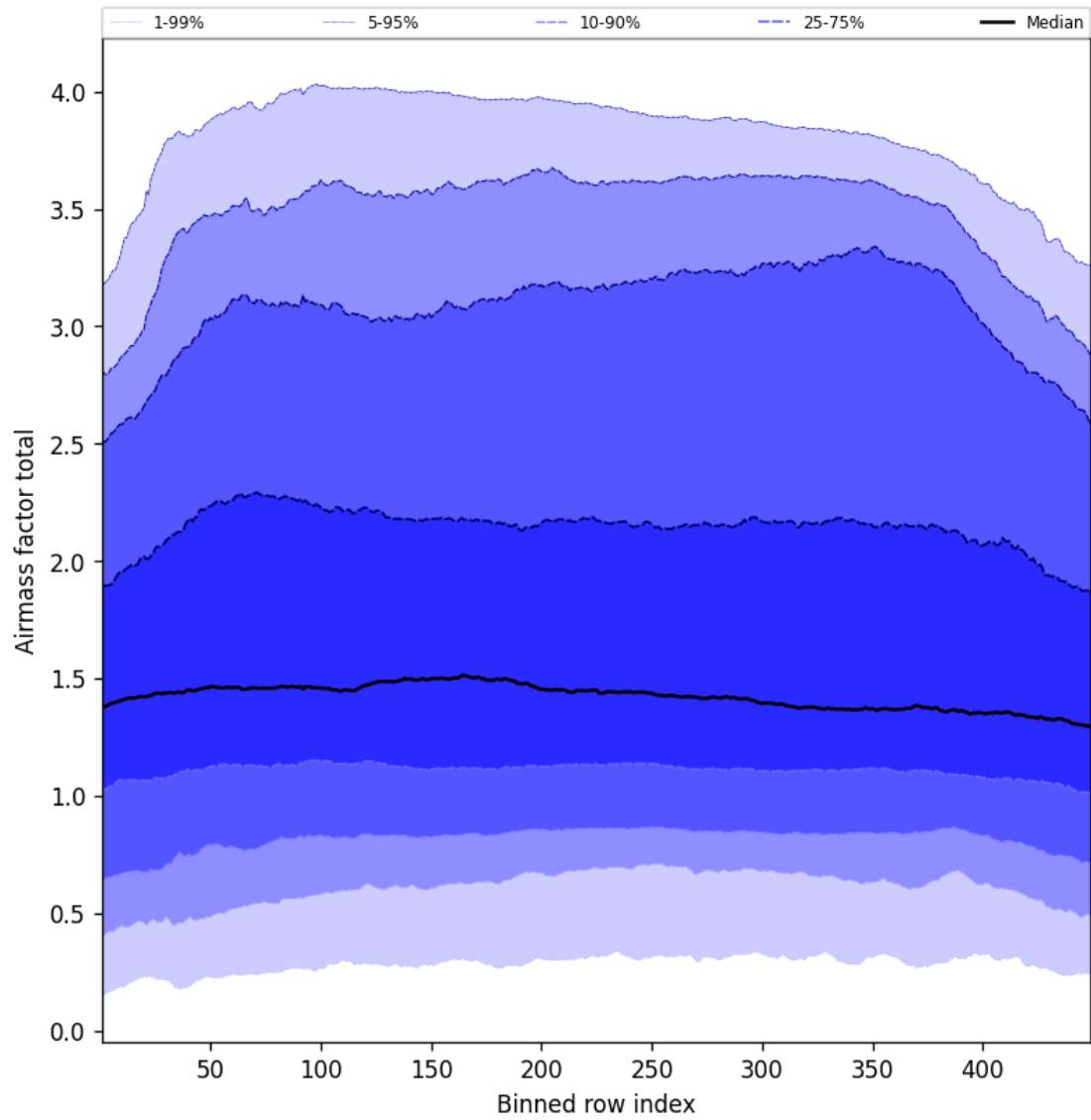
Figure 52: Along track statistics of “Airmass factor total” for 2025-05-15 to 2025-05-16
