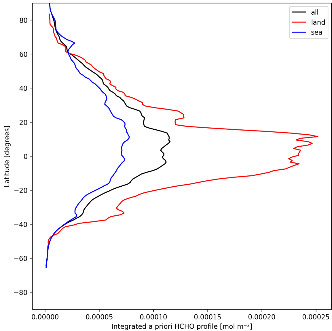
Figure 27: Zonal average of “Integrated a priori HCHO profile” for 2025-05-15 to 2025-05-16.
