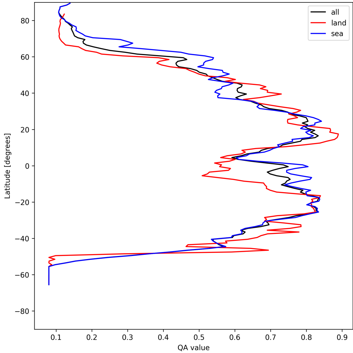
Figure 18: Zonal average of “QA value” for 2025-05-15 to 2025-05-16.
