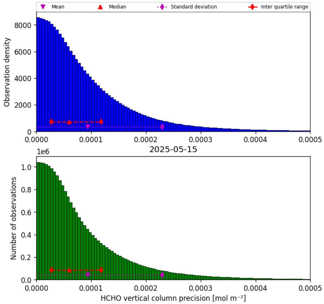
Figure 34: Histogram of “HCHO vertical column precision” for 2025-05-15 to 2025-05-16
