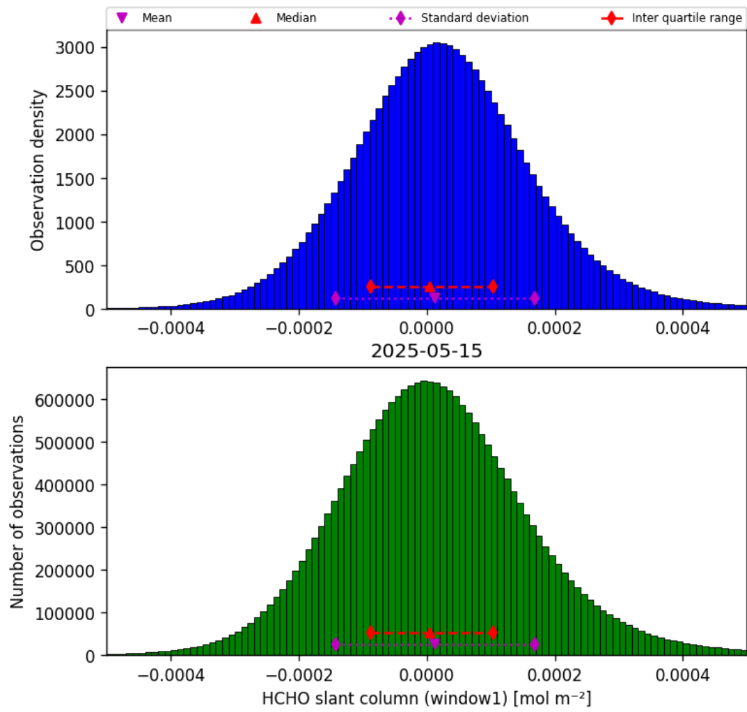
Figure 36: Histogram of “HCHO slant column (window1)” for 2025-05-15 to 2025-05-16
