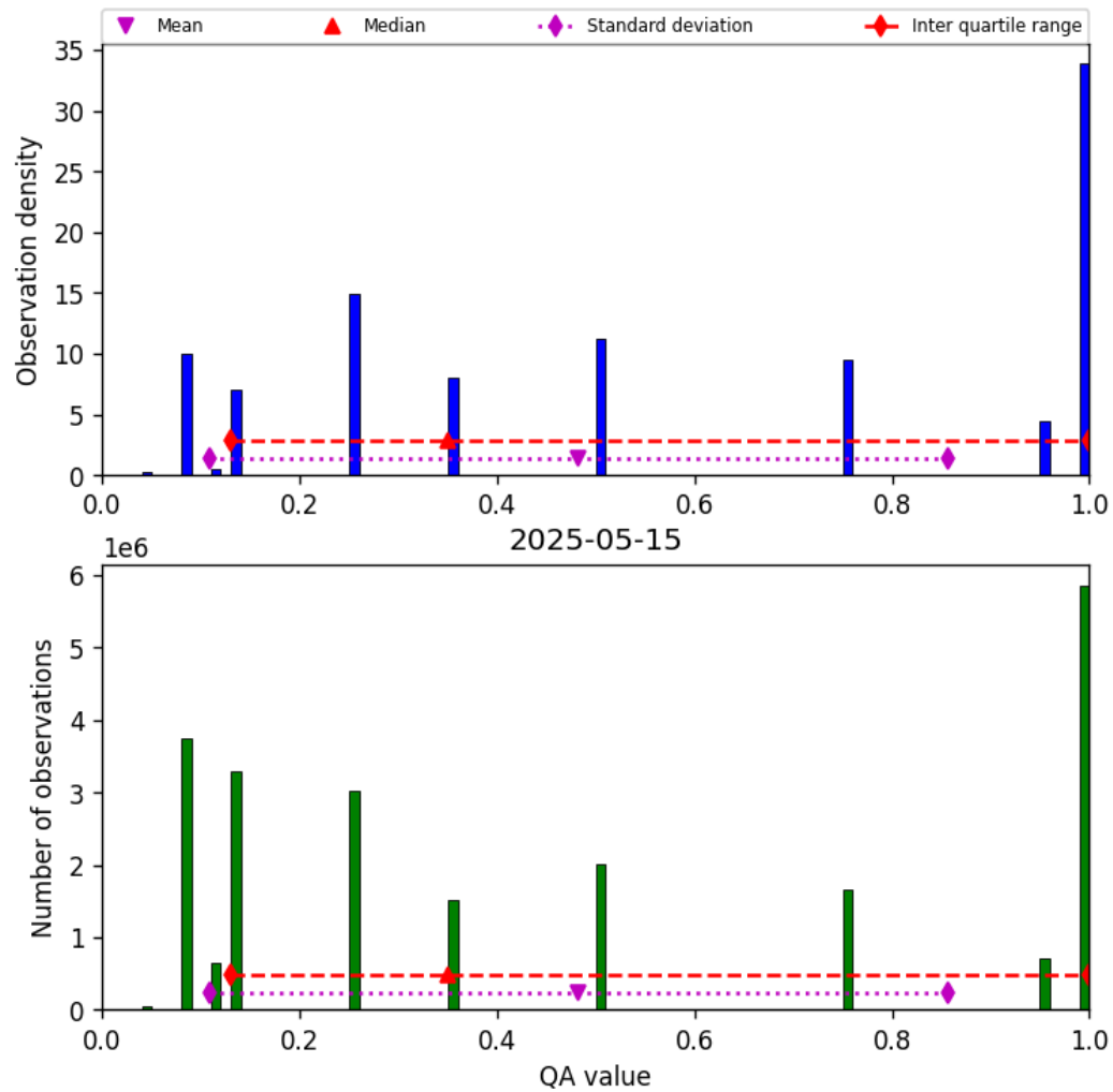
Figure 32: Histogram of “QA value” for 2025-05-15 to 2025-05-16
