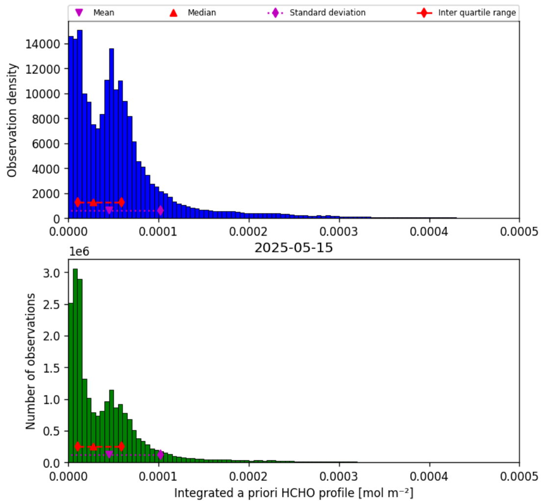
Figure 41: Histogram of “Integrated a priori HCHO profile” for 2025-05-15 to 2025-05-16
