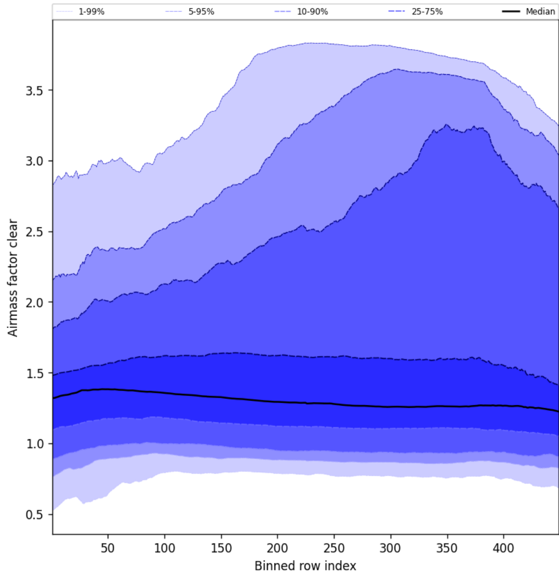
Figure 54: Along track statistics of “Airmass factor clear” for 2025-05-15 to 2025-05-16
