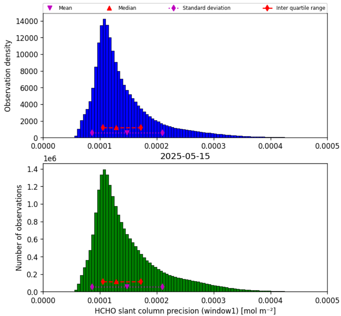
Figure 37: Histogram of “HCHO slant column precision (window1)” for 2025-05-15 to 2025-05-16
