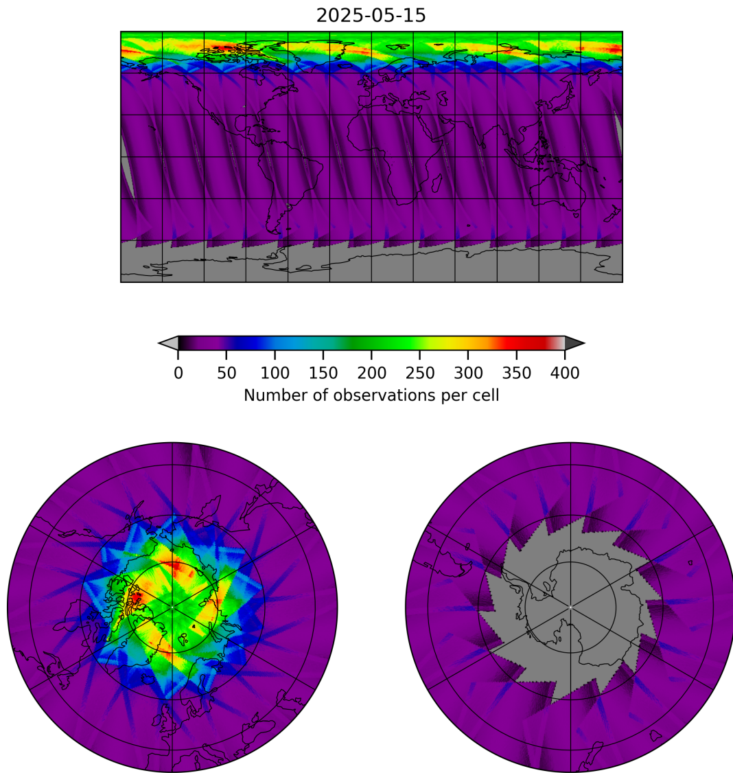
Figure 17: Map of the number of observations for 2025-05-15 to 2025-05-16
