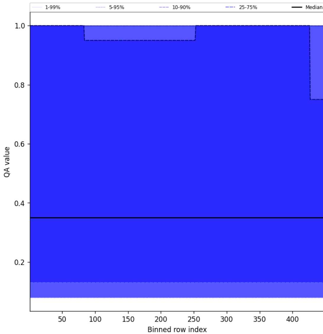
Figure 46: Along track statistics of “QA value” for 2025-05-15 to 2025-05-16
