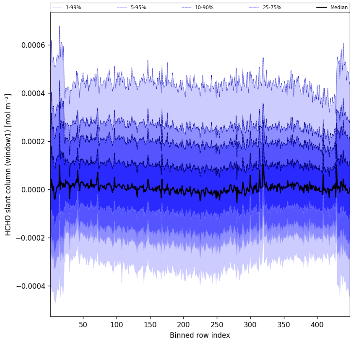
Figure 50: Along track statistics of “HCHO slant column (window1)” for 2025-05-15 to 2025-05-16
