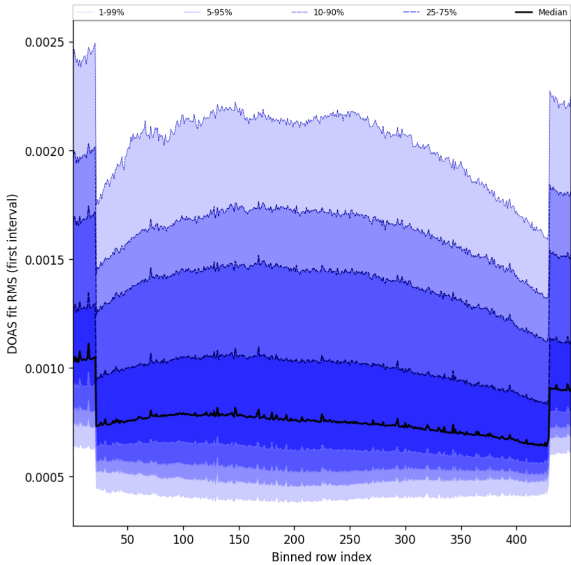
Figure 58: Along track statistics of “DOAS fit RMS (first interval)” for 2025-05-15 to 2025-05-16
