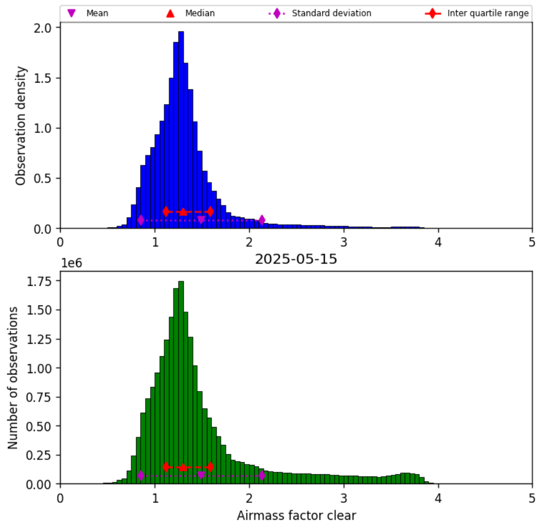
Figure 40: Histogram of “Airmass factor clear” for 2025-05-15 to 2025-05-16
