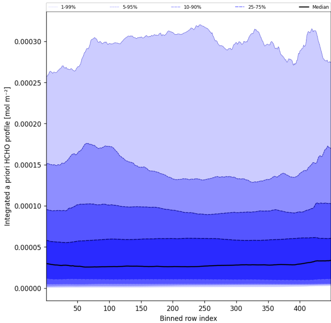
Figure 55: Along track statistics of “Integrated a priori HCHO profile” for 2025-05-15 to 2025-05-16
