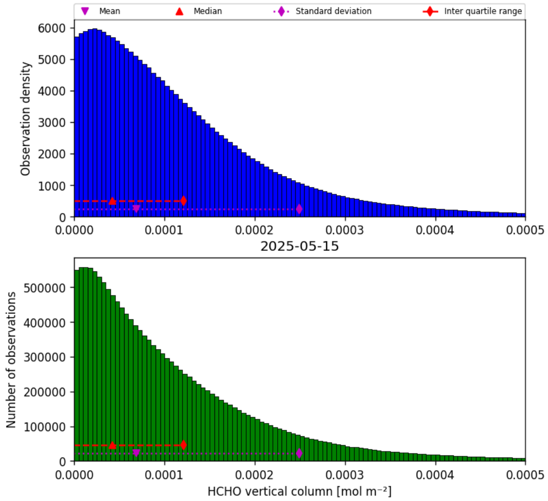
Figure 33: Histogram of “HCHO vertical column” for 2025-05-15 to 2025-05-16
