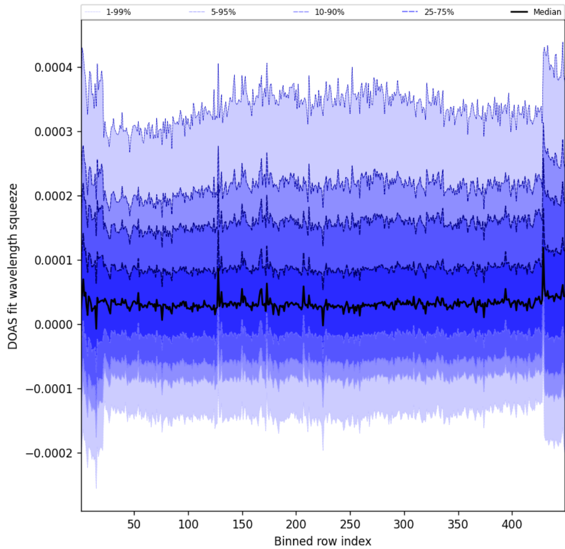
Figure 57: Along track statistics of “DOAS fit wavelength squeeze” for 2025-05-15 to 2025-05-16
