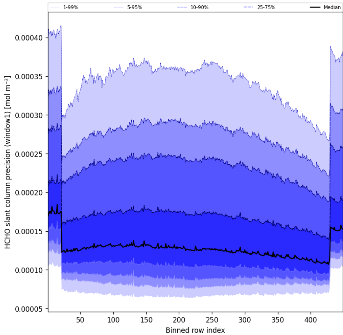
Figure 51: Along track statistics of “HCHO slant column precision (window1)” for 2025-05-15 to 2025-05-16
