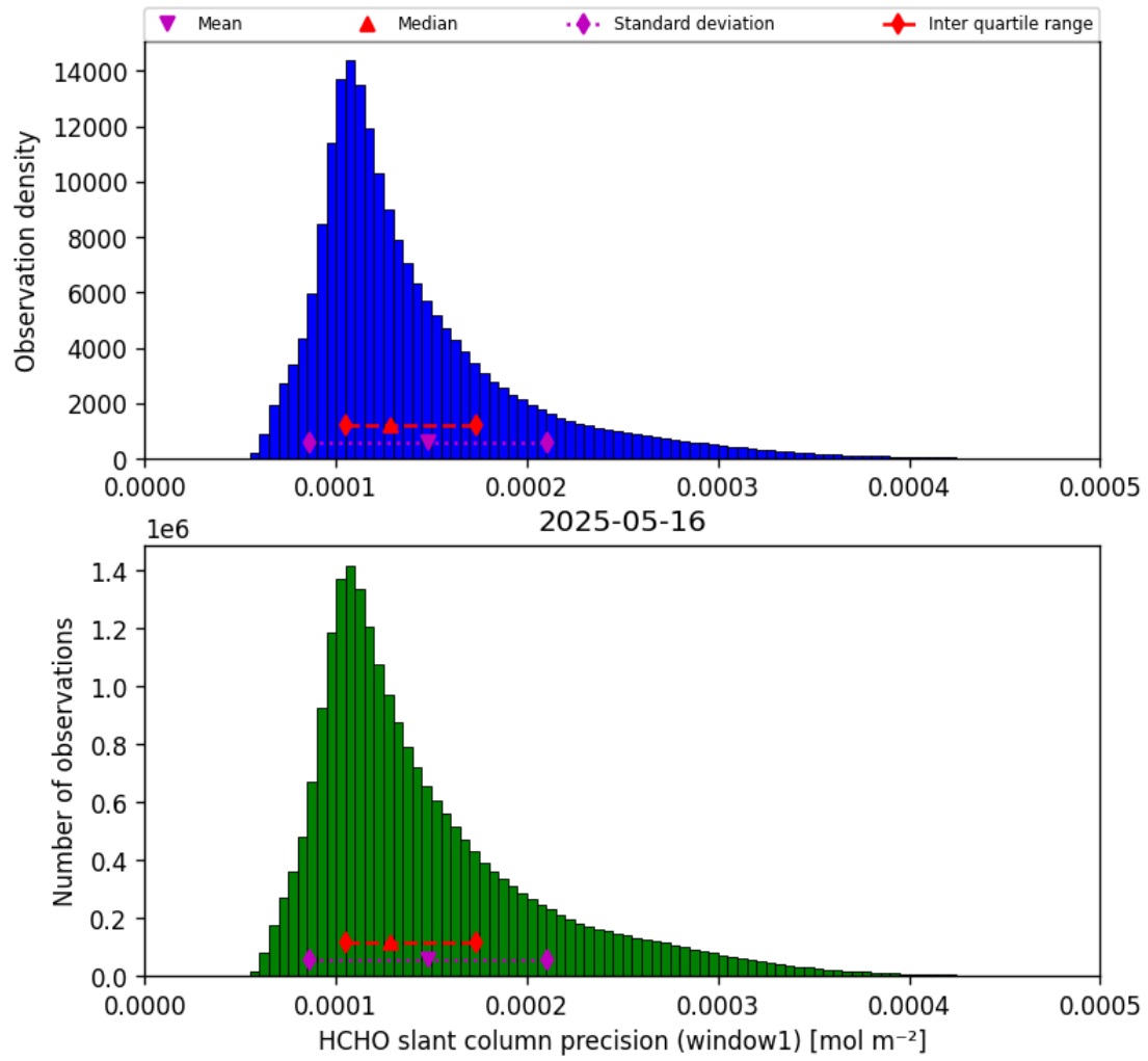
Figure 37: Histogram of “HCHO slant column precision (window1)” for 2025-05-16 to 2025-05-17
