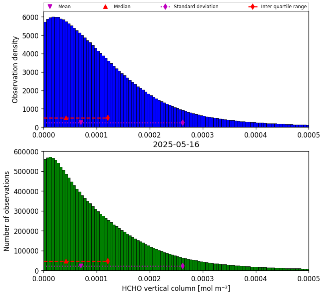
Figure 33: Histogram of “HCHO vertical column” for 2025-05-16 to 2025-05-17
