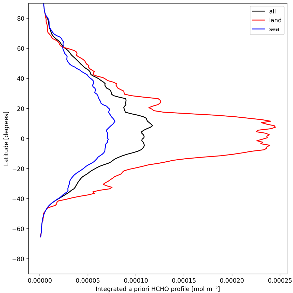
Figure 27: Zonal average of “Integrated a priori HCHO profile” for 2025-05-16 to 2025-05-17.
