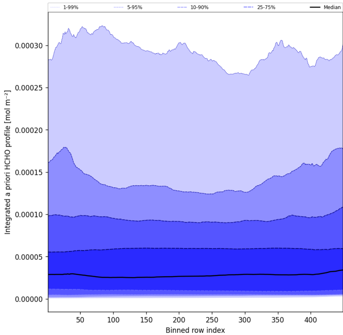
Figure 55: Along track statistics of "Integrated a priori HCHO profile" for 2025-05-16 to 2025-05-17
