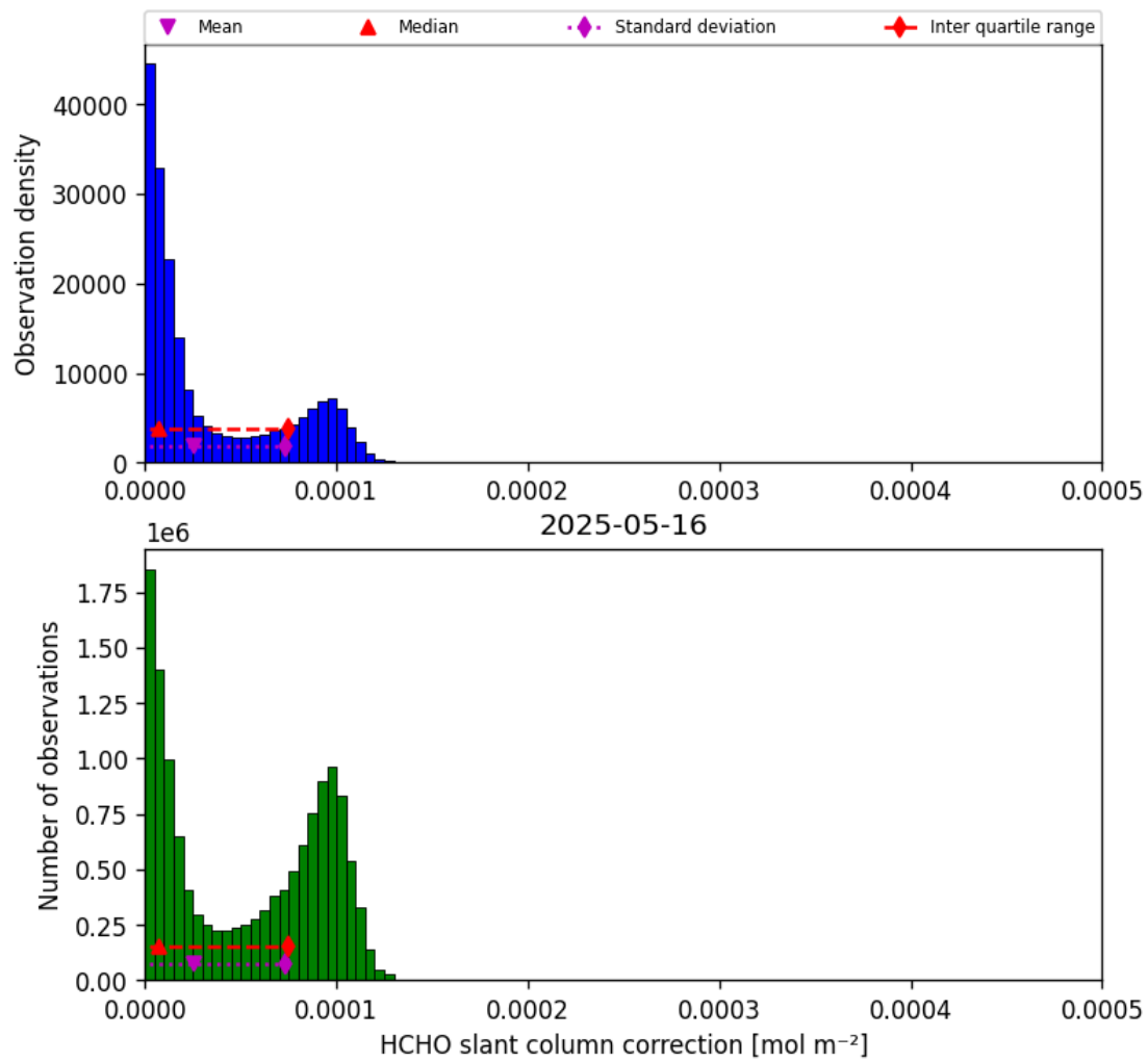
Figure 45: Histogram of “HCHO slant column correction” for 2025-05-16 to 2025-05-17
