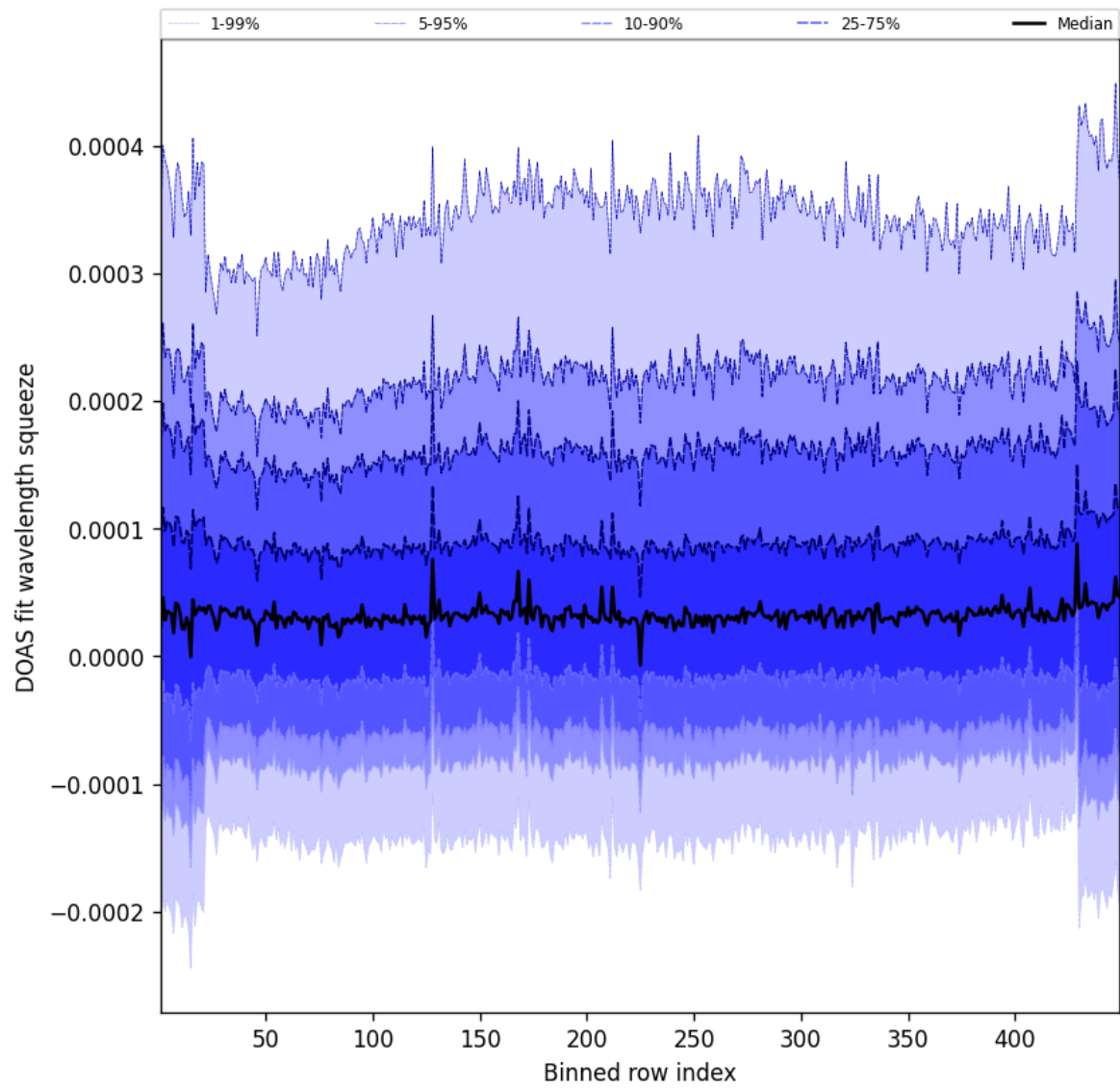
Figure 57: Along track statistics of “DOAS fit wavelength squeeze” for 2025-05-16 to 2025-05-17
