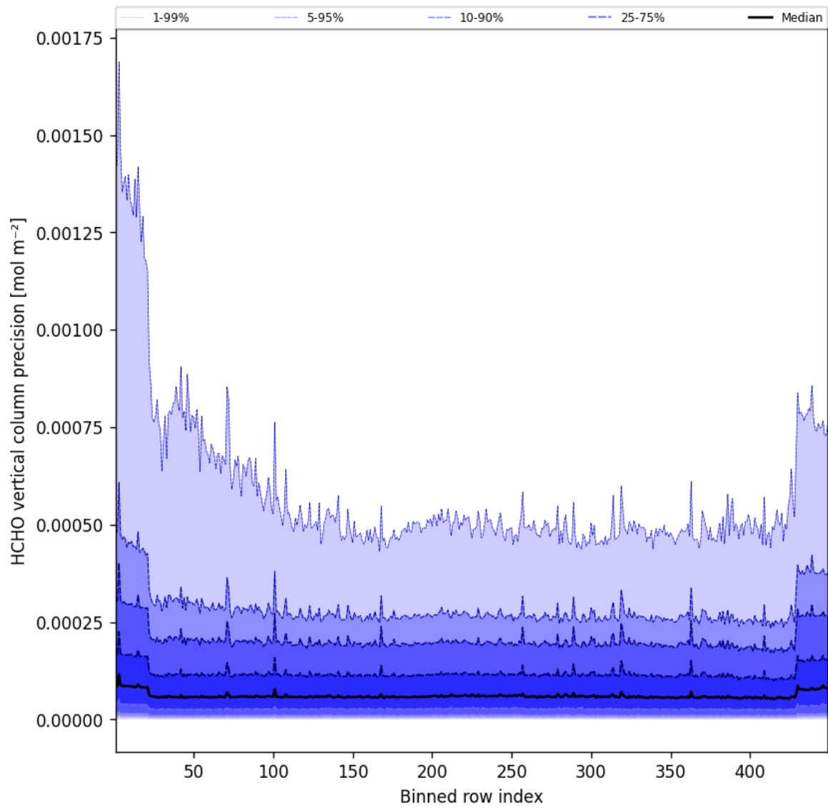
Figure 48: Along track statistics of “HCHO vertical column precision” for 2025-05-16 to 2025-05-17
