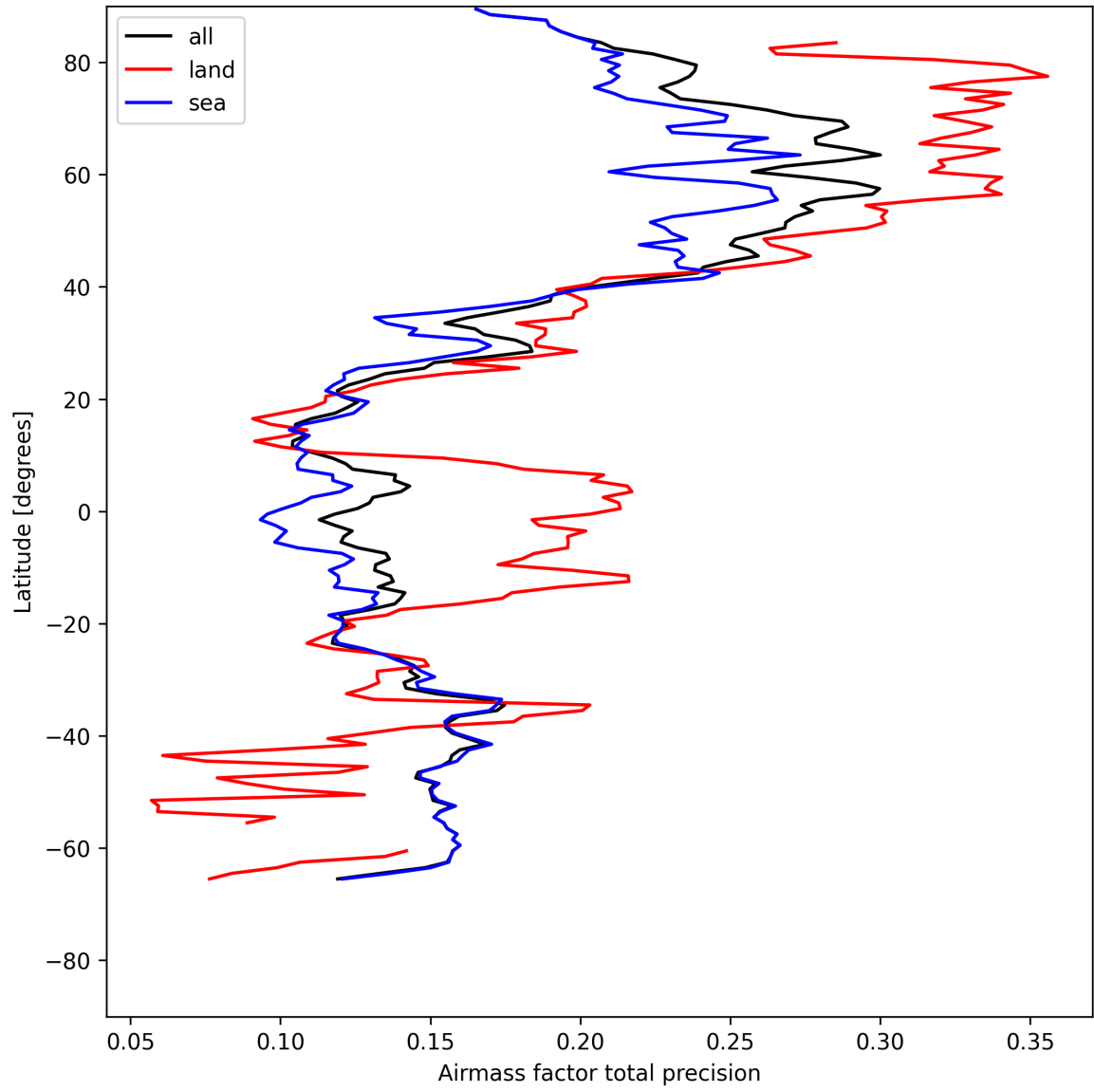
Figure 25: Zonal average of “Airmass factor total precision” for 2025-05-16 to 2025-05-17.
