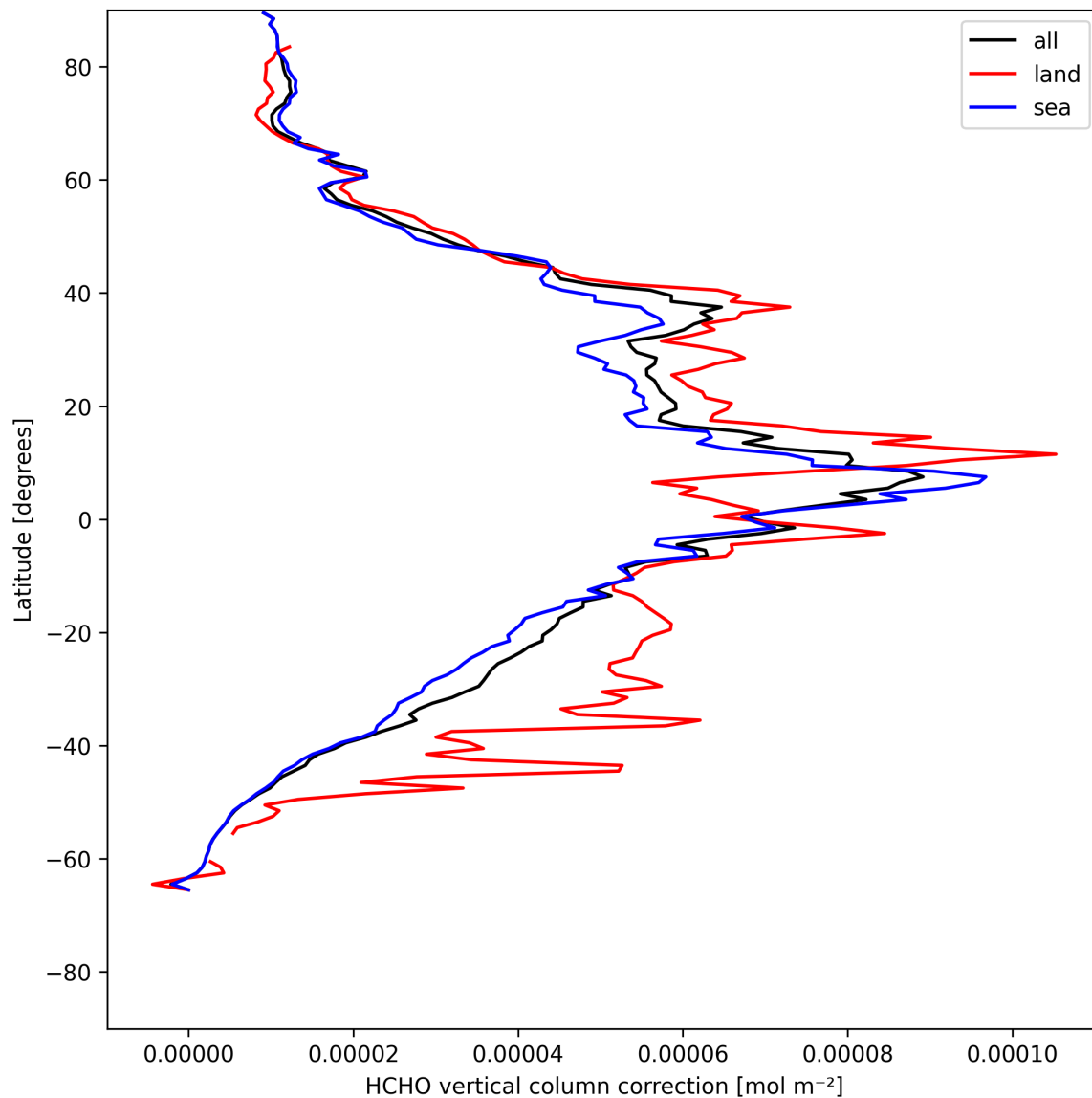
Figure 21: Zonal average of “HCHO vertical column correction” for 2025-05-16 to 2025-05-17.
