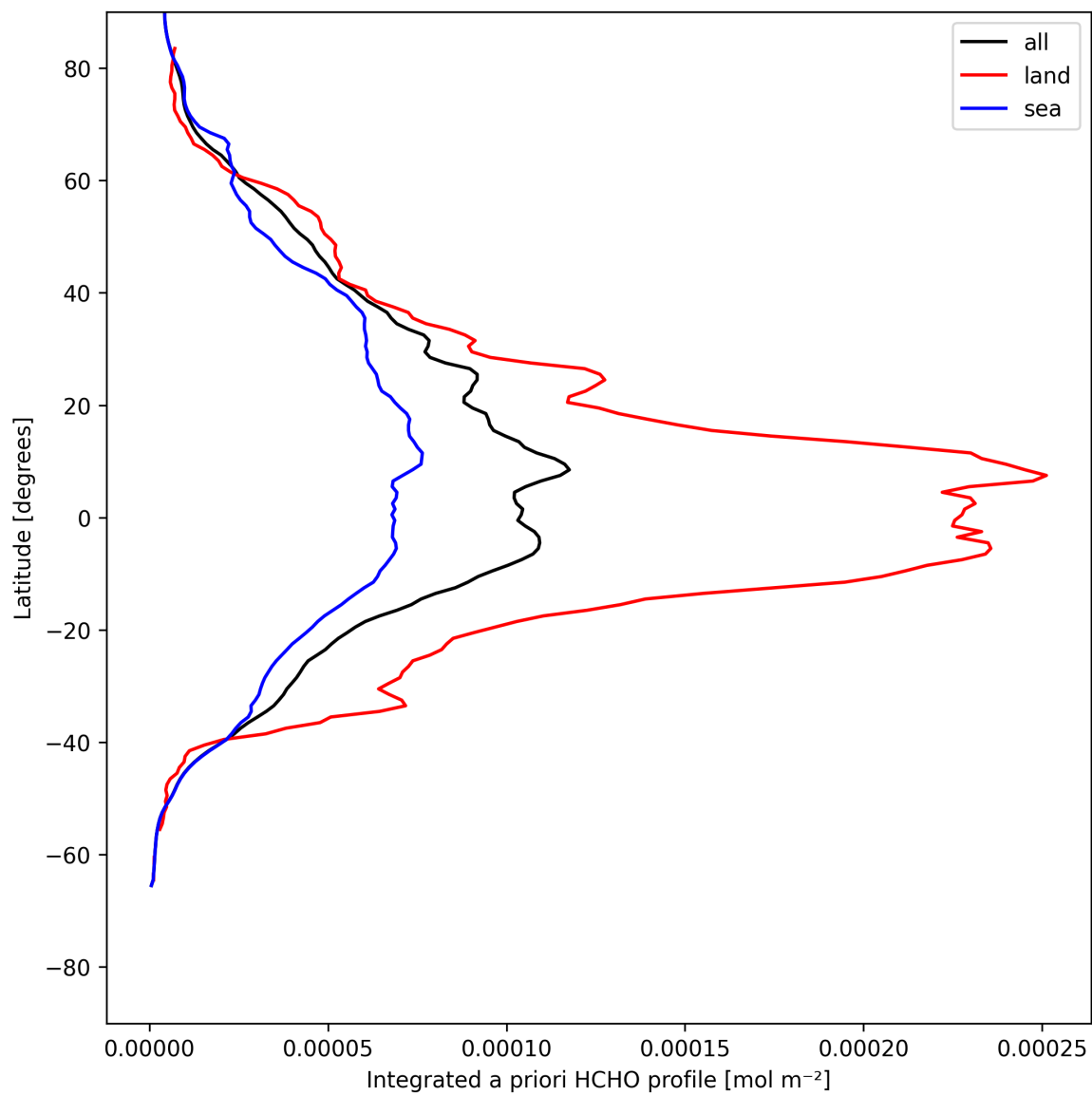
Figure 27: Zonal average of “Integrated a priori HCHO profile” for 2025-05-17 to 2025-05-18.
