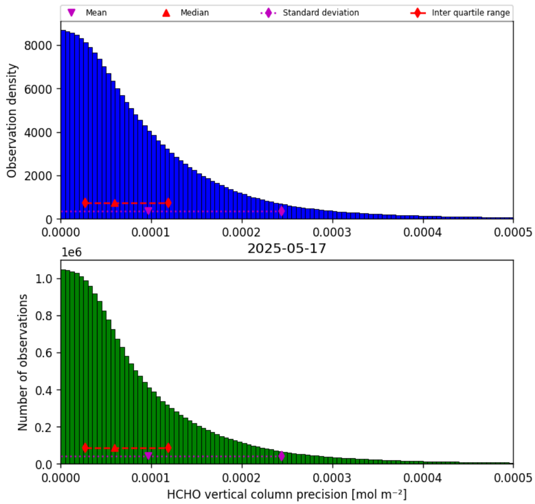
Figure 34: Histogram of “HCHO vertical column precision” for 2025-05-17 to 2025-05-18
