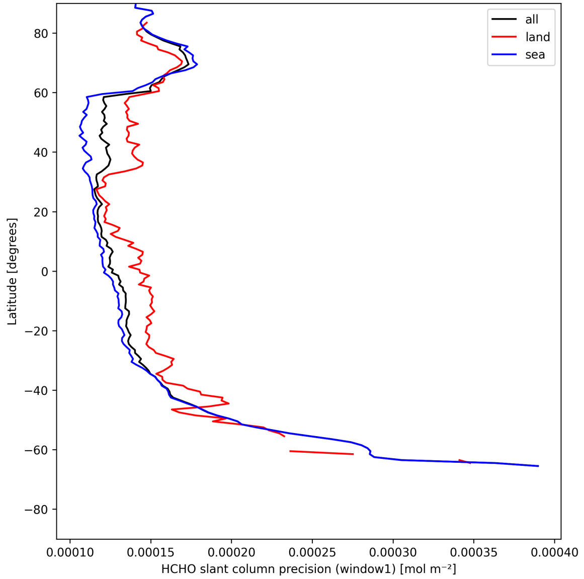
Figure 23: Zonal average of “HCHO slant column precision (window1)” for 2025-05-17 to 2025-05-18.
