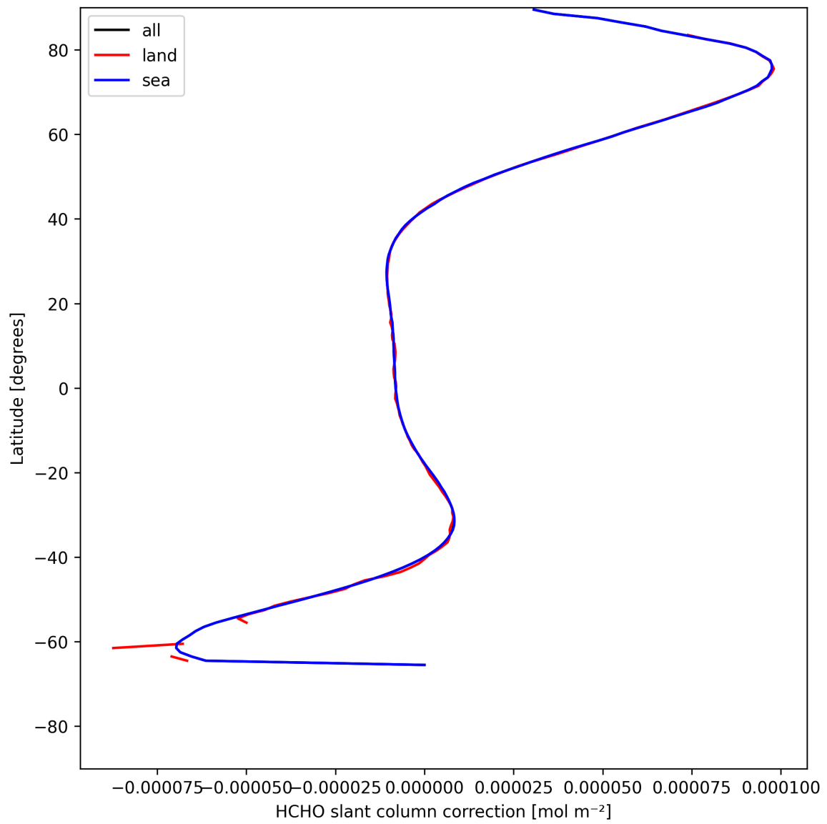
Figure 31: Zonal average of “HCHO slant column correction” for 2025-05-17 to 2025-05-18.
