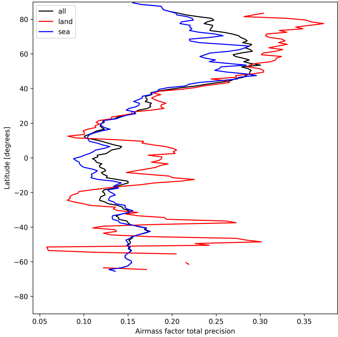
Figure 25: Zonal average of “Airmass factor total precision” for 2025-05-17 to 2025-05-18.
