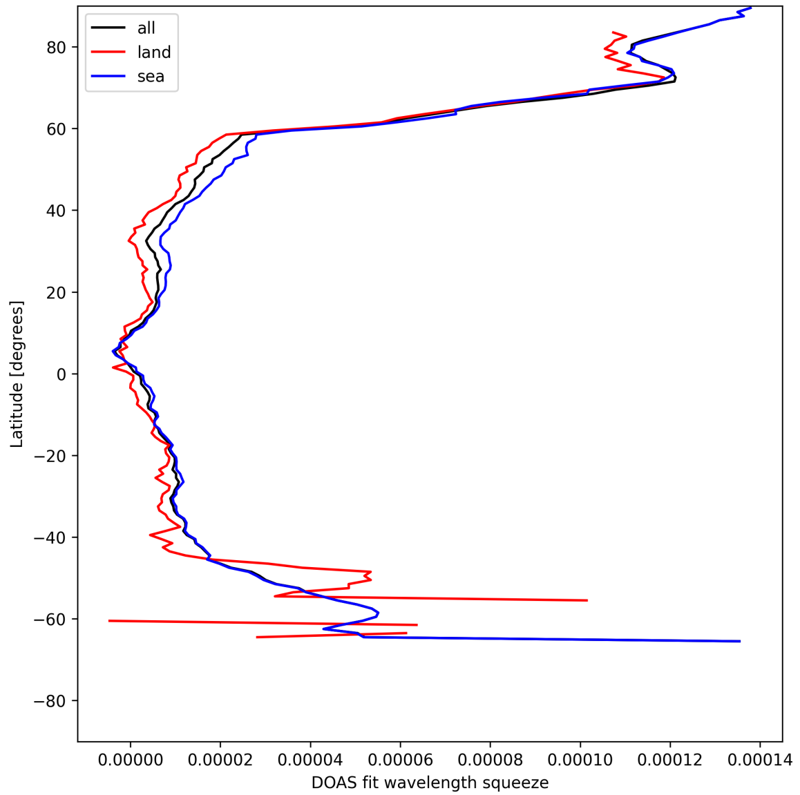
Figure 29: Zonal average of “DOAS fit wavelength squeeze” for 2025-05-17 to 2025-05-18.
