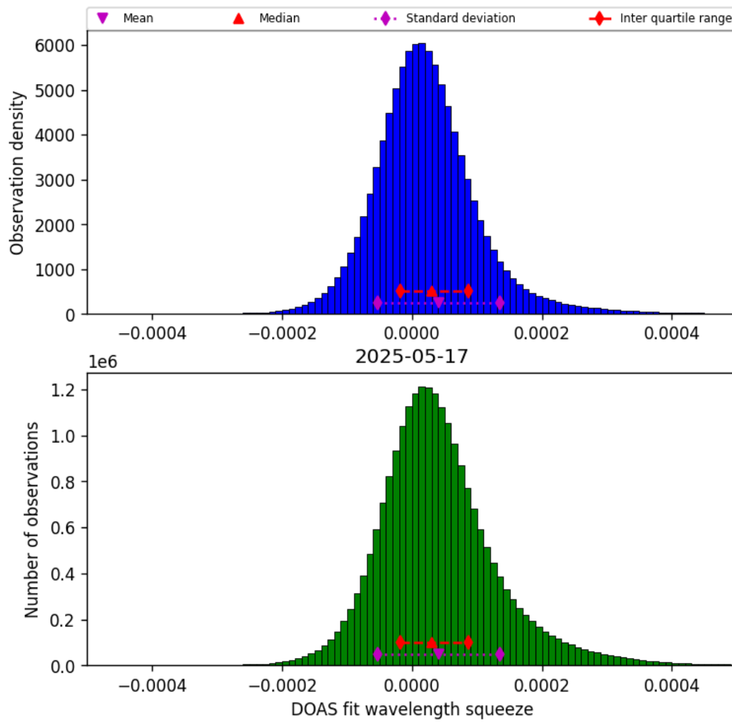
Figure 43: Histogram of “DOAS fit wavelength squeeze” for 2025-05-17 to 2025-05-18
