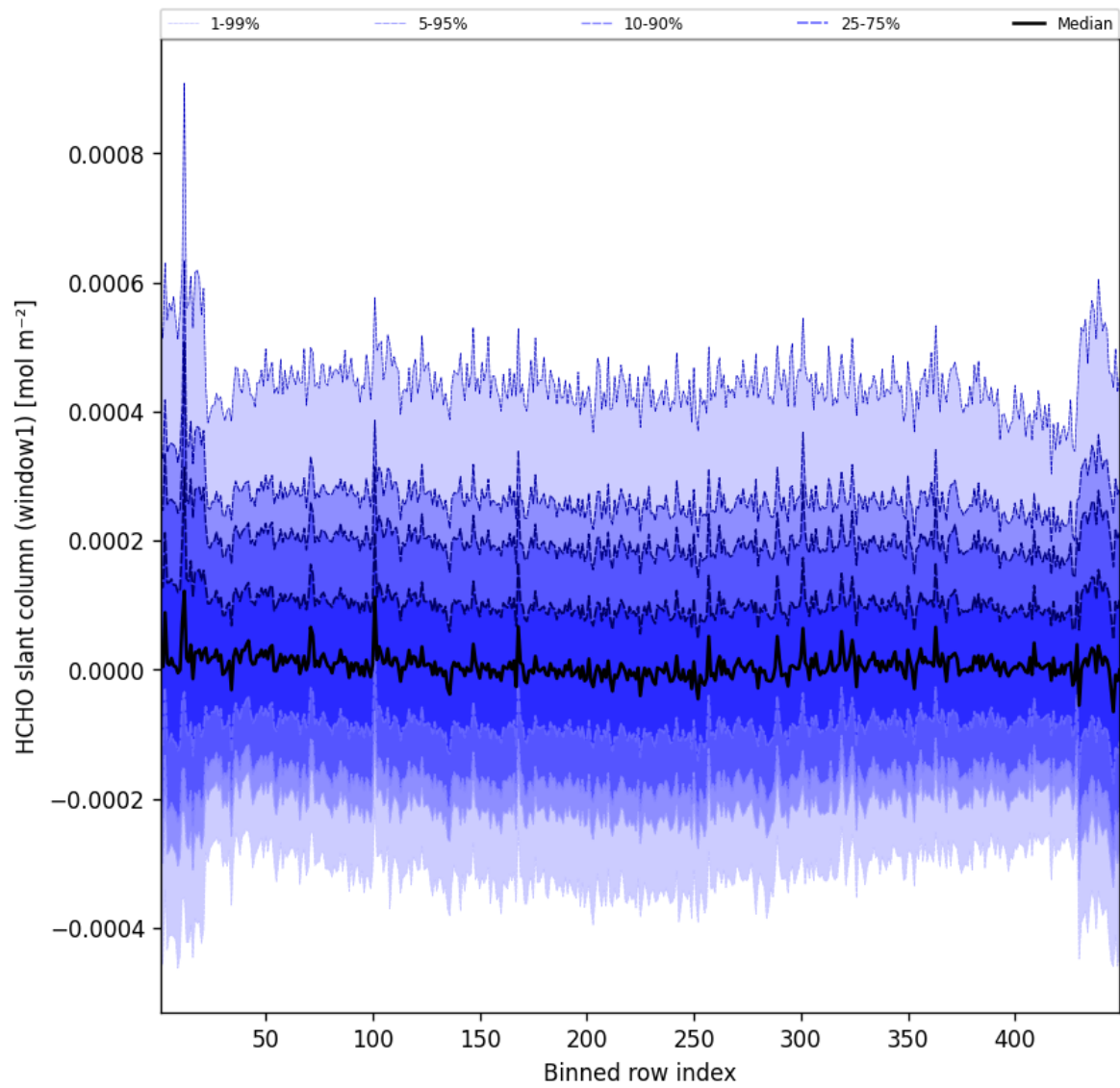
Figure 50: Along track statistics of “HCHO slant column (window1)” for 2025-05-17 to 2025-05-18
