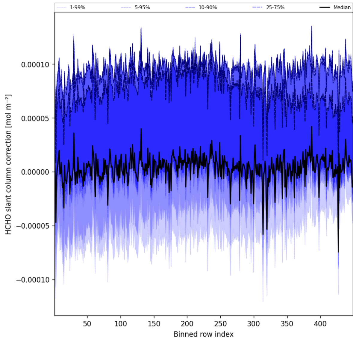
Figure 59: Along track statistics of “HCHO slant column correction” for 2025-05-17 to 2025-05-18
