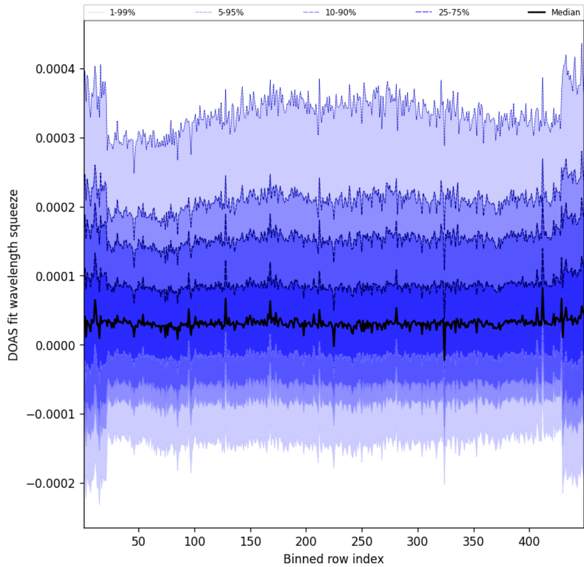
Figure 57: Along track statistics of “DOAS fit wavelength squeeze” for 2025-05-17 to 2025-05-18
