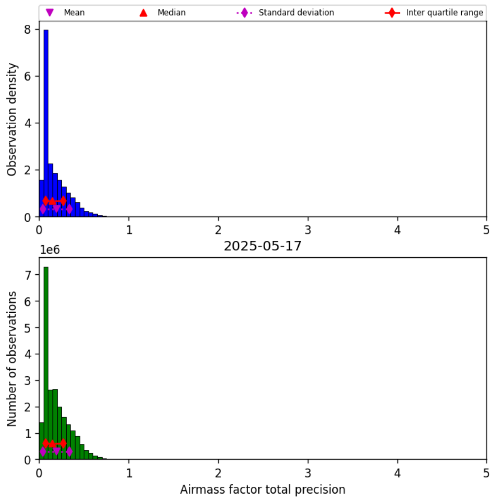
Figure 39: Histogram of “Airmass factor total precision” for 2025-05-17 to 2025-05-18
