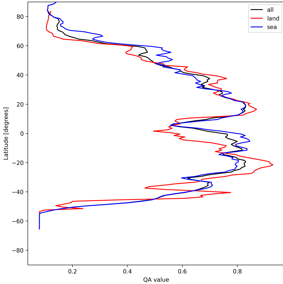
Figure 18: Zonal average of “QA value” for 2025-05-17 to 2025-05-18.
