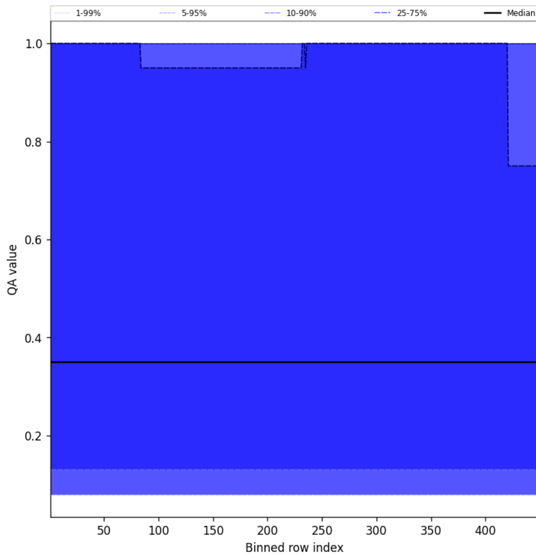
Figure 46: Along track statistics of “QA value” for 2025-05-17 to 2025-05-18
