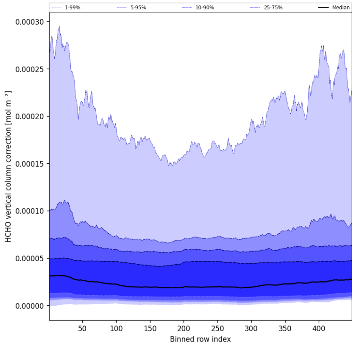
Figure 49: Along track statistics of “HCHO vertical column correction” for 2025-05-17 to 2025-05-18
