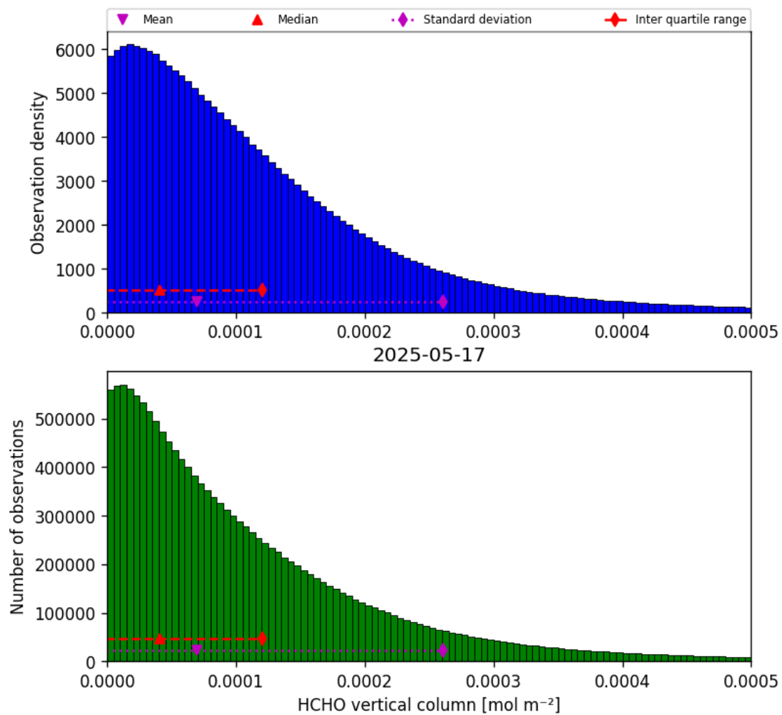
Figure 33: Histogram of “HCHO vertical column” for 2025-05-17 to 2025-05-18
