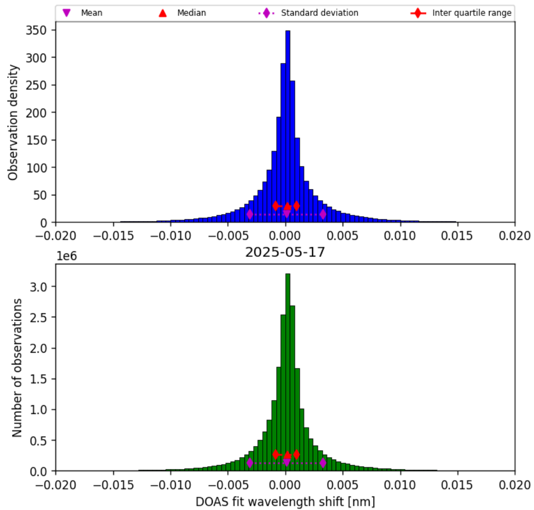
Figure 42: Histogram of “DOAS fit wavelength shift” for 2025-05-17 to 2025-05-18
