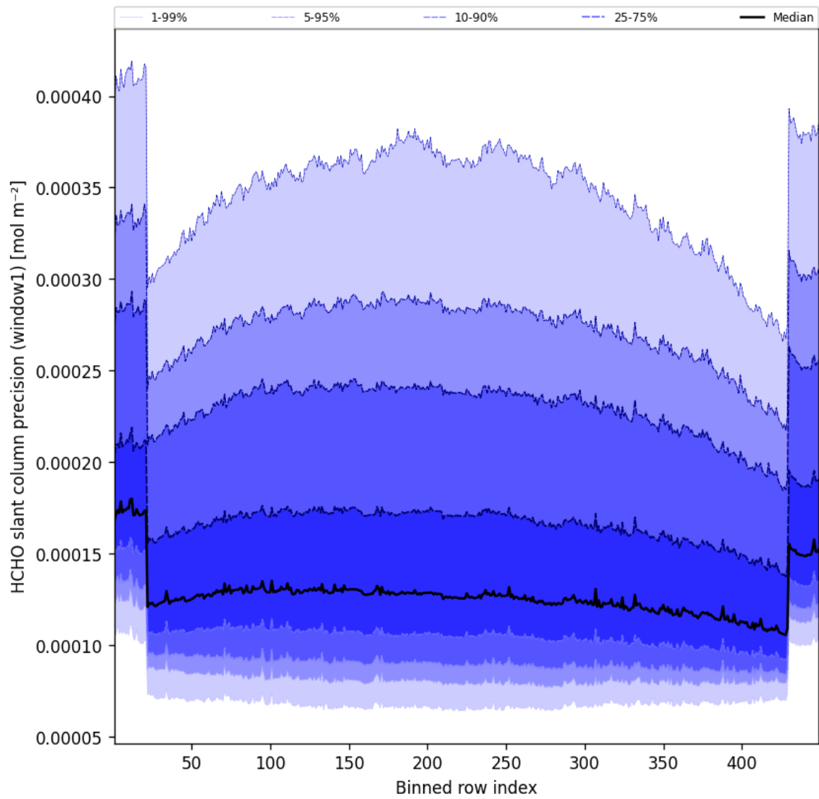
Figure 51: Along track statistics of “HCHO slant column precision (window1)” for 2025-05-17 to 2025-05-18
