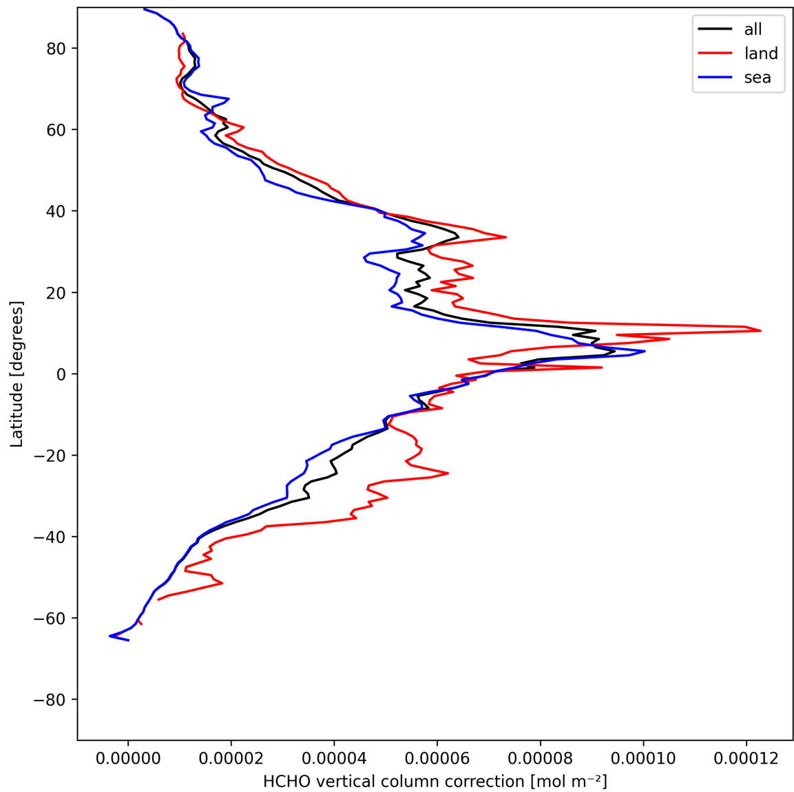
Figure 21: Zonal average of “HCHO vertical column correction” for 2025-05-17 to 2025-05-18.
