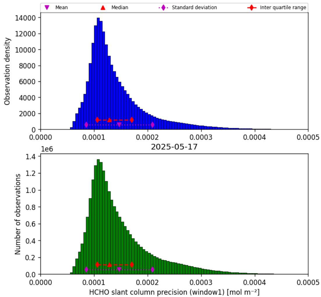
Figure 37: Histogram of “HCHO slant column precision (window1)” for 2025-05-17 to 2025-05-18
