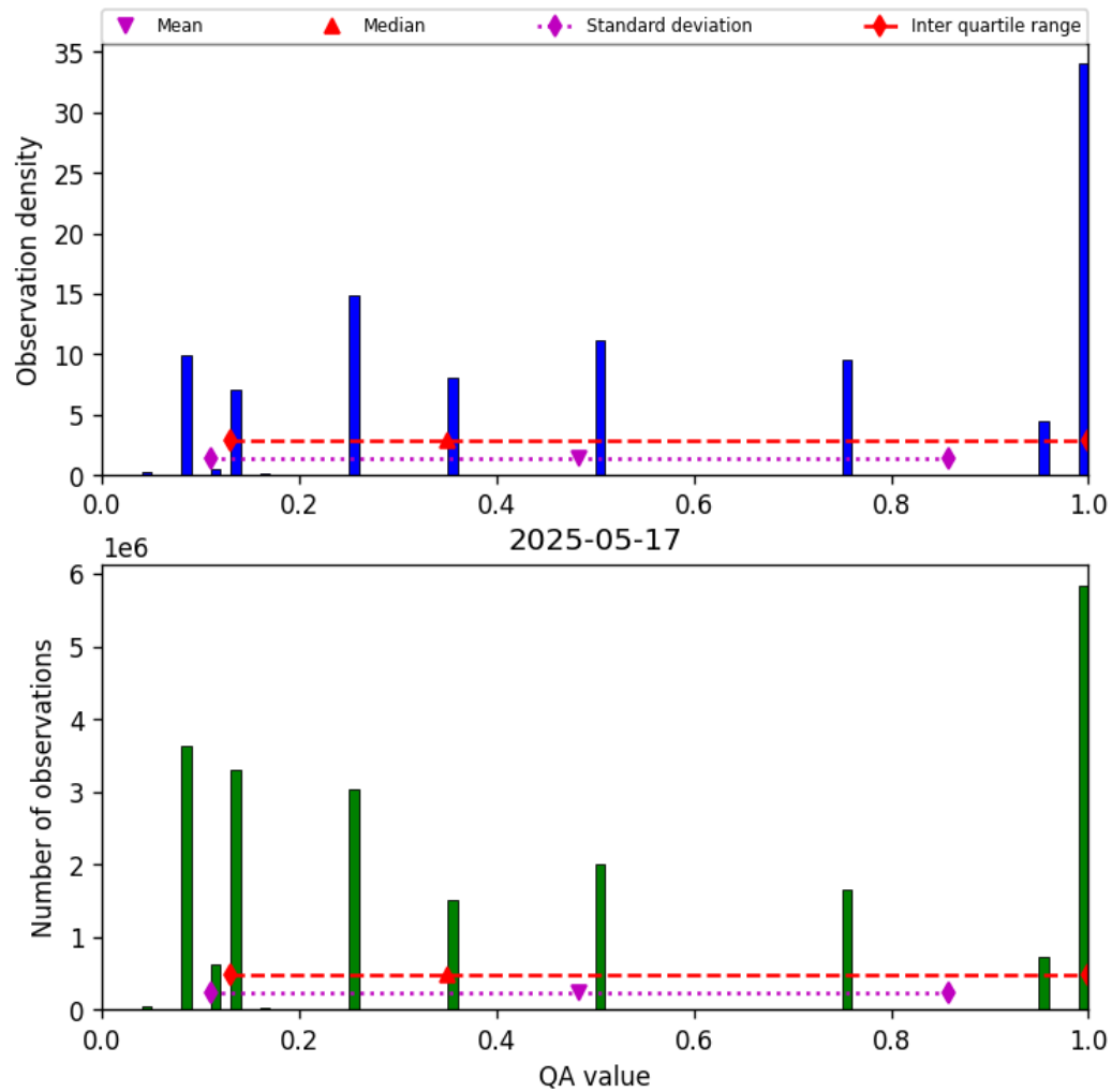
Figure 32: Histogram of “QA value” for 2025-05-17 to 2025-05-18
