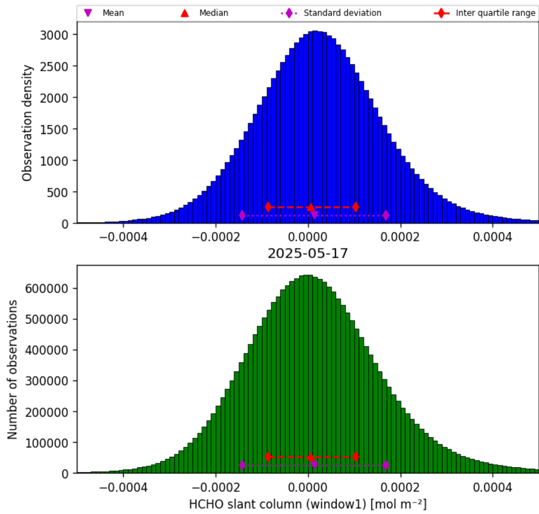
Figure 36: Histogram of “HCHO slant column (window1)” for 2025-05-17 to 2025-05-18
