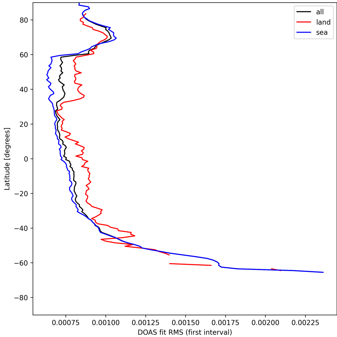
Figure 30: Zonal average of “DOAS fit RMS (first interval)” for 2025-05-17 to 2025-05-18.
