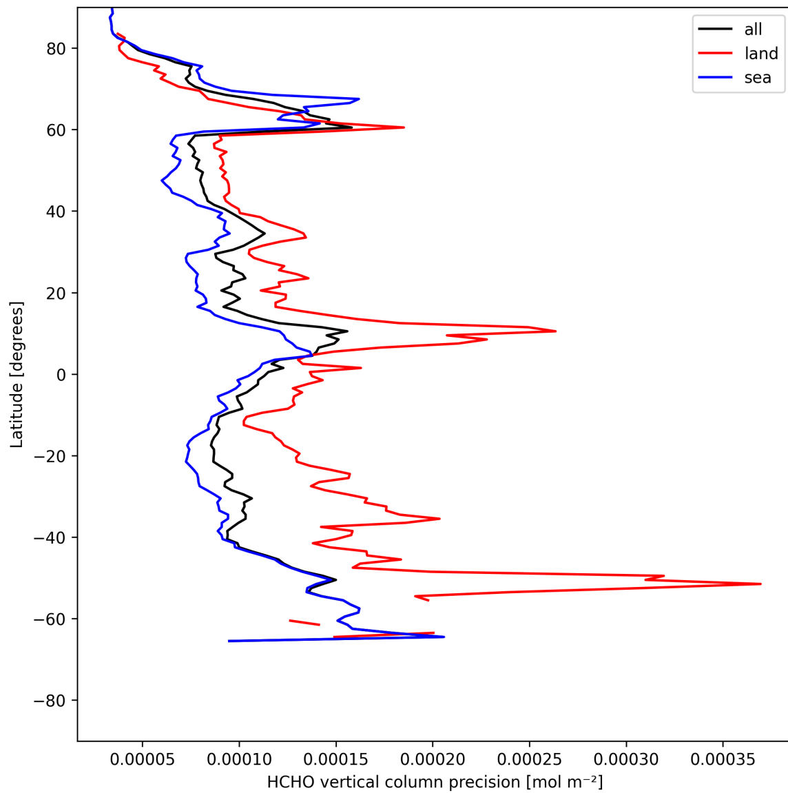
Figure 20: Zonal average of “HCHO vertical column precision” for 2025-05-17 to 2025-05-18.
