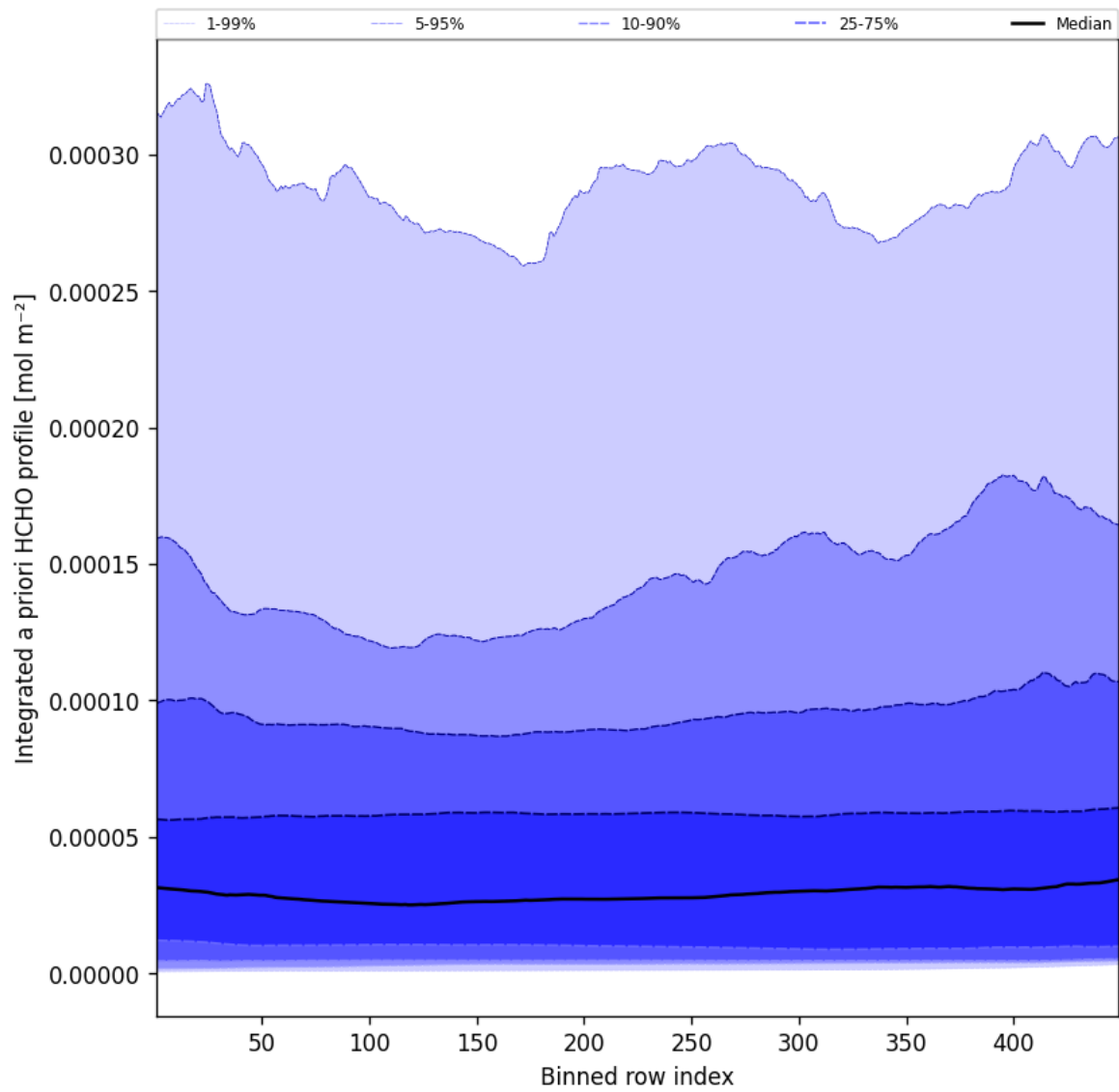
Figure 55: Along track statistics of “Integrated a priori HCHO profile” for 2025-05-17 to 2025-05-18
