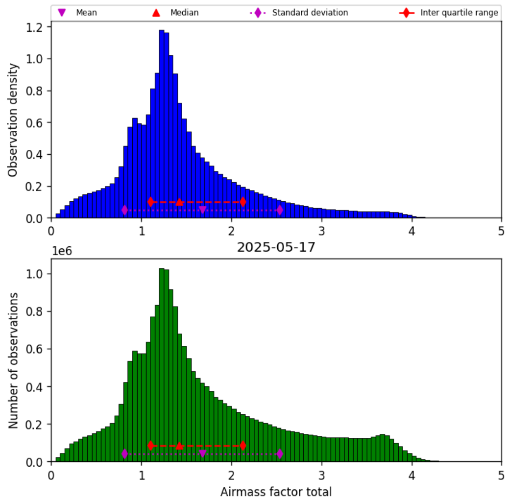
Figure 38: Histogram of “Airmass factor total” for 2025-05-17 to 2025-05-18
