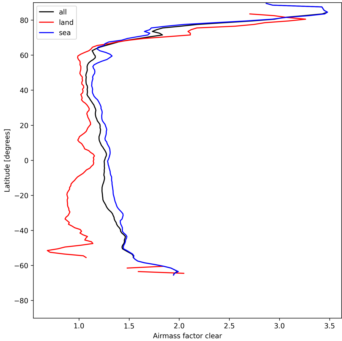
Figure 26: Zonal average of “Airmass factor clear” for 2025-05-17 to 2025-05-18.
