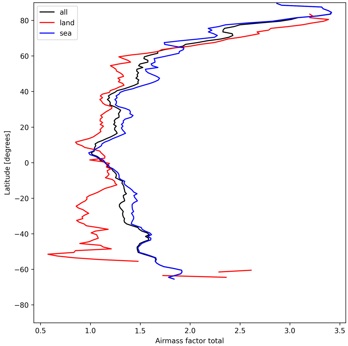
Figure 24: Zonal average of “Airmass factor total” for 2025-05-17 to 2025-05-18.
