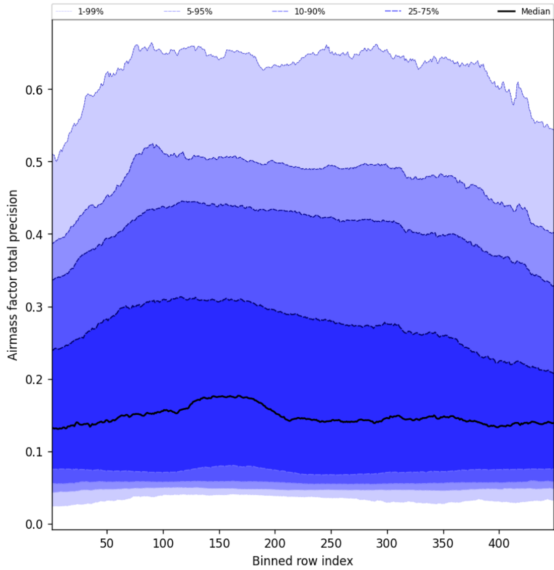
Figure 53: Along track statistics of “Airmass factor total precision” for 2025-05-17 to 2025-05-18
