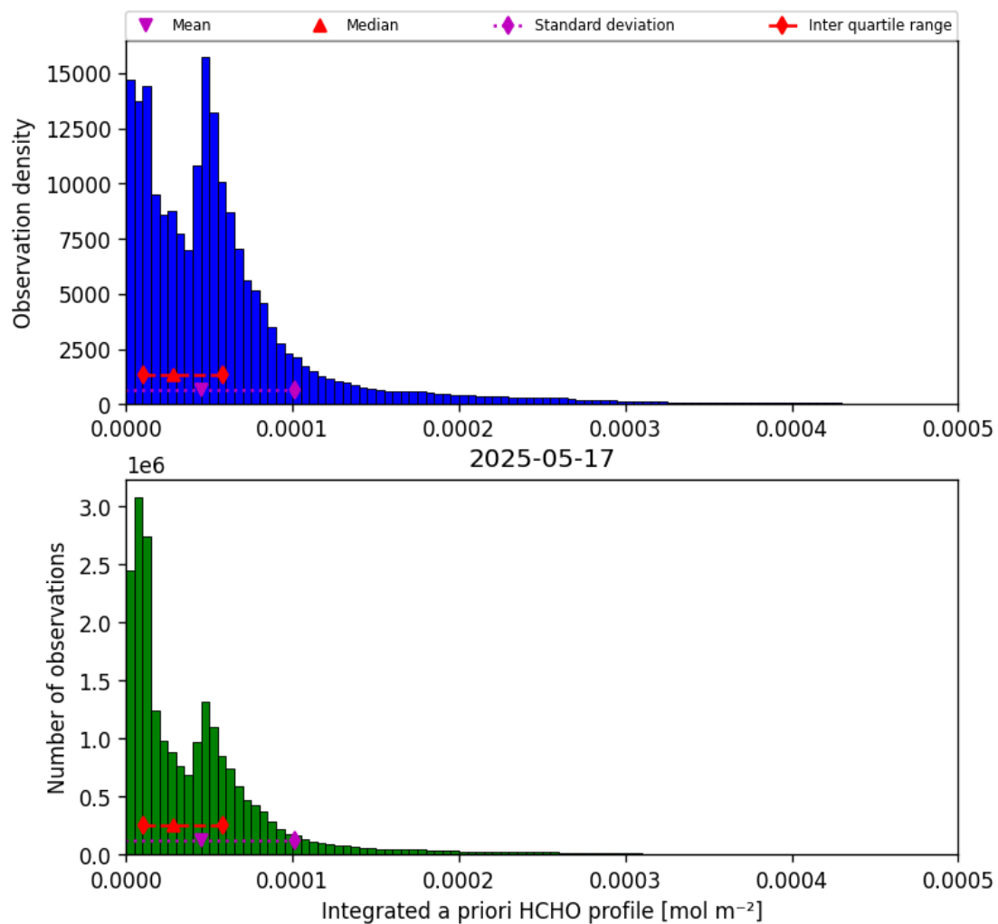
Figure 41: Histogram of “Integrated a priori HCHO profile” for 2025-05-17 to 2025-05-18
