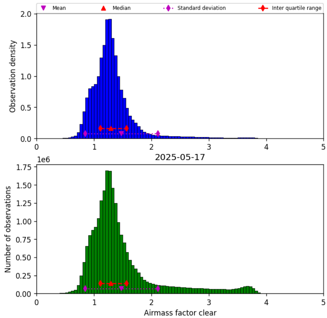
Figure 40: Histogram of “Airmass factor clear” for 2025-05-17 to 2025-05-18
