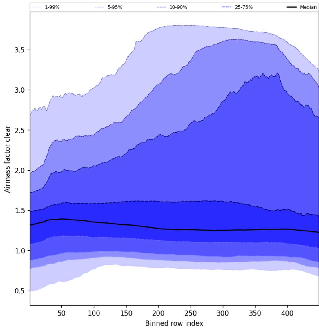
Figure 54: Along track statistics of “Airmass factor clear” for 2025-05-17 to 2025-05-18
