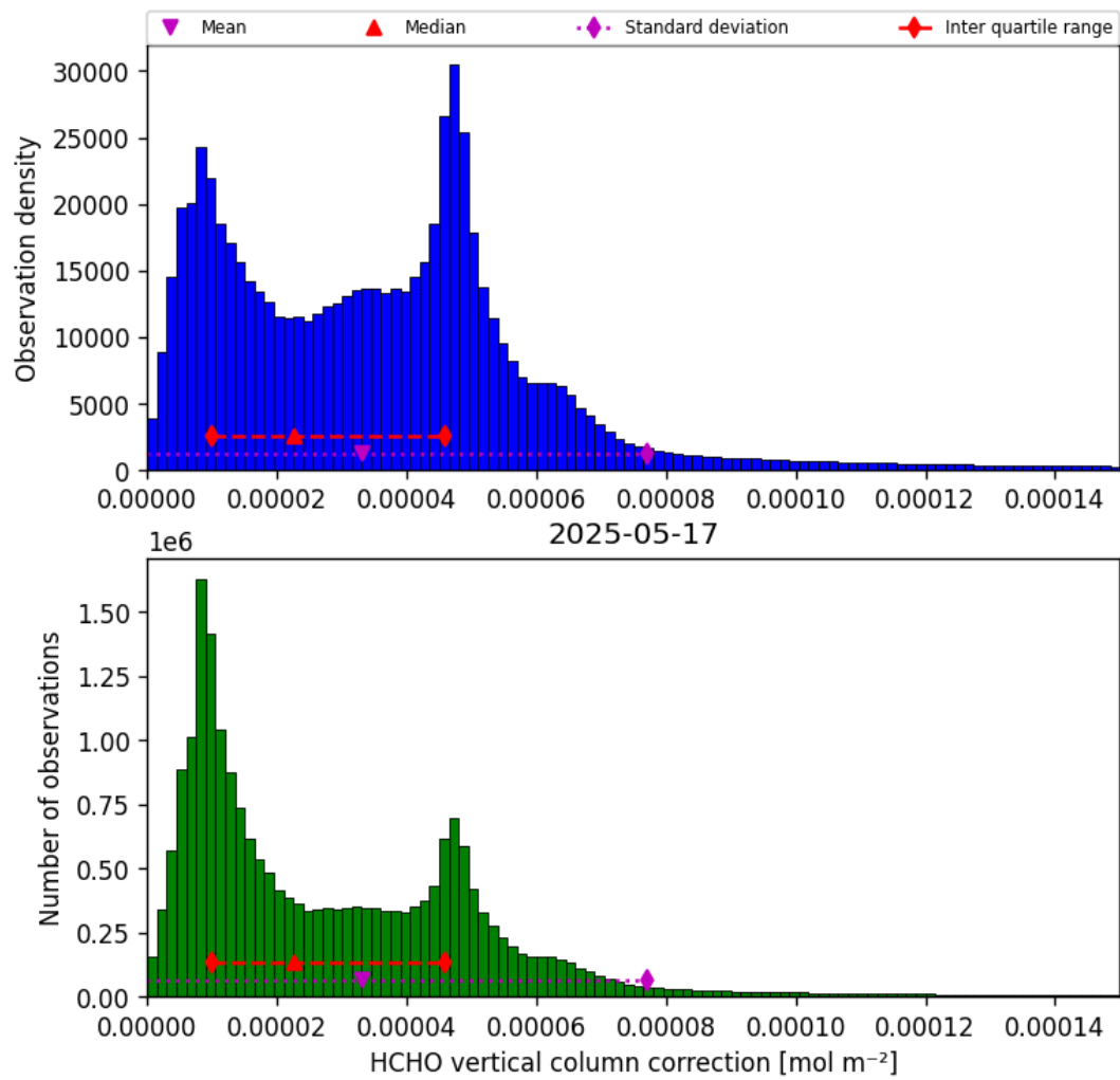
Figure 35: Histogram of “HCHO vertical column correction” for 2025-05-17 to 2025-05-18
