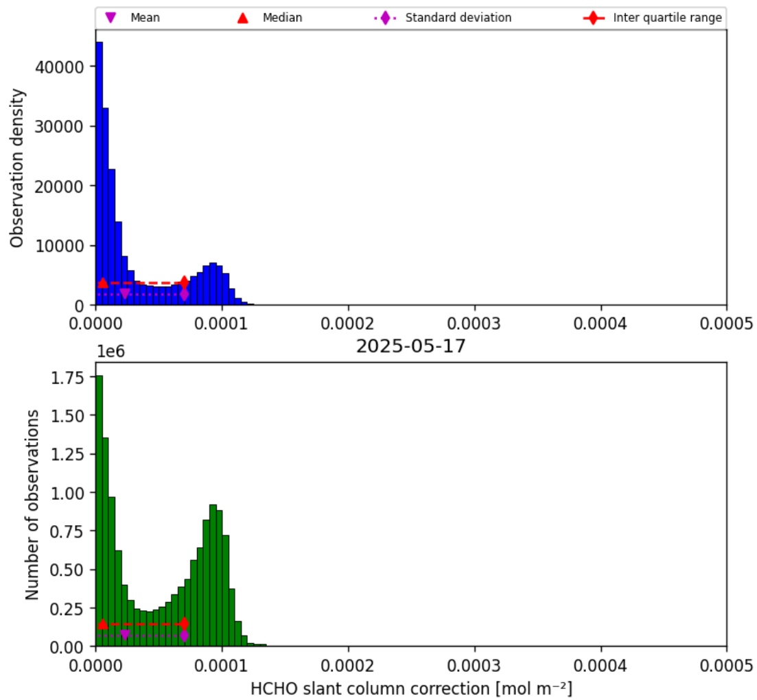
Figure 45: Histogram of “HCHO slant column correction” for 2025-05-17 to 2025-05-18
