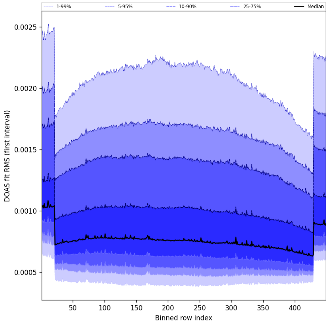
Figure 58: Along track statistics of “DOAS fit RMS (first interval)” for 2025-05-17 to 2025-05-18
