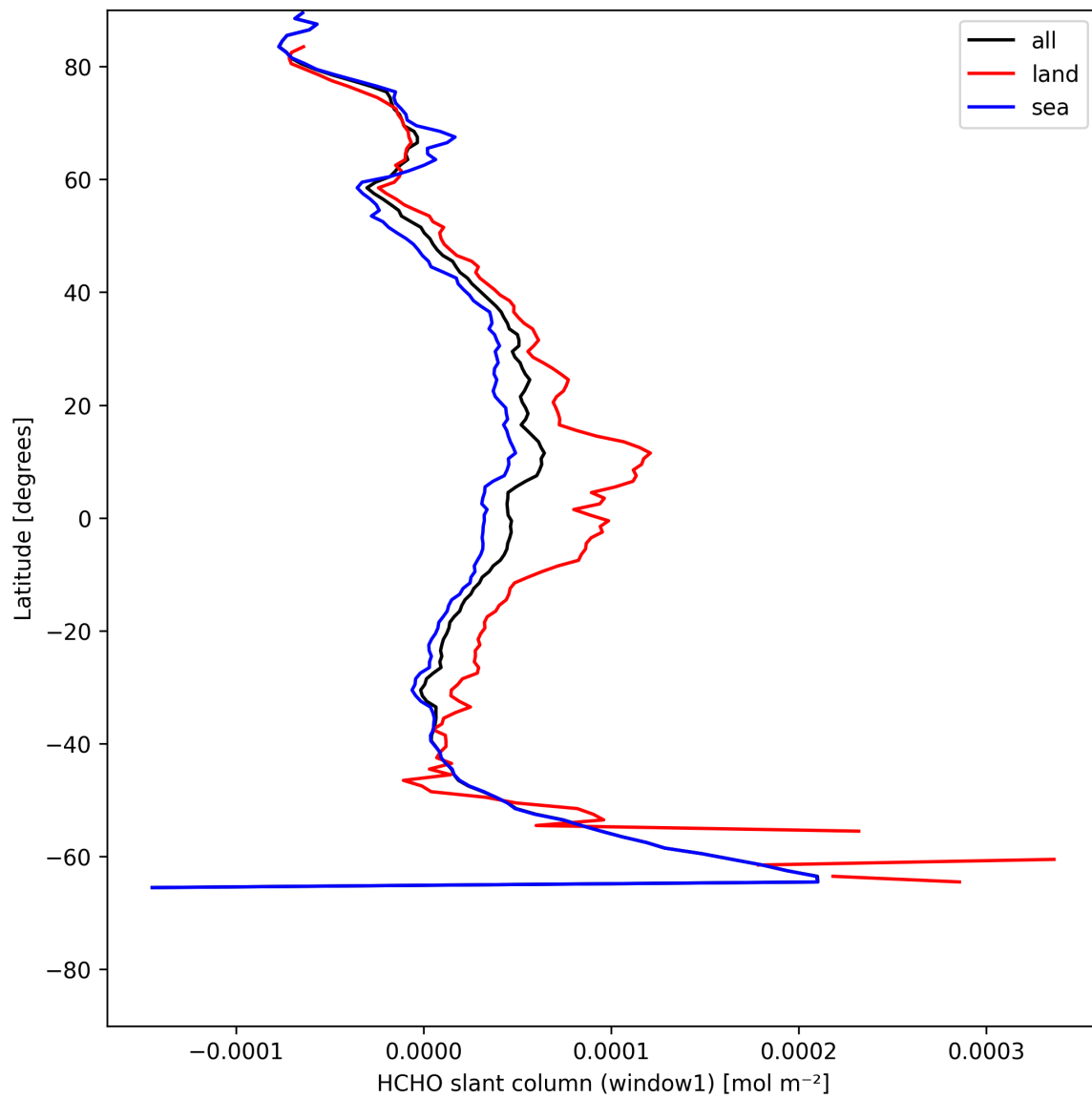
Figure 22: Zonal average of “HCHO slant column (window1)” for 2025-05-17 to 2025-05-18.
