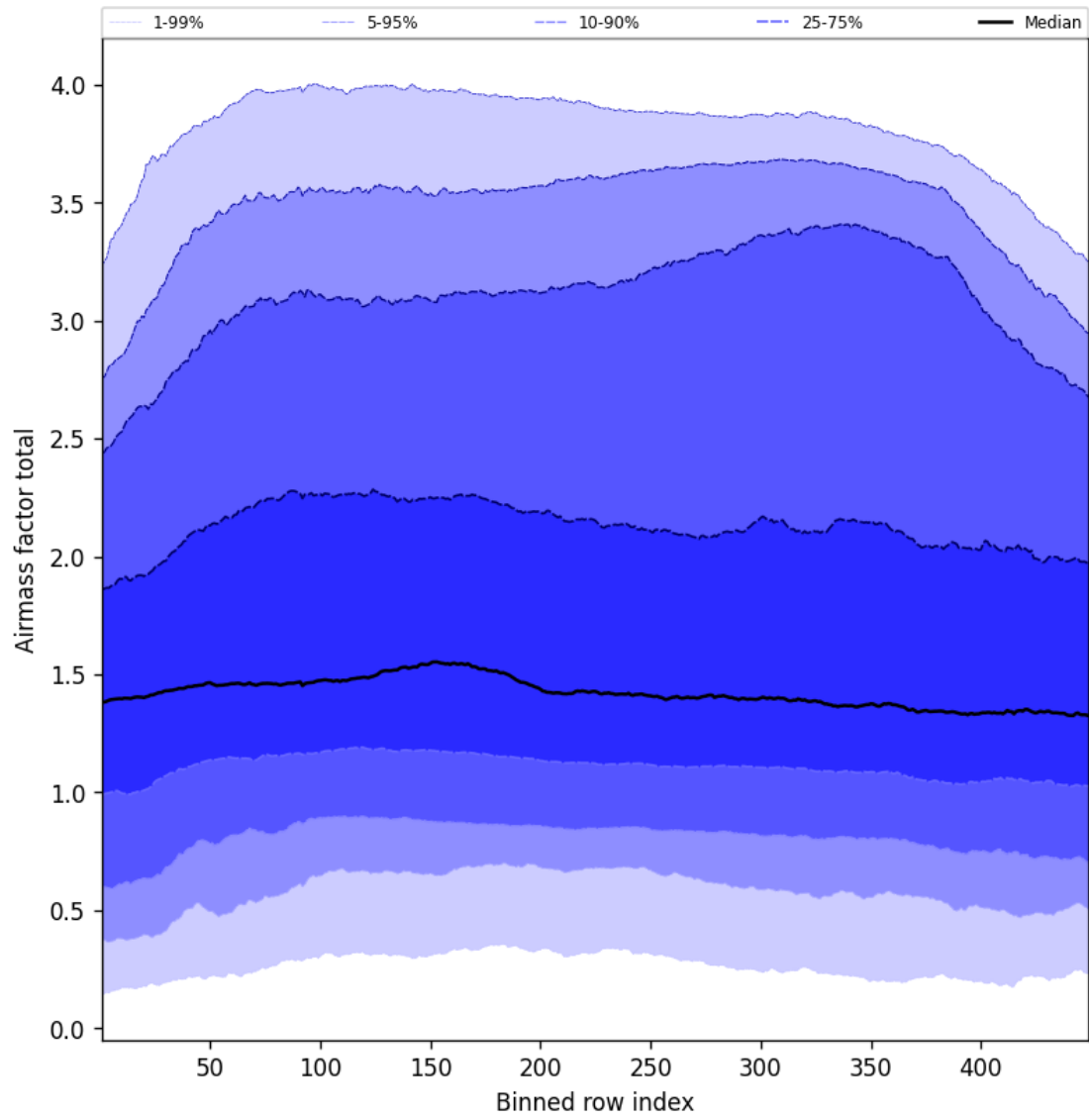
Figure 52: Along track statistics of “Airmass factor total” for 2025-05-17 to 2025-05-18
