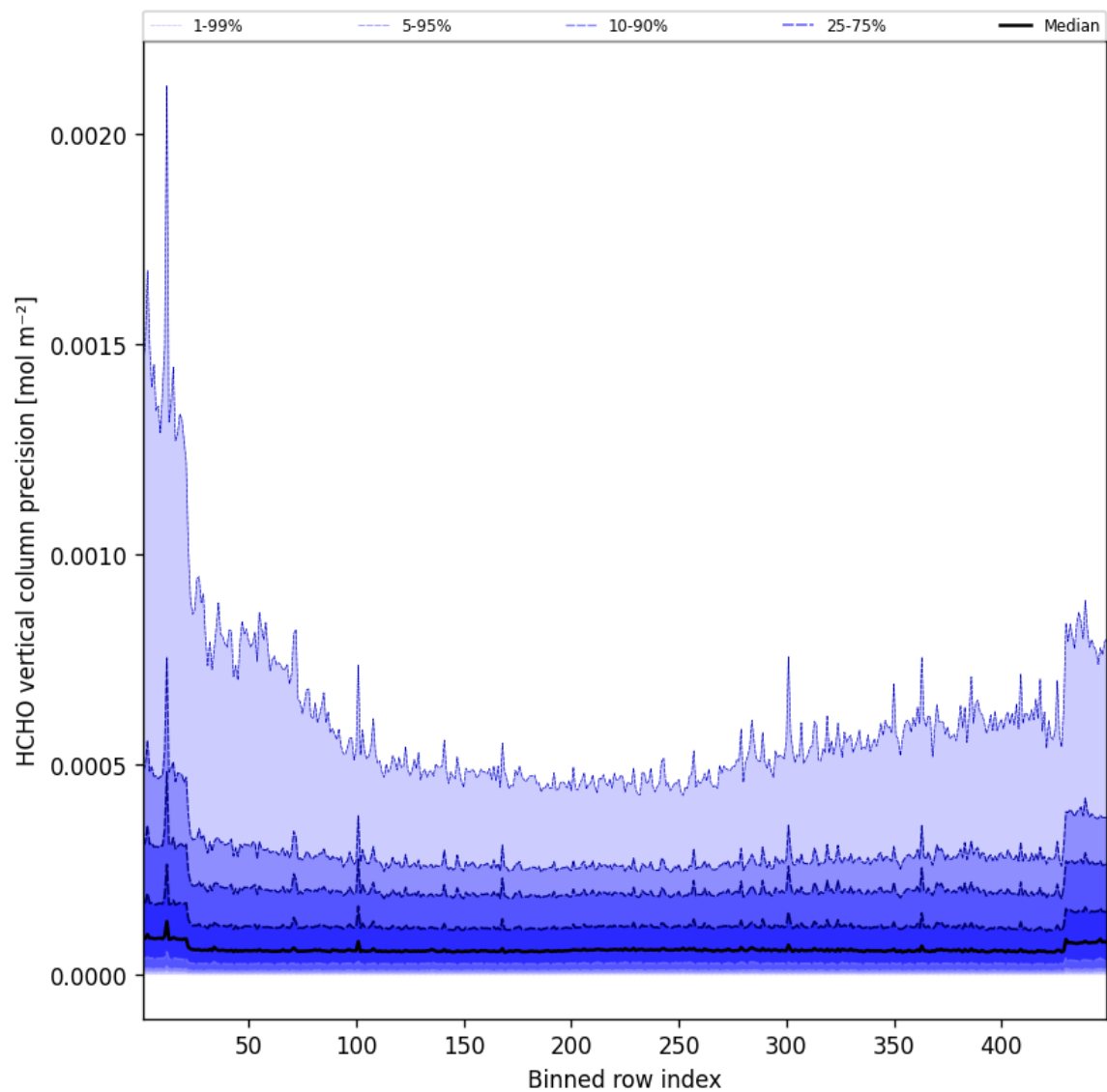
Figure 48: Along track statistics of “HCHO vertical column precision” for 2025-05-17 to 2025-05-18
