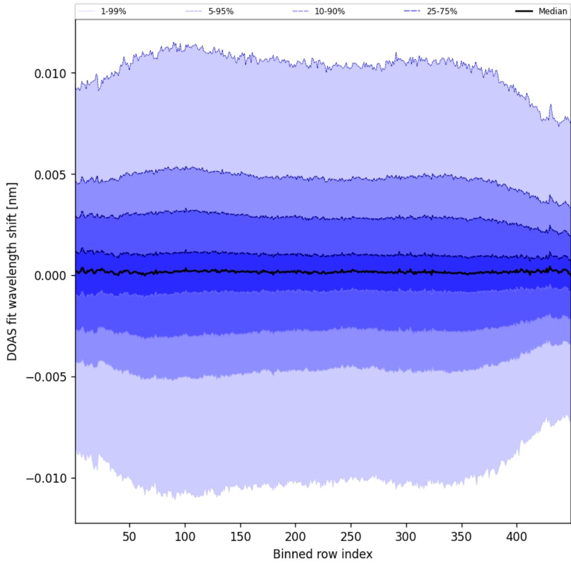
Figure 56: Along track statistics of “DOAS fit wavelength shift” for 2025-05-17 to 2025-05-18
