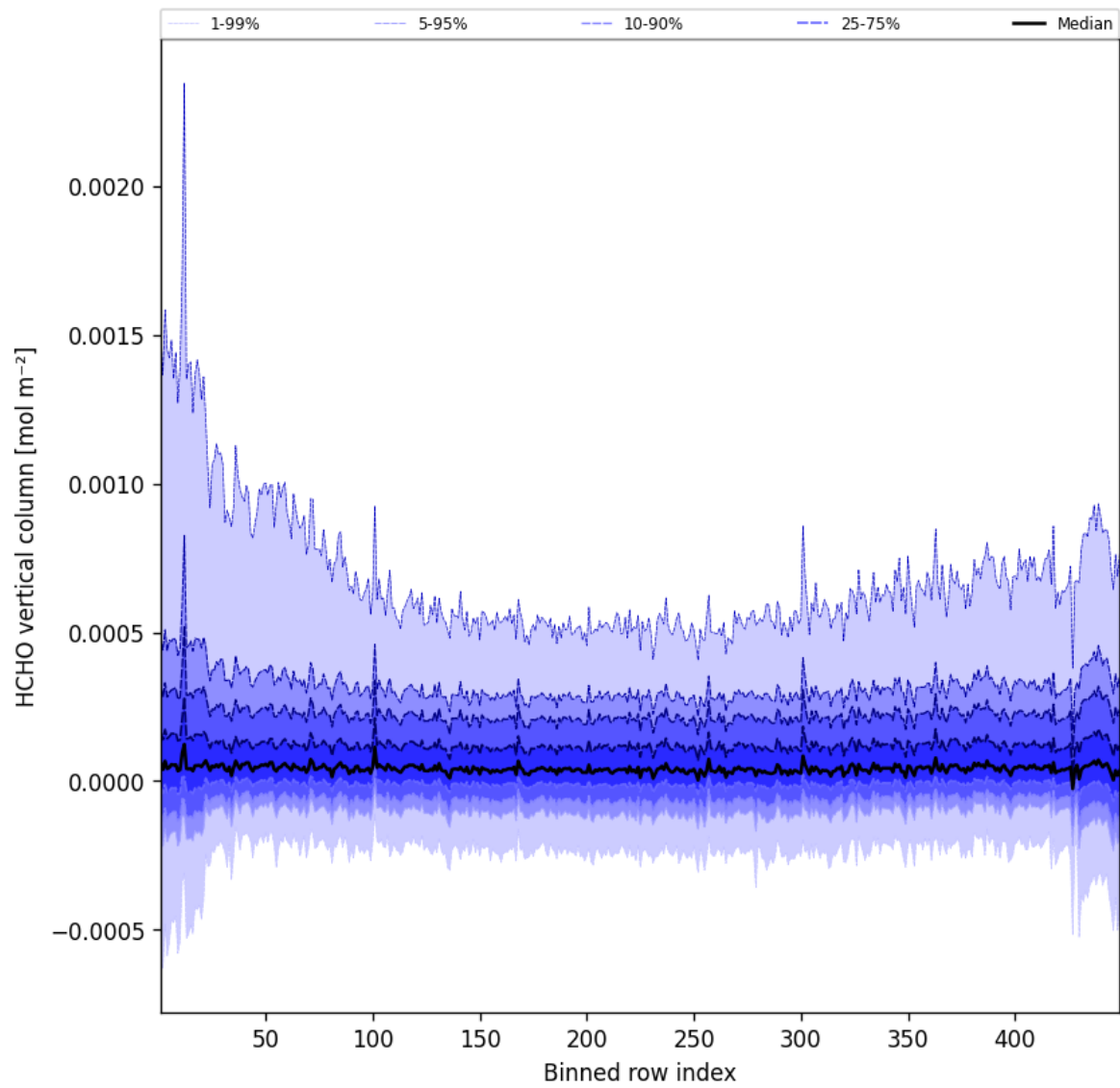
Figure 47: Along track statistics of “HCHO vertical column” for 2025-05-17 to 2025-05-18
