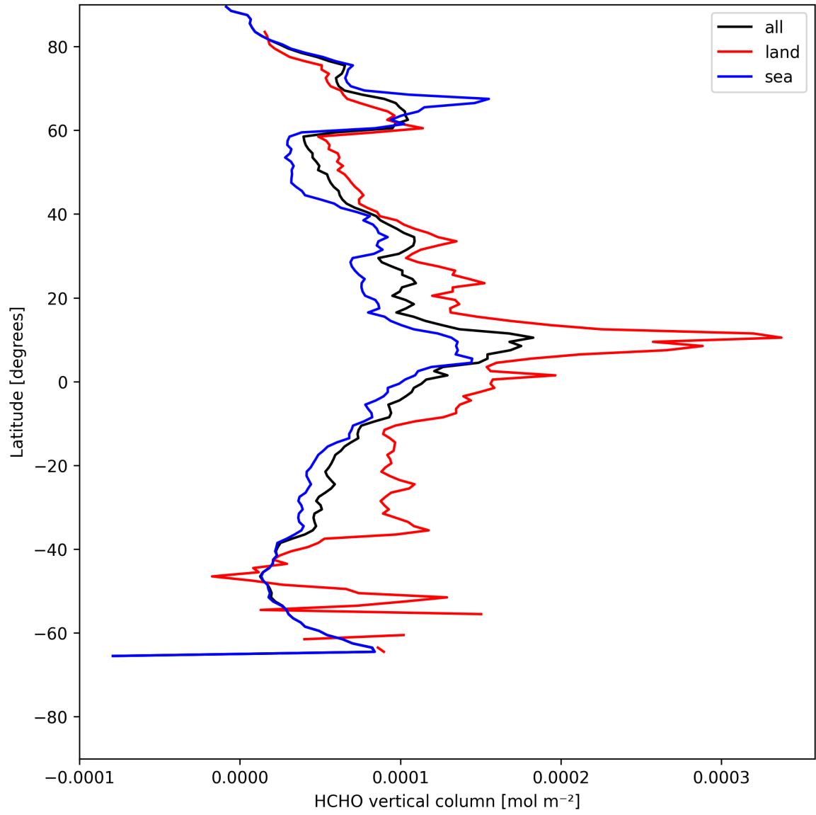
Figure 19: Zonal average of “HCHO vertical column” for 2025-05-17 to 2025-05-18.
