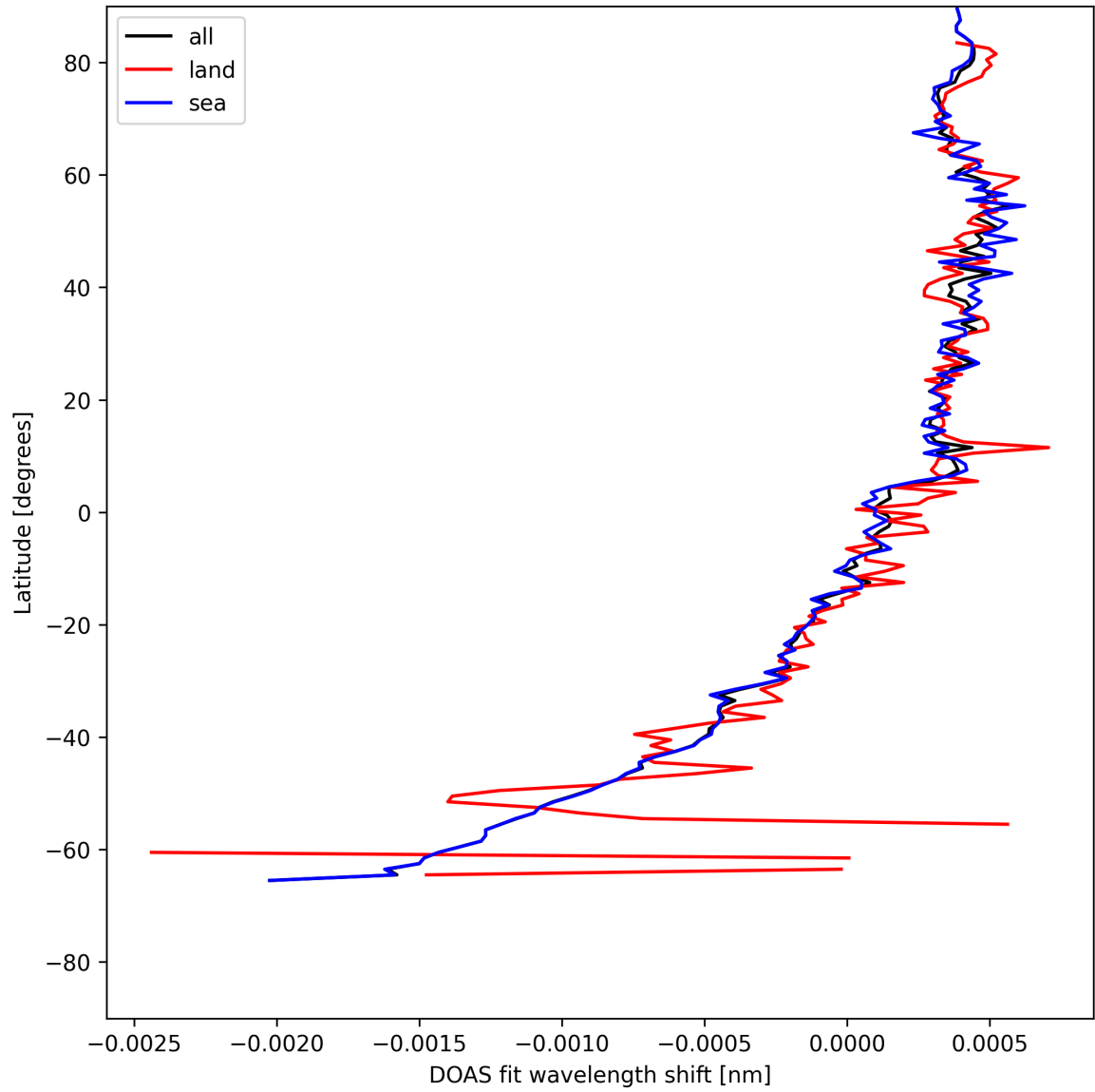
Figure 28: Zonal average of “DOAS fit wavelength shift” for 2025-05-17 to 2025-05-18.
