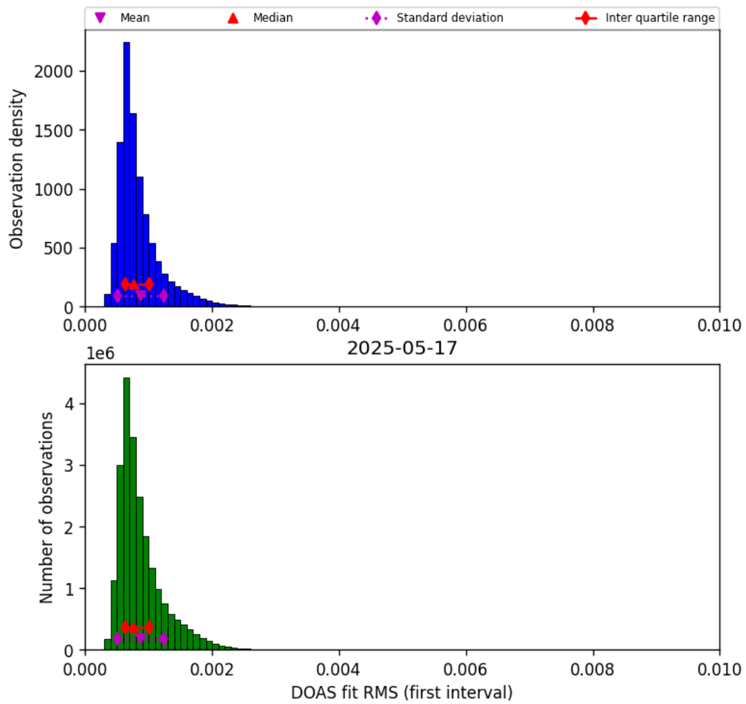
Figure 44: Histogram of "DOAS fit RMS (first interval)" for 2025-05-17 to 2025-05-18
