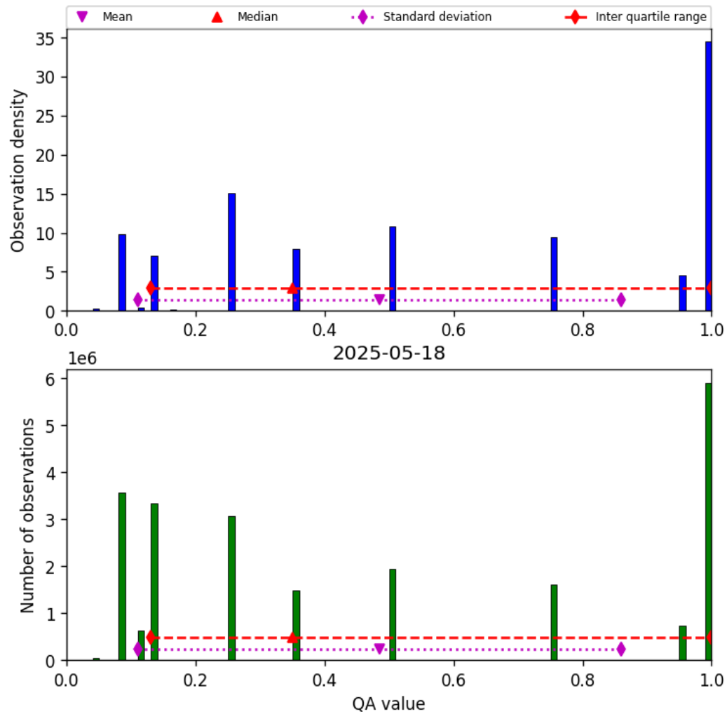
Figure 32: Histogram of “QA value” for 2025-05-18 to 2025-05-19
