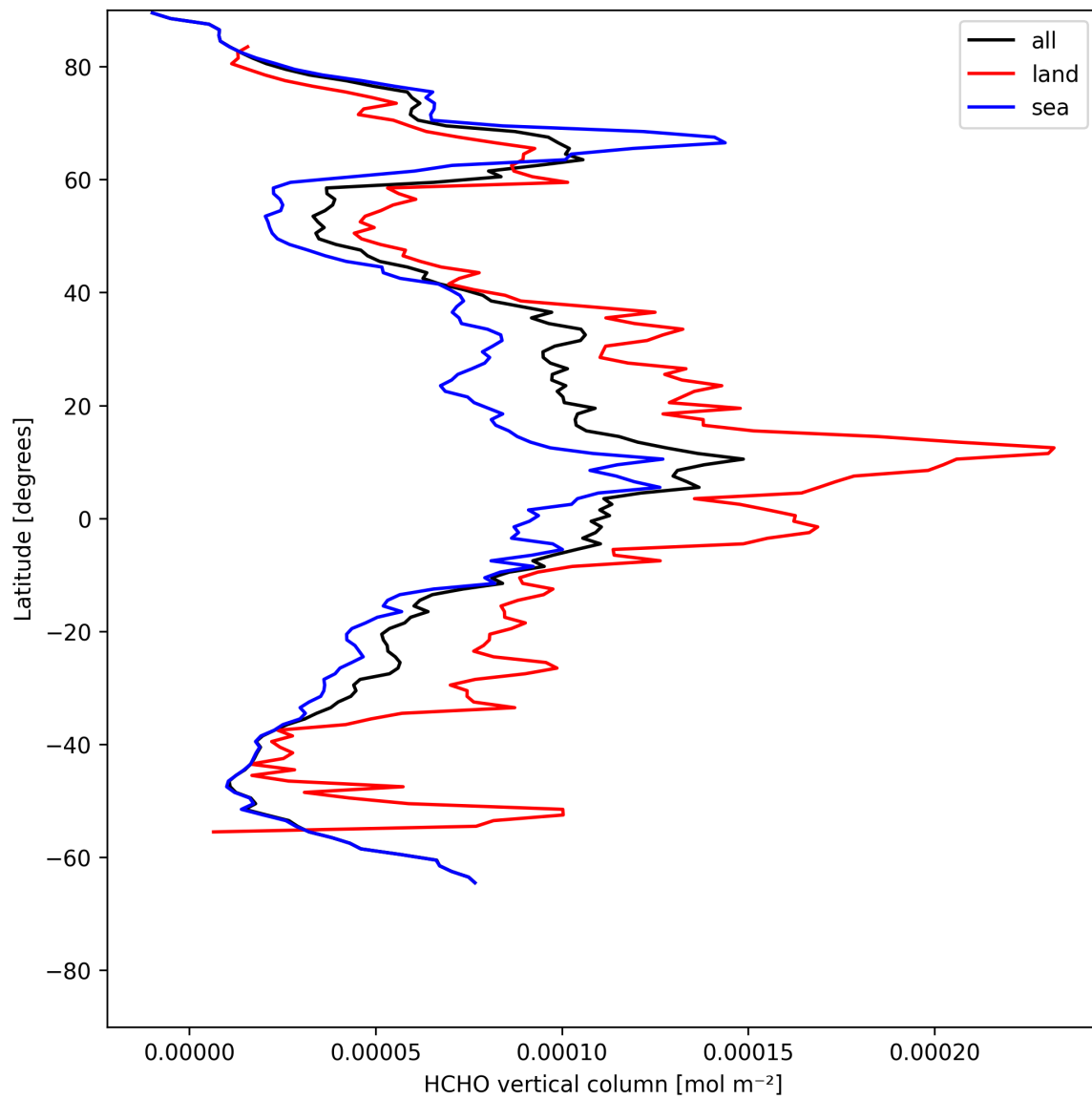
Figure 19: Zonal average of “HCHO vertical column” for 2025-05-18 to 2025-05-19.
