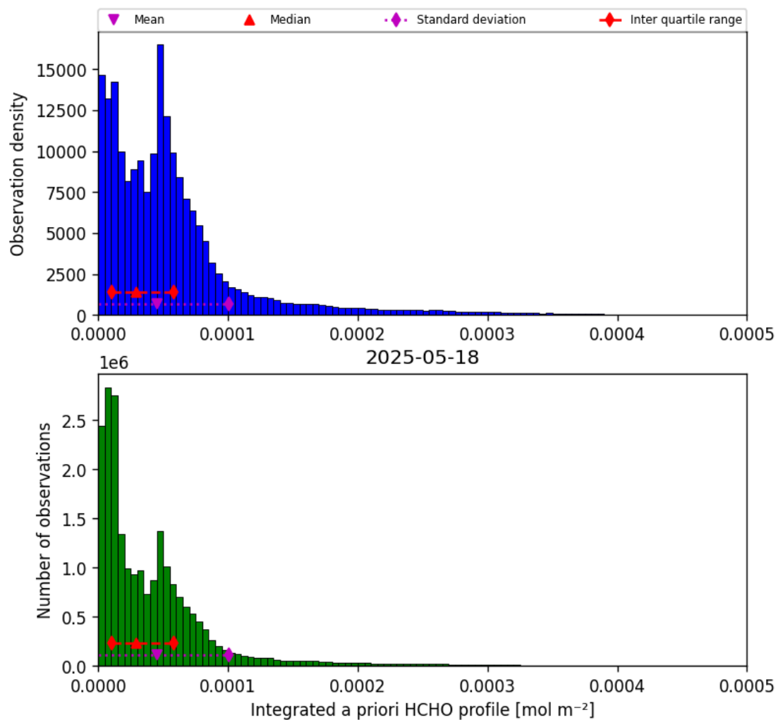
Figure 41: Histogram of “Integrated a priori HCHO profile” for 2025-05-18 to 2025-05-19
