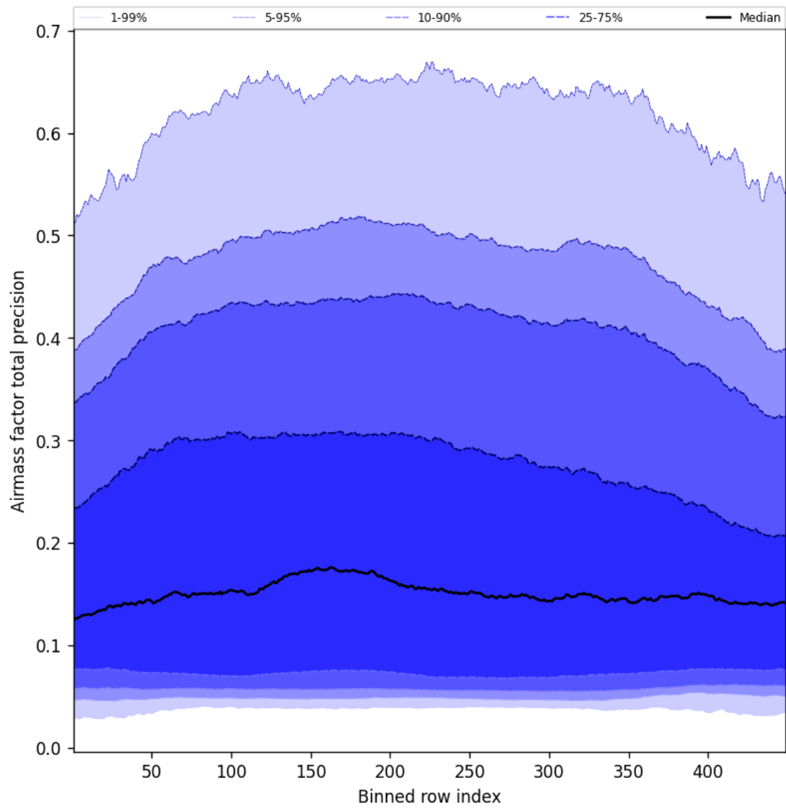
Figure 53: Along track statistics of “Airmass factor total precision” for 2025-05-18 to 2025-05-19
