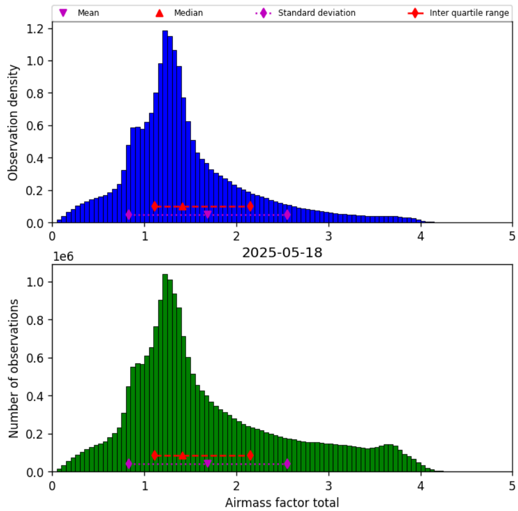
Figure 38: Histogram of “Airmass factor total” for 2025-05-18 to 2025-05-19
