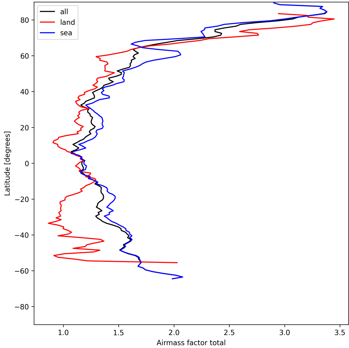
Figure 24: Zonal average of “Airmass factor total” for 2025-05-18 to 2025-05-19.
