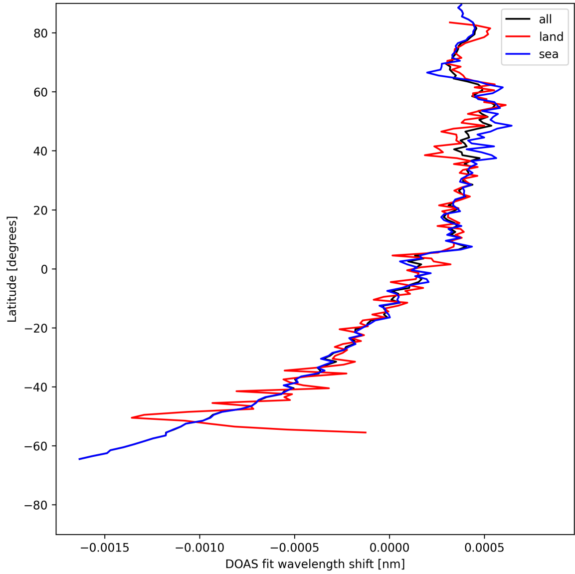
Figure 28: Zonal average of “DOAS fit wavelength shift” for 2025-05-18 to 2025-05-19.
