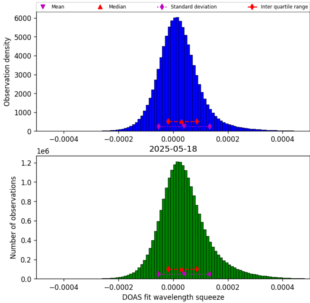
Figure 43: Histogram of “DOAS fit wavelength squeeze” for 2025-05-18 to 2025-05-19
