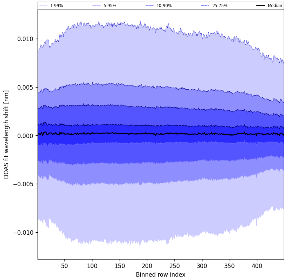
Figure 56: Along track statistics of “DOAS fit wavelength shift” for 2025-05-18 to 2025-05-19
