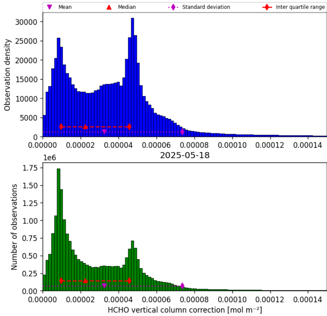
Figure 35: Histogram of “HCHO vertical column correction” for 2025-05-18 to 2025-05-19
