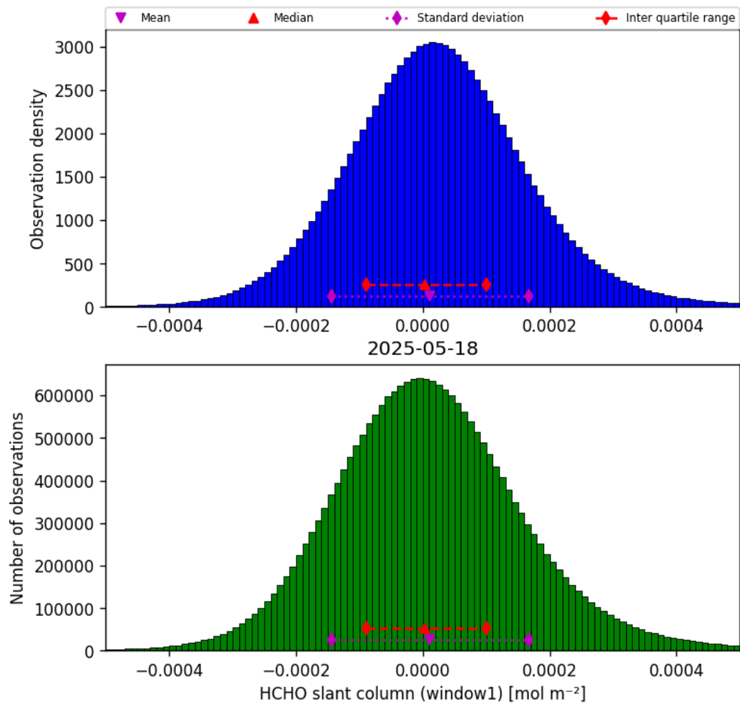
Figure 36: Histogram of “HCHO slant column (window1)” for 2025-05-18 to 2025-05-19
