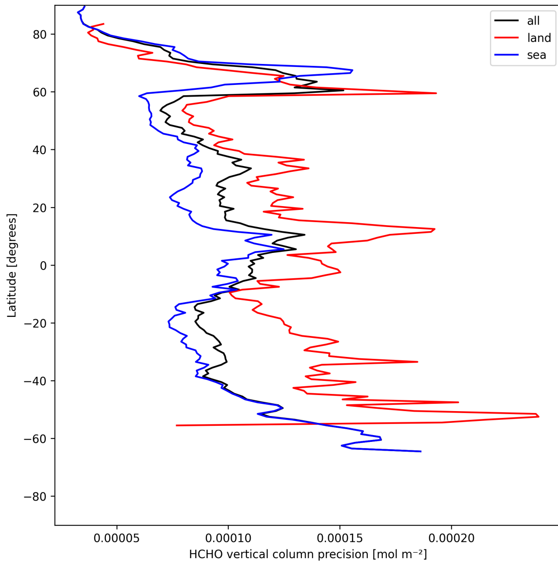
Figure 20: Zonal average of “HCHO vertical column precision” for 2025-05-18 to 2025-05-19.
