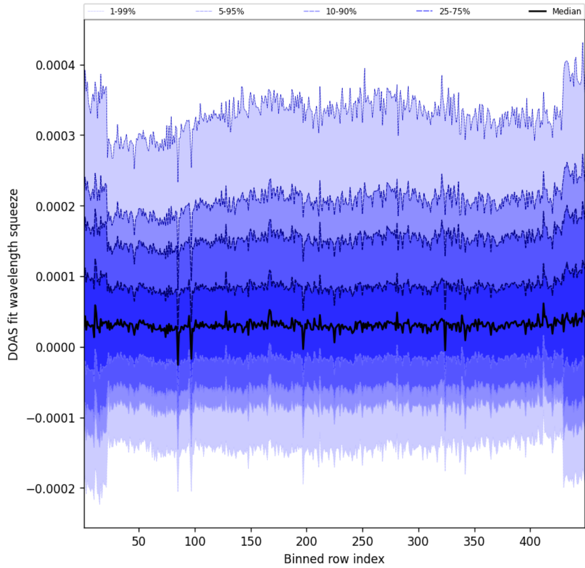
Figure 57: Along track statistics of “DOAS fit wavelength squeeze” for 2025-05-18 to 2025-05-19
