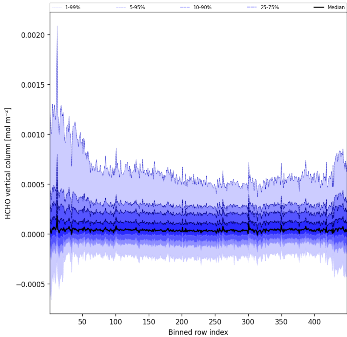
Figure 47: Along track statistics of “HCHO vertical column” for 2025-05-18 to 2025-05-19
