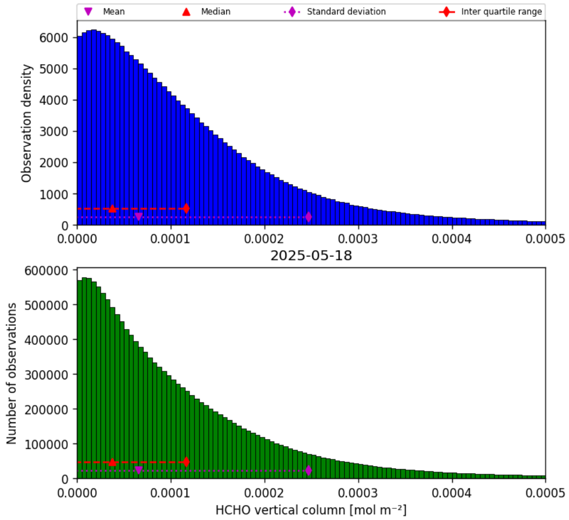
Figure 33: Histogram of “HCHO vertical column” for 2025-05-18 to 2025-05-19
