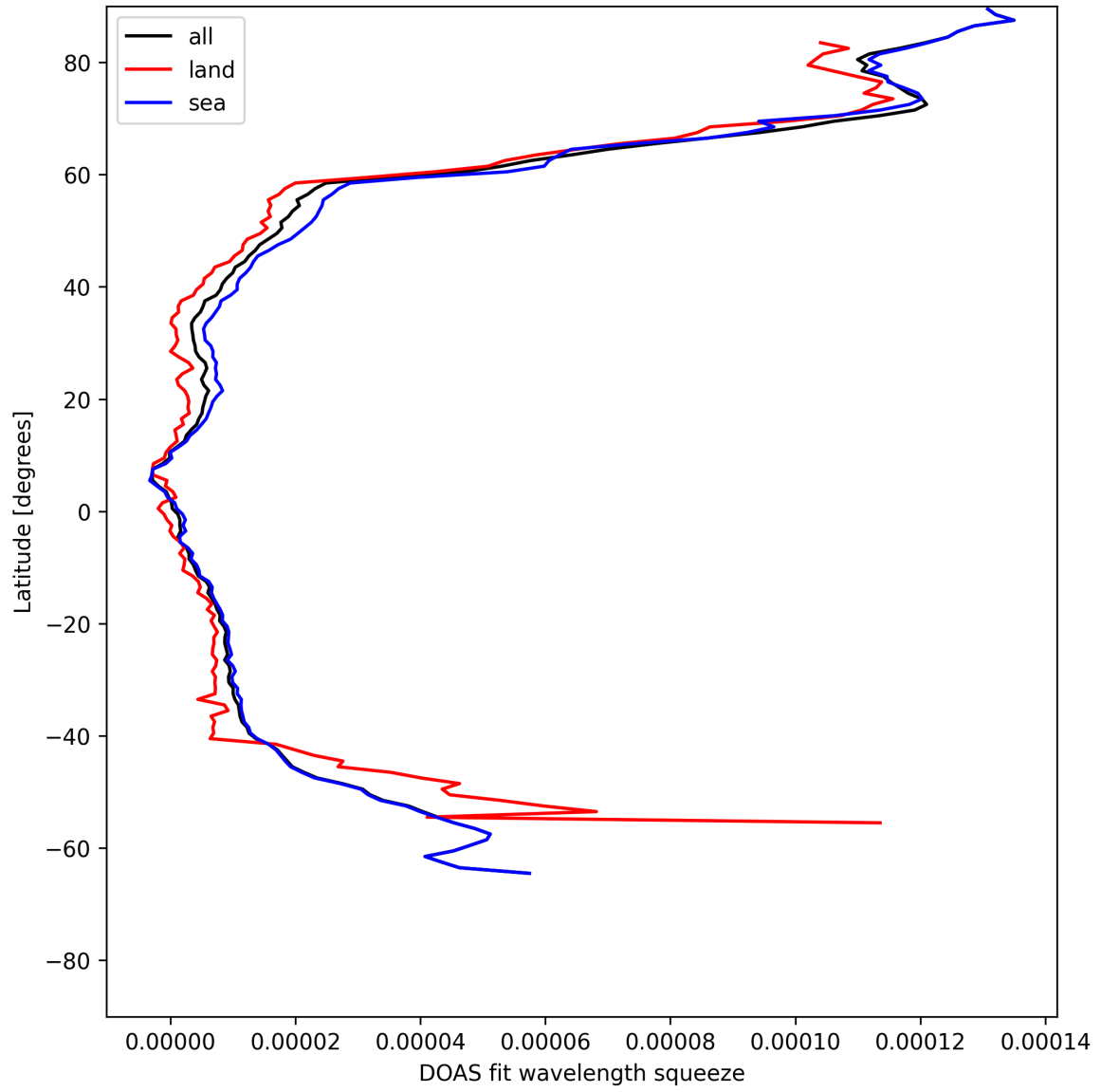
Figure 29: Zonal average of “DOAS fit wavelength squeeze” for 2025-05-18 to 2025-05-19.
