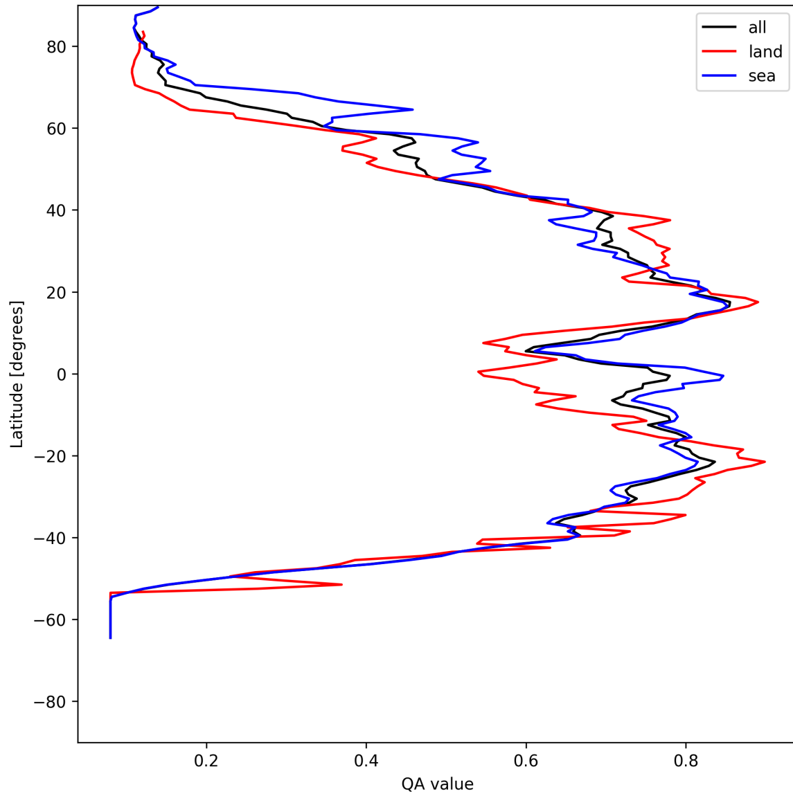
Figure 18: Zonal average of “QA value” for 2025-05-18 to 2025-05-19.
