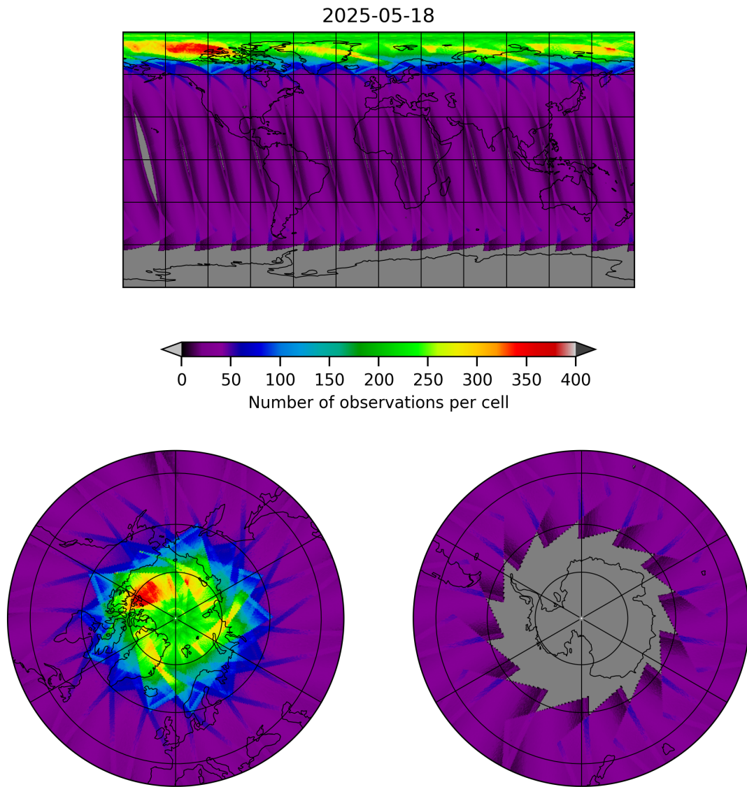
Figure 17: Map of the number of observations for 2025-05-18 to 2025-05-19
