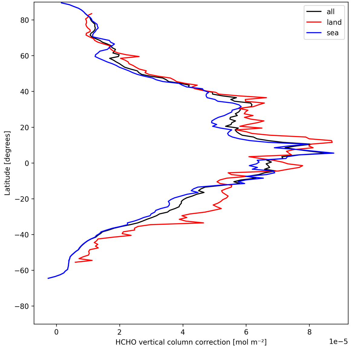
Figure 21: Zonal average of “HCHO vertical column correction” for 2025-05-18 to 2025-05-19.
