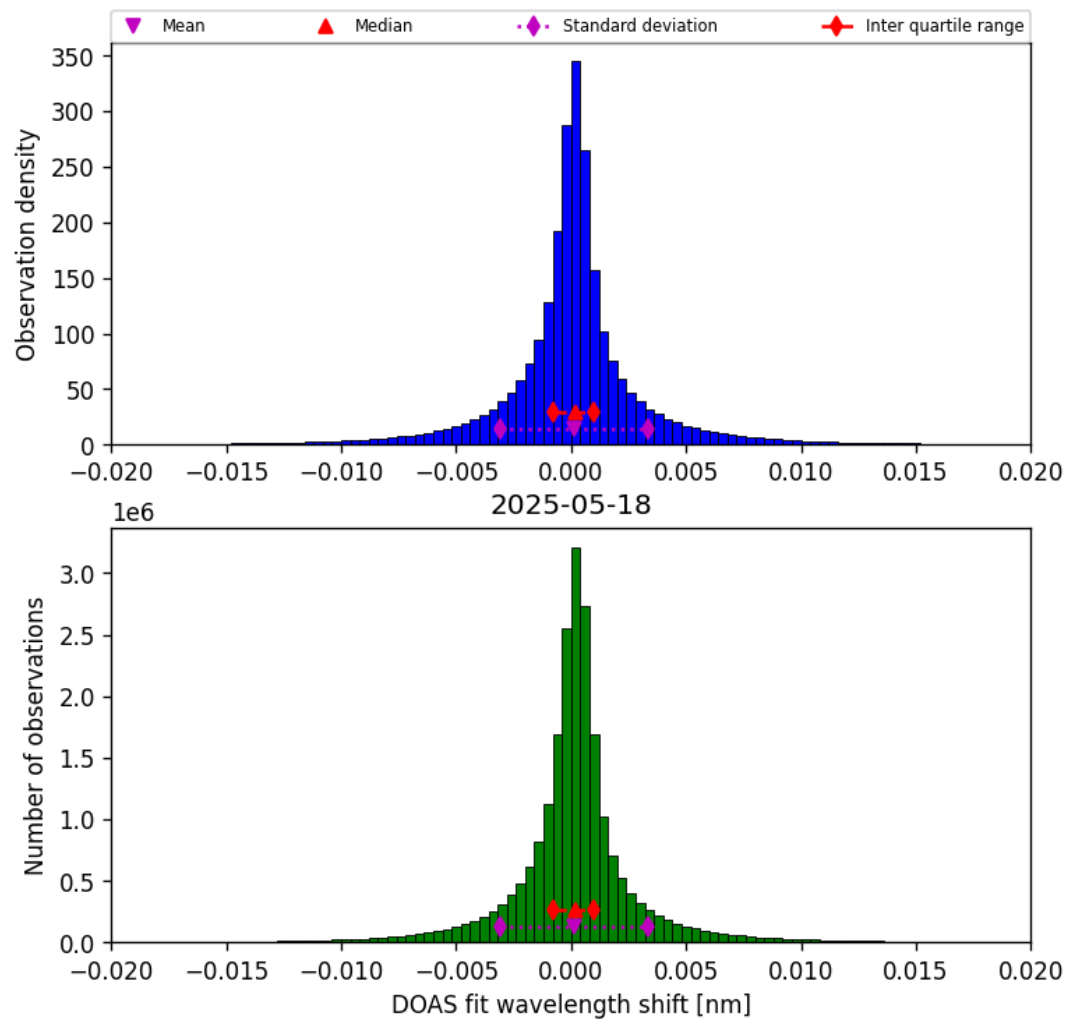
Figure 42: Histogram of “DOAS fit wavelength shift” for 2025-05-18 to 2025-05-19
