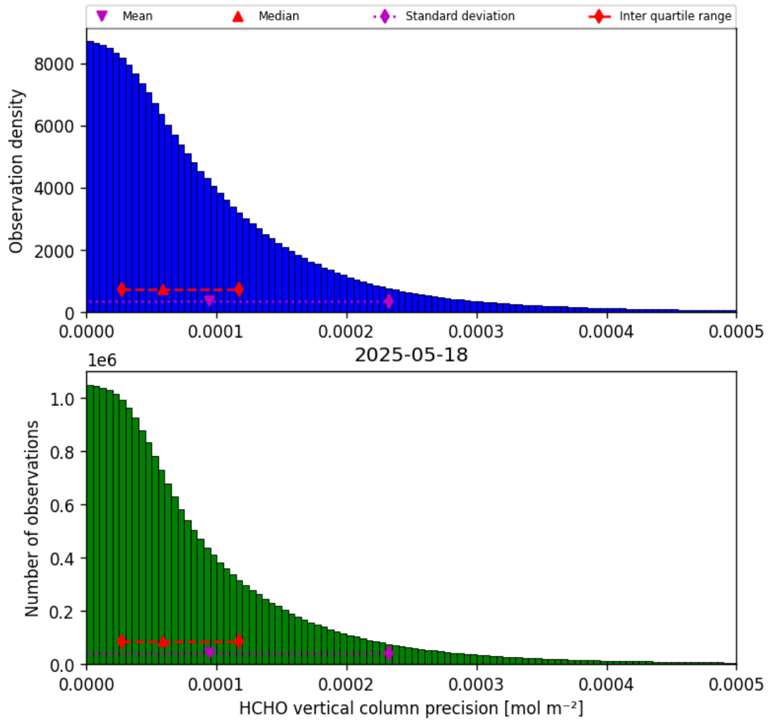
Figure 34: Histogram of “HCHO vertical column precision” for 2025-05-18 to 2025-05-19
