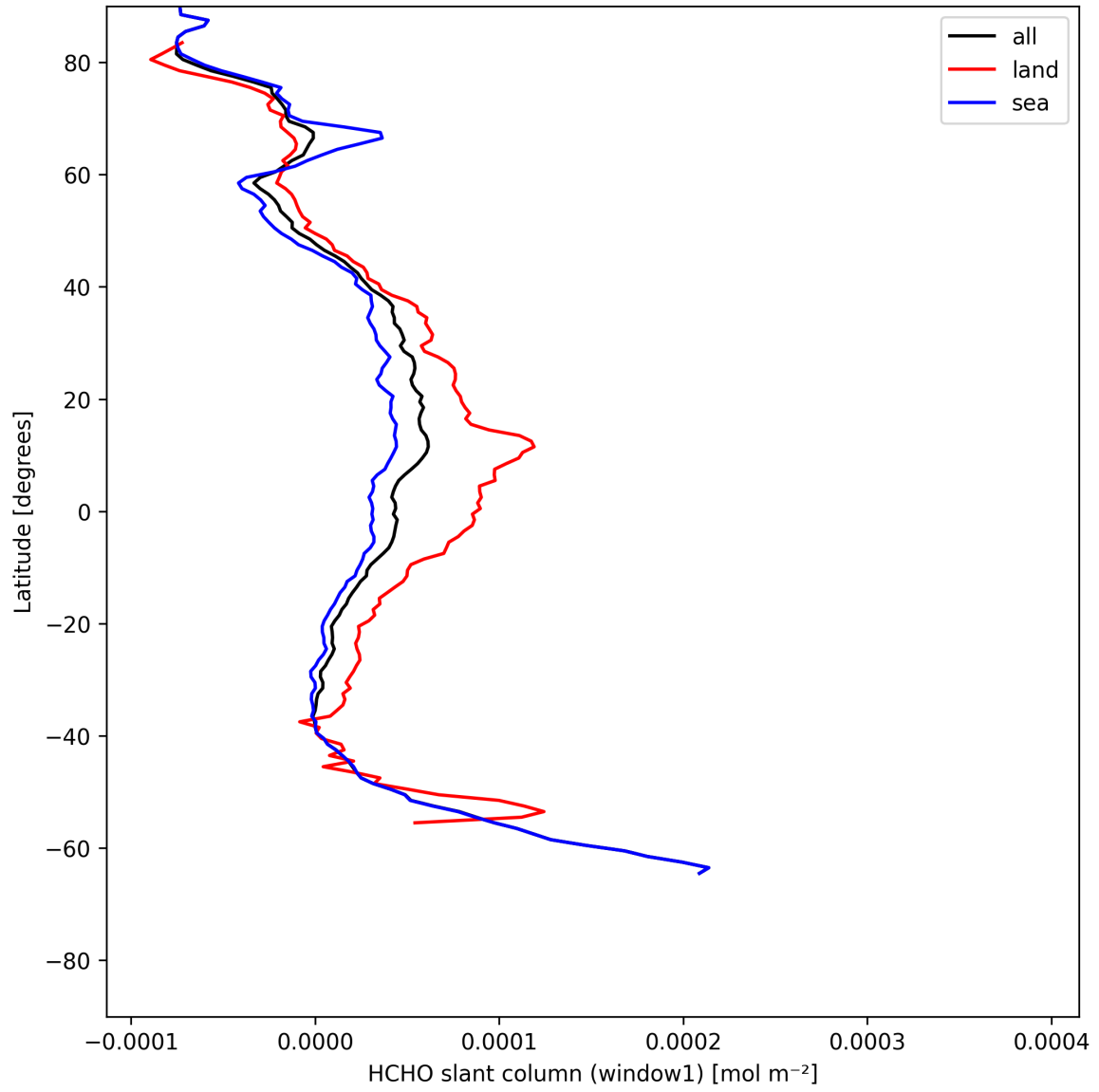
Figure 22: Zonal average of “HCHO slant column (window1)” for 2025-05-18 to 2025-05-19.
