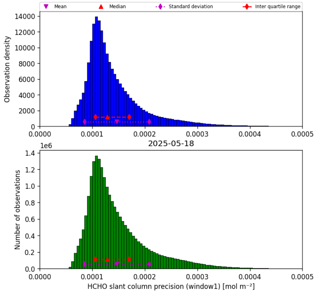
Figure 37: Histogram of “HCHO slant column precision (window1)” for 2025-05-18 to 2025-05-19
