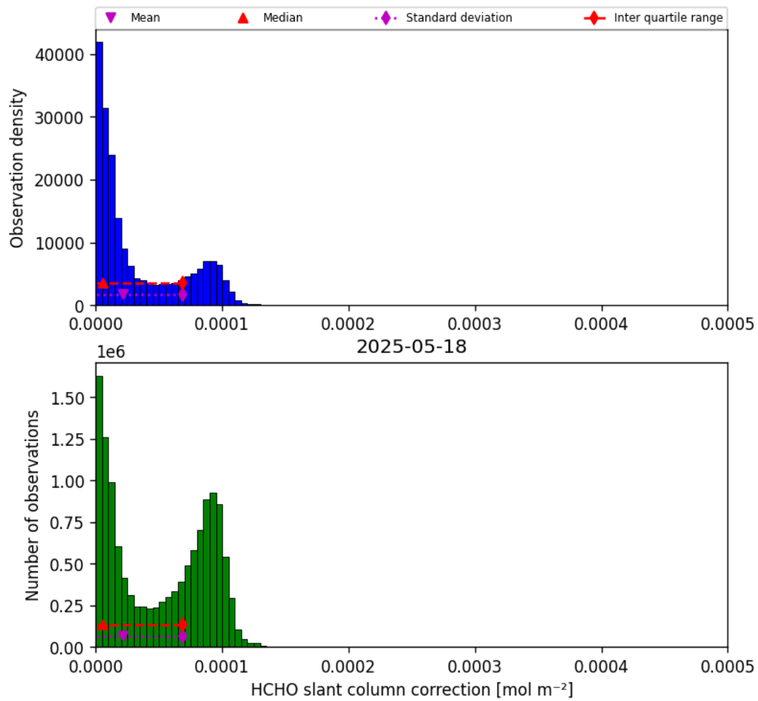
Figure 45: Histogram of “HCHO slant column correction” for 2025-05-18 to 2025-05-19
