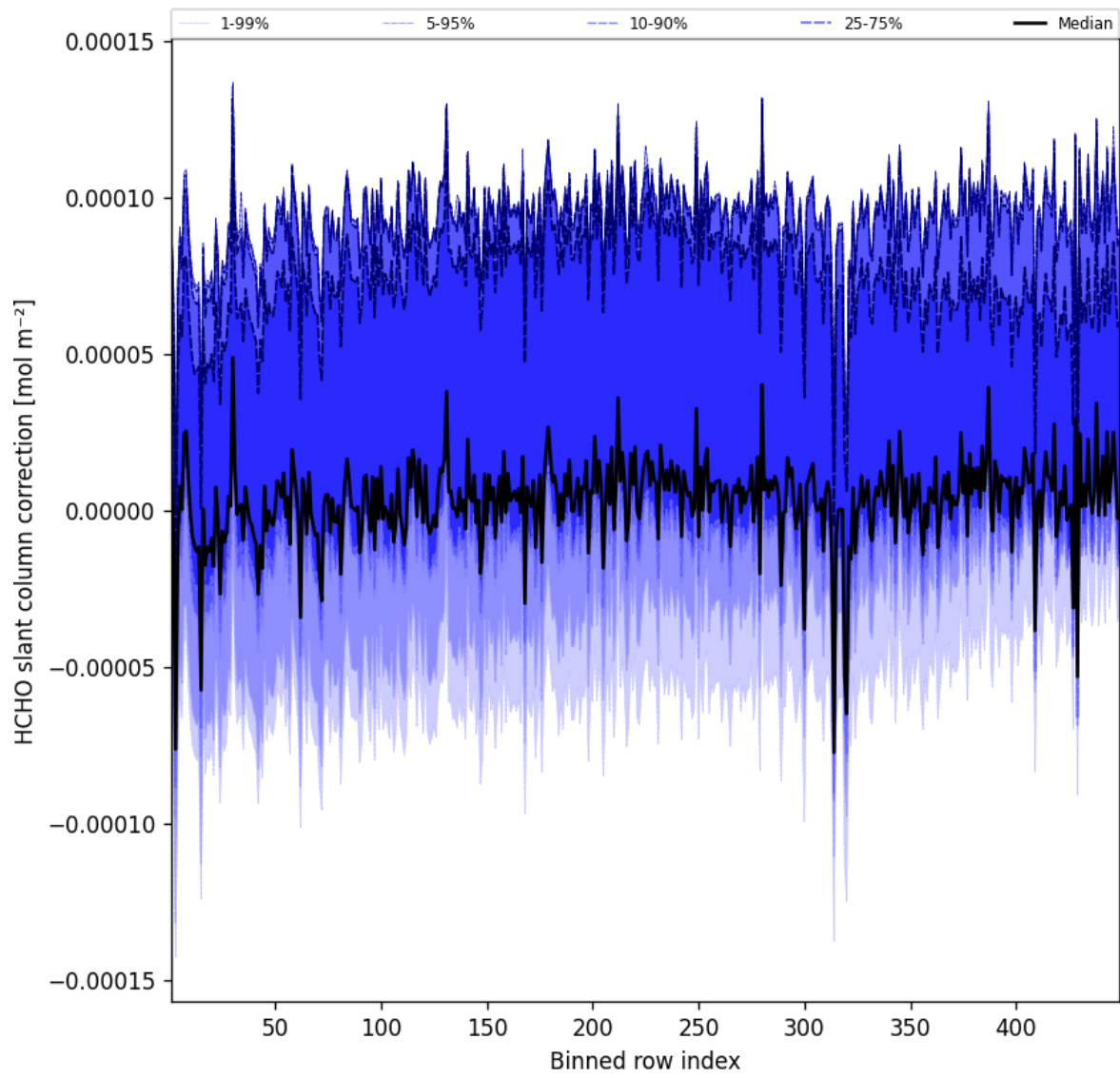
Figure 59: Along track statistics of “HCHO slant column correction” for 2025-05-18 to 2025-05-19
