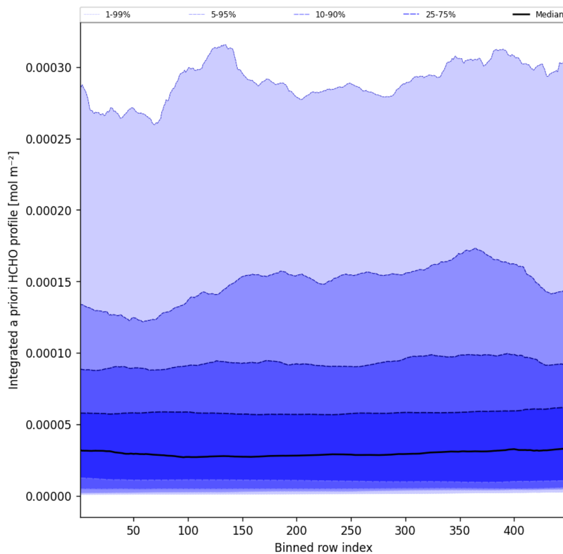
Figure 55: Along track statistics of “Integrated a priori HCHO profile” for 2025-05-18 to 2025-05-19
