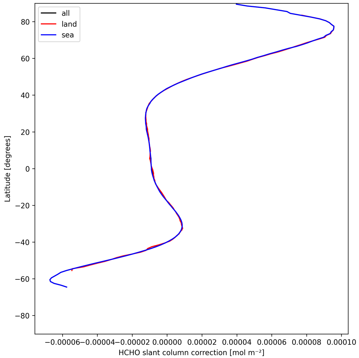
Figure 31: Zonal average of “HCHO slant column correction” for 2025-05-18 to 2025-05-19.
