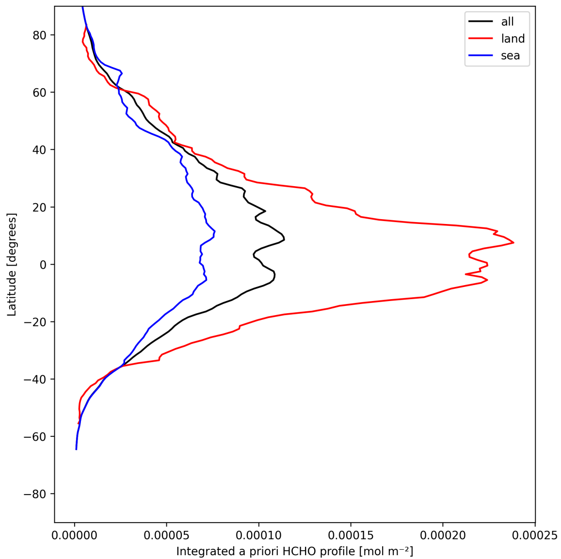
Figure 27: Zonal average of “Integrated a priori HCHO profile” for 2025-05-18 to 2025-05-19.
