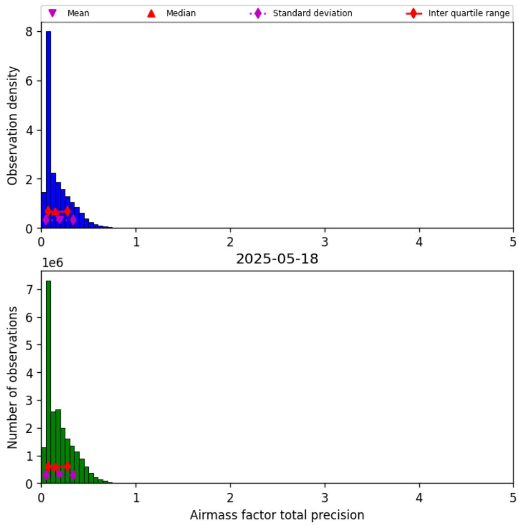
Figure 39: Histogram of “Airmass factor total precision” for 2025-05-18 to 2025-05-19
