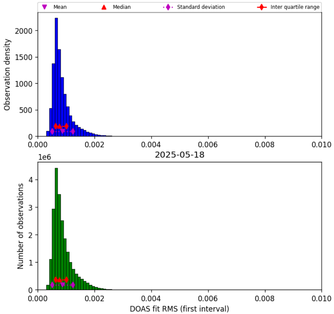
Figure 44: Histogram of “DOAS fit RMS (first interval)” for 2025-05-18 to 2025-05-19
