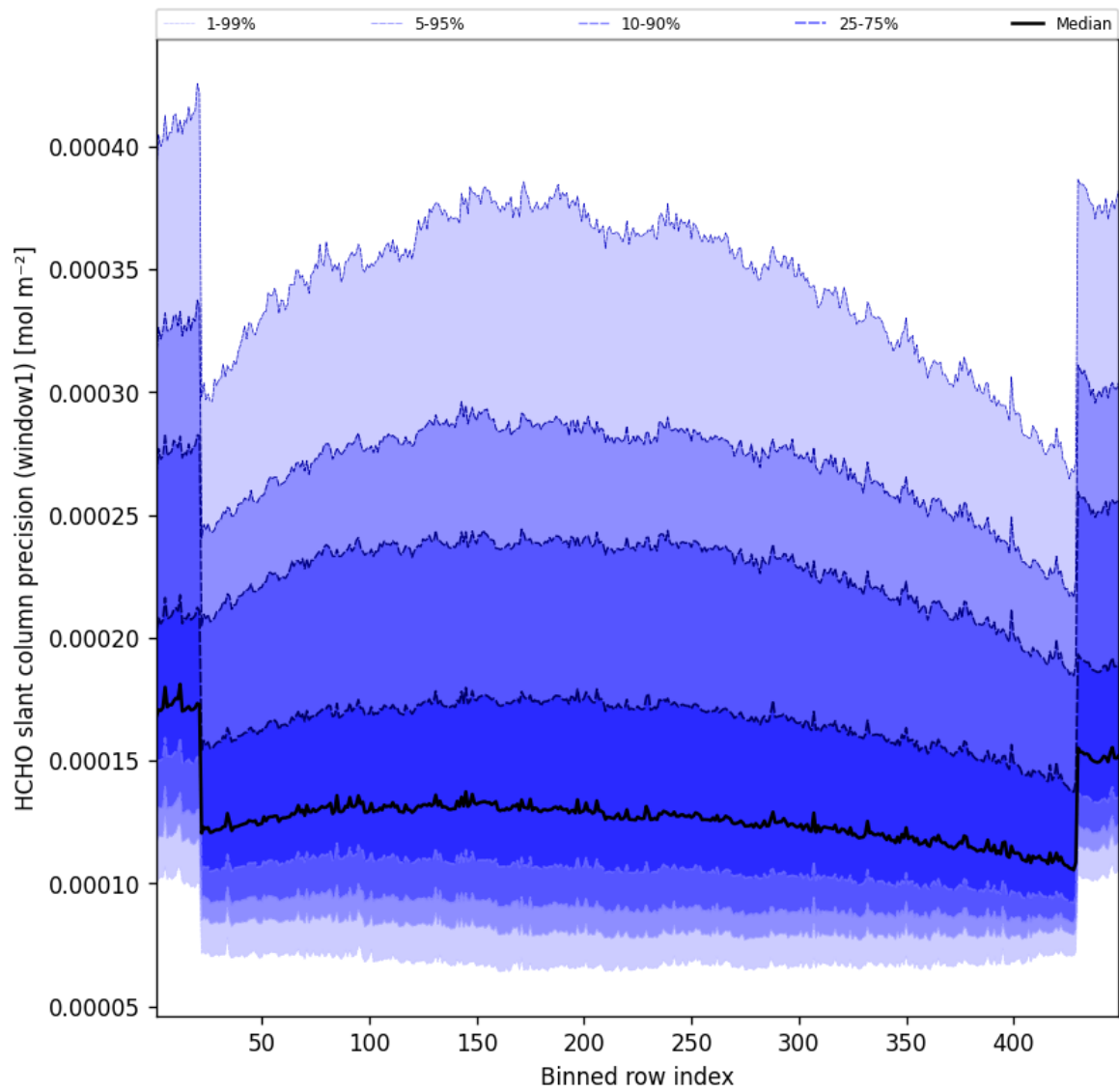
Figure 51: Along track statistics of “HCHO slant column precision (window1)” for 2025-05-18 to 2025-05-19
