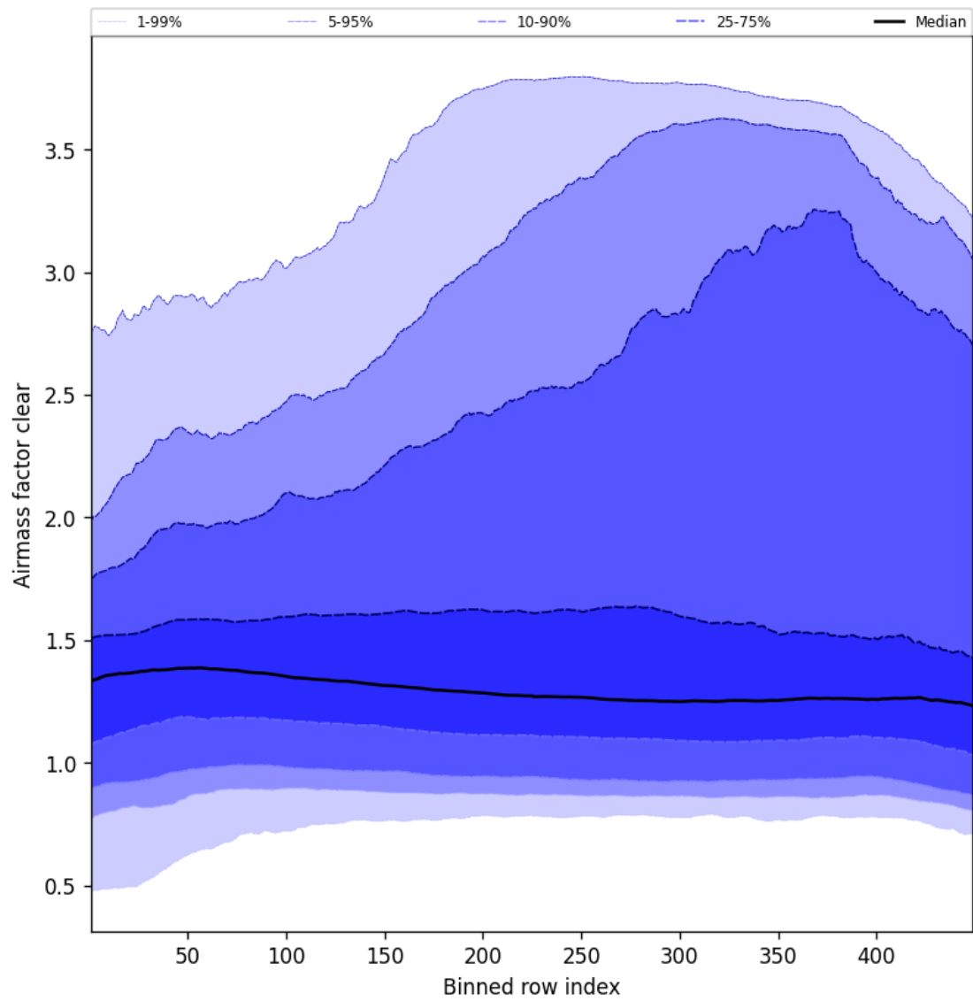
Figure 54: Along track statistics of “Airmass factor clear” for 2025-05-18 to 2025-05-19
