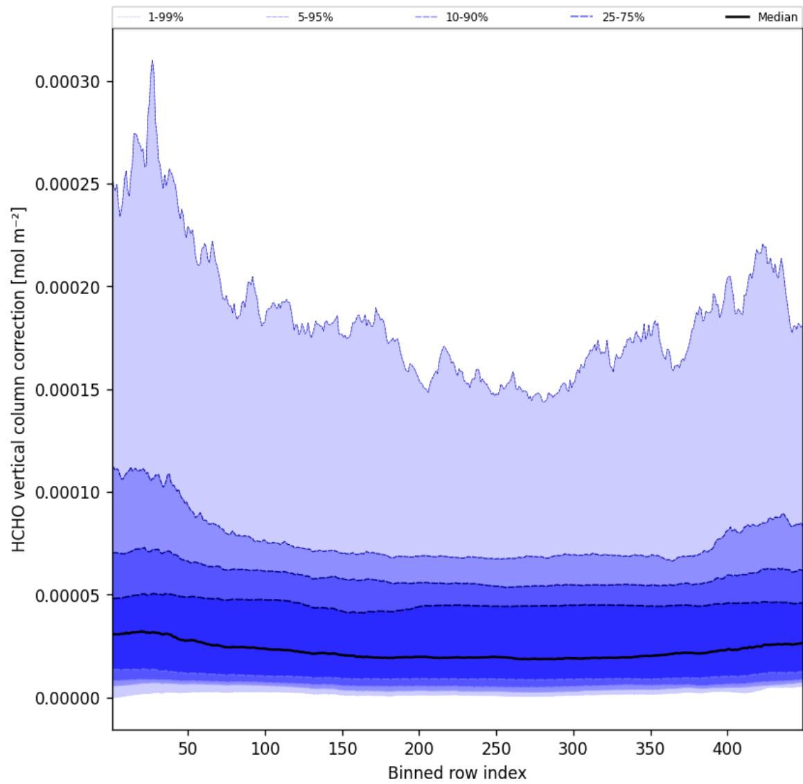
Figure 49: Along track statistics of “HCHO vertical column correction” for 2025-05-18 to 2025-05-19
