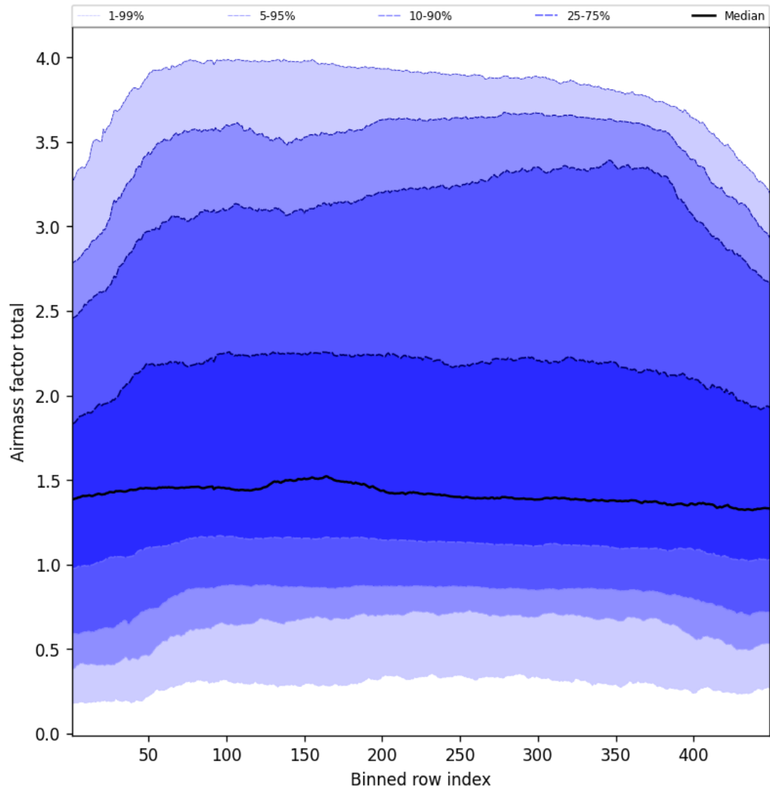
Figure 52: Along track statistics of “Airmass factor total” for 2025-05-18 to 2025-05-19
