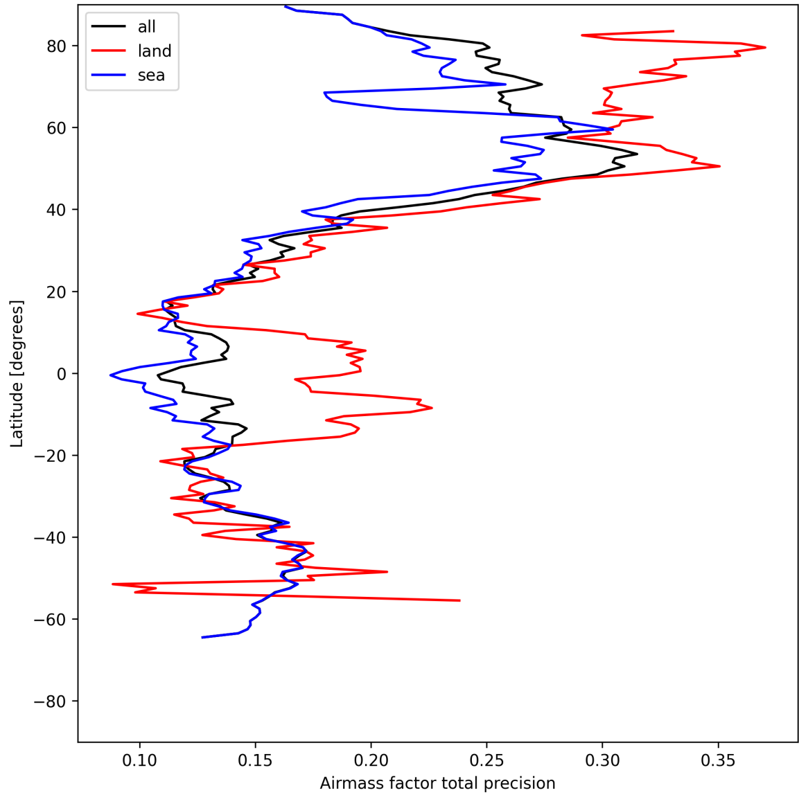
Figure 25: Zonal average of “Airmass factor total precision” for 2025-05-18 to 2025-05-19.
