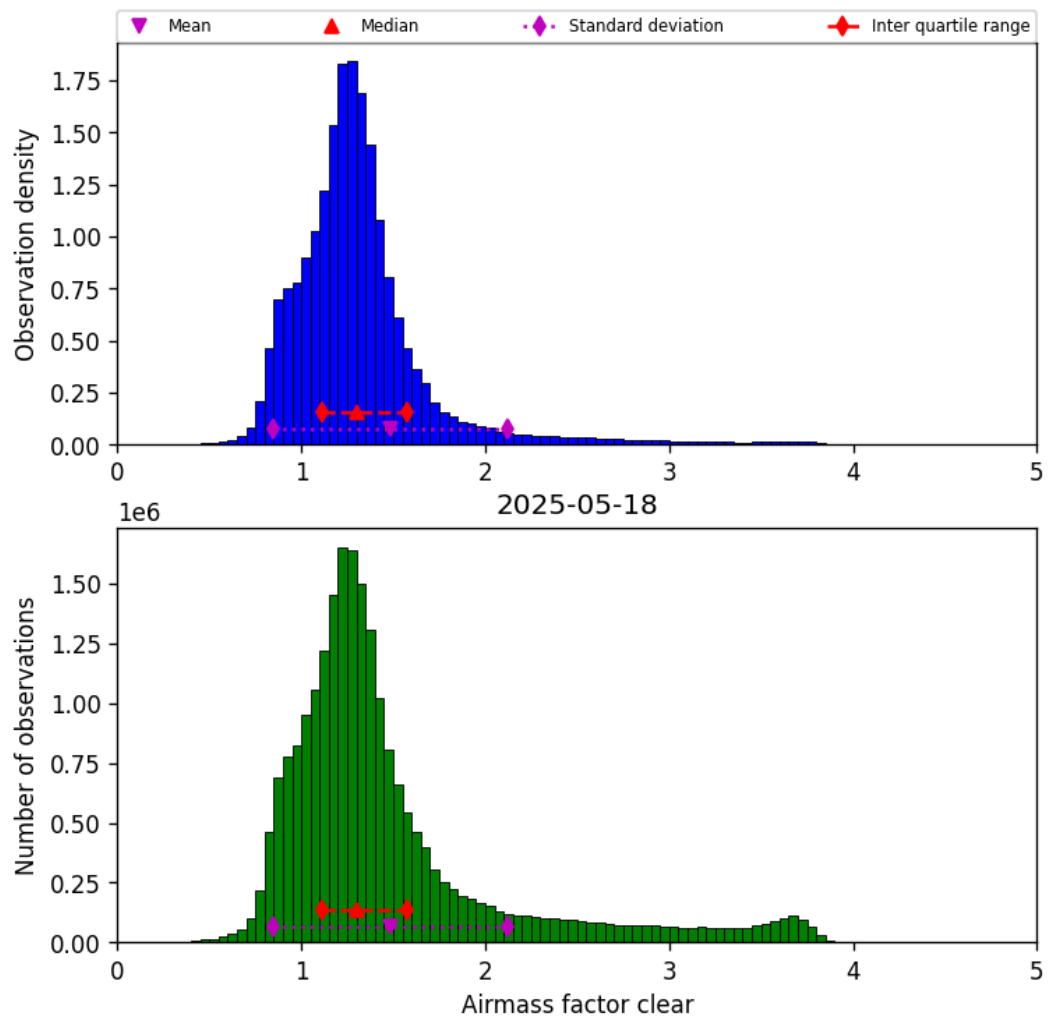
Figure 40: Histogram of “Airmass factor clear” for 2025-05-18 to 2025-05-19
