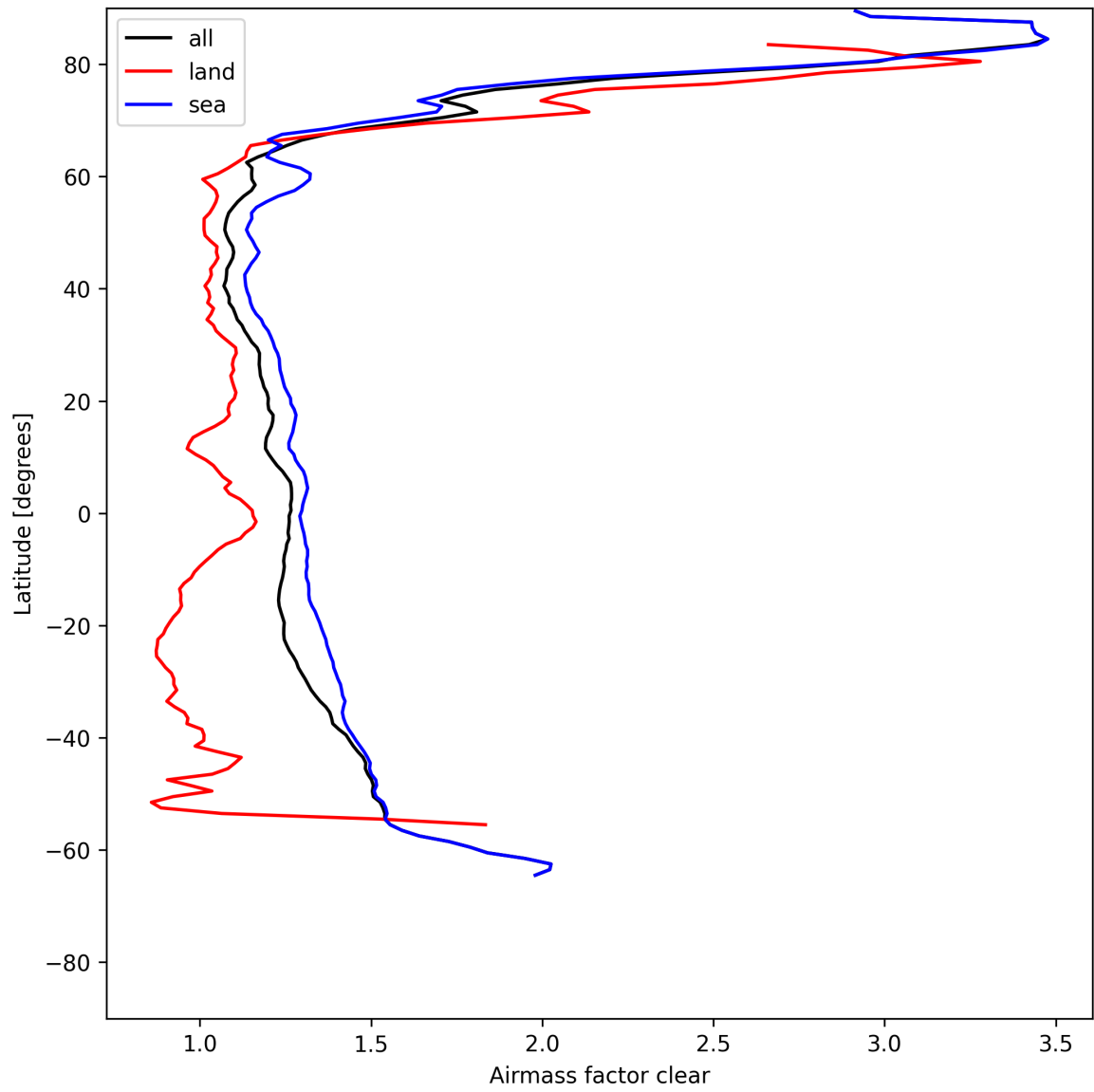
Figure 26: Zonal average of “Airmass factor clear” for 2025-05-18 to 2025-05-19.
