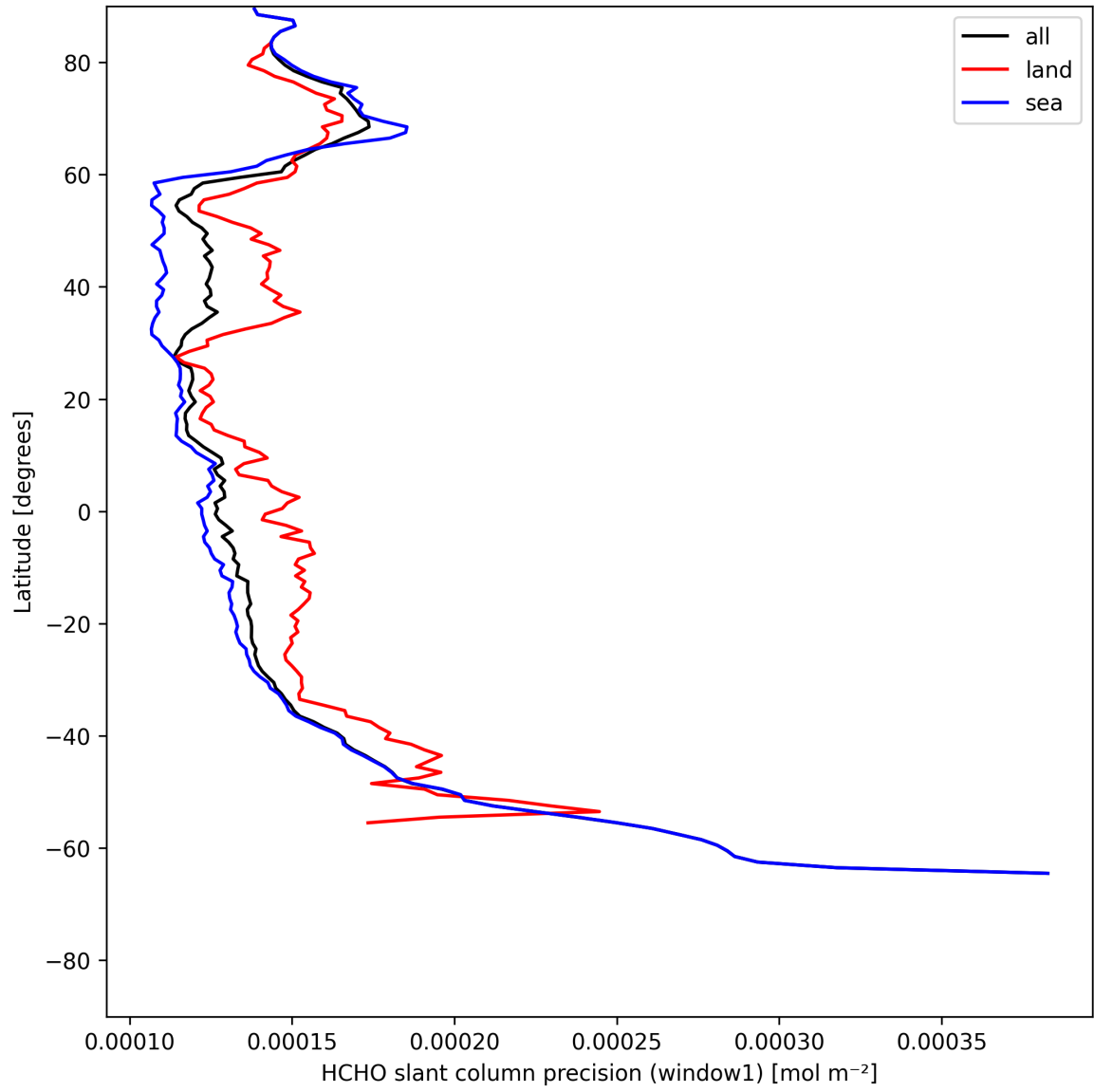
Figure 23: Zonal average of "HCHO slant column precision (window1)" for 2025-05-18 to 2025-05-19.
