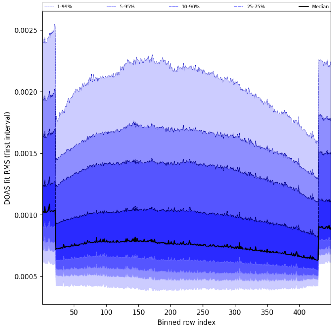
Figure 58: Along track statistics of “DOAS fit RMS (first interval)” for 2025-05-18 to 2025-05-19
