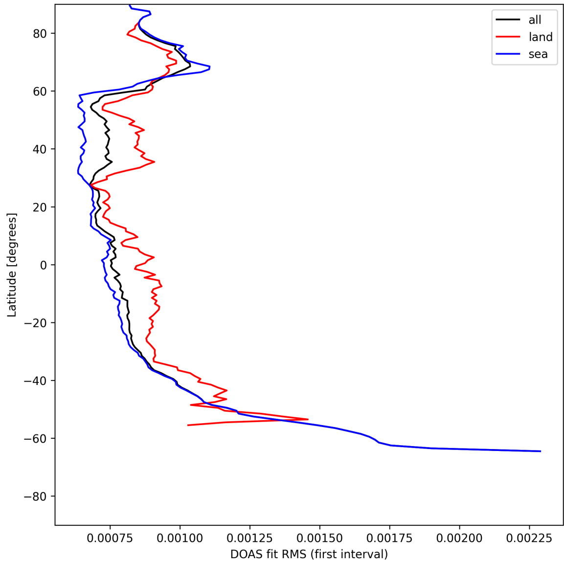
Figure 30: Zonal average of “DOAS fit RMS (first interval)” for 2025-05-18 to 2025-05-19.
