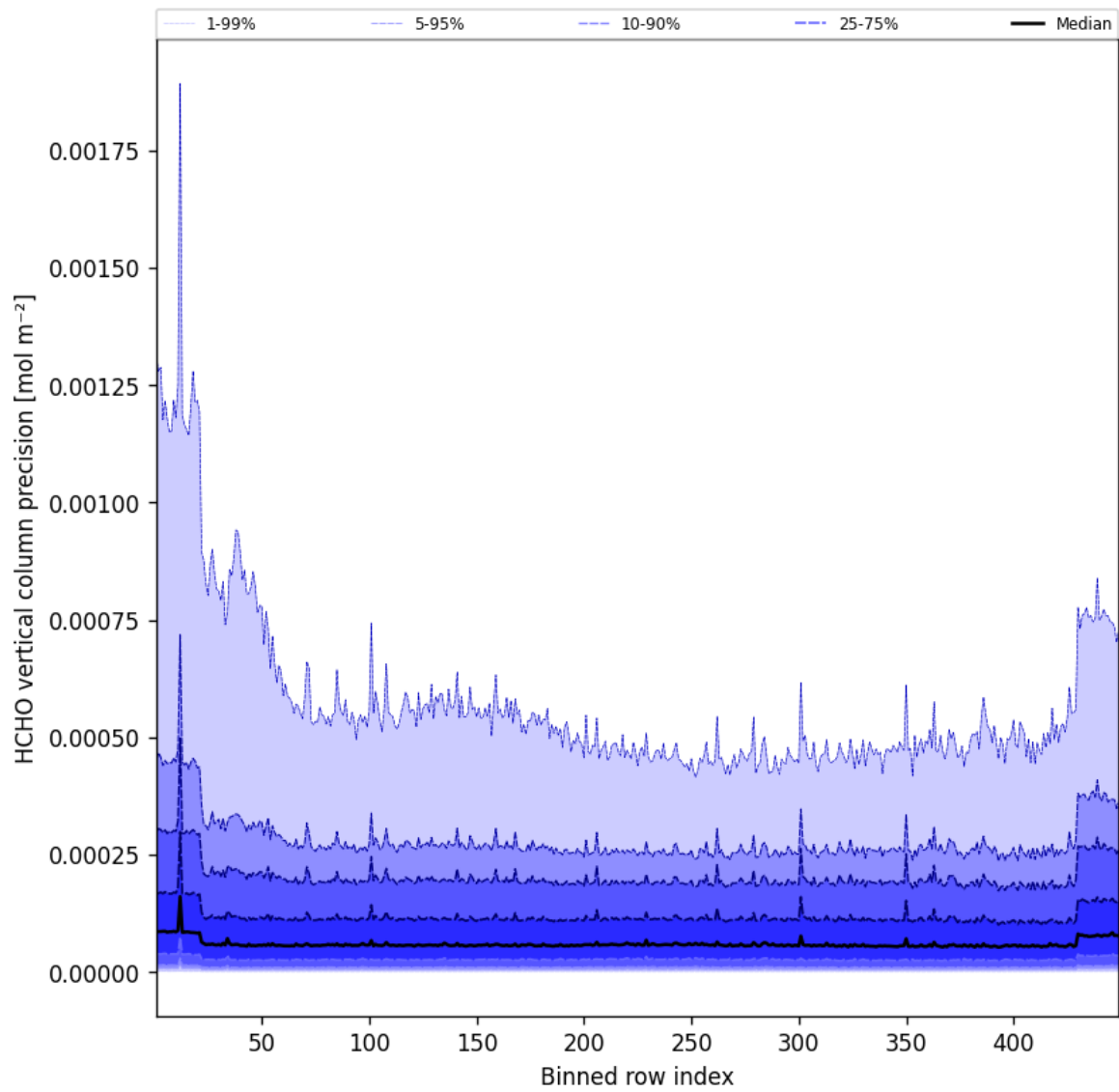
Figure 48: Along track statistics of “HCHO vertical column precision” for 2025-05-18 to 2025-05-19
