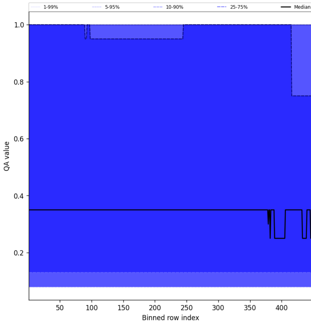
Figure 46: Along track statistics of “QA value” for 2025-05-18 to 2025-05-19
