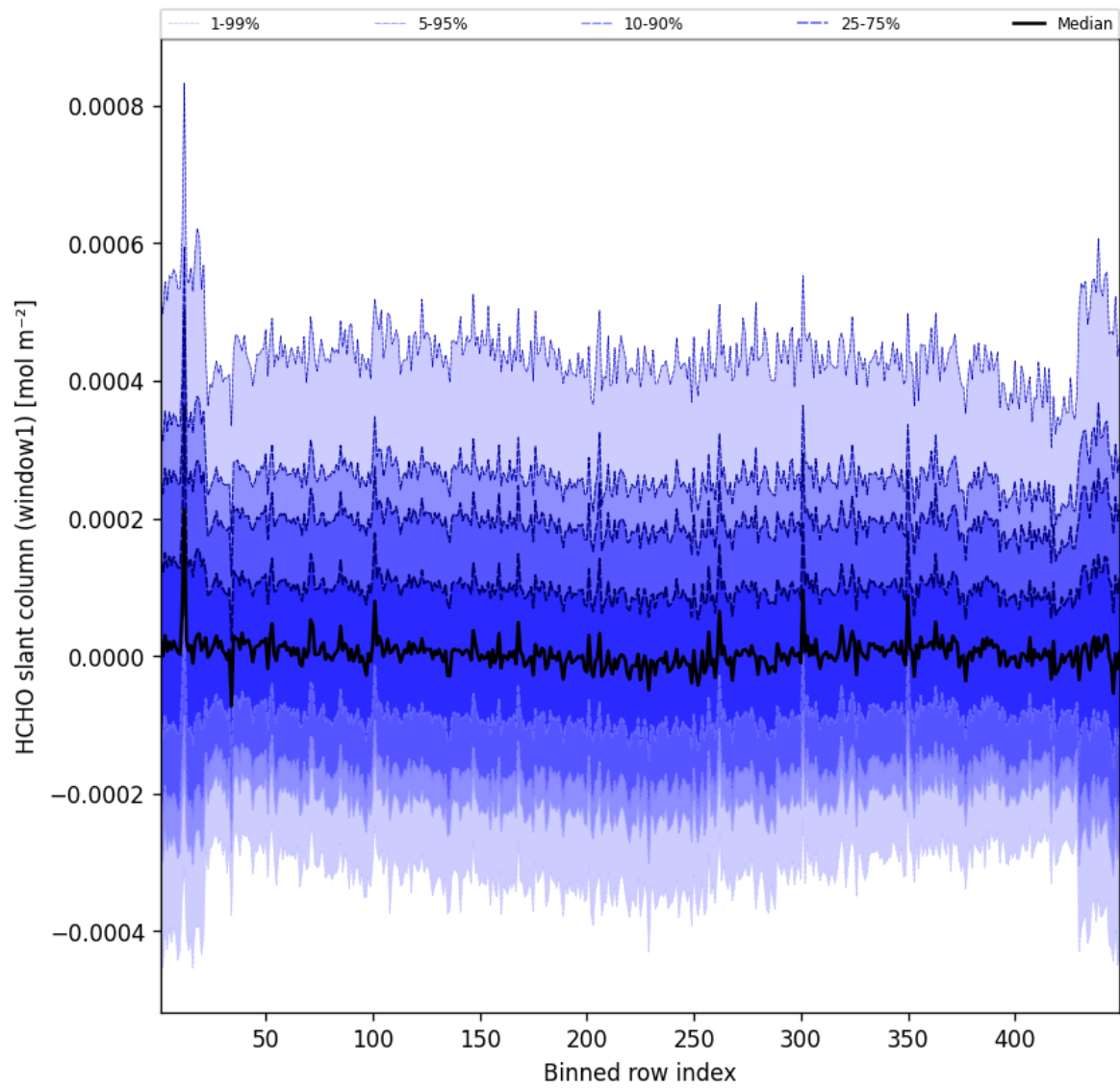
Figure 50: Along track statistics of “HCHO slant column (window1)” for 2025-05-18 to 2025-05-19
