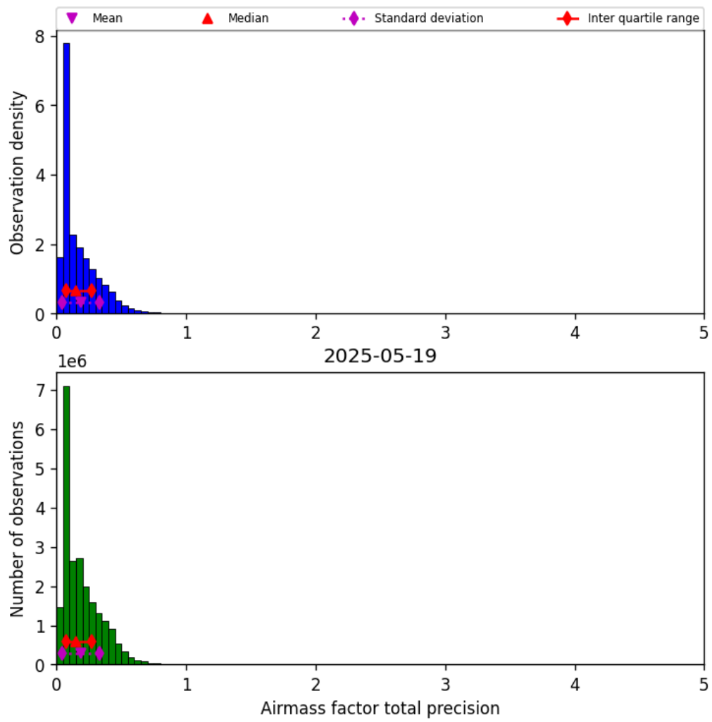
Figure 39: Histogram of “Airmass factor total precision” for 2025-05-19 to 2025-05-19
