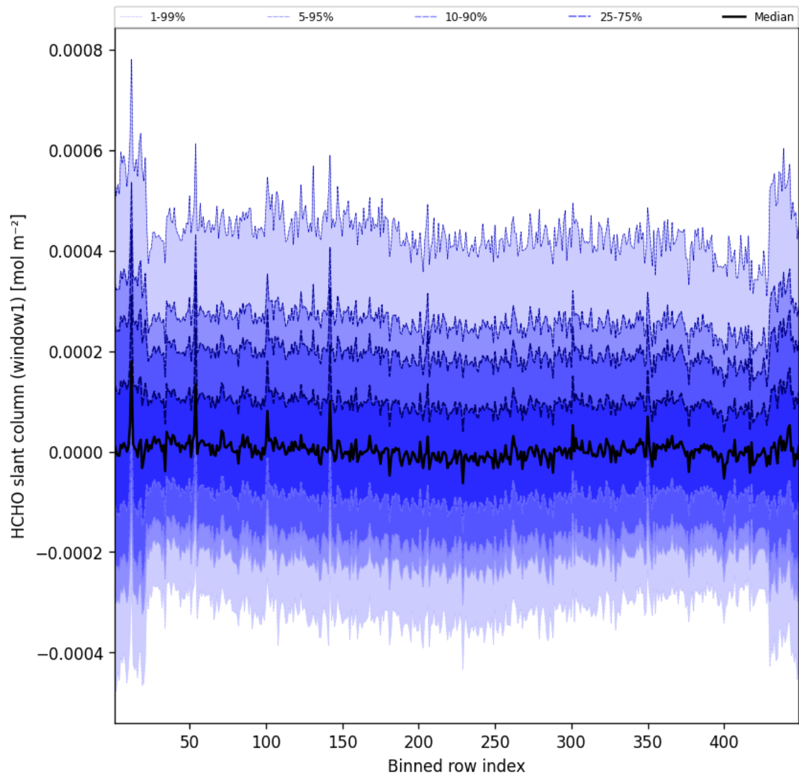
Figure 50: Along track statistics of “HCHO slant column (window1)” for 2025-05-19 to 2025-05-19
