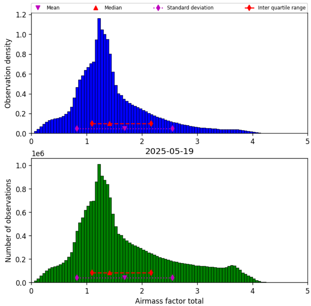
Figure 38: Histogram of “Airmass factor total” for 2025-05-19 to 2025-05-19
