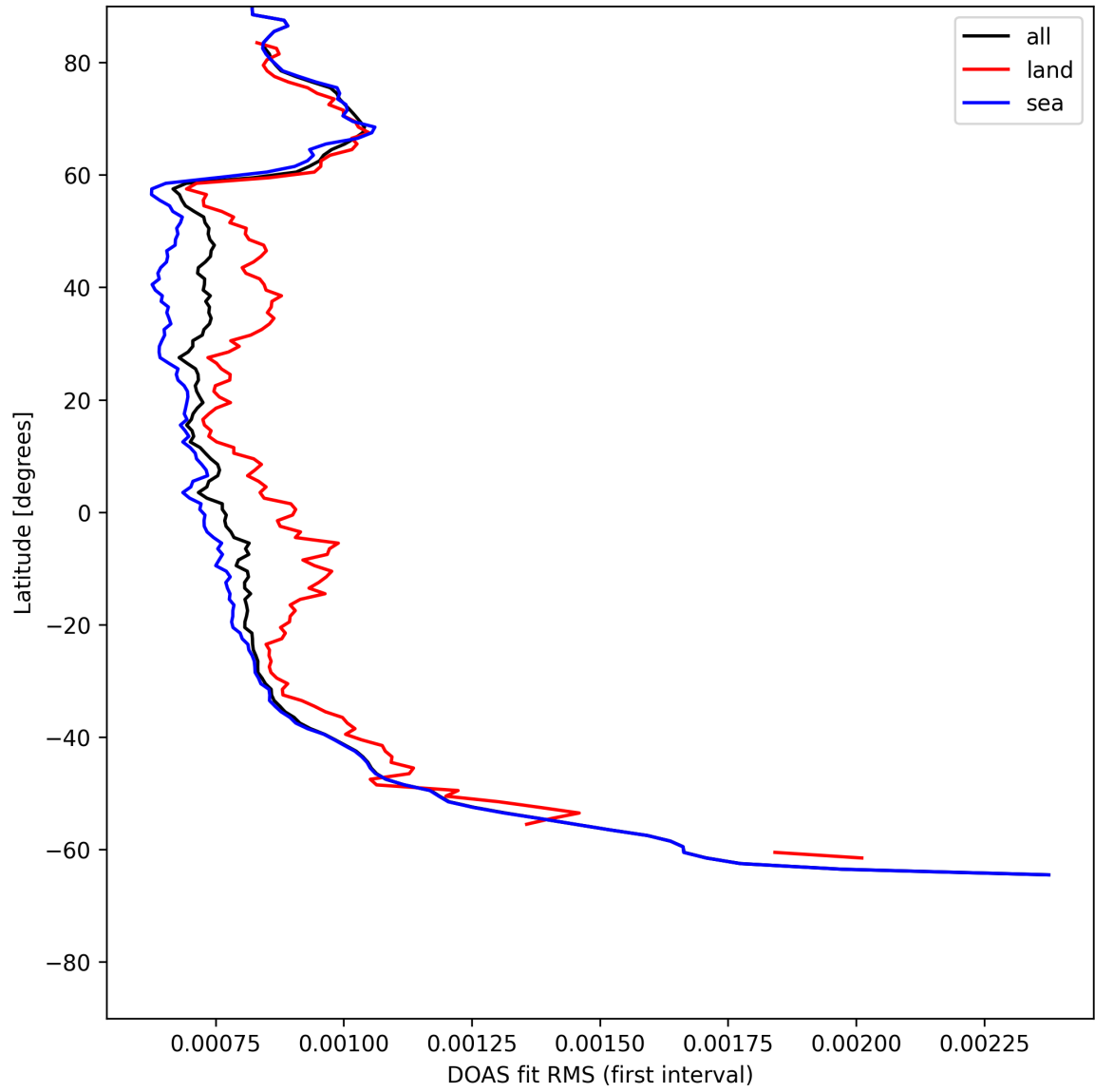
Figure 30: Zonal average of “DOAS fit RMS (first interval)” for 2025-05-19 to 2025-05-19.
