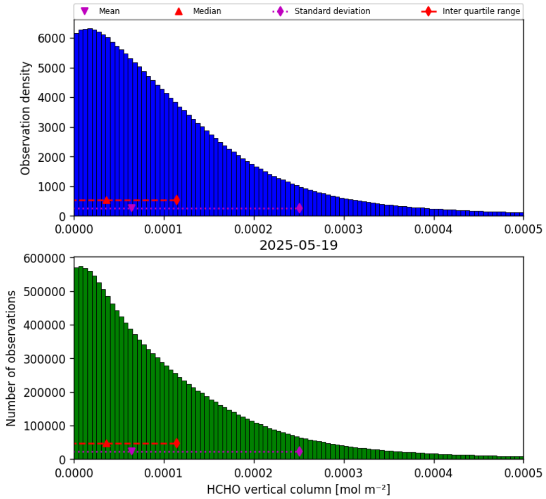
Figure 33: Histogram of “HCHO vertical column” for 2025-05-19 to 2025-05-19
