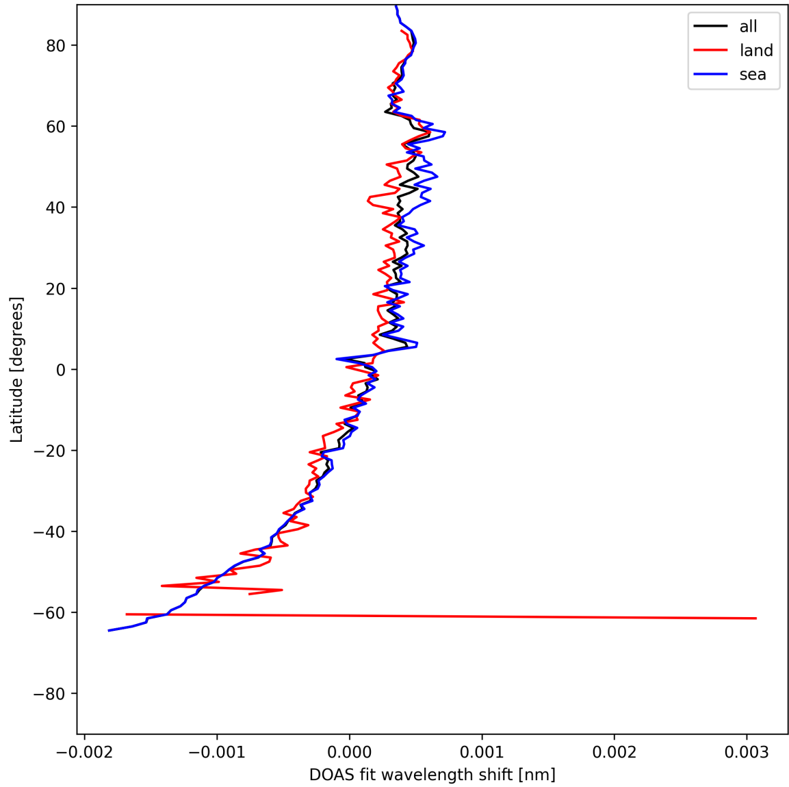
Figure 28: Zonal average of “DOAS fit wavelength shift” for 2025-05-19 to 2025-05-19.
