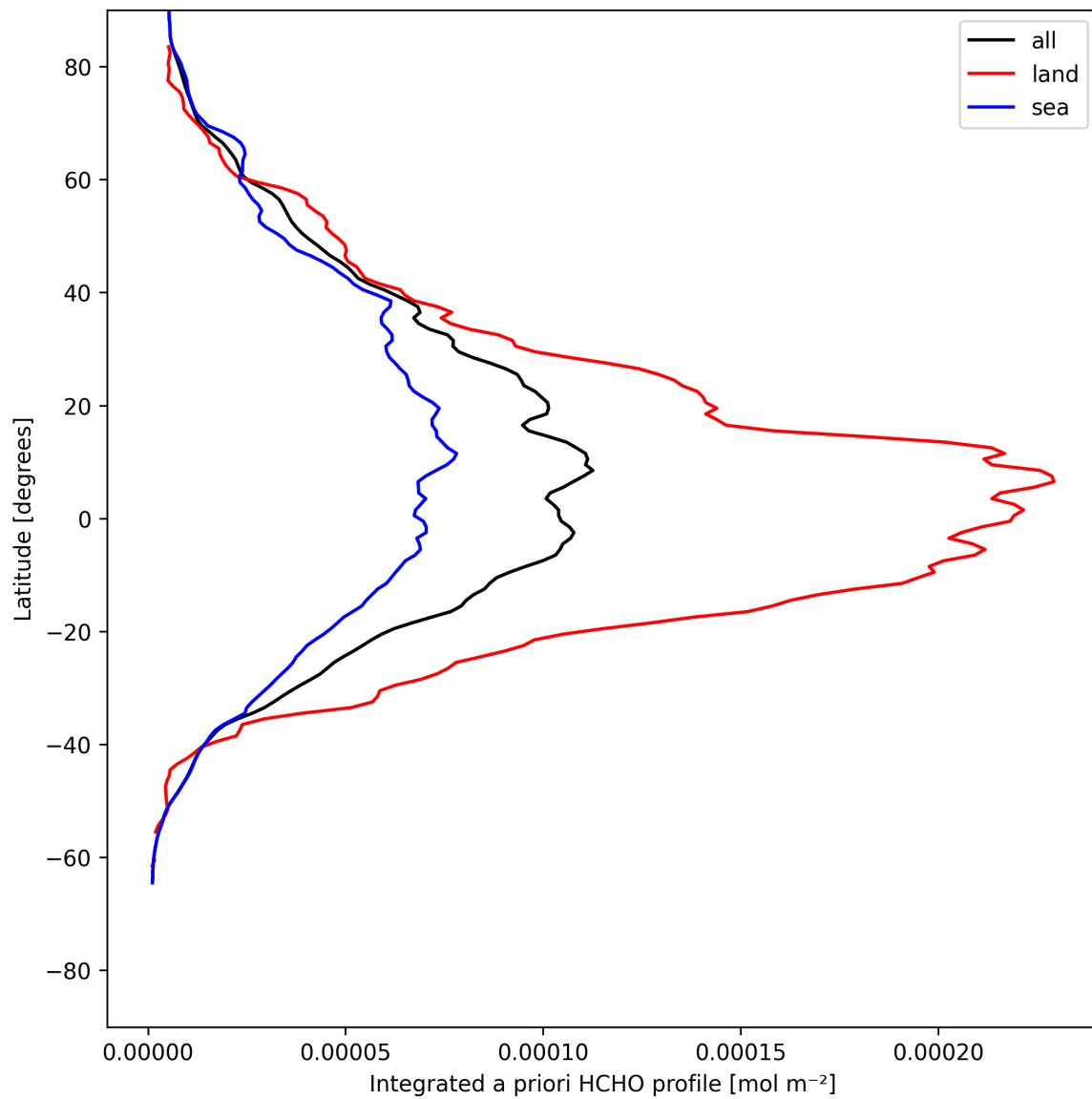
Figure 27: Zonal average of “Integrated a priori HCHO profile” for 2025-05-19 to 2025-05-19.
