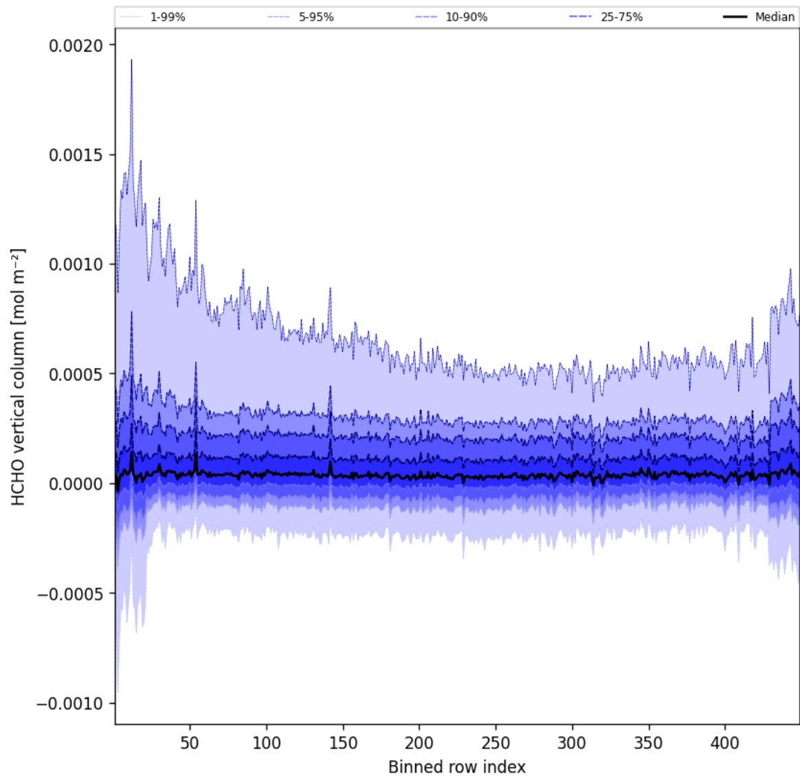
Figure 47: Along track statistics of “HCHO vertical column” for 2025-05-19 to 2025-05-19
