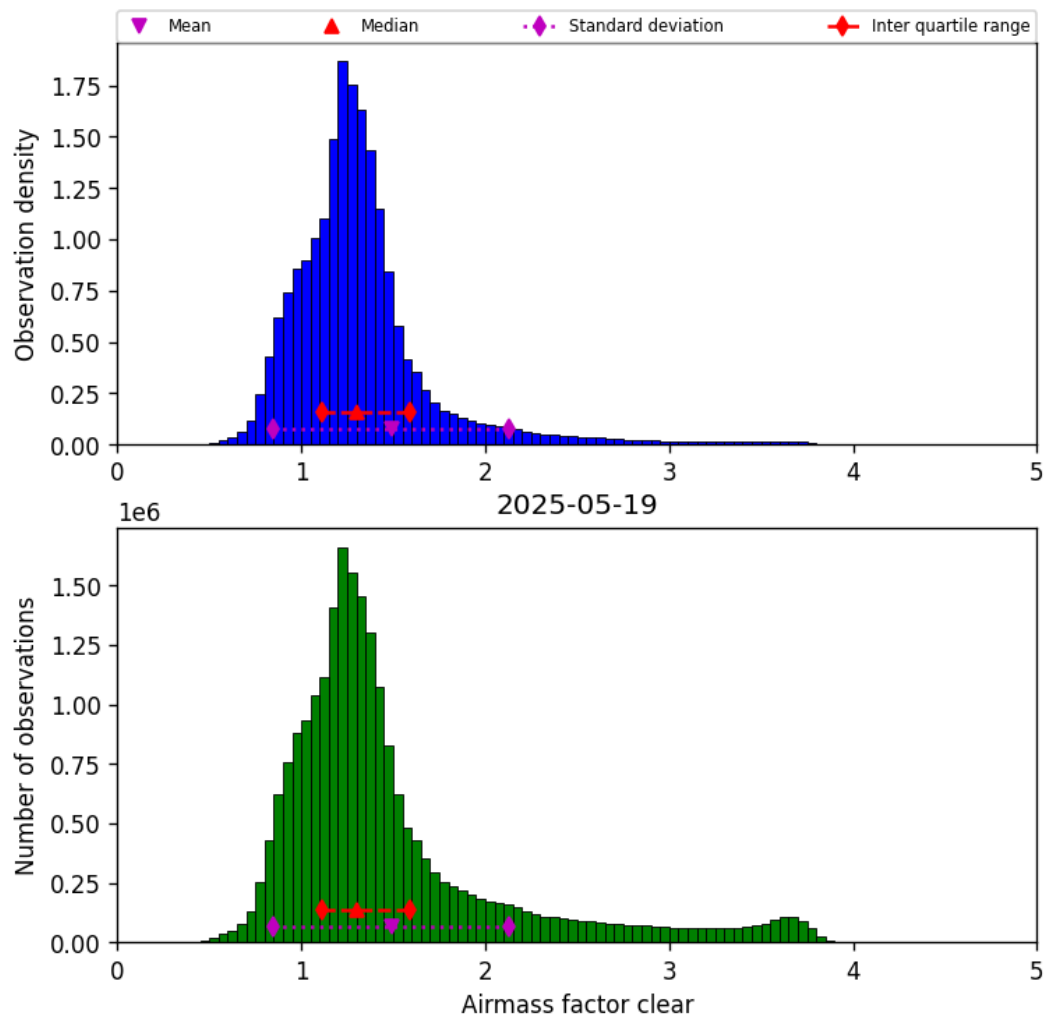
Figure 40: Histogram of “Airmass factor clear” for 2025-05-19 to 2025-05-19
