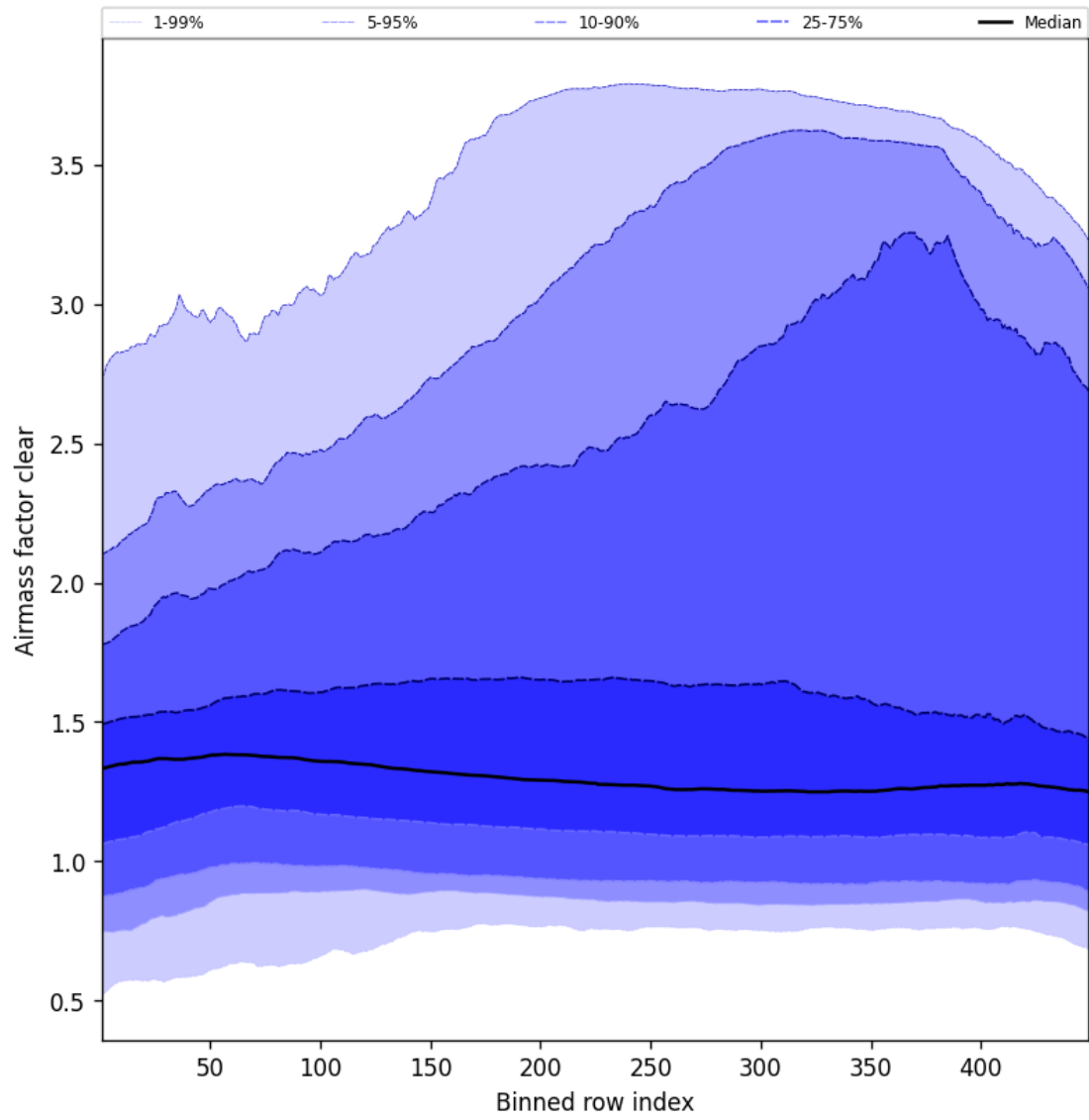
Figure 54: Along track statistics of “Airmass factor clear” for 2025-05-19 to 2025-05-19
