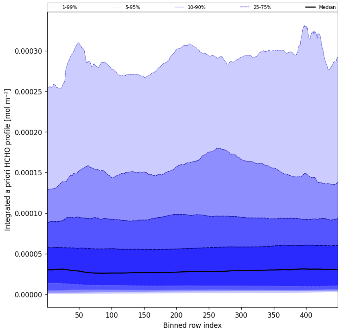
Figure 55: Along track statistics of "Integrated a priori HCHO profile" for 2025-05-19 to 2025-05-19
