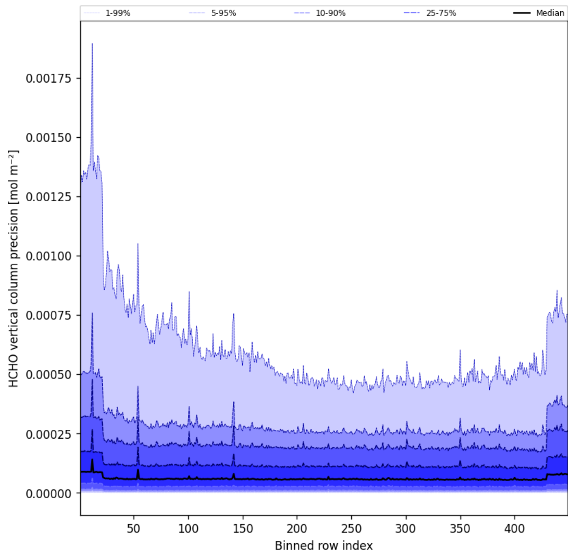
Figure 48: Along track statistics of “HCHO vertical column precision” for 2025-05-19 to 2025-05-19
