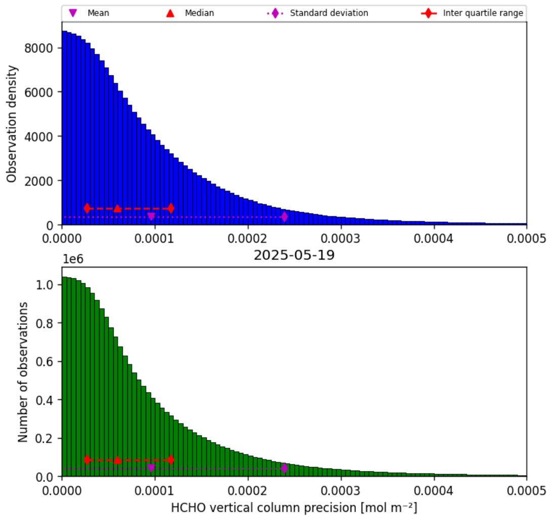
Figure 34: Histogram of “HCHO vertical column precision” for 2025-05-19 to 2025-05-19
