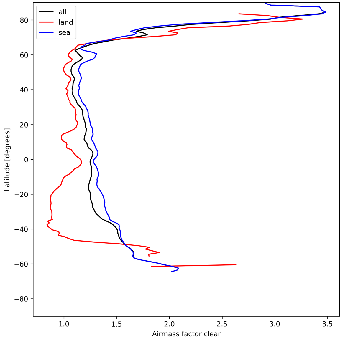
Figure 26: Zonal average of “Airmass factor clear” for 2025-05-19 to 2025-05-19.
