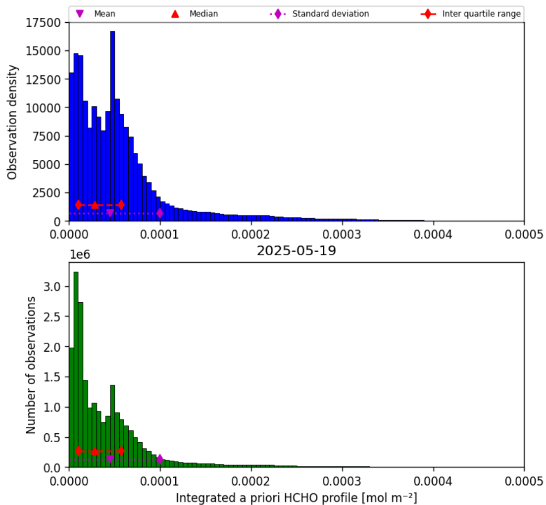
Figure 41: Histogram of “Integrated a priori HCHO profile” for 2025-05-19 to 2025-05-19
