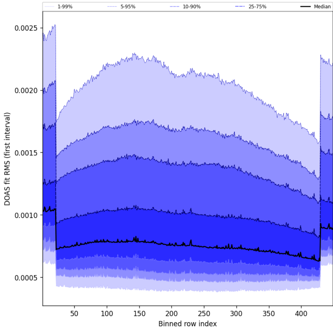
Figure 58: Along track statistics of “DOAS fit RMS (first interval)” for 2025-05-19 to 2025-05-19
