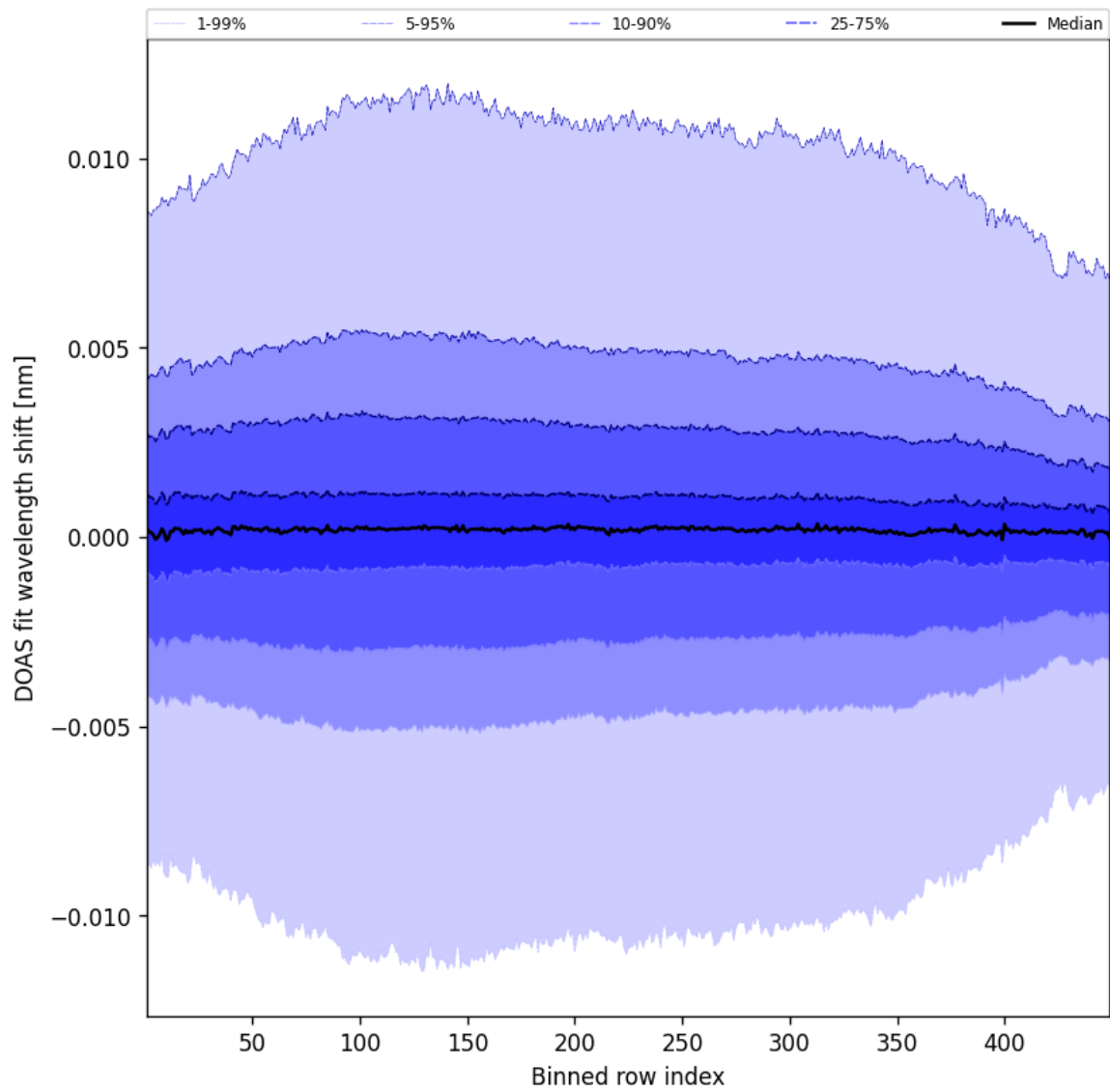
Figure 56: Along track statistics of “DOAS fit wavelength shift” for 2025-05-19 to 2025-05-19
