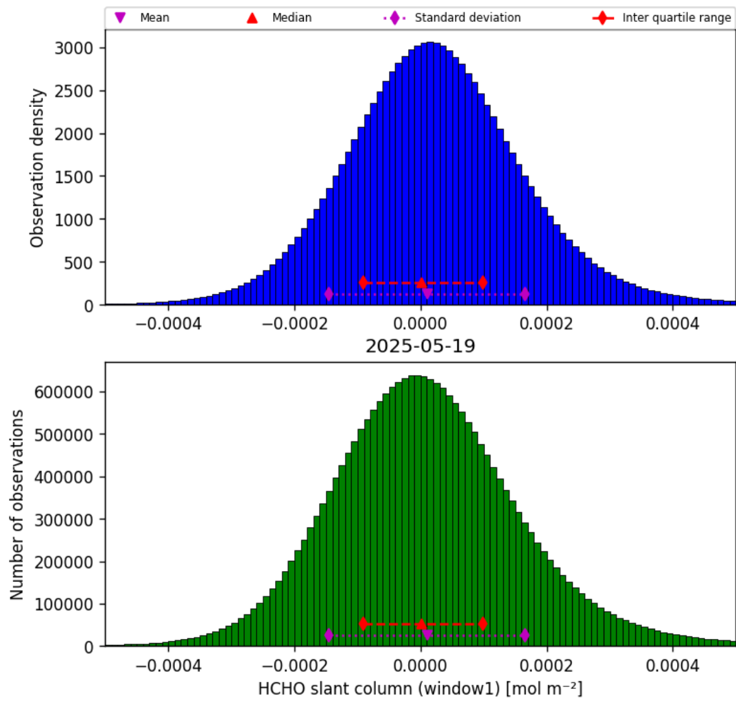
Figure 36: Histogram of “HCHO slant column (window1)” for 2025-05-19 to 2025-05-19
