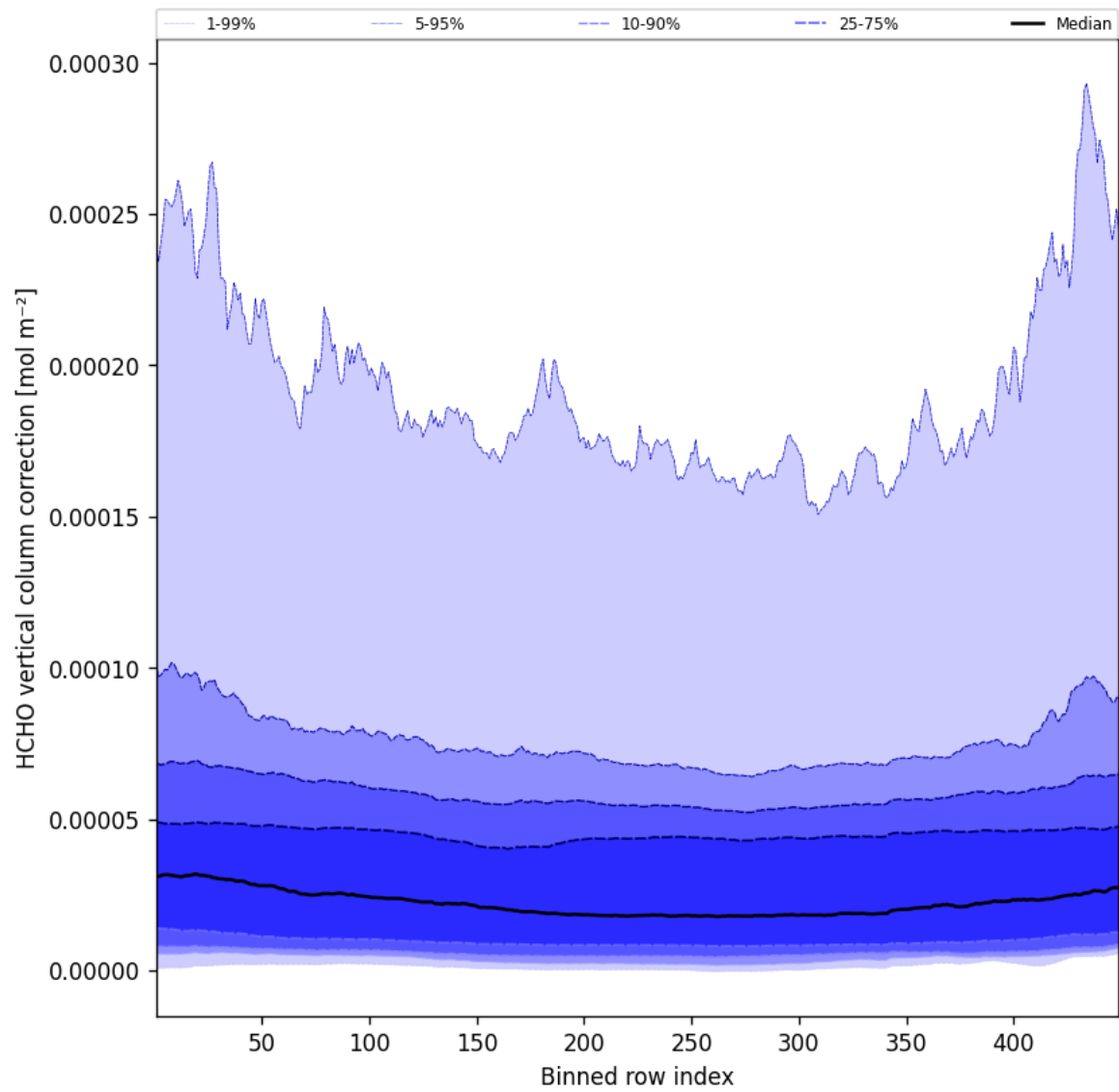
Figure 49: Along track statistics of “HCHO vertical column correction” for 2025-05-19 to 2025-05-19
