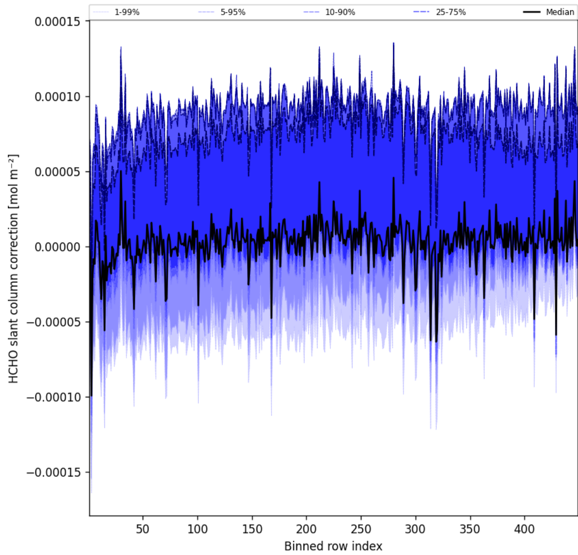
Figure 59: Along track statistics of “HCHO slant column correction” for 2025-05-19 to 2025-05-19
