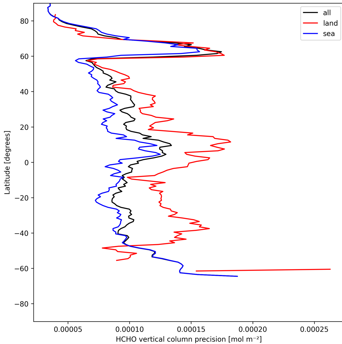
Figure 20: Zonal average of “HCHO vertical column precision” for 2025-05-19 to 2025-05-19.
