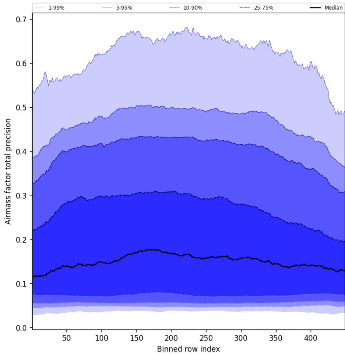
Figure 53: Along track statistics of “Airmass factor total precision” for 2025-05-19 to 2025-05-19
