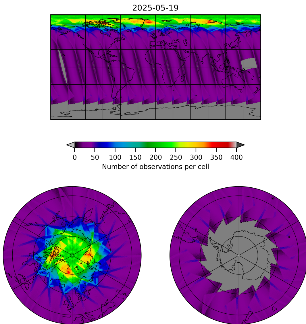
Figure 17: Map of the number of observations for 2025-05-19 to 2025-05-19
