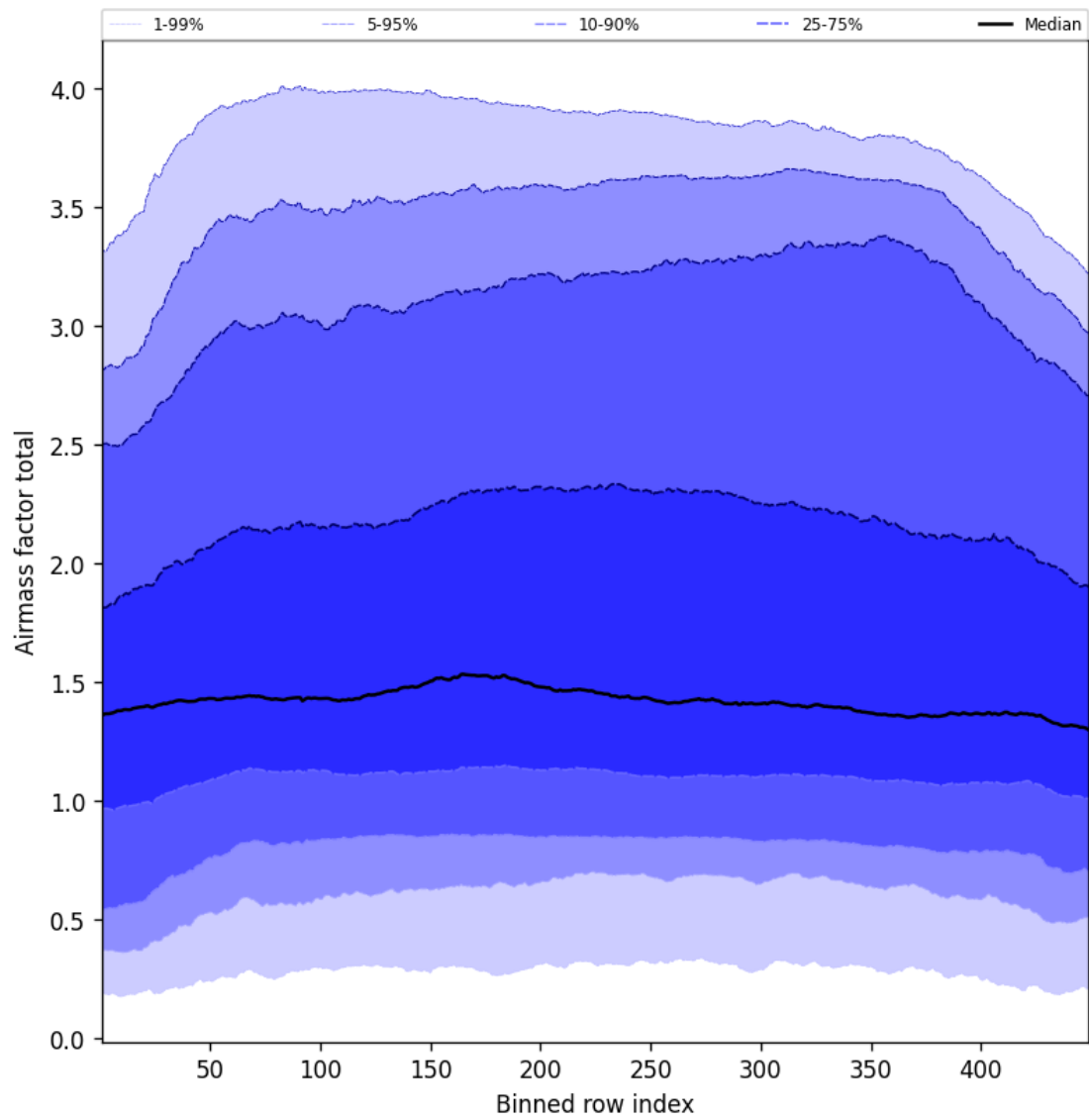
Figure 52: Along track statistics of “Airmass factor total” for 2025-05-19 to 2025-05-19
