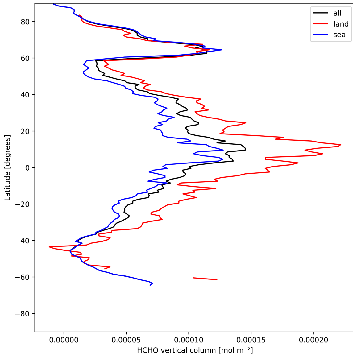
Figure 19: Zonal average of “HCHO vertical column” for 2025-05-19 to 2025-05-19.
