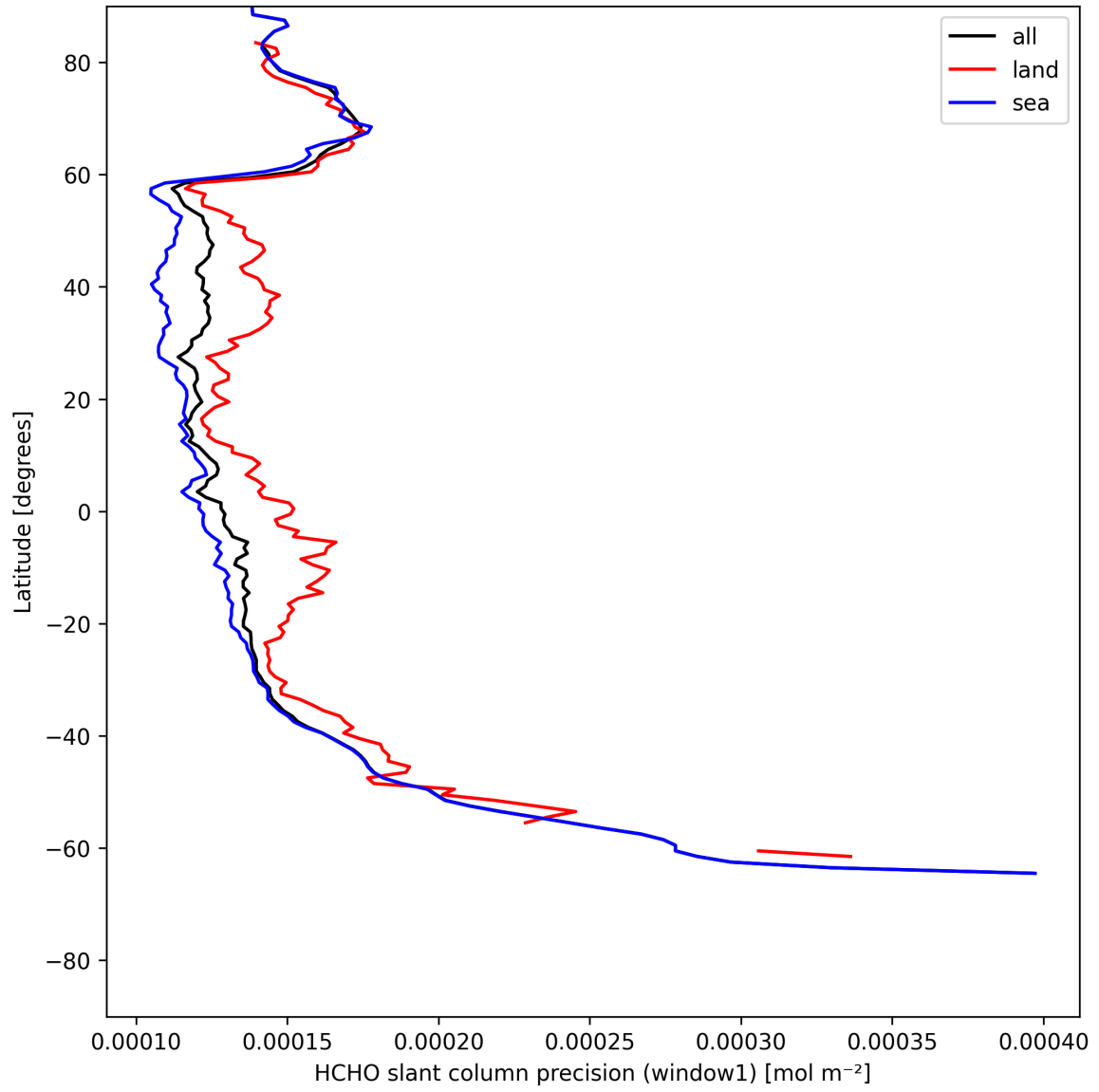
Figure 23: Zonal average of “HCHO slant column precision (window1)” for 2025-05-19 to 2025-05-19.
