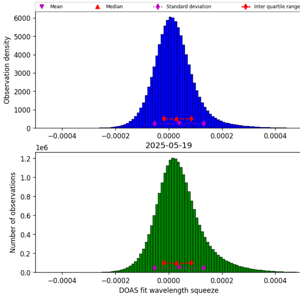
Figure 43: Histogram of “DOAS fit wavelength squeeze” for 2025-05-19 to 2025-05-19
