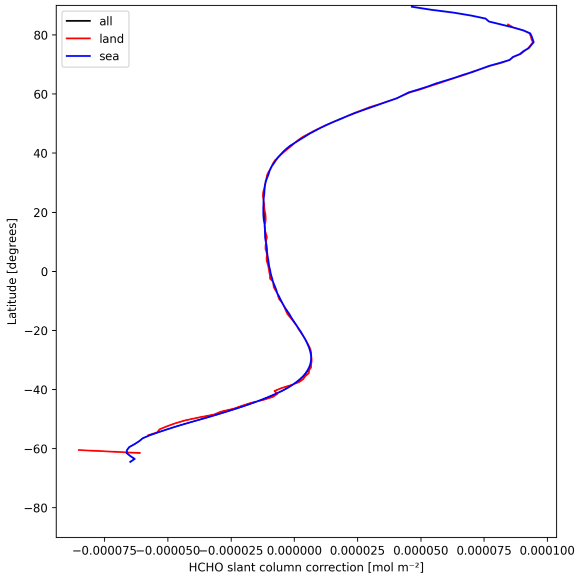
Figure 31: Zonal average of “HCHO slant column correction” for 2025-05-19 to 2025-05-19.
