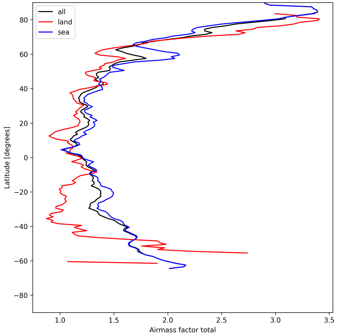
Figure 24: Zonal average of “Airmass factor total” for 2025-05-19 to 2025-05-19.
