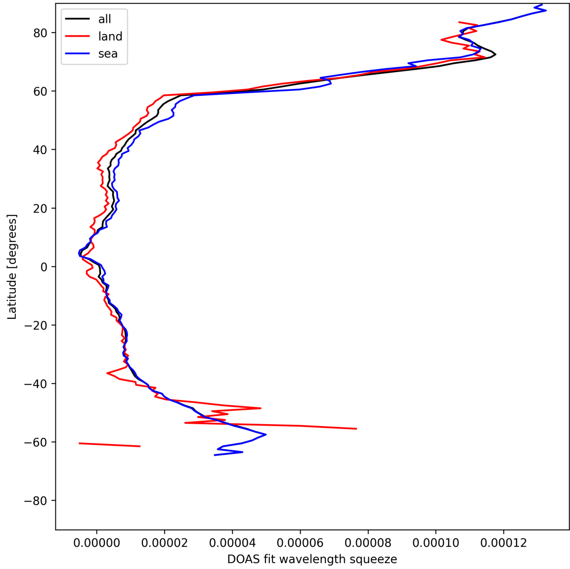
Figure 29: Zonal average of “DOAS fit wavelength squeeze” for 2025-05-19 to 2025-05-19.
