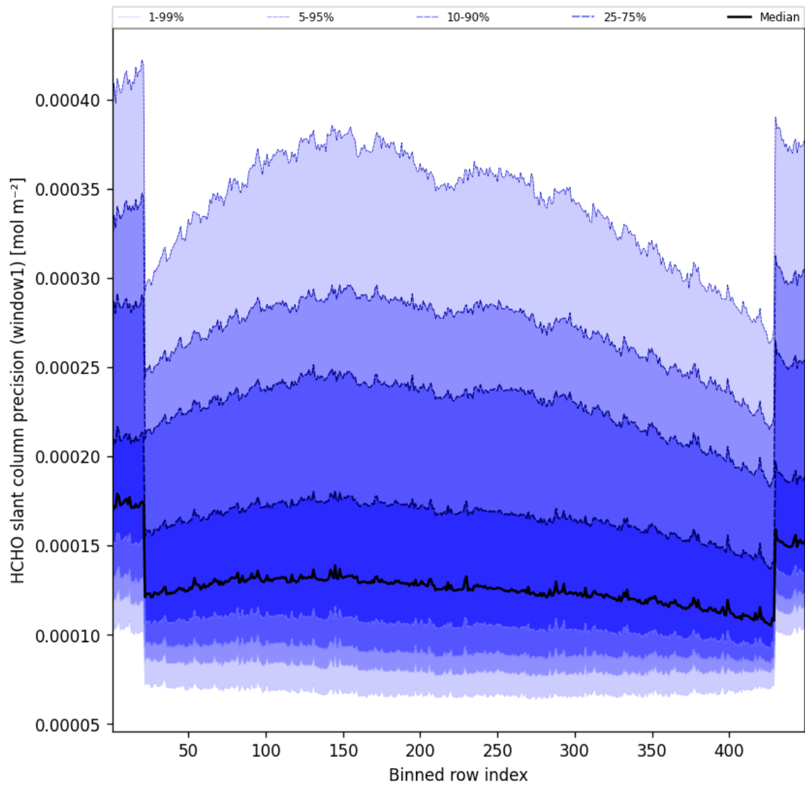
Figure 51: Along track statistics of “HCHO slant column precision (window1)” for 2025-05-19 to 2025-05-19
