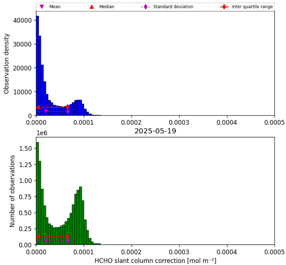
Figure 45: Histogram of “HCHO slant column correction” for 2025-05-19 to 2025-05-19
