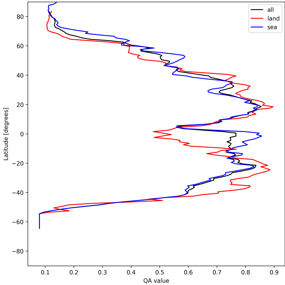
Figure 18: Zonal average of “QA value” for 2025-05-19 to 2025-05-19.
