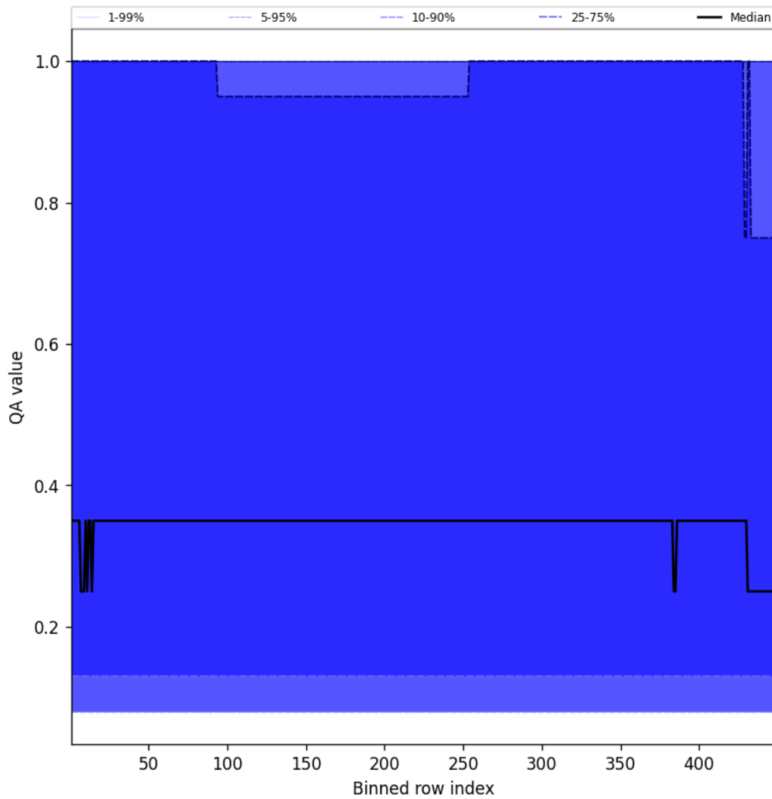
Figure 46: Along track statistics of “QA value” for 2025-05-19 to 2025-05-19
