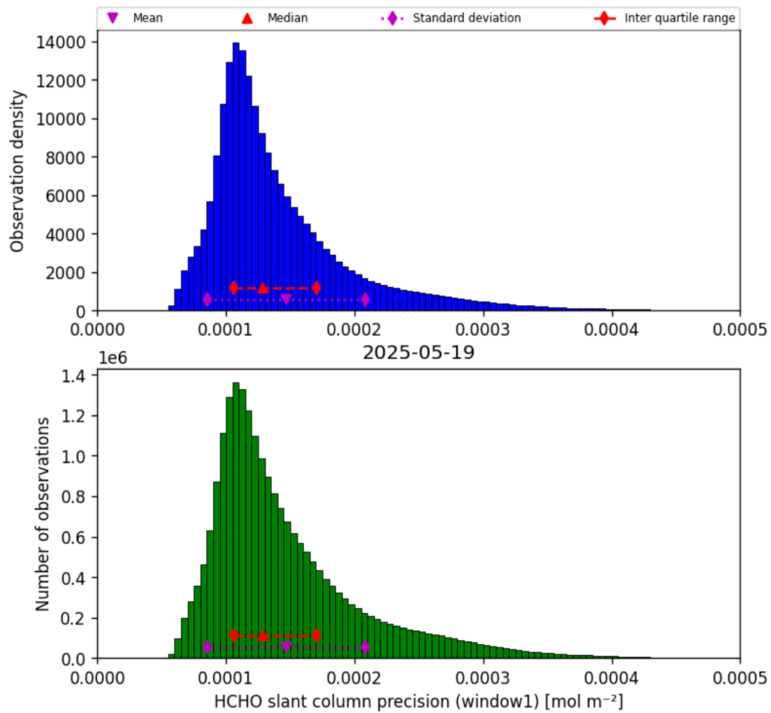
Figure 37: Histogram of “HCHO slant column precision (window1)” for 2025-05-19 to 2025-05-19
