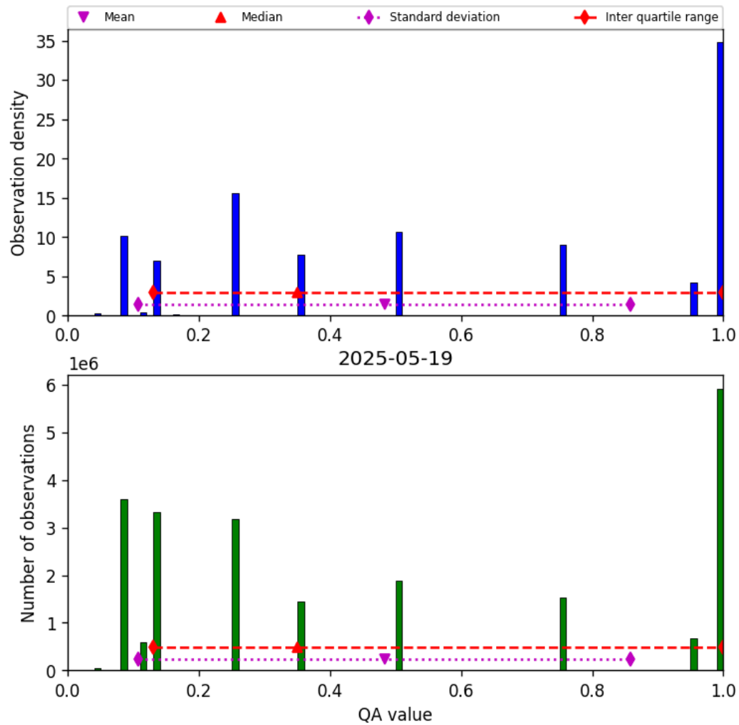
Figure 32: Histogram of “QA value” for 2025-05-19 to 2025-05-19
