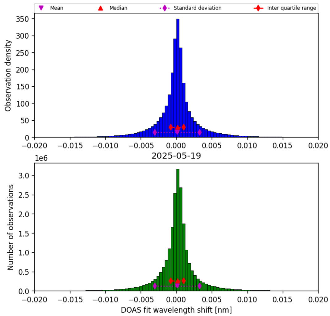
Figure 42: Histogram of “DOAS fit wavelength shift” for 2025-05-19 to 2025-05-19
