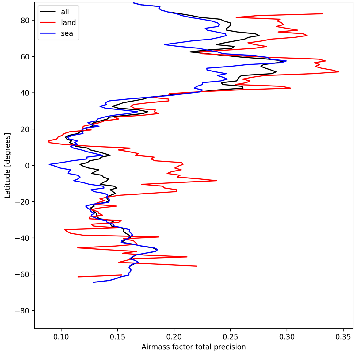
Figure 25: Zonal average of “Airmass factor total precision” for 2025-05-19 to 2025-05-19.
