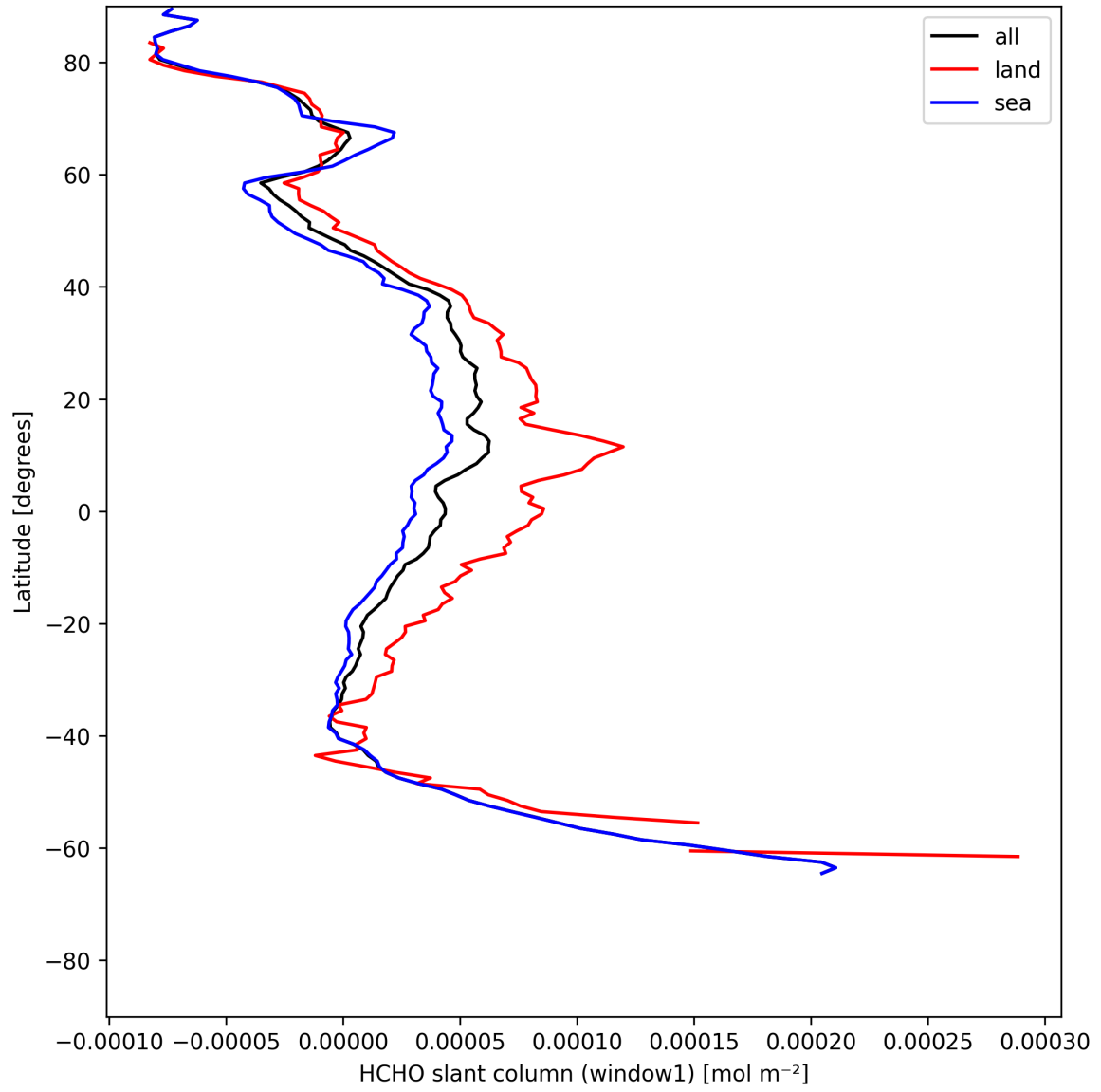
Figure 22: Zonal average of “HCHO slant column (window1)” for 2025-05-19 to 2025-05-19.
