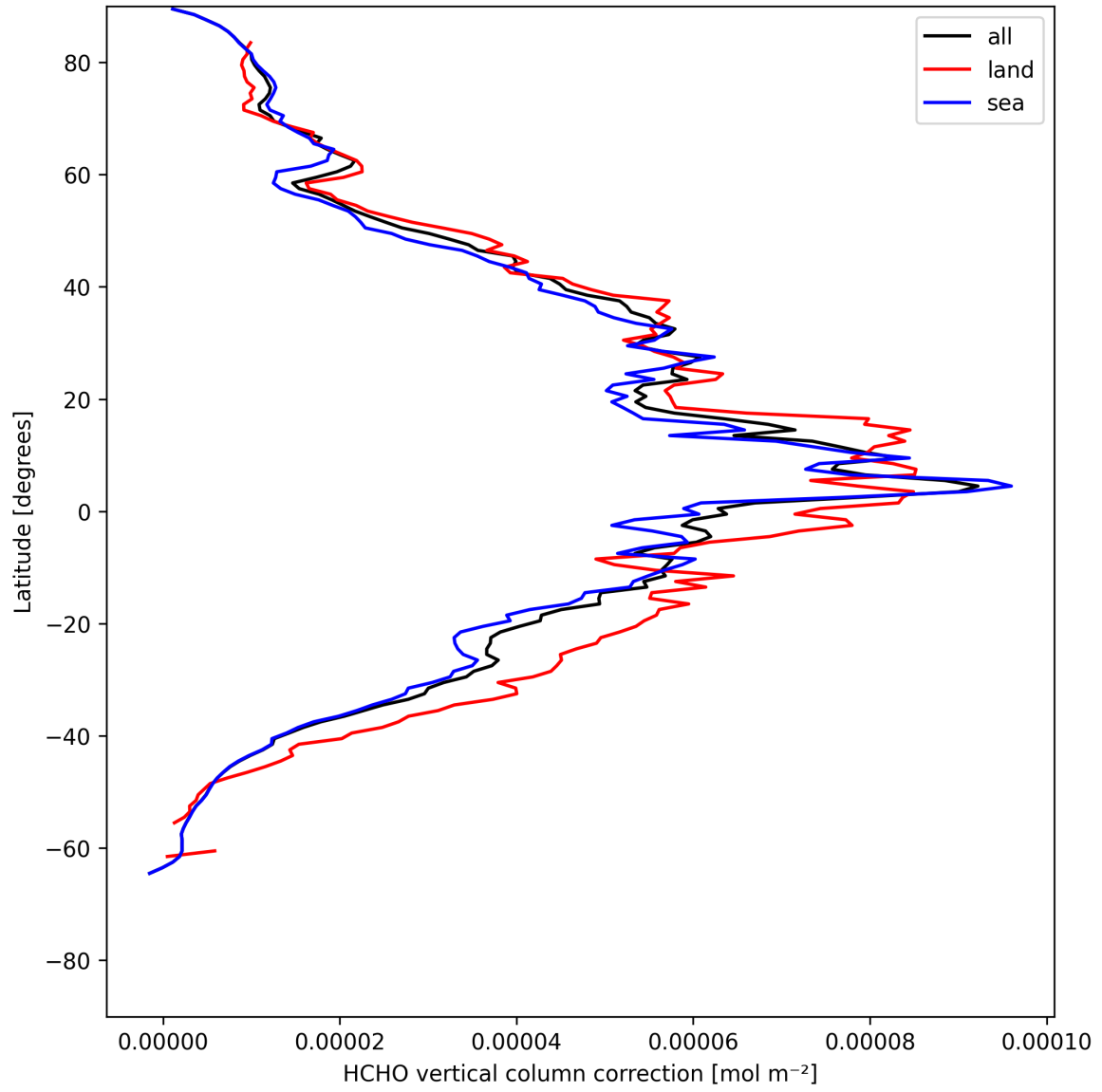
Figure 21: Zonal average of “HCHO vertical column correction” for 2025-05-19 to 2025-05-19.
