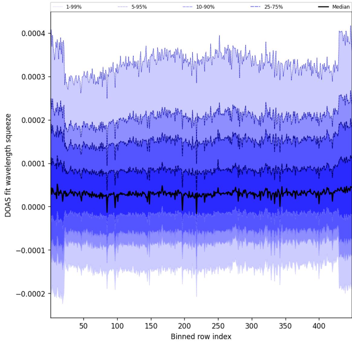
Figure 57: Along track statistics of “DOAS fit wavelength squeeze” for 2025-05-19 to 2025-05-19
