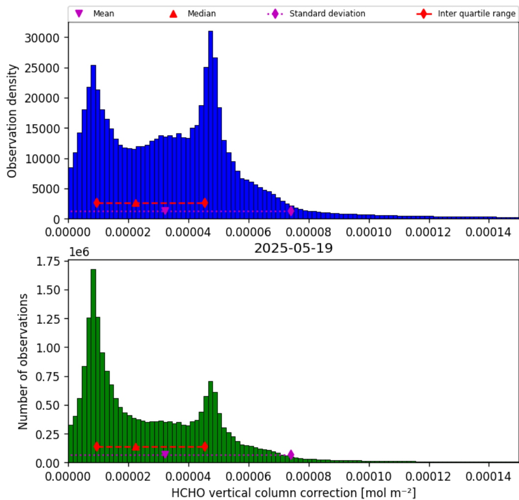
Figure 35: Histogram of “HCHO vertical column correction” for 2025-05-19 to 2025-05-19
