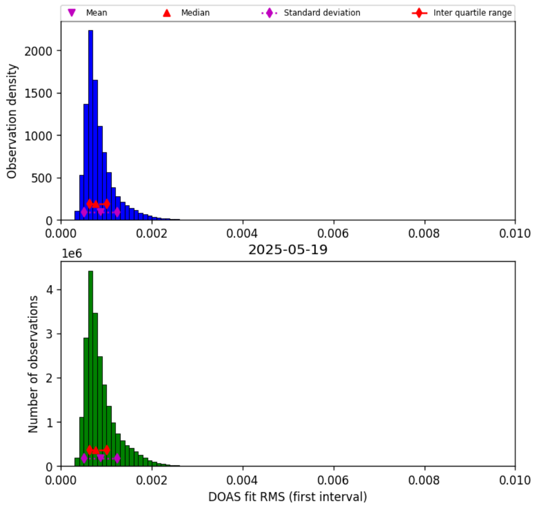
Figure 44: Histogram of “DOAS fit RMS (first interval)” for 2025-05-19 to 2025-05-19
