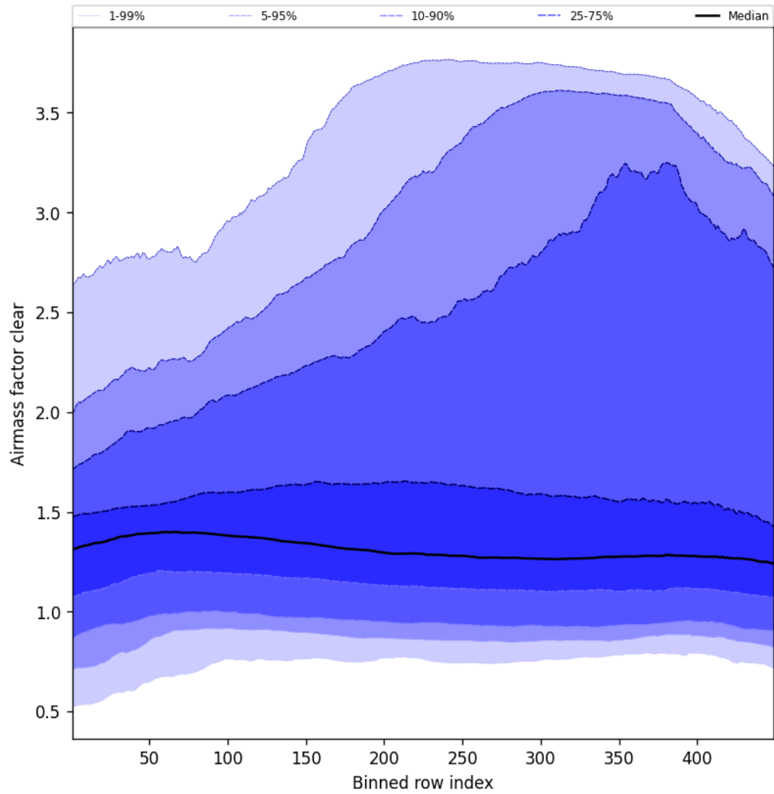
Figure 54: Along track statistics of “Airmass factor clear” for 2025-05-20 to 2025-05-21
