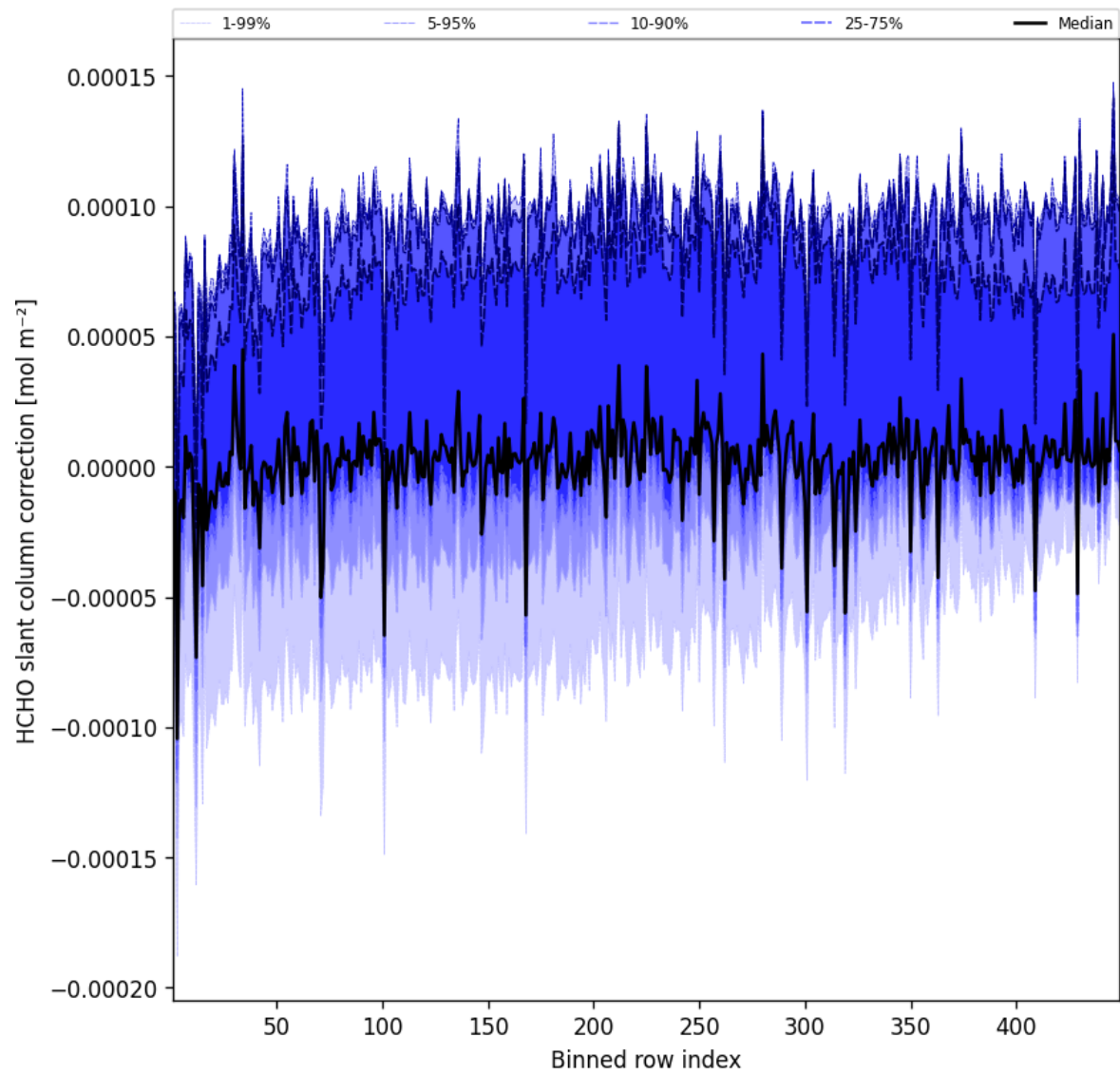
Figure 59: Along track statistics of “HCHO slant column correction” for 2025-05-20 to 2025-05-21
