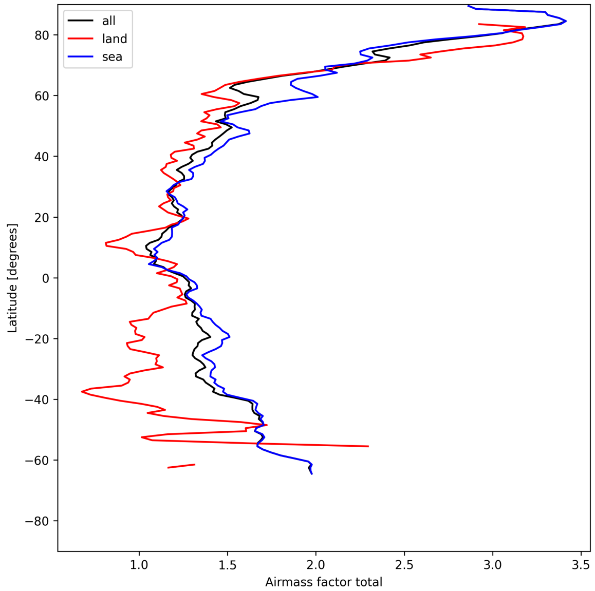
Figure 24: Zonal average of “Airmass factor total” for 2025-05-20 to 2025-05-21.
