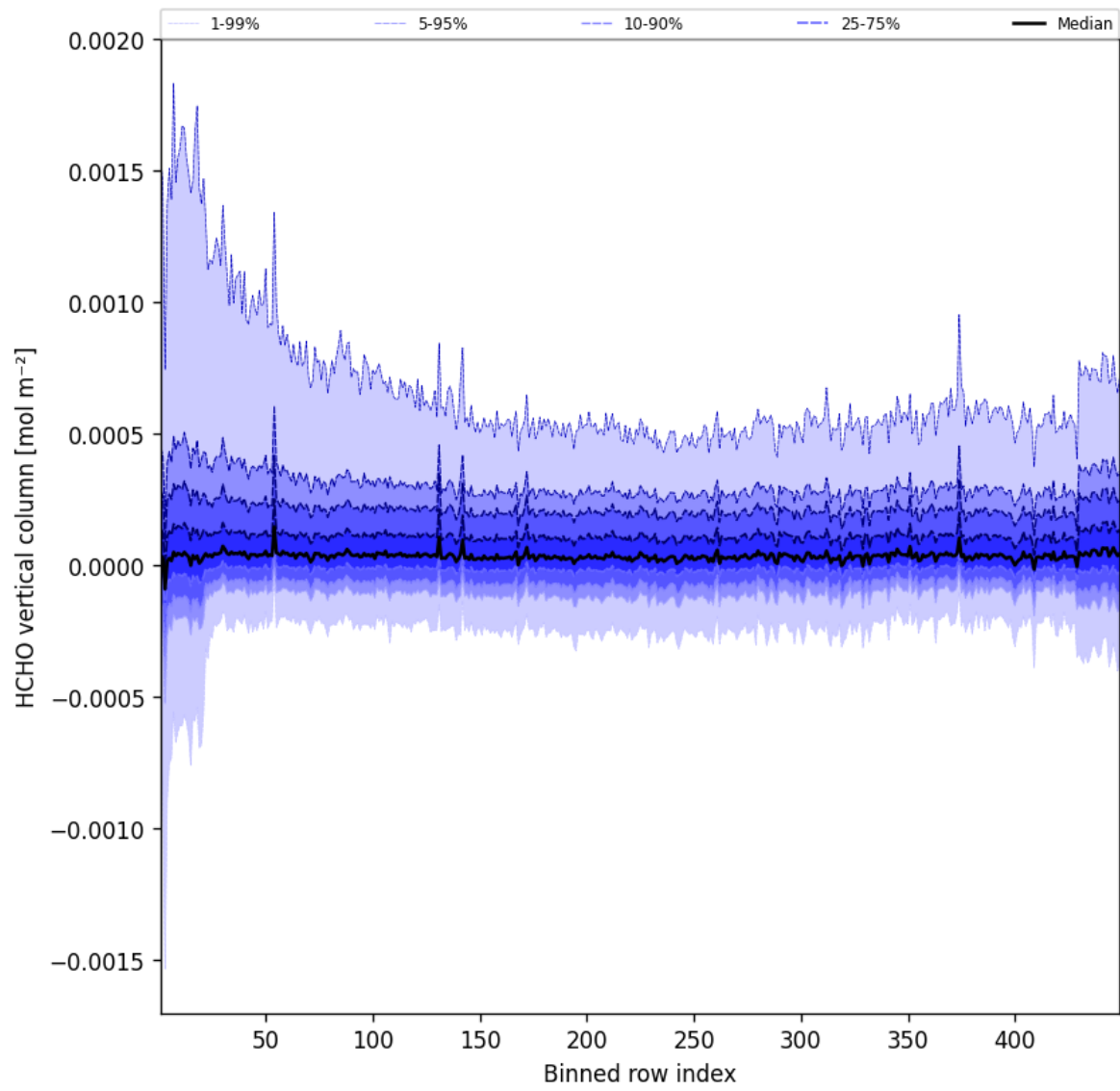
Figure 47: Along track statistics of “HCHO vertical column” for 2025-05-20 to 2025-05-21
