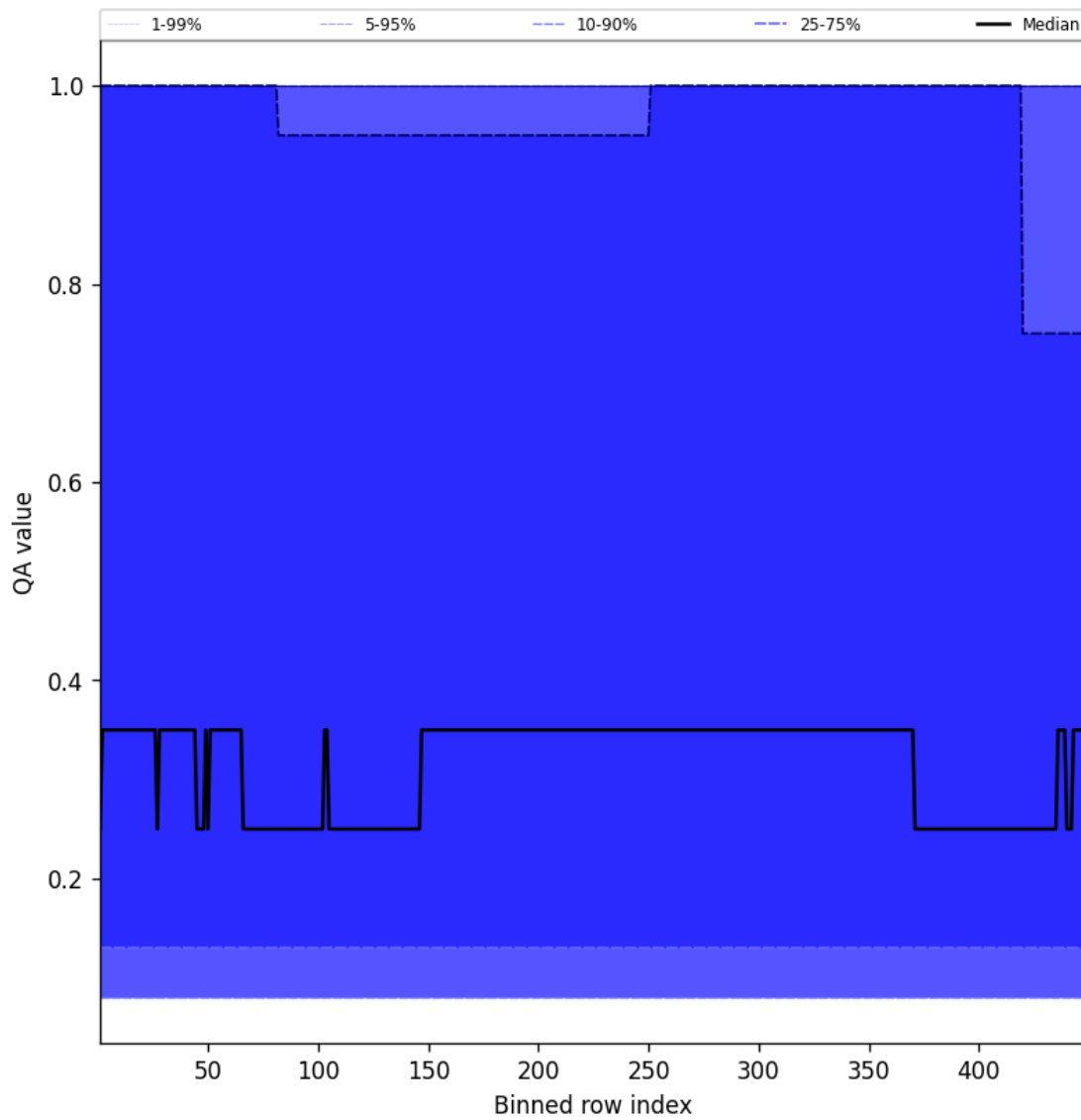
Figure 46: Along track statistics of “QA value” for 2025-05-20 to 2025-05-21
