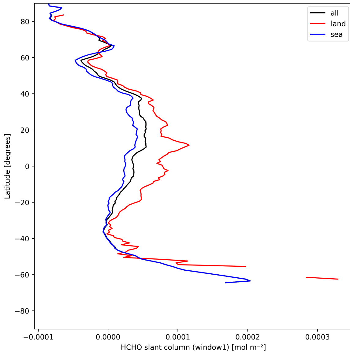
Figure 22: Zonal average of “HCHO slant column (window1)” for 2025-05-20 to 2025-05-21.
