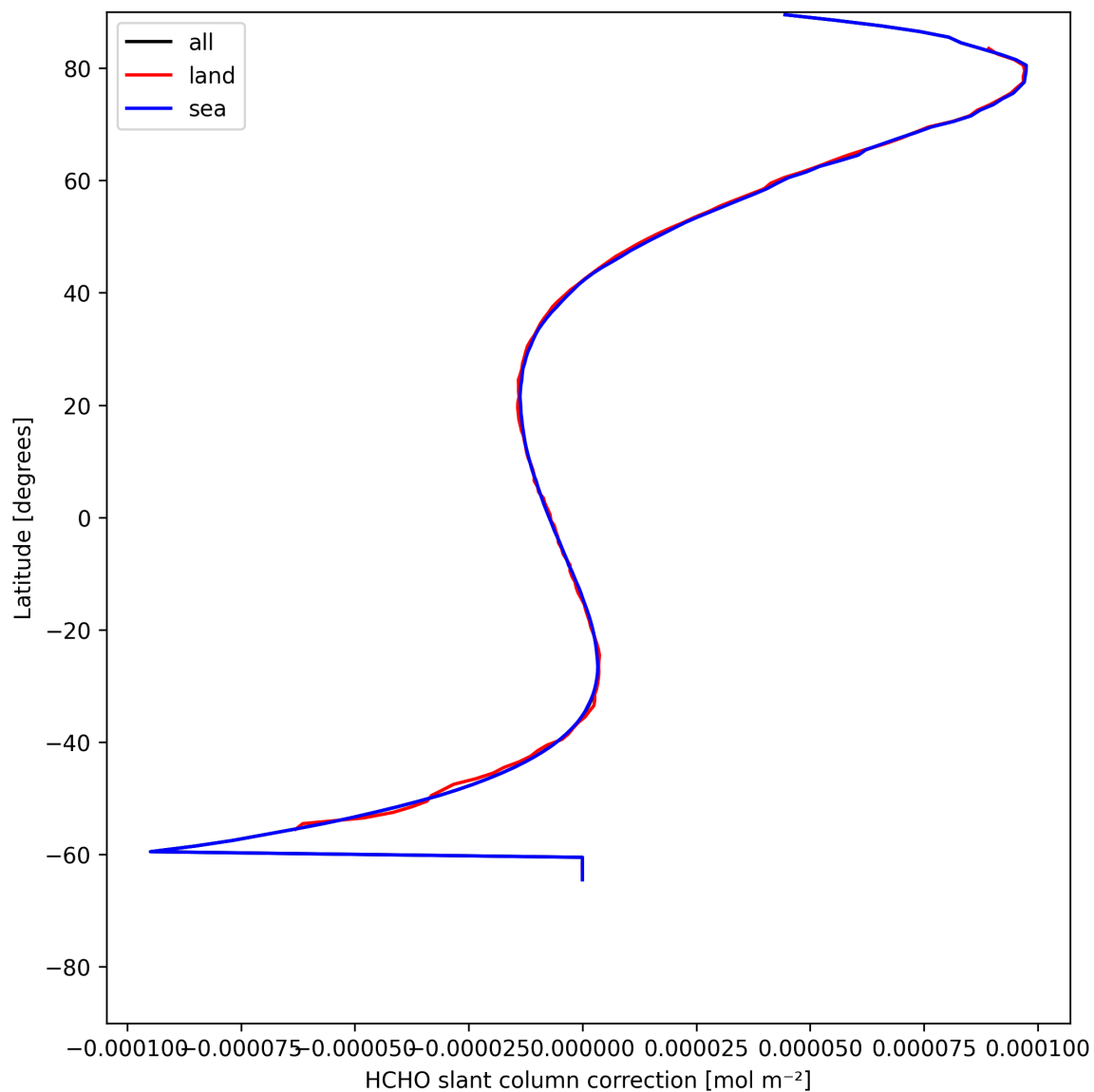
Figure 31: Zonal average of “HCHO slant column correction” for 2025-05-20 to 2025-05-21.
