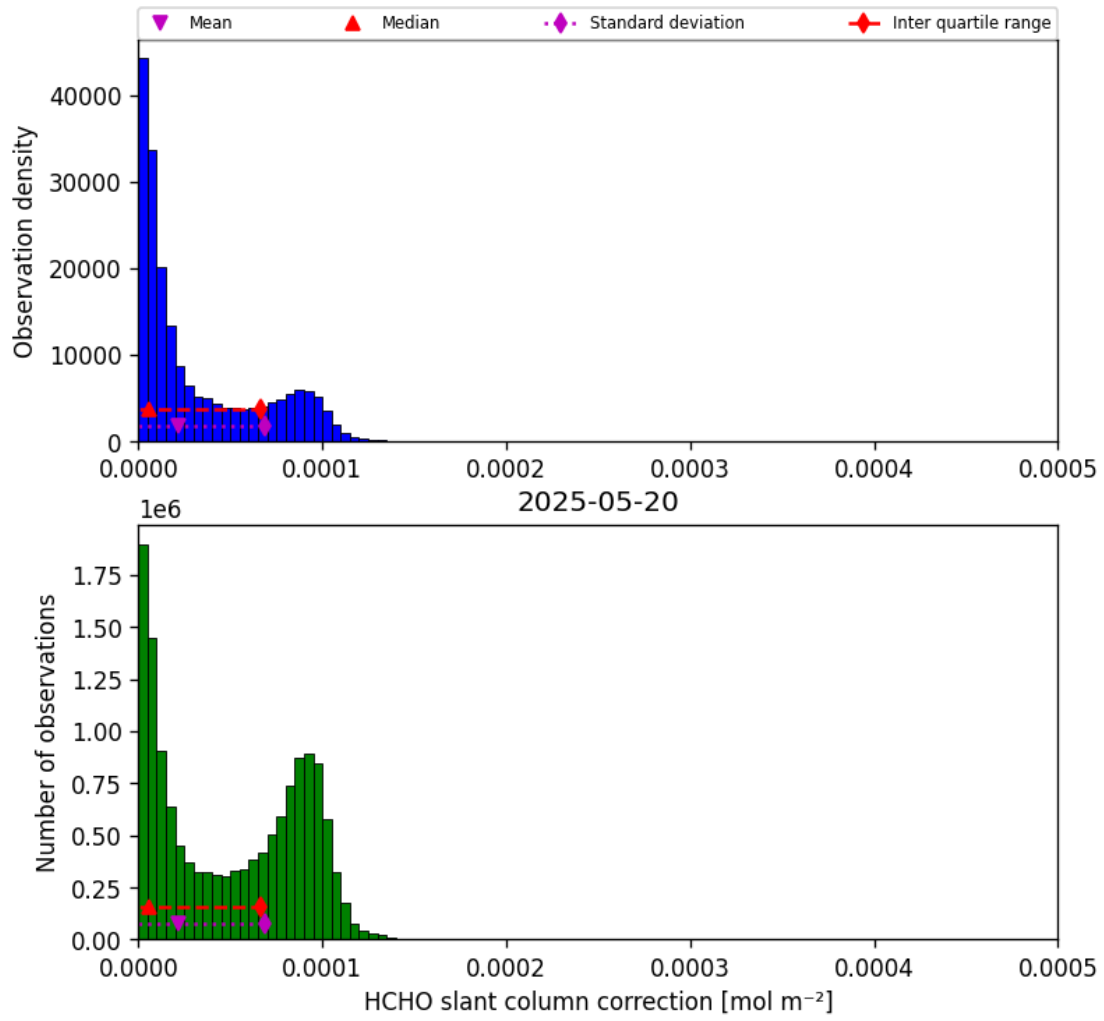
Figure 45: Histogram of "HCHO slant column correction" for 2025-05-20 to 2025-05-21
