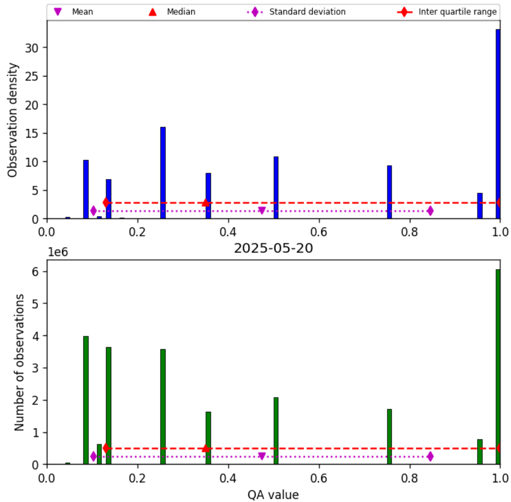
Figure 32: Histogram of “QA value” for 2025-05-20 to 2025-05-21
