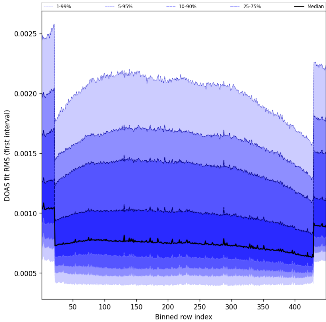
Figure 58: Along track statistics of “DOAS fit RMS (first interval)” for 2025-05-20 to 2025-05-21
