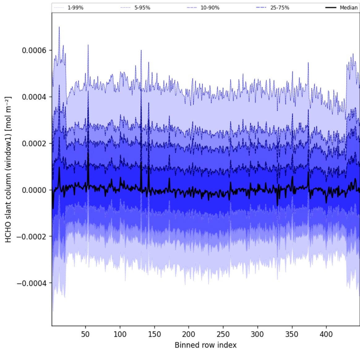
Figure 50: Along track statistics of “HCHO slant column (window1)” for 2025-05-20 to 2025-05-21
