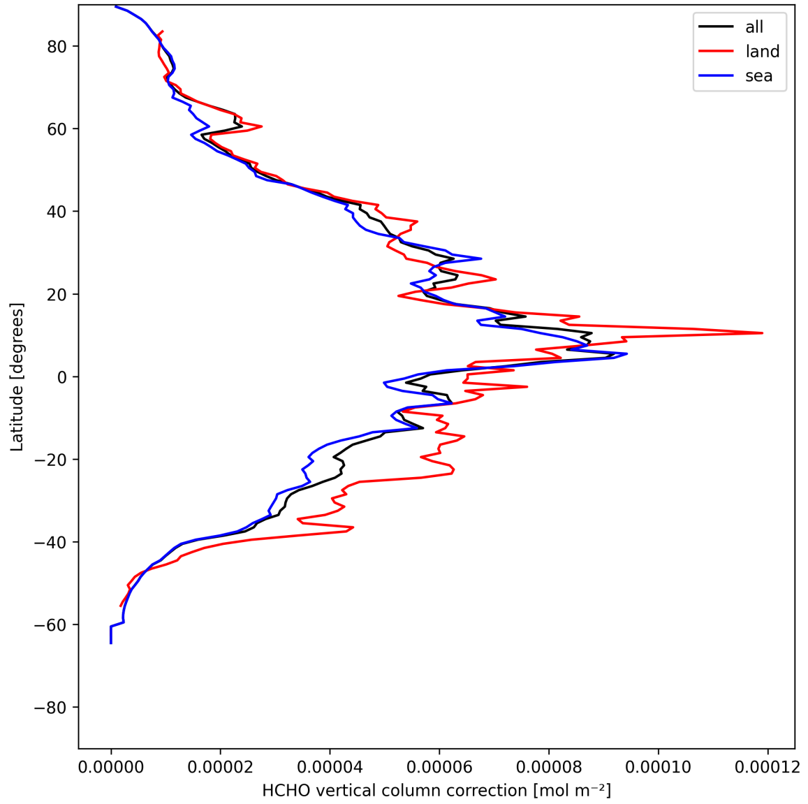
Figure 21: Zonal average of “HCHO vertical column correction” for 2025-05-20 to 2025-05-21.
