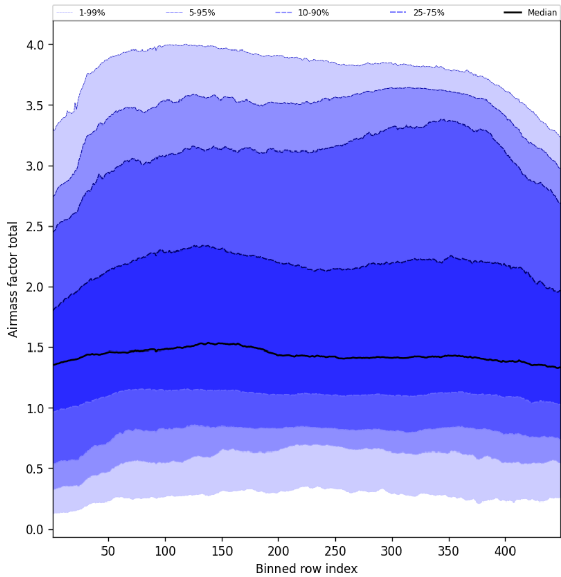
Figure 52: Along track statistics of “Airmass factor total” for 2025-05-20 to 2025-05-21
