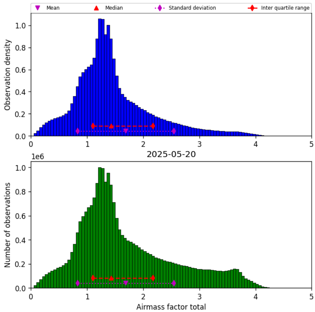
Figure 38: Histogram of “Airmass factor total” for 2025-05-20 to 2025-05-21
