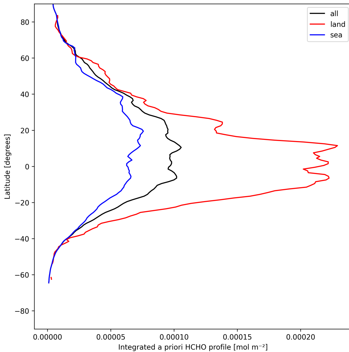
Figure 27: Zonal average of “Integrated a priori HCHO profile” for 2025-05-20 to 2025-05-21.
