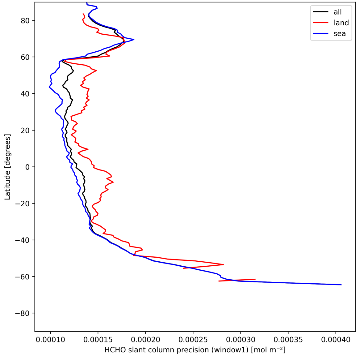
Figure 23: Zonal average of “HCHO slant column precision (window1)” for 2025-05-20 to 2025-05-21.
