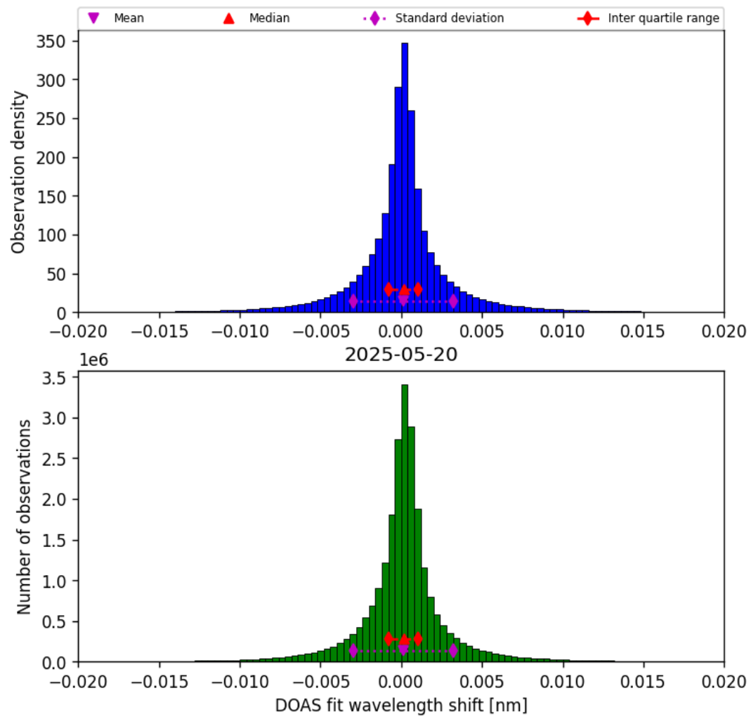
Figure 42: Histogram of “DOAS fit wavelength shift” for 2025-05-20 to 2025-05-21
