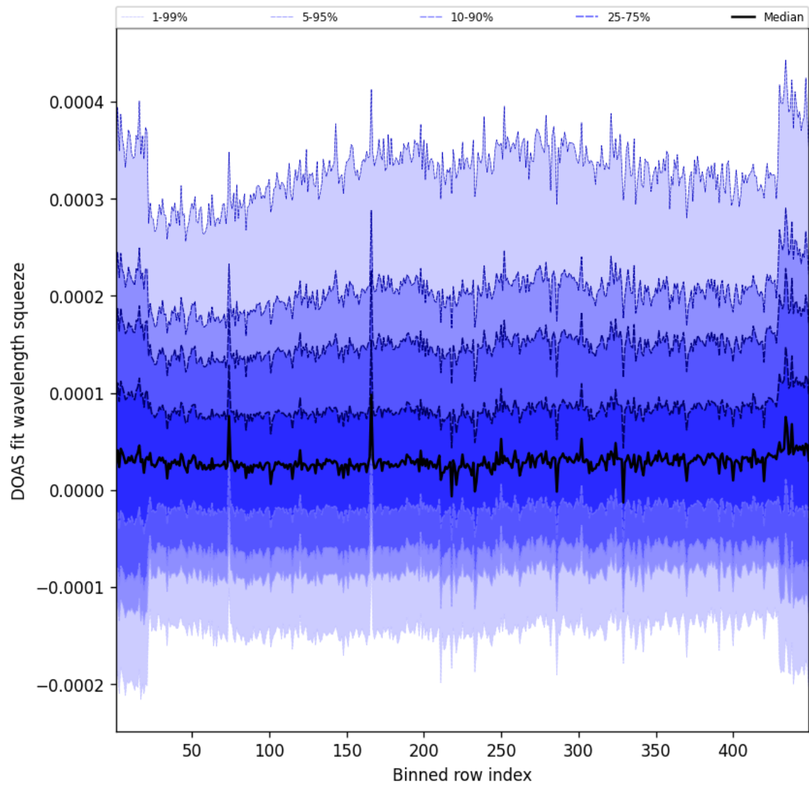
Figure 57: Along track statistics of “DOAS fit wavelength squeeze” for 2025-05-21 to 2025-05-22
