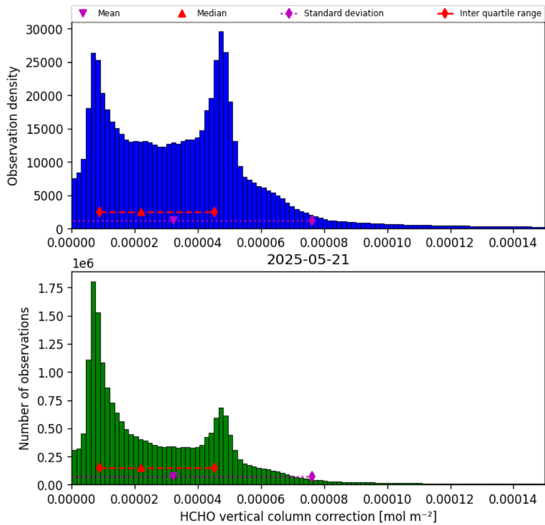
Figure 35: Histogram of “HCHO vertical column correction” for 2025-05-21 to 2025-05-22
