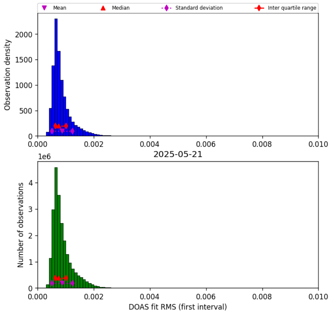
Figure 44: Histogram of "DOAS fit RMS (first interval)" for 2025-05-21 to 2025-05-22
