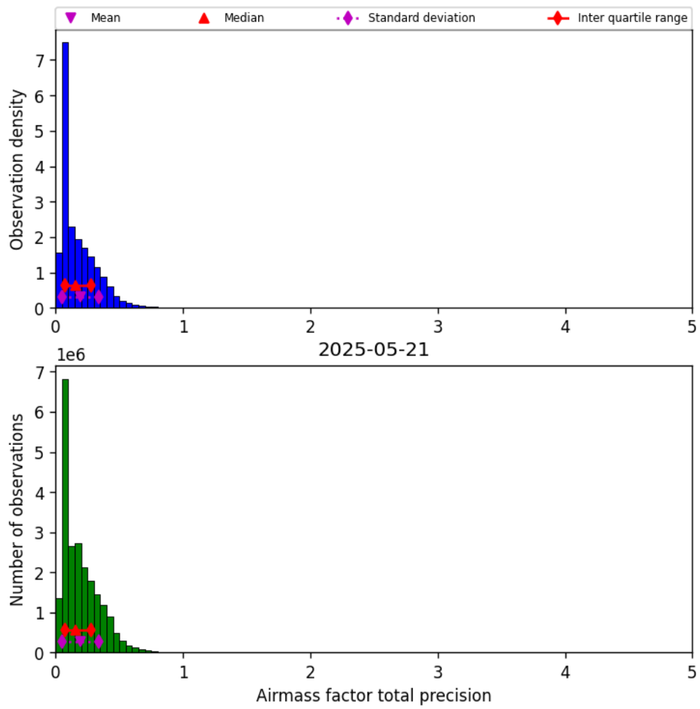
Figure 39: Histogram of “Airmass factor total precision” for 2025-05-21 to 2025-05-22
