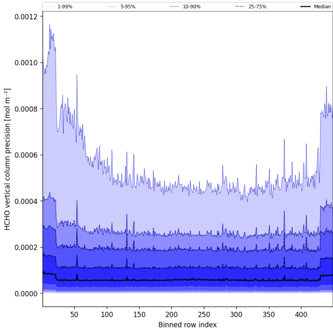
Figure 48: Along track statistics of “HCHO vertical column precision” for 2025-05-21 to 2025-05-22
