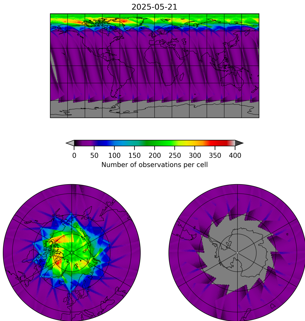
Figure 17: Map of the number of observations for 2025-05-21 to 2025-05-22
