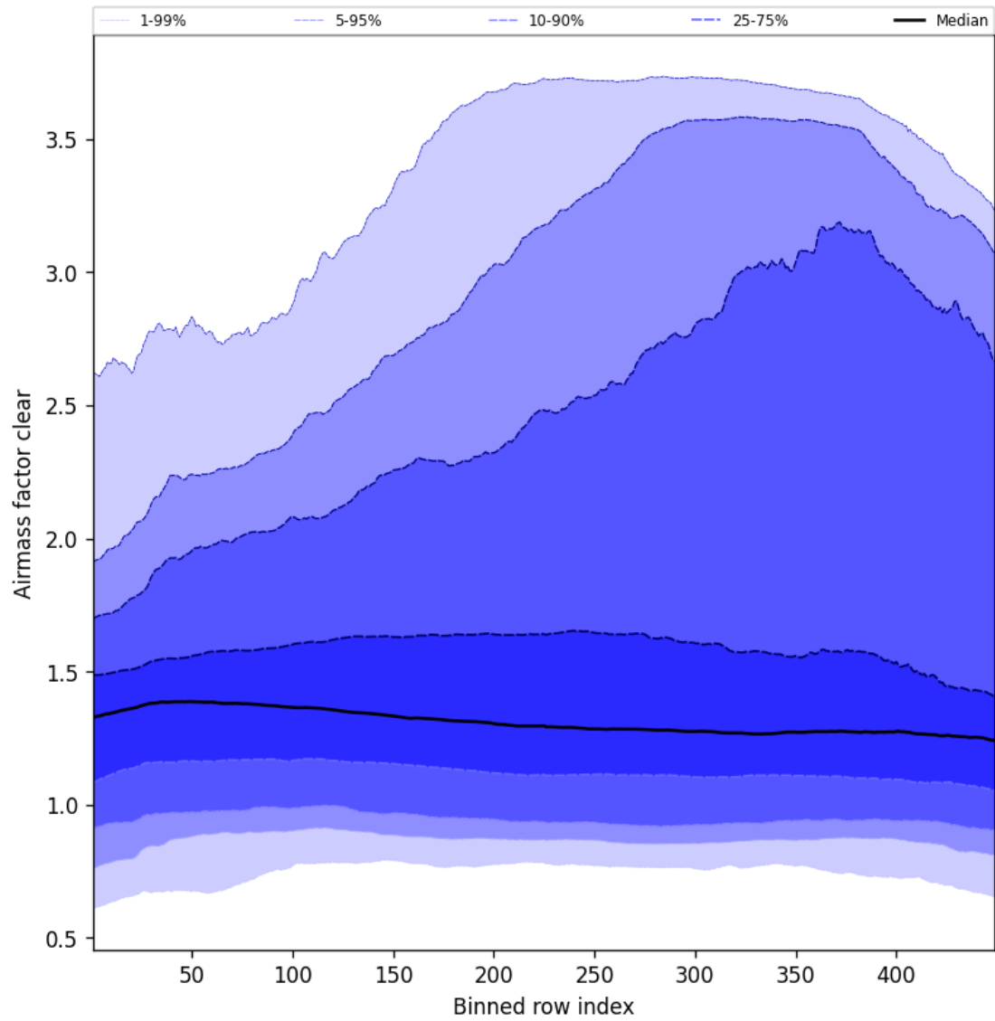
Figure 54: Along track statistics of “Airmass factor clear” for 2025-05-21 to 2025-05-22
