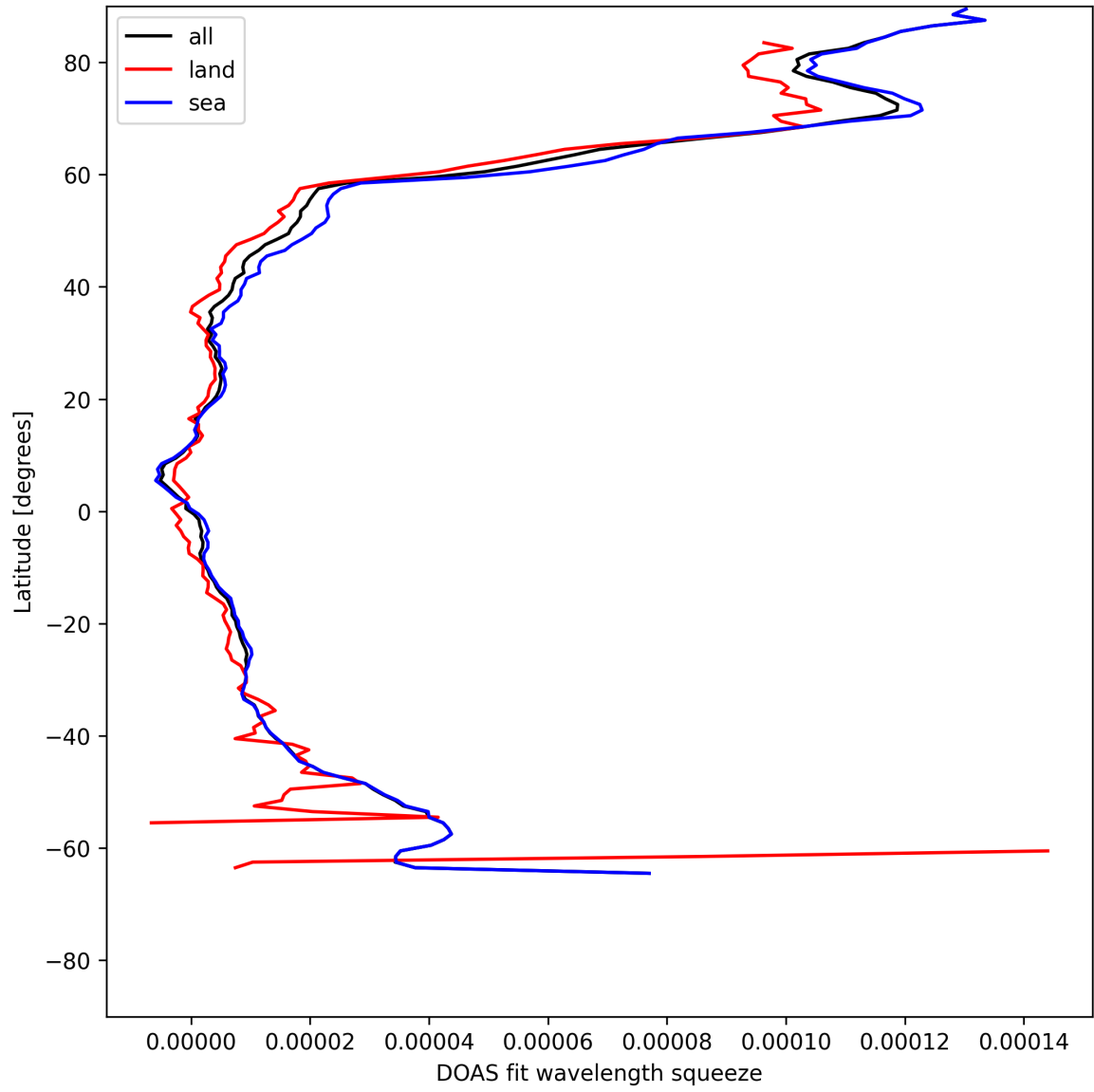
Figure 29: Zonal average of “DOAS fit wavelength squeeze” for 2025-05-21 to 2025-05-22.
