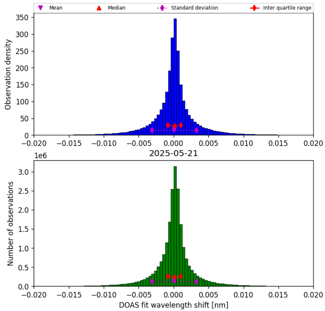
Figure 42: Histogram of “DOAS fit wavelength shift” for 2025-05-21 to 2025-05-22
