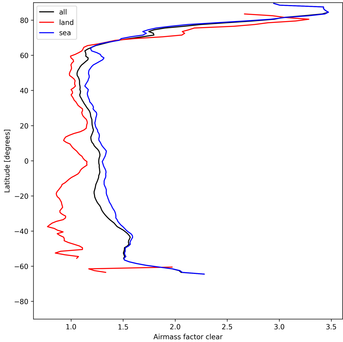
Figure 26: Zonal average of “Airmass factor clear” for 2025-05-21 to 2025-05-22.
