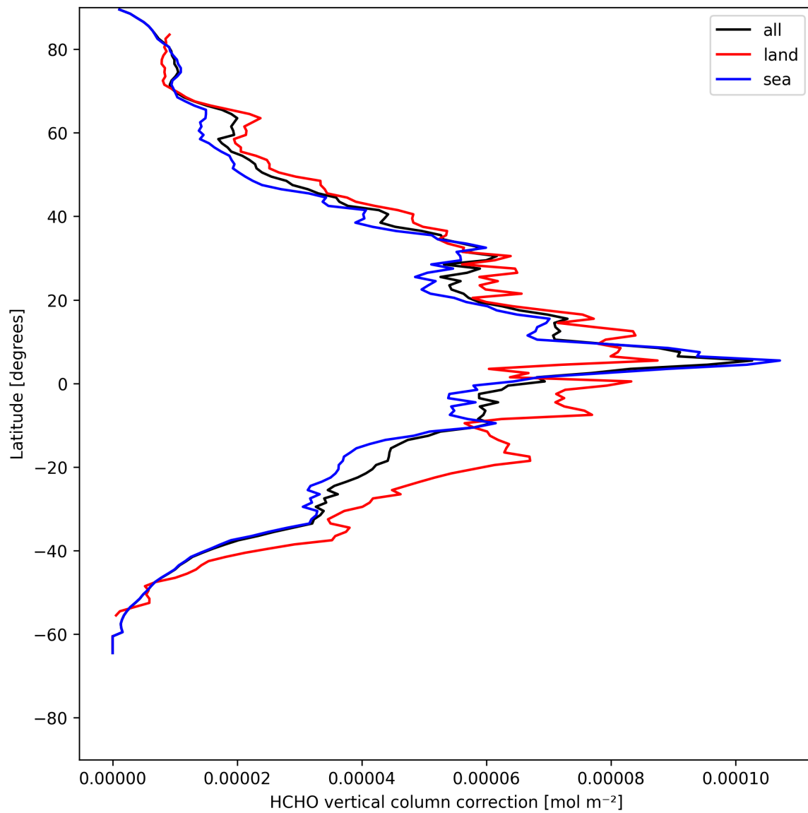
Figure 21: Zonal average of “HCHO vertical column correction” for 2025-05-21 to 2025-05-22.
