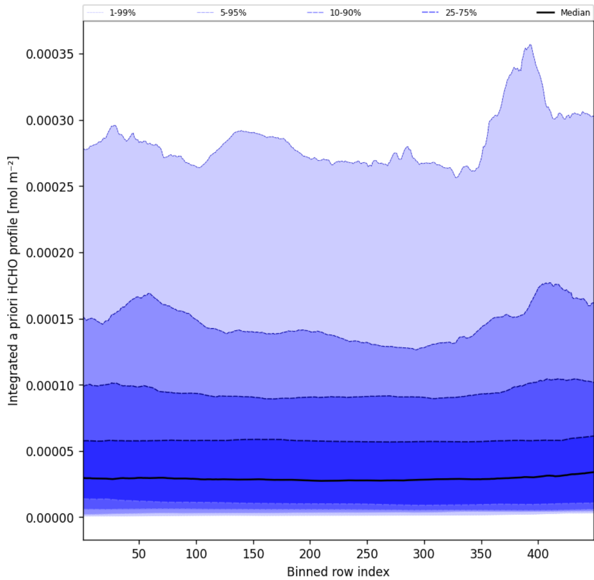
Figure 55: Along track statistics of "Integrated a priori HCHO profile" for 2025-05-21 to 2025-05-22
