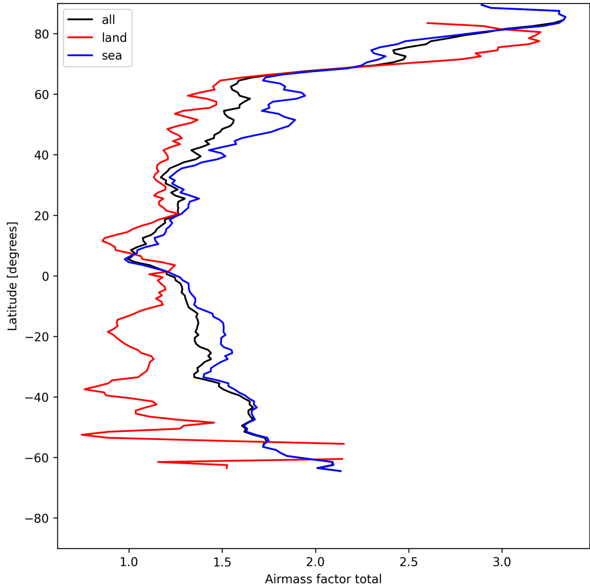
Figure 24: Zonal average of “Airmass factor total” for 2025-05-21 to 2025-05-22.
