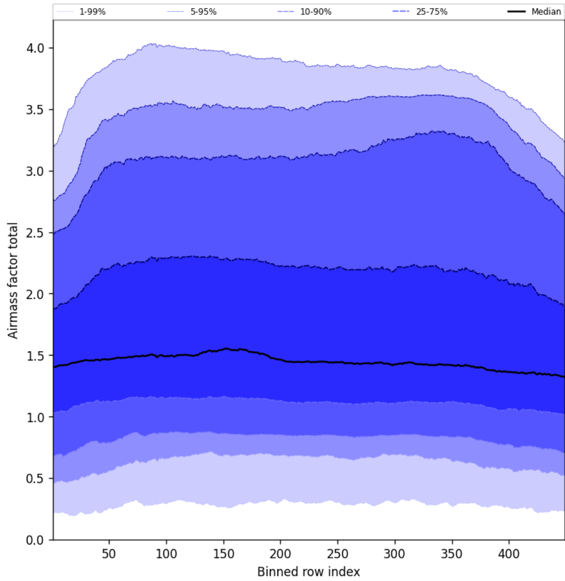
Figure 52: Along track statistics of “Airmass factor total” for 2025-05-21 to 2025-05-22
