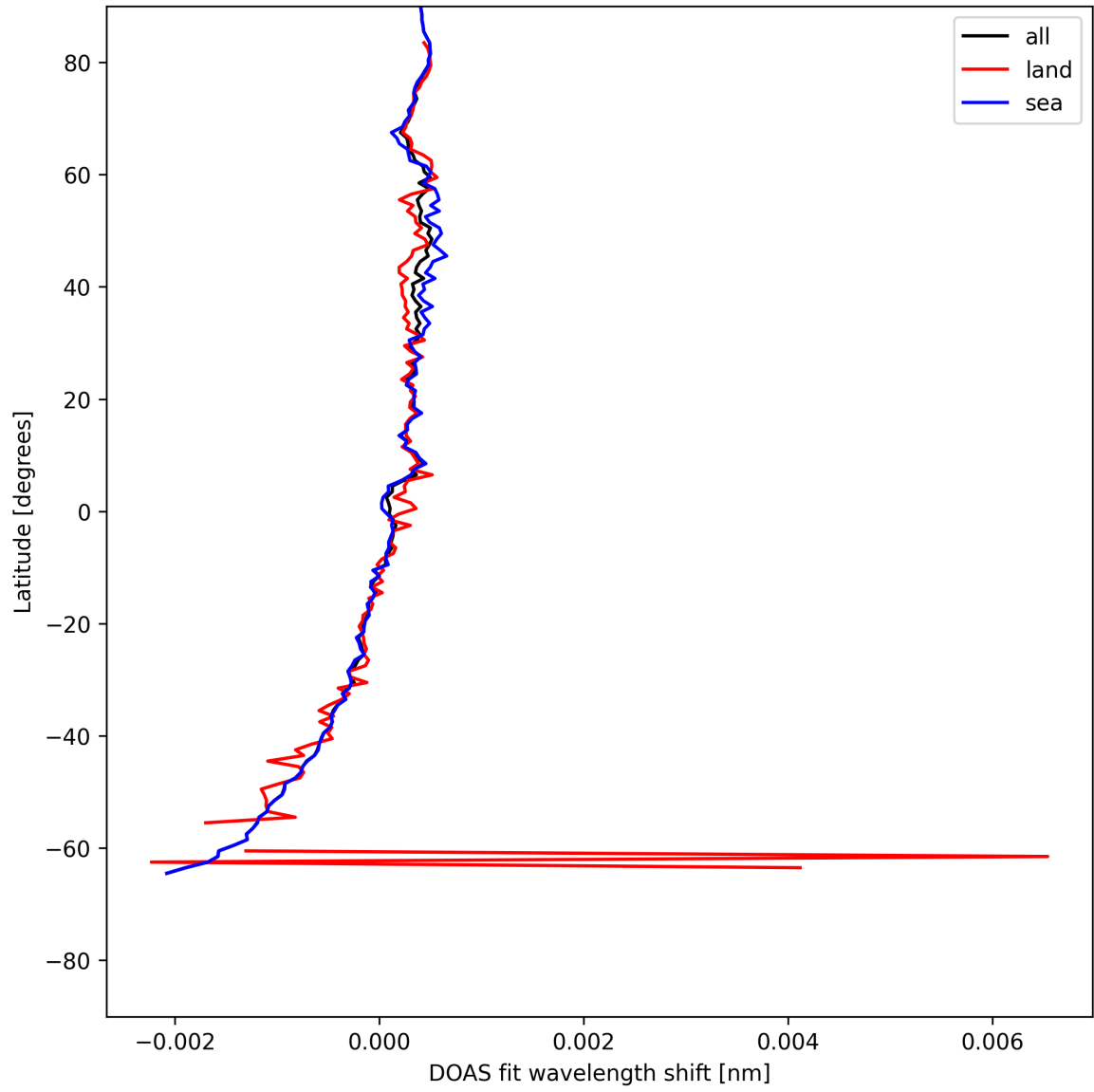
Figure 28: Zonal average of "DOAS fit wavelength shift" for 2025-05-21 to 2025-05-22.
