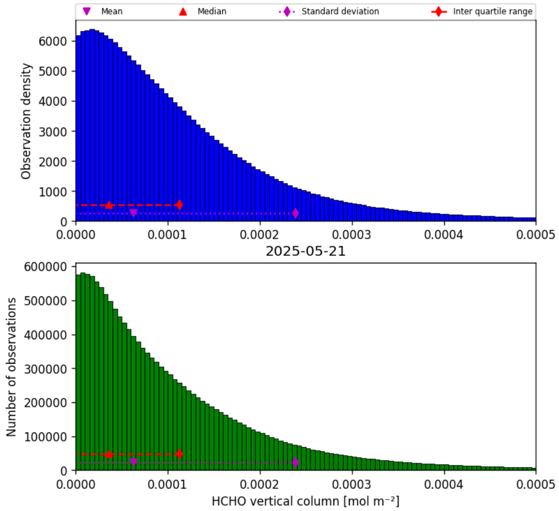
Figure 33: Histogram of “HCHO vertical column” for 2025-05-21 to 2025-05-22
