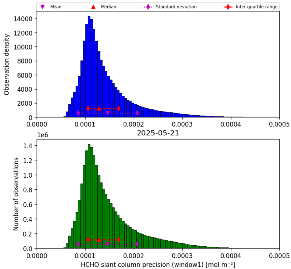
Figure 37: Histogram of “HCHO slant column precision (window1)” for 2025-05-21 to 2025-05-22
