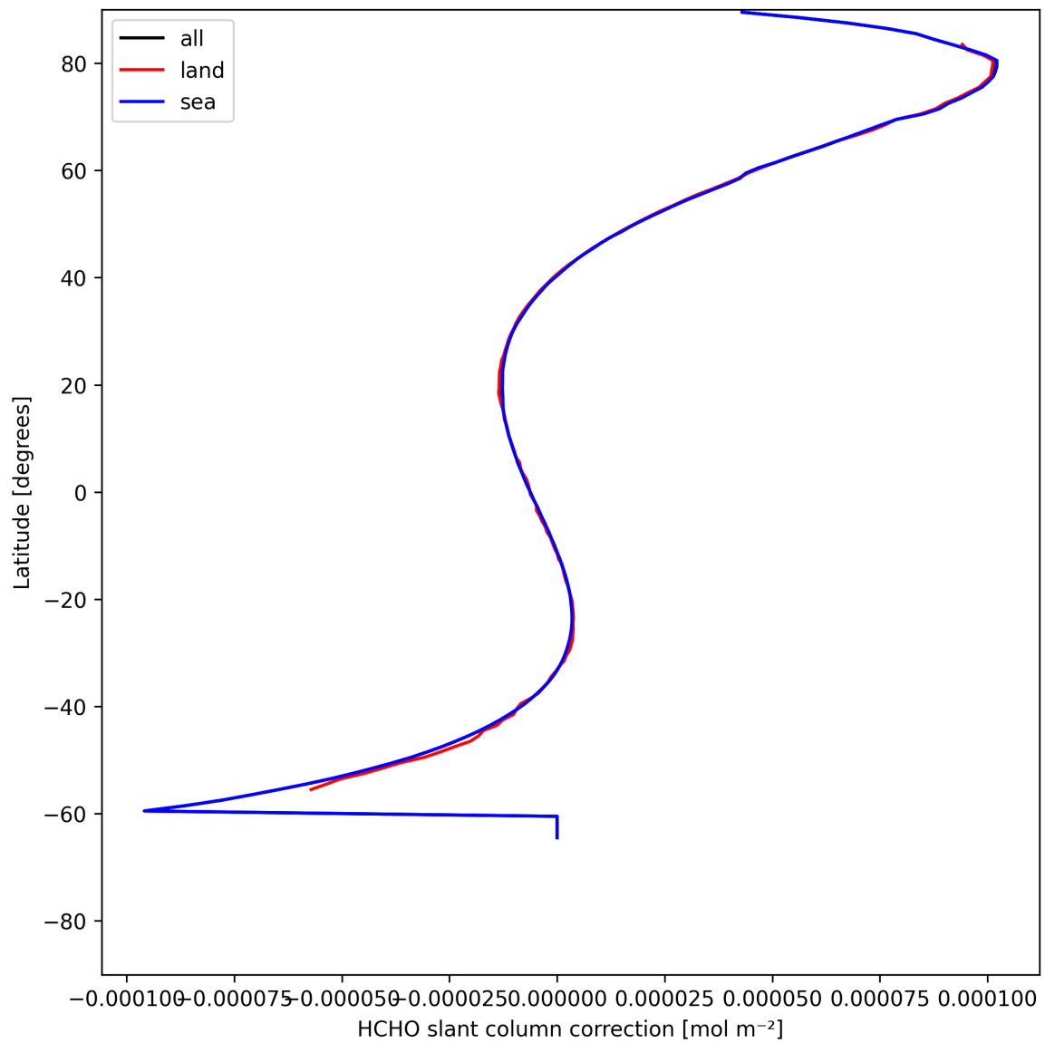
Figure 31: Zonal average of “HCHO slant column correction” for 2025-05-21 to 2025-05-22.
