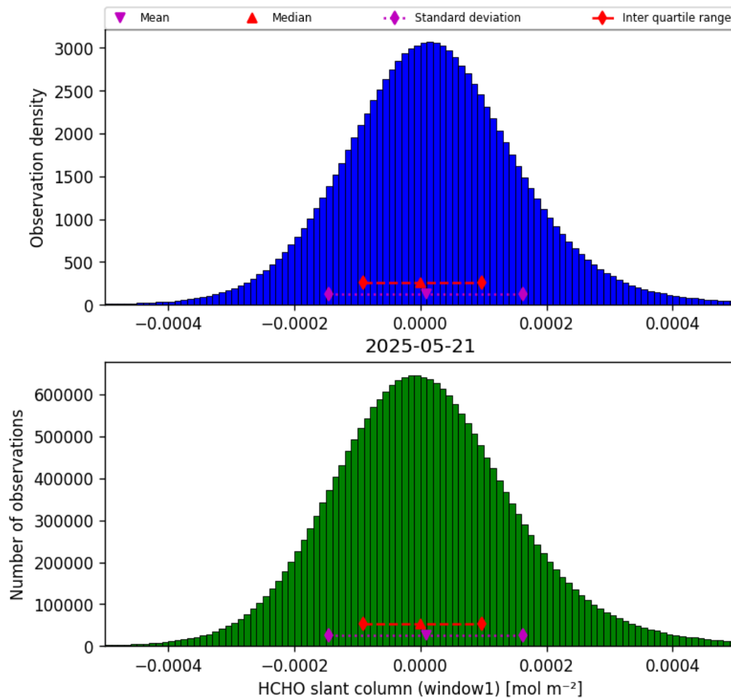
Figure 36: Histogram of “HCHO slant column (window1)” for 2025-05-21 to 2025-05-22
