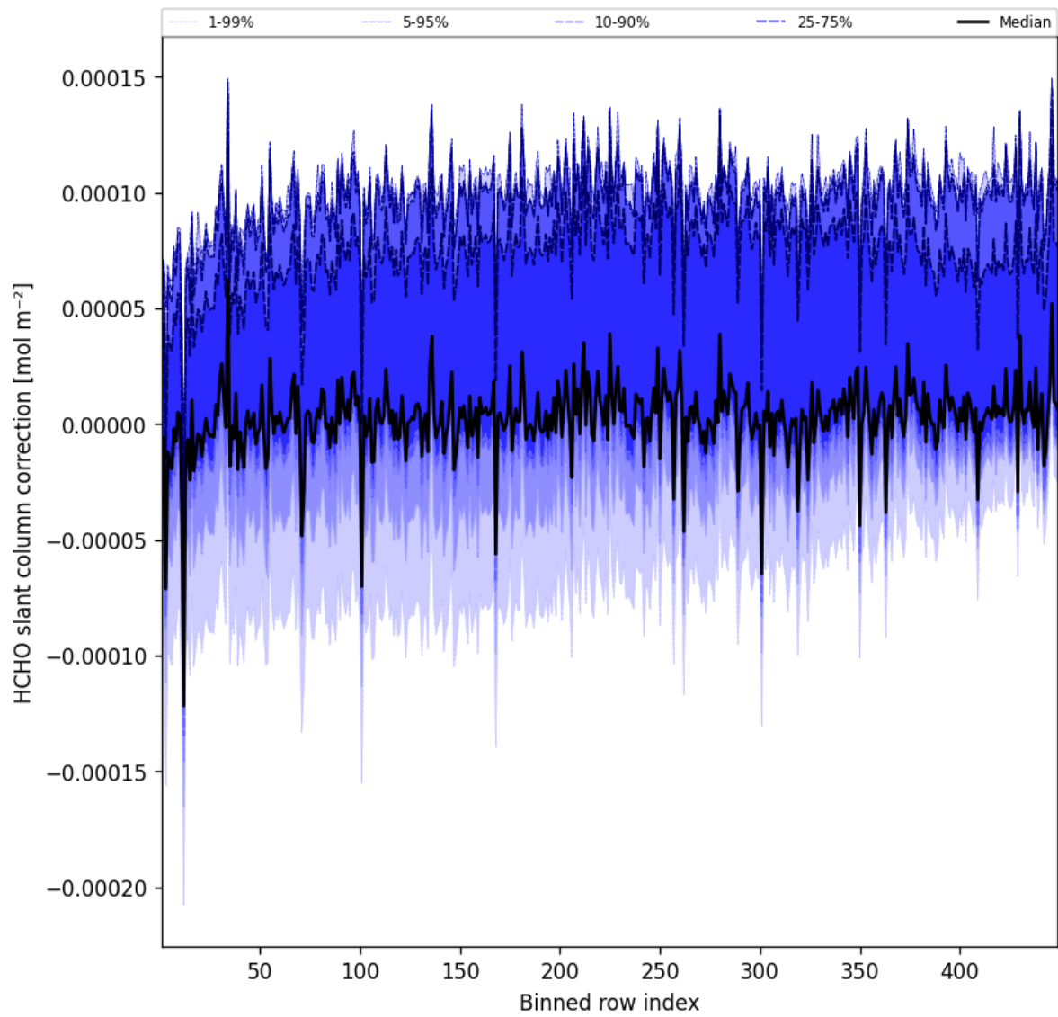
Figure 59: Along track statistics of “HCHO slant column correction” for 2025-05-21 to 2025-05-22
