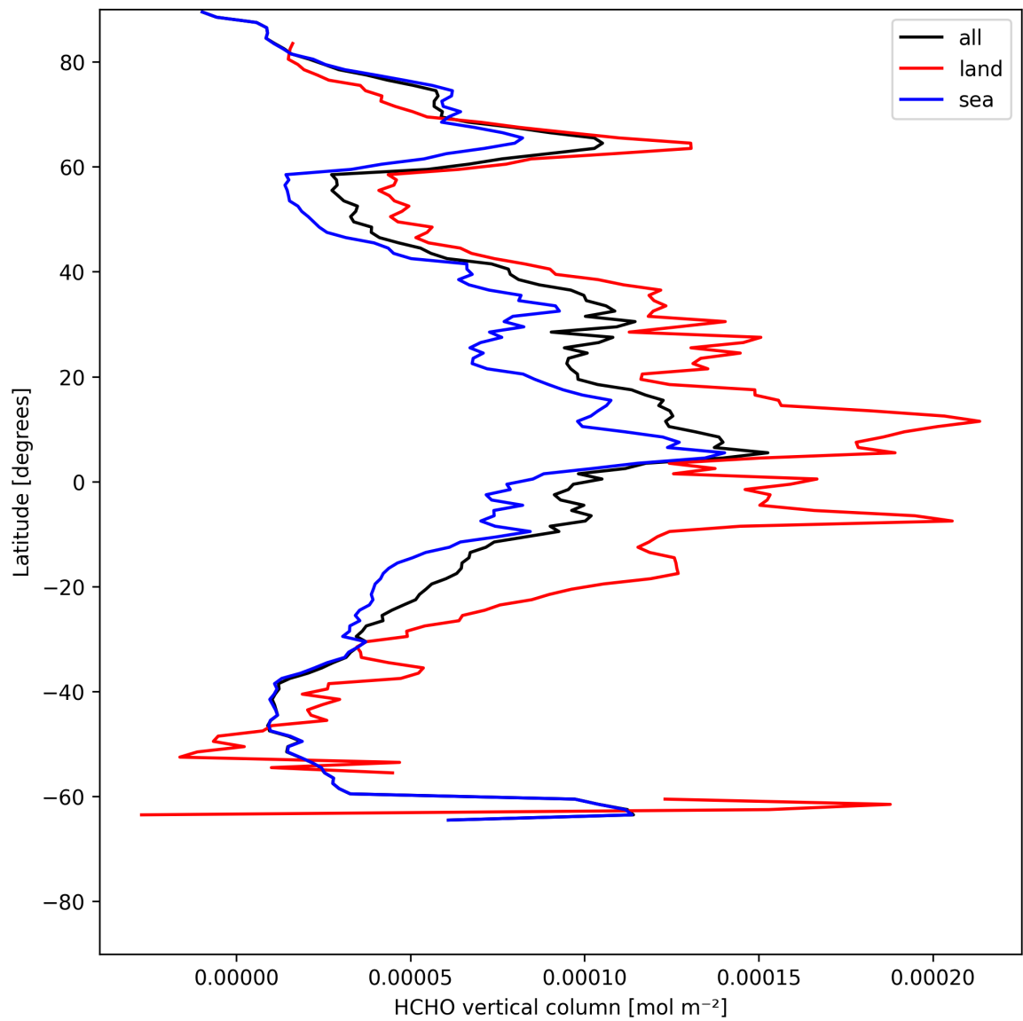
Figure 19: Zonal average of “HCHO vertical column” for 2025-05-21 to 2025-05-22.
