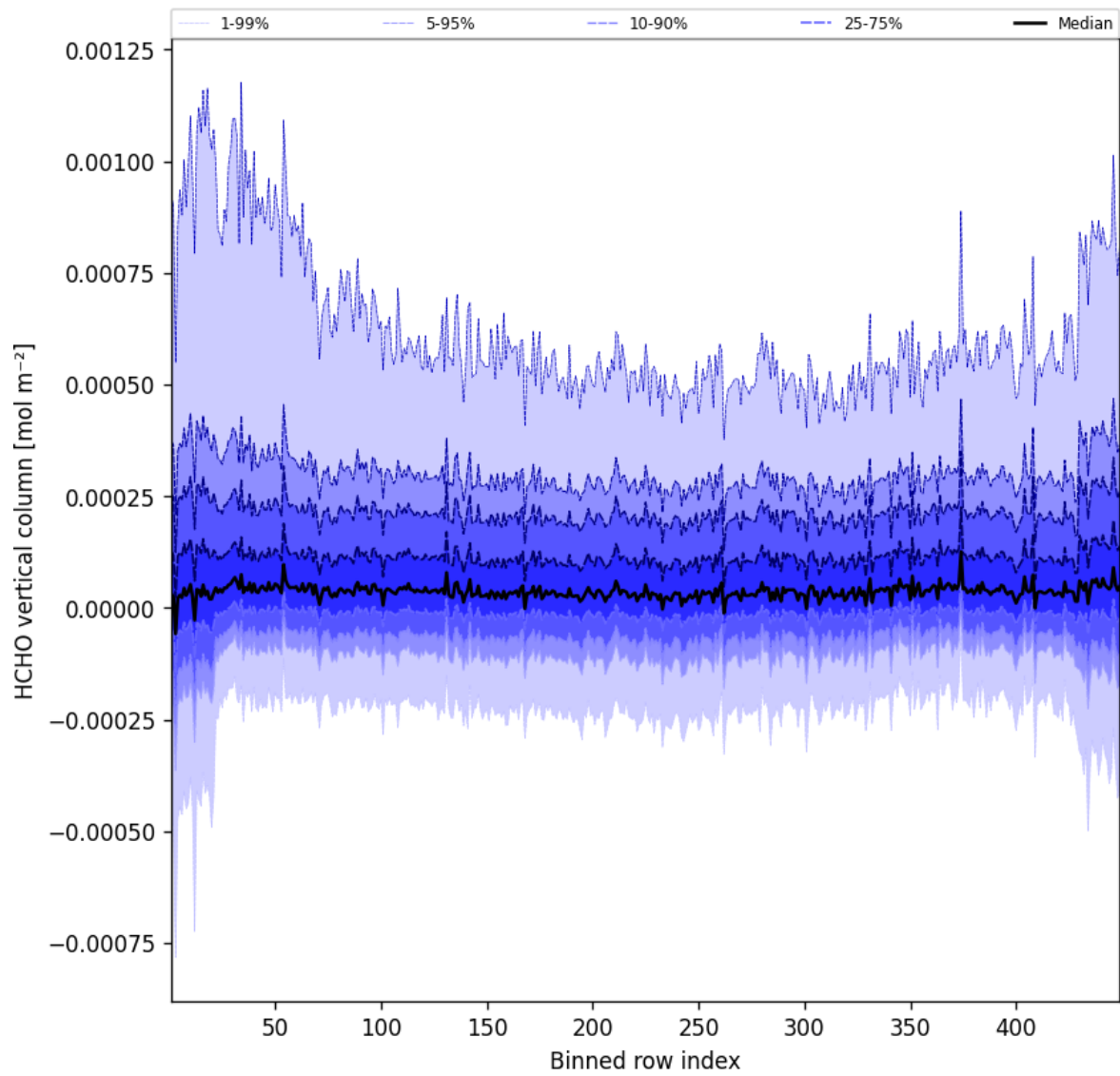
Figure 47: Along track statistics of “HCHO vertical column” for 2025-05-21 to 2025-05-22
