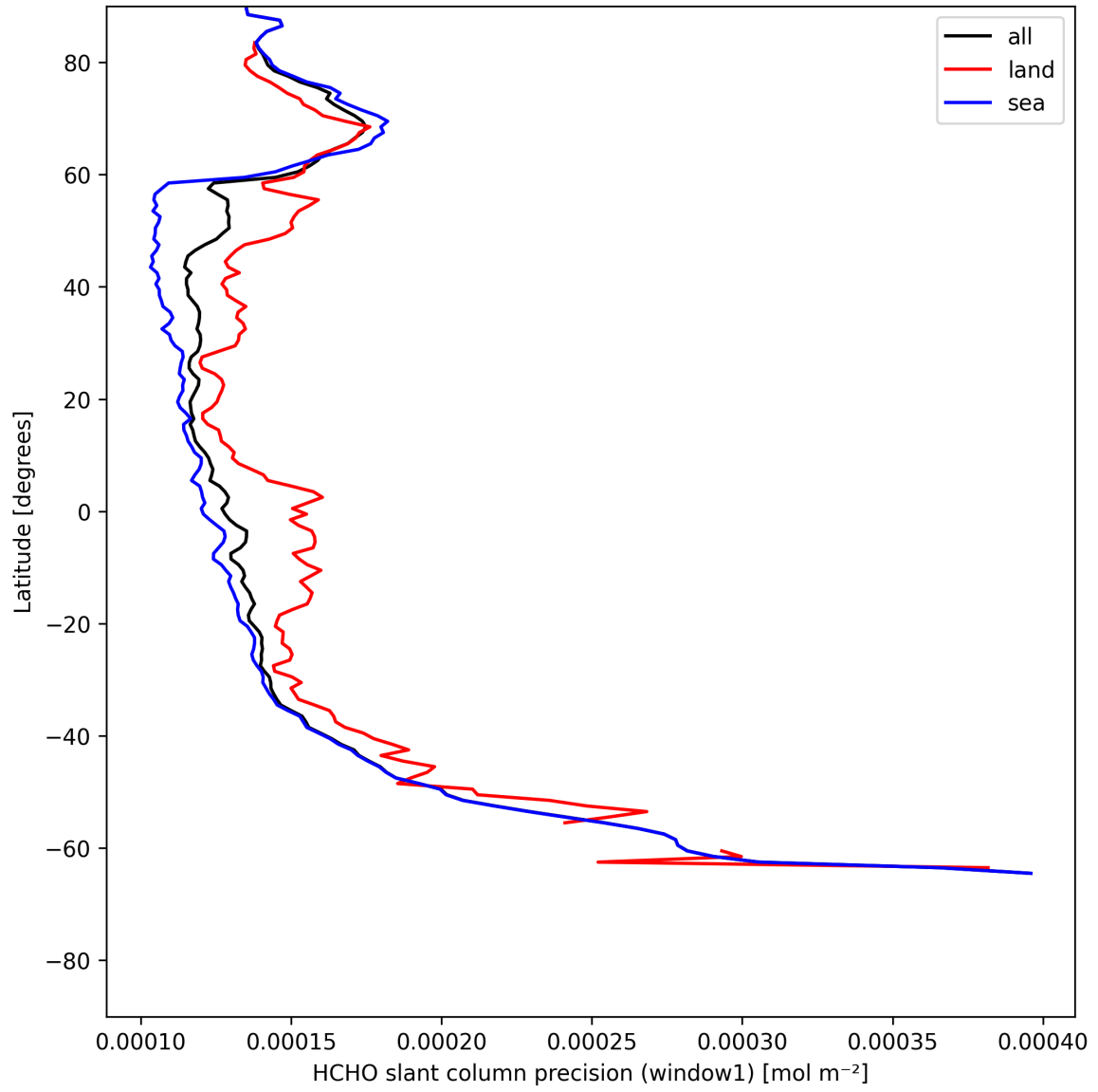
Figure 23: Zonal average of “HCHO slant column precision (window1)” for 2025-05-21 to 2025-05-22.
