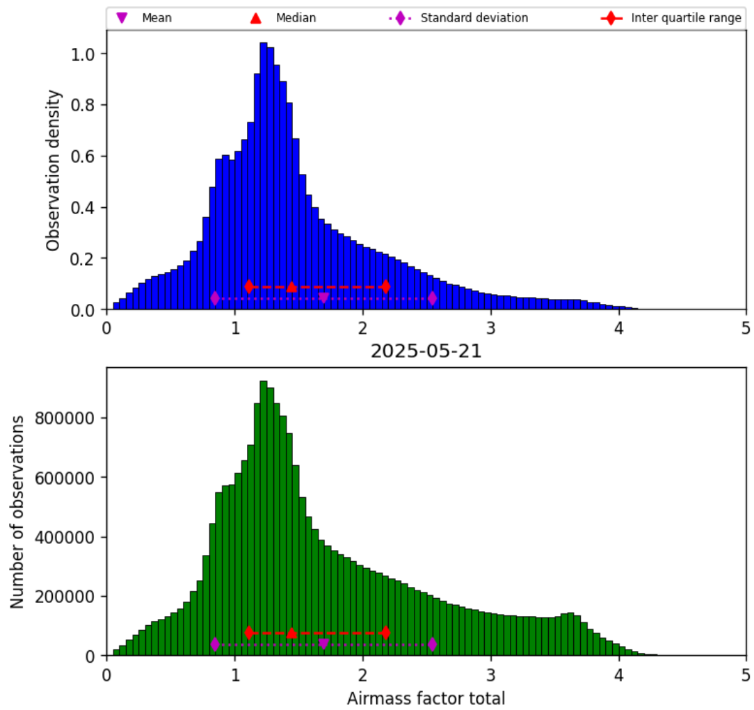
Figure 38: Histogram of “Airmass factor total” for 2025-05-21 to 2025-05-22
