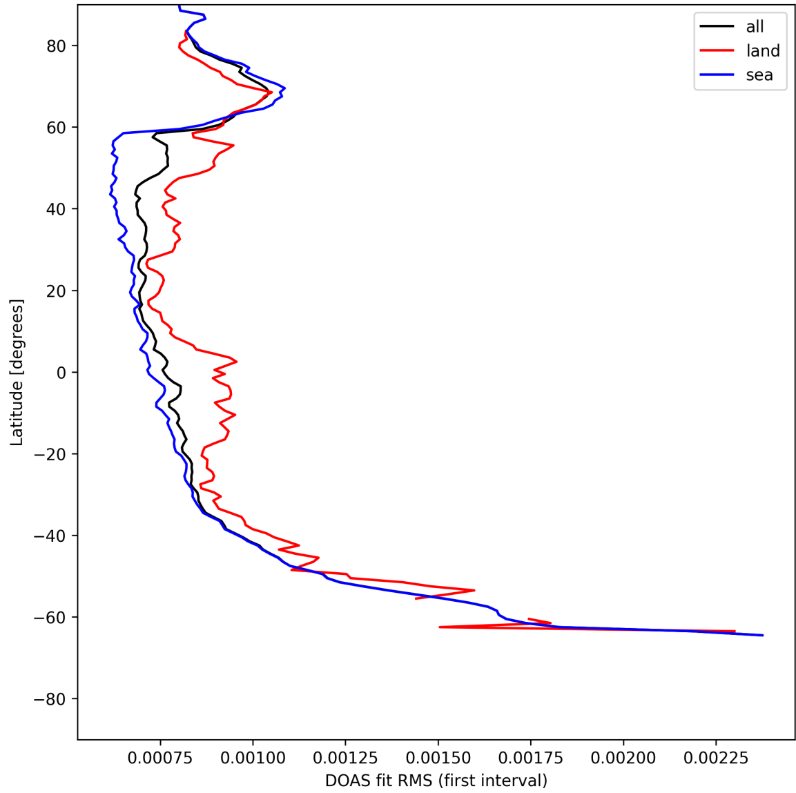
Figure 30: Zonal average of "DOAS fit RMS (first interval)" for 2025-05-21 to 2025-05-22.
