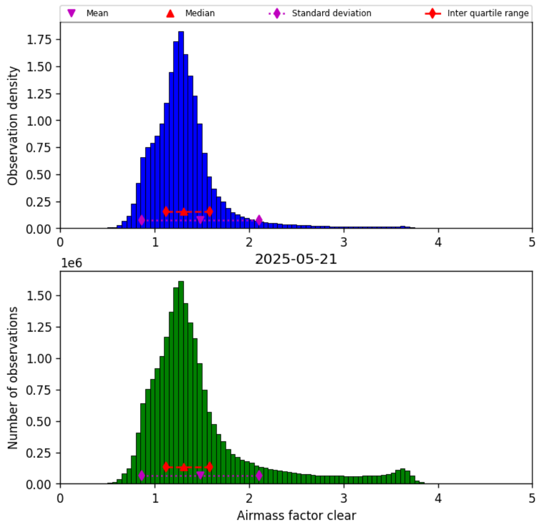
Figure 40: Histogram of “Airmass factor clear” for 2025-05-21 to 2025-05-22
