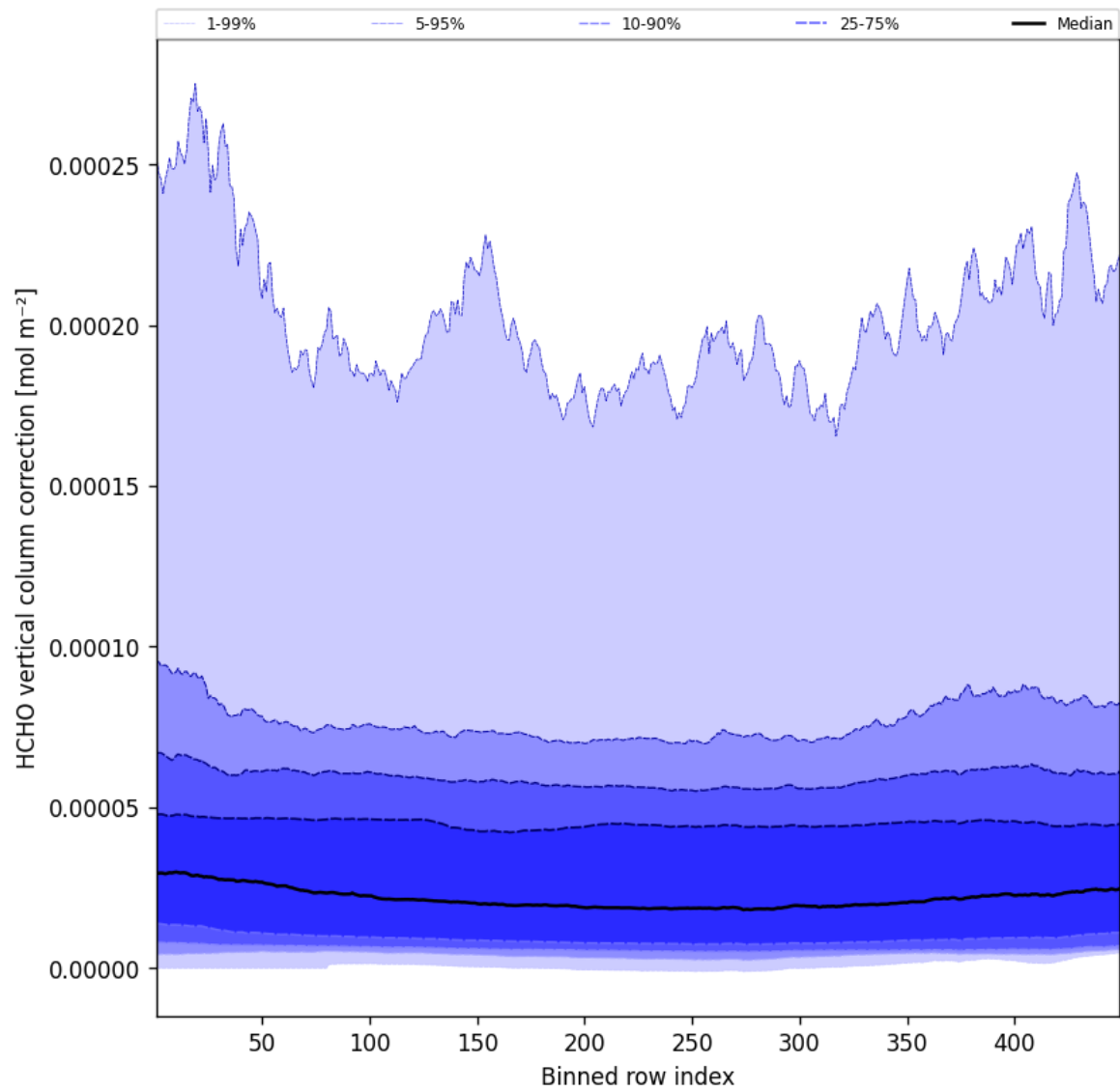
Figure 49: Along track statistics of “HCHO vertical column correction” for 2025-05-21 to 2025-05-22
