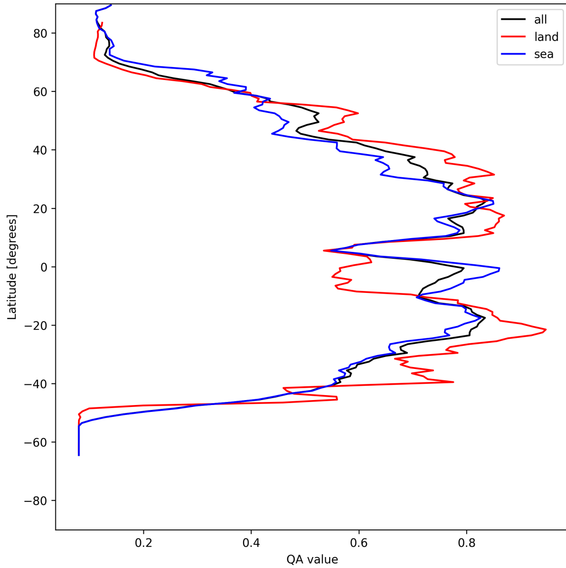
Figure 18: Zonal average of “QA value” for 2025-05-21 to 2025-05-22.
