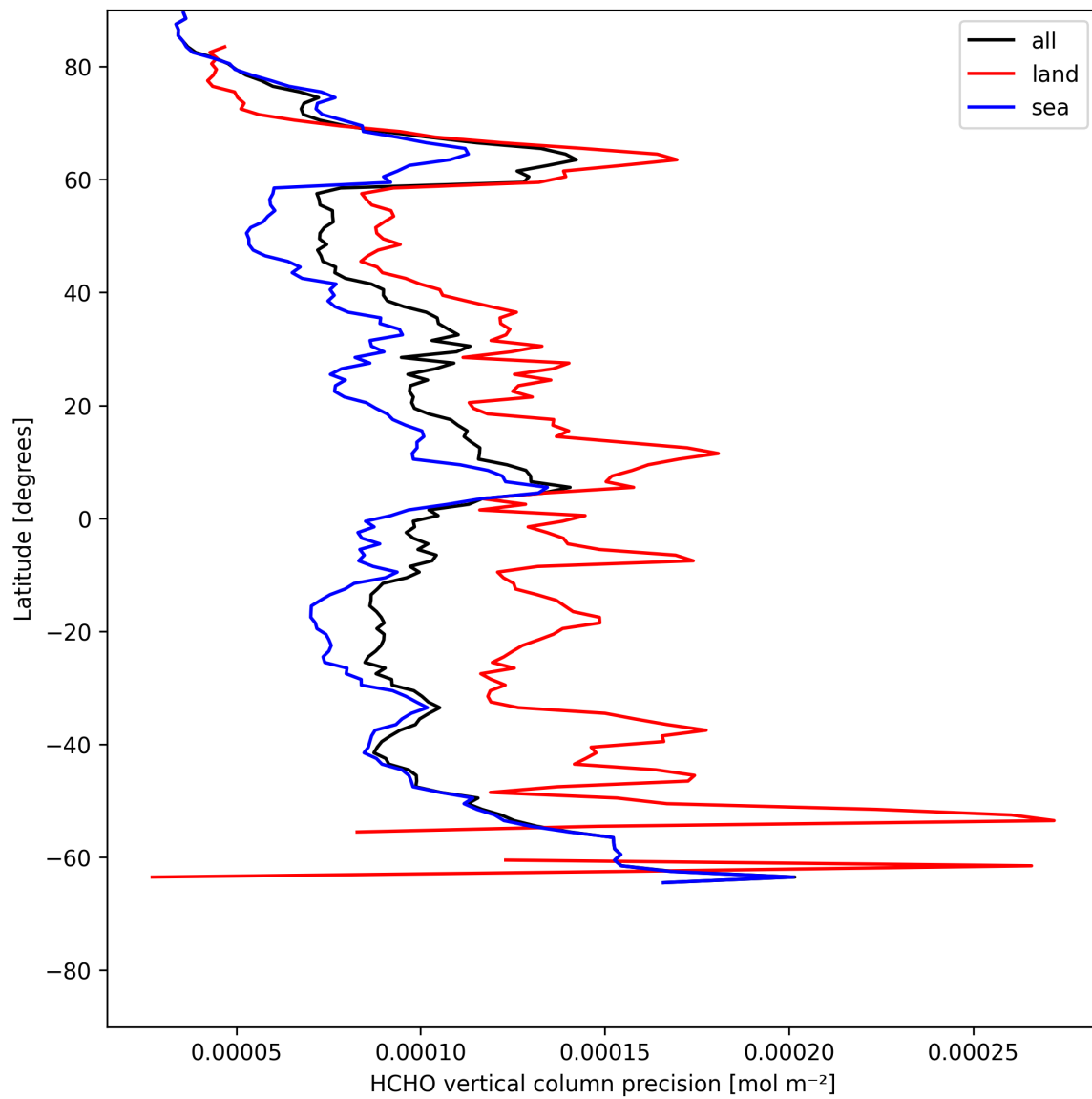
Figure 20: Zonal average of “HCHO vertical column precision” for 2025-05-21 to 2025-05-22.
