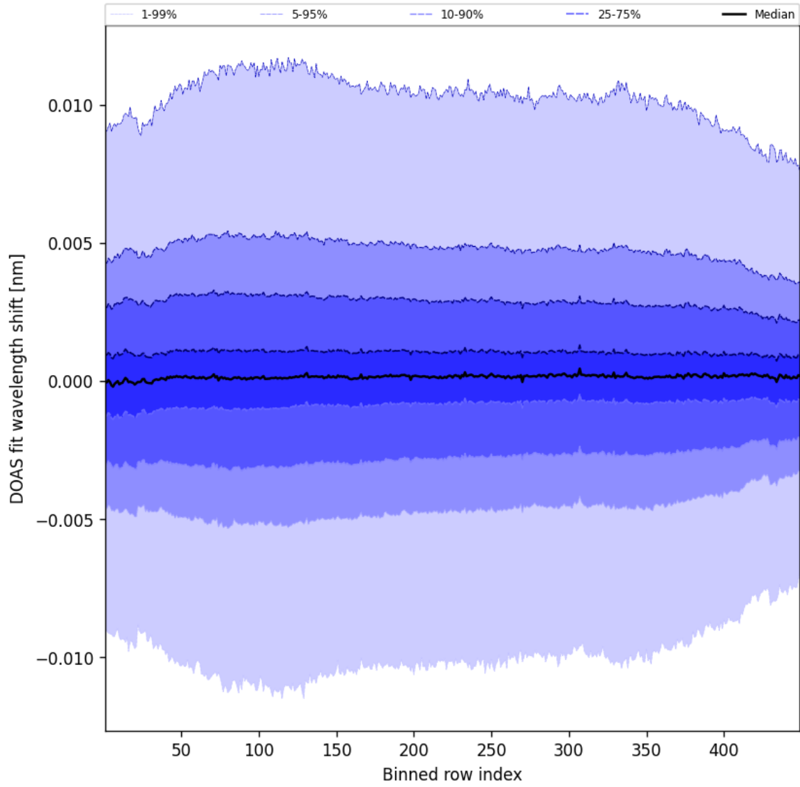
Figure 56: Along track statistics of “DOAS fit wavelength shift” for 2025-05-21 to 2025-05-22
