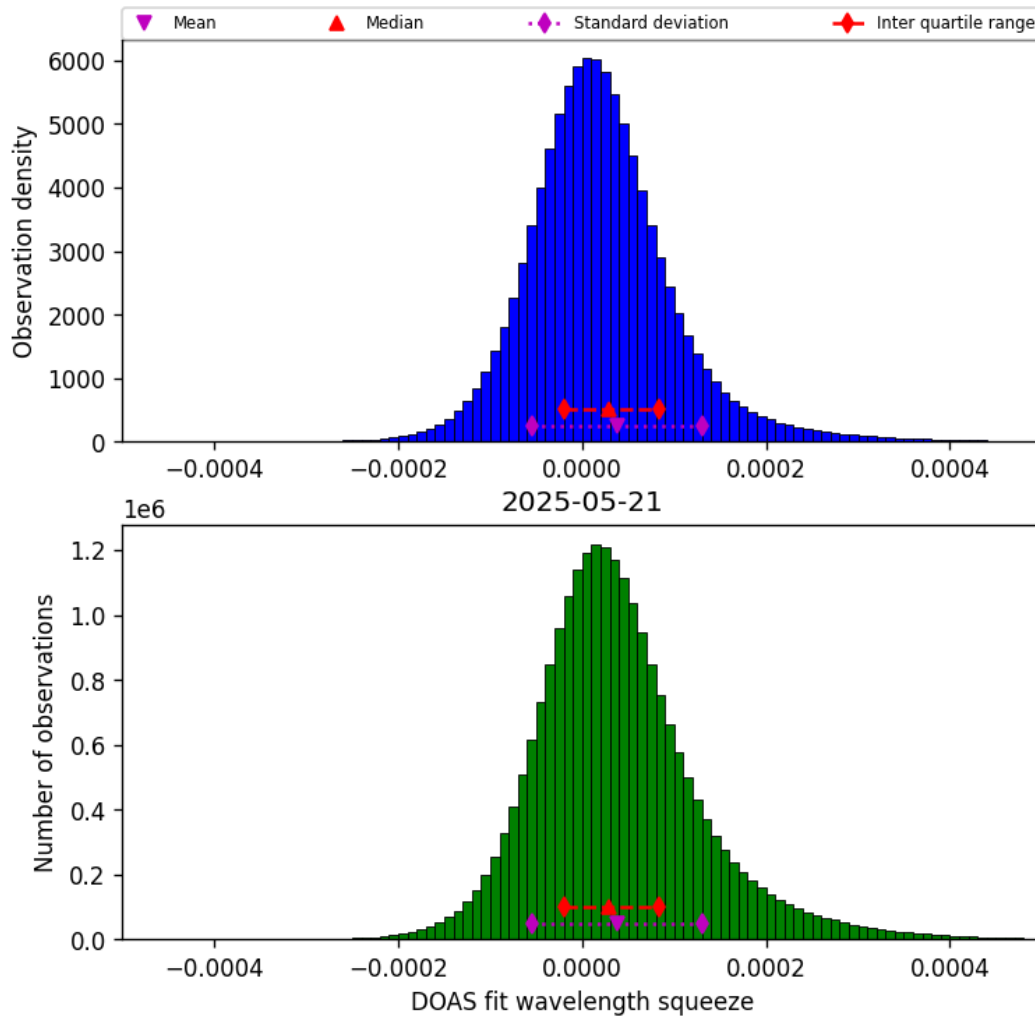
Figure 43: Histogram of “DOAS fit wavelength squeeze” for 2025-05-21 to 2025-05-22
