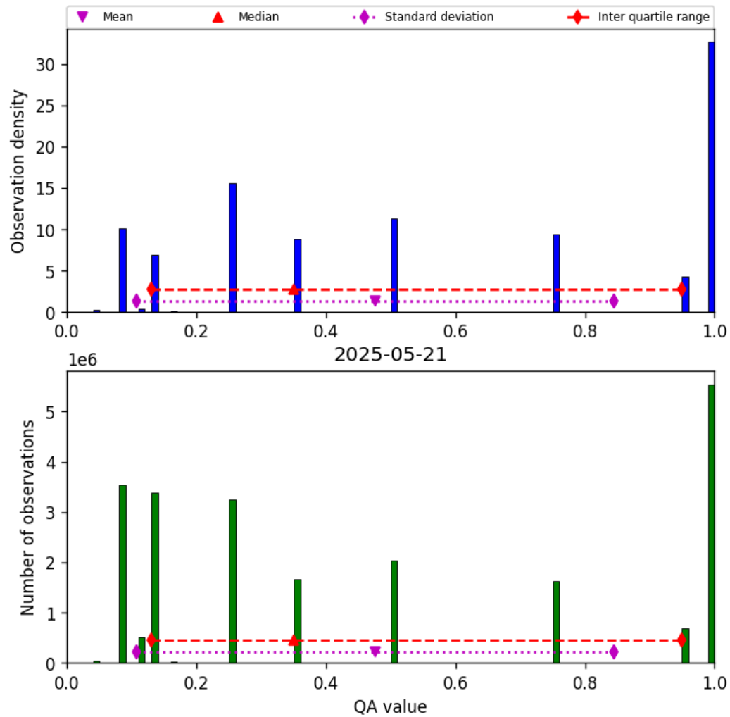
Figure 32: Histogram of “QA value” for 2025-05-21 to 2025-05-22
