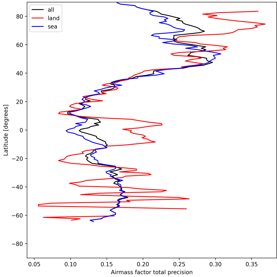
Figure 25: Zonal average of “Airmass factor total precision” for 2025-05-21 to 2025-05-22.
