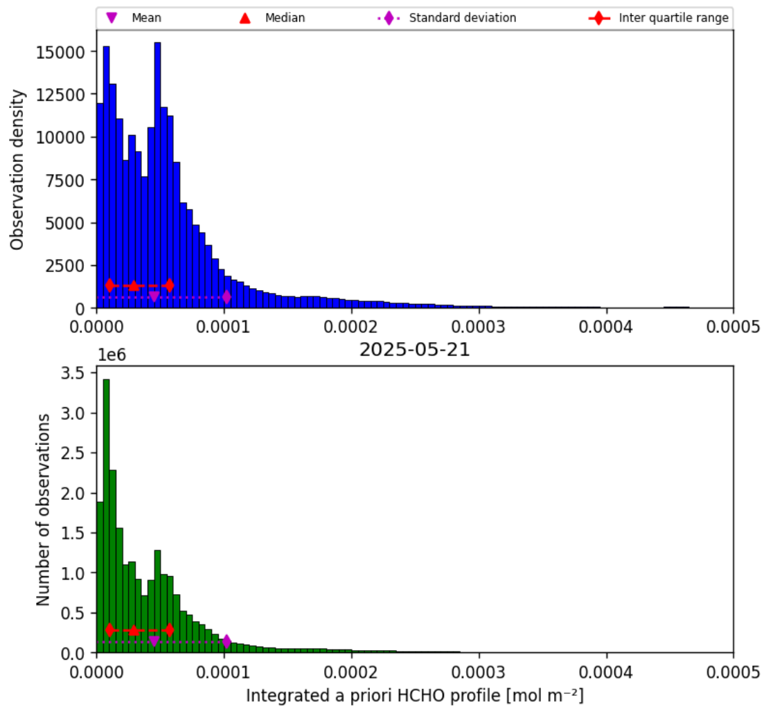
Figure 41: Histogram of “Integrated a priori HCHO profile” for 2025-05-21 to 2025-05-22
