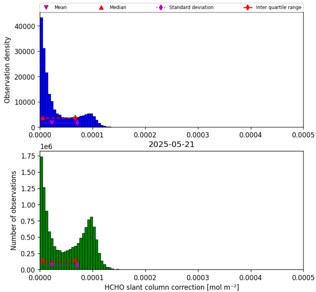
Figure 45: Histogram of “HCHO slant column correction” for 2025-05-21 to 2025-05-22
