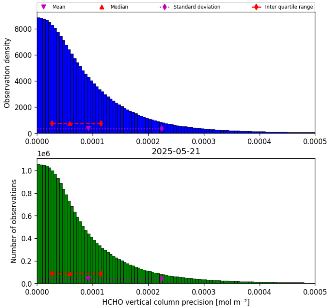
Figure 34: Histogram of “HCHO vertical column precision” for 2025-05-21 to 2025-05-22
