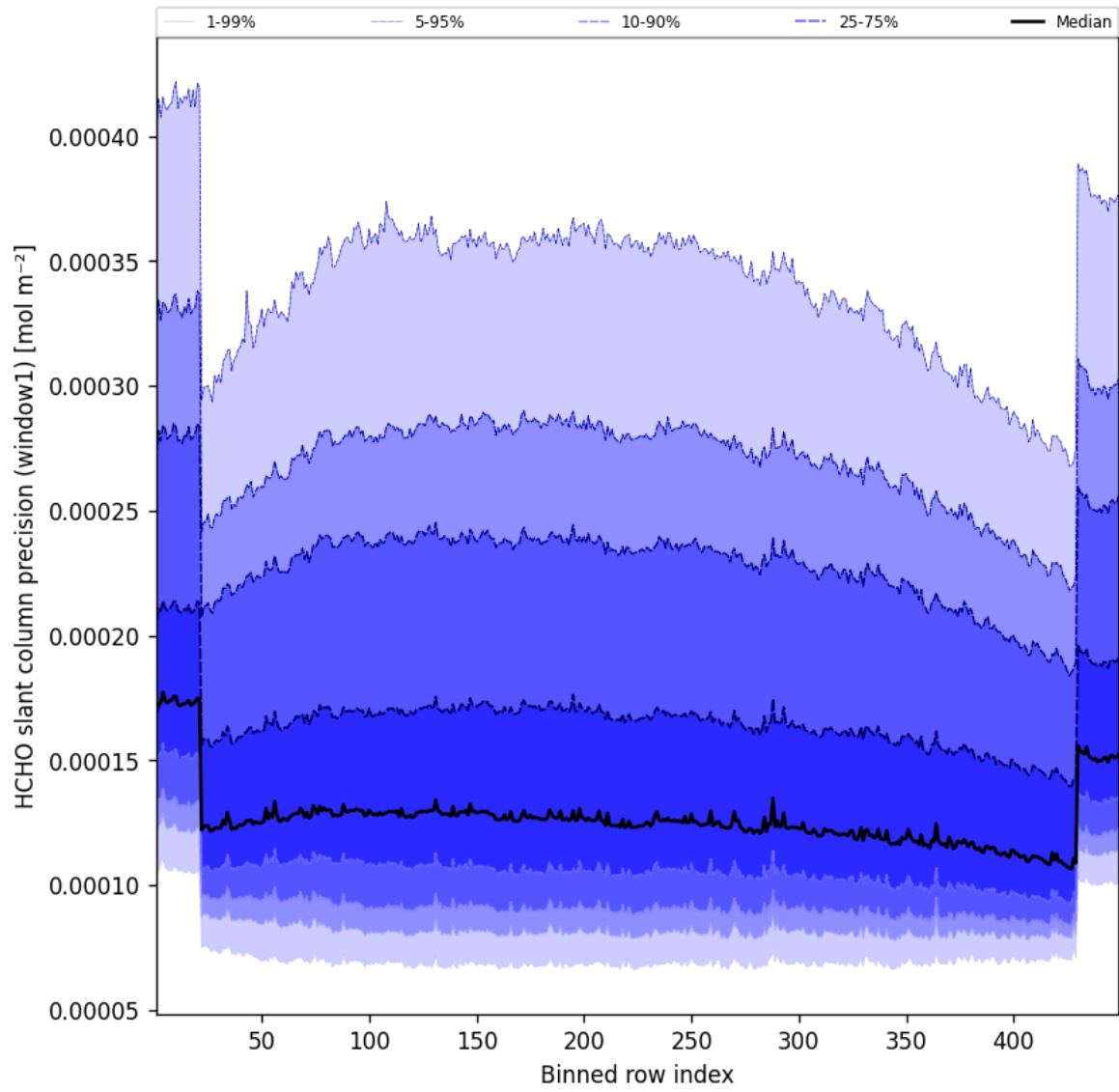
Figure 51: Along track statistics of “HCHO slant column precision (window1)” for 2025-05-21 to 2025-05-22
