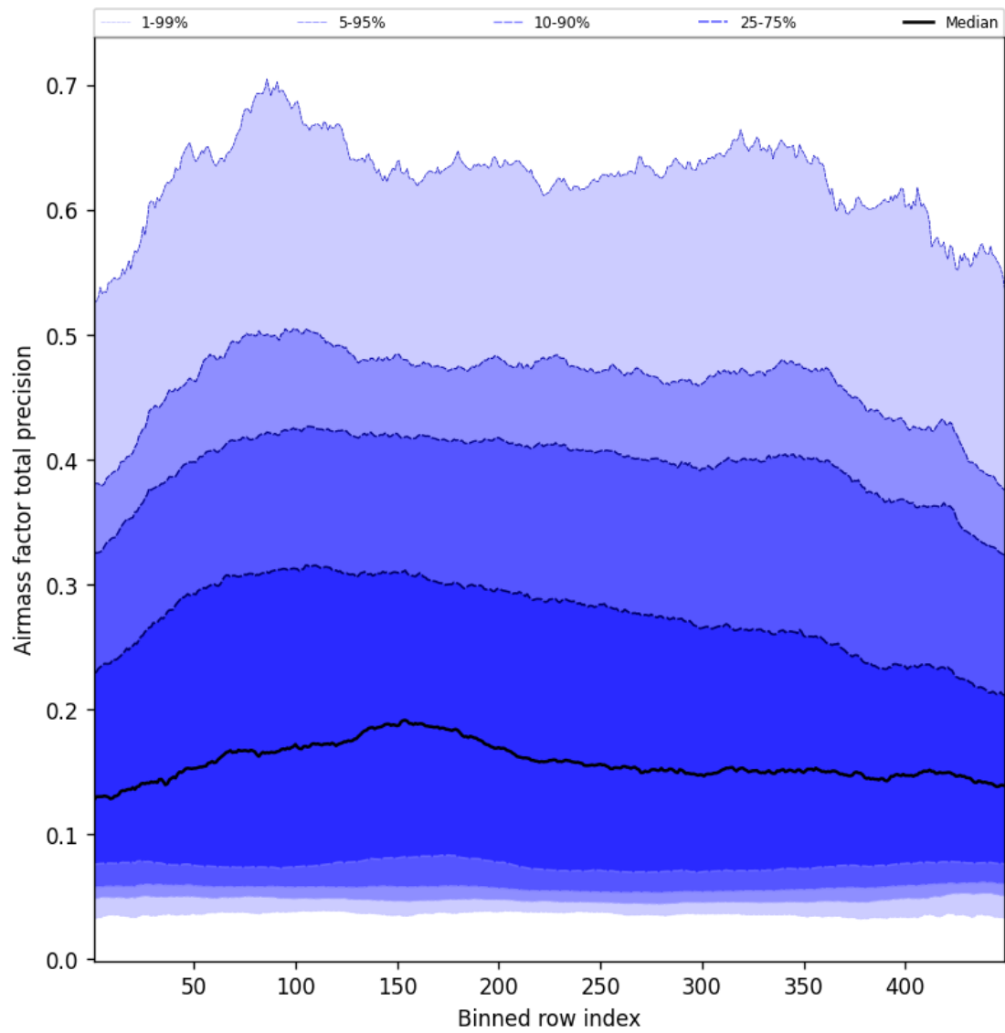
Figure 53: Along track statistics of “Airmass factor total precision” for 2025-05-21 to 2025-05-22
