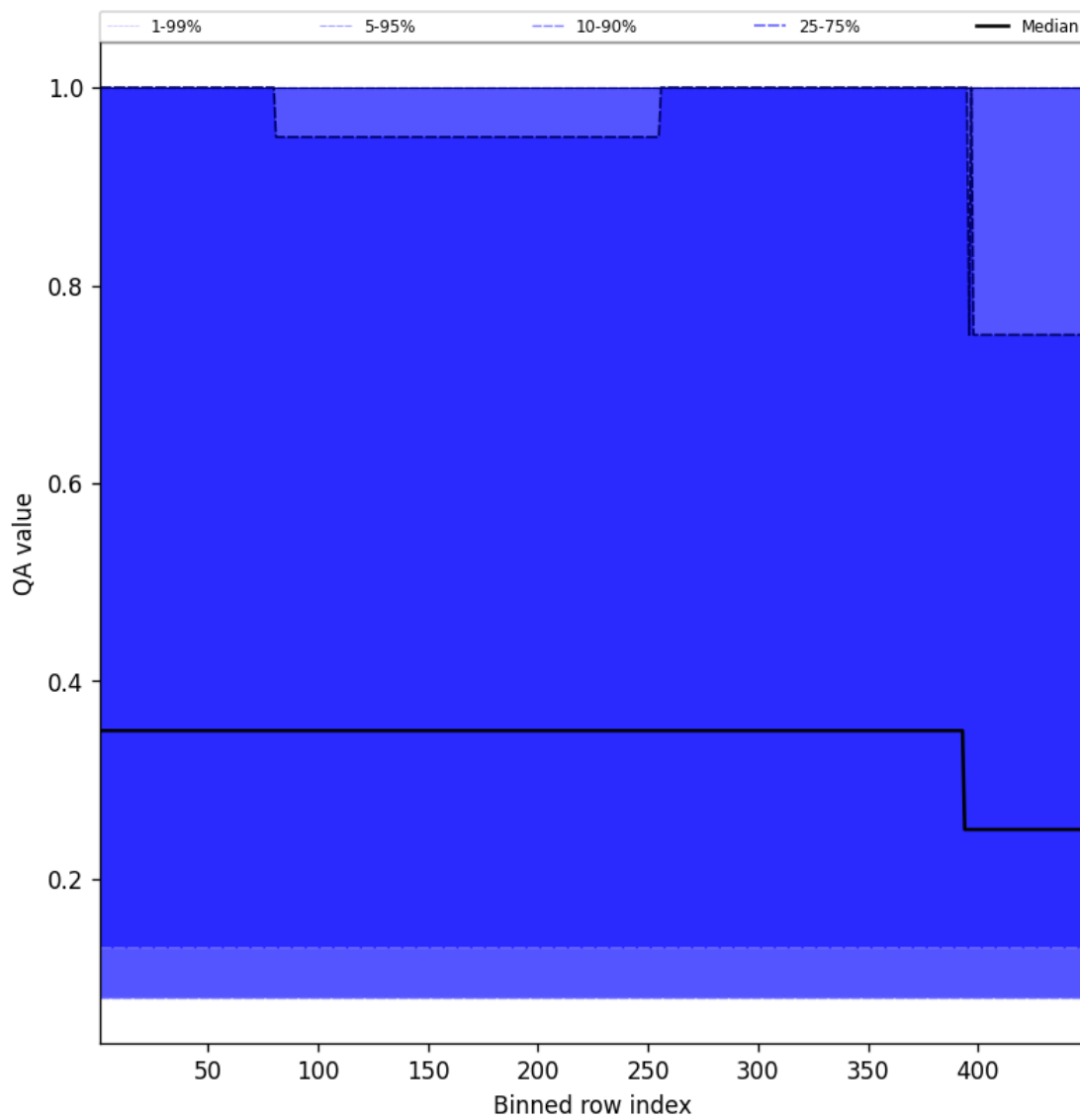
Figure 46: Along track statistics of “QA value” for 2025-05-21 to 2025-05-22
