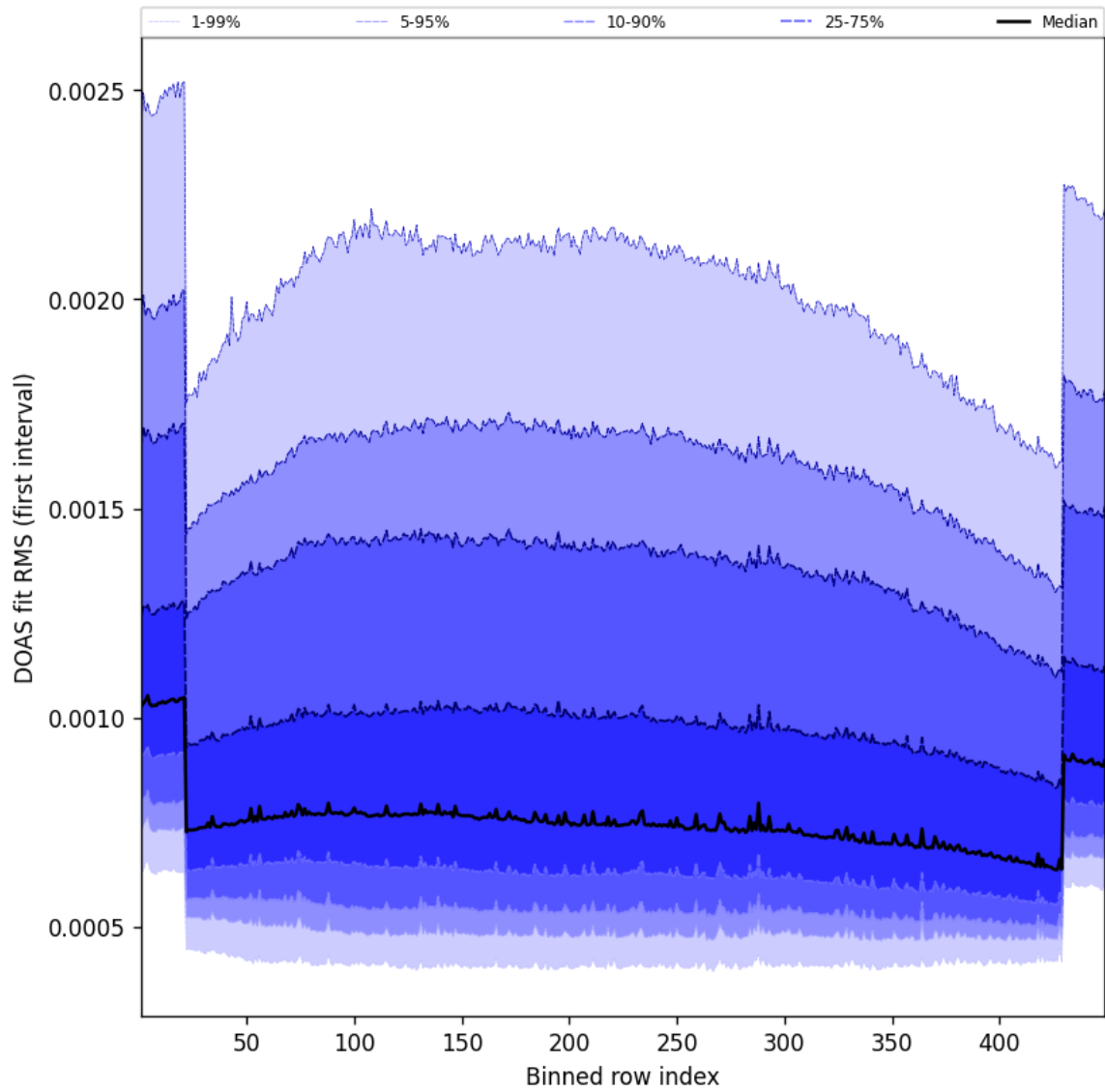
Figure 58: Along track statistics of “DOAS fit RMS (first interval)” for 2025-05-21 to 2025-05-22
