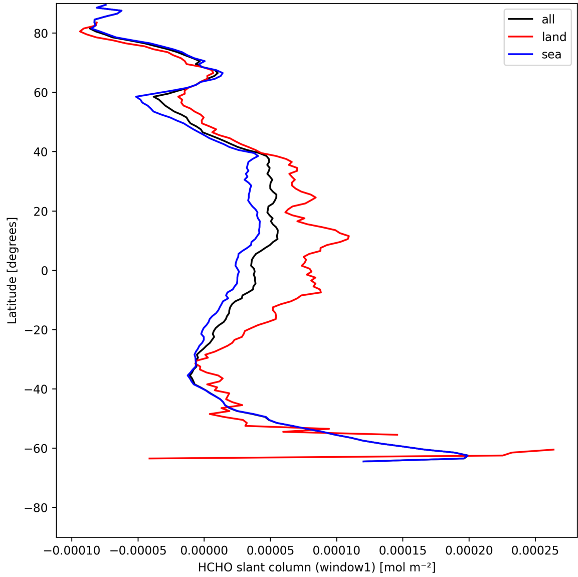
Figure 22: Zonal average of “HCHO slant column (window1)” for 2025-05-21 to 2025-05-22.
