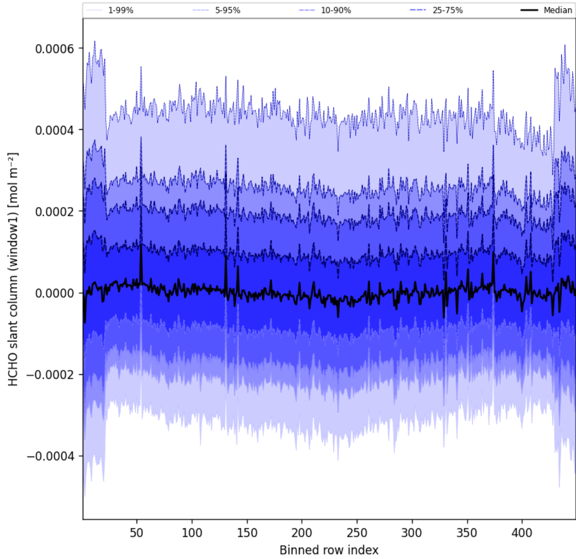
Figure 50: Along track statistics of “HCHO slant column (window1)” for 2025-05-21 to 2025-05-22
