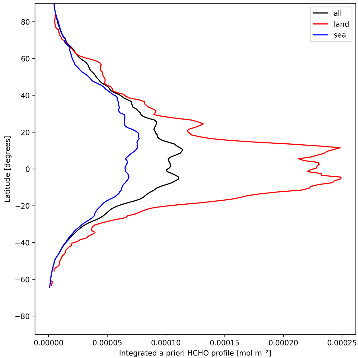
Figure 27: Zonal average of “Integrated a priori HCHO profile” for 2025-05-21 to 2025-05-22.
