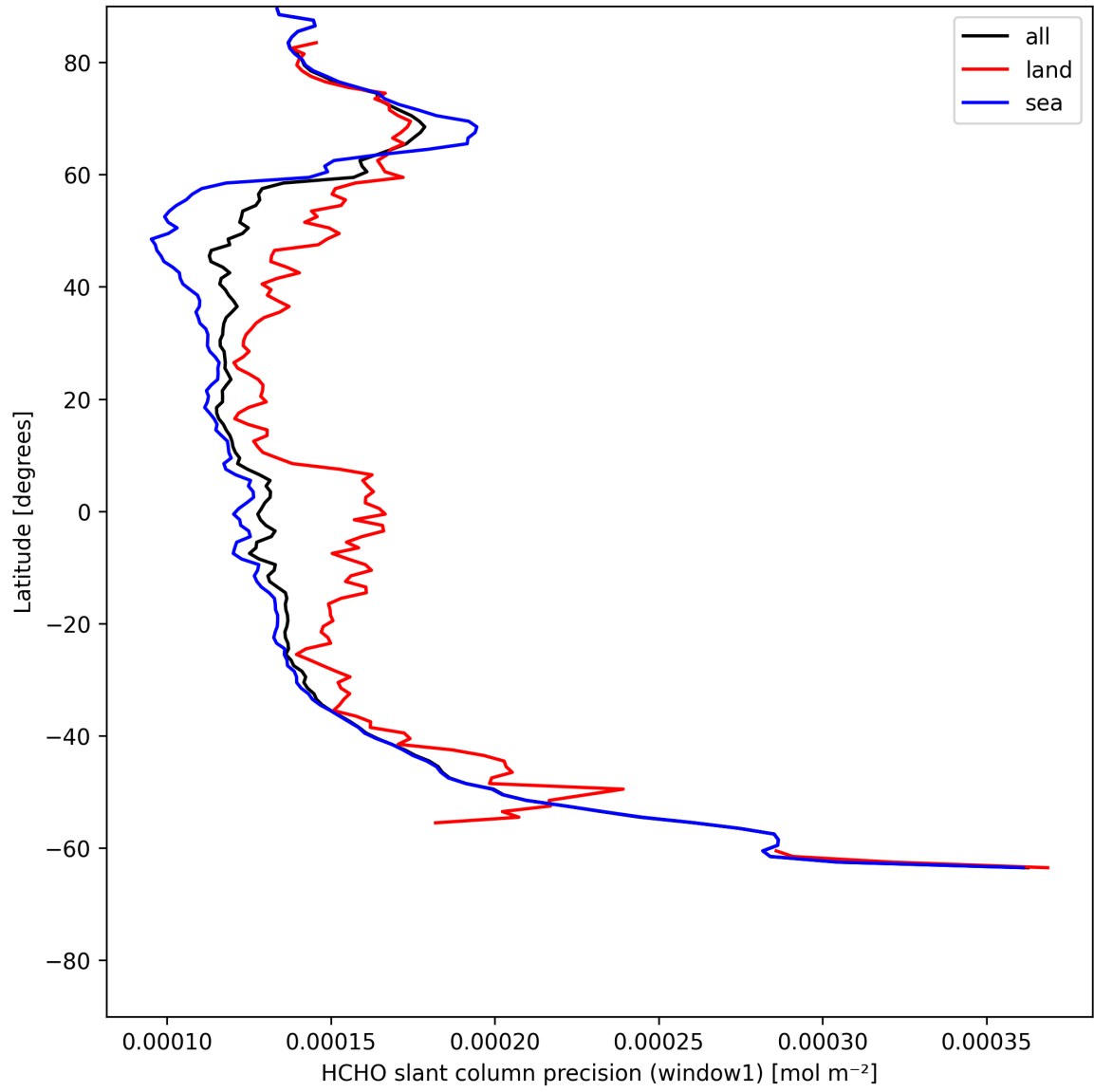
Figure 23: Zonal average of “HCHO slant column precision (window1)” for 2025-05-22 to 2025-05-23.
