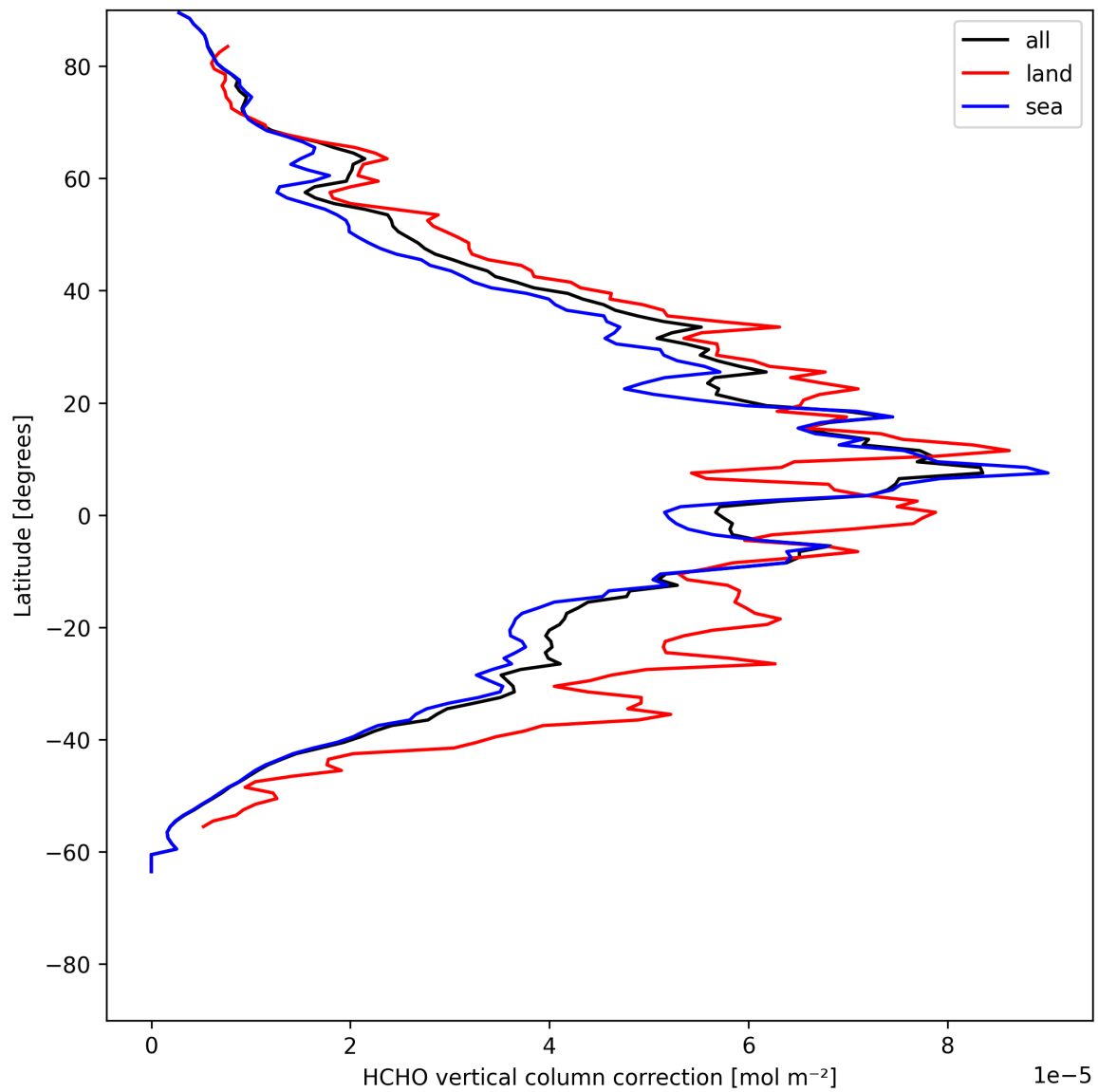
Figure 21: Zonal average of “HCHO vertical column correction” for 2025-05-22 to 2025-05-23.
