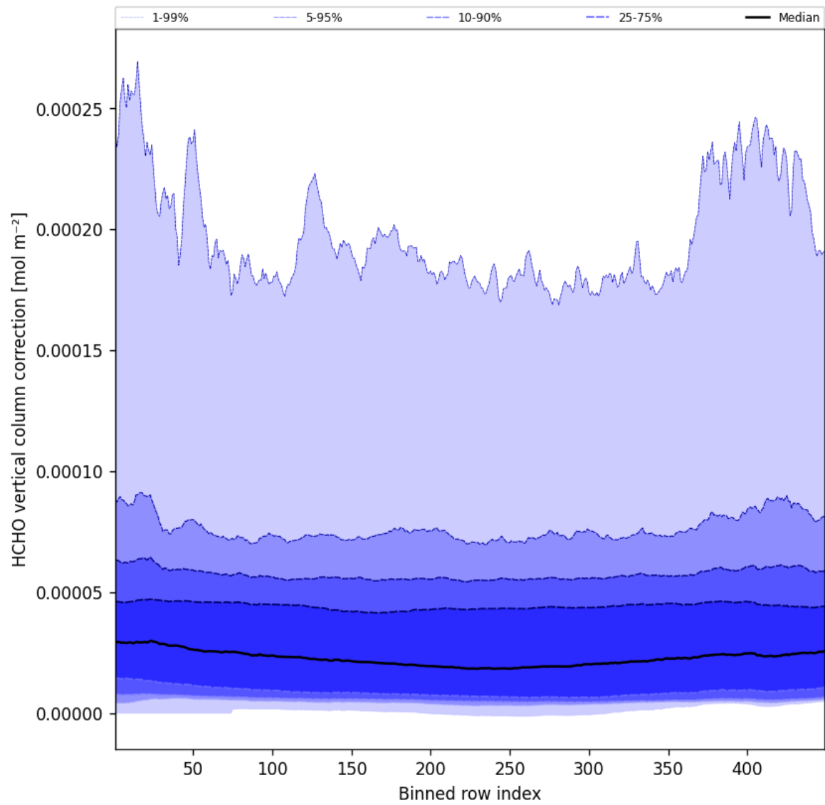
Figure 49: Along track statistics of “HCHO vertical column correction” for 2025-05-22 to 2025-05-23
