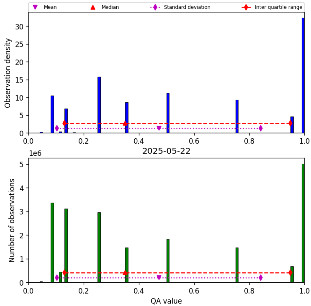
Figure 32: Histogram of “QA value” for 2025-05-22 to 2025-05-23
