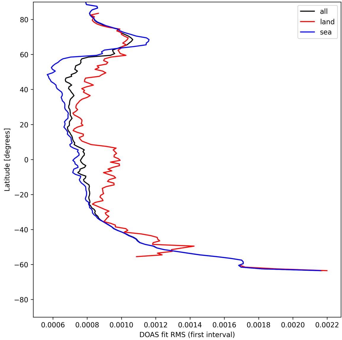
Figure 30: Zonal average of "DOAS fit RMS (first interval)" for 2025-05-22 to 2025-05-23.
