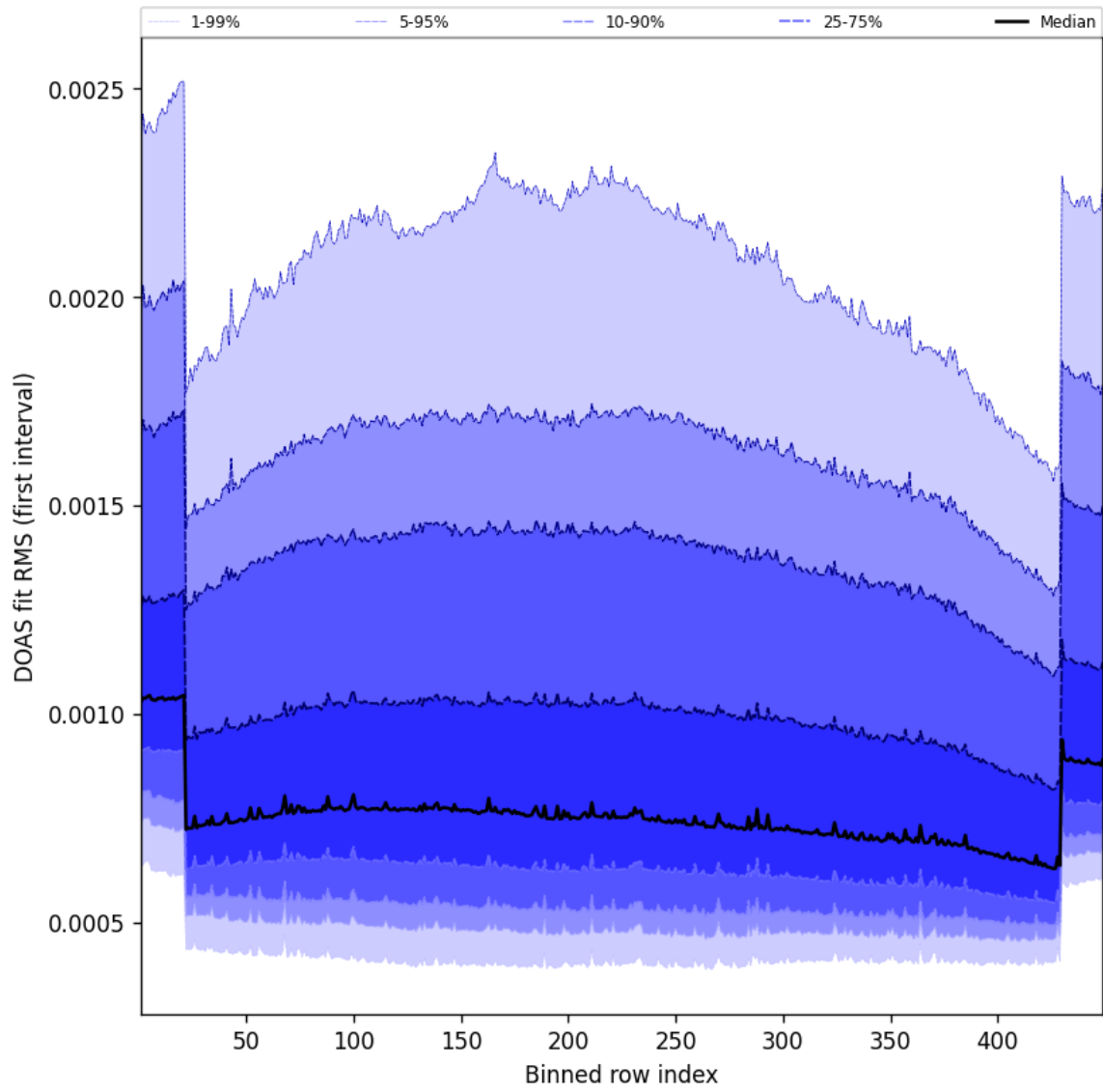
Figure 58: Along track statistics of “DOAS fit RMS (first interval)” for 2025-05-22 to 2025-05-23
