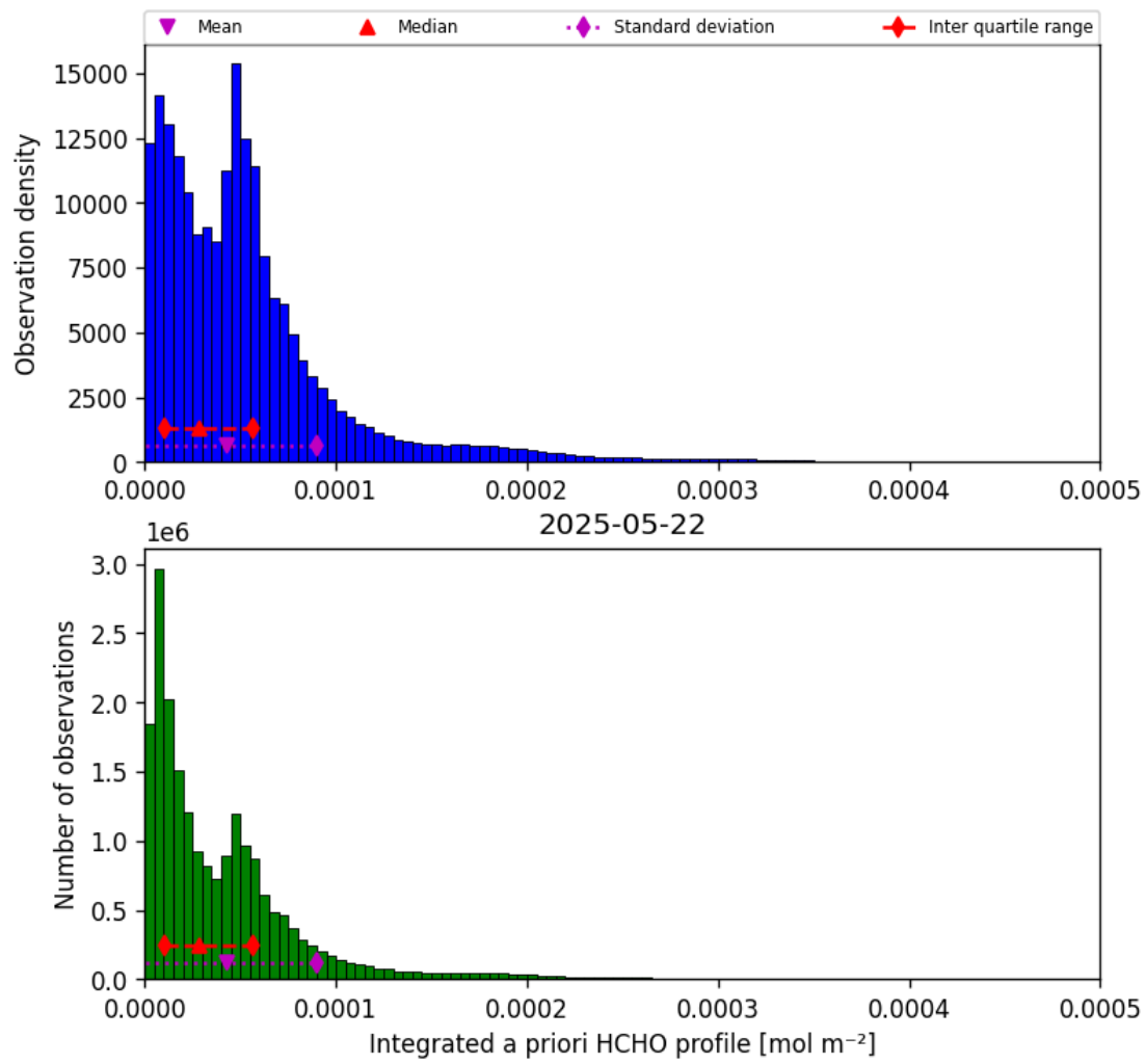
Figure 41: Histogram of “Integrated a priori HCHO profile” for 2025-05-22 to 2025-05-23
