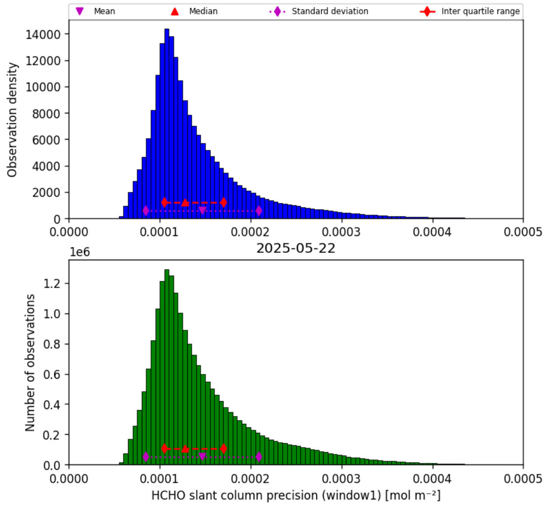
Figure 37: Histogram of “HCHO slant column precision (window1)” for 2025-05-22 to 2025-05-23
