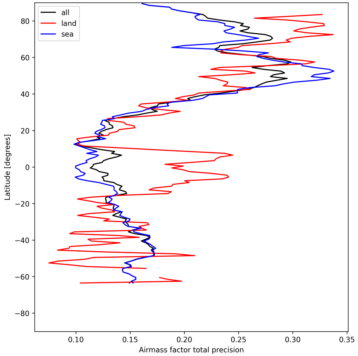
Figure 25: Zonal average of “Airmass factor total precision” for 2025-05-22 to 2025-05-23.
