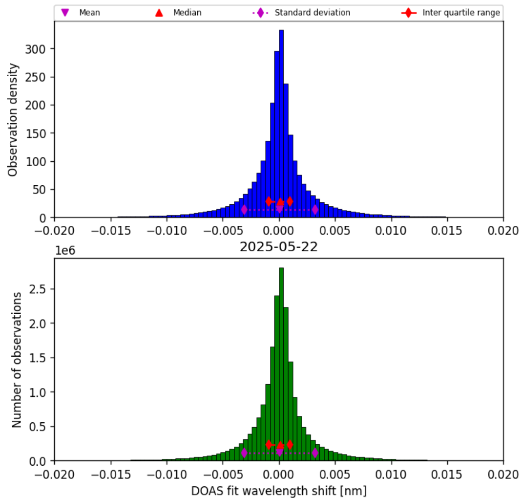
Figure 42: Histogram of “DOAS fit wavelength shift” for 2025-05-22 to 2025-05-23
