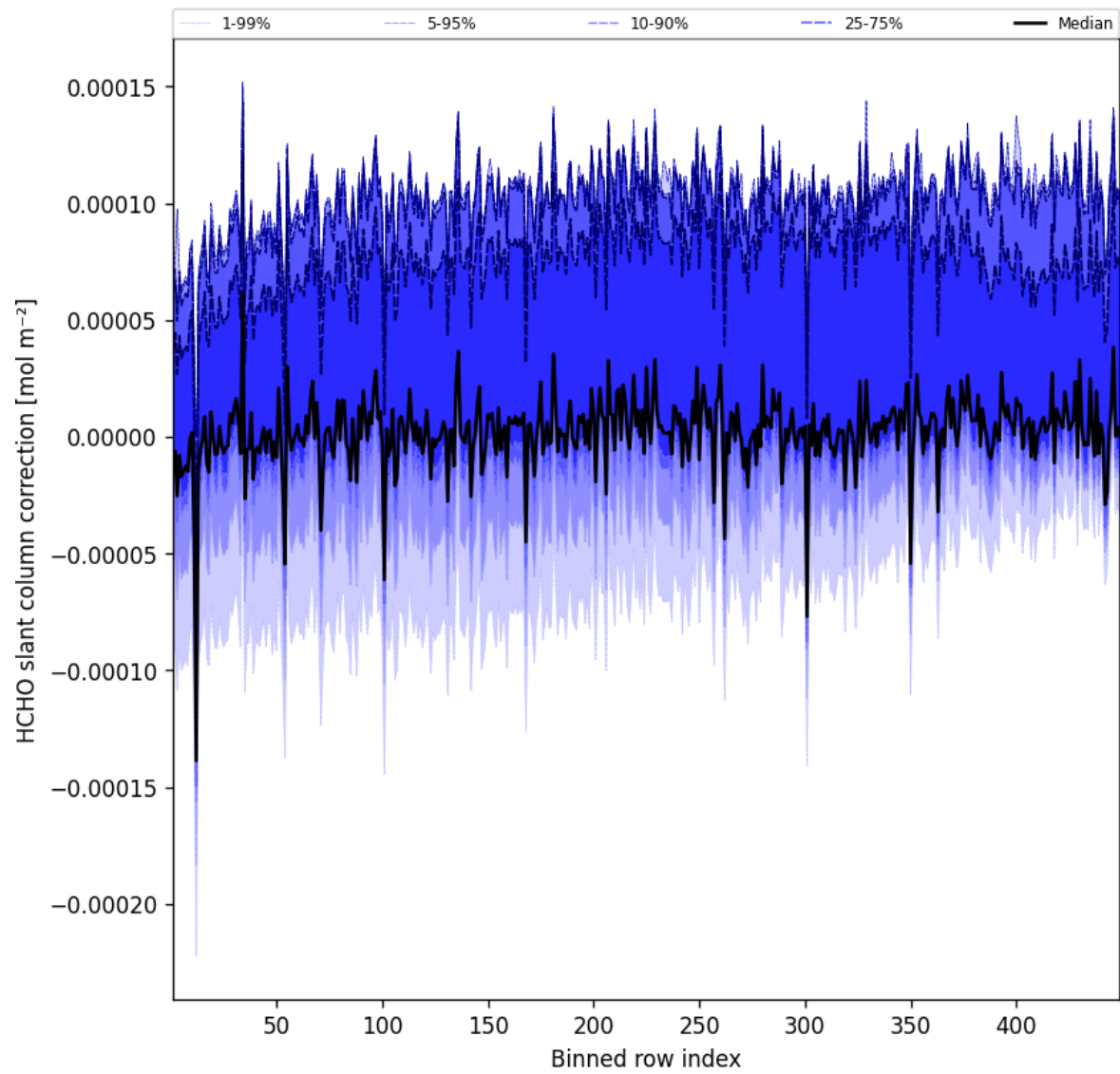
Figure 59: Along track statistics of “HCHO slant column correction” for 2025-05-22 to 2025-05-23
