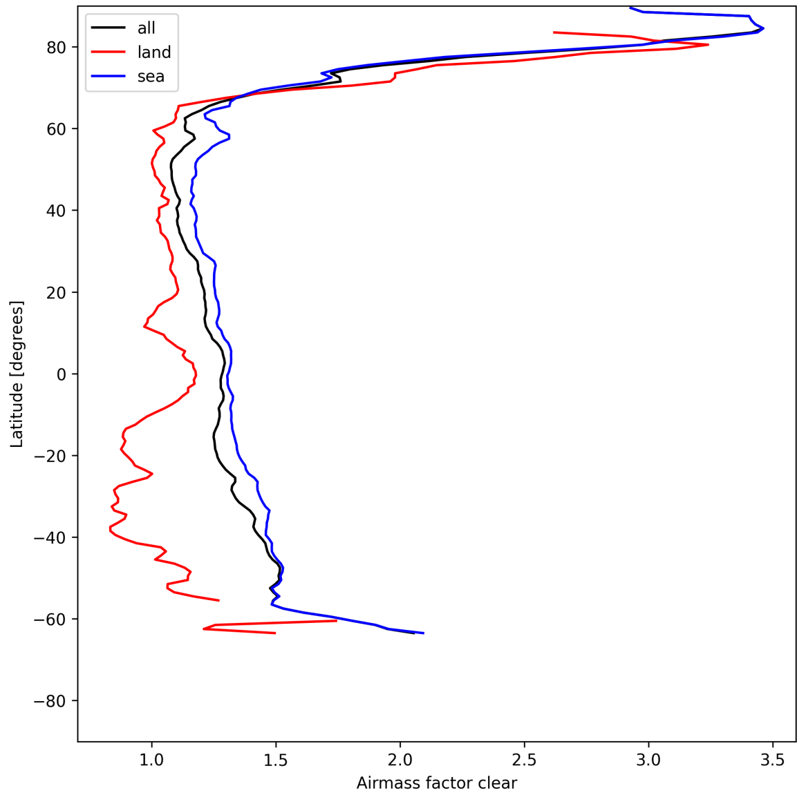
Figure 26: Zonal average of “Airmass factor clear” for 2025-05-22 to 2025-05-23.
