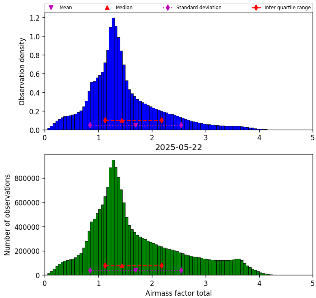
Figure 38: Histogram of “Airmass factor total” for 2025-05-22 to 2025-05-23
