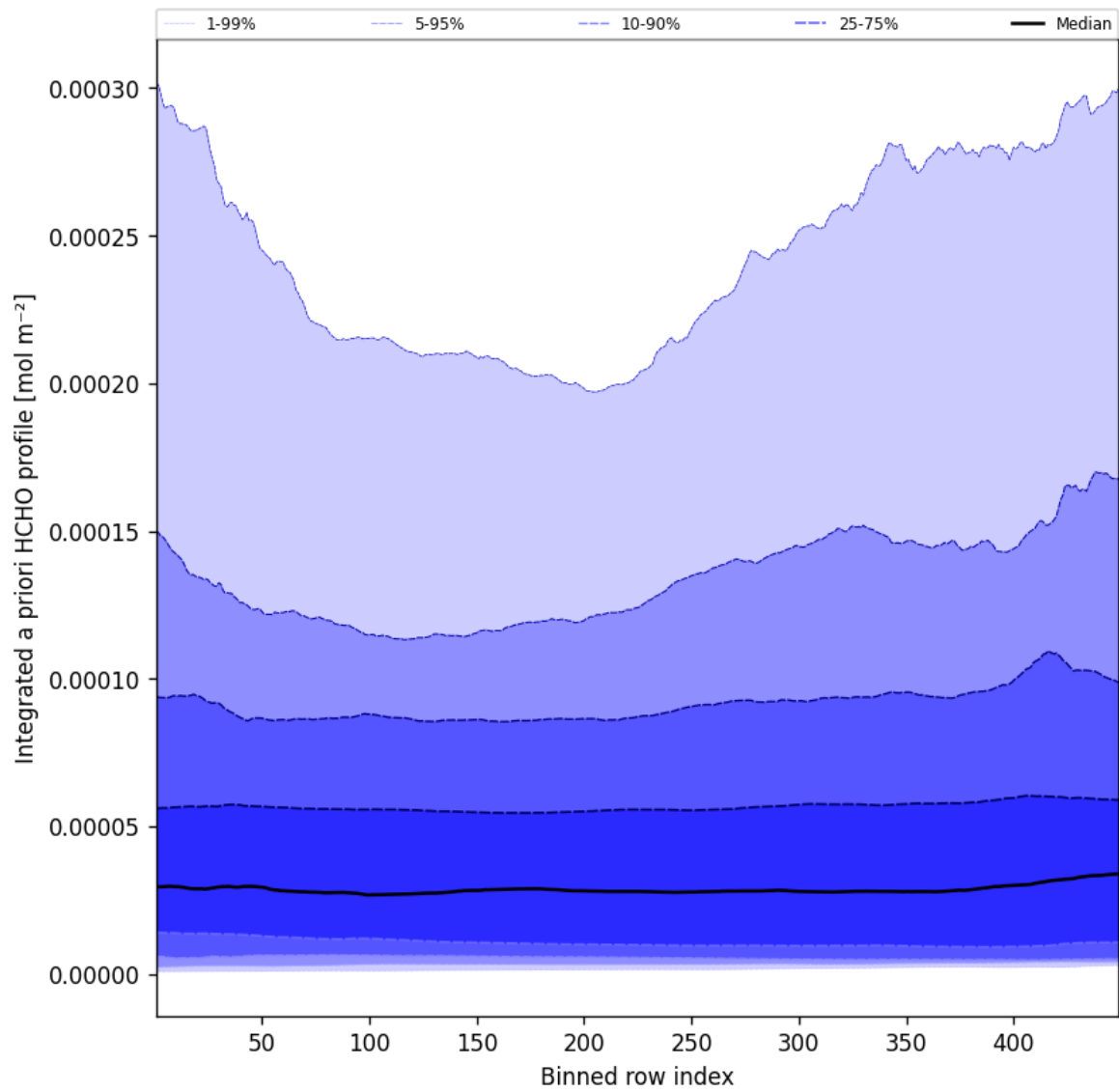
Figure 55: Along track statistics of "Integrated a priori HCHO profile" for 2025-05-22 to 2025-05-23
