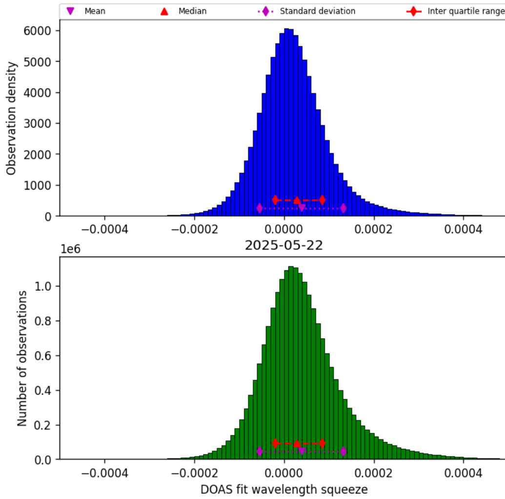
Figure 43: Histogram of “DOAS fit wavelength squeeze” for 2025-05-22 to 2025-05-23
