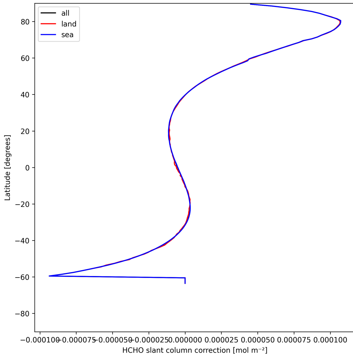
Figure 31: Zonal average of “HCHO slant column correction” for 2025-05-22 to 2025-05-23.
