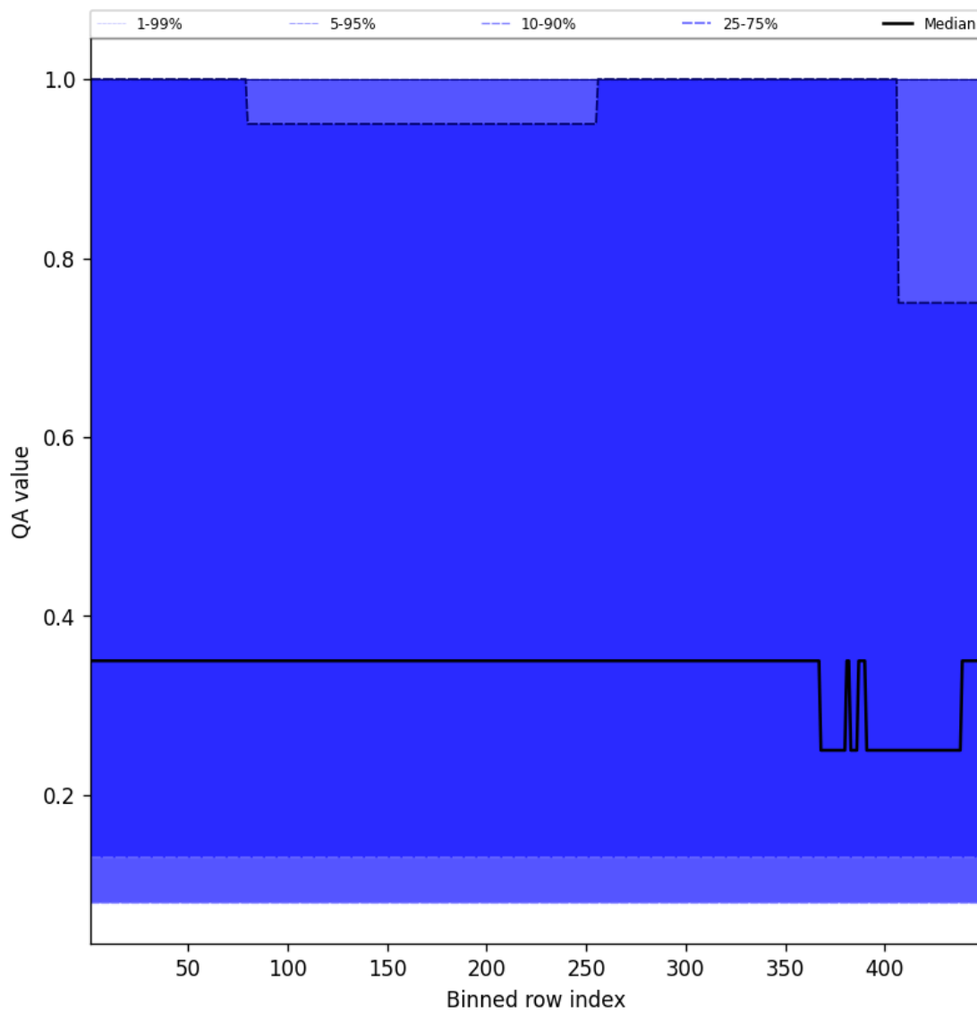
Figure 46: Along track statistics of “QA value” for 2025-05-22 to 2025-05-23
