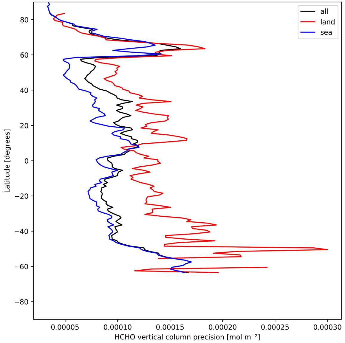
Figure 20: Zonal average of “HCHO vertical column precision” for 2025-05-22 to 2025-05-23.
