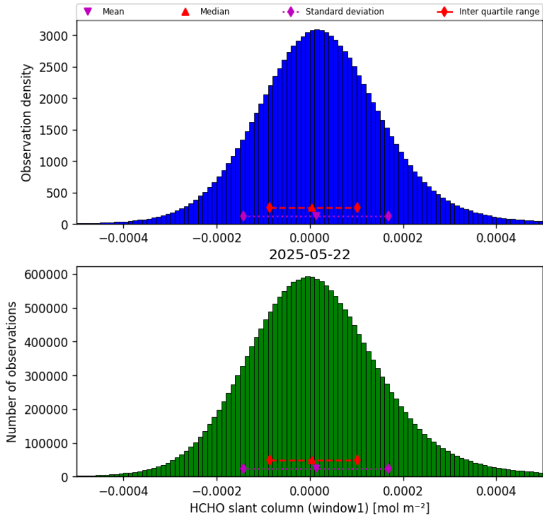
Figure 36: Histogram of “HCHO slant column (window1)” for 2025-05-22 to 2025-05-23
