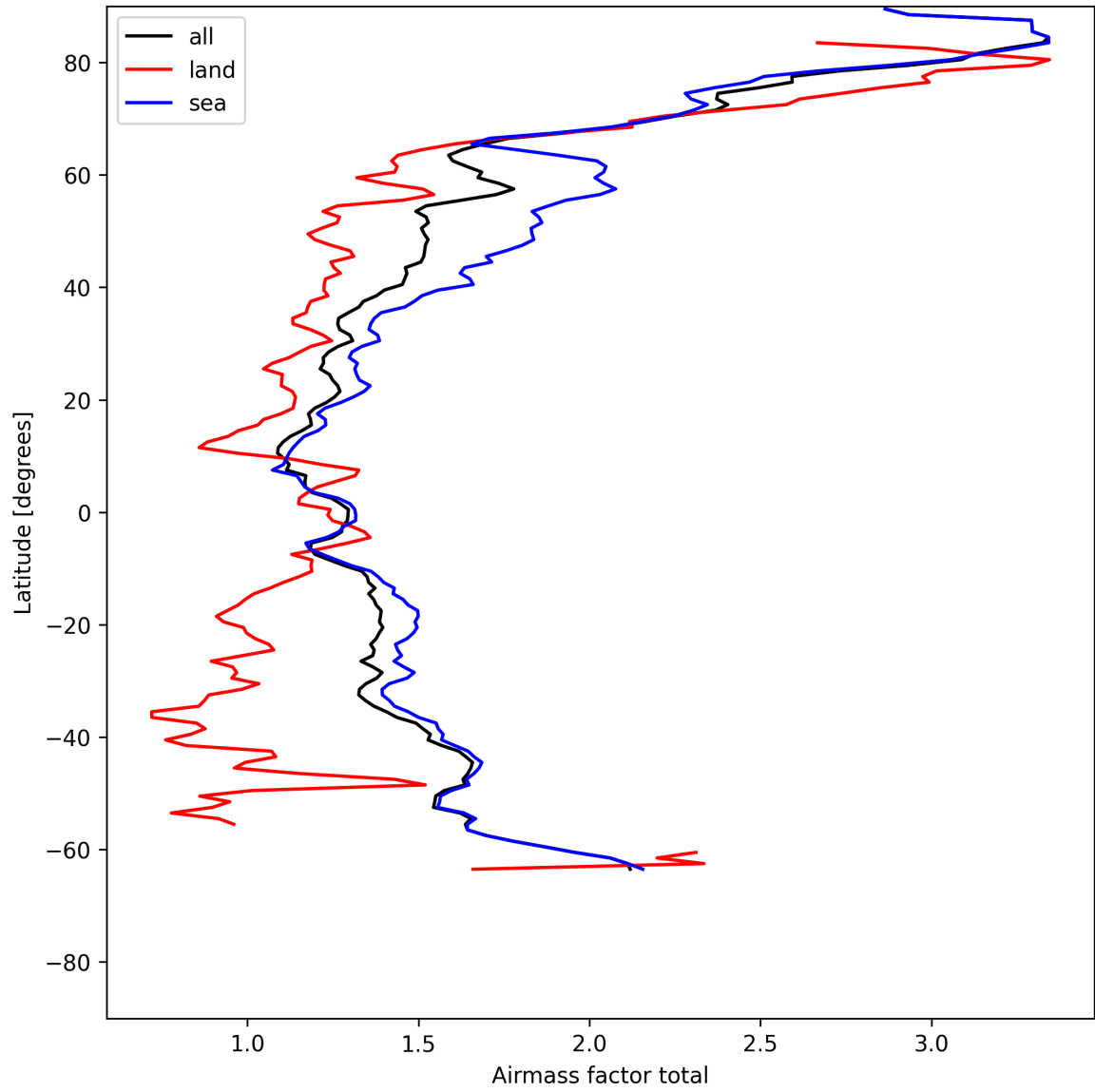
Figure 24: Zonal average of “Airmass factor total” for 2025-05-22 to 2025-05-23.
