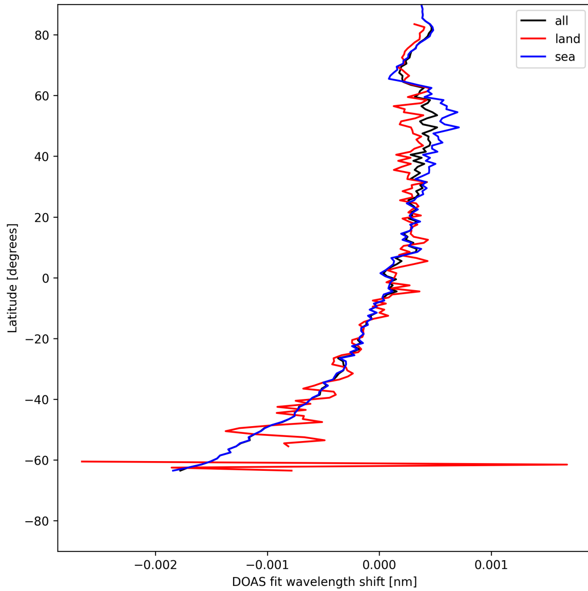
Figure 28: Zonal average of “DOAS fit wavelength shift” for 2025-05-22 to 2025-05-23.
