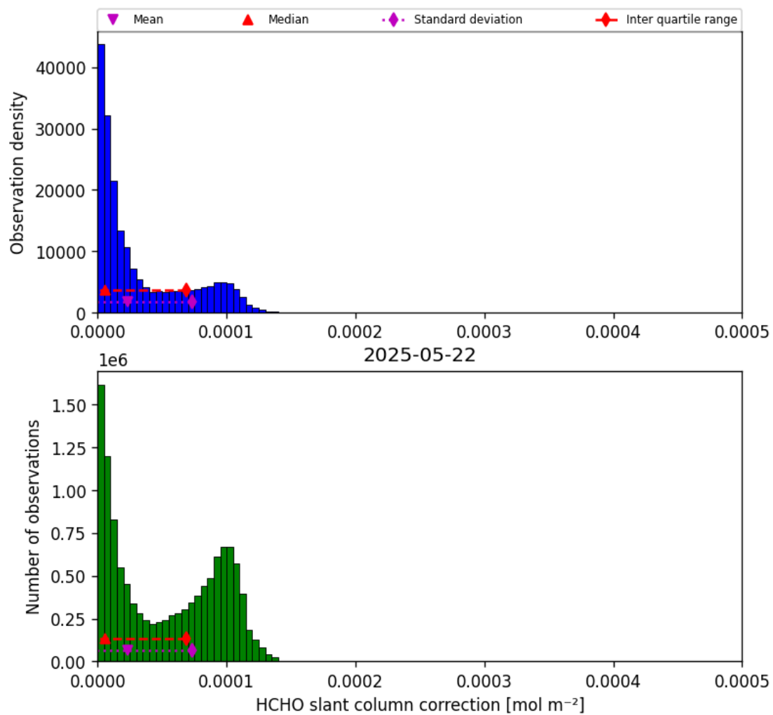
Figure 45: Histogram of “HCHO slant column correction” for 2025-05-22 to 2025-05-23
