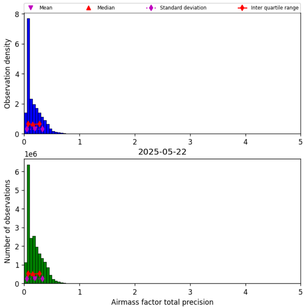
Figure 39: Histogram of “Airmass factor total precision” for 2025-05-22 to 2025-05-23
