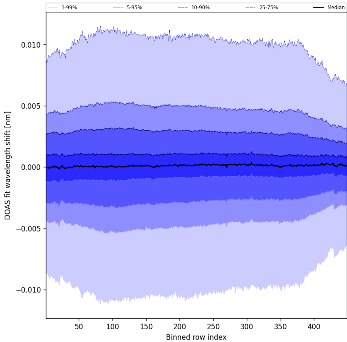
Figure 56: Along track statistics of “DOAS fit wavelength shift” for 2025-05-22 to 2025-05-23
