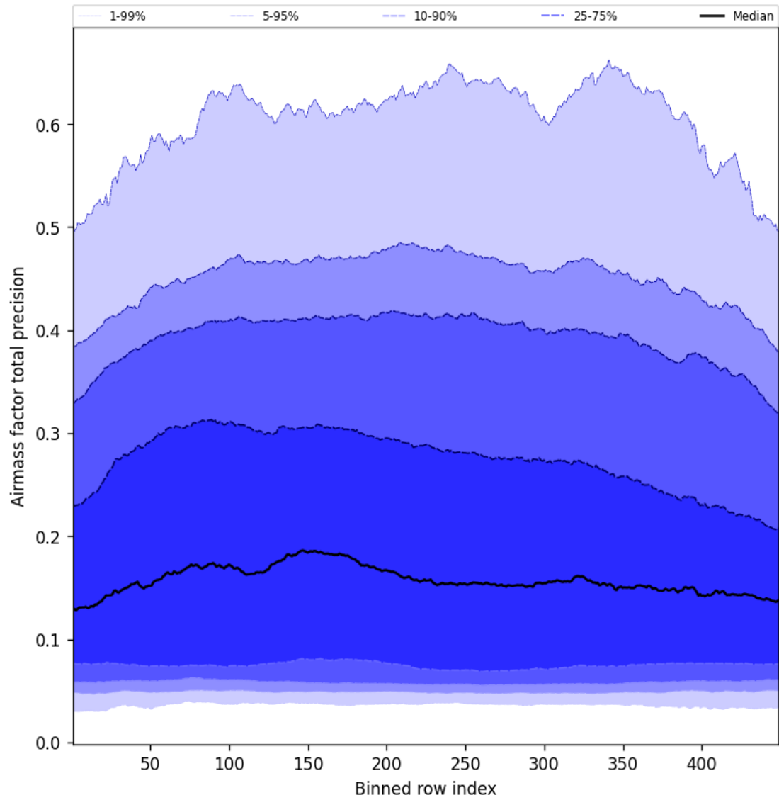
Figure 53: Along track statistics of “Airmass factor total precision” for 2025-05-22 to 2025-05-23
