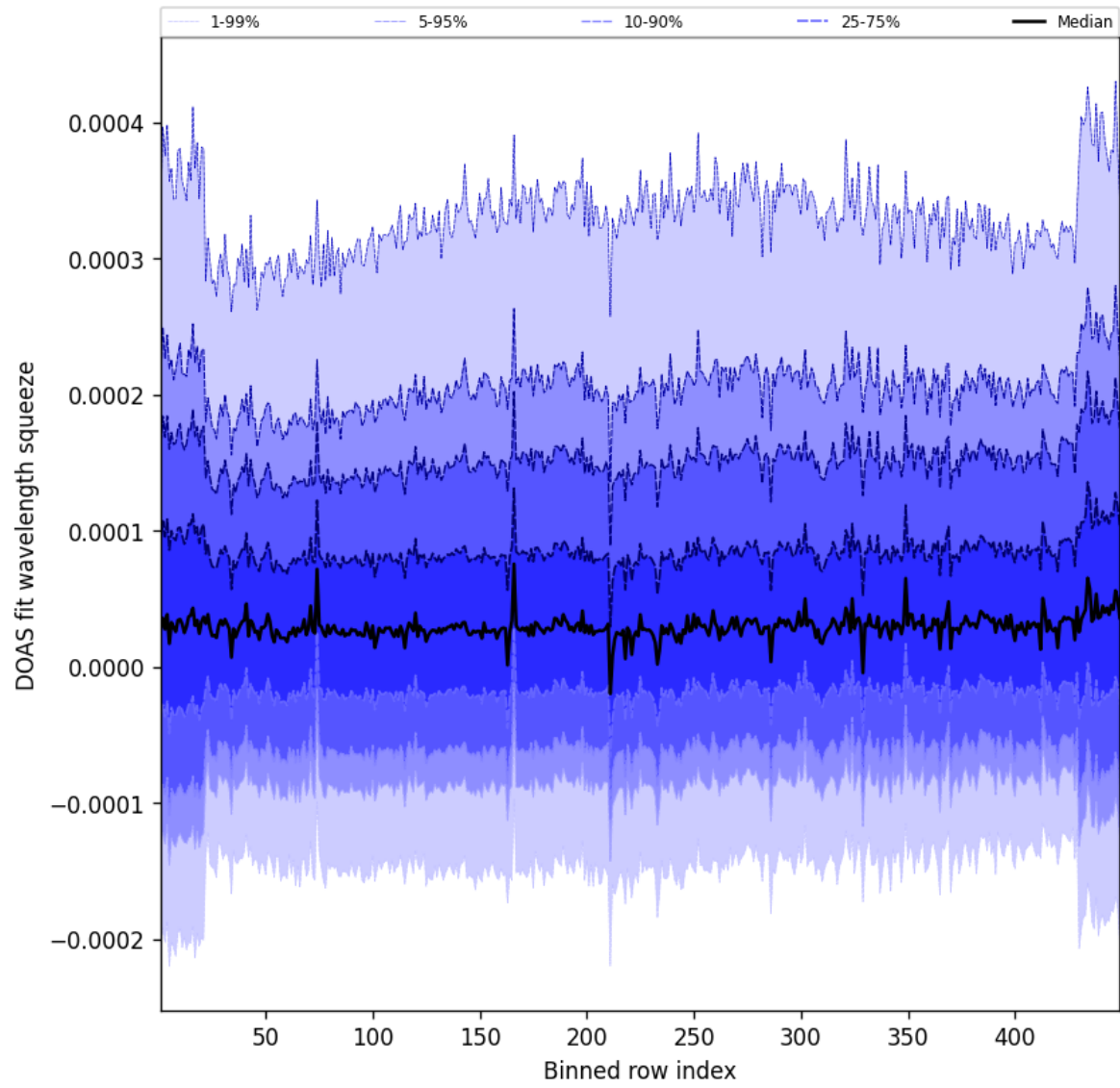
Figure 57: Along track statistics of “DOAS fit wavelength squeeze” for 2025-05-22 to 2025-05-23
