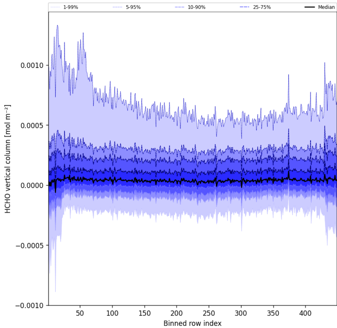
Figure 47: Along track statistics of “HCHO vertical column” for 2025-05-22 to 2025-05-23
