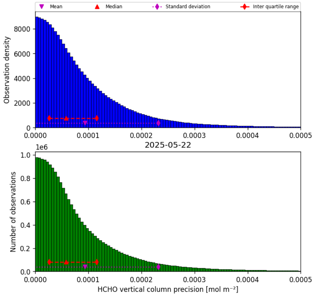
Figure 34: Histogram of “HCHO vertical column precision” for 2025-05-22 to 2025-05-23
