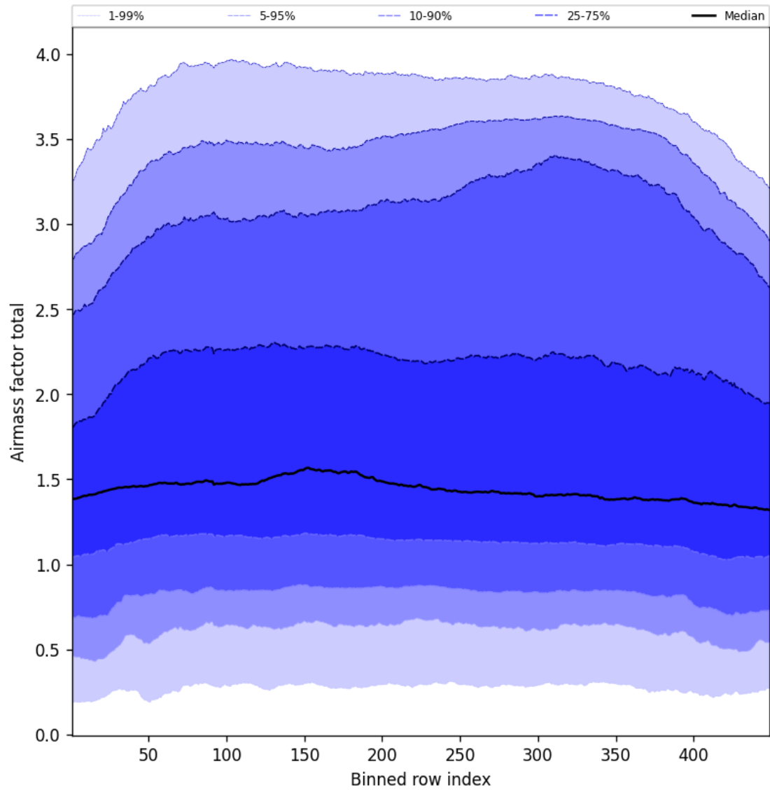
Figure 52: Along track statistics of “Airmass factor total” for 2025-05-22 to 2025-05-23
