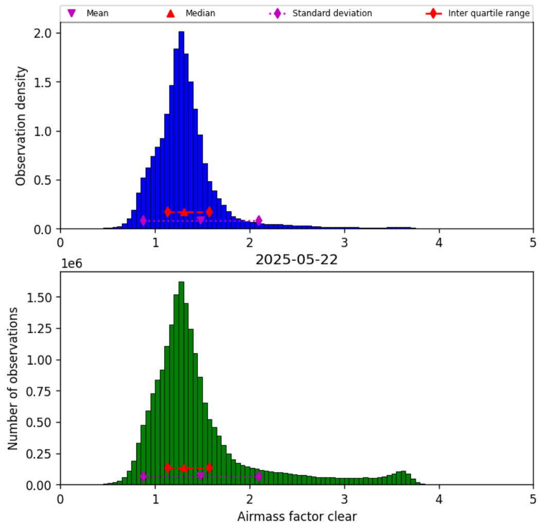
Figure 40: Histogram of “Airmass factor clear” for 2025-05-22 to 2025-05-23
