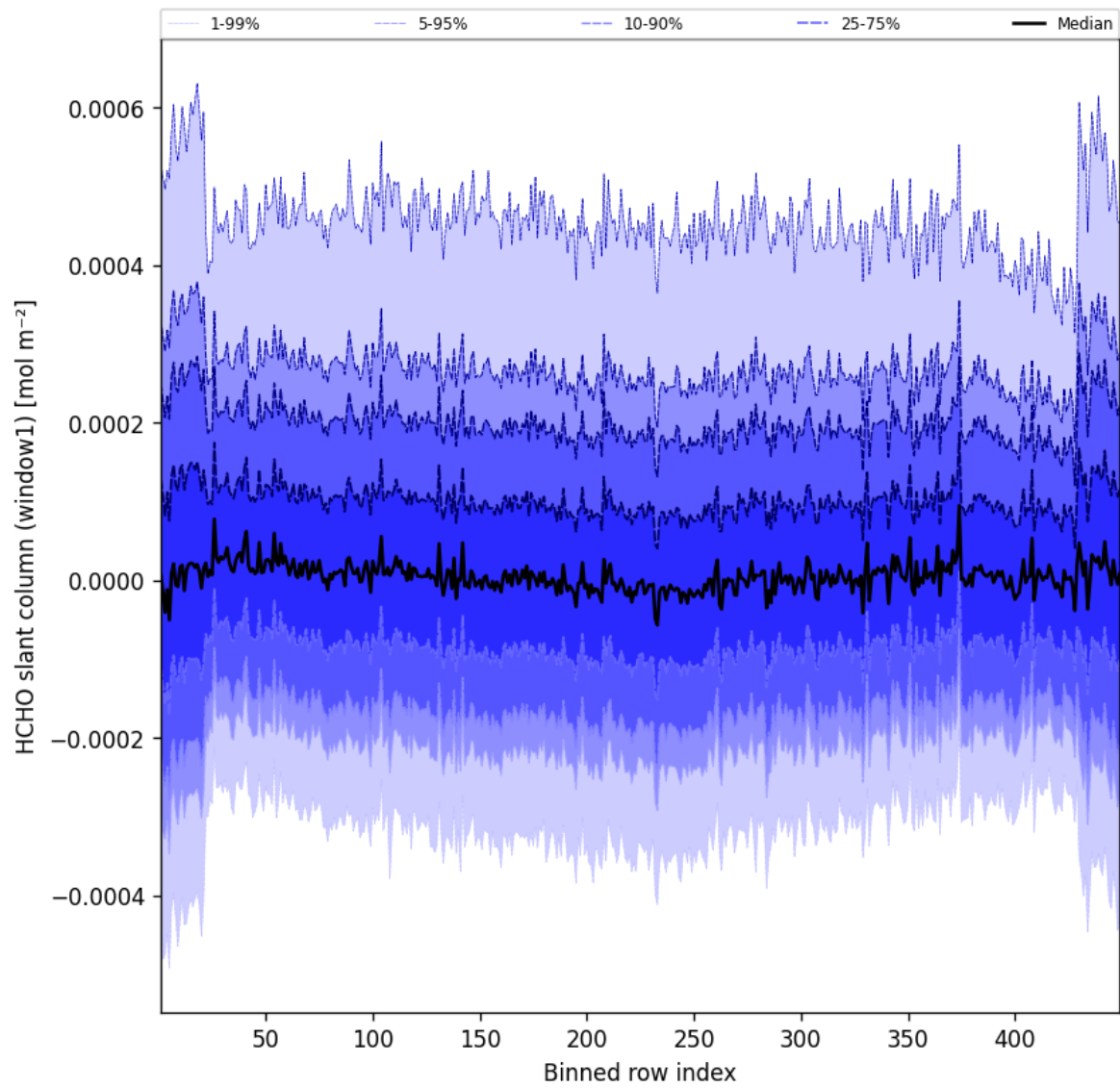
Figure 50: Along track statistics of “HCHO slant column (window1)” for 2025-05-22 to 2025-05-23
