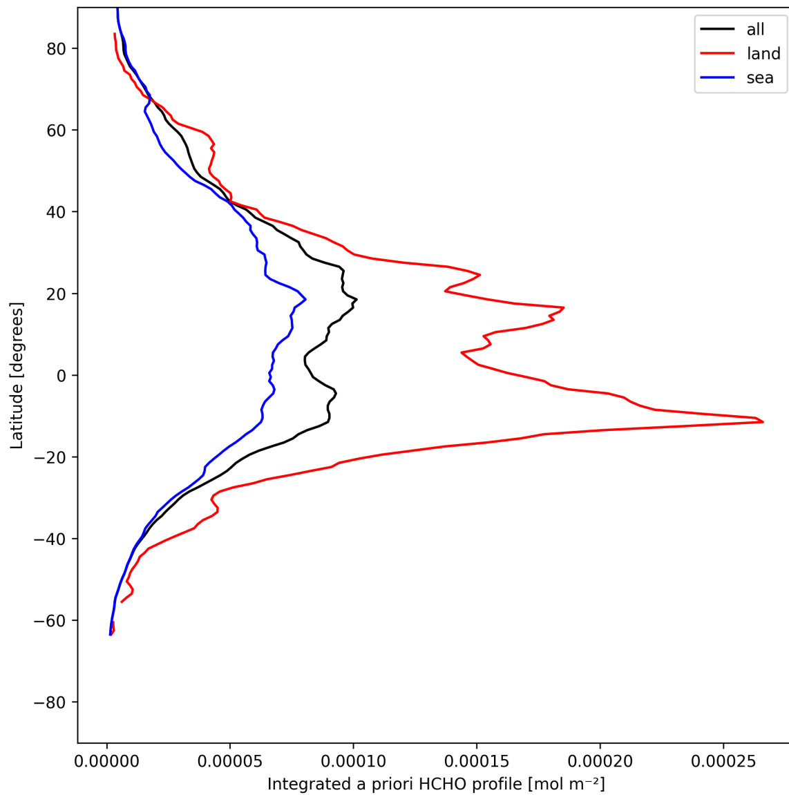
Figure 27: Zonal average of “Integrated a priori HCHO profile” for 2025-05-22 to 2025-05-23.
