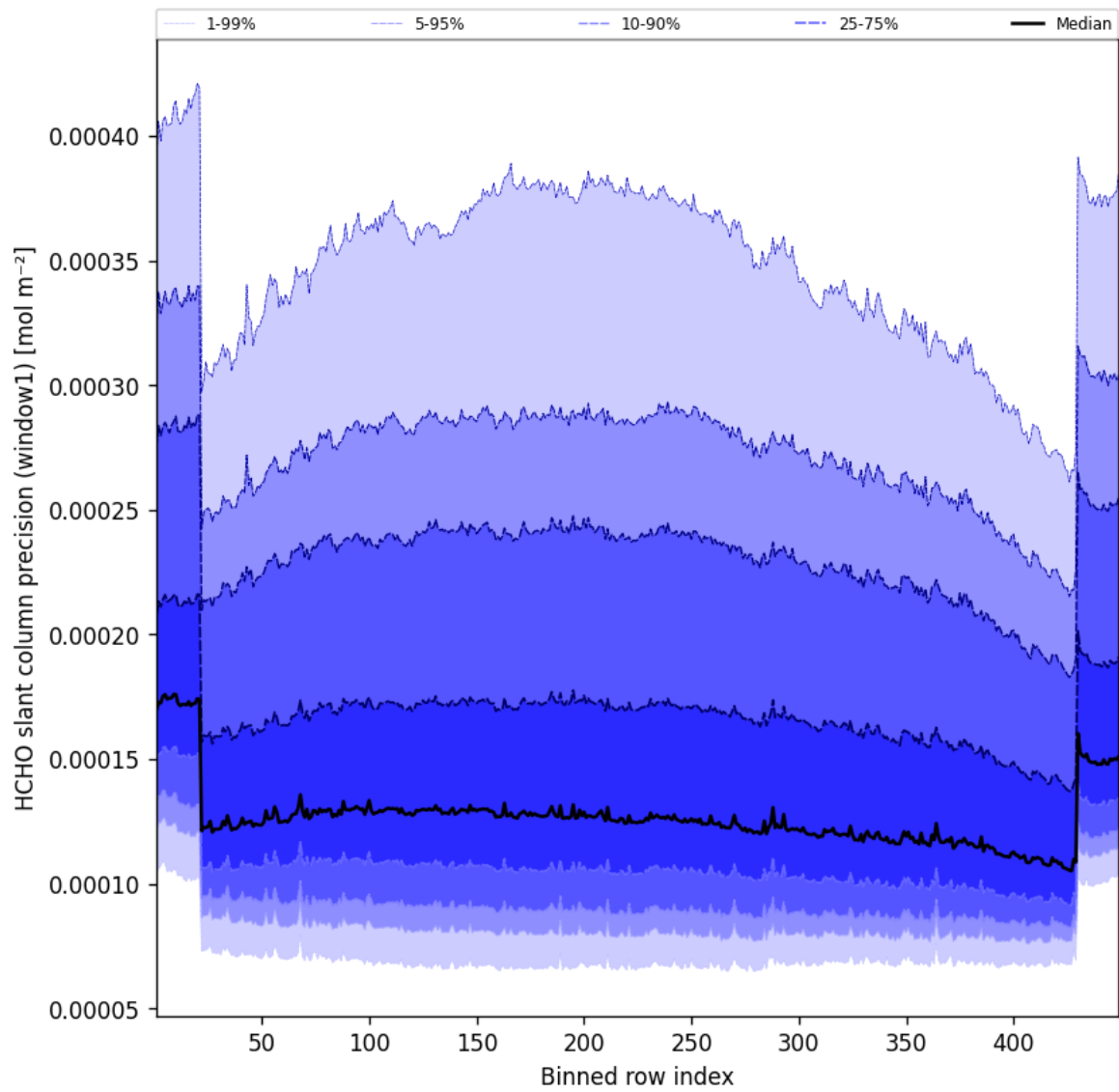
Figure 51: Along track statistics of “HCHO slant column precision (window1)” for 2025-05-22 to 2025-05-23
