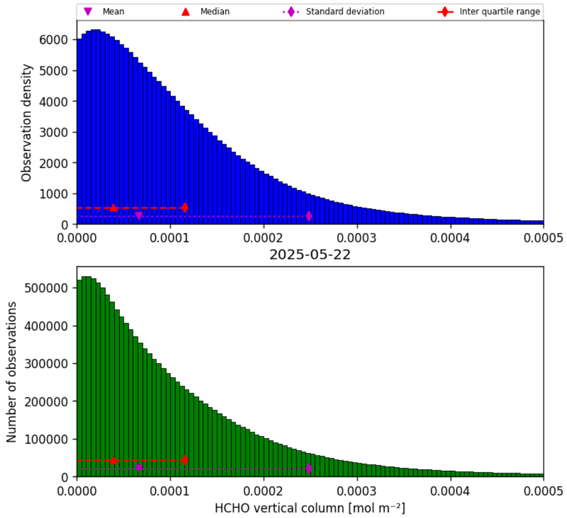
Figure 33: Histogram of “HCHO vertical column” for 2025-05-22 to 2025-05-23
