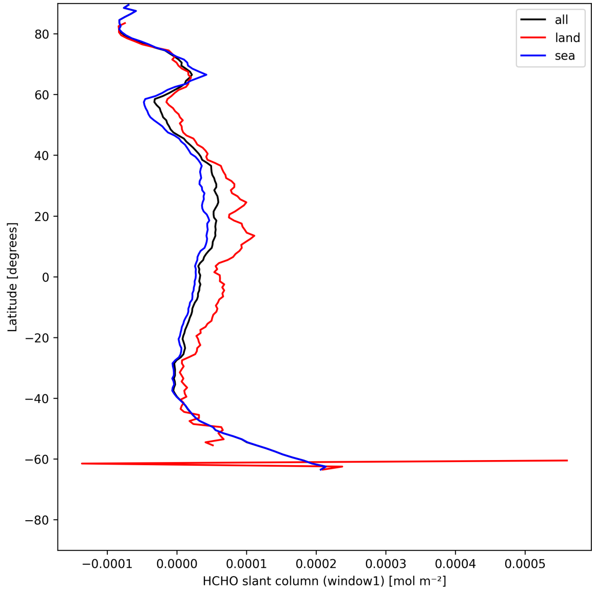
Figure 22: Zonal average of “HCHO slant column (window1)” for 2025-05-22 to 2025-05-23.
