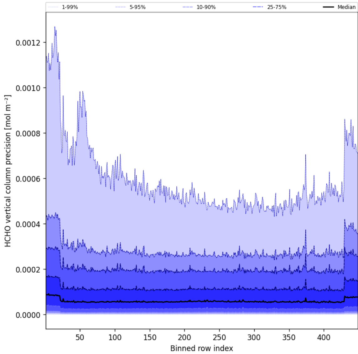
Figure 48: Along track statistics of “HCHO vertical column precision” for 2025-05-22 to 2025-05-23
