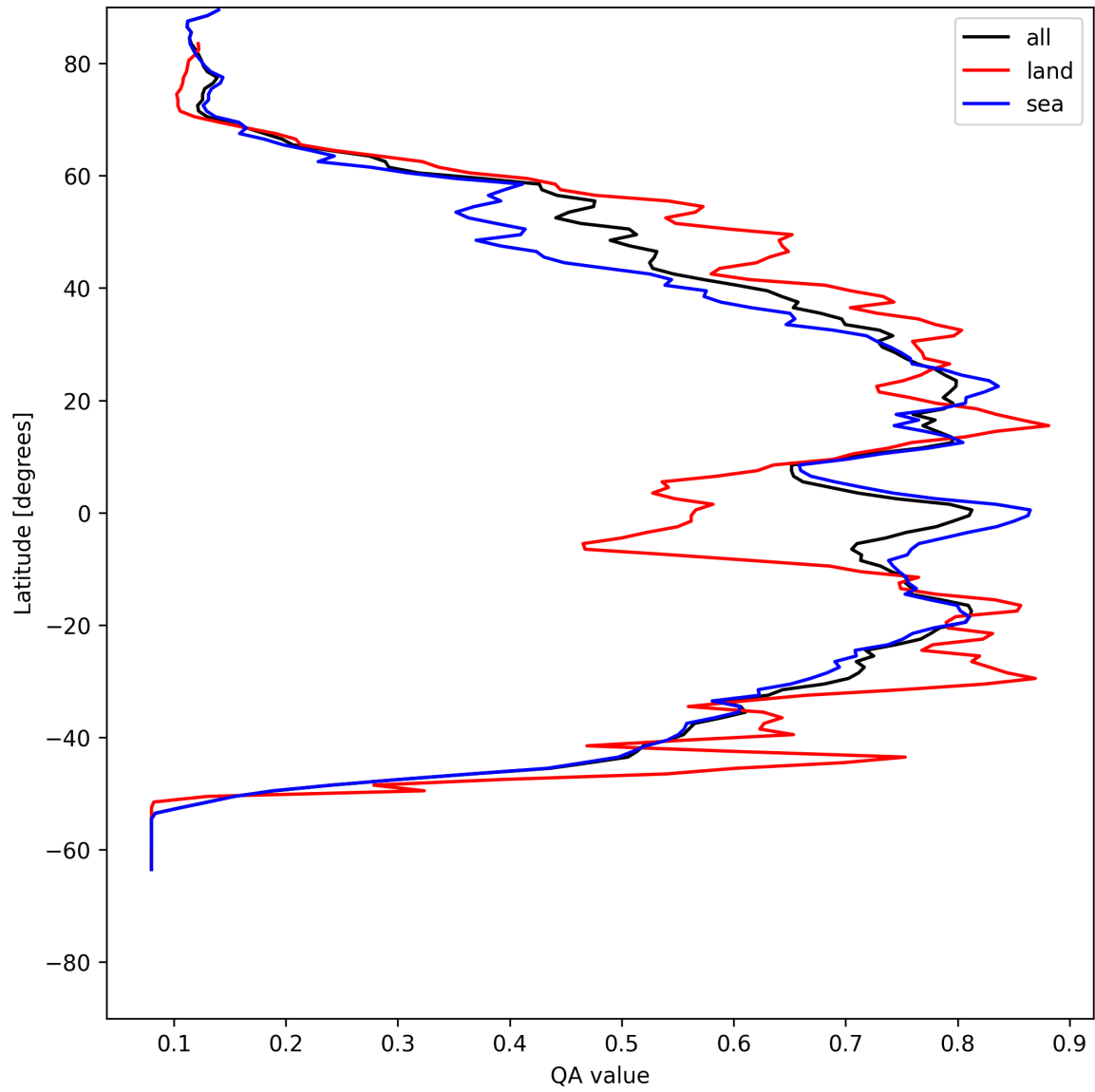
Figure 18: Zonal average of “QA value” for 2025-05-22 to 2025-05-23.
