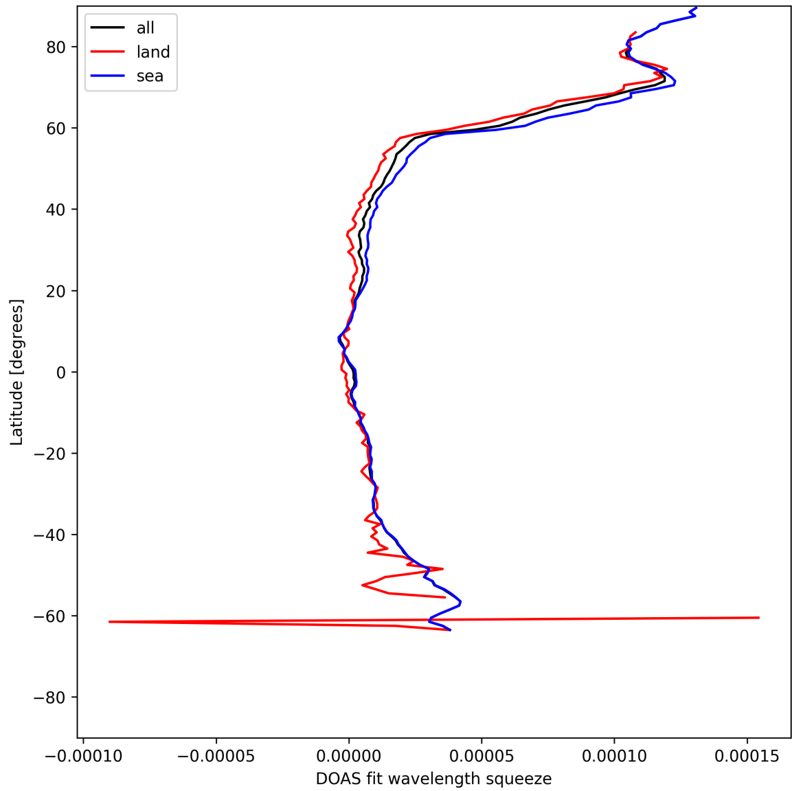
Figure 29: Zonal average of “DOAS fit wavelength squeeze” for 2025-05-22 to 2025-05-23.
