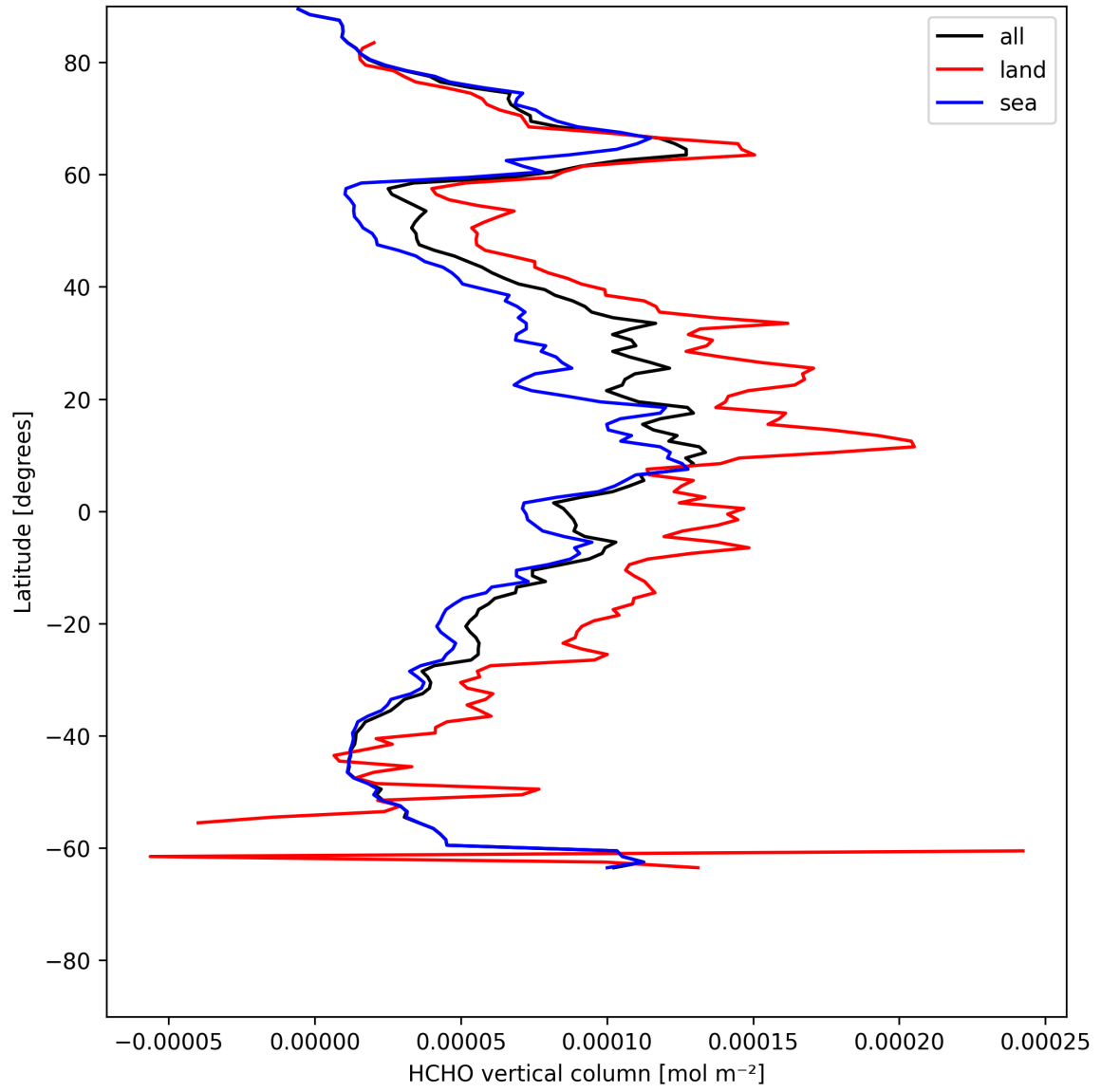
Figure 19: Zonal average of “HCHO vertical column” for 2025-05-22 to 2025-05-23.
