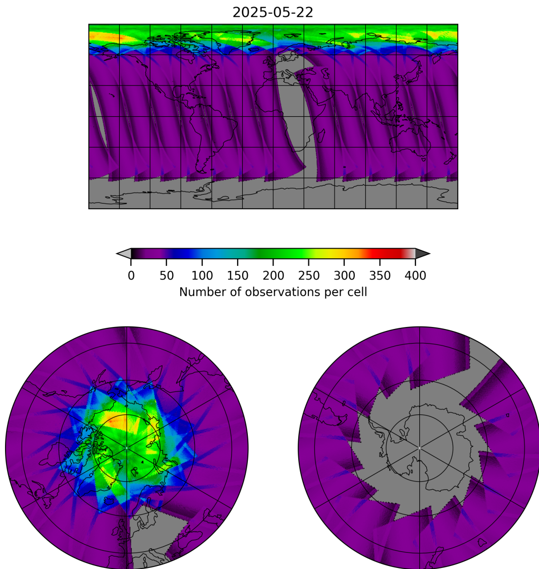
Figure 17: Map of the number of observations for 2025-05-22 to 2025-05-23
