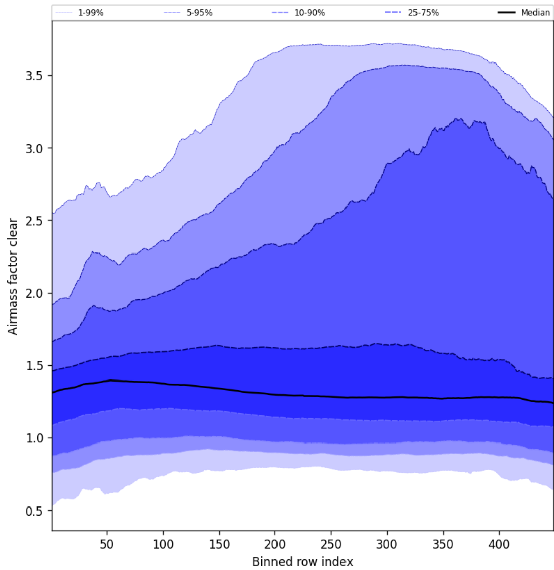
Figure 54: Along track statistics of “Airmass factor clear” for 2025-05-22 to 2025-05-23
