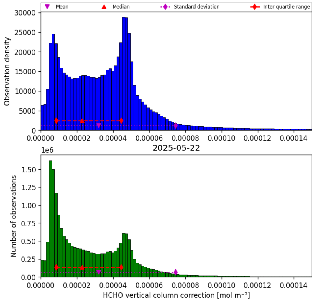
Figure 35: Histogram of “HCHO vertical column correction” for 2025-05-22 to 2025-05-23
