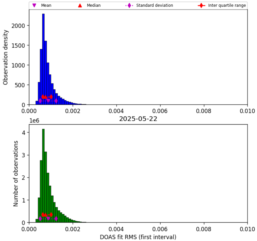
Figure 44: Histogram of “DOAS fit RMS (first interval)” for 2025-05-22 to 2025-05-23
