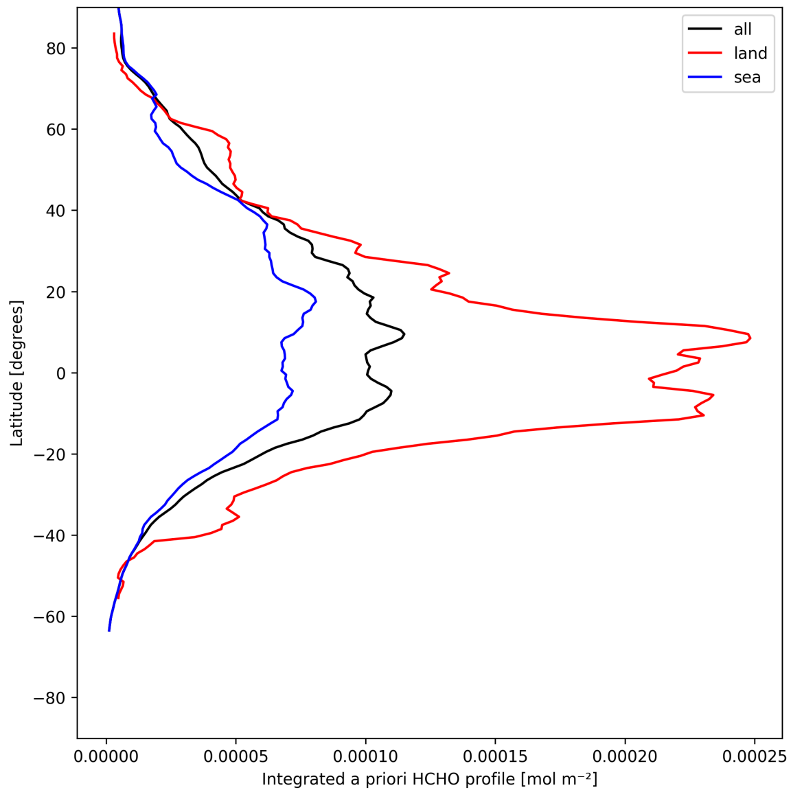
Figure 27: Zonal average of “Integrated a priori HCHO profile” for 2025-05-23 to 2025-05-24.
