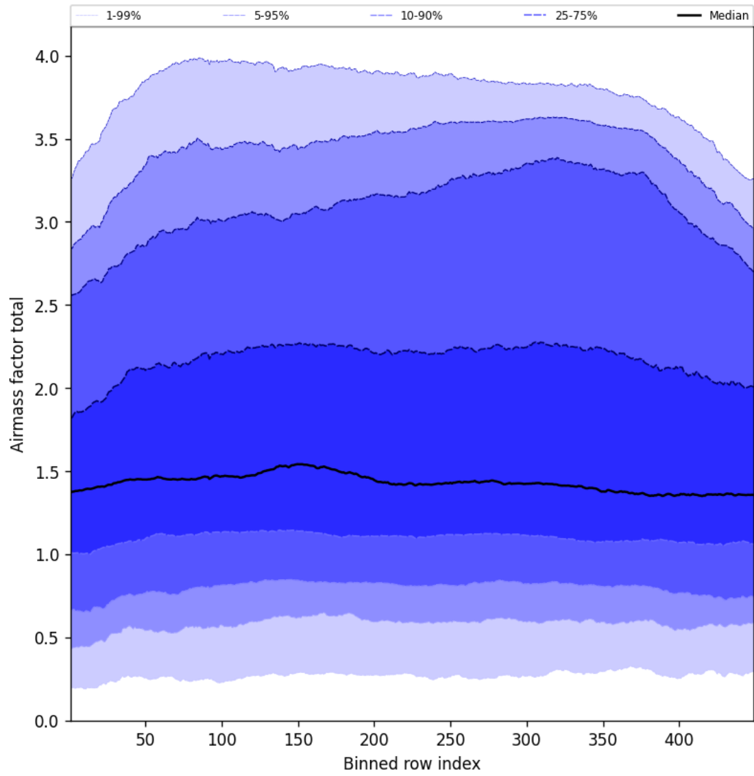
Figure 52: Along track statistics of “Airmass factor total” for 2025-05-23 to 2025-05-24
