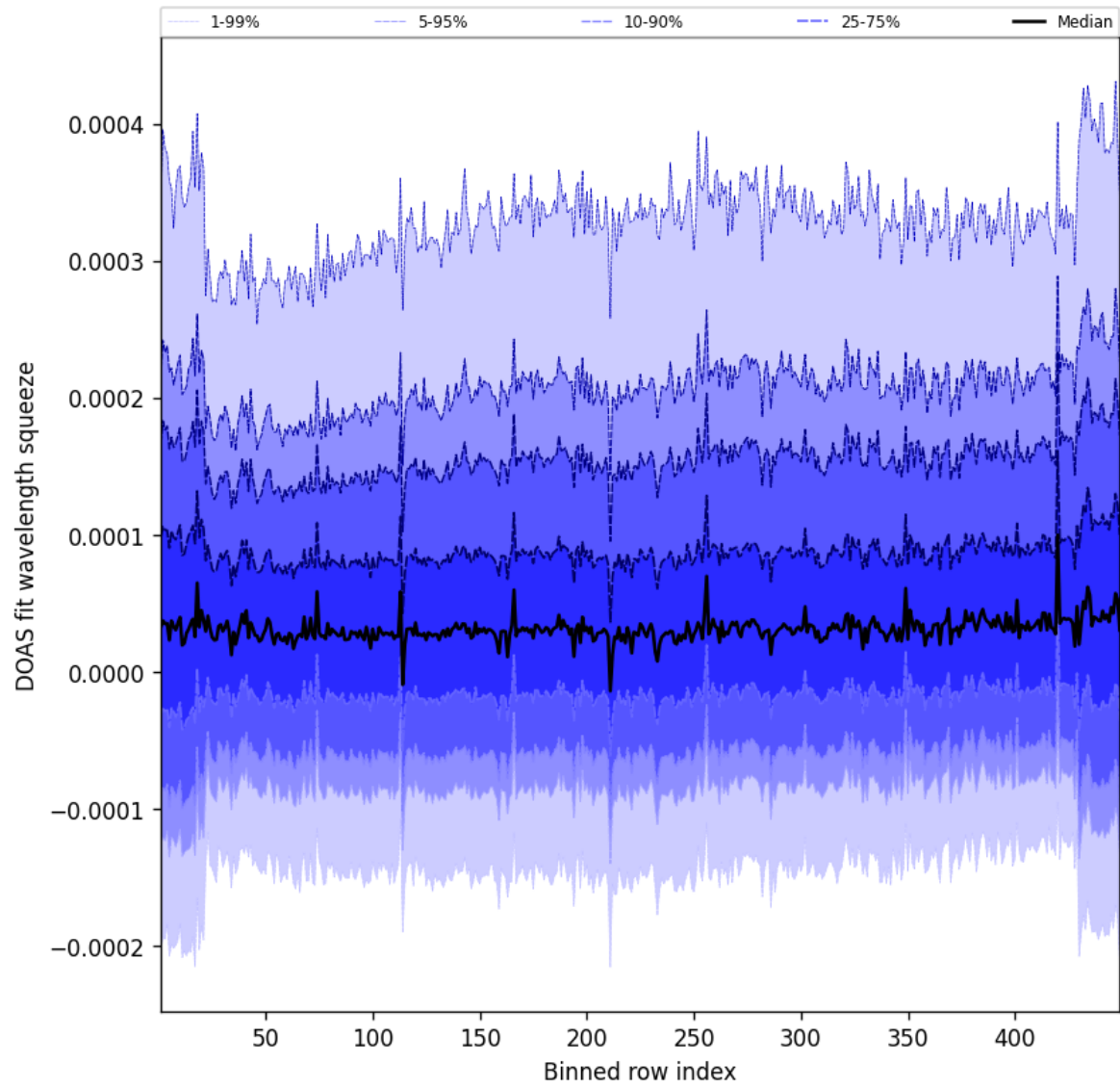
Figure 57: Along track statistics of “DOAS fit wavelength squeeze” for 2025-05-23 to 2025-05-24
