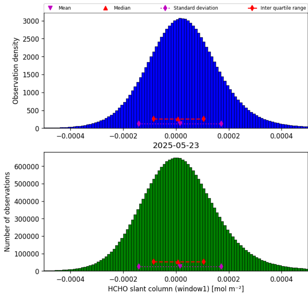
Figure 36: Histogram of “HCHO slant column (window1)” for 2025-05-23 to 2025-05-24
