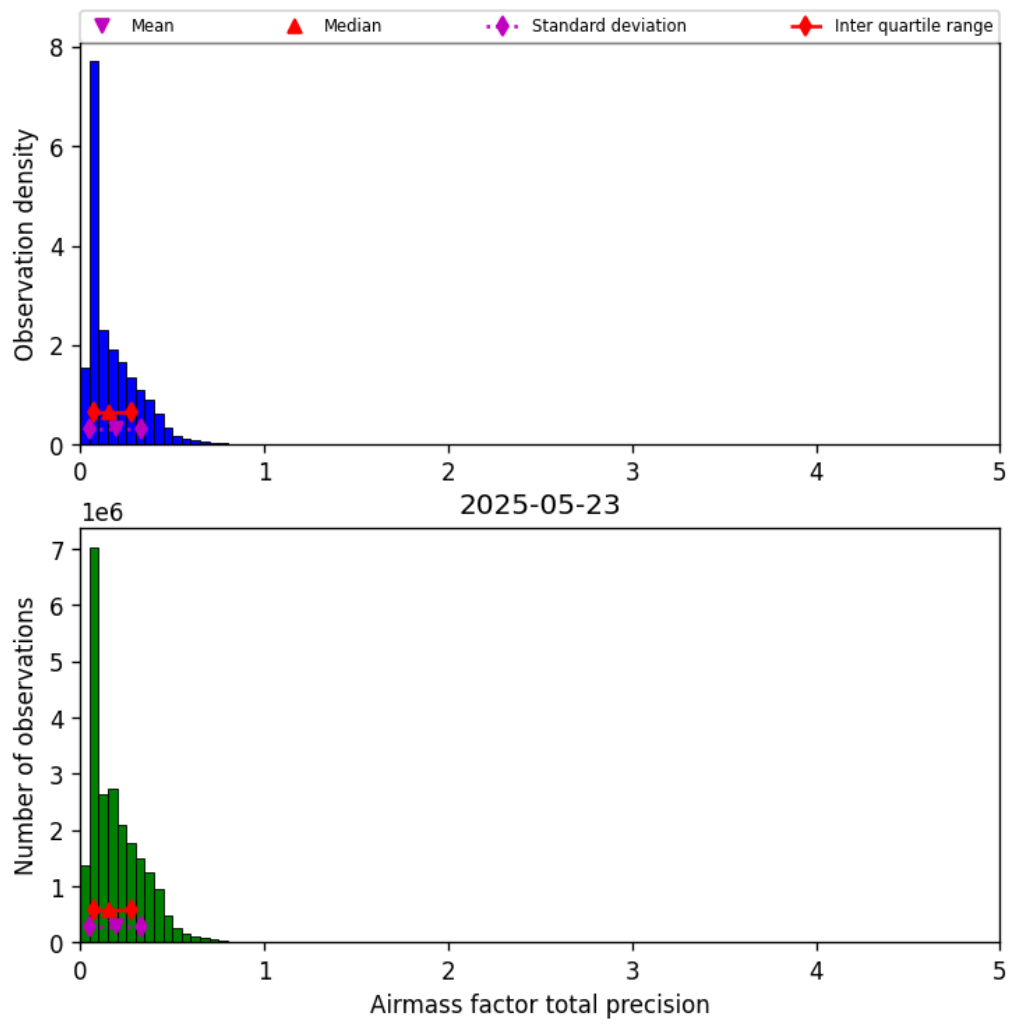
Figure 39: Histogram of “Airmass factor total precision” for 2025-05-23 to 2025-05-24
