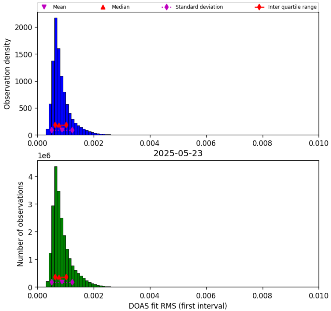
Figure 44: Histogram of “DOAS fit RMS (first interval)” for 2025-05-23 to 2025-05-24
