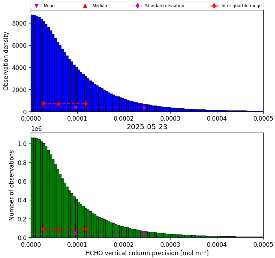
Figure 34: Histogram of “HCHO vertical column precision” for 2025-05-23 to 2025-05-24
