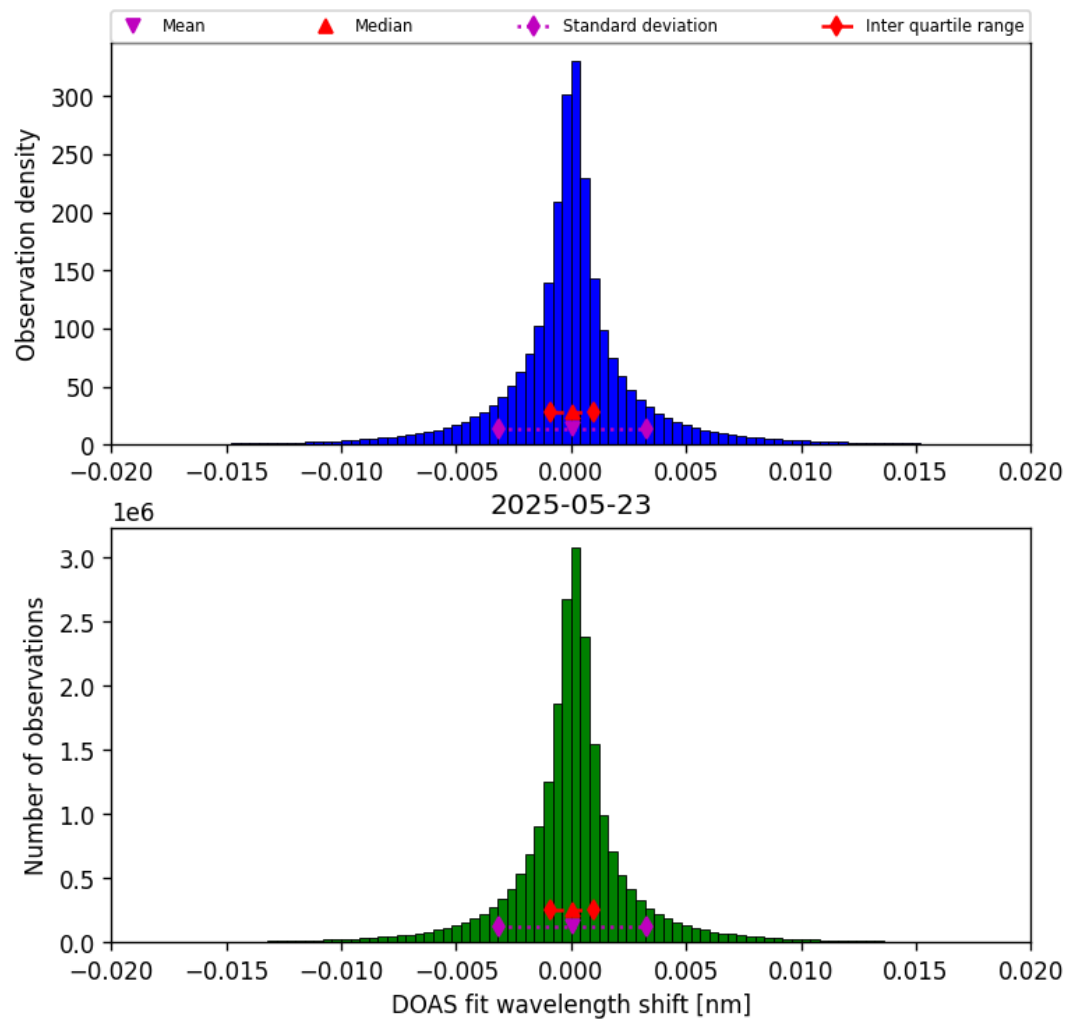
Figure 42: Histogram of “DOAS fit wavelength shift” for 2025-05-23 to 2025-05-24
