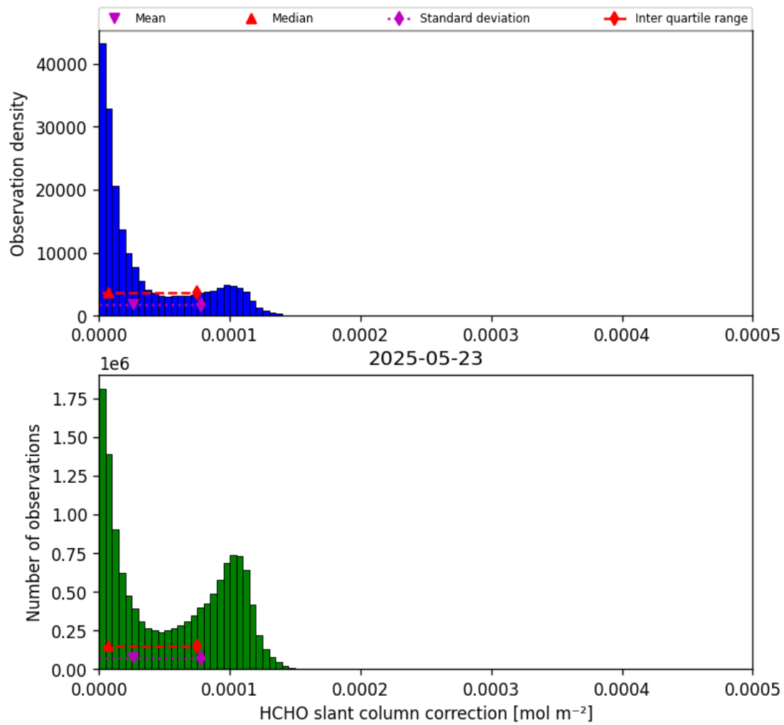
Figure 45: Histogram of “HCHO slant column correction” for 2025-05-23 to 2025-05-24
