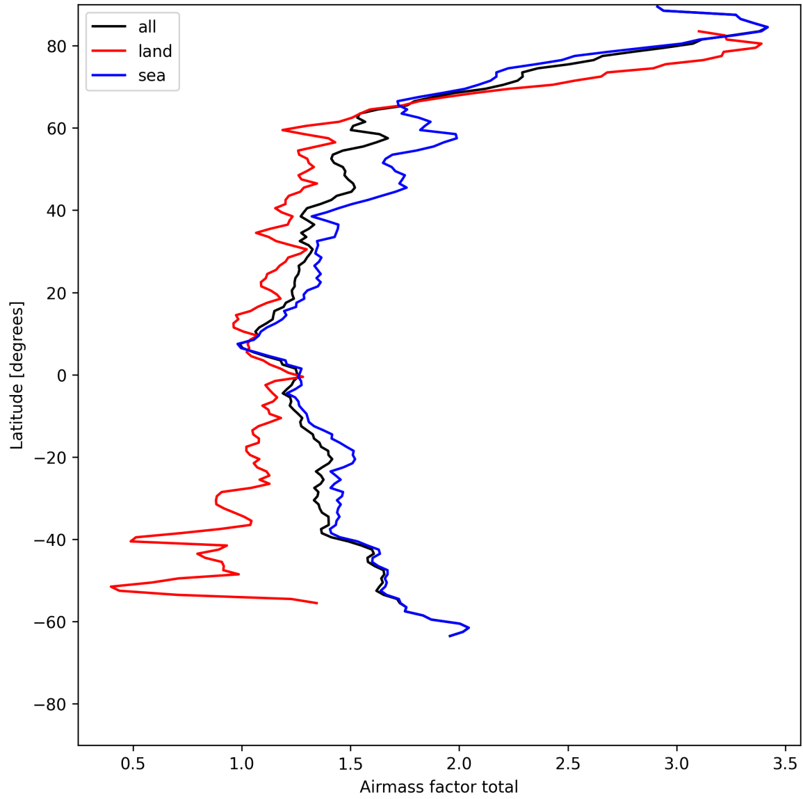
Figure 24: Zonal average of “Airmass factor total” for 2025-05-23 to 2025-05-24.
