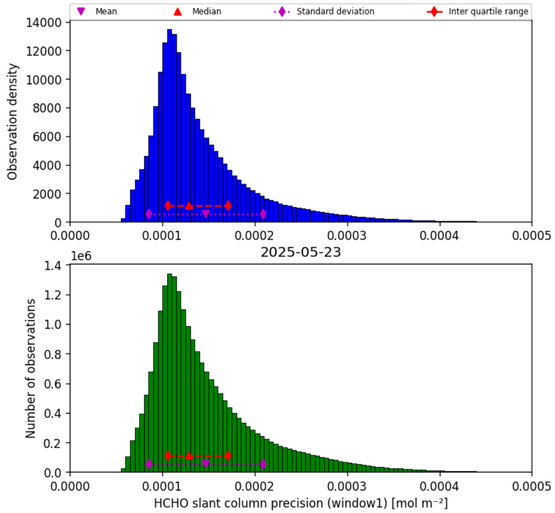
Figure 37: Histogram of “HCHO slant column precision (window1)” for 2025-05-23 to 2025-05-24
