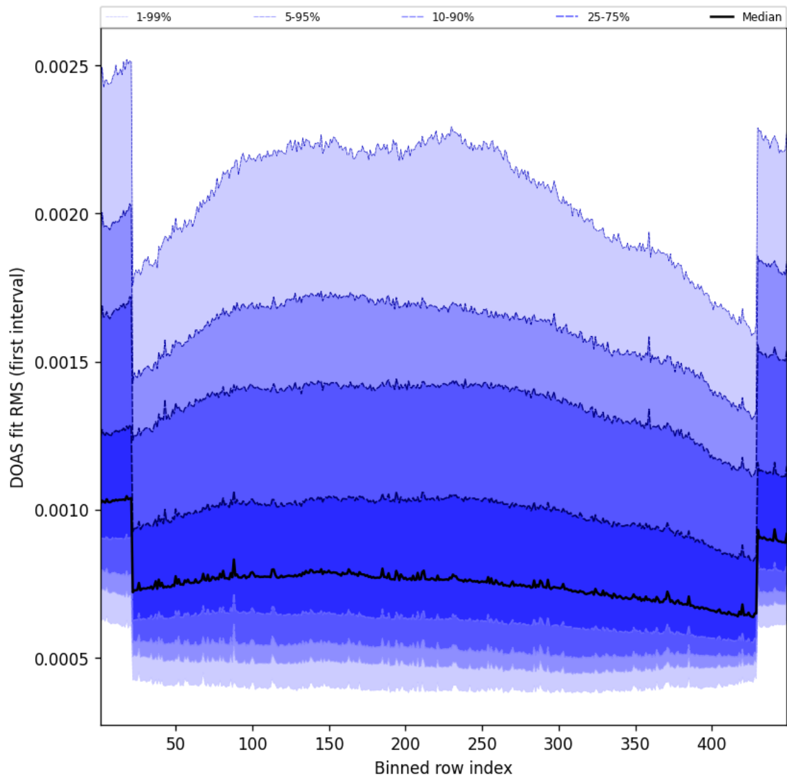
Figure 58: Along track statistics of “DOAS fit RMS (first interval)” for 2025-05-23 to 2025-05-24
