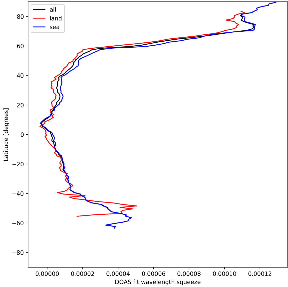
Figure 29: Zonal average of “DOAS fit wavelength squeeze” for 2025-05-23 to 2025-05-24.
