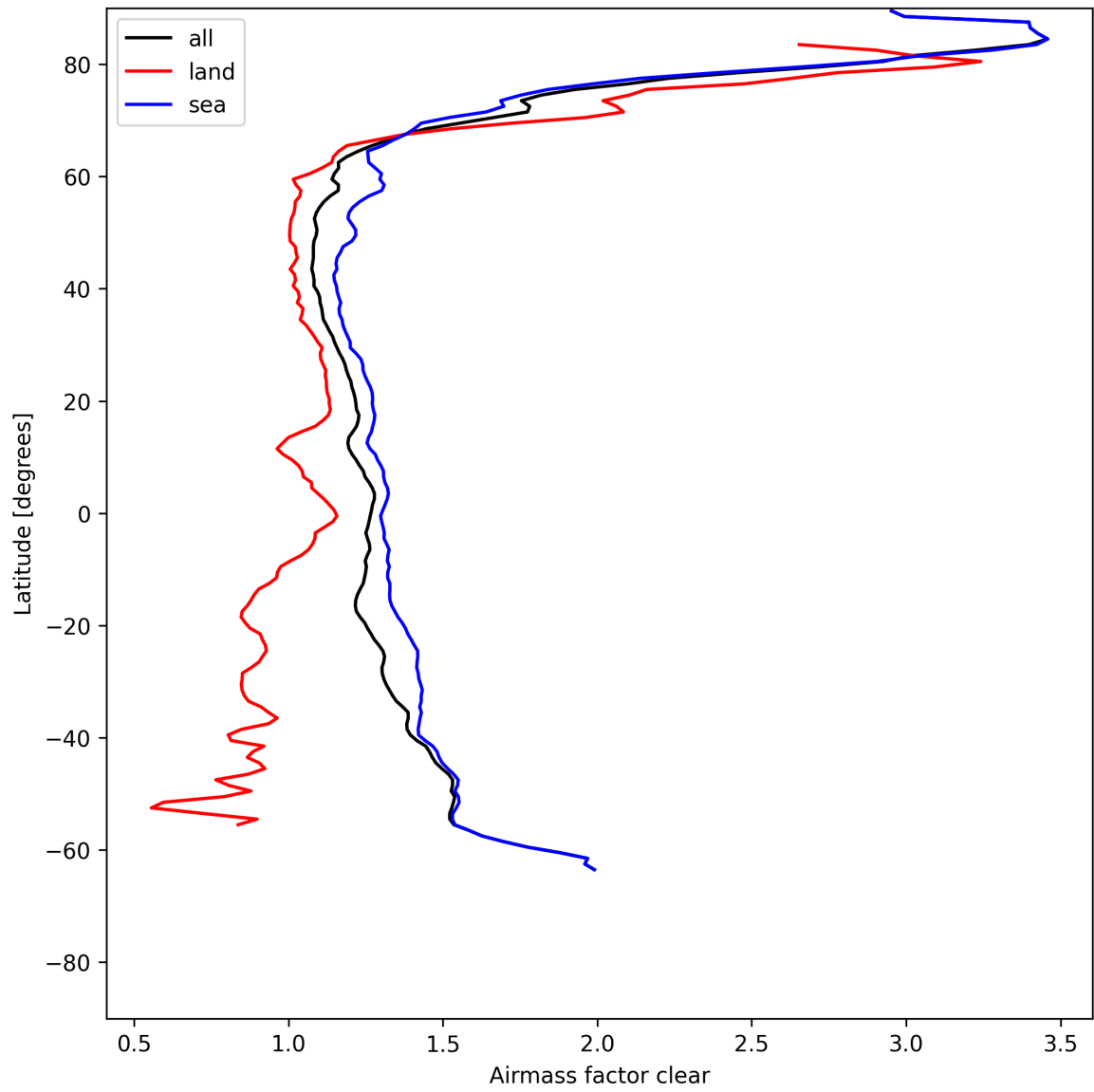
Figure 26: Zonal average of “Airmass factor clear” for 2025-05-23 to 2025-05-24.
