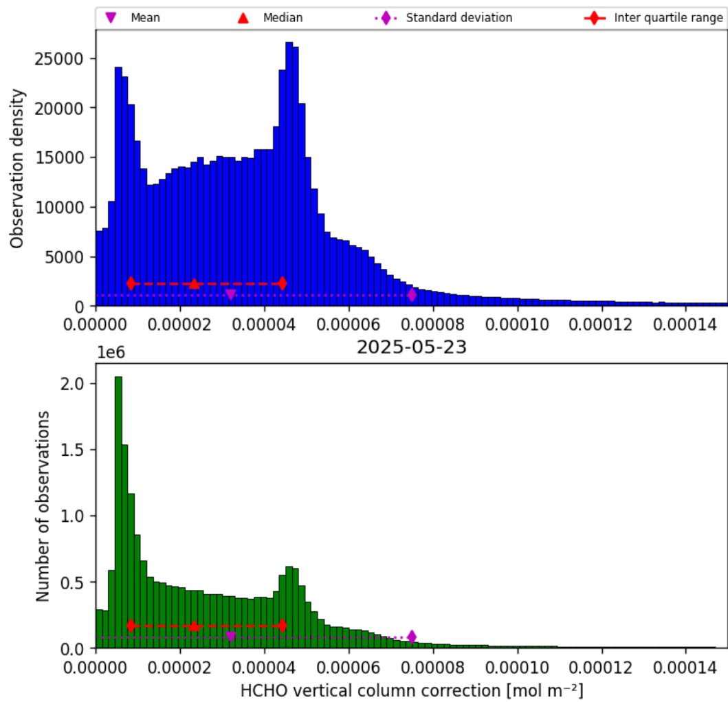
Figure 35: Histogram of “HCHO vertical column correction” for 2025-05-23 to 2025-05-24
