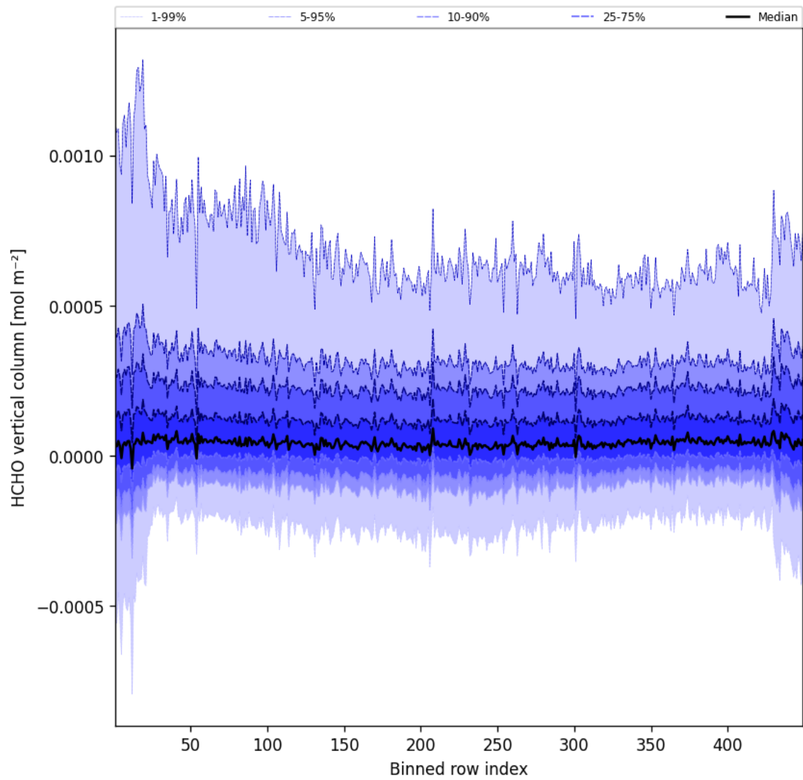
Figure 47: Along track statistics of “HCHO vertical column” for 2025-05-23 to 2025-05-24
