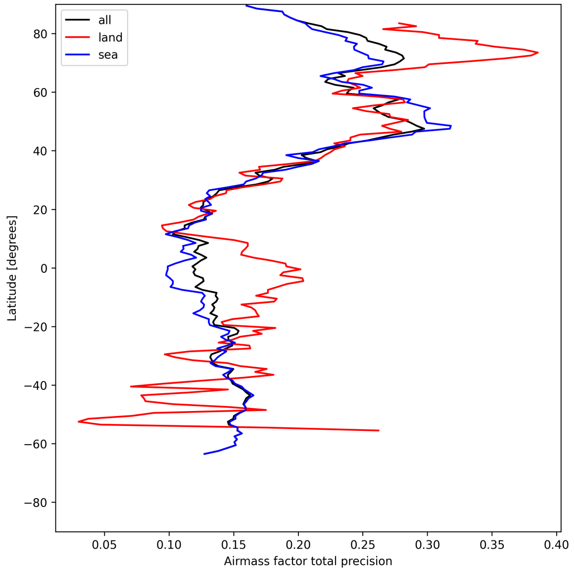
Figure 25: Zonal average of “Airmass factor total precision” for 2025-05-23 to 2025-05-24.
