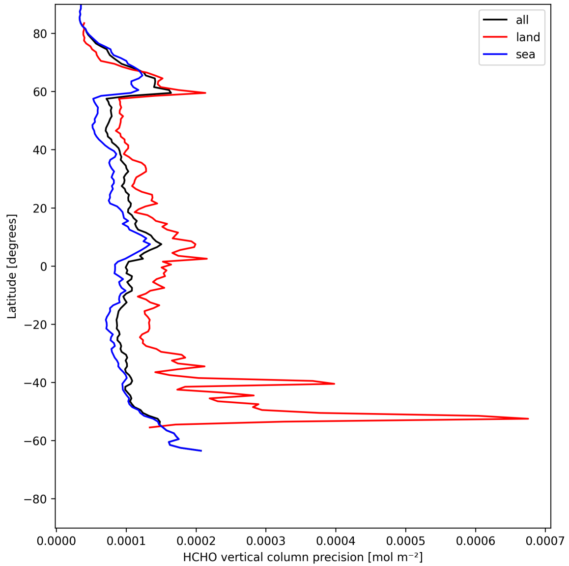
Figure 20: Zonal average of “HCHO vertical column precision” for 2025-05-23 to 2025-05-24.
