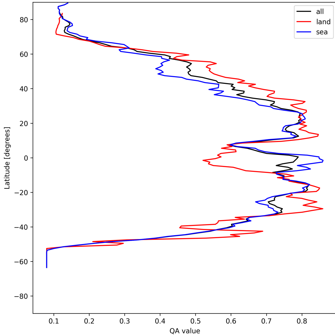
Figure 18: Zonal average of “QA value” for 2025-05-23 to 2025-05-24.
