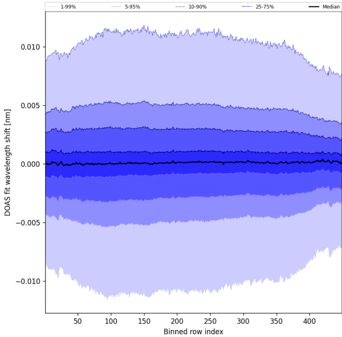
Figure 56: Along track statistics of “DOAS fit wavelength shift” for 2025-05-23 to 2025-05-24
