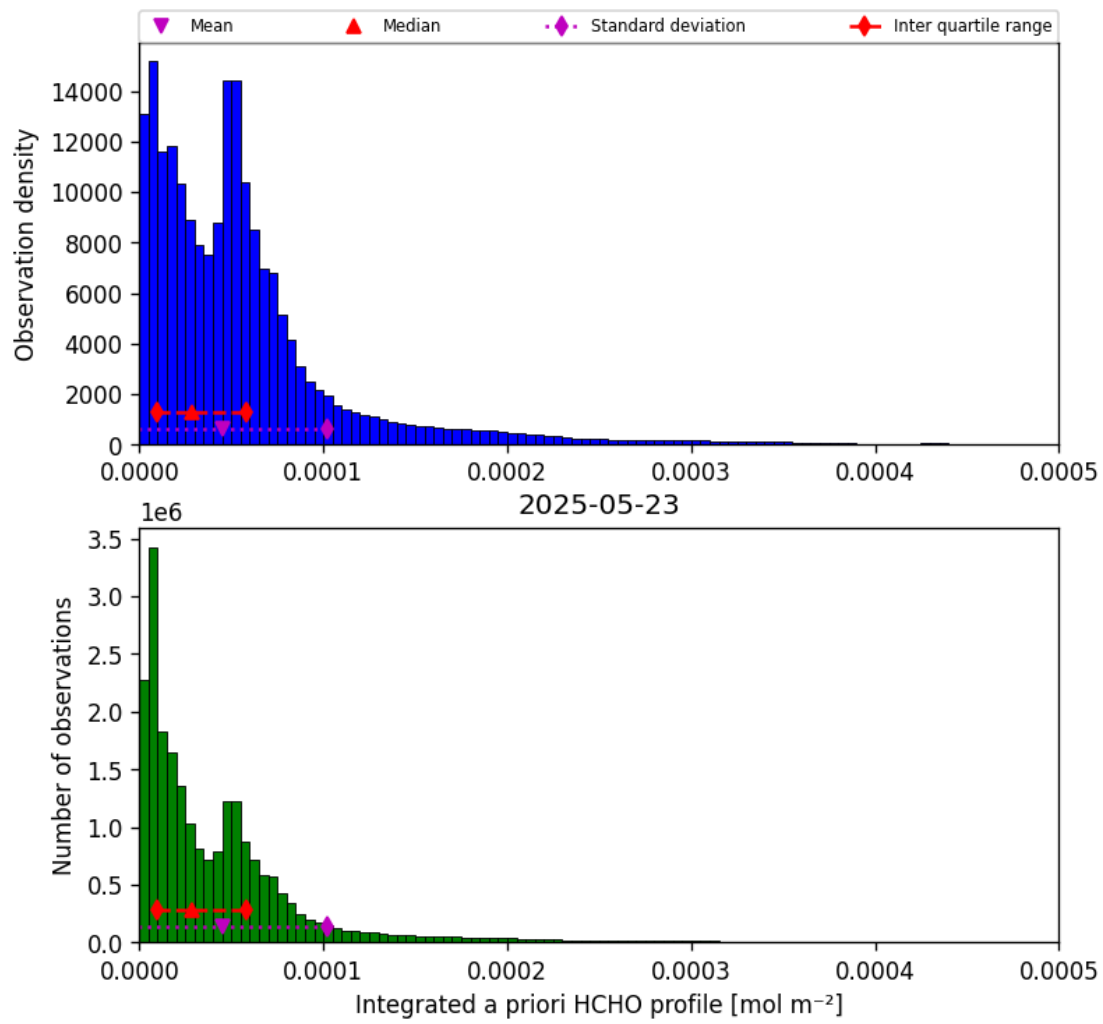
Figure 41: Histogram of “Integrated a priori HCHO profile” for 2025-05-23 to 2025-05-24
