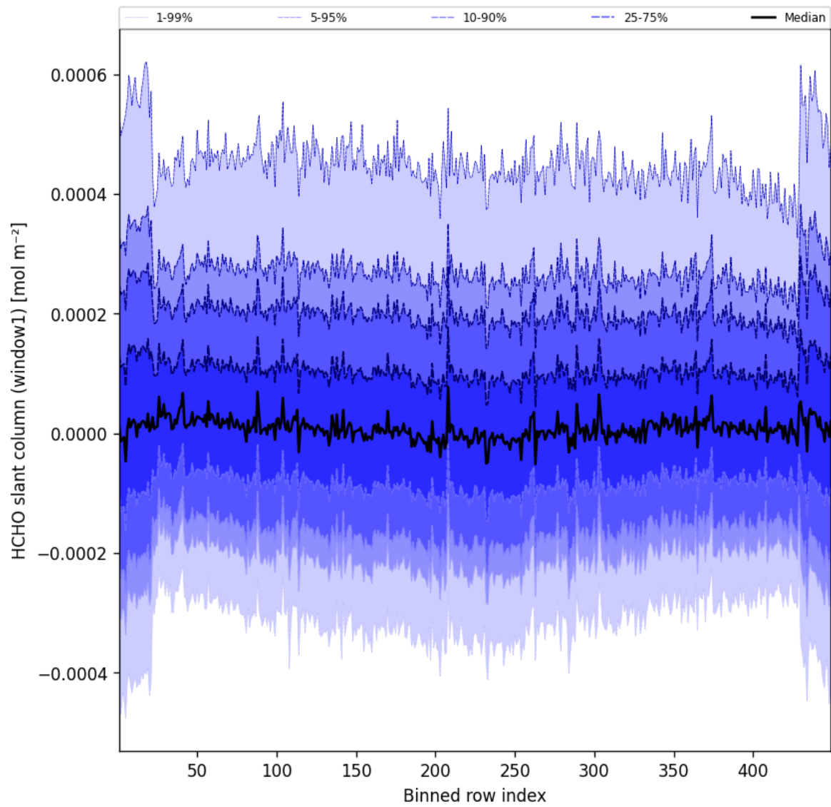
Figure 50: Along track statistics of “HCHO slant column (window1)” for 2025-05-23 to 2025-05-24
