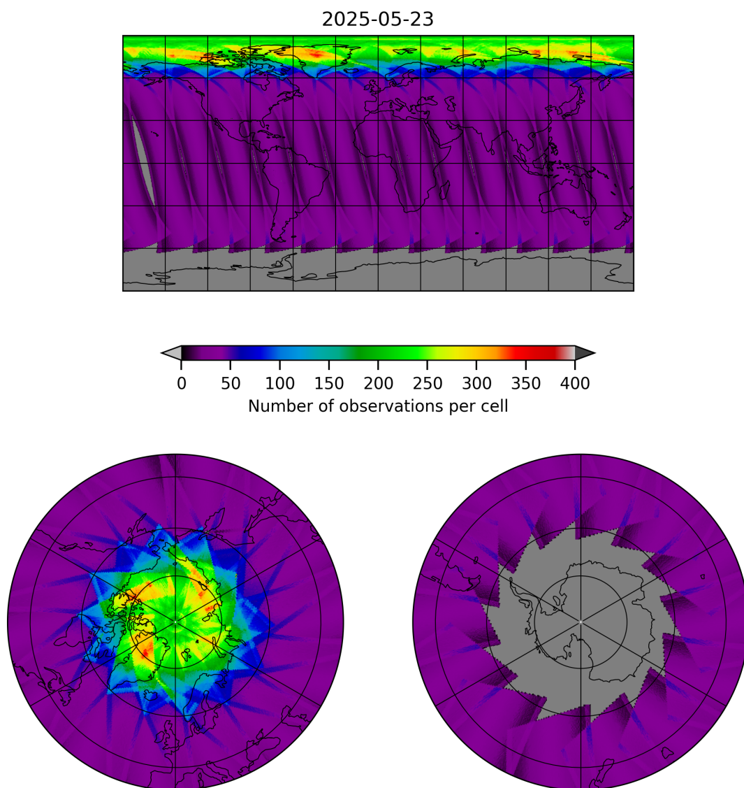
Figure 17: Map of the number of observations for 2025-05-23 to 2025-05-24
