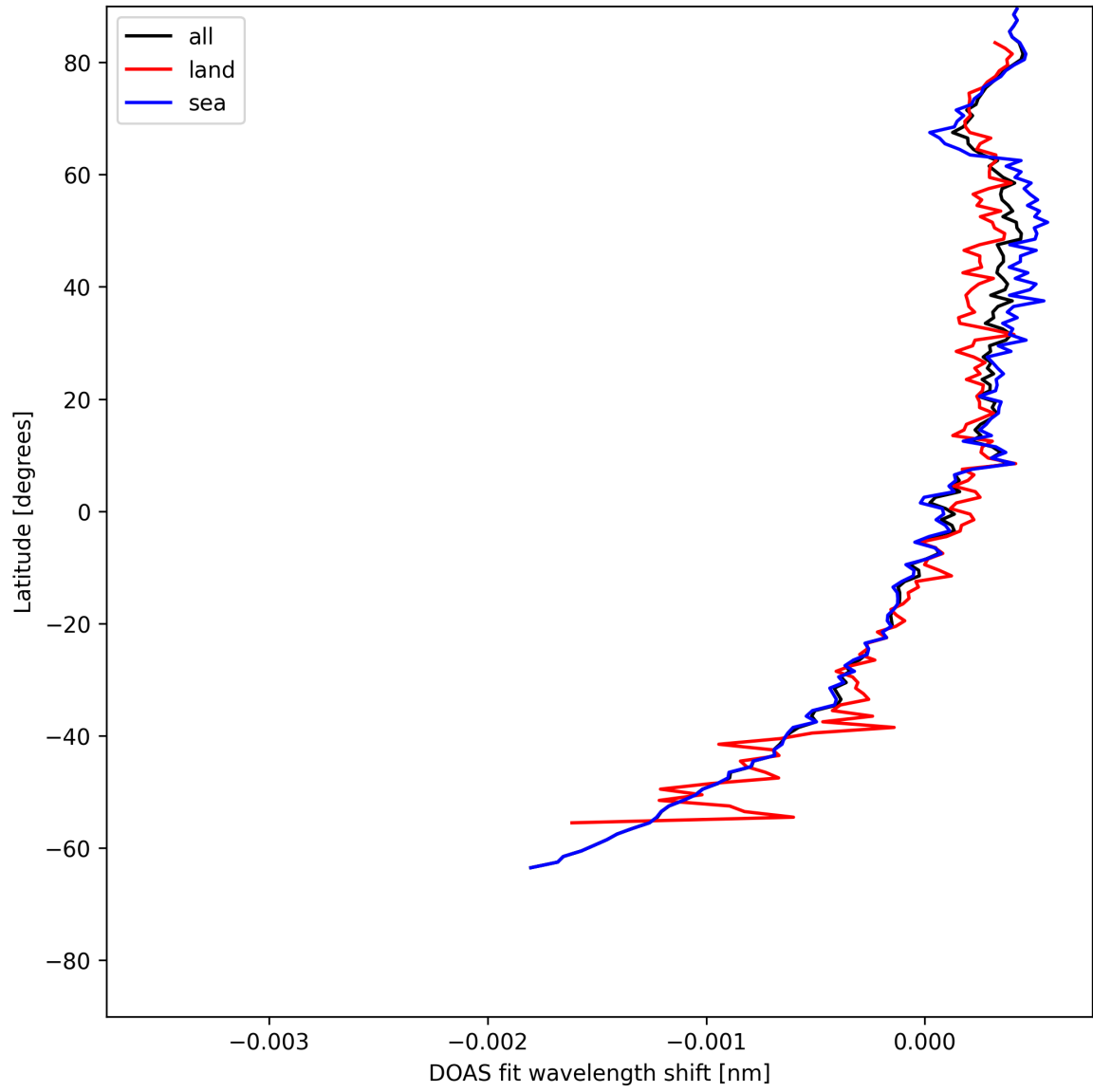
Figure 28: Zonal average of "DOAS fit wavelength shift" for 2025-05-23 to 2025-05-24.
