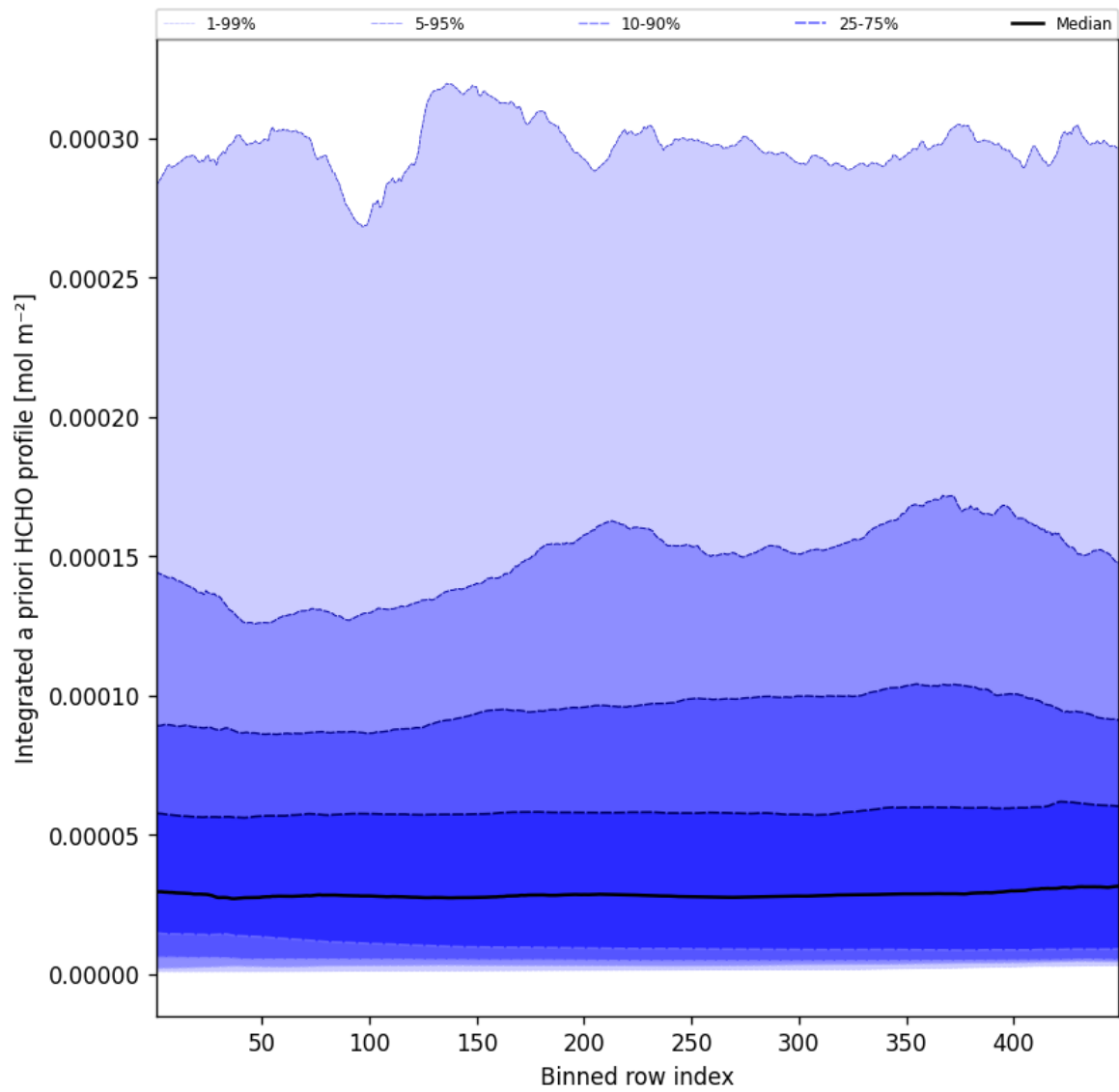
Figure 55: Along track statistics of “Integrated a priori HCHO profile” for 2025-05-23 to 2025-05-24
