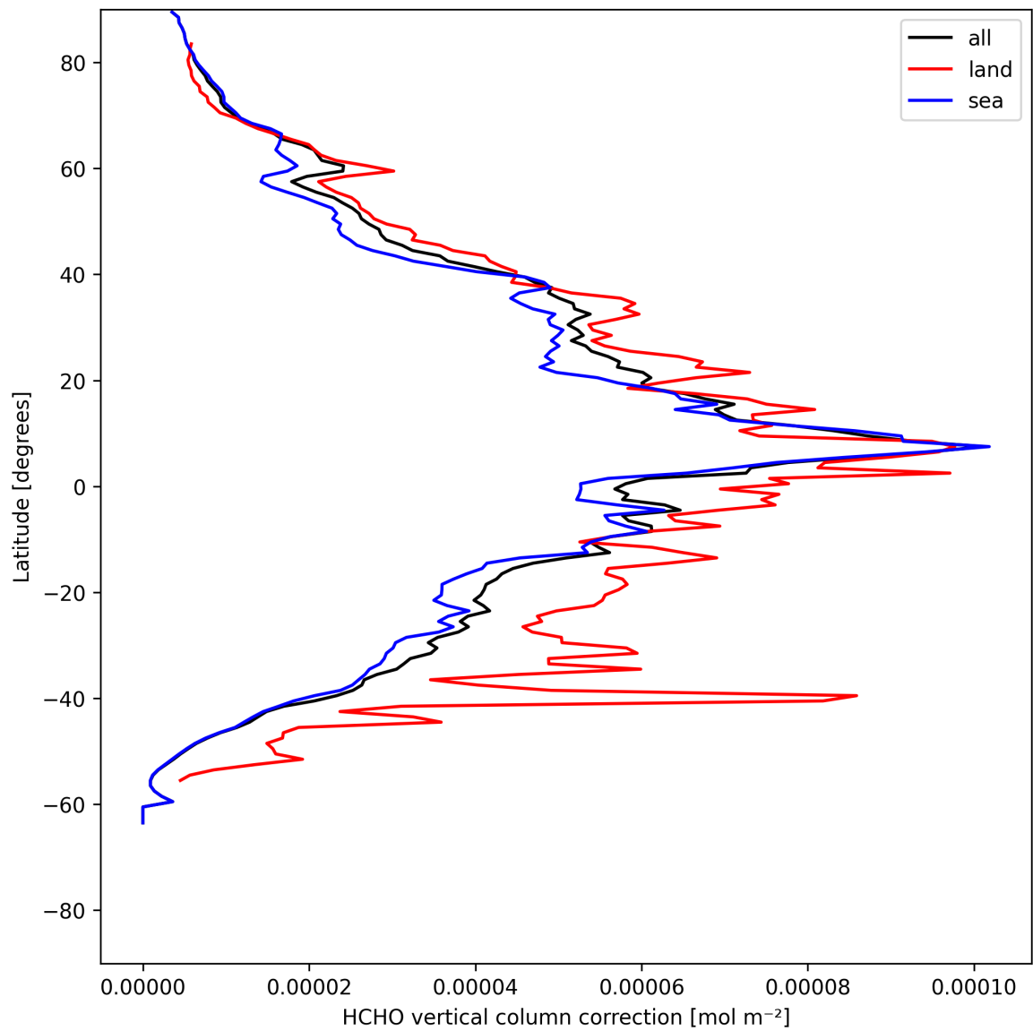
Figure 21: Zonal average of “HCHO vertical column correction” for 2025-05-23 to 2025-05-24.
