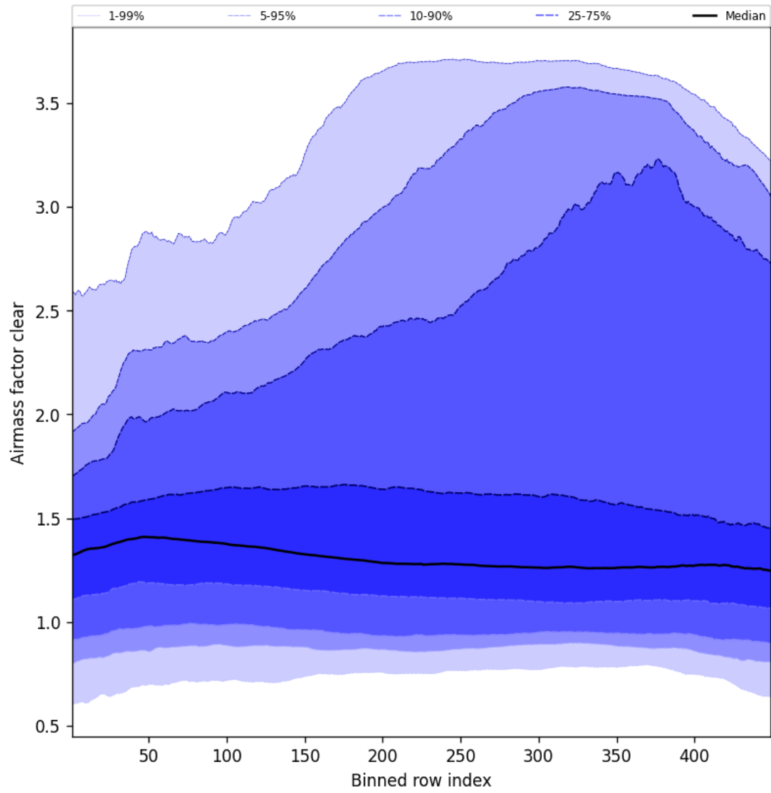
Figure 54: Along track statistics of “Airmass factor clear” for 2025-05-23 to 2025-05-24
