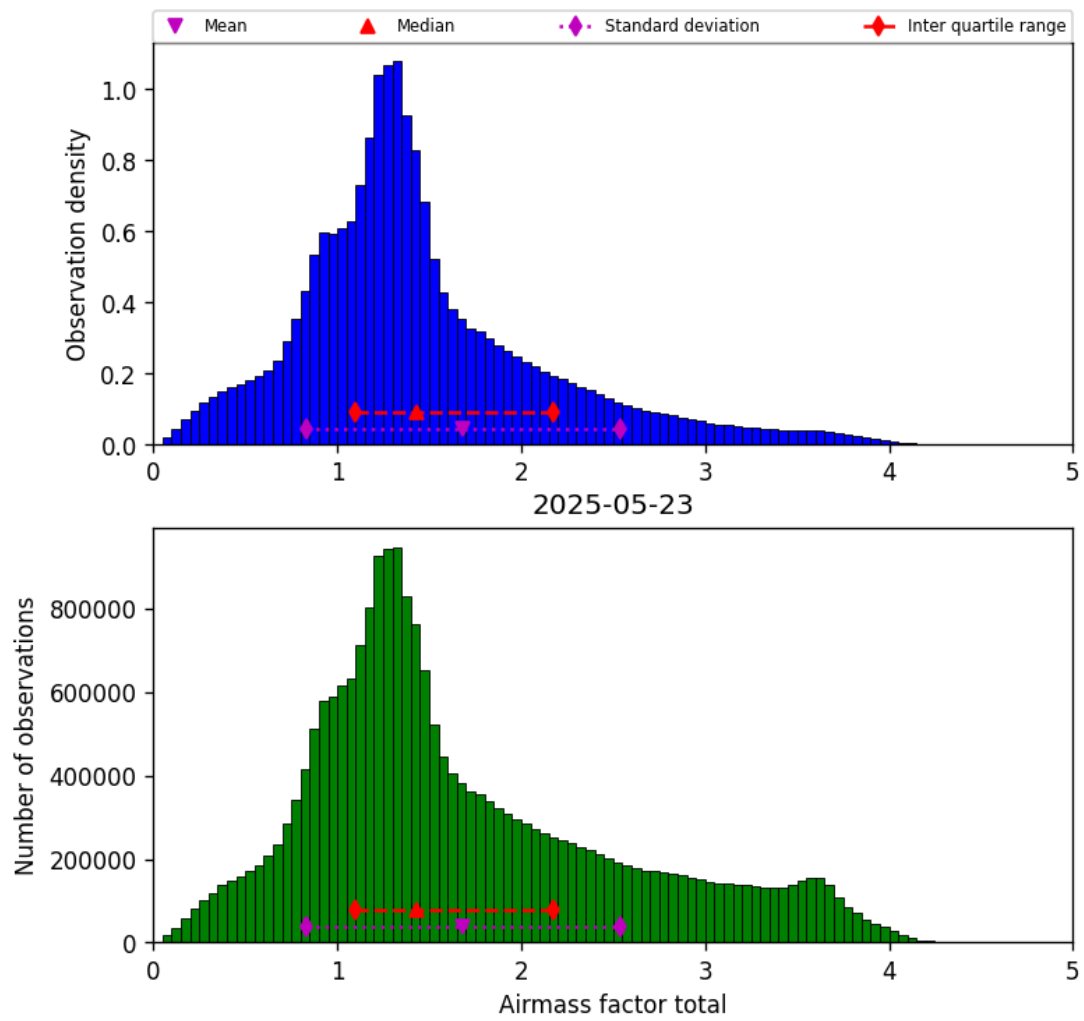
Figure 38: Histogram of “Airmass factor total” for 2025-05-23 to 2025-05-24
