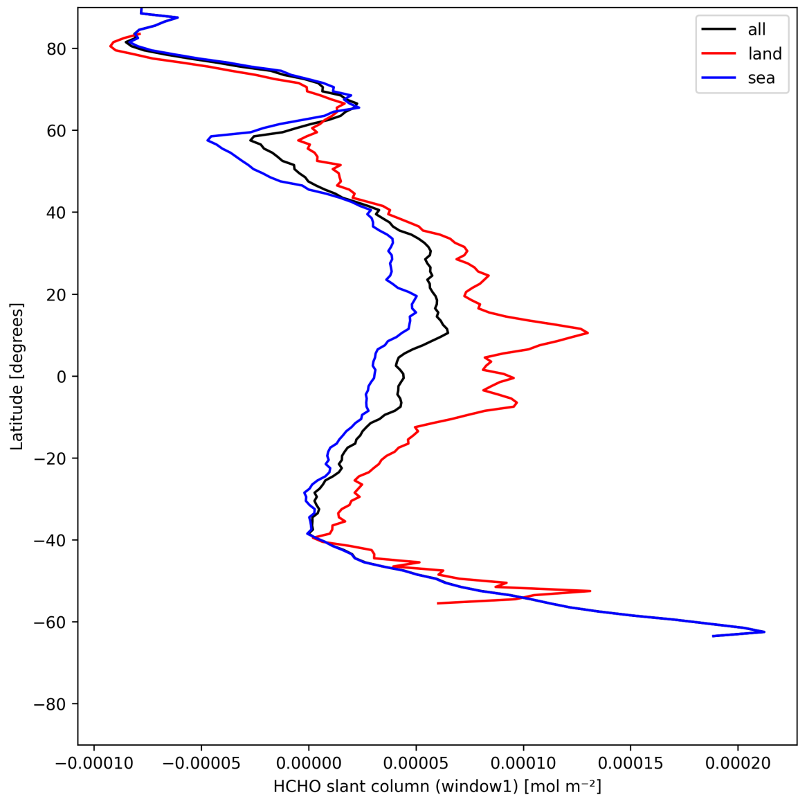
Figure 22: Zonal average of “HCHO slant column (window1)” for 2025-05-23 to 2025-05-24.
