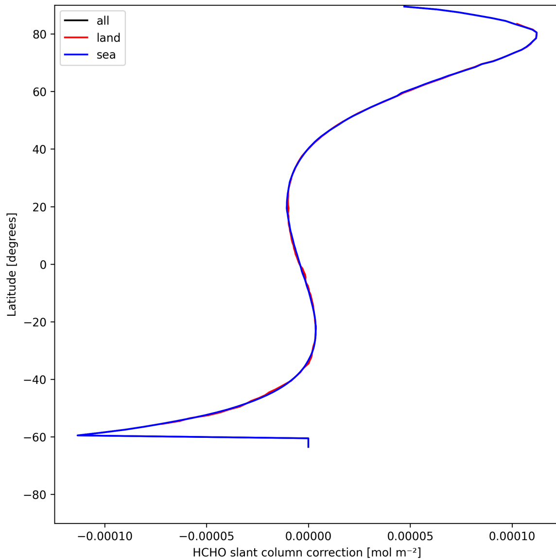
Figure 31: Zonal average of “HCHO slant column correction” for 2025-05-23 to 2025-05-24.
