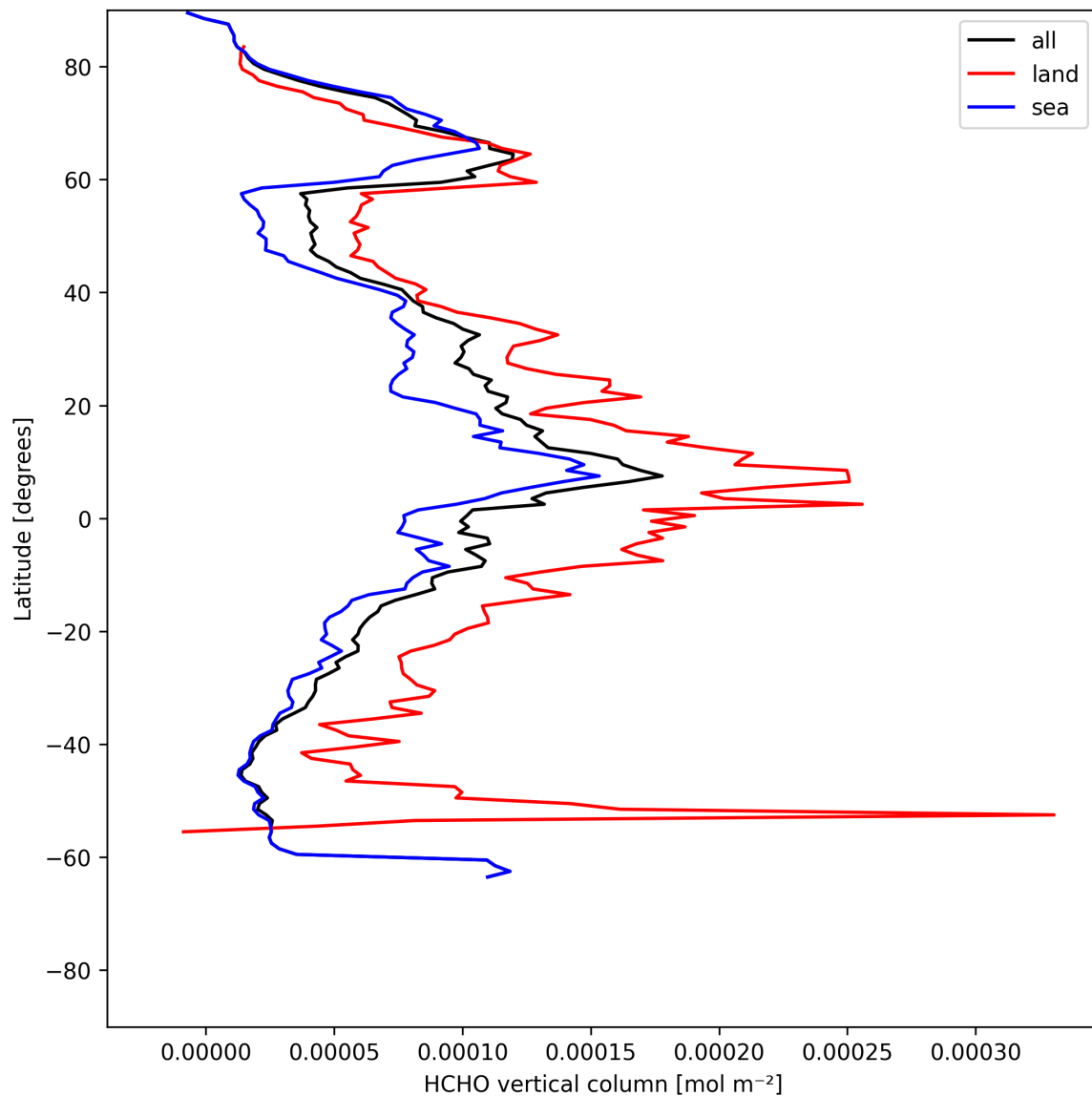
Figure 19: Zonal average of “HCHO vertical column” for 2025-05-23 to 2025-05-24.
