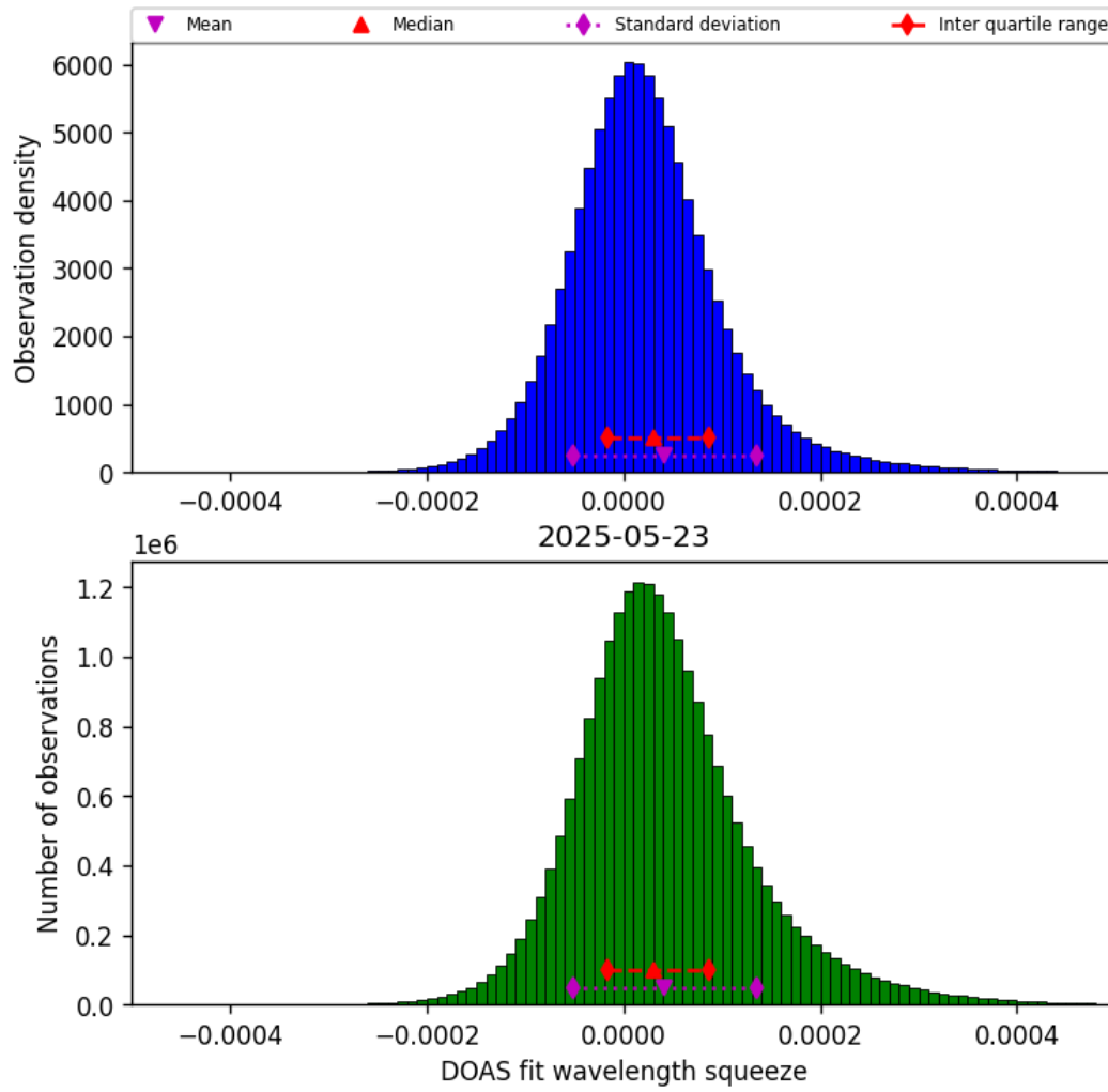
Figure 43: Histogram of “DOAS fit wavelength squeeze” for 2025-05-23 to 2025-05-24
