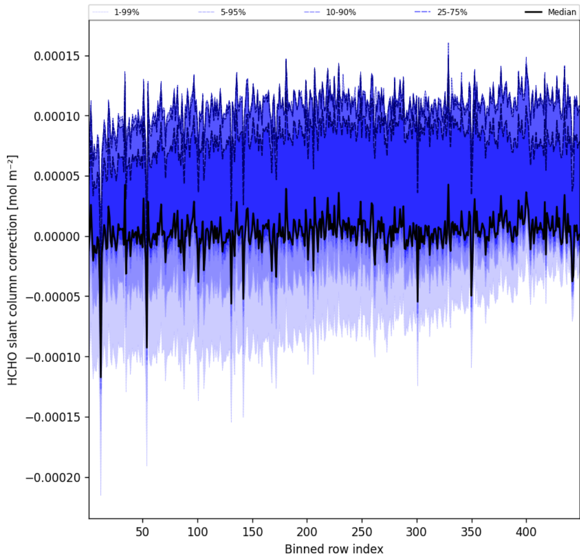
Figure 59: Along track statistics of “HCHO slant column correction” for 2025-05-23 to 2025-05-24
