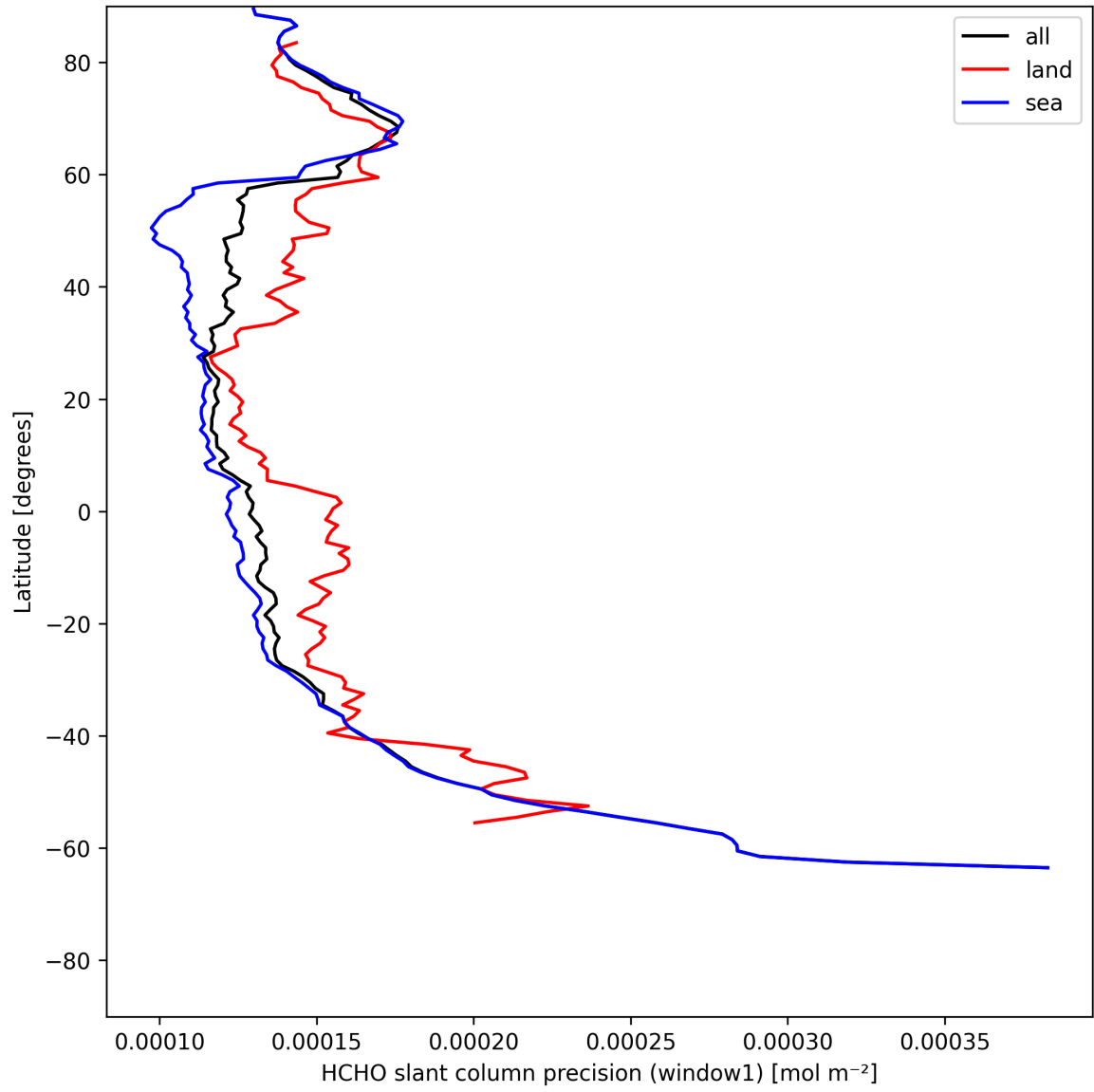
Figure 23: Zonal average of “HCHO slant column precision (window1)” for 2025-05-23 to 2025-05-24.
