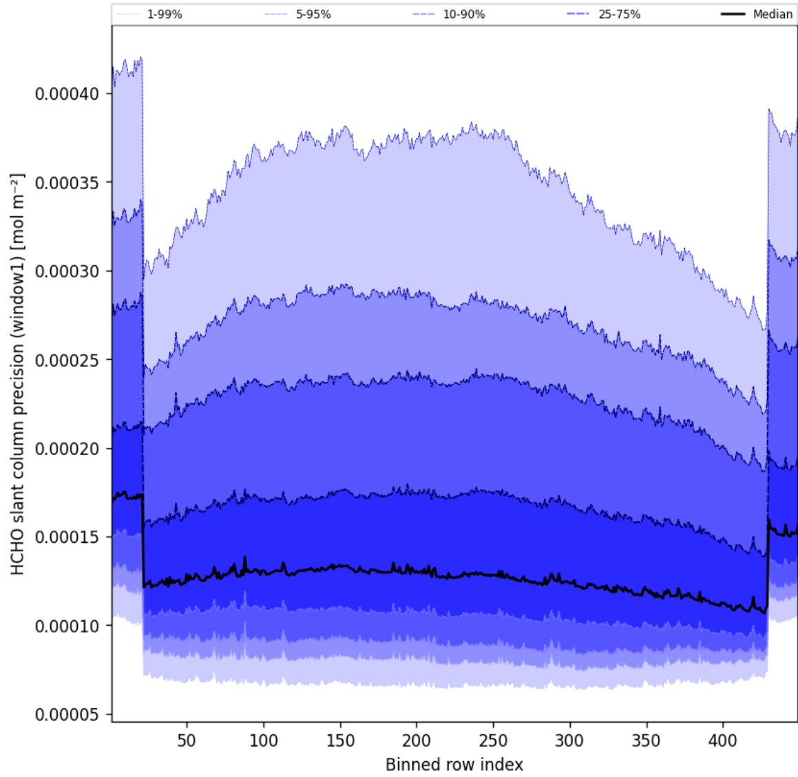
Figure 51: Along track statistics of “HCHO slant column precision (window1)” for 2025-05-23 to 2025-05-24
