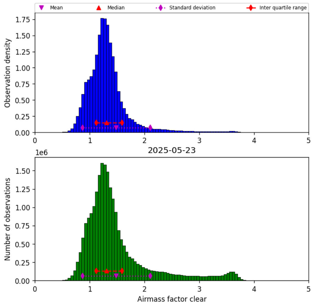
Figure 40: Histogram of “Airmass factor clear” for 2025-05-23 to 2025-05-24
