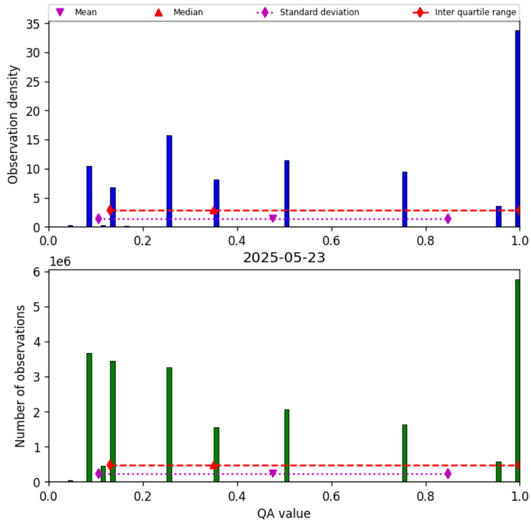
Figure 32: Histogram of “QA value” for 2025-05-23 to 2025-05-24
