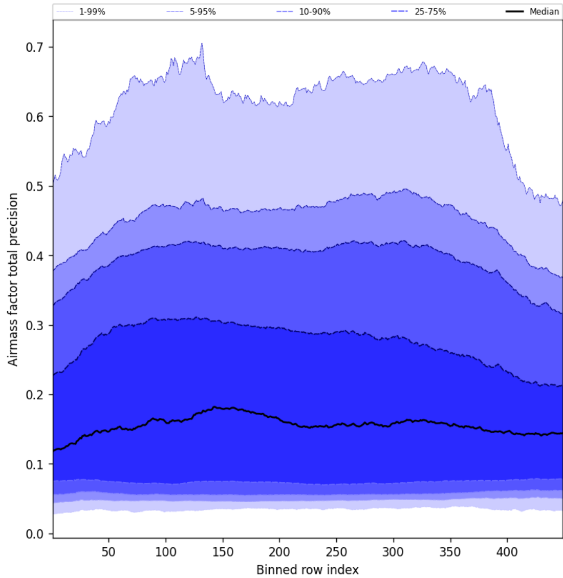
Figure 53: Along track statistics of “Airmass factor total precision” for 2025-05-23 to 2025-05-24
