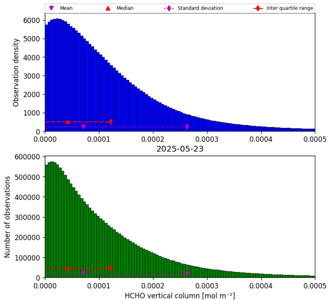
Figure 33: Histogram of “HCHO vertical column” for 2025-05-23 to 2025-05-24
