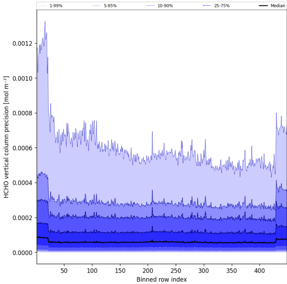
Figure 48: Along track statistics of “HCHO vertical column precision” for 2025-05-23 to 2025-05-24
