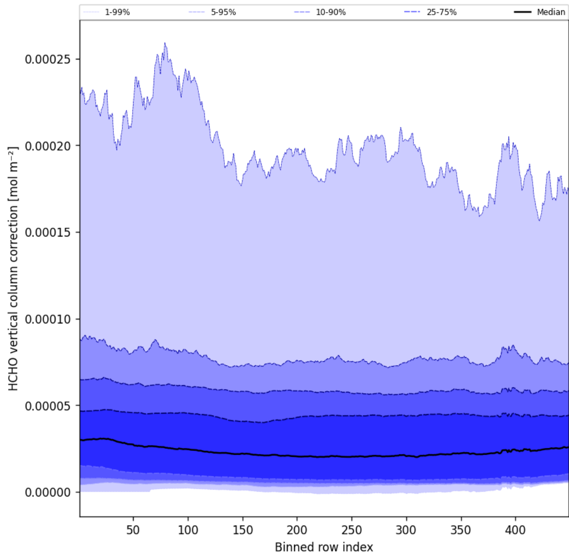
Figure 49: Along track statistics of “HCHO vertical column correction” for 2025-05-23 to 2025-05-24
