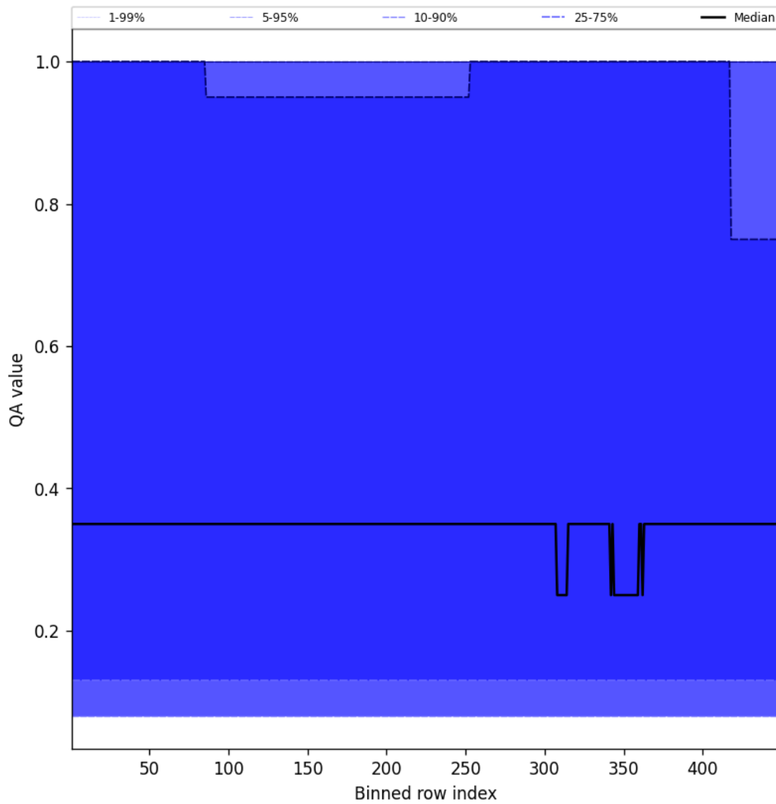
Figure 46: Along track statistics of “QA value” for 2025-05-23 to 2025-05-24
