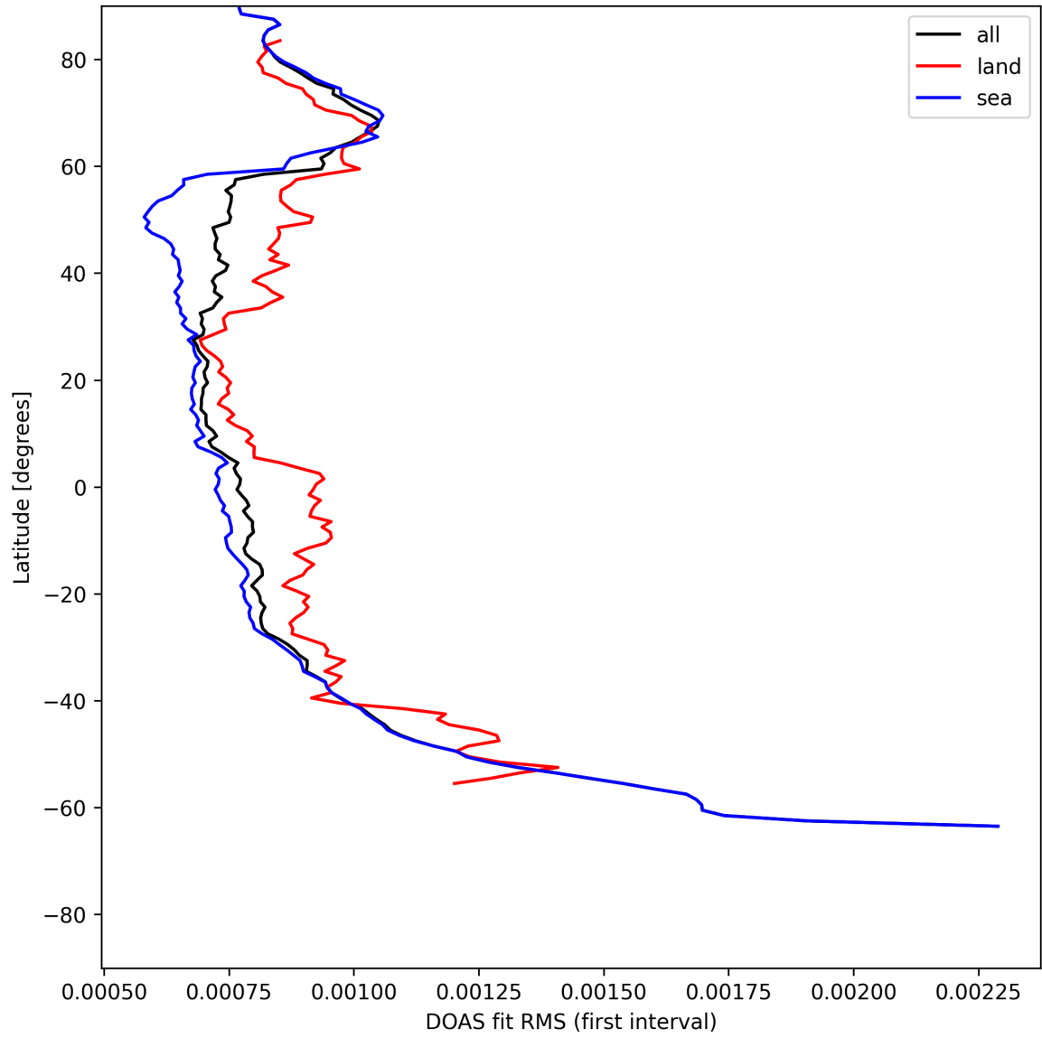
Figure 30: Zonal average of "DOAS fit RMS (first interval)" for 2025-05-23 to 2025-05-24.
