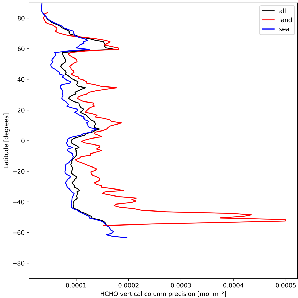
Figure 20: Zonal average of “HCHO vertical column precision” for 2025-05-24 to 2025-05-24.
