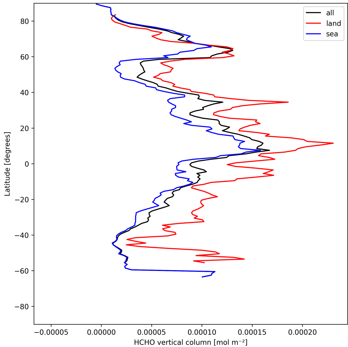
Figure 19: Zonal average of “HCHO vertical column” for 2025-05-24 to 2025-05-24.
