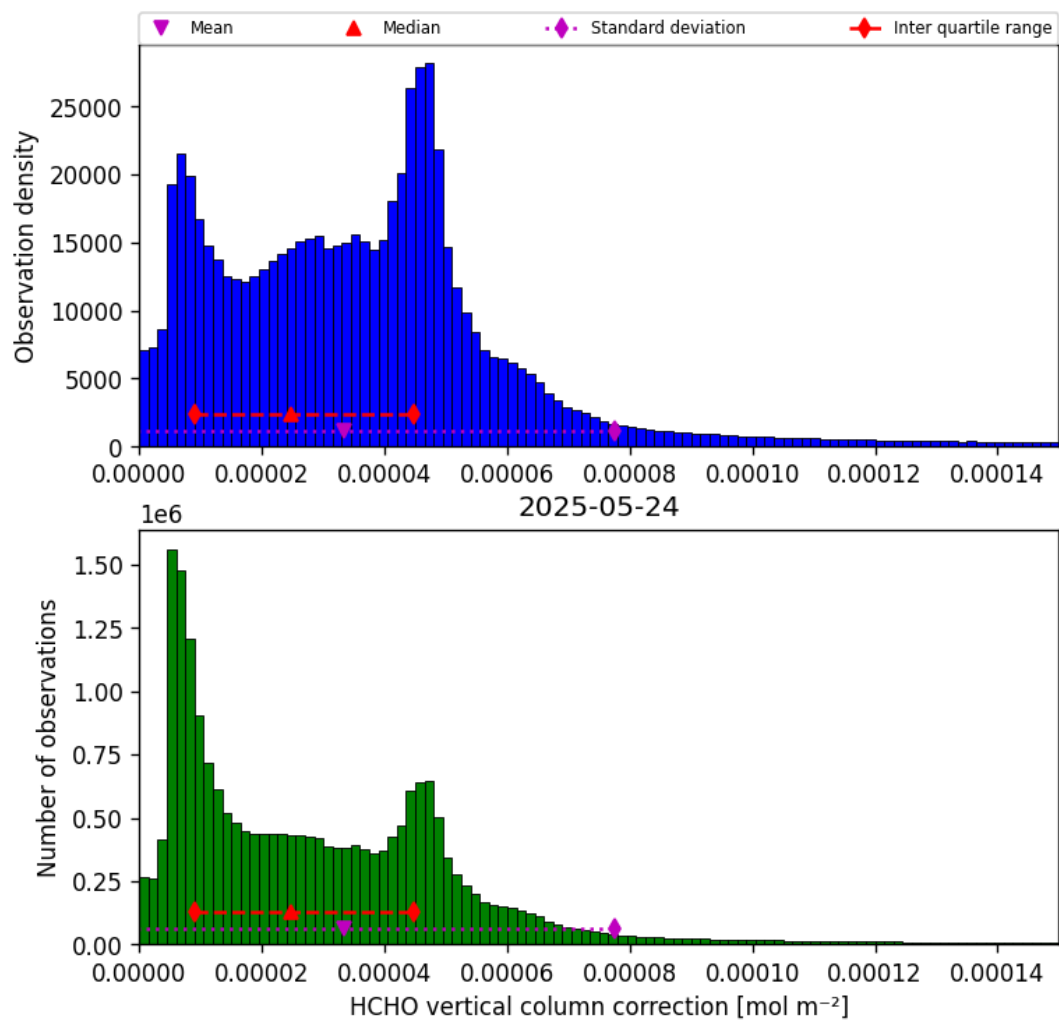
Figure 35: Histogram of “HCHO vertical column correction” for 2025-05-24 to 2025-05-24
