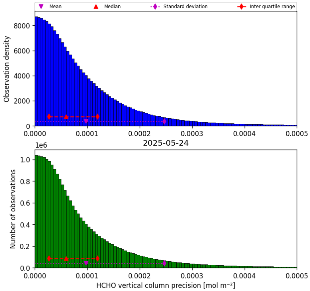
Figure 34: Histogram of “HCHO vertical column precision” for 2025-05-24 to 2025-05-24
