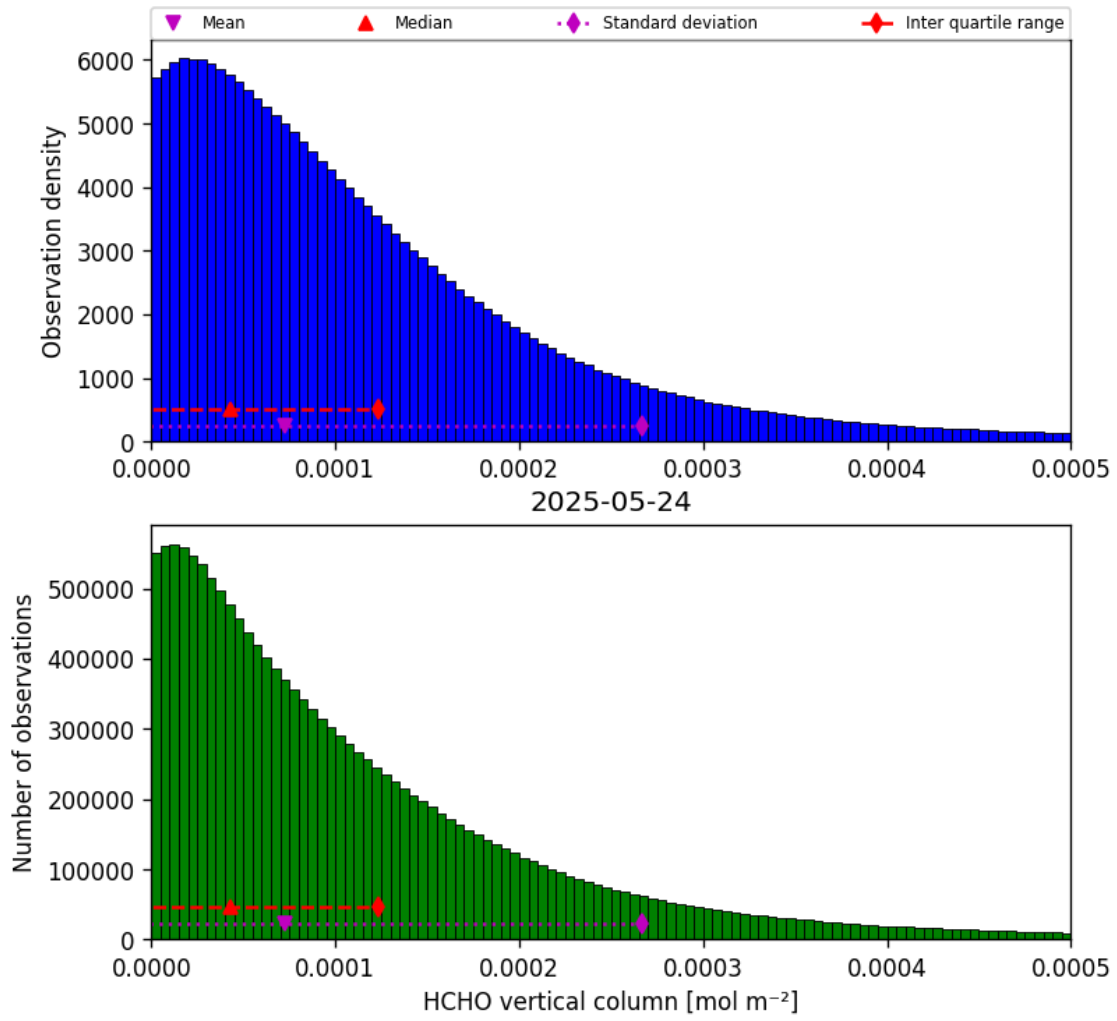
Figure 33: Histogram of “HCHO vertical column” for 2025-05-24 to 2025-05-24
