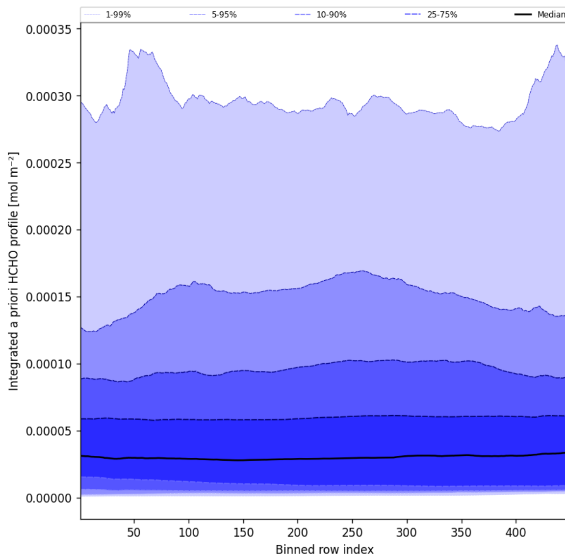
Figure 55: Along track statistics of “Integrated a priori HCHO profile” for 2025-05-24 to 2025-05-24
