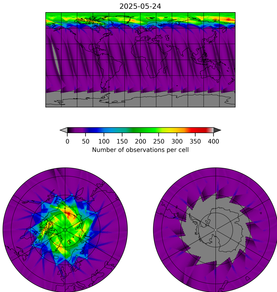
Figure 17: Map of the number of observations for 2025-05-24 to 2025-05-24
