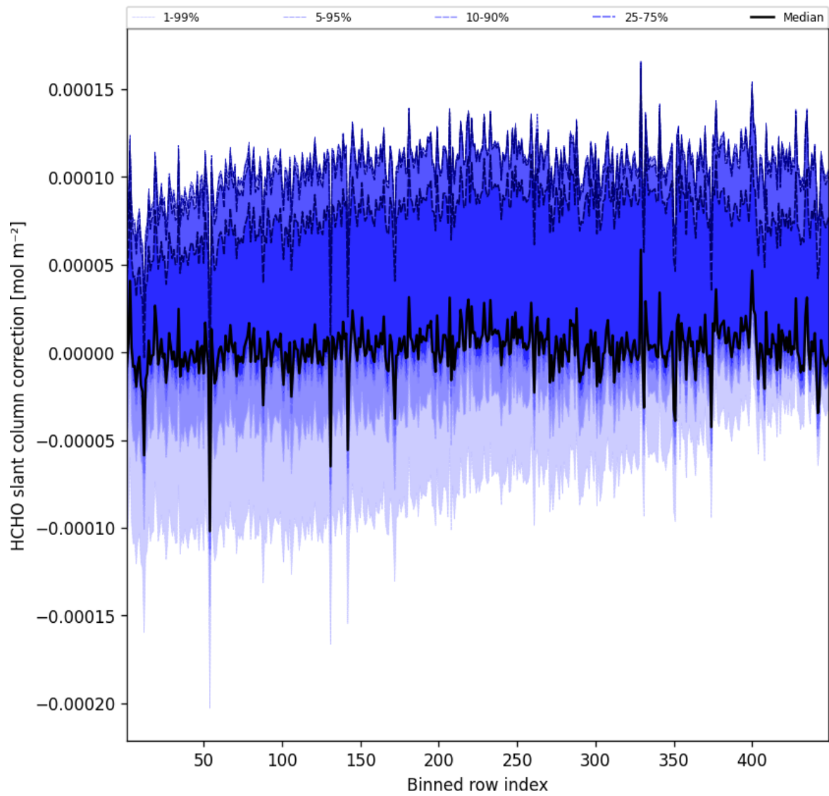
Figure 59: Along track statistics of “HCHO slant column correction” for 2025-05-24 to 2025-05-24
