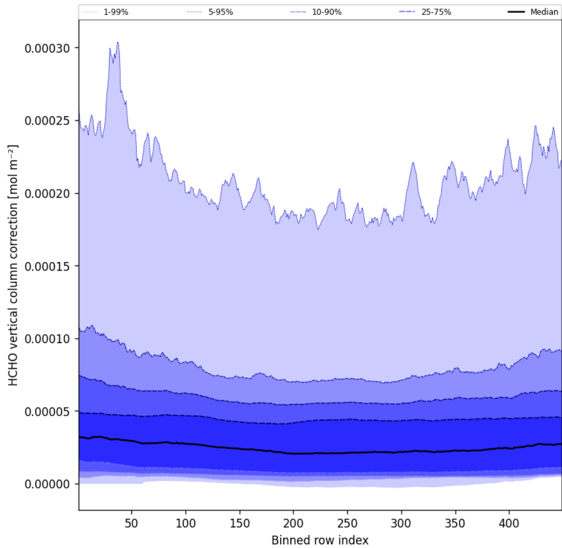
Figure 49: Along track statistics of “HCHO vertical column correction” for 2025-05-24 to 2025-05-24
