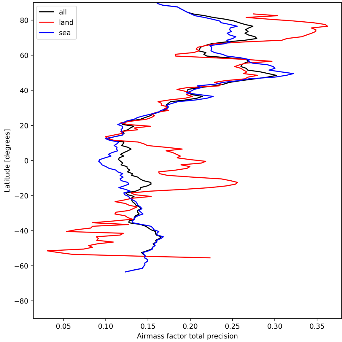
Figure 25: Zonal average of “Airmass factor total precision” for 2025-05-24 to 2025-05-24.
