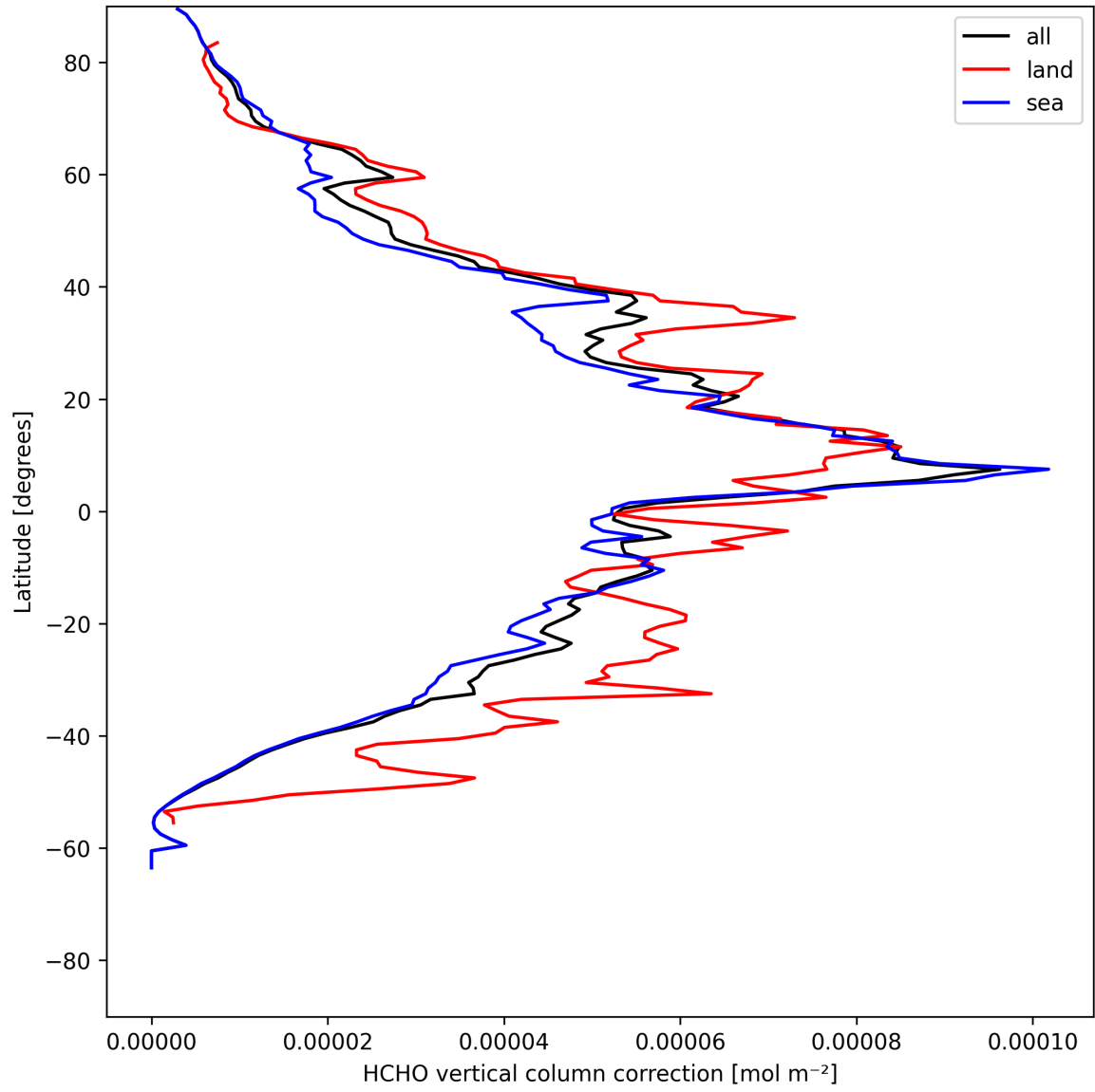
Figure 21: Zonal average of “HCHO vertical column correction” for 2025-05-24 to 2025-05-24.
