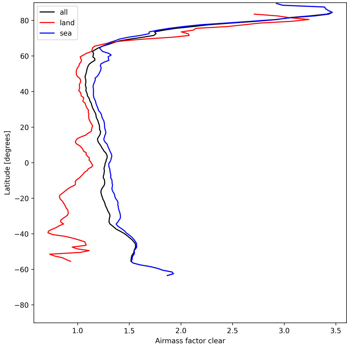
Figure 26: Zonal average of “Airmass factor clear” for 2025-05-24 to 2025-05-24.
