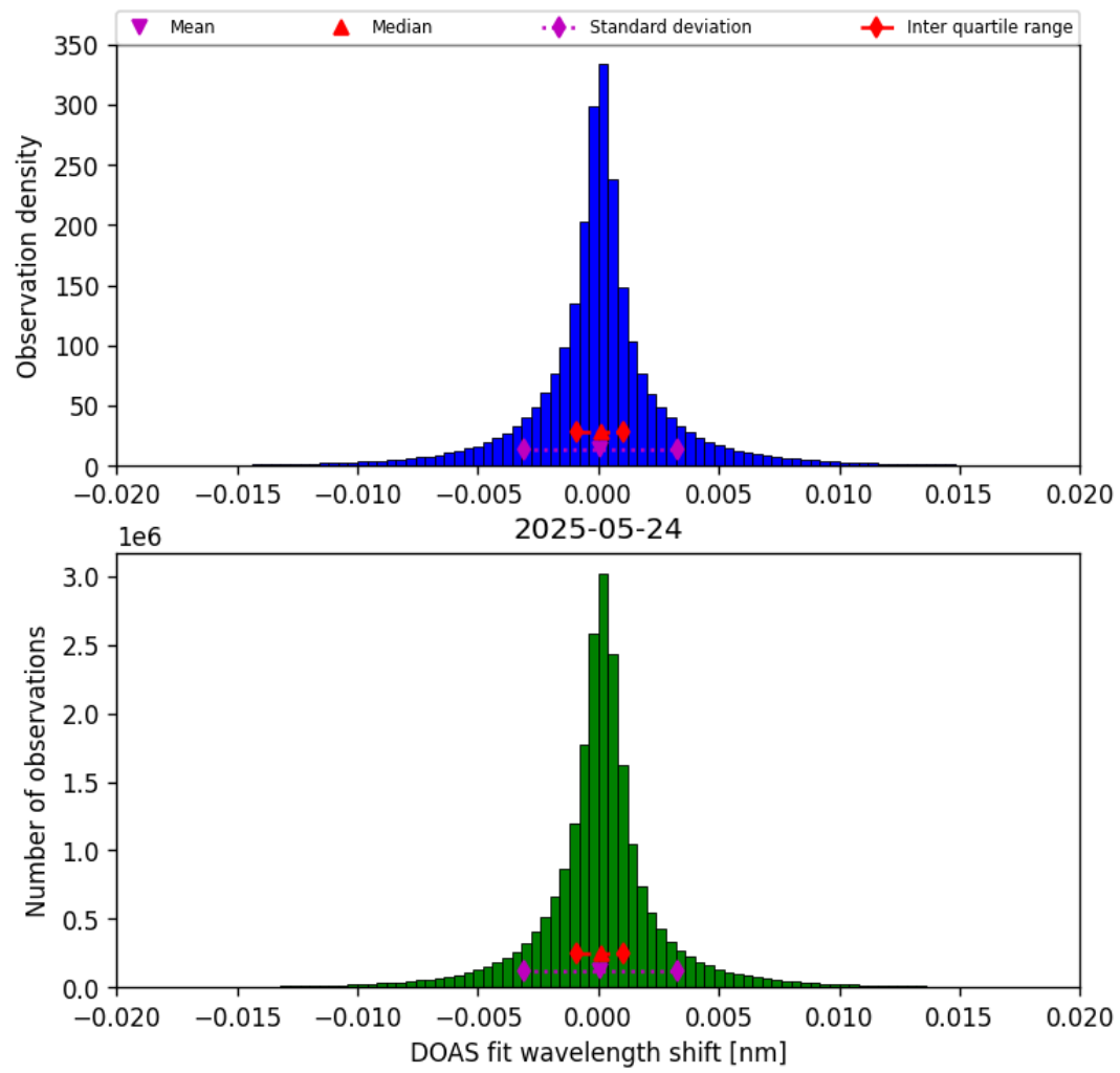
Figure 42: Histogram of “DOAS fit wavelength shift” for 2025-05-24 to 2025-05-24
