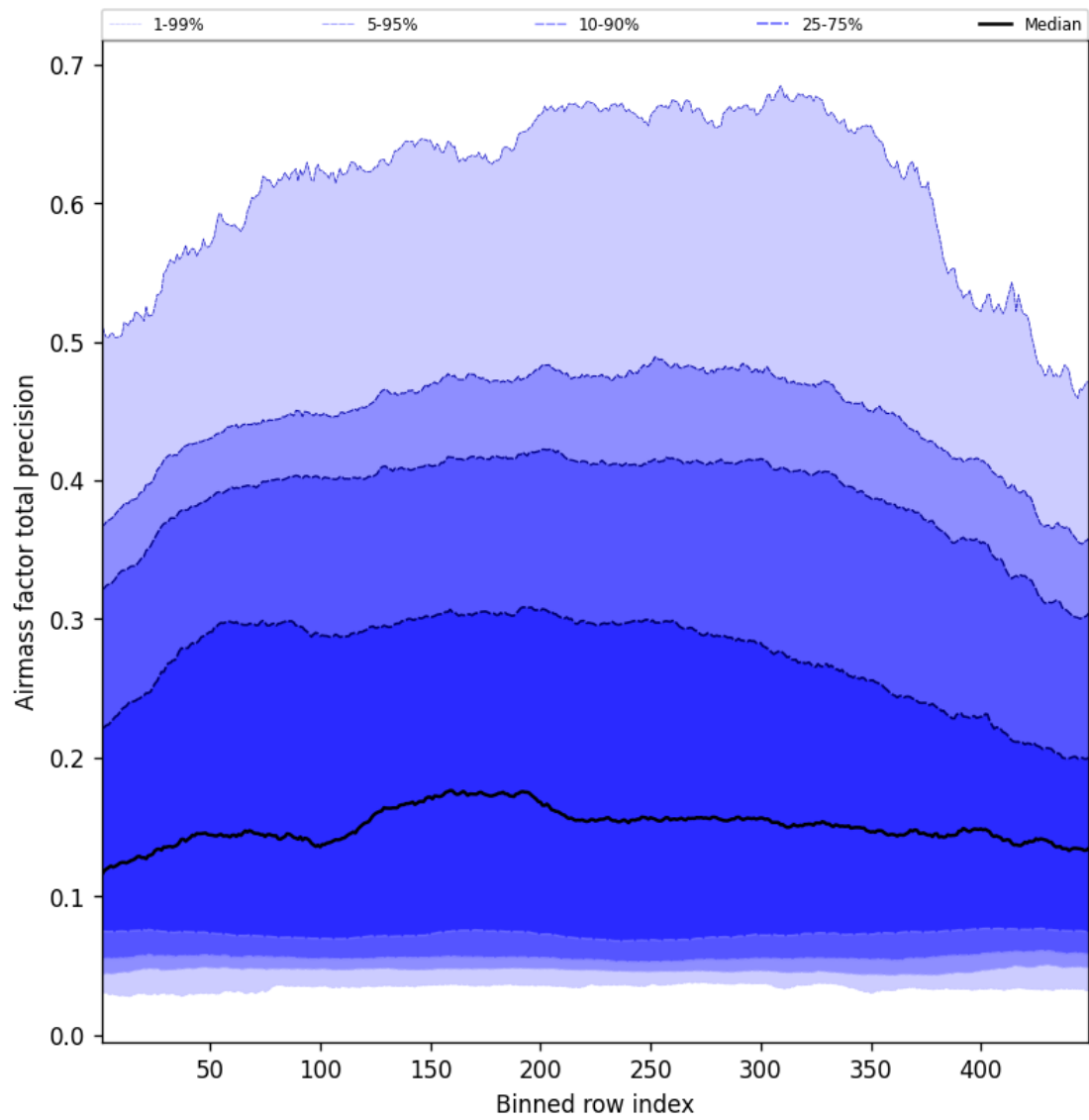
Figure 53: Along track statistics of “Airmass factor total precision” for 2025-05-24 to 2025-05-24
