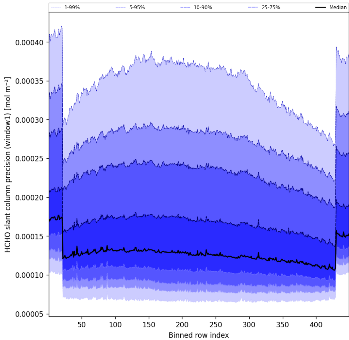
Figure 51: Along track statistics of “HCHO slant column precision (window1)” for 2025-05-24 to 2025-05-24
