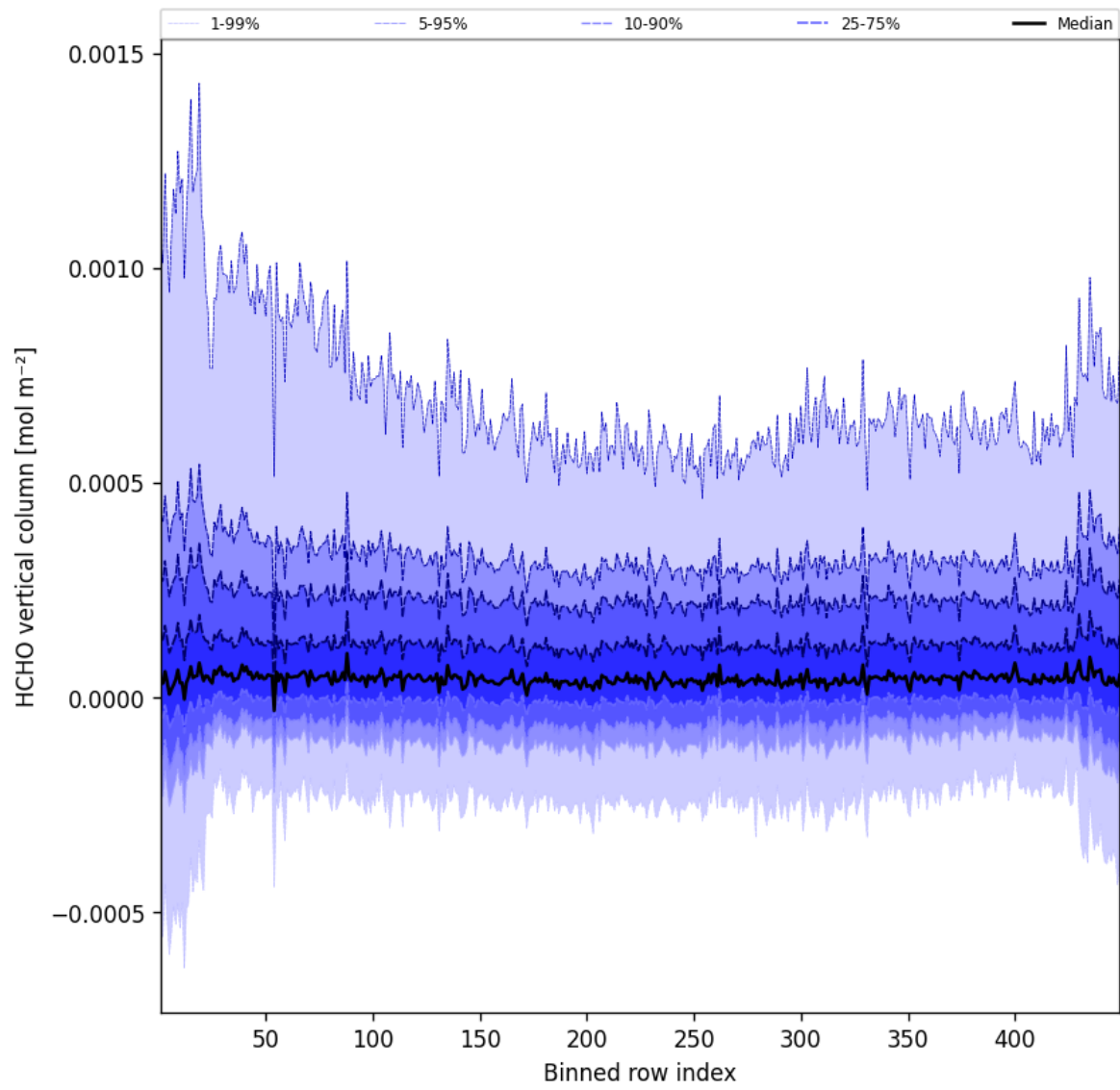
Figure 47: Along track statistics of “HCHO vertical column” for 2025-05-24 to 2025-05-24
