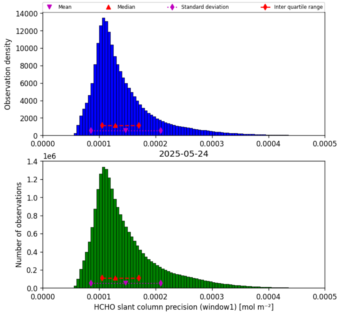
Figure 37: Histogram of “HCHO slant column precision (window1)” for 2025-05-24 to 2025-05-24
