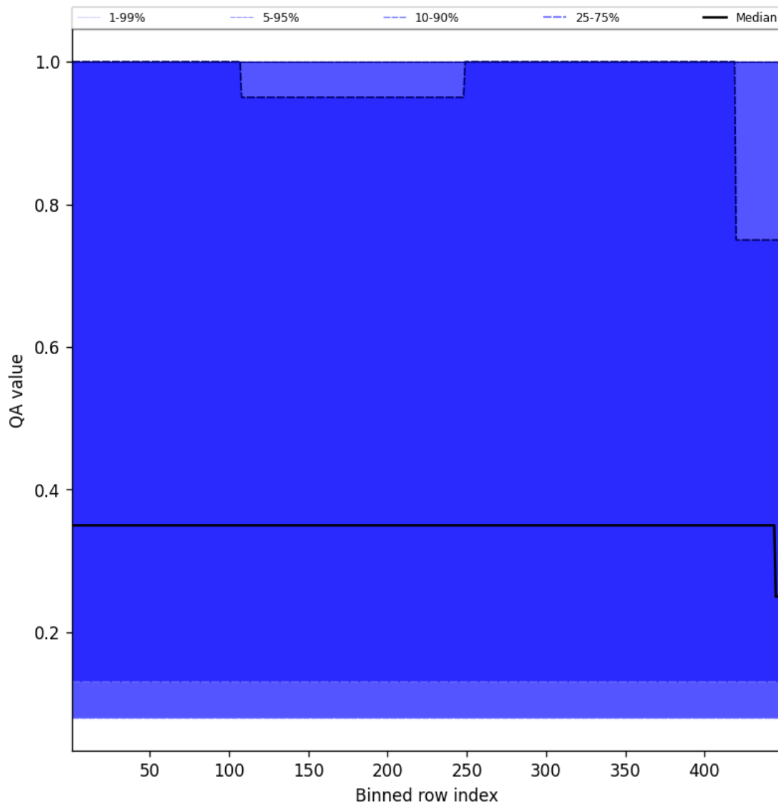
Figure 46: Along track statistics of "QA value" for 2025-05-24 to 2025-05-24
