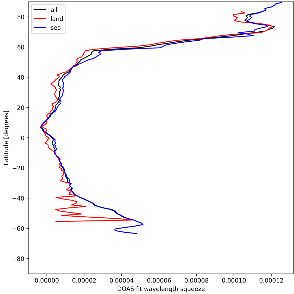
Figure 29: Zonal average of “DOAS fit wavelength squeeze” for 2025-05-24 to 2025-05-24.
