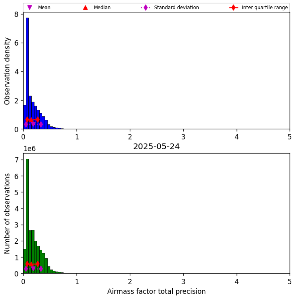
Figure 39: Histogram of “Airmass factor total precision” for 2025-05-24 to 2025-05-24
