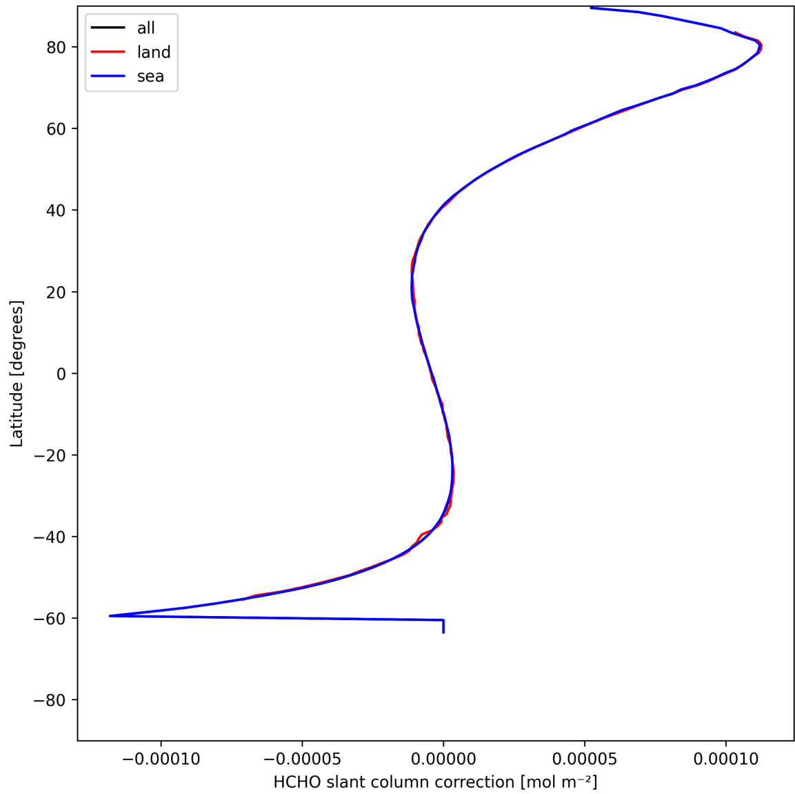
Figure 31: Zonal average of “HCHO slant column correction” for 2025-05-24 to 2025-05-24.
