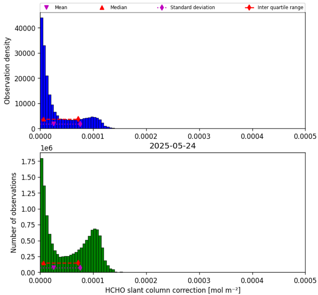
Figure 45: Histogram of “HCHO slant column correction” for 2025-05-24 to 2025-05-24
