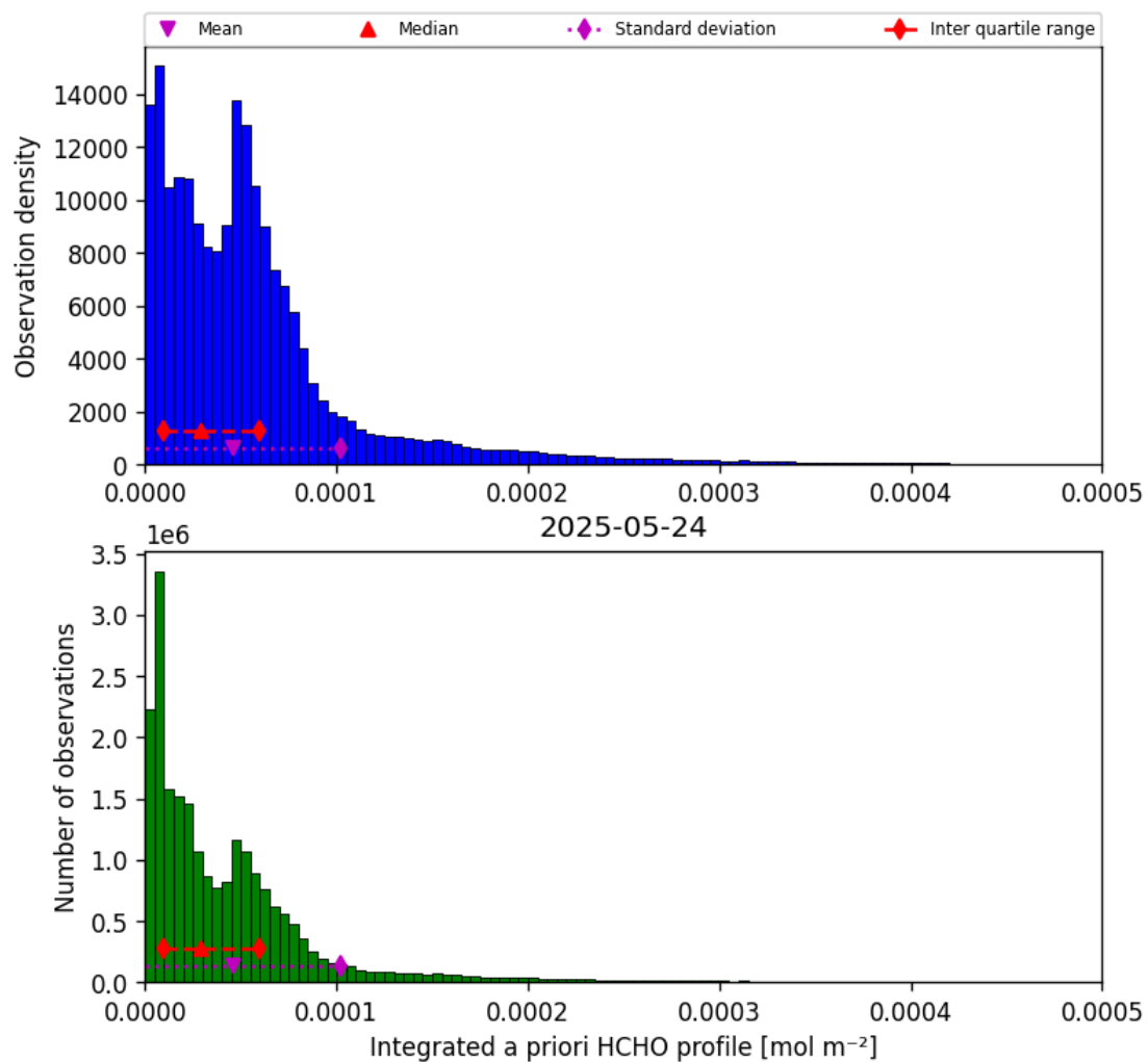
Figure 41: Histogram of “Integrated a priori HCHO profile” for 2025-05-24 to 2025-05-24
