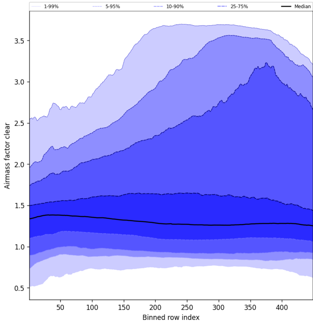
Figure 54: Along track statistics of “Air mass factor clear” for 2025-05-24 to 2025-05-24
