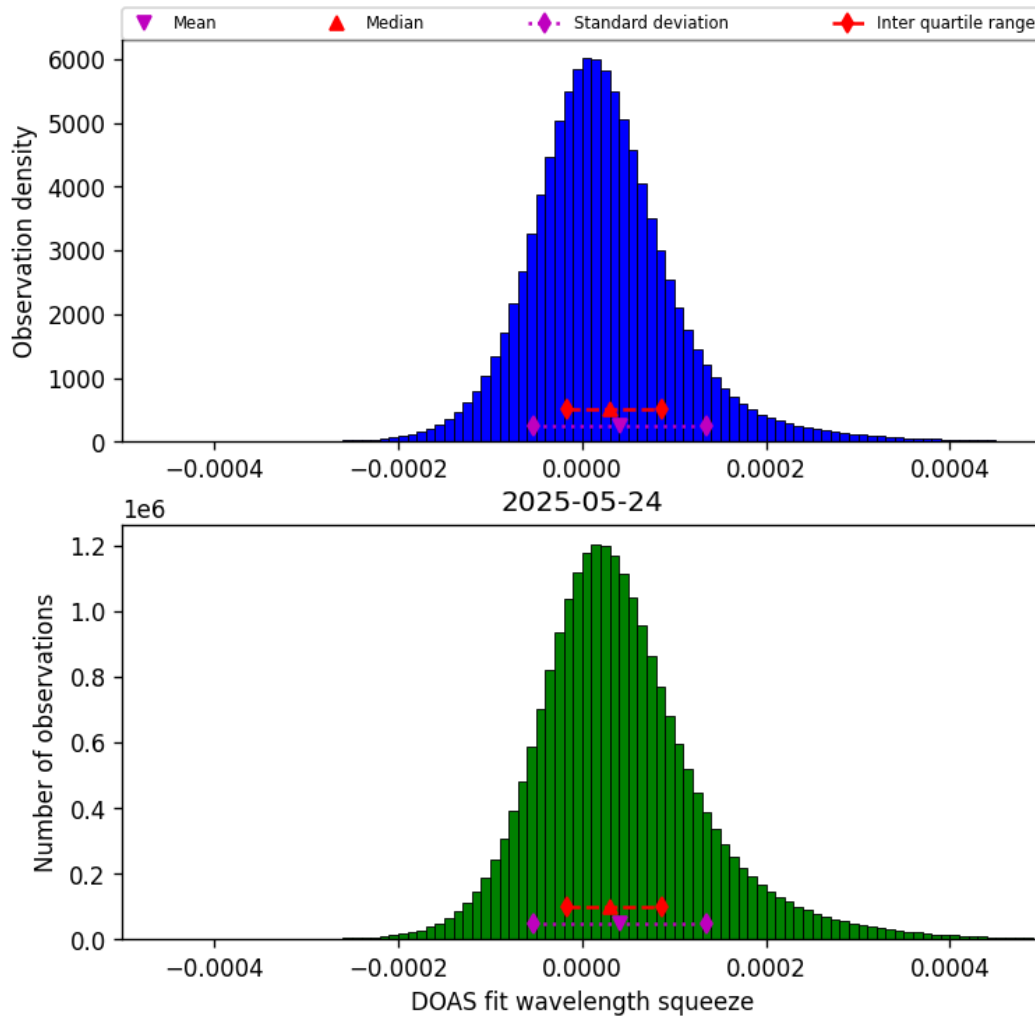
Figure 43: Histogram of “DOAS fit wavelength squeeze” for 2025-05-24 to 2025-05-24
