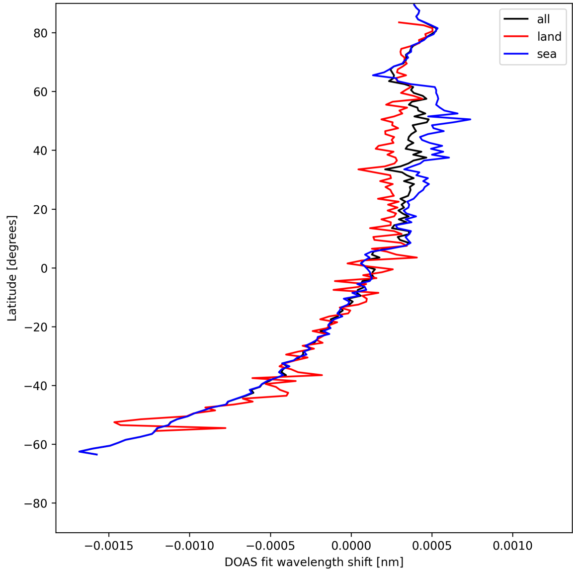
Figure 28: Zonal average of “DOAS fit wavelength shift” for 2025-05-24 to 2025-05-24.
