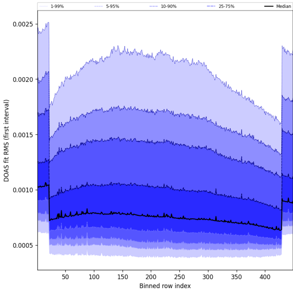
Figure 58: Along track statistics of “DOAS fit RMS (first interval)” for 2025-05-24 to 2025-05-24
