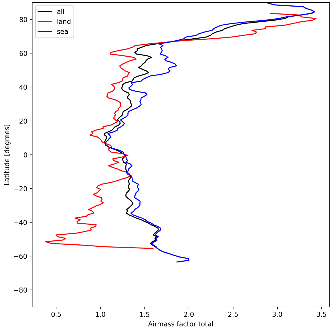
Figure 24: Zonal average of “Airmass factor total” for 2025-05-24 to 2025-05-24.
