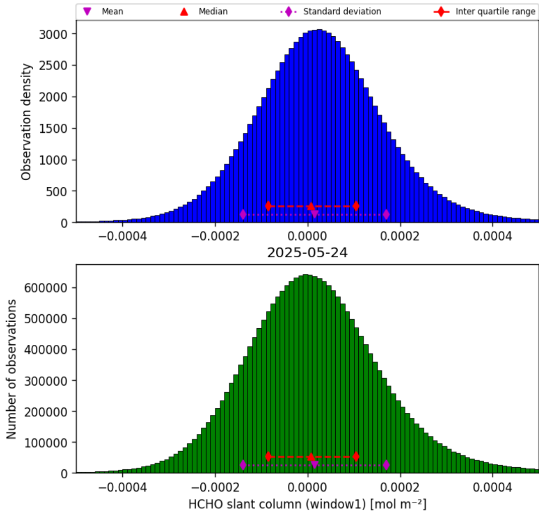
Figure 36: Histogram of “HCHO slant column (window1)” for 2025-05-24 to 2025-05-24
