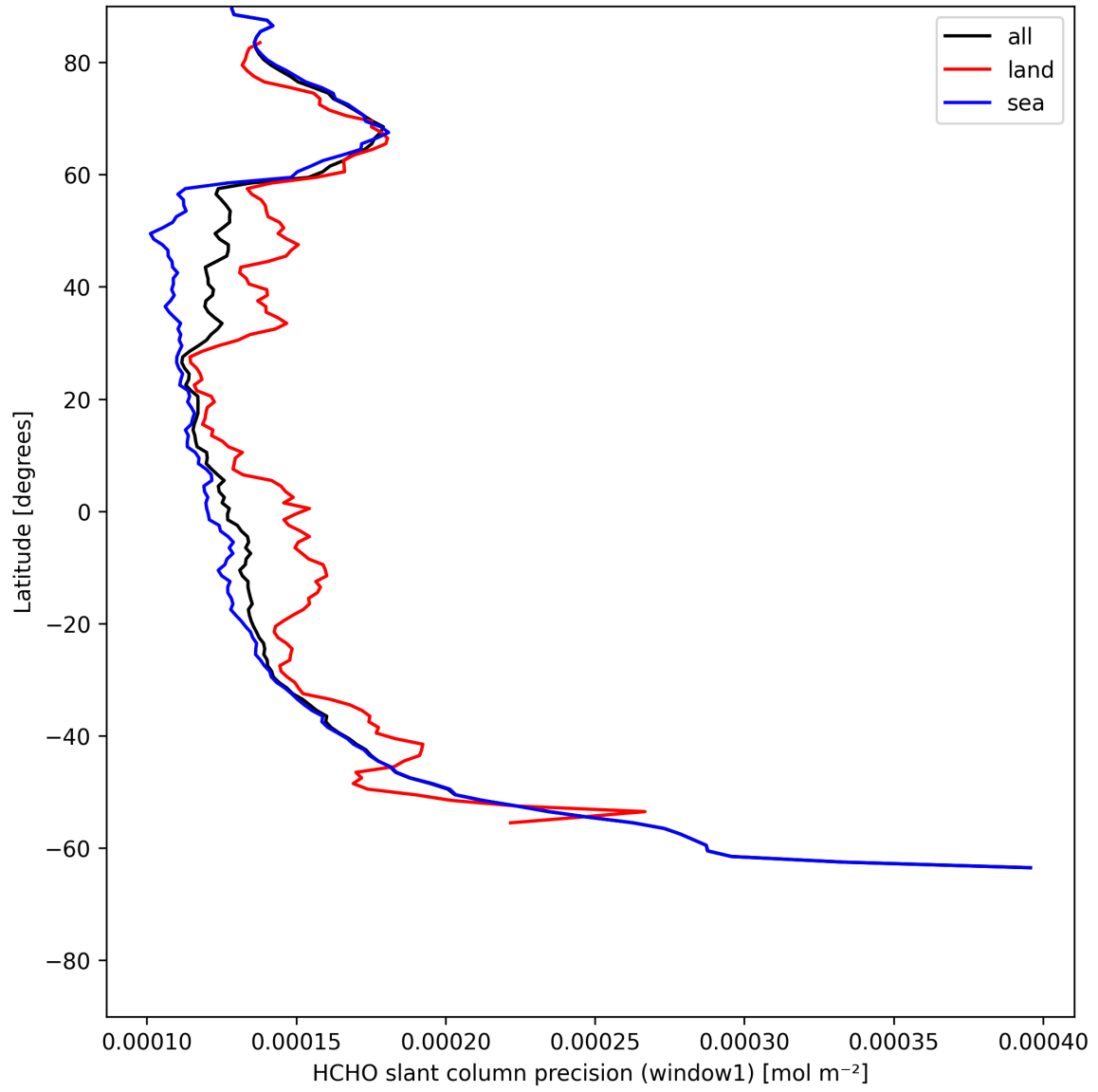
Figure 23: Zonal average of “HCHO slant column precision (window1)” for 2025-05-24 to 2025-05-24.
