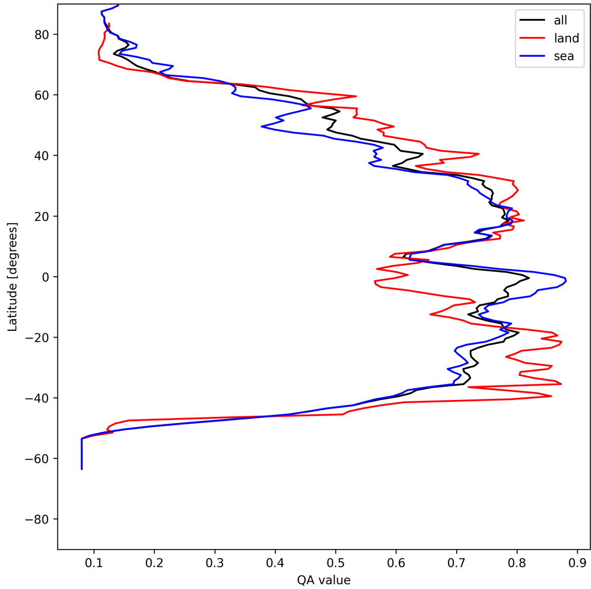
Figure 18: Zonal average of “QA value” for 2025-05-24 to 2025-05-24.
