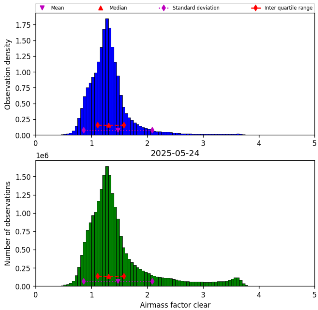
Figure 40: Histogram of “Airmass factor clear” for 2025-05-24 to 2025-05-24
