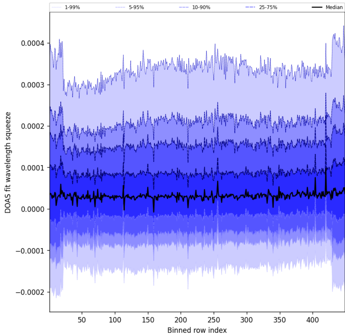
Figure 57: Along track statistics of “DOAS fit wavelength squeeze” for 2025-05-24 to 2025-05-24
