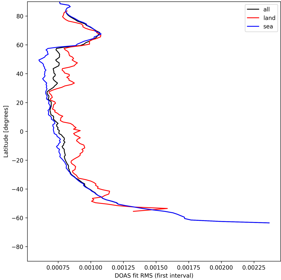
Figure 30: Zonal average of "DOAS fit RMS (first interval)" for 2025-05-24 to 2025-05-24.
