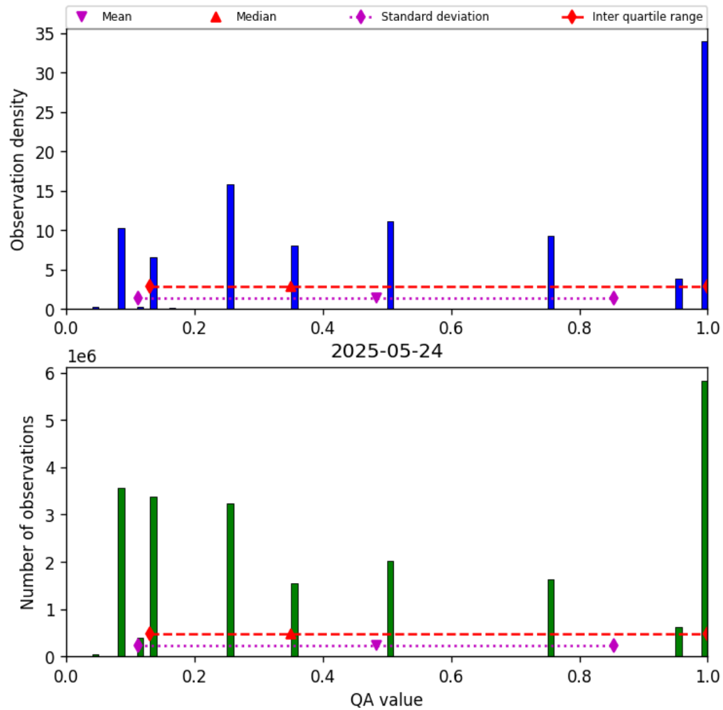
Figure 32: Histogram of “QA value” for 2025-05-24 to 2025-05-24
