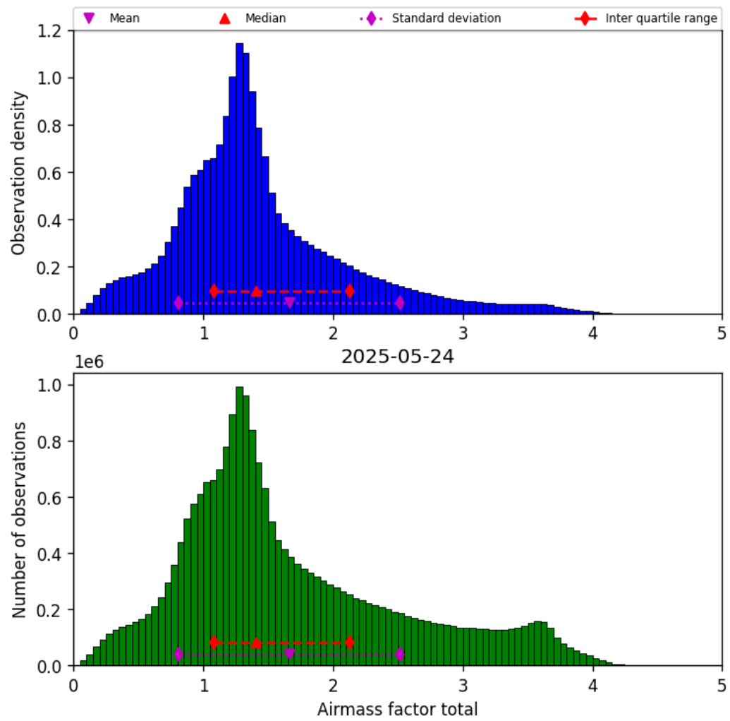
Figure 38: Histogram of “Airmass factor total” for 2025-05-24 to 2025-05-24
