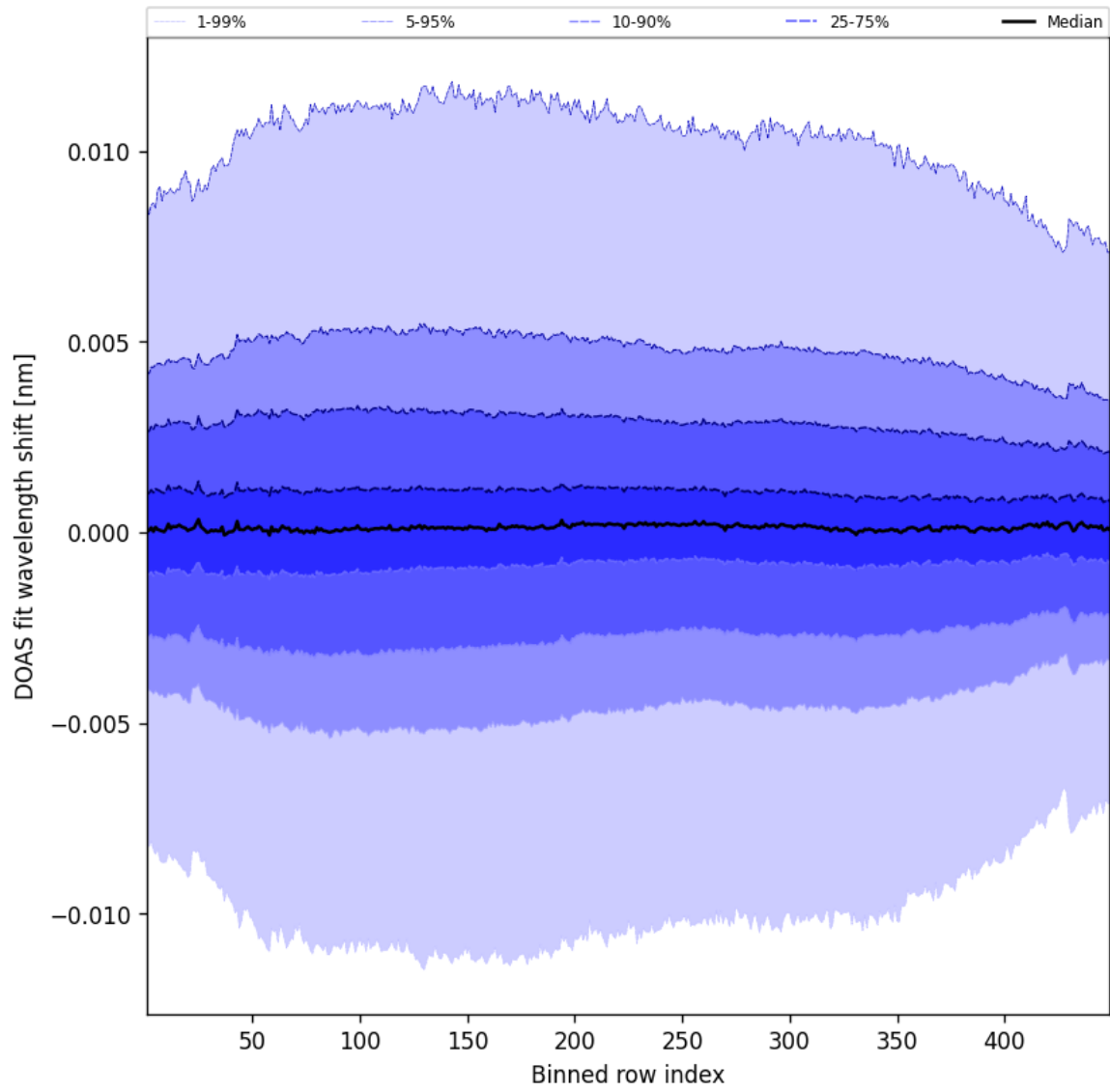
Figure 56: Along track statistics of “DOAS fit wavelength shift” for 2025-05-24 to 2025-05-24
