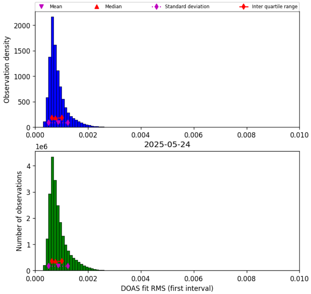
Figure 44: Histogram of “DOAS fit RMS (first interval)” for 2025-05-24 to 2025-05-24
