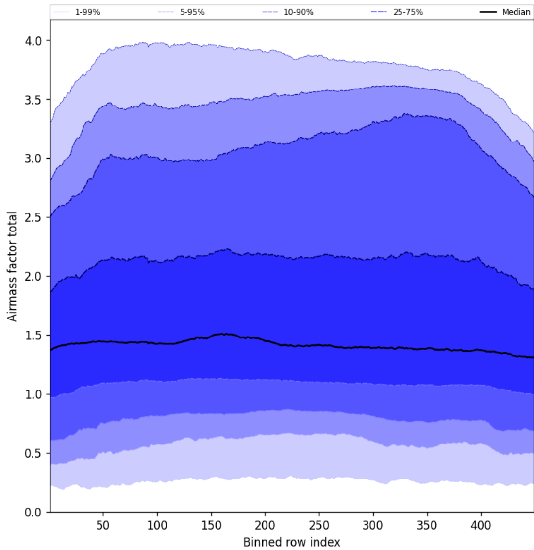
Figure 52: Along track statistics of “Airmass factor total” for 2025-05-24 to 2025-05-24
