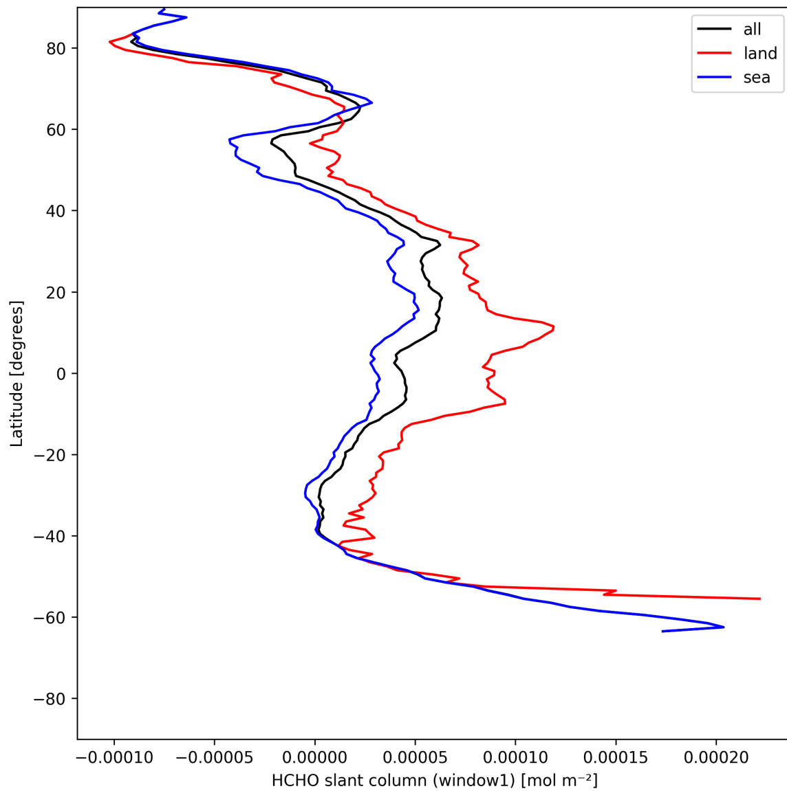
Figure 22: Zonal average of “HCHO slant column (window1)” for 2025-05-24 to 2025-05-24.
