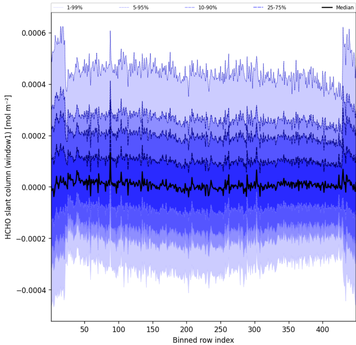
Figure 50: Along track statistics of “HCHO slant column (window1)” for 2025-05-24 to 2025-05-24
