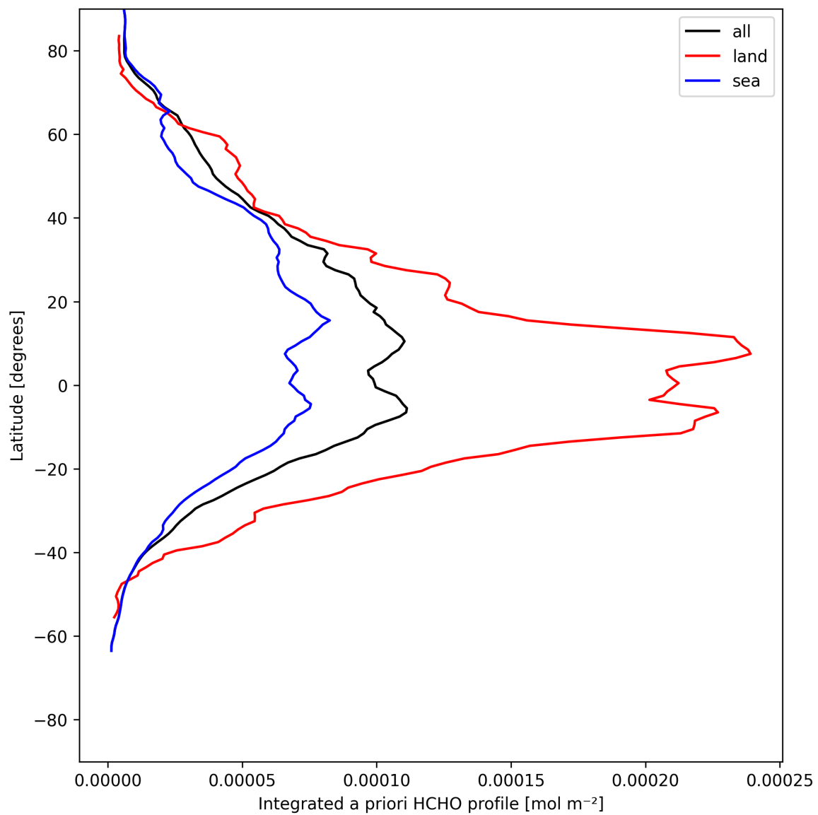
Figure 27: Zonal average of “Integrated a priori HCHO profile” for 2025-05-24 to 2025-05-24.
