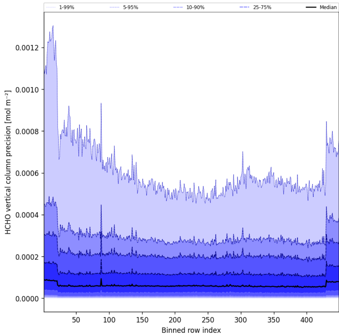
Figure 48: Along track statistics of “HCHO vertical column precision” for 2025-05-24 to 2025-05-24
