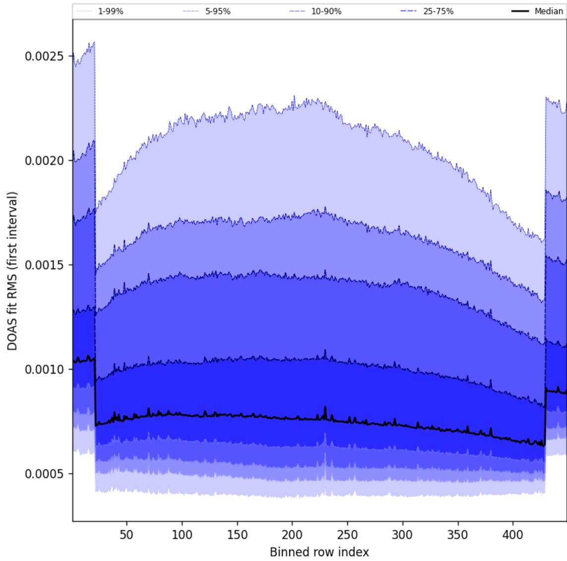
Figure 58: Along track statistics of “DOAS fit RMS (first interval)” for 2025-05-25 to 2025-05-26
