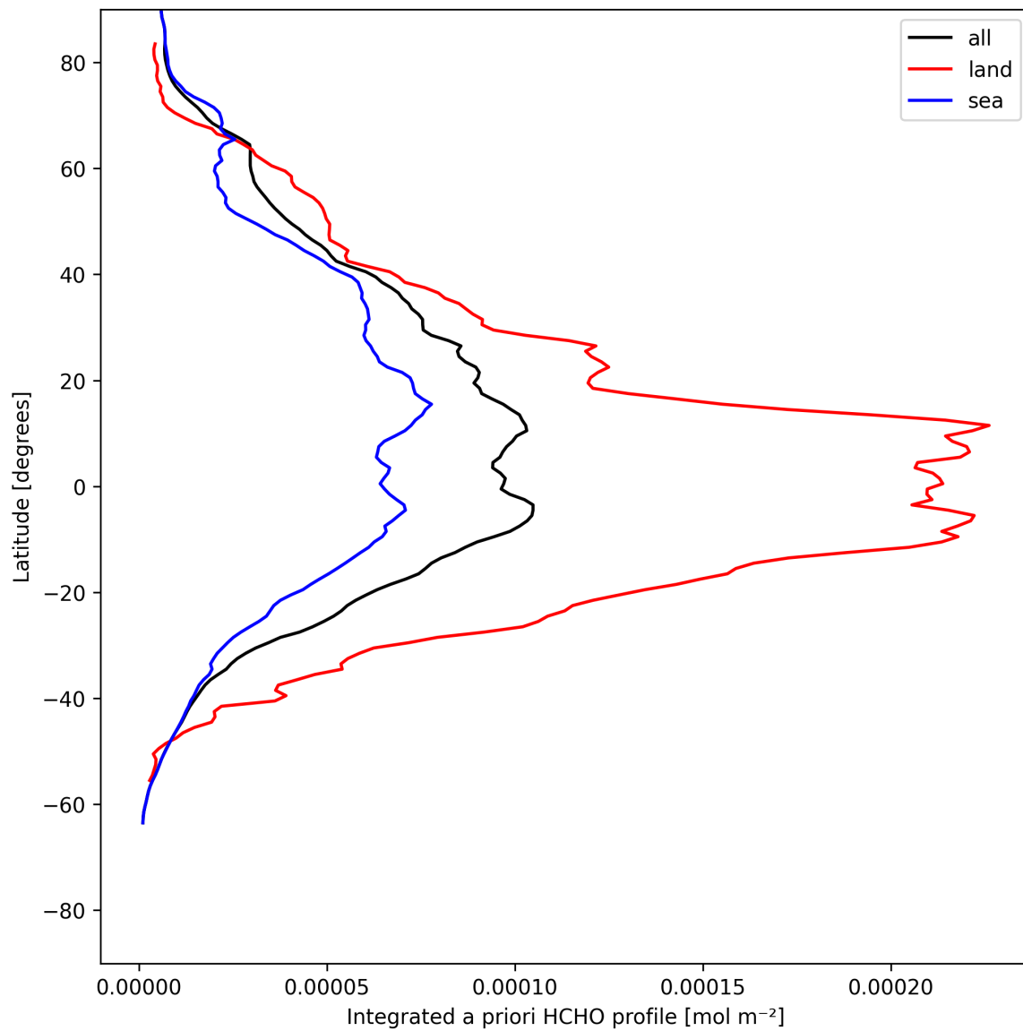
Figure 27: Zonal average of “Integrated a priori HCHO profile” for 2025-05-25 to 2025-05-26.
