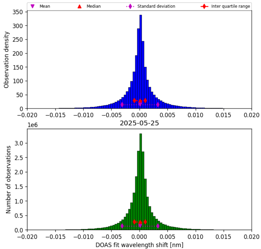
Figure 42: Histogram of “DOAS fit wavelength shift” for 2025-05-25 to 2025-05-26
