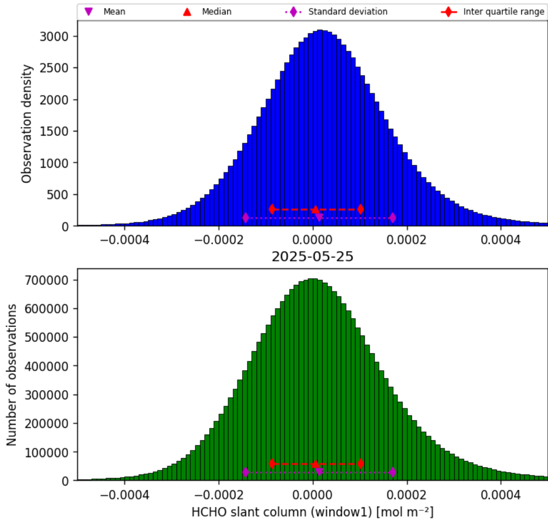
Figure 36: Histogram of “HCHO slant column (window1)” for 2025-05-25 to 2025-05-26
