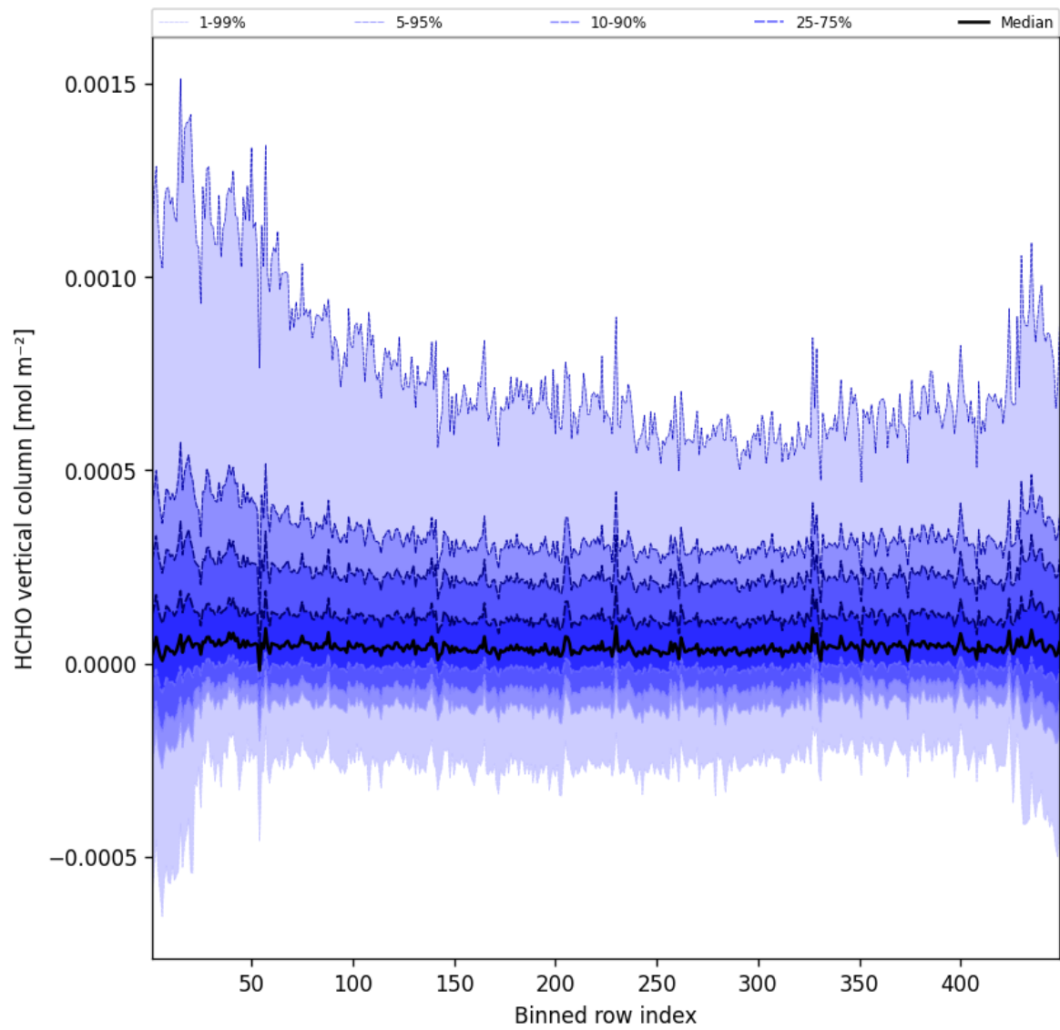
Figure 47: Along track statistics of “HCHO vertical column” for 2025-05-25 to 2025-05-26
