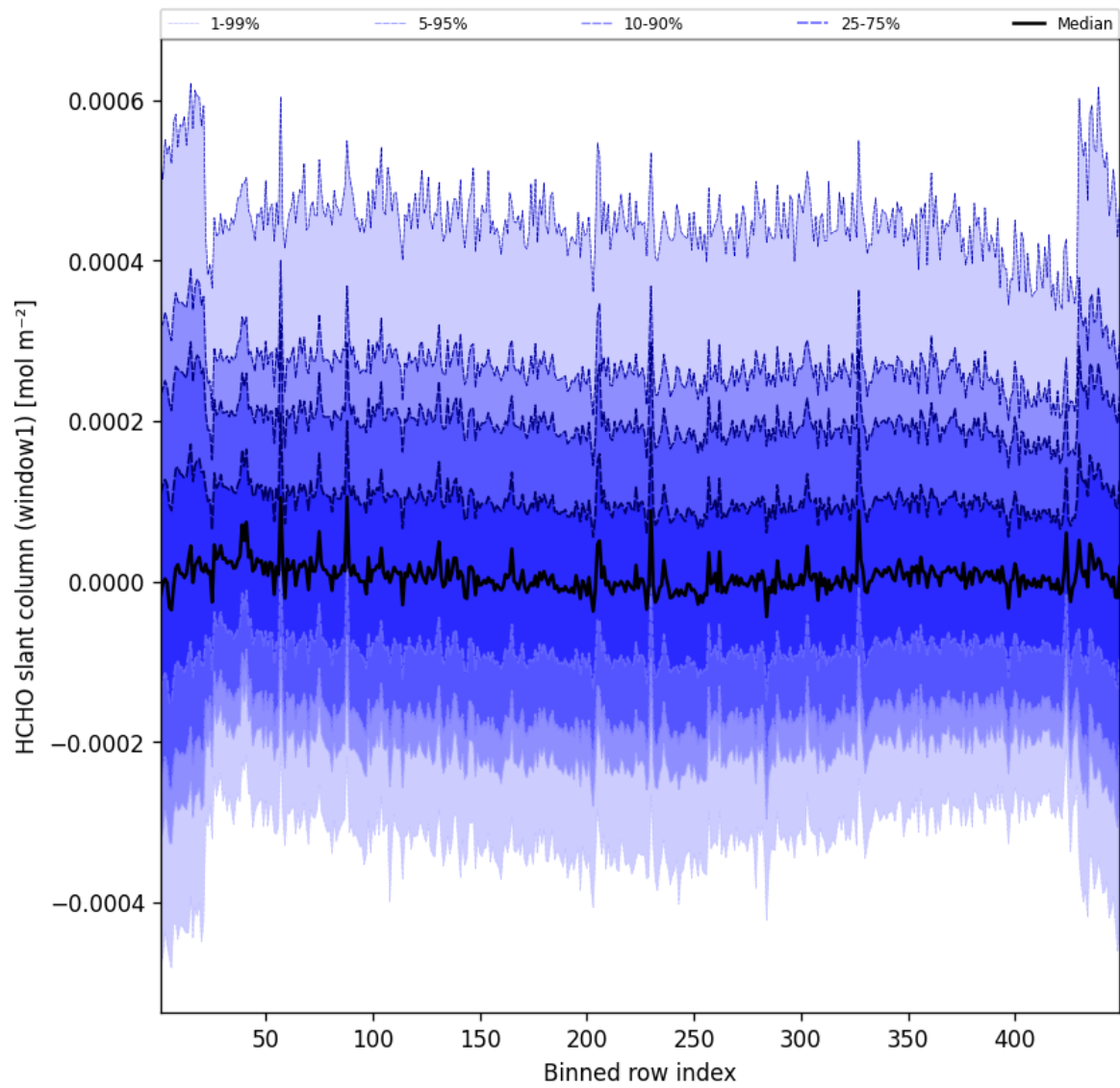
Figure 50: Along track statistics of “HCHO slant column (window1)” for 2025-05-25 to 2025-05-26
