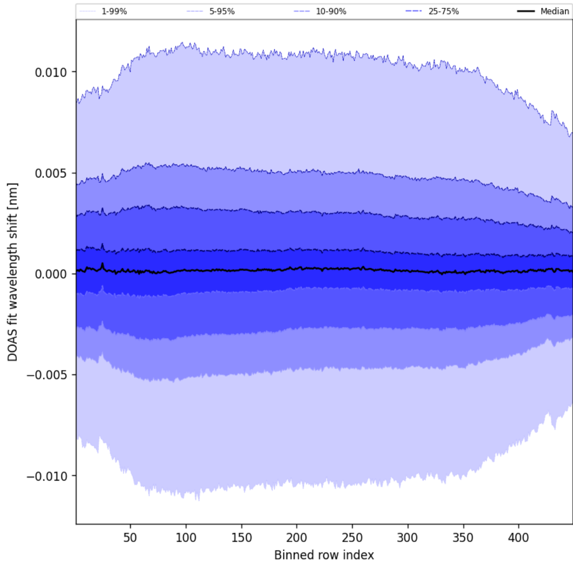
Figure 56: Along track statistics of “DOAS fit wavelength shift” for 2025-05-25 to 2025-05-26
