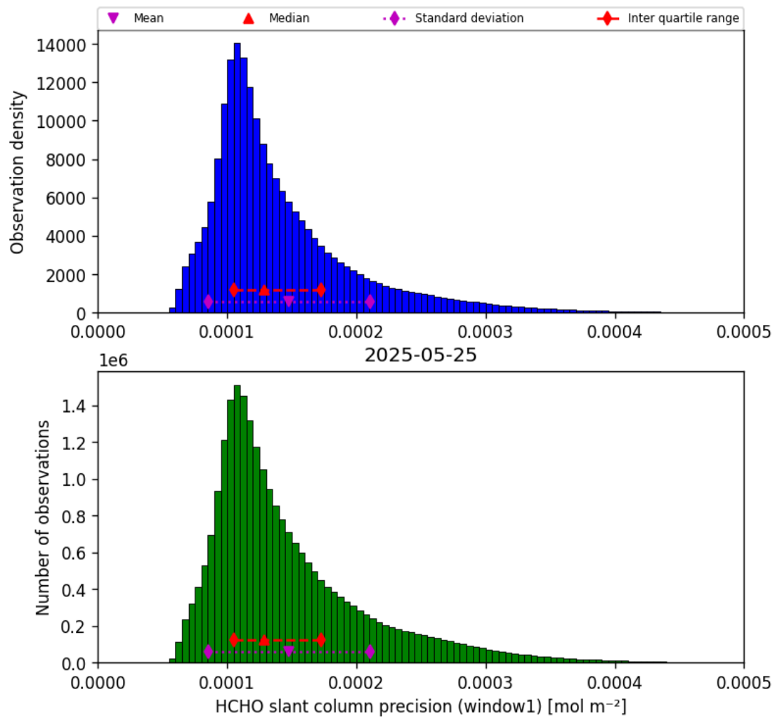
Figure 37: Histogram of “HCHO slant column precision (window1)” for 2025-05-25 to 2025-05-26
