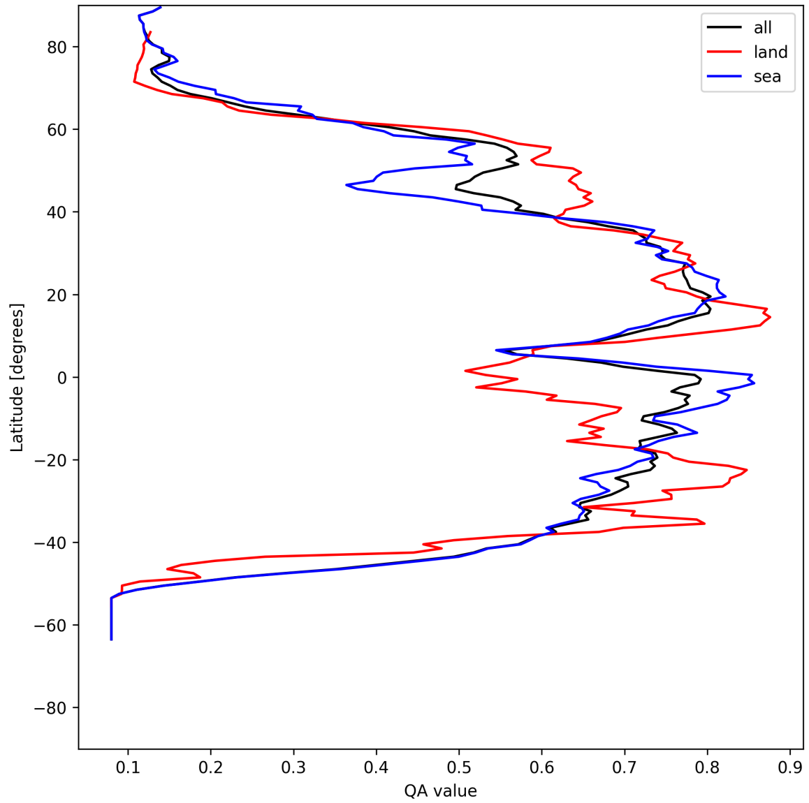
Figure 18: Zonal average of “QA value” for 2025-05-25 to 2025-05-26.
