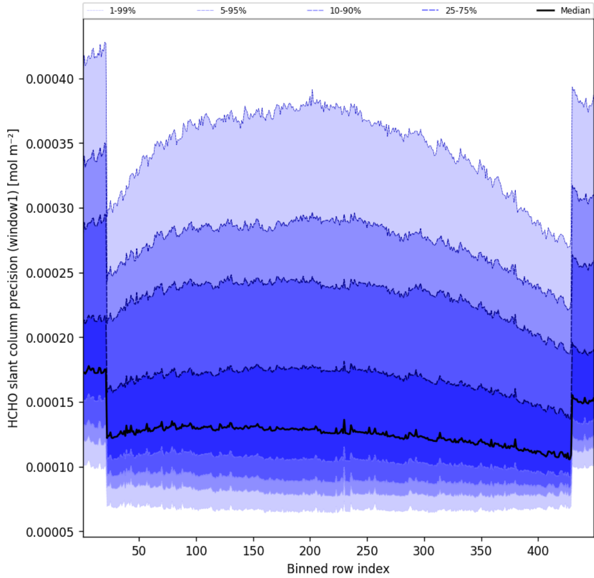
Figure 51: Along track statistics of “HCHO slant column precision (window1)” for 2025-05-25 to 2025-05-26
