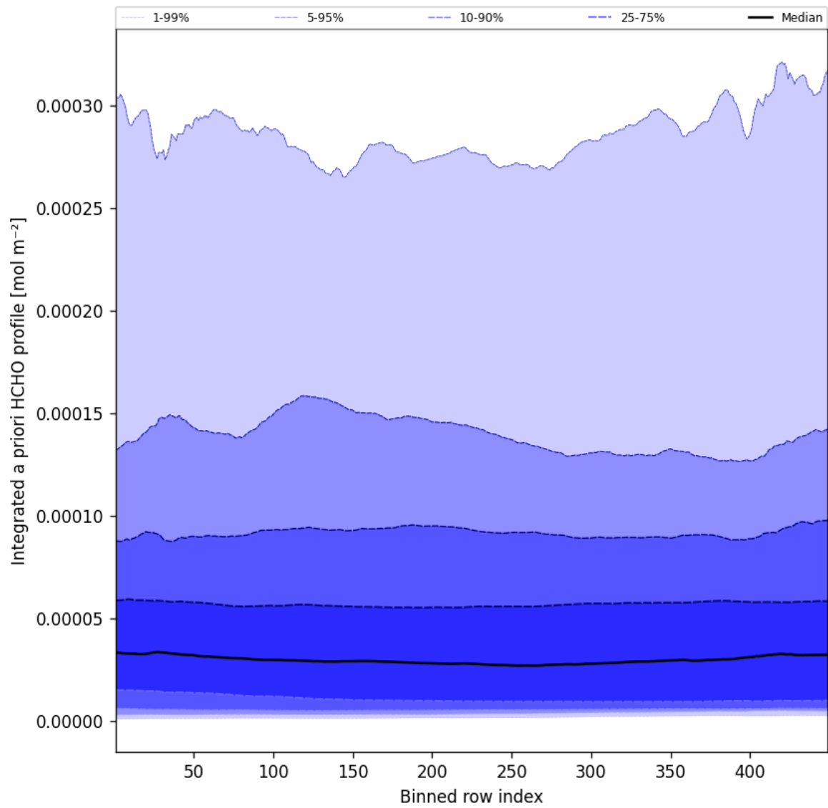
Figure 55: Along track statistics of “Integrated a priori HCHO profile” for 2025-05-25 to 2025-05-26
