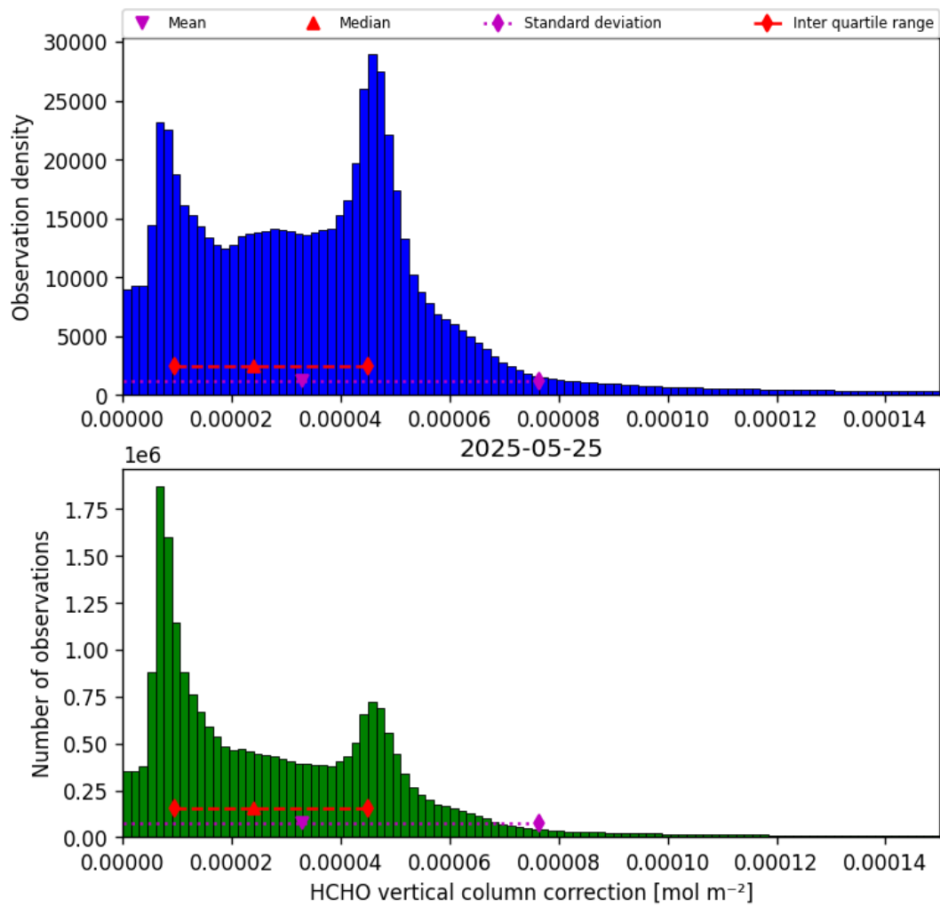
Figure 35: Histogram of “HCHO vertical column correction” for 2025-05-25 to 2025-05-26
