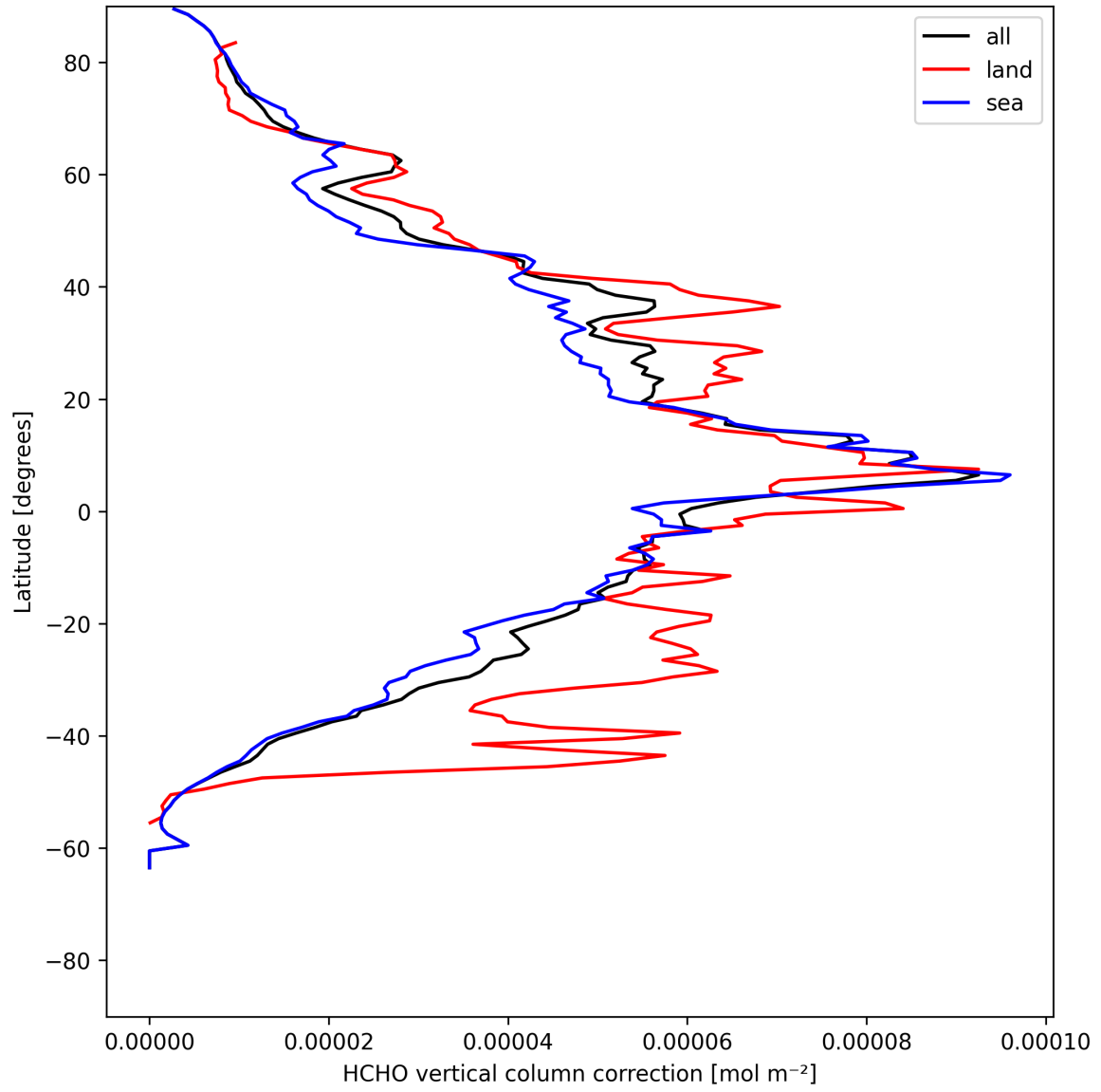
Figure 21: Zonal average of “HCHO vertical column correction” for 2025-05-25 to 2025-05-26.
