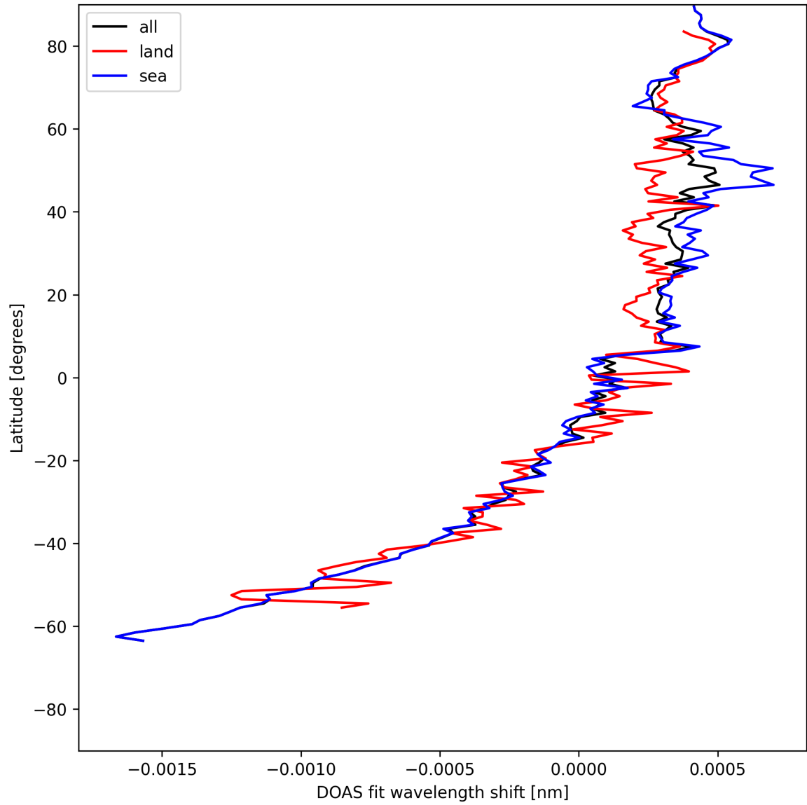
Figure 28: Zonal average of “DOAS fit wavelength shift” for 2025-05-25 to 2025-05-26.
