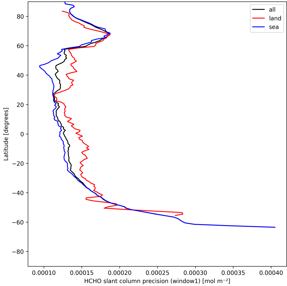
Figure 23: Zonal average of “HCHO slant column precision (window1)” for 2025-05-25 to 2025-05-26.
