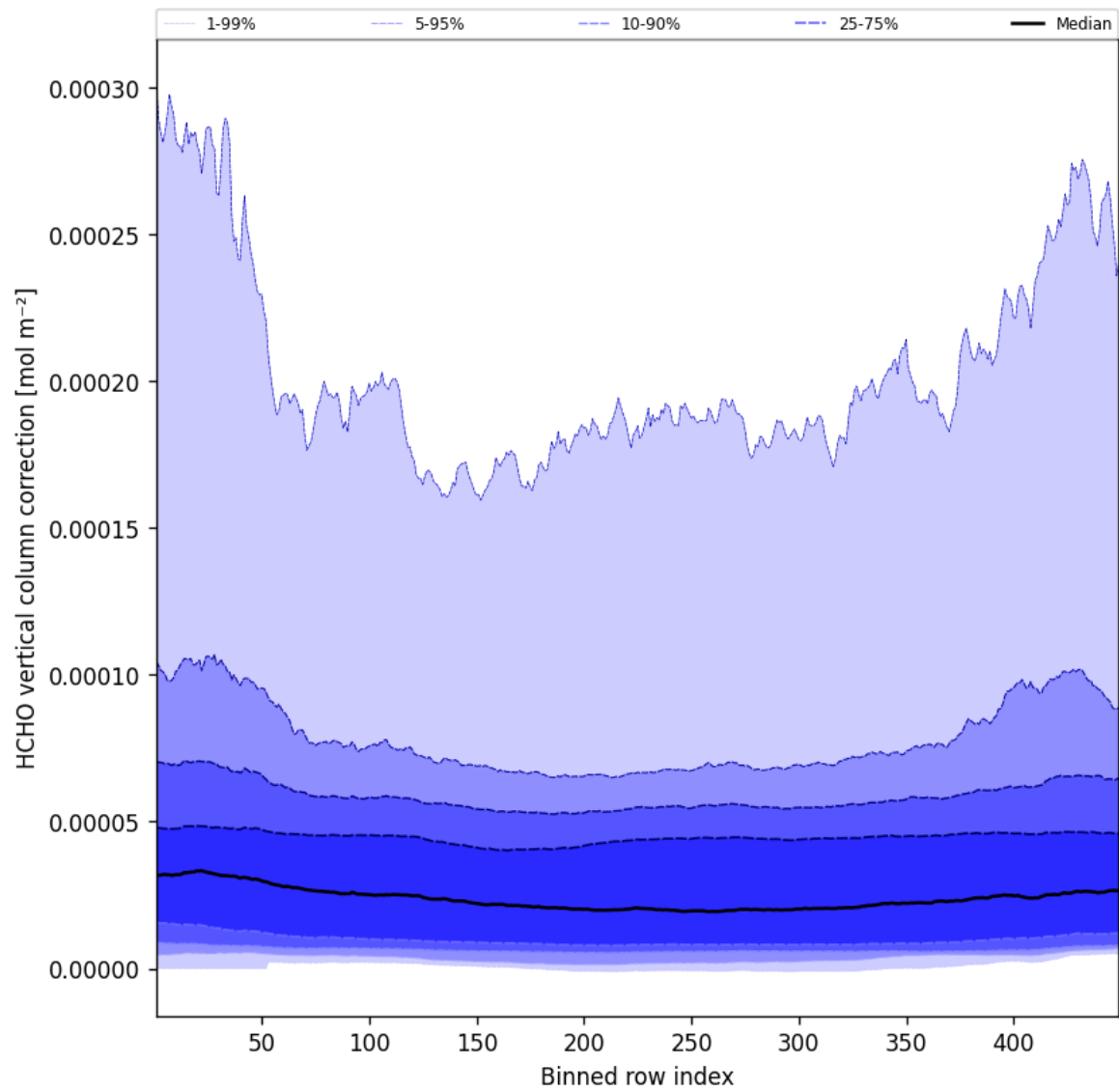
Figure 49: Along track statistics of “HCHO vertical column correction” for 2025-05-25 to 2025-05-26
