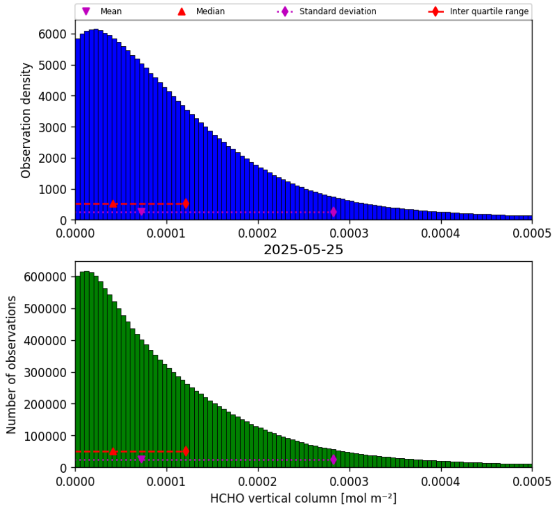
Figure 33: Histogram of “HCHO vertical column” for 2025-05-25 to 2025-05-26
