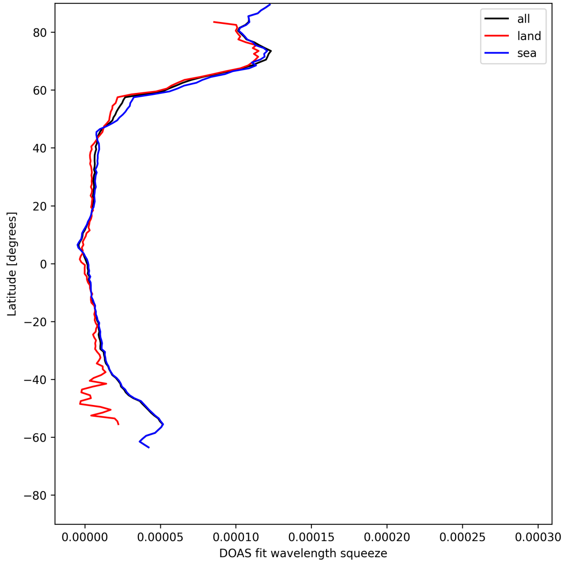
Figure 29: Zonal average of “DOAS fit wavelength squeeze” for 2025-05-25 to 2025-05-26.
