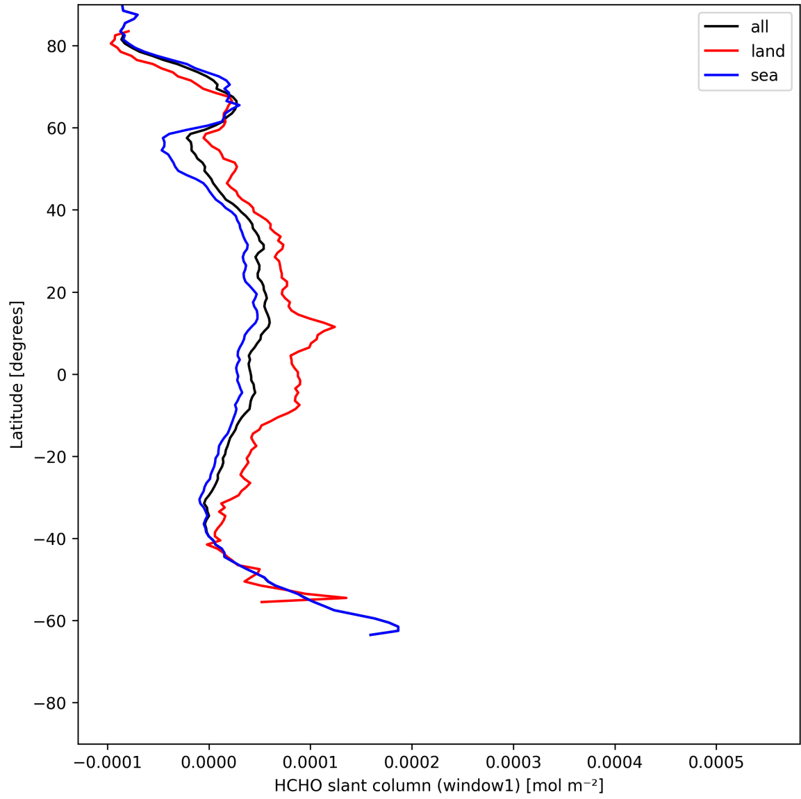
Figure 22: Zonal average of “HCHO slant column (window1)” for 2025-05-25 to 2025-05-26.
