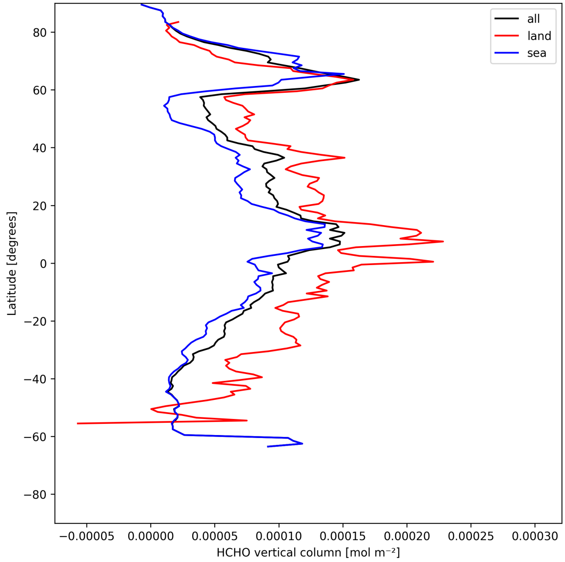
Figure 19: Zonal average of “HCHO vertical column” for 2025-05-25 to 2025-05-26.
