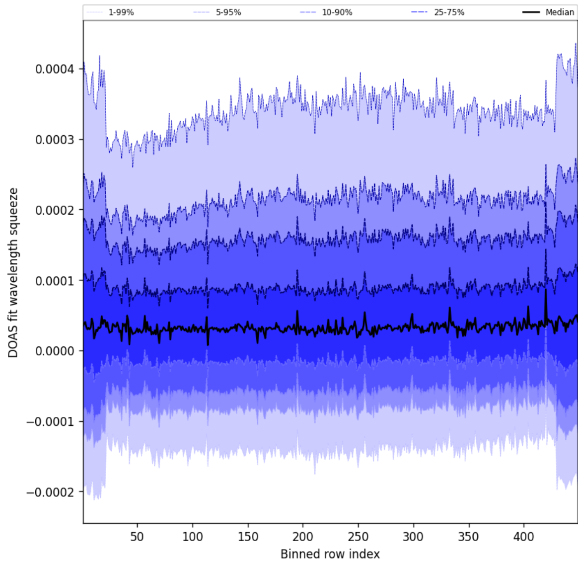
Figure 57: Along track statistics of “DOAS fit wavelength squeeze” for 2025-05-25 to 2025-05-26
