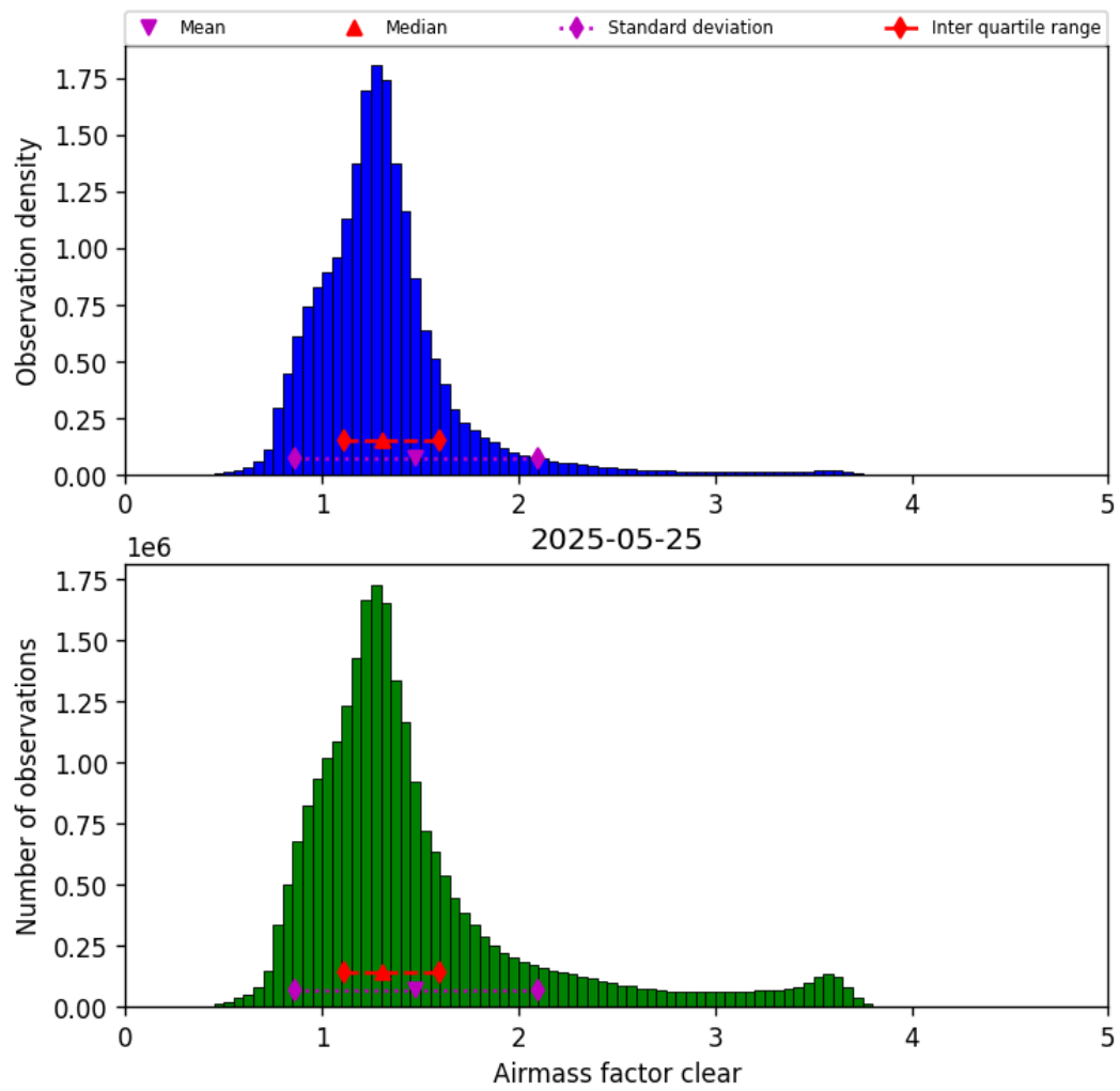
Figure 40: Histogram of “Airmass factor clear” for 2025-05-25 to 2025-05-26
