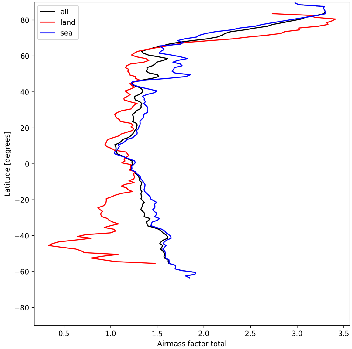
Figure 24: Zonal average of “Airmass factor total” for 2025-05-25 to 2025-05-26.
