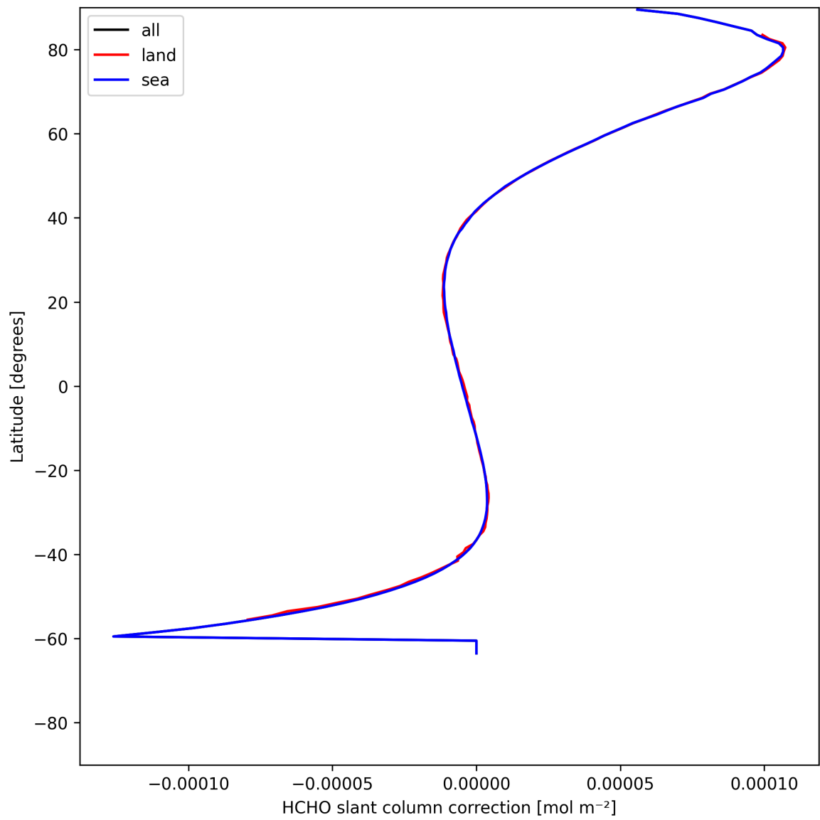
Figure 31: Zonal average of “HCHO slant column correction” for 2025-05-25 to 2025-05-26.
