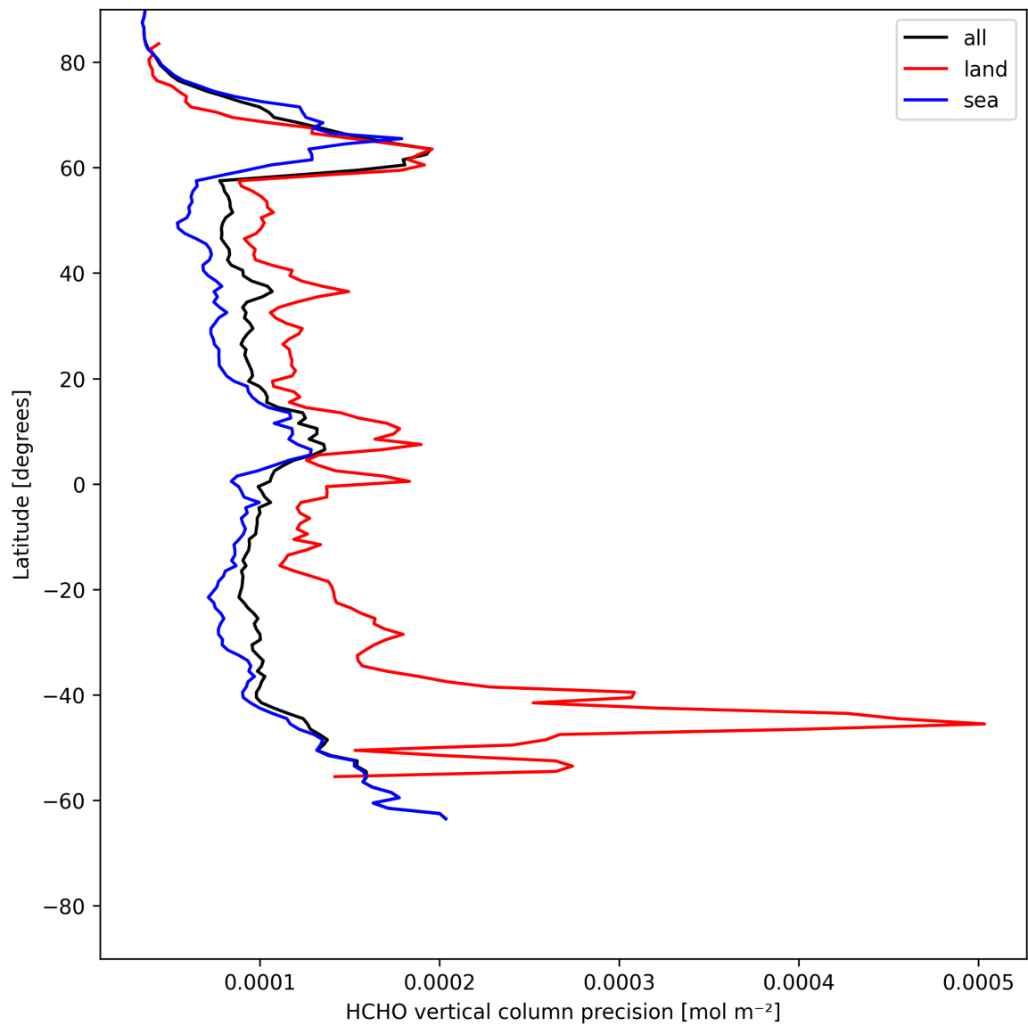
Figure 20: Zonal average of “HCHO vertical column precision” for 2025-05-25 to 2025-05-26.
