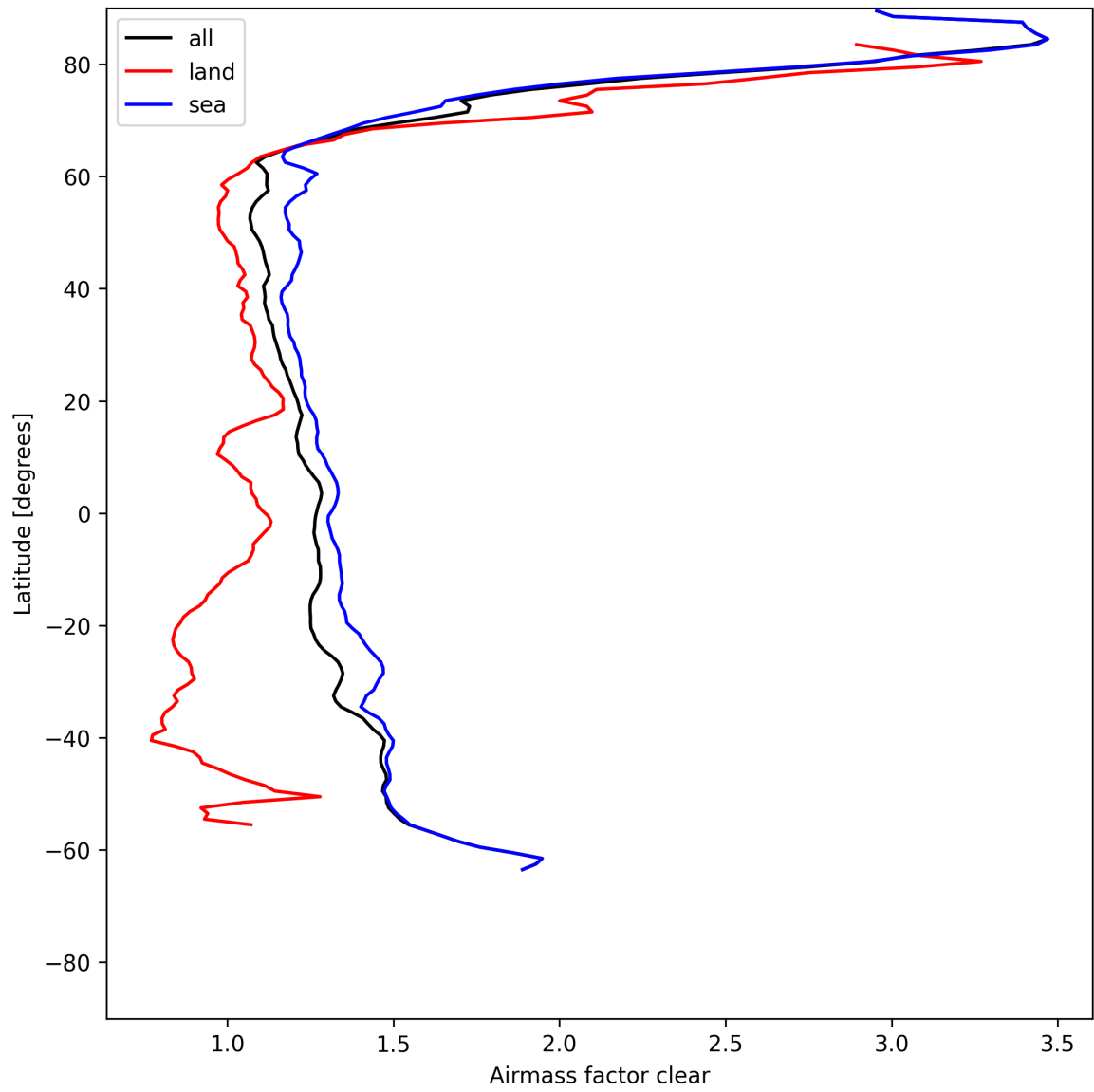
Figure 26: Zonal average of “Airmass factor clear” for 2025-05-25 to 2025-05-26.
