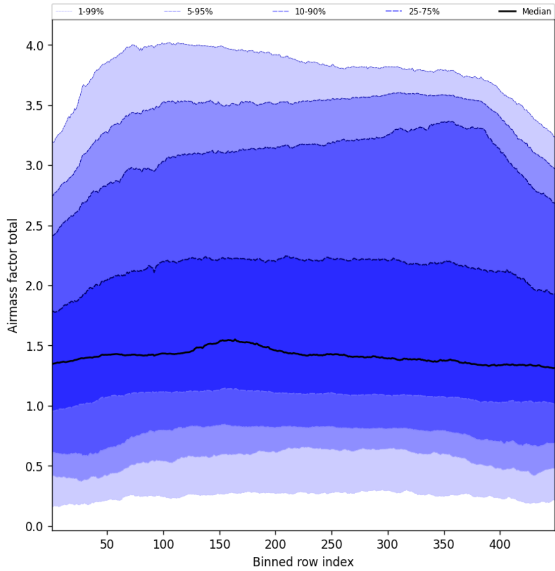
Figure 52: Along track statistics of “Airmass factor total” for 2025-05-25 to 2025-05-26
