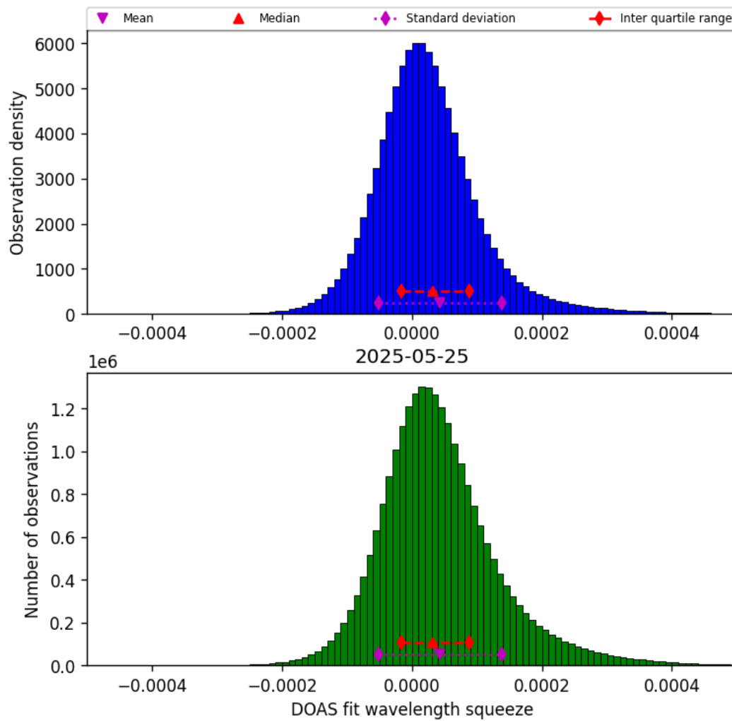
Figure 43: Histogram of “DOAS fit wavelength squeeze” for 2025-05-25 to 2025-05-26
