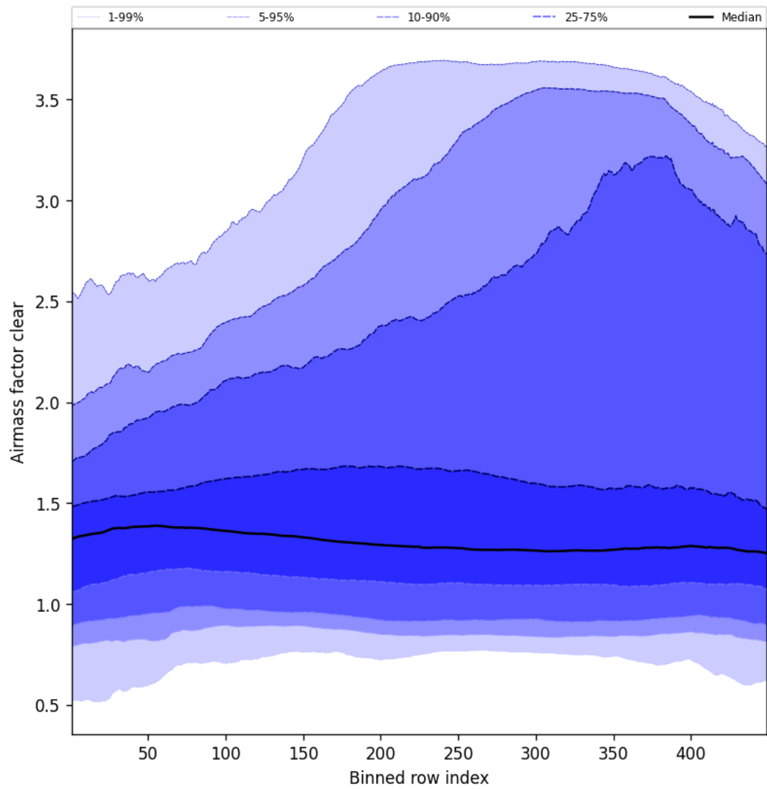
Figure 54: Along track statistics of “Airmass factor clear” for 2025-05-25 to 2025-05-26
