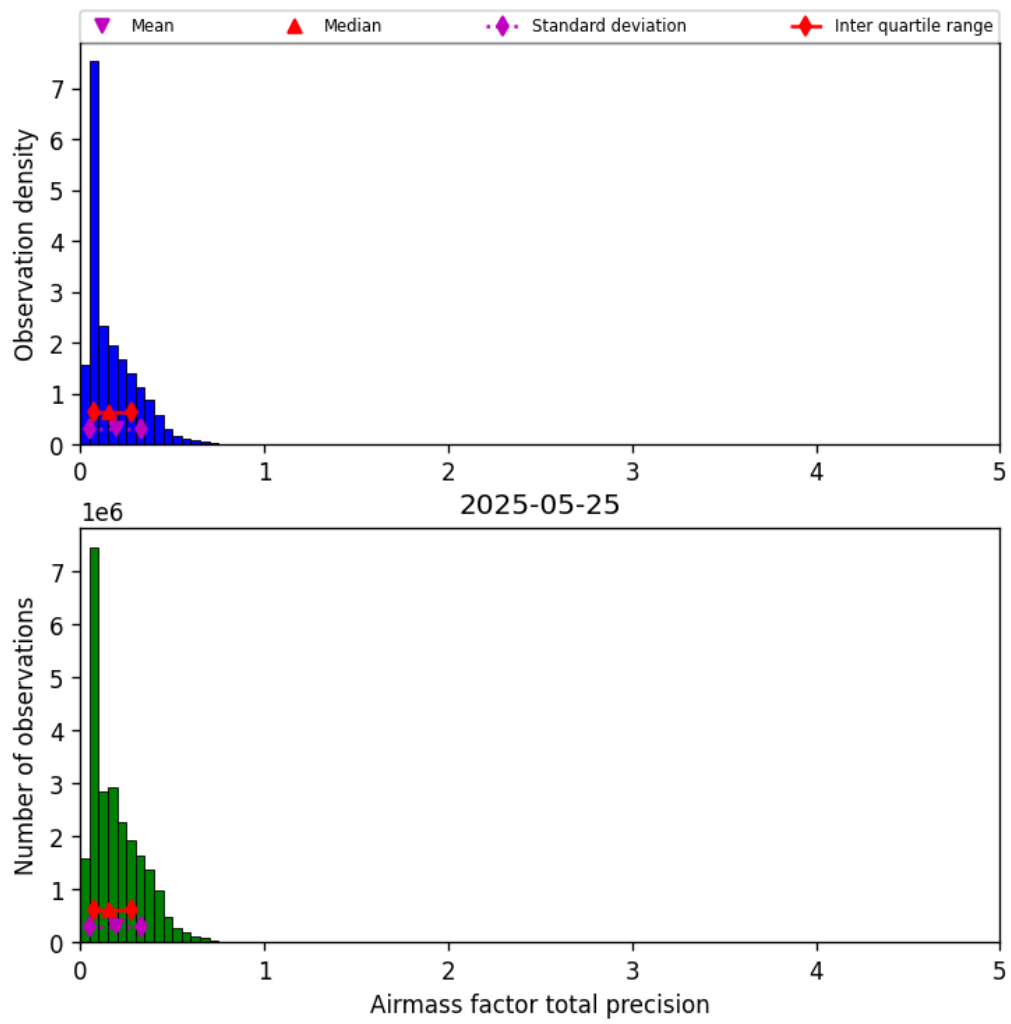
Figure 39: Histogram of “Airmass factor total precision” for 2025-05-25 to 2025-05-26
