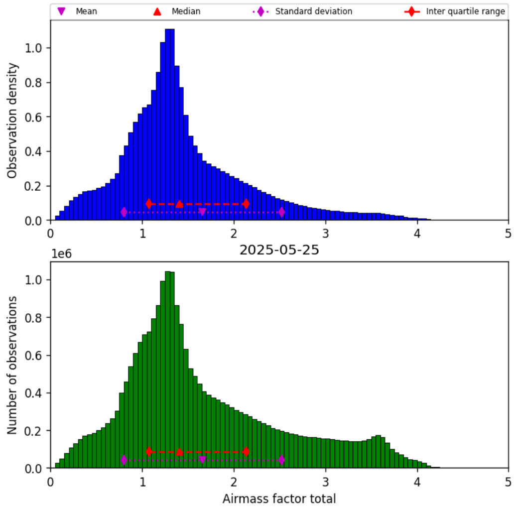
Figure 38: Histogram of “Airmass factor total” for 2025-05-25 to 2025-05-26
