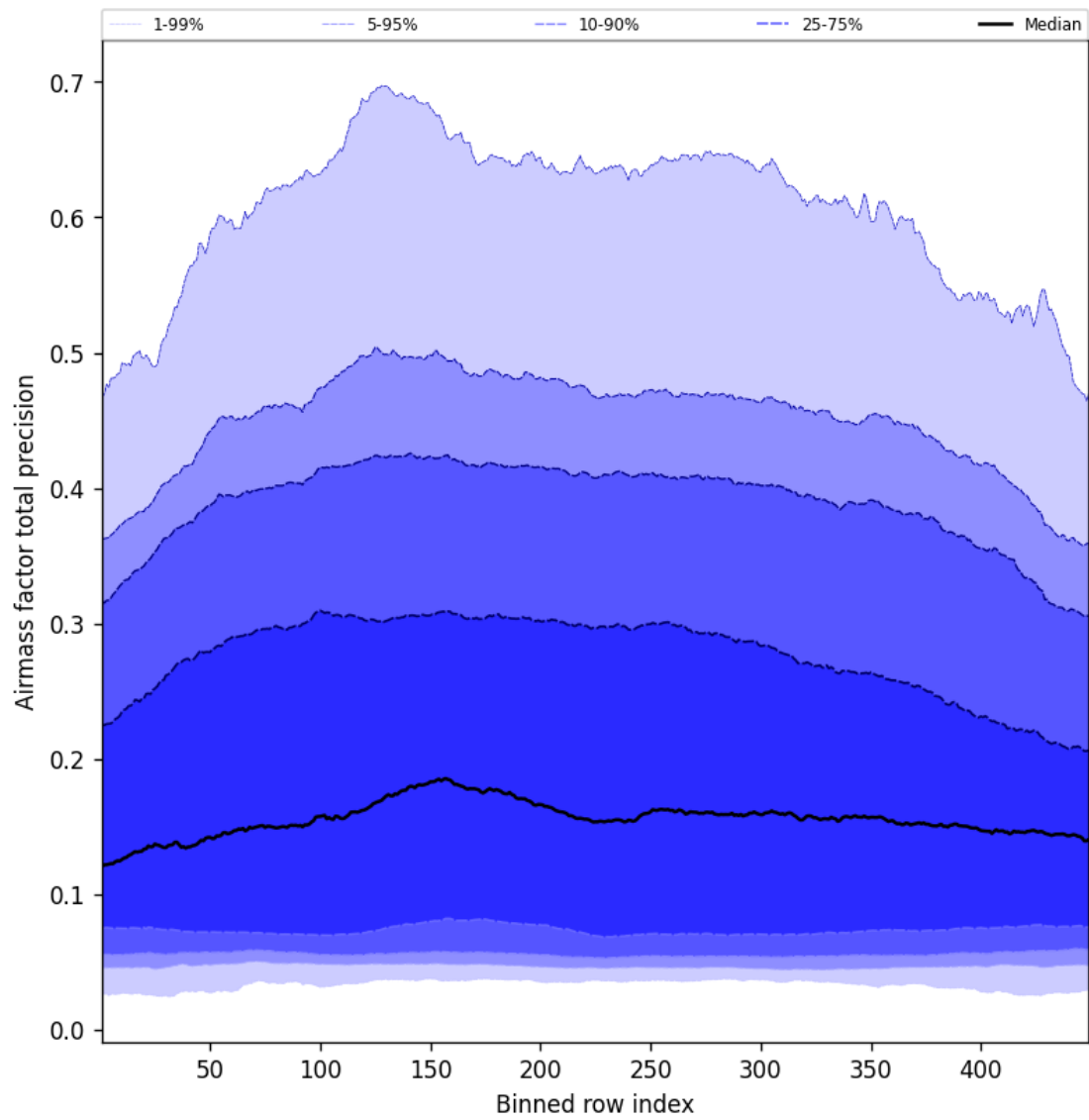
Figure 53: Along track statistics of “Airmass factor total precision” for 2025-05-25 to 2025-05-26
