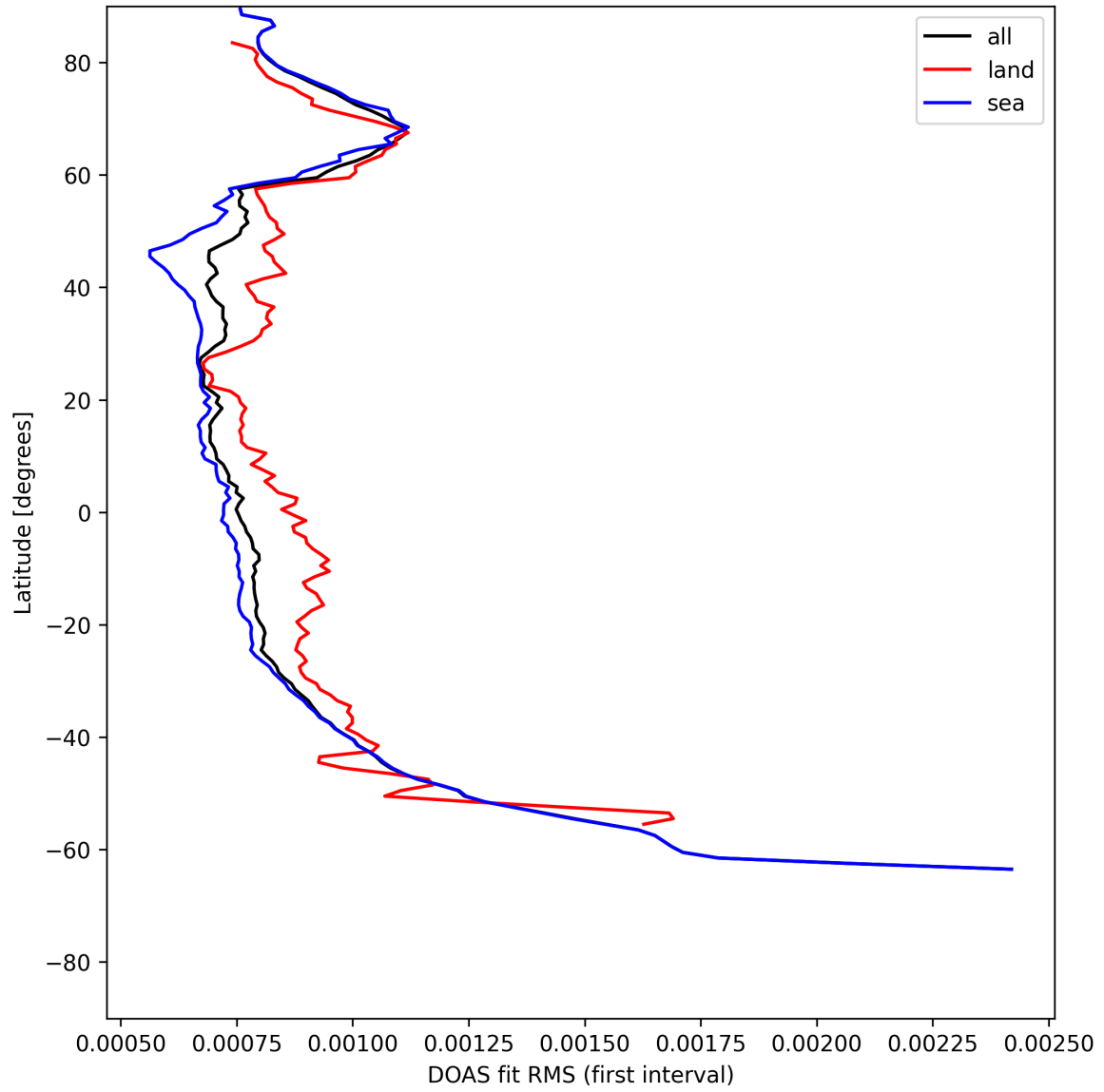
Figure 30: Zonal average of “DOAS fit RMS (first interval)” for 2025-05-25 to 2025-05-26.
