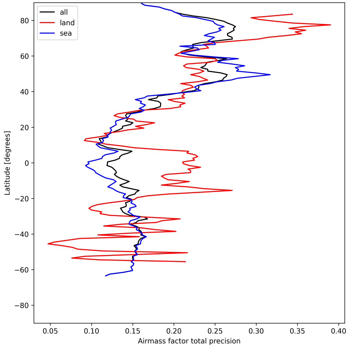
Figure 25: Zonal average of “Airmass factor total precision” for 2025-05-25 to 2025-05-26.
