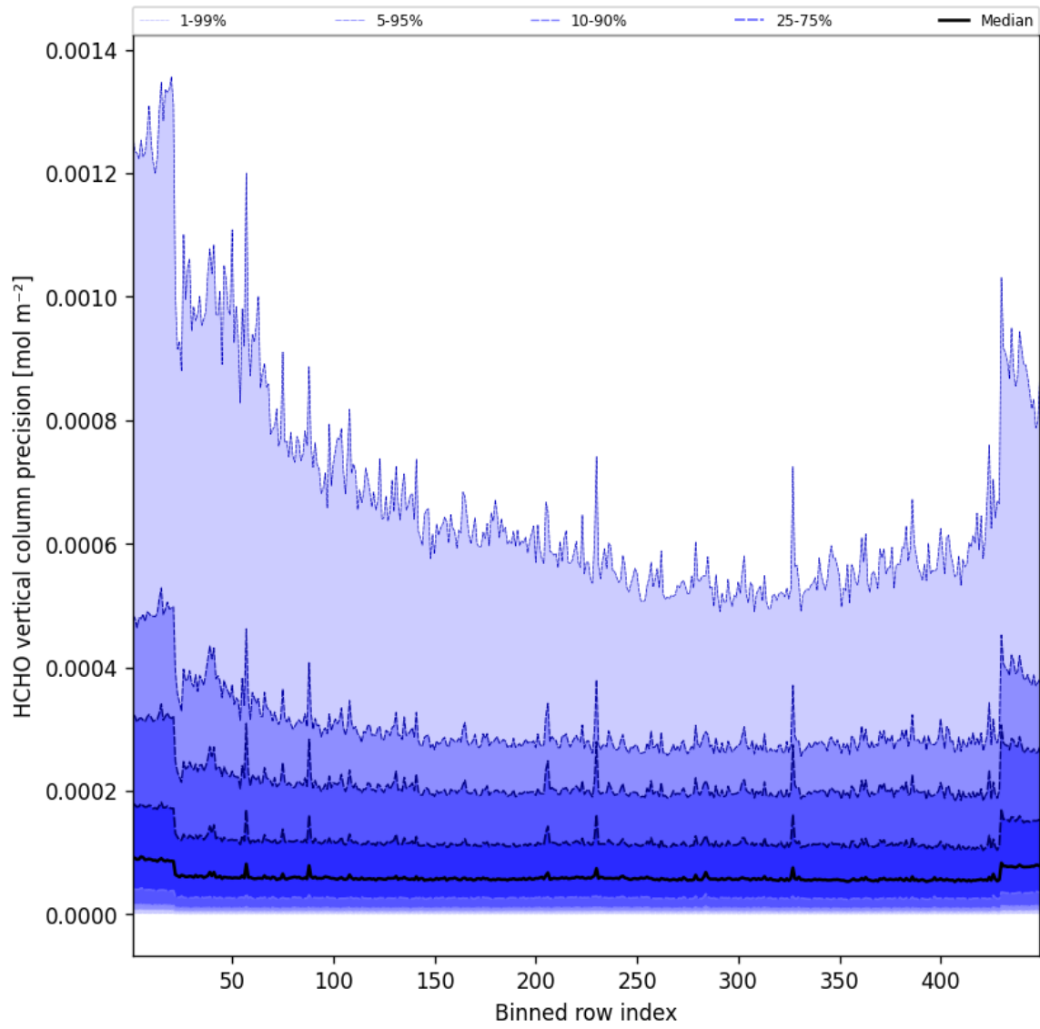
Figure 48: Along track statistics of “HCHO vertical column precision” for 2025-05-25 to 2025-05-26
