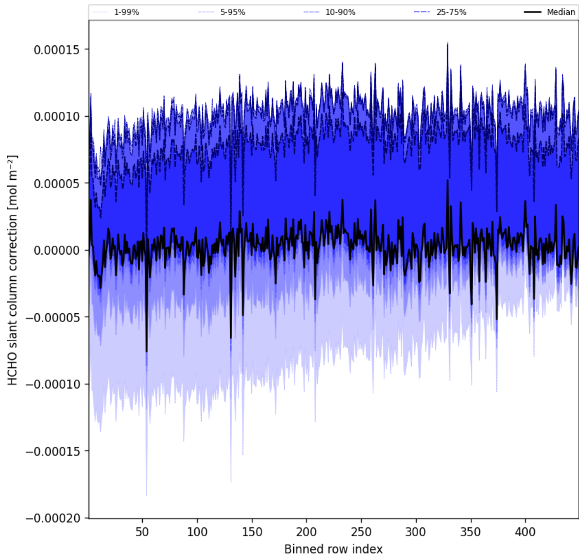
Figure 59: Along track statistics of “HCHO slant column correction” for 2025-05-25 to 2025-05-26
