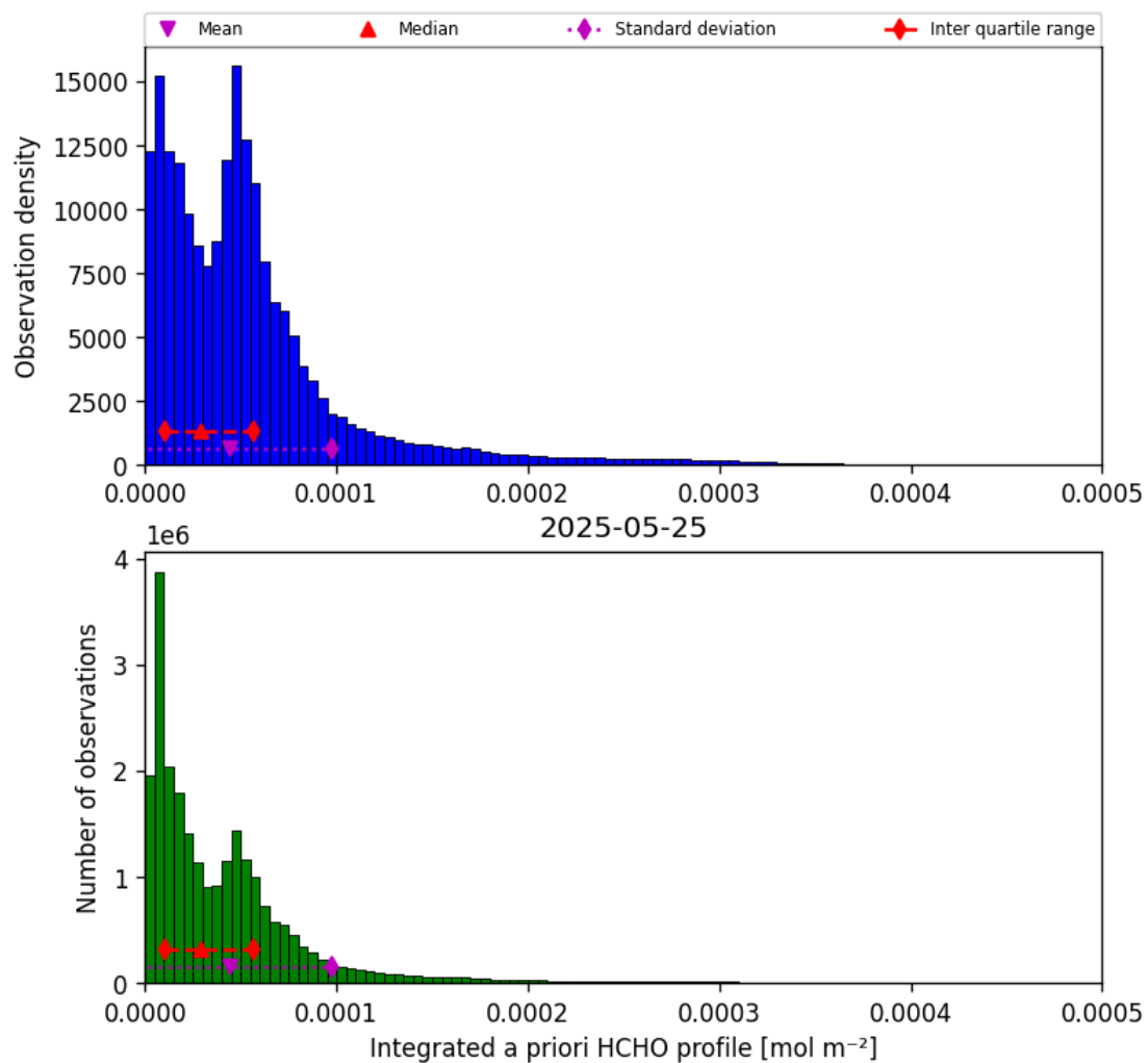
Figure 41: Histogram of “Integrated a priori HCHO profile” for 2025-05-25 to 2025-05-26
