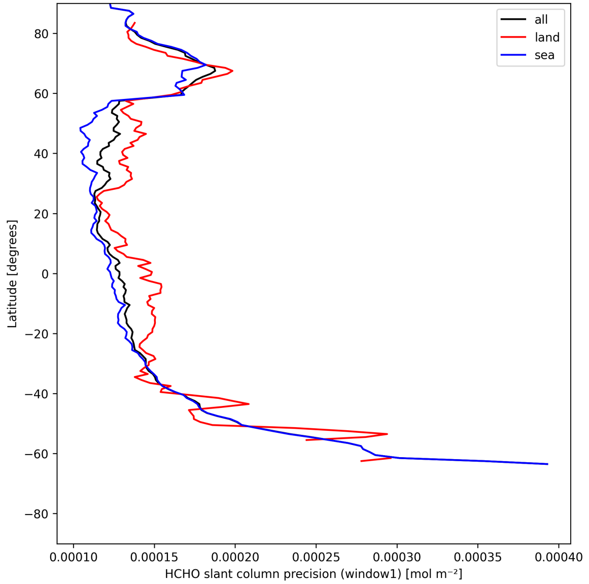
Figure 23: Zonal average of “HCHO slant column precision (window1)” for 2025-05-26 to 2025-05-27.
