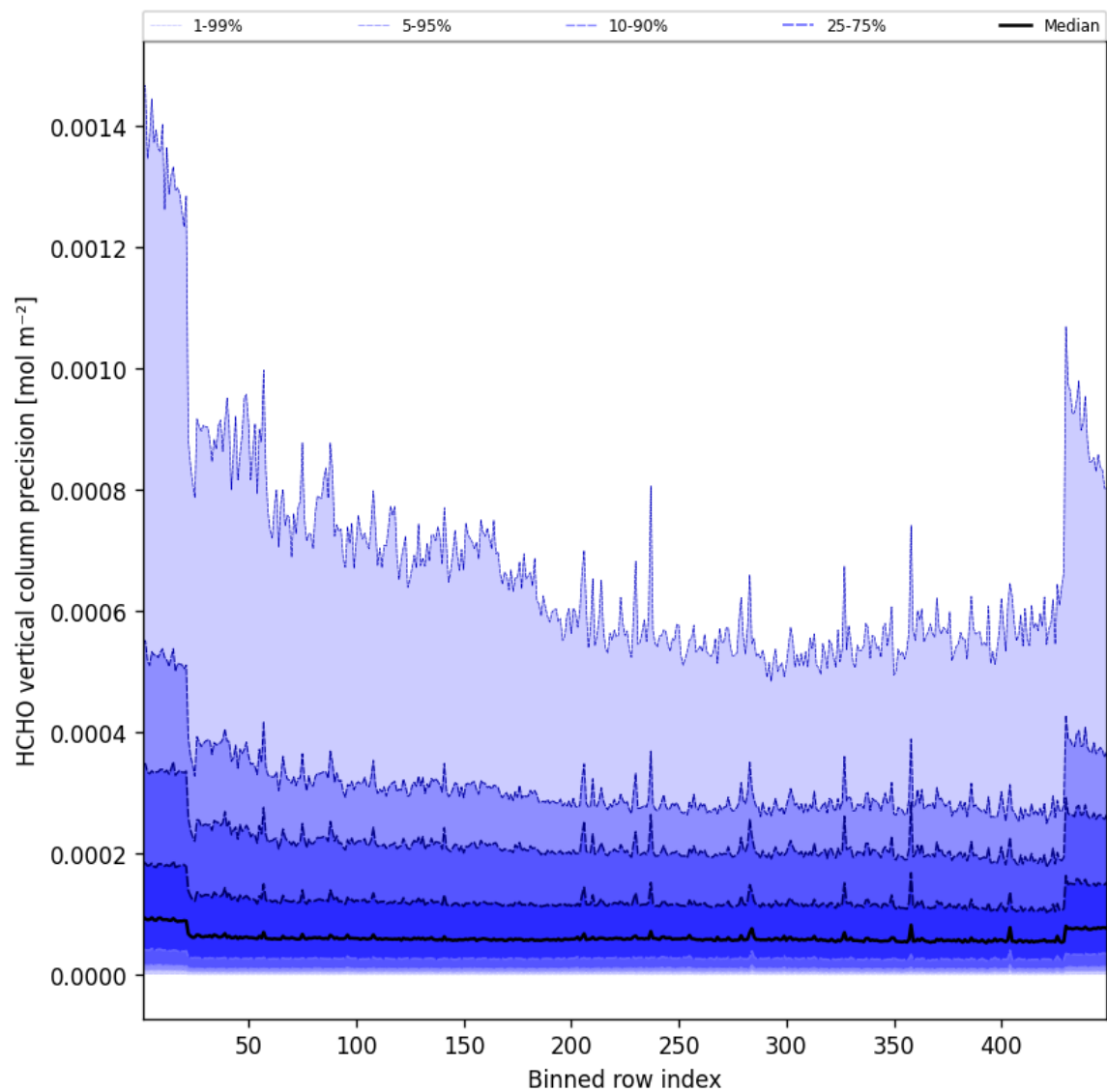
Figure 48: Along track statistics of “HCHO vertical column precision” for 2025-05-26 to 2025-05-27
