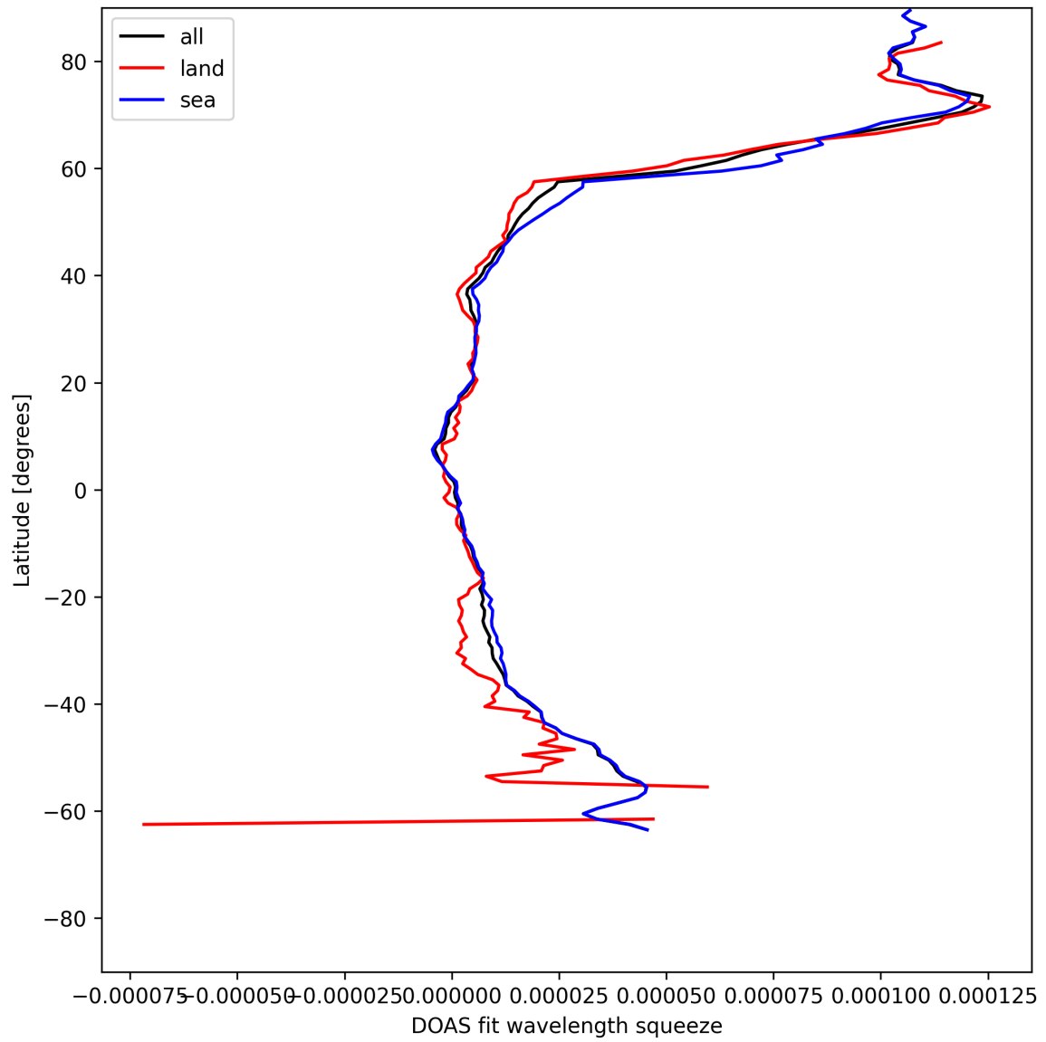
Figure 29: Zonal average of “DOAS fit wavelength squeeze” for 2025-05-26 to 2025-05-27.
