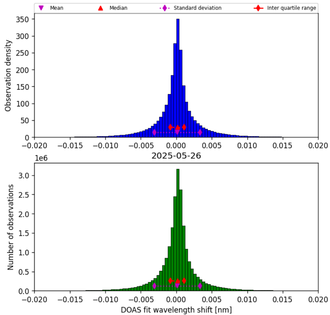
Figure 42: Histogram of “DOAS fit wavelength shift” for 2025-05-26 to 2025-05-27
