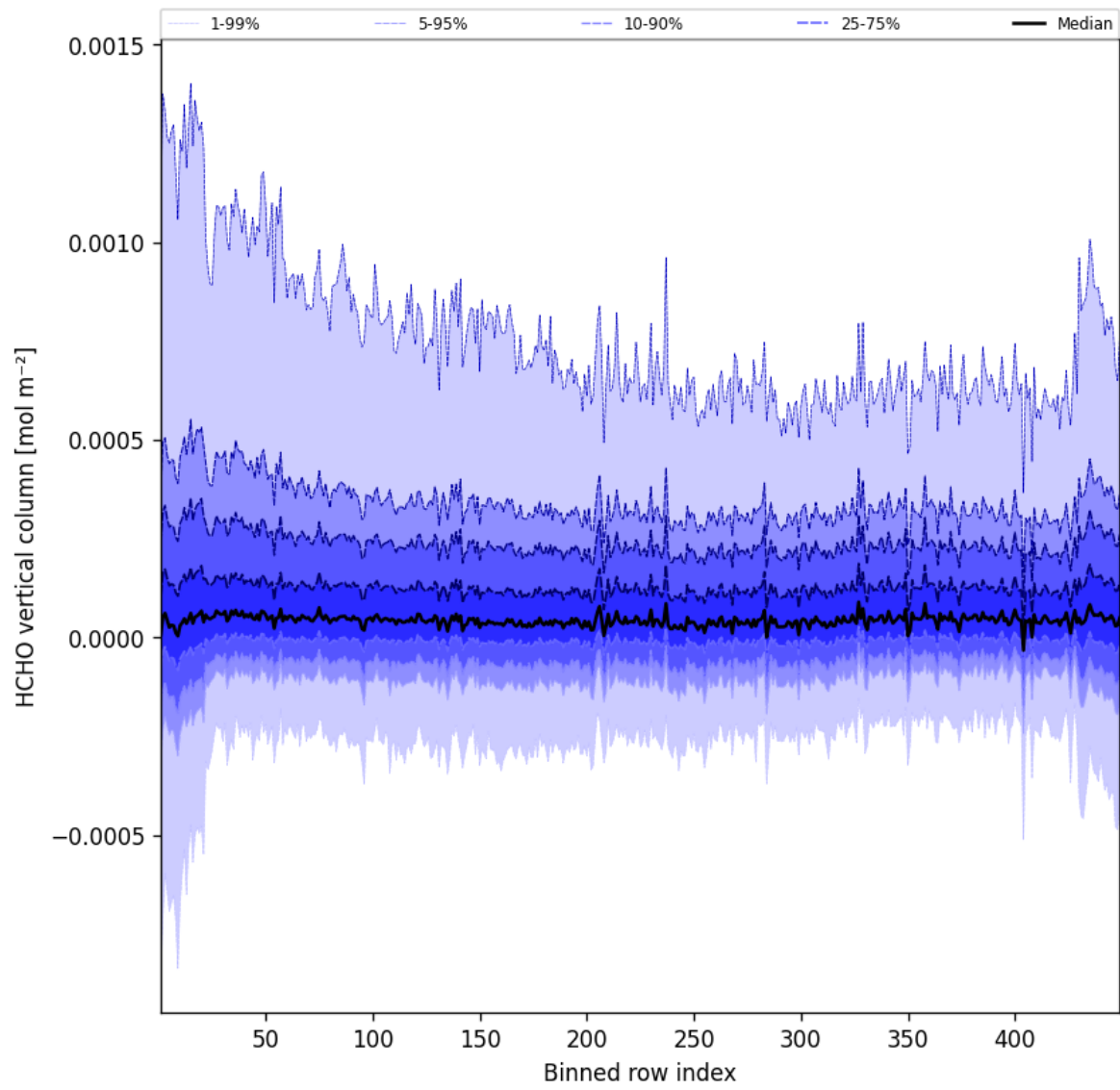
Figure 47: Along track statistics of “HCHO vertical column” for 2025-05-26 to 2025-05-27
