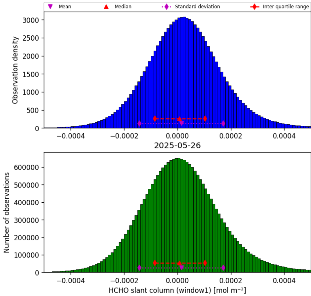
Figure 36: Histogram of “HCHO slant column (window1)” for 2025-05-26 to 2025-05-27
