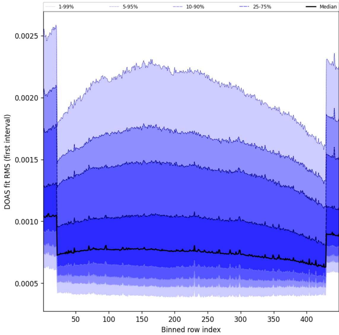
Figure 58: Along track statistics of “DOAS fit RMS (first interval)” for 2025-05-26 to 2025-05-27
