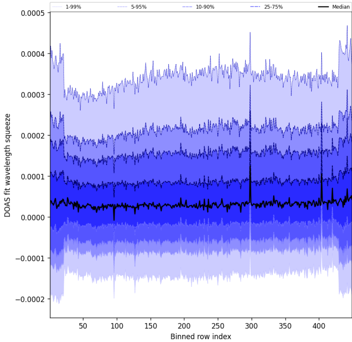
Figure 57: Along track statistics of “DOAS fit wavelength squeeze” for 2025-05-26 to 2025-05-27
