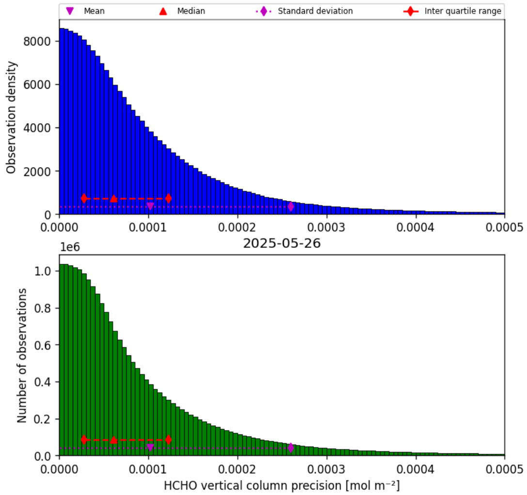
Figure 34: Histogram of “HCHO vertical column precision” for 2025-05-26 to 2025-05-27
