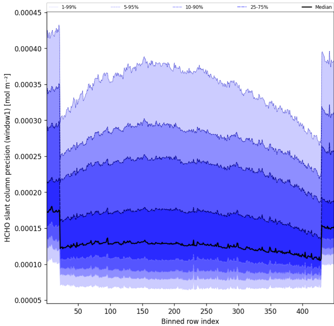
Figure 51: Along track statistics of “HCHO slant column precision (window1)” for 2025-05-26 to 2025-05-27
