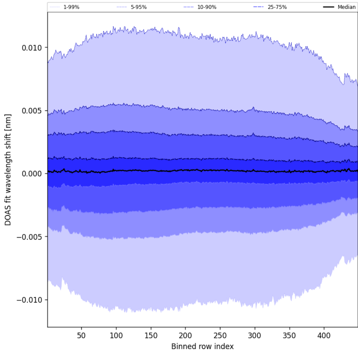
Figure 56: Along track statistics of “DOAS fit wavelength shift” for 2025-05-26 to 2025-05-27
