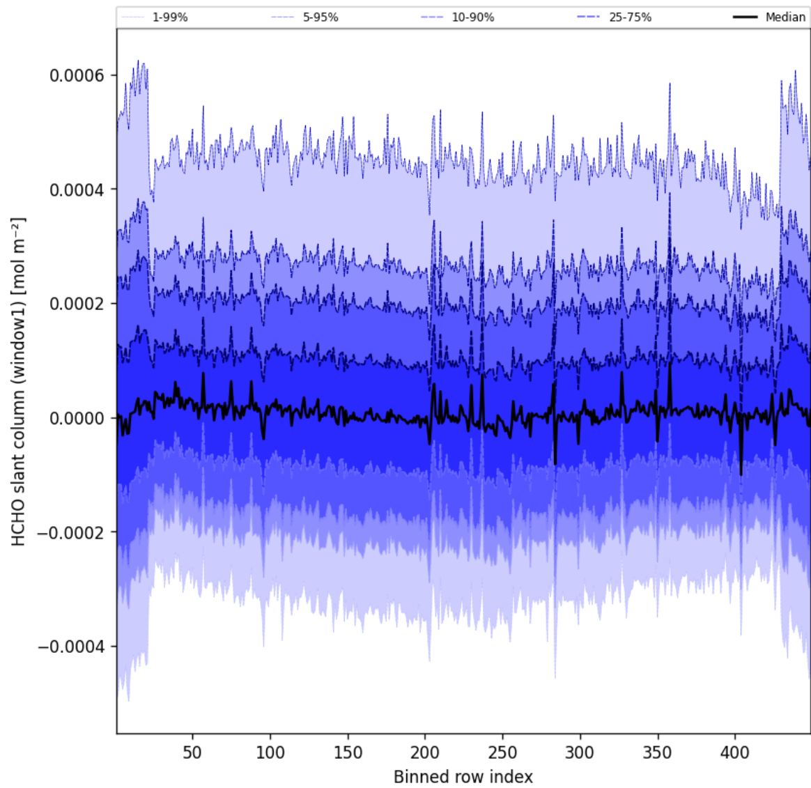
Figure 50: Along track statistics of “HCHO slant column (window1)” for 2025-05-26 to 2025-05-27
