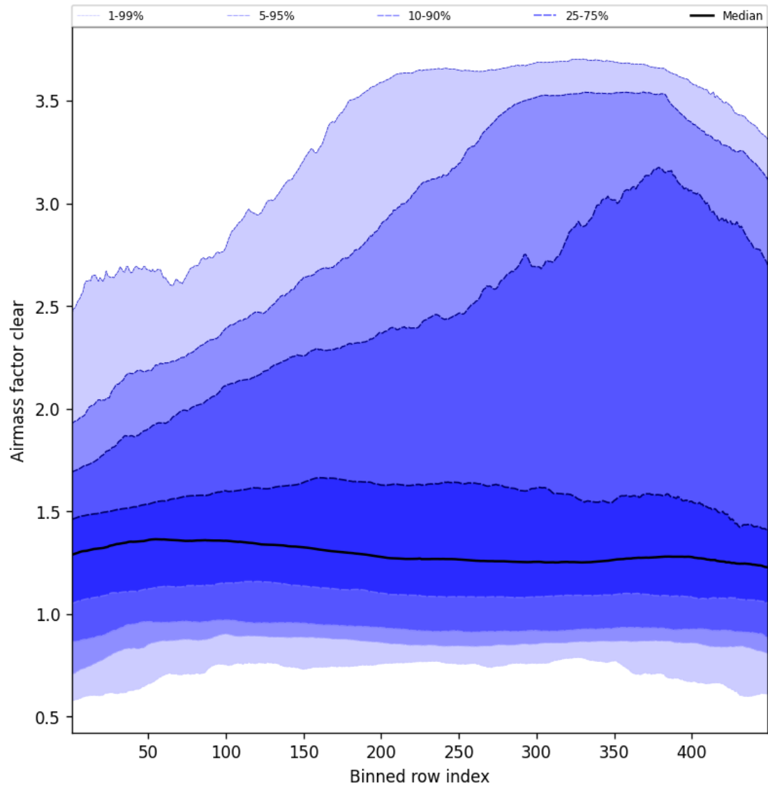
Figure 54: Along track statistics of “Airmass factor clear” for 2025-05-26 to 2025-05-27
