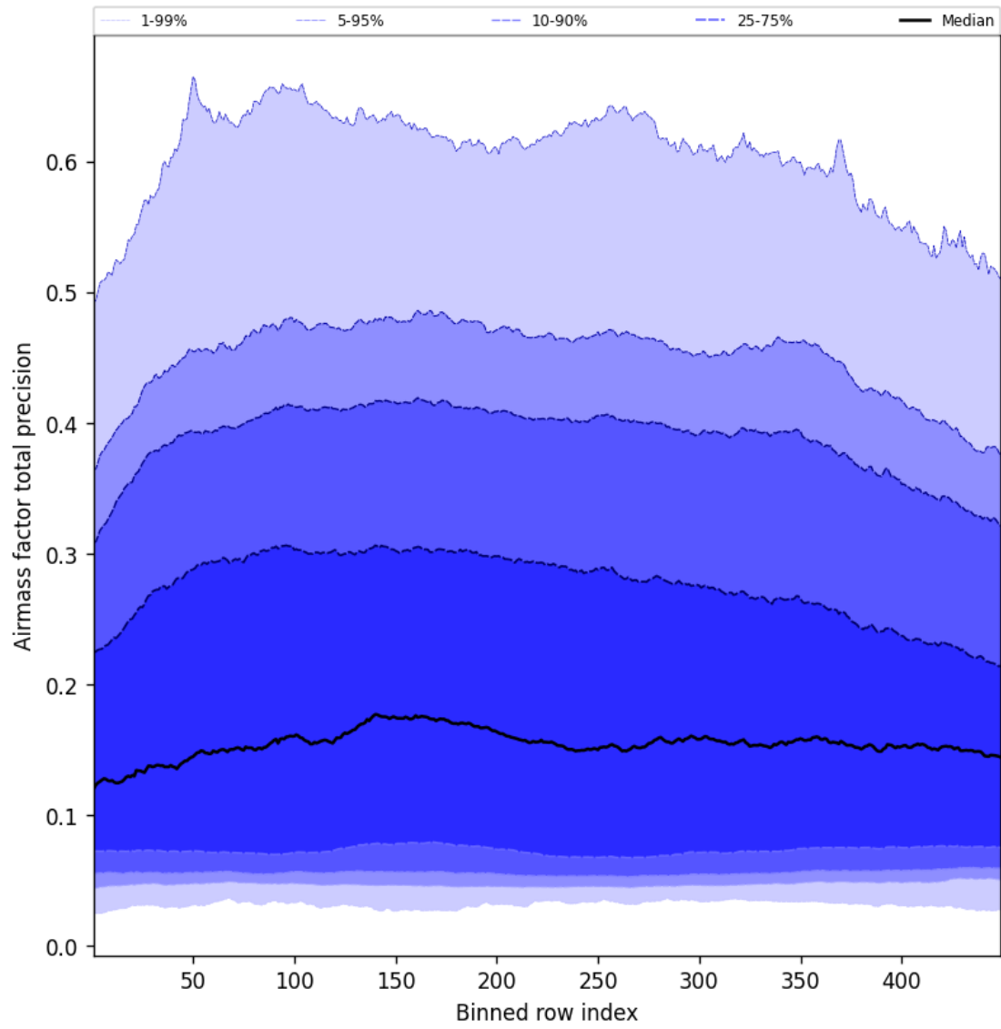
Figure 53: Along track statistics of “Airmass factor total precision” for 2025-05-26 to 2025-05-27
