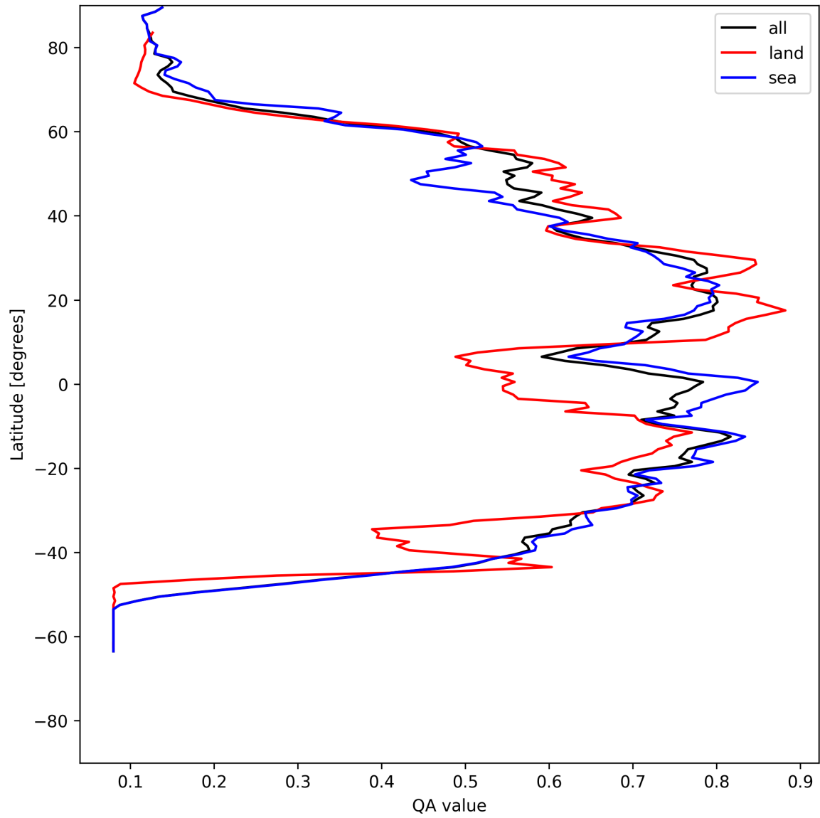
Figure 18: Zonal average of “QA value” for 2025-05-26 to 2025-05-27.
