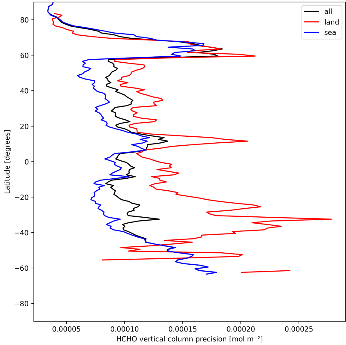
Figure 20: Zonal average of “HCHO vertical column precision” for 2025-05-26 to 2025-05-27.
