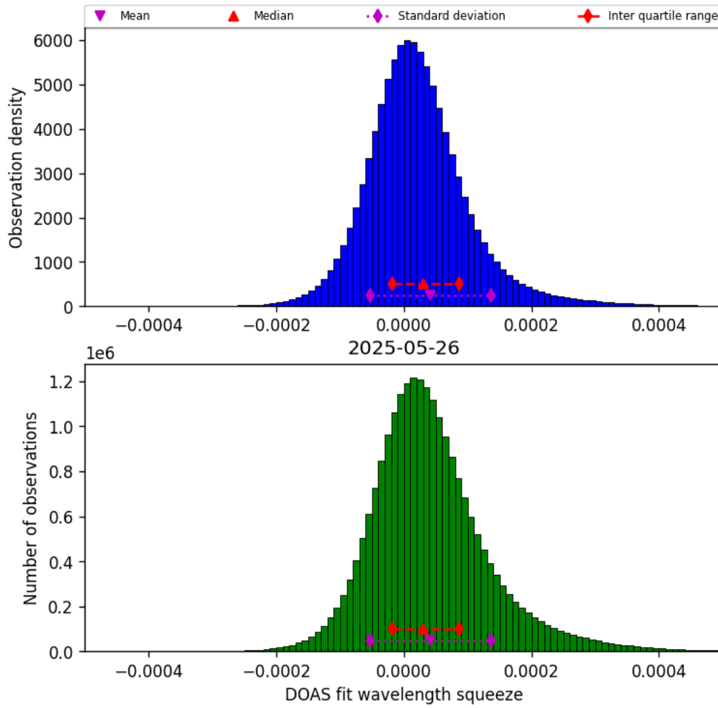
Figure 43: Histogram of “DOAS fit wavelength squeeze” for 2025-05-26 to 2025-05-27
