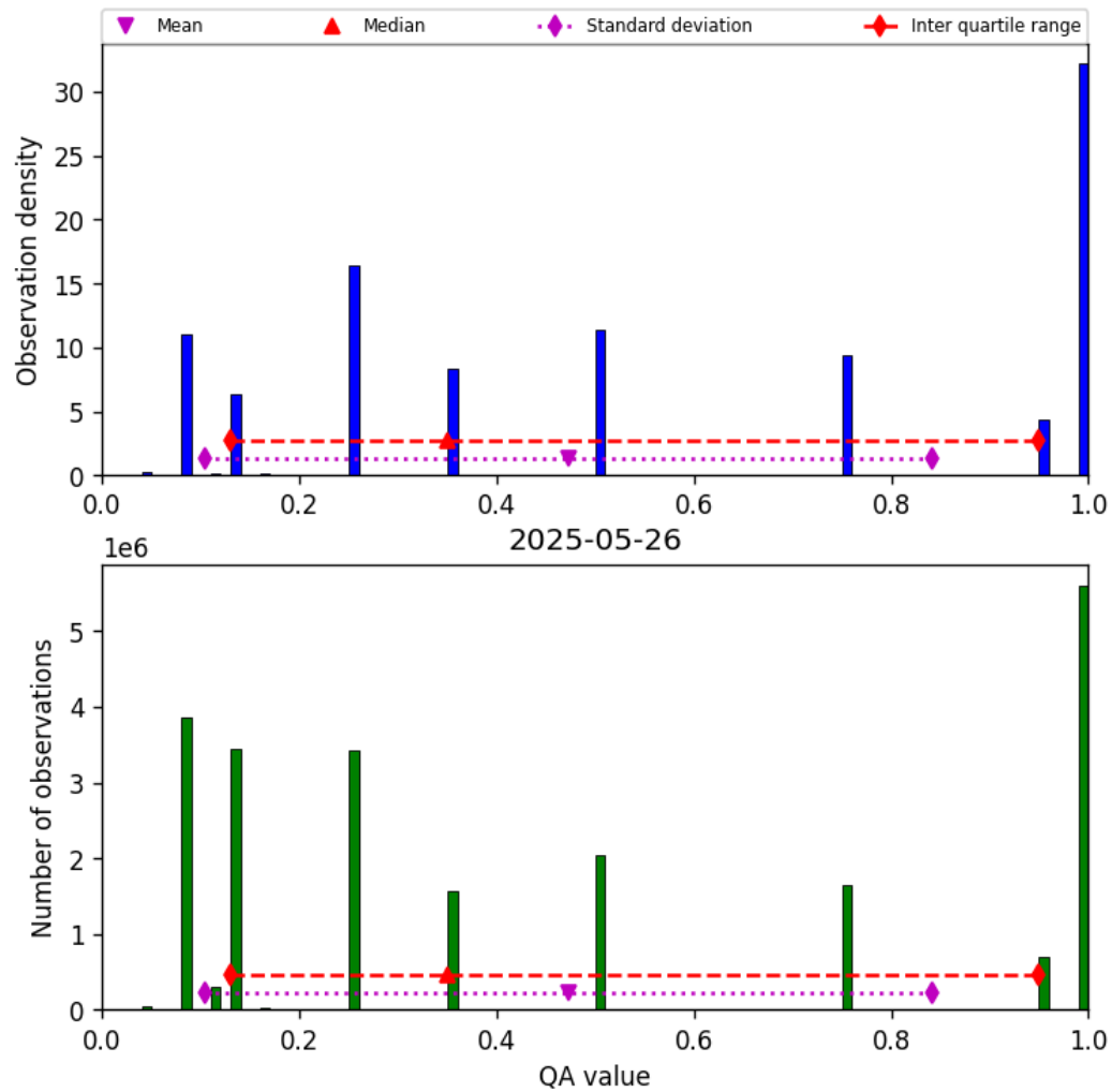
Figure 32: Histogram of “QA value” for 2025-05-26 to 2025-05-27
