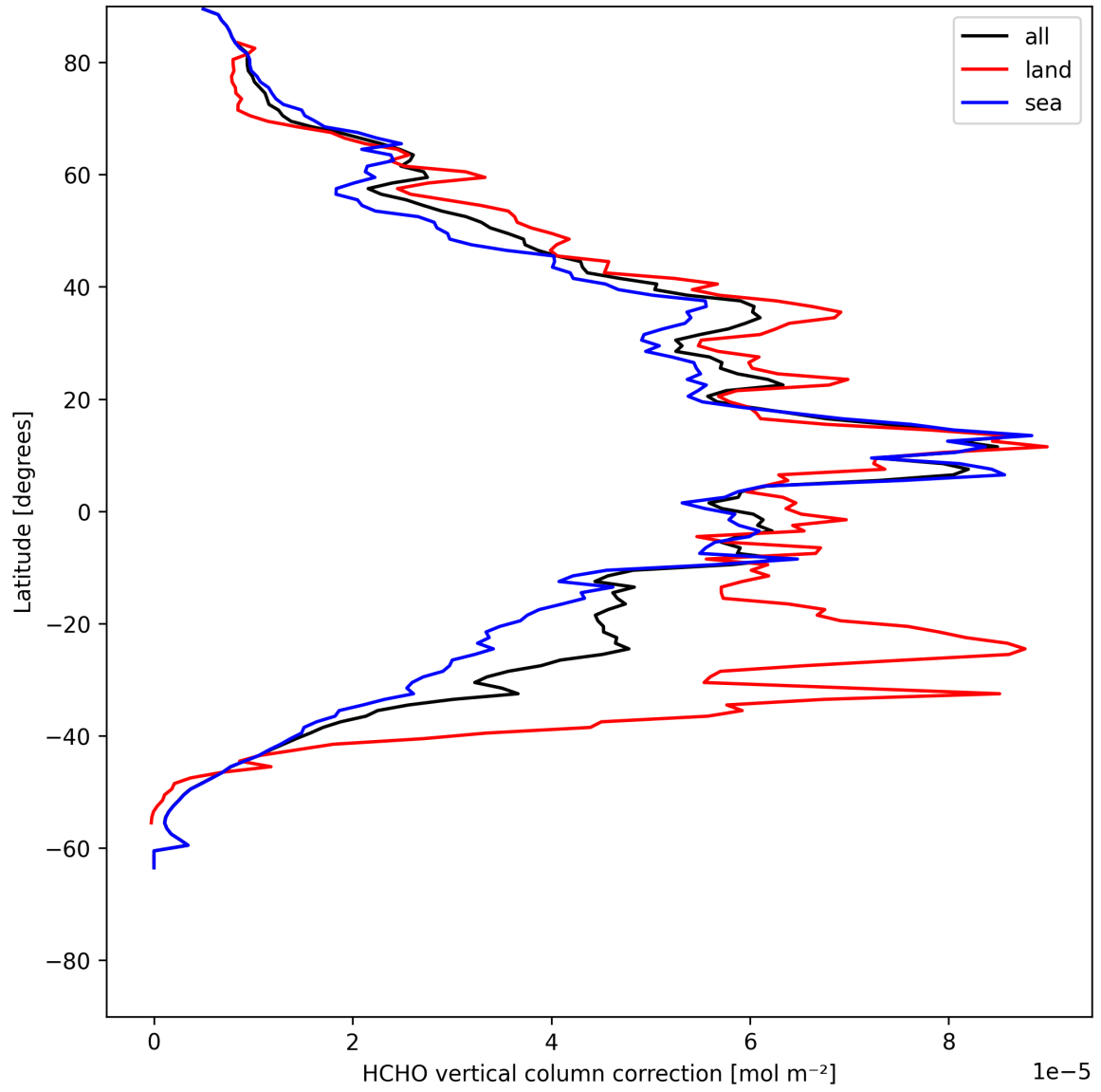
Figure 21: Zonal average of “HCHO vertical column correction” for 2025-05-26 to 2025-05-27.
