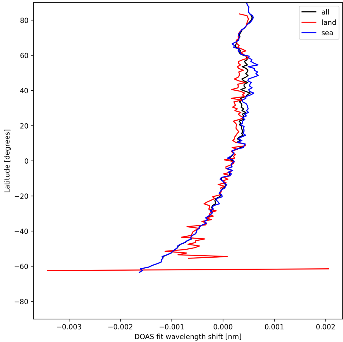
Figure 28: Zonal average of "DOAS fit wavelength shift" for 2025-05-26 to 2025-05-27.
